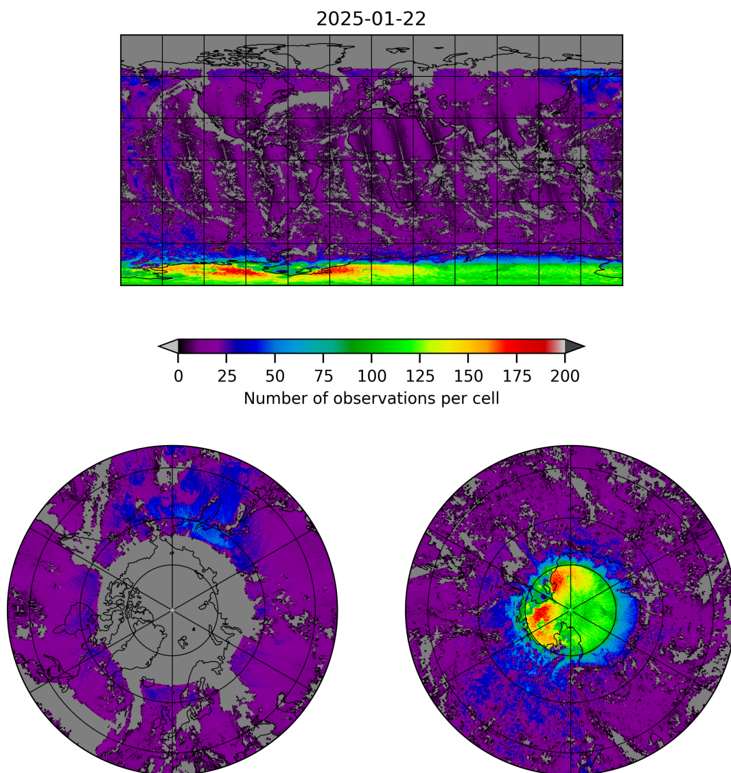
Figure 8: Map of the number of observations for 2025-01-21 to 2025-01-23
