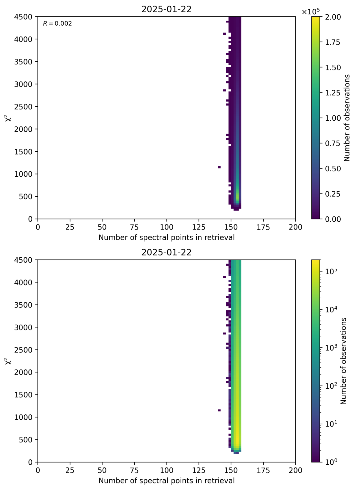
Figure 58: Scatter density plot of “Number of spectral points in retrieval” against “ \chi^2 ” for 2025-01-21 to 2025-01-23.
