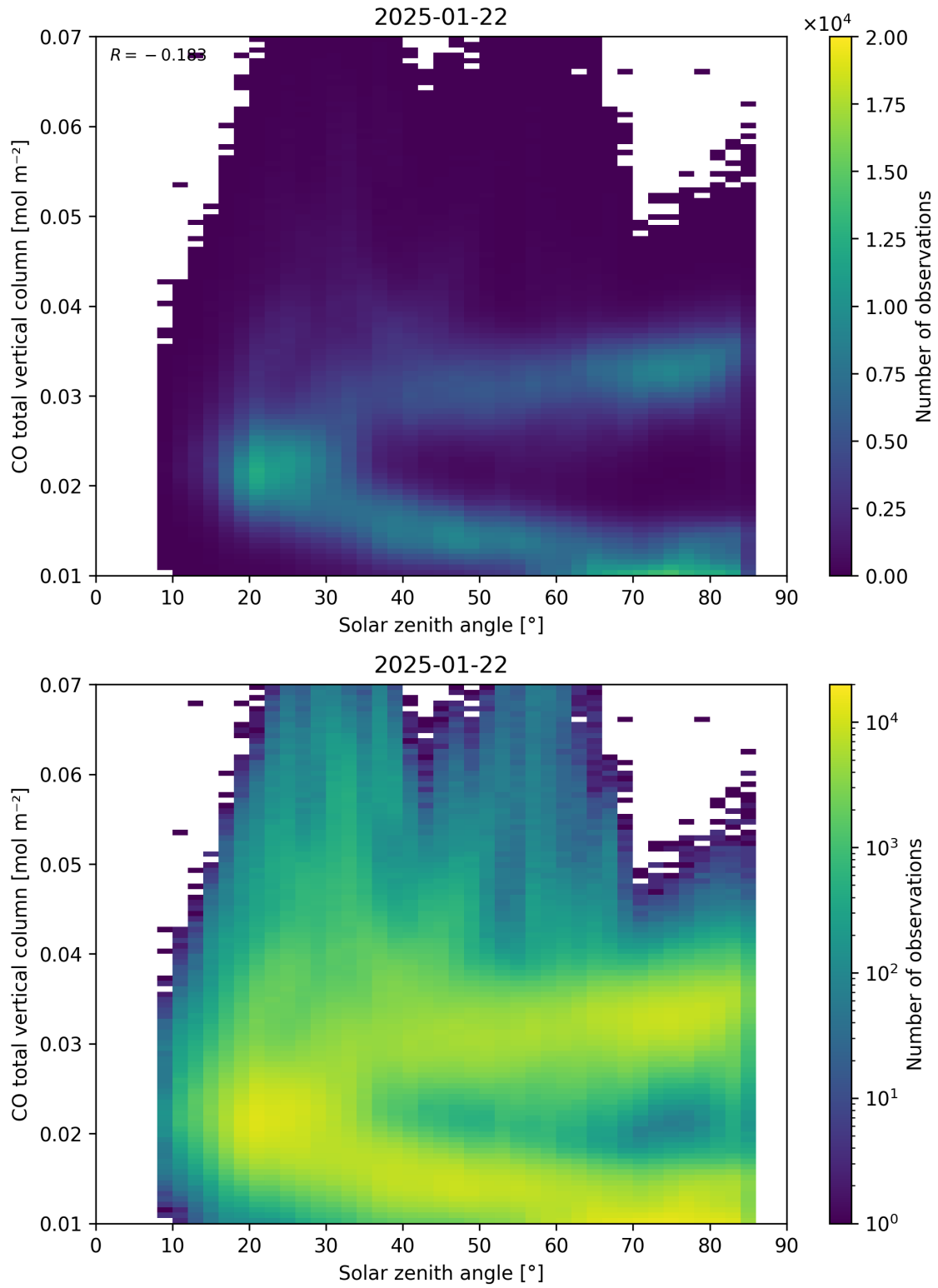
Figure 61: Scatter density plot of “Solar zenith angle” against “CO total vertical column” for 2025-01-21 to 2025-01-23.
