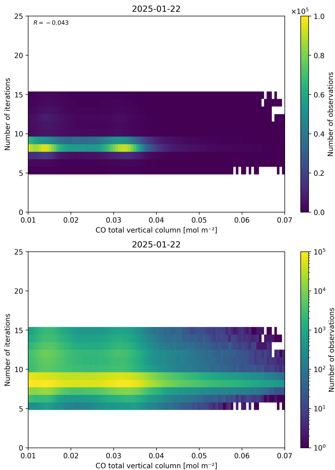
Figure 42: Scatter density plot of “CO total vertical column” against “Number of iterations” for 2025-01-21 to 2025-01-23.
