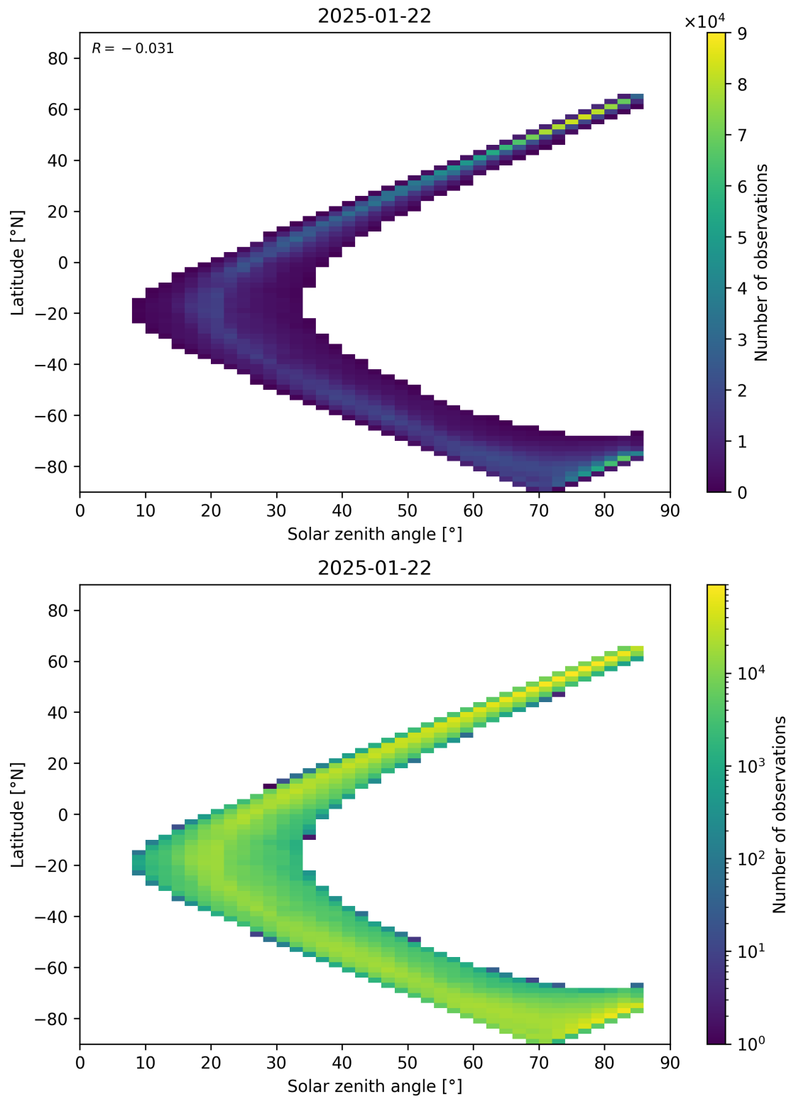
Figure 66: Scatter density plot of “Solar zenith angle” against “Latitude” for 2025-01-21 to 2025-01-23.
