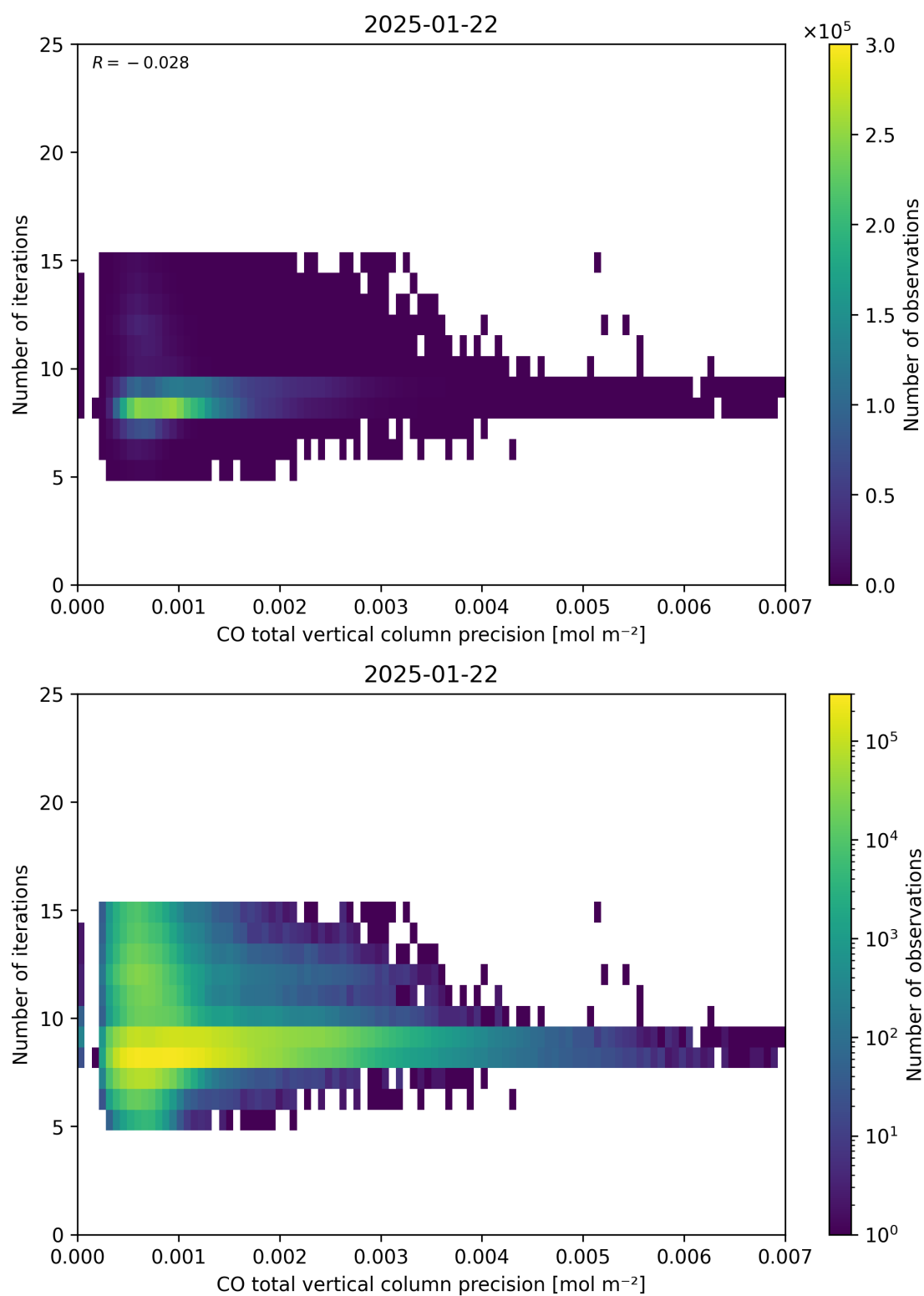
Figure 46: Scatter density plot of “CO total vertical column precision” against “Number of iterations” for 2025-01-21 to 2025-01-23.
