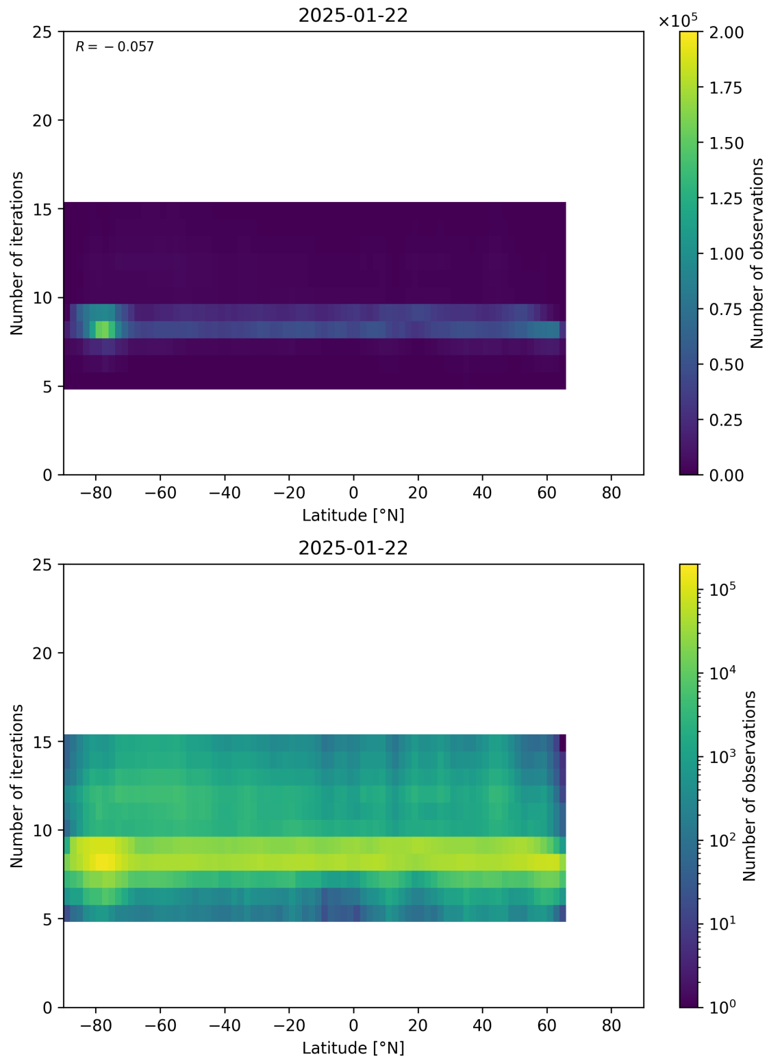
Figure 56: Scatter density plot of “Latitude” against “Number of iterations” for 2025-01-21 to 2025-01-23.
