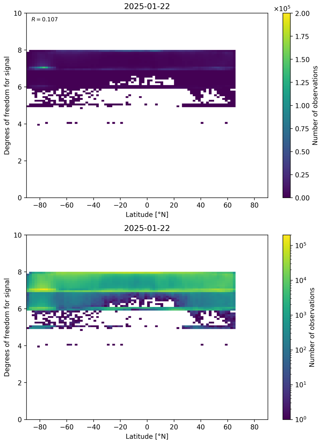
Figure 55: Scatter density plot of “Latitude” against “Degrees of freedom for signal” for 2025-01-21 to 2025-01-23.
