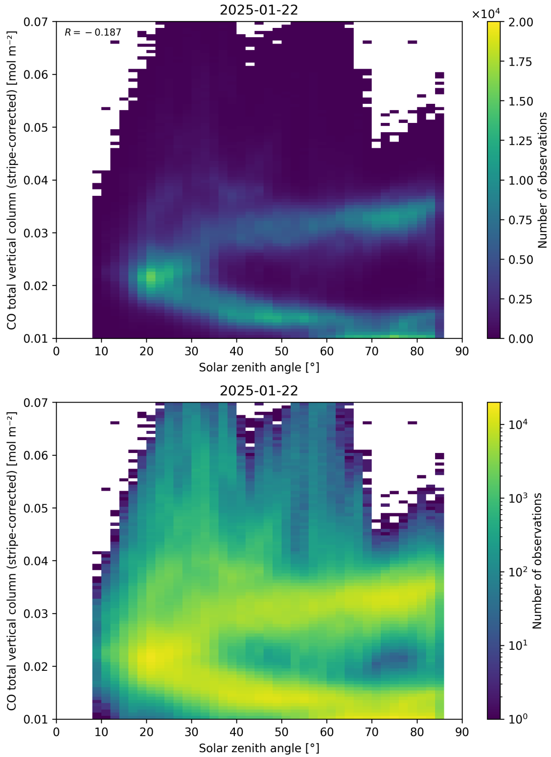
Figure 62: Scatter density plot of “Solar zenith angle” against “CO total vertical column (stripe-corrected)” for 2025-01-21 to 2025-01-23.
