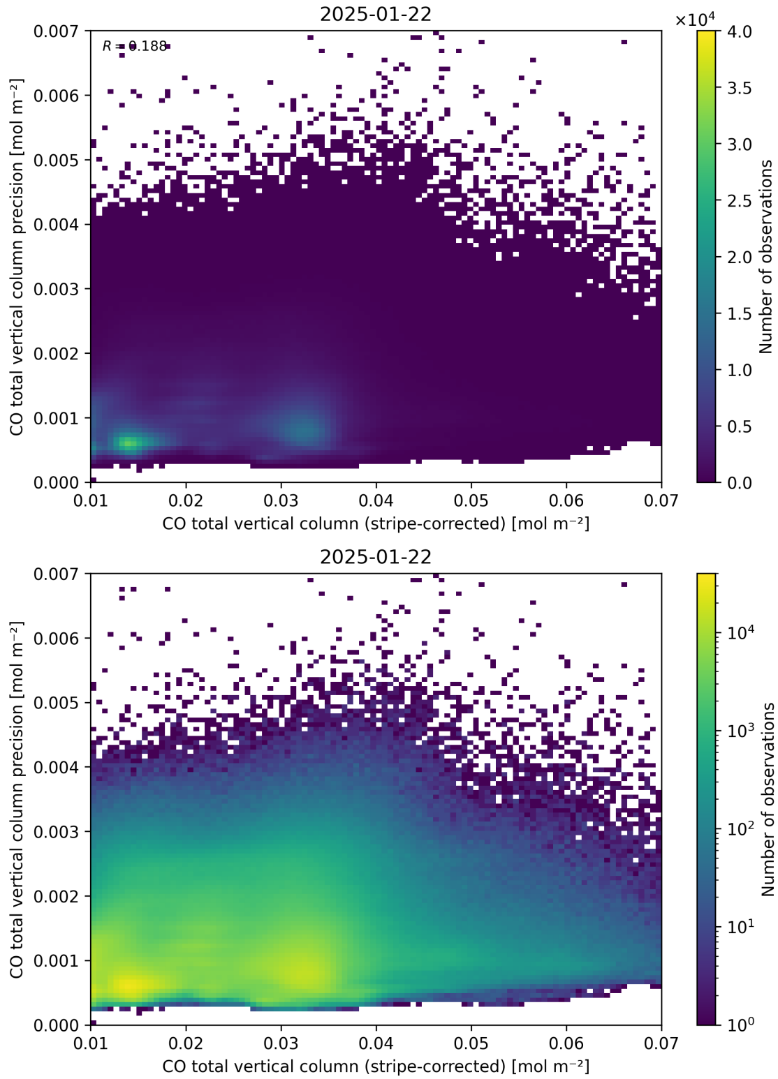
Figure 36: Scatter density plot of “CO total vertical column (stripe-corrected)” against “CO total vertical column precision” for 2025-01-21 to 2025-01-23.
