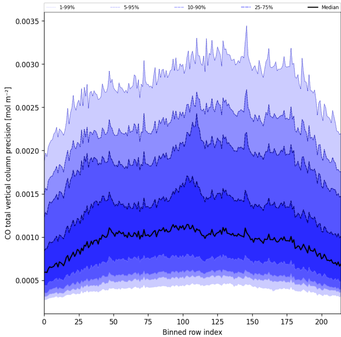
Figure 28: Along track statistics of “CO total vertical column precision” for 2025-01-21 to 2025-01-23
