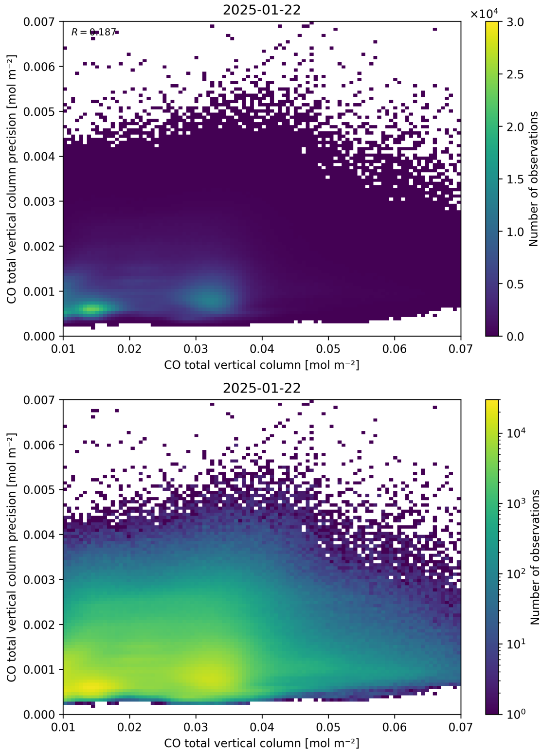
Figure 34: Scatter density plot of “CO total vertical column” against “CO total vertical column precision” for 2025-01-21 to 2025-01-23.
