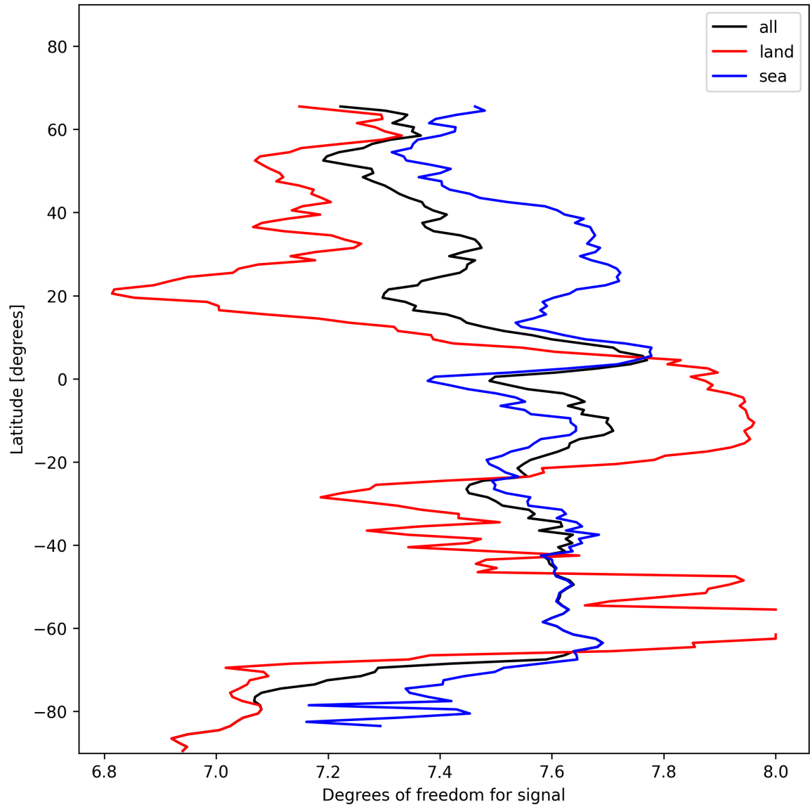
Figure 15: Zonal average of “Degrees of freedom for signal” for 2025-01-21 to 2025-01-23.
