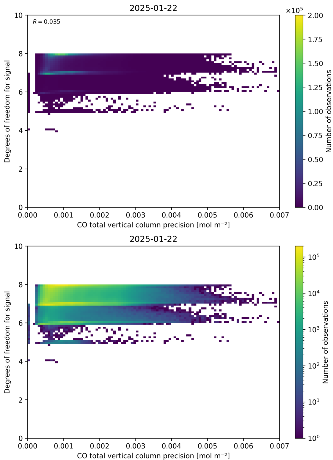
Figure 45: Scatter density plot of “CO total vertical column precision” against “Degrees of freedom for signal” for 2025-01-21 to 2025-01-23.
