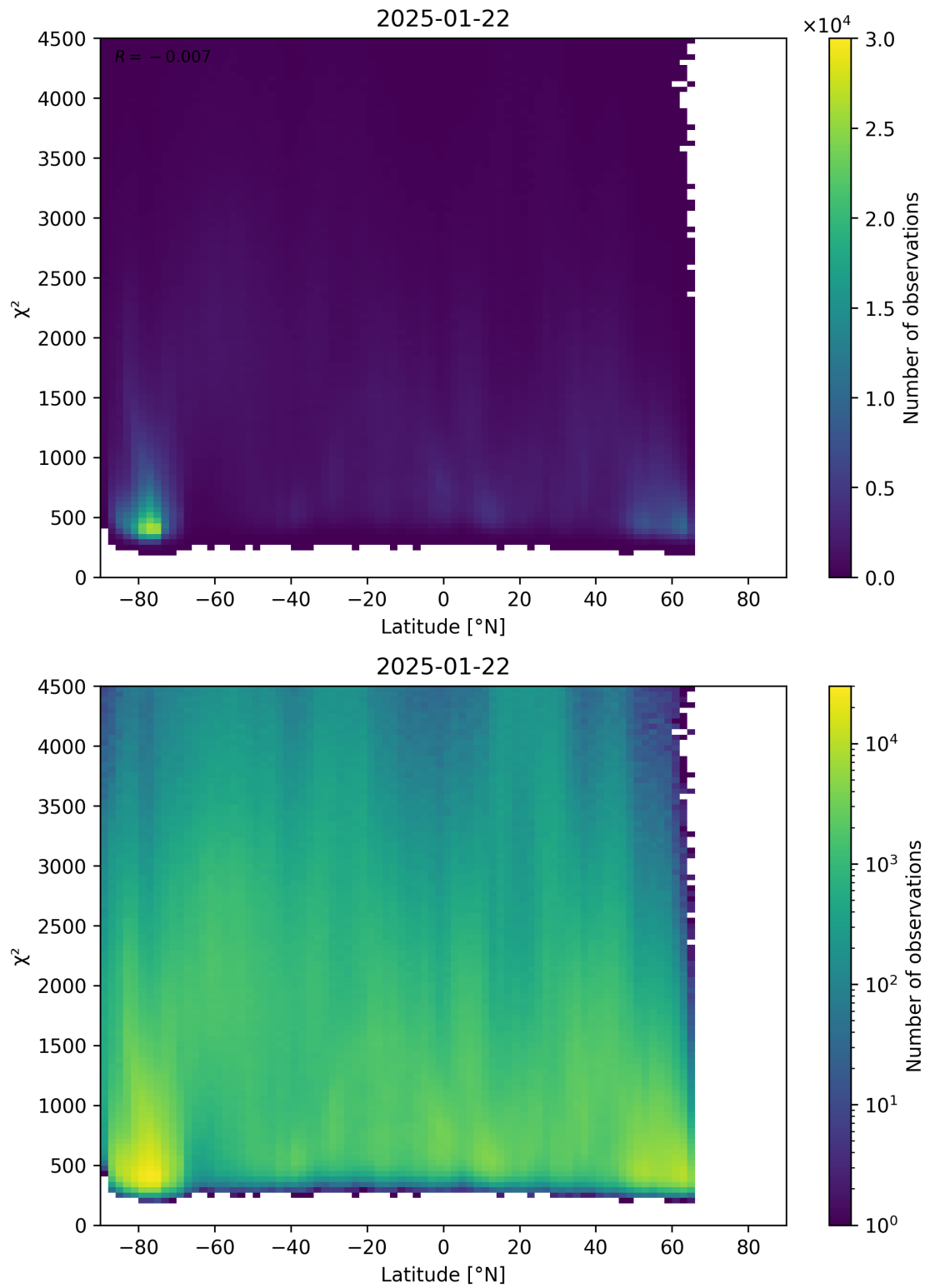
Figure 54: Scatter density plot of “Latitude” against “ \chi^2 ” for 2025-01-21 to 2025-01-23.
