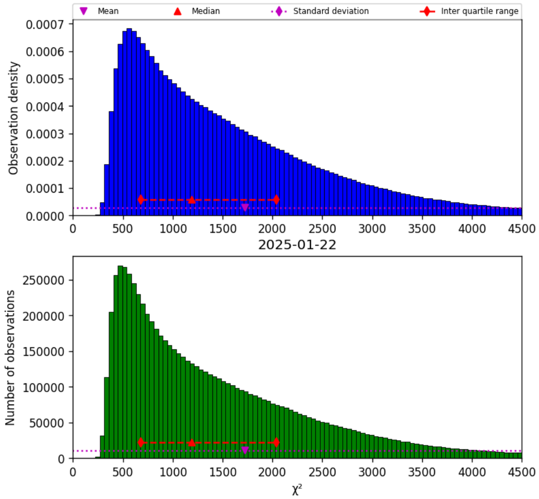
Figure 22: Histogram of “ \chi^2 ” for 2025-01-21 to 2025-01-23
