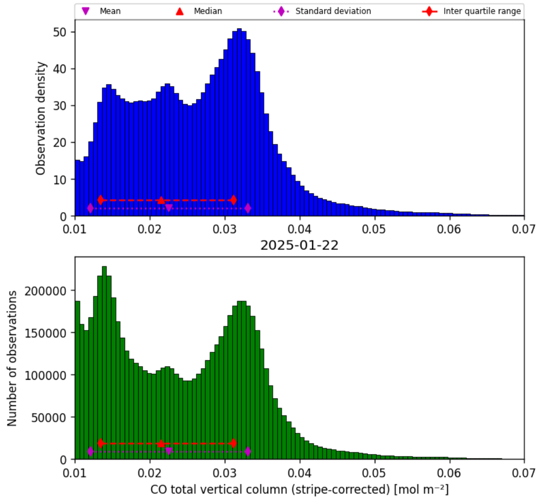
Figure 19: Histogram of “CO total vertical column (stripe-corrected)” for 2025-01-21 to 2025-01-23
