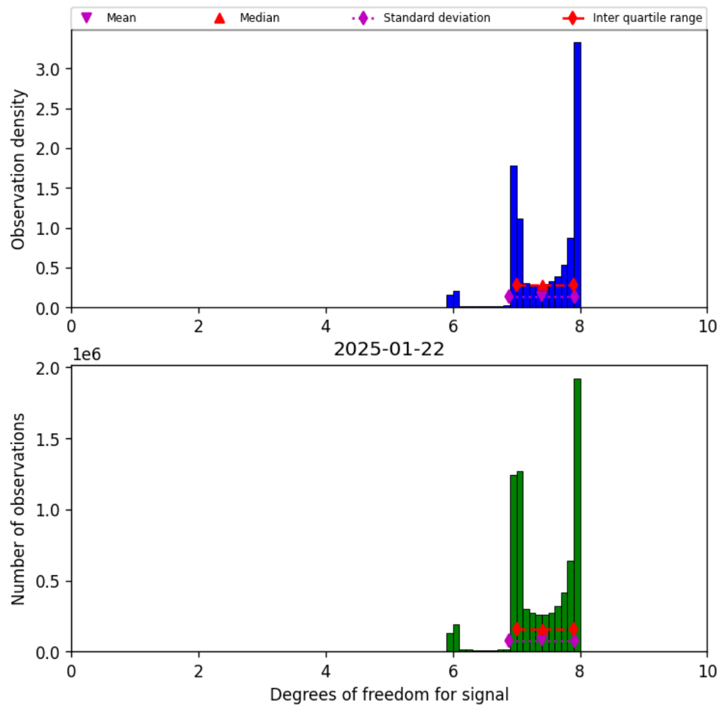
Figure 23: Histogram of “Degrees of freedom for signal” for 2025-01-21 to 2025-01-23
