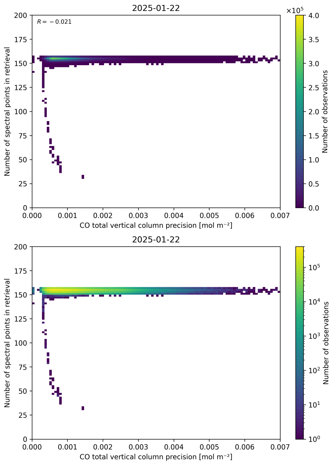
Figure 47: Scatter density plot of “CO total vertical column precision” against “Number of spectral points in retrieval” for 2025-01-21 to 2025-01-23.
