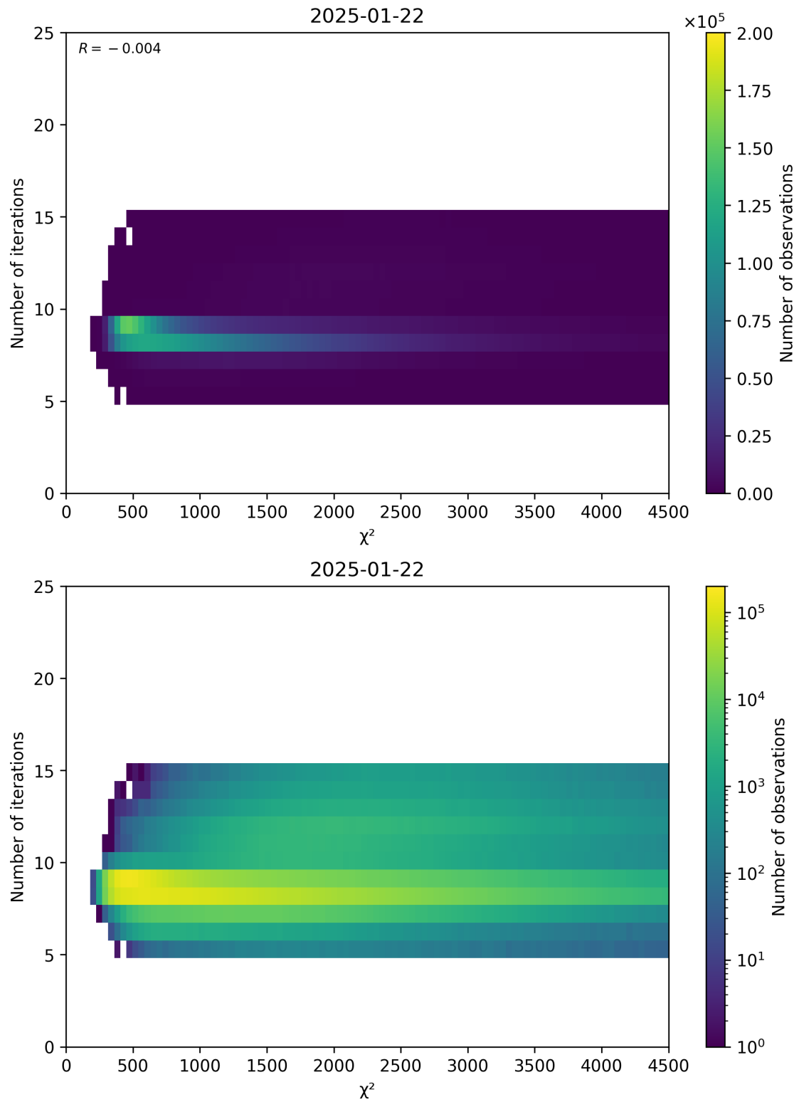
Figure 49: Scatter density plot of “ \chi^2 ” against “Number of iterations” for 2025-01-21 to 2025-01-23.
