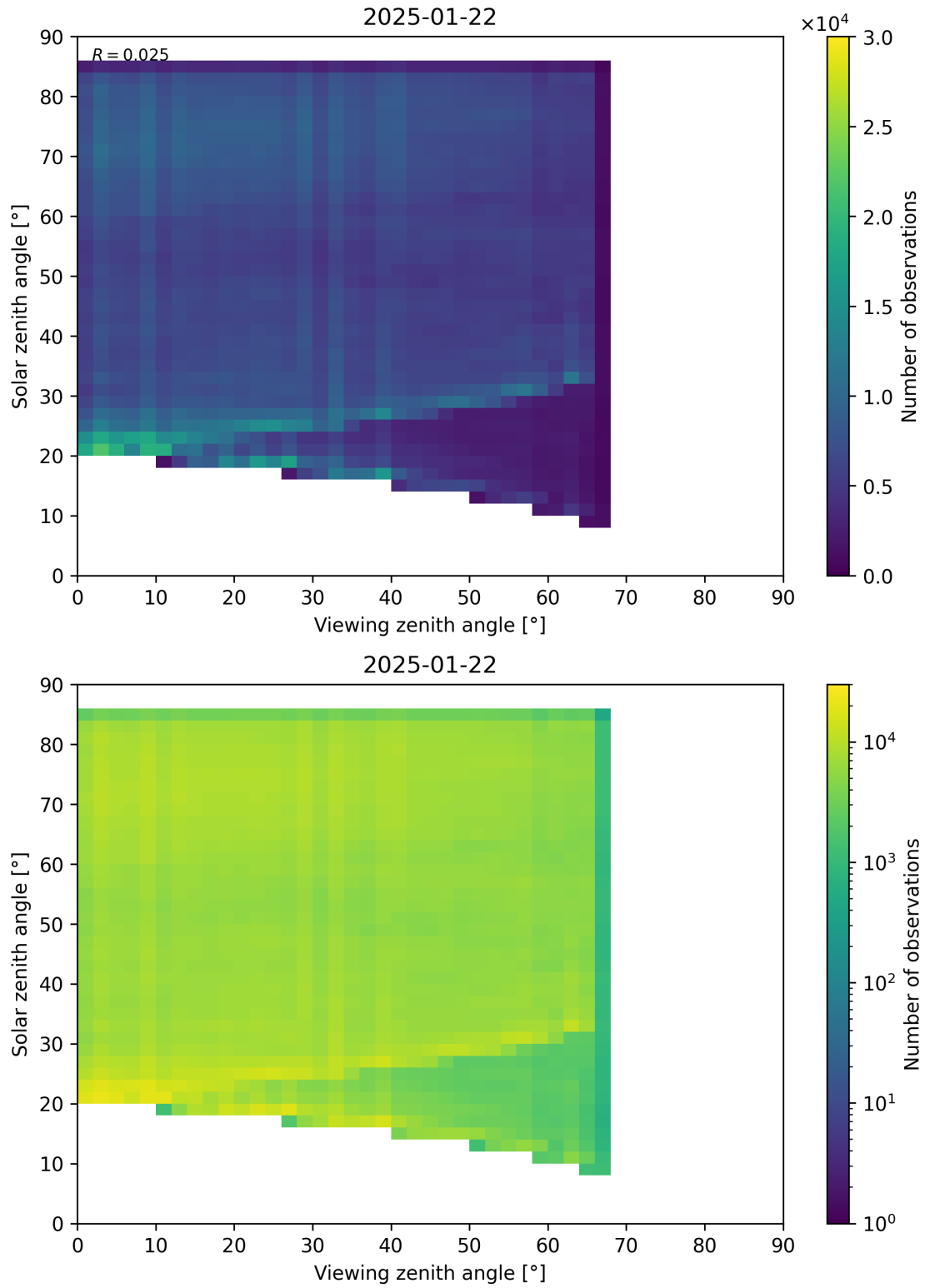
Figure 77: Scatter density plot of “Viewing zenith angle” against “Solar zenith angle” for 2025-01-21 to 2025-01-23.
