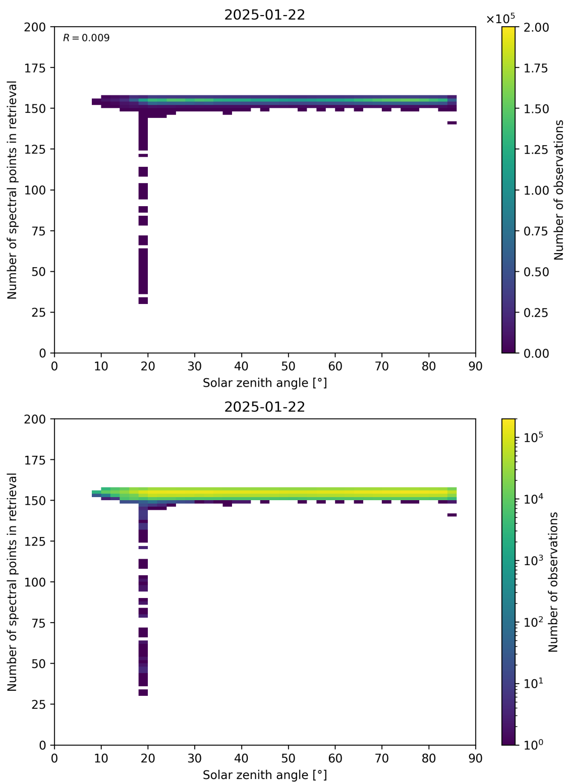
Figure 68: Scatter density plot of “Solar zenith angle” against “Number of spectral points in retrieval” for 2025-01-21 to 2025-01-23.
