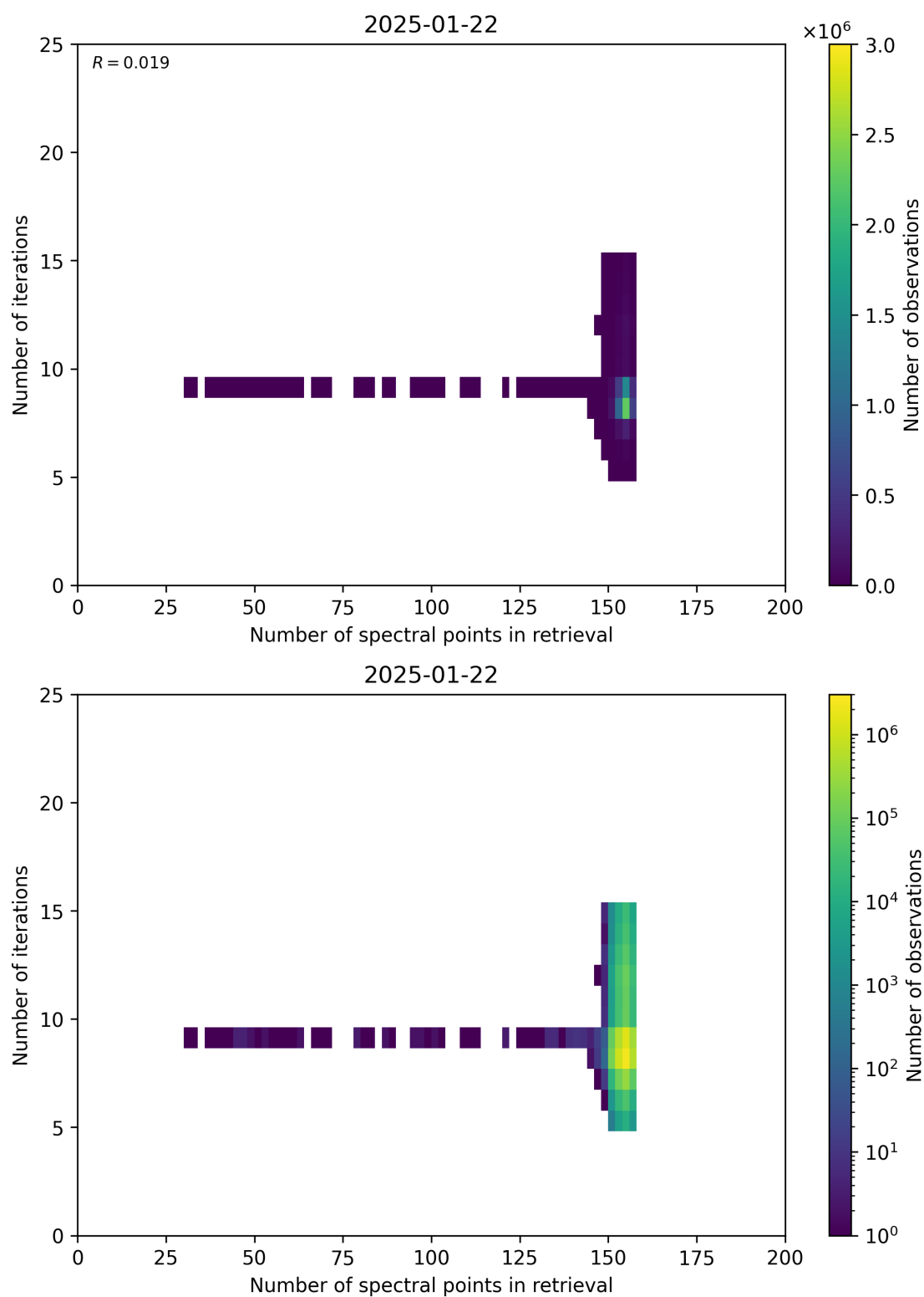
Figure 60: Scatter density plot of “Number of spectral points in retrieval” against “Number of iterations” for 2025-01-21 to 2025-01-23.
