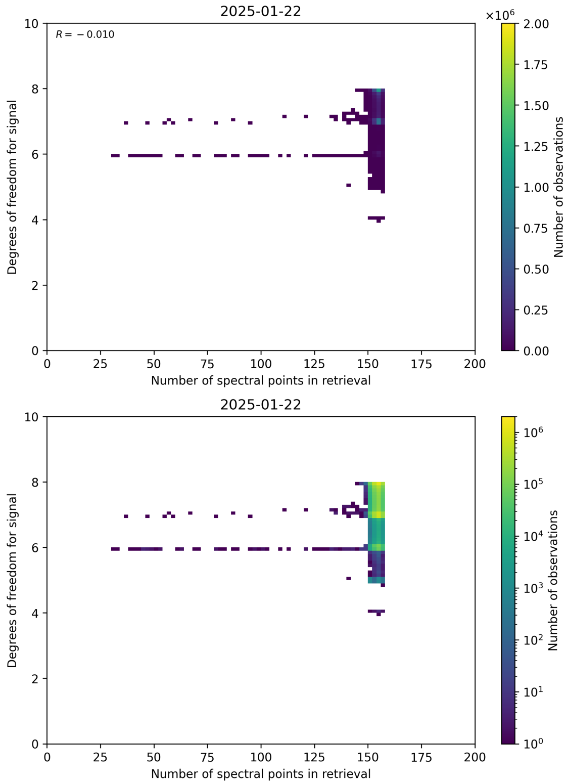
Figure 59: Scatter density plot of “Number of spectral points in retrieval” against “Degrees of freedom for signal” for 2025-01-21 to 2025-01-23.
