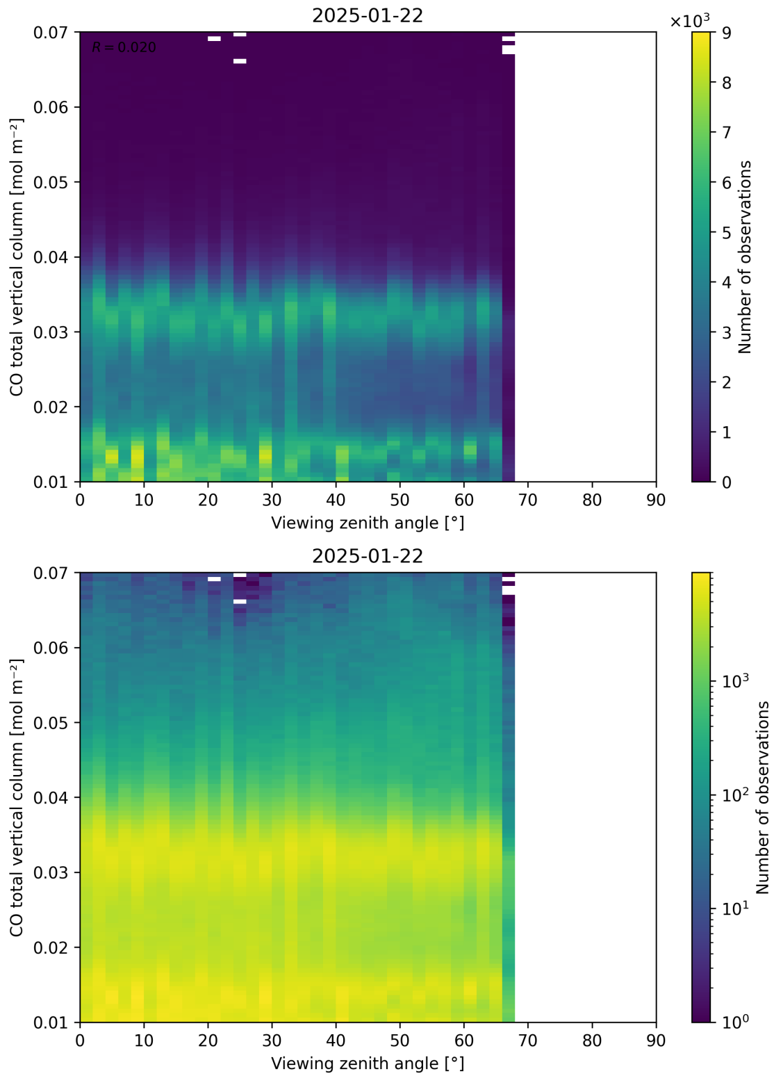
Figure 69: Scatter density plot of “Viewing zenith angle” against “CO total vertical column” for 2025-01-21 to 2025-01-23.
