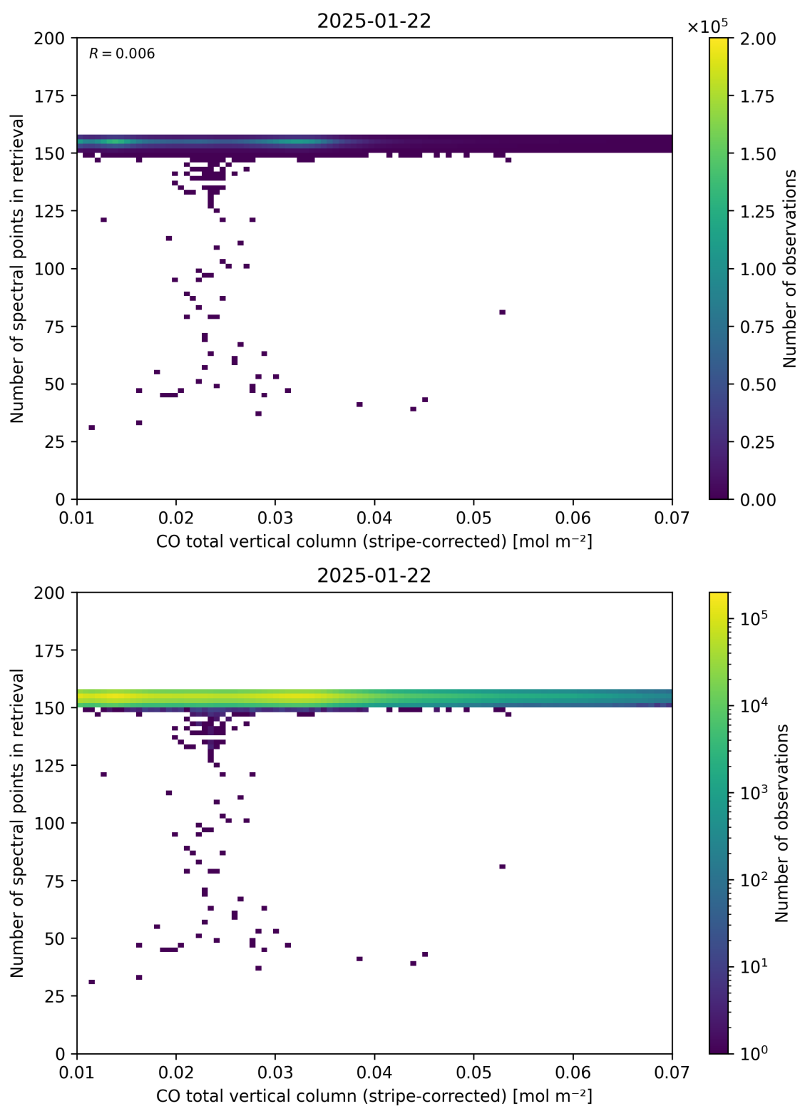
Figure 40: Scatter density plot of “CO total vertical column (stripe-corrected)” against “Number of spectral points in retrieval” for 2025-01-21 to 2025-01-23.
