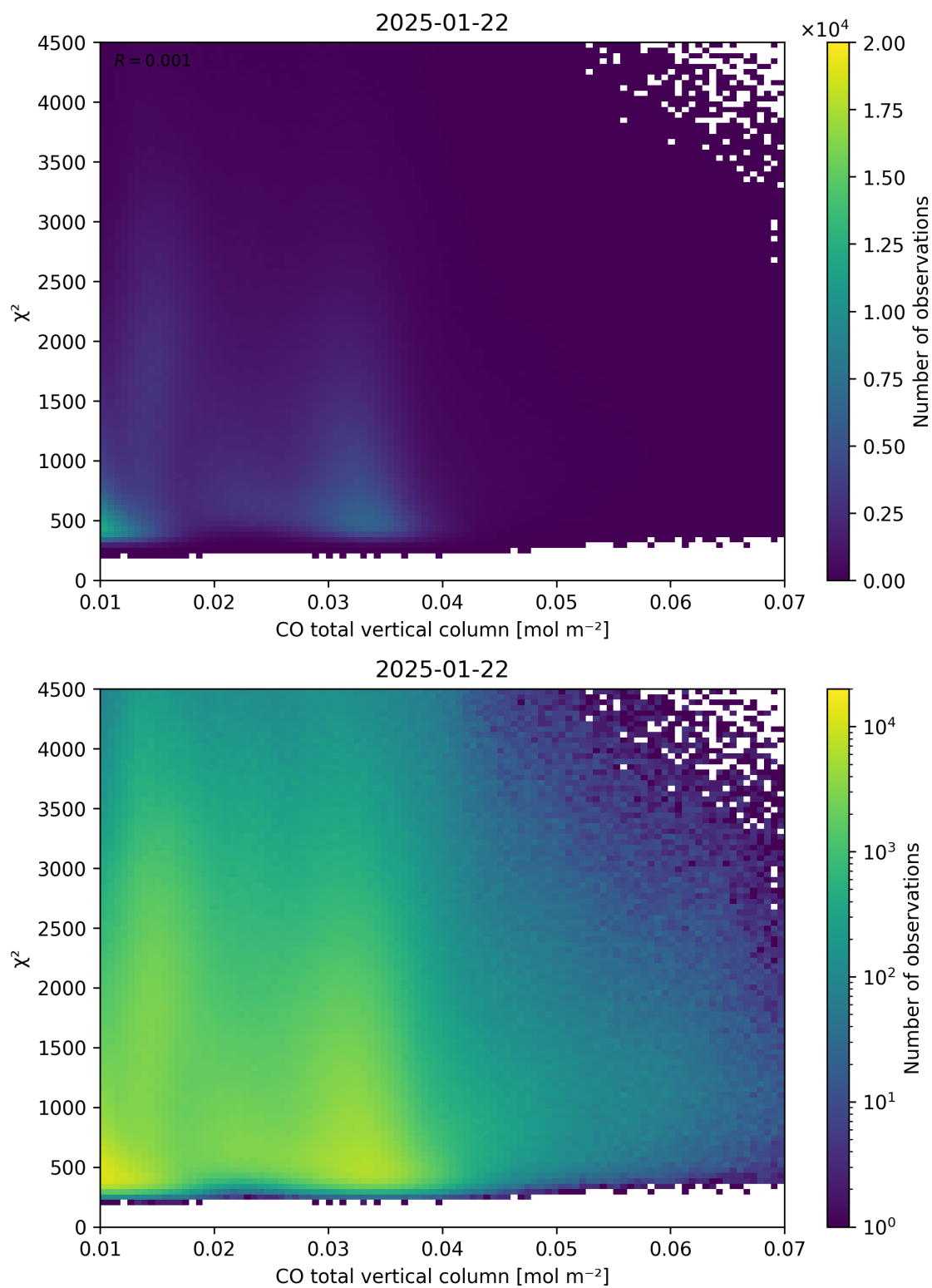
Figure 35: Scatter density plot of “CO total vertical column” against “ \chi^2 ” for 2025-01-21 to 2025-01-23.
