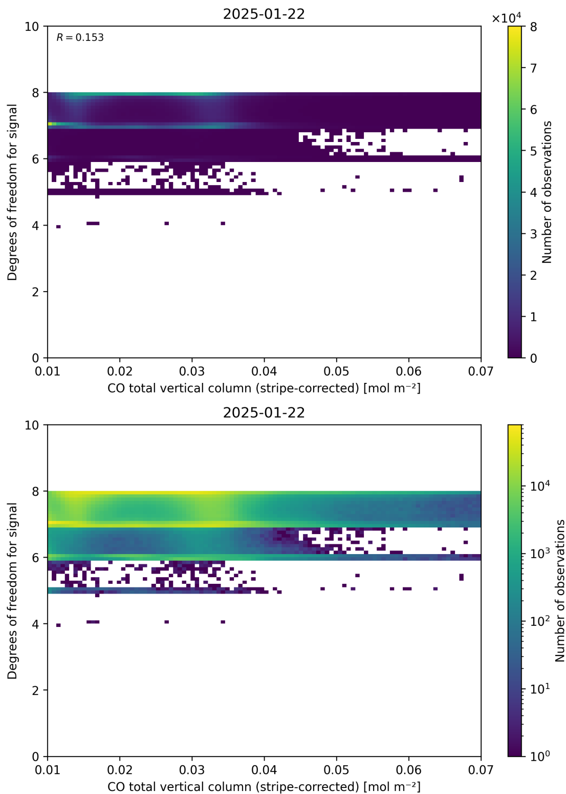
Figure 38: Scatter density plot of “CO total vertical column (stripe-corrected)” against “Degrees of freedom for signal” for 2025-01-21 to 2025-01-23.
