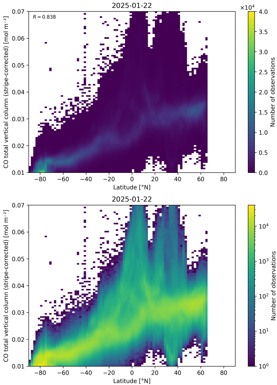
Figure 52: Scatter density plot of “Latitude” against “CO total vertical column (stripe-corrected)” for 2025-01-21 to 2025-01-23.
