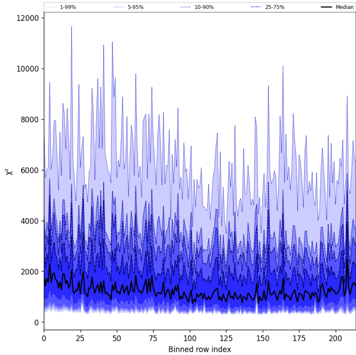
Figure 30: Along track statistics of “ \chi^2 ” for 2025-01-21 to 2025-01-23
