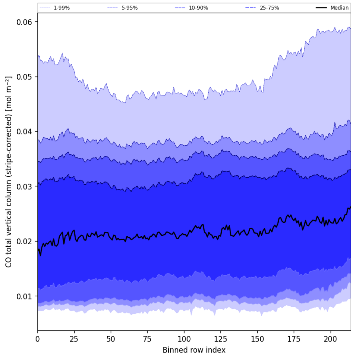
Figure 27: Along track statistics of “CO total vertical column (stripe-corrected)” for 2025-01-21 to 2025-01-23
