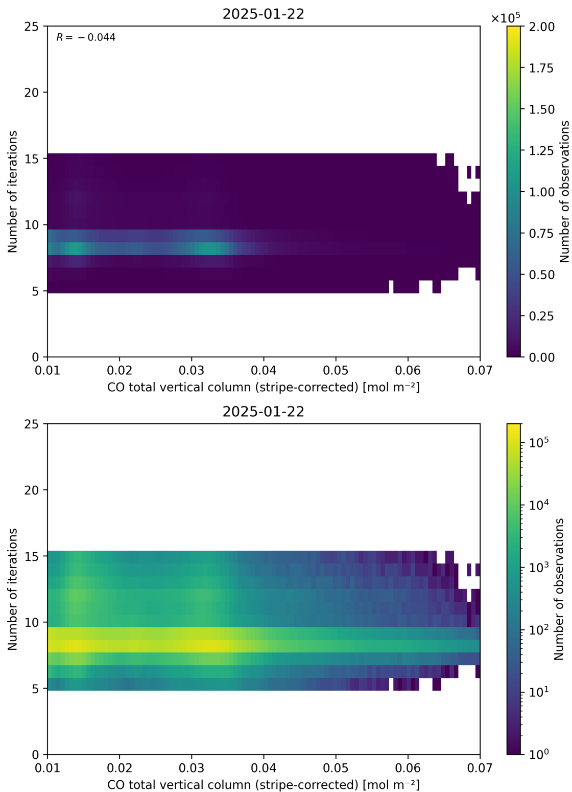
Figure 39: Scatter density plot of “CO total vertical column (stripe-corrected)” against “Number of iterations” for 2025-01-21 to 2025-01-23.
