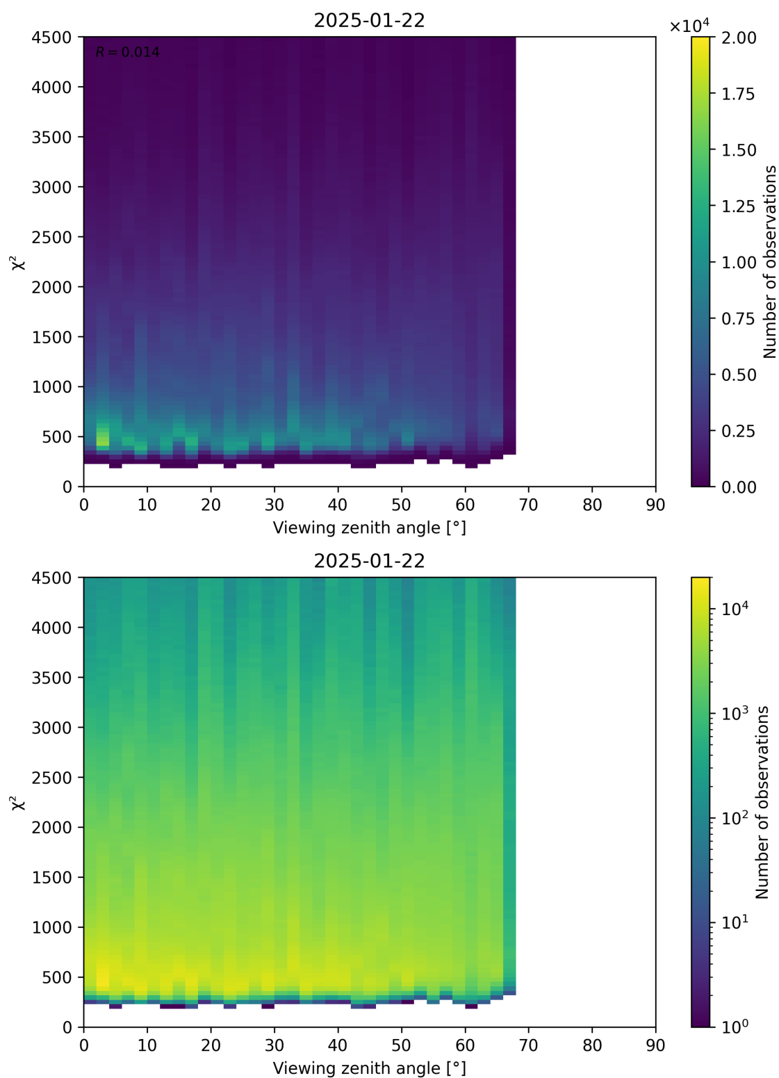
Figure 72: Scatter density plot of “Viewing zenith angle” against “ \chi^2 ” for 2025-01-21 to 2025-01-23.
