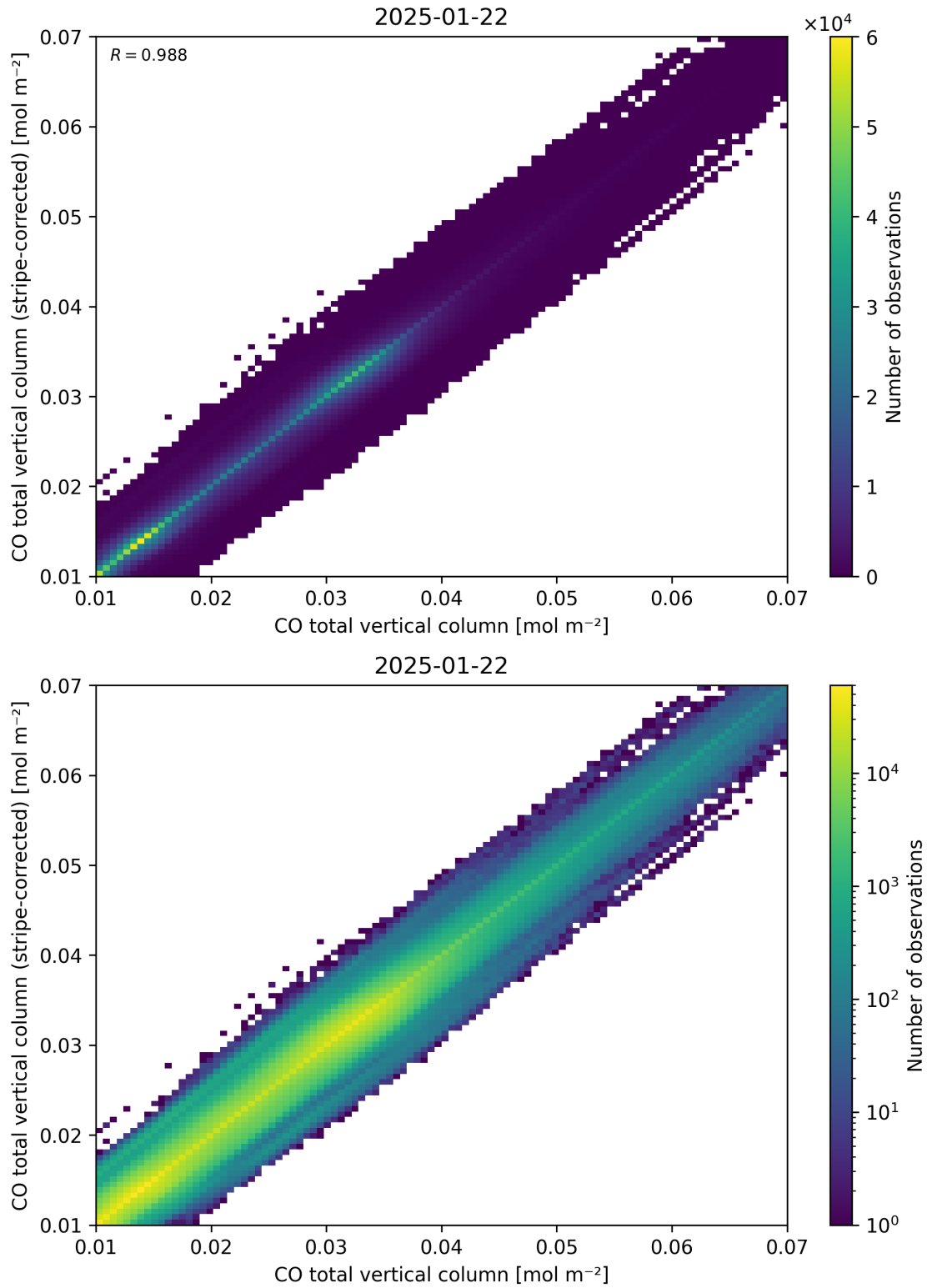
Figure 33: Scatter density plot of “CO total vertical column” against “CO total vertical column (stripe-corrected)” for 2025-01-21 to 2025-01-23.
