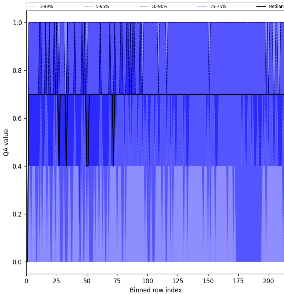
Figure 25: Along track statistics of “QA value” for 2025-01-21 to 2025-01-23
