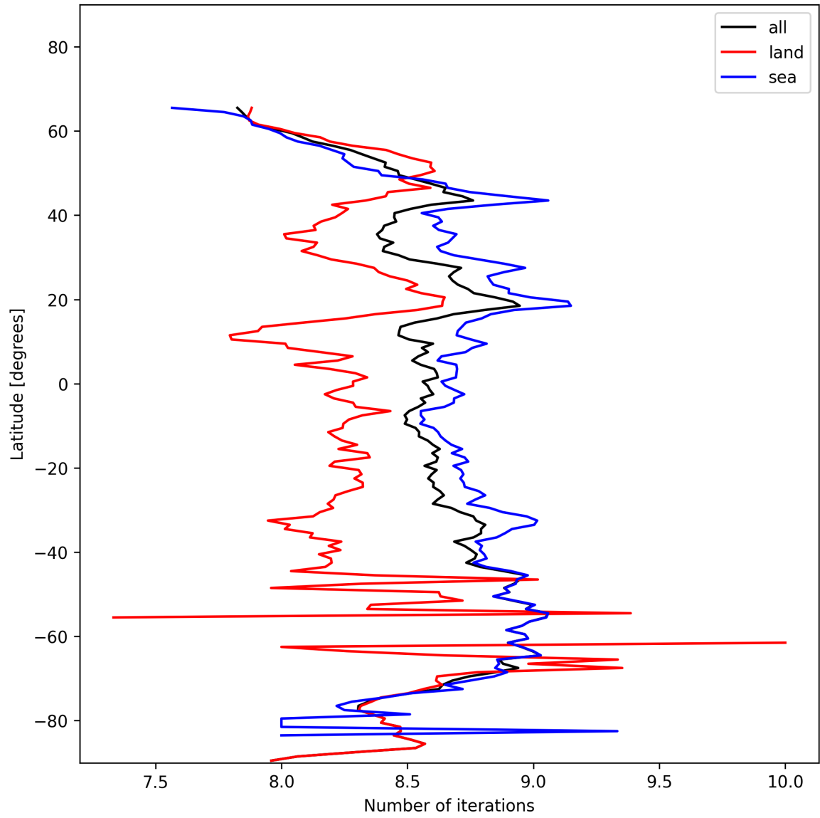
Figure 16: Zonal average of “Number of iterations” for 2025-01-21 to 2025-01-23.
