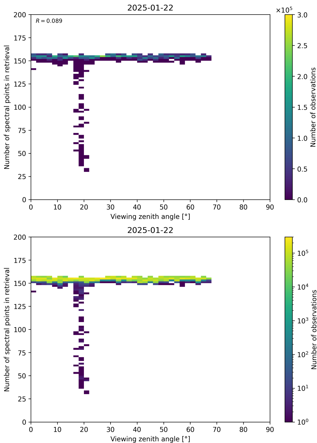
Figure 76: Scatter density plot of “Viewing zenith angle” against “Number of spectral points in retrieval” for 2025-01-21 to 2025-01-23.
