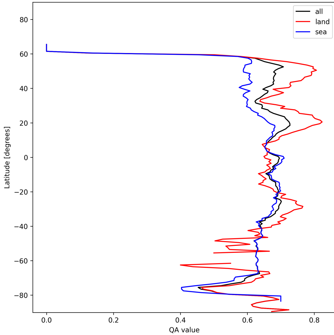
Figure 9: Zonal average of “QA value” for 2025-01-21 to 2025-01-23.
