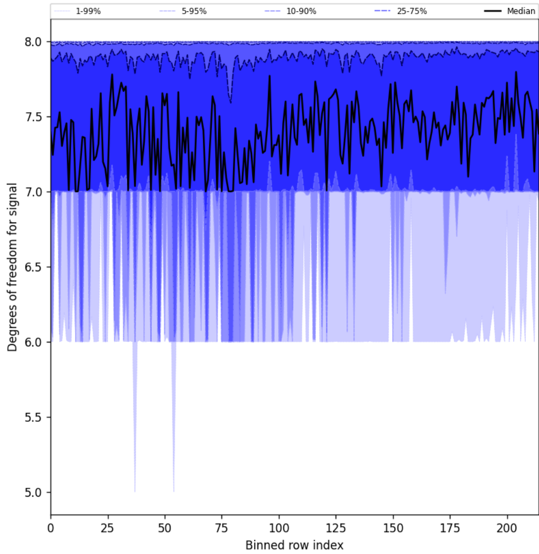
Figure 31: Along track statistics of “Degrees of freedom for signal” for 2025-01-21 to 2025-01-23
