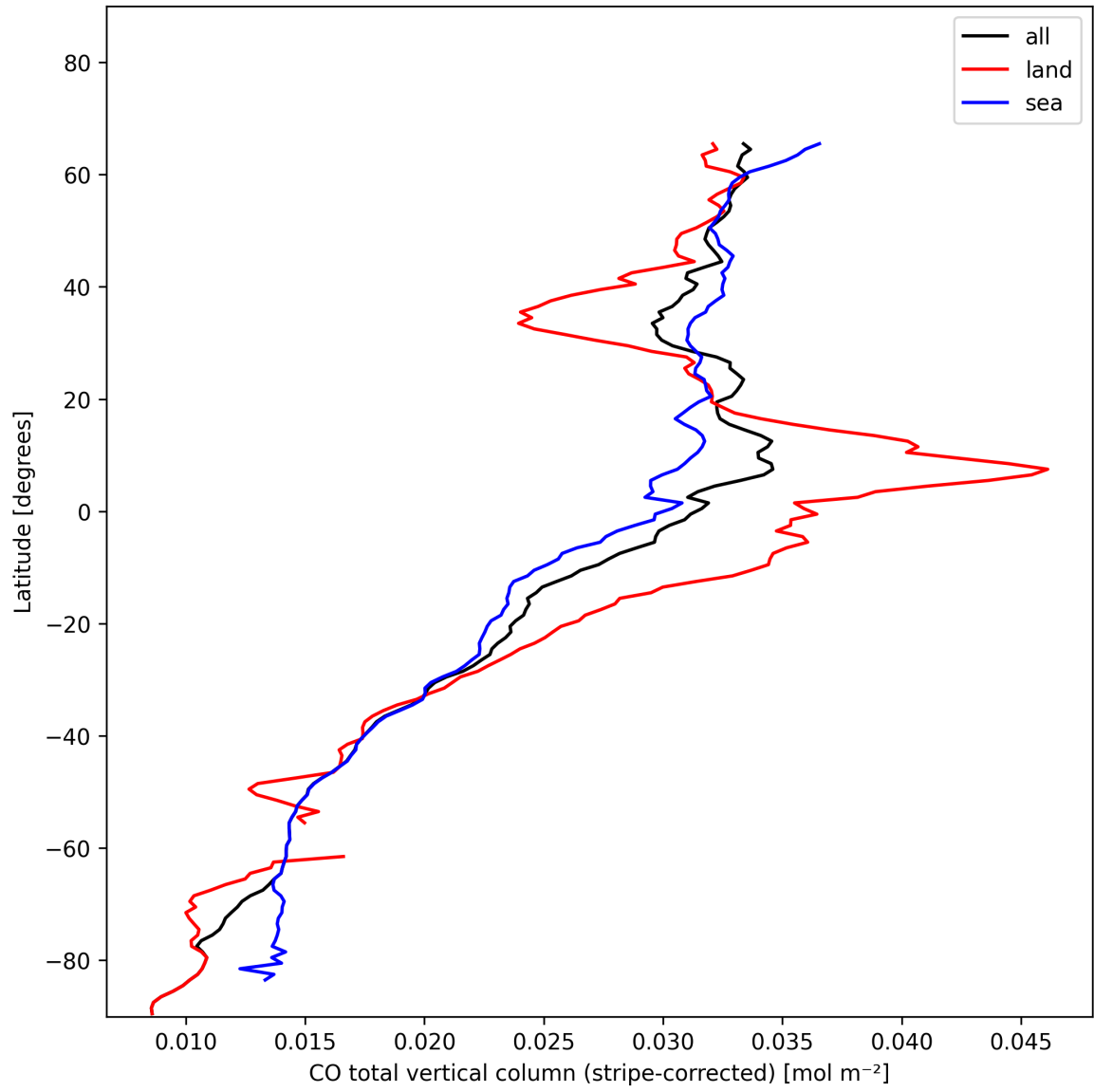
Figure 11: Zonal average of “CO total vertical column (stripe-corrected)” for 2025-01-21 to 2025-01-23.
