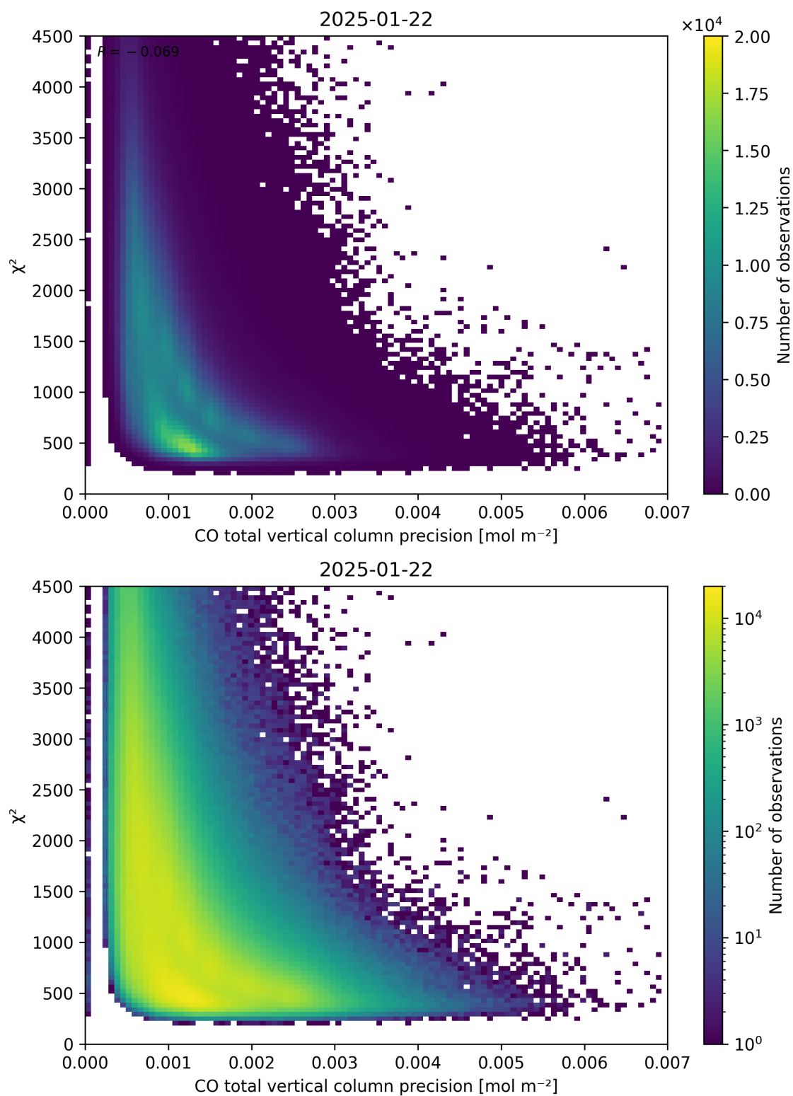
Figure 44: Scatter density plot of “CO total vertical column precision” against “ \chi^2 ” for 2025-01-21 to 2025-01-23.
