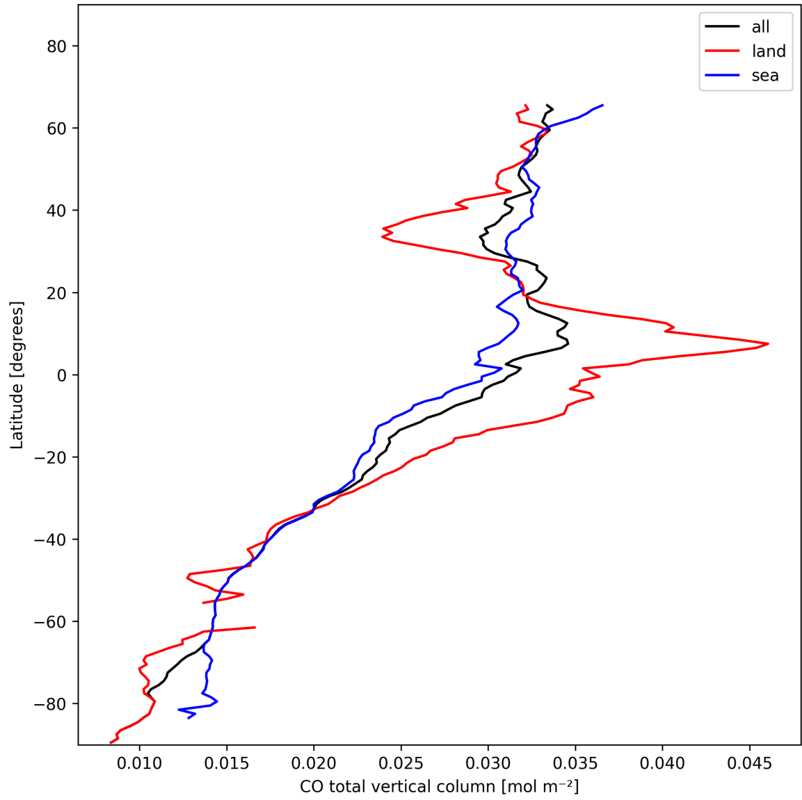
Figure 10: Zonal average of “CO total vertical column” for 2025-01-21 to 2025-01-23.
