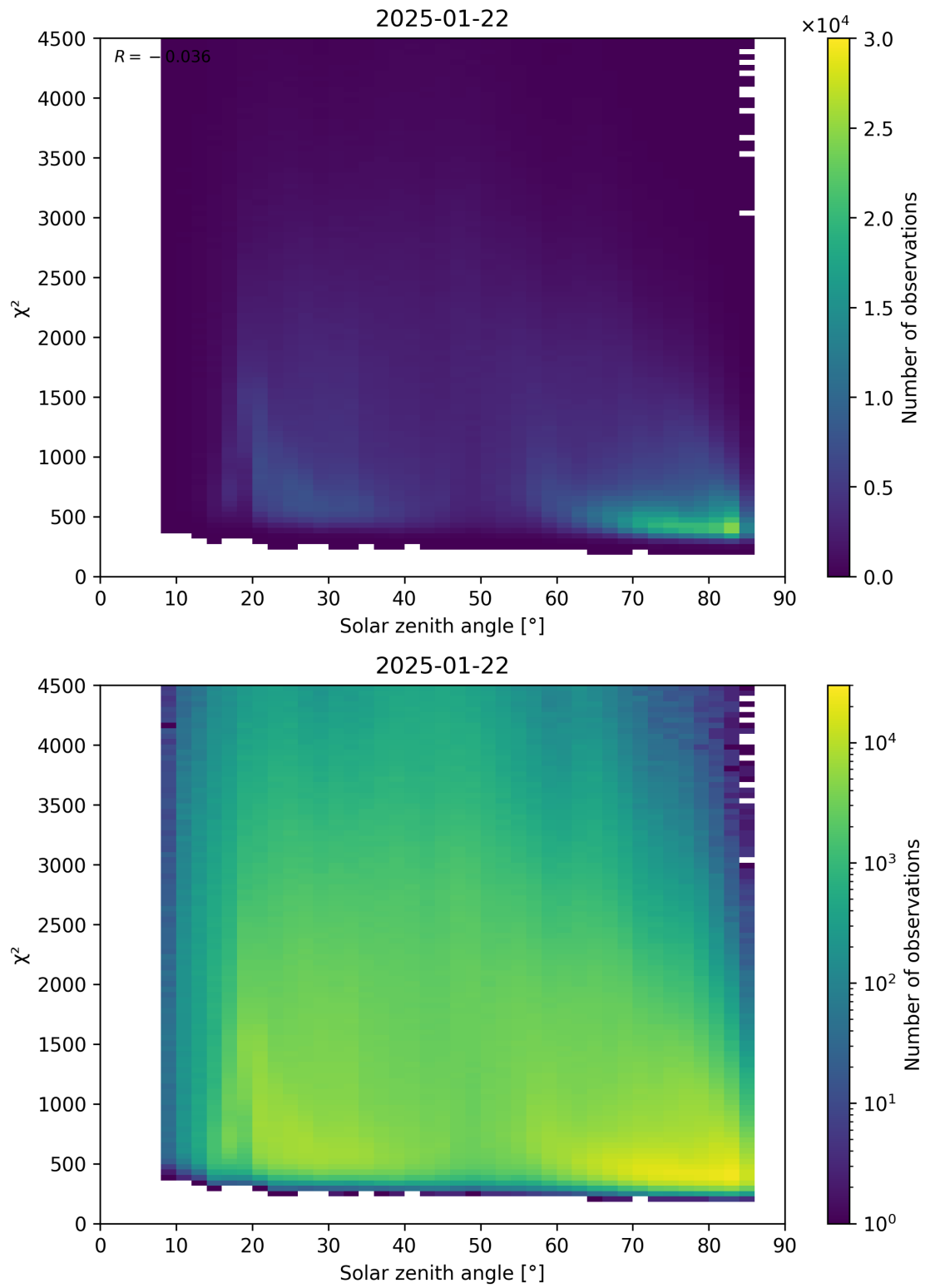
Figure 64: Scatter density plot of “Solar zenith angle” against “ \chi^2 ” for 2025-01-21 to 2025-01-23.
