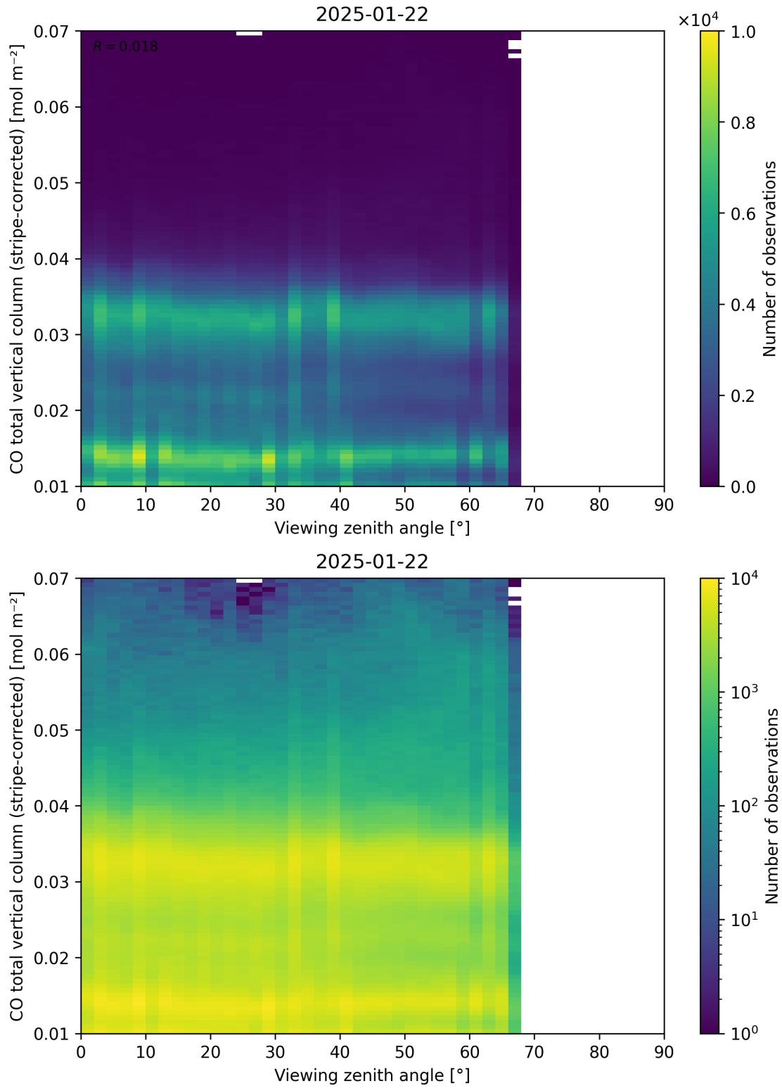
Figure 70: Scatter density plot of “Viewing zenith angle” against “CO total vertical column (stripe-corrected)” for 2025-01-21 to 2025-01-23.
