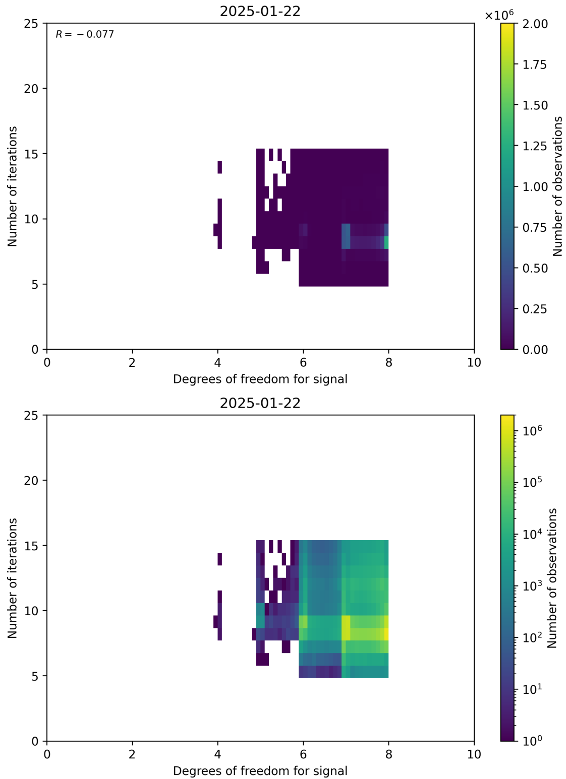
Figure 50: Scatter density plot of “Degrees of freedom for signal” against “Number of iterations” for 2025-01-21 to 2025-01-23.
