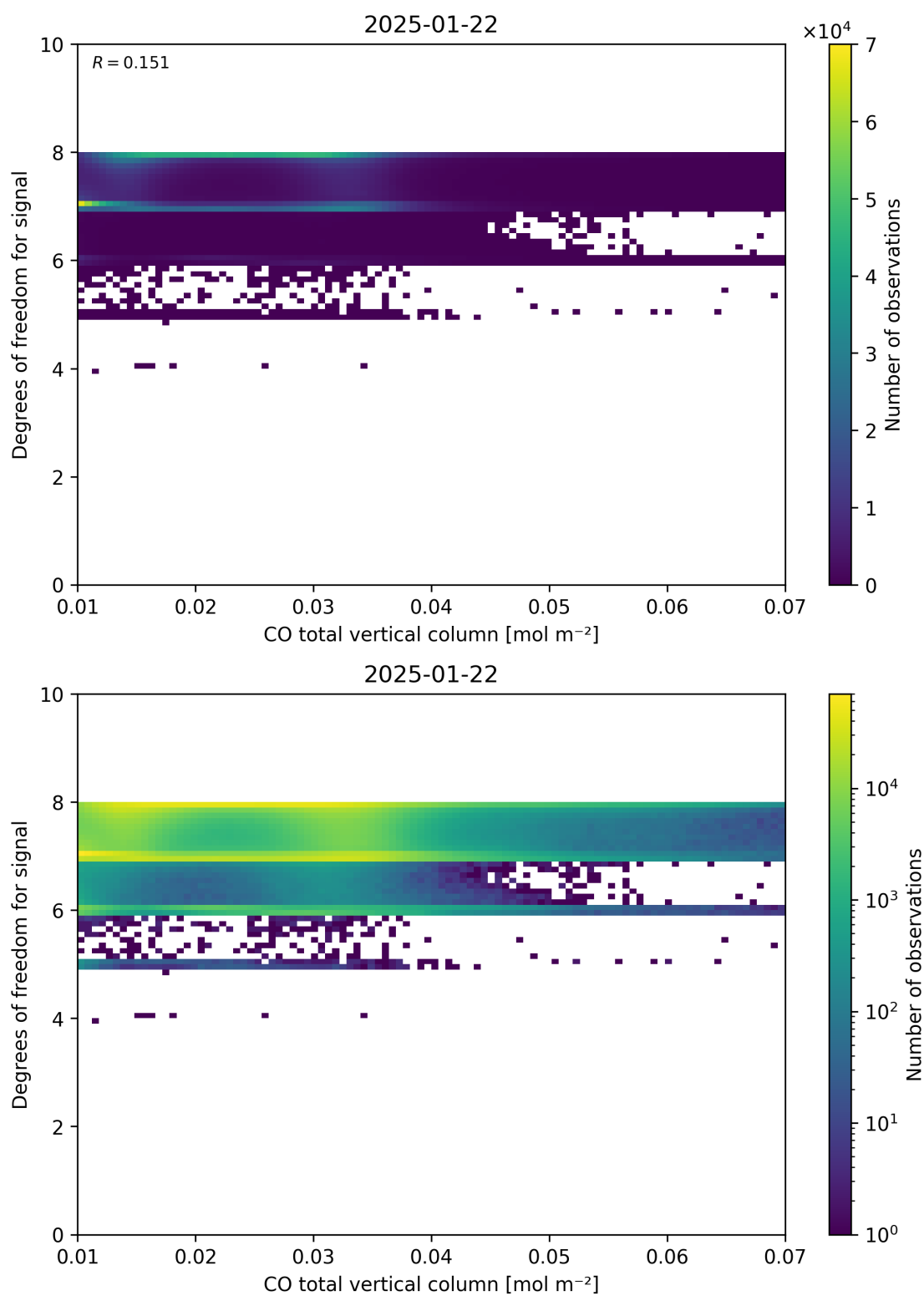
Figure 41: Scatter density plot of “CO total vertical column” against “Degrees of freedom for signal” for 2025-01-21 to 2025-01-23.
