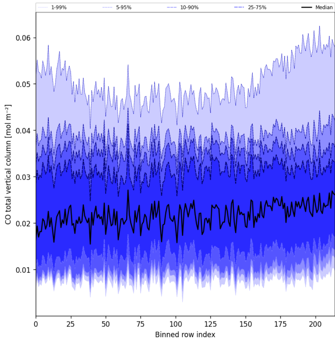
Figure 26: Along track statistics of “CO total vertical column” for 2025-01-21 to 2025-01-23
