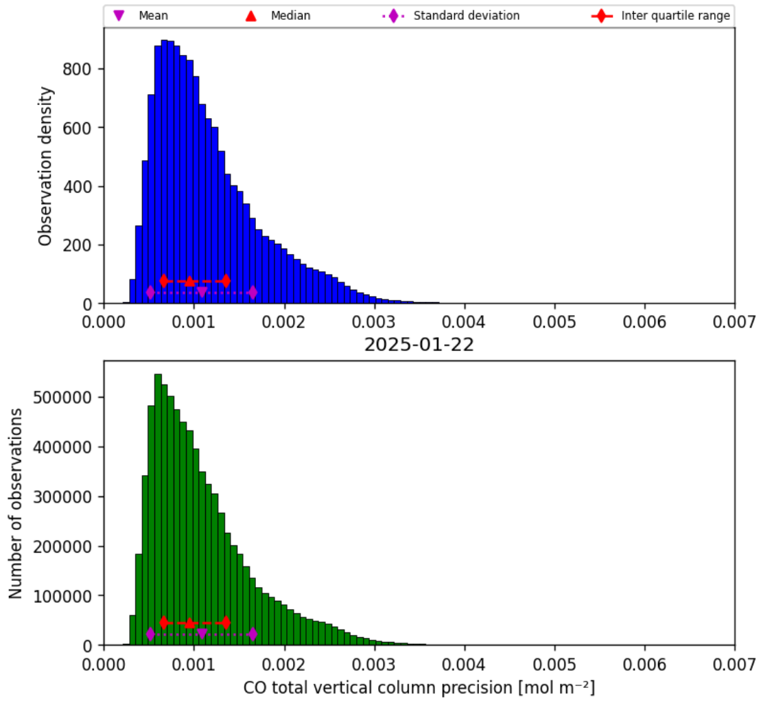
Figure 20: Histogram of “CO total vertical column precision” for 2025-01-21 to 2025-01-23
