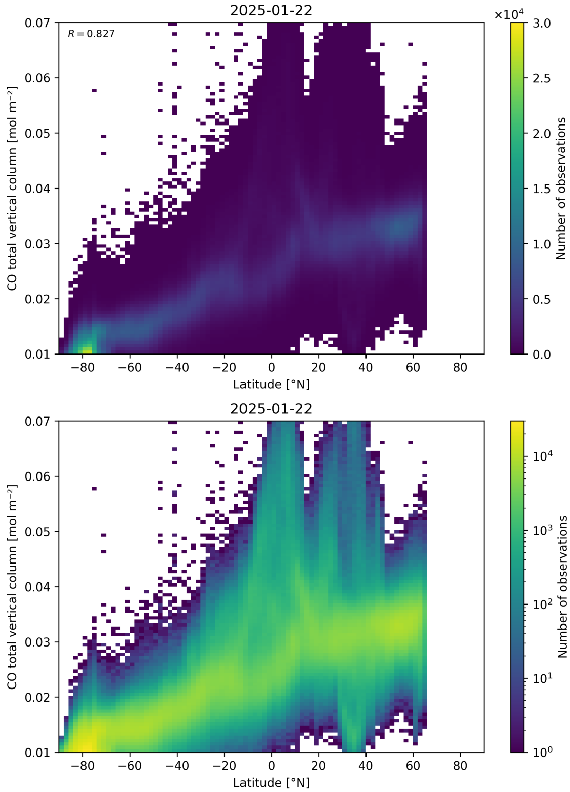
Figure 51: Scatter density plot of “Latitude” against “CO total vertical column” for 2025-01-21 to 2025-01-23.
