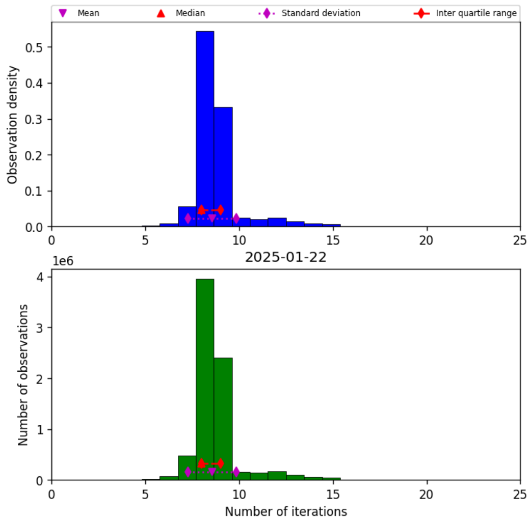
Figure 24: Histogram of “Number of iterations” for 2025-01-21 to 2025-01-23
