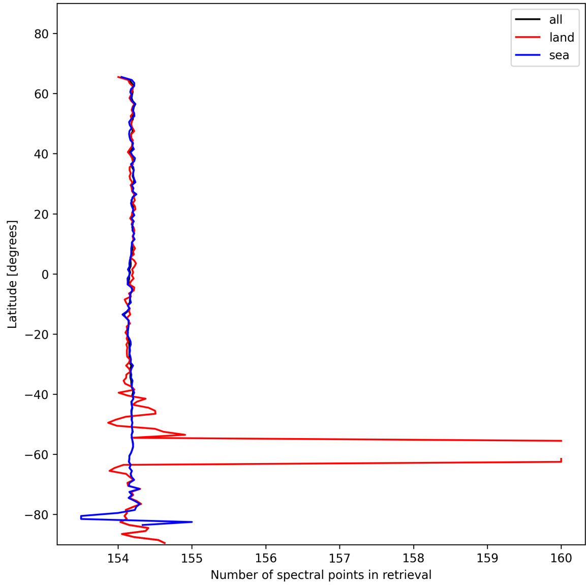
Figure 13: Zonal average of “Number of spectral points in retrieval” for 2025-01-21 to 2025-01-23.
