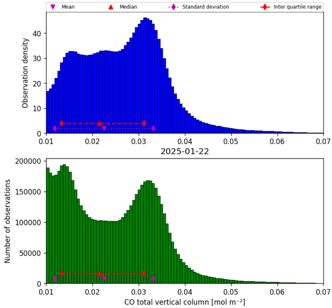
Figure 18: Histogram of “CO total vertical column” for 2025-01-21 to 2025-01-23
