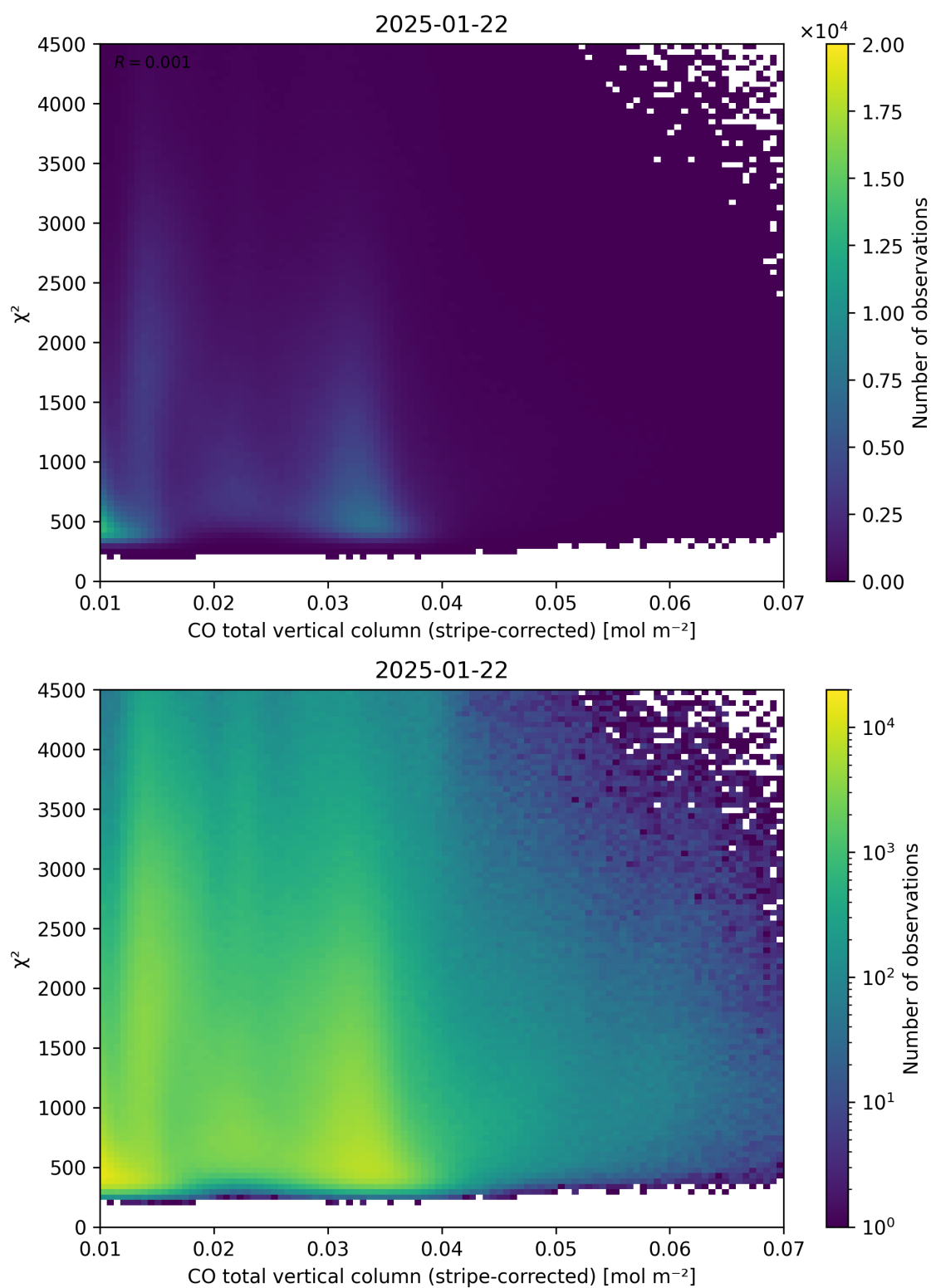
Figure 37: Scatter density plot of “CO total vertical column (stripe-corrected)” against “ \chi^2 ” for 2025-01-21 to 2025-01-23.
