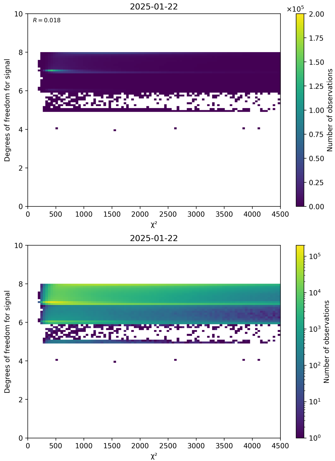
Figure 48: Scatter density plot of “ \chi^2 ” against “Degrees of freedom for signal” for 2025-01-21 to 2025-01-23.
