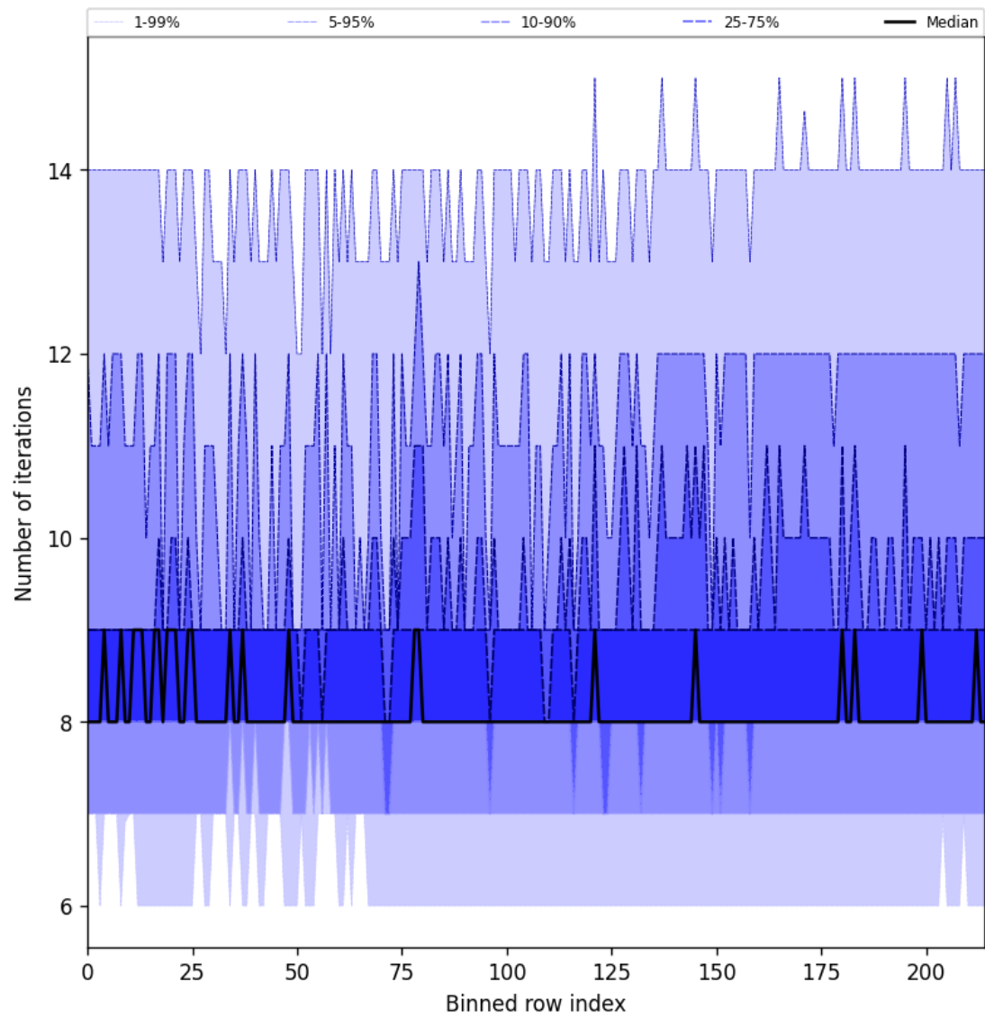
Figure 32: Along track statistics of “Number of iterations” for 2025-01-21 to 2025-01-23
