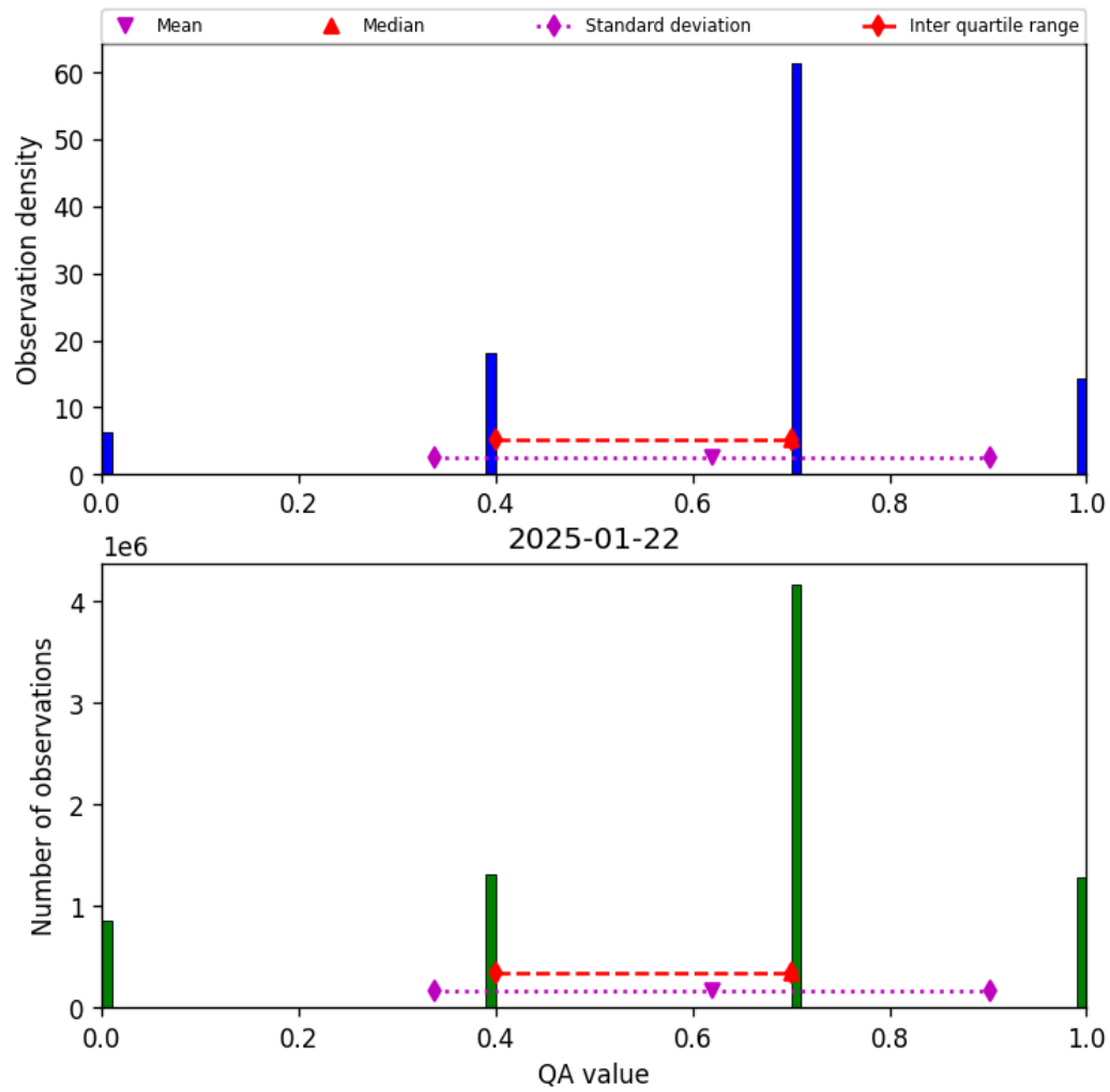
Figure 17: Histogram of “QA value” for 2025-01-21 to 2025-01-23
