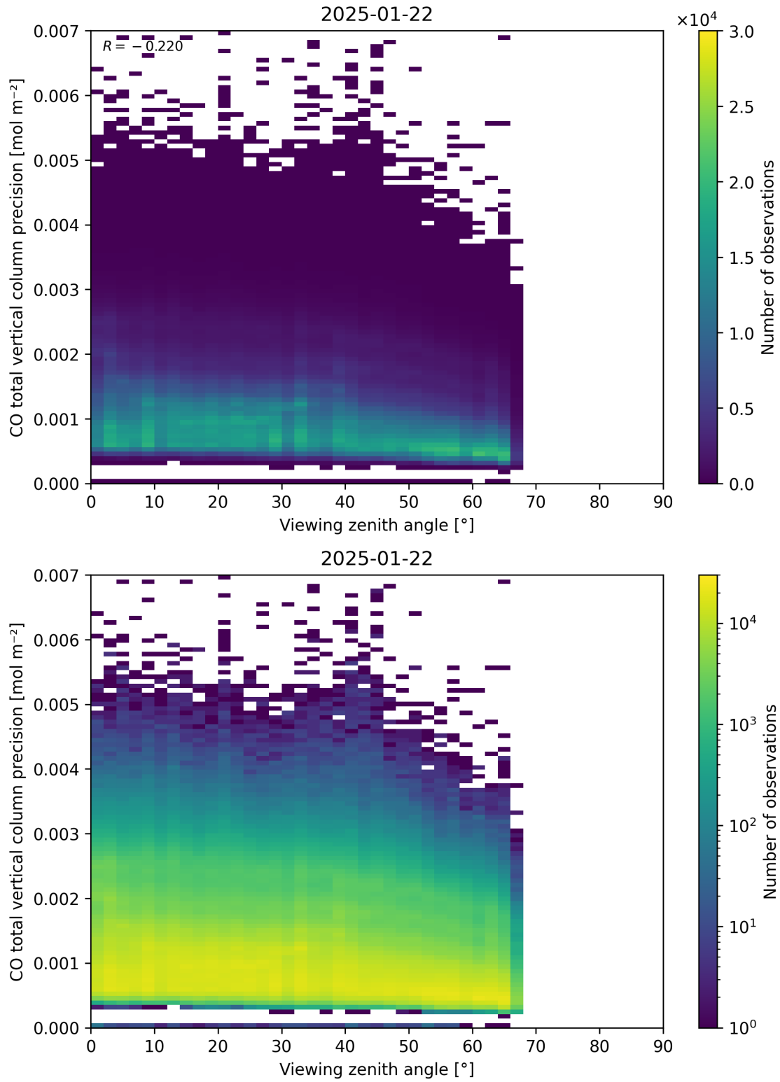
Figure 71: Scatter density plot of “Viewing zenith angle” against “CO total vertical column precision” for 2025-01-21 to 2025-01-23.
