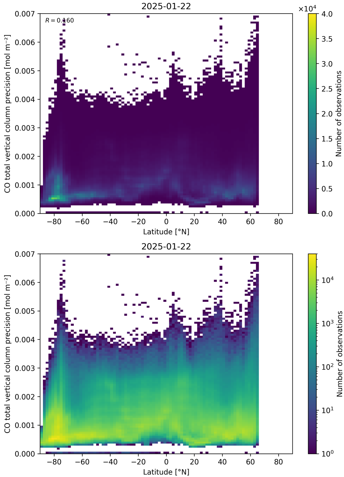
Figure 53: Scatter density plot of “Latitude” against “CO total vertical column precision” for 2025-01-21 to 2025-01-23.
