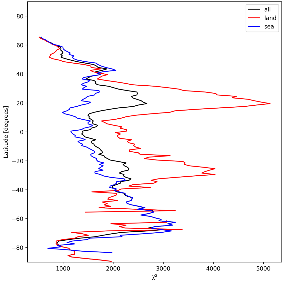
Figure 14: Zonal average of “ \chi^2 ” for 2025-01-21 to 2025-01-23.
