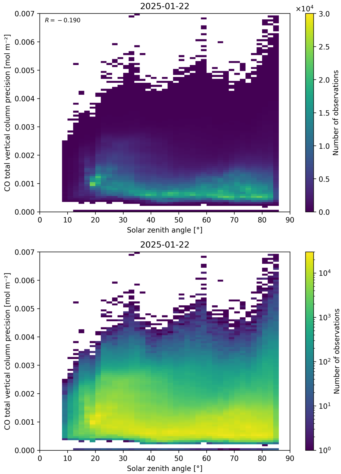
Figure 63: Scatter density plot of “Solar zenith angle” against “CO total vertical column precision” for 2025-01-21 to 2025-01-23.
