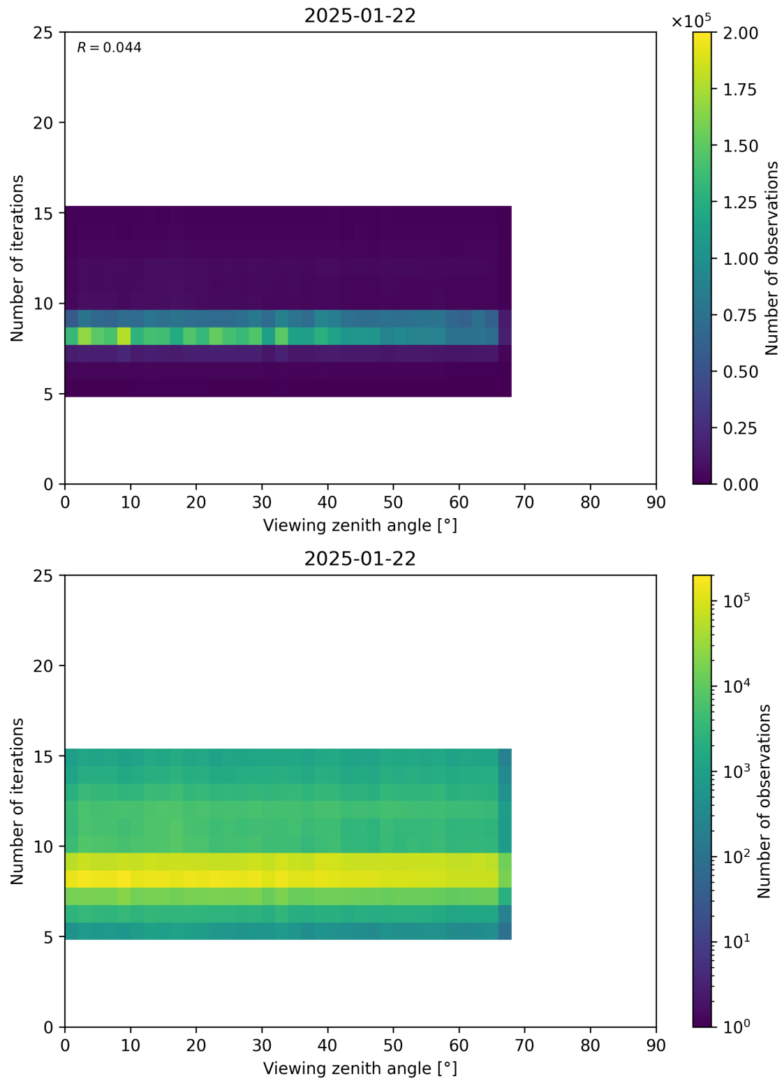
Figure 75: Scatter density plot of “Viewing zenith angle” against “Number of iterations” for 2025-01-21 to 2025-01-23.
