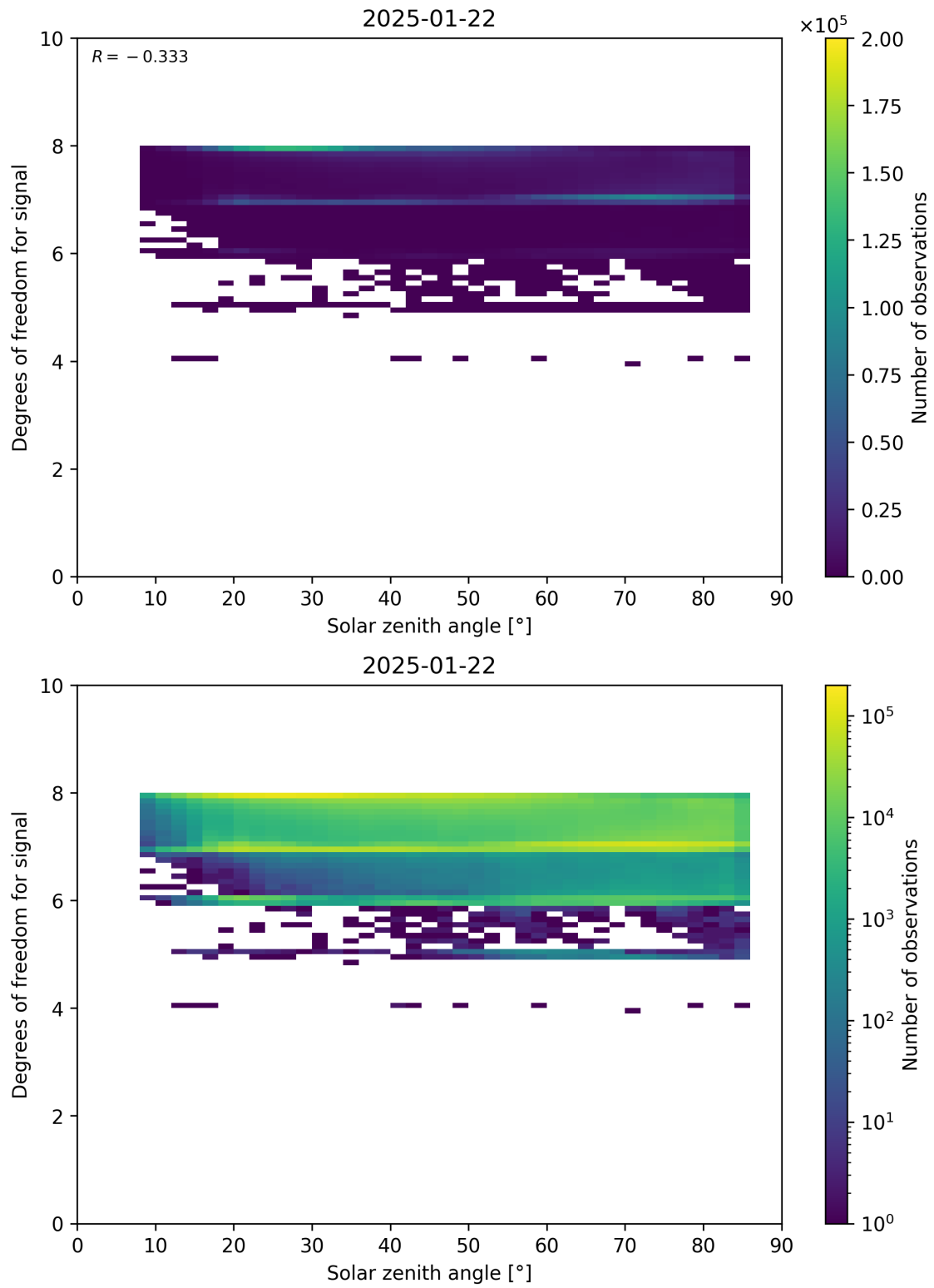
Figure 65: Scatter density plot of “Solar zenith angle” against “Degrees of freedom for signal” for 2025-01-21 to 2025-01-23.
