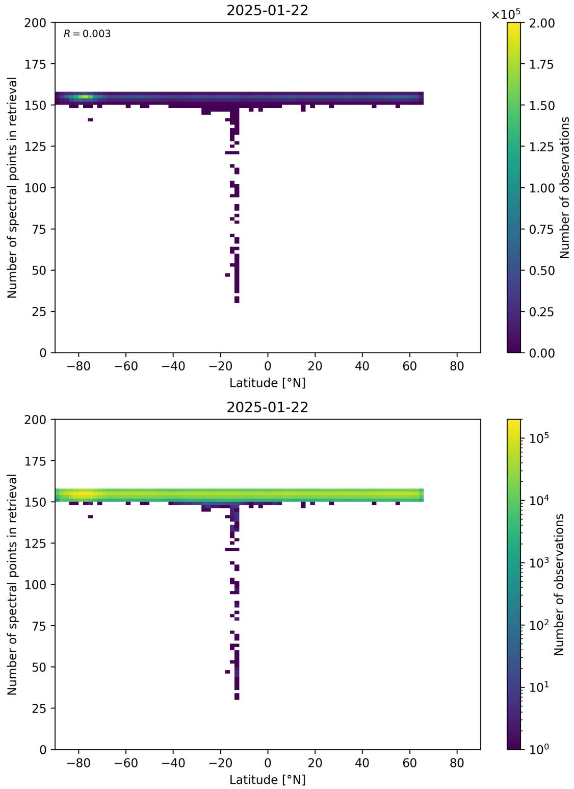
Figure 57: Scatter density plot of “Latitude” against “Number of spectral points in retrieval” for 2025-01-21 to 2025-01-23.
