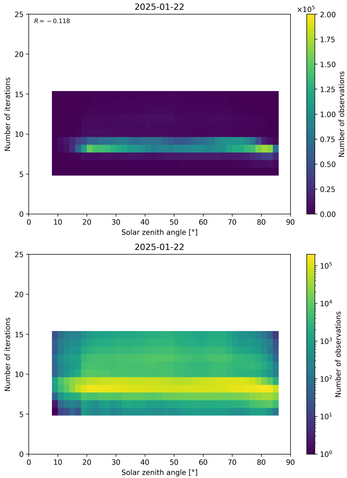
Figure 67: Scatter density plot of “Solar zenith angle” against “Number of iterations” for 2025-01-21 to 2025-01-23.
