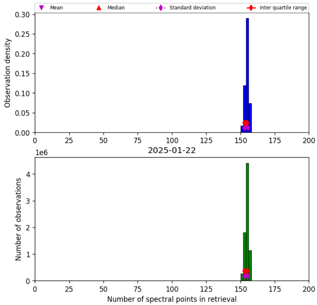
Figure 21: Histogram of “Number of spectral points in retrieval” for 2025-01-21 to 2025-01-23
