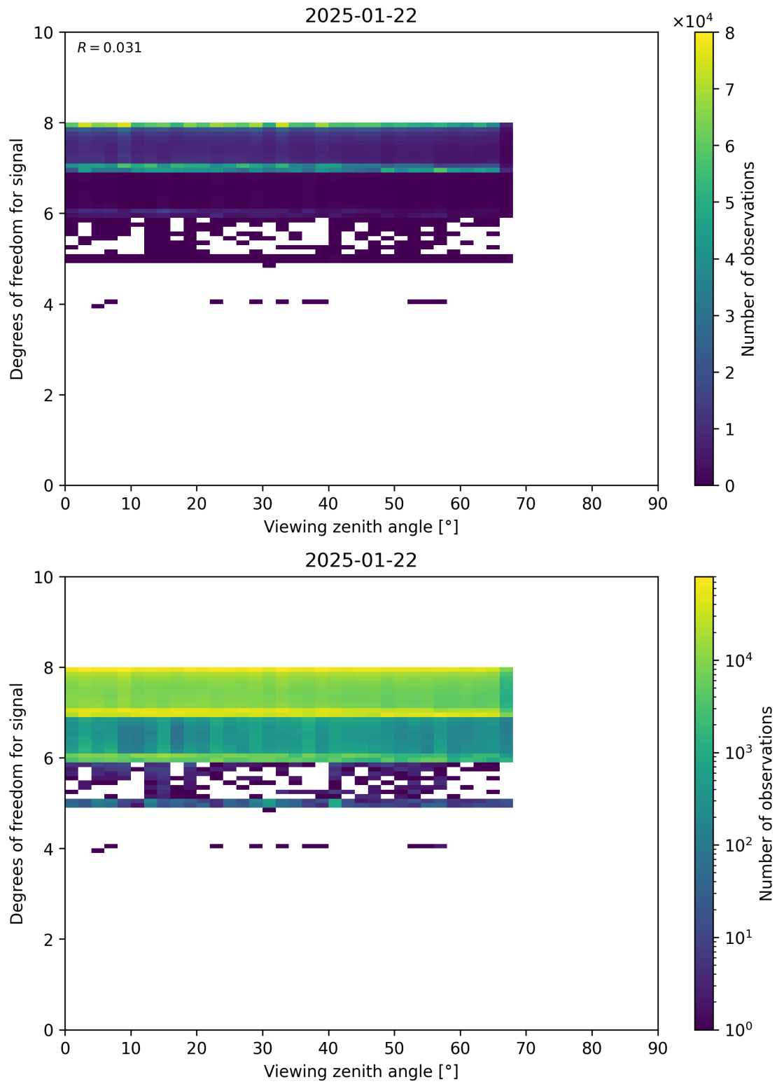
Figure 73: Scatter density plot of “Viewing zenith angle” against “Degrees of freedom for signal” for 2025-01-21 to 2025-01-23.
