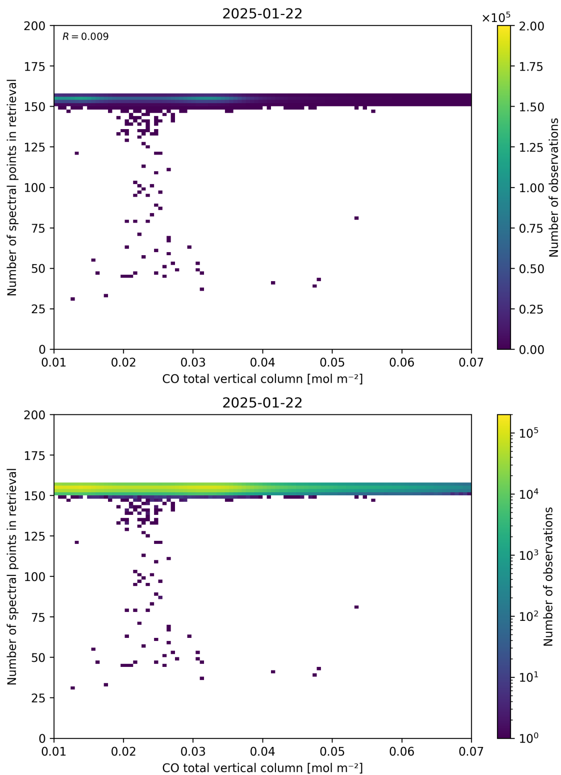
Figure 43: Scatter density plot of “CO total vertical column” against “Number of spectral points in retrieval” for 2025-01-21 to 2025-01-23.
