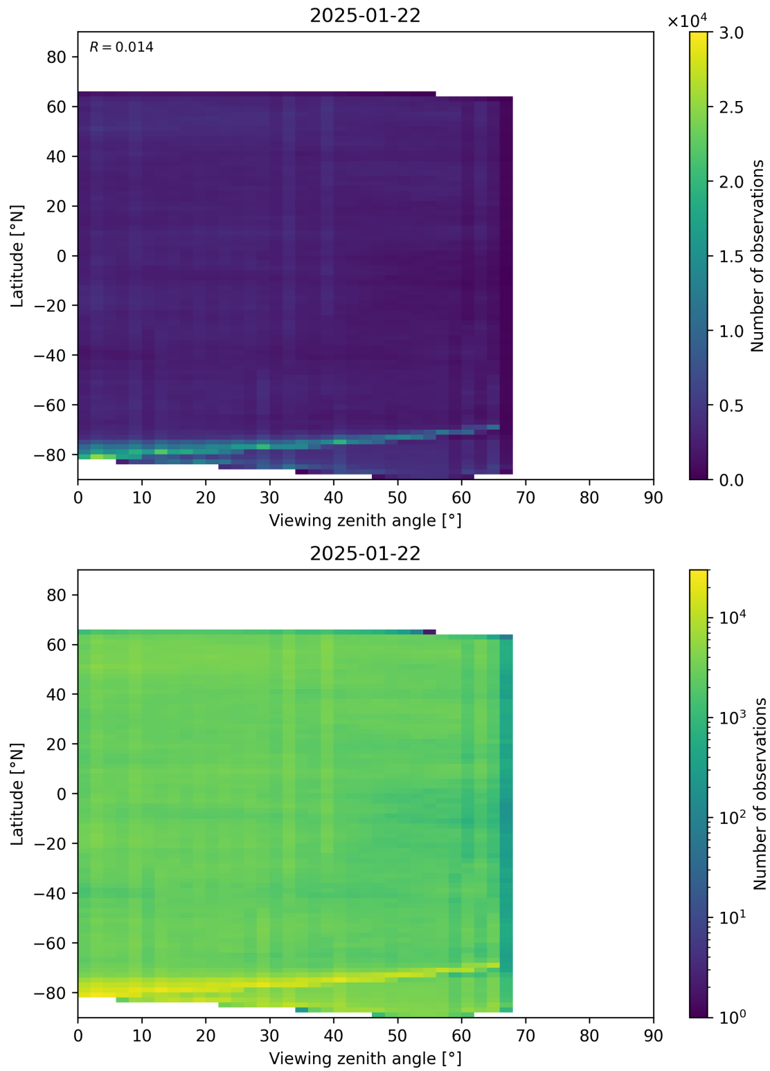
Figure 74: Scatter density plot of “Viewing zenith angle” against “Latitude” for 2025-01-21 to 2025-01-23.
