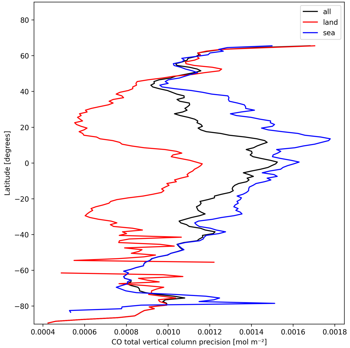
Figure 12: Zonal average of “CO total vertical column precision” for 2025-01-21 to 2025-01-23.
