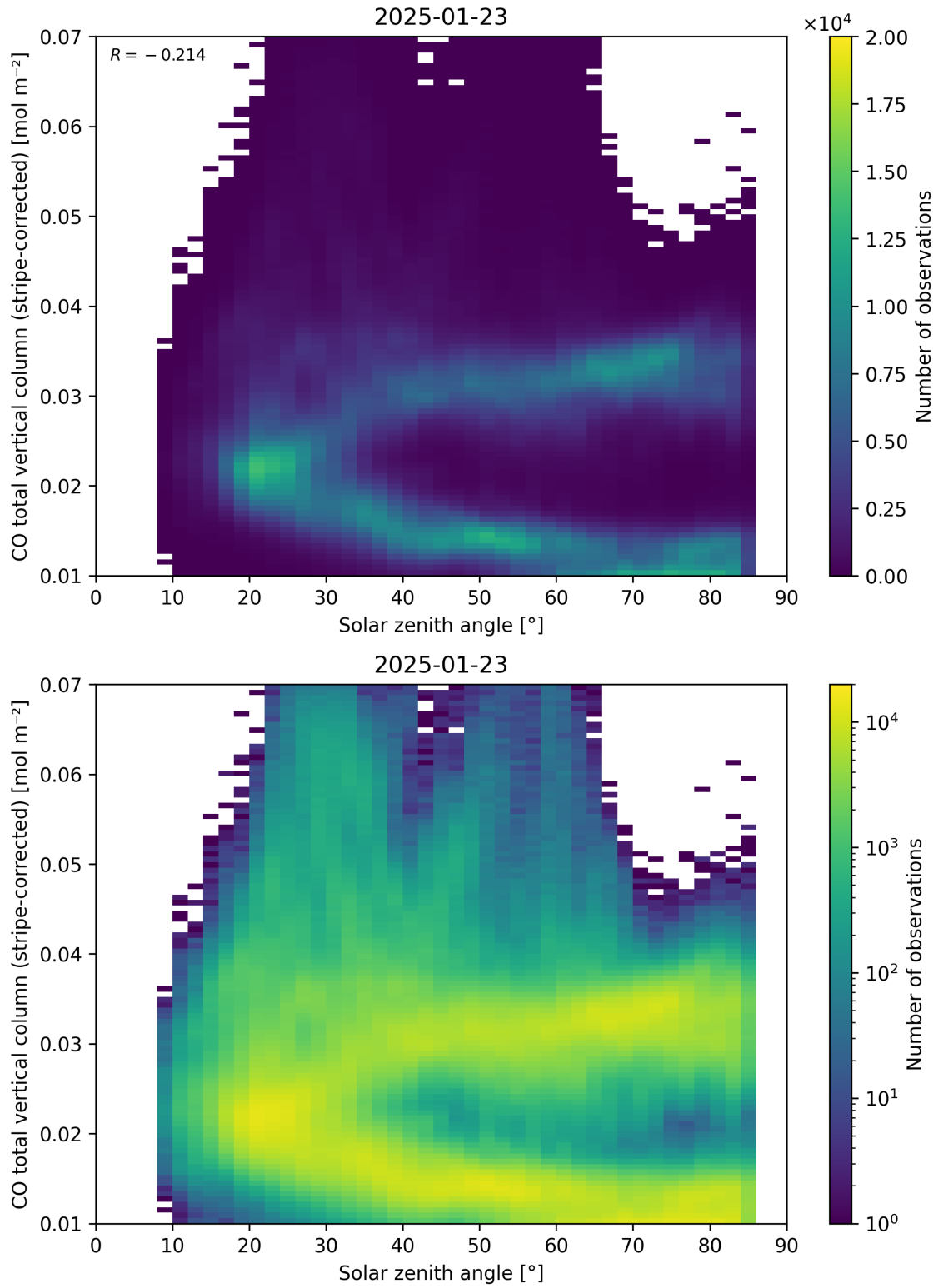
Figure 62: Scatter density plot of “Solar zenith angle” against “CO total vertical column (stripe-corrected)” for 2025-01-23 to 2025-01-24.
