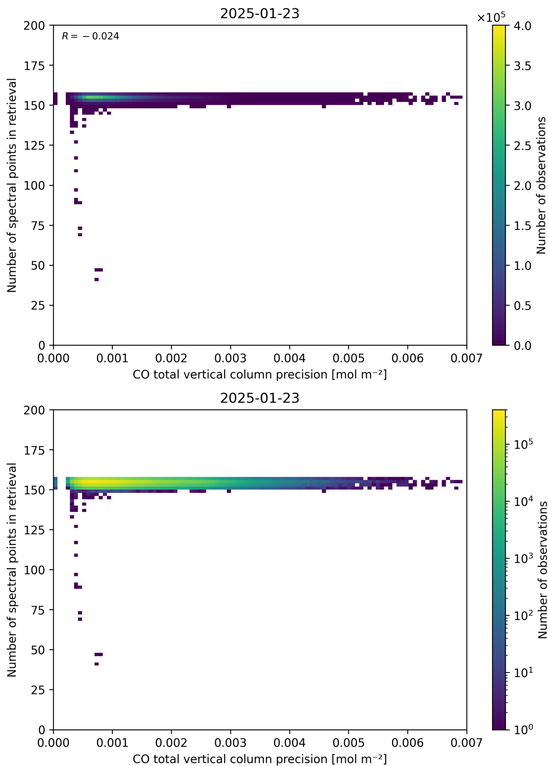
Figure 47: Scatter density plot of “CO total vertical column precision” against “Number of spectral points in retrieval” for 2025-01-23 to 2025-01-24.
