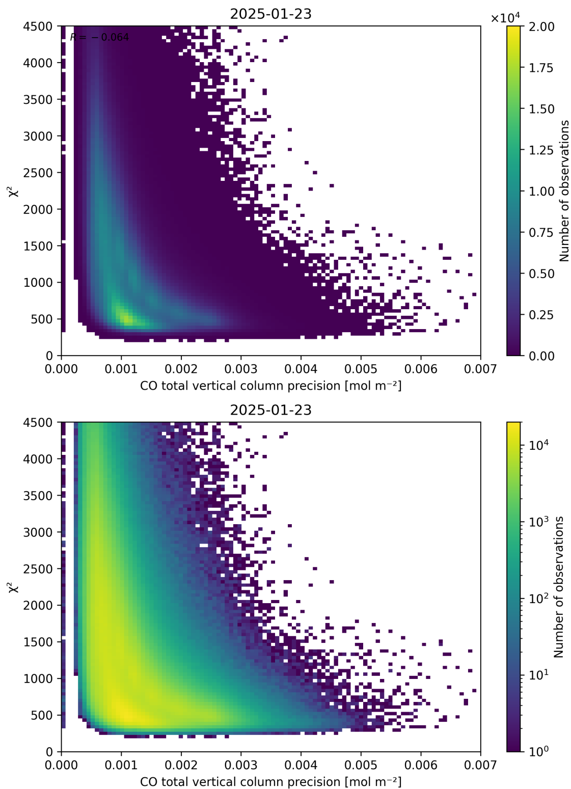
Figure 44: Scatter density plot of “CO total vertical column precision” against “ \chi^2 ” for 2025-01-23 to 2025-01-24.
