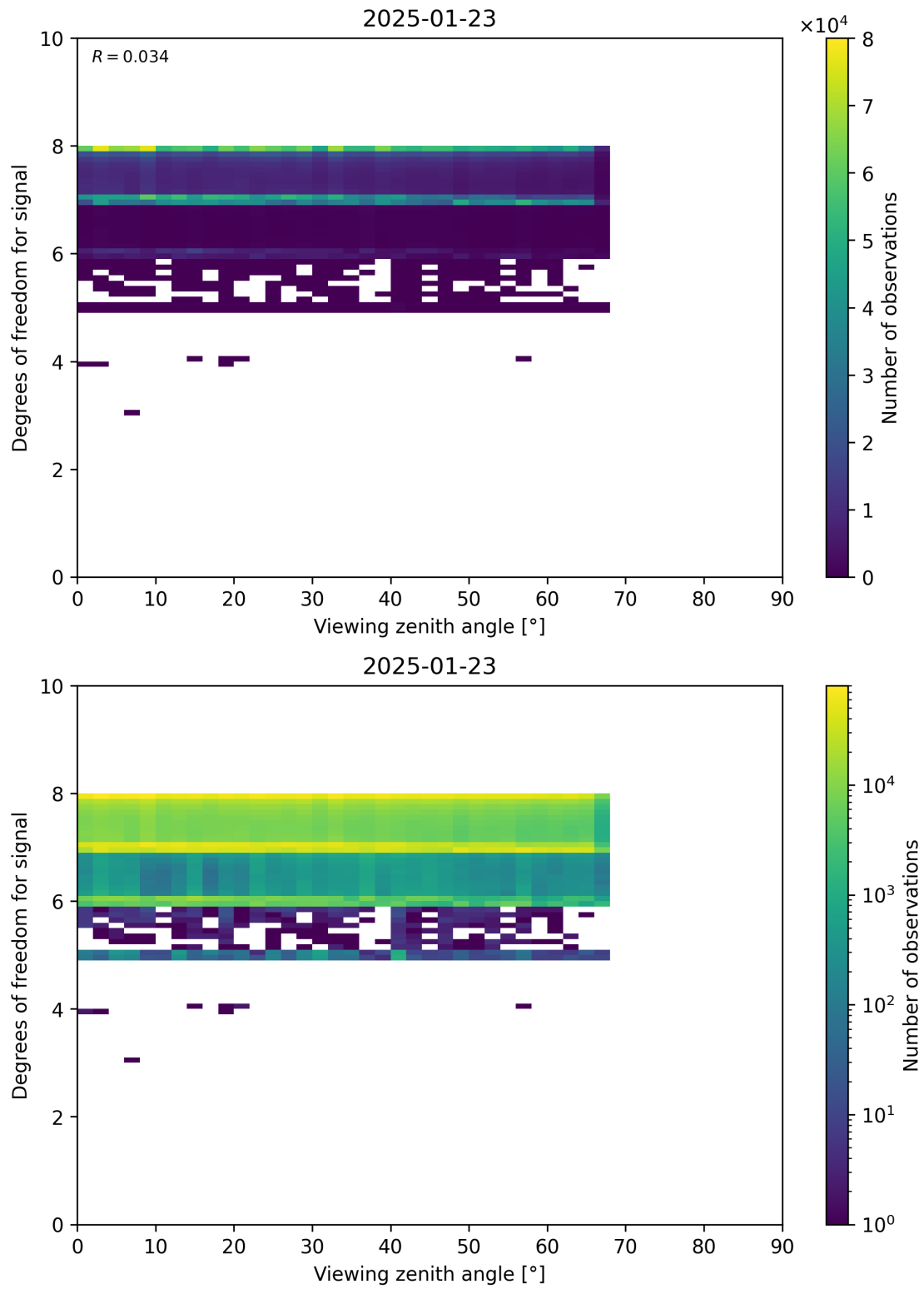
Figure 73: Scatter density plot of “Viewing zenith angle” against “Degrees of freedom for signal” for 2025-01-23 to 2025-01-24.
