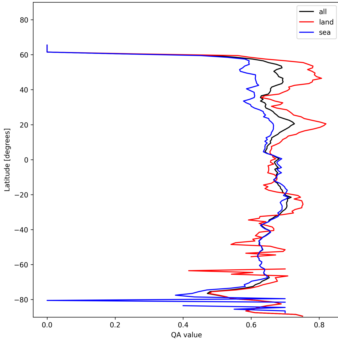
Figure 9: Zonal average of “QA value” for 2025-01-23 to 2025-01-24.
