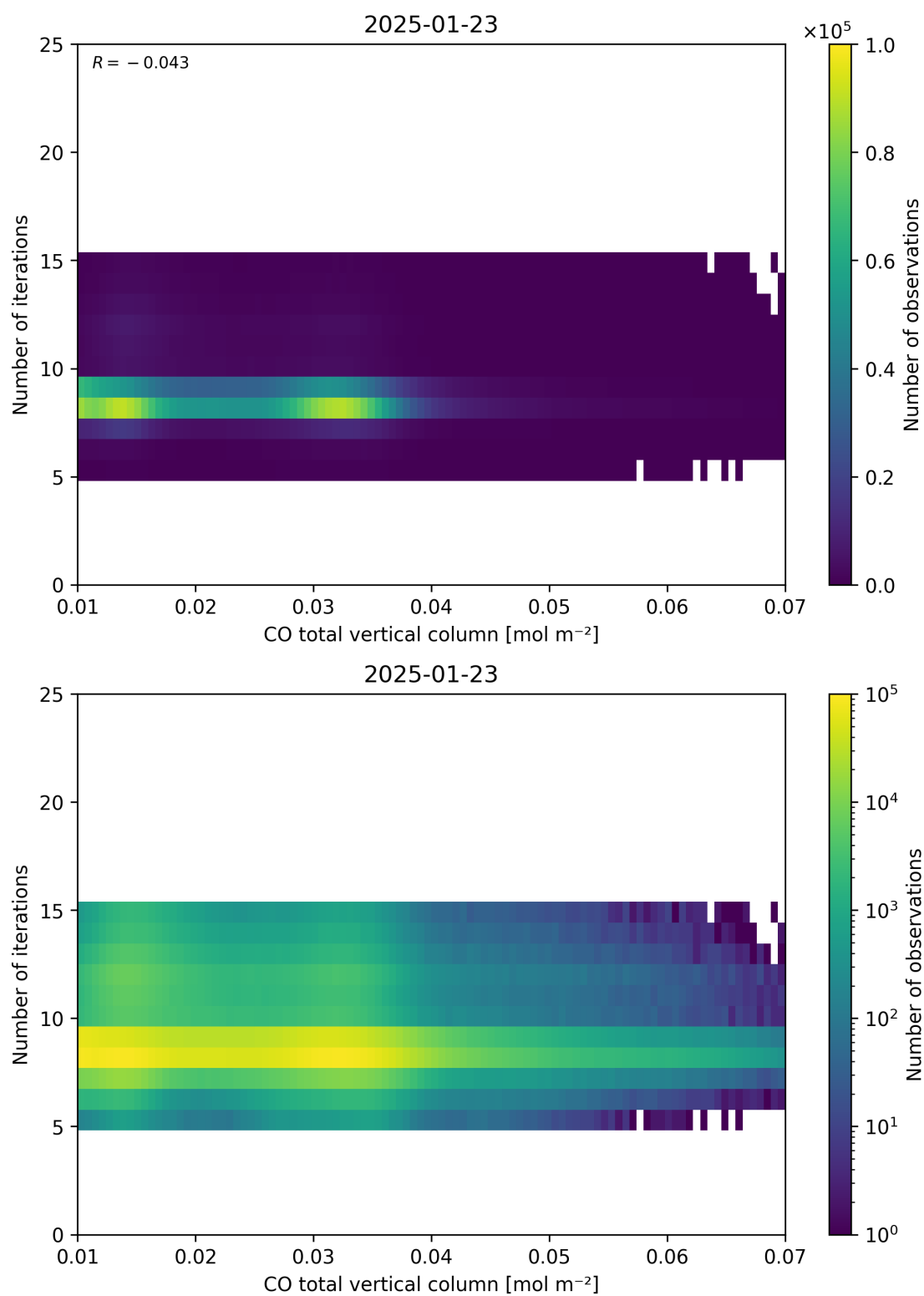
Figure 42: Scatter density plot of “CO total vertical column” against “Number of iterations” for 2025-01-23 to 2025-01-24.
