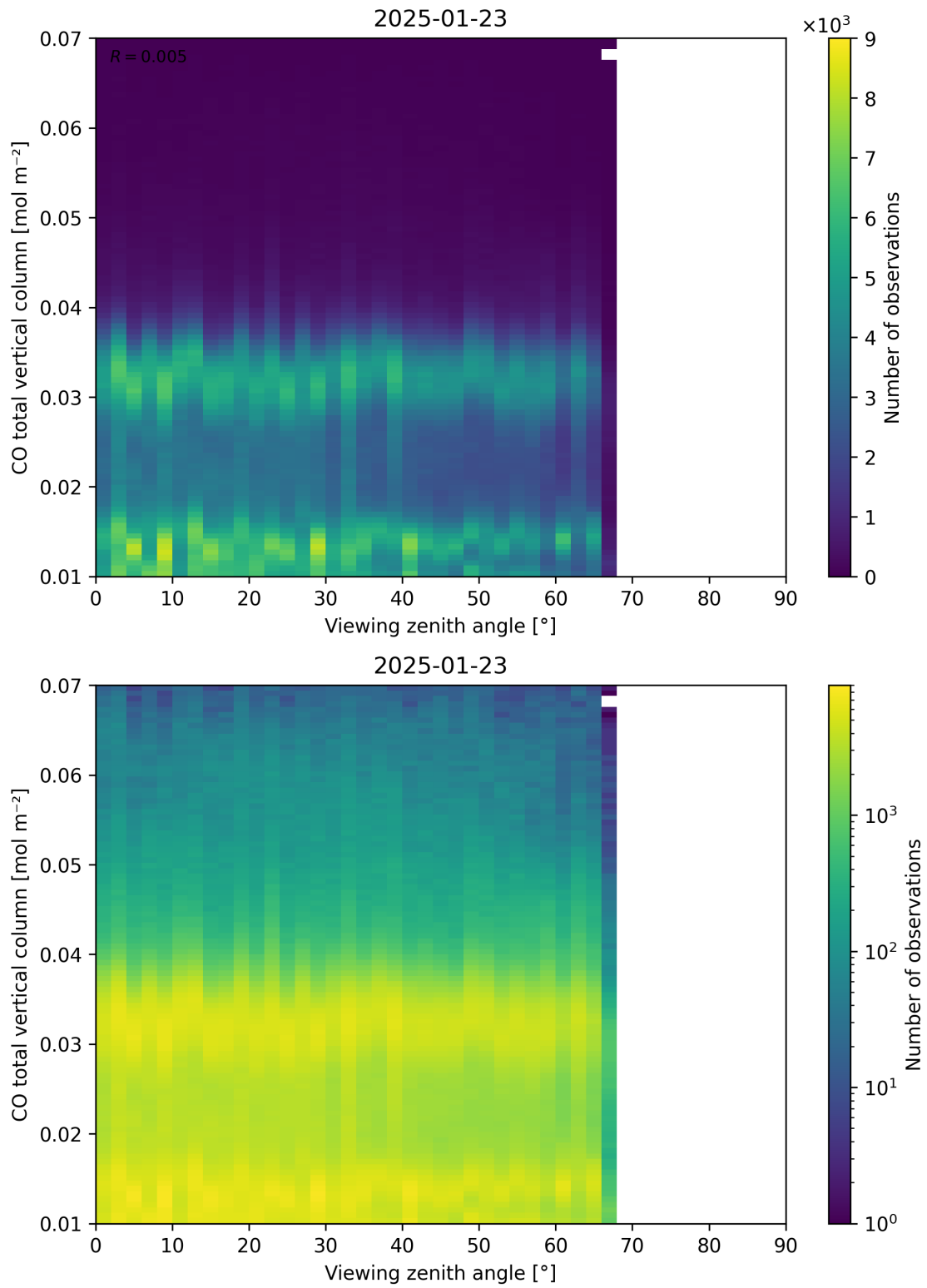
Figure 69: Scatter density plot of “Viewing zenith angle” against “CO total vertical column” for 2025-01-23 to 2025-01-24.
