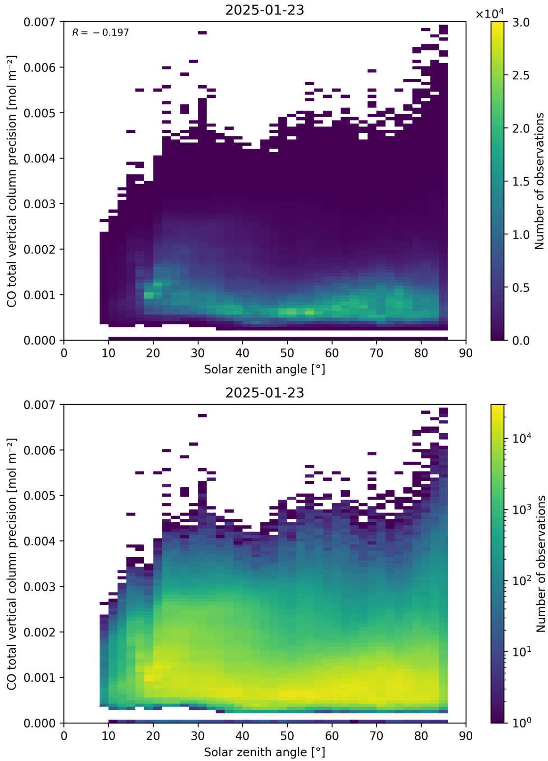
Figure 63: Scatter density plot of “Solar zenith angle” against “CO total vertical column precision” for 2025-01-23 to 2025-01-24.
