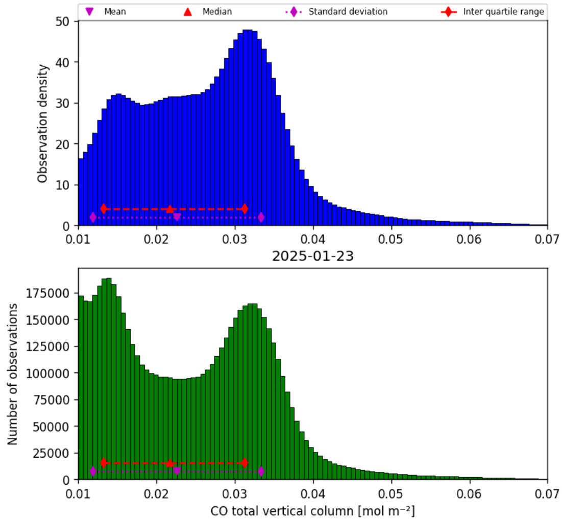
Figure 18: Histogram of “CO total vertical column” for 2025-01-23 to 2025-01-24
