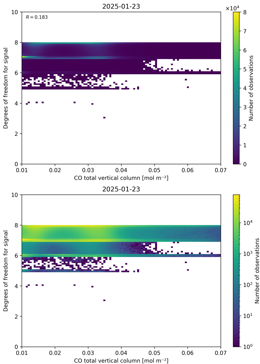
Figure 41: Scatter density plot of “CO total vertical column” against “Degrees of freedom for signal” for 2025-01-23 to 2025-01-24.
