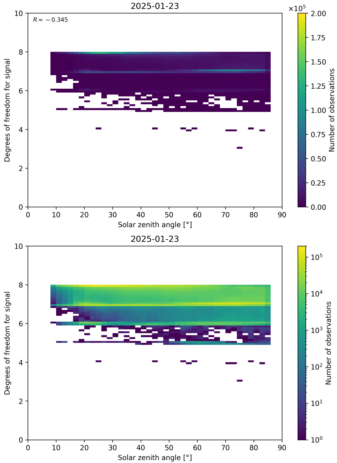
Figure 65: Scatter density plot of “Solar zenith angle” against “Degrees of freedom for signal” for 2025-01-23 to 2025-01-24.
