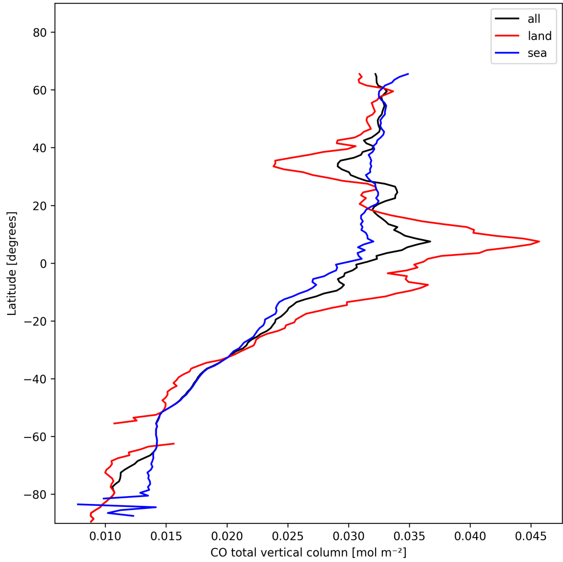
Figure 10: Zonal average of “CO total vertical column” for 2025-01-23 to 2025-01-24.
