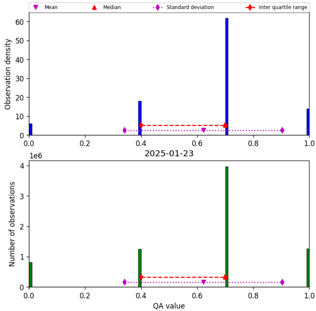
Figure 17: Histogram of “QA value” for 2025-01-23 to 2025-01-24
