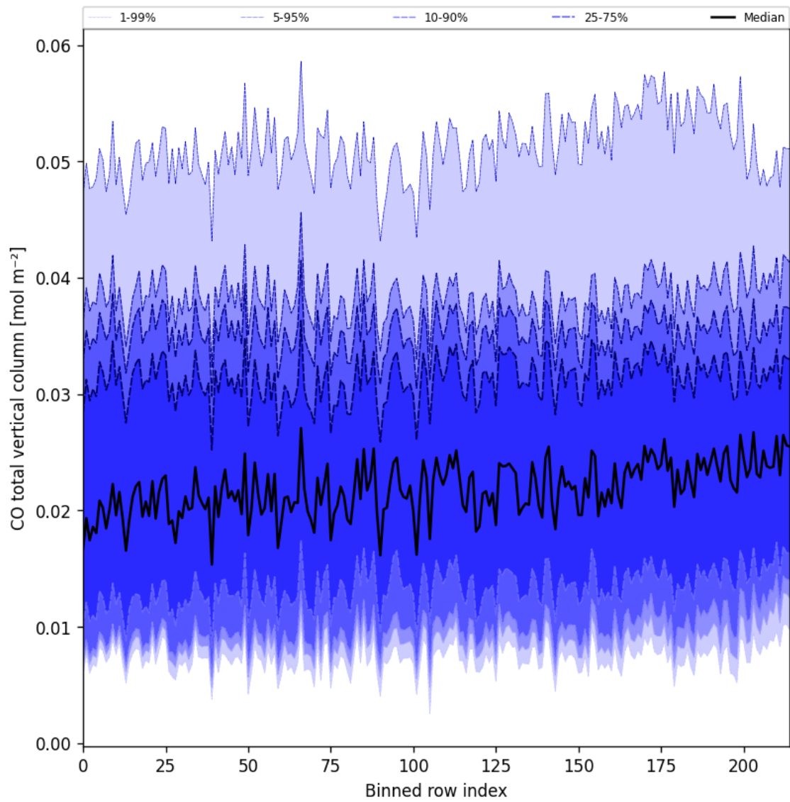
Figure 26: Along track statistics of “CO total vertical column” for 2025-01-23 to 2025-01-24
