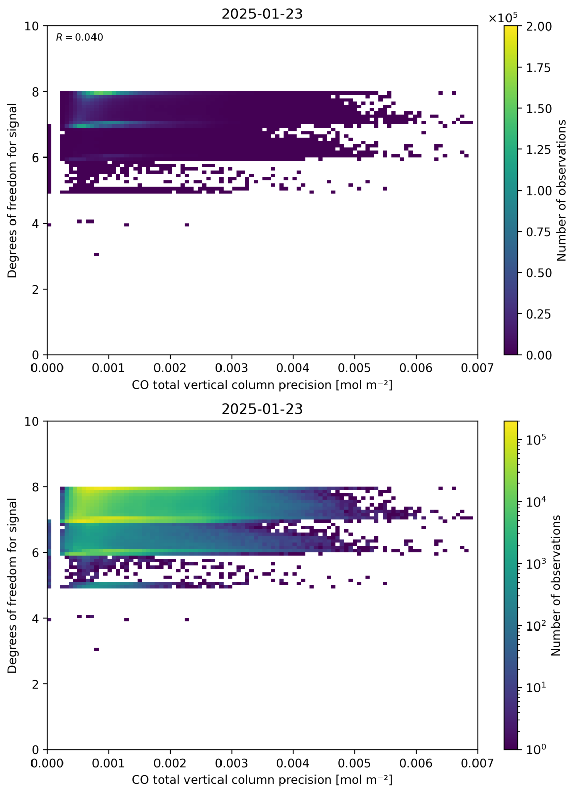
Figure 45: Scatter density plot of “CO total vertical column precision” against “Degrees of freedom for signal” for 2025-01-23 to 2025-01-24.
