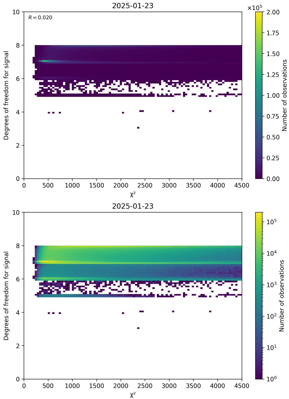
Figure 48: Scatter density plot of “ \chi^2 ” against “Degrees of freedom for signal” for 2025-01-23 to 2025-01-24.
