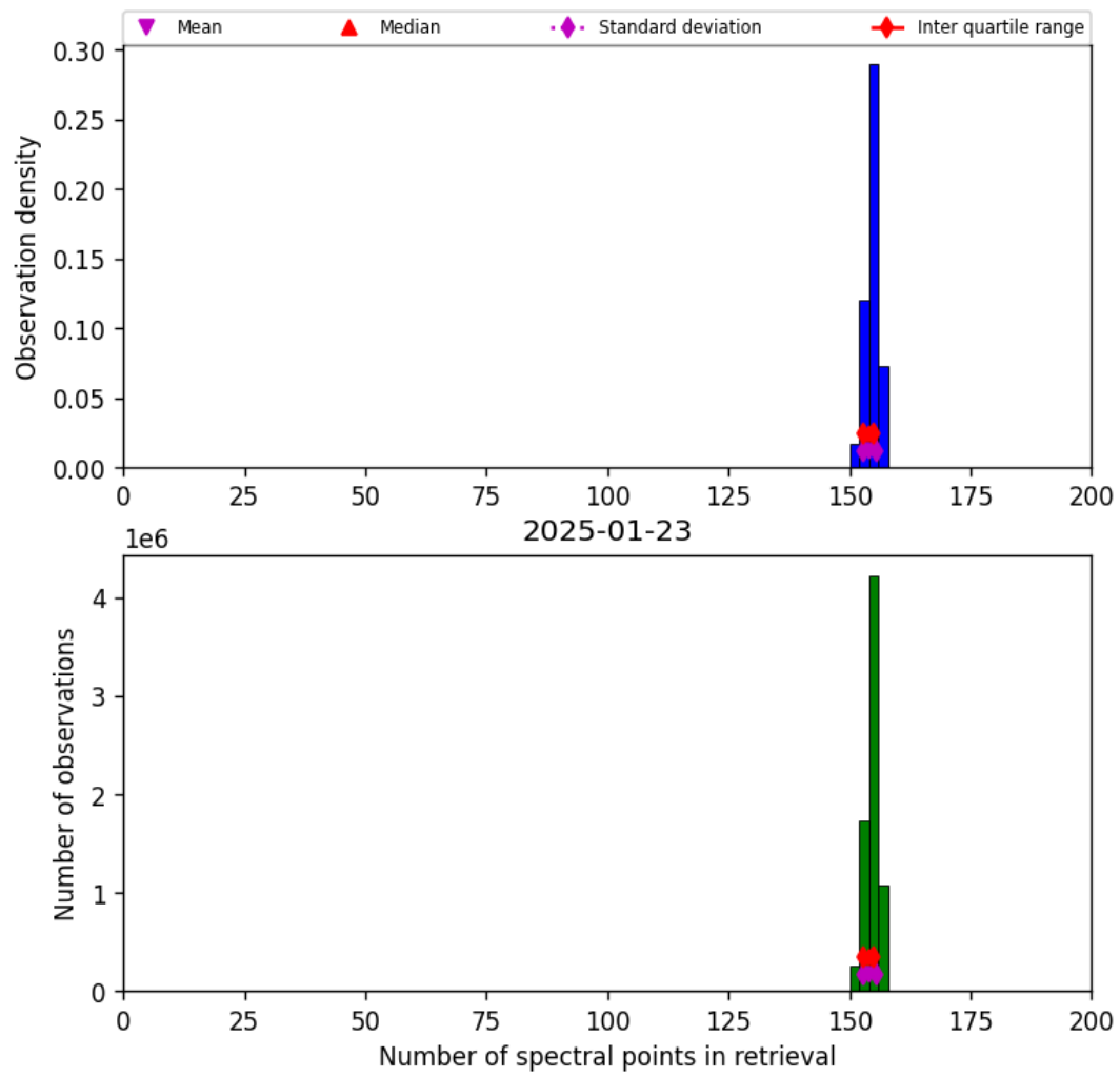
Figure 21: Histogram of “Number of spectral points in retrieval” for 2025-01-23 to 2025-01-24
