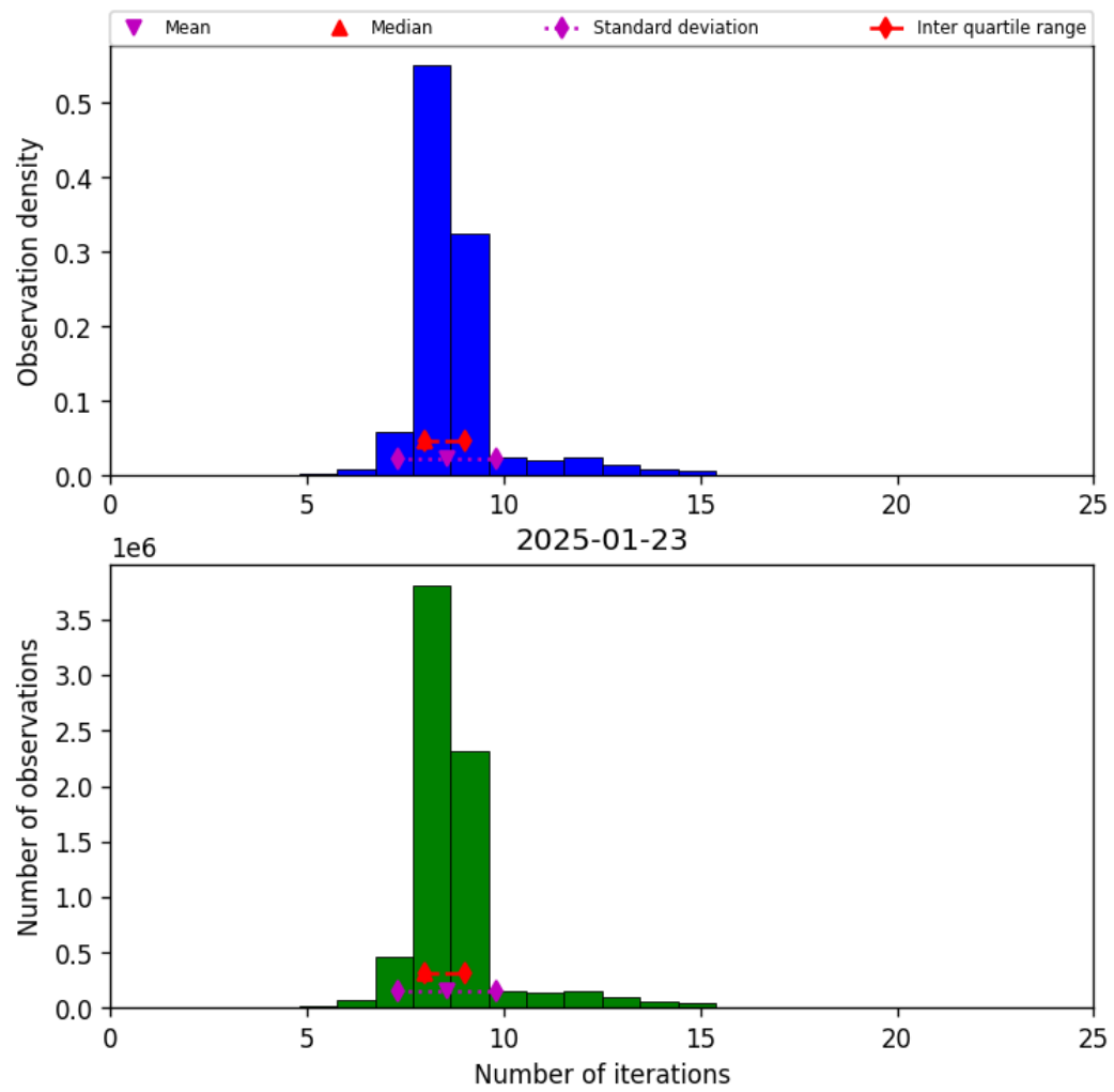
Figure 24: Histogram of “Number of iterations” for 2025-01-23 to 2025-01-24
