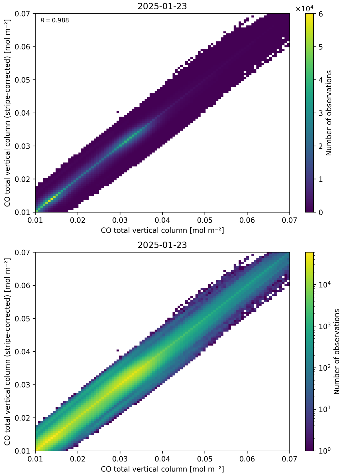
Figure 33: Scatter density plot of “CO total vertical column” against “CO total vertical column (stripe-corrected)” for 2025-01-23 to 2025-01-24.
