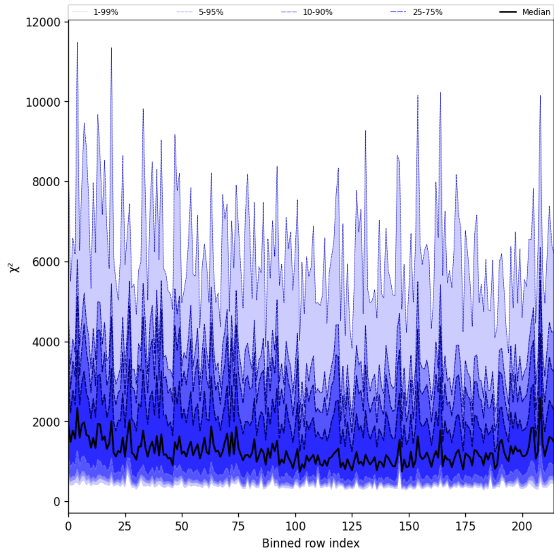
Figure 30: Along track statistics of “ \chi^2 ” for 2025-01-23 to 2025-01-24
