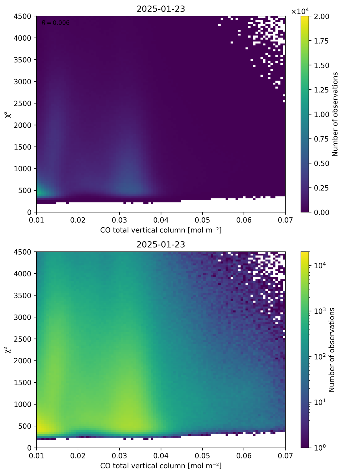
Figure 35: Scatter density plot of “CO total vertical column” against “ \chi^2 ” for 2025-01-23 to 2025-01-24.
