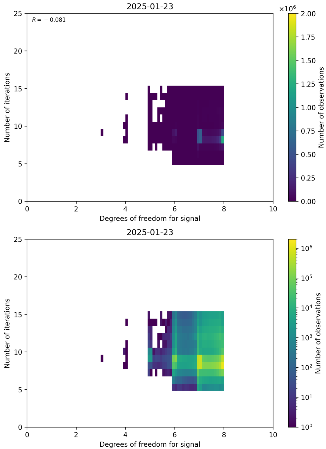
Figure 50: Scatter density plot of “Degrees of freedom for signal” against “Number of iterations” for 2025-01-23 to 2025-01-24.
