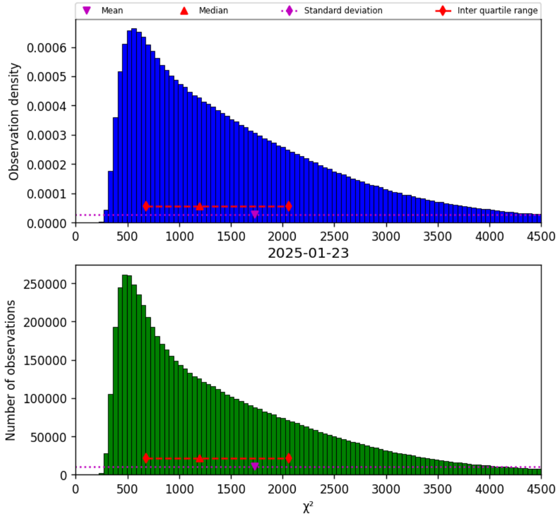
Figure 22: Histogram of “ \chi^2 ” for 2025-01-23 to 2025-01-24
