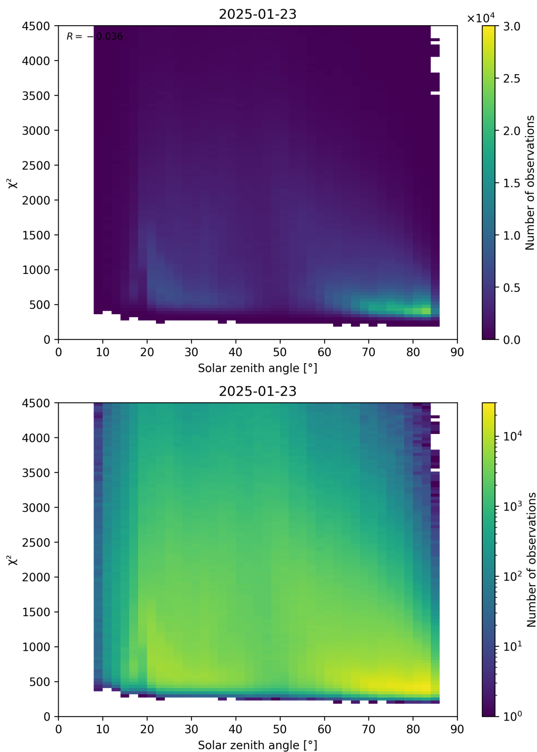
Figure 64: Scatter density plot of “Solar zenith angle” against “ \chi^2 ” for 2025-01-23 to 2025-01-24.
