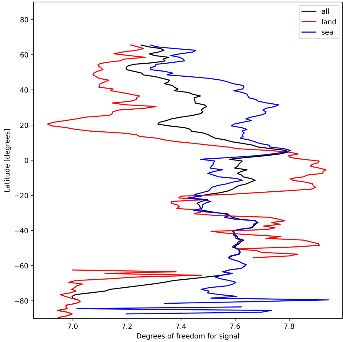
Figure 15: Zonal average of “Degrees of freedom for signal” for 2025-01-23 to 2025-01-24.
