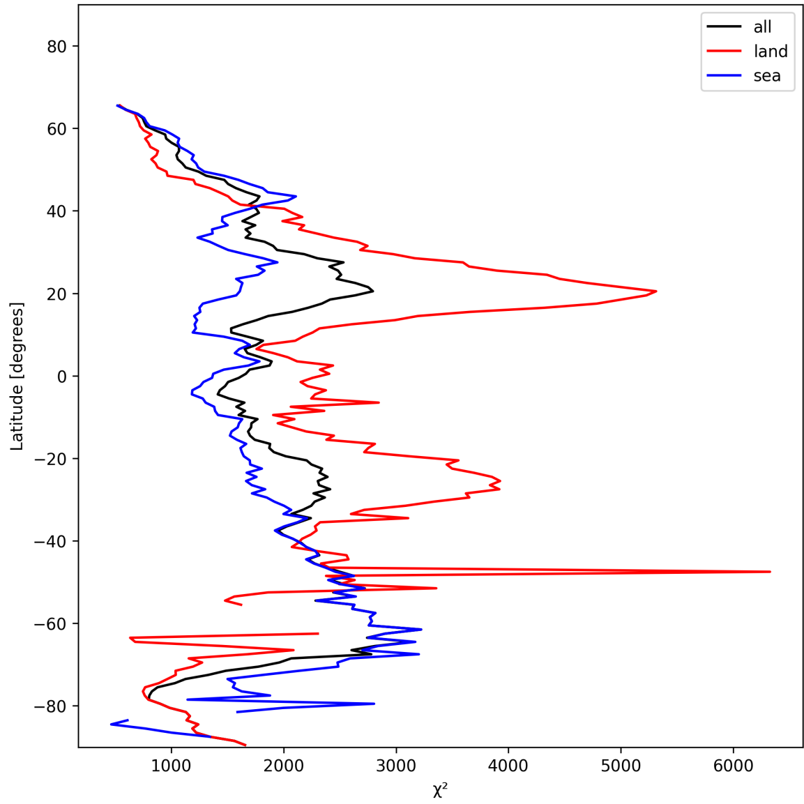
Figure 14: Zonal average of “ \chi^2 ” for 2025-01-23 to 2025-01-24.
