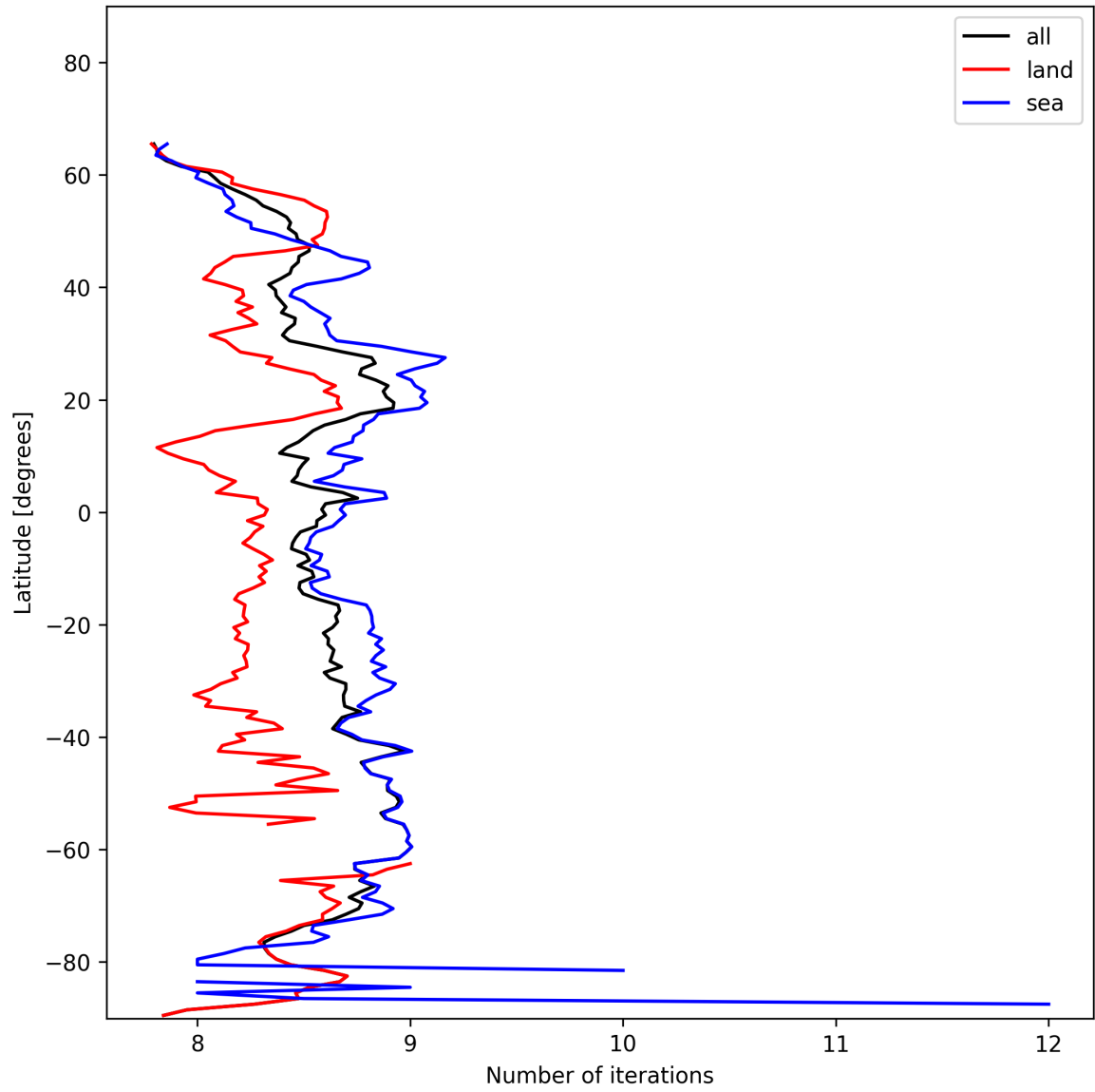
Figure 16: Zonal average of “Number of iterations” for 2025-01-23 to 2025-01-24.
