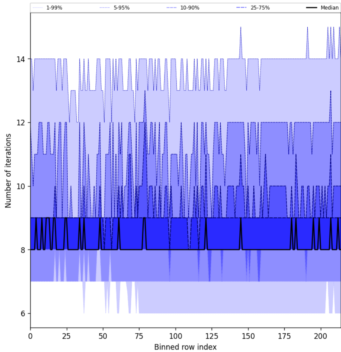
Figure 32: Along track statistics of “Number of iterations” for 2025-01-23 to 2025-01-24
