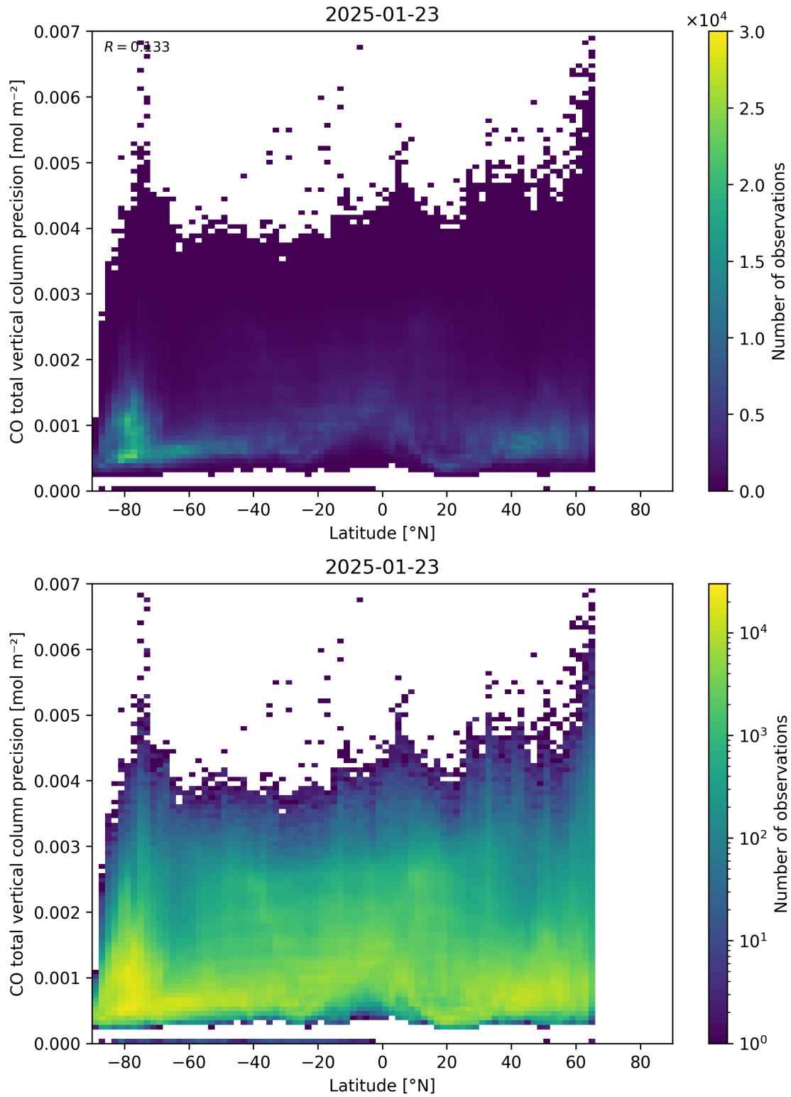
Figure 53: Scatter density plot of “Latitude” against “CO total vertical column precision” for 2025-01-23 to 2025-01-24.
