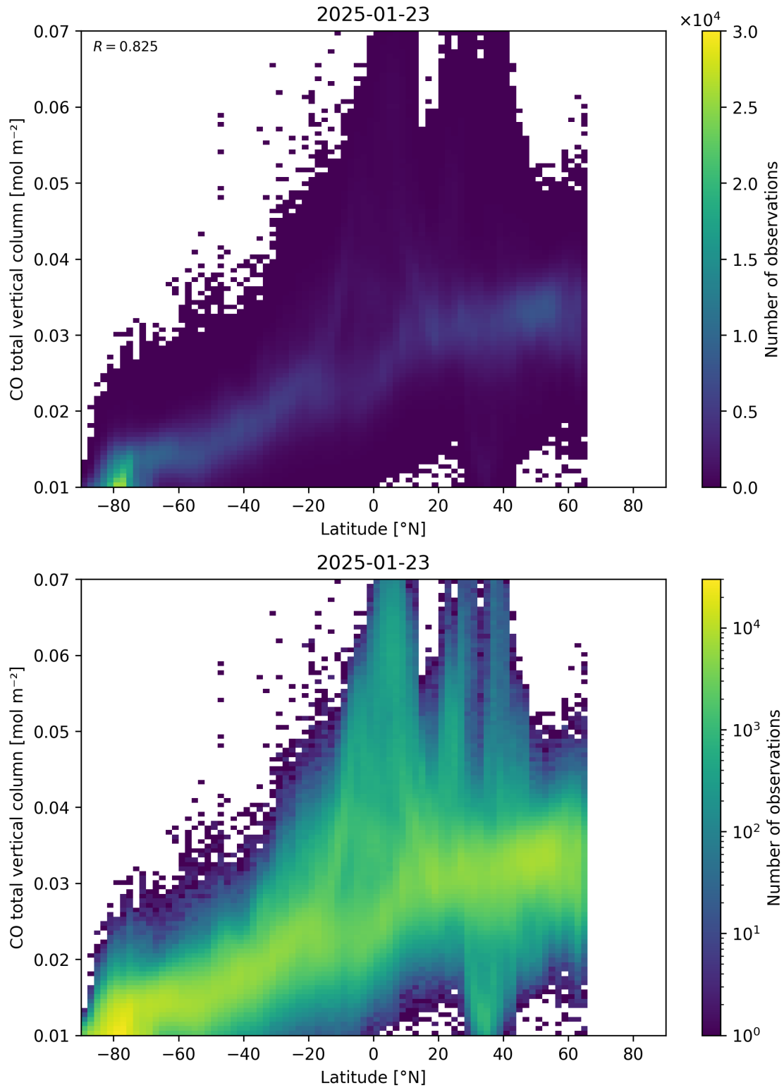
Figure 51: Scatter density plot of “Latitude” against “CO total vertical column” for 2025-01-23 to 2025-01-24.
