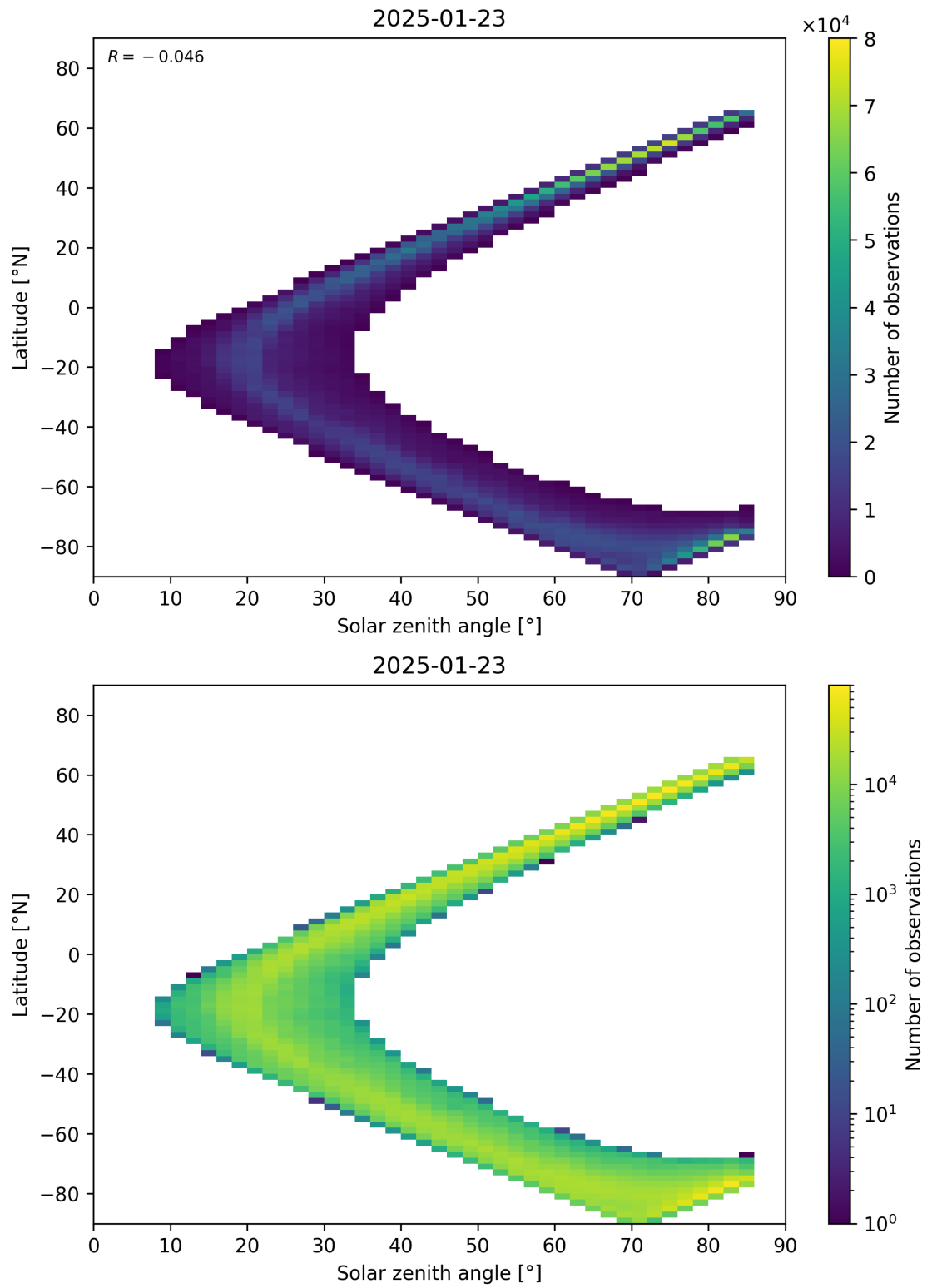
Figure 66: Scatter density plot of “Solar zenith angle” against “Latitude” for 2025-01-23 to 2025-01-24.
