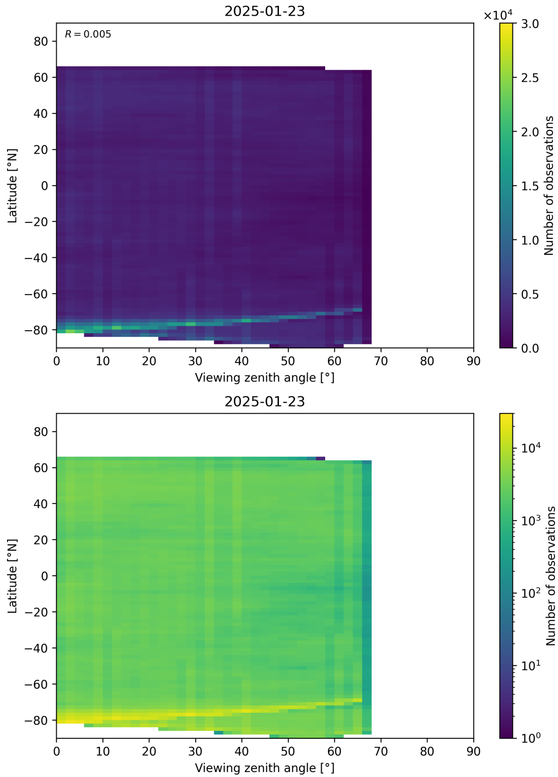
Figure 74: Scatter density plot of “Viewing zenith angle” against “Latitude” for 2025-01-23 to 2025-01-24.
