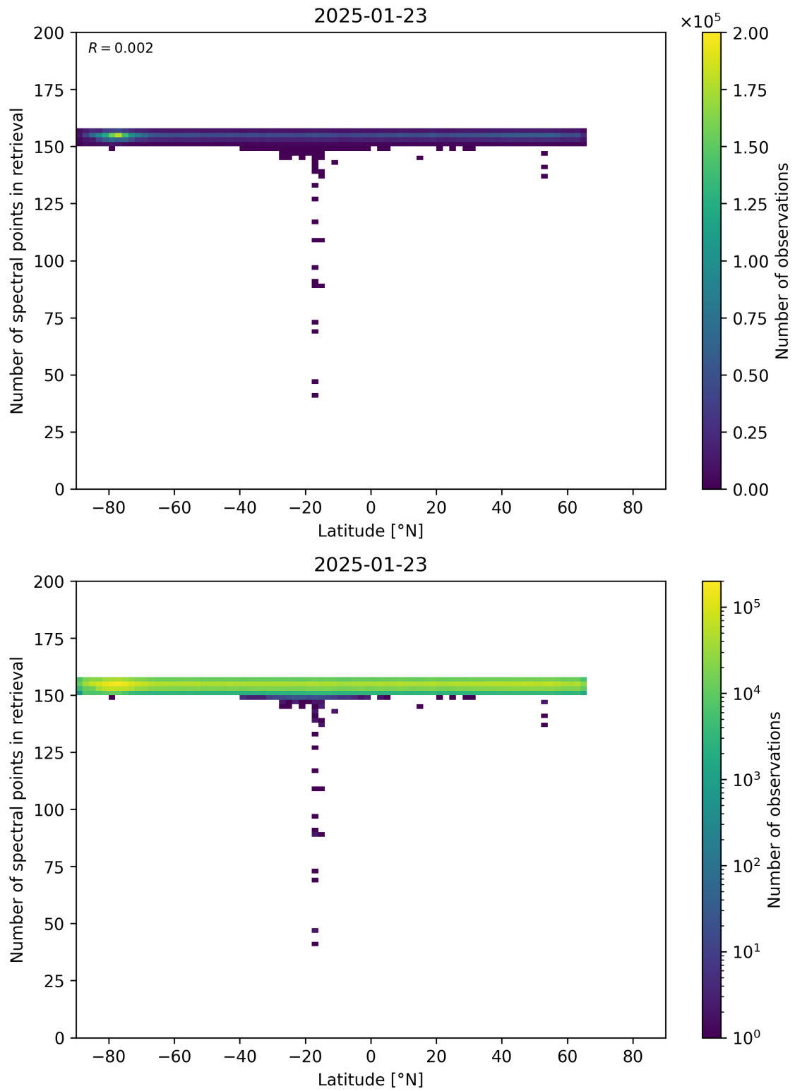
Figure 57: Scatter density plot of “Latitude” against “Number of spectral points in retrieval” for 2025-01-23 to 2025-01-24.
