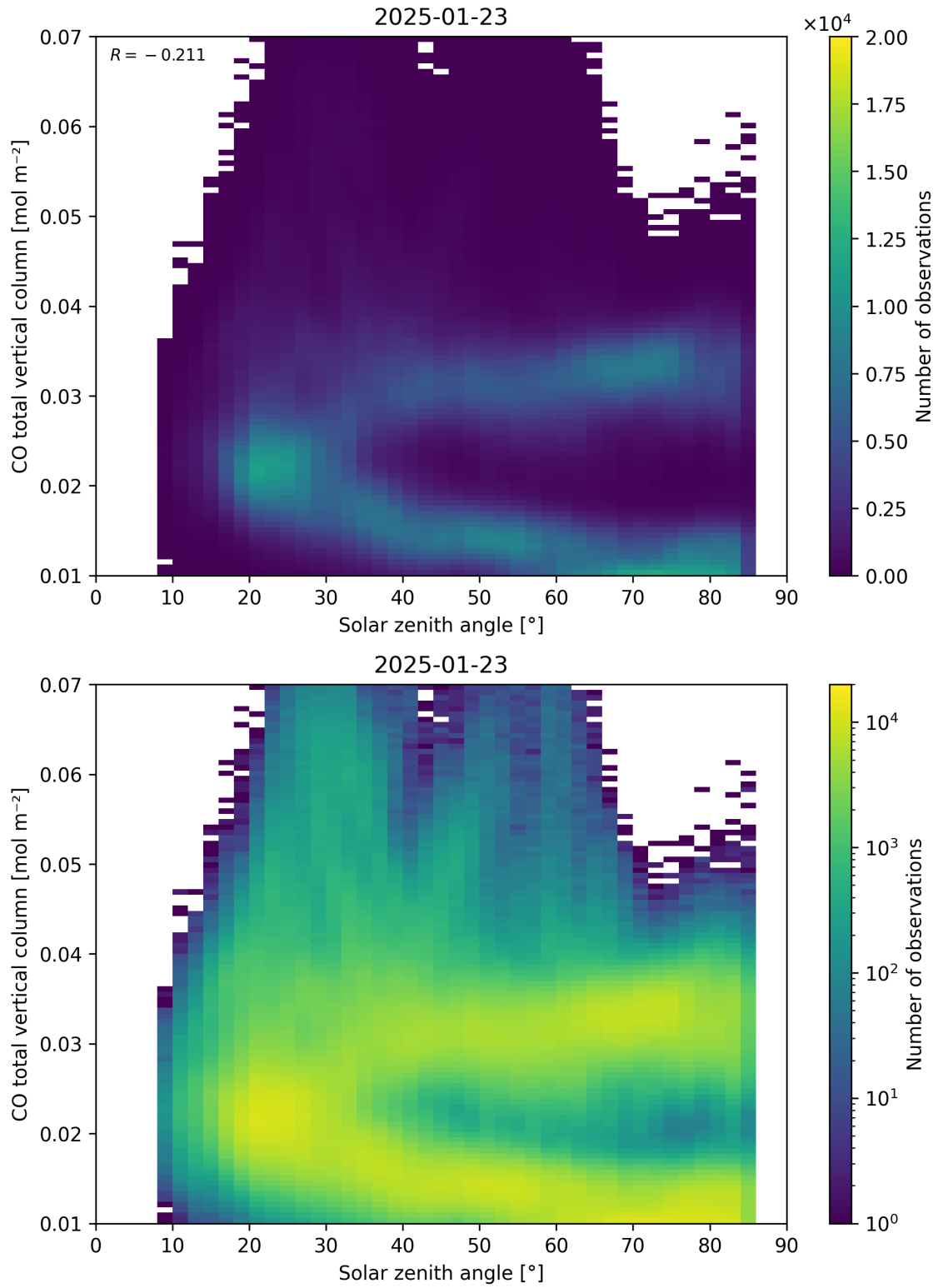
Figure 61: Scatter density plot of “Solar zenith angle” against “CO total vertical column” for 2025-01-23 to 2025-01-24.
