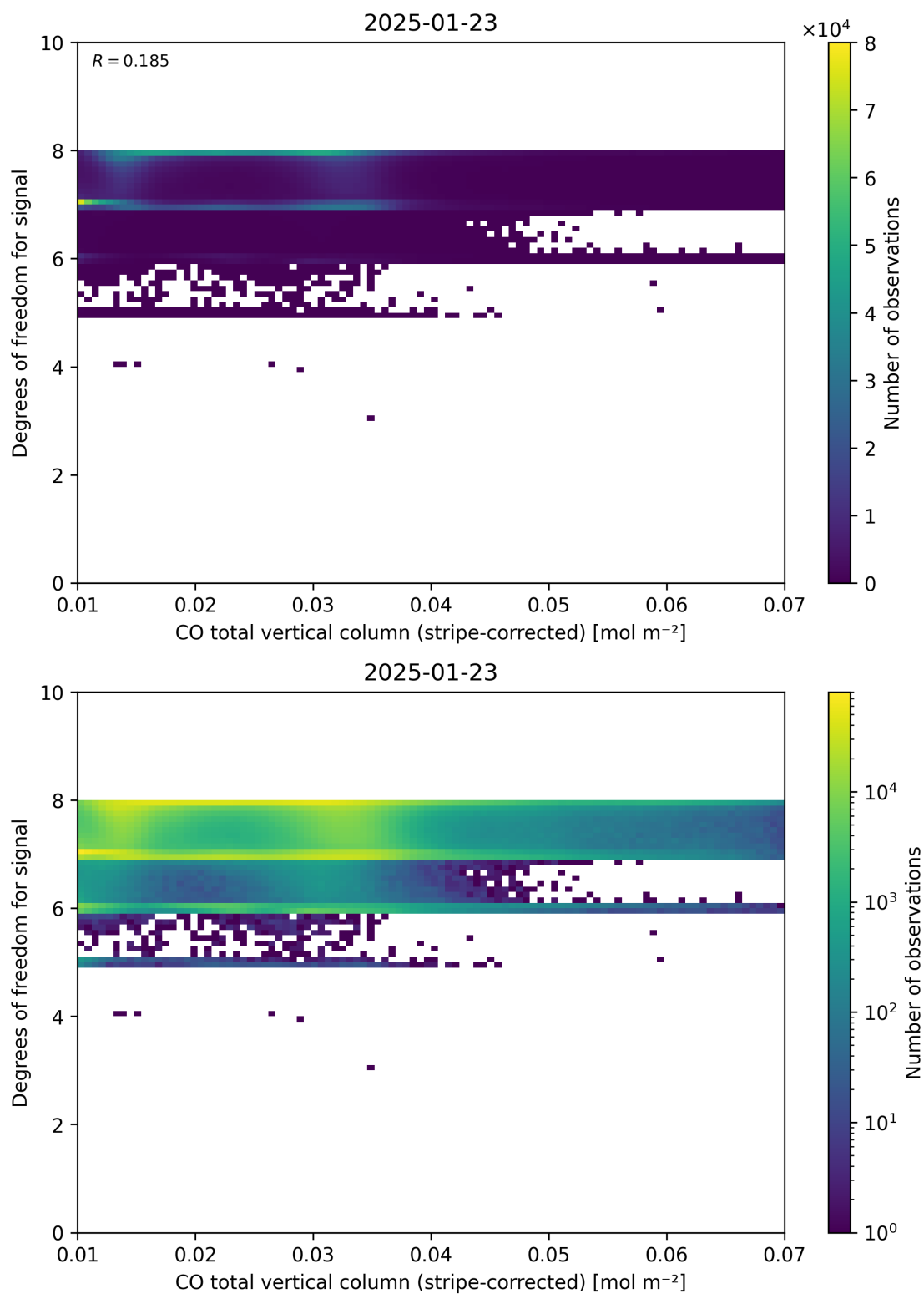
Figure 38: Scatter density plot of “CO total vertical column (stripe-corrected)” against “Degrees of freedom for signal” for 2025-01-23 to 2025-01-24.
