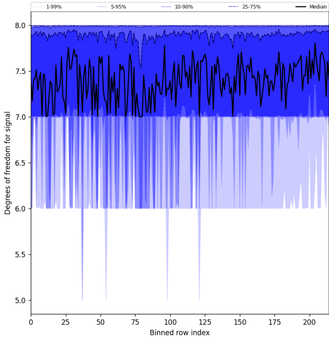
Figure 31: Along track statistics of “Degrees of freedom for signal” for 2025-01-23 to 2025-01-24
