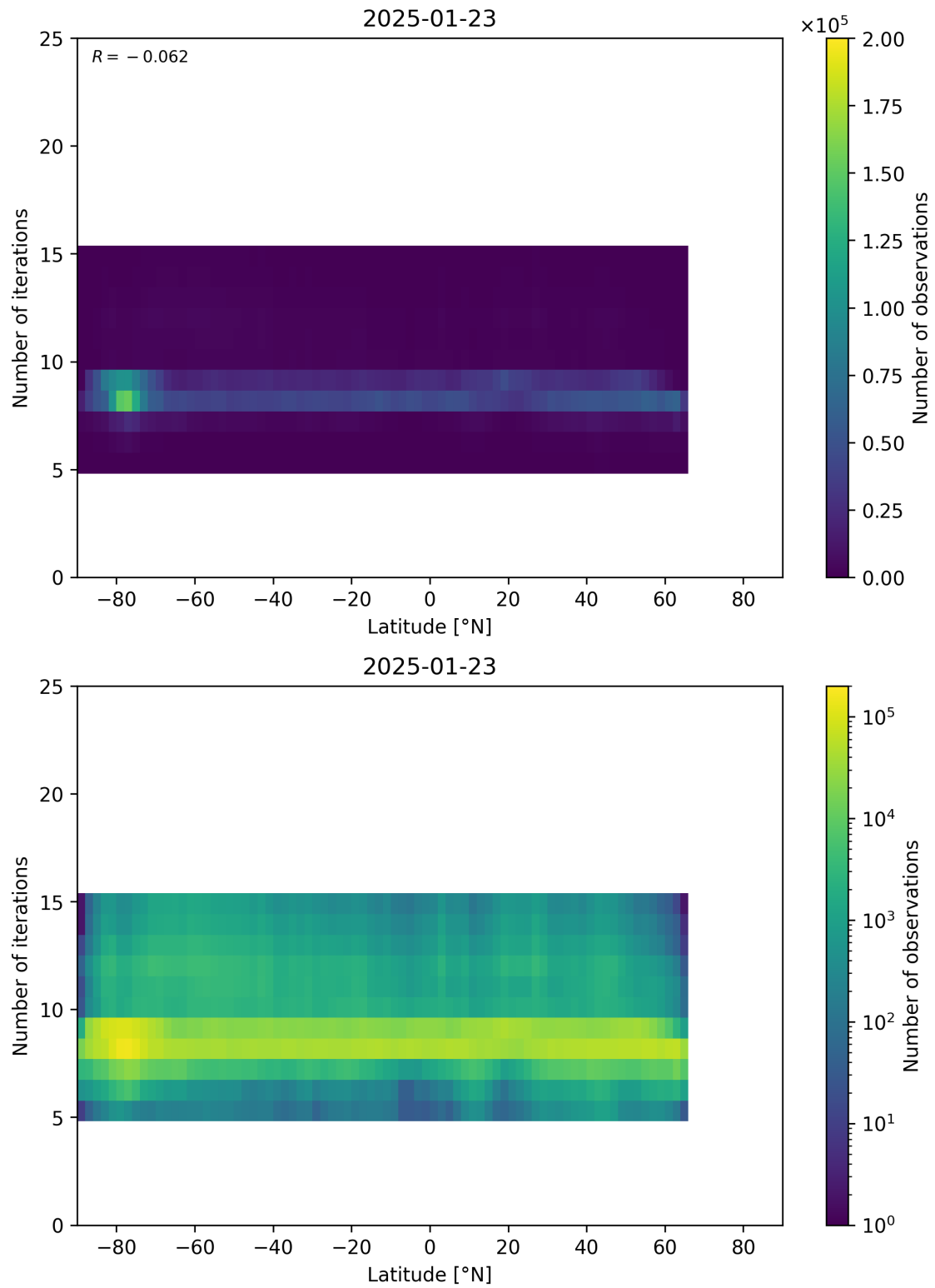
Figure 56: Scatter density plot of “Latitude” against “Number of iterations” for 2025-01-23 to 2025-01-24.
