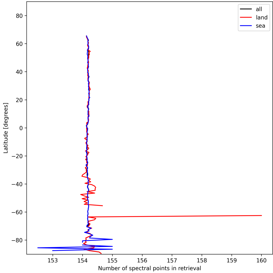
Figure 13: Zonal average of “Number of spectral points in retrieval” for 2025-01-23 to 2025-01-24.
