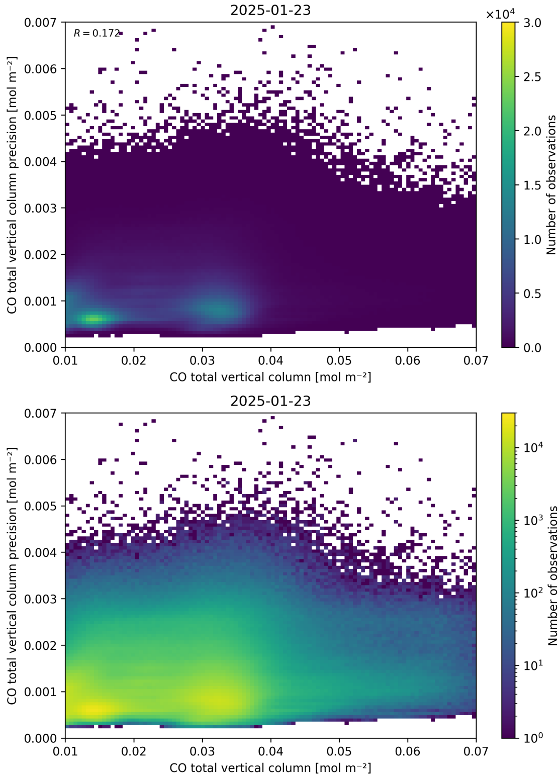
Figure 34: Scatter density plot of “CO total vertical column” against “CO total vertical column precision” for 2025-01-23 to 2025-01-24.
