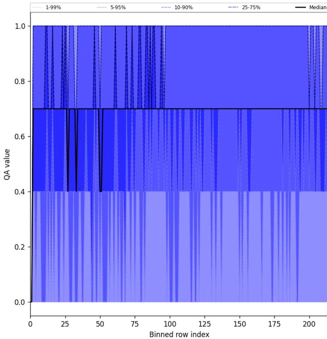
Figure 25: Along track statistics of “QA value” for 2025-01-23 to 2025-01-24
