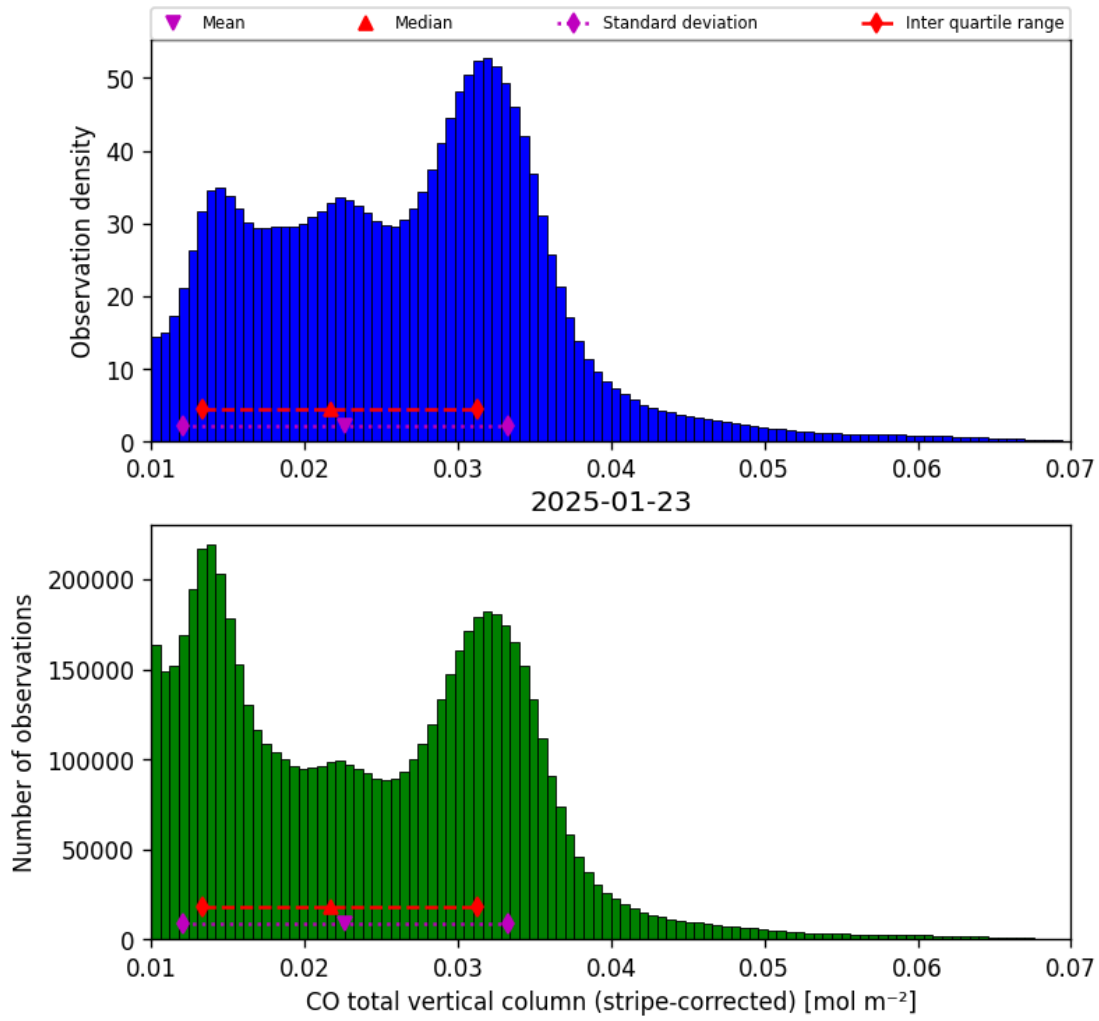
Figure 19: Histogram of “CO total vertical column (stripe-corrected)” for 2025-01-23 to 2025-01-24
