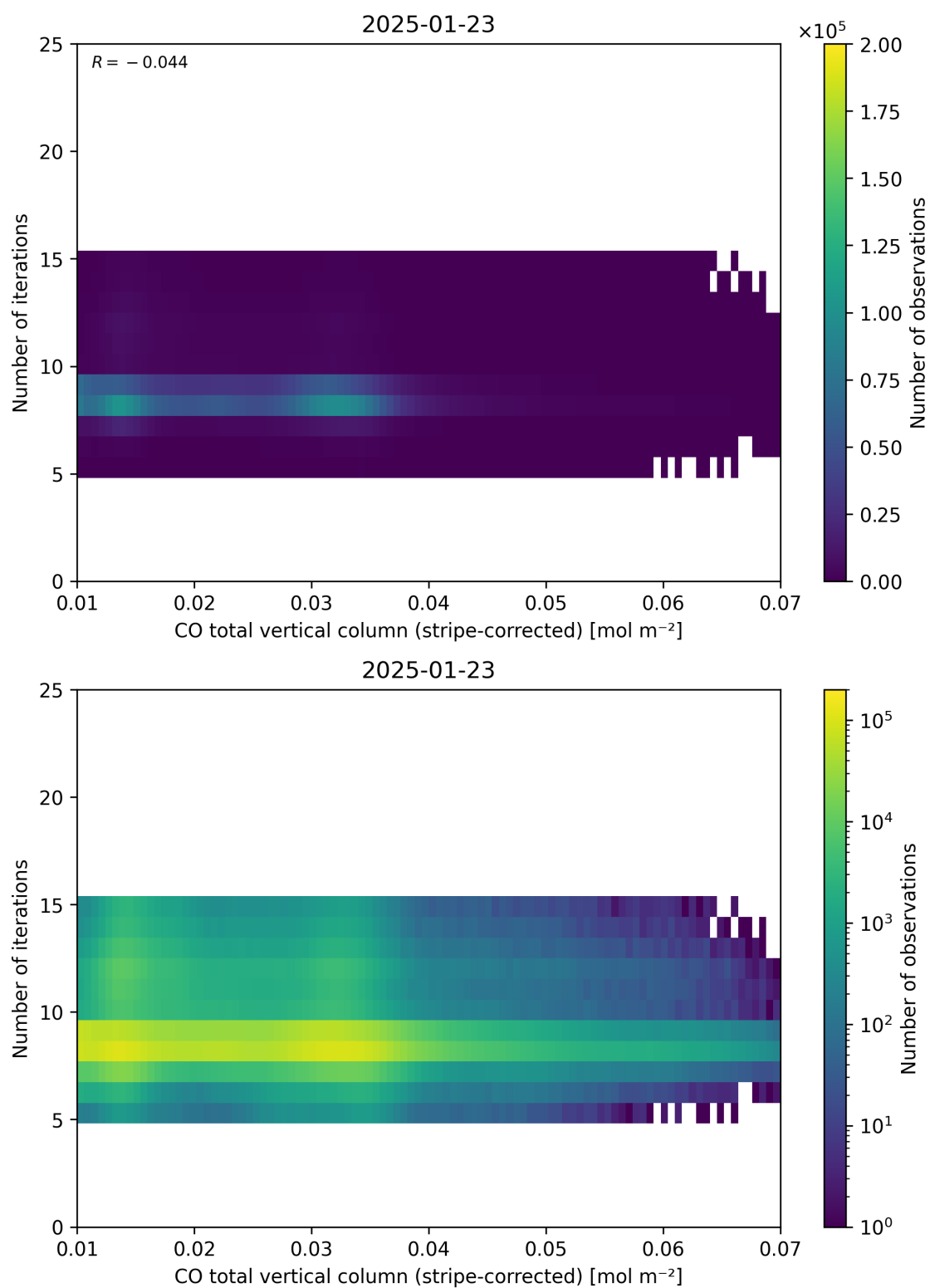
Figure 39: Scatter density plot of “CO total vertical column (stripe-corrected)” against “Number of iterations” for 2025-01-23 to 2025-01-24.
