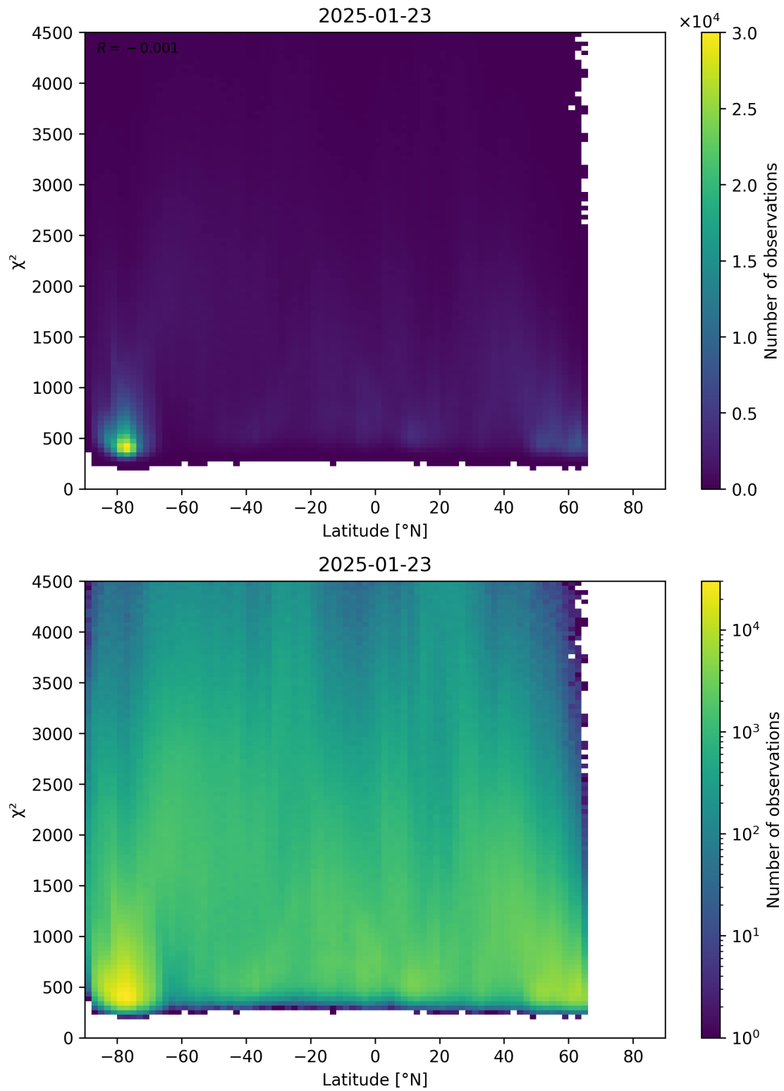
Figure 54: Scatter density plot of “Latitude” against “ \chi^2 ” for 2025-01-23 to 2025-01-24.
