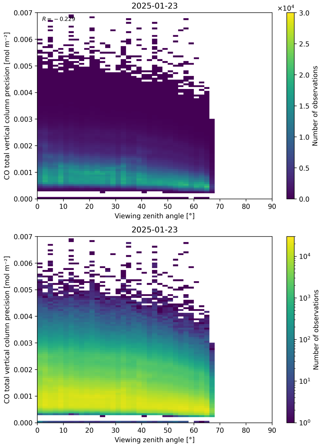
Figure 71: Scatter density plot of “Viewing zenith angle” against “CO total vertical column precision” for 2025-01-23 to 2025-01-24.
