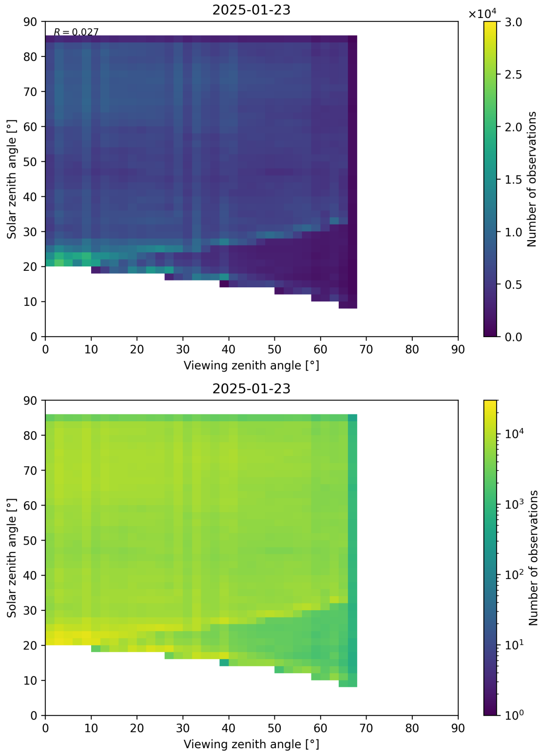
Figure 77: Scatter density plot of “Viewing zenith angle” against “Solar zenith angle” for 2025-01-23 to 2025-01-24.
