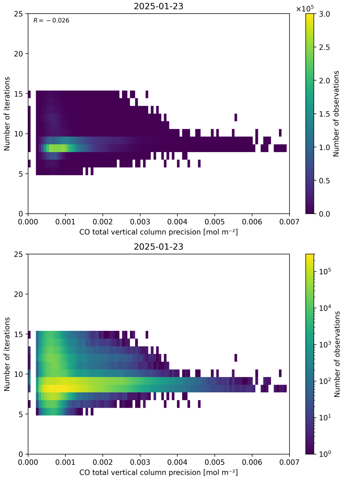
Figure 46: Scatter density plot of “CO total vertical column precision” against “Number of iterations” for 2025-01-23 to 2025-01-24.
