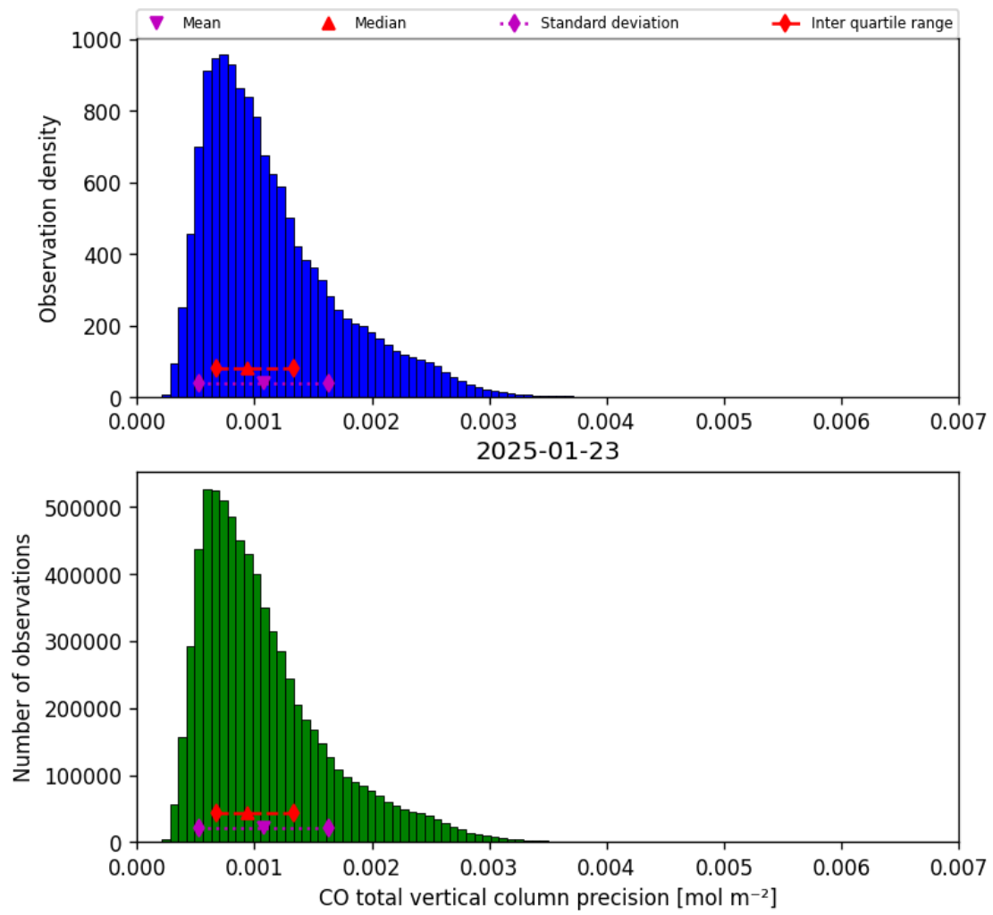
Figure 20: Histogram of “CO total vertical column precision” for 2025-01-23 to 2025-01-24
