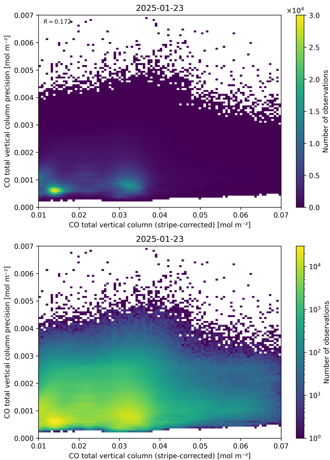
Figure 36: Scatter density plot of “CO total vertical column (stripe-corrected)” against “CO total vertical column precision” for 2025-01-23 to 2025-01-24.
