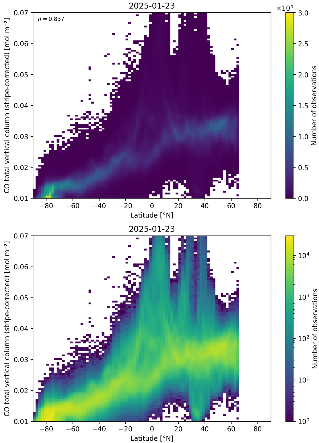
Figure 52: Scatter density plot of “Latitude” against “CO total vertical column (stripe-corrected)” for 2025-01-23 to 2025-01-24.
