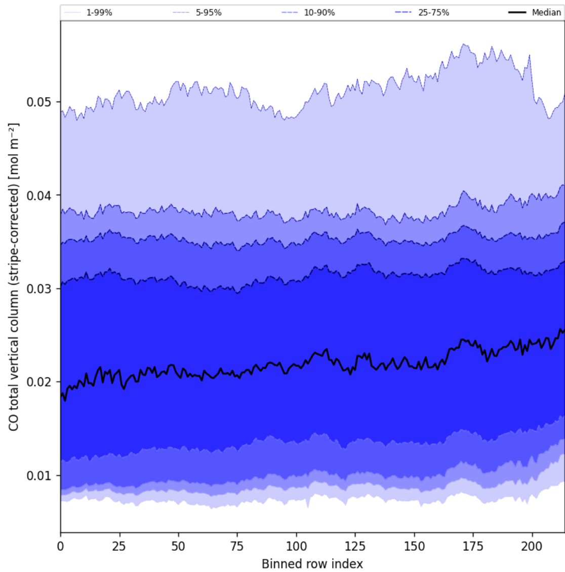
Figure 27: Along track statistics of “CO total vertical column (stripe-corrected)” for 2025-01-23 to 2025-01-24
