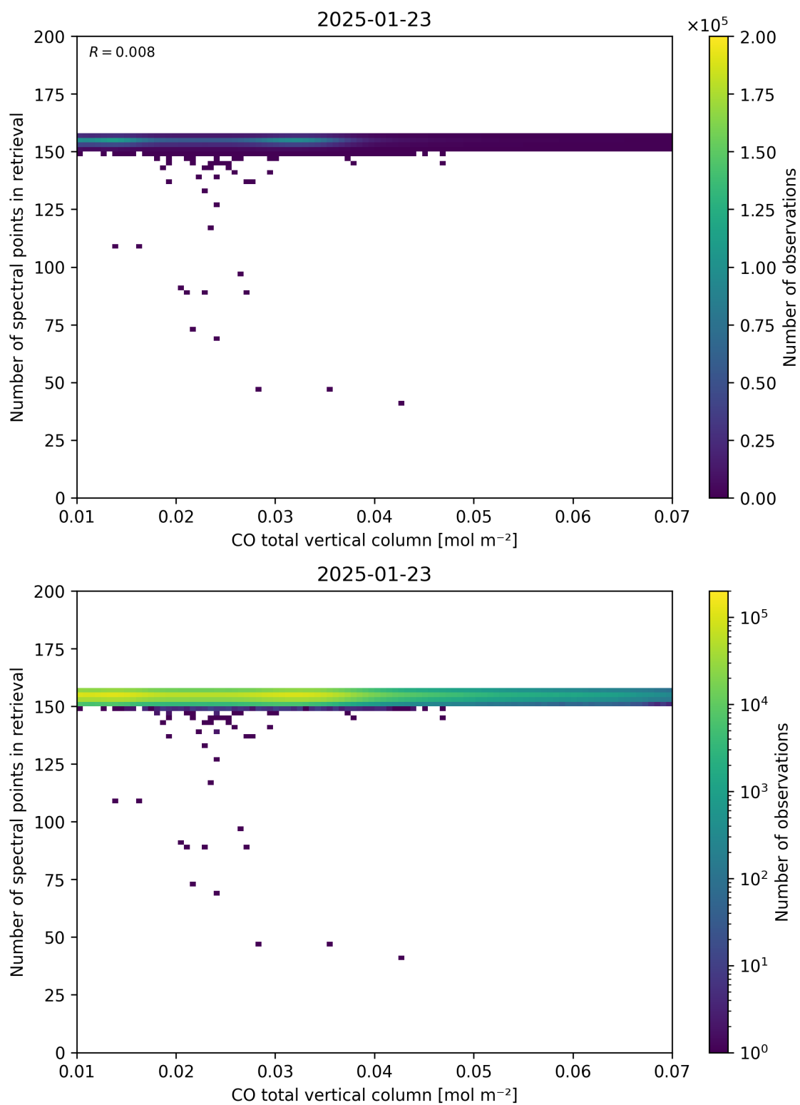
Figure 43: Scatter density plot of “CO total vertical column” against “Number of spectral points in retrieval” for 2025-01-23 to 2025-01-24.
