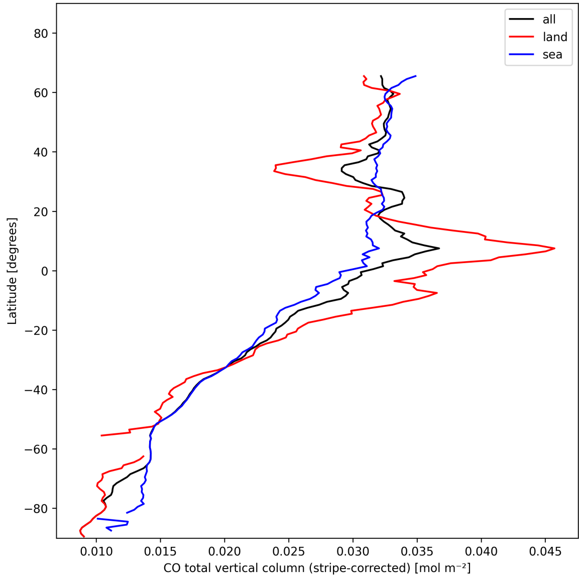
Figure 11: Zonal average of “CO total vertical column (stripe-corrected)” for 2025-01-23 to 2025-01-24.
