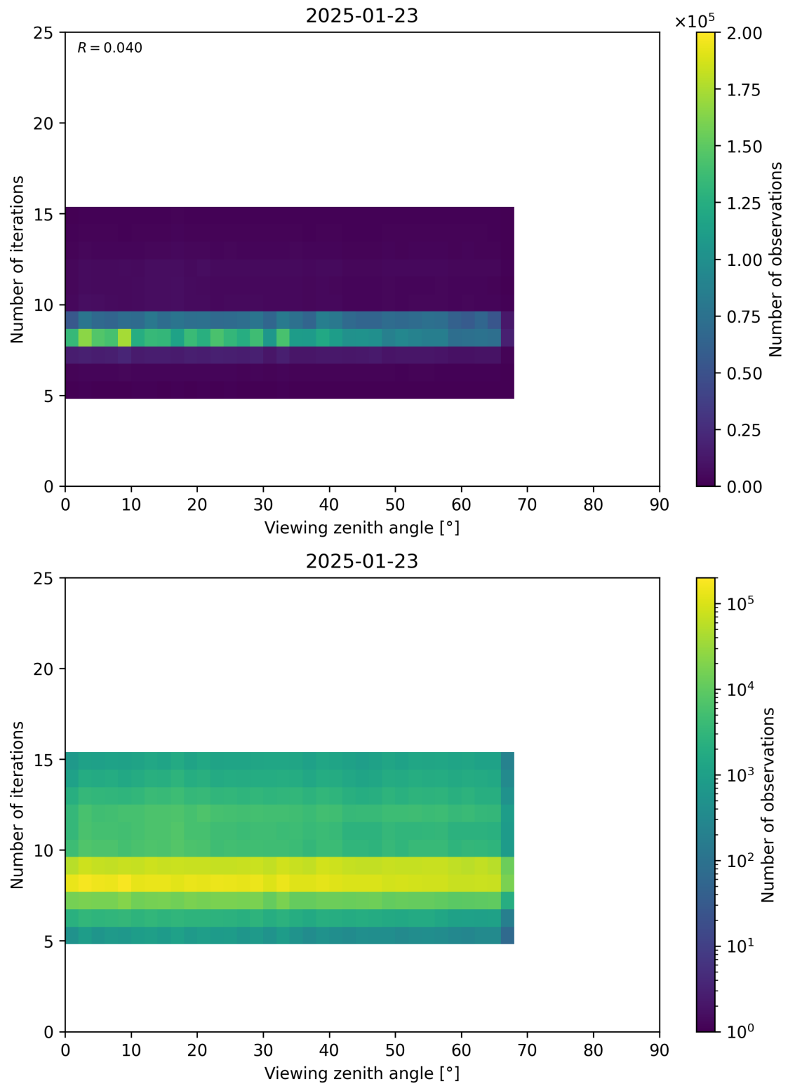
Figure 75: Scatter density plot of “Viewing zenith angle” against “Number of iterations” for 2025-01-23 to 2025-01-24.
