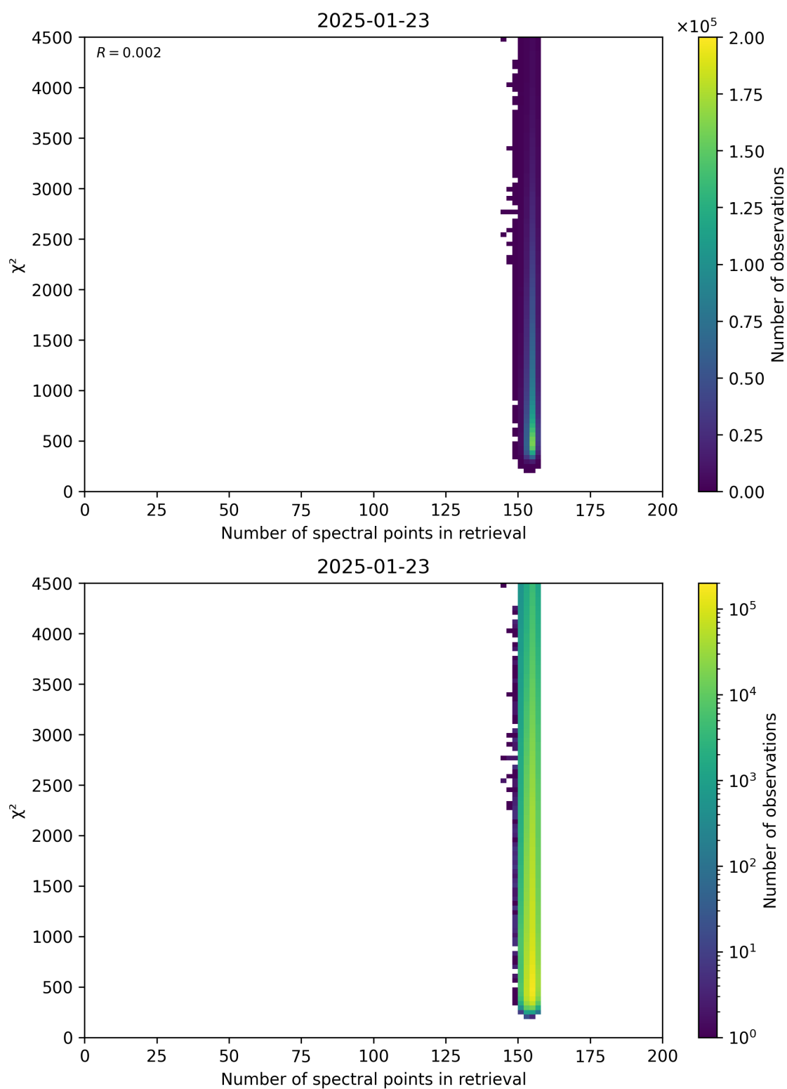
Figure 58: Scatter density plot of “Number of spectral points in retrieval” against “ \chi^2 ” for 2025-01-23 to 2025-01-24.
