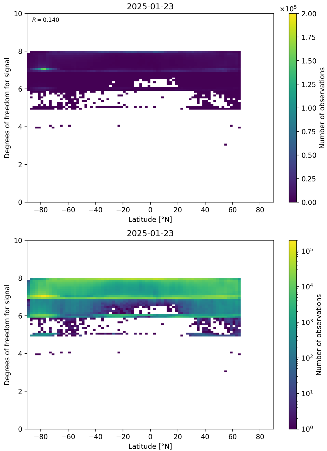
Figure 55: Scatter density plot of “Latitude” against “Degrees of freedom for signal” for 2025-01-23 to 2025-01-24.
