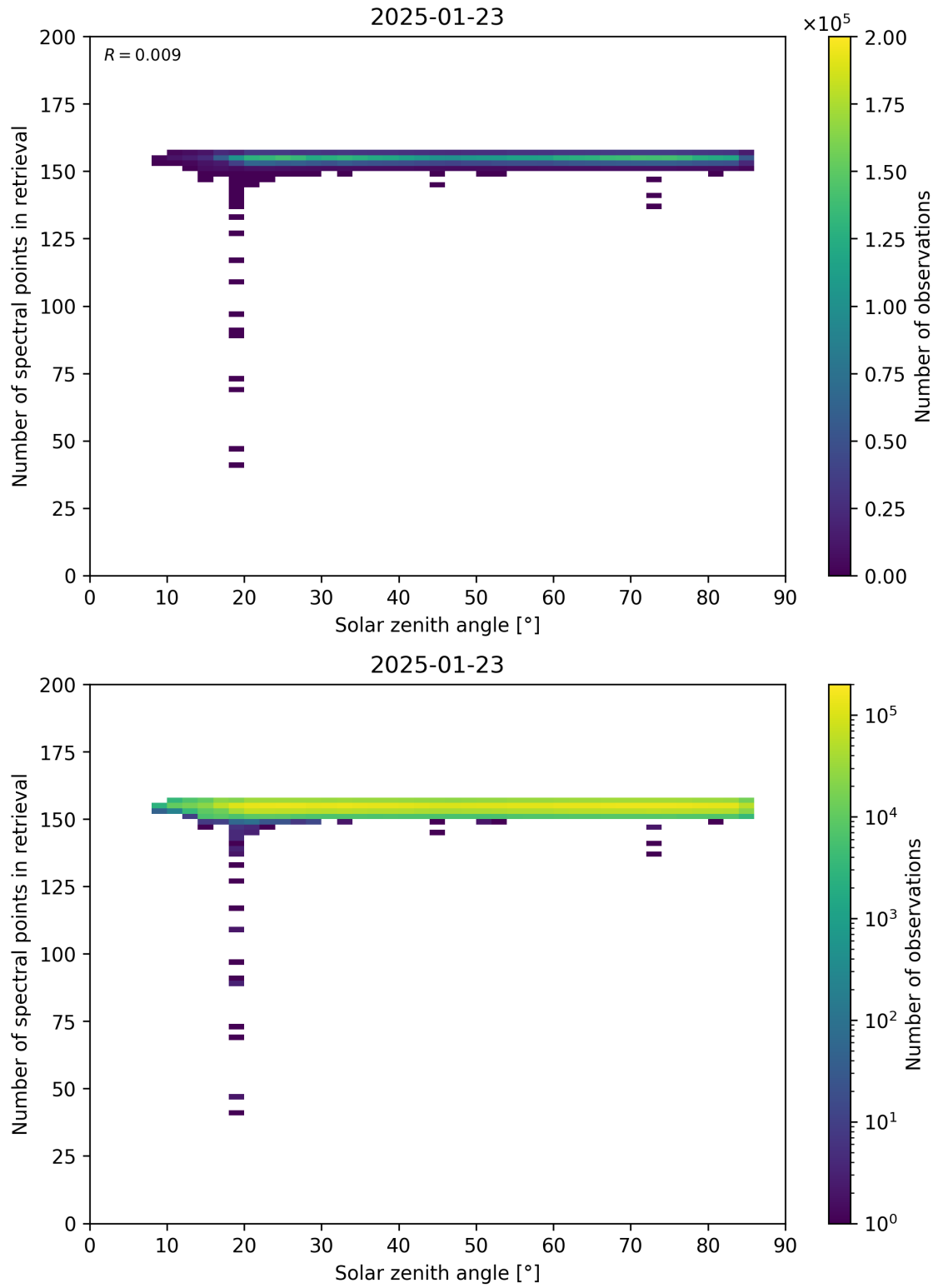
Figure 68: Scatter density plot of “Solar zenith angle” against “Number of spectral points in retrieval” for 2025-01-23 to 2025-01-24.
