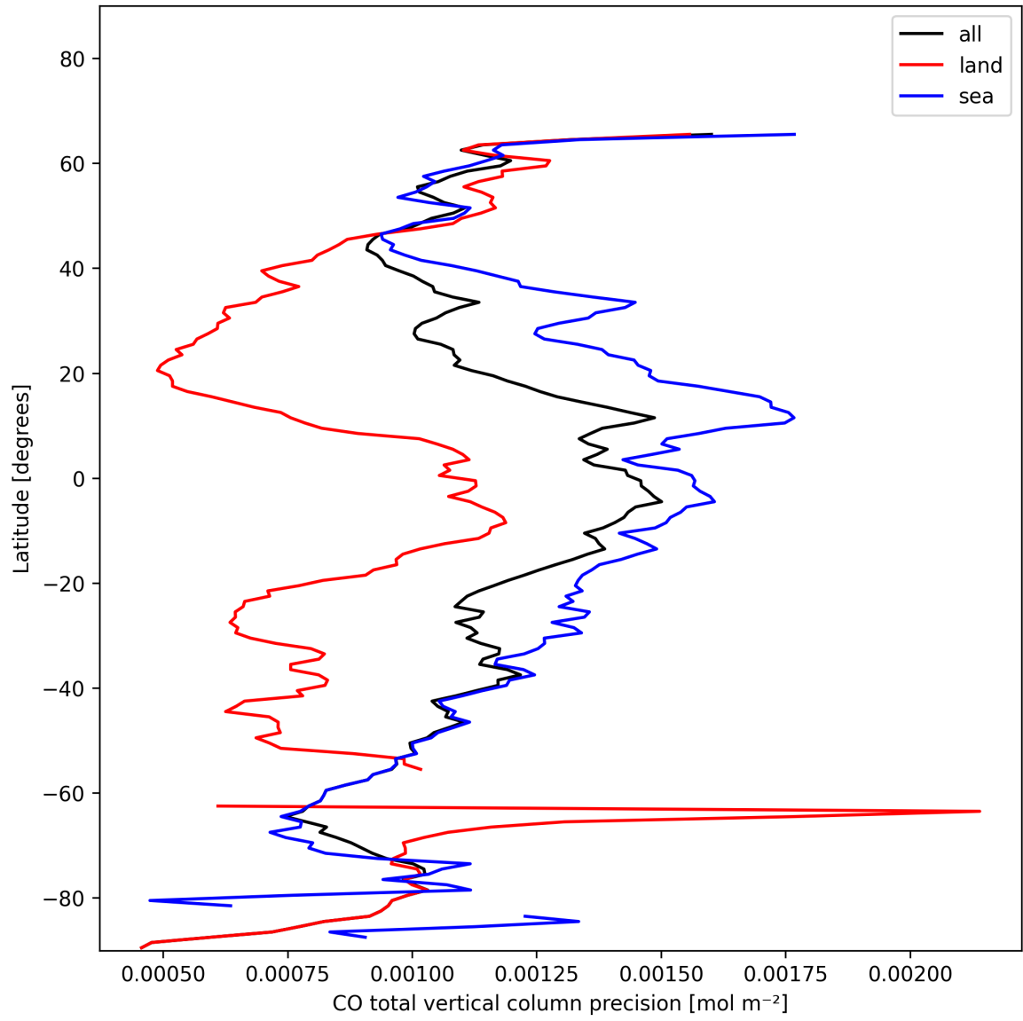
Figure 12: Zonal average of “CO total vertical column precision” for 2025-01-23 to 2025-01-24.
