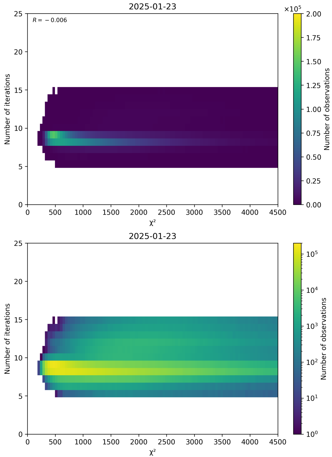
Figure 49: Scatter density plot of “ \chi^2 ” against “Number of iterations” for 2025-01-23 to 2025-01-24.
