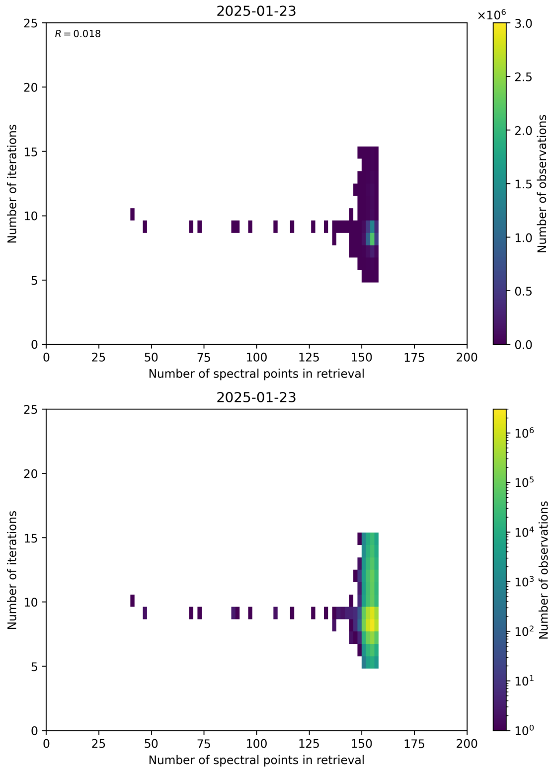
Figure 60: Scatter density plot of “Number of spectral points in retrieval” against “Number of iterations” for 2025-01-23 to 2025-01-24.
