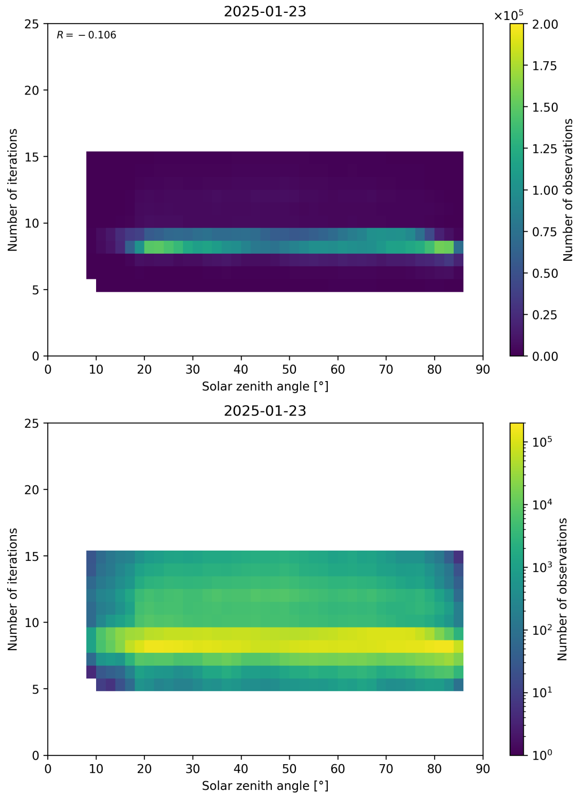
Figure 67: Scatter density plot of “Solar zenith angle” against “Number of iterations” for 2025-01-23 to 2025-01-24.
