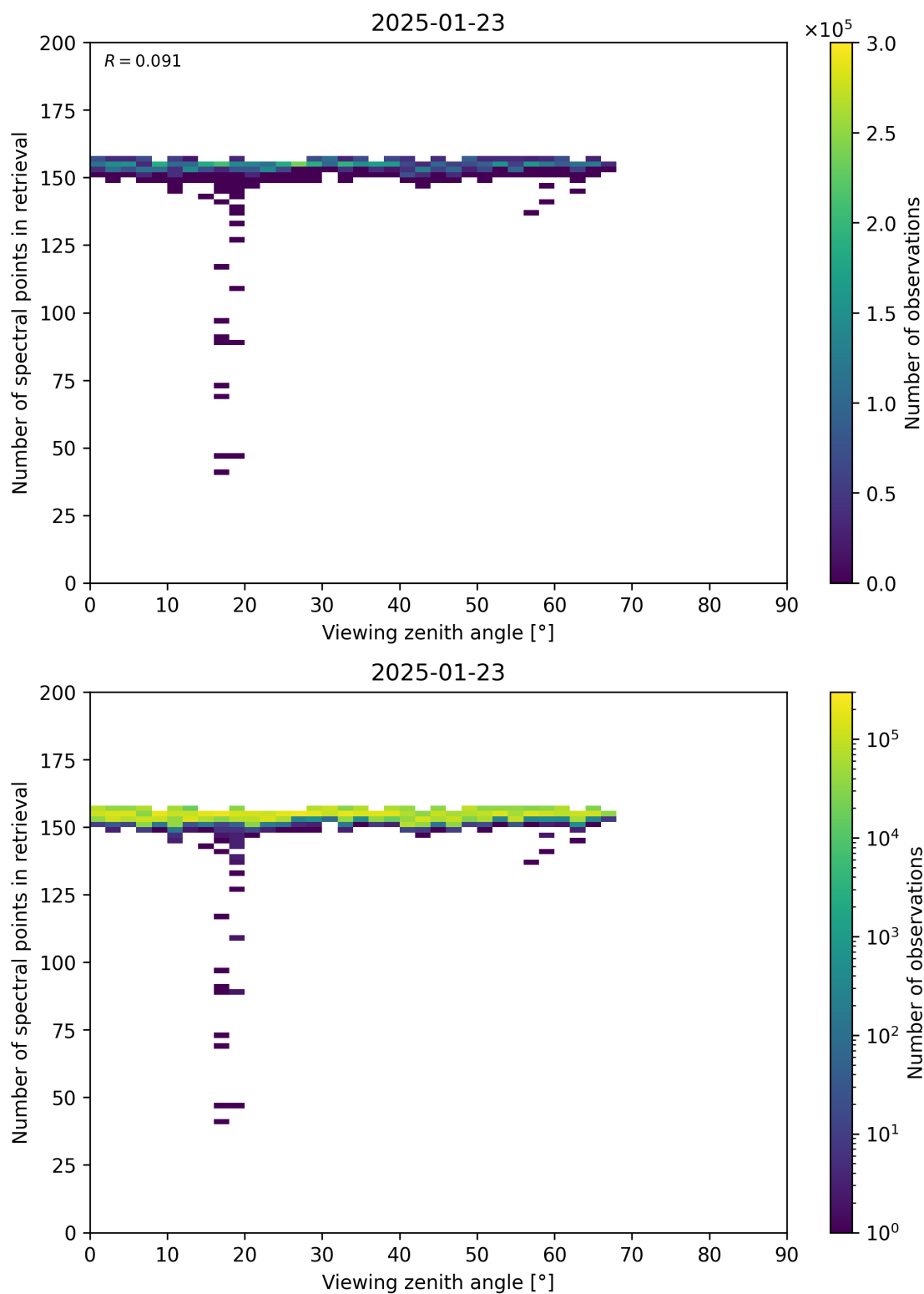
Figure 76: Scatter density plot of “Viewing zenith angle” against “Number of spectral points in retrieval” for 2025-01-23 to 2025-01-24.
