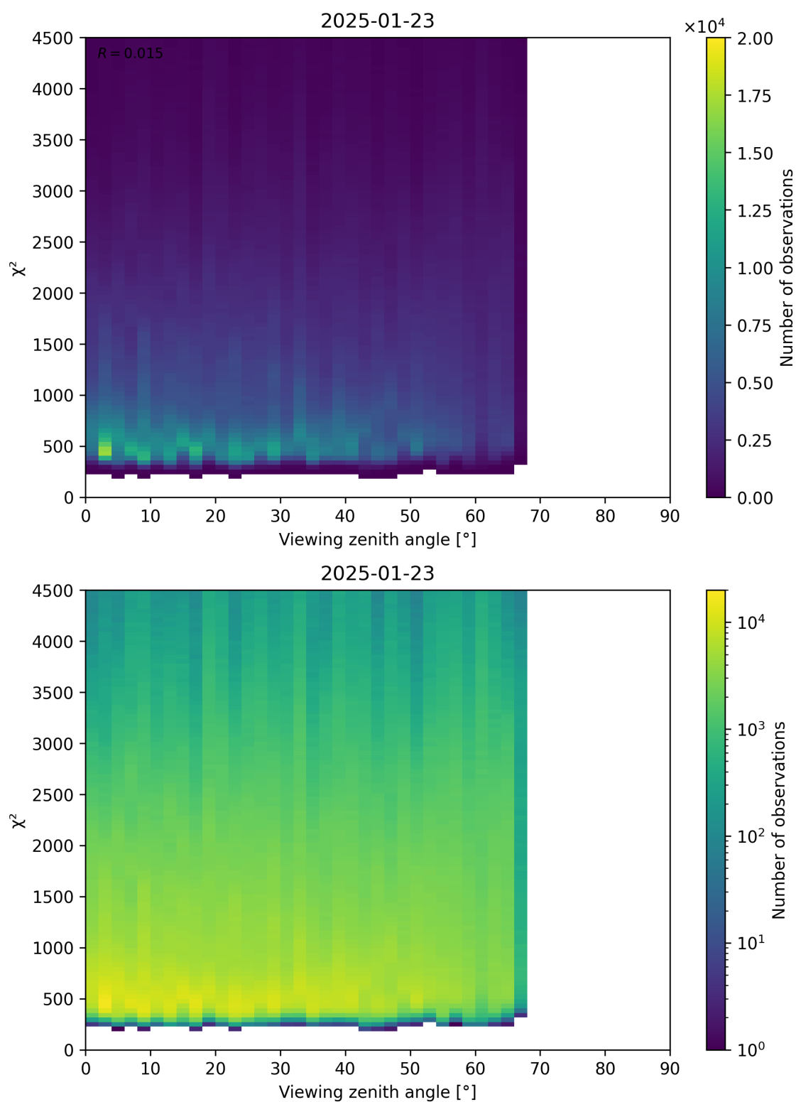
Figure 72: Scatter density plot of “Viewing zenith angle” against “ \chi^2 ” for 2025-01-23 to 2025-01-24.
