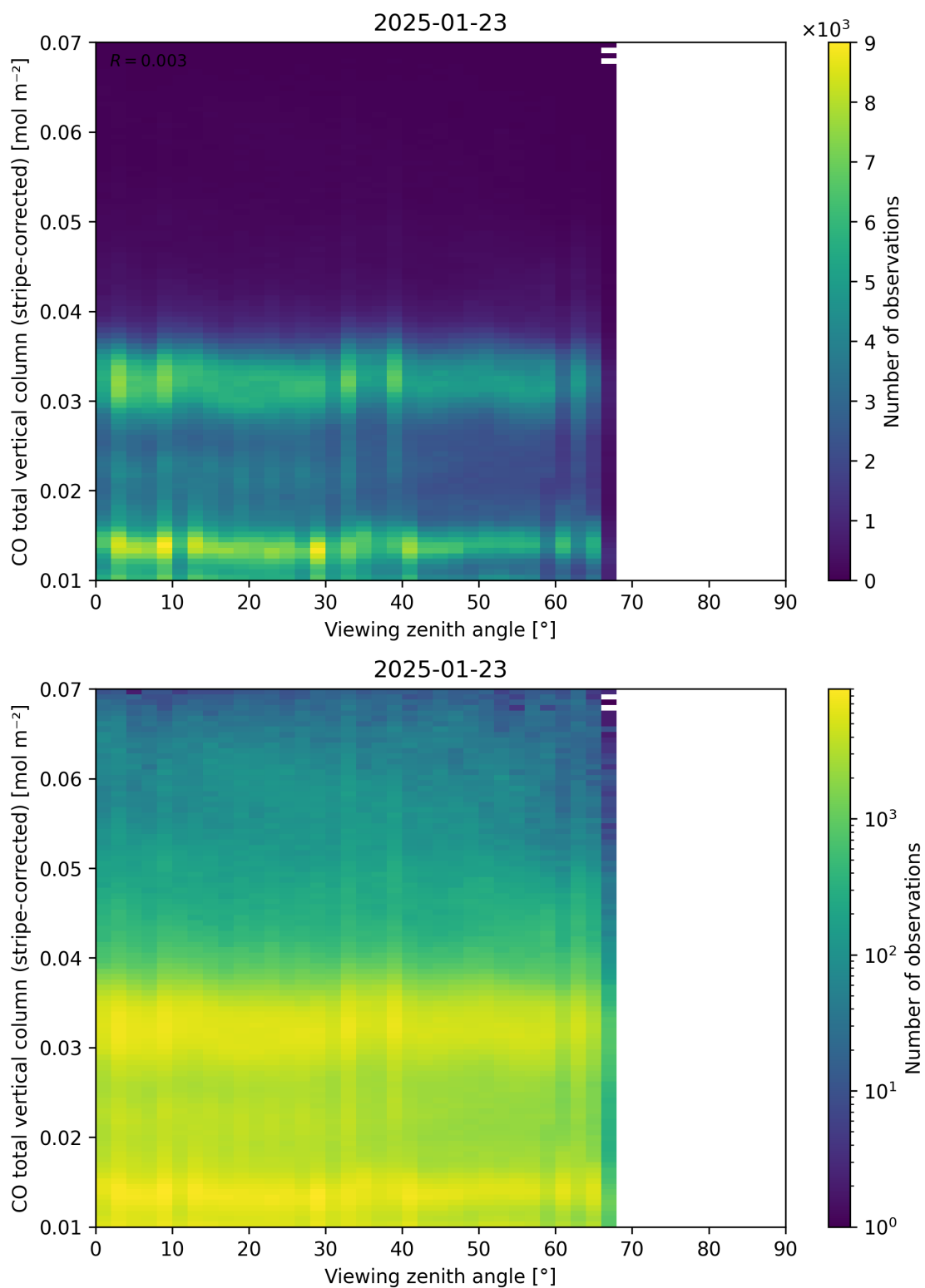
Figure 70: Scatter density plot of “Viewing zenith angle” against “CO total vertical column (stripe-corrected)” for 2025-01-23 to 2025-01-24.
