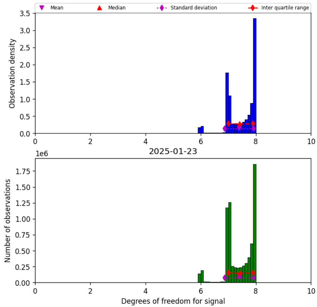
Figure 23: Histogram of “Degrees of freedom for signal” for 2025-01-23 to 2025-01-24
