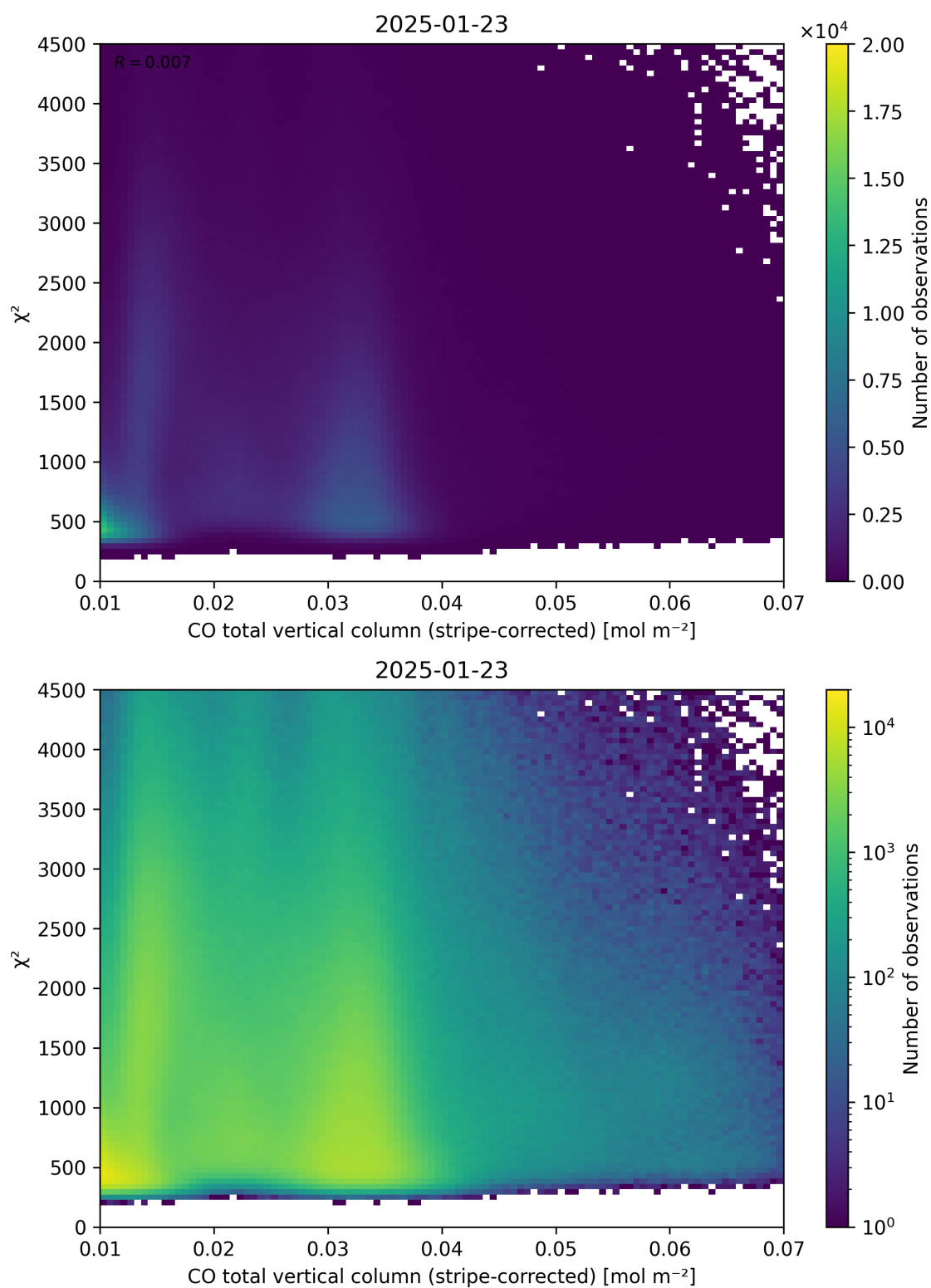
Figure 37: Scatter density plot of “CO total vertical column (stripe-corrected)” against “ \chi^2 ” for 2025-01-23 to 2025-01-24.
