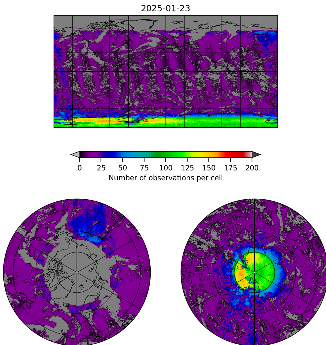
Figure 8: Map of the number of observations for 2025-01-23 to 2025-01-24
