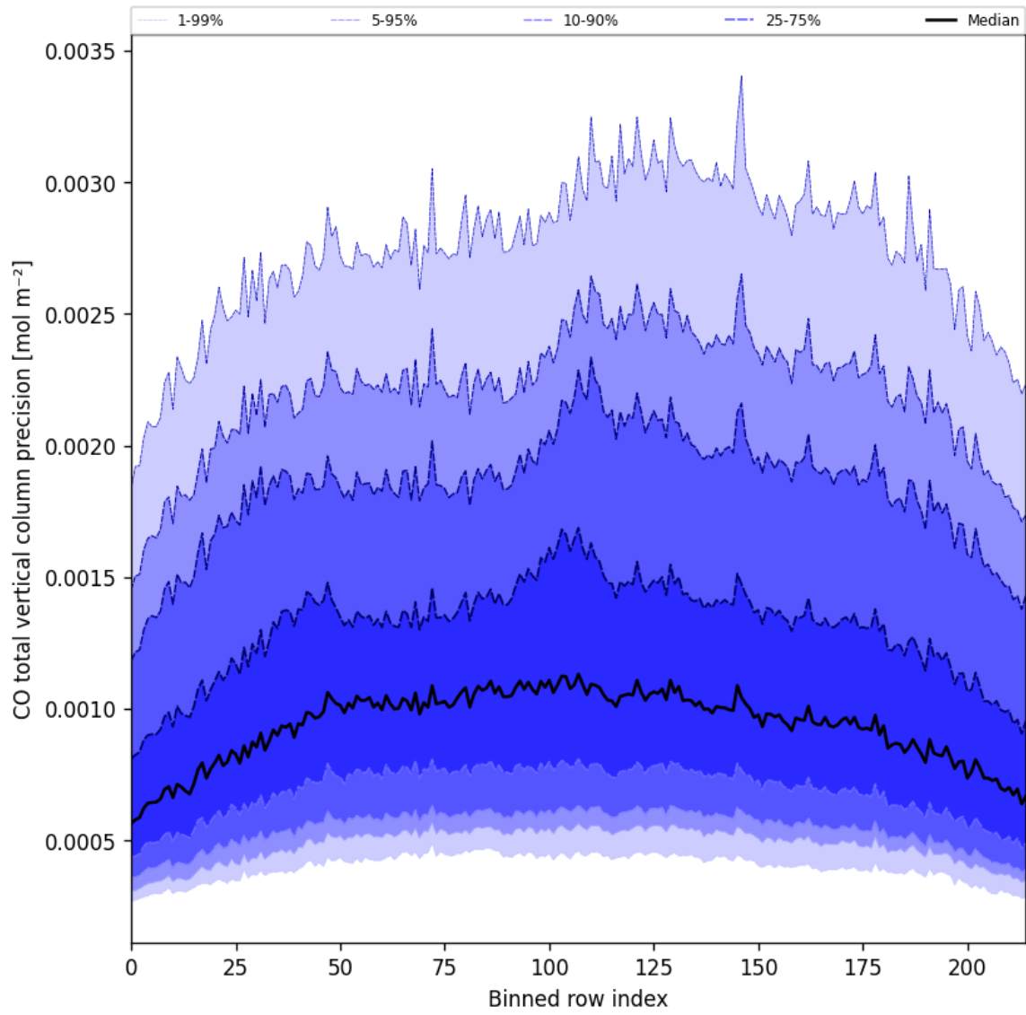
Figure 28: Along track statistics of “CO total vertical column precision” for 2025-01-23 to 2025-01-24
