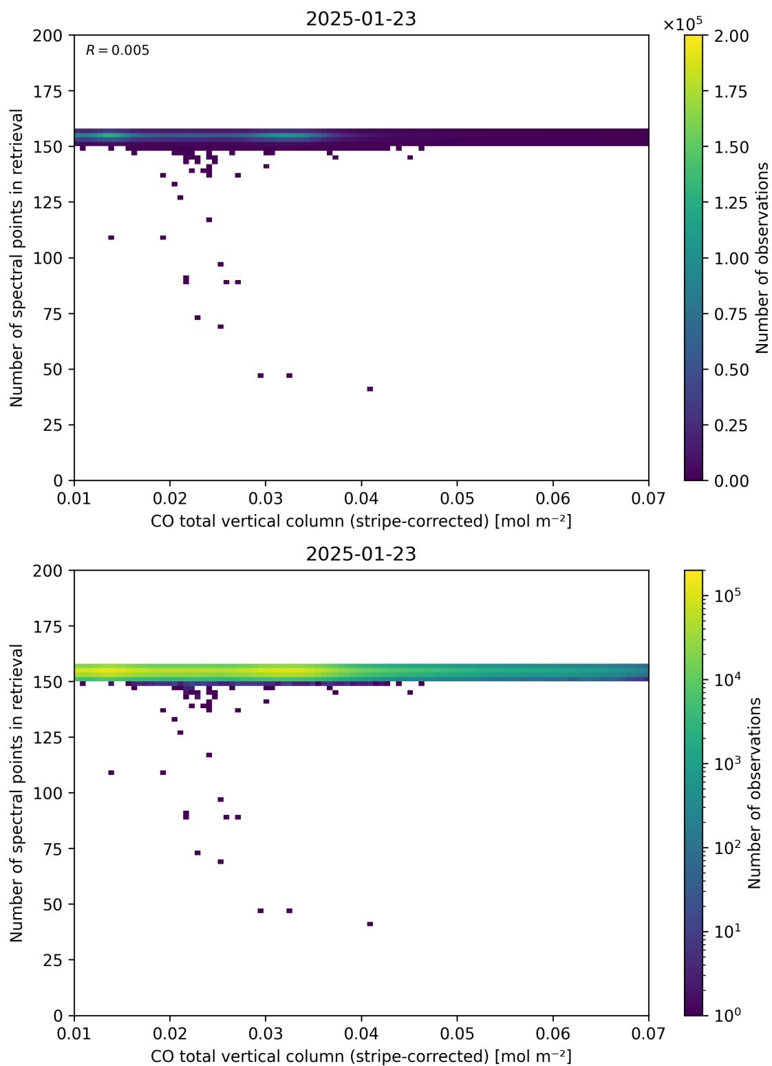
Figure 40: Scatter density plot of “CO total vertical column (stripe-corrected)” against “Number of spectral points in retrieval” for 2025-01-23 to 2025-01-24.
