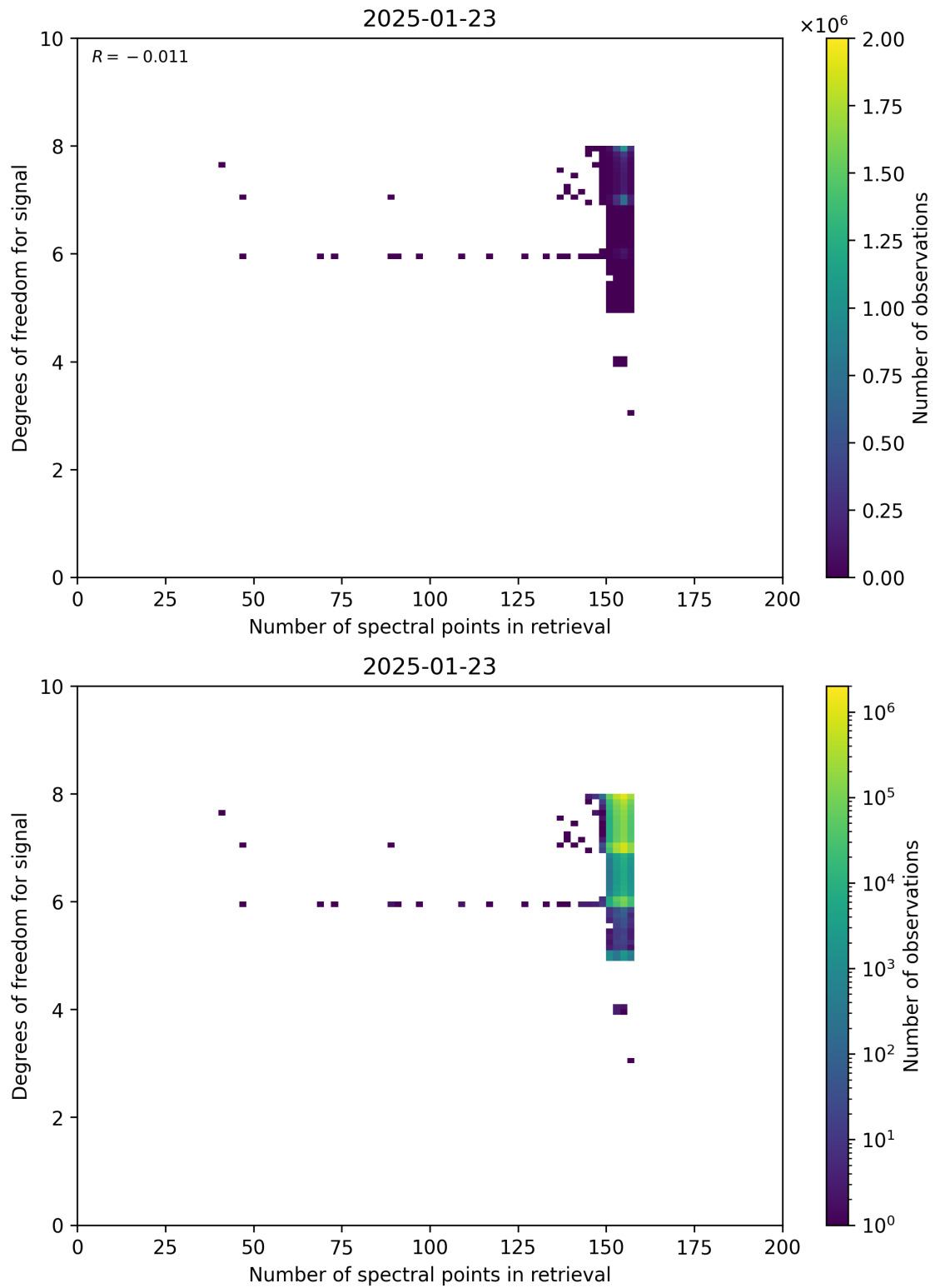
Figure 59: Scatter density plot of “Number of spectral points in retrieval” against “Degrees of freedom for signal” for 2025-01-23 to 2025-01-24.
