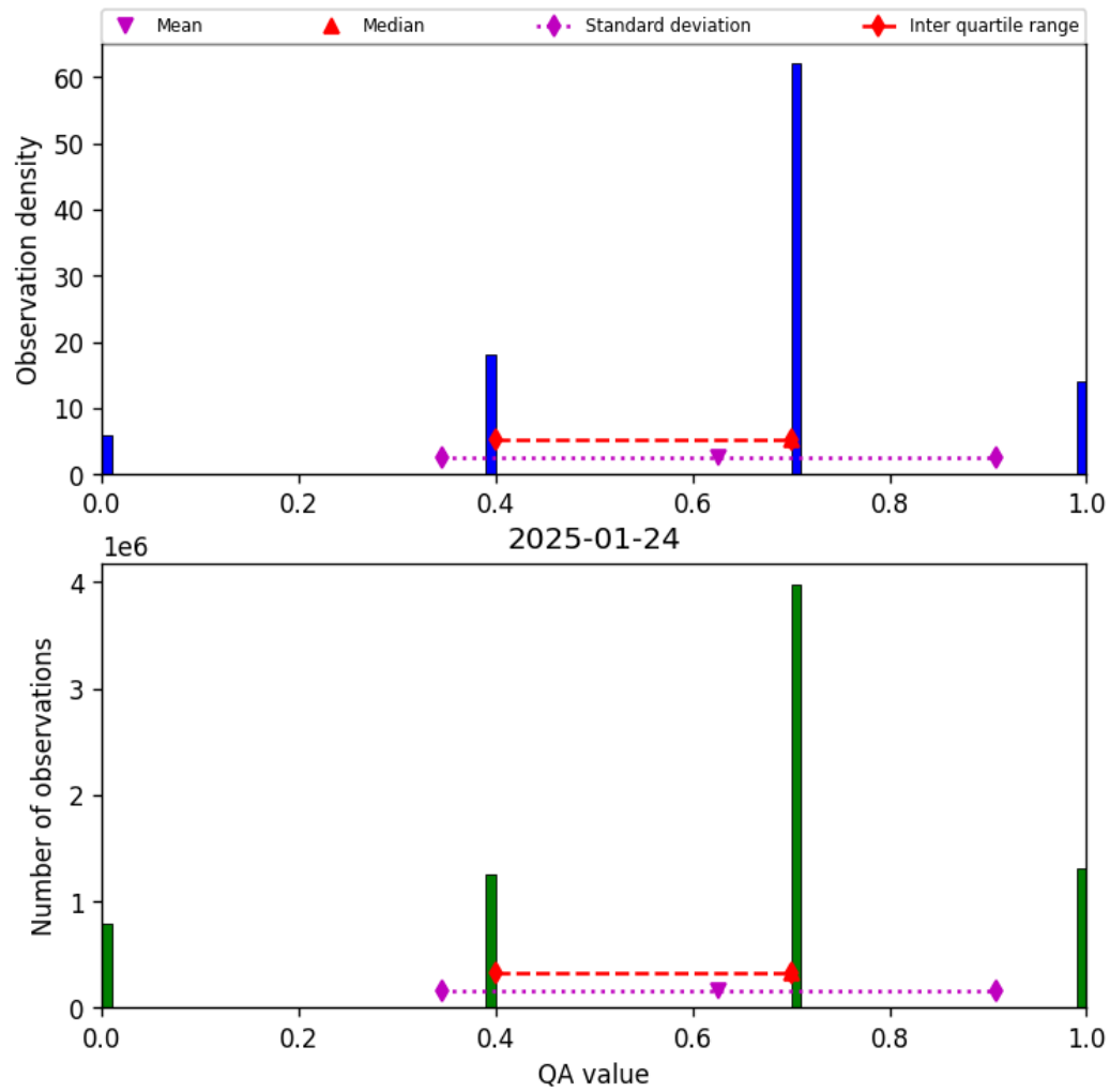
Figure 17: Histogram of “QA value” for 2025-01-23 to 2025-01-25
