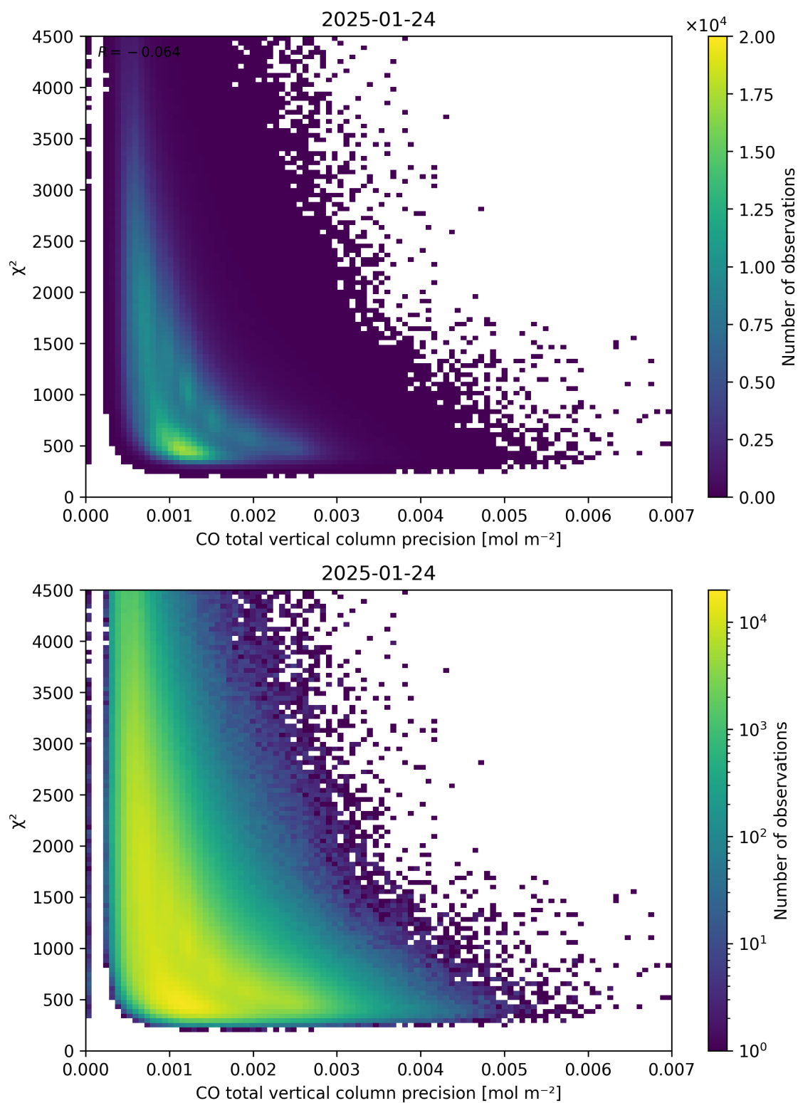
Figure 44: Scatter density plot of “CO total vertical column precision” against “ \chi^2 ” for 2025-01-23 to 2025-01-25.
