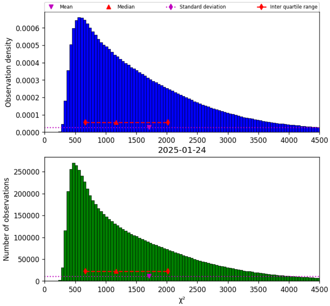
Figure 22: Histogram of “ \chi^2 ” for 2025-01-23 to 2025-01-25
