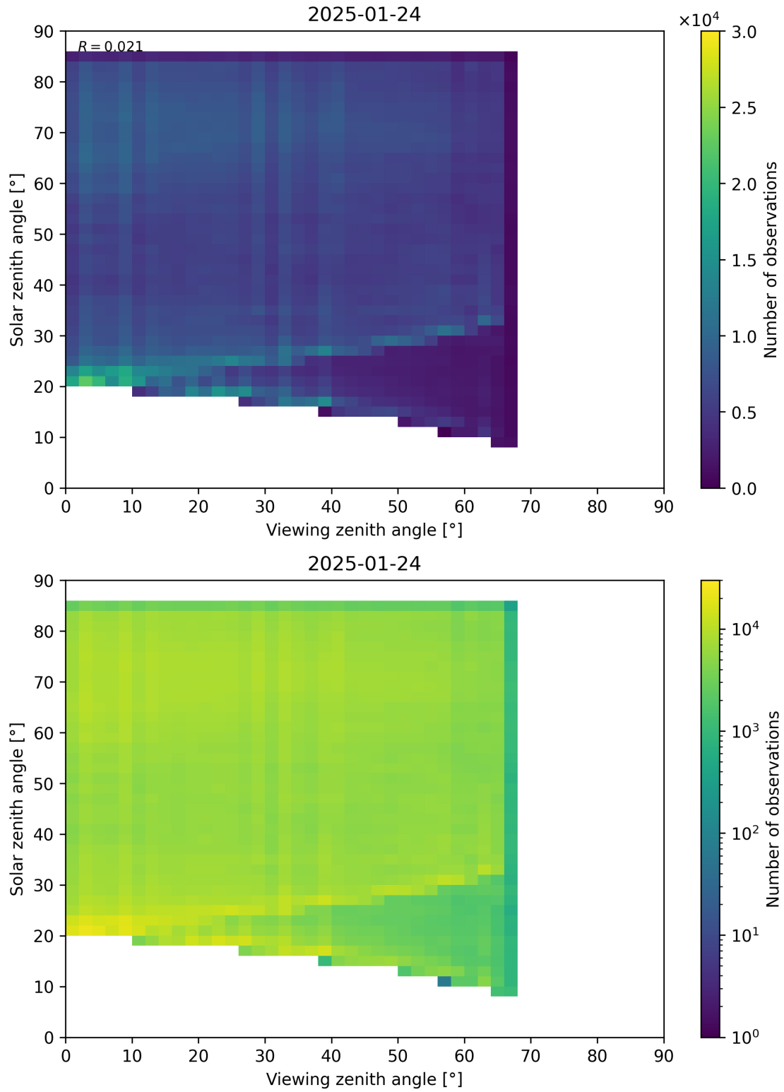
Figure 77: Scatter density plot of “Viewing zenith angle” against “Solar zenith angle” for 2025-01-23 to 2025-01-25.
