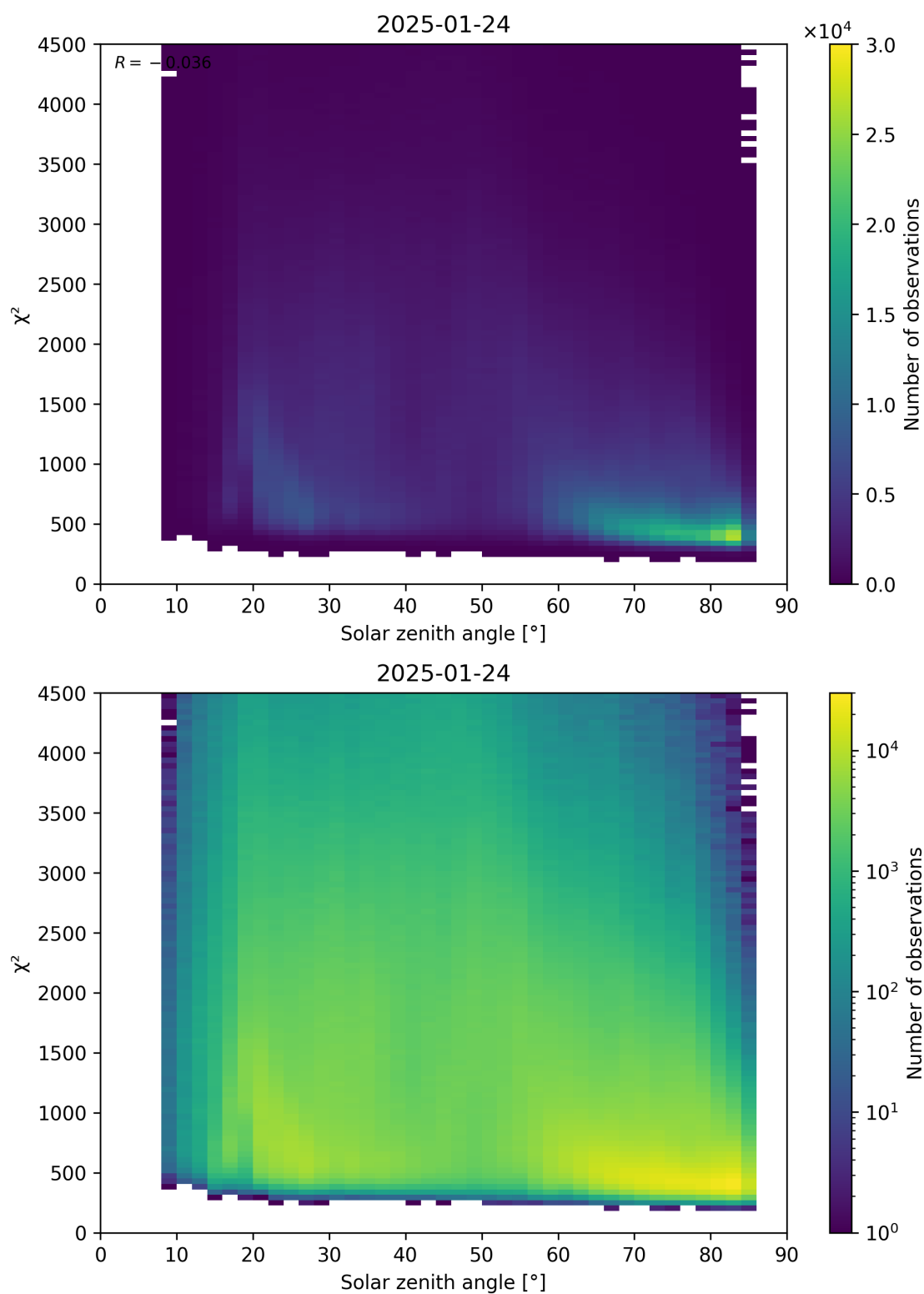
Figure 64: Scatter density plot of “Solar zenith angle” against “ \chi^2 ” for 2025-01-23 to 2025-01-25.
