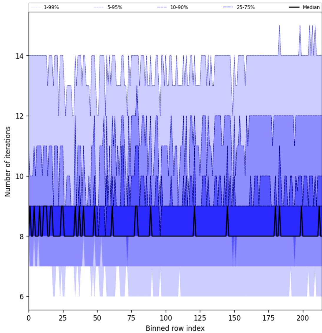
Figure 32: Along track statistics of “Number of iterations” for 2025-01-23 to 2025-01-25
