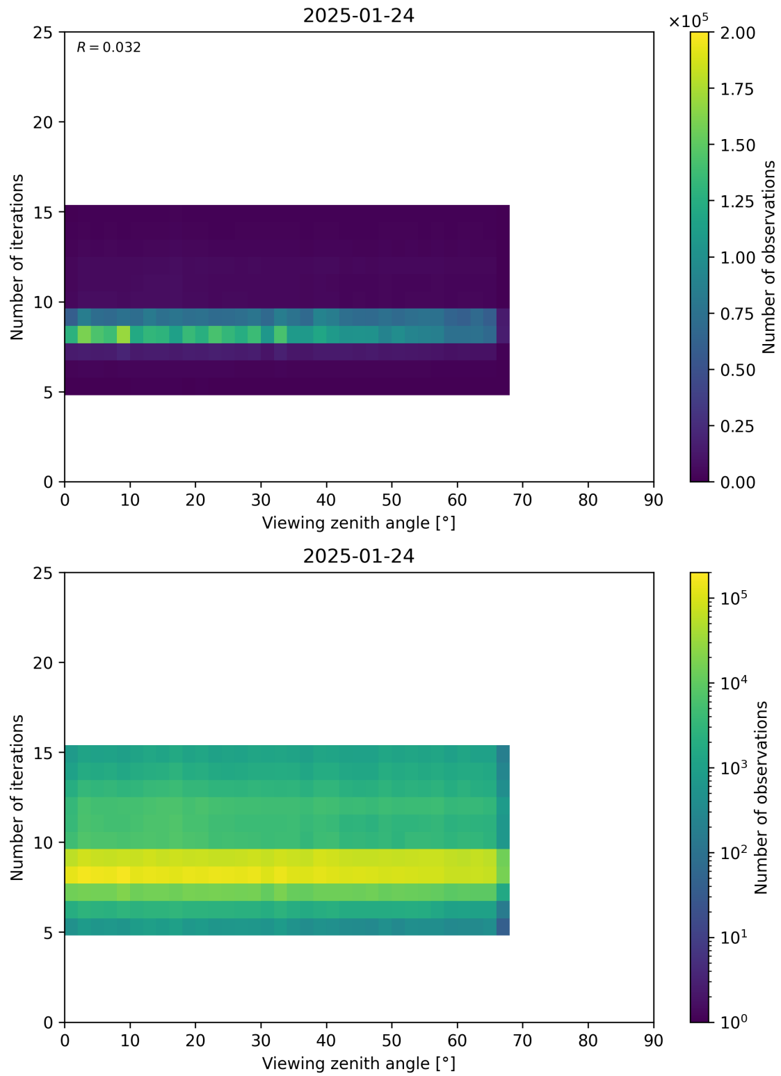
Figure 75: Scatter density plot of “Viewing zenith angle” against “Number of iterations” for 2025-01-23 to 2025-01-25.
