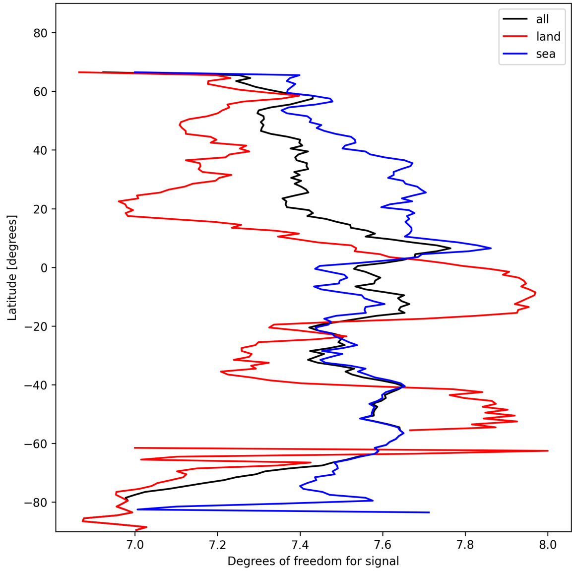
Figure 15: Zonal average of “Degrees of freedom for signal” for 2025-01-23 to 2025-01-25.
