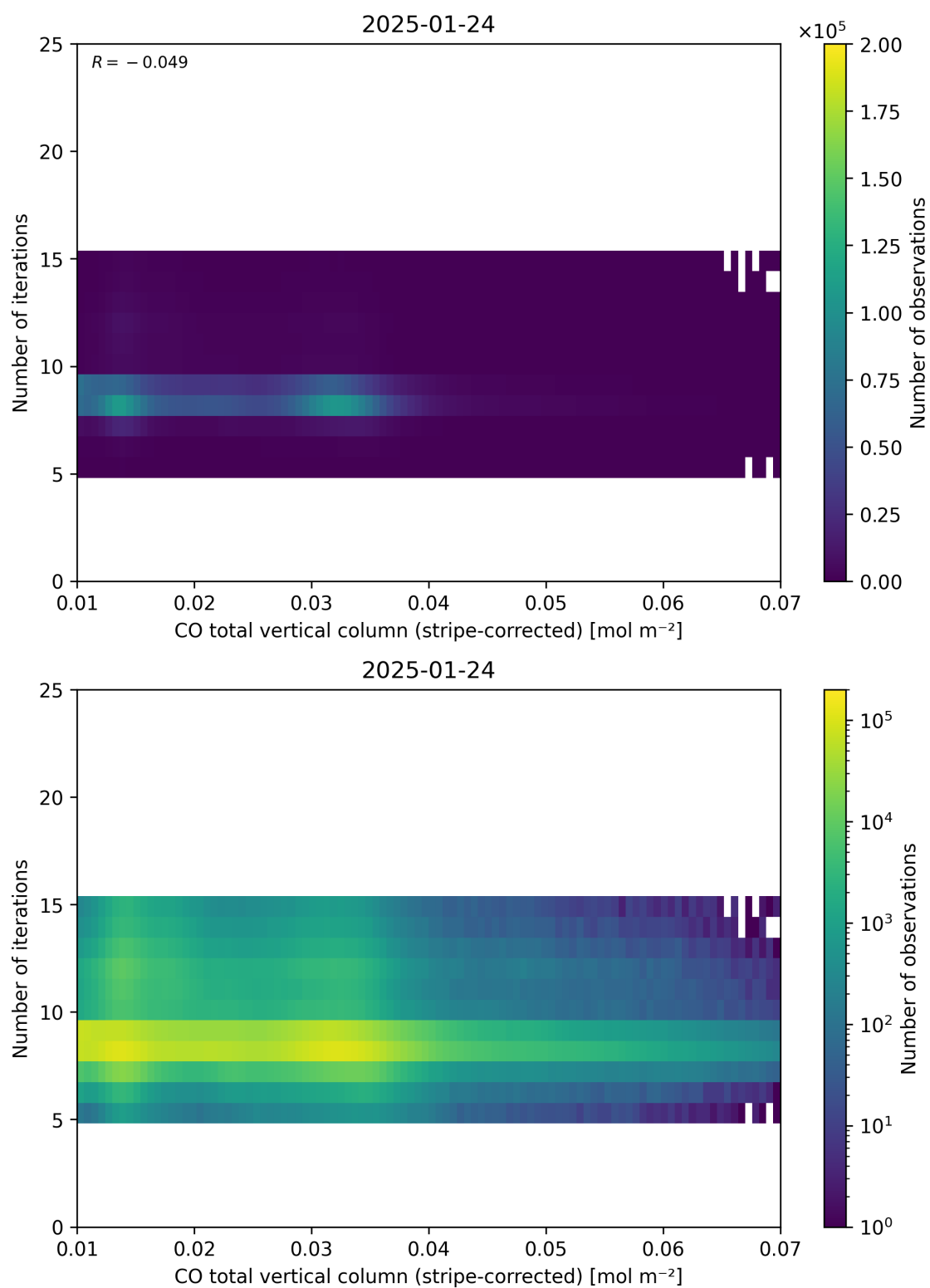
Figure 39: Scatter density plot of “CO total vertical column (stripe-corrected)” against “Number of iterations” for 2025-01-23 to 2025-01-25.
