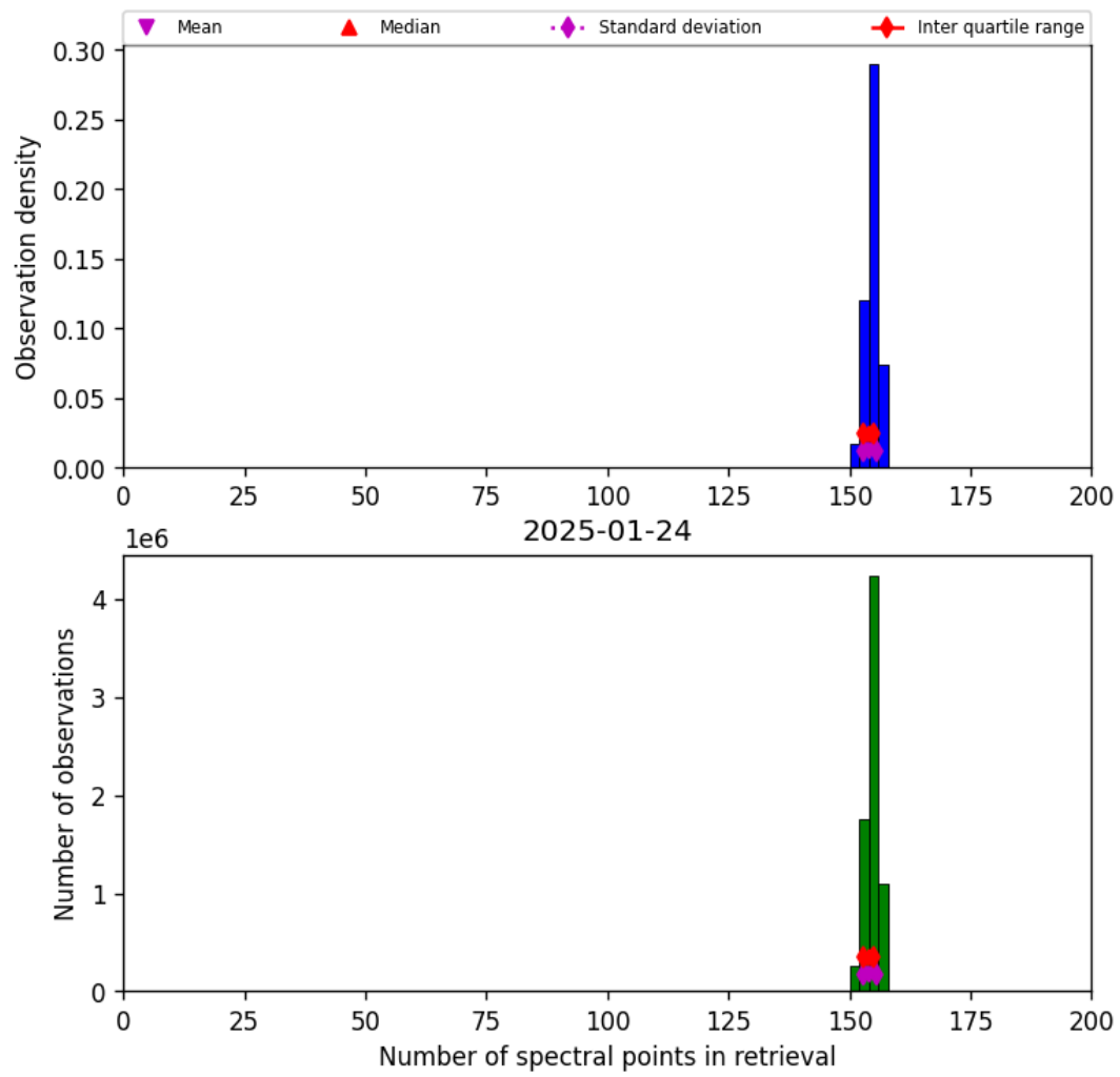
Figure 21: Histogram of “Number of spectral points in retrieval” for 2025-01-23 to 2025-01-25
