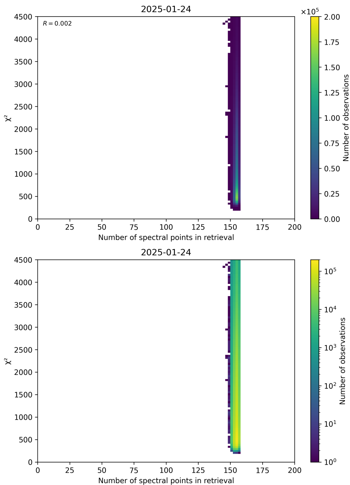
Figure 58: Scatter density plot of “Number of spectral points in retrieval” against “ \chi^2 ” for 2025-01-23 to 2025-01-25.
