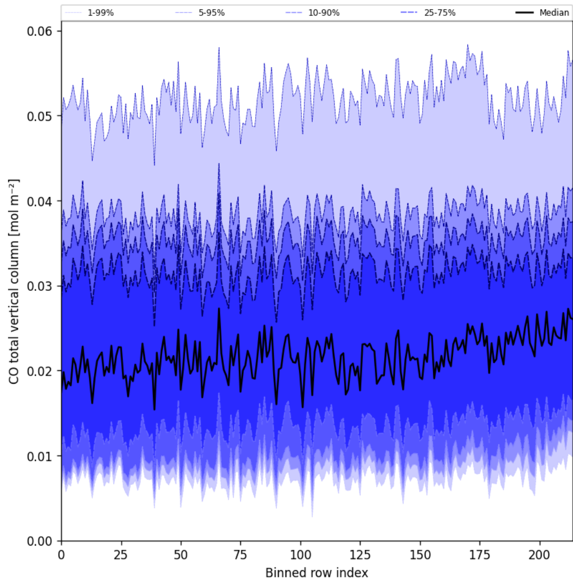
Figure 26: Along track statistics of “CO total vertical column” for 2025-01-23 to 2025-01-25
