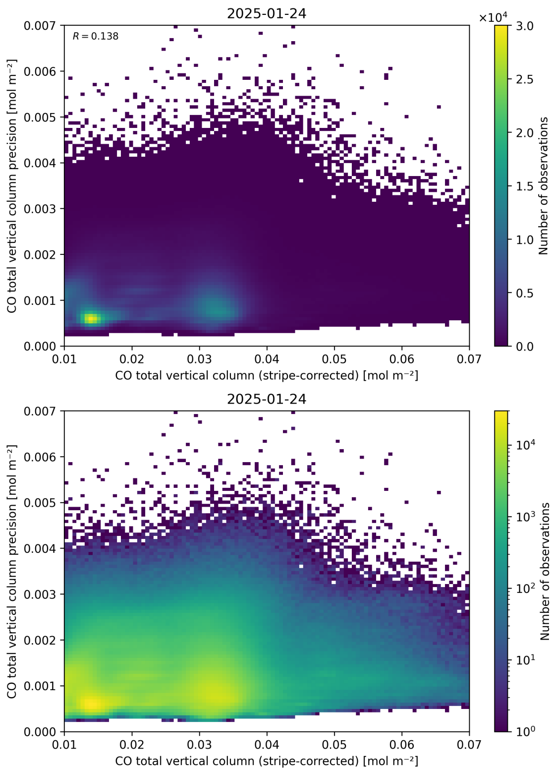
Figure 36: Scatter density plot of “CO total vertical column (stripe-corrected)” against “CO total vertical column precision” for 2025-01-23 to 2025-01-25.
