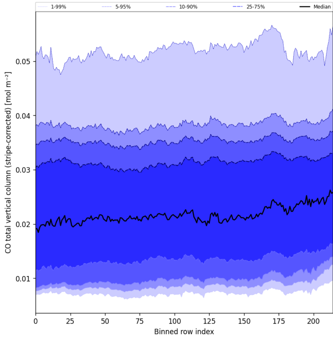
Figure 27: Along track statistics of “CO total vertical column (stripe-corrected)” for 2025-01-23 to 2025-01-25
