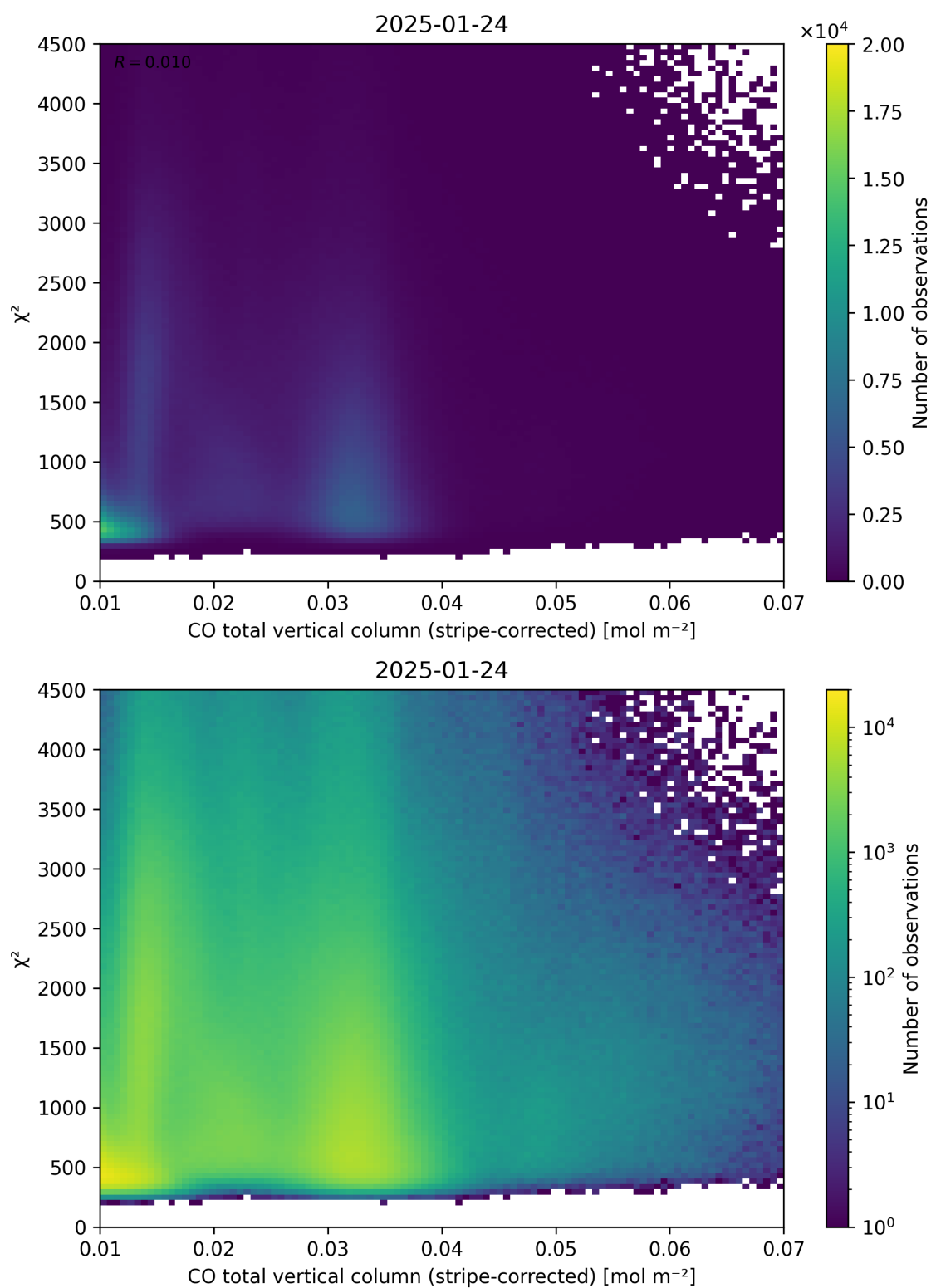
Figure 37: Scatter density plot of “CO total vertical column (stripe-corrected)” against “ \chi^2 ” for 2025-01-23 to 2025-01-25.
