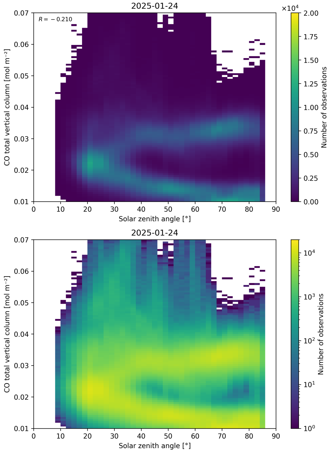
Figure 61: Scatter density plot of “Solar zenith angle” against “CO total vertical column” for 2025-01-23 to 2025-01-25.
