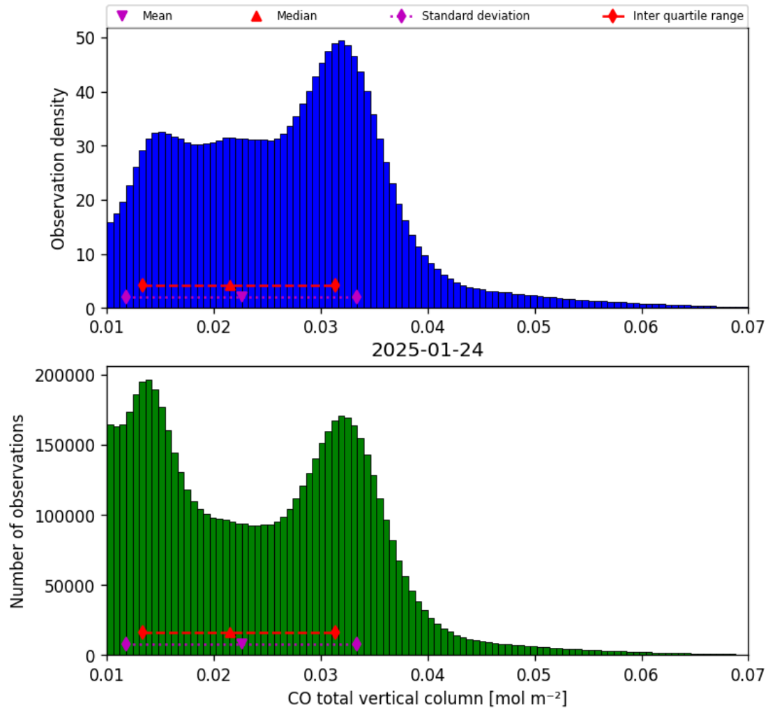
Figure 18: Histogram of “CO total vertical column” for 2025-01-23 to 2025-01-25
