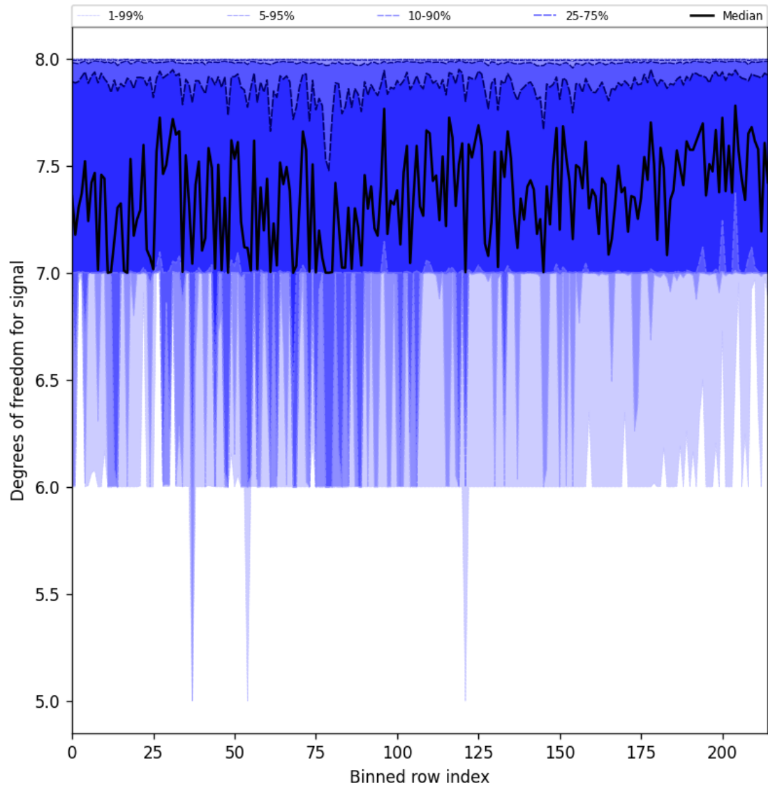
Figure 31: Along track statistics of “Degrees of freedom for signal” for 2025-01-23 to 2025-01-25
