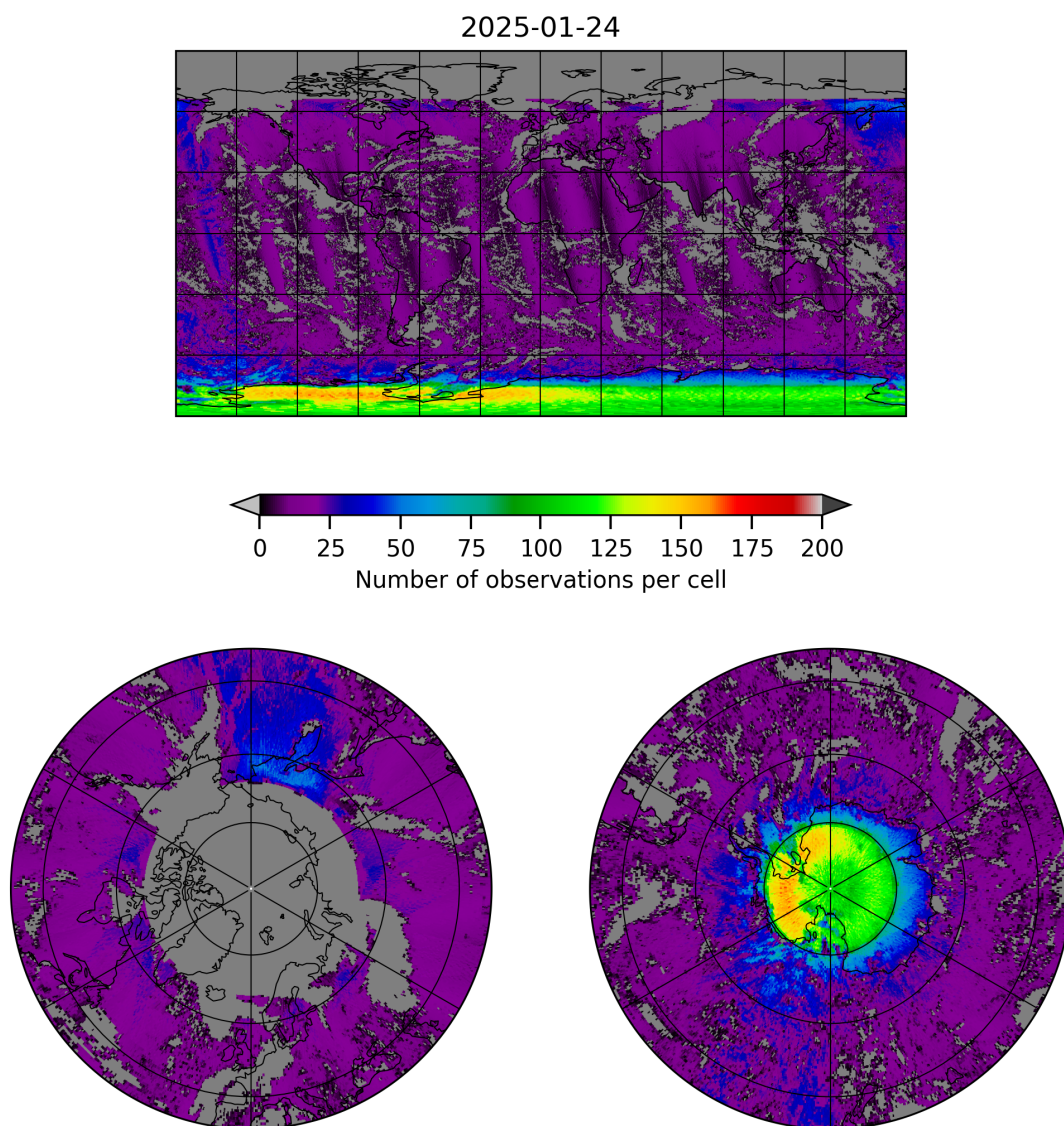
Figure 8: Map of the number of observations for 2025-01-23 to 2025-01-25
