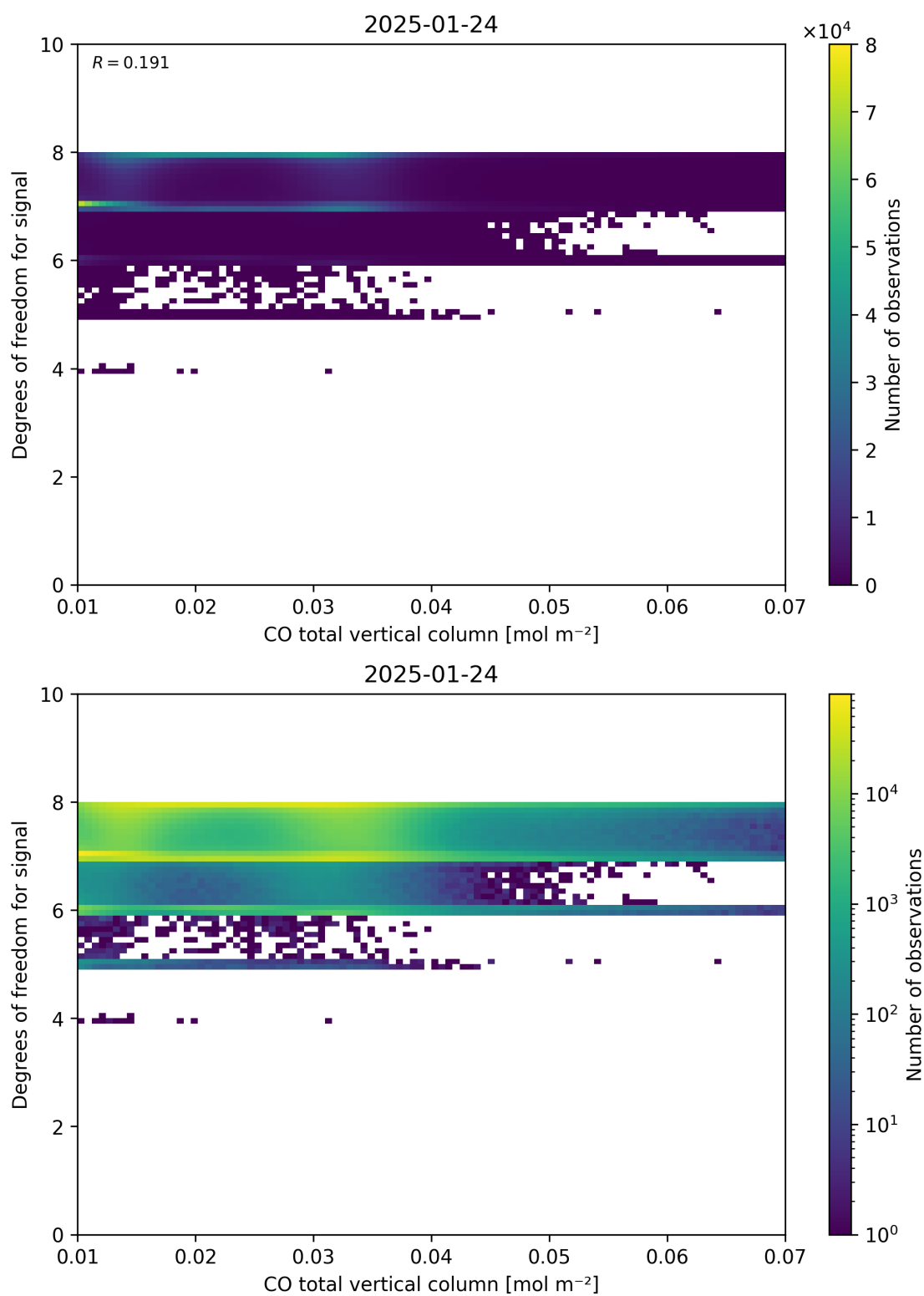
Figure 41: Scatter density plot of “CO total vertical column” against “Degrees of freedom for signal” for 2025-01-23 to 2025-01-25.
