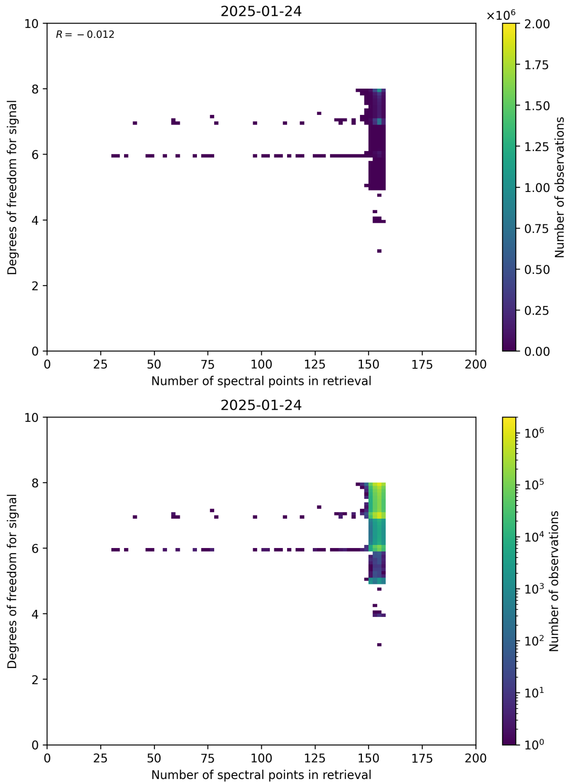
Figure 59: Scatter density plot of “Number of spectral points in retrieval” against “Degrees of freedom for signal” for 2025-01-23 to 2025-01-25.
