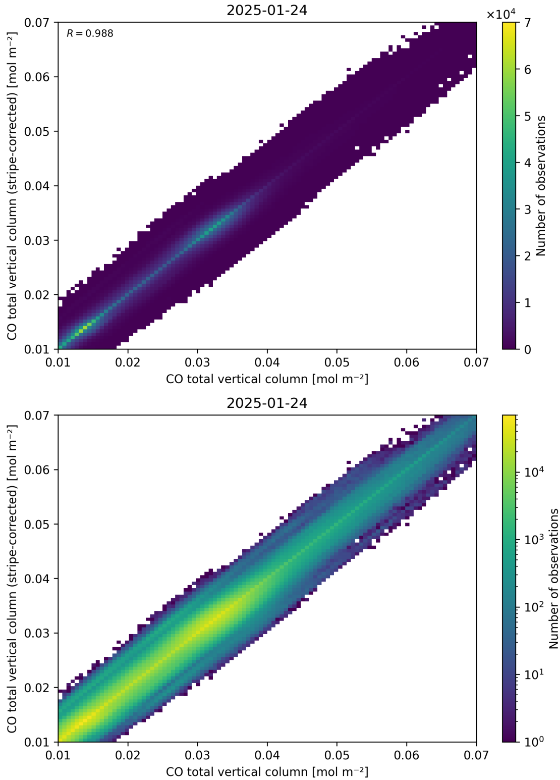
Figure 33: Scatter density plot of “CO total vertical column” against “CO total vertical column (stripe-corrected)” for 2025-01-23 to 2025-01-25.
