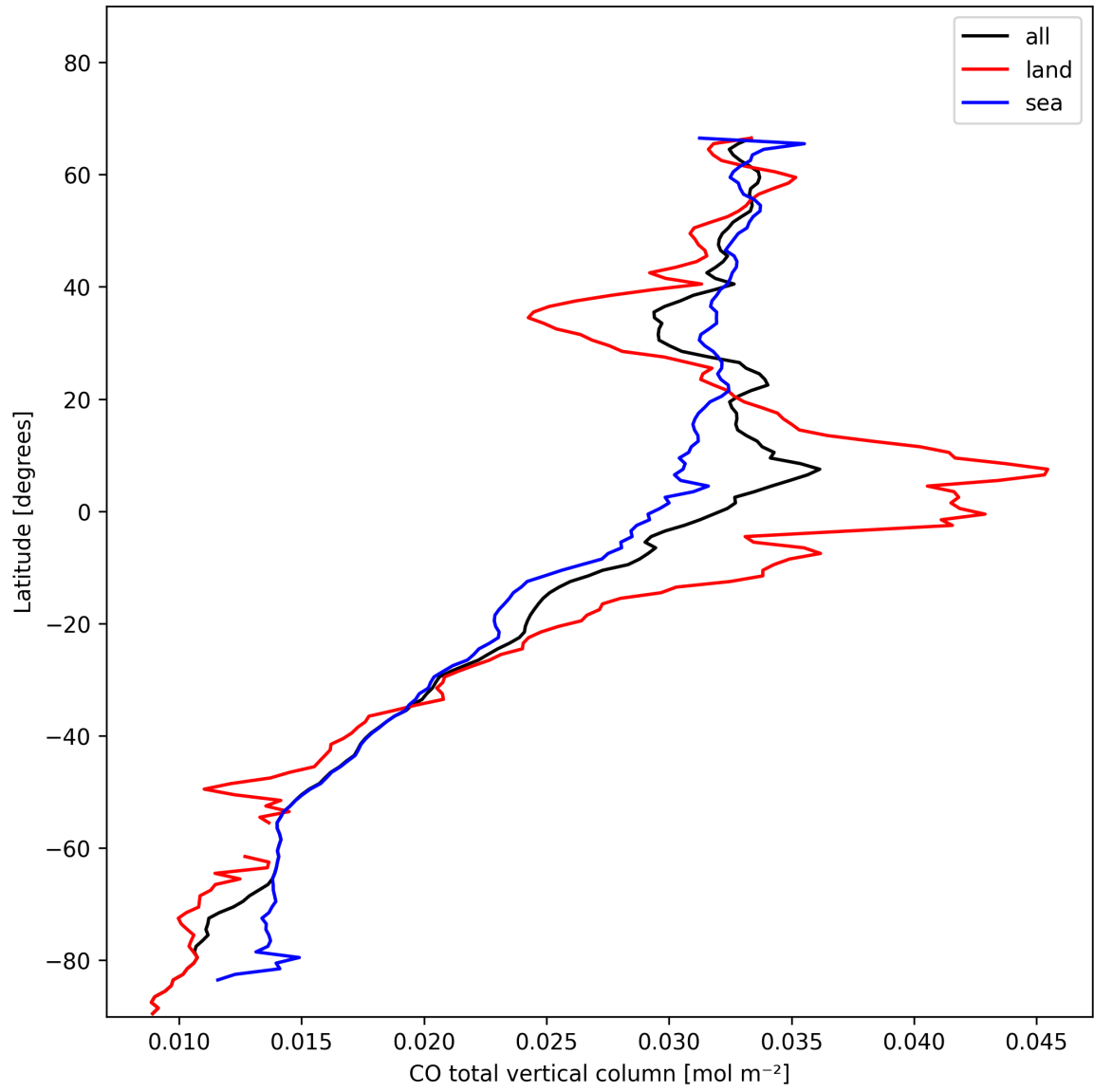
Figure 10: Zonal average of “CO total vertical column” for 2025-01-23 to 2025-01-25.
