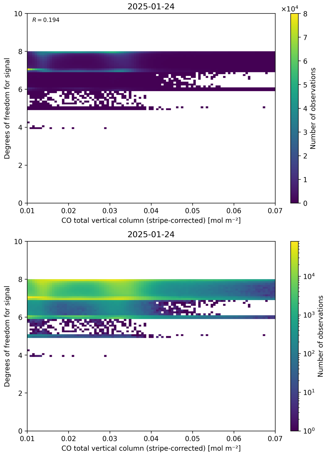
Figure 38: Scatter density plot of “CO total vertical column (stripe-corrected)” against “Degrees of freedom for signal” for 2025-01-23 to 2025-01-25.
