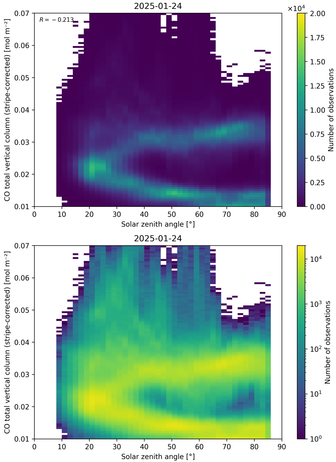
Figure 62: Scatter density plot of “Solar zenith angle” against “CO total vertical column (stripe-corrected)” for 2025-01-23 to 2025-01-25.
