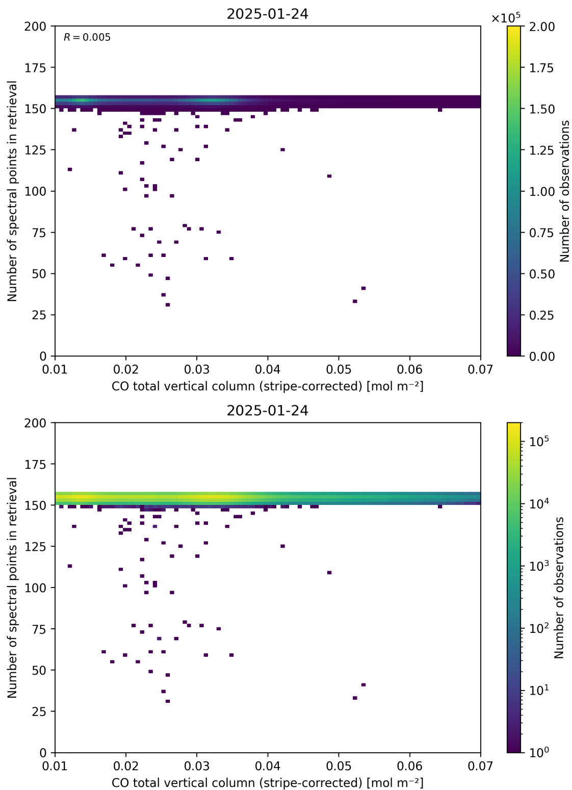
Figure 40: Scatter density plot of “CO total vertical column (stripe-corrected)” against “Number of spectral points in retrieval” for 2025-01-23 to 2025-01-25.
