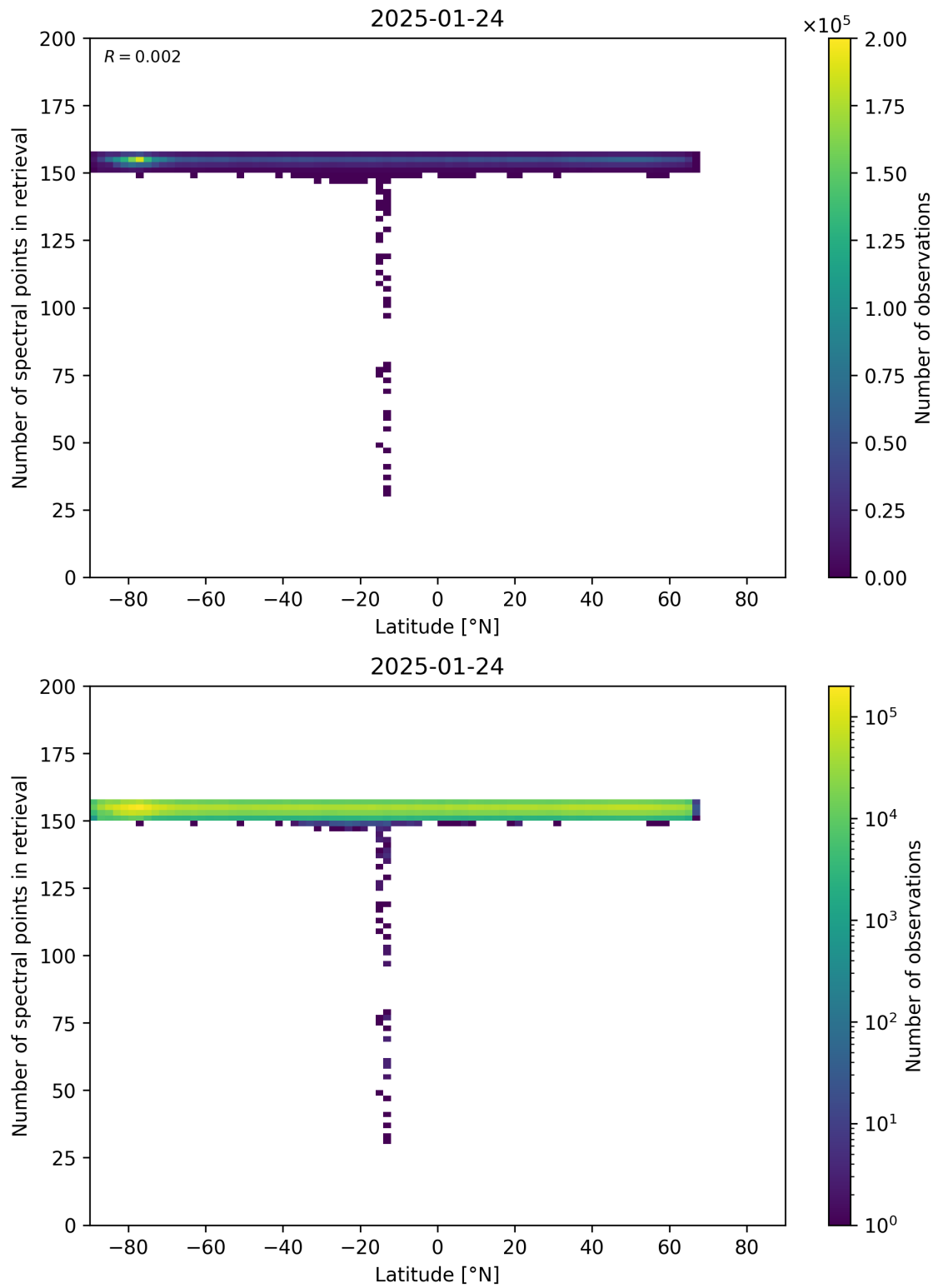
Figure 57: Scatter density plot of “Latitude” against “Number of spectral points in retrieval” for 2025-01-23 to 2025-01-25.
