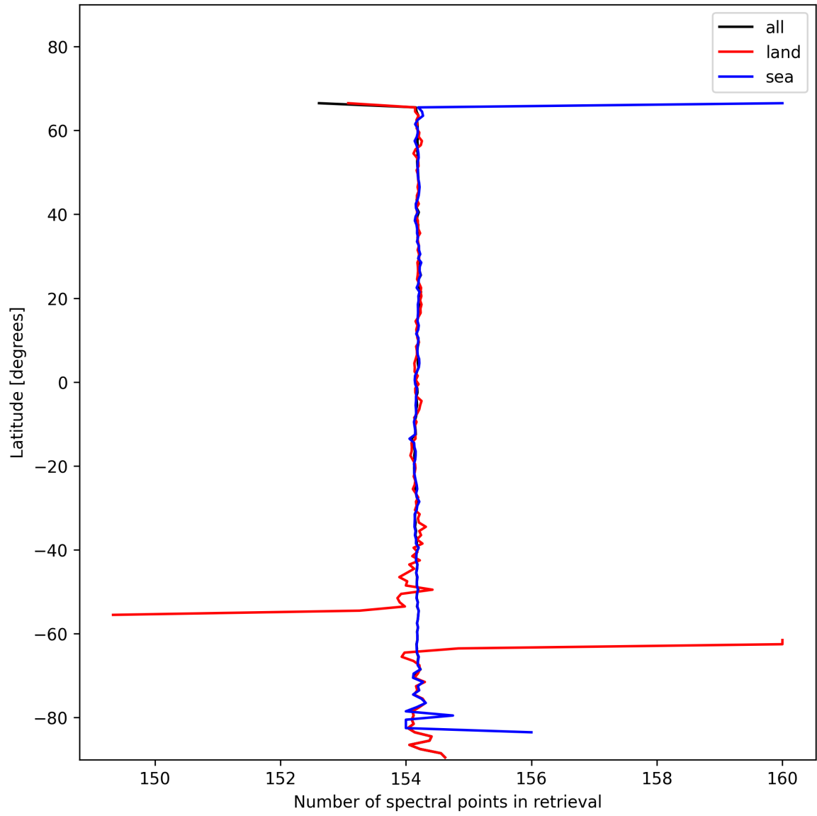
Figure 13: Zonal average of “Number of spectral points in retrieval” for 2025-01-23 to 2025-01-25.
