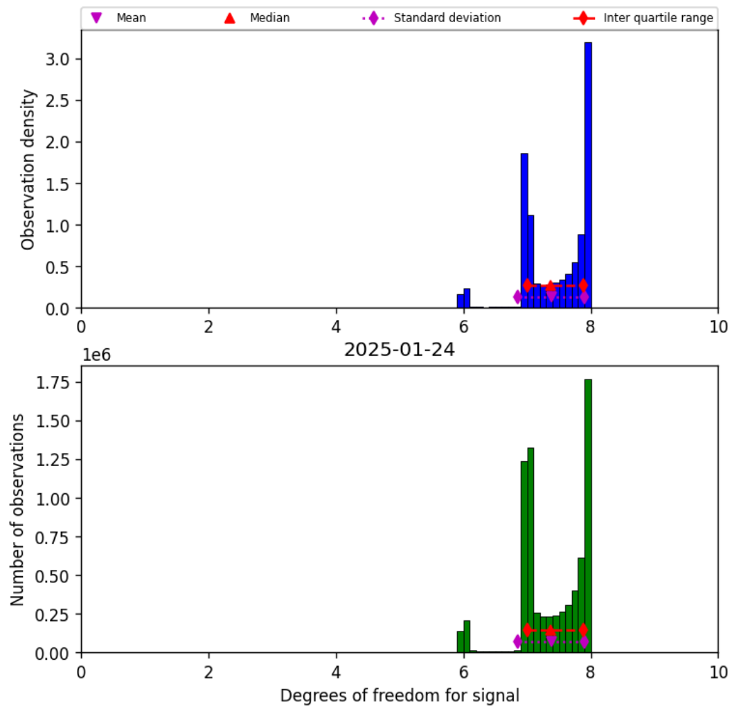
Figure 23: Histogram of “Degrees of freedom for signal” for 2025-01-23 to 2025-01-25
