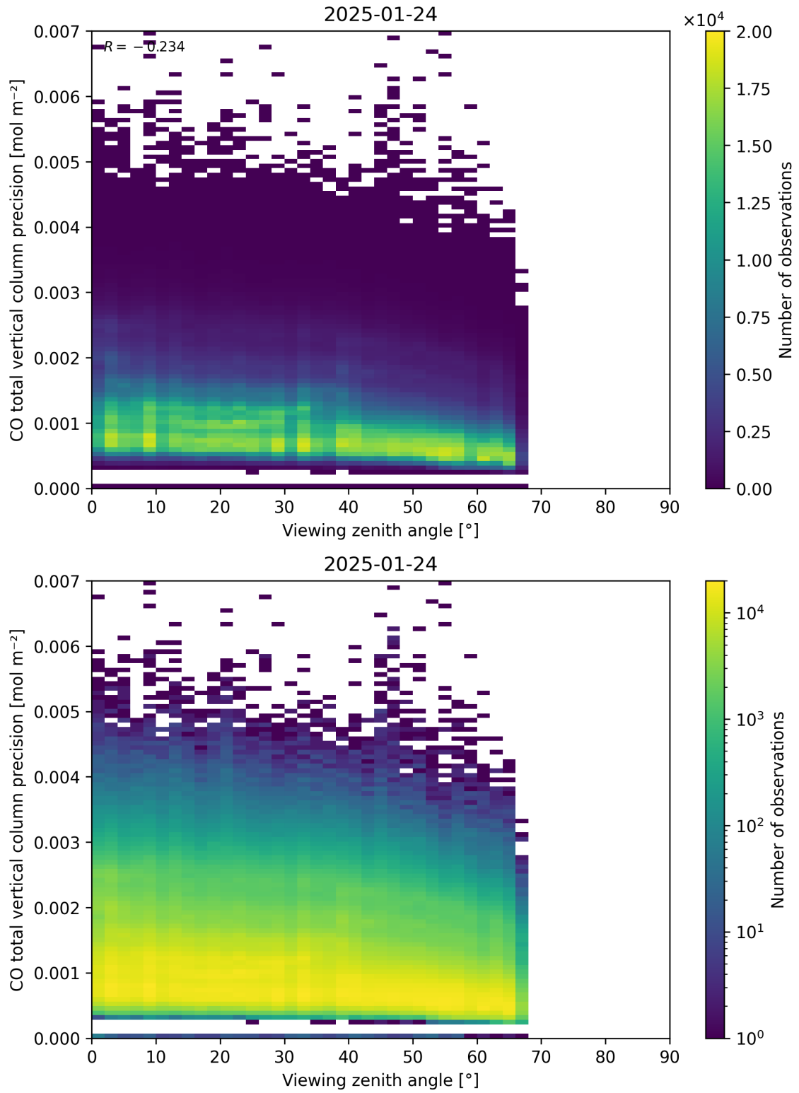
Figure 71: Scatter density plot of “Viewing zenith angle” against “CO total vertical column precision” for 2025-01-23 to 2025-01-25.
