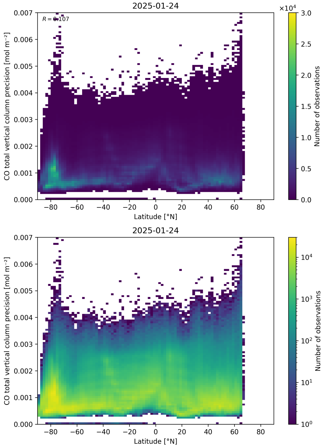
Figure 53: Scatter density plot of “Latitude” against “CO total vertical column precision” for 2025-01-23 to 2025-01-25.
