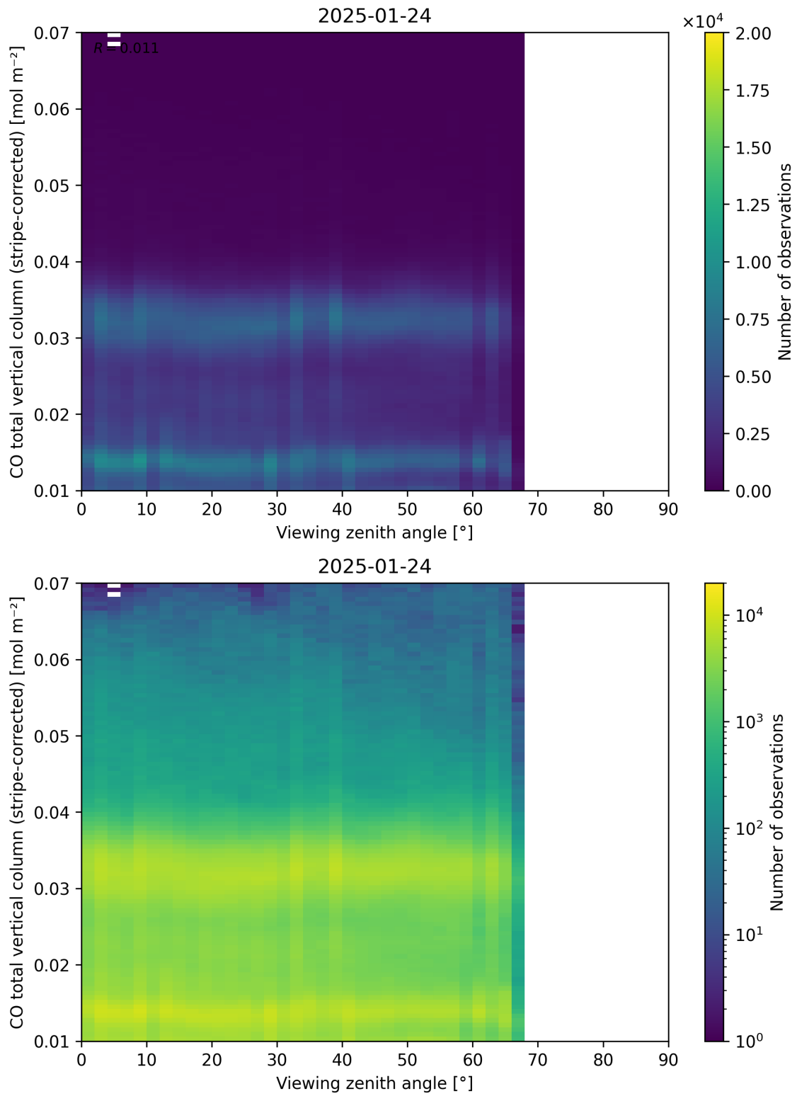
Figure 70: Scatter density plot of “Viewing zenith angle” against “CO total vertical column (stripe-corrected)” for 2025-01-23 to 2025-01-25.
