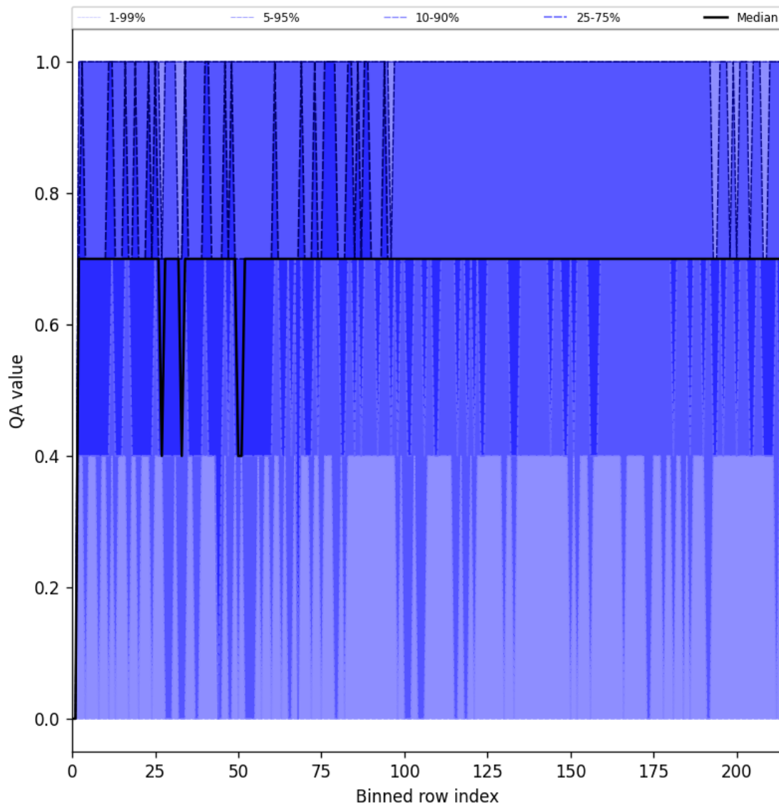
Figure 25: Along track statistics of “QA value” for 2025-01-23 to 2025-01-25
