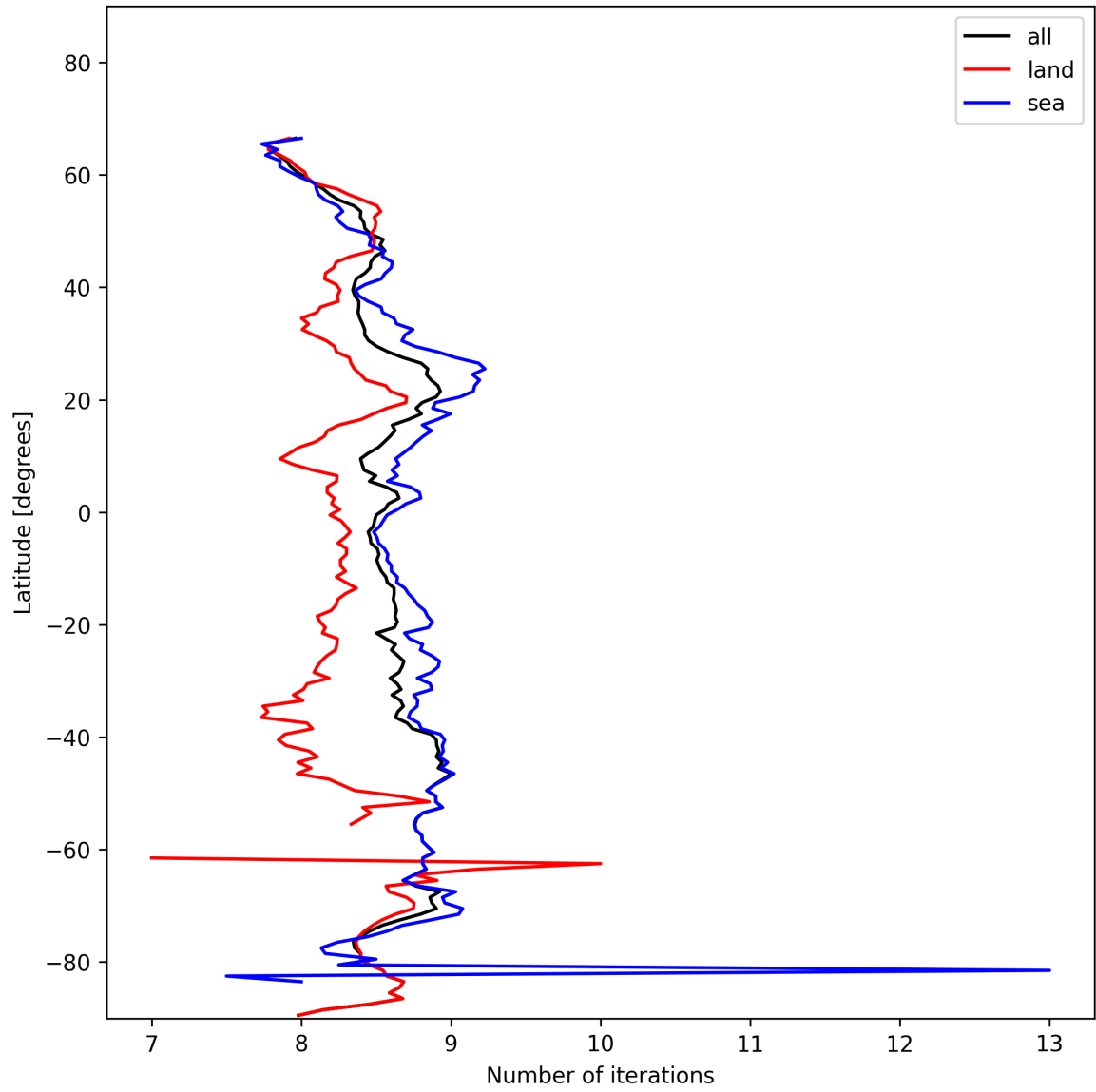
Figure 16: Zonal average of “Number of iterations” for 2025-01-23 to 2025-01-25.
