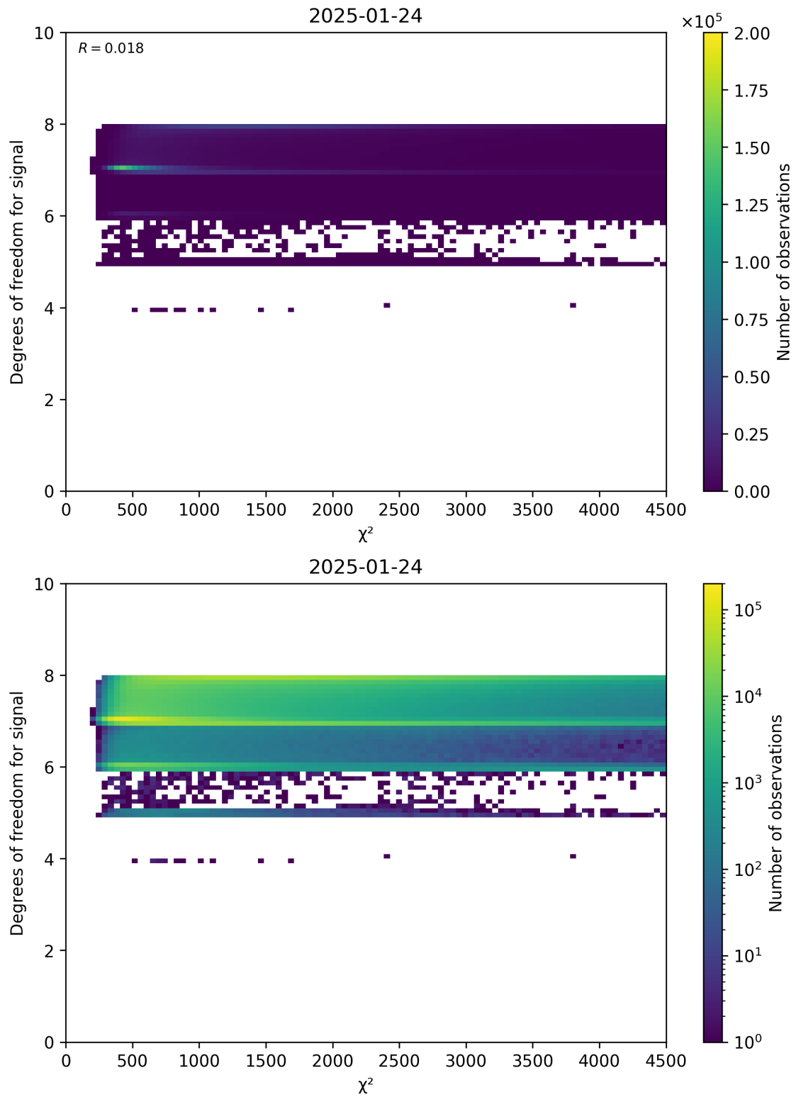
Figure 48: Scatter density plot of “ \chi^2 ” against “Degrees of freedom for signal” for 2025-01-23 to 2025-01-25.
