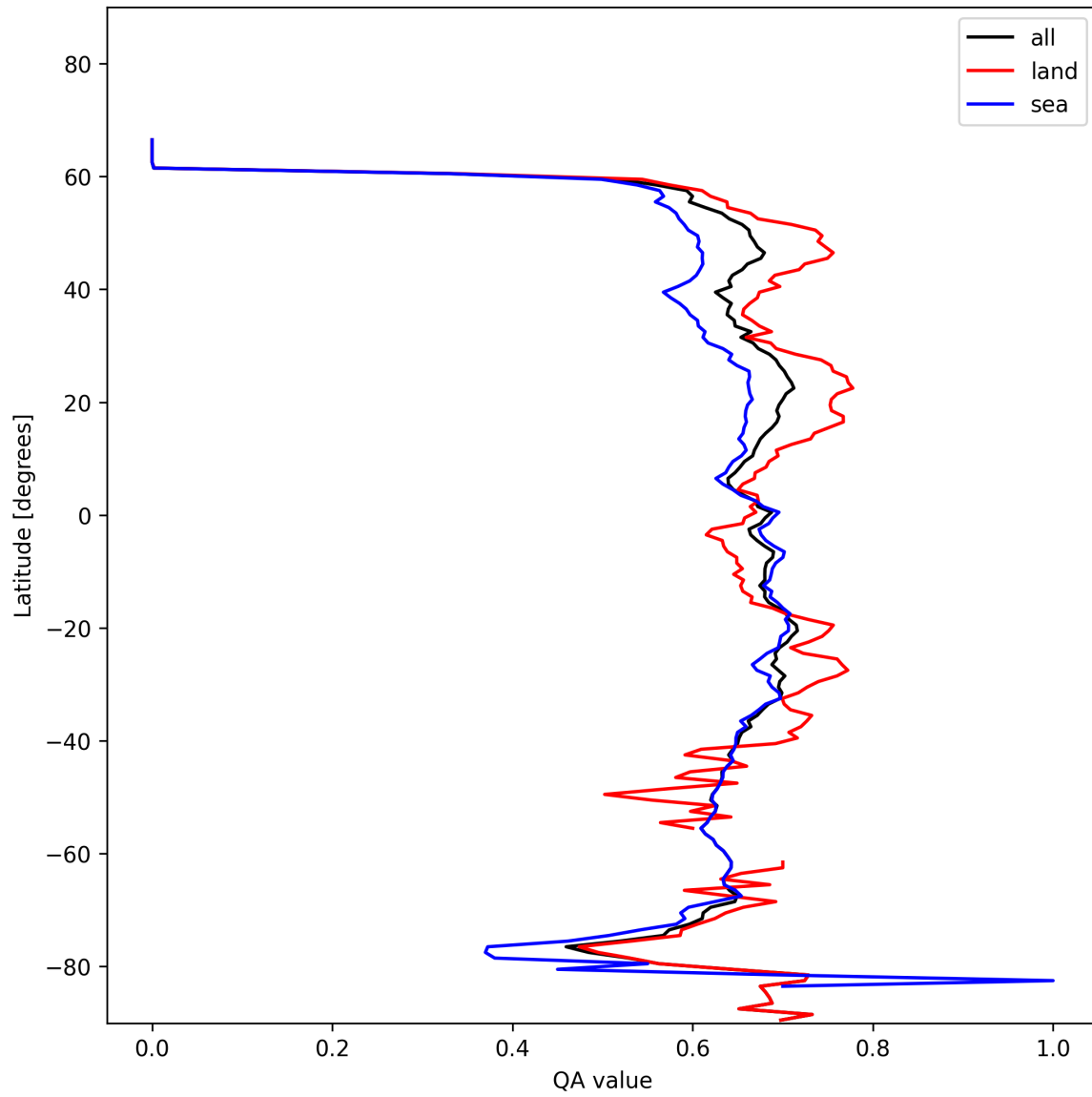
Figure 9: Zonal average of “QA value” for 2025-01-23 to 2025-01-25.
