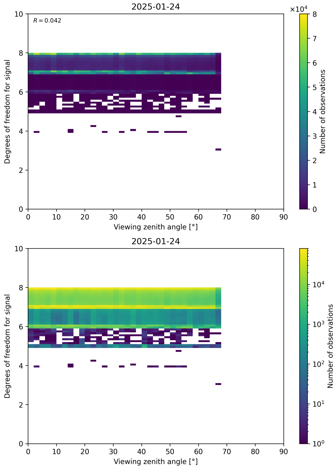
Figure 73: Scatter density plot of “Viewing zenith angle” against “Degrees of freedom for signal” for 2025-01-23 to 2025-01-25.
