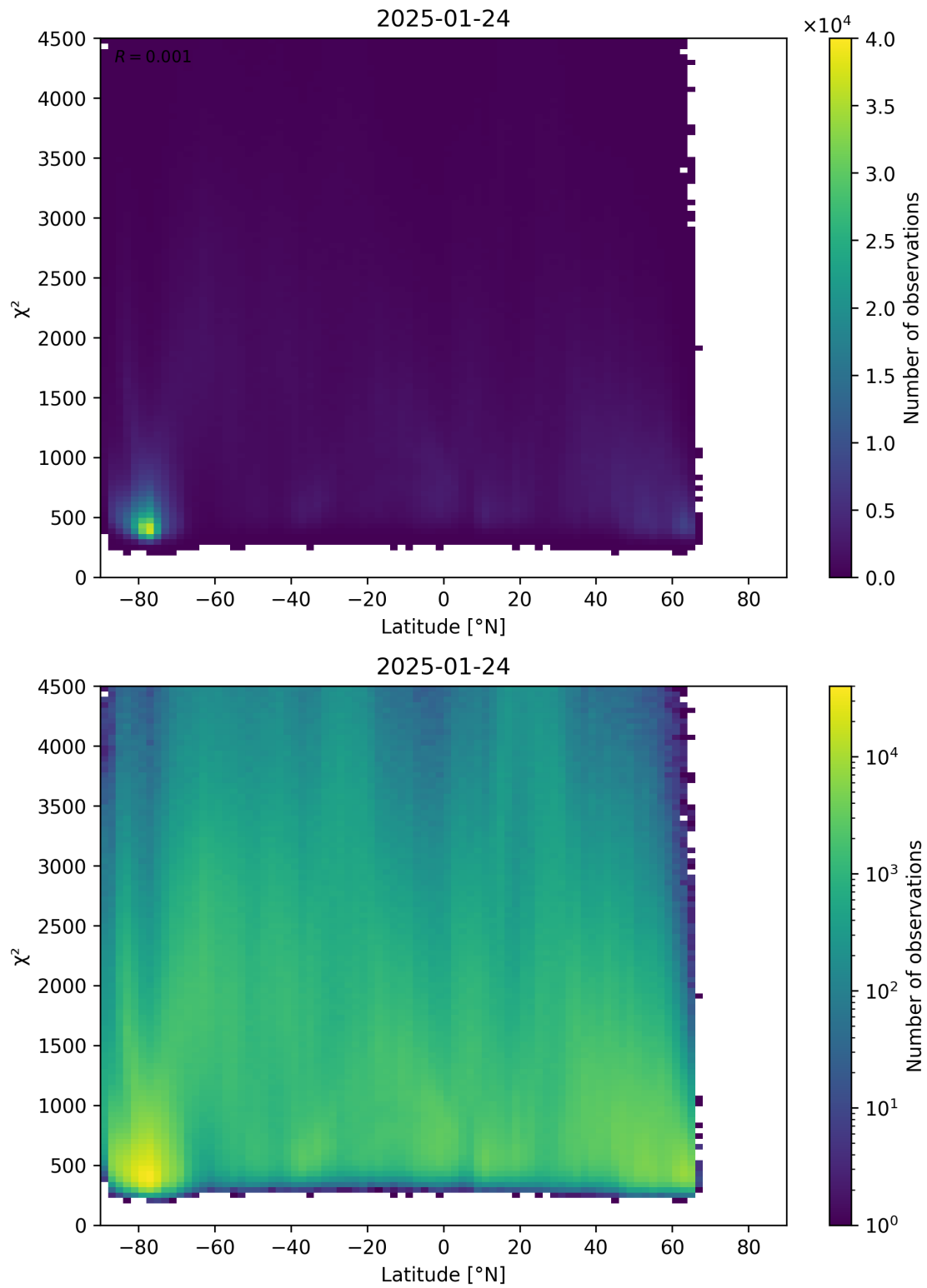
Figure 54: Scatter density plot of “Latitude” against “ \chi^2 ” for 2025-01-23 to 2025-01-25.
