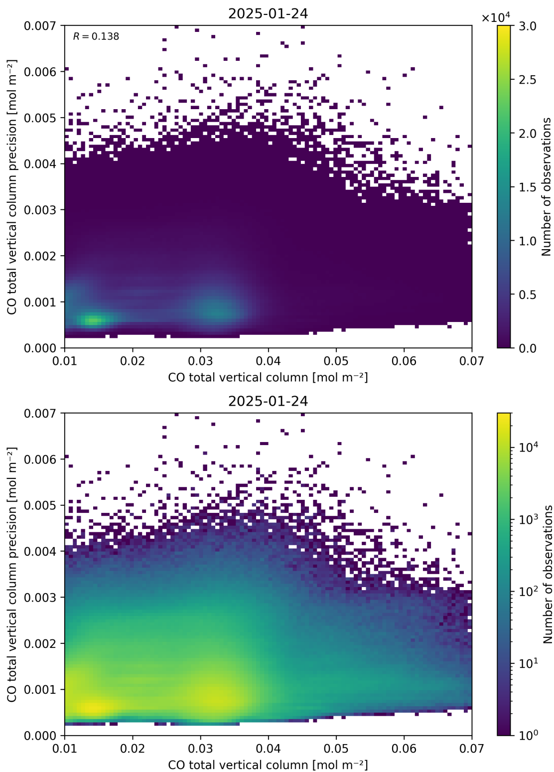
Figure 34: Scatter density plot of “CO total vertical column” against “CO total vertical column precision” for 2025-01-23 to 2025-01-25.
