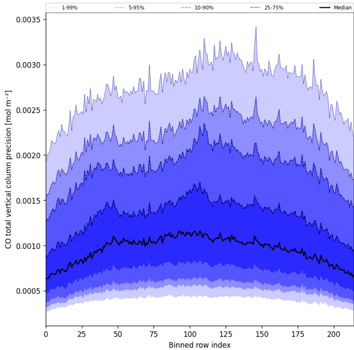
Figure 28: Along track statistics of “CO total vertical column precision” for 2025-01-23 to 2025-01-25
