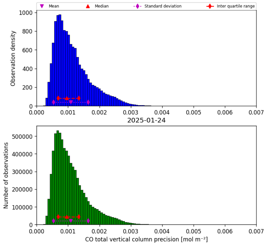
Figure 20: Histogram of “CO total vertical column precision” for 2025-01-23 to 2025-01-25
