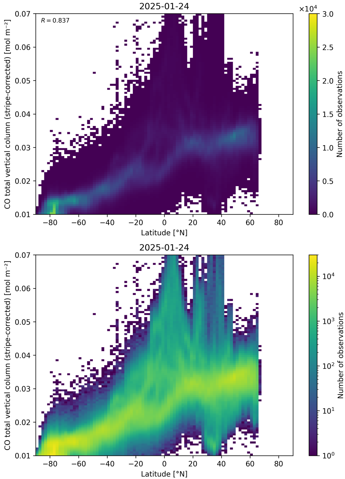
Figure 52: Scatter density plot of “Latitude” against “CO total vertical column (stripe-corrected)” for 2025-01-23 to 2025-01-25.
