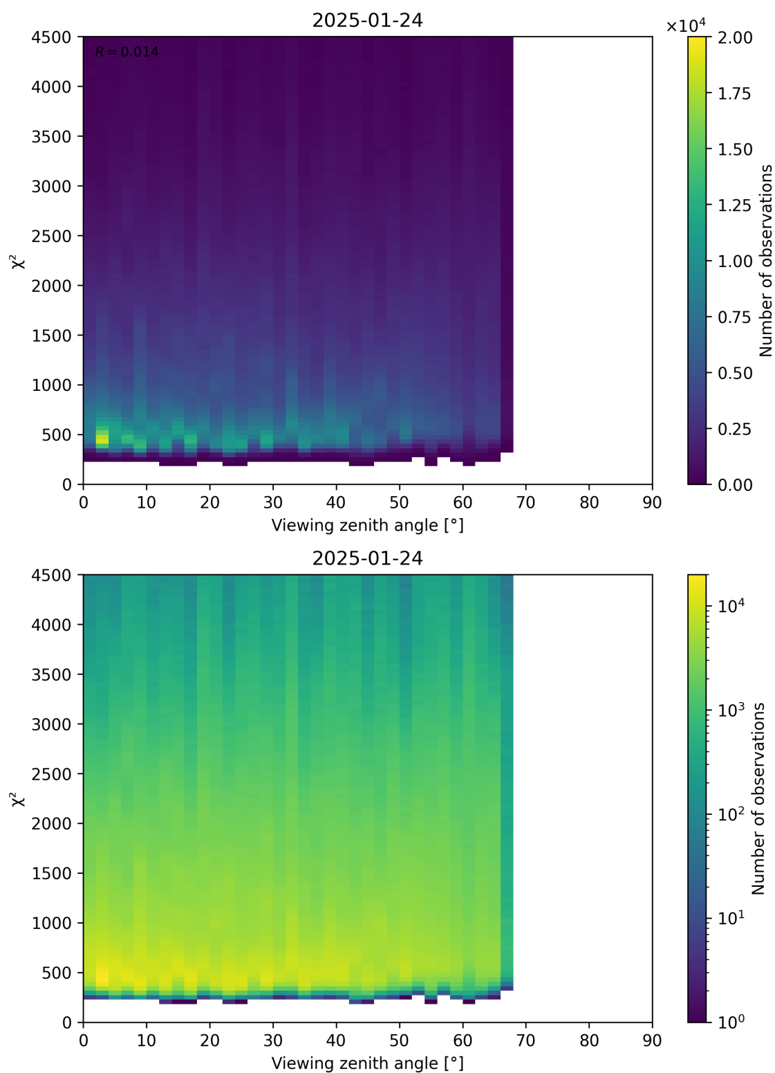
Figure 72: Scatter density plot of “Viewing zenith angle” against “ \chi^2 ” for 2025-01-23 to 2025-01-25.
