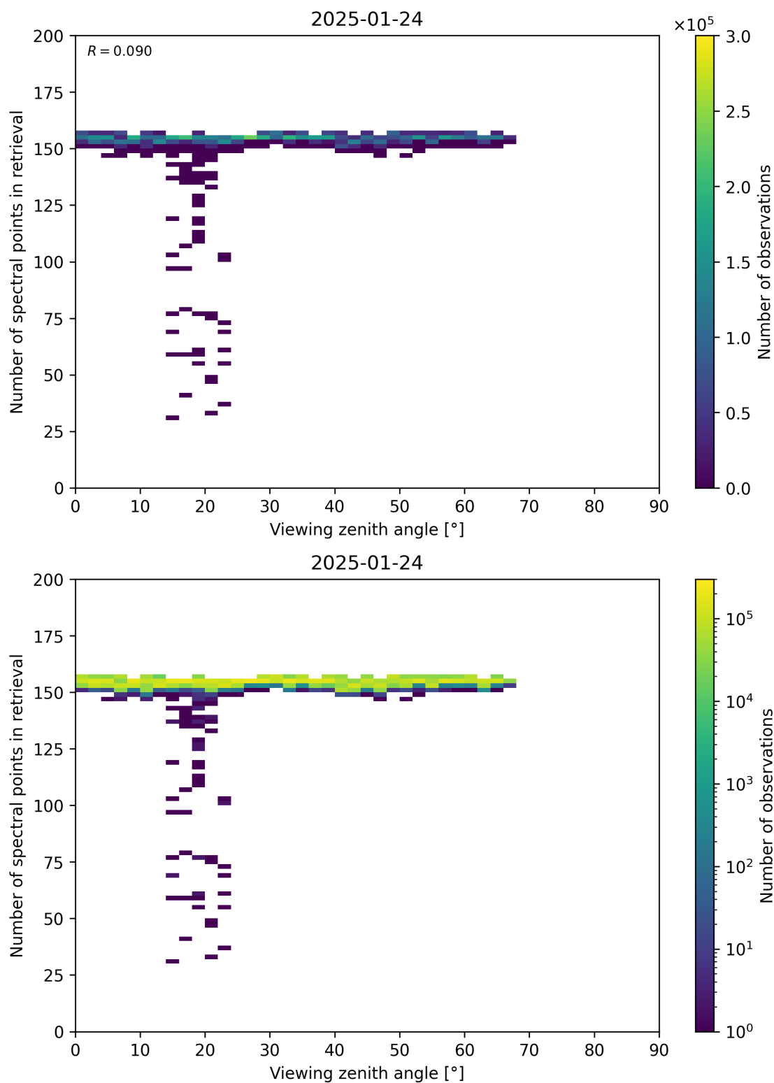
Figure 76: Scatter density plot of “Viewing zenith angle” against “Number of spectral points in retrieval” for 2025-01-23 to 2025-01-25.
