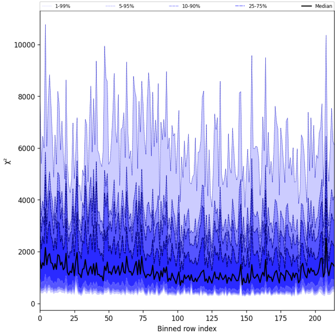
Figure 30: Along track statistics of “ \chi^2 ” for 2025-01-23 to 2025-01-25
