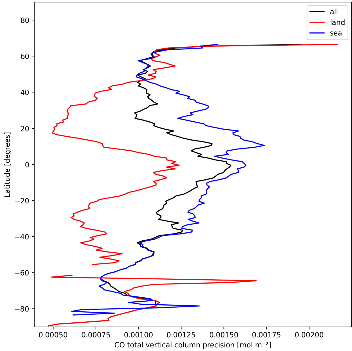
Figure 12: Zonal average of "CO total vertical column precision" for 2025-01-23 to 2025-01-25.
