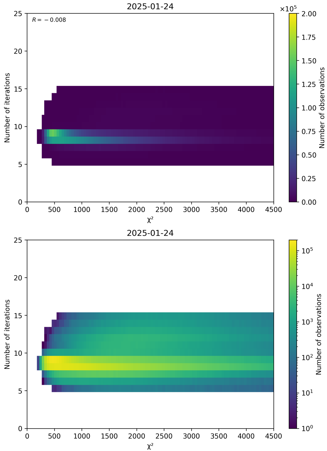
Figure 49: Scatter density plot of “ \chi^2 ” against “Number of iterations” for 2025-01-23 to 2025-01-25.
