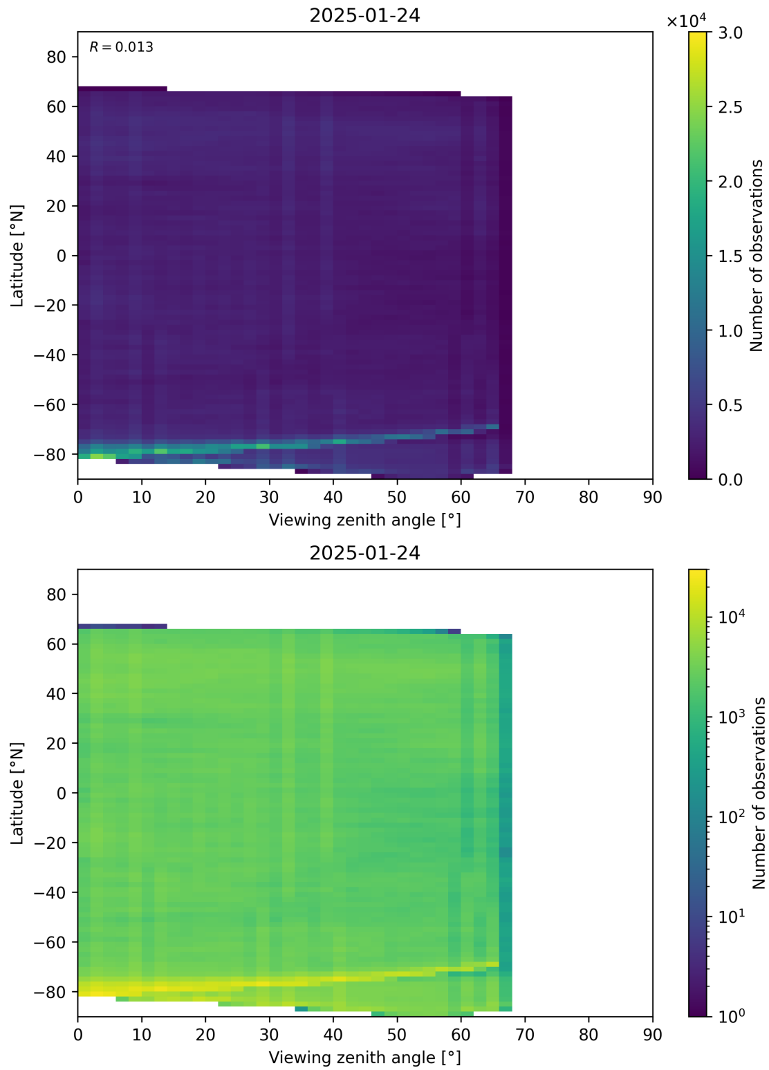
Figure 74: Scatter density plot of “Viewing zenith angle” against “Latitude” for 2025-01-23 to 2025-01-25.
