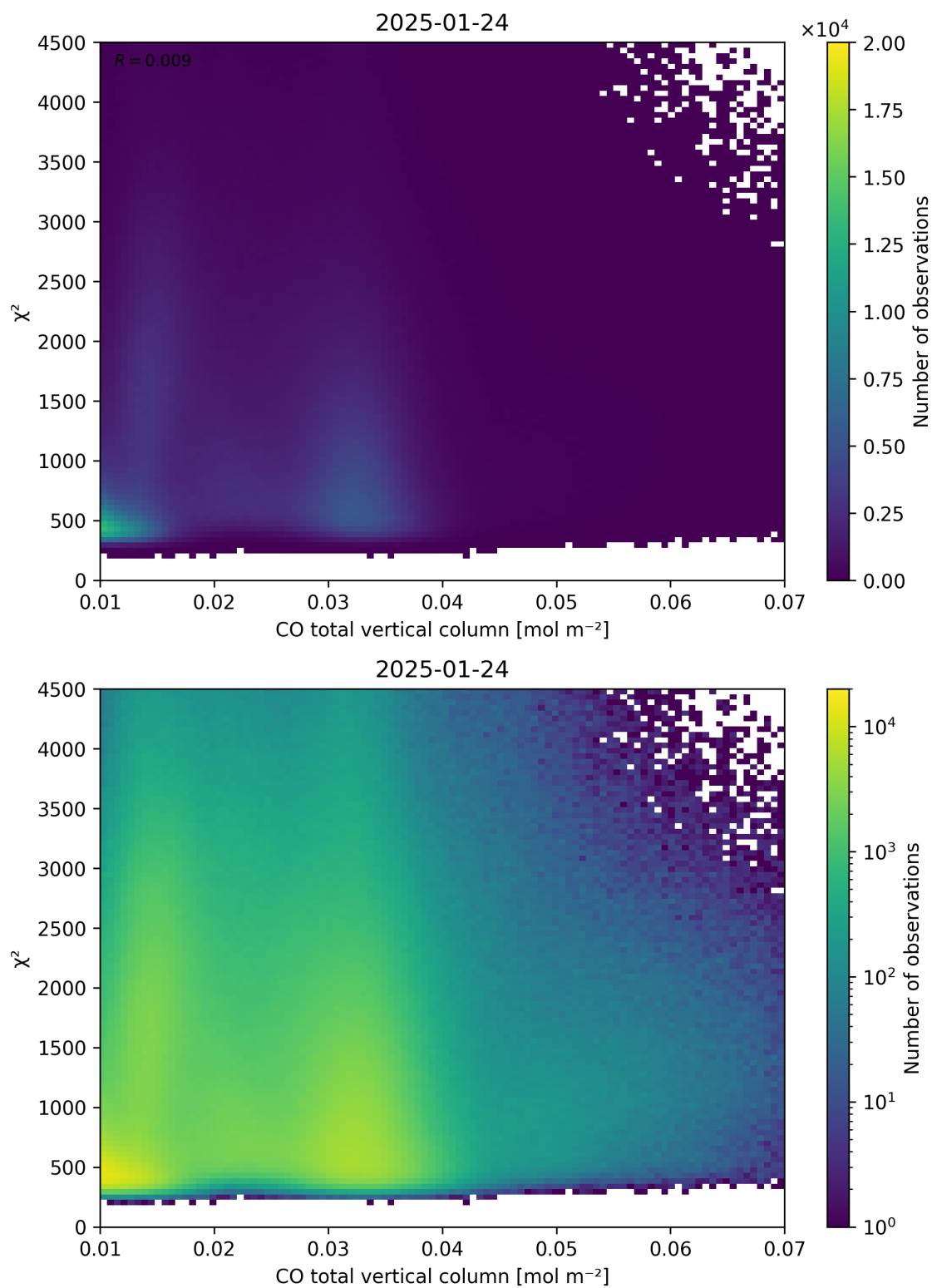
Figure 35: Scatter density plot of “CO total vertical column” against “ \chi^2 ” for 2025-01-23 to 2025-01-25.
