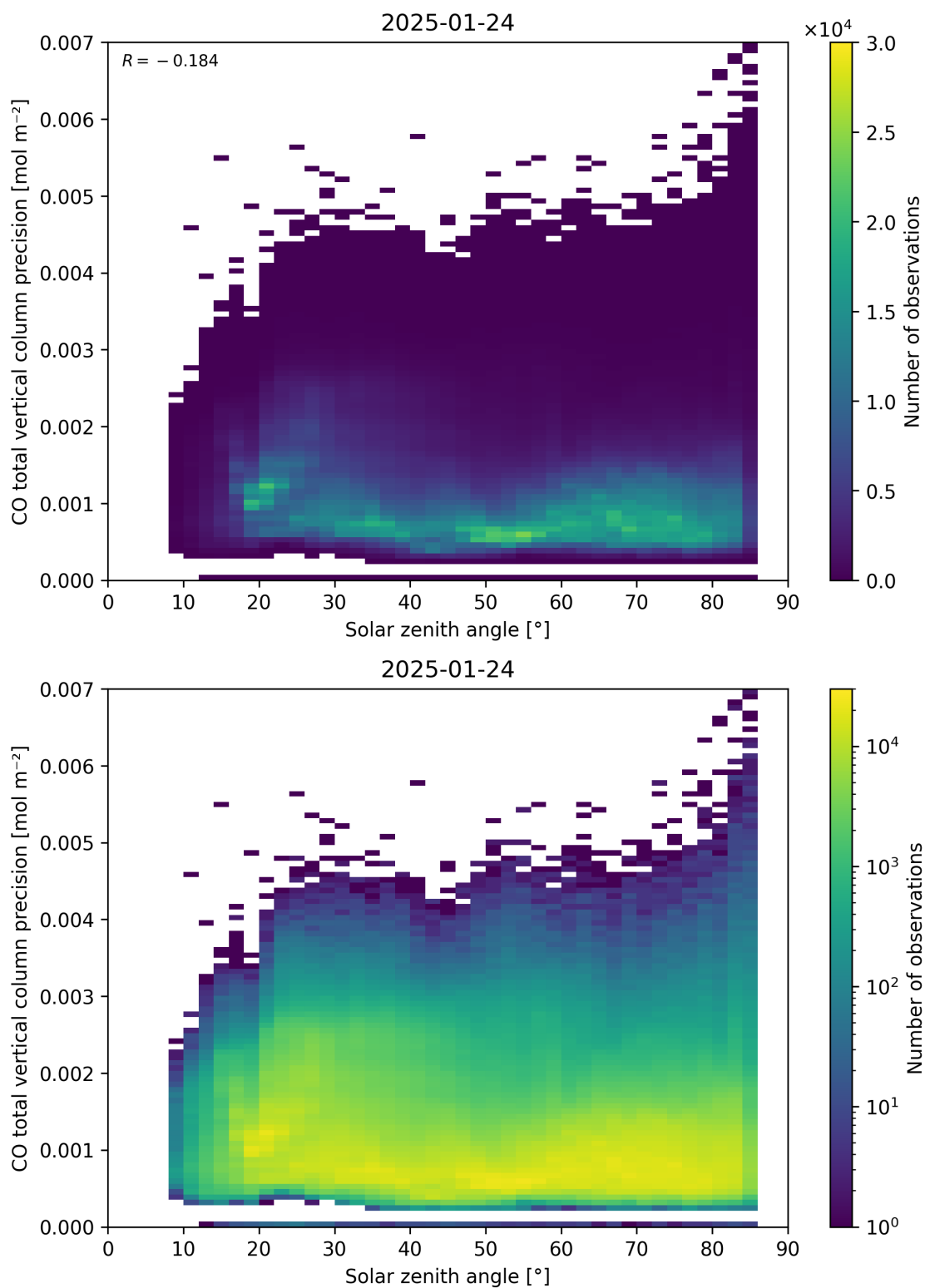
Figure 63: Scatter density plot of “Solar zenith angle” against “CO total vertical column precision” for 2025-01-23 to 2025-01-25.
