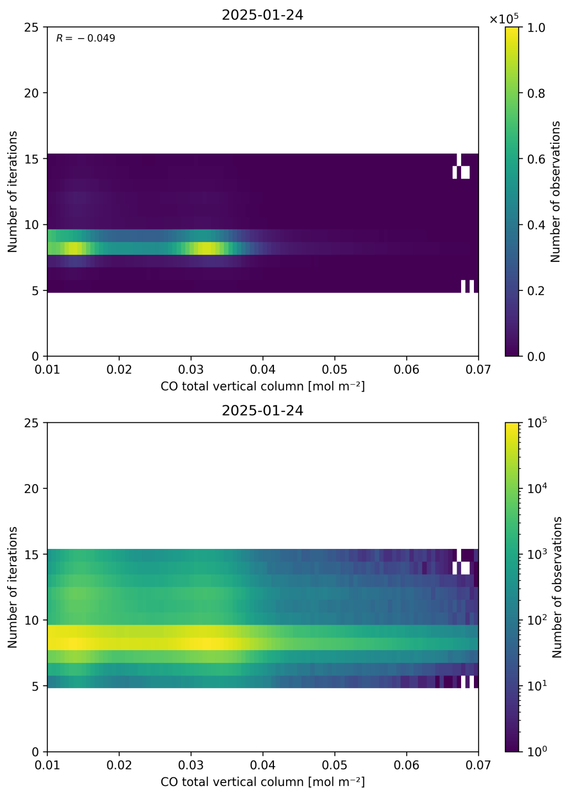
Figure 42: Scatter density plot of “CO total vertical column” against “Number of iterations” for 2025-01-23 to 2025-01-25.
