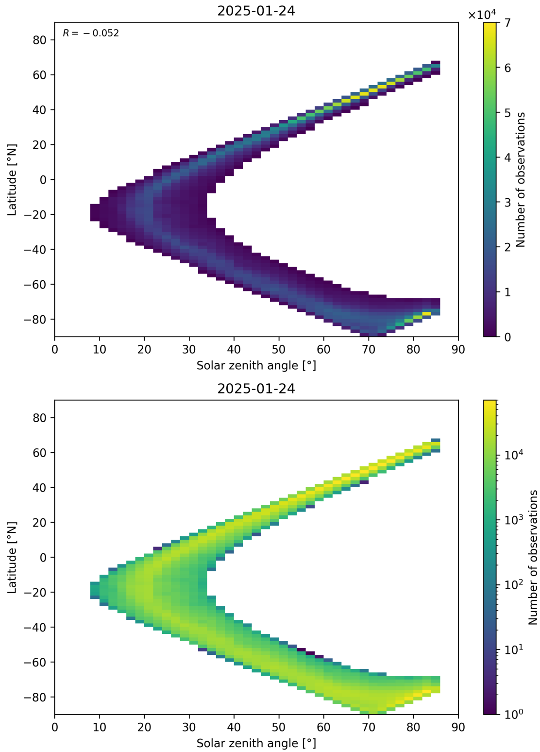
Figure 66: Scatter density plot of “Solar zenith angle” against “Latitude” for 2025-01-23 to 2025-01-25.
