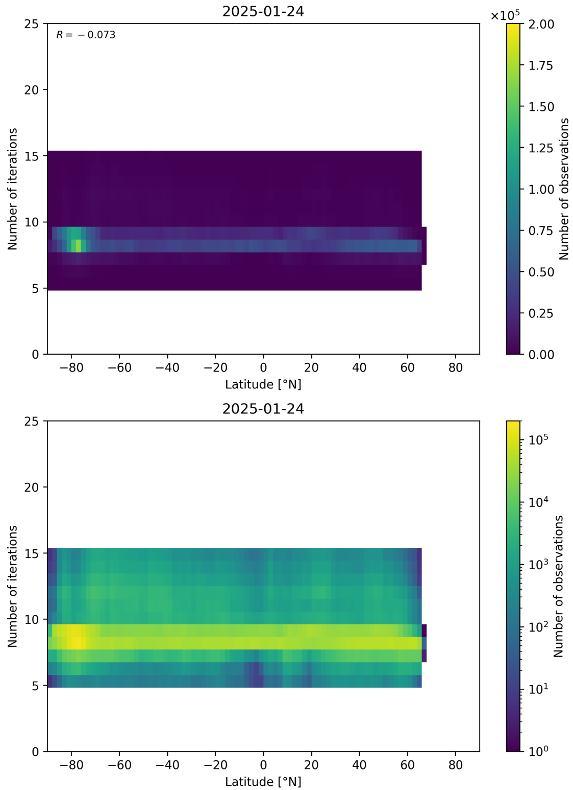
Figure 56: Scatter density plot of “Latitude” against “Number of iterations” for 2025-01-23 to 2025-01-25.
