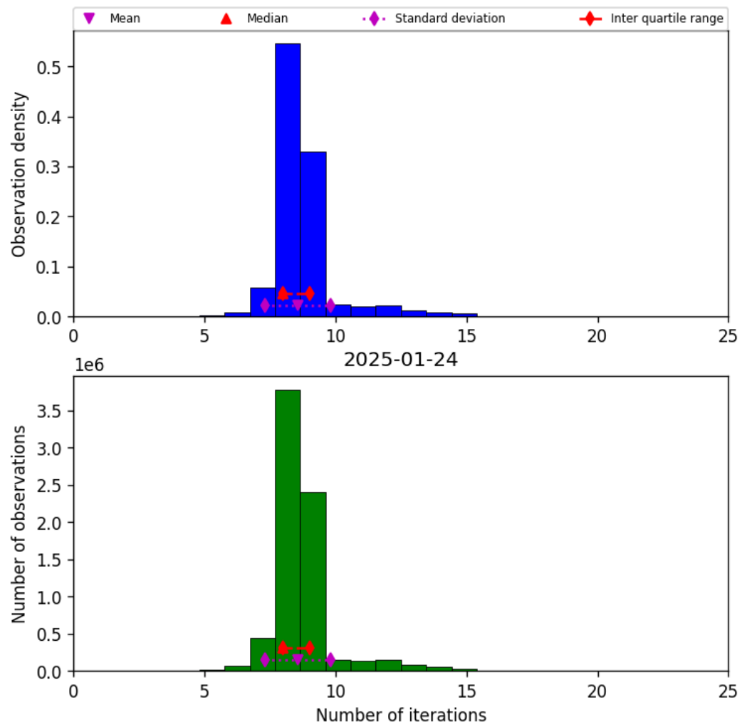
Figure 24: Histogram of “Number of iterations” for 2025-01-23 to 2025-01-25
