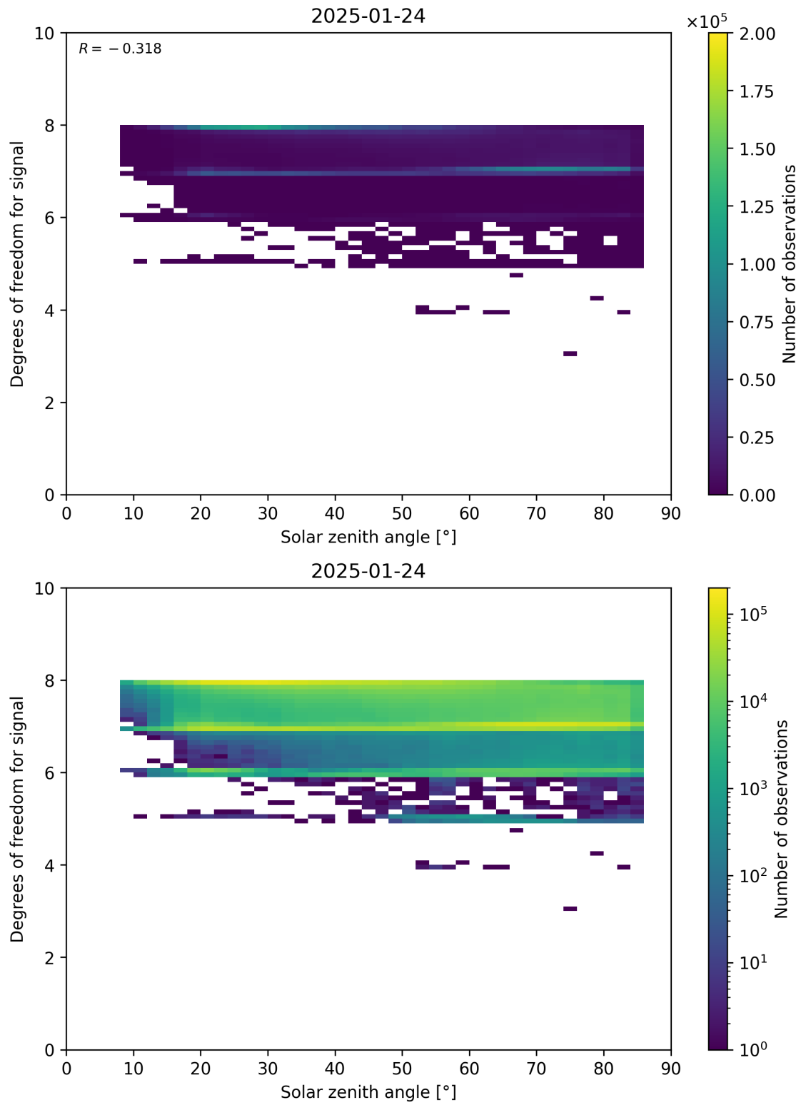
Figure 65: Scatter density plot of “Solar zenith angle” against “Degrees of freedom for signal” for 2025-01-23 to 2025-01-25.
