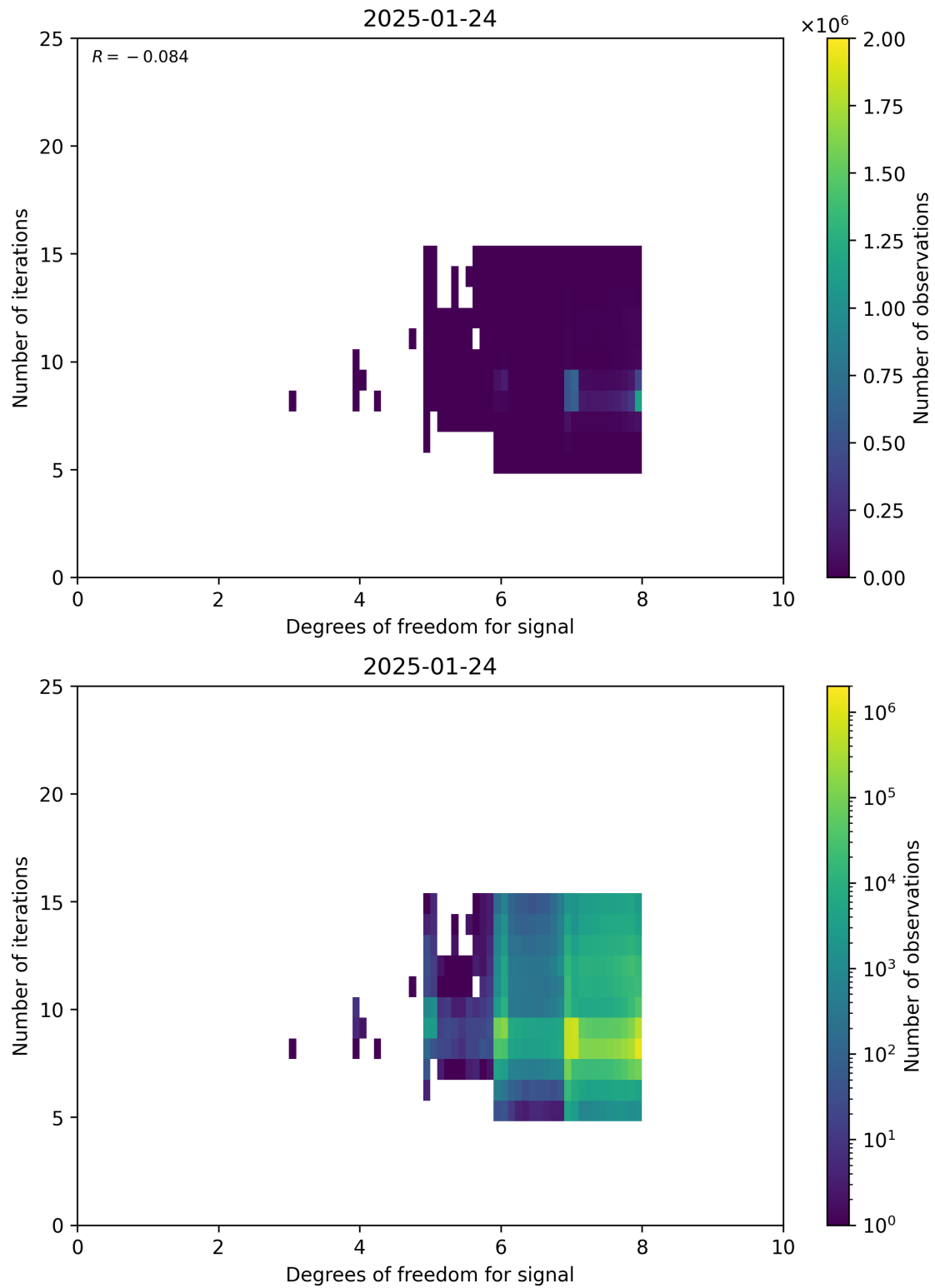
Figure 50: Scatter density plot of “Degrees of freedom for signal” against “Number of iterations” for 2025-01-23 to 2025-01-25.
