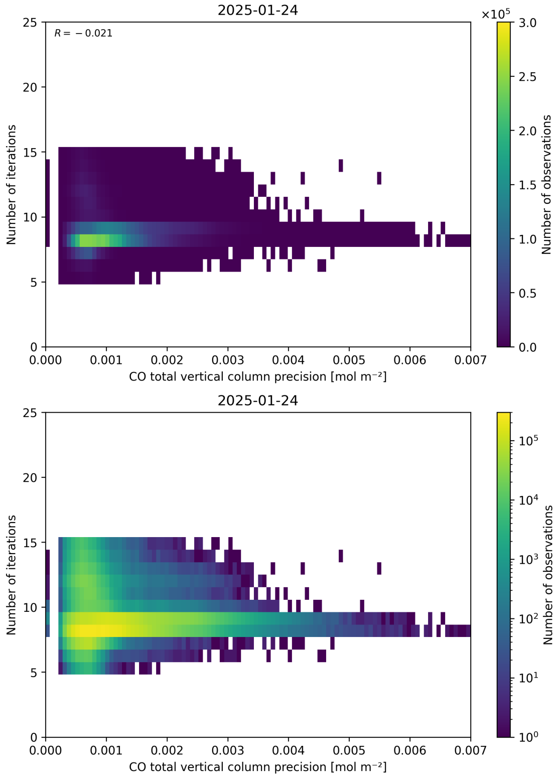
Figure 46: Scatter density plot of “CO total vertical column precision” against “Number of iterations” for 2025-01-23 to 2025-01-25.
