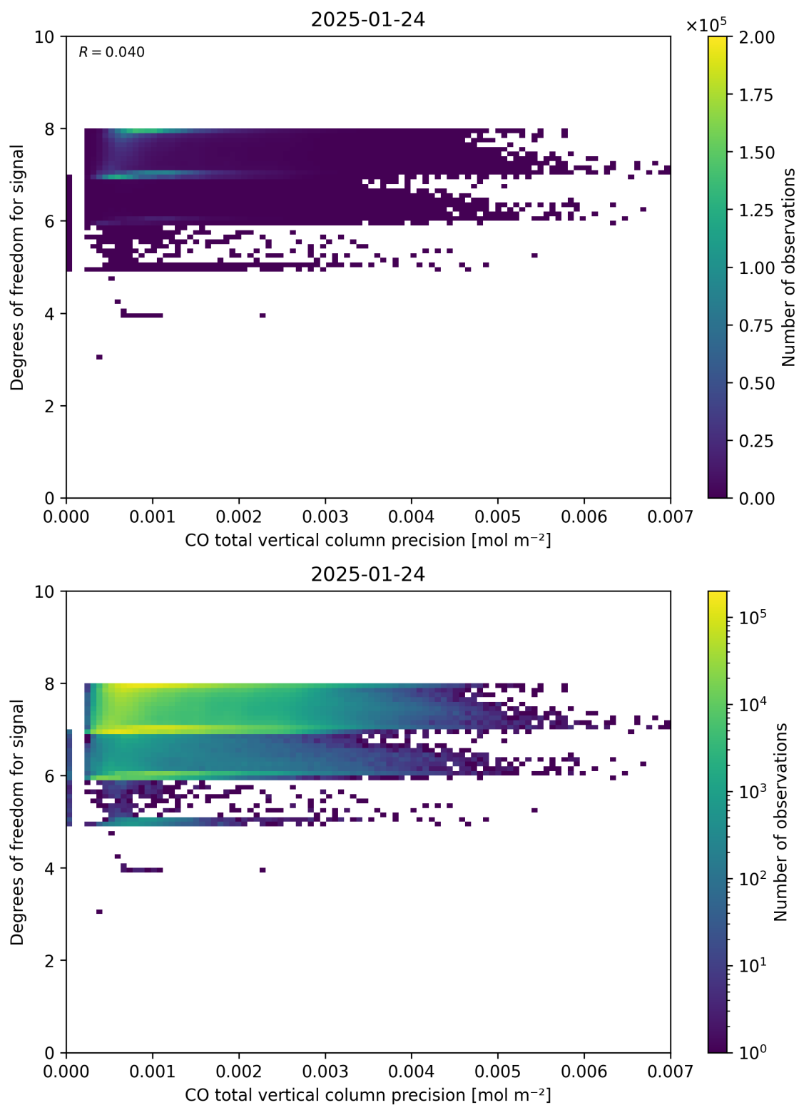
Figure 45: Scatter density plot of “CO total vertical column precision” against “Degrees of freedom for signal” for 2025-01-23 to 2025-01-25.
