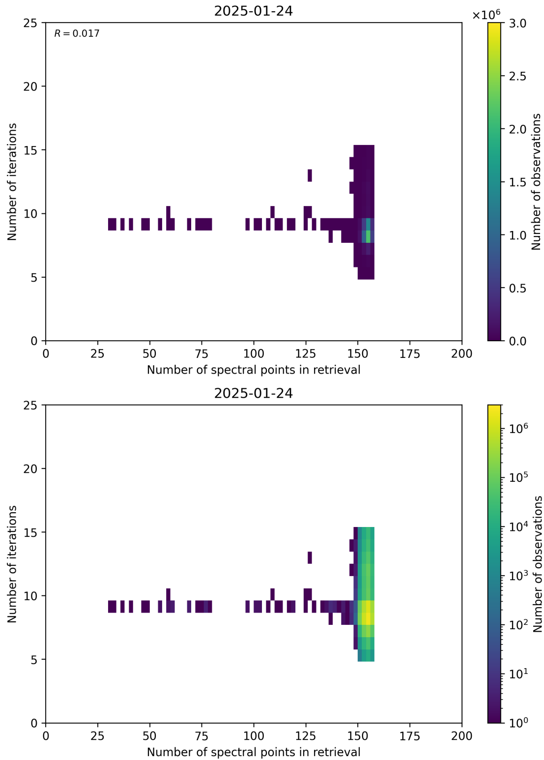
Figure 60: Scatter density plot of “Number of spectral points in retrieval” against “Number of iterations” for 2025-01-23 to 2025-01-25.
