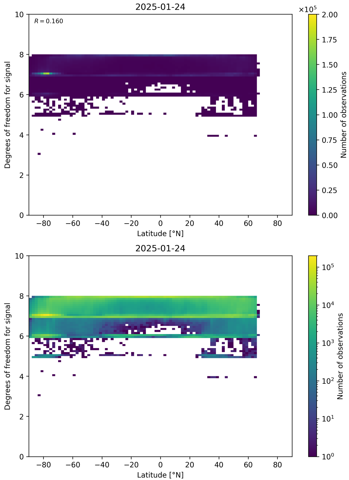
Figure 55: Scatter density plot of “Latitude” against “Degrees of freedom for signal” for 2025-01-23 to 2025-01-25.
