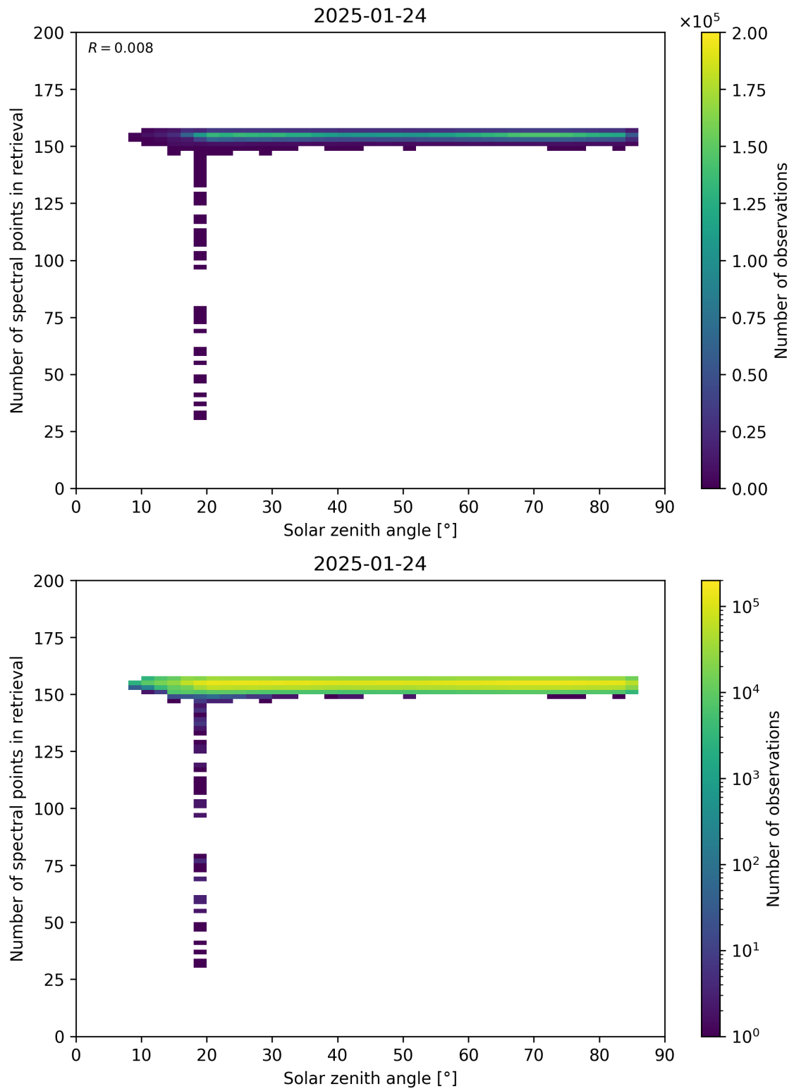
Figure 68: Scatter density plot of “Solar zenith angle” against “Number of spectral points in retrieval” for 2025-01-23 to 2025-01-25.
