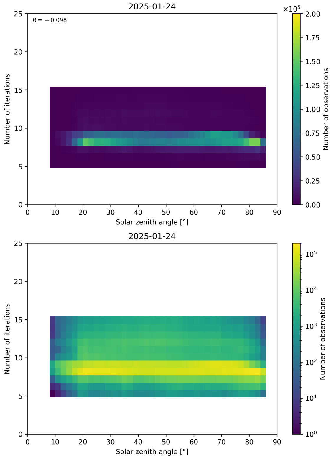
Figure 67: Scatter density plot of “Solar zenith angle” against “Number of iterations” for 2025-01-23 to 2025-01-25.
