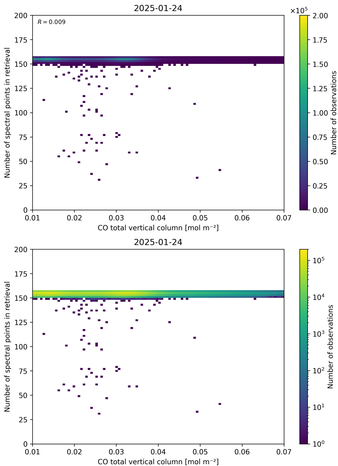
Figure 43: Scatter density plot of “CO total vertical column” against “Number of spectral points in retrieval” for 2025-01-23 to 2025-01-25.
