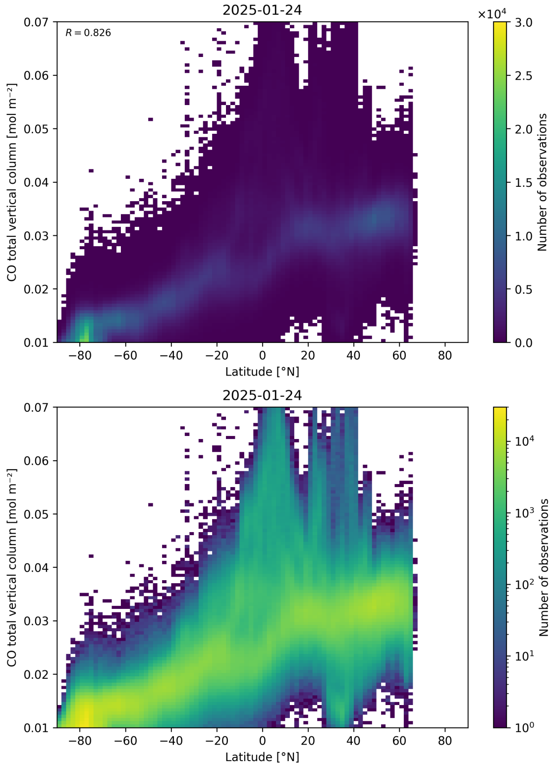
Figure 51: Scatter density plot of “Latitude” against “CO total vertical column” for 2025-01-23 to 2025-01-25.
