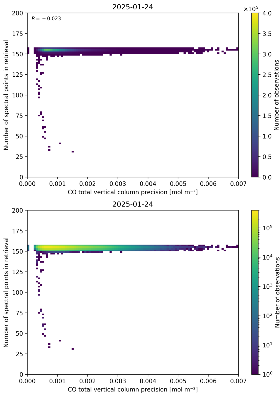
Figure 47: Scatter density plot of “CO total vertical column precision” against “Number of spectral points in retrieval” for 2025-01-23 to 2025-01-25.
