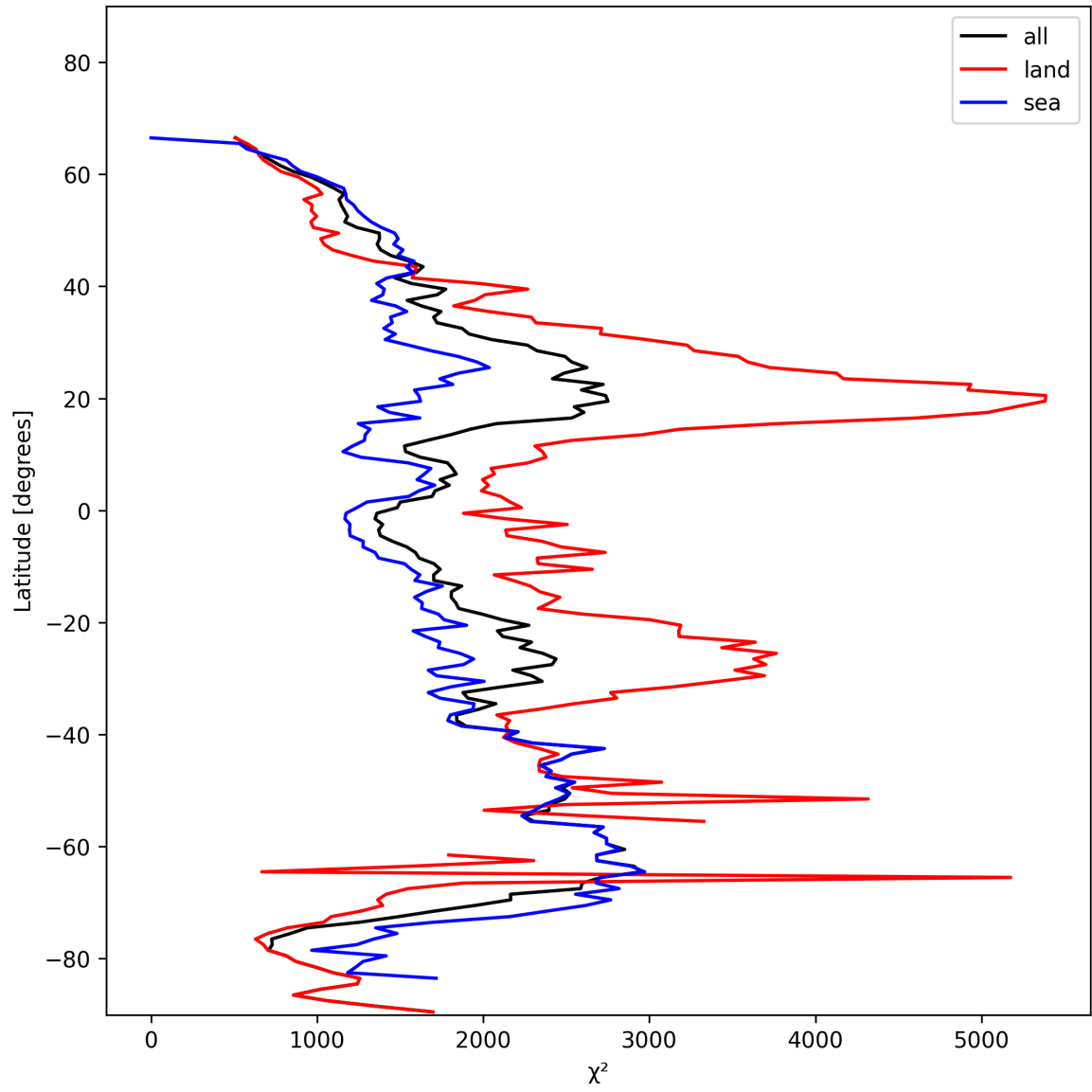
Figure 14: Zonal average of “ \chi^2 ” for 2025-01-23 to 2025-01-25.
