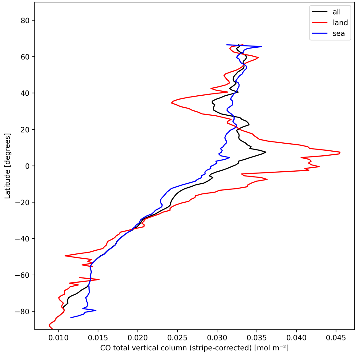
Figure 11: Zonal average of “CO total vertical column (stripe-corrected)” for 2025-01-23 to 2025-01-25.
