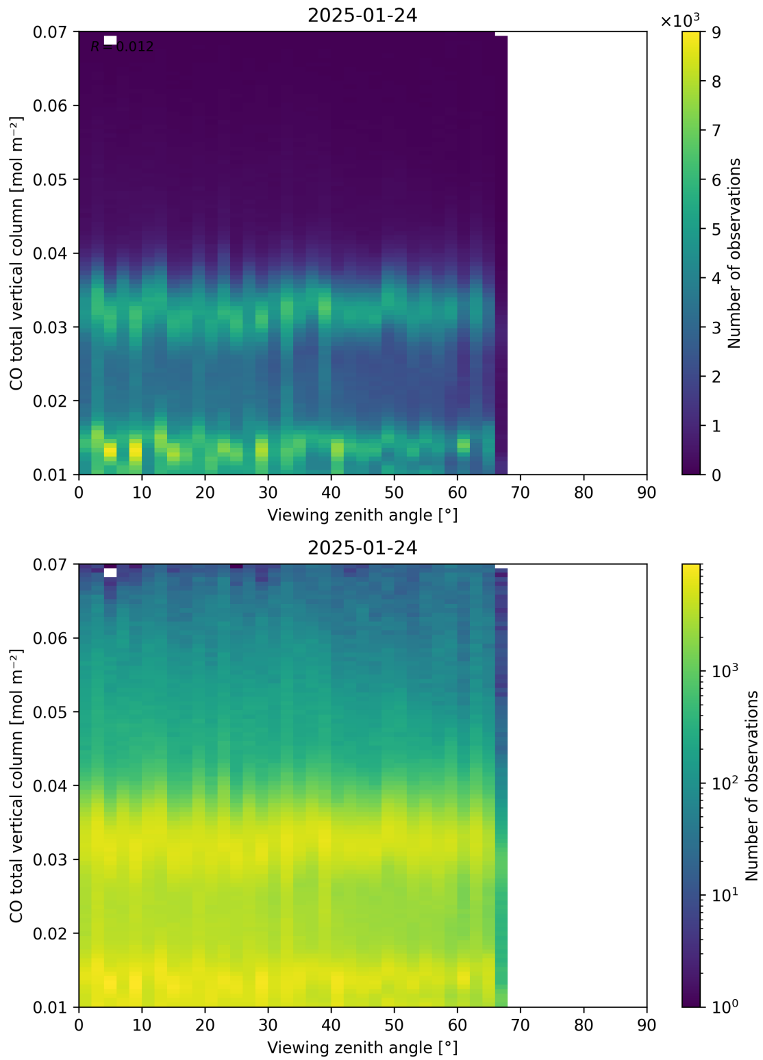
Figure 69: Scatter density plot of “Viewing zenith angle” against “CO total vertical column” for 2025-01-23 to 2025-01-25.
