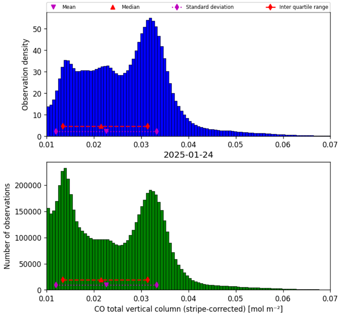
Figure 19: Histogram of “CO total vertical column (stripe-corrected)” for 2025-01-23 to 2025-01-25
