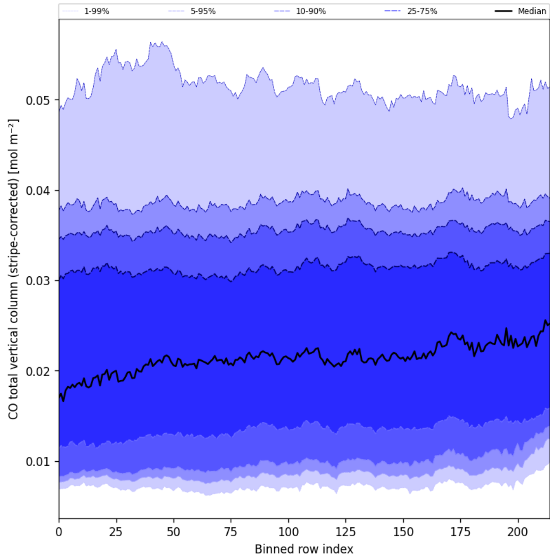
Figure 27: Along track statistics of “CO total vertical column (stripe-corrected)” for 2025-01-24 to 2025-01-26
