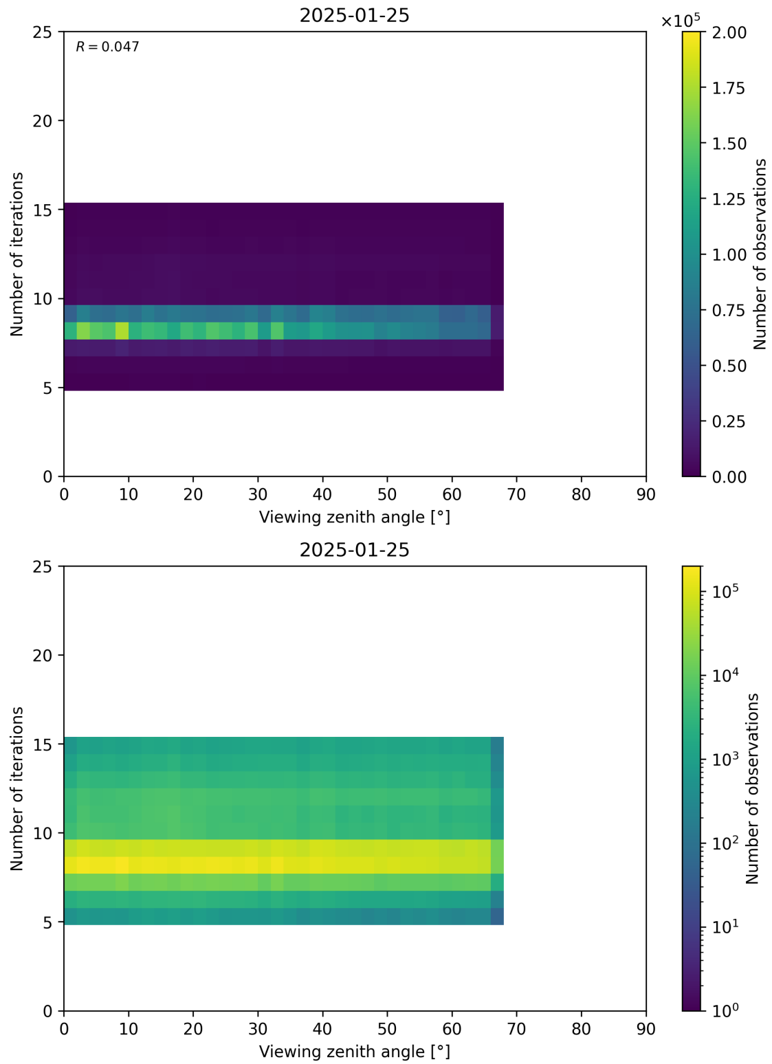
Figure 75: Scatter density plot of “Viewing zenith angle” against “Number of iterations” for 2025-01-24 to 2025-01-26.
