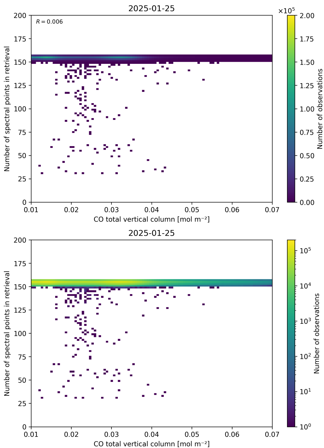
Figure 43: Scatter density plot of “CO total vertical column” against “Number of spectral points in retrieval” for 2025-01-24 to 2025-01-26.
