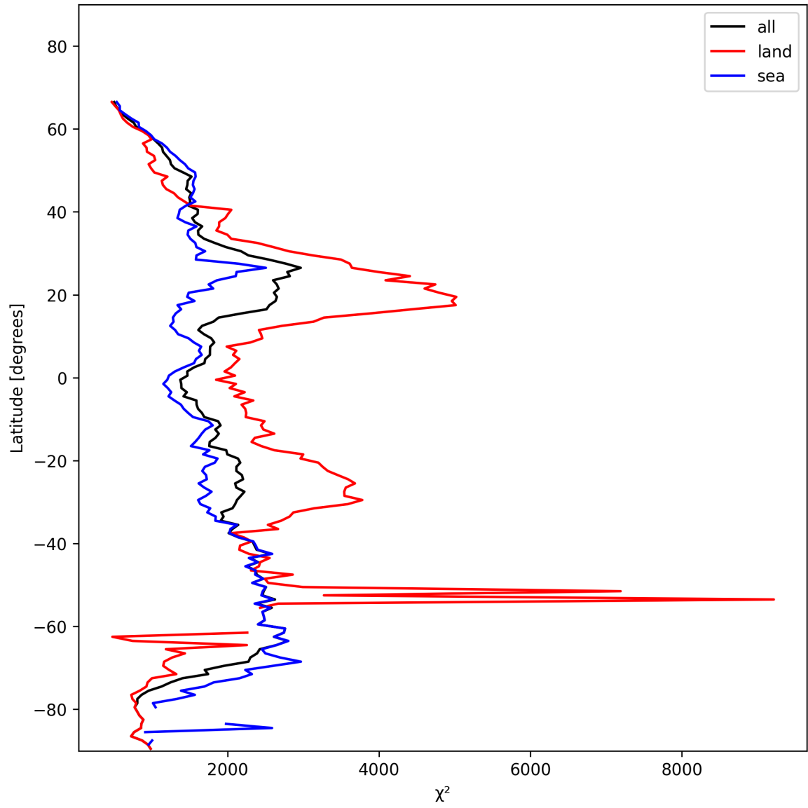
Figure 14: Zonal average of “ \chi^2 ” for 2025-01-24 to 2025-01-26.
