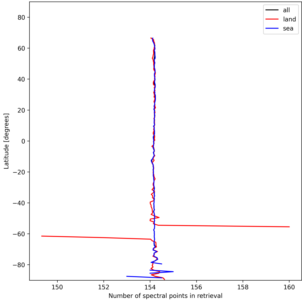
Figure 13: Zonal average of “Number of spectral points in retrieval” for 2025-01-24 to 2025-01-26.
