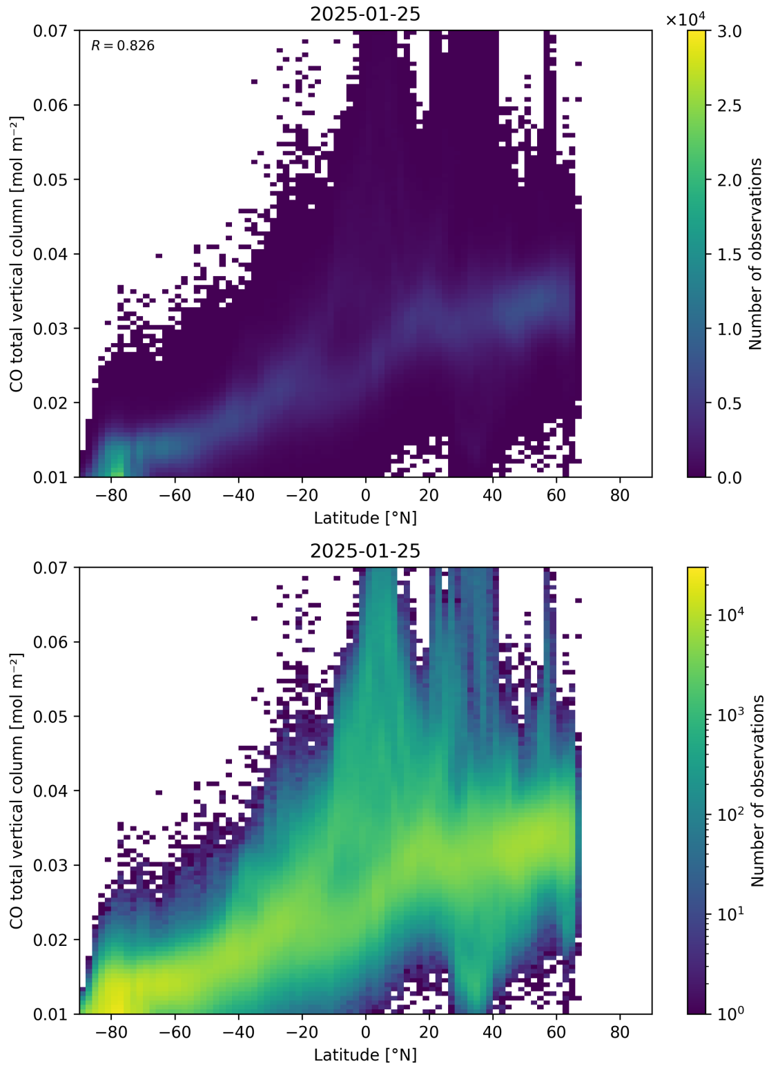
Figure 51: Scatter density plot of “Latitude” against “CO total vertical column” for 2025-01-24 to 2025-01-26.
