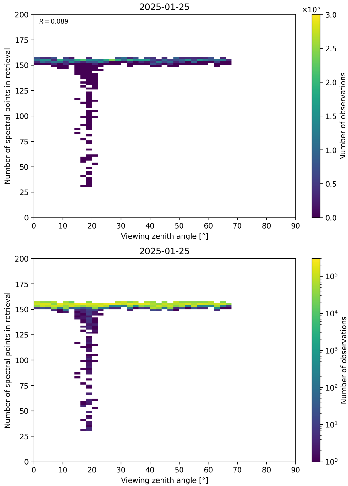
Figure 76: Scatter density plot of “Viewing zenith angle” against “Number of spectral points in retrieval” for 2025-01-24 to 2025-01-26.
