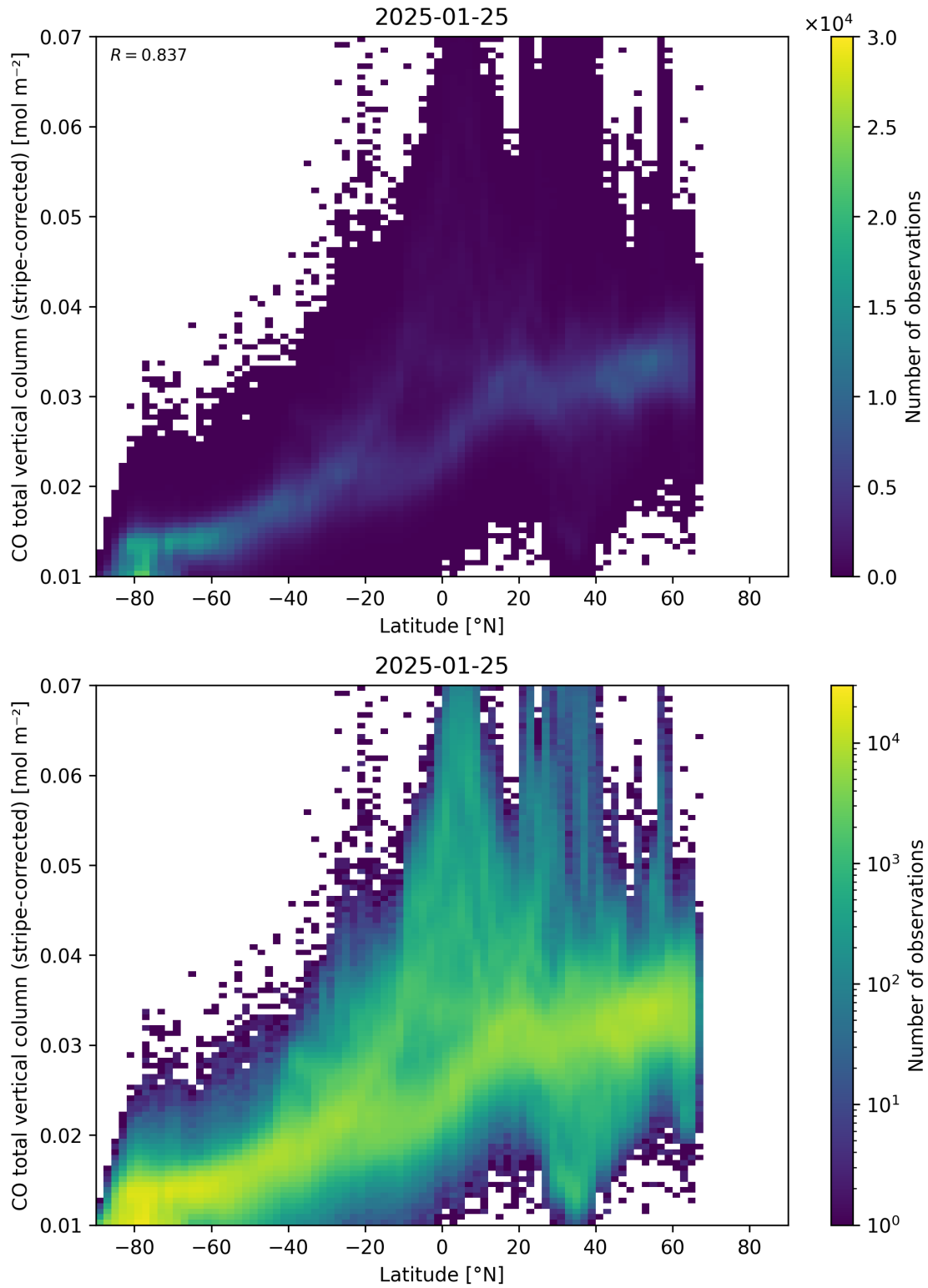
Figure 52: Scatter density plot of “Latitude” against “CO total vertical column (stripe-corrected)” for 2025-01-24 to 2025-01-26.
