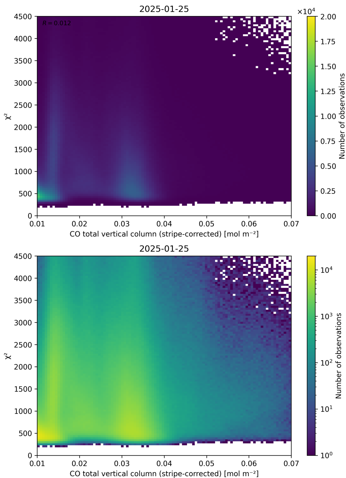
Figure 37: Scatter density plot of “CO total vertical column (stripe-corrected)” against “ \chi^2 ” for 2025-01-24 to 2025-01-26.
