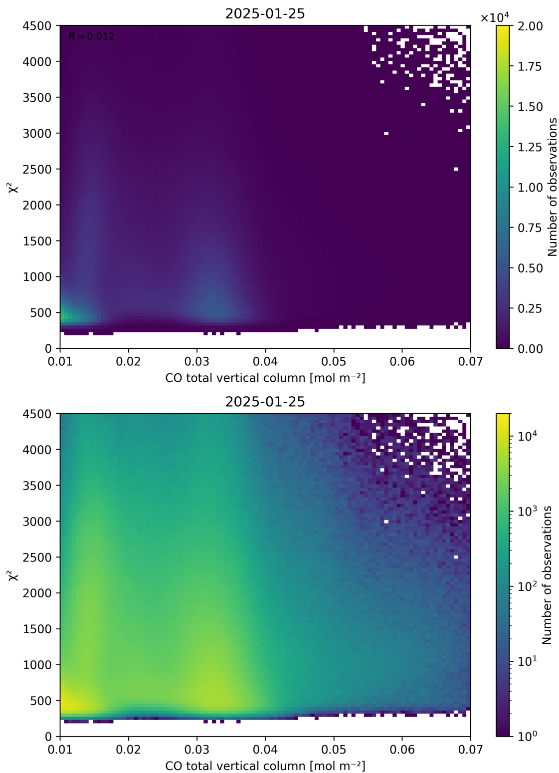
Figure 35: Scatter density plot of “CO total vertical column” against “ \chi^2 ” for 2025-01-24 to 2025-01-26.
