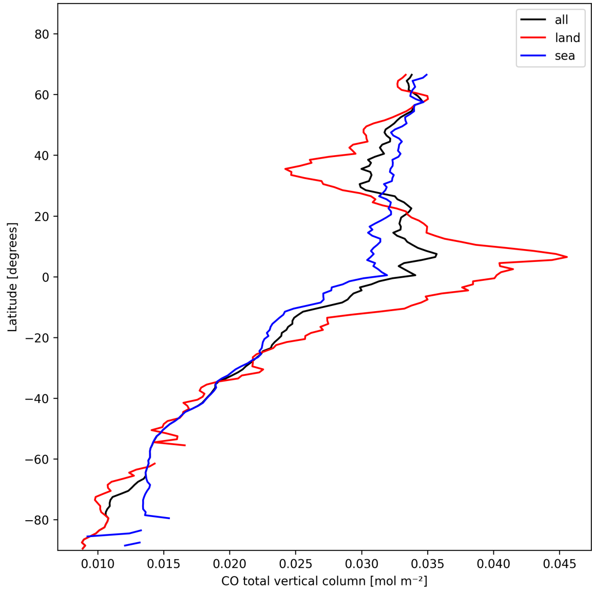
Figure 10: Zonal average of “CO total vertical column” for 2025-01-24 to 2025-01-26.
