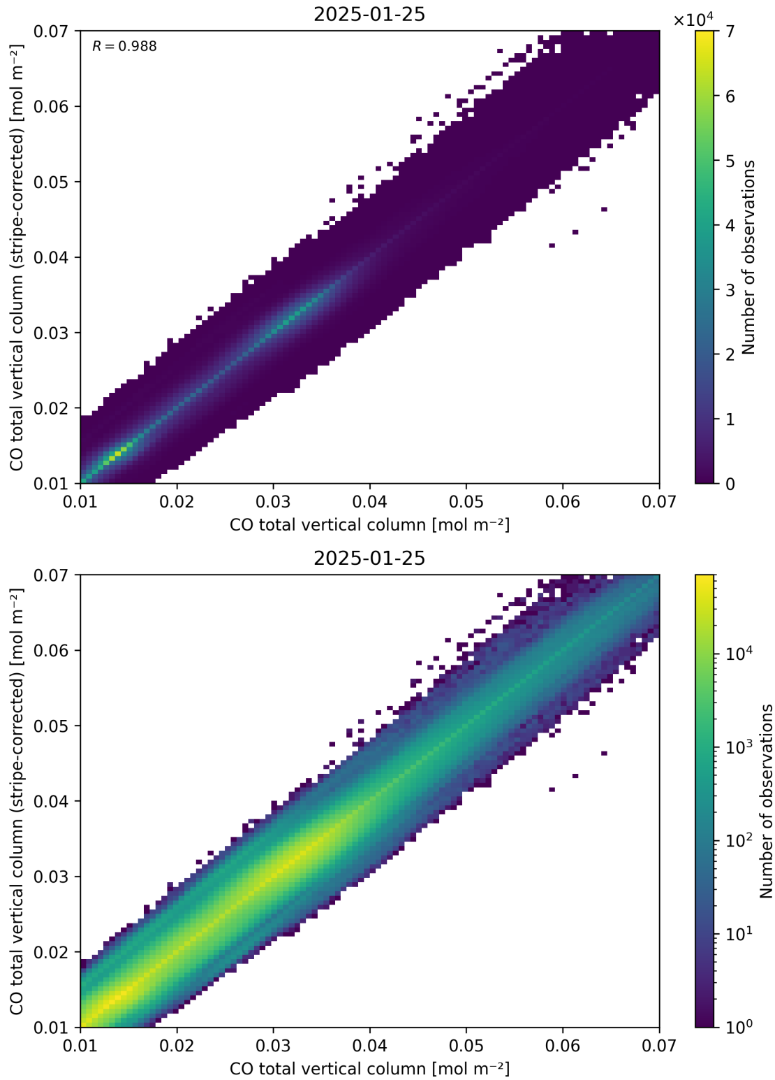
Figure 33: Scatter density plot of “CO total vertical column” against “CO total vertical column (stripe-corrected)” for 2025-01-24 to 2025-01-26.
