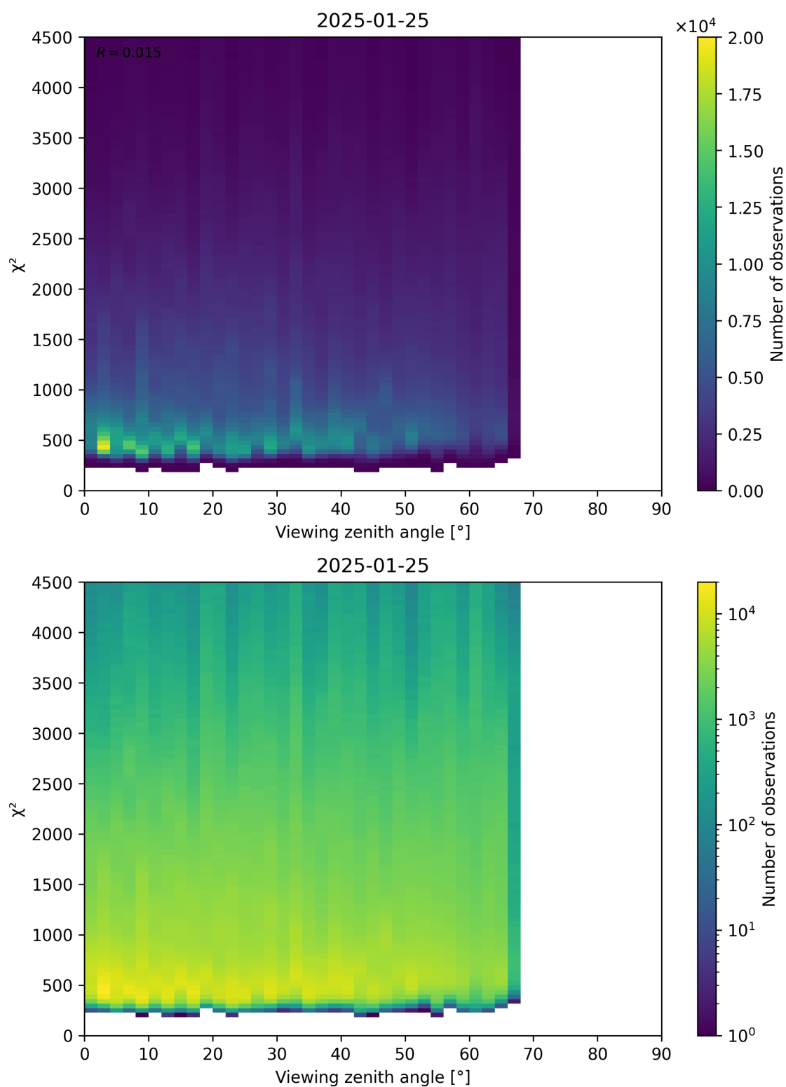
Figure 72: Scatter density plot of “Viewing zenith angle” against “ \chi^2 ” for 2025-01-24 to 2025-01-26.
