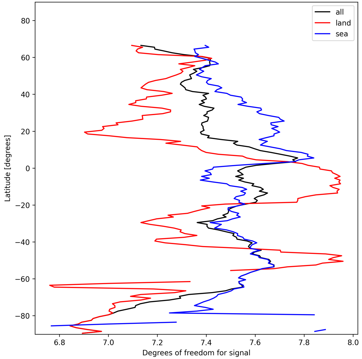
Figure 15: Zonal average of “Degrees of freedom for signal” for 2025-01-24 to 2025-01-26.
