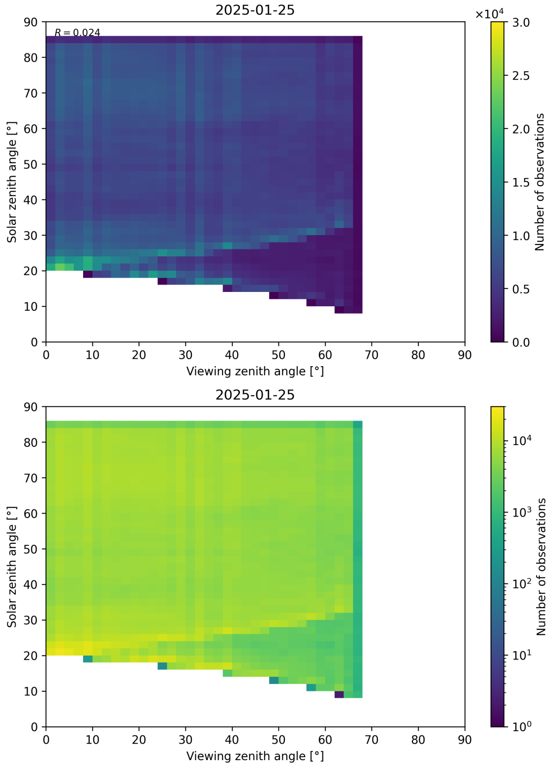
Figure 77: Scatter density plot of “Viewing zenith angle” against “Solar zenith angle” for 2025-01-24 to 2025-01-26.
