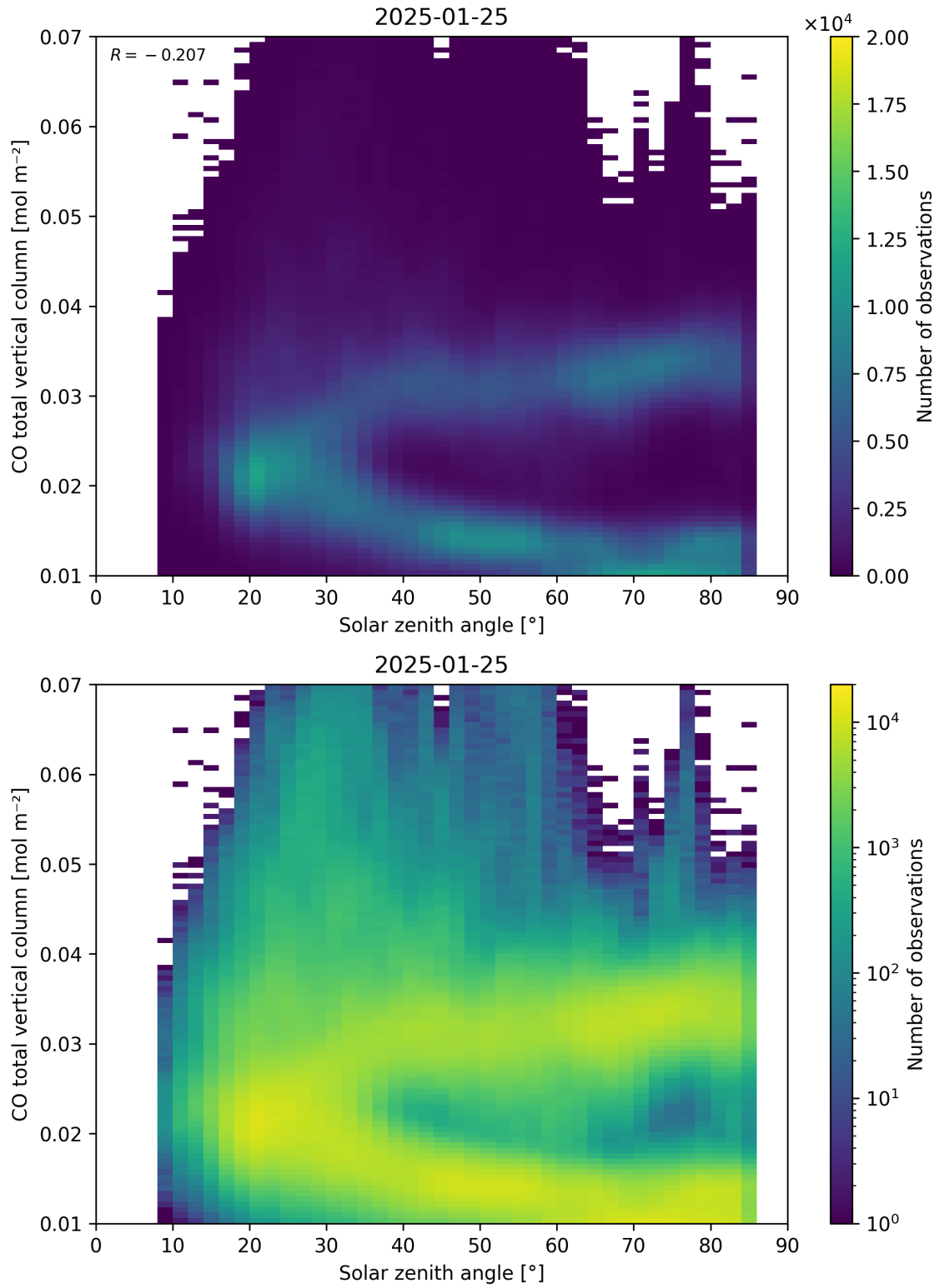
Figure 61: Scatter density plot of “Solar zenith angle” against “CO total vertical column” for 2025-01-24 to 2025-01-26.
