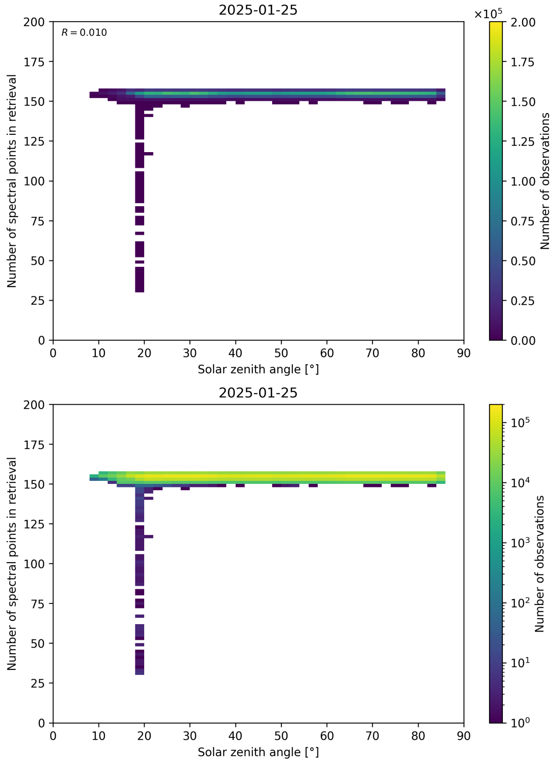
Figure 68: Scatter density plot of “Solar zenith angle” against “Number of spectral points in retrieval” for 2025-01-24 to 2025-01-26.
