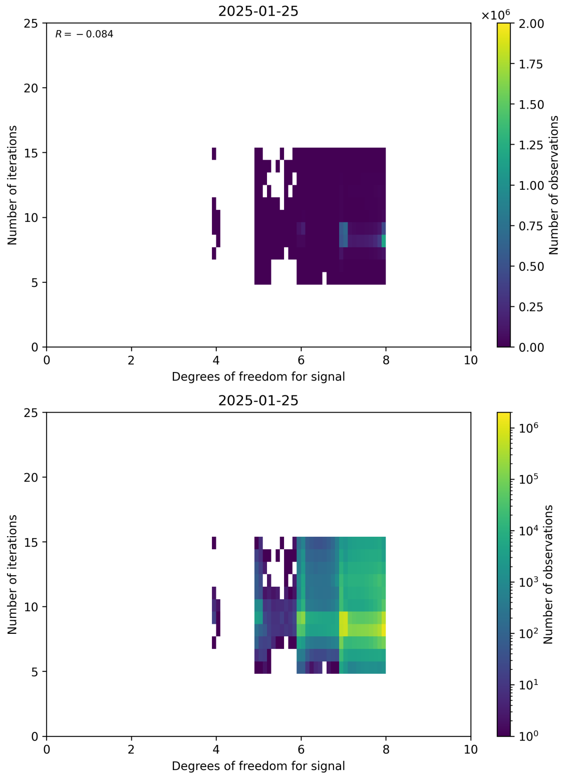
Figure 50: Scatter density plot of “Degrees of freedom for signal” against “Number of iterations” for 2025-01-24 to 2025-01-26.
