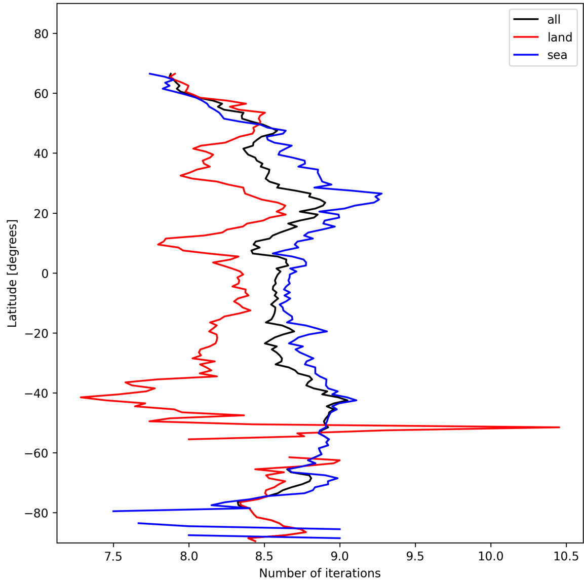
Figure 16: Zonal average of “Number of iterations” for 2025-01-24 to 2025-01-26.
