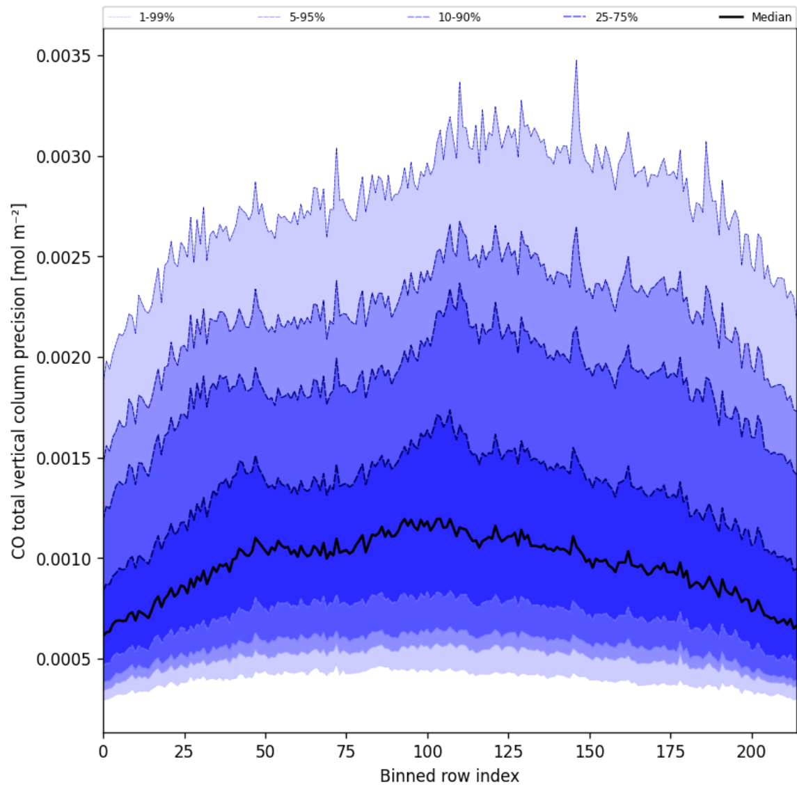
Figure 28: Along track statistics of “CO total vertical column precision” for 2025-01-24 to 2025-01-26
