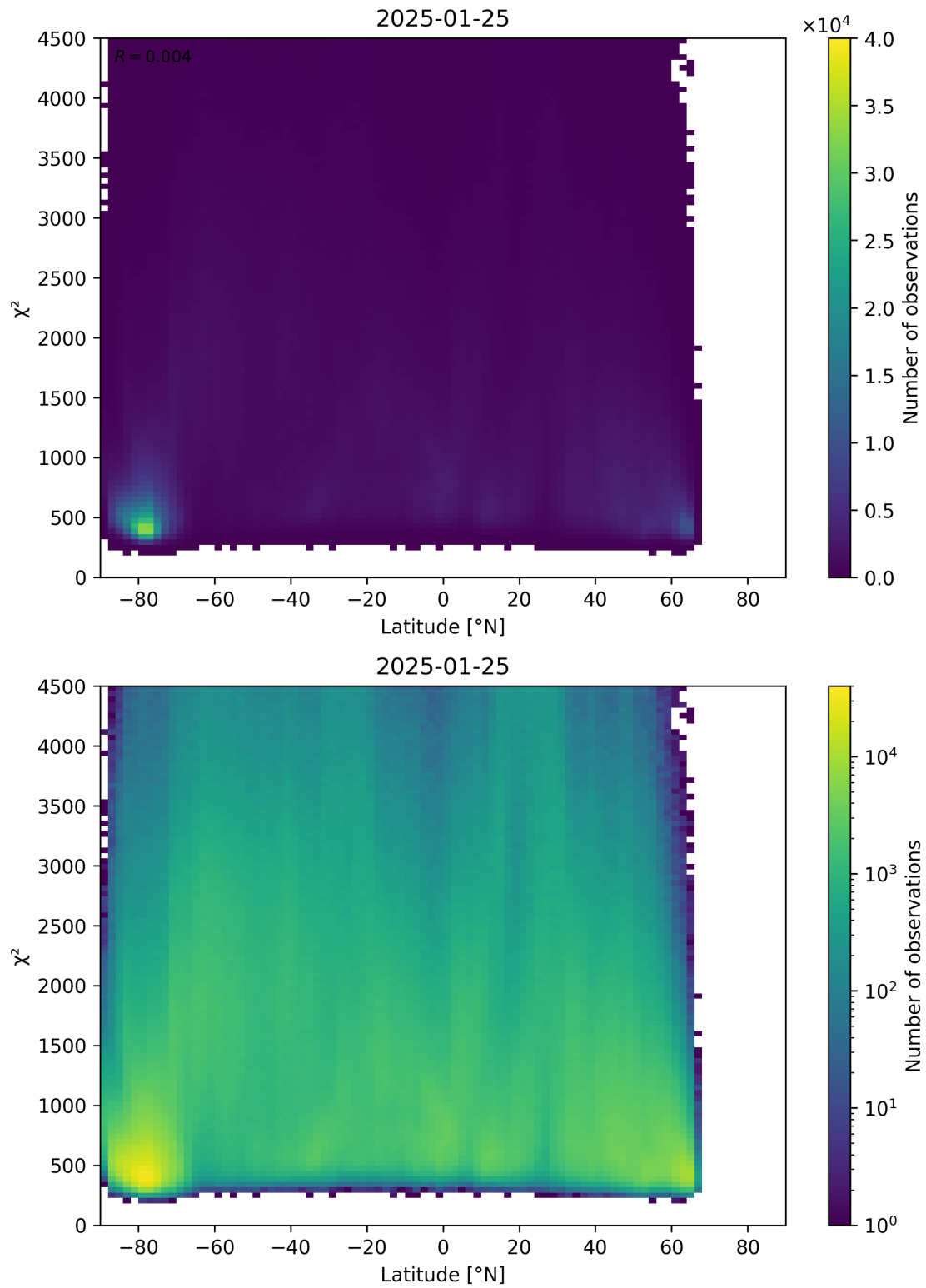
Figure 54: Scatter density plot of “Latitude” against “ \chi^2 ” for 2025-01-24 to 2025-01-26.
