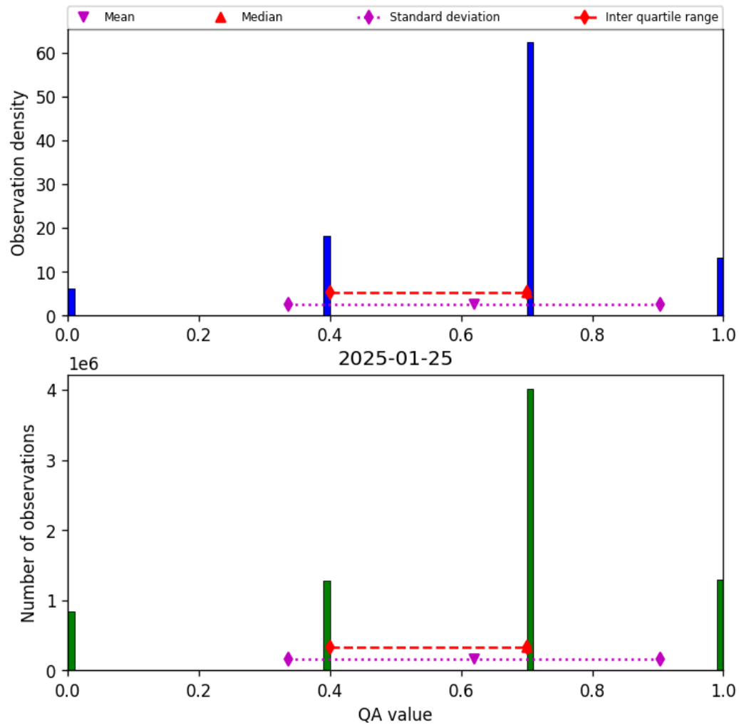
Figure 17: Histogram of “QA value” for 2025-01-24 to 2025-01-26
