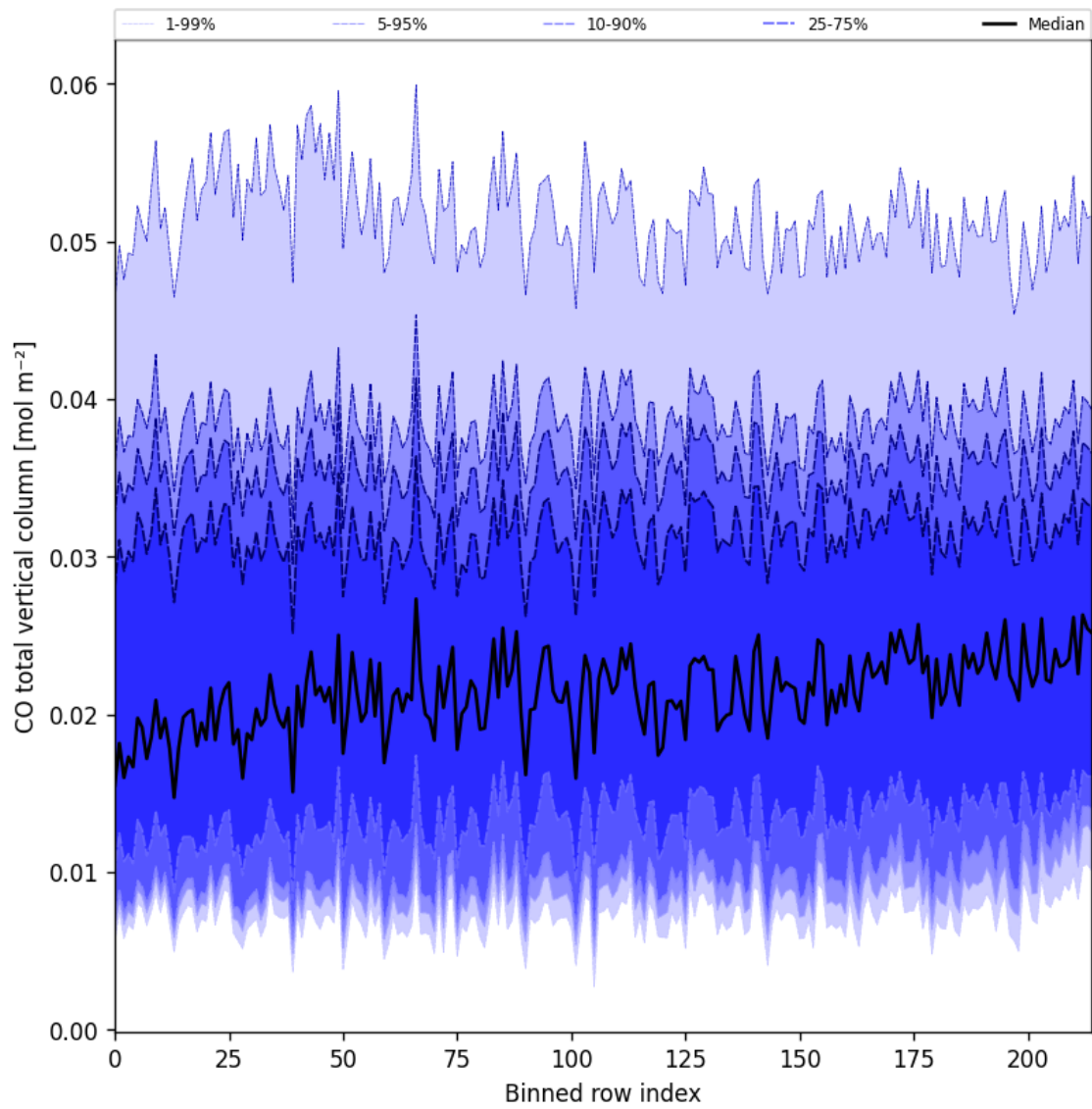
Figure 26: Along track statistics of “CO total vertical column” for 2025-01-24 to 2025-01-26
