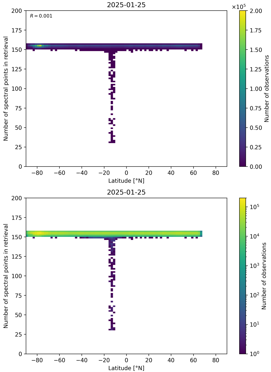
Figure 57: Scatter density plot of “Latitude” against “Number of spectral points in retrieval” for 2025-01-24 to 2025-01-26.
