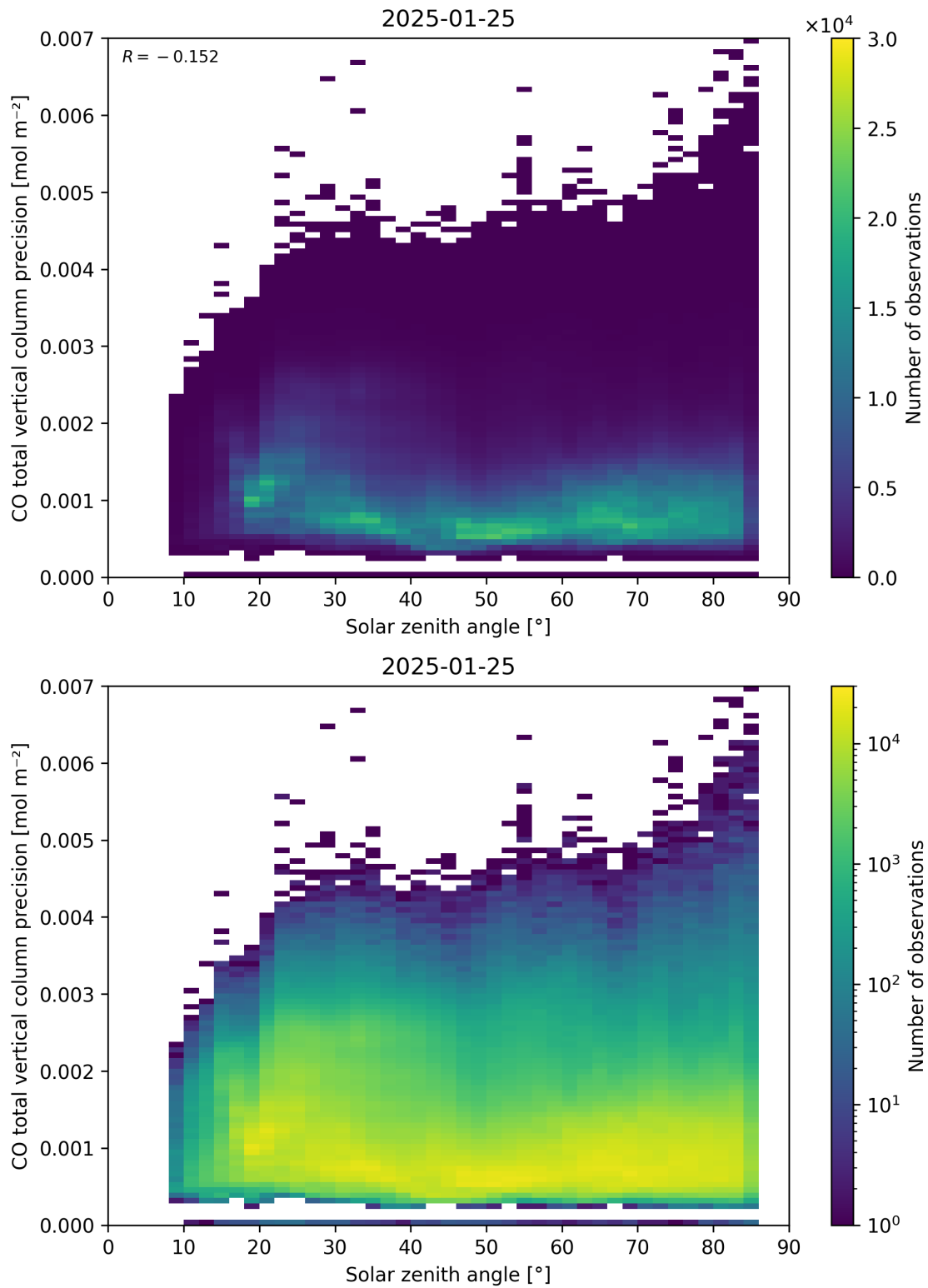
Figure 63: Scatter density plot of “Solar zenith angle” against “CO total vertical column precision” for 2025-01-24 to 2025-01-26.
