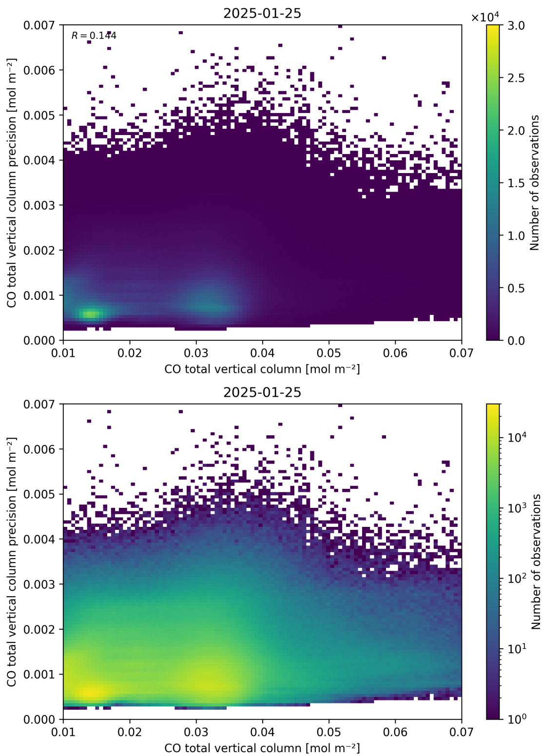
Figure 34: Scatter density plot of “CO total vertical column” against “CO total vertical column precision” for 2025-01-24 to 2025-01-26.
