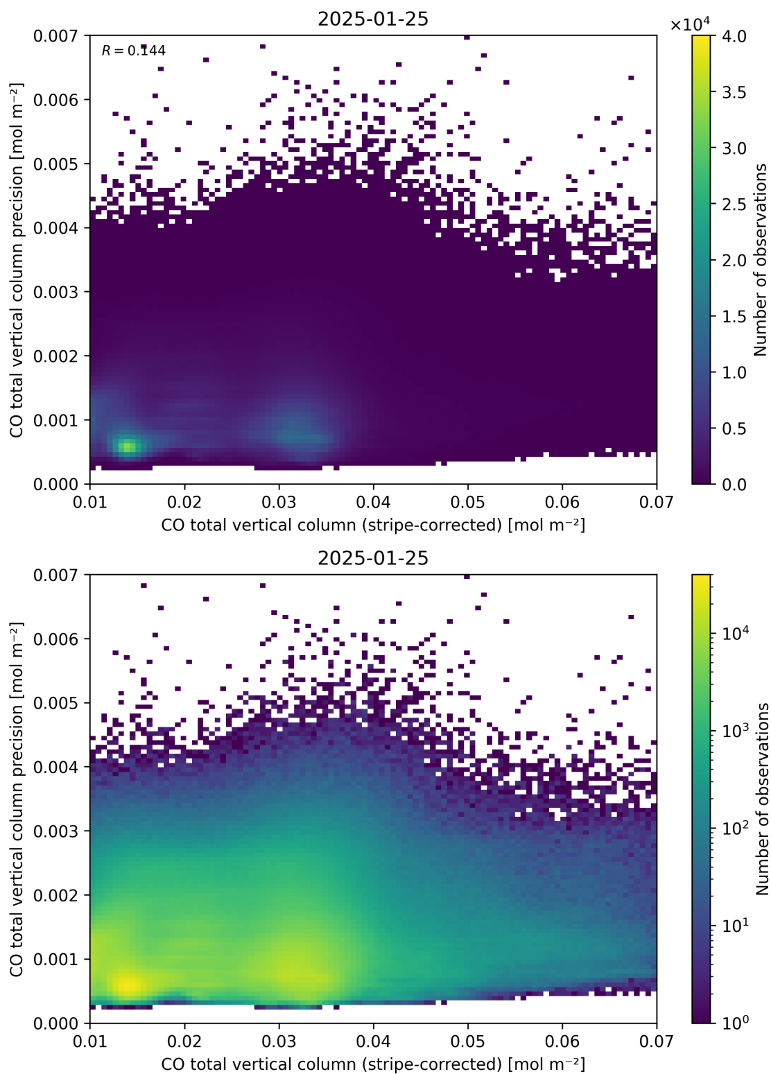
Figure 36: Scatter density plot of “CO total vertical column (stripe-corrected)” against “CO total vertical column precision” for 2025-01-24 to 2025-01-26.
