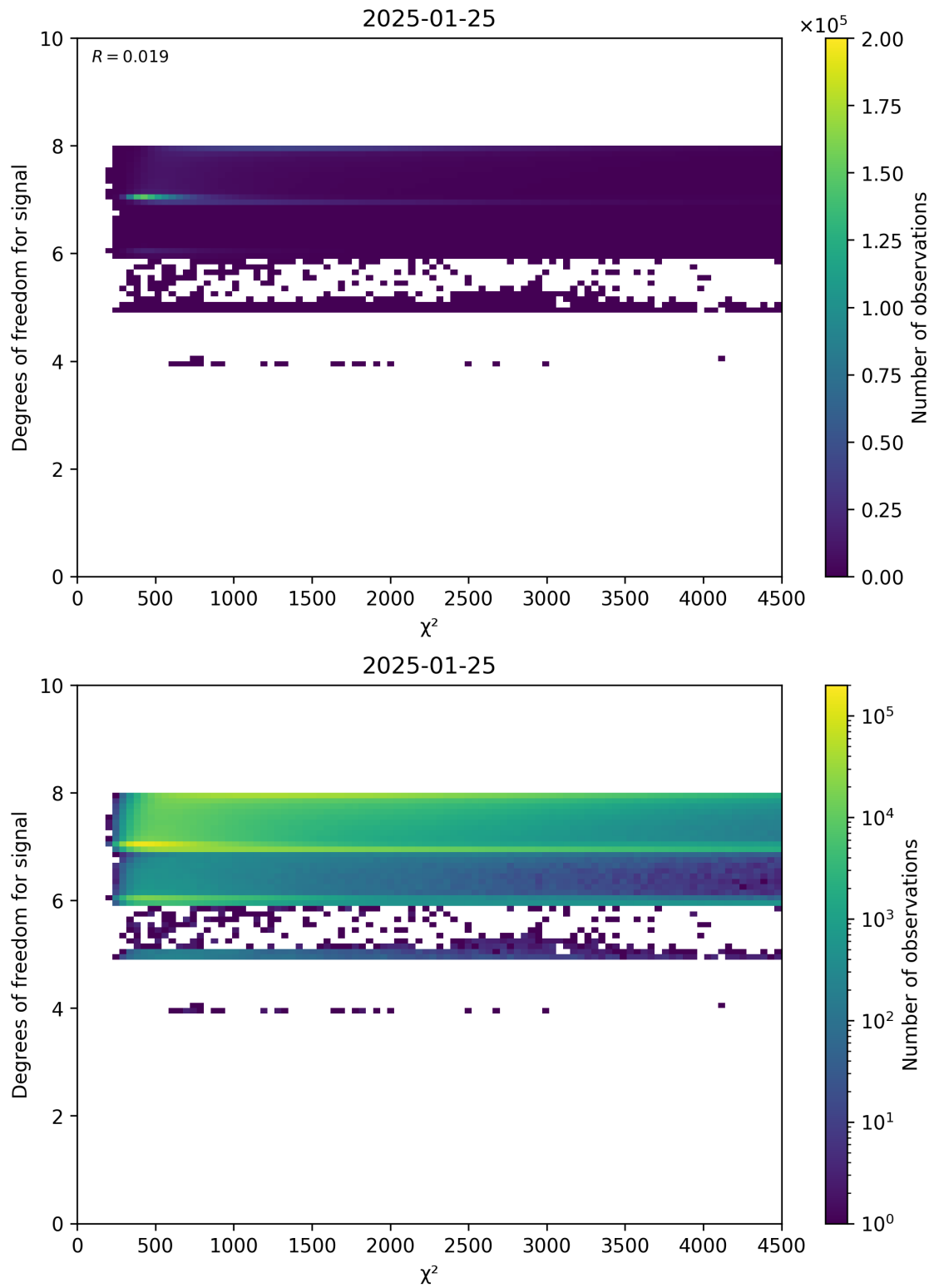
Figure 48: Scatter density plot of “ \chi^2 ” against “Degrees of freedom for signal” for 2025-01-24 to 2025-01-26.
