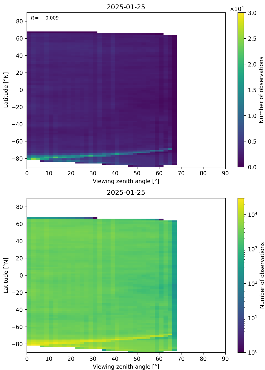
Figure 74: Scatter density plot of “Viewing zenith angle” against “Latitude” for 2025-01-24 to 2025-01-26.
