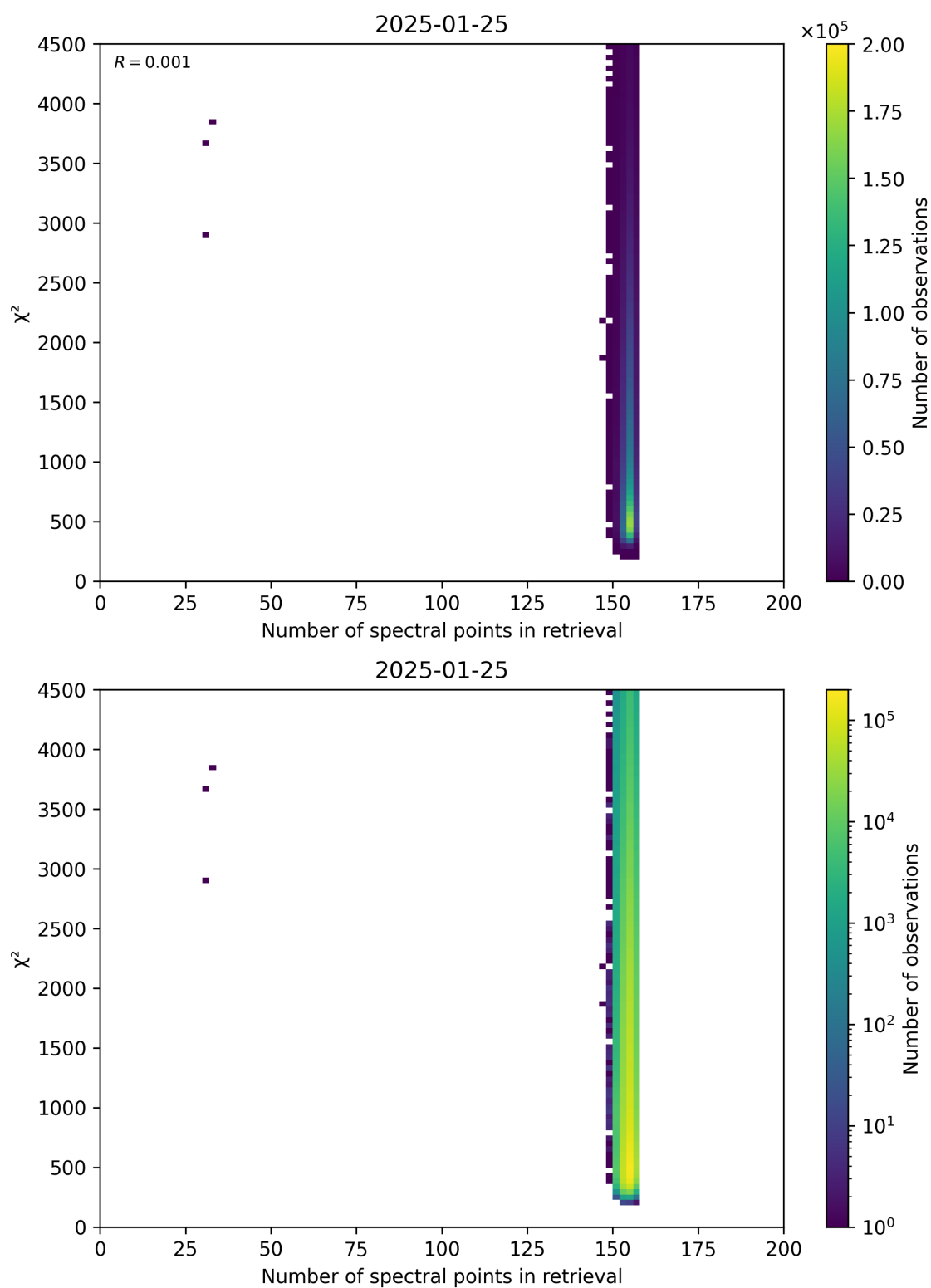
Figure 58: Scatter density plot of “Number of spectral points in retrieval” against “ \chi^2 ” for 2025-01-24 to 2025-01-26.
