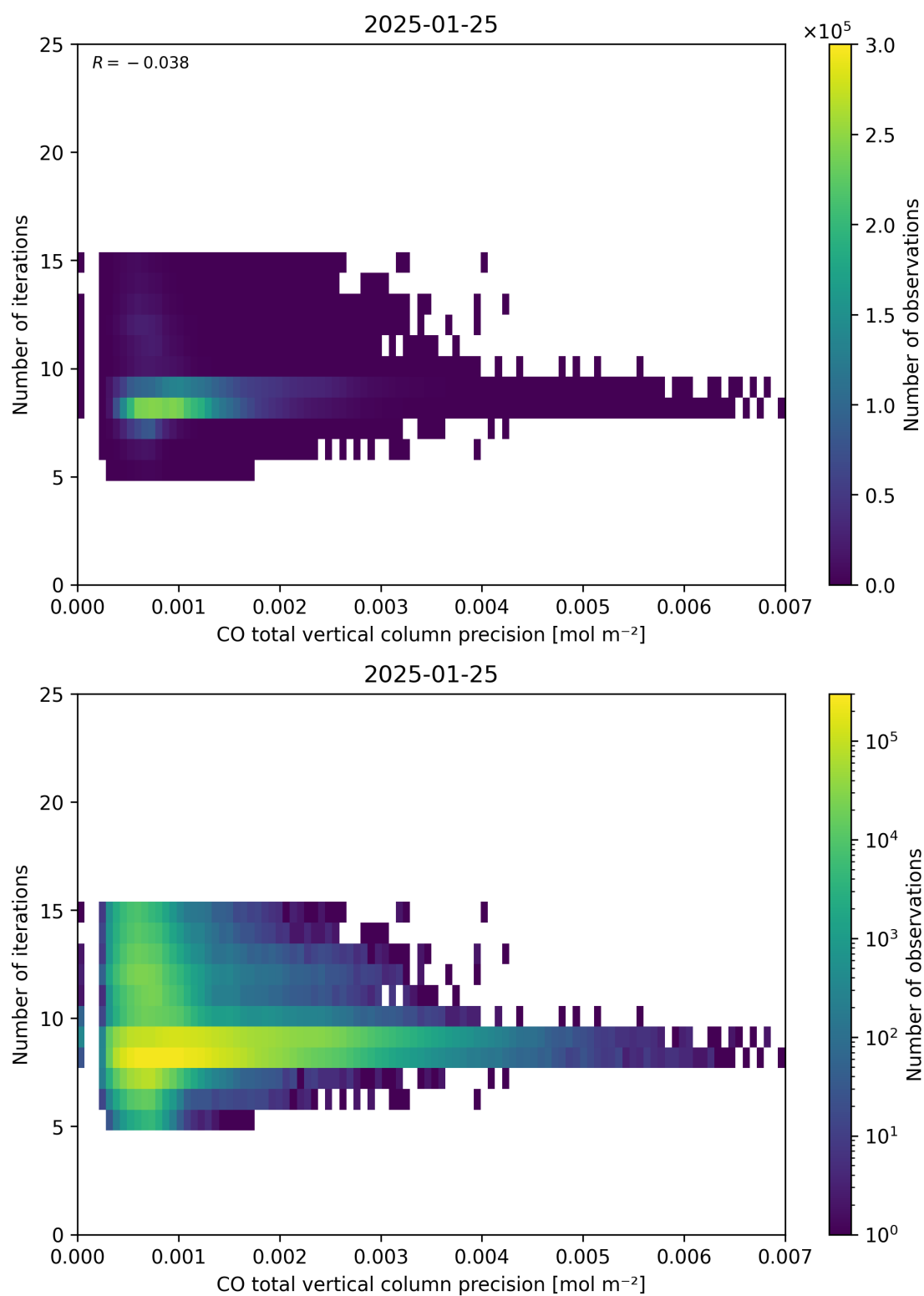
Figure 46: Scatter density plot of “CO total vertical column precision” against “Number of iterations” for 2025-01-24 to 2025-01-26.
