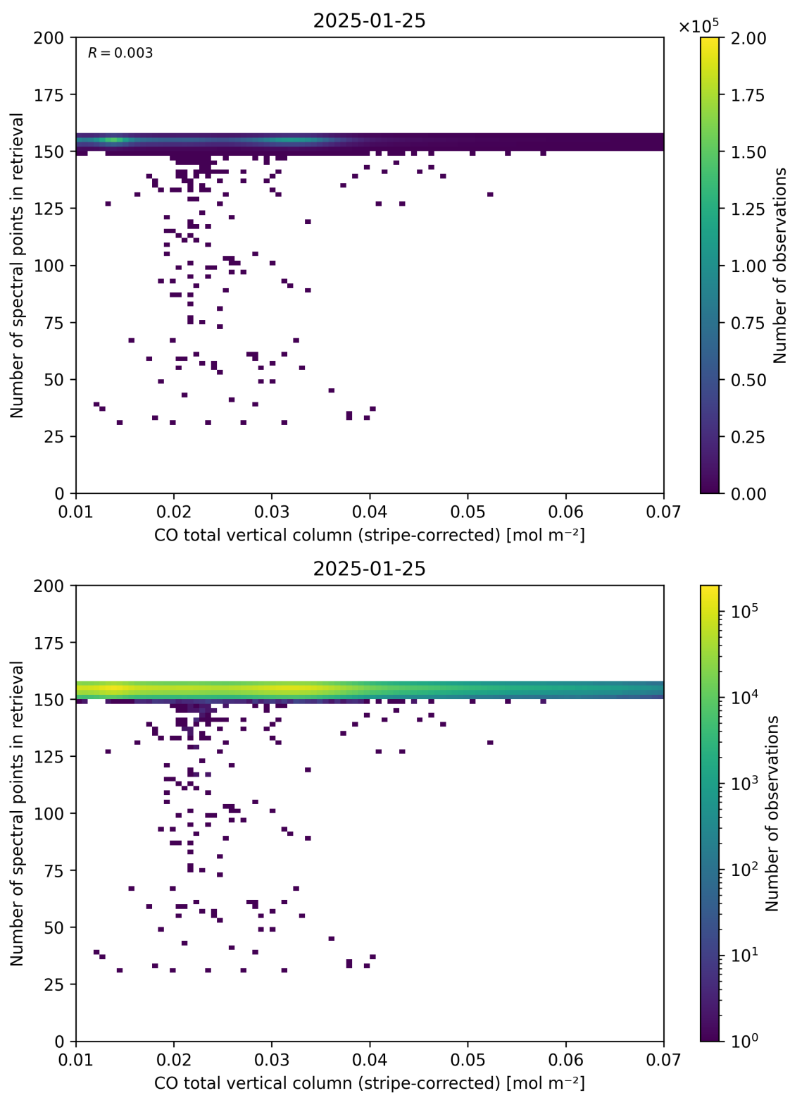
Figure 40: Scatter density plot of “CO total vertical column (stripe-corrected)” against “Number of spectral points in retrieval” for 2025-01-24 to 2025-01-26.
