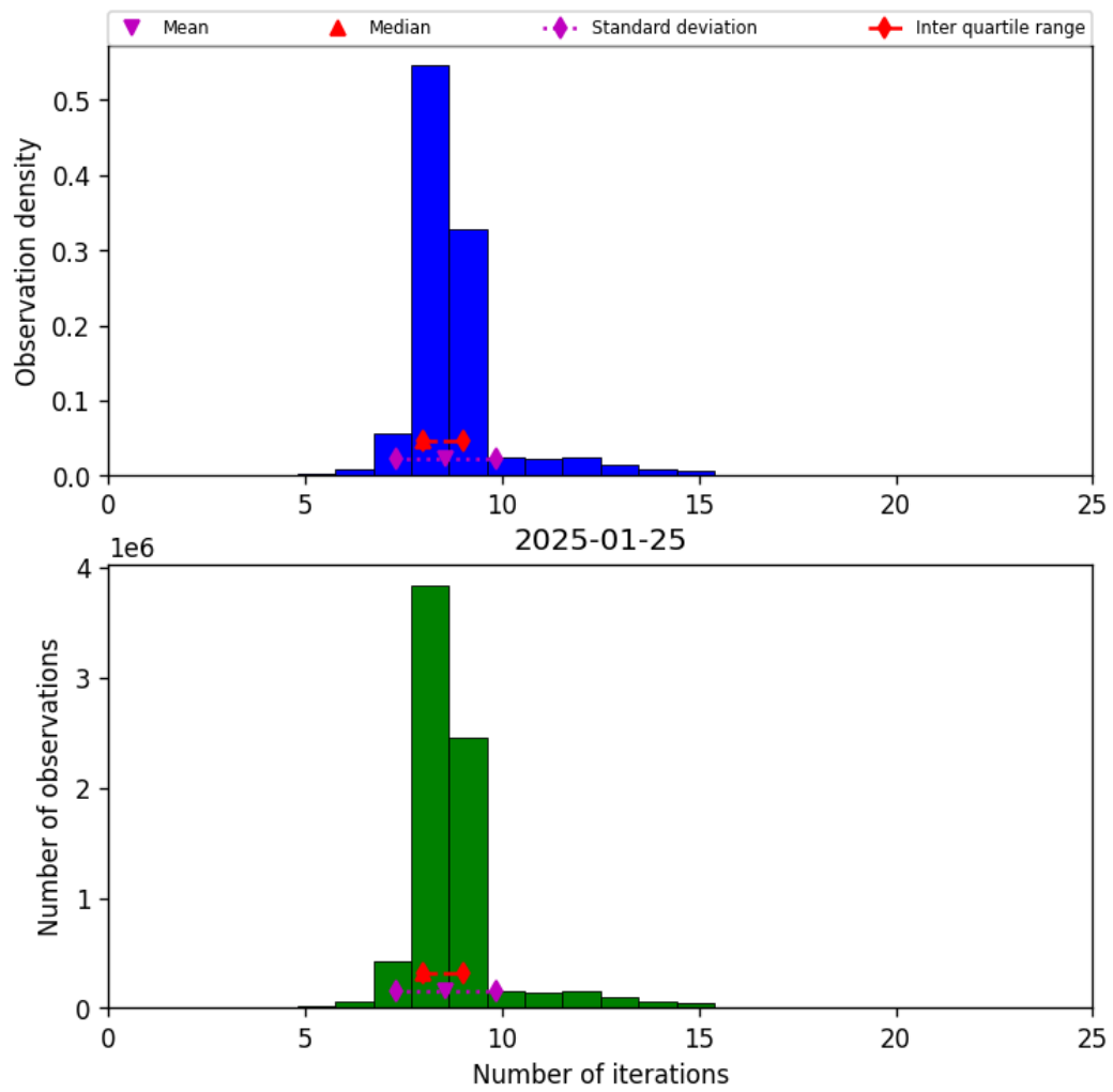
Figure 24: Histogram of “Number of iterations” for 2025-01-24 to 2025-01-26
