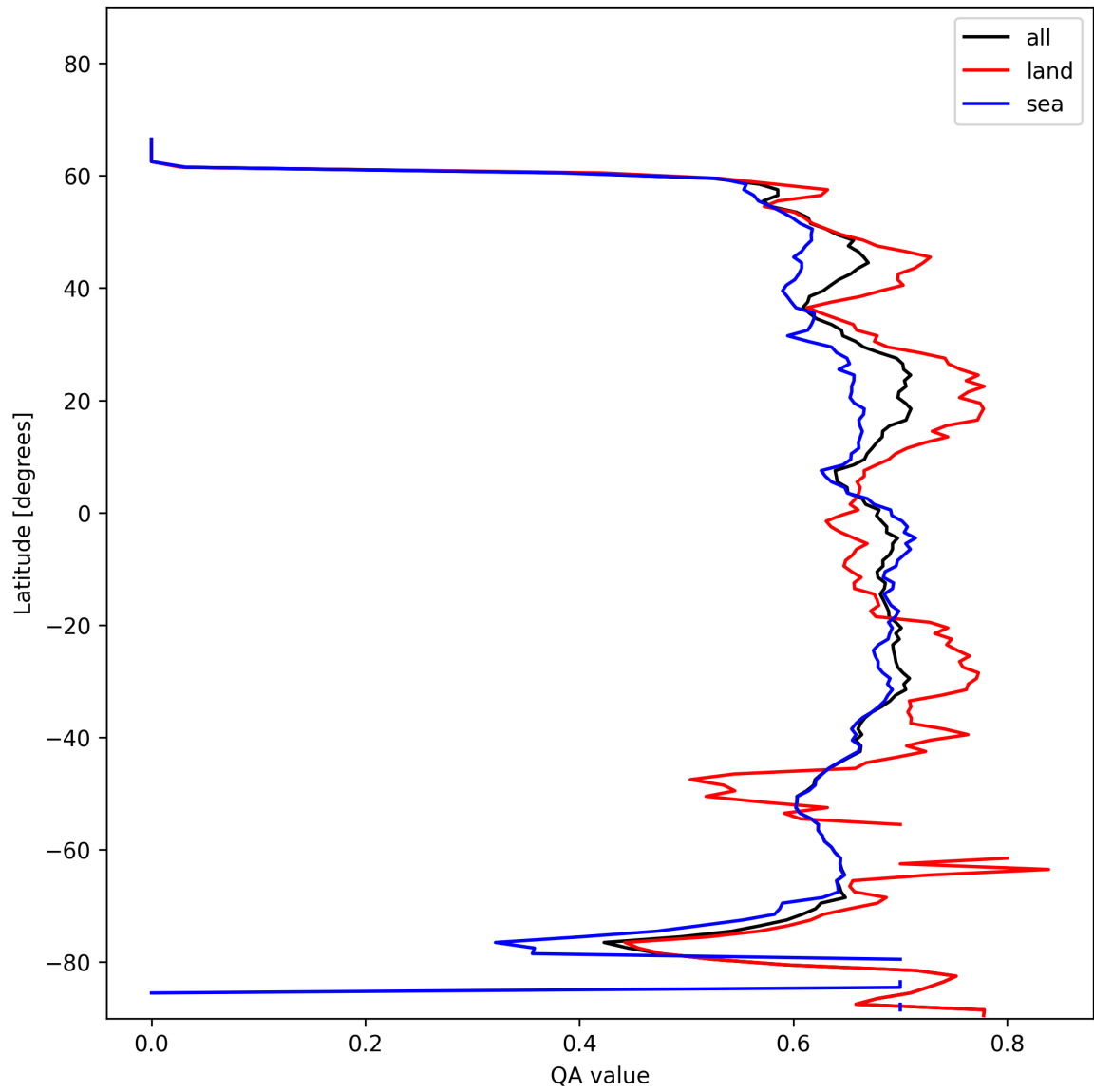
Figure 9: Zonal average of “QA value” for 2025-01-24 to 2025-01-26.
