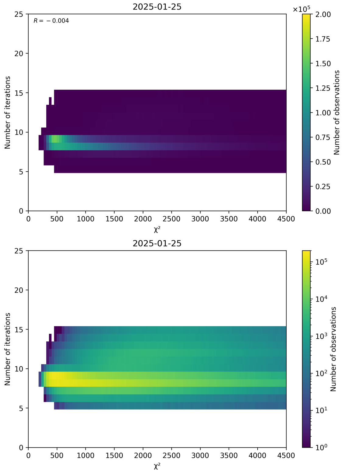
Figure 49: Scatter density plot of “ \chi^2 ” against “Number of iterations” for 2025-01-24 to 2025-01-26.
