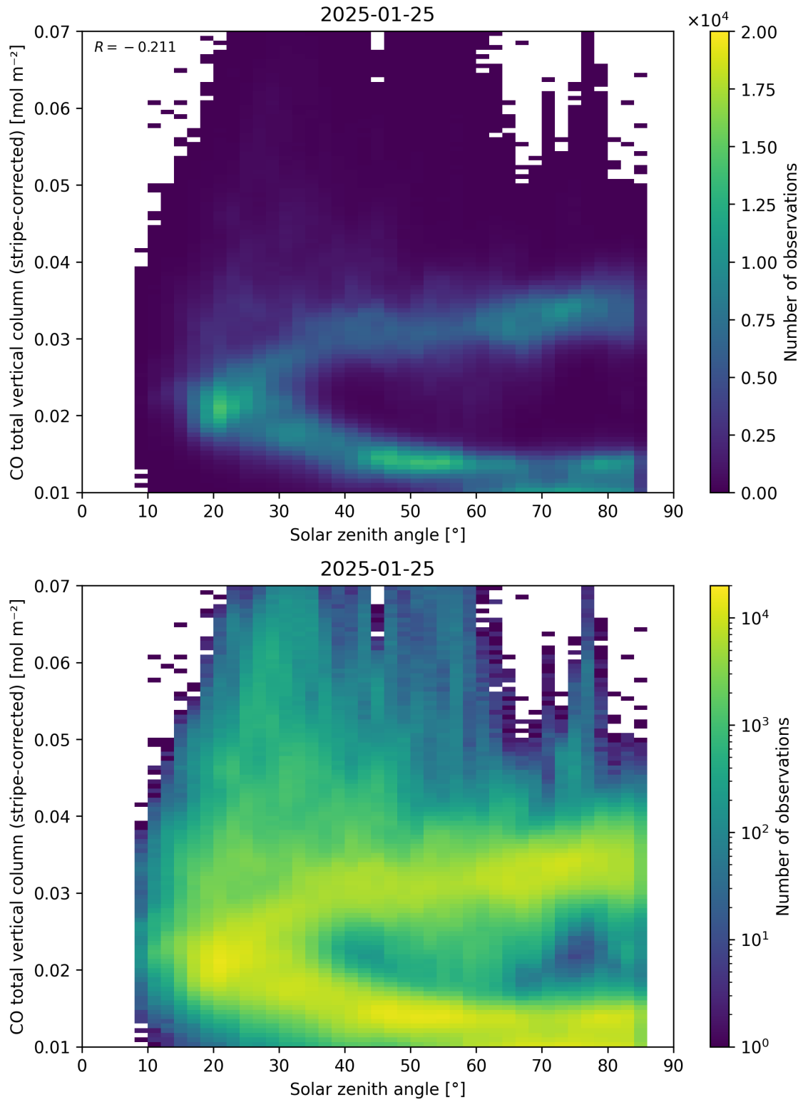
Figure 62: Scatter density plot of “Solar zenith angle” against “CO total vertical column (stripe-corrected)” for 2025-01-24 to 2025-01-26.
