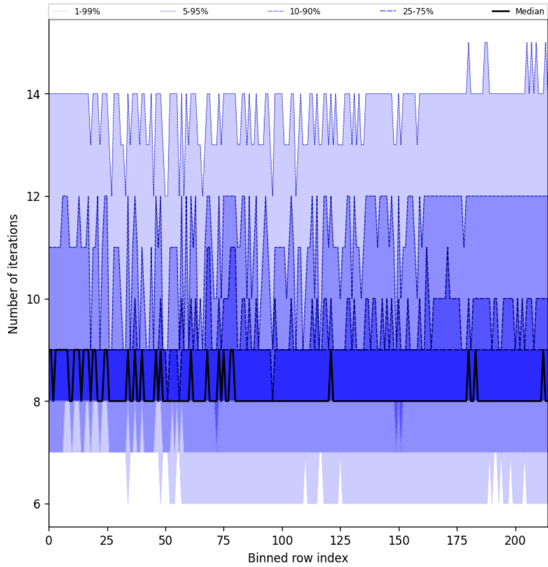
Figure 32: Along track statistics of “Number of iterations” for 2025-01-24 to 2025-01-26
