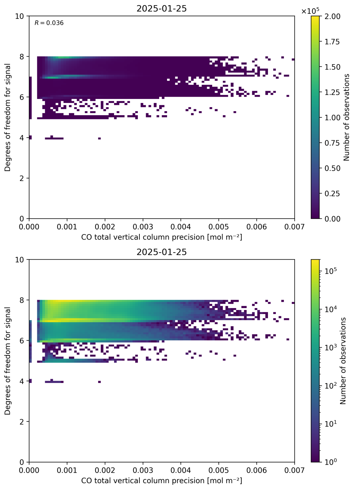
Figure 45: Scatter density plot of “CO total vertical column precision” against “Degrees of freedom for signal” for 2025-01-24 to 2025-01-26.
