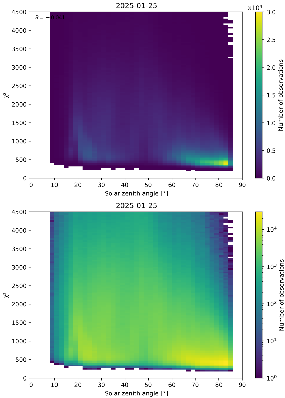
Figure 64: Scatter density plot of “Solar zenith angle” against “ \chi^2 ” for 2025-01-24 to 2025-01-26.
