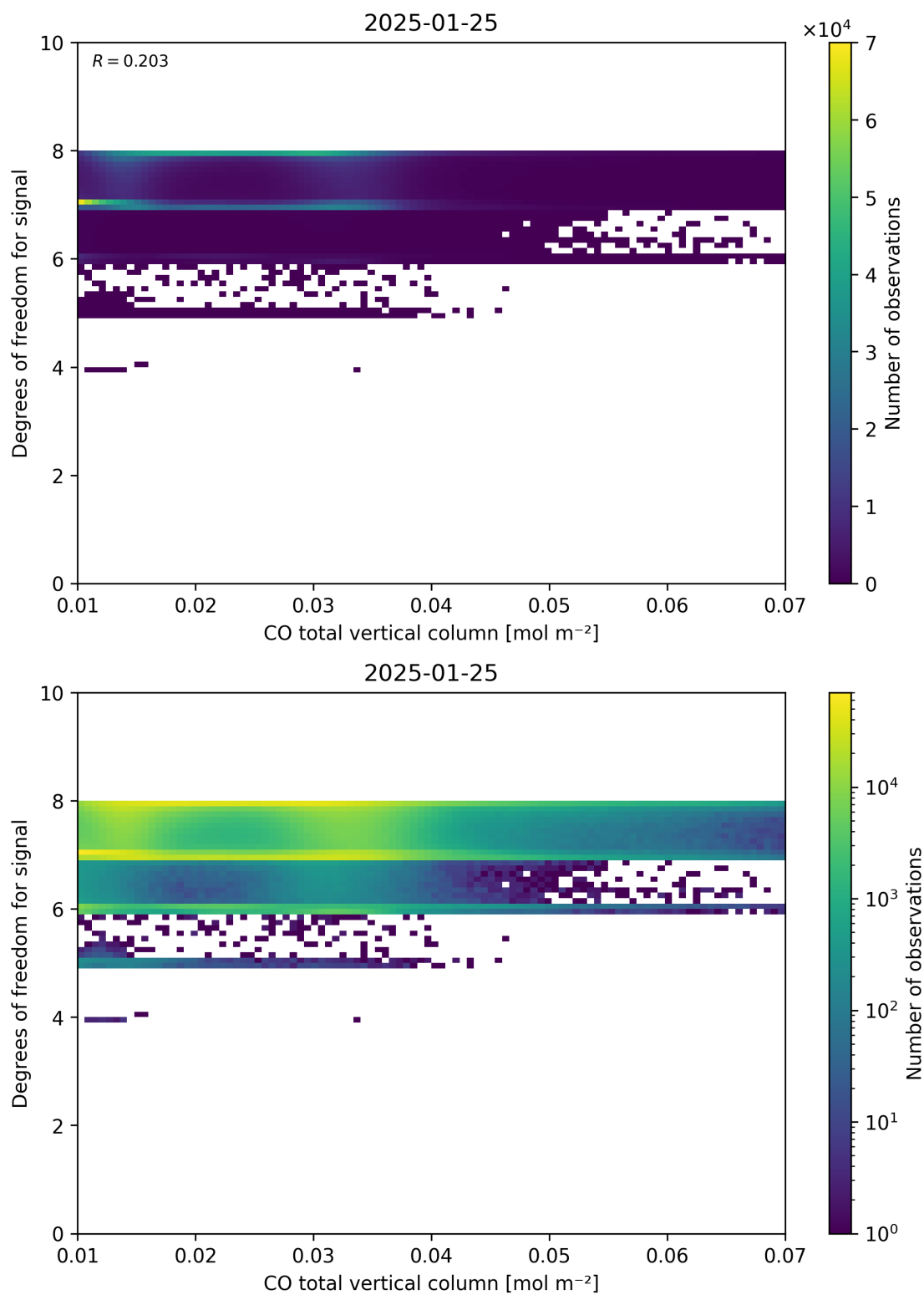
Figure 41: Scatter density plot of “CO total vertical column” against “Degrees of freedom for signal” for 2025-01-24 to 2025-01-26.
