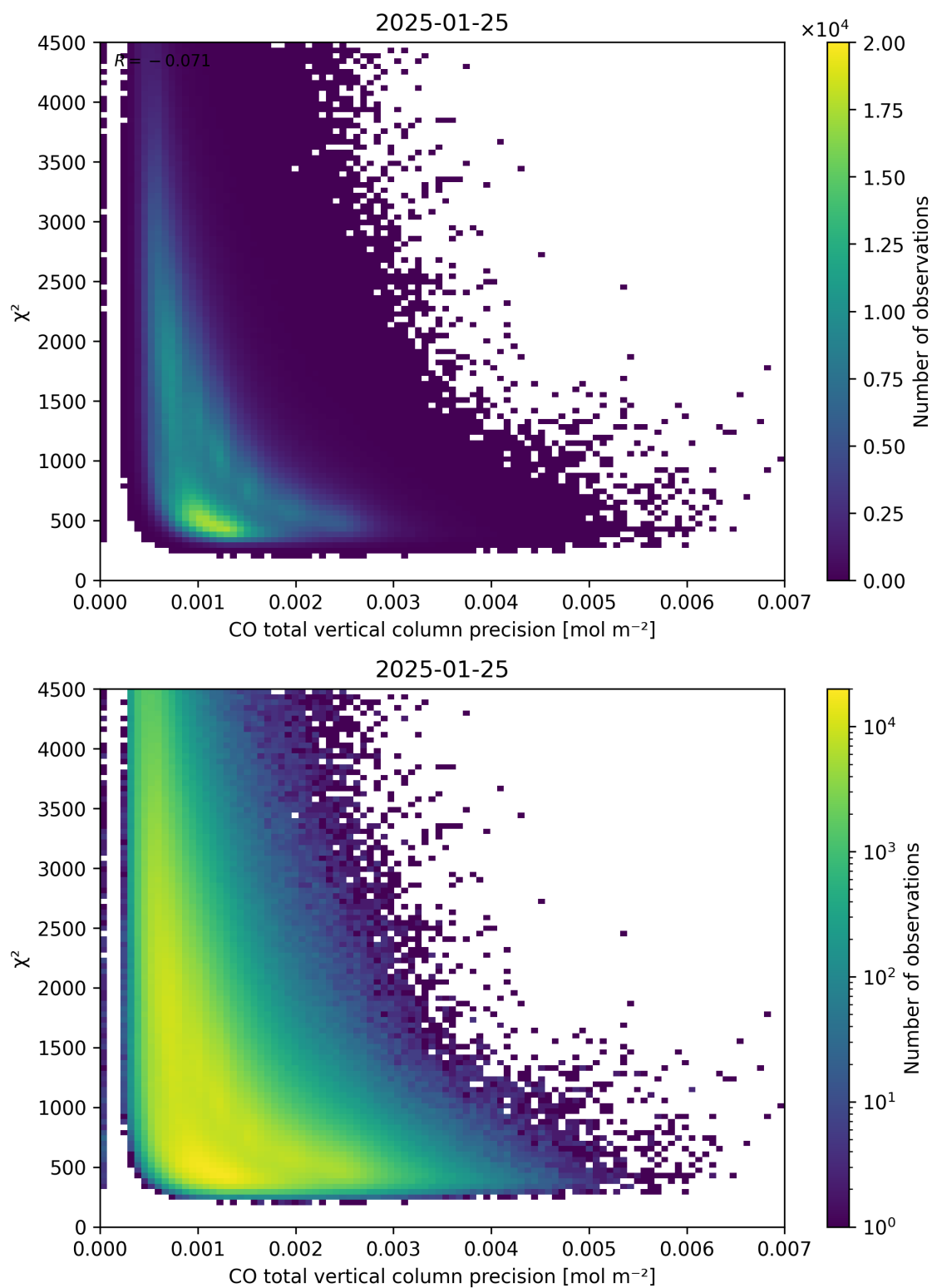
Figure 44: Scatter density plot of “CO total vertical column precision” against “ \chi^2 ” for 2025-01-24 to 2025-01-26.
