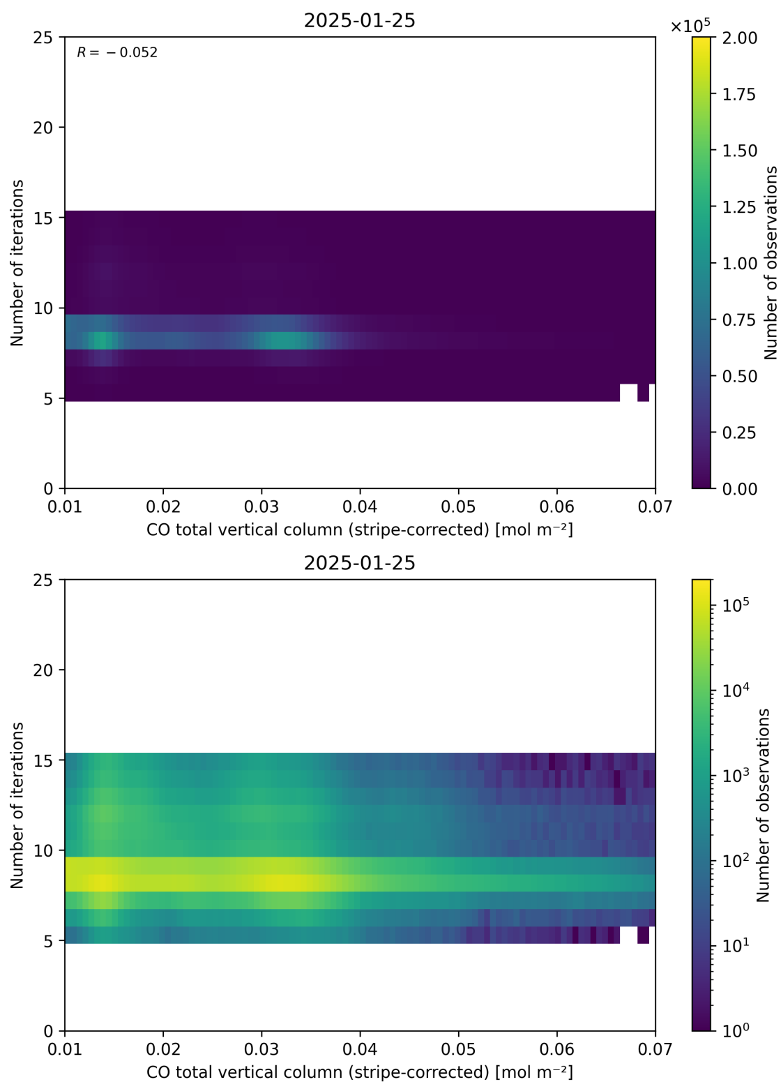
Figure 39: Scatter density plot of “CO total vertical column (stripe-corrected)” against “Number of iterations” for 2025-01-24 to 2025-01-26.
