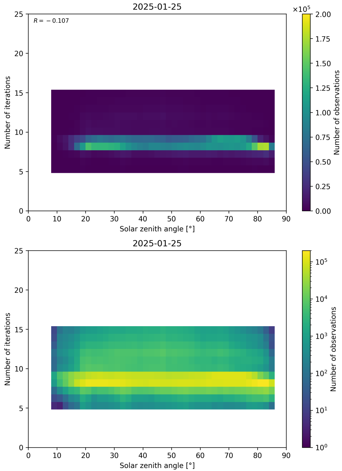
Figure 67: Scatter density plot of “Solar zenith angle” against “Number of iterations” for 2025-01-24 to 2025-01-26.
