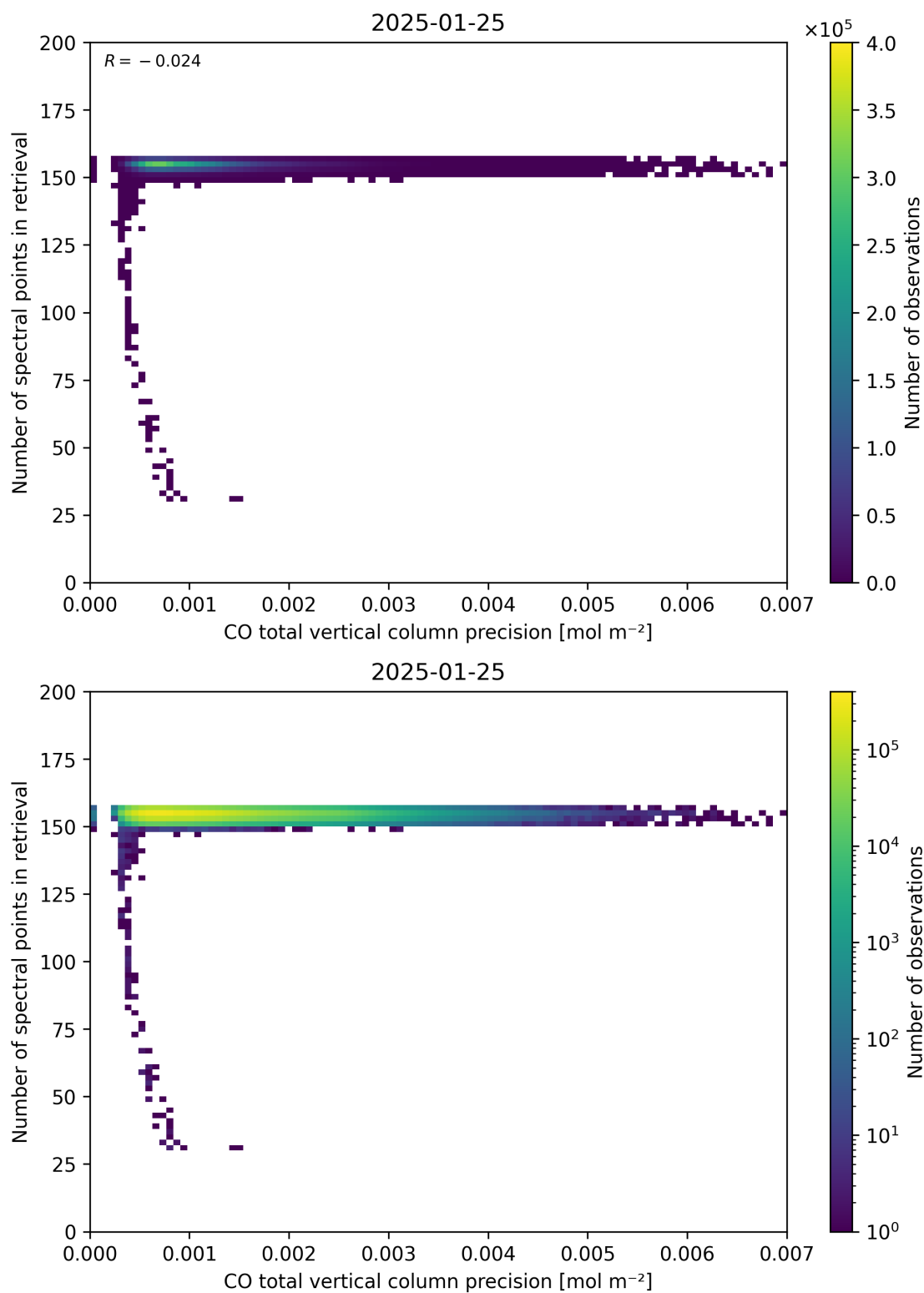
Figure 47: Scatter density plot of “CO total vertical column precision” against “Number of spectral points in retrieval” for 2025-01-24 to 2025-01-26.
