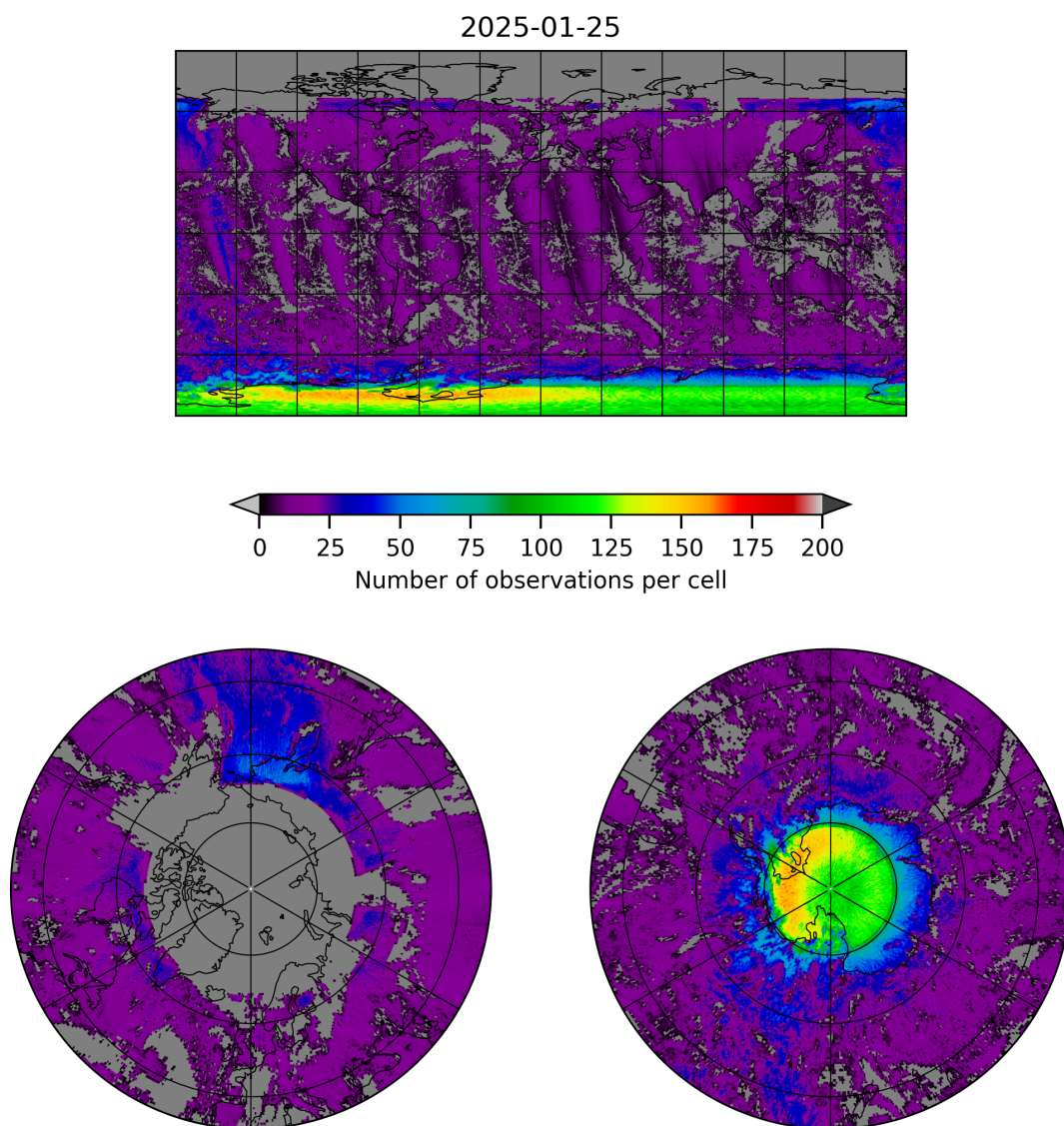
Figure 8: Map of the number of observations for 2025-01-24 to 2025-01-26
