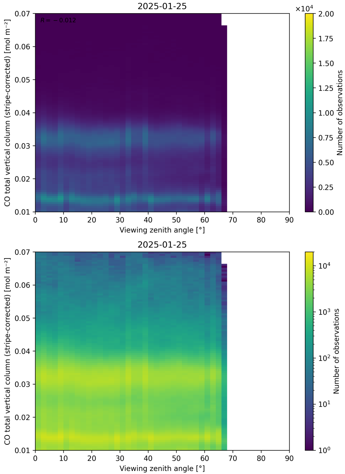
Figure 70: Scatter density plot of “Viewing zenith angle” against “CO total vertical column (stripe-corrected)” for 2025-01-24 to 2025-01-26.
