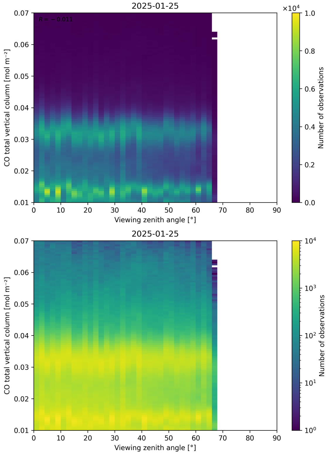
Figure 69: Scatter density plot of “Viewing zenith angle” against “CO total vertical column” for 2025-01-24 to 2025-01-26.
