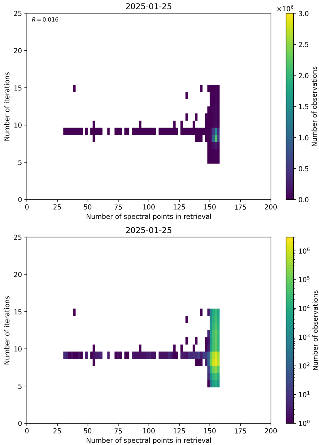
Figure 60: Scatter density plot of “Number of spectral points in retrieval” against “Number of iterations” for 2025-01-24 to 2025-01-26.
