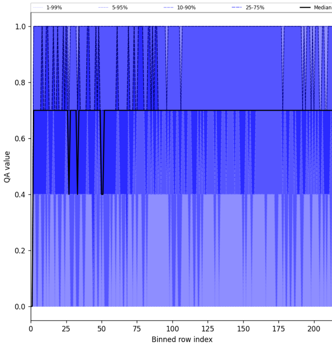
Figure 25: Along track statistics of “QA value” for 2025-01-24 to 2025-01-26
