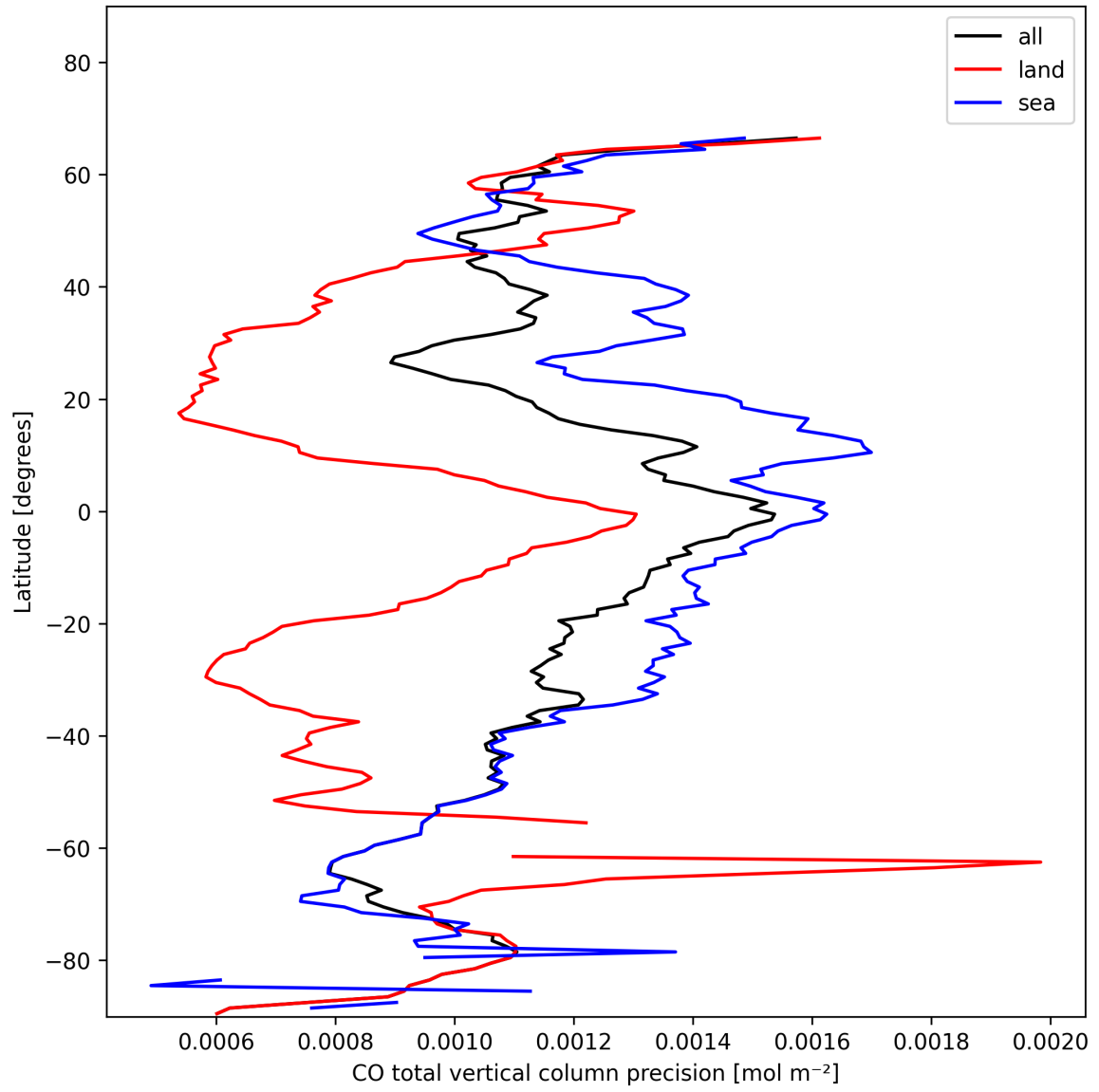
Figure 12: Zonal average of “CO total vertical column precision” for 2025-01-24 to 2025-01-26.
