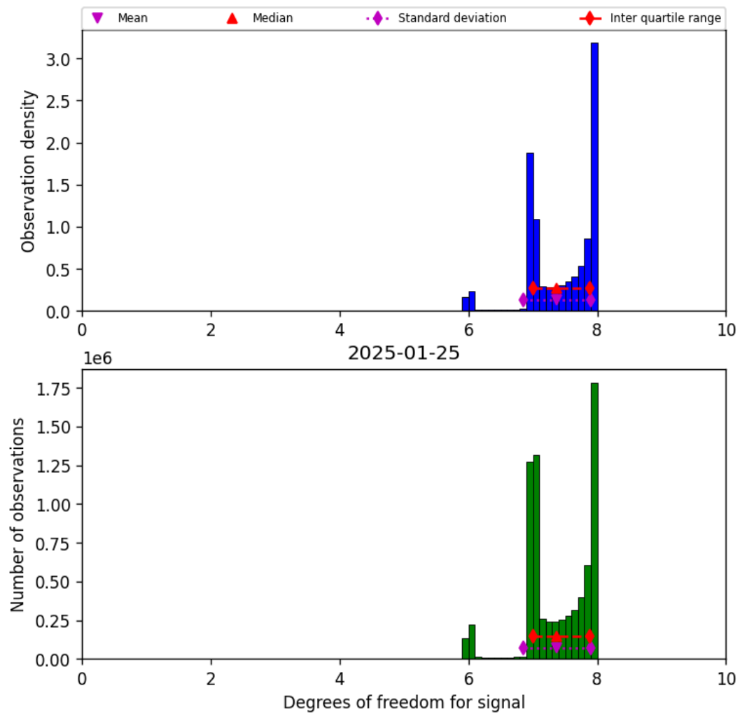
Figure 23: Histogram of “Degrees of freedom for signal” for 2025-01-24 to 2025-01-26
