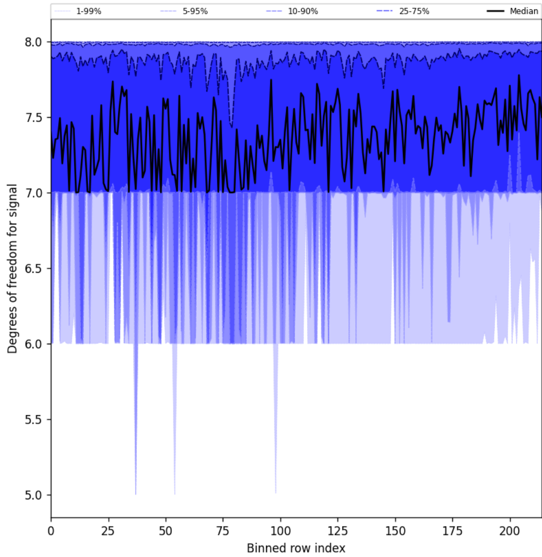
Figure 31: Along track statistics of “Degrees of freedom for signal” for 2025-01-24 to 2025-01-26
