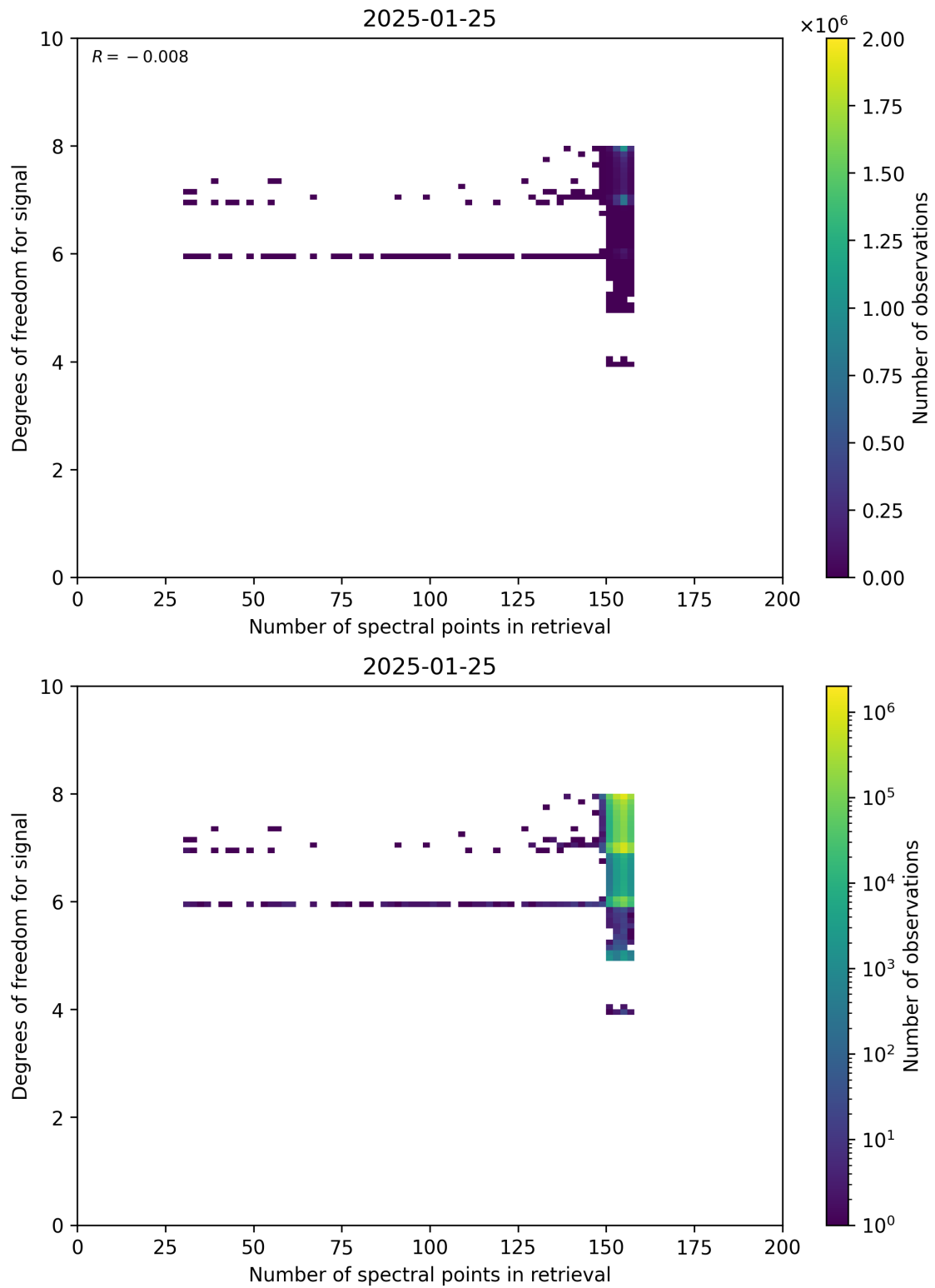
Figure 59: Scatter density plot of “Number of spectral points in retrieval” against “Degrees of freedom for signal” for 2025-01-24 to 2025-01-26.
