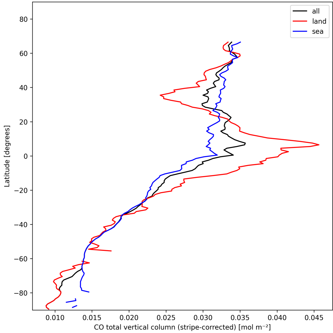
Figure 11: Zonal average of “CO total vertical column (stripe-corrected)” for 2025-01-24 to 2025-01-26.
