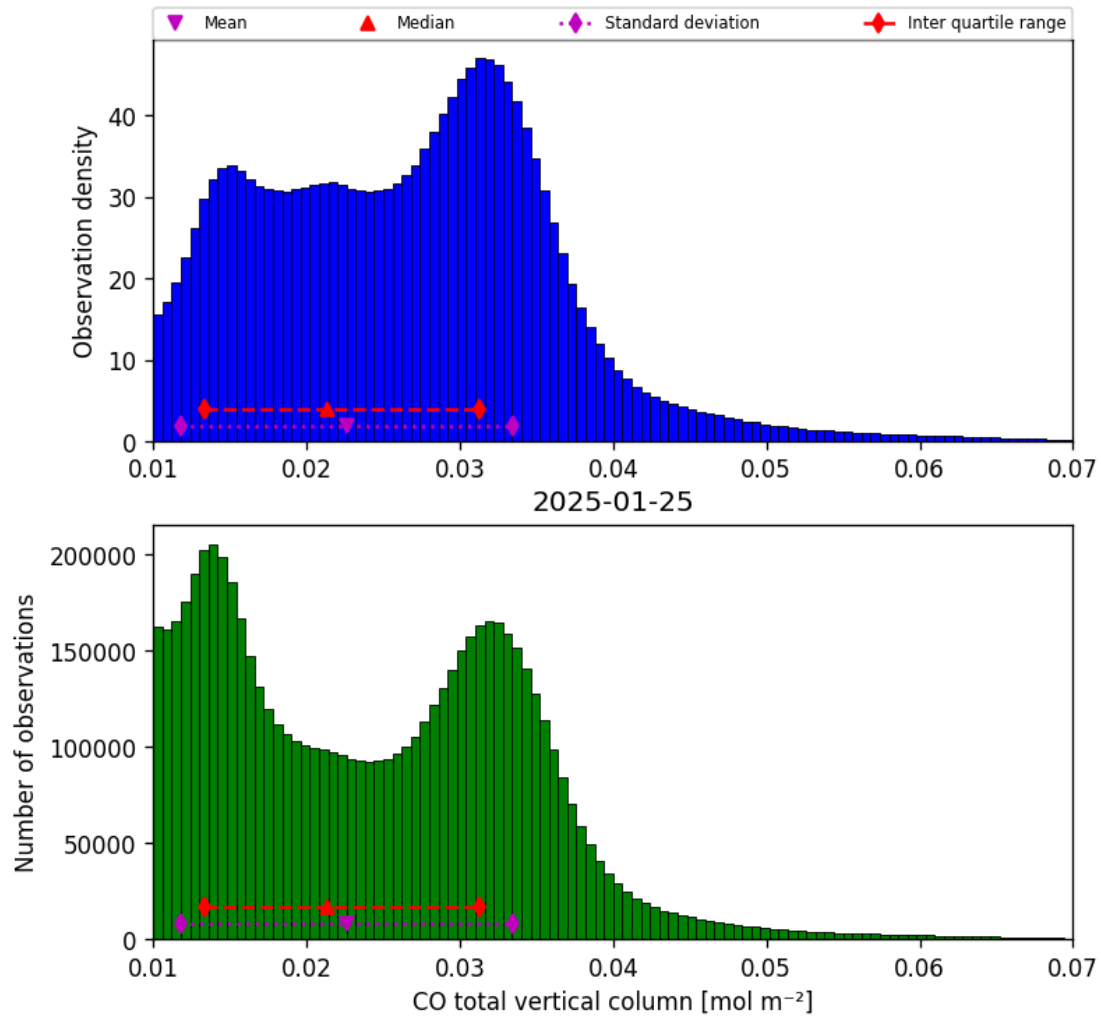
Figure 18: Histogram of “CO total vertical column” for 2025-01-24 to 2025-01-26
