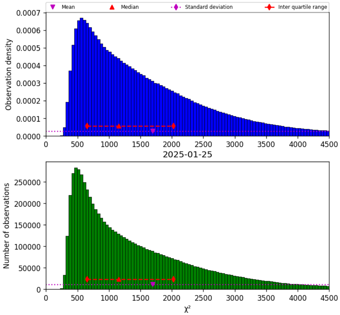
Figure 22: Histogram of “ \chi^2 ” for 2025-01-24 to 2025-01-26
