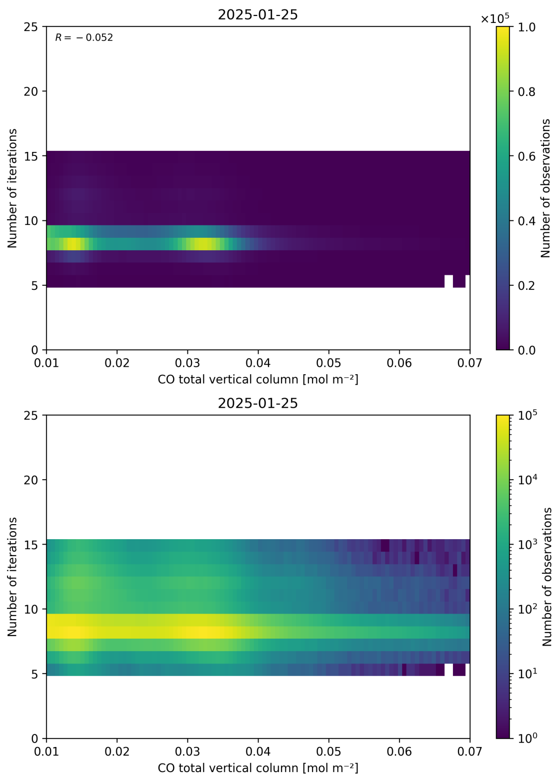
Figure 42: Scatter density plot of “CO total vertical column” against “Number of iterations” for 2025-01-24 to 2025-01-26.
