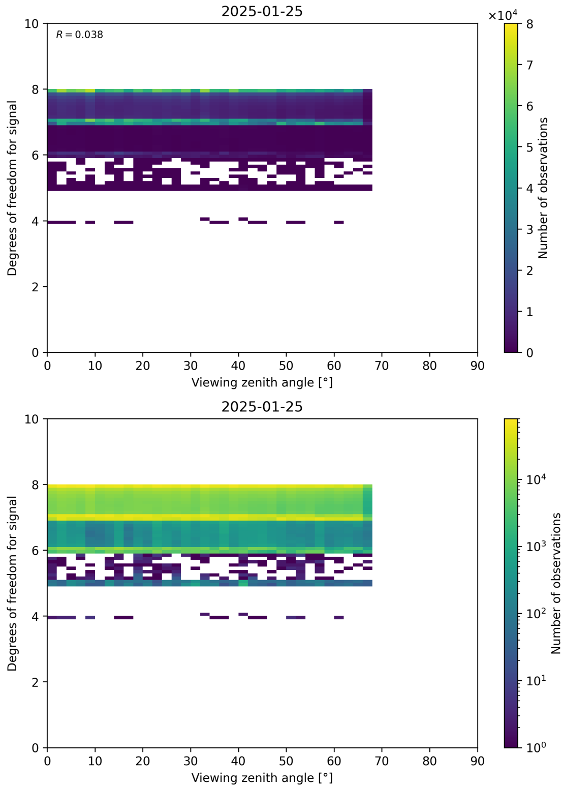
Figure 73: Scatter density plot of “Viewing zenith angle” against “Degrees of freedom for signal” for 2025-01-24 to 2025-01-26.
