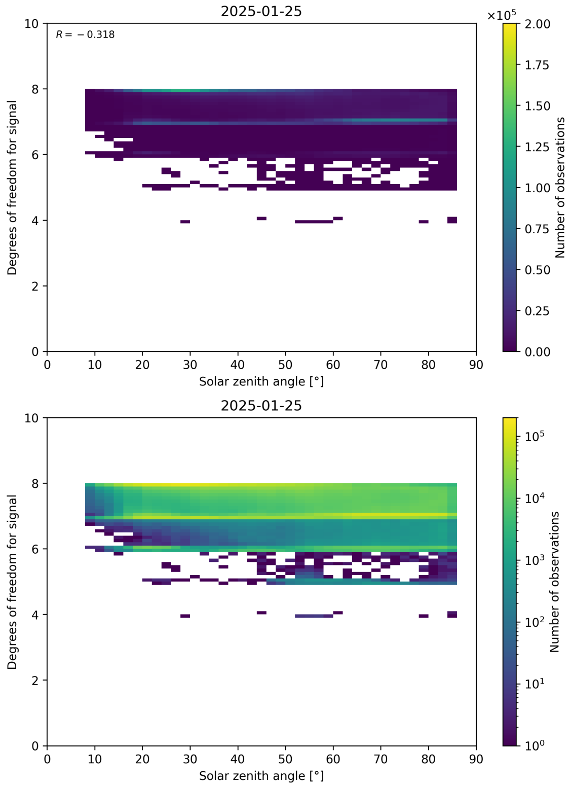
Figure 65: Scatter density plot of “Solar zenith angle” against “Degrees of freedom for signal” for 2025-01-24 to 2025-01-26.
