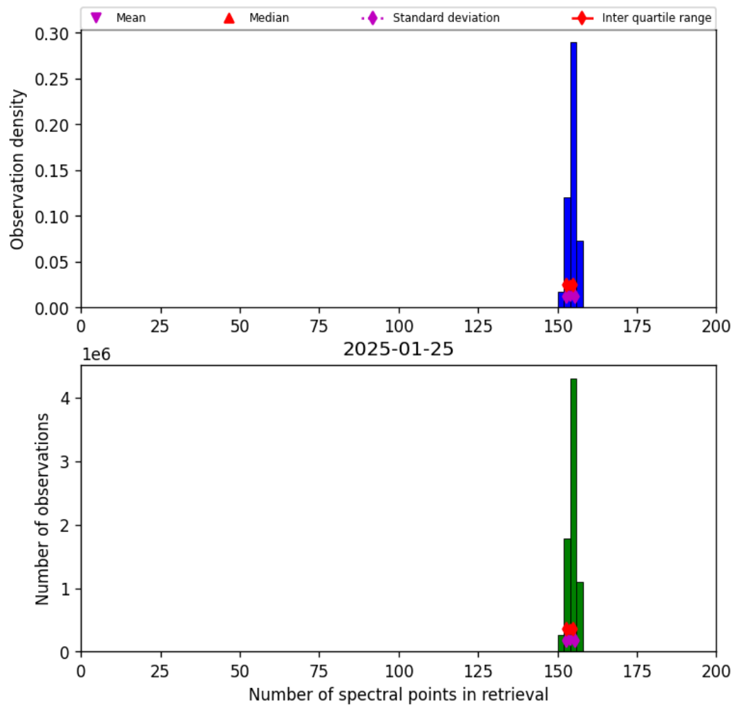
Figure 21: Histogram of “Number of spectral points in retrieval” for 2025-01-24 to 2025-01-26
