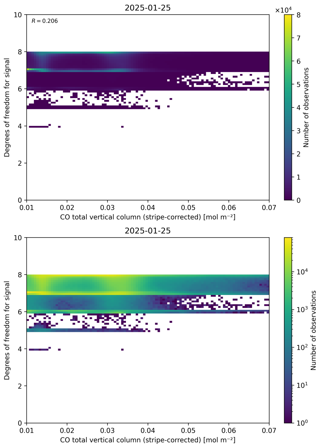
Figure 38: Scatter density plot of “CO total vertical column (stripe-corrected)” against “Degrees of freedom for signal” for 2025-01-24 to 2025-01-26.
