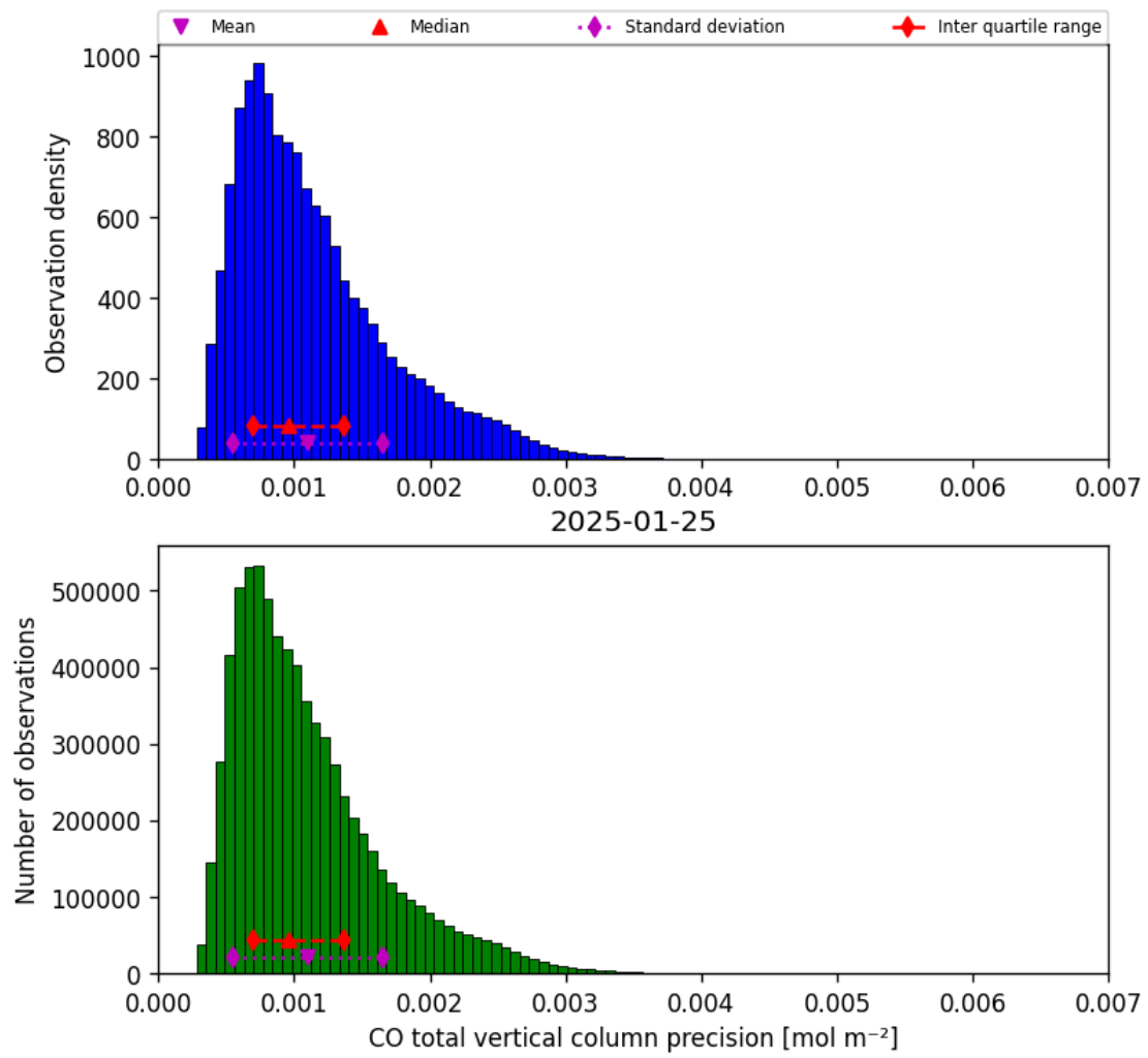
Figure 20: Histogram of “CO total vertical column precision” for 2025-01-24 to 2025-01-26
