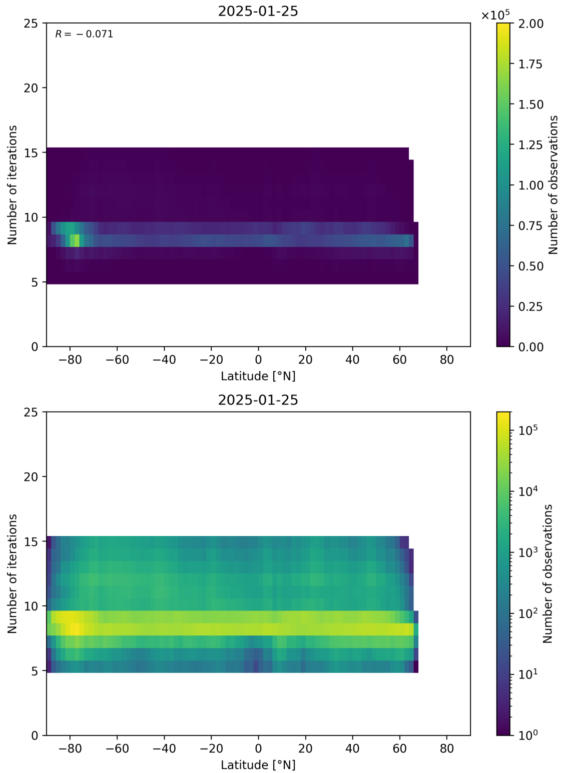
Figure 56: Scatter density plot of “Latitude” against “Number of iterations” for 2025-01-24 to 2025-01-26.
