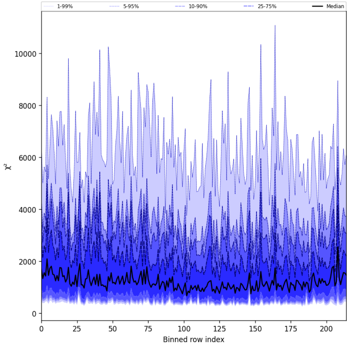
Figure 30: Along track statistics of “ \chi^2 ” for 2025-01-24 to 2025-01-26
