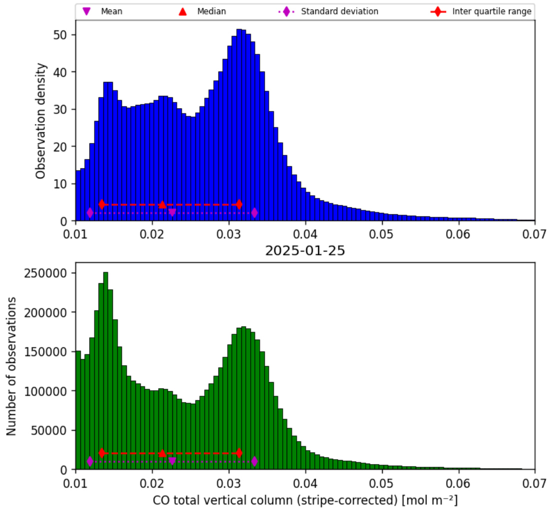
Figure 19: Histogram of “CO total vertical column (stripe-corrected)” for 2025-01-24 to 2025-01-26
