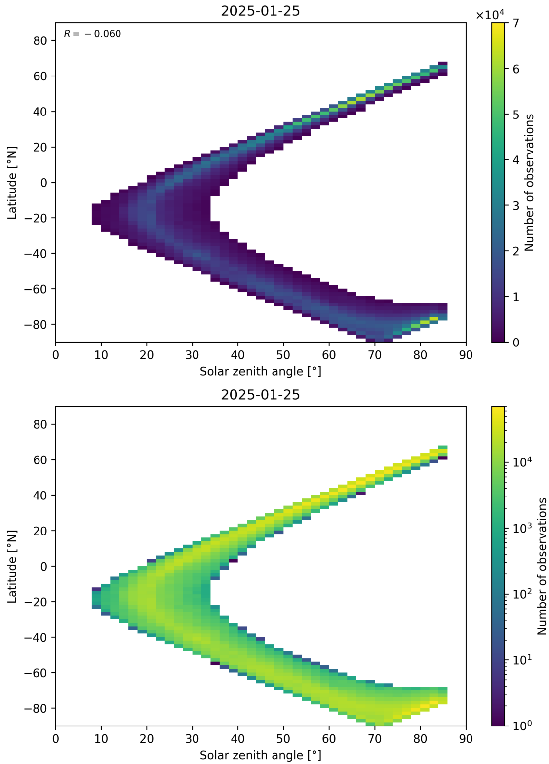
Figure 66: Scatter density plot of “Solar zenith angle” against “Latitude” for 2025-01-24 to 2025-01-26.
