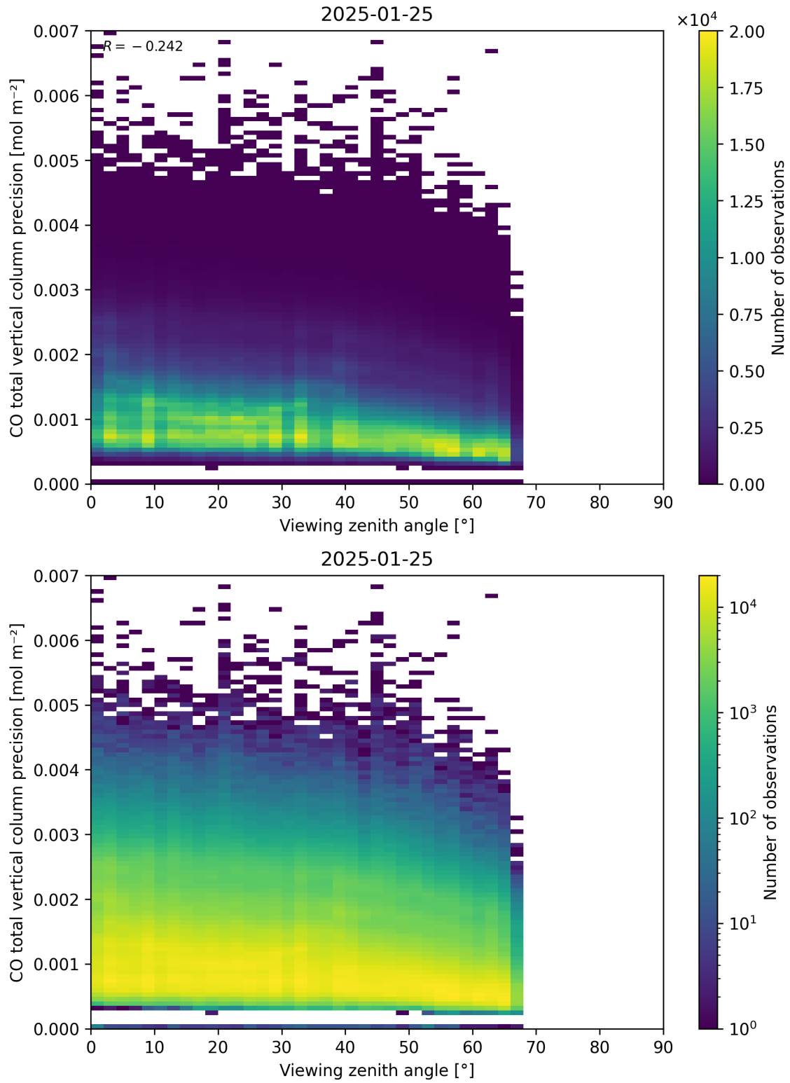
Figure 71: Scatter density plot of “Viewing zenith angle” against “CO total vertical column precision” for 2025-01-24 to 2025-01-26.
