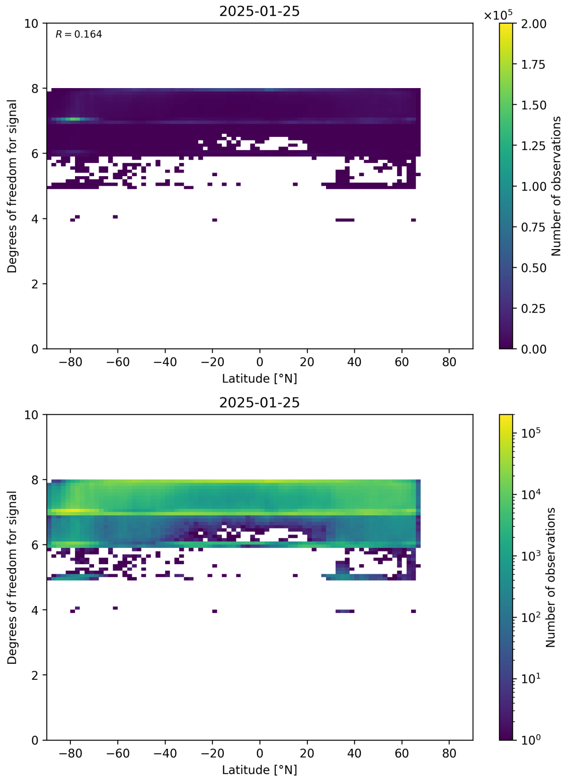
Figure 55: Scatter density plot of “Latitude” against “Degrees of freedom for signal” for 2025-01-24 to 2025-01-26.
