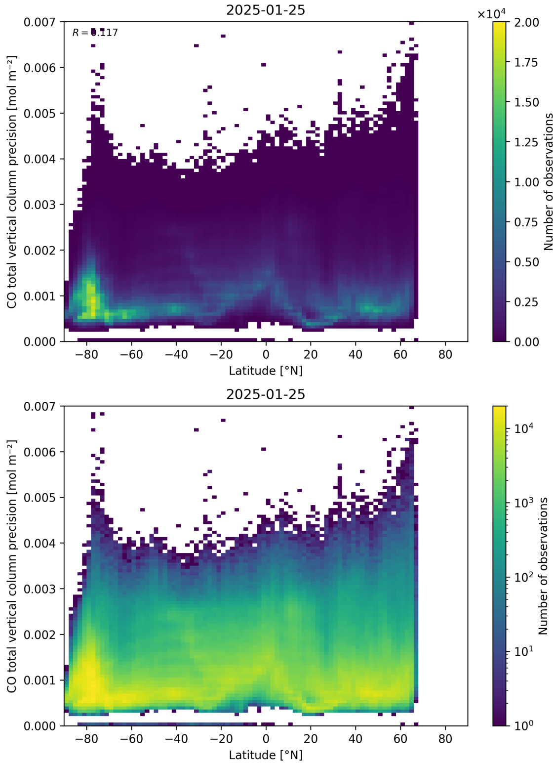
Figure 53: Scatter density plot of “Latitude” against “CO total vertical column precision” for 2025-01-24 to 2025-01-26.
