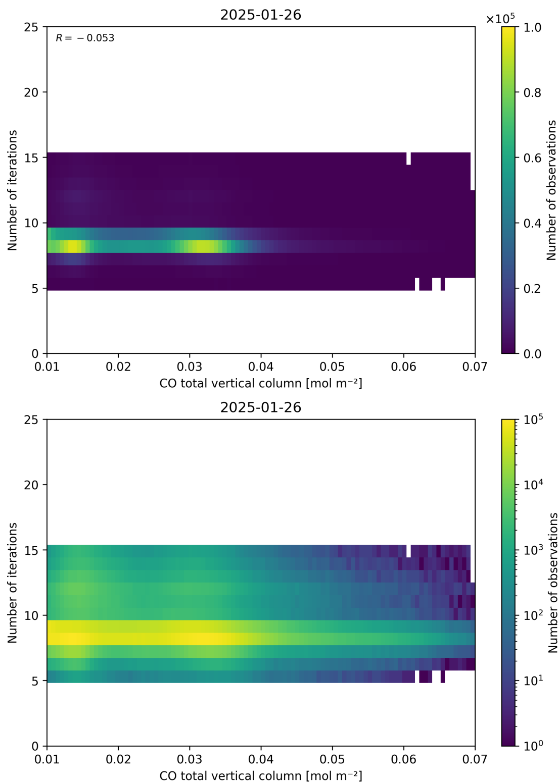
Figure 42: Scatter density plot of “CO total vertical column” against “Number of iterations” for 2025-01-25 to 2025-01-27.
