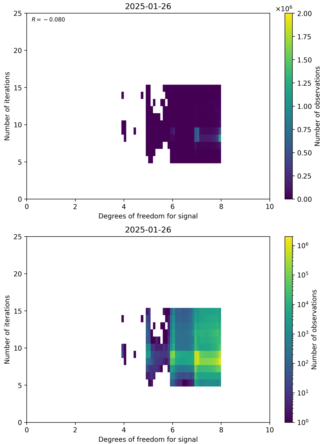
Figure 50: Scatter density plot of “Degrees of freedom for signal” against “Number of iterations” for 2025-01-25 to 2025-01-27.
