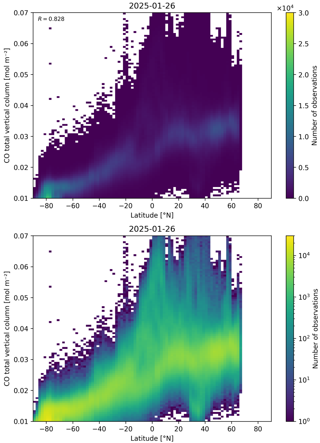
Figure 51: Scatter density plot of “Latitude” against “CO total vertical column” for 2025-01-25 to 2025-01-27.
