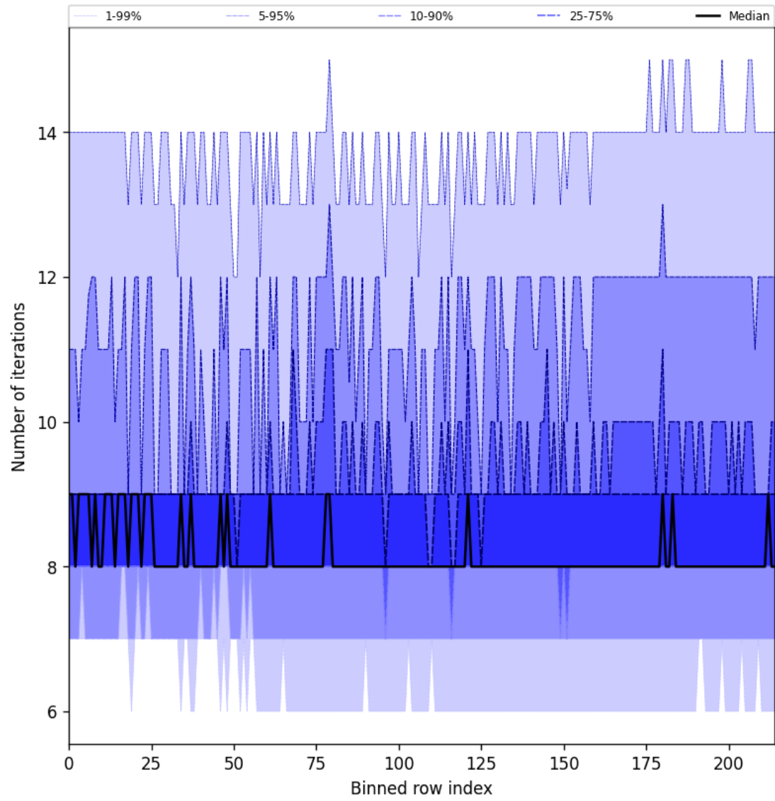
Figure 32: Along track statistics of “Number of iterations” for 2025-01-25 to 2025-01-27
