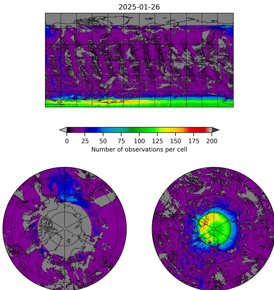
Figure 8: Map of the number of observations for 2025-01-25 to 2025-01-27
