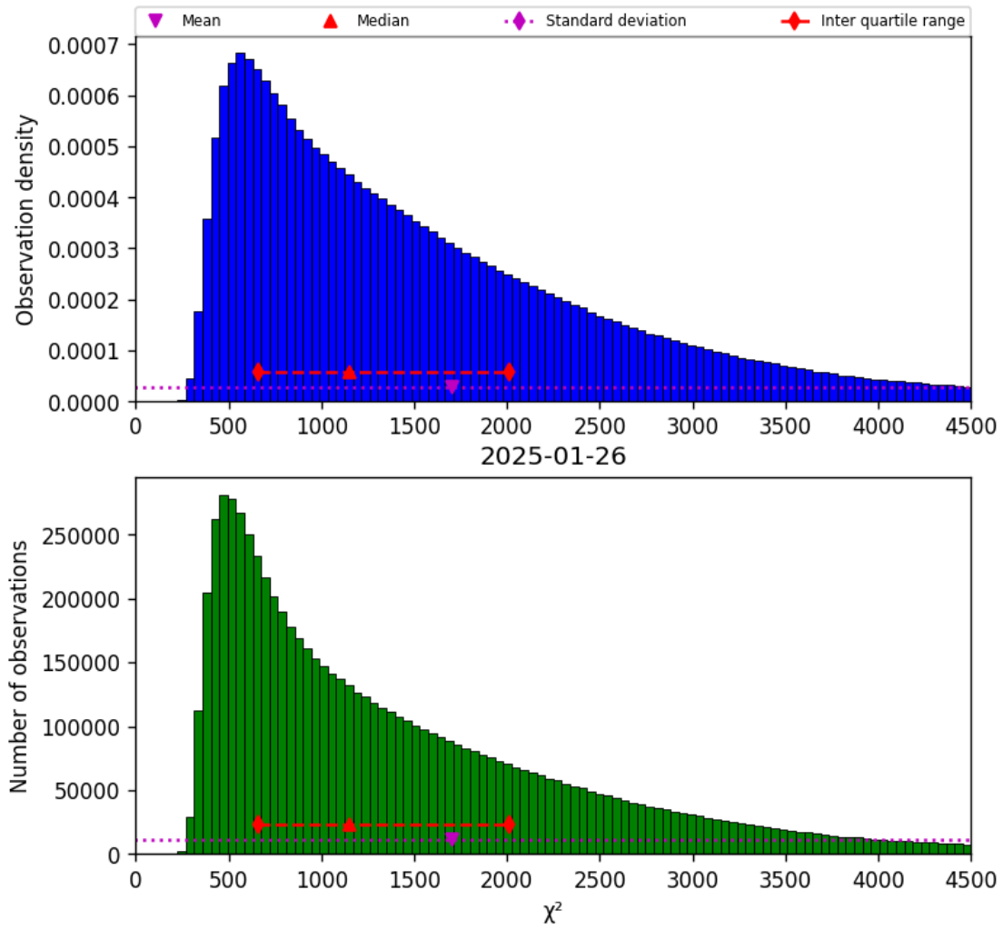
Figure 22: Histogram of “ \chi^2 ” for 2025-01-25 to 2025-01-27
