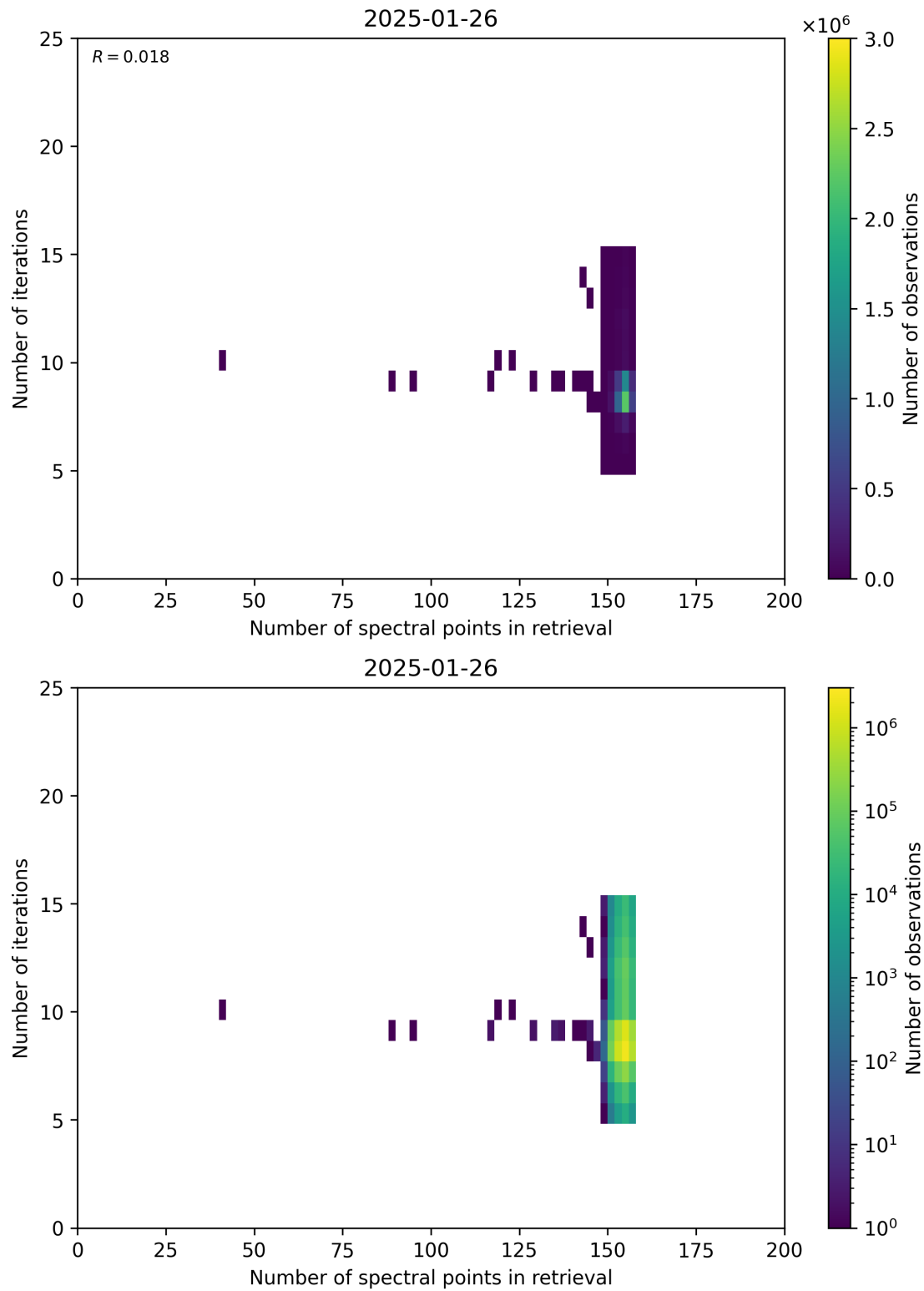
Figure 60: Scatter density plot of “Number of spectral points in retrieval” against “Number of iterations” for 2025-01-25 to 2025-01-27.
