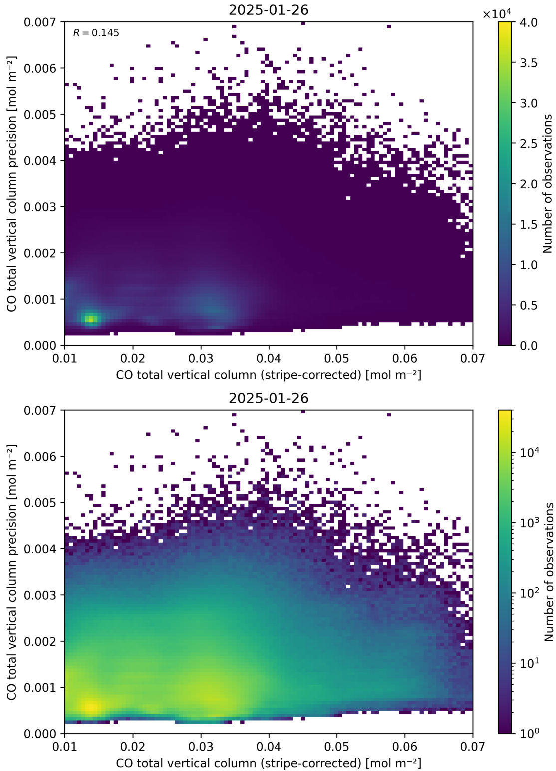
Figure 36: Scatter density plot of “CO total vertical column (stripe-corrected)” against “CO total vertical column precision” for 2025-01-25 to 2025-01-27.
