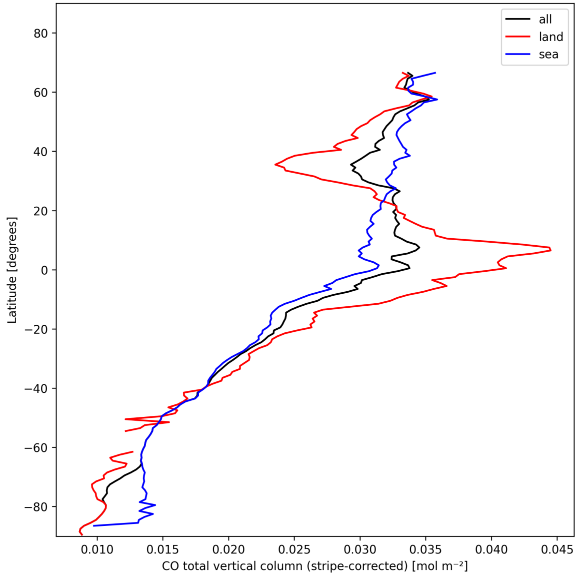
Figure 11: Zonal average of “CO total vertical column (stripe-corrected)” for 2025-01-25 to 2025-01-27.
