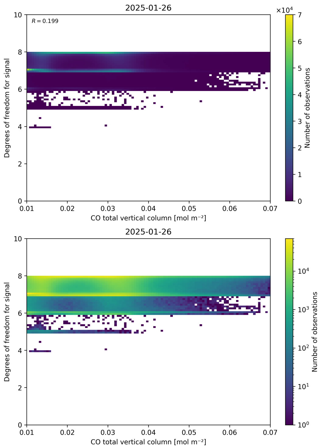
Figure 41: Scatter density plot of “CO total vertical column” against “Degrees of freedom for signal” for 2025-01-25 to 2025-01-27.
