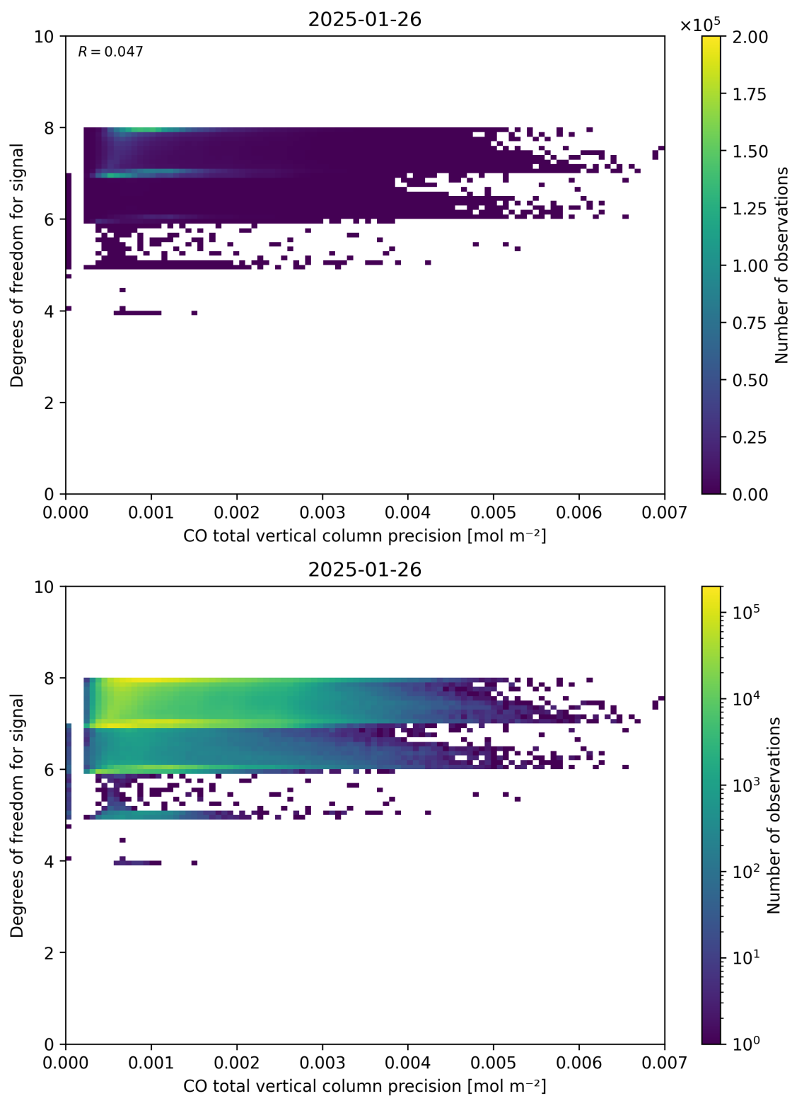
Figure 45: Scatter density plot of “CO total vertical column precision” against “Degrees of freedom for signal” for 2025-01-25 to 2025-01-27.
