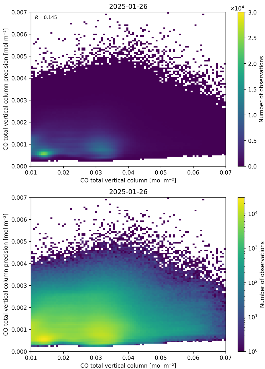
Figure 34: Scatter density plot of “CO total vertical column” against “CO total vertical column precision” for 2025-01-25 to 2025-01-27.
