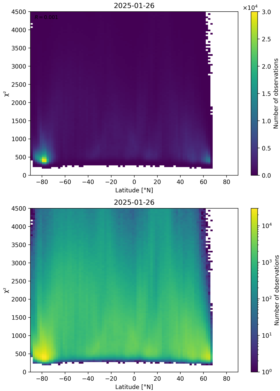
Figure 54: Scatter density plot of “Latitude” against “ \chi^2 ” for 2025-01-25 to 2025-01-27.
