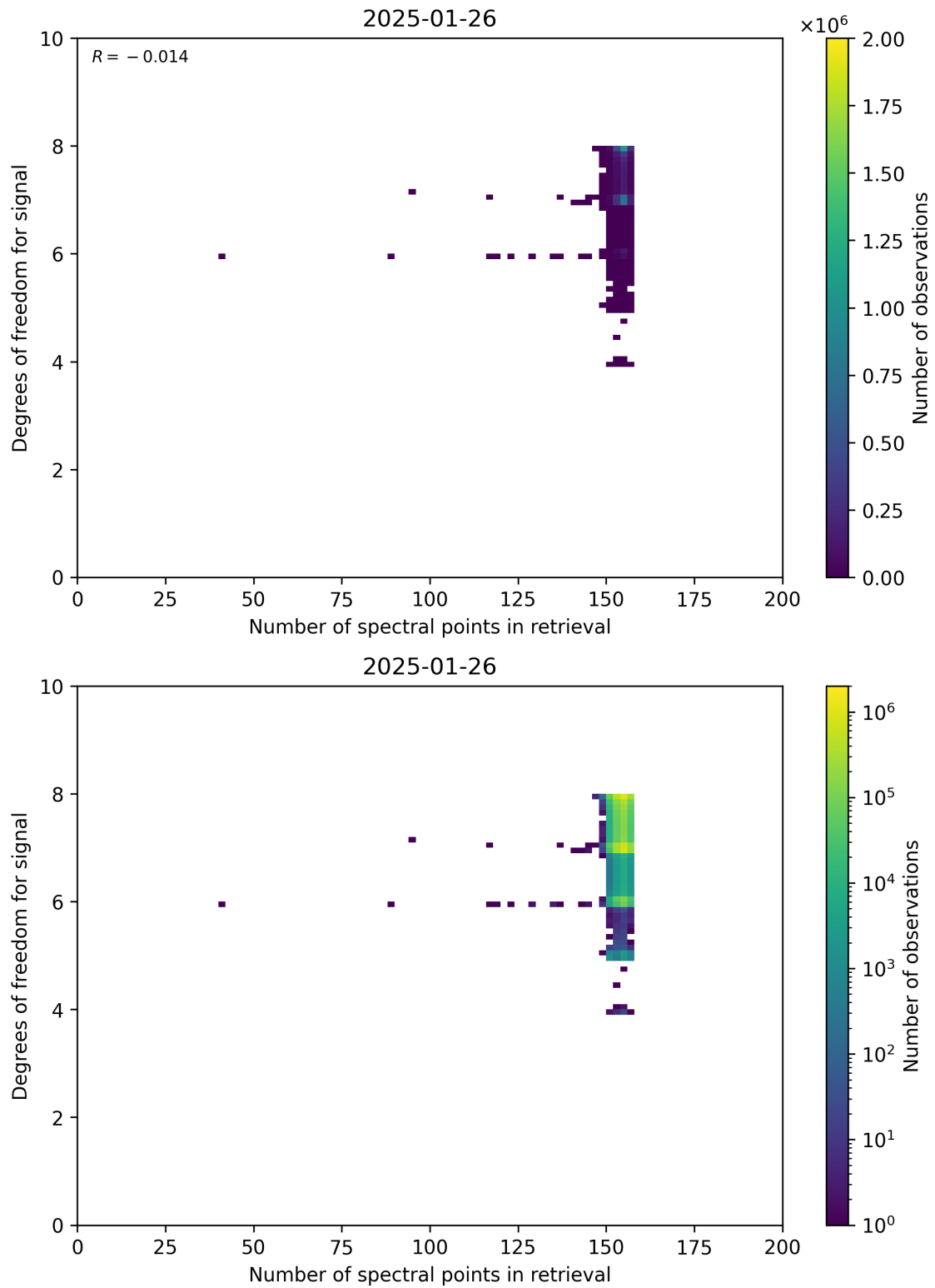
Figure 59: Scatter density plot of “Number of spectral points in retrieval” against “Degrees of freedom for signal” for 2025-01-25 to 2025-01-27.
