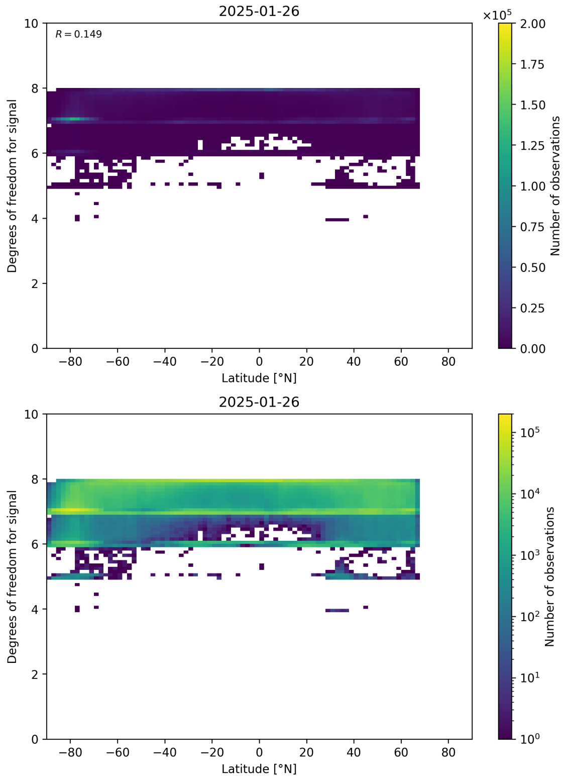
Figure 55: Scatter density plot of “Latitude” against “Degrees of freedom for signal” for 2025-01-25 to 2025-01-27.
