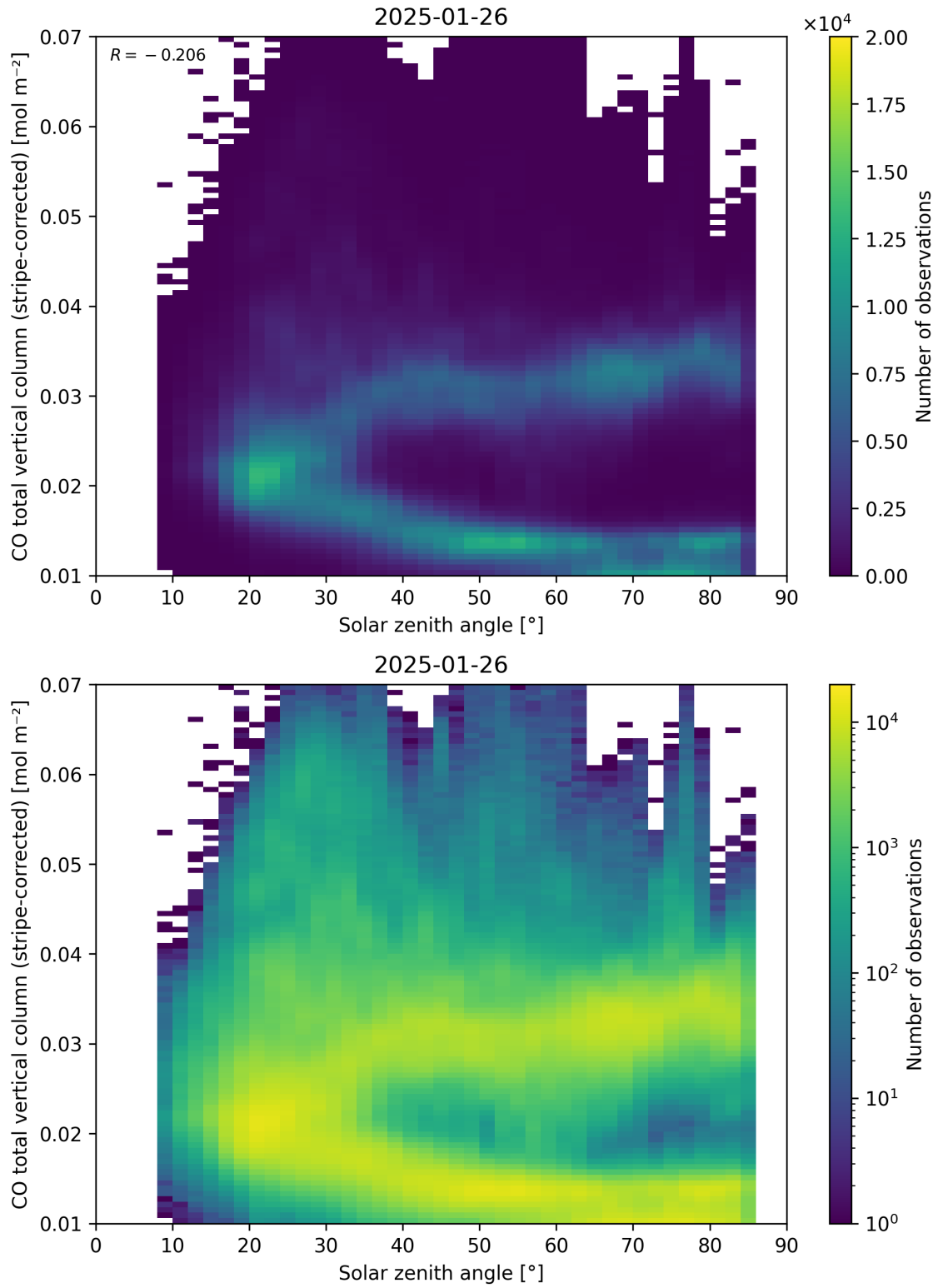
Figure 62: Scatter density plot of “Solar zenith angle” against “CO total vertical column (stripe-corrected)” for 2025-01-25 to 2025-01-27.
