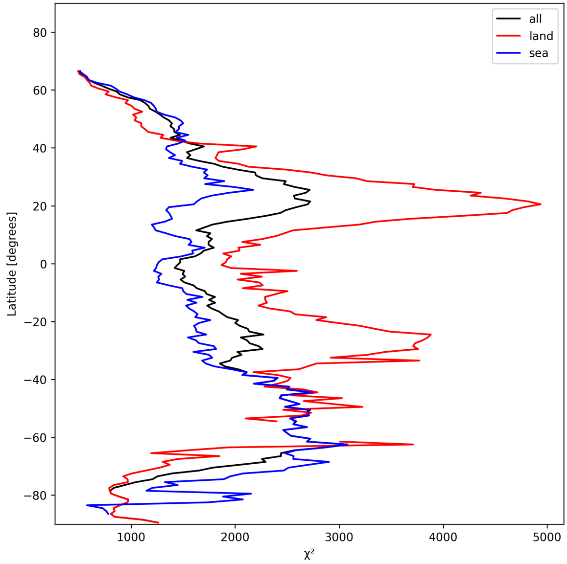
Figure 14: Zonal average of “ \chi^2 ” for 2025-01-25 to 2025-01-27.
