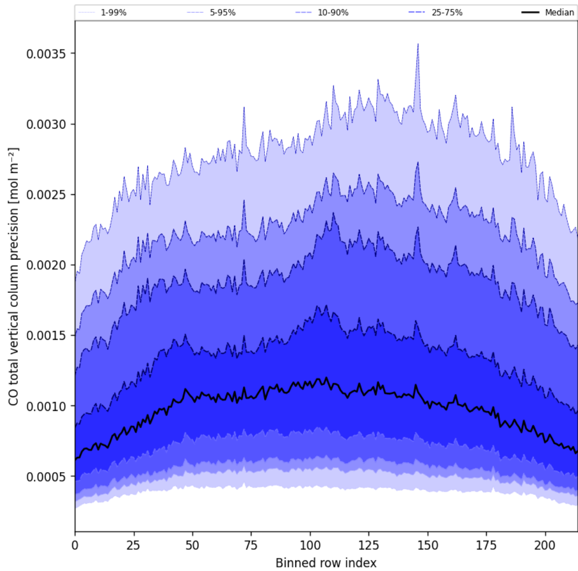
Figure 28: Along track statistics of “CO total vertical column precision” for 2025-01-25 to 2025-01-27
