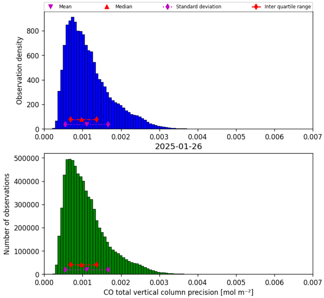
Figure 20: Histogram of “CO total vertical column precision” for 2025-01-25 to 2025-01-27
