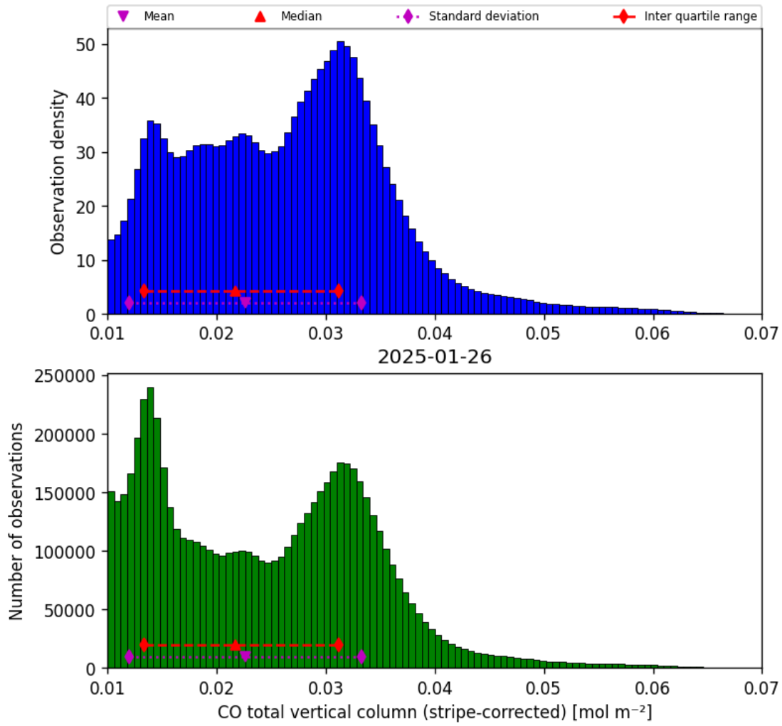
Figure 19: Histogram of “CO total vertical column (stripe-corrected)” for 2025-01-25 to 2025-01-27
