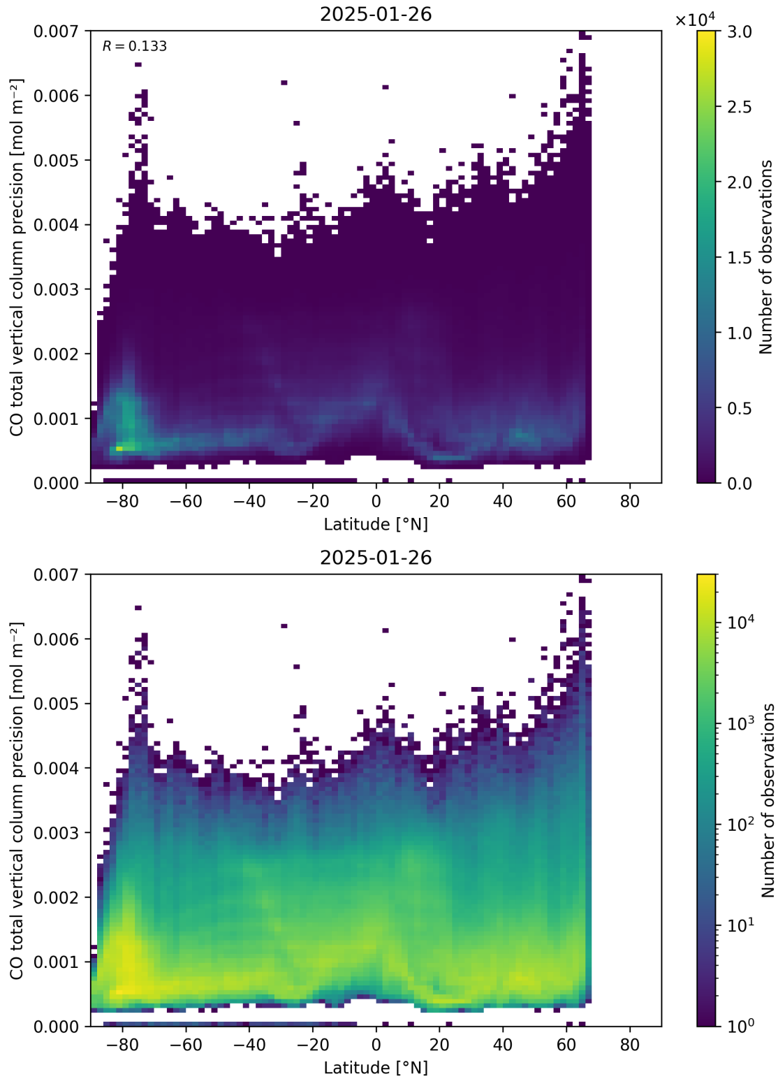
Figure 53: Scatter density plot of “Latitude” against “CO total vertical column precision” for 2025-01-25 to 2025-01-27.
