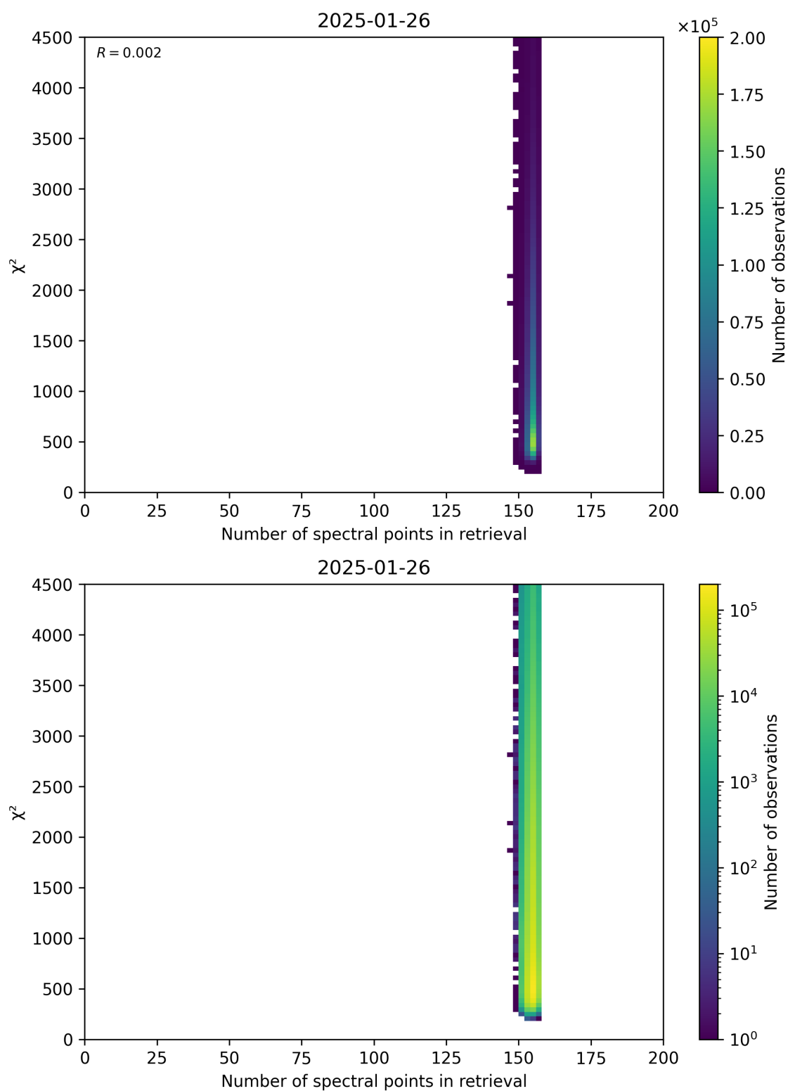
Figure 58: Scatter density plot of “Number of spectral points in retrieval” against “ \chi^2 ” for 2025-01-25 to 2025-01-27.
