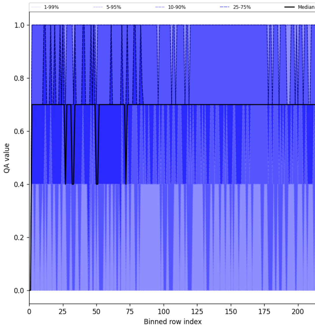
Figure 25: Along track statistics of “QA value” for 2025-01-25 to 2025-01-27
