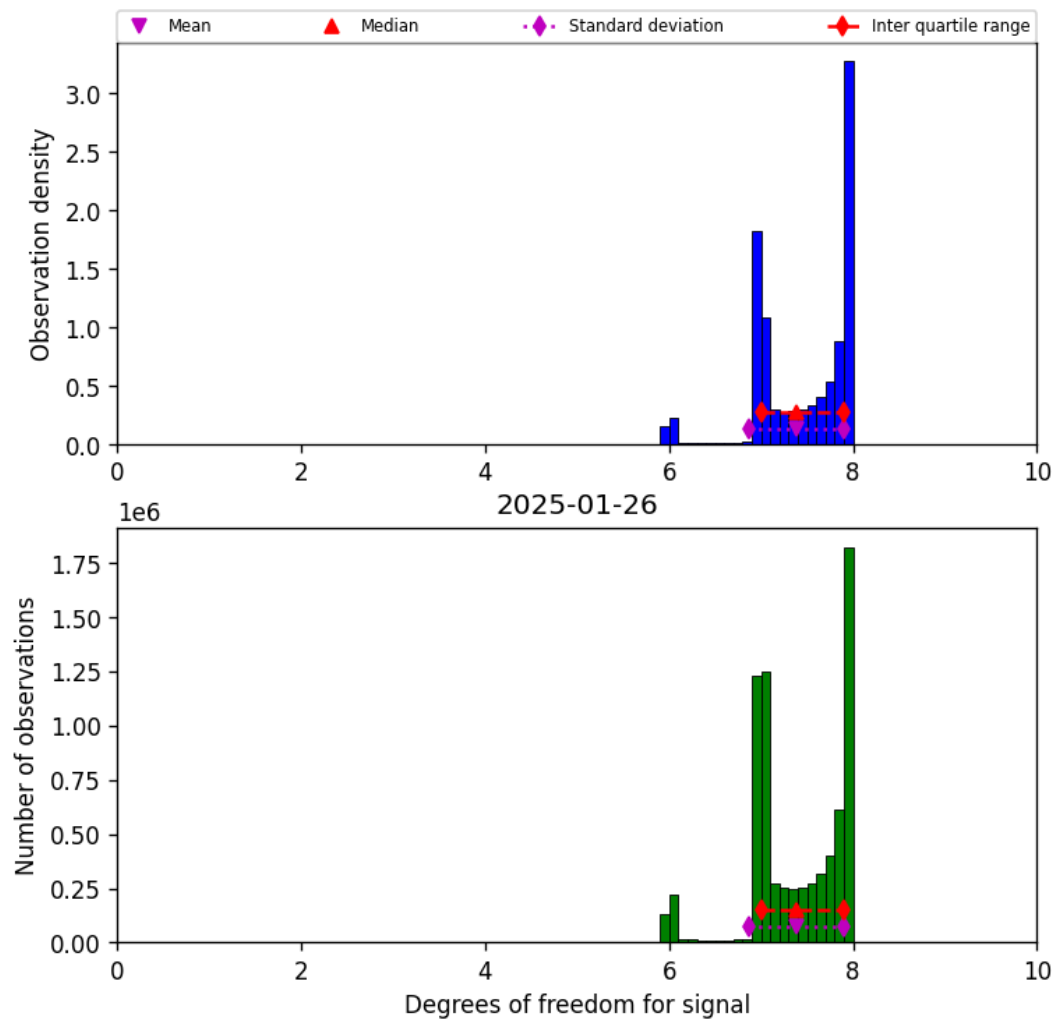
Figure 23: Histogram of “Degrees of freedom for signal” for 2025-01-25 to 2025-01-27
