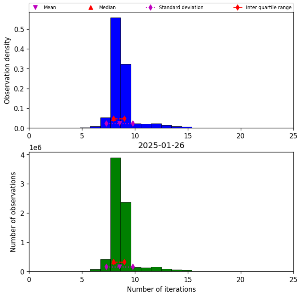
Figure 24: Histogram of “Number of iterations” for 2025-01-25 to 2025-01-27
