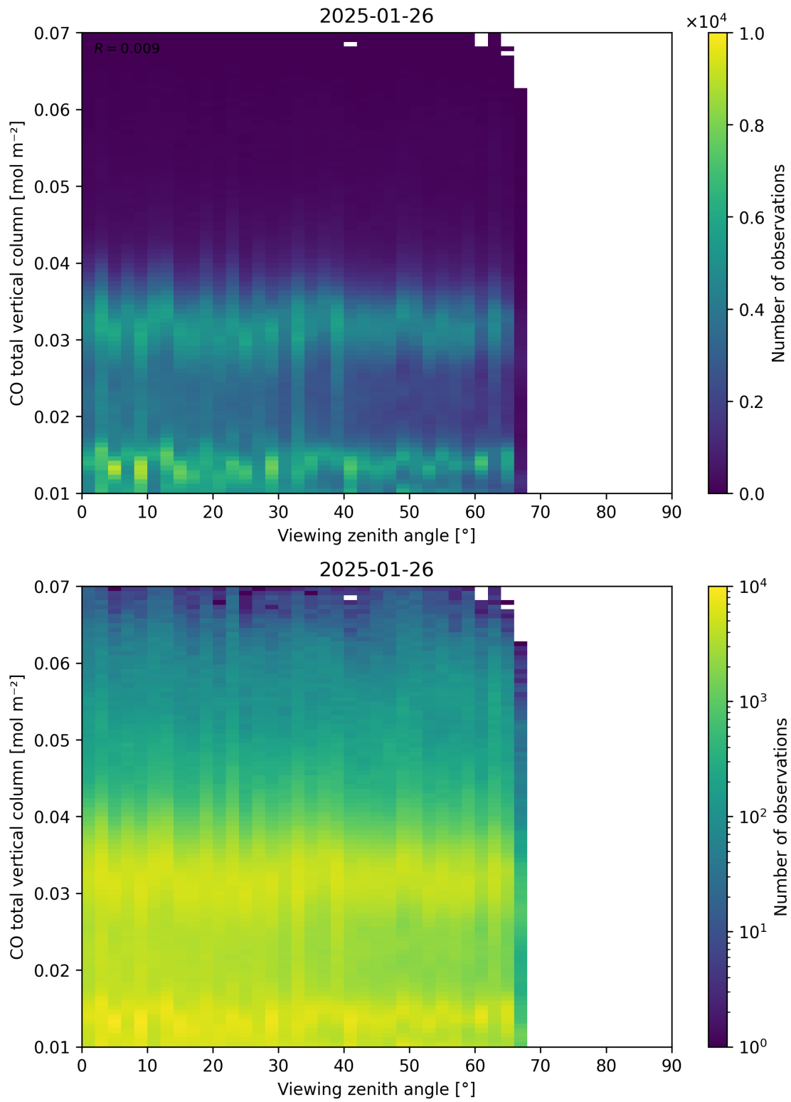
Figure 69: Scatter density plot of “Viewing zenith angle” against “CO total vertical column” for 2025-01-25 to 2025-01-27.
