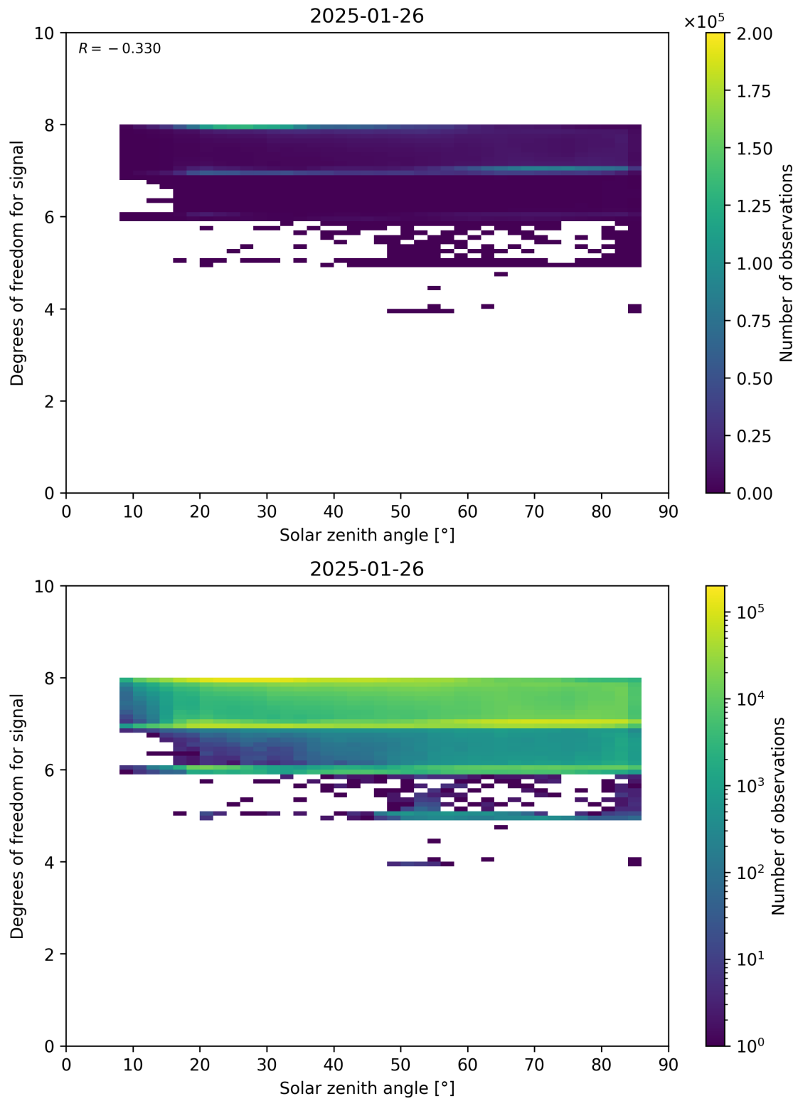
Figure 65: Scatter density plot of “Solar zenith angle” against “Degrees of freedom for signal” for 2025-01-25 to 2025-01-27.
