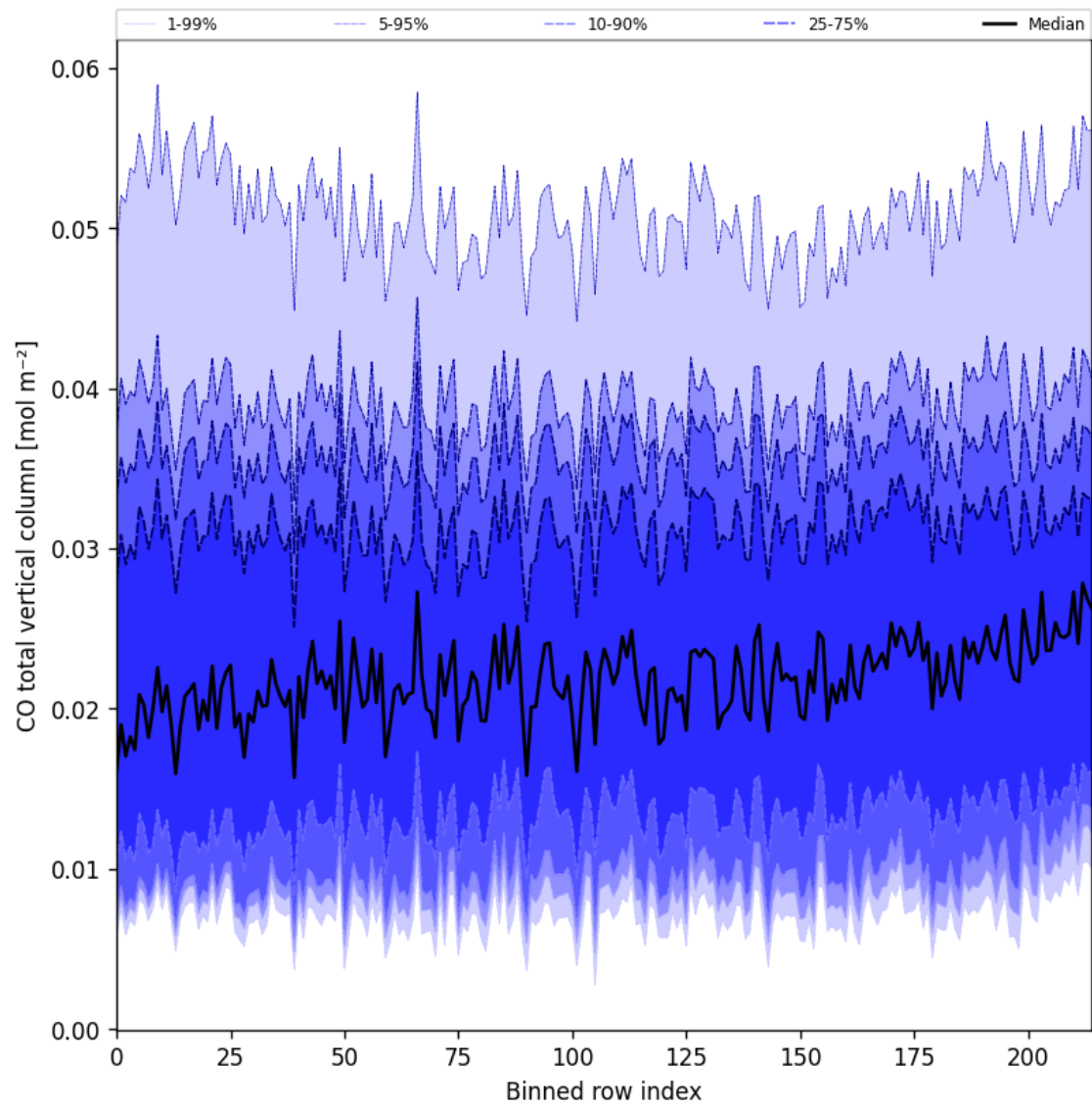
Figure 26: Along track statistics of “CO total vertical column” for 2025-01-25 to 2025-01-27
