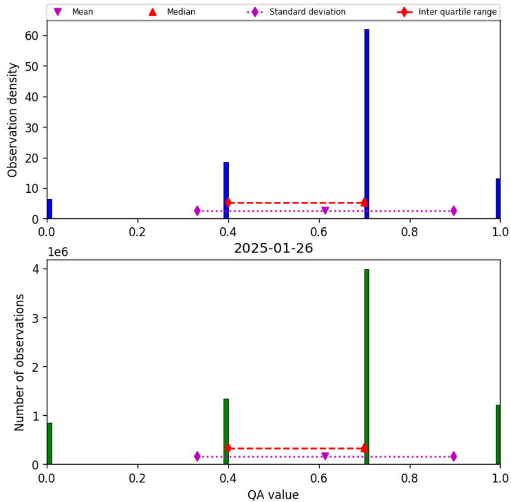
Figure 17: Histogram of “QA value” for 2025-01-25 to 2025-01-27
