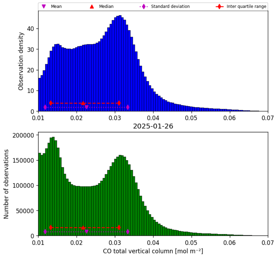
Figure 18: Histogram of “CO total vertical column” for 2025-01-25 to 2025-01-27
