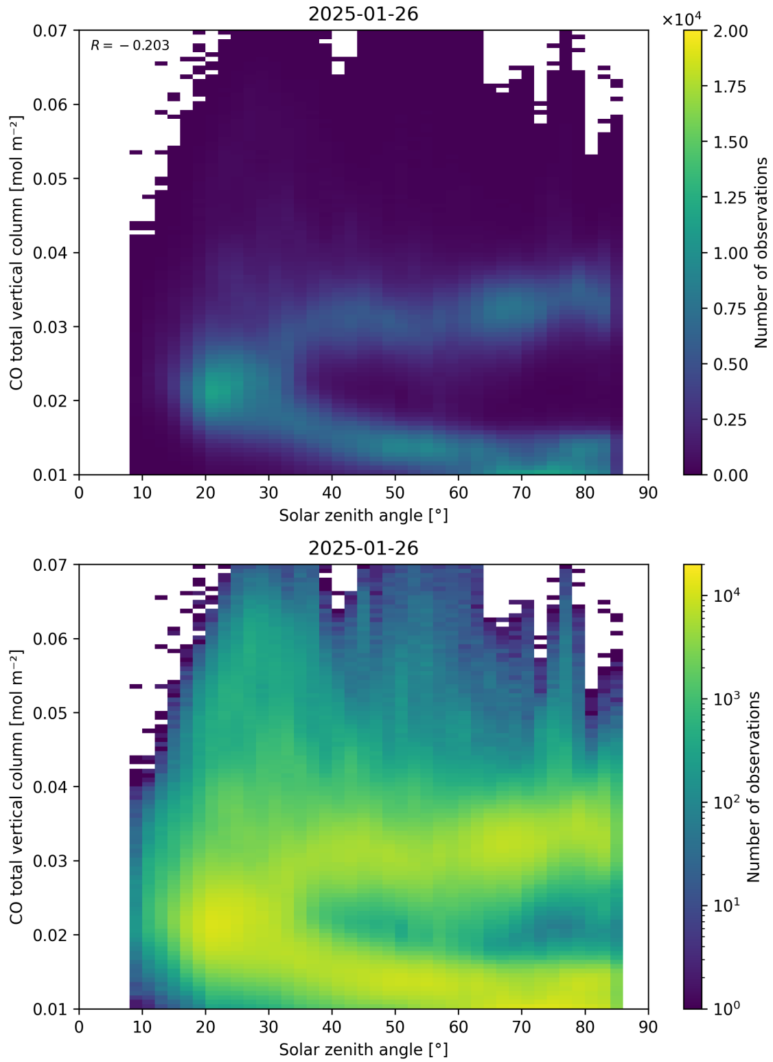
Figure 61: Scatter density plot of “Solar zenith angle” against “CO total vertical column” for 2025-01-25 to 2025-01-27.
