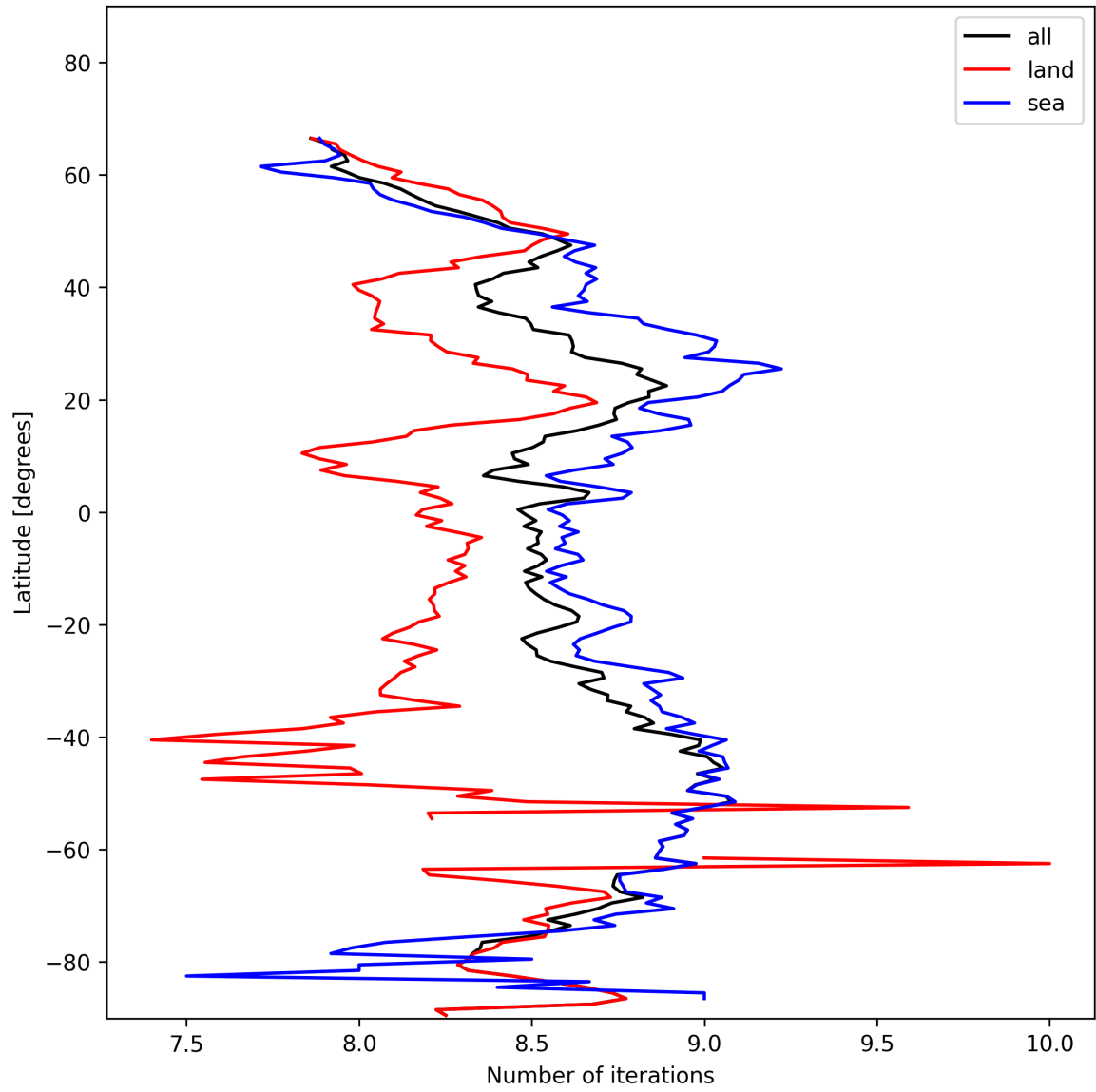
Figure 16: Zonal average of “Number of iterations” for 2025-01-25 to 2025-01-27.
