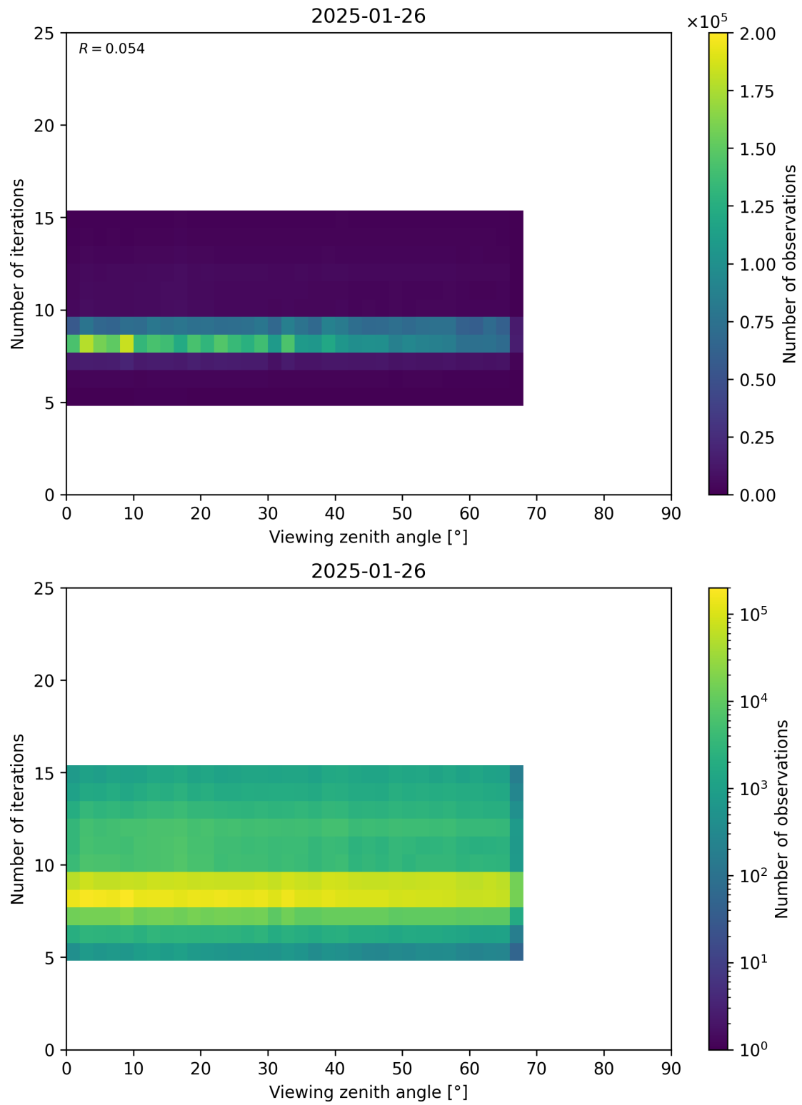
Figure 75: Scatter density plot of “Viewing zenith angle” against “Number of iterations” for 2025-01-25 to 2025-01-27.
