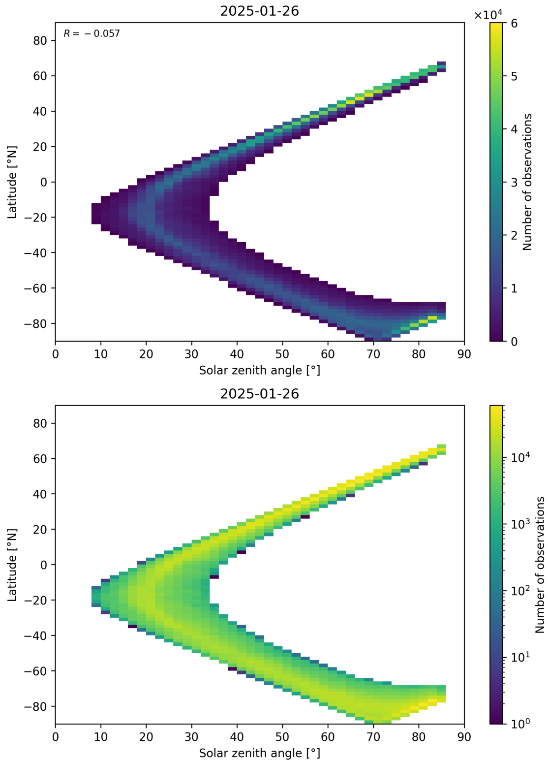
Figure 66: Scatter density plot of “Solar zenith angle” against “Latitude” for 2025-01-25 to 2025-01-27.
