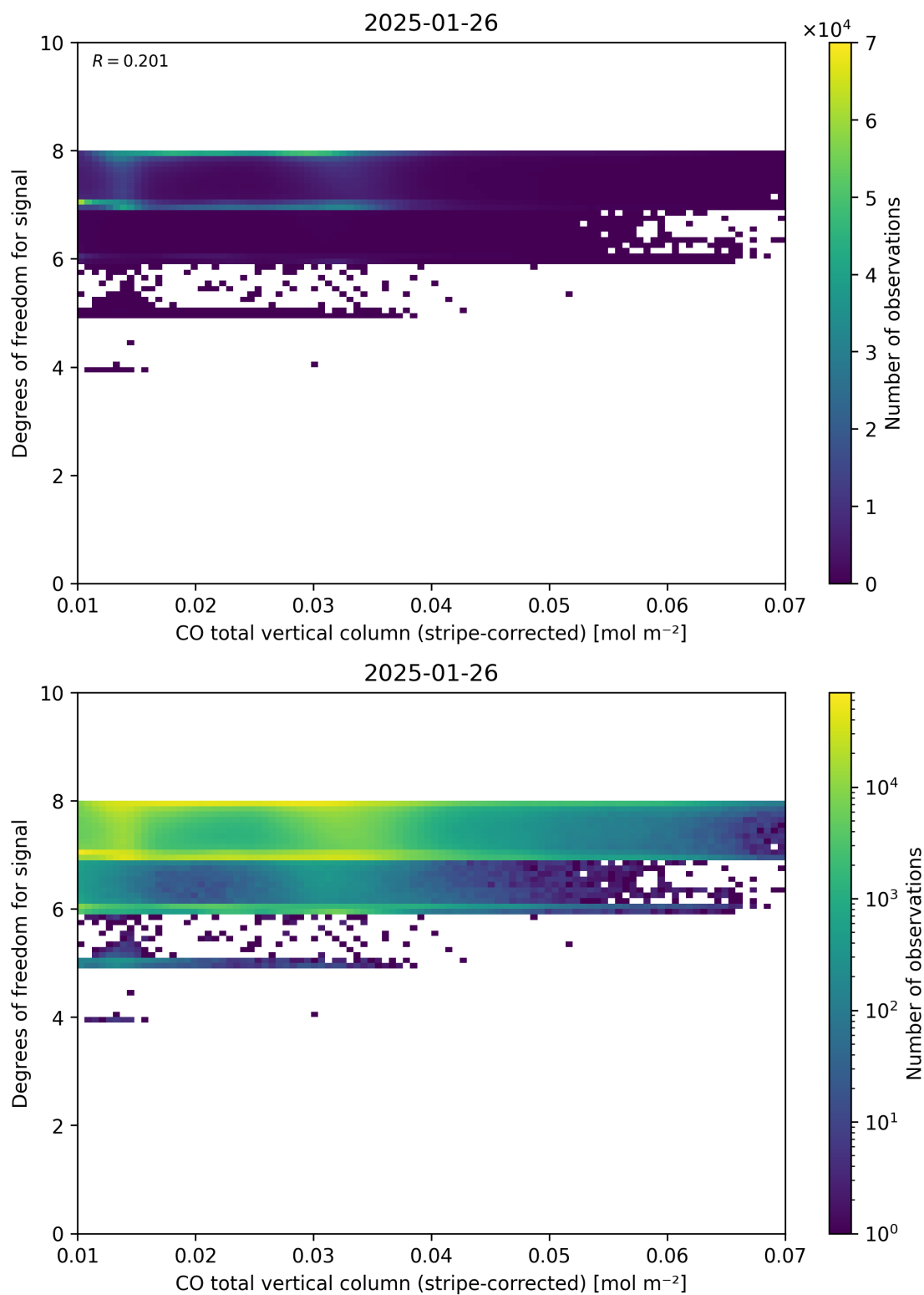
Figure 38: Scatter density plot of “CO total vertical column (stripe-corrected)” against “Degrees of freedom for signal” for 2025-01-25 to 2025-01-27.
