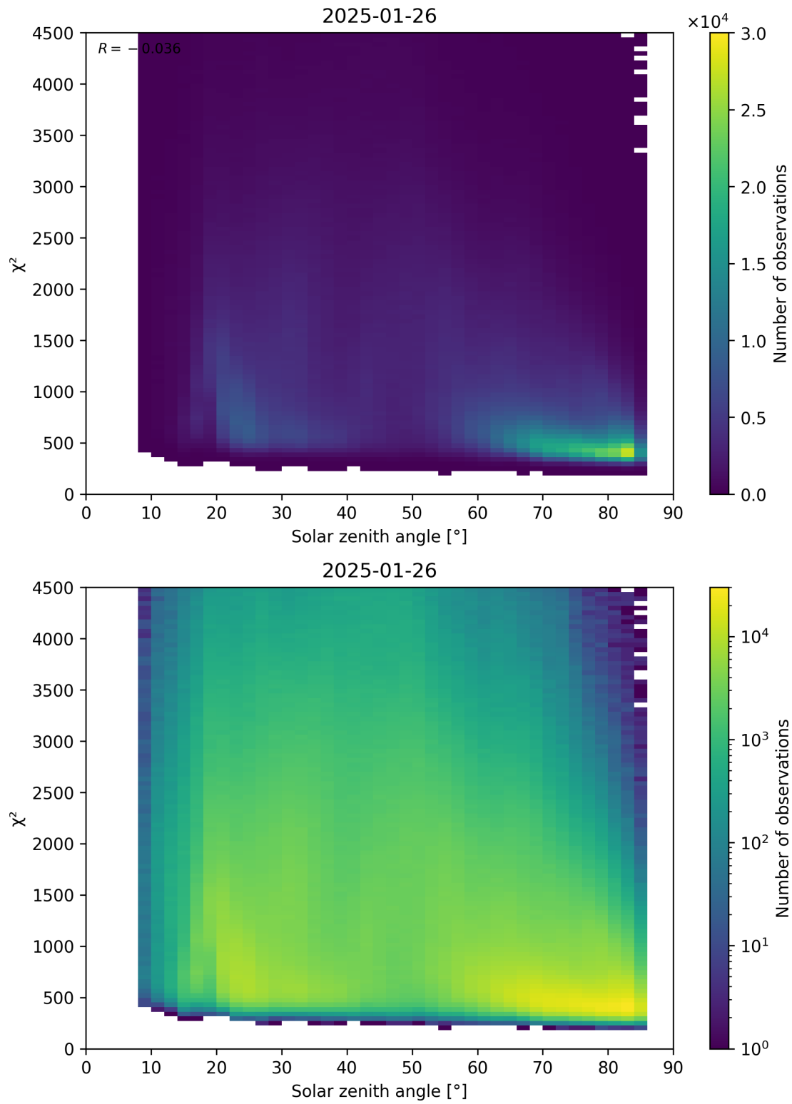
Figure 64: Scatter density plot of “Solar zenith angle” against “ \chi^2 ” for 2025-01-25 to 2025-01-27.
