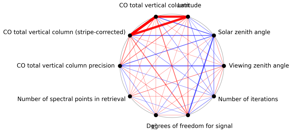
Figure 1: Map of correlation graph for 2025-01-25 to 2025-01-27.
