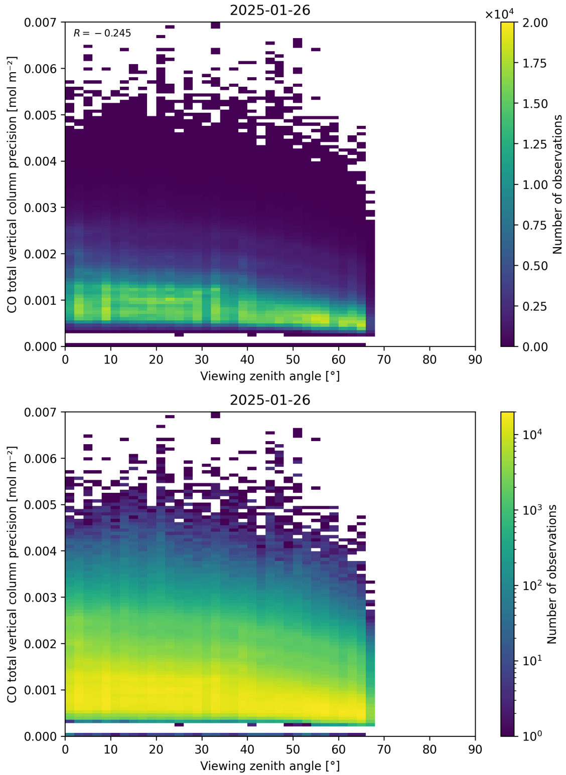
Figure 71: Scatter density plot of “Viewing zenith angle” against “CO total vertical column precision” for 2025-01-25 to 2025-01-27.
