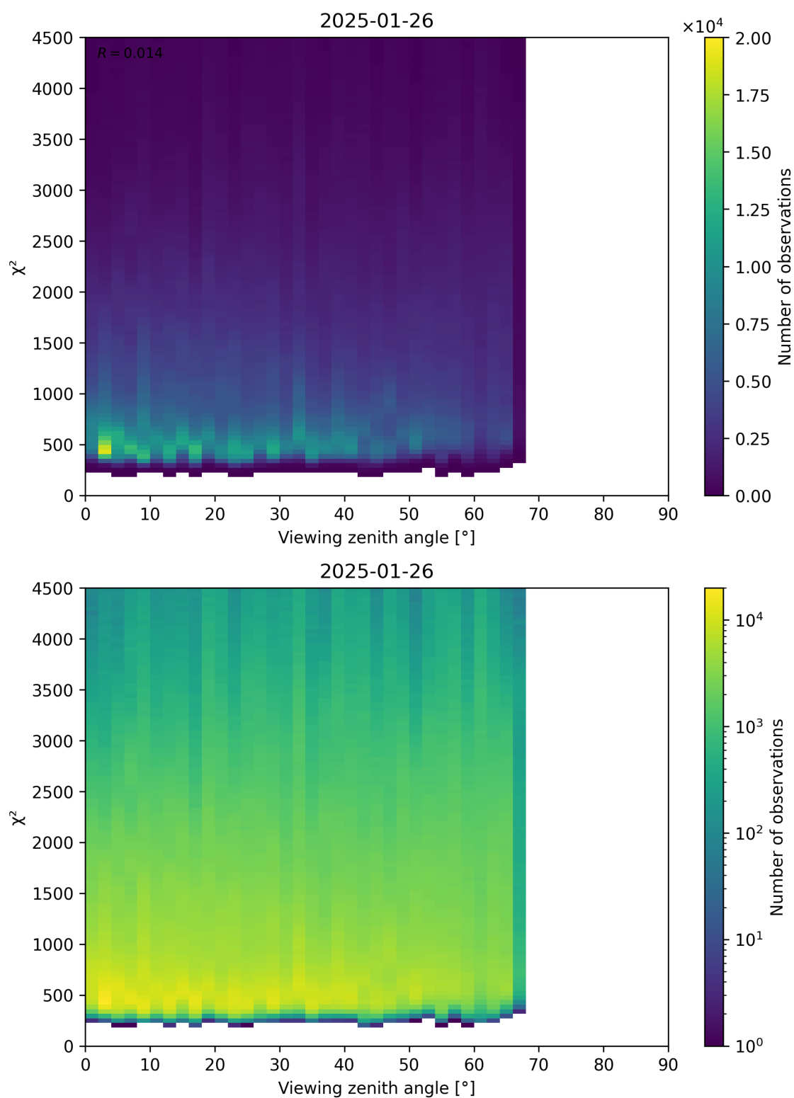
Figure 72: Scatter density plot of “Viewing zenith angle” against “ \chi^2 ” for 2025-01-25 to 2025-01-27.
