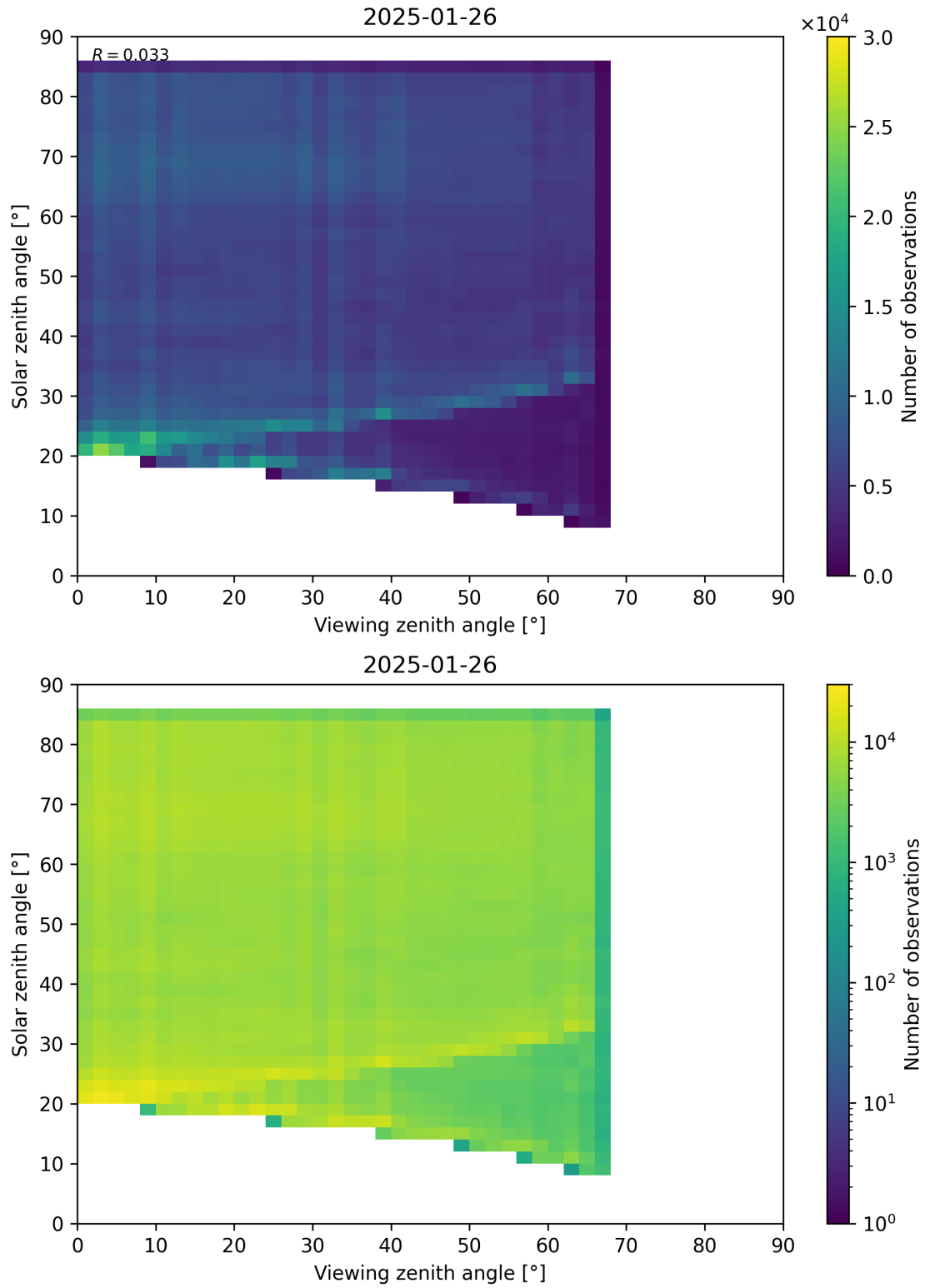
Figure 77: Scatter density plot of “Viewing zenith angle” against “Solar zenith angle” for 2025-01-25 to 2025-01-27.
