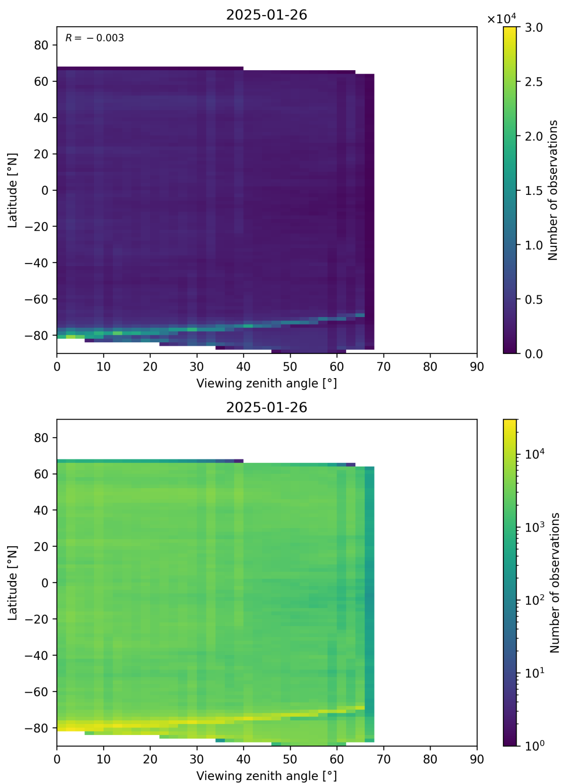
Figure 74: Scatter density plot of “Viewing zenith angle” against “Latitude” for 2025-01-25 to 2025-01-27.
