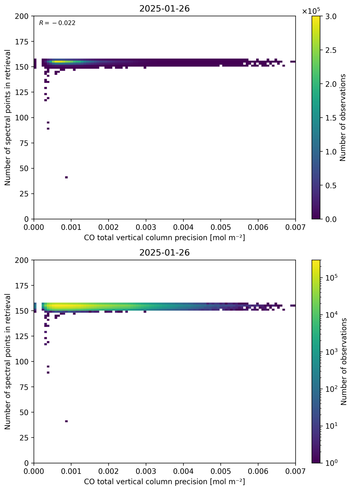
Figure 47: Scatter density plot of “CO total vertical column precision” against “Number of spectral points in retrieval” for 2025-01-25 to 2025-01-27.
