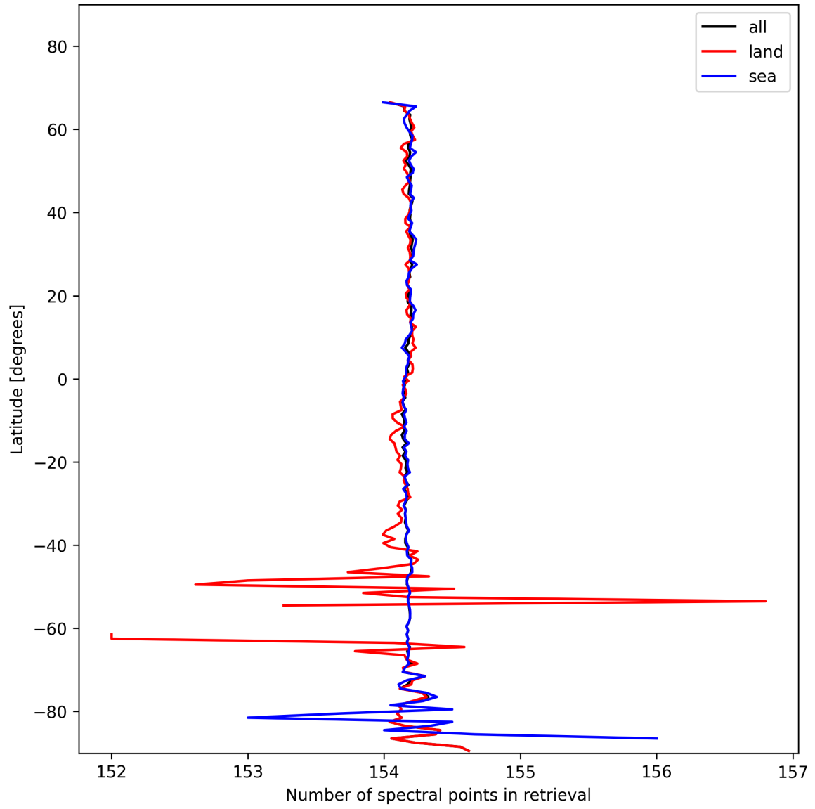
Figure 13: Zonal average of “Number of spectral points in retrieval” for 2025-01-25 to 2025-01-27.
