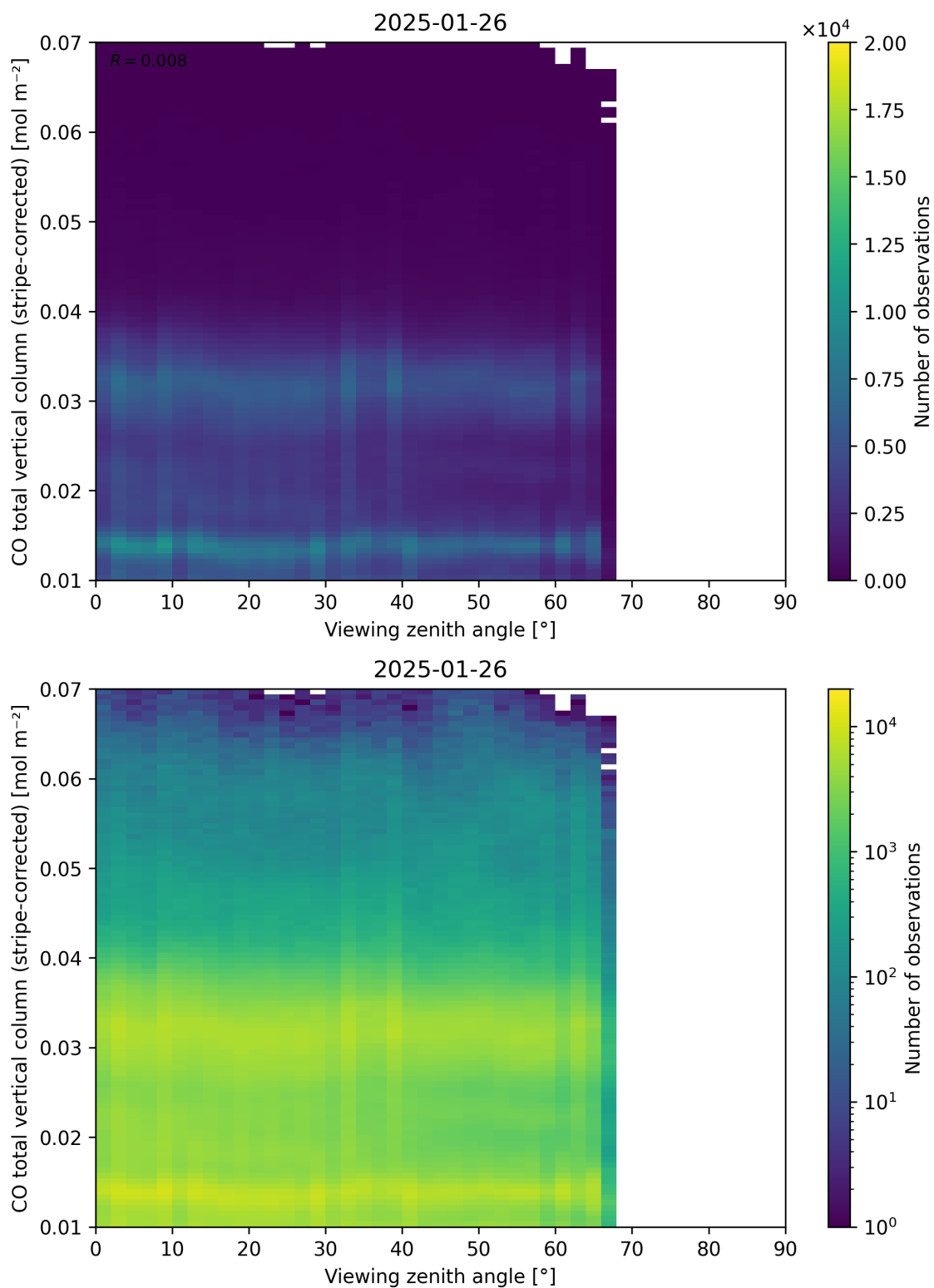
Figure 70: Scatter density plot of “Viewing zenith angle” against “CO total vertical column (stripe-corrected)” for 2025-01-25 to 2025-01-27.
