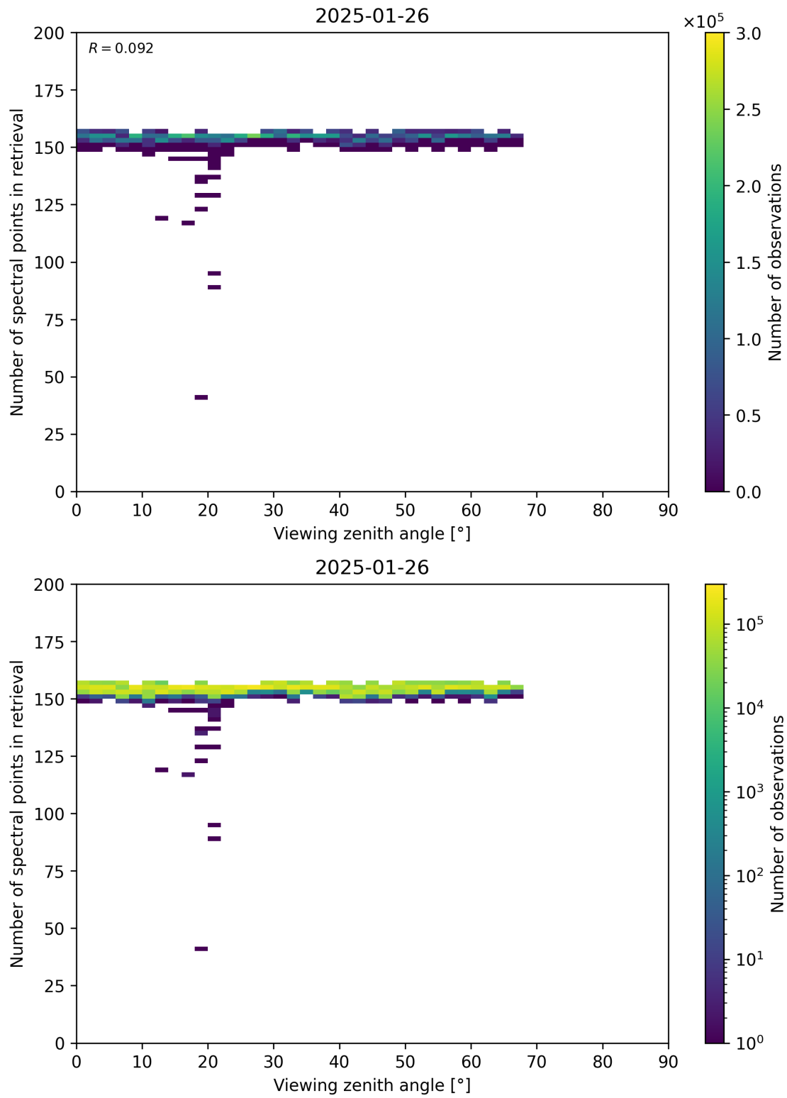
Figure 76: Scatter density plot of “Viewing zenith angle” against “Number of spectral points in retrieval” for 2025-01-25 to 2025-01-27.
