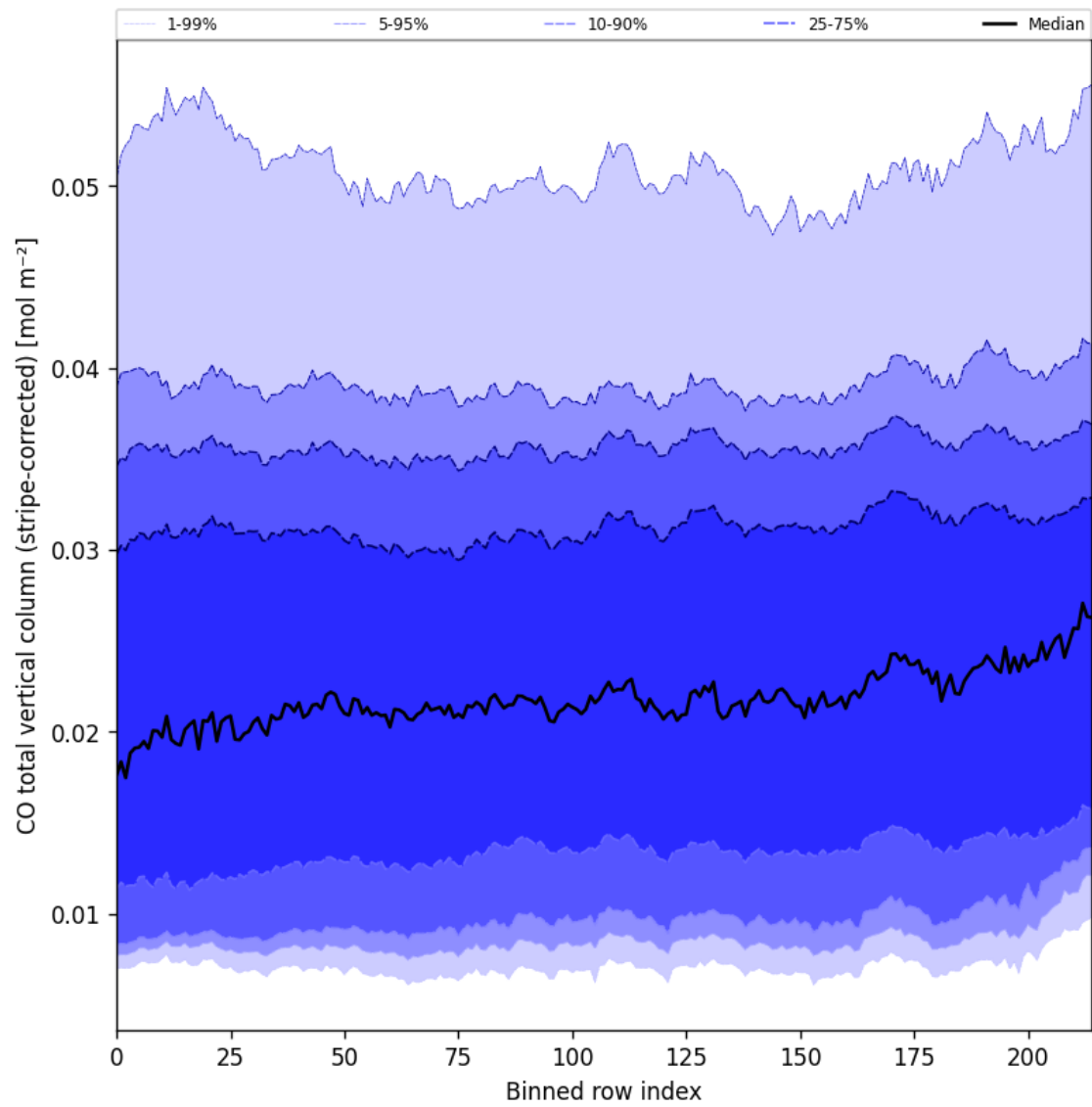
Figure 27: Along track statistics of “CO total vertical column (stripe-corrected)” for 2025-01-25 to 2025-01-27
