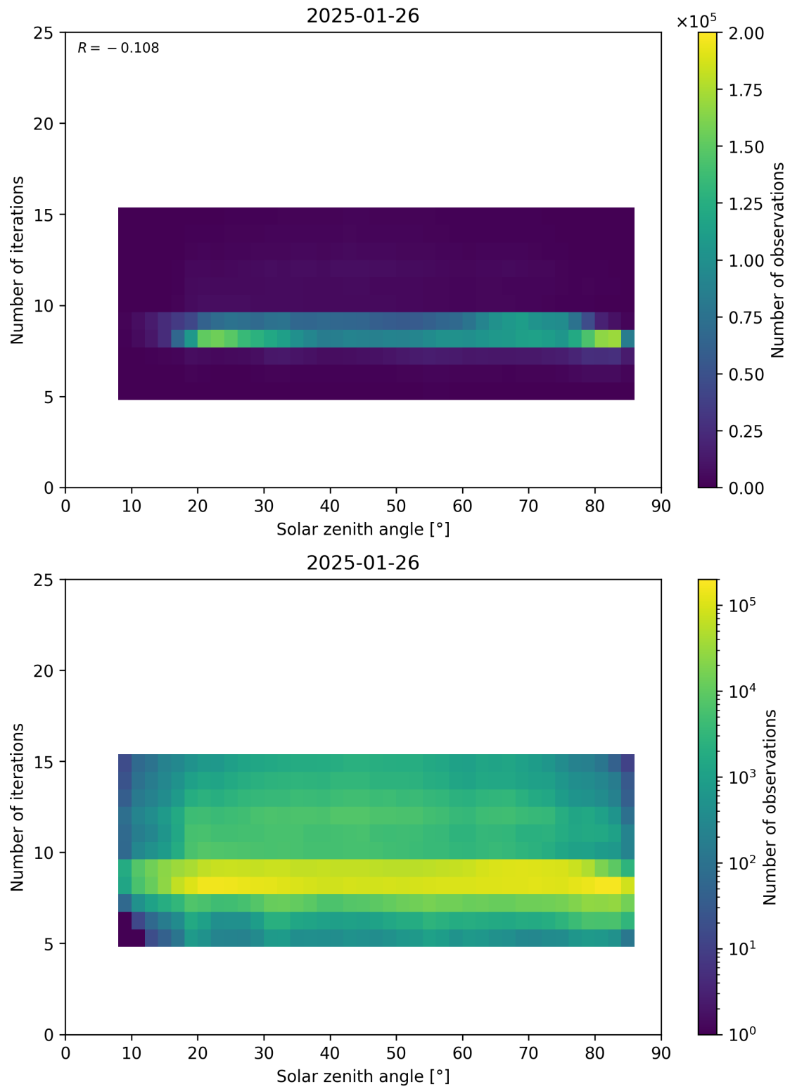
Figure 67: Scatter density plot of “Solar zenith angle” against “Number of iterations” for 2025-01-25 to 2025-01-27.
