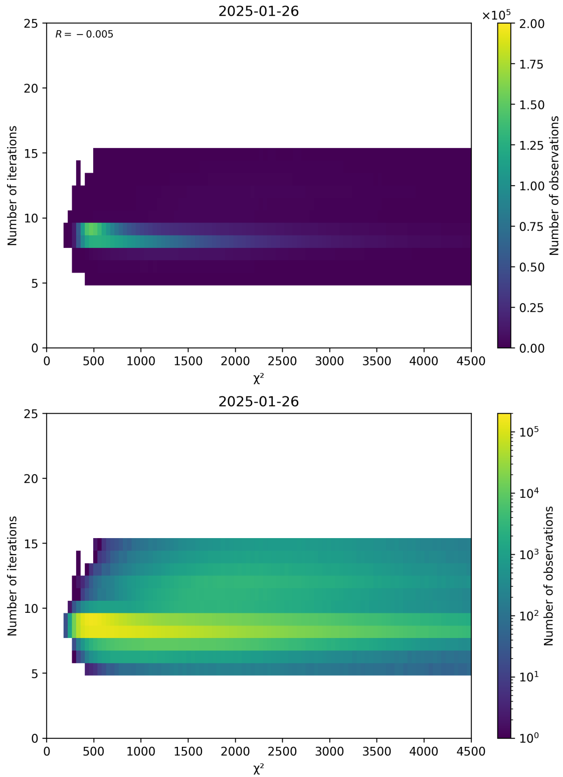
Figure 49: Scatter density plot of “ \chi^2 ” against “Number of iterations” for 2025-01-25 to 2025-01-27.
