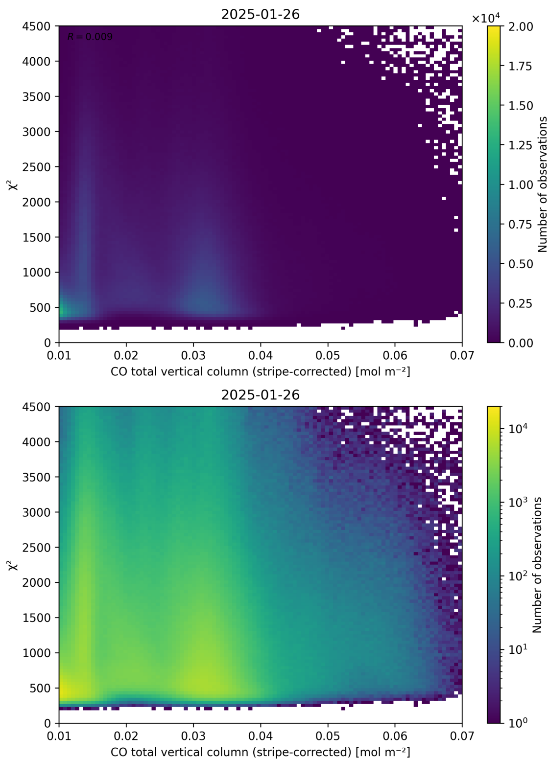
Figure 37: Scatter density plot of “CO total vertical column (stripe-corrected)” against “ \chi^2 ” for 2025-01-25 to 2025-01-27.
