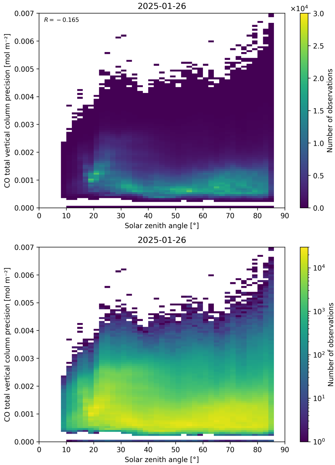
Figure 63: Scatter density plot of “Solar zenith angle” against “CO total vertical column precision” for 2025-01-25 to 2025-01-27.
