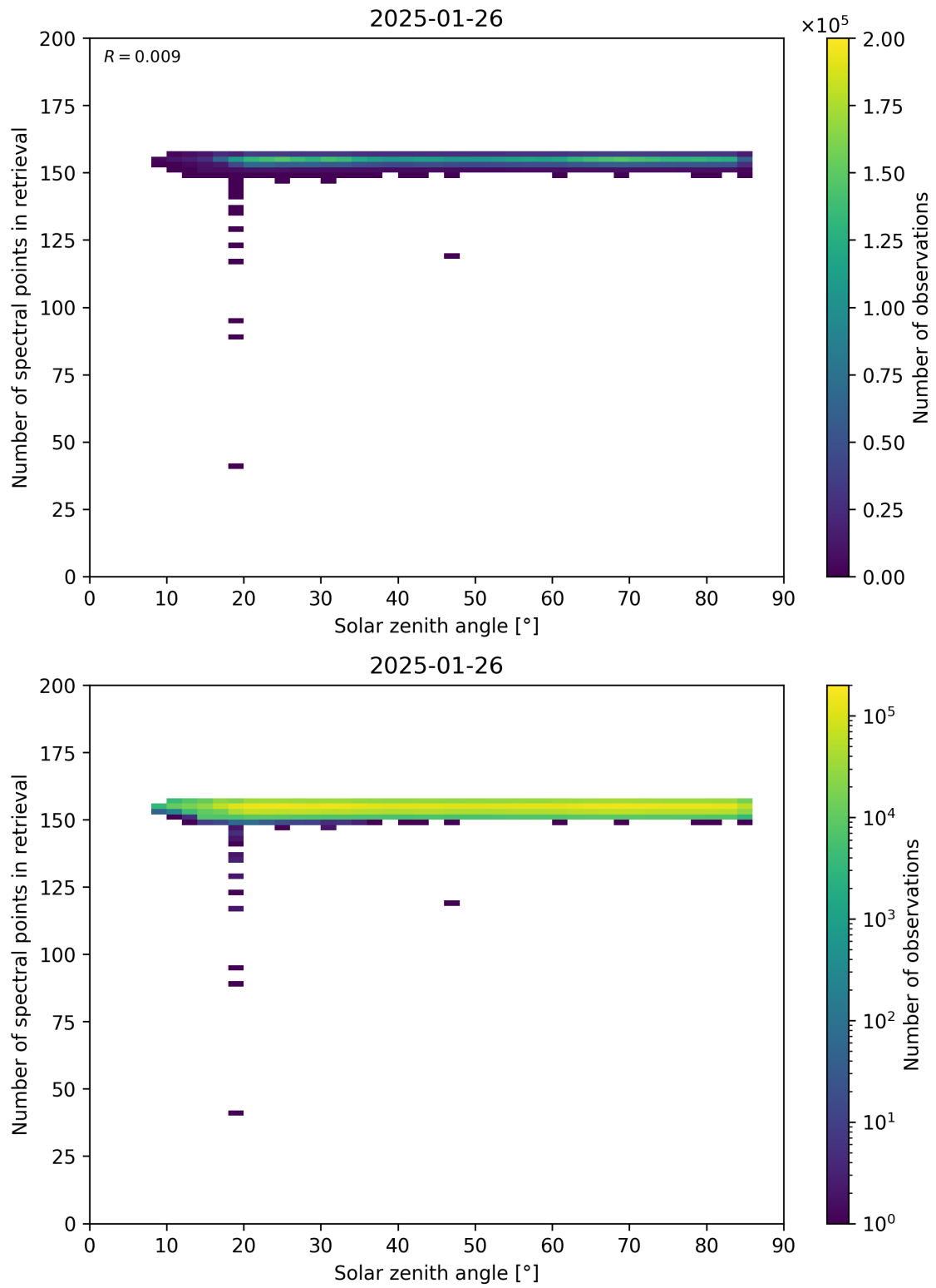
Figure 68: Scatter density plot of “Solar zenith angle” against “Number of spectral points in retrieval” for 2025-01-25 to 2025-01-27.
