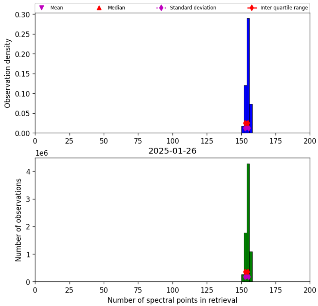
Figure 21: Histogram of “Number of spectral points in retrieval” for 2025-01-25 to 2025-01-27
