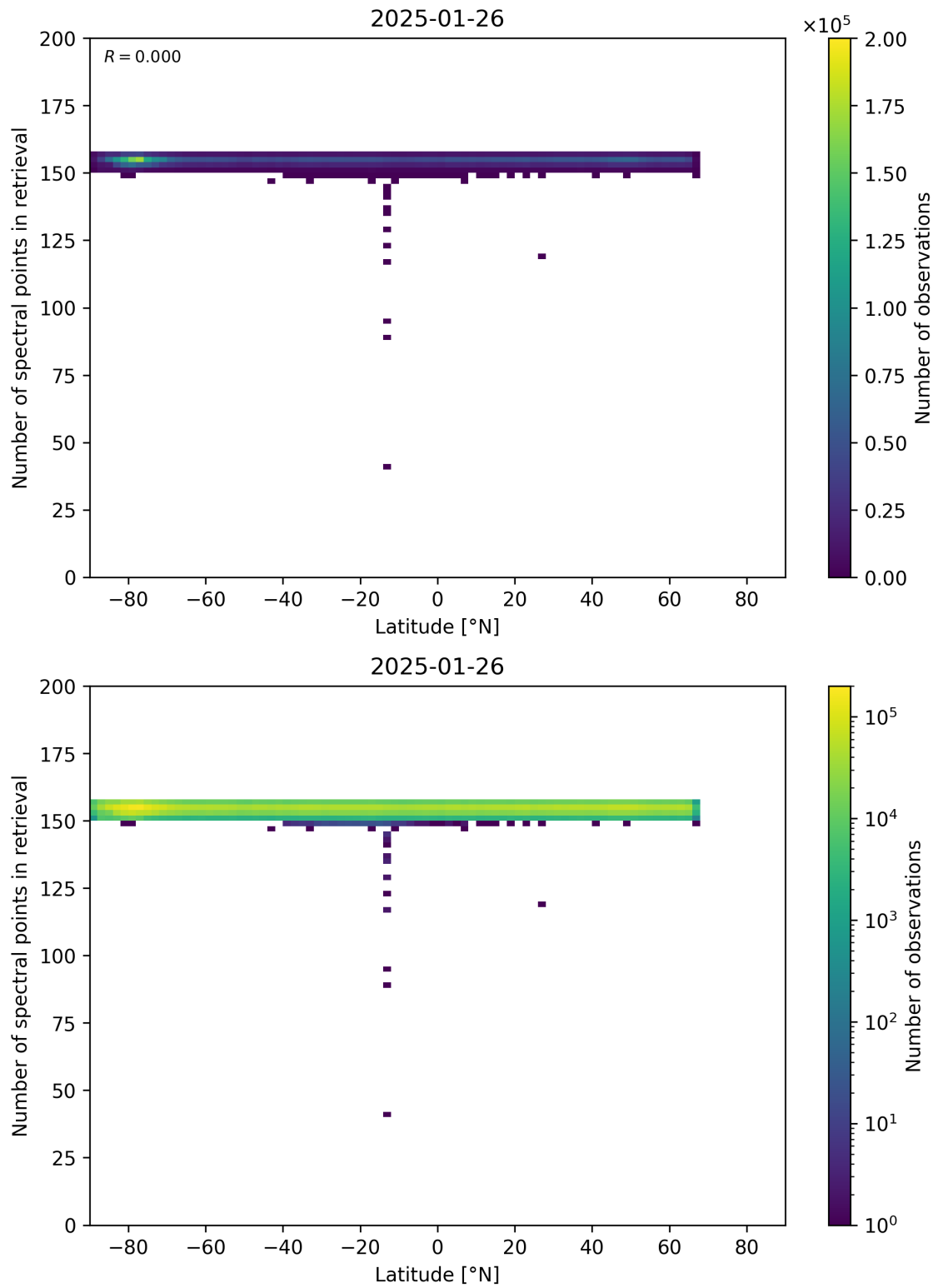
Figure 57: Scatter density plot of “Latitude” against “Number of spectral points in retrieval” for 2025-01-25 to 2025-01-27.
