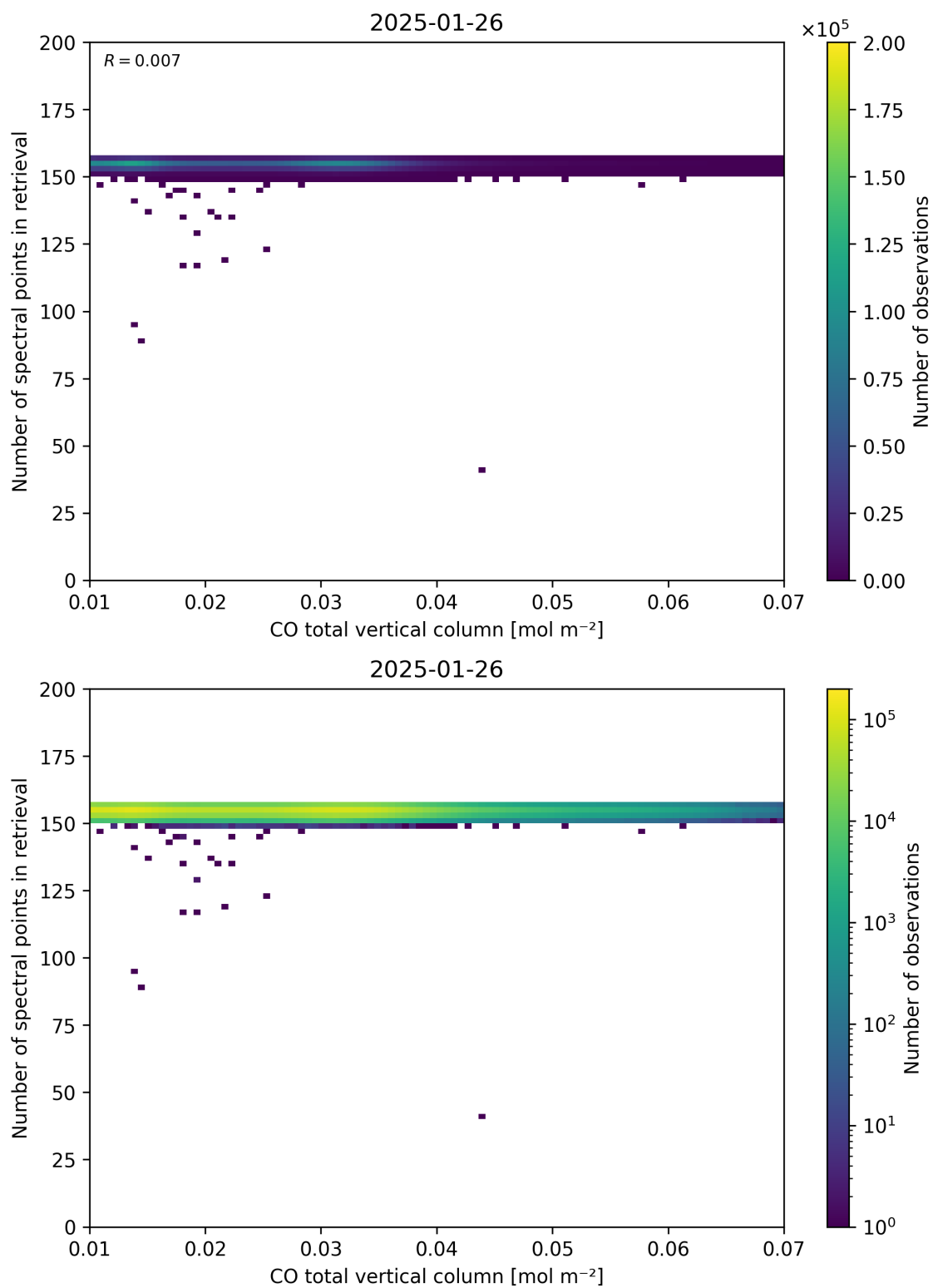
Figure 43: Scatter density plot of “CO total vertical column” against “Number of spectral points in retrieval” for 2025-01-25 to 2025-01-27.
