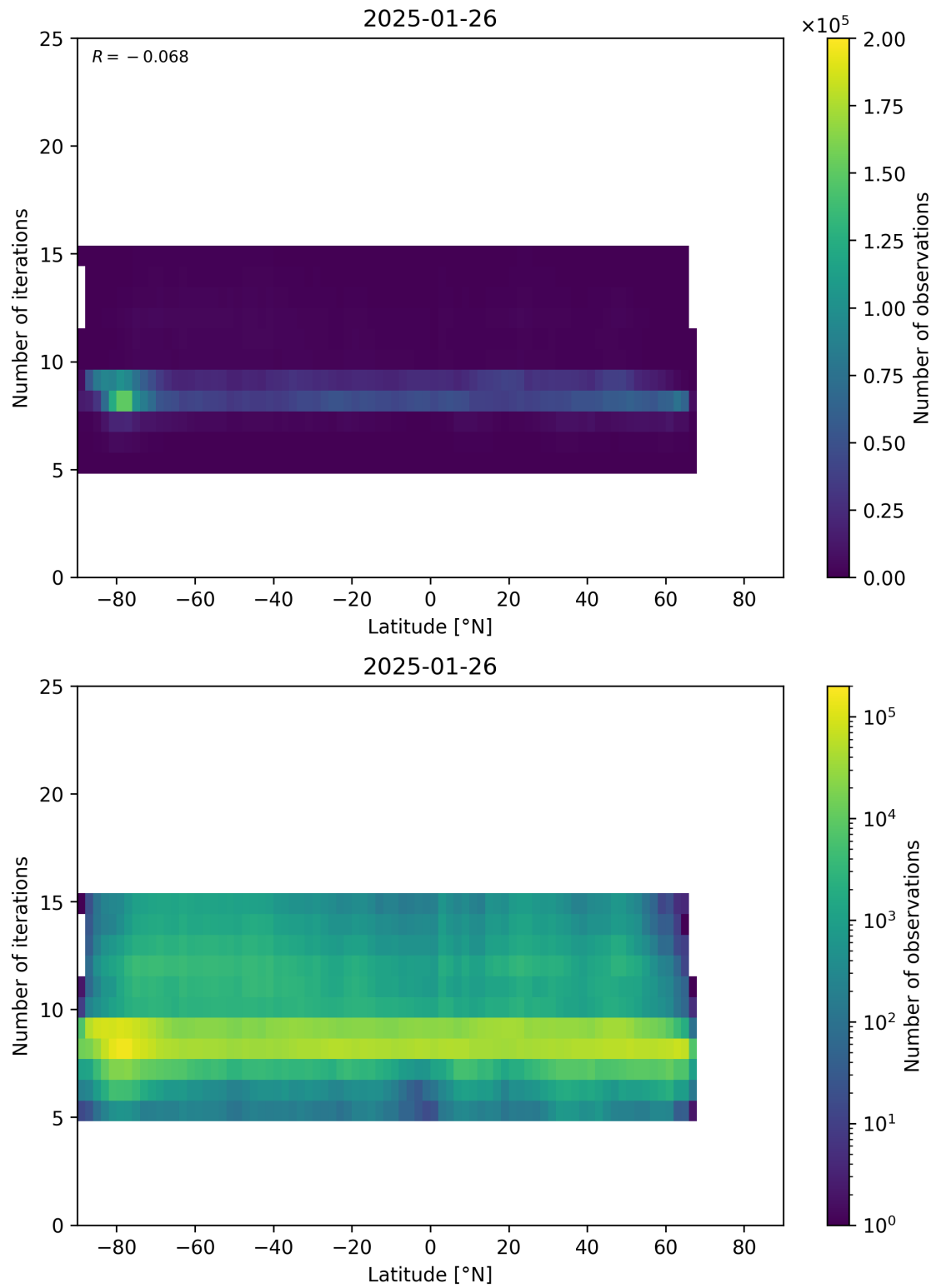
Figure 56: Scatter density plot of “Latitude” against “Number of iterations” for 2025-01-25 to 2025-01-27.
