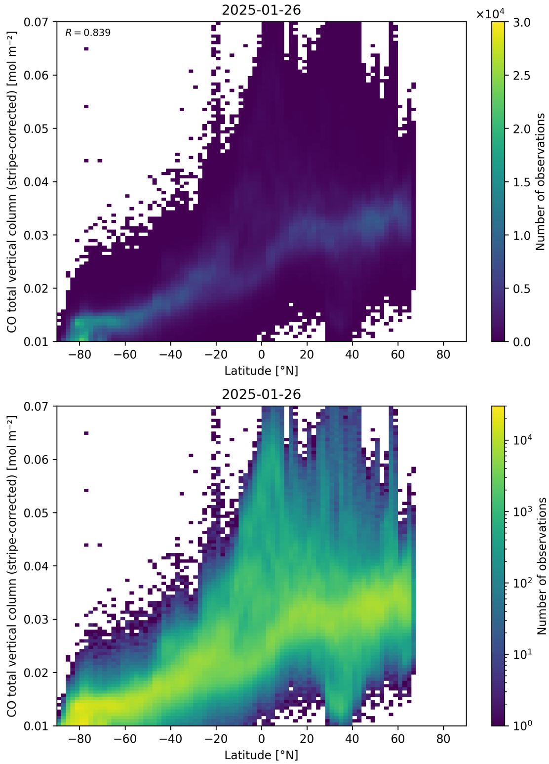
Figure 52: Scatter density plot of “Latitude” against “CO total vertical column (stripe-corrected)” for 2025-01-25 to 2025-01-27.
