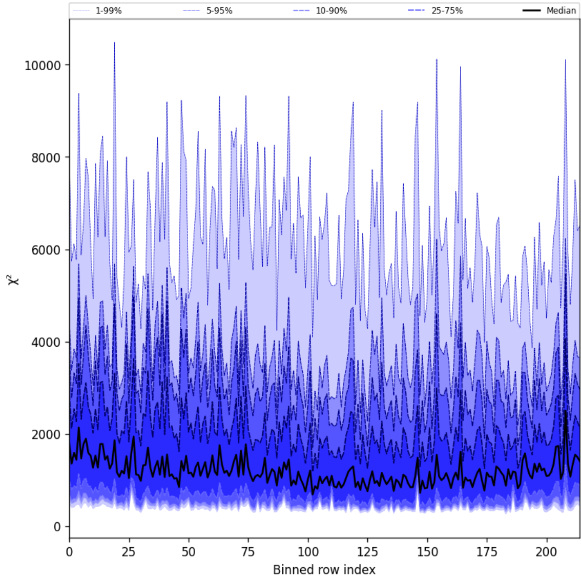
Figure 30: Along track statistics of “ \chi^2 ” for 2025-01-25 to 2025-01-27
