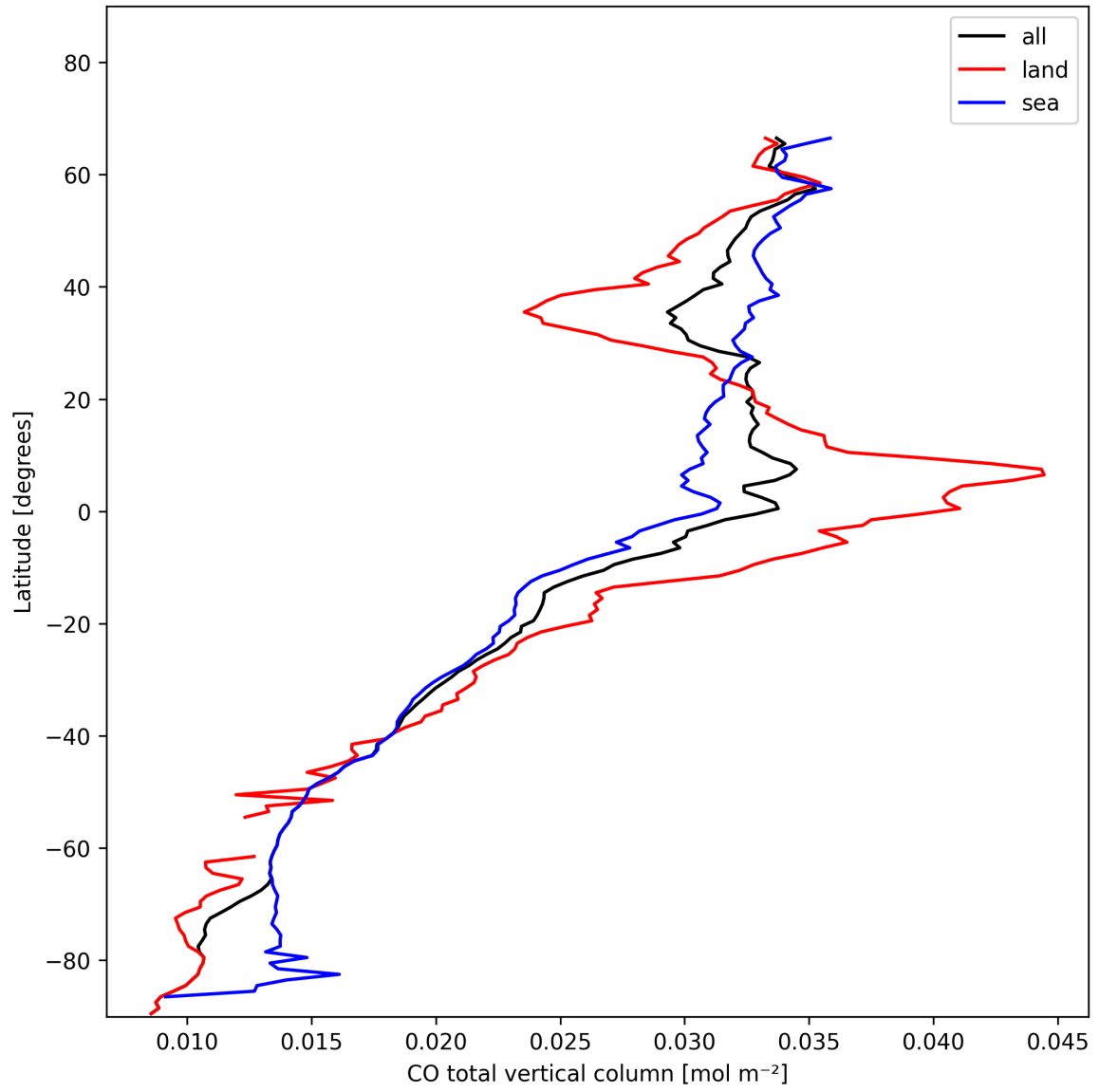
Figure 10: Zonal average of “CO total vertical column” for 2025-01-25 to 2025-01-27.
