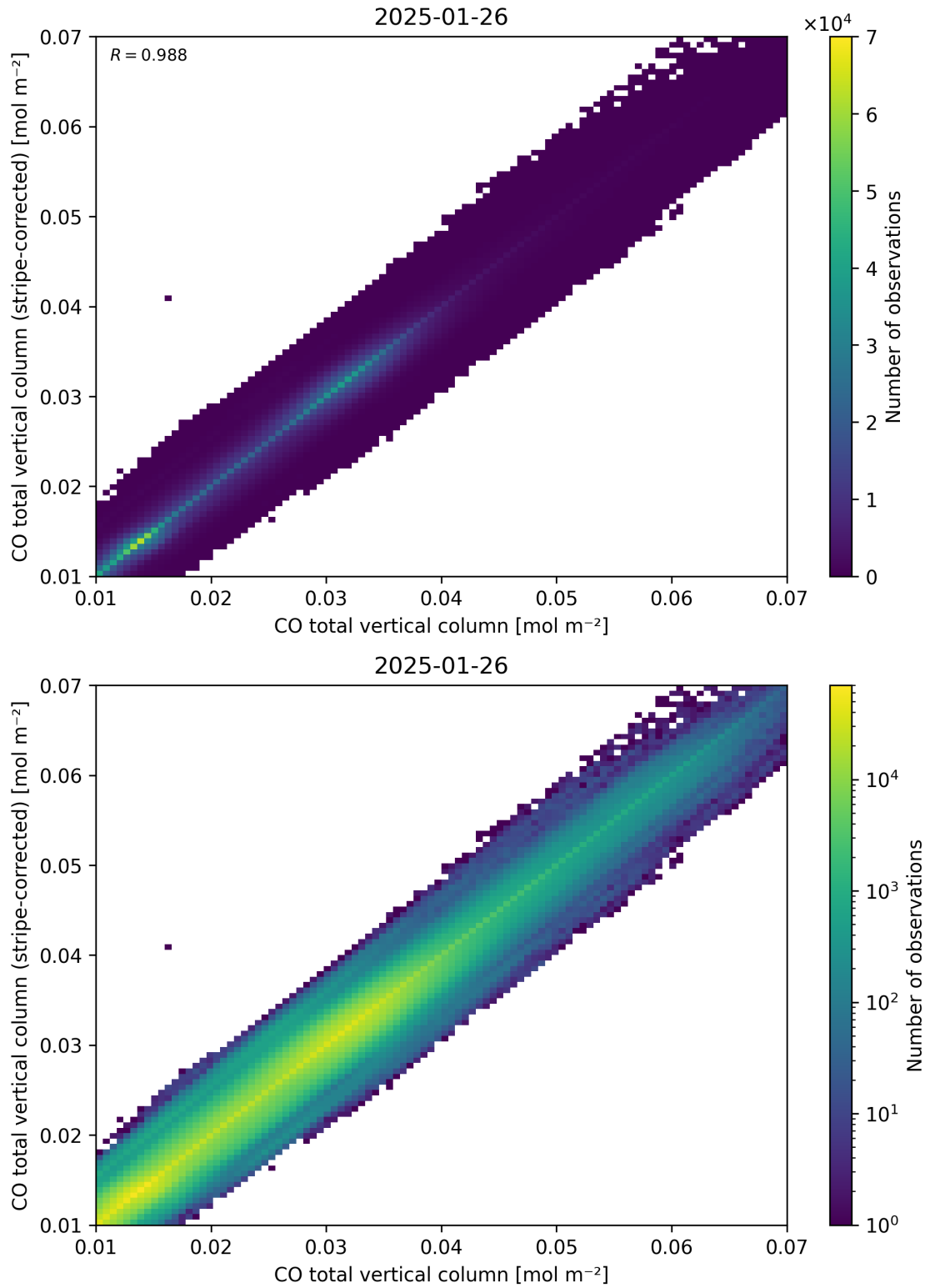
Figure 33: Scatter density plot of “CO total vertical column” against “CO total vertical column (stripe-corrected)” for 2025-01-25 to 2025-01-27.
