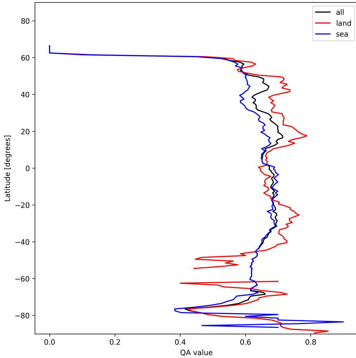
Figure 9: Zonal average of “QA value” for 2025-01-25 to 2025-01-27.
