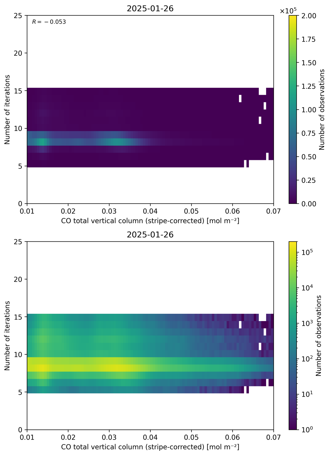
Figure 39: Scatter density plot of “CO total vertical column (stripe-corrected)” against “Number of iterations” for 2025-01-25 to 2025-01-27.
