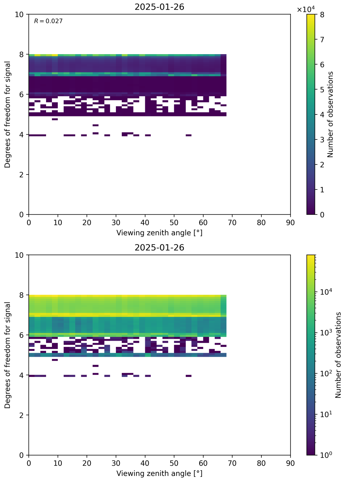
Figure 73: Scatter density plot of “Viewing zenith angle” against “Degrees of freedom for signal” for 2025-01-25 to 2025-01-27.
