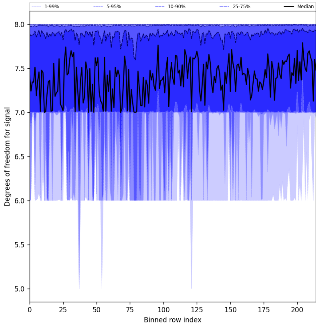
Figure 31: Along track statistics of “Degrees of freedom for signal” for 2025-01-25 to 2025-01-27
