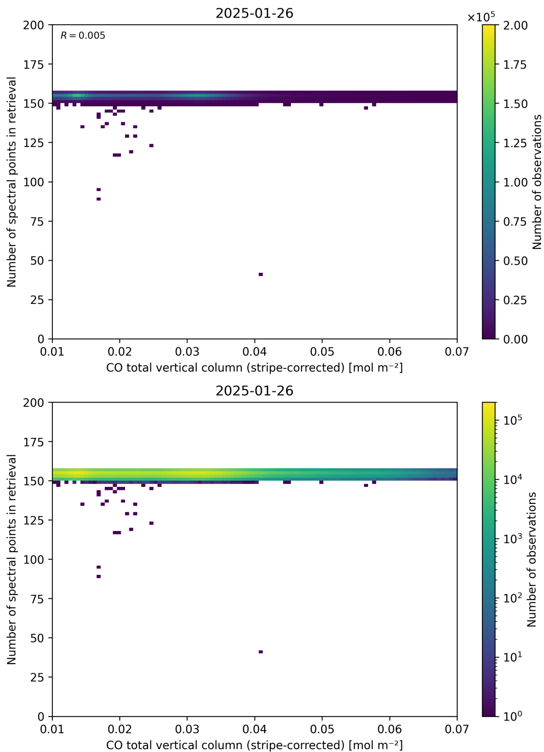
Figure 40: Scatter density plot of “CO total vertical column (stripe-corrected)” against “Number of spectral points in retrieval” for 2025-01-25 to 2025-01-27.
