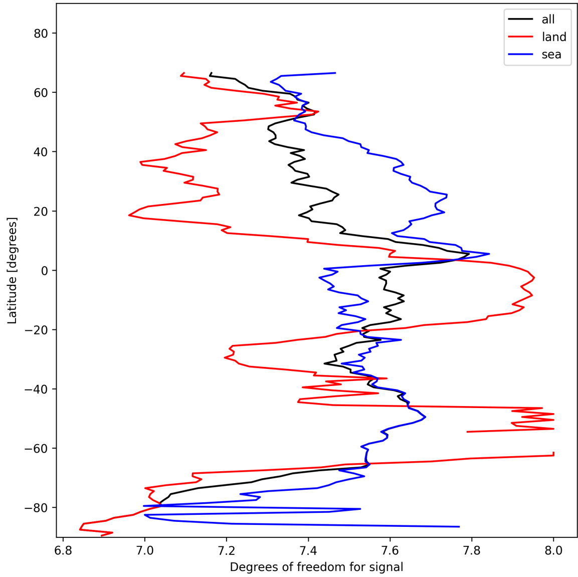
Figure 15: Zonal average of “Degrees of freedom for signal” for 2025-01-25 to 2025-01-27.
