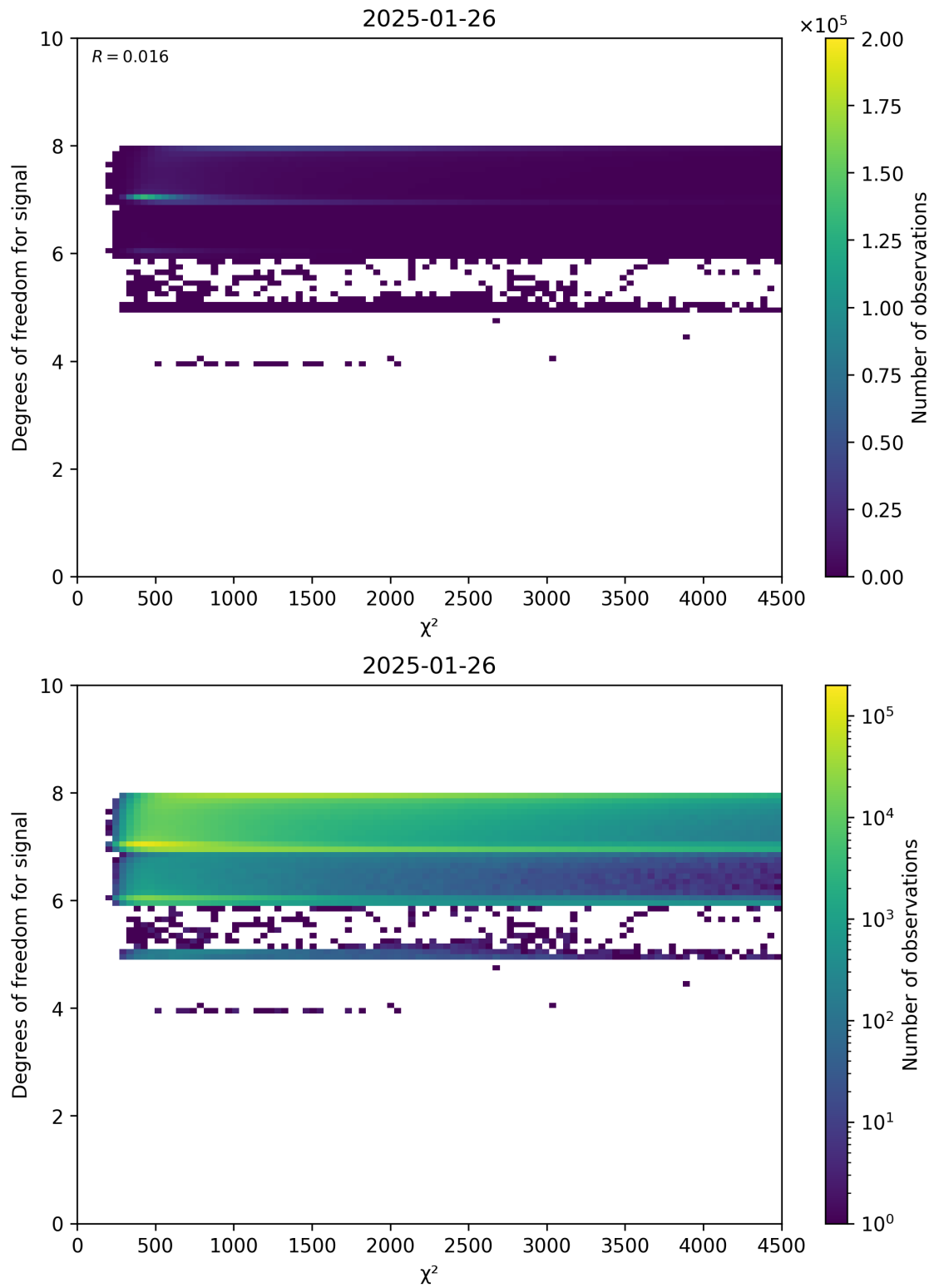
Figure 48: Scatter density plot of “ \chi^2 ” against “Degrees of freedom for signal” for 2025-01-25 to 2025-01-27.
