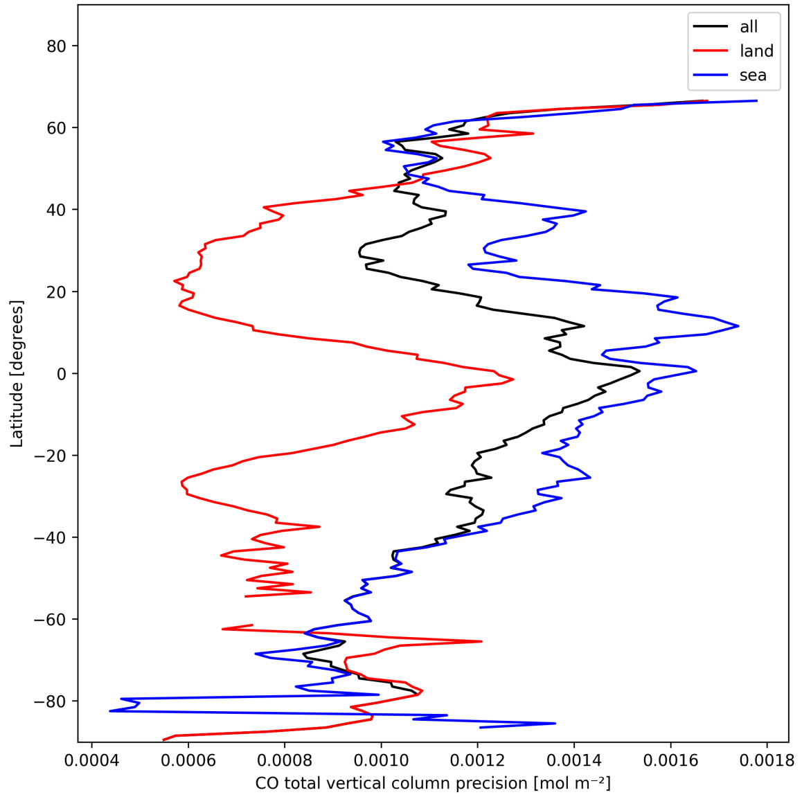
Figure 12: Zonal average of “CO total vertical column precision” for 2025-01-25 to 2025-01-27.
