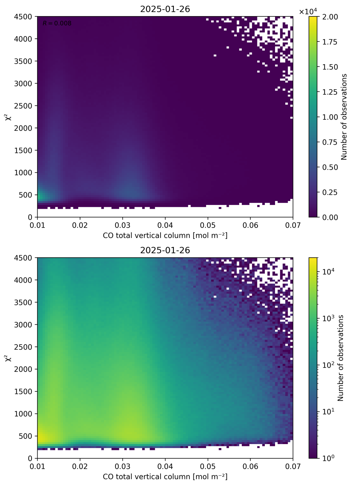
Figure 35: Scatter density plot of “CO total vertical column” against “ \chi^2 ” for 2025-01-25 to 2025-01-27.
