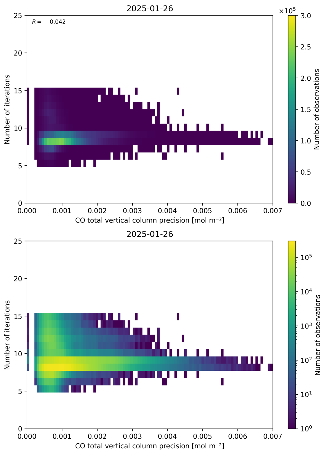
Figure 46: Scatter density plot of “CO total vertical column precision” against “Number of iterations” for 2025-01-25 to 2025-01-27.
