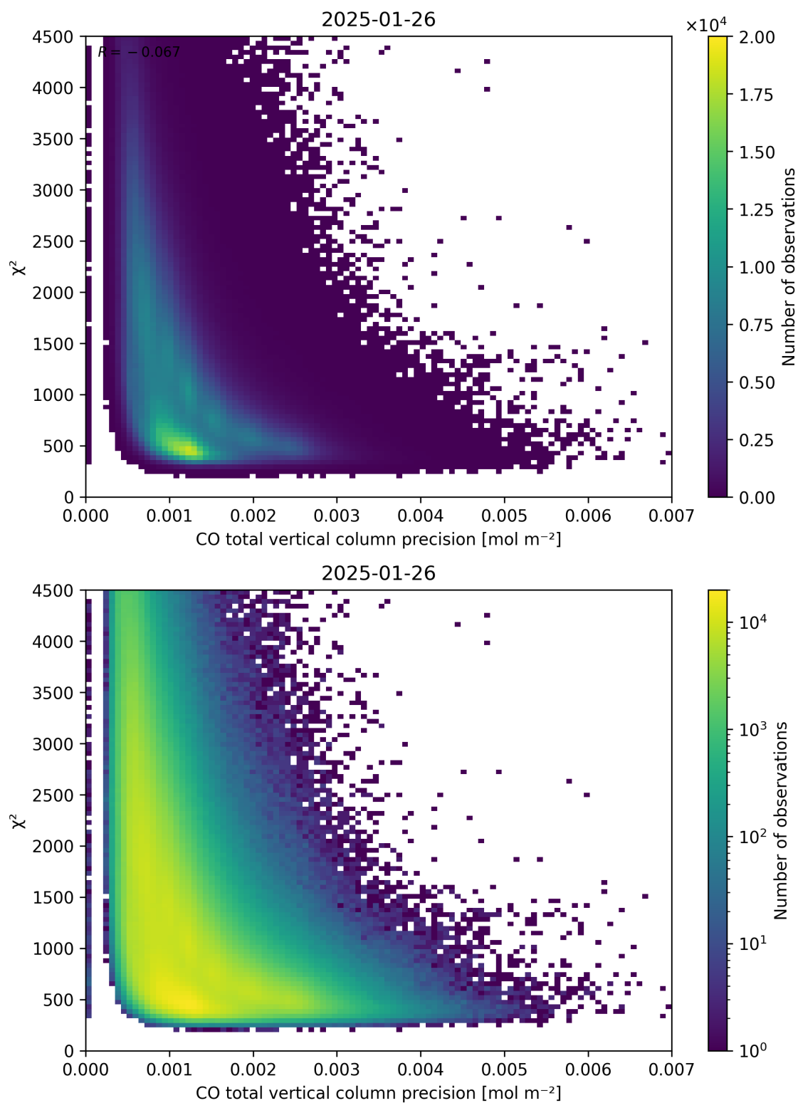
Figure 44: Scatter density plot of “CO total vertical column precision” against “ \chi^2 ” for 2025-01-25 to 2025-01-27.
