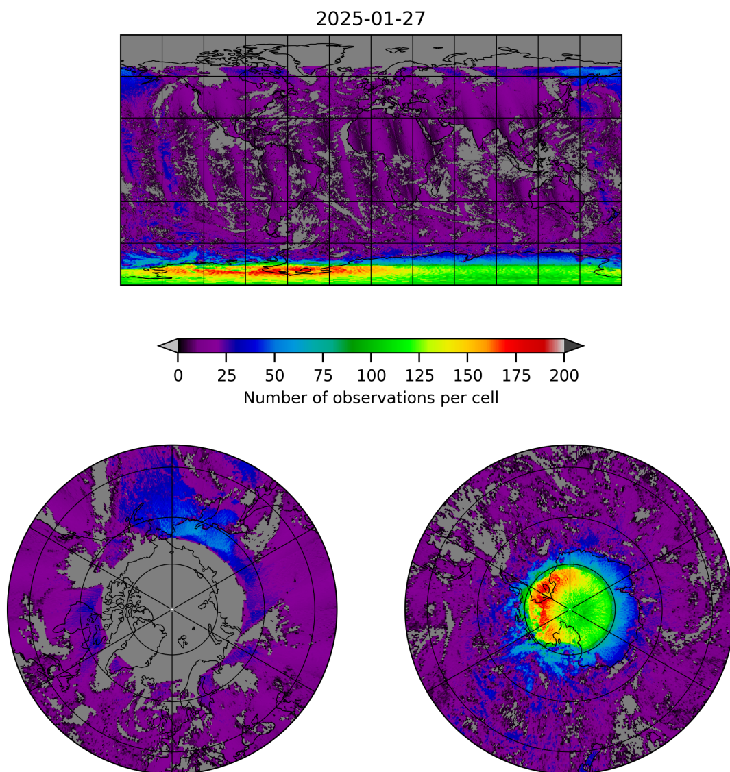
Figure 8: Map of the number of observations for 2025-01-26 to 2025-01-28
