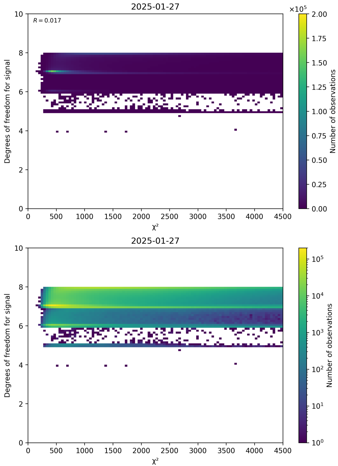
Figure 48: Scatter density plot of “ \chi^2 ” against “Degrees of freedom for signal” for 2025-01-26 to 2025-01-28.
