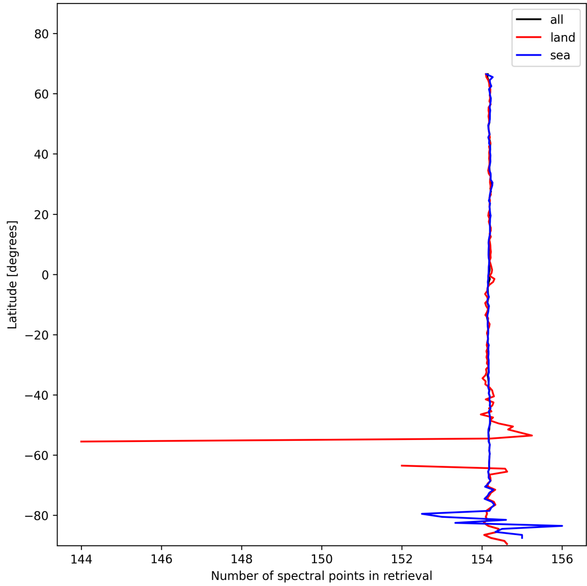
Figure 13: Zonal average of “Number of spectral points in retrieval” for 2025-01-26 to 2025-01-28.
