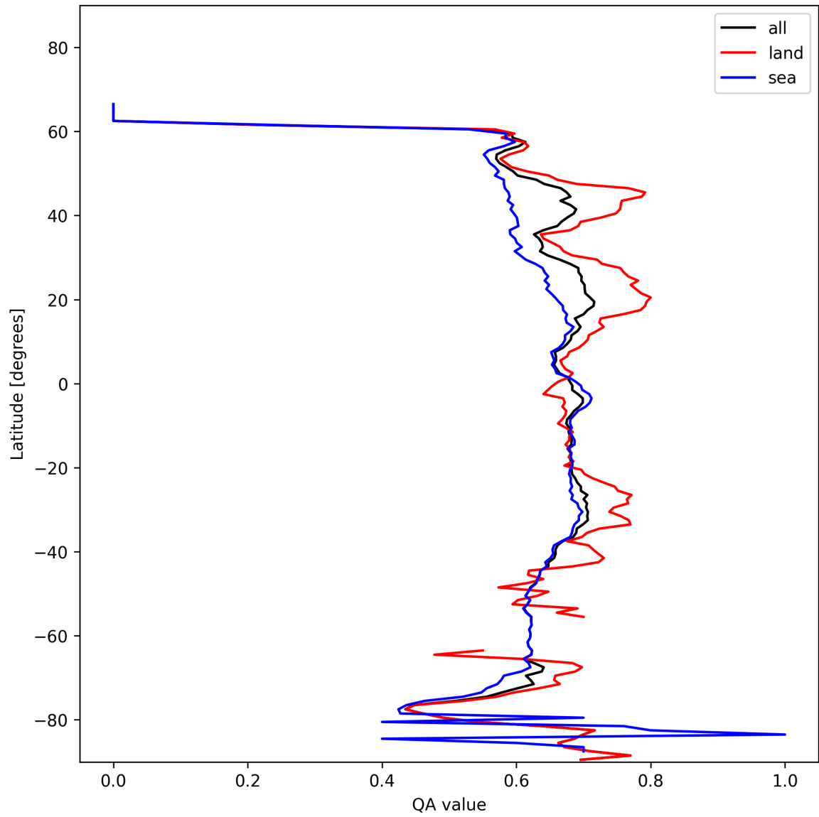
Figure 9: Zonal average of “QA value” for 2025-01-26 to 2025-01-28.
