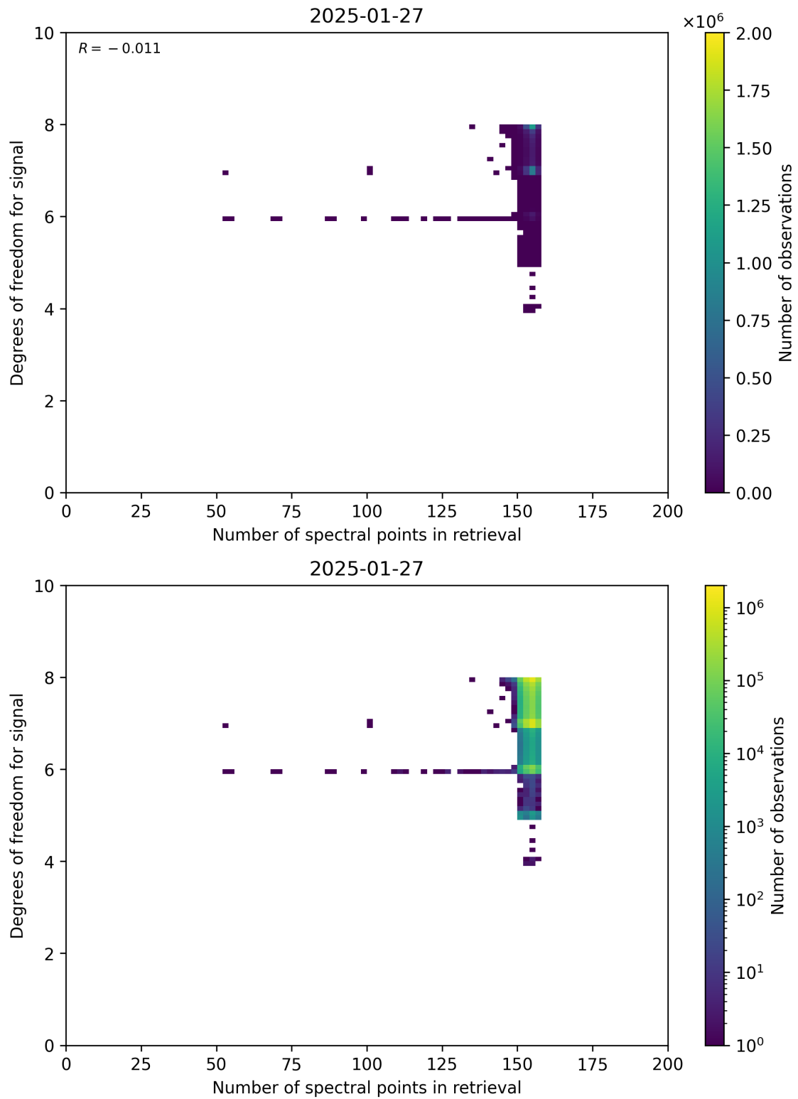
Figure 59: Scatter density plot of “Number of spectral points in retrieval” against “Degrees of freedom for signal” for 2025-01-26 to 2025-01-28.
