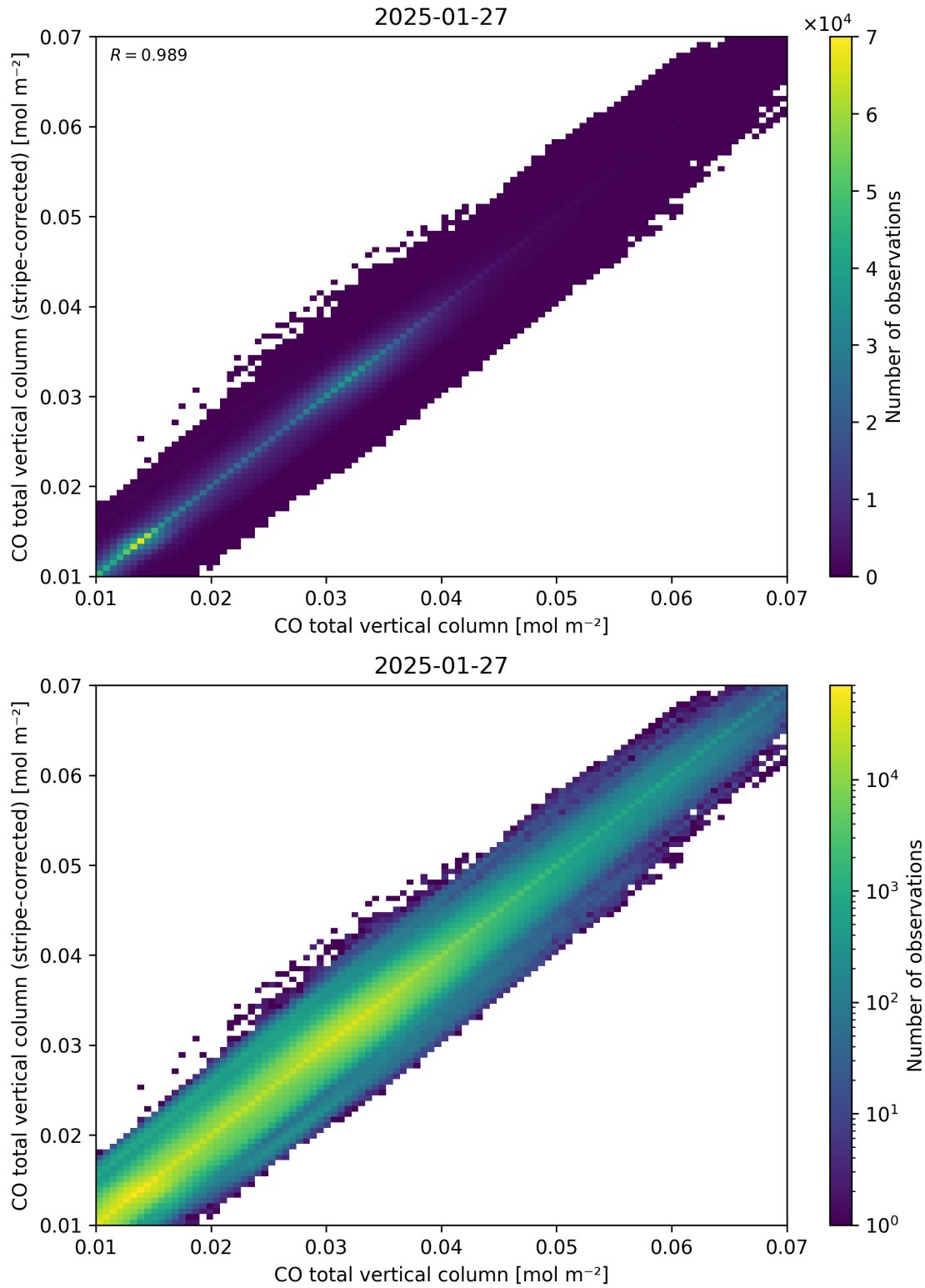
Figure 33: Scatter density plot of “CO total vertical column” against “CO total vertical column (stripe-corrected)” for 2025-01-26 to 2025-01-28.
