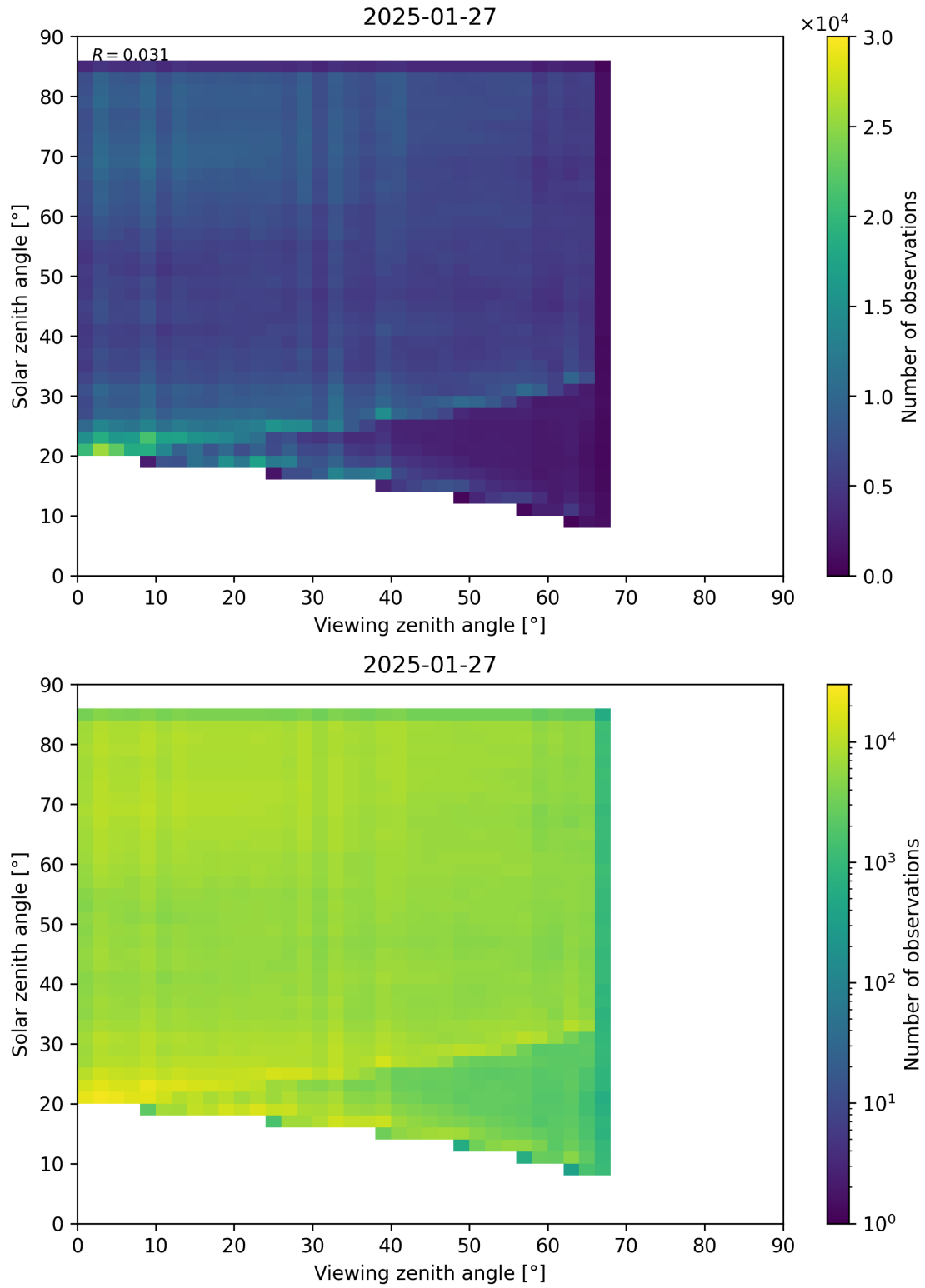
Figure 77: Scatter density plot of “Viewing zenith angle” against “Solar zenith angle” for 2025-01-26 to 2025-01-28.
