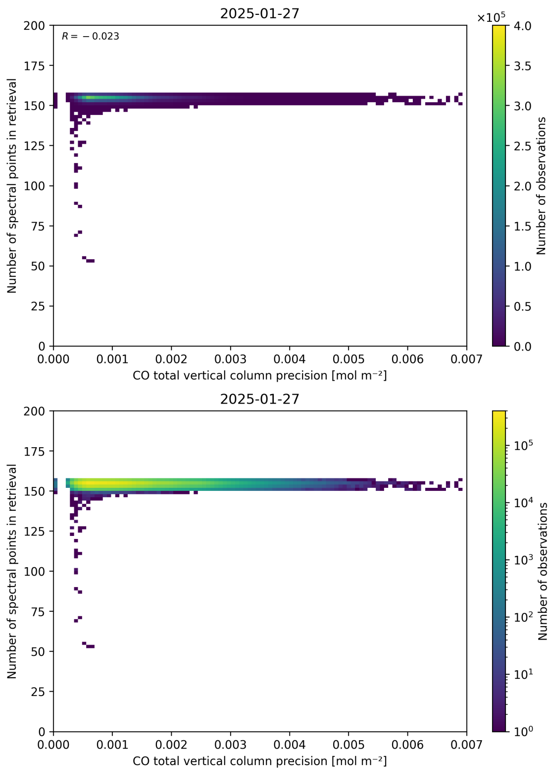
Figure 47: Scatter density plot of “CO total vertical column precision” against “Number of spectral points in retrieval” for 2025-01-26 to 2025-01-28.
