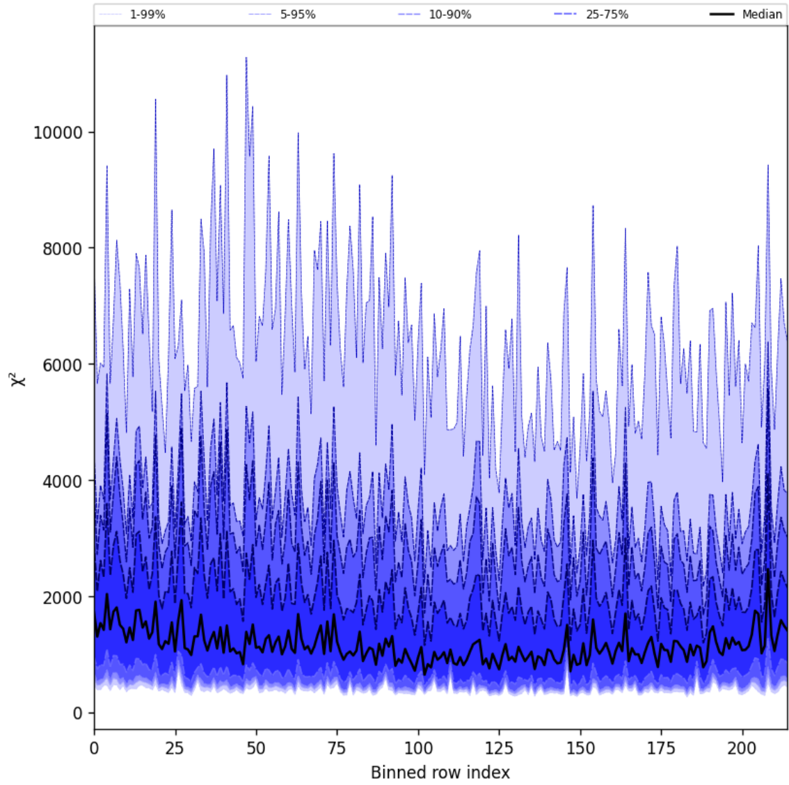
Figure 30: Along track statistics of “ \chi^2 ” for 2025-01-26 to 2025-01-28
