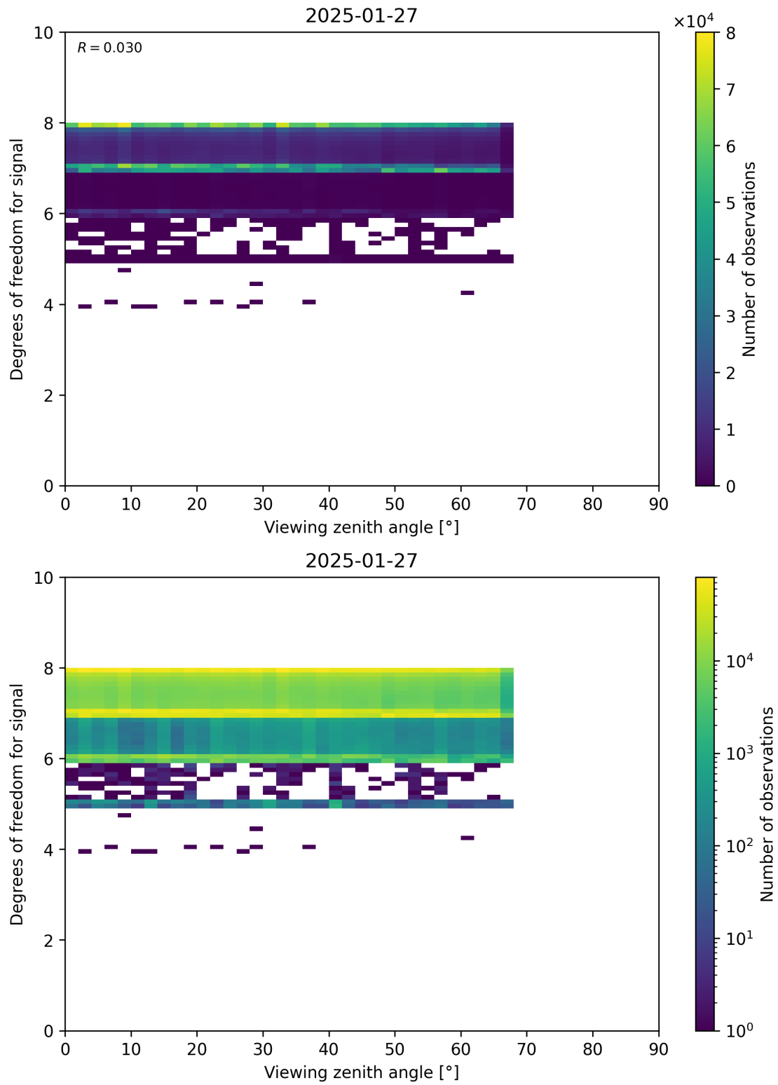
Figure 73: Scatter density plot of “Viewing zenith angle” against “Degrees of freedom for signal” for 2025-01-26 to 2025-01-28.
