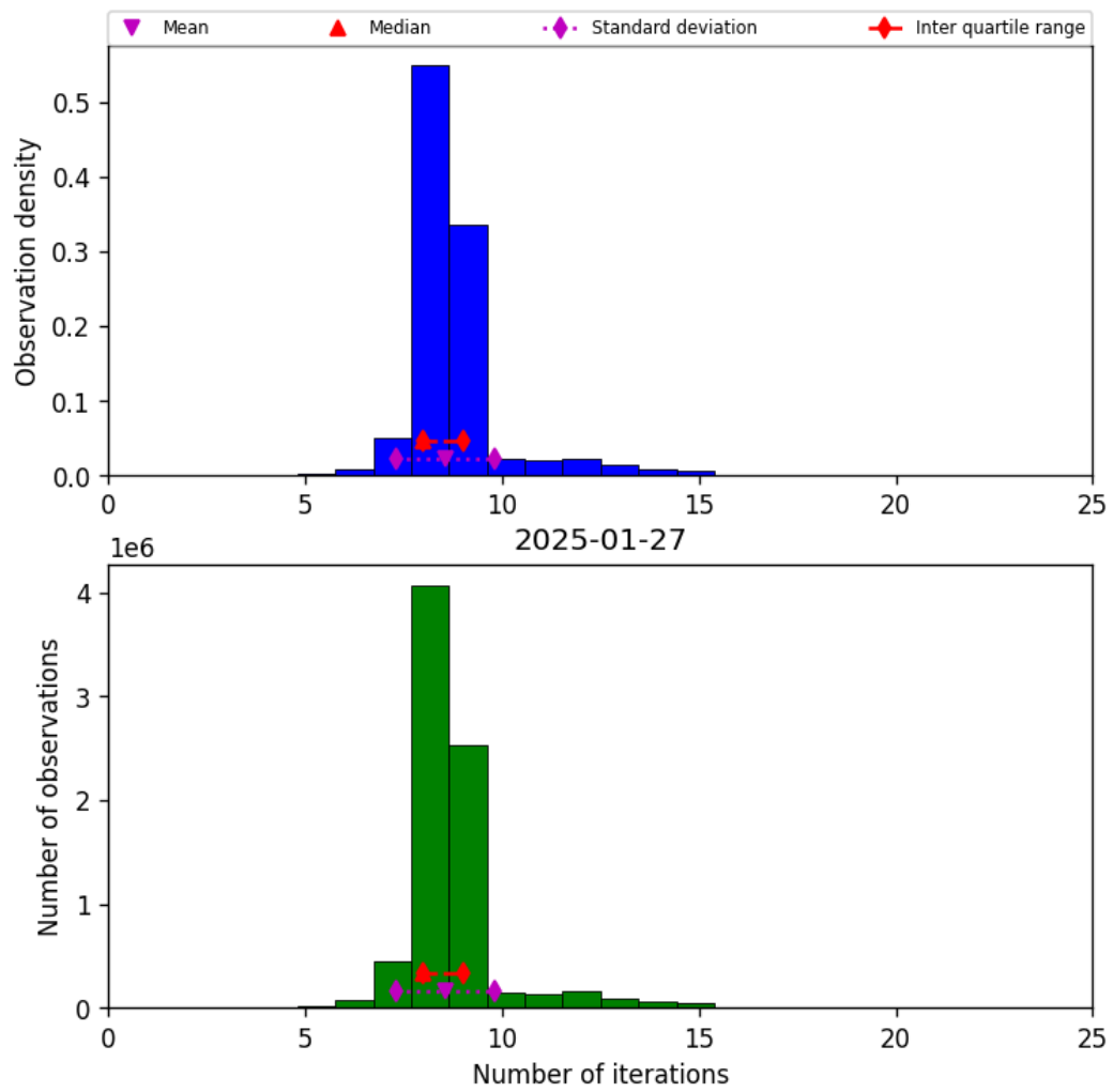
Figure 24: Histogram of “Number of iterations” for 2025-01-26 to 2025-01-28
