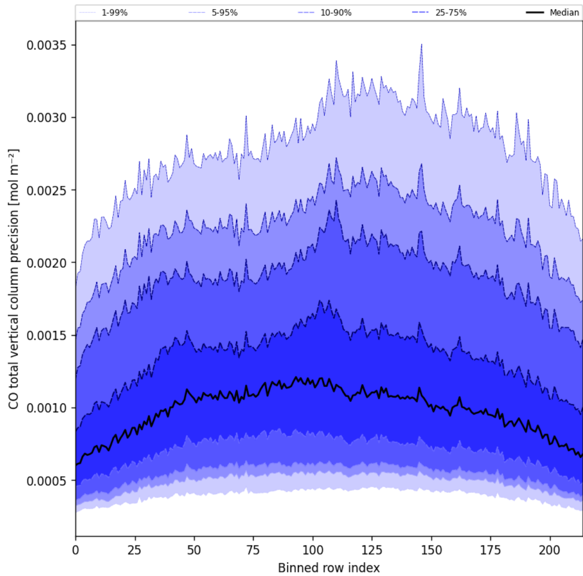
Figure 28: Along track statistics of “CO total vertical column precision” for 2025-01-26 to 2025-01-28
