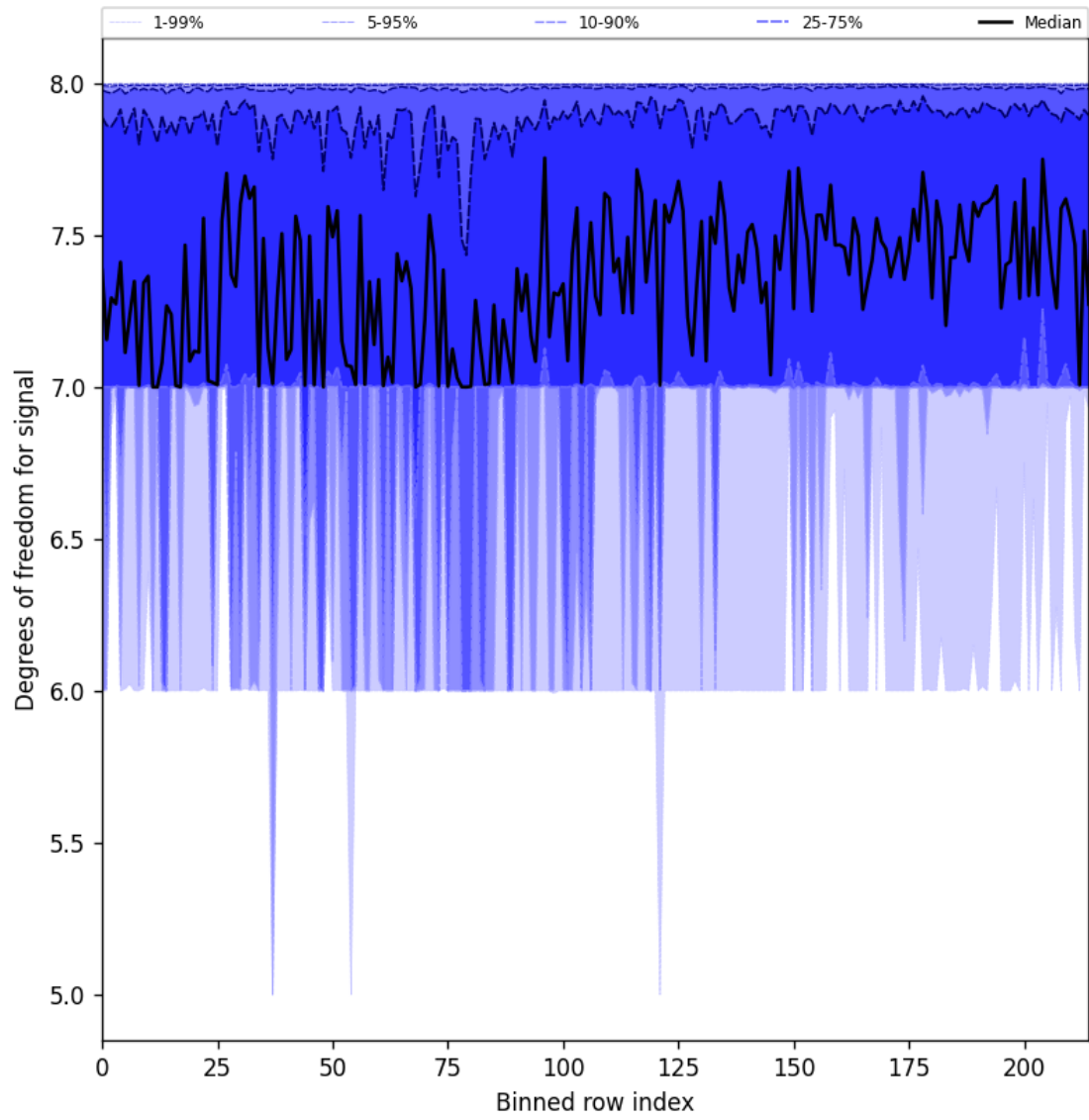
Figure 31: Along track statistics of “Degrees of freedom for signal” for 2025-01-26 to 2025-01-28
