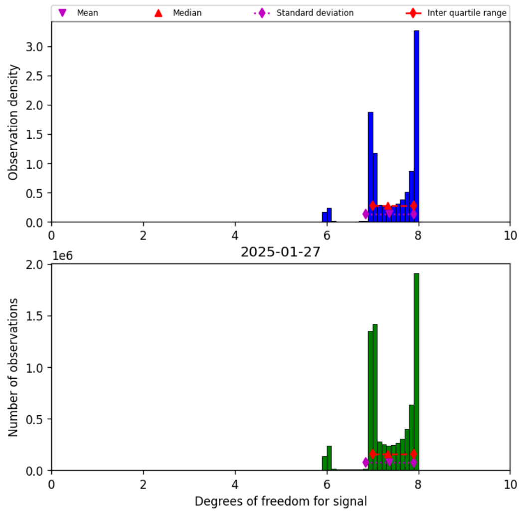
Figure 23: Histogram of “Degrees of freedom for signal” for 2025-01-26 to 2025-01-28
