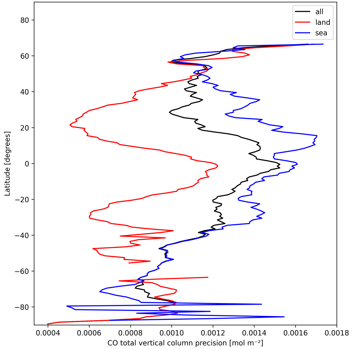
Figure 12: Zonal average of “CO total vertical column precision” for 2025-01-26 to 2025-01-28.
