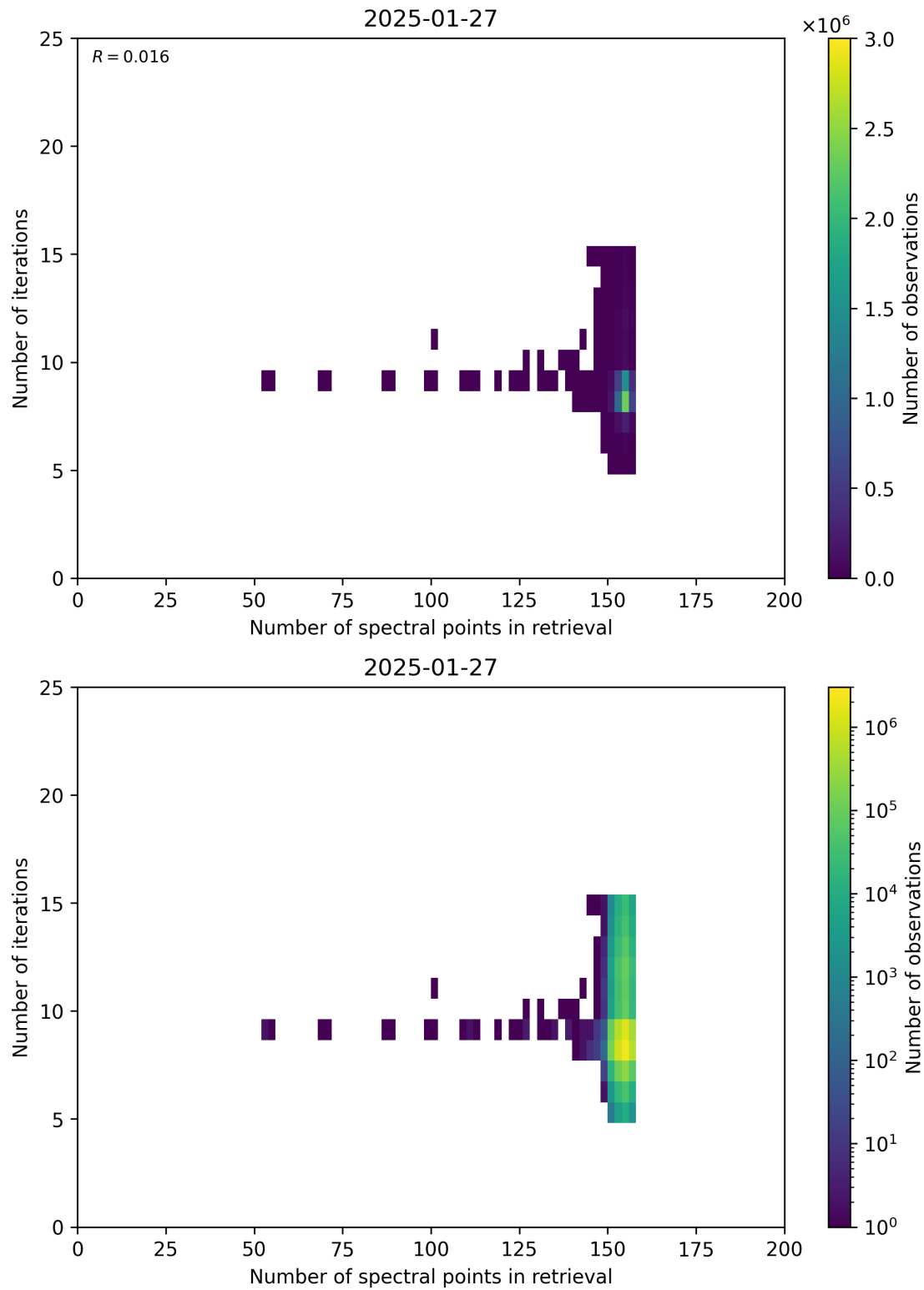
Figure 60: Scatter density plot of “Number of spectral points in retrieval” against “Number of iterations” for 2025-01-26 to 2025-01-28.
