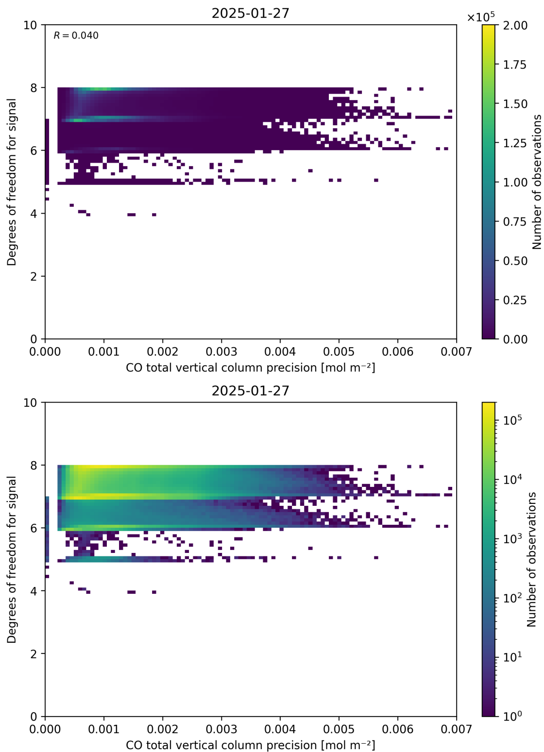
Figure 45: Scatter density plot of “CO total vertical column precision” against “Degrees of freedom for signal” for 2025-01-26 to 2025-01-28.
