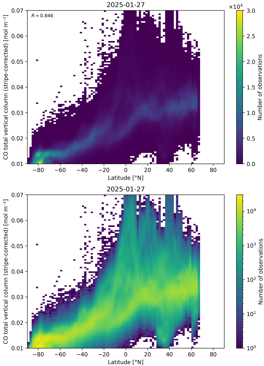
Figure 52: Scatter density plot of “Latitude” against “CO total vertical column (stripe-corrected)” for 2025-01-26 to 2025-01-28.
