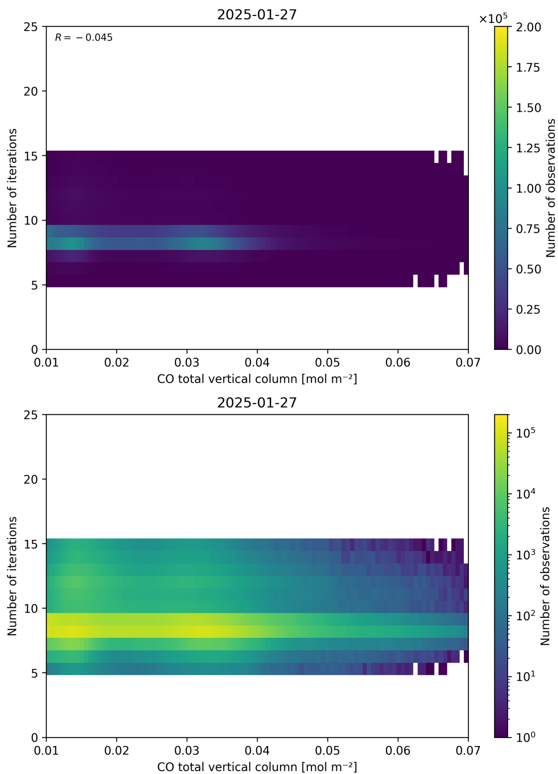
Figure 42: Scatter density plot of “CO total vertical column” against “Number of iterations” for 2025-01-26 to 2025-01-28.
