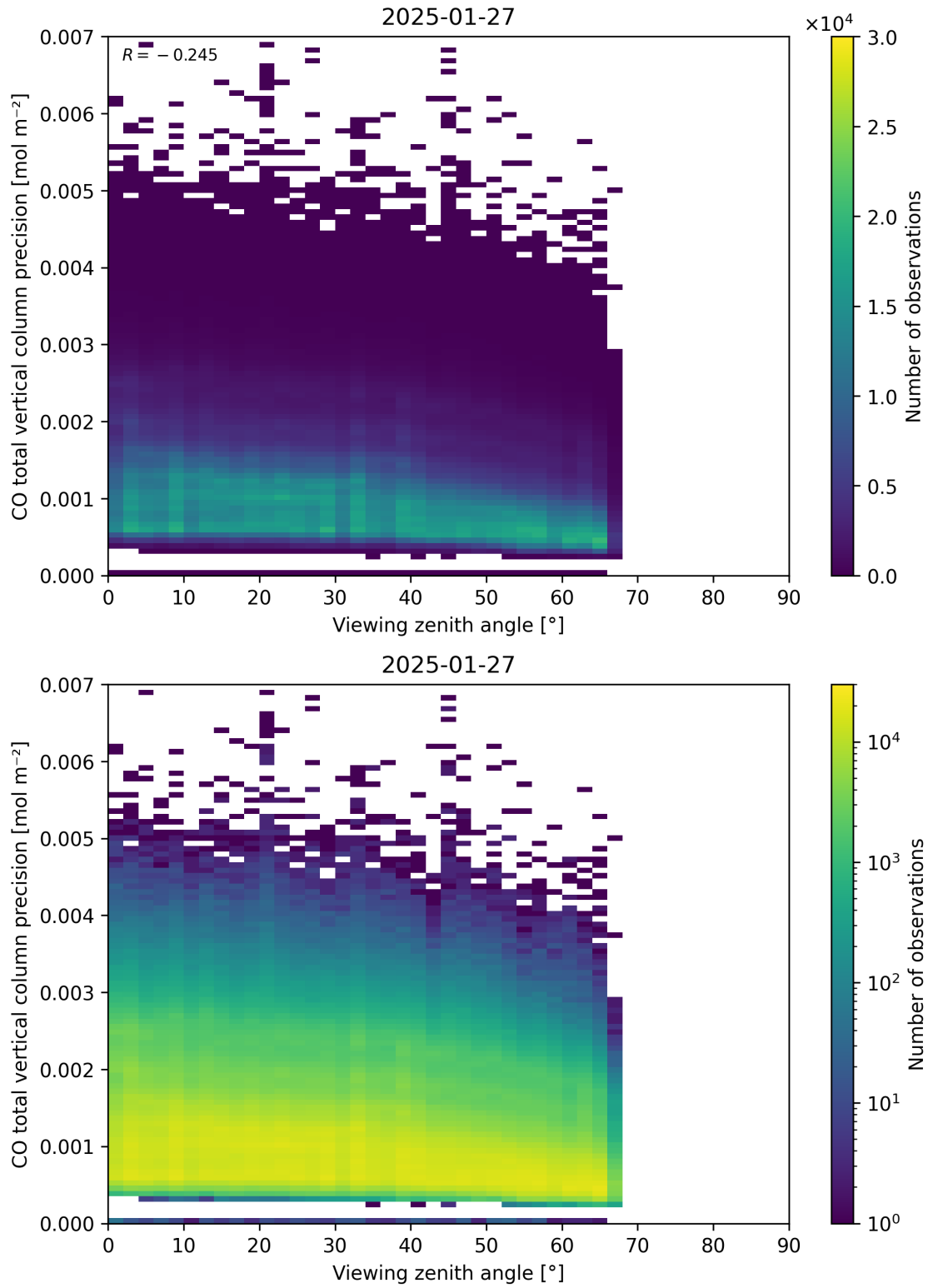
Figure 71: Scatter density plot of “Viewing zenith angle” against “CO total vertical column precision” for 2025-01-26 to 2025-01-28.
