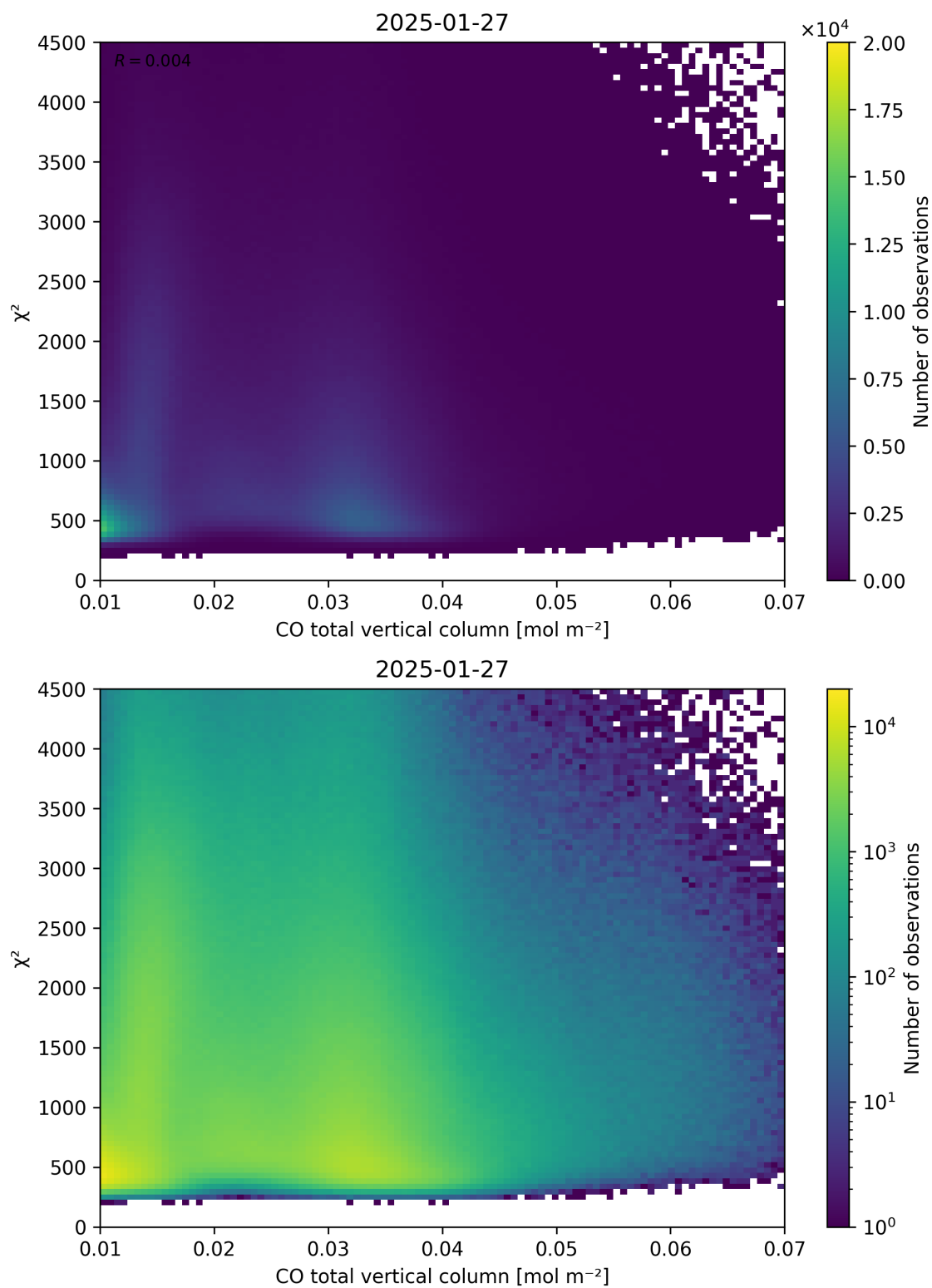
Figure 35: Scatter density plot of “CO total vertical column” against “ \chi^2 ” for 2025-01-26 to 2025-01-28.
