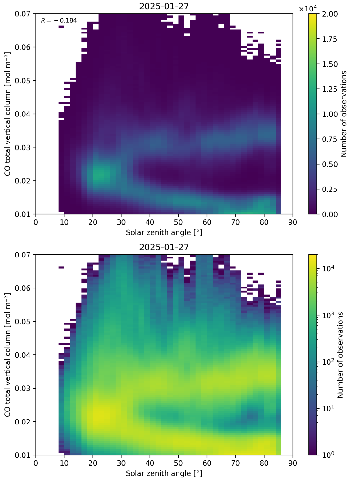
Figure 61: Scatter density plot of “Solar zenith angle” against “CO total vertical column” for 2025-01-26 to 2025-01-28.
