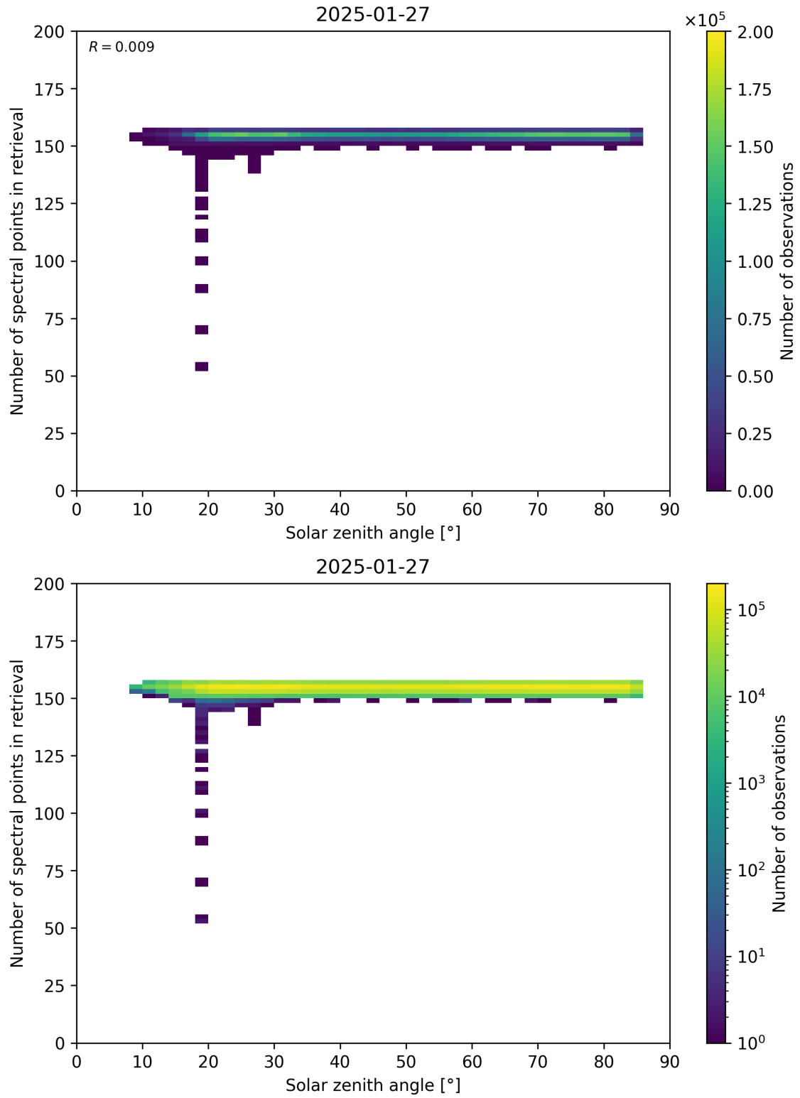
Figure 68: Scatter density plot of “Solar zenith angle” against “Number of spectral points in retrieval” for 2025-01-26 to 2025-01-28.
