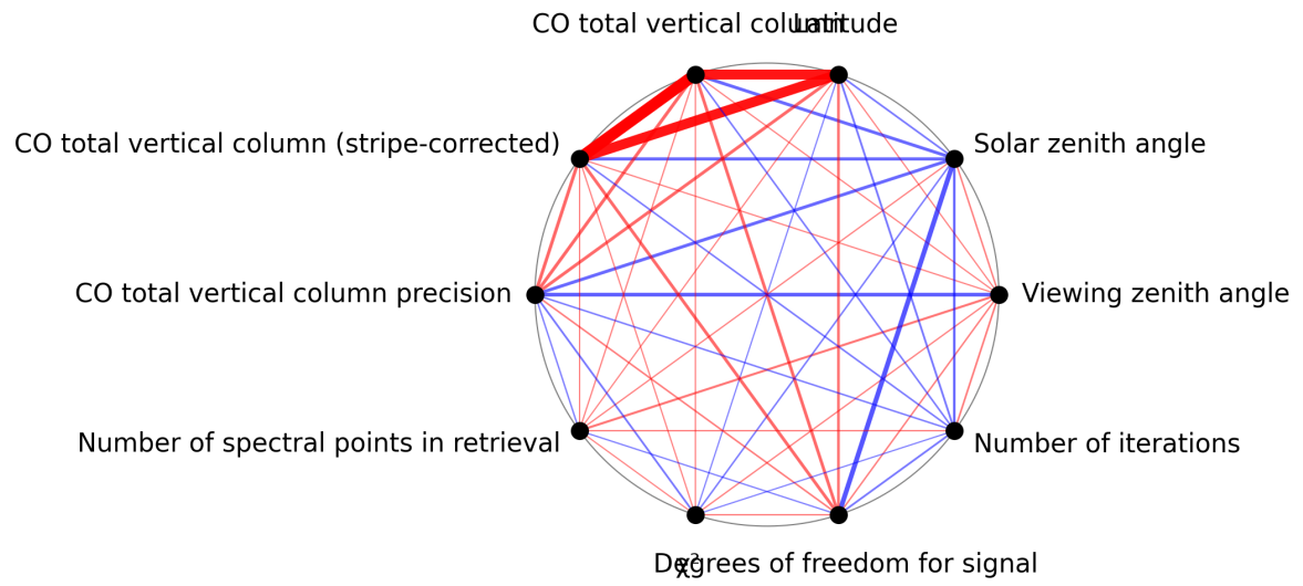
Figure 1: Map of correlation graph for 2025-01-26 to 2025-01-28.
