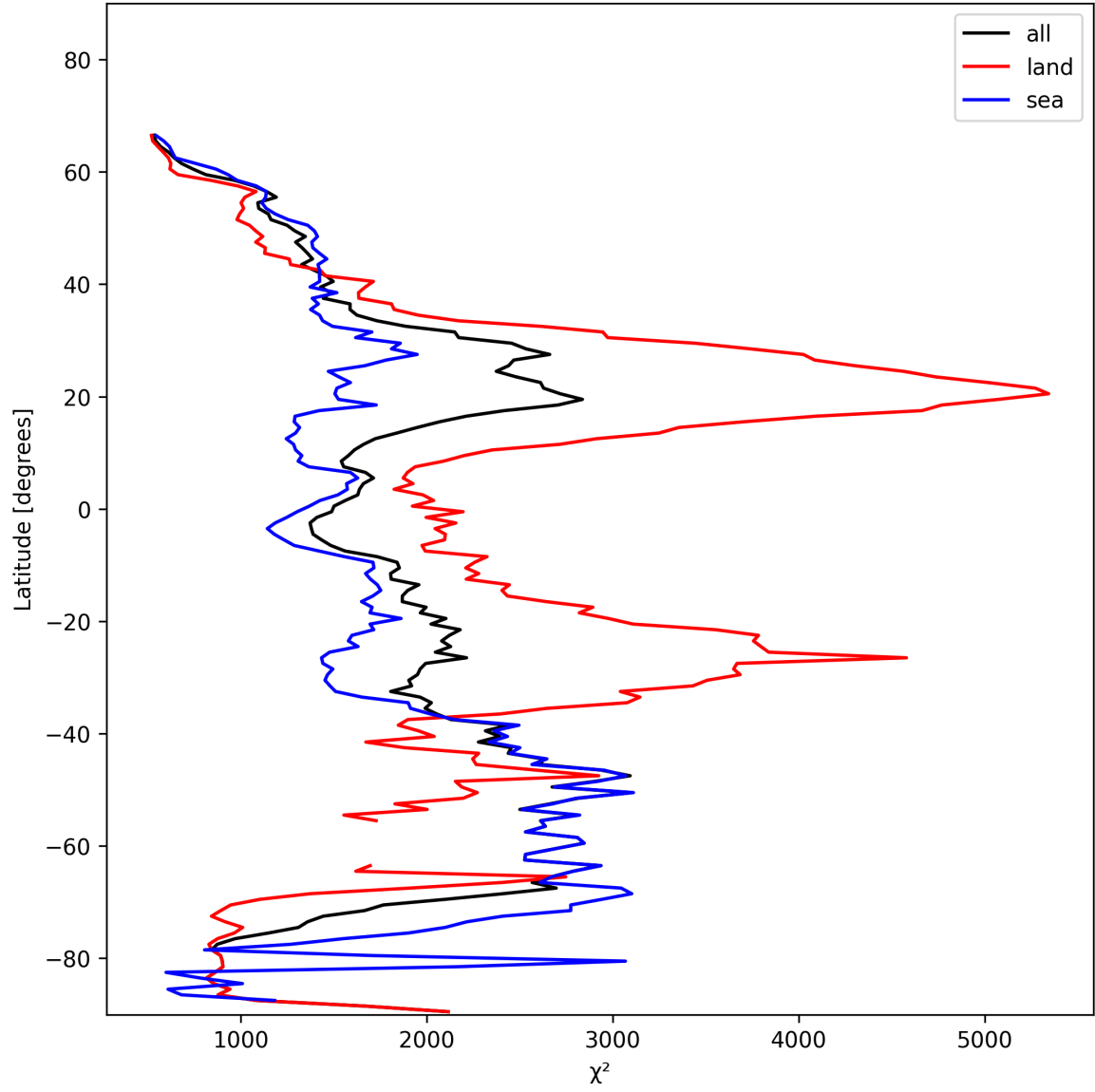
Figure 14: Zonal average of “ \chi^2 ” for 2025-01-26 to 2025-01-28.
