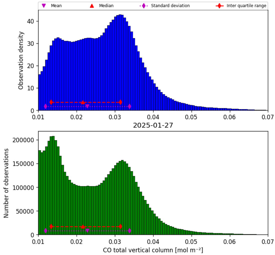
Figure 18: Histogram of “CO total vertical column” for 2025-01-26 to 2025-01-28
