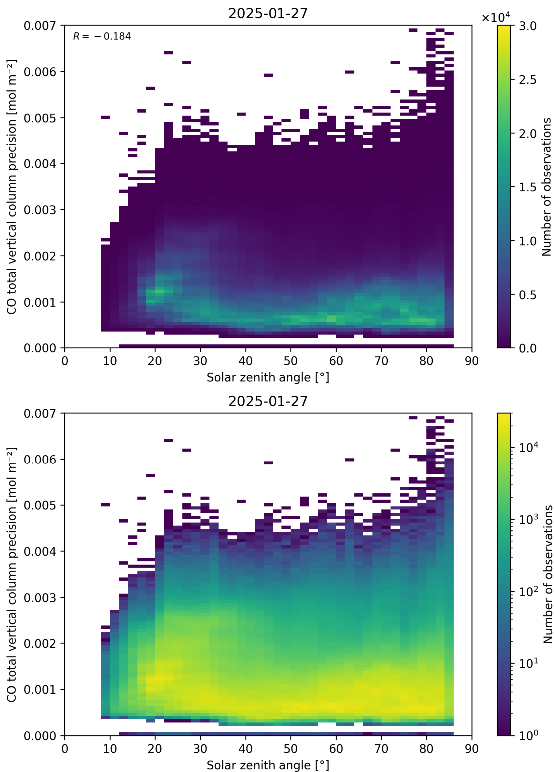
Figure 63: Scatter density plot of “Solar zenith angle” against “CO total vertical column precision” for 2025-01-26 to 2025-01-28.
