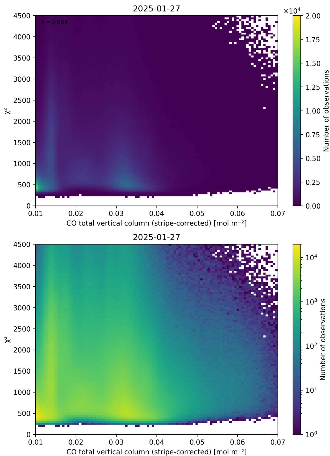
Figure 37: Scatter density plot of “CO total vertical column (stripe-corrected)” against “ \chi^2 ” for 2025-01-26 to 2025-01-28.
