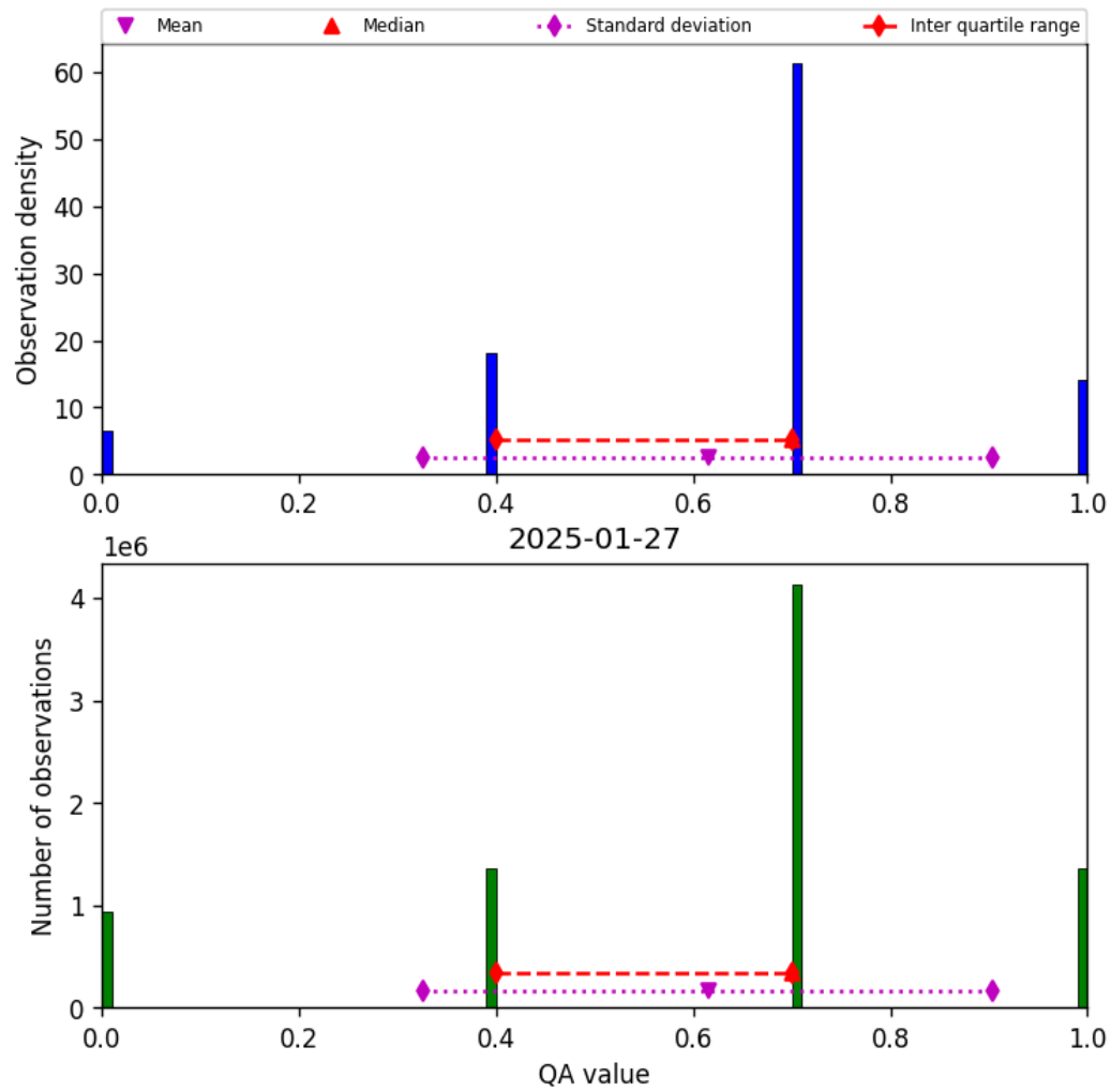
Figure 17: Histogram of “QA value” for 2025-01-26 to 2025-01-28
