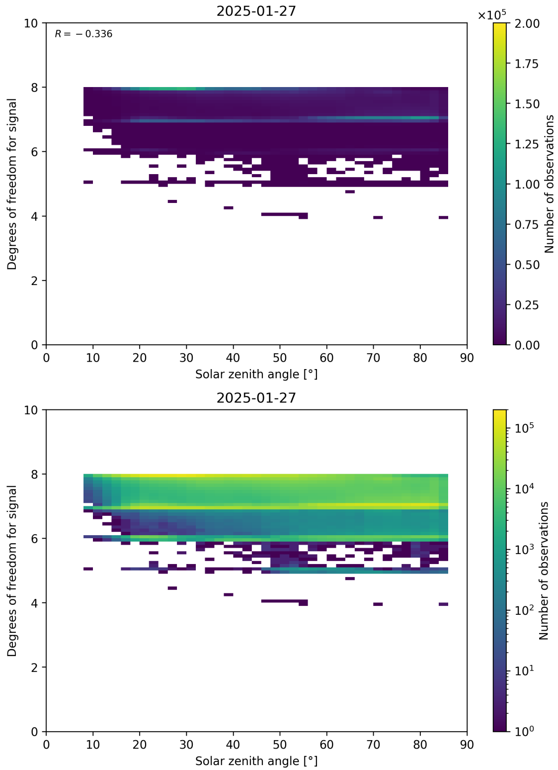
Figure 65: Scatter density plot of “Solar zenith angle” against “Degrees of freedom for signal” for 2025-01-26 to 2025-01-28.
