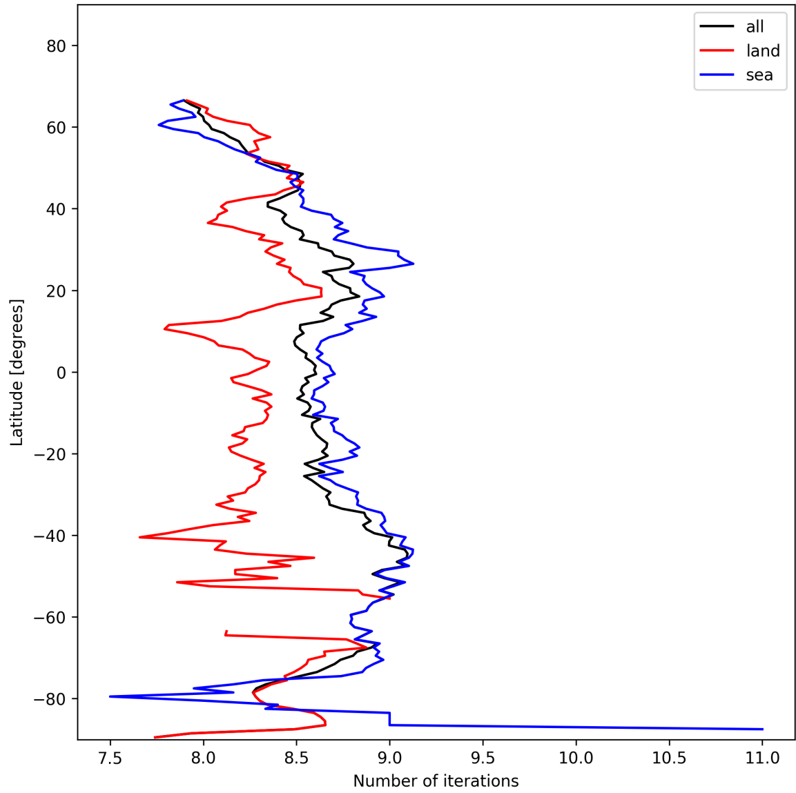
Figure 16: Zonal average of “Number of iterations” for 2025-01-26 to 2025-01-28.
