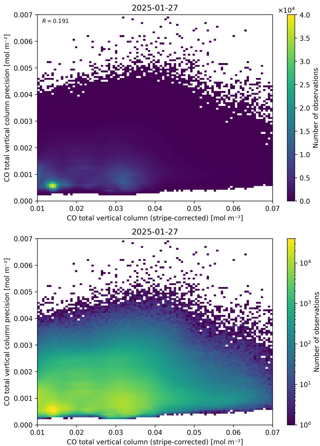
Figure 36: Scatter density plot of “CO total vertical column (stripe-corrected)” against “CO total vertical column precision” for 2025-01-26 to 2025-01-28.
