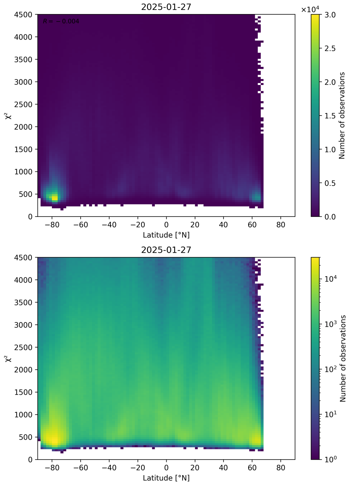
Figure 54: Scatter density plot of “Latitude” against “ \chi^2 ” for 2025-01-26 to 2025-01-28.
