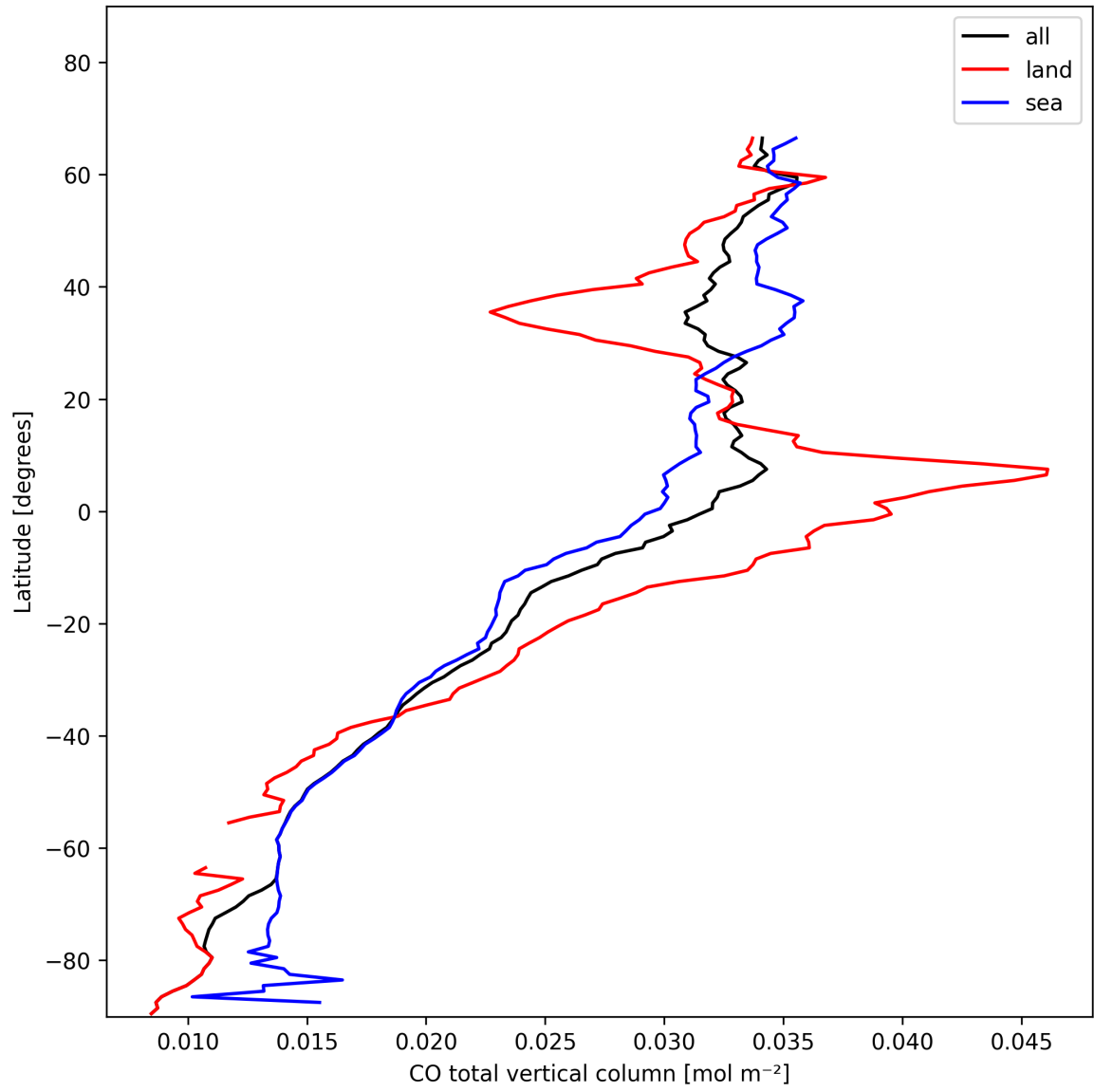
Figure 10: Zonal average of “CO total vertical column” for 2025-01-26 to 2025-01-28.
