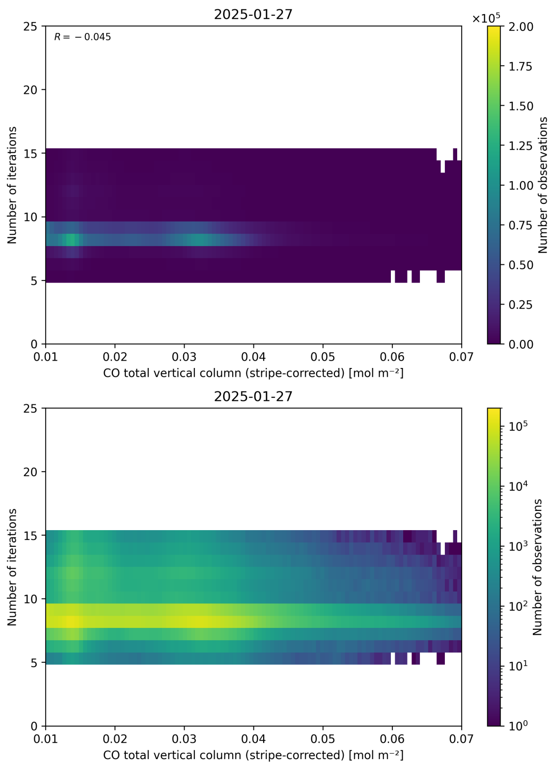
Figure 39: Scatter density plot of “CO total vertical column (stripe-corrected)” against “Number of iterations” for 2025-01-26 to 2025-01-28.
