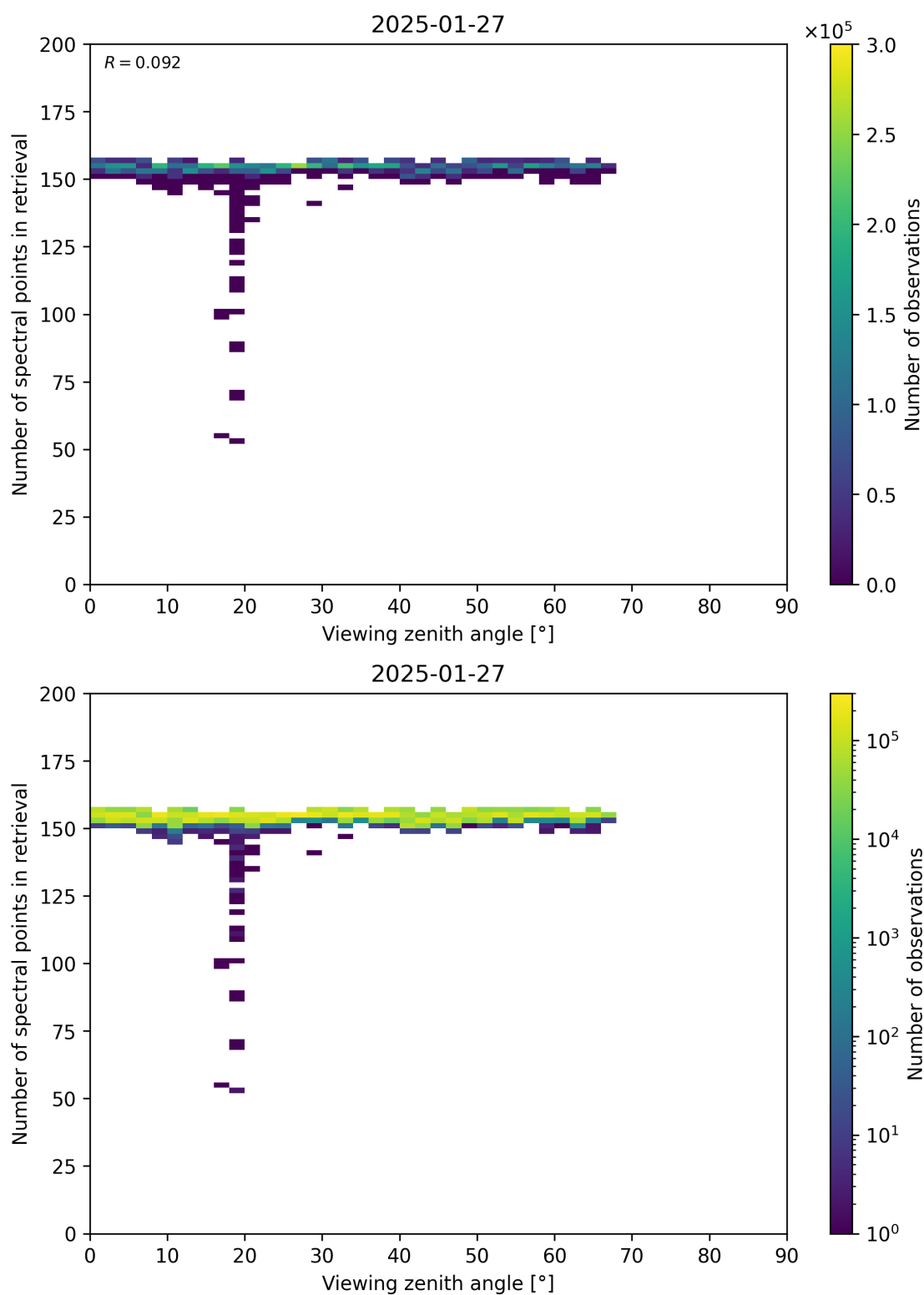
Figure 76: Scatter density plot of “Viewing zenith angle” against “Number of spectral points in retrieval” for 2025-01-26 to 2025-01-28.
