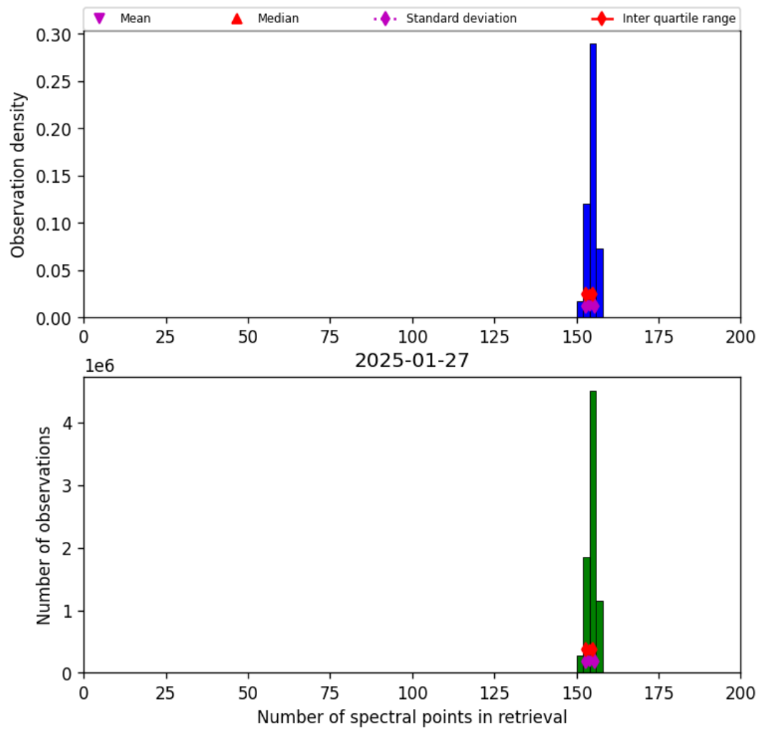
Figure 21: Histogram of “Number of spectral points in retrieval” for 2025-01-26 to 2025-01-28
