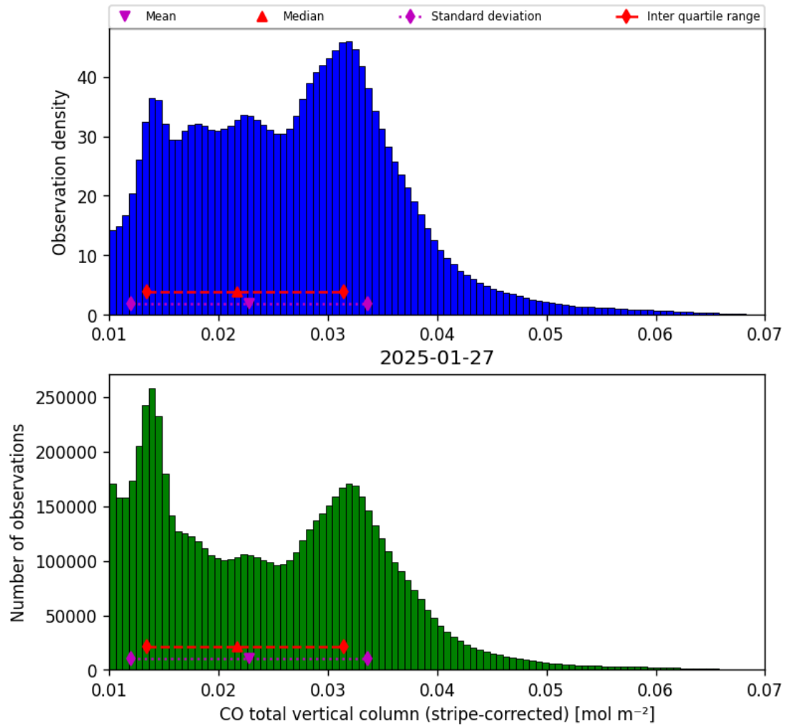
Figure 19: Histogram of “CO total vertical column (stripe-corrected)” for 2025-01-26 to 2025-01-28
