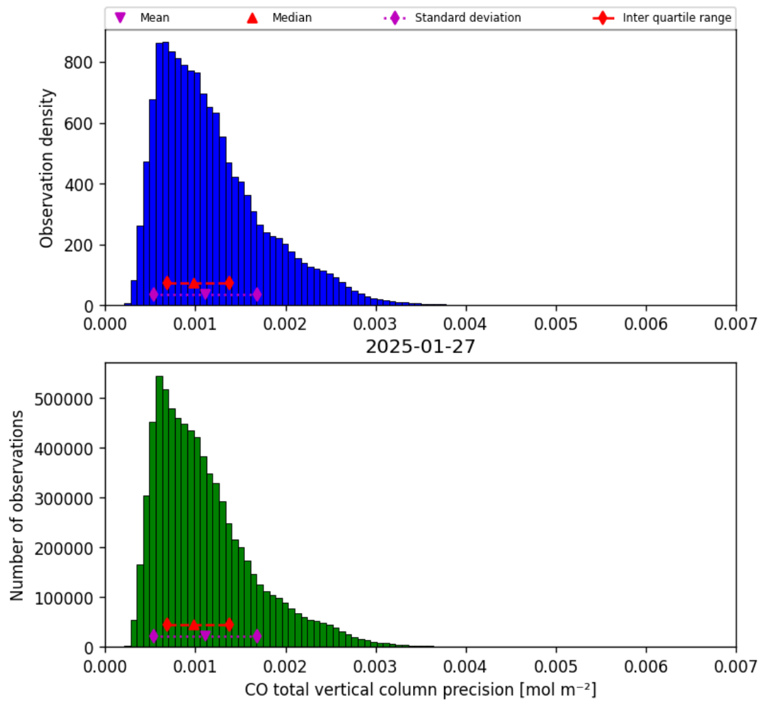
Figure 20: Histogram of “CO total vertical column precision” for 2025-01-26 to 2025-01-28
