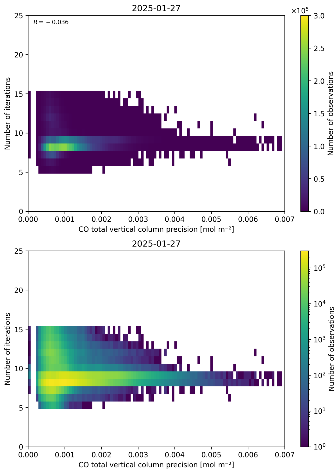
Figure 46: Scatter density plot of “CO total vertical column precision” against “Number of iterations” for 2025-01-26 to 2025-01-28.
