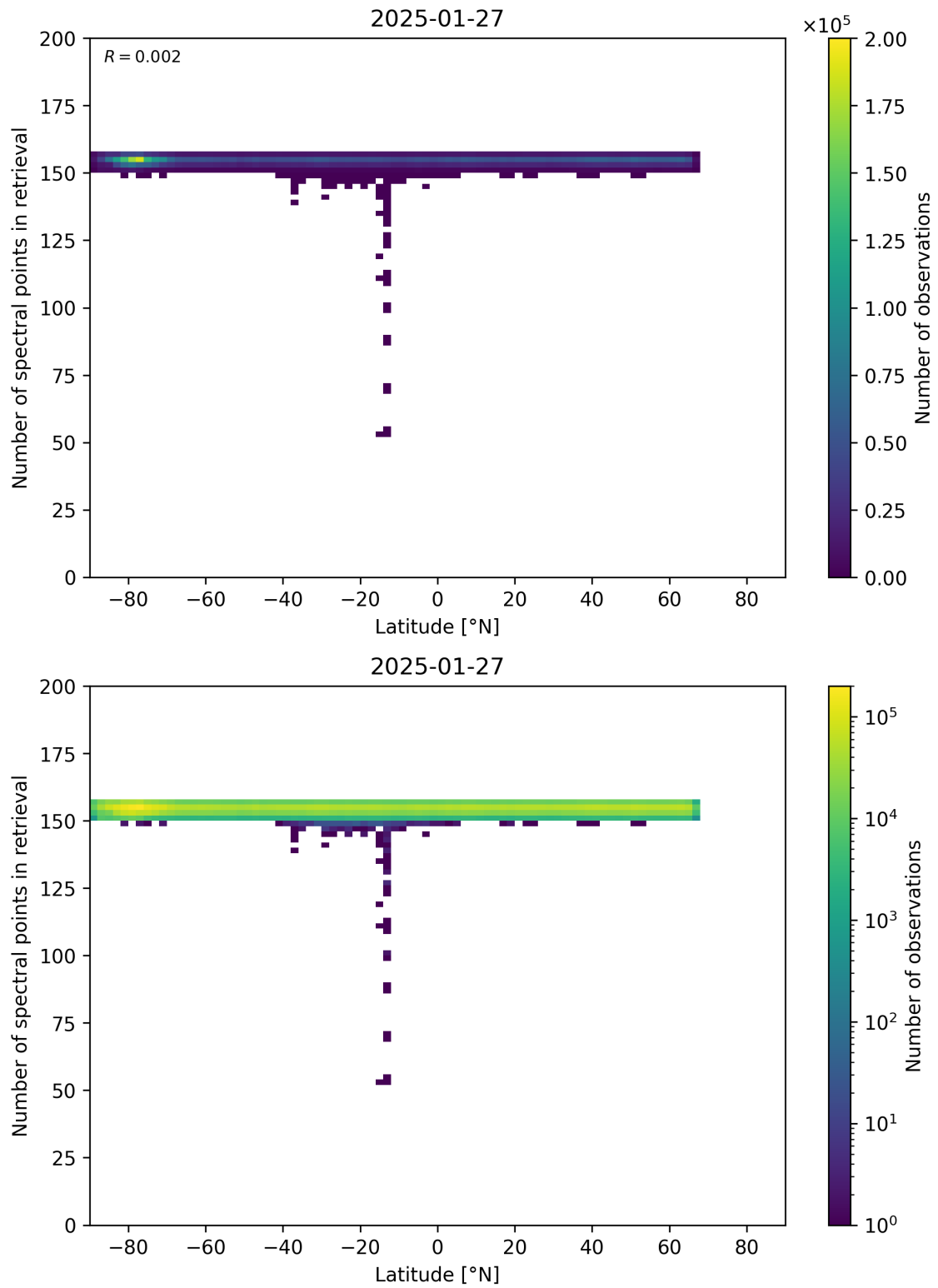
Figure 57: Scatter density plot of “Latitude” against “Number of spectral points in retrieval” for 2025-01-26 to 2025-01-28.
