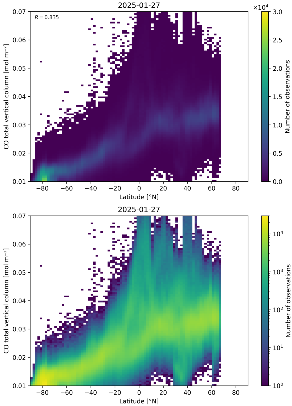
Figure 51: Scatter density plot of “Latitude” against “CO total vertical column” for 2025-01-26 to 2025-01-28.
