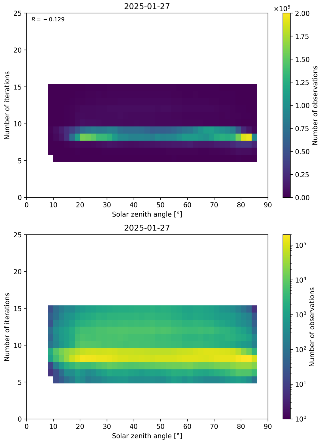
Figure 67: Scatter density plot of “Solar zenith angle” against “Number of iterations” for 2025-01-26 to 2025-01-28.
