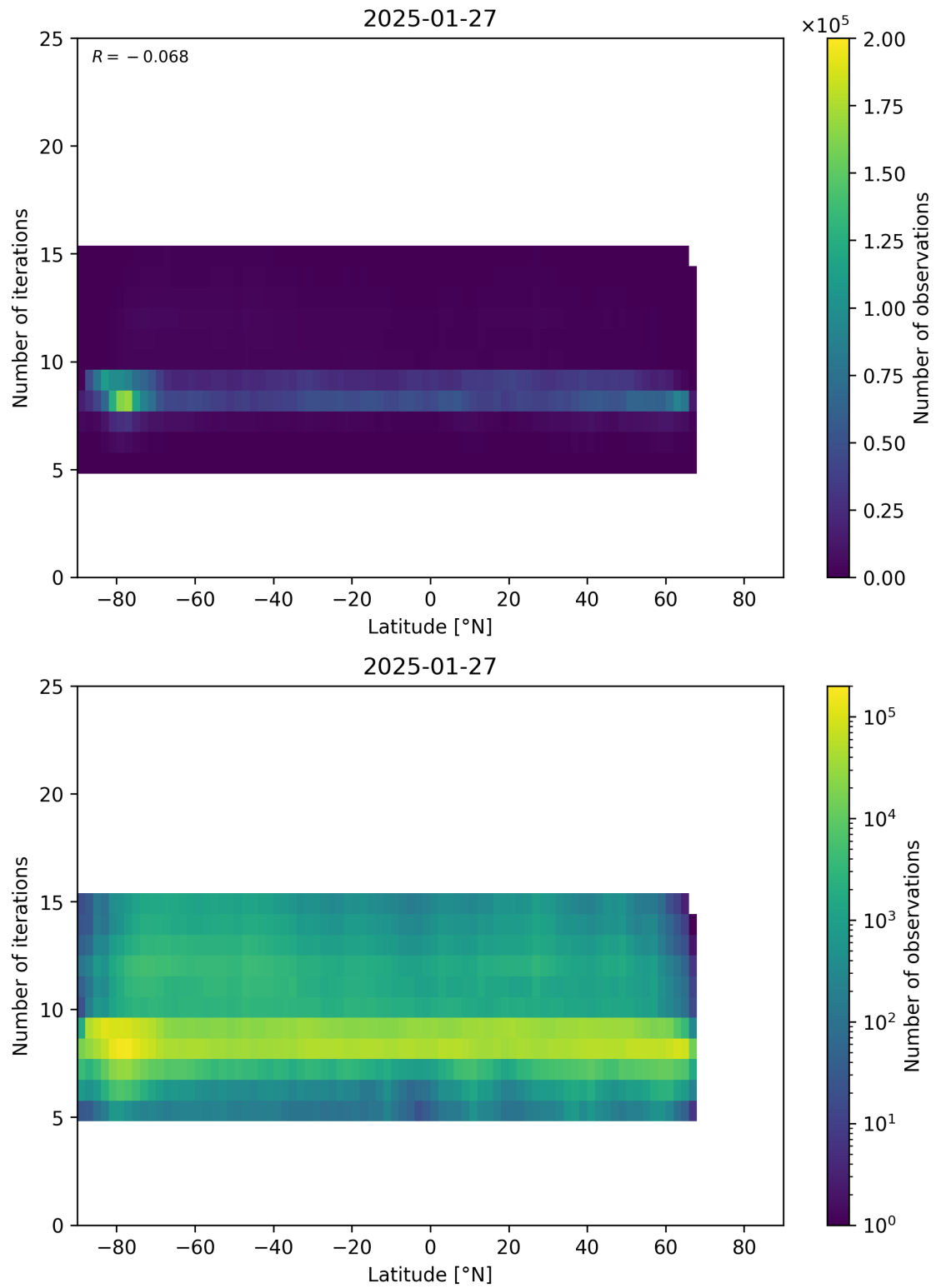
Figure 56: Scatter density plot of “Latitude” against “Number of iterations” for 2025-01-26 to 2025-01-28.
