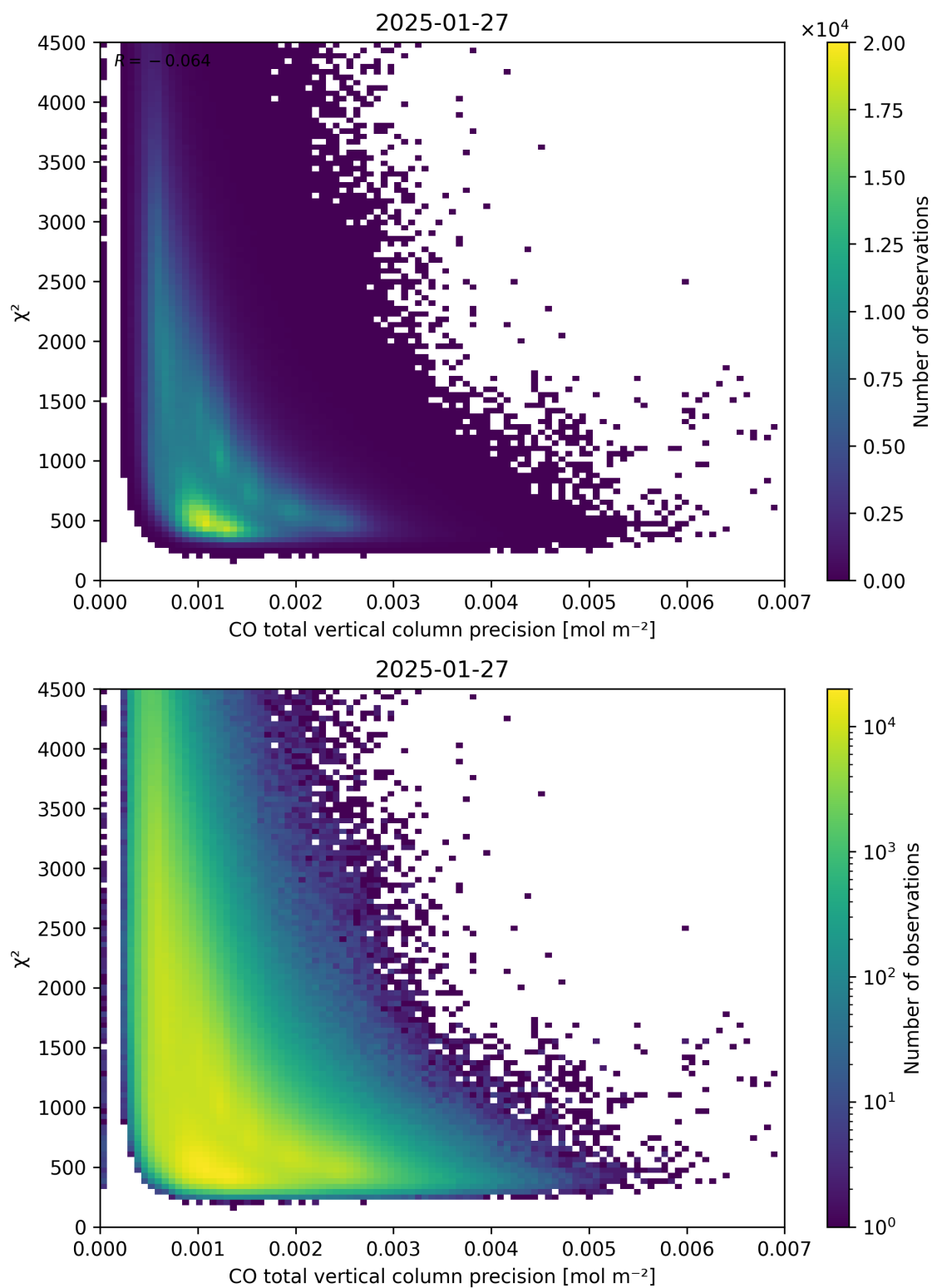
Figure 44: Scatter density plot of “CO total vertical column precision” against “ \chi^2 ” for 2025-01-26 to 2025-01-28.
