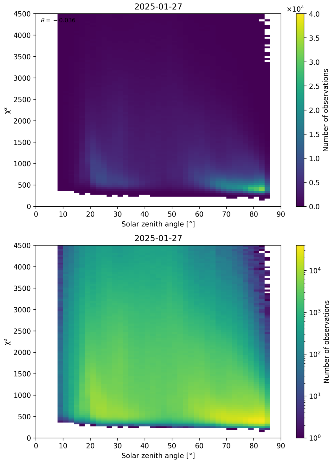
Figure 64: Scatter density plot of “Solar zenith angle” against “ \chi^2 ” for 2025-01-26 to 2025-01-28.
