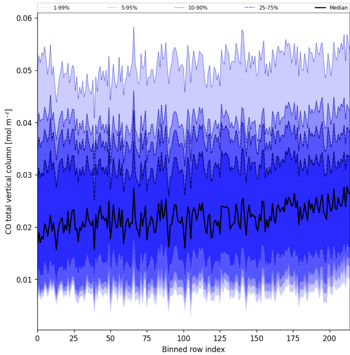
Figure 26: Along track statistics of “CO total vertical column” for 2025-01-26 to 2025-01-28
