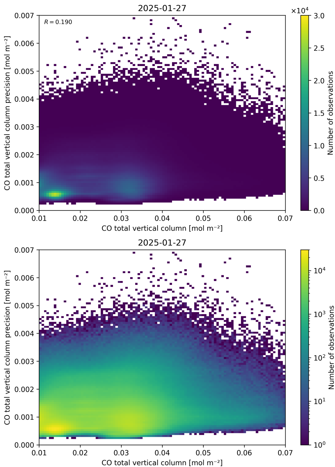
Figure 34: Scatter density plot of “CO total vertical column” against “CO total vertical column precision” for 2025-01-26 to 2025-01-28.
