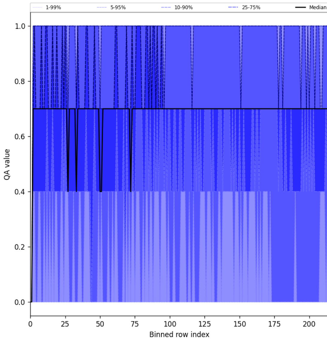
Figure 25: Along track statistics of “QA value” for 2025-01-26 to 2025-01-28
