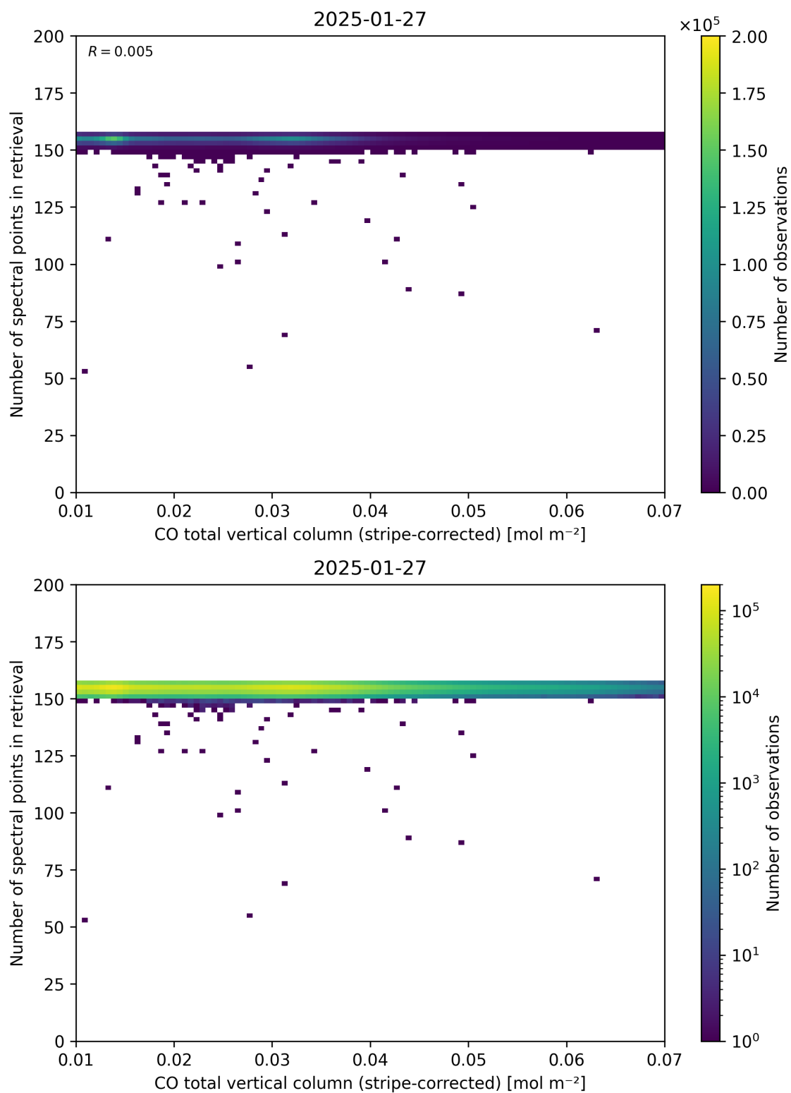
Figure 40: Scatter density plot of “CO total vertical column (stripe-corrected)” against “Number of spectral points in retrieval” for 2025-01-26 to 2025-01-28.
