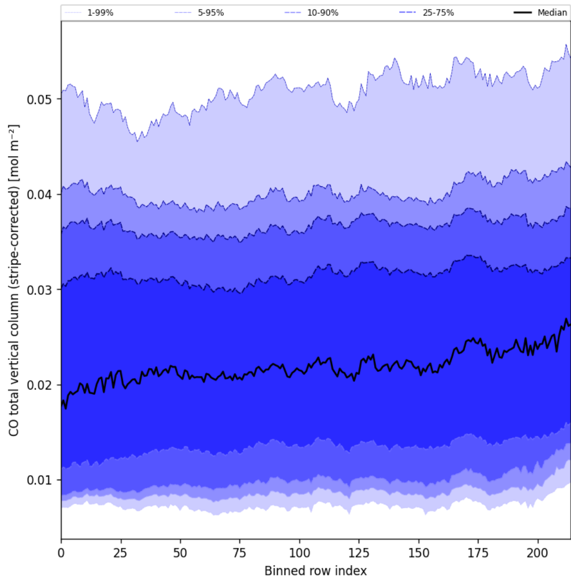
Figure 27: Along track statistics of “CO total vertical column (stripe-corrected)” for 2025-01-26 to 2025-01-28
