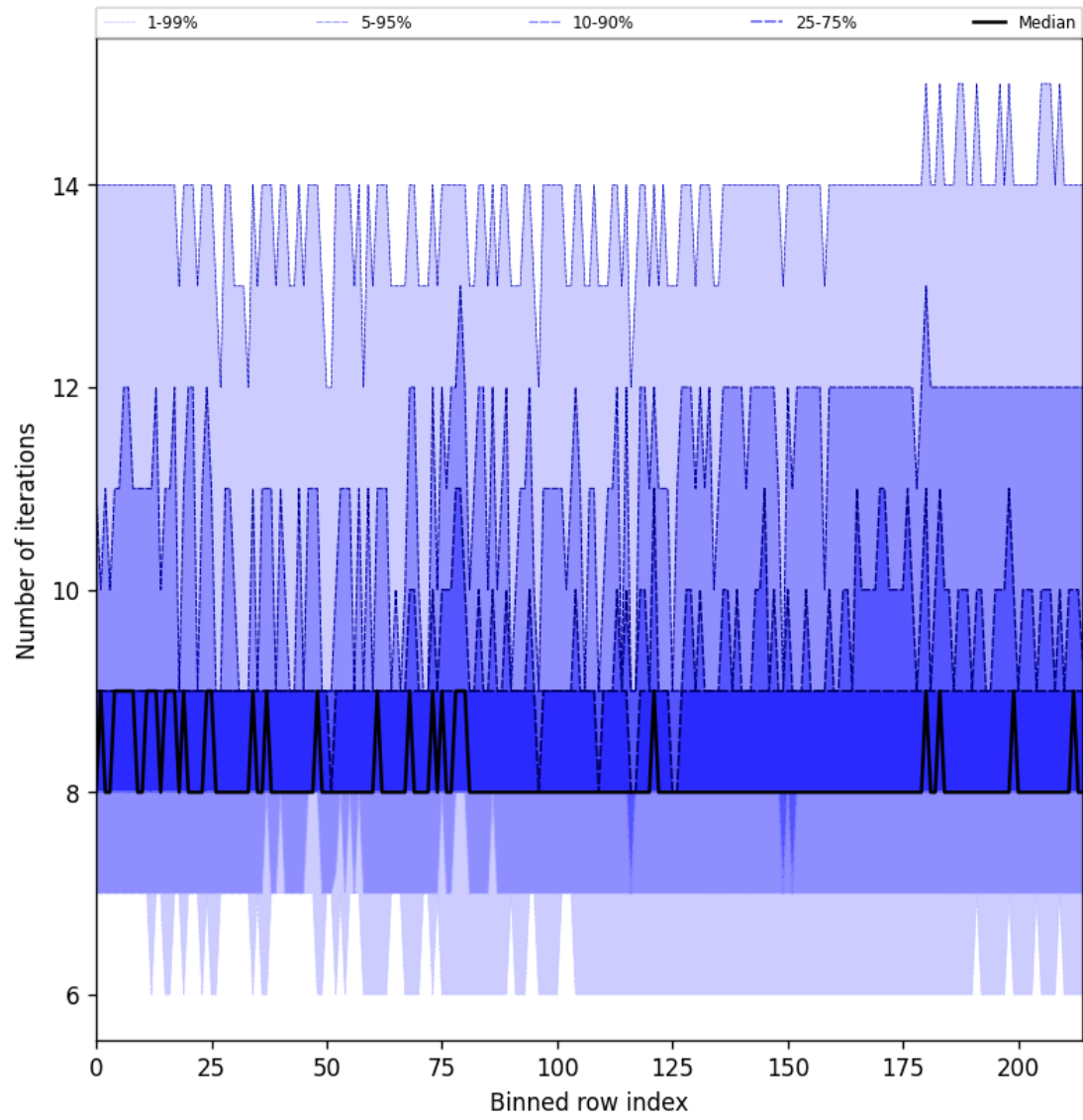
Figure 32: Along track statistics of “Number of iterations” for 2025-01-26 to 2025-01-28
