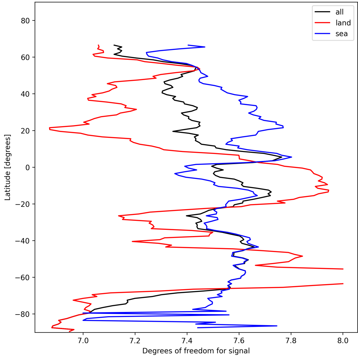
Figure 15: Zonal average of “Degrees of freedom for signal” for 2025-01-26 to 2025-01-28.
