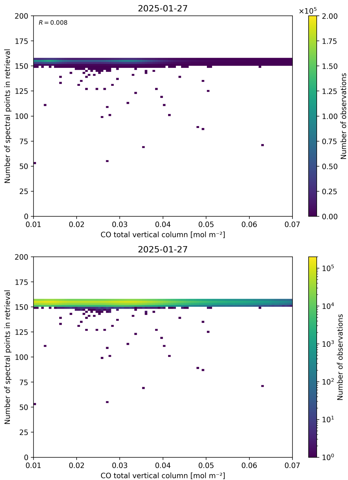
Figure 43: Scatter density plot of “CO total vertical column” against “Number of spectral points in retrieval” for 2025-01-26 to 2025-01-28.
