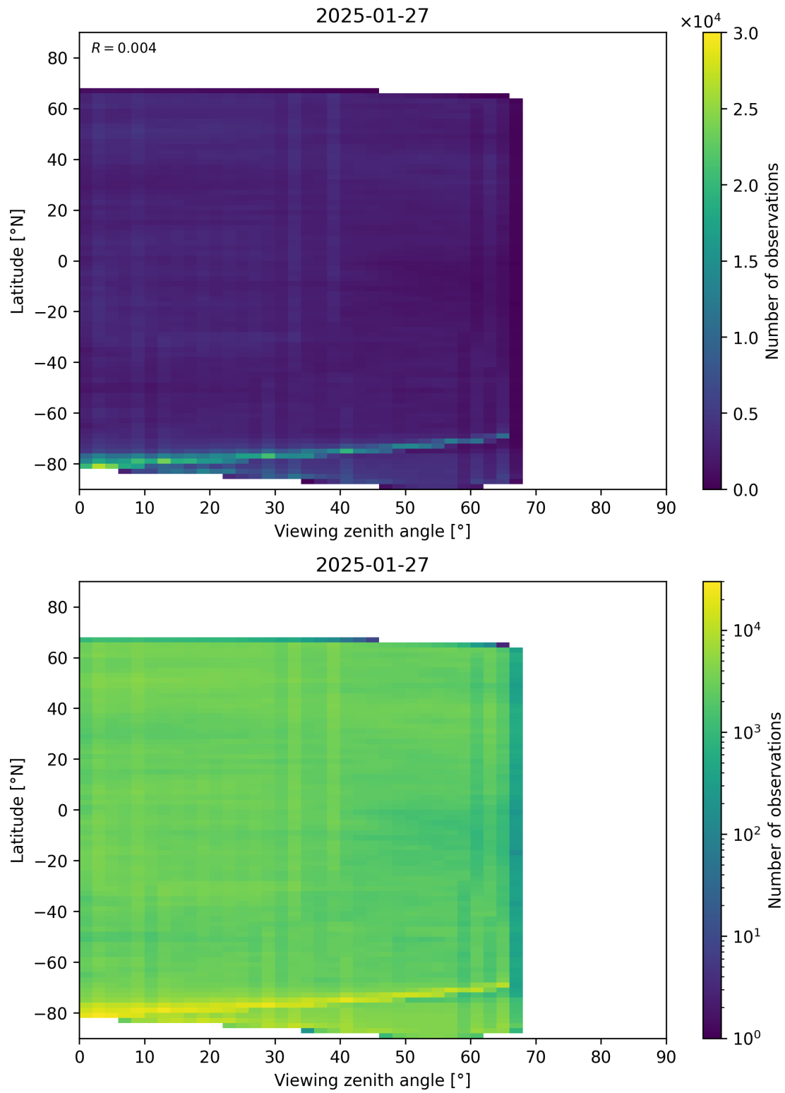
Figure 74: Scatter density plot of “Viewing zenith angle” against “Latitude” for 2025-01-26 to 2025-01-28.
