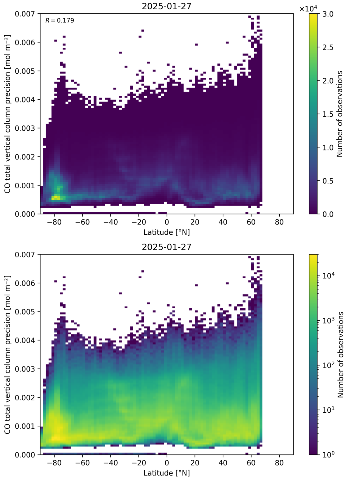
Figure 53: Scatter density plot of “Latitude” against “CO total vertical column precision” for 2025-01-26 to 2025-01-28.
