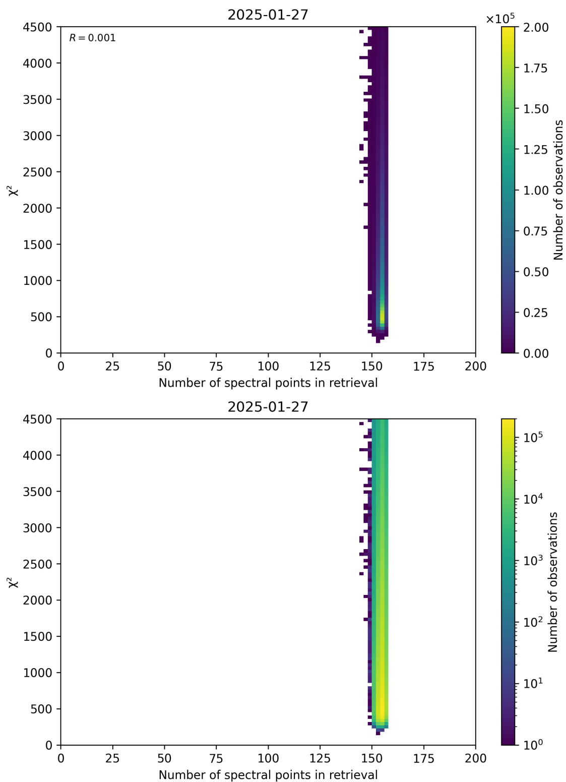
Figure 58: Scatter density plot of “Number of spectral points in retrieval” against “ \chi^2 ” for 2025-01-26 to 2025-01-28.
