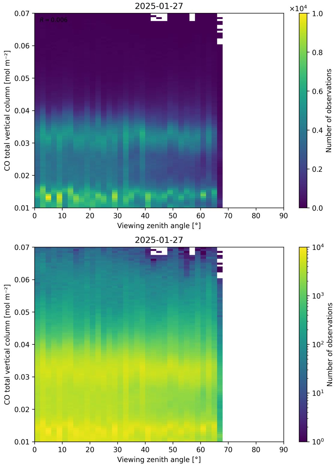
Figure 69: Scatter density plot of “Viewing zenith angle” against “CO total vertical column” for 2025-01-26 to 2025-01-28.
