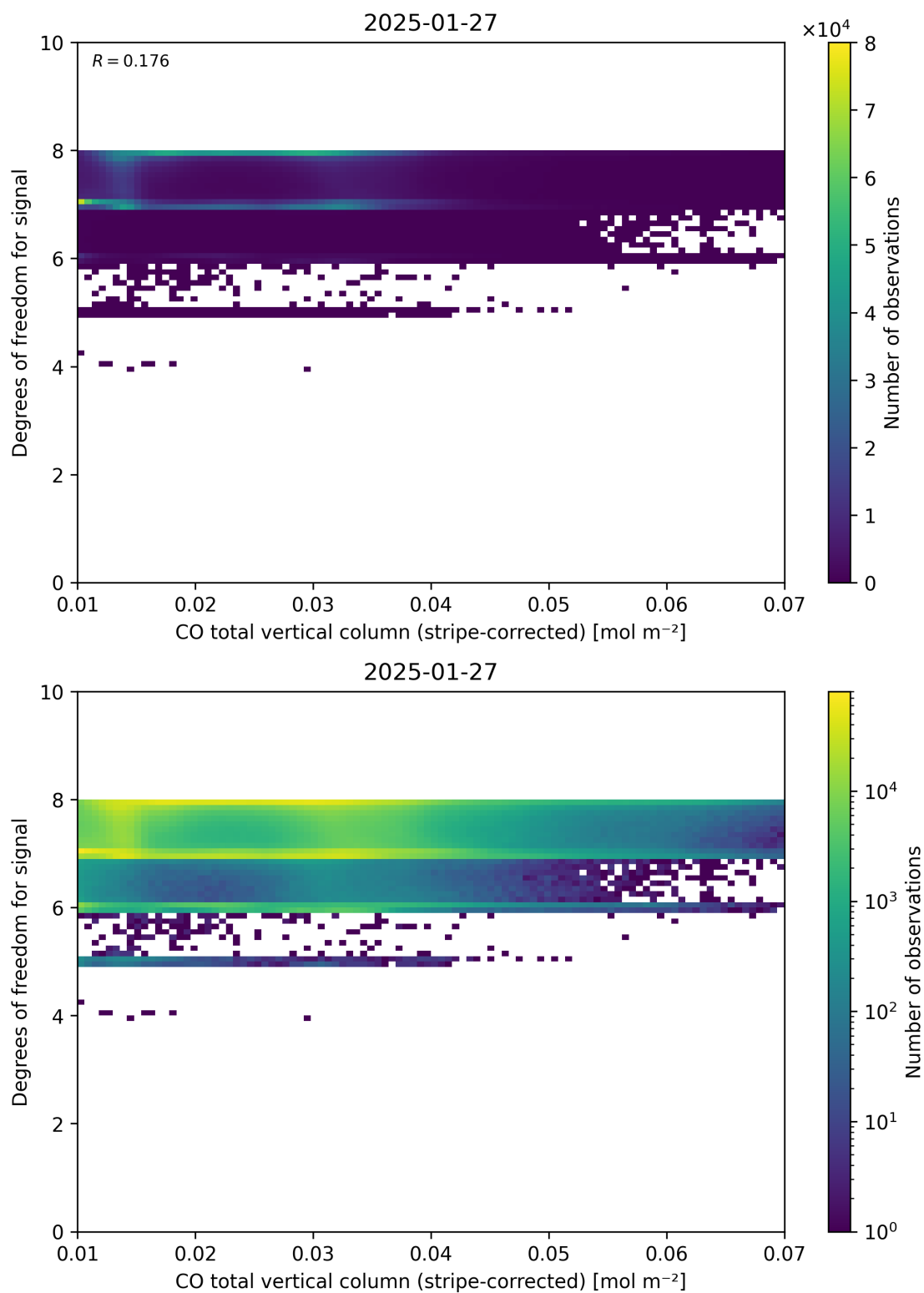
Figure 38: Scatter density plot of “CO total vertical column (stripe-corrected)” against “Degrees of freedom for signal” for 2025-01-26 to 2025-01-28.
