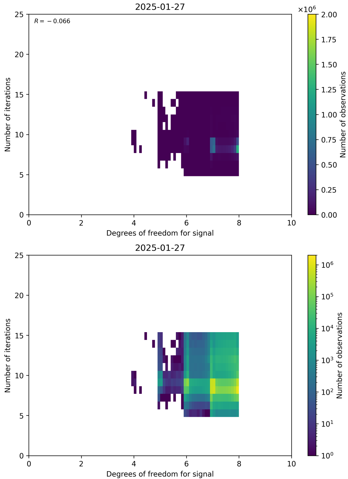
Figure 50: Scatter density plot of “Degrees of freedom for signal” against “Number of iterations” for 2025-01-26 to 2025-01-28.
