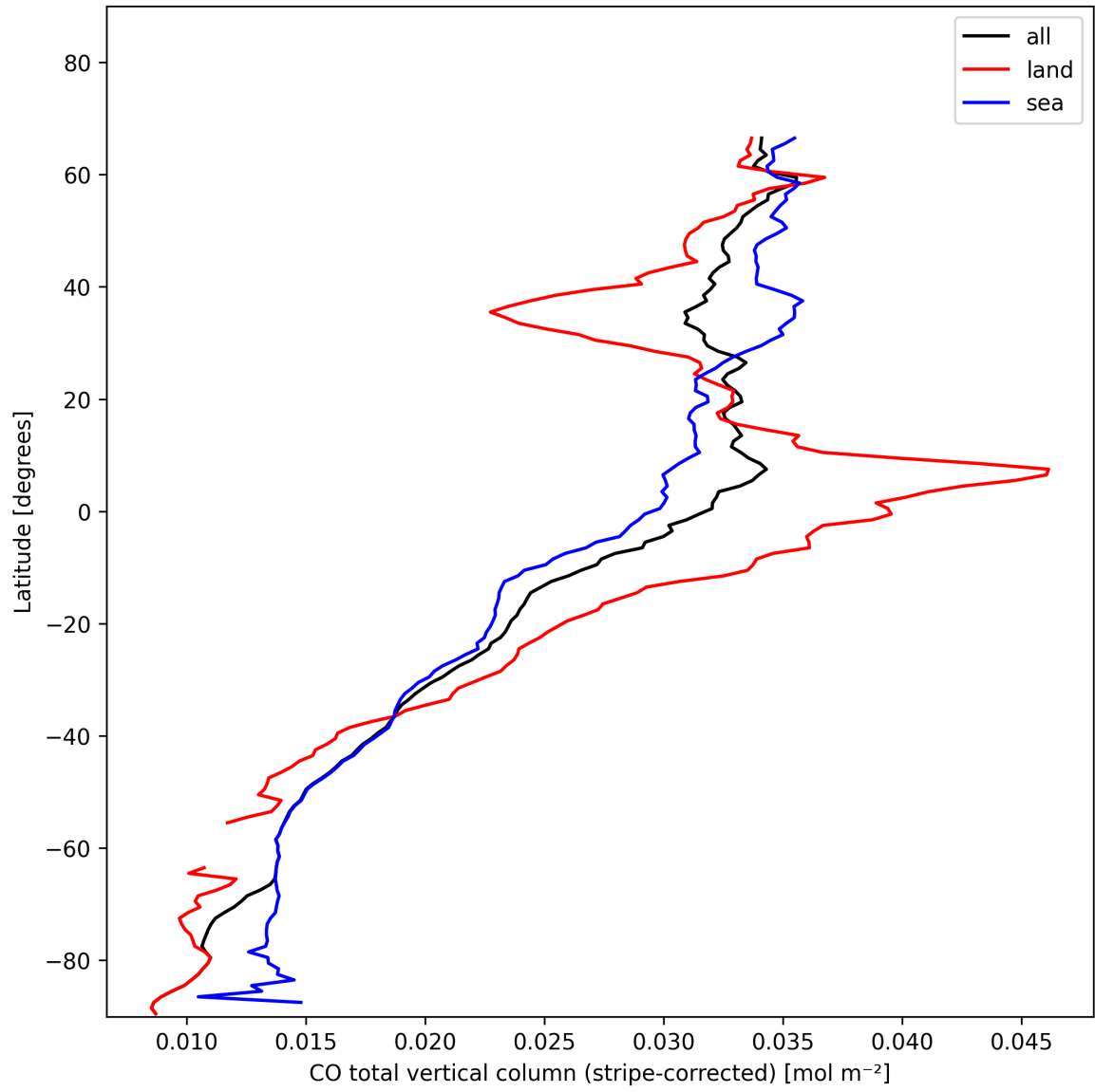
Figure 11: Zonal average of “CO total vertical column (stripe-corrected)” for 2025-01-26 to 2025-01-28.
