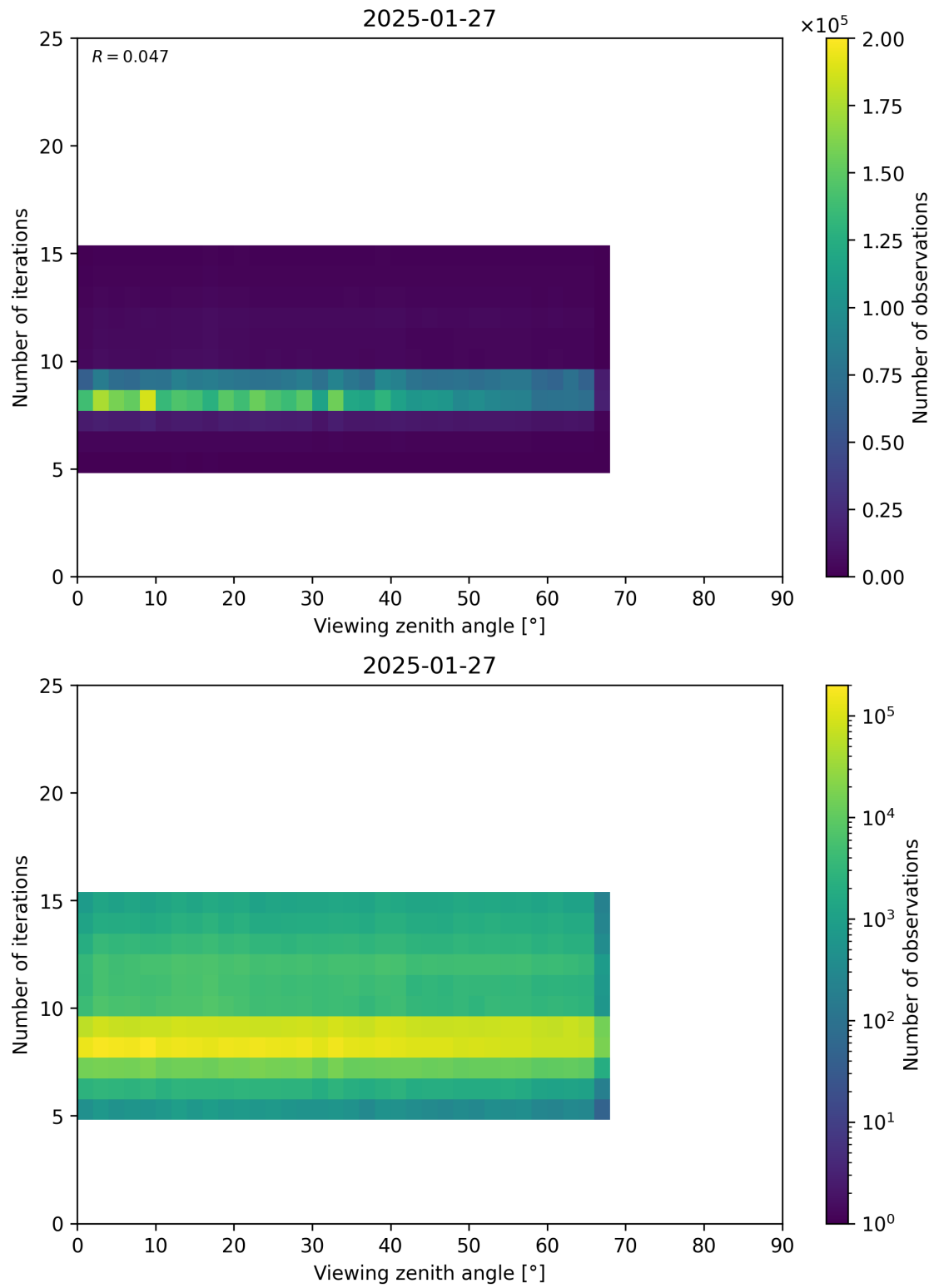
Figure 75: Scatter density plot of “Viewing zenith angle” against “Number of iterations” for 2025-01-26 to 2025-01-28.
