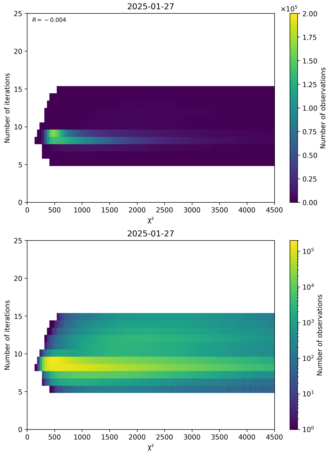
Figure 49: Scatter density plot of “ \chi^2 ” against “Number of iterations” for 2025-01-26 to 2025-01-28.
