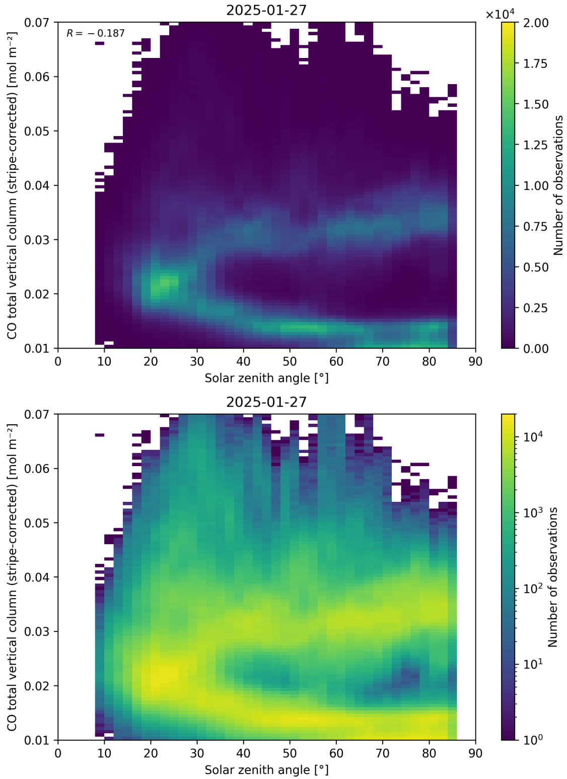
Figure 62: Scatter density plot of “Solar zenith angle” against “CO total vertical column (stripe-corrected)” for 2025-01-26 to 2025-01-28.
