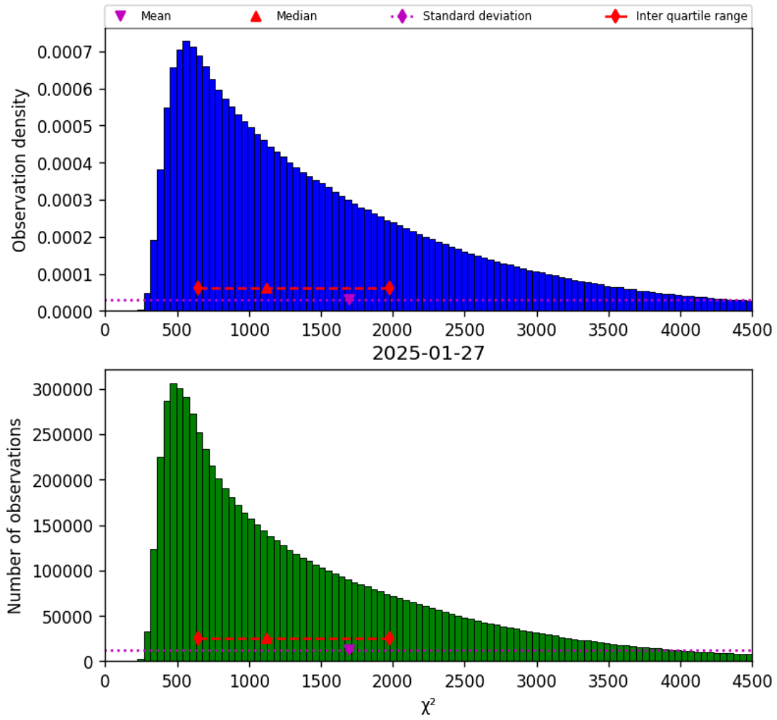
Figure 22: Histogram of “ \chi^2 ” for 2025-01-26 to 2025-01-28
