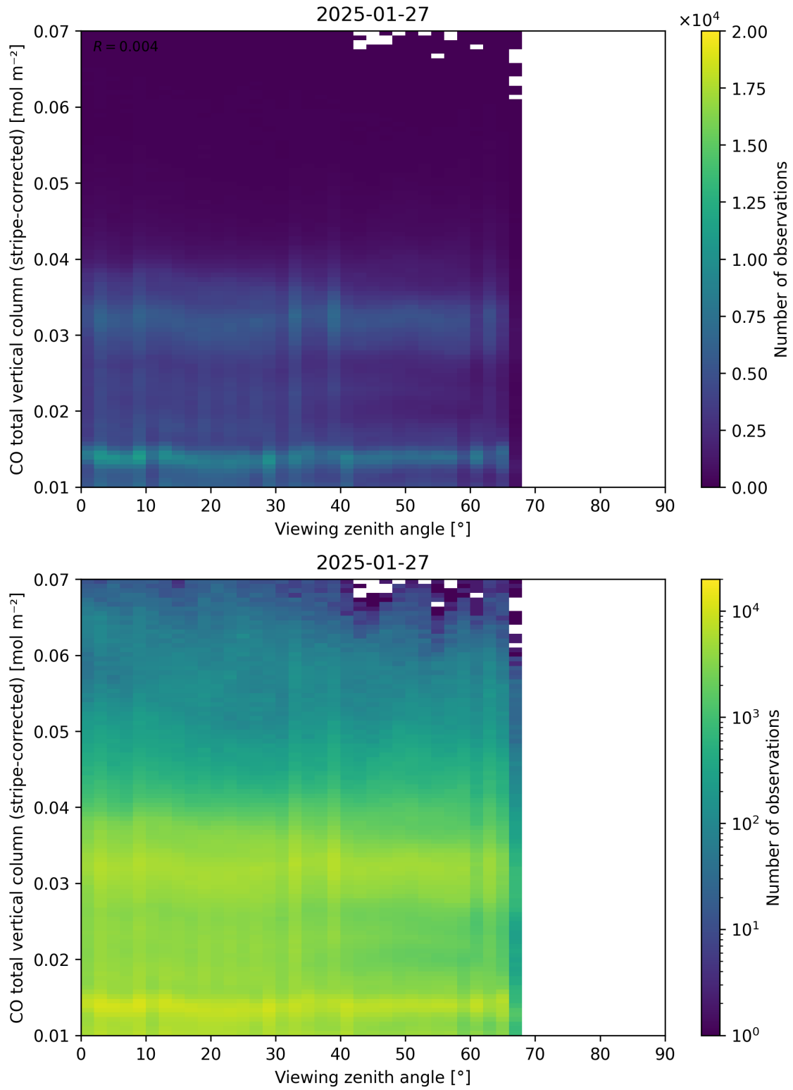
Figure 70: Scatter density plot of “Viewing zenith angle” against “CO total vertical column (stripe-corrected)” for 2025-01-26 to 2025-01-28.
