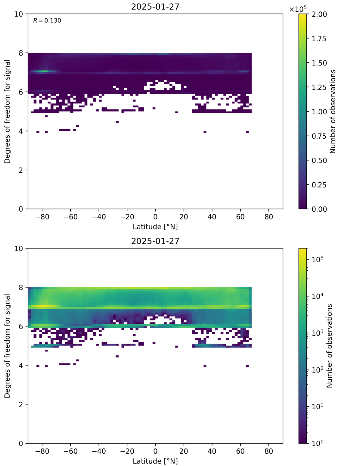
Figure 55: Scatter density plot of “Latitude” against “Degrees of freedom for signal” for 2025-01-26 to 2025-01-28.
