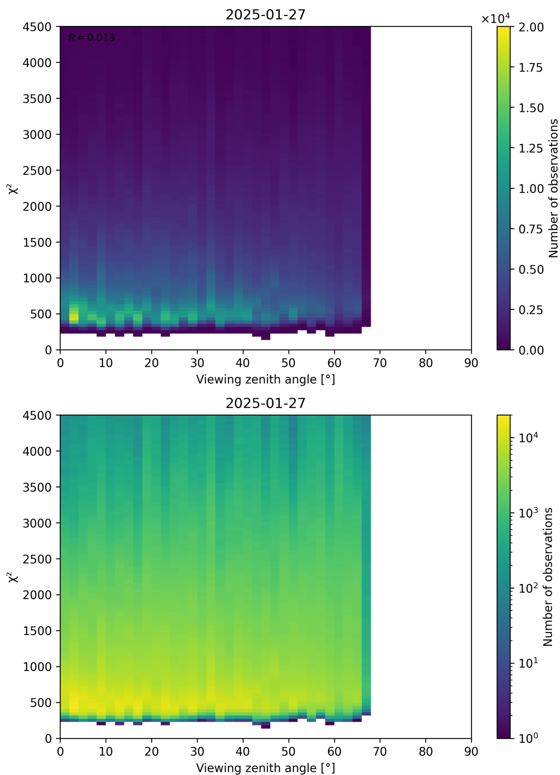
Figure 72: Scatter density plot of “Viewing zenith angle” against “ \chi^2 ” for 2025-01-26 to 2025-01-28.
