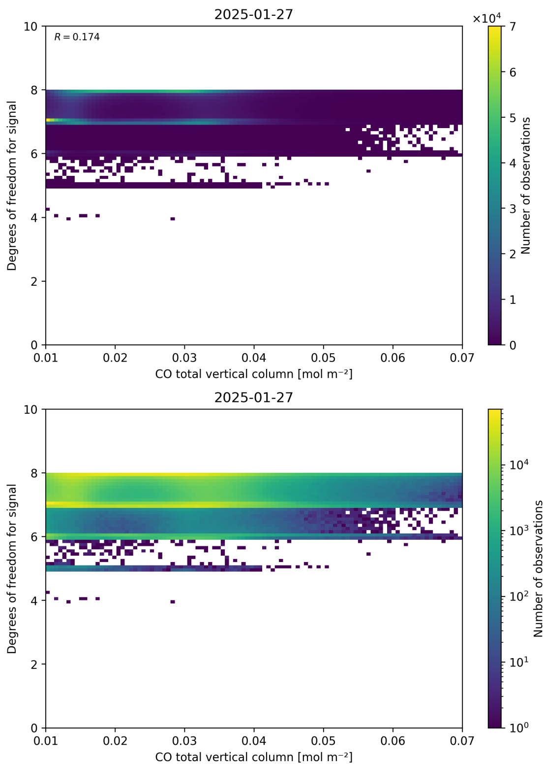
Figure 41: Scatter density plot of “CO total vertical column” against “Degrees of freedom for signal” for 2025-01-26 to 2025-01-28.
