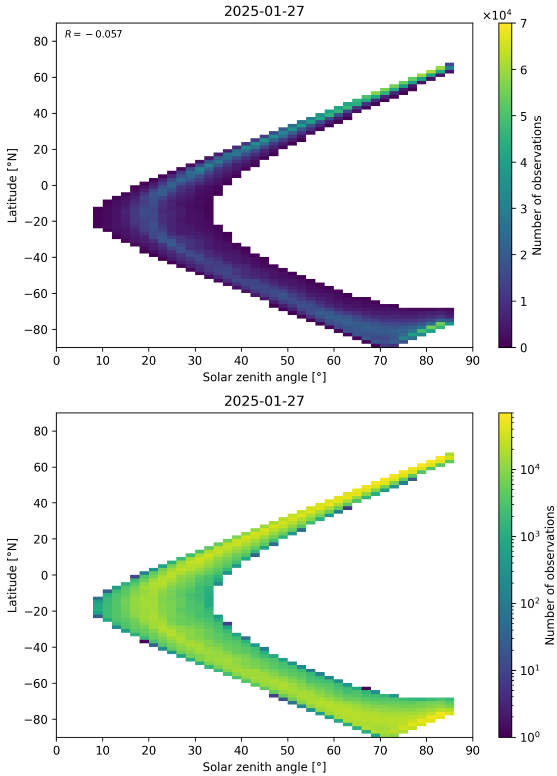
Figure 66: Scatter density plot of “Solar zenith angle” against “Latitude” for 2025-01-26 to 2025-01-28.
