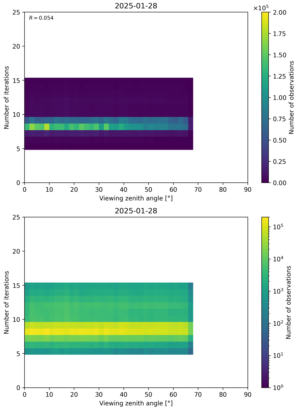
Figure 75: Scatter density plot of “Viewing zenith angle” against “Number of iterations” for 2025-01-28 to 2025-01-29.
