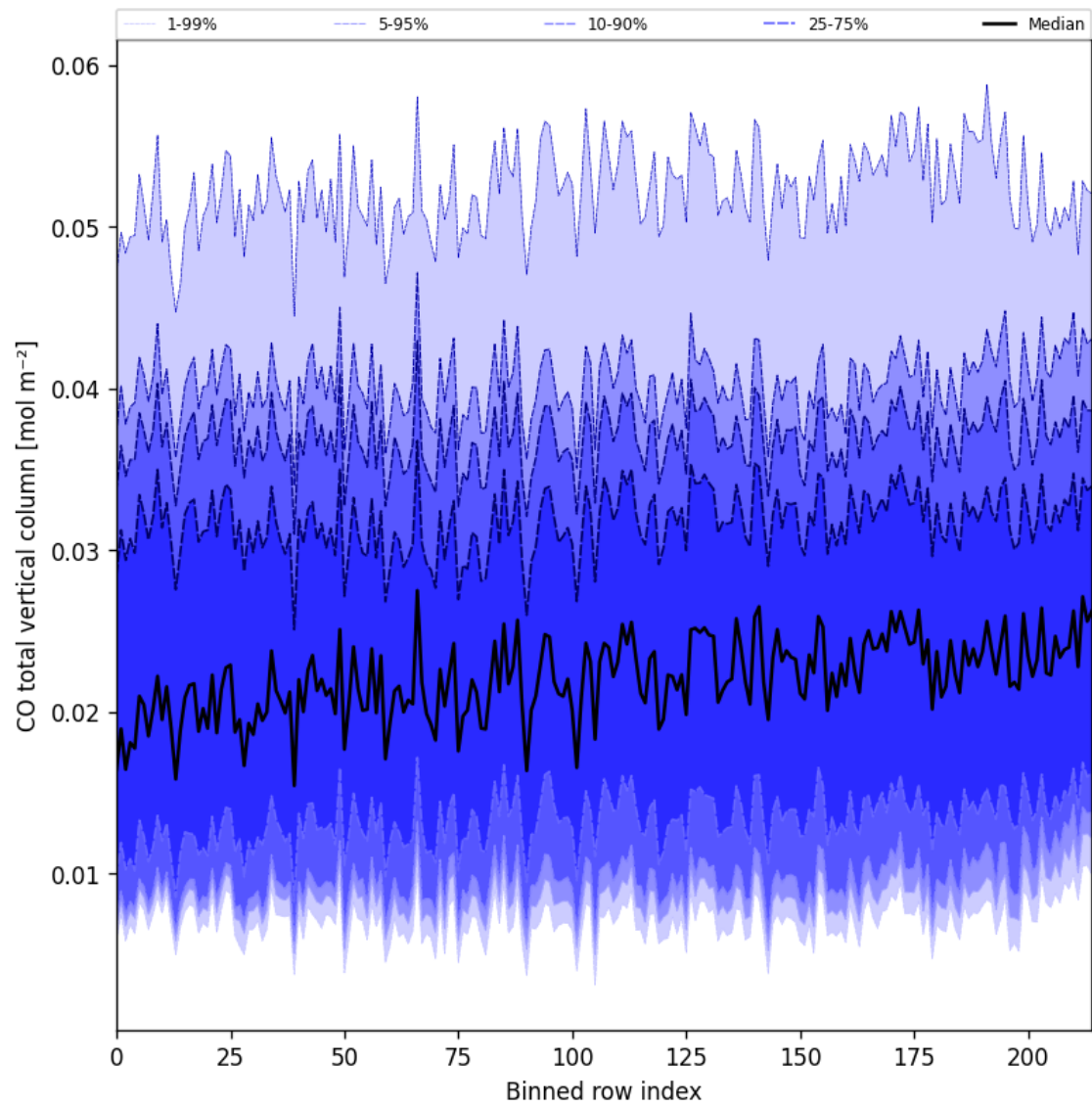
Figure 26: Along track statistics of “CO total vertical column” for 2025-01-28 to 2025-01-29
