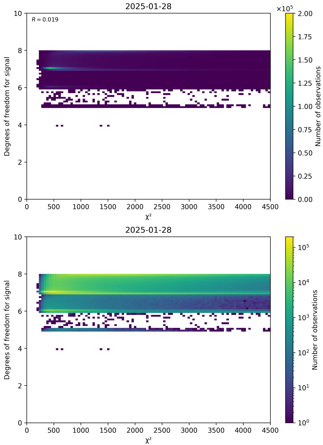
Figure 48: Scatter density plot of “ \chi^2 ” against “Degrees of freedom for signal” for 2025-01-28 to 2025-01-29.
