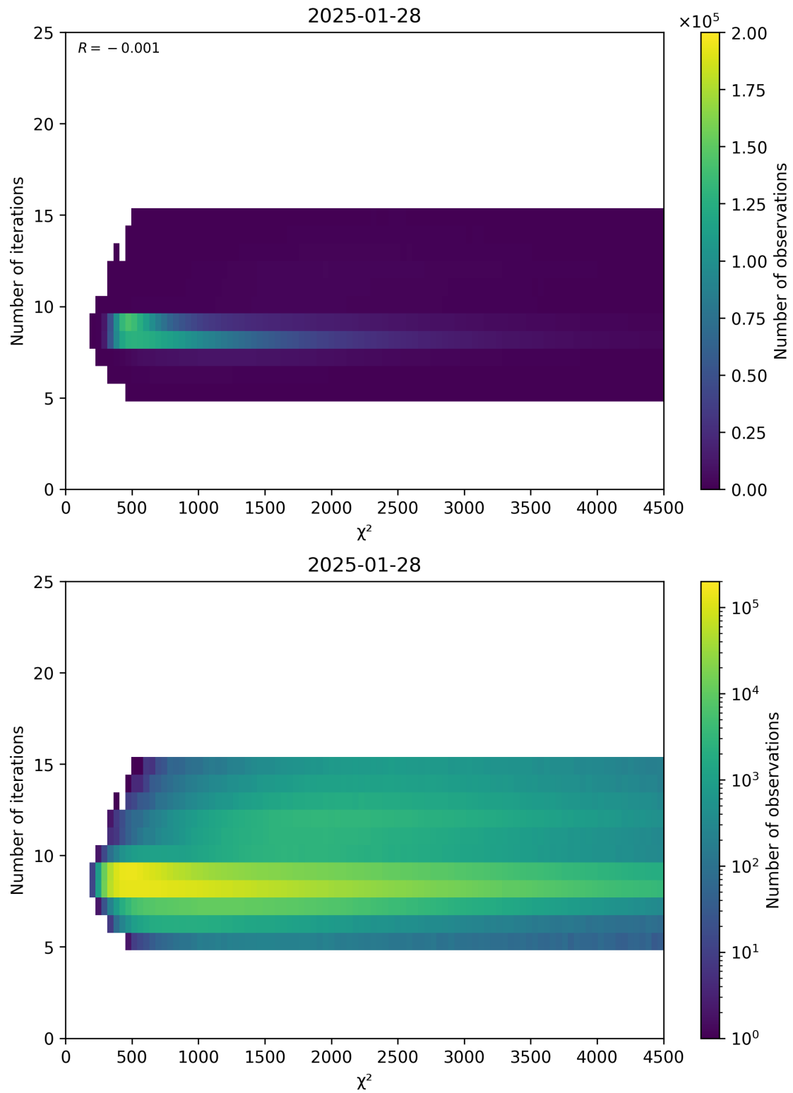
Figure 49: Scatter density plot of “ \chi^2 ” against “Number of iterations” for 2025-01-28 to 2025-01-29.
