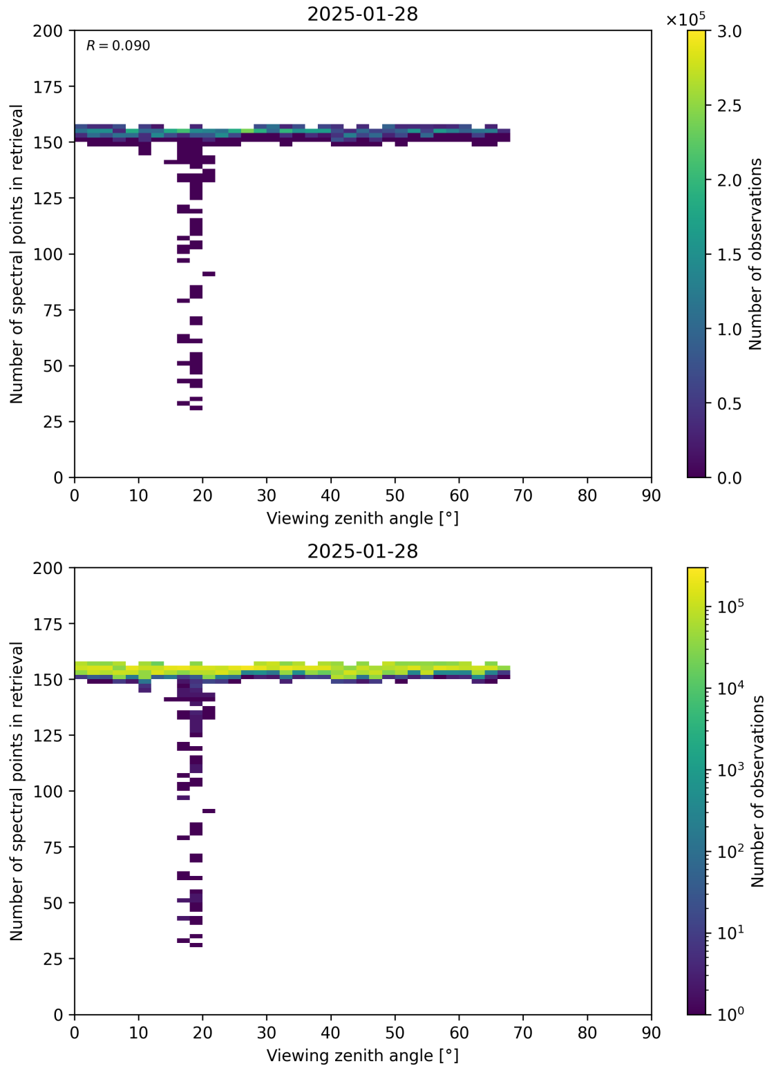
Figure 76: Scatter density plot of “Viewing zenith angle” against “Number of spectral points in retrieval” for 2025-01-28 to 2025-01-29.
