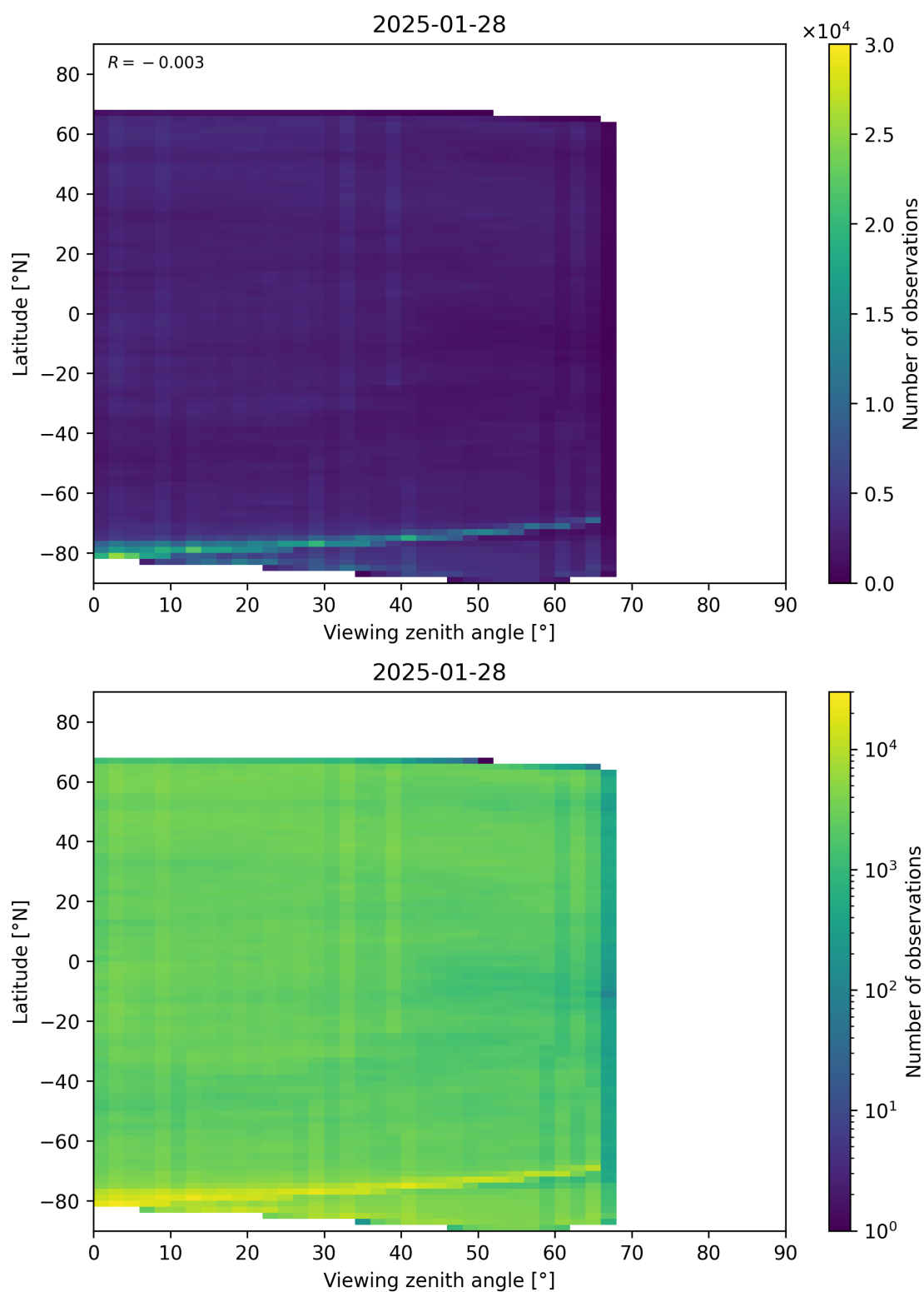
Figure 74: Scatter density plot of “Viewing zenith angle” against “Latitude” for 2025-01-28 to 2025-01-29.
