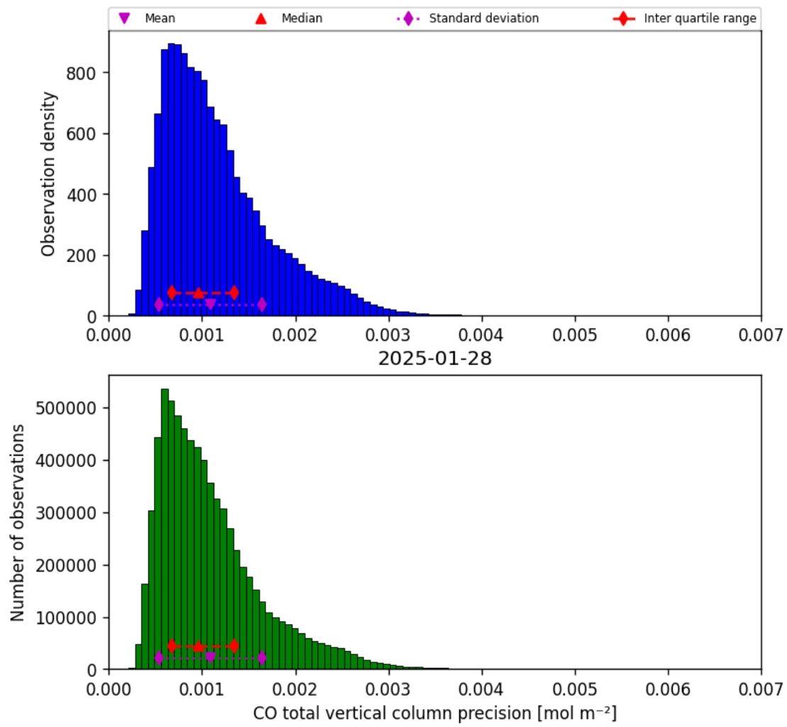
Figure 20: Histogram of “CO total vertical column precision” for 2025-01-28 to 2025-01-29
