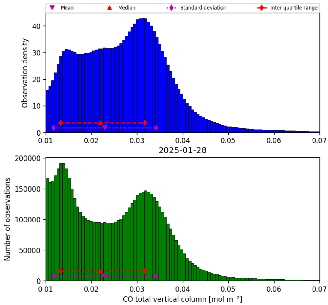
Figure 18: Histogram of “CO total vertical column” for 2025-01-28 to 2025-01-29
