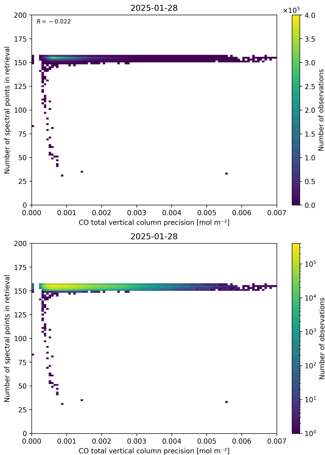
Figure 47: Scatter density plot of “CO total vertical column precision” against “Number of spectral points in retrieval” for 2025-01-28 to 2025-01-29.
