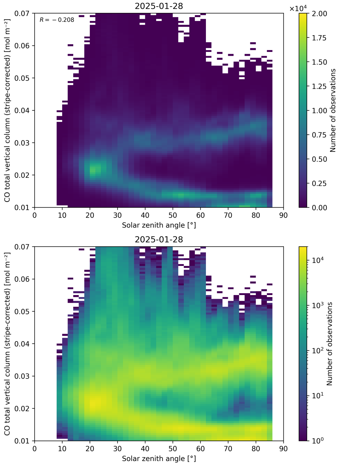
Figure 62: Scatter density plot of “Solar zenith angle” against “CO total vertical column (stripe-corrected)” for 2025-01-28 to 2025-01-29.
