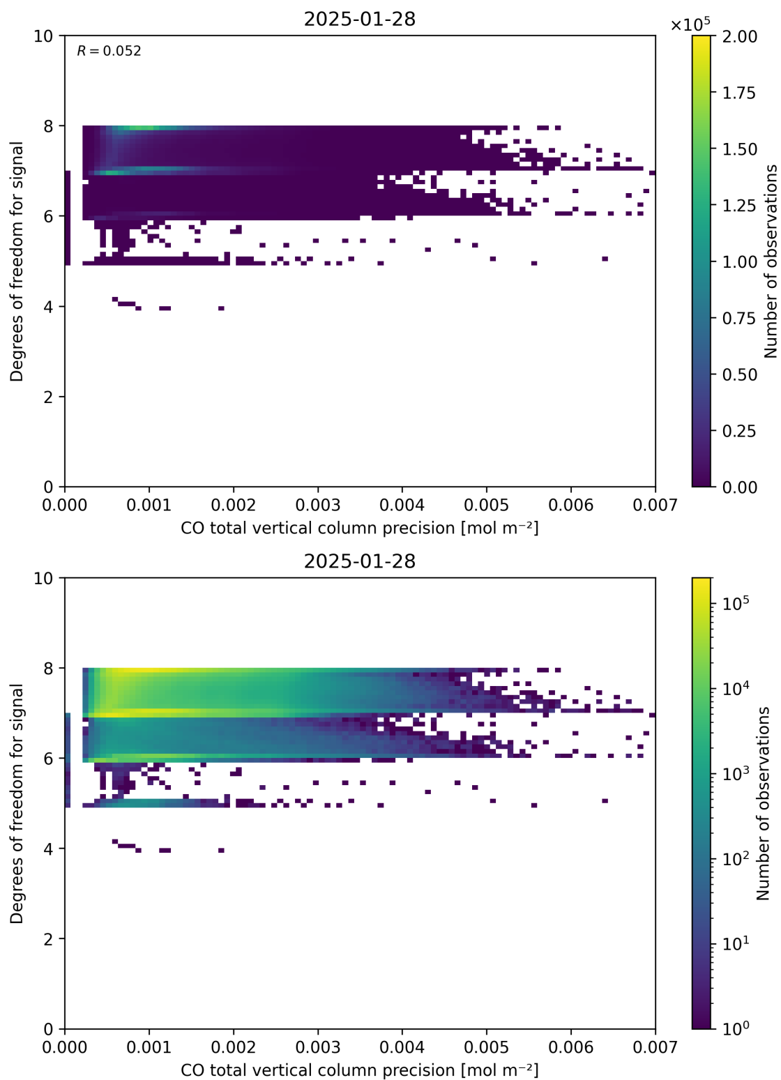
Figure 45: Scatter density plot of “CO total vertical column precision” against “Degrees of freedom for signal” for 2025-01-28 to 2025-01-29.
