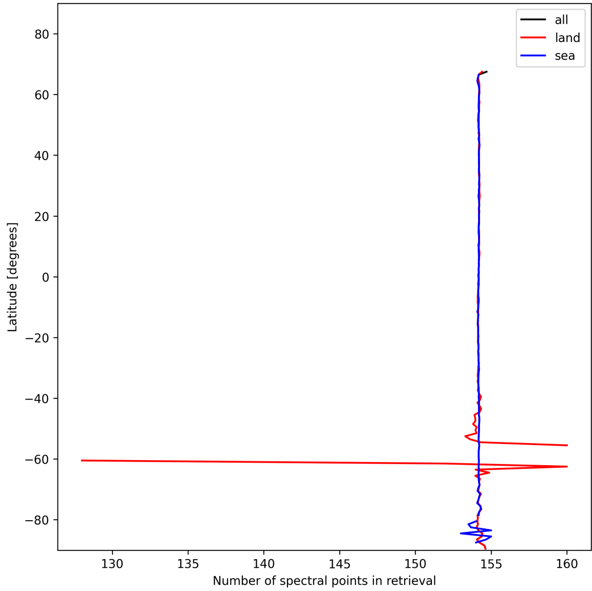
Figure 13: Zonal average of “Number of spectral points in retrieval” for 2025-01-28 to 2025-01-29.
