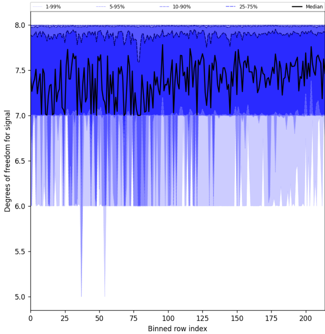
Figure 31: Along track statistics of “Degrees of freedom for signal” for 2025-01-28 to 2025-01-29
