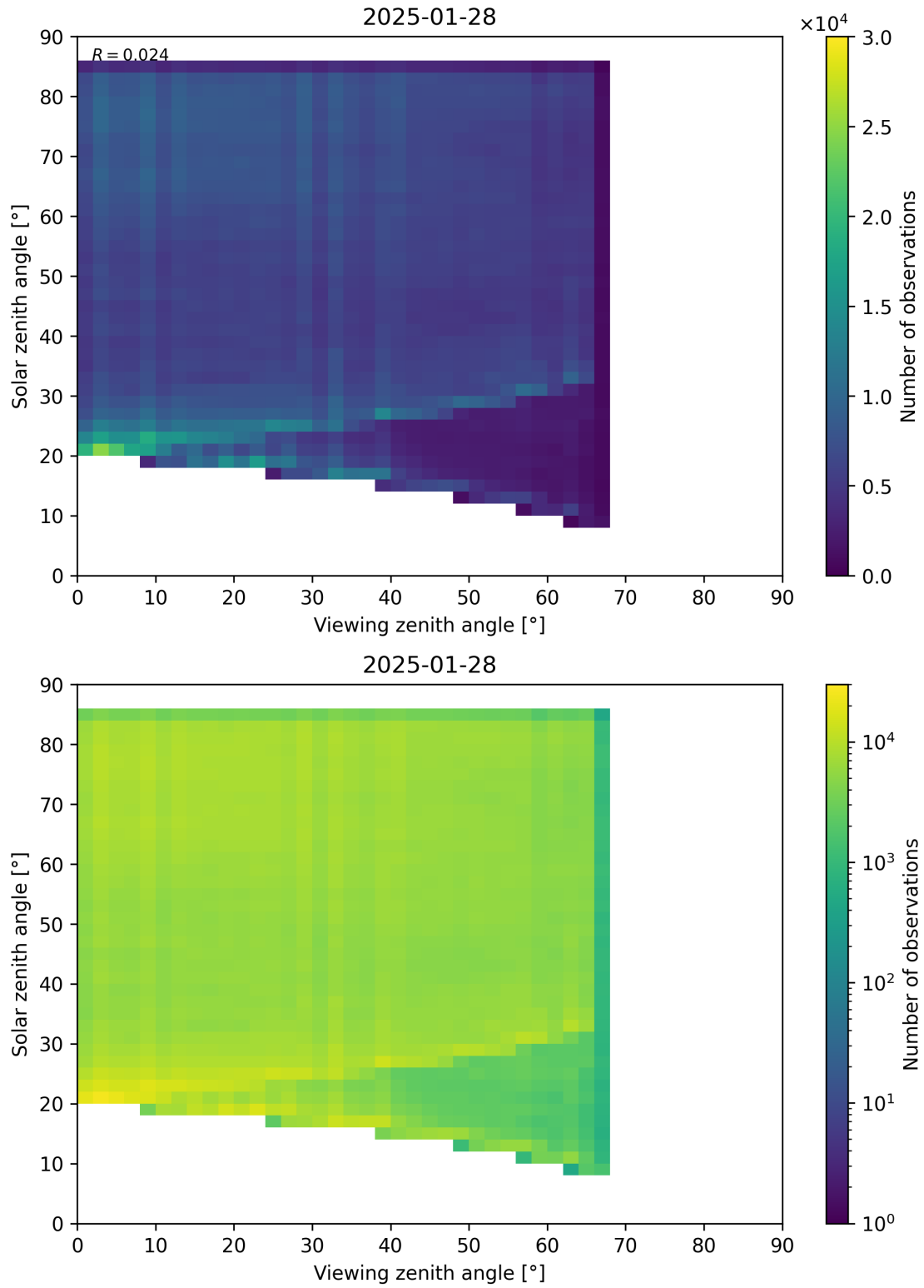
Figure 77: Scatter density plot of “Viewing zenith angle” against “Solar zenith angle” for 2025-01-28 to 2025-01-29.
