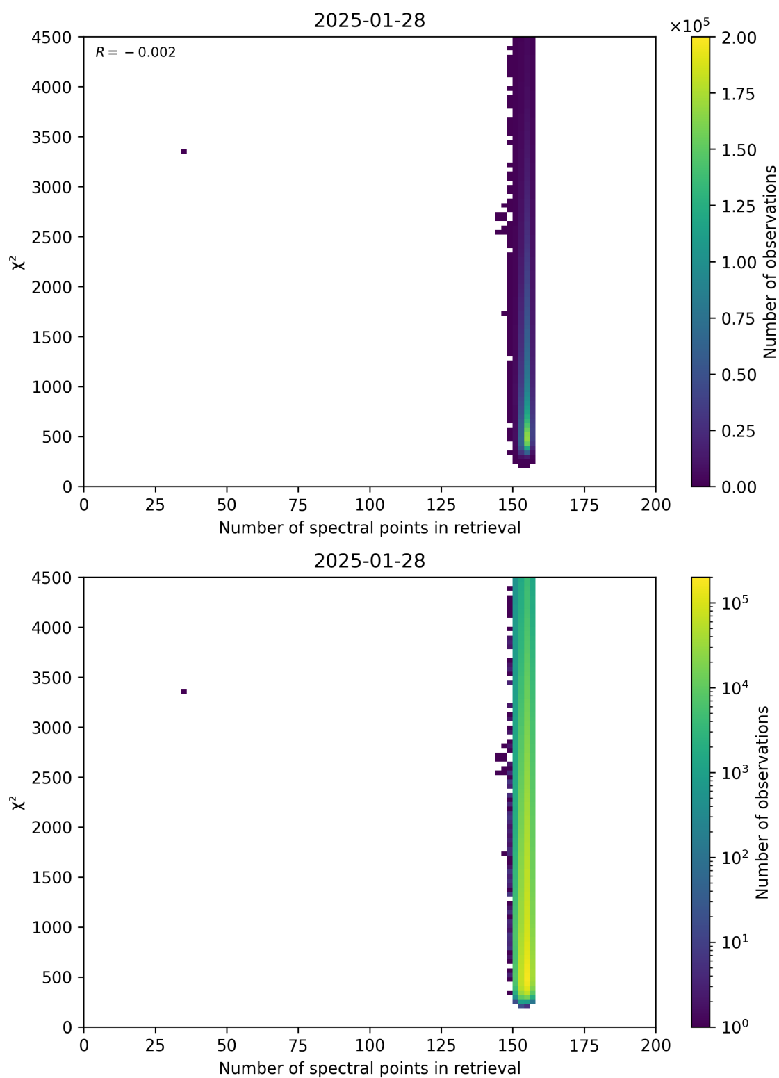
Figure 58: Scatter density plot of “Number of spectral points in retrieval” against “ \chi^2 ” for 2025-01-28 to 2025-01-29.
