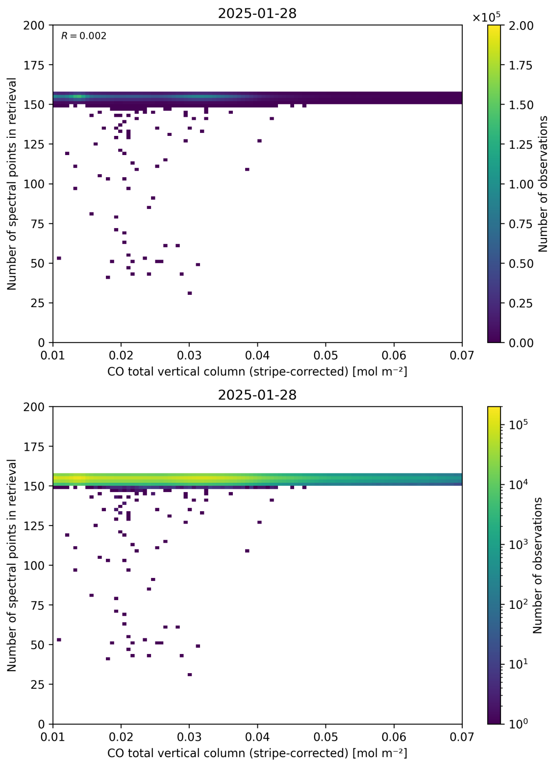
Figure 40: Scatter density plot of “CO total vertical column (stripe-corrected)” against “Number of spectral points in retrieval” for 2025-01-28 to 2025-01-29.
