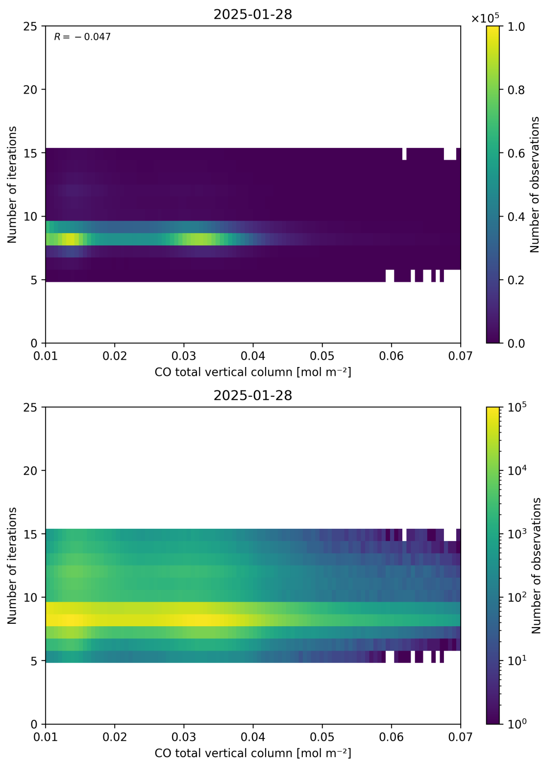
Figure 42: Scatter density plot of “CO total vertical column” against “Number of iterations” for 2025-01-28 to 2025-01-29.
