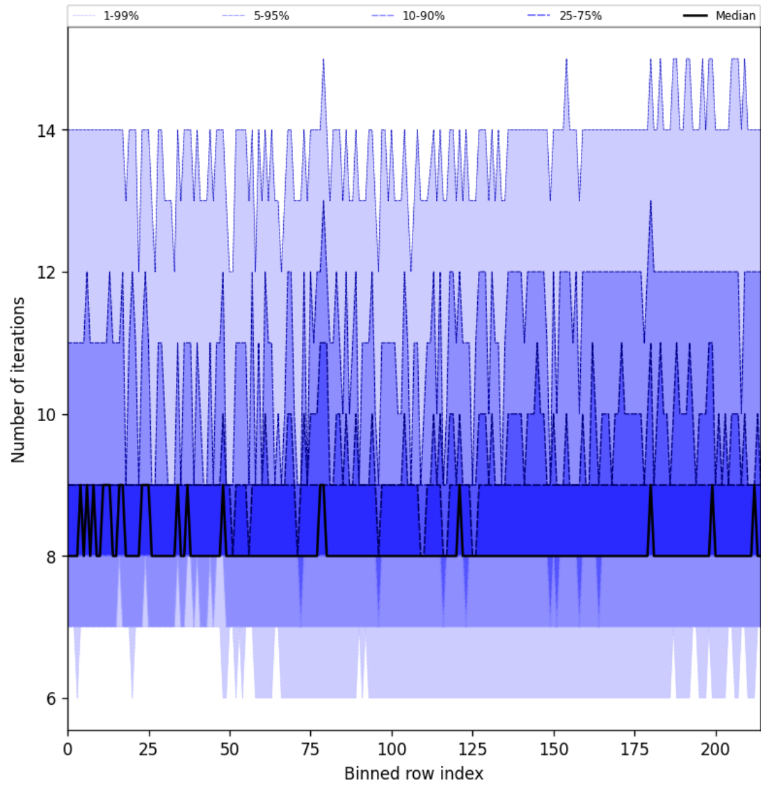
Figure 32: Along track statistics of “Number of iterations” for 2025-01-28 to 2025-01-29
