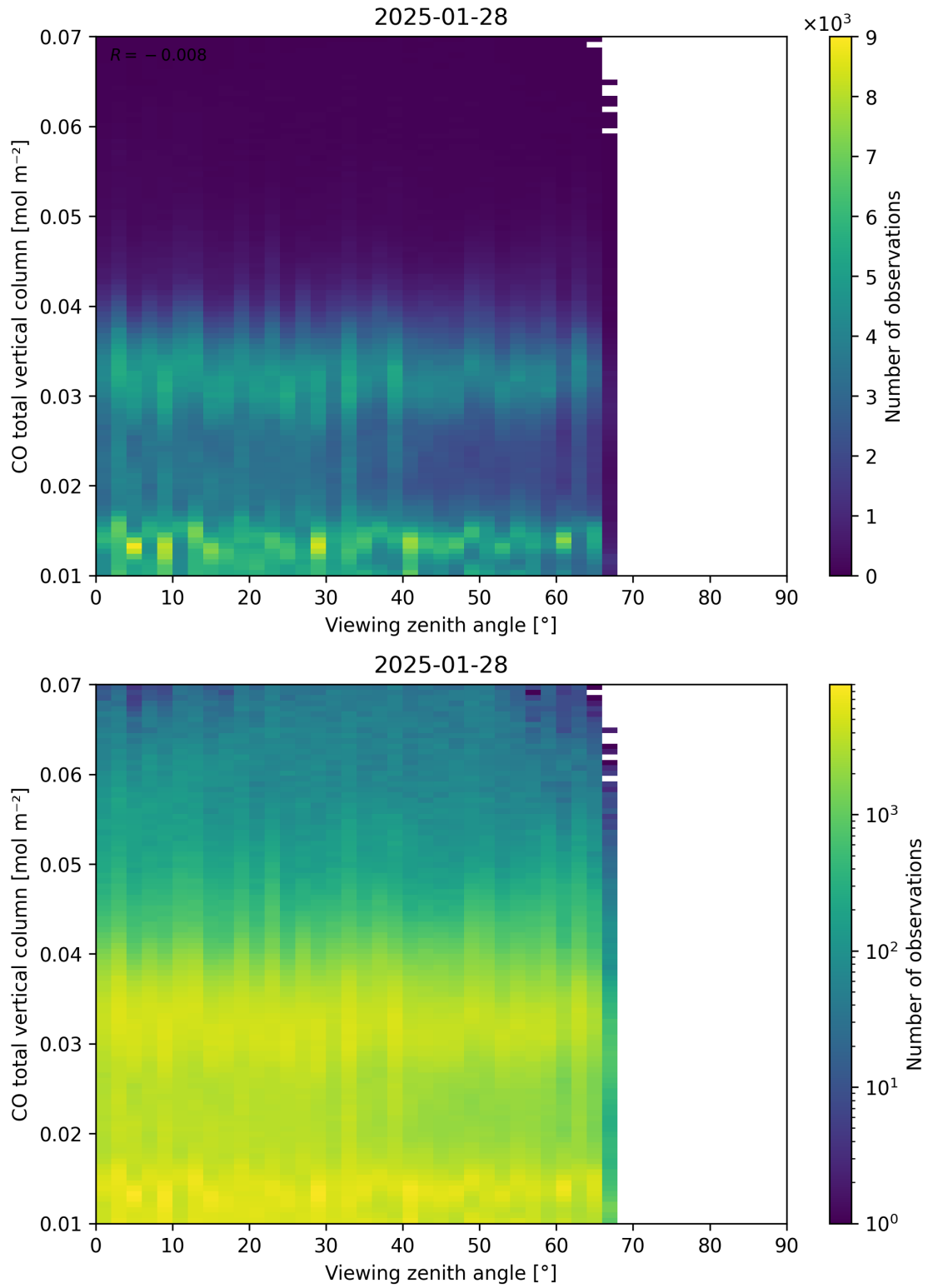
Figure 69: Scatter density plot of “Viewing zenith angle” against “CO total vertical column” for 2025-01-28 to 2025-01-29.
