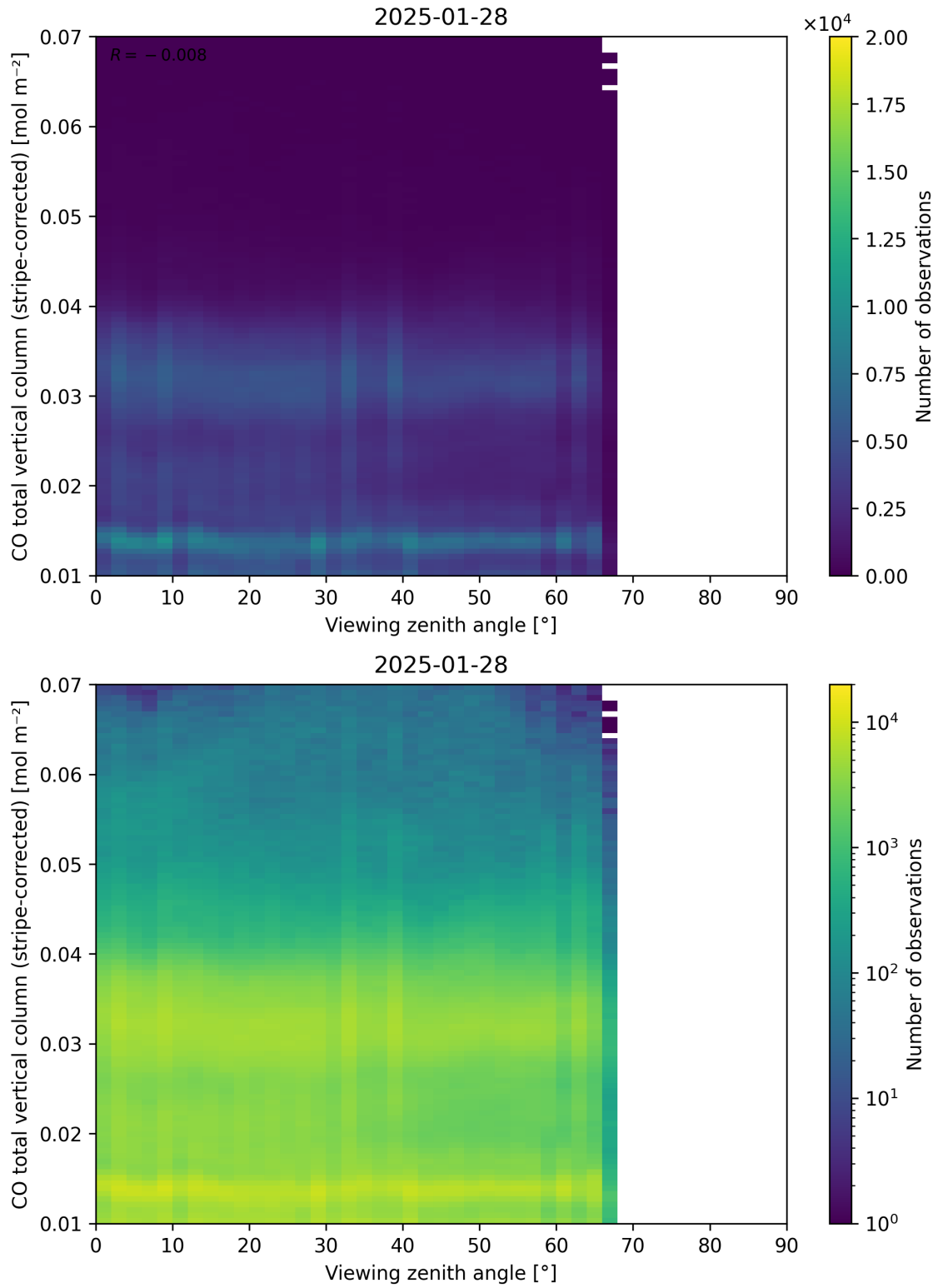
Figure 70: Scatter density plot of “Viewing zenith angle” against “CO total vertical column (stripe-corrected)” for 2025-01-28 to 2025-01-29.
