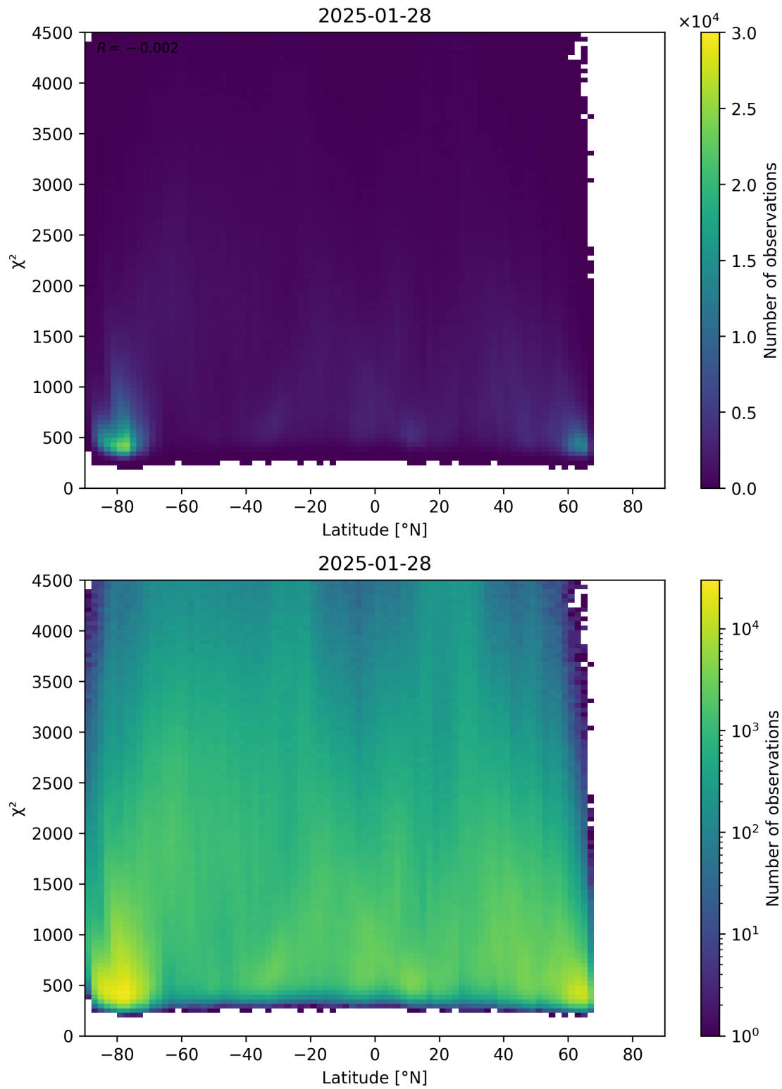
Figure 54: Scatter density plot of “Latitude” against “ \chi^2 ” for 2025-01-28 to 2025-01-29.
