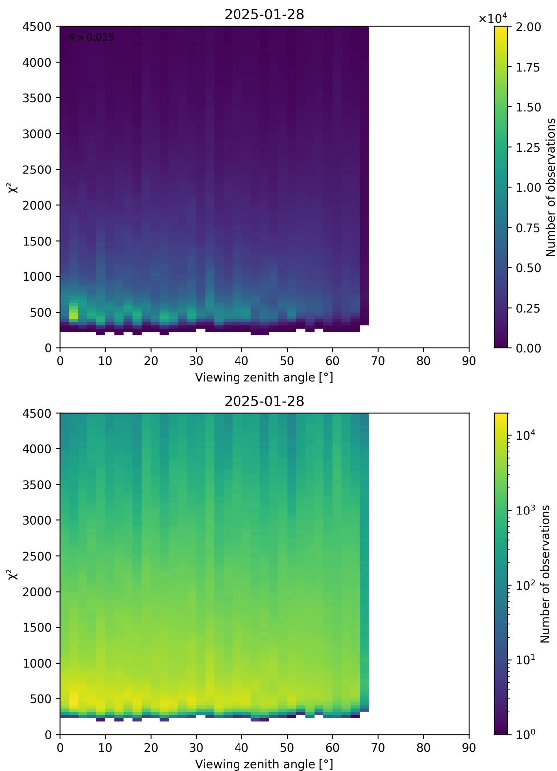
Figure 72: Scatter density plot of “Viewing zenith angle” against “ \chi^2 ” for 2025-01-28 to 2025-01-29.
