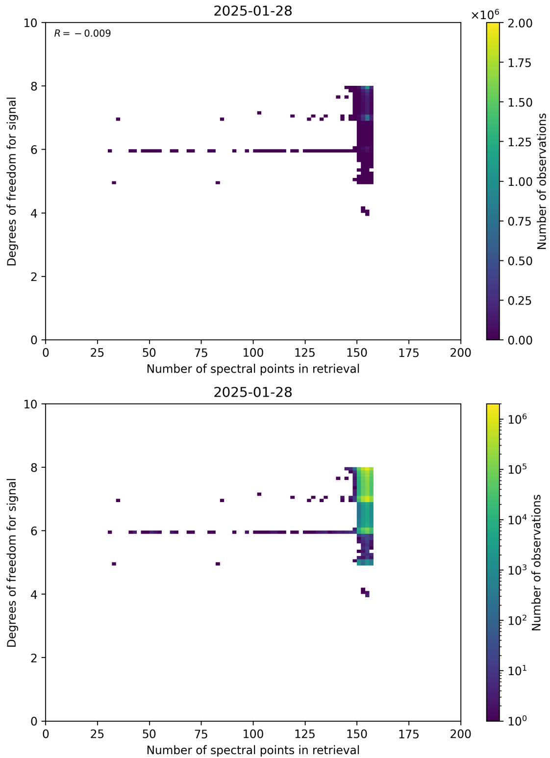
Figure 59: Scatter density plot of “Number of spectral points in retrieval” against “Degrees of freedom for signal” for 2025-01-28 to 2025-01-29.
