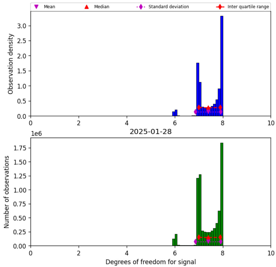
Figure 23: Histogram of “Degrees of freedom for signal” for 2025-01-28 to 2025-01-29
