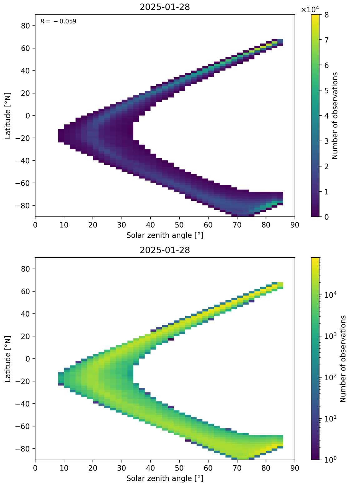
Figure 66: Scatter density plot of “Solar zenith angle” against “Latitude” for 2025-01-28 to 2025-01-29.
