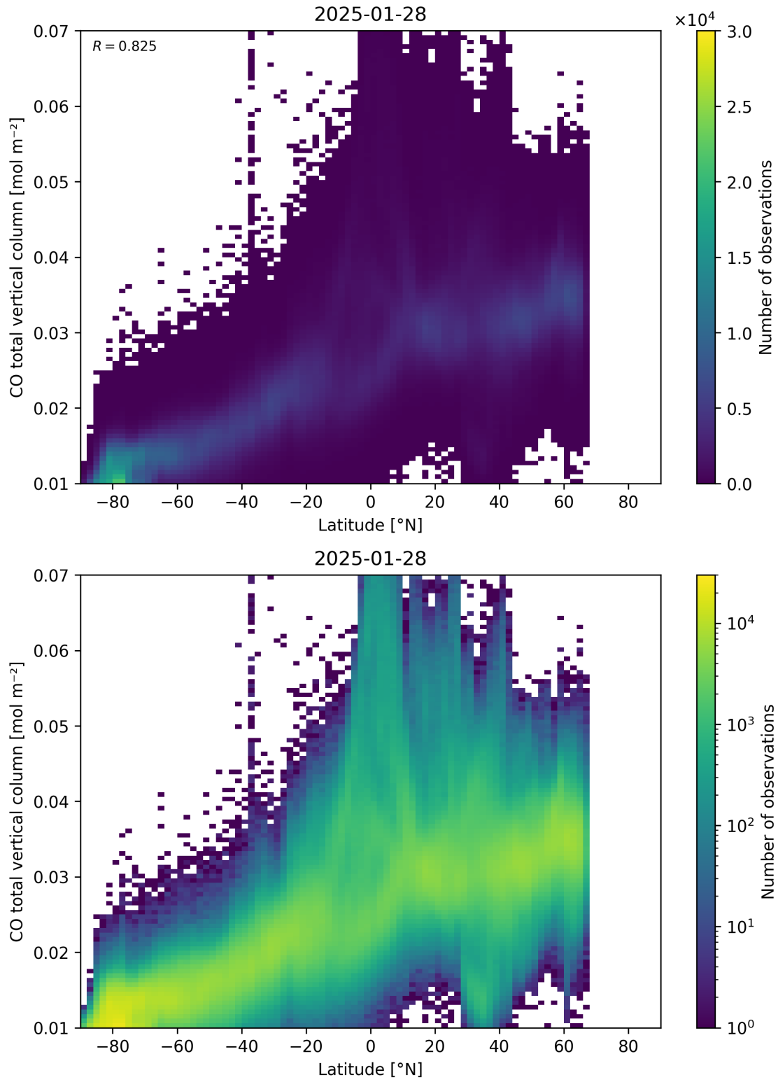
Figure 51: Scatter density plot of “Latitude” against “CO total vertical column” for 2025-01-28 to 2025-01-29.
