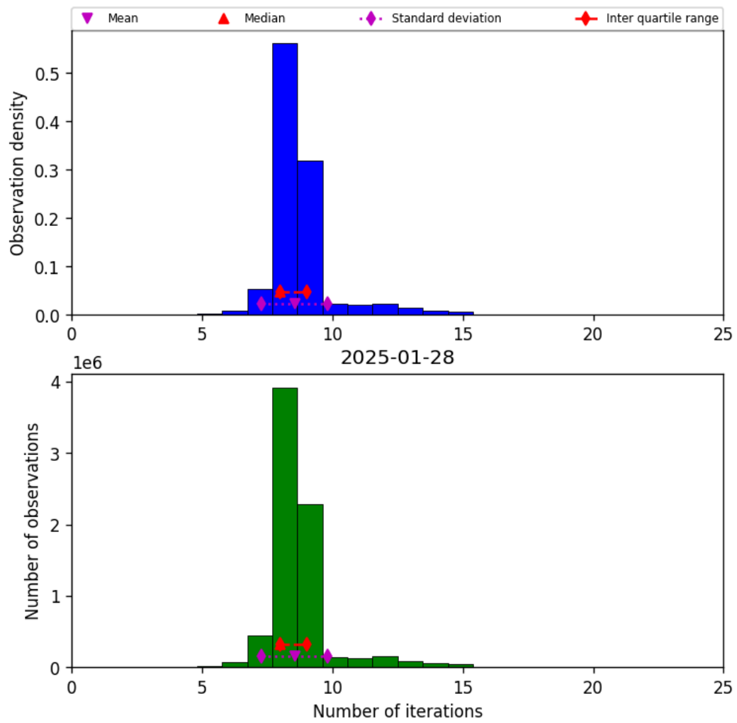
Figure 24: Histogram of “Number of iterations” for 2025-01-28 to 2025-01-29
