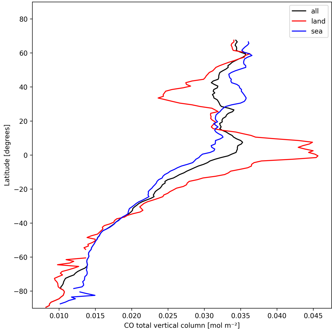
Figure 10: Zonal average of “CO total vertical column” for 2025-01-28 to 2025-01-29.
