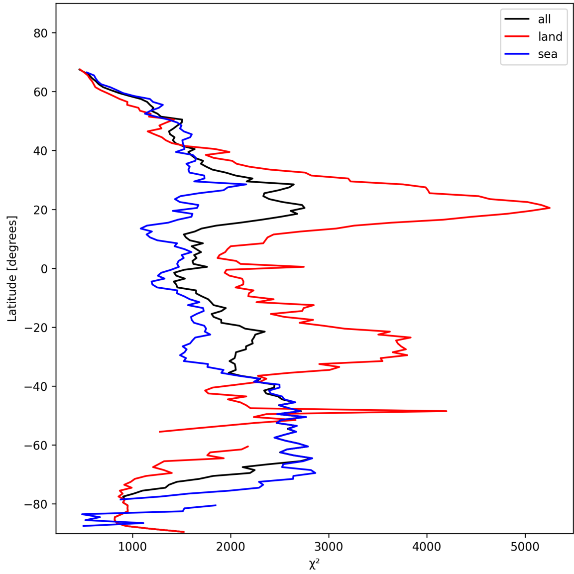
Figure 14: Zonal average of “ \chi^2 ” for 2025-01-28 to 2025-01-29.
