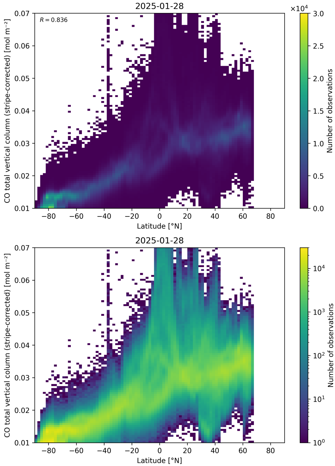
Figure 52: Scatter density plot of “Latitude” against “CO total vertical column (stripe-corrected)” for 2025-01-28 to 2025-01-29.
