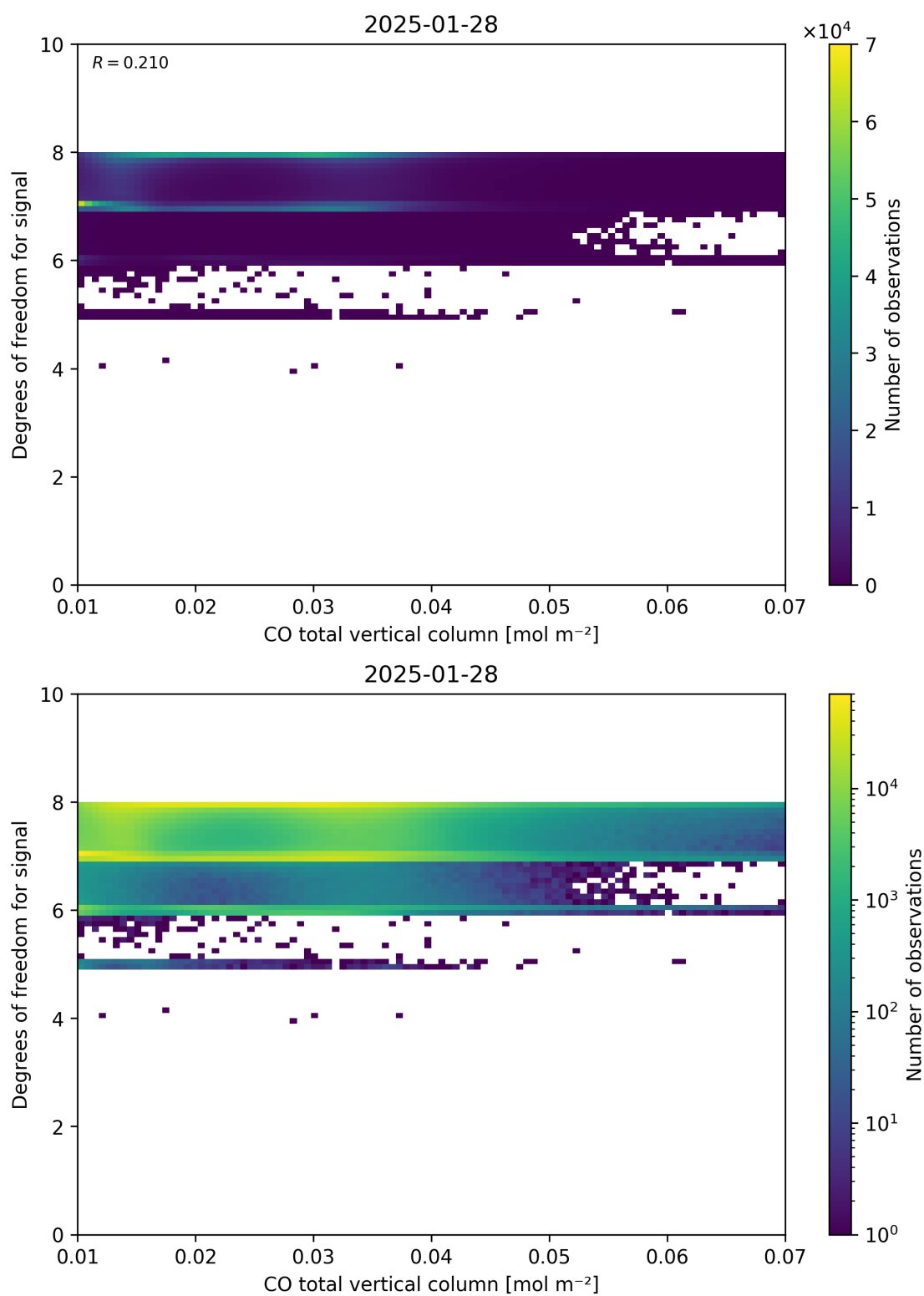
Figure 41: Scatter density plot of “CO total vertical column” against “Degrees of freedom for signal” for 2025-01-28 to 2025-01-29.
