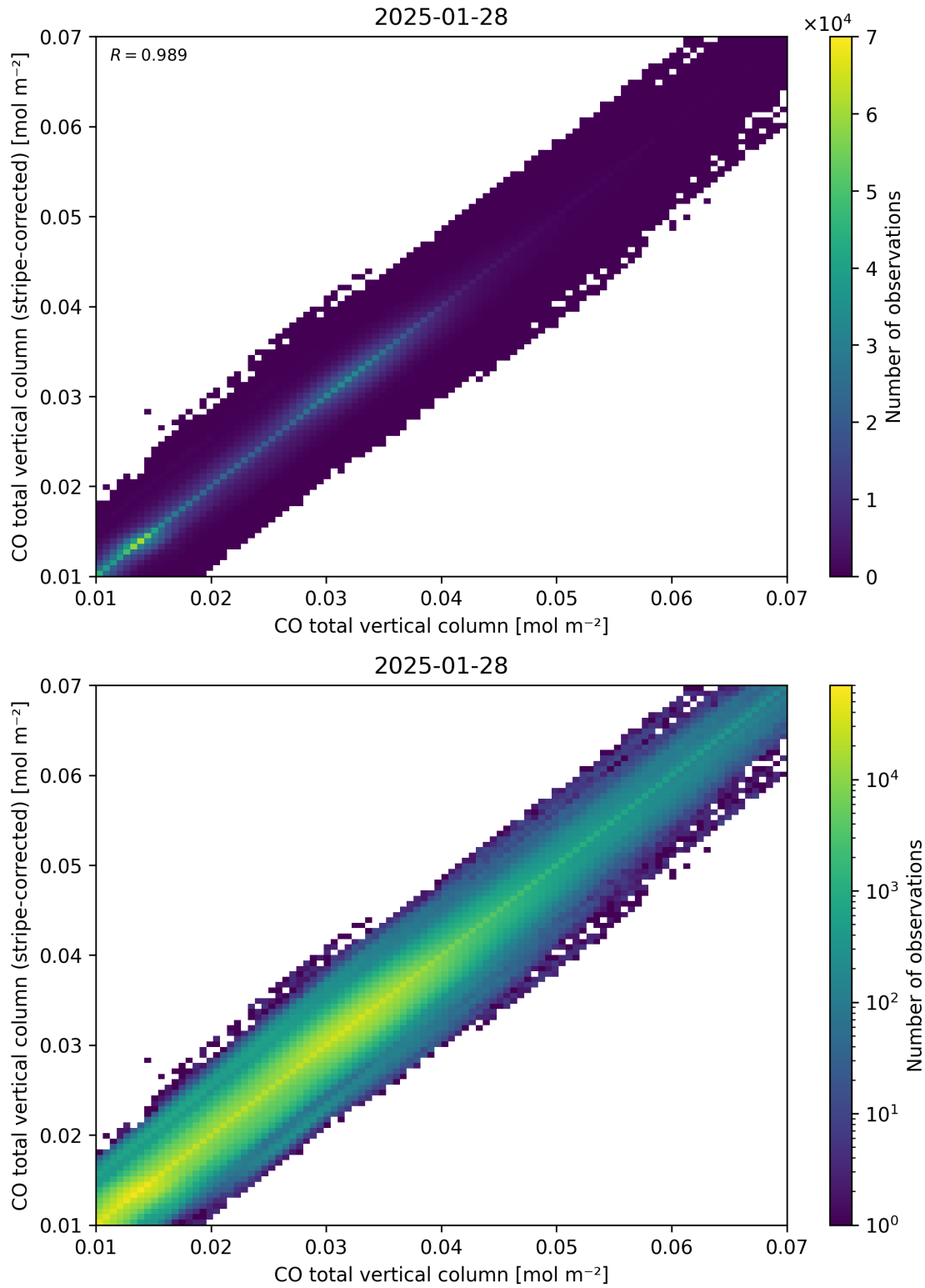
Figure 33: Scatter density plot of “CO total vertical column” against “CO total vertical column (stripe-corrected)” for 2025-01-28 to 2025-01-29.
