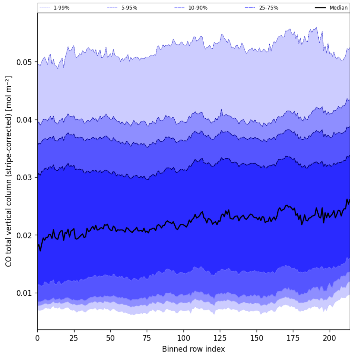
Figure 27: Along track statistics of “CO total vertical column (stripe-corrected)” for 2025-01-28 to 2025-01-29
