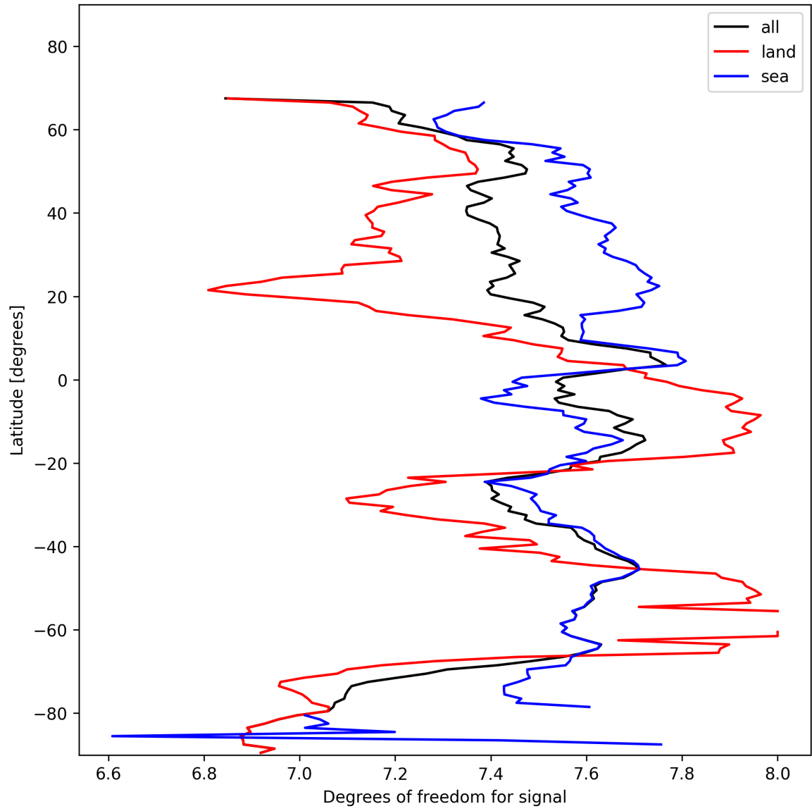
Figure 15: Zonal average of “Degrees of freedom for signal” for 2025-01-28 to 2025-01-29.
