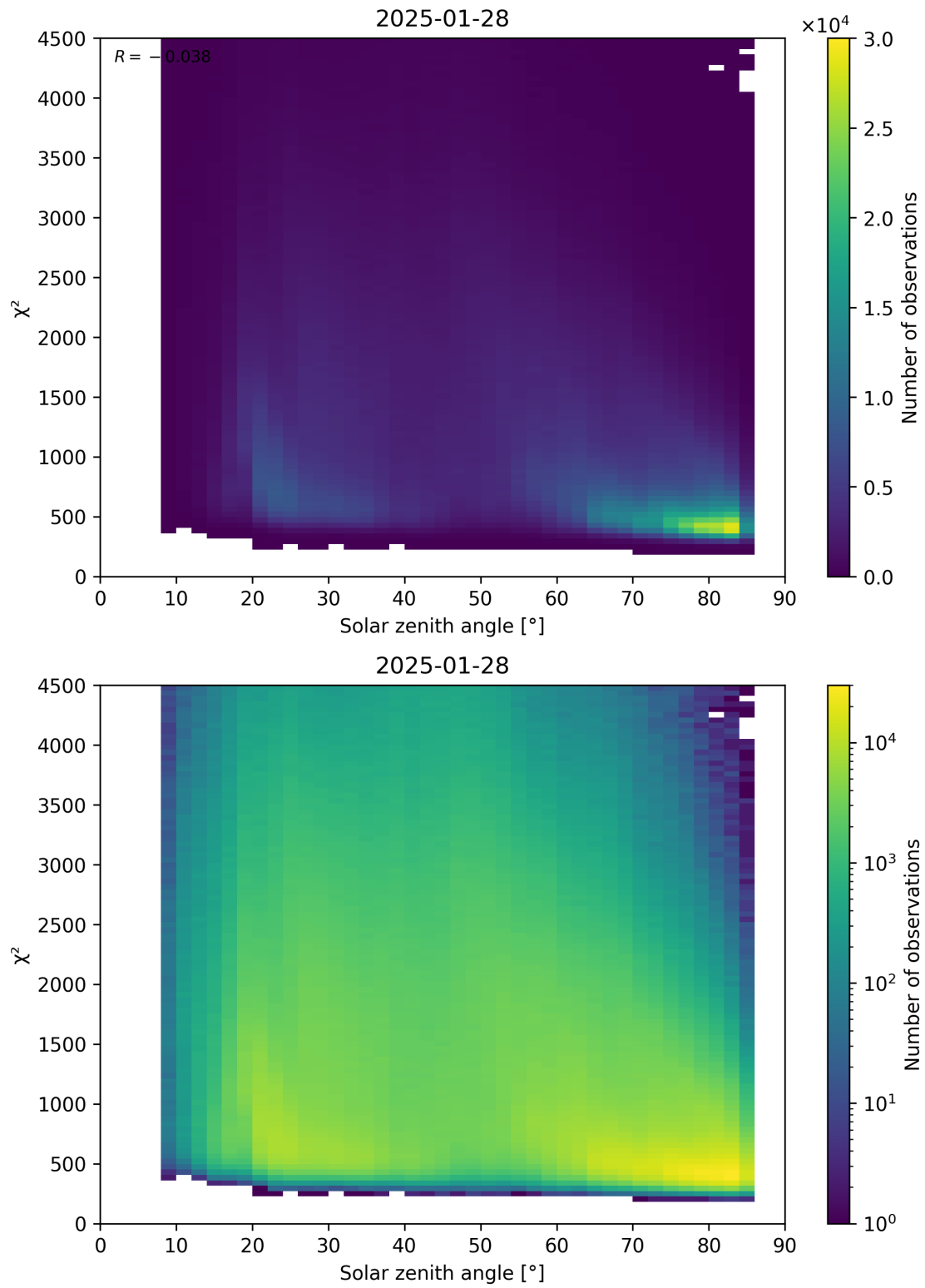
Figure 64: Scatter density plot of “Solar zenith angle” against “ \chi^2 ” for 2025-01-28 to 2025-01-29.
