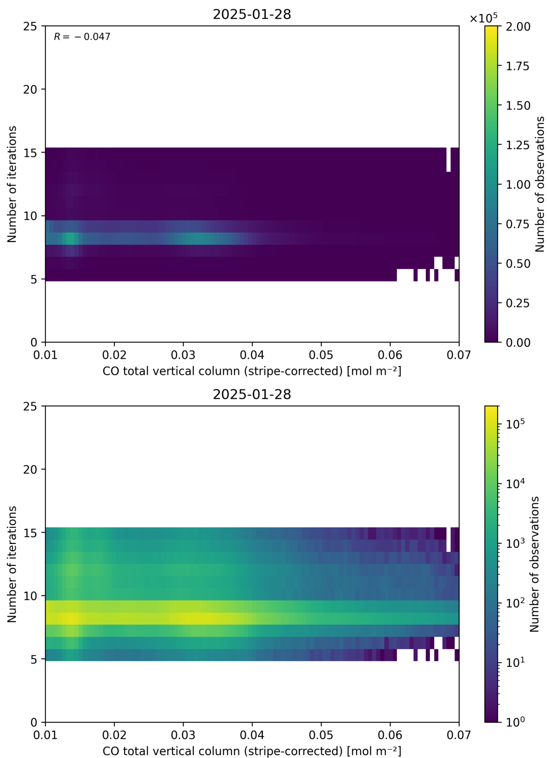
Figure 39: Scatter density plot of “CO total vertical column (stripe-corrected)” against “Number of iterations” for 2025-01-28 to 2025-01-29.
