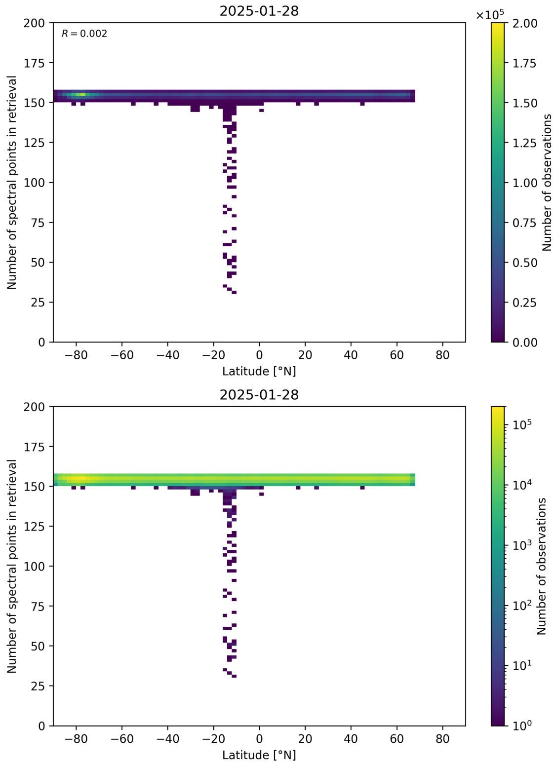
Figure 57: Scatter density plot of “Latitude” against “Number of spectral points in retrieval” for 2025-01-28 to 2025-01-29.
