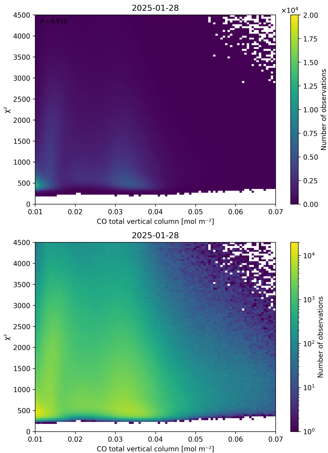
Figure 35: Scatter density plot of “CO total vertical column” against “ \chi^2 ” for 2025-01-28 to 2025-01-29.
