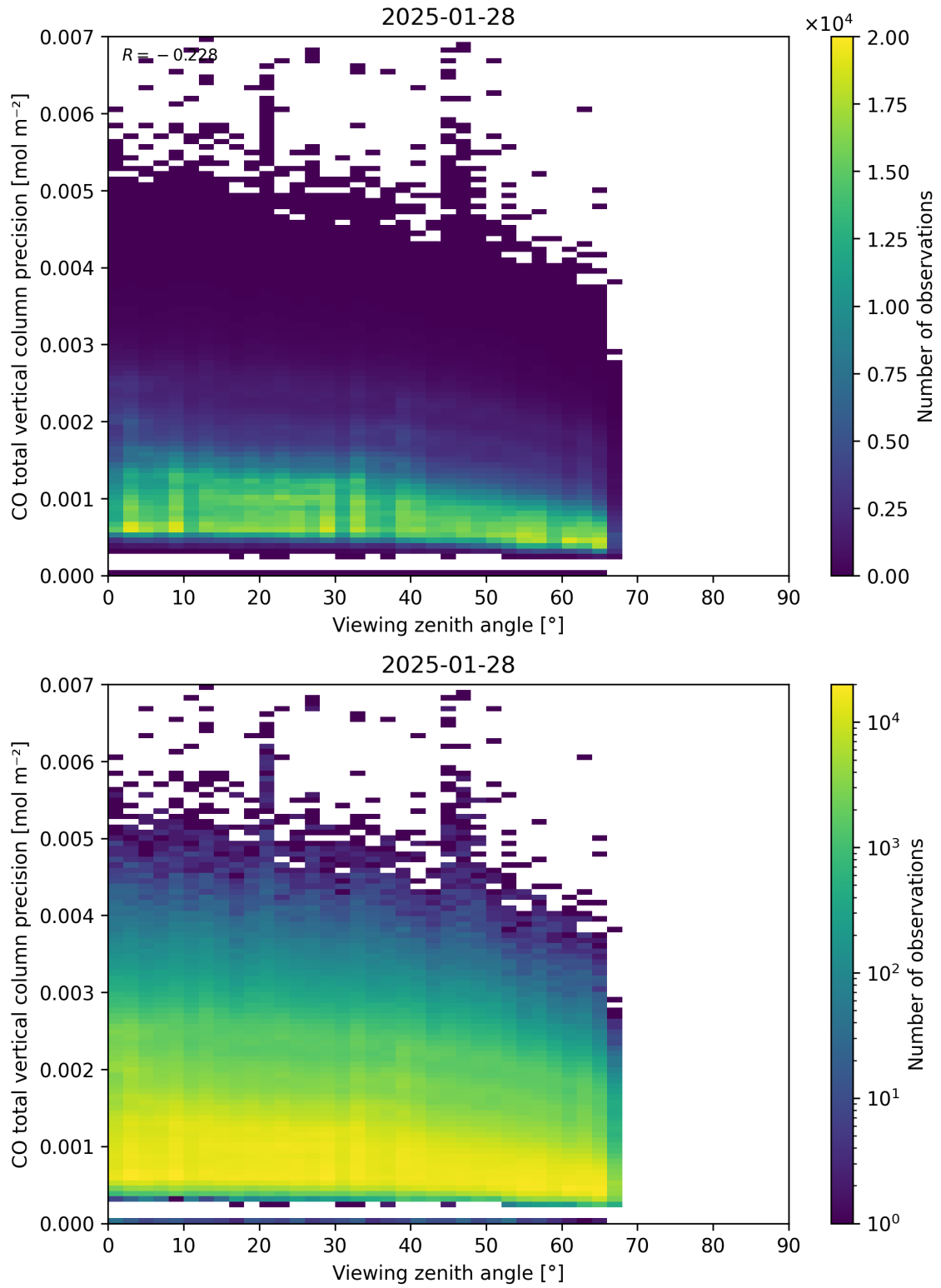
Figure 71: Scatter density plot of “Viewing zenith angle” against “CO total vertical column precision” for 2025-01-28 to 2025-01-29.
