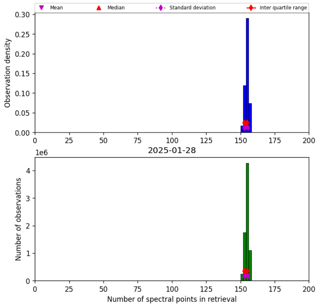
Figure 21: Histogram of “Number of spectral points in retrieval” for 2025-01-28 to 2025-01-29
