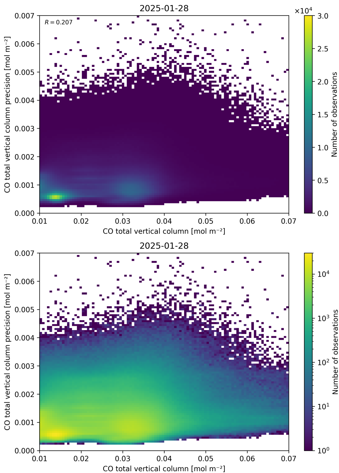
Figure 34: Scatter density plot of “CO total vertical column” against “CO total vertical column precision” for 2025-01-28 to 2025-01-29.
