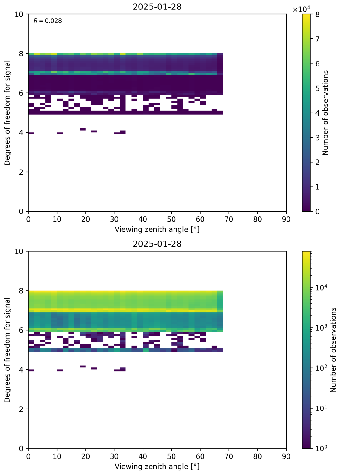
Figure 73: Scatter density plot of “Viewing zenith angle” against “Degrees of freedom for signal” for 2025-01-28 to 2025-01-29.
