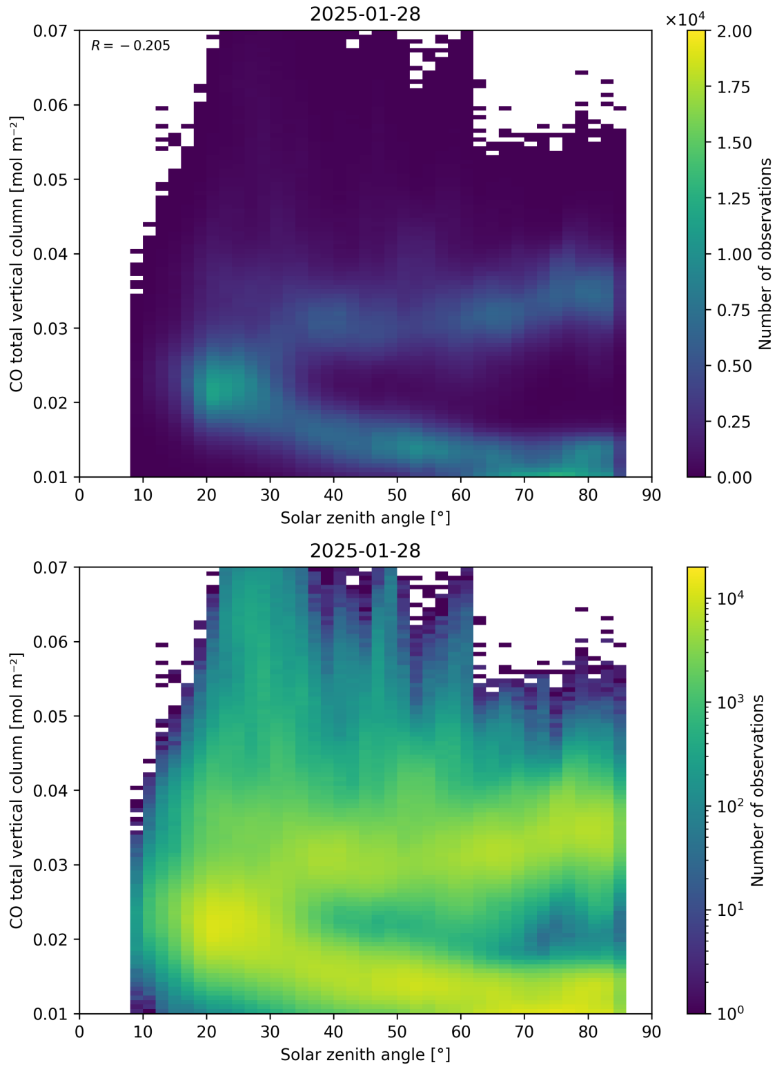
Figure 61: Scatter density plot of “Solar zenith angle” against “CO total vertical column” for 2025-01-28 to 2025-01-29.
