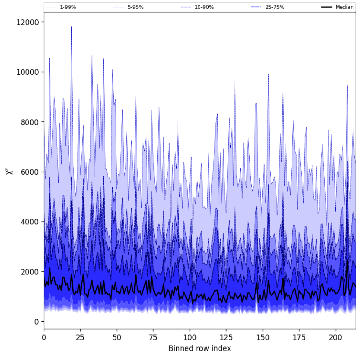
Figure 30: Along track statistics of “ \chi^2 ” for 2025-01-28 to 2025-01-29
