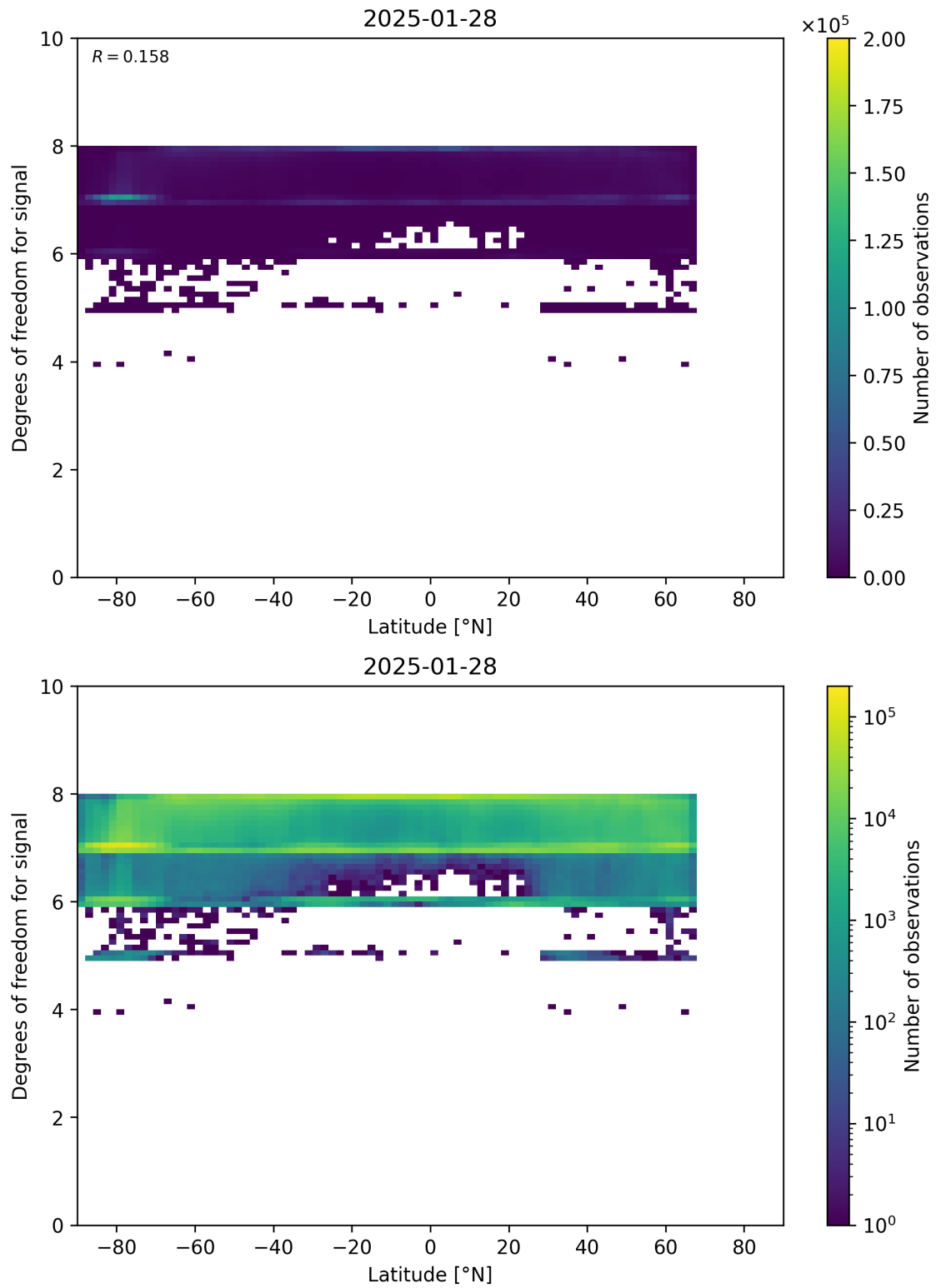
Figure 55: Scatter density plot of “Latitude” against “Degrees of freedom for signal” for 2025-01-28 to 2025-01-29.
