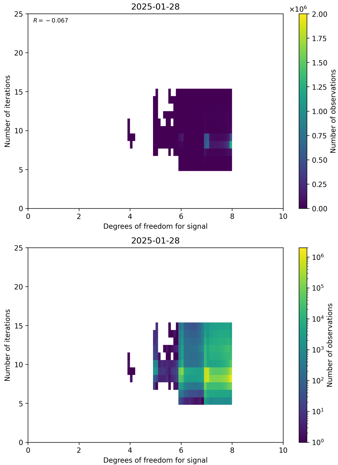
Figure 50: Scatter density plot of “Degrees of freedom for signal” against “Number of iterations” for 2025-01-28 to 2025-01-29.
