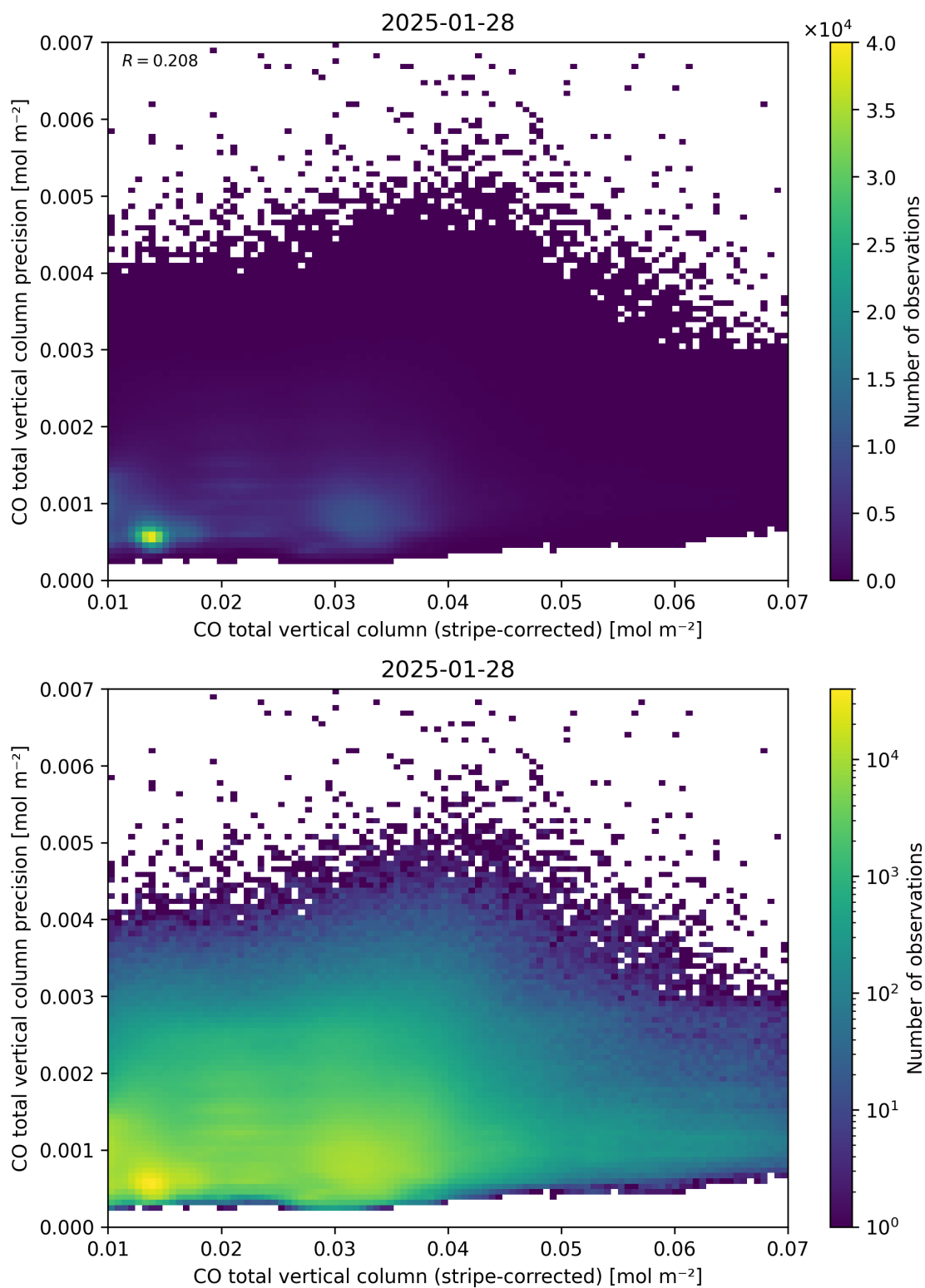
Figure 36: Scatter density plot of “CO total vertical column (stripe-corrected)” against “CO total vertical column precision” for 2025-01-28 to 2025-01-29.
