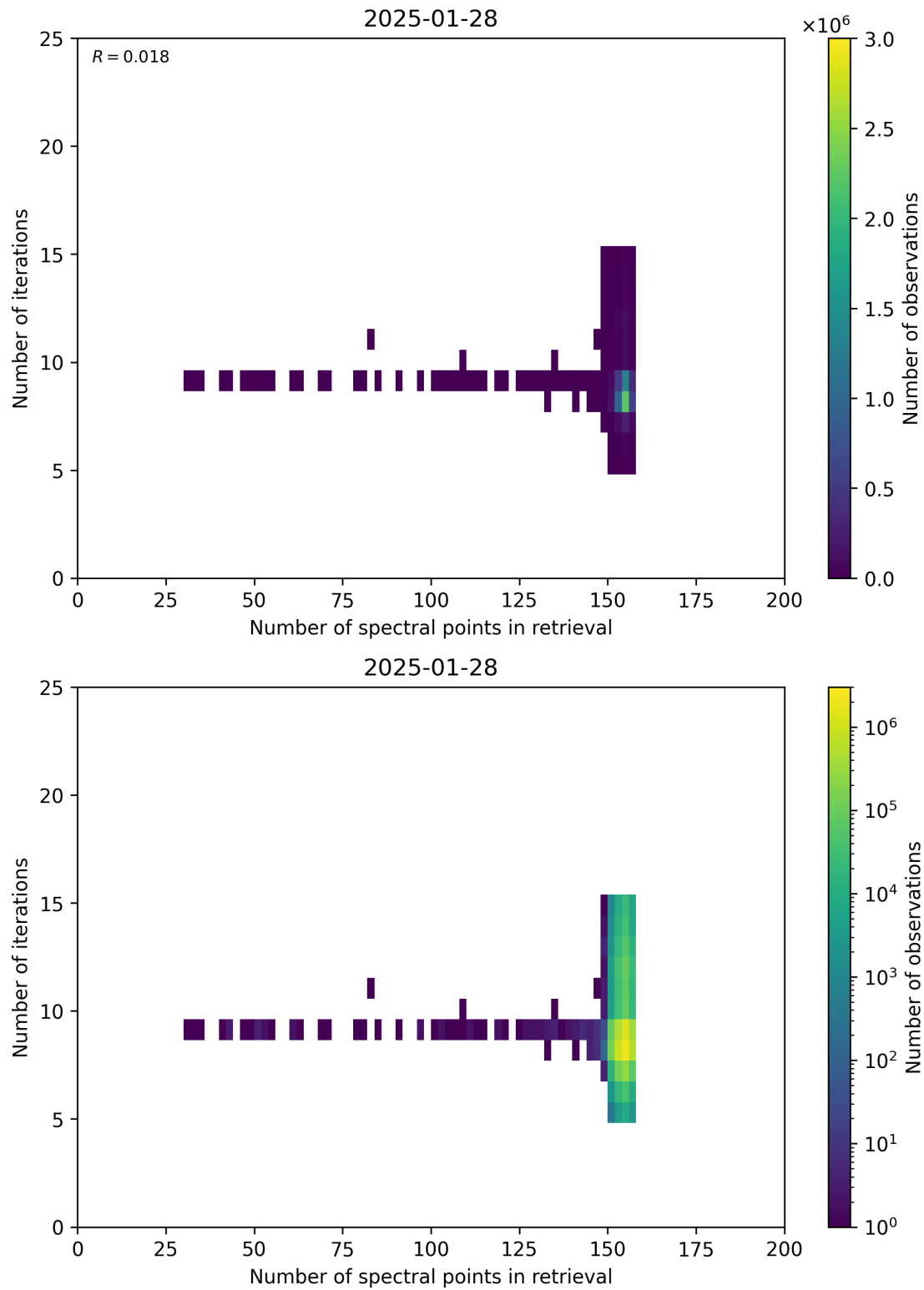
Figure 60: Scatter density plot of “Number of spectral points in retrieval” against “Number of iterations” for 2025-01-28 to 2025-01-29.
