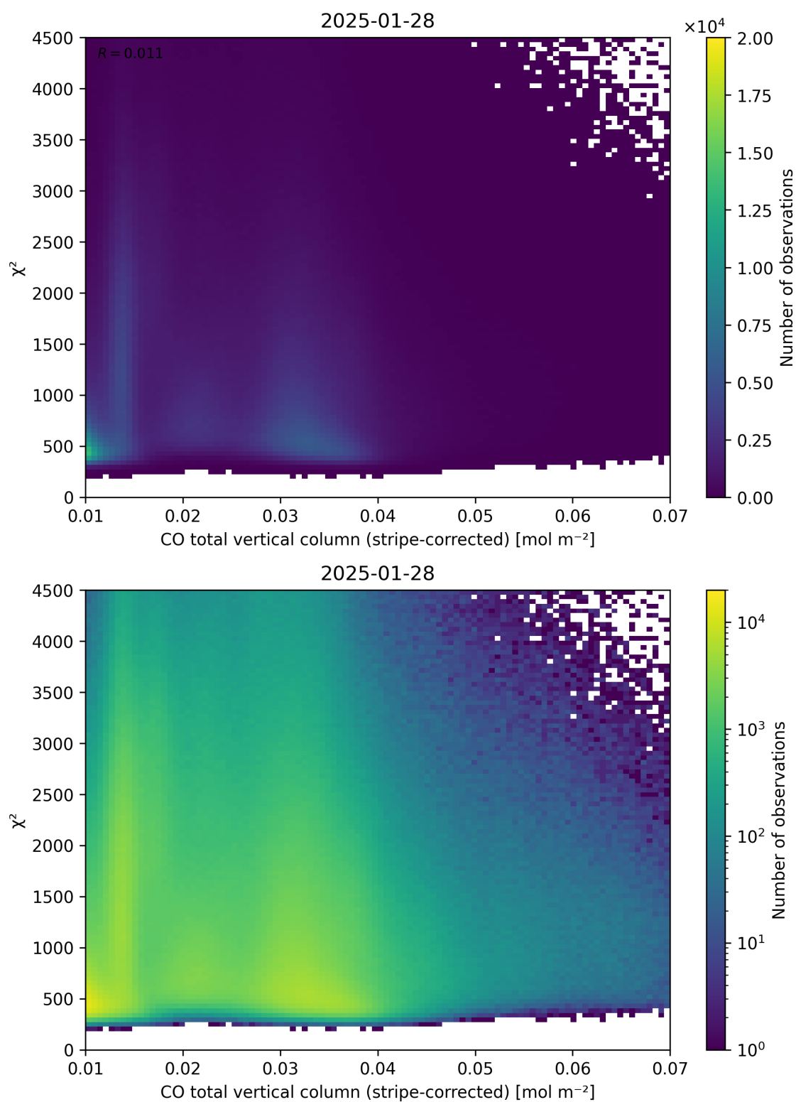
Figure 37: Scatter density plot of “CO total vertical column (stripe-corrected)” against “ \chi^2 ” for 2025-01-28 to 2025-01-29.
