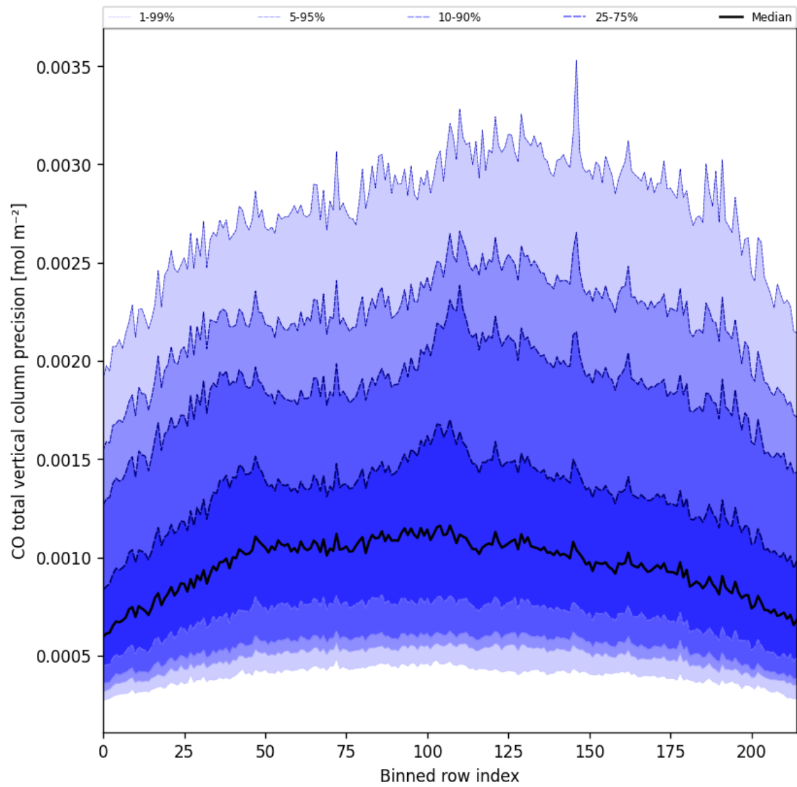
Figure 28: Along track statistics of “CO total vertical column precision” for 2025-01-28 to 2025-01-29
