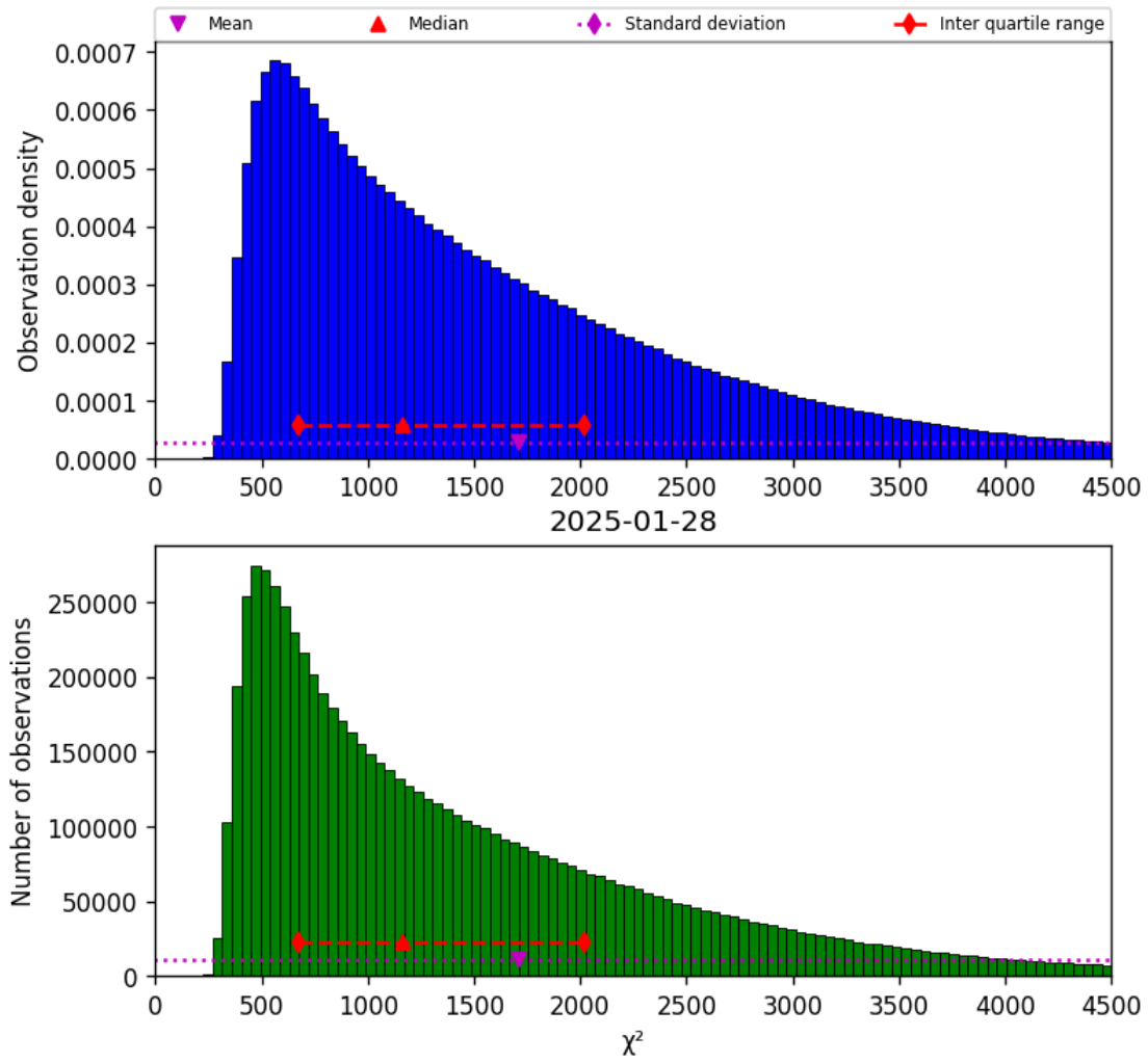
Figure 22: Histogram of “ \chi^2 ” for 2025-01-28 to 2025-01-29
