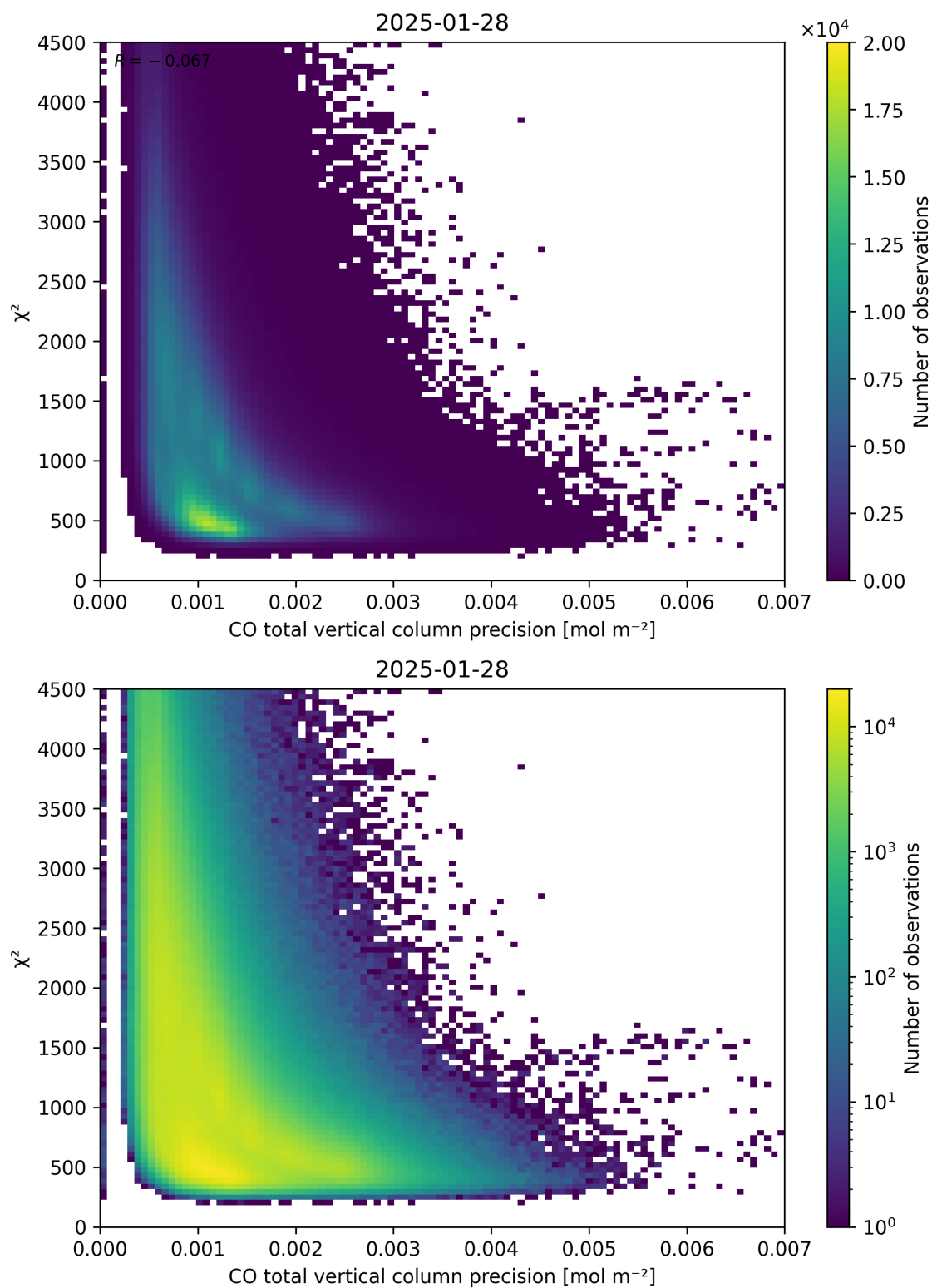
Figure 44: Scatter density plot of “CO total vertical column precision” against “ \chi^2 ” for 2025-01-28 to 2025-01-29.
