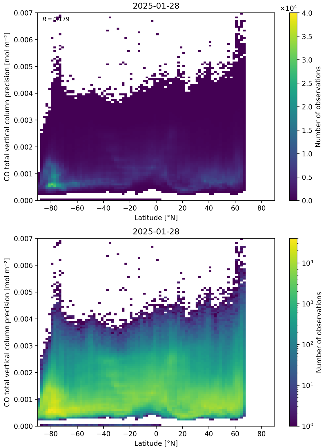
Figure 53: Scatter density plot of “Latitude” against “CO total vertical column precision” for 2025-01-28 to 2025-01-29.
