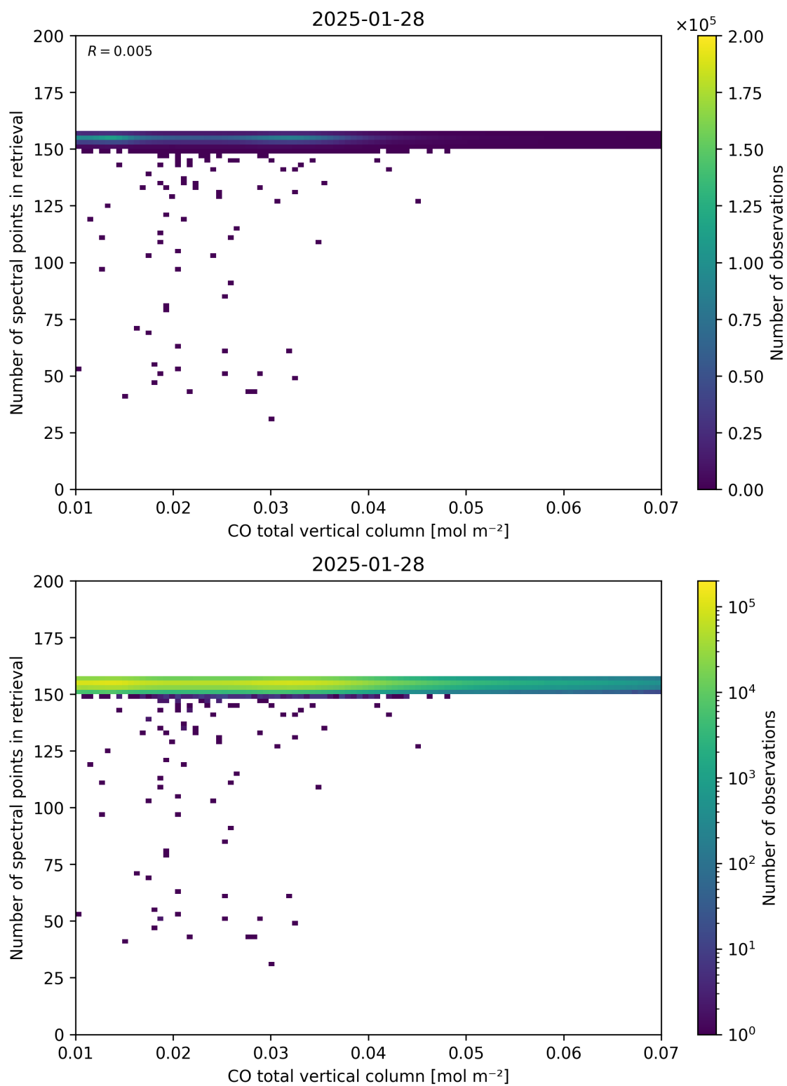
Figure 43: Scatter density plot of “CO total vertical column” against “Number of spectral points in retrieval” for 2025-01-28 to 2025-01-29.
