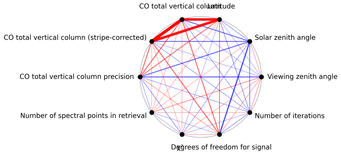
Figure 1: Map of correlation graph for 2025-01-28 to 2025-01-29.
