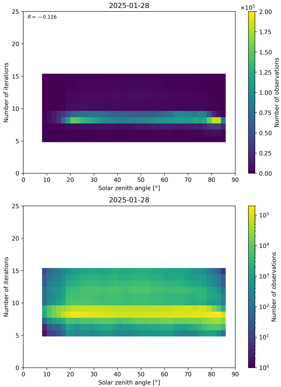
Figure 67: Scatter density plot of “Solar zenith angle” against “Number of iterations” for 2025-01-28 to 2025-01-29.
