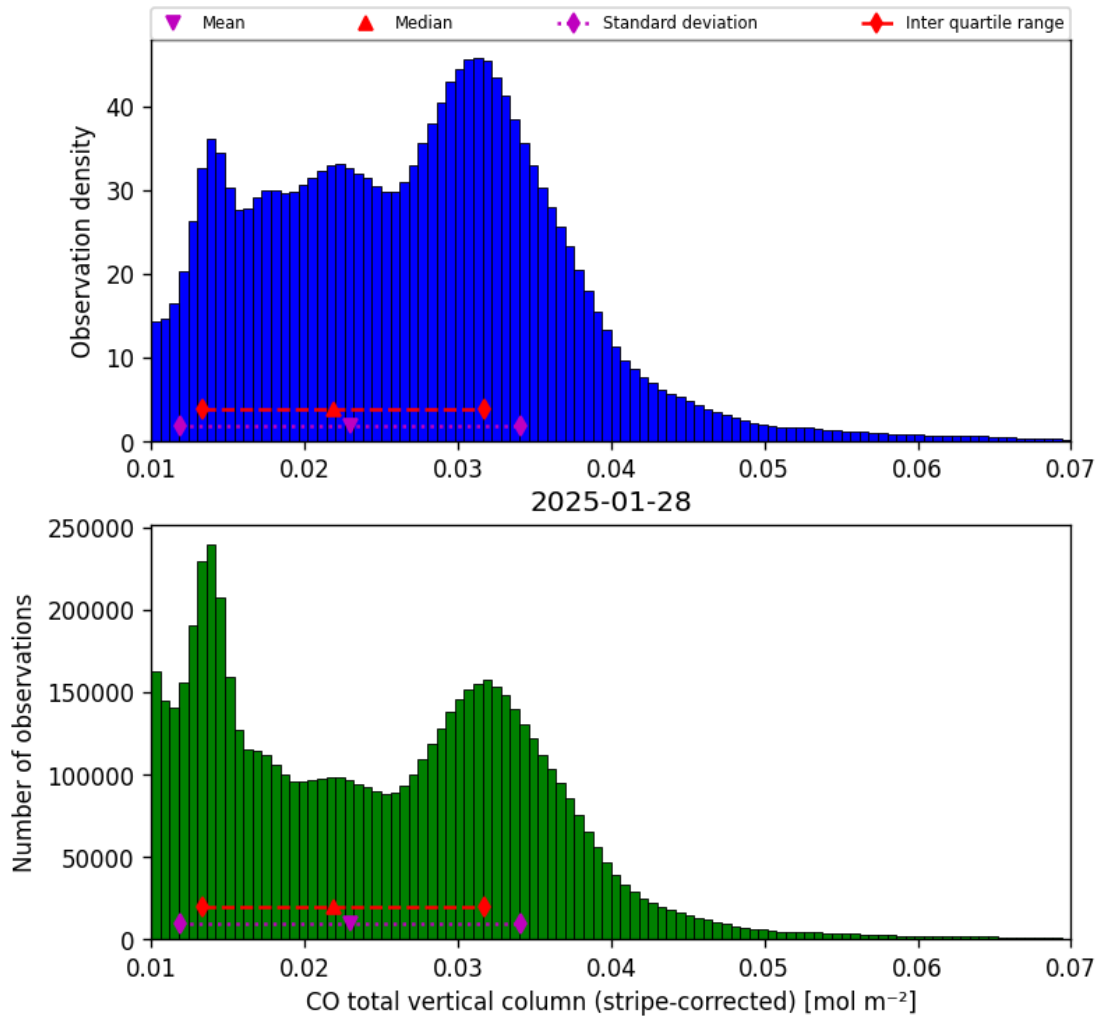
Figure 19: Histogram of “CO total vertical column (stripe-corrected)” for 2025-01-28 to 2025-01-29
