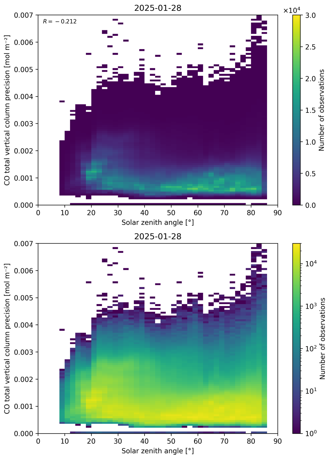
Figure 63: Scatter density plot of “Solar zenith angle” against “CO total vertical column precision” for 2025-01-28 to 2025-01-29.
