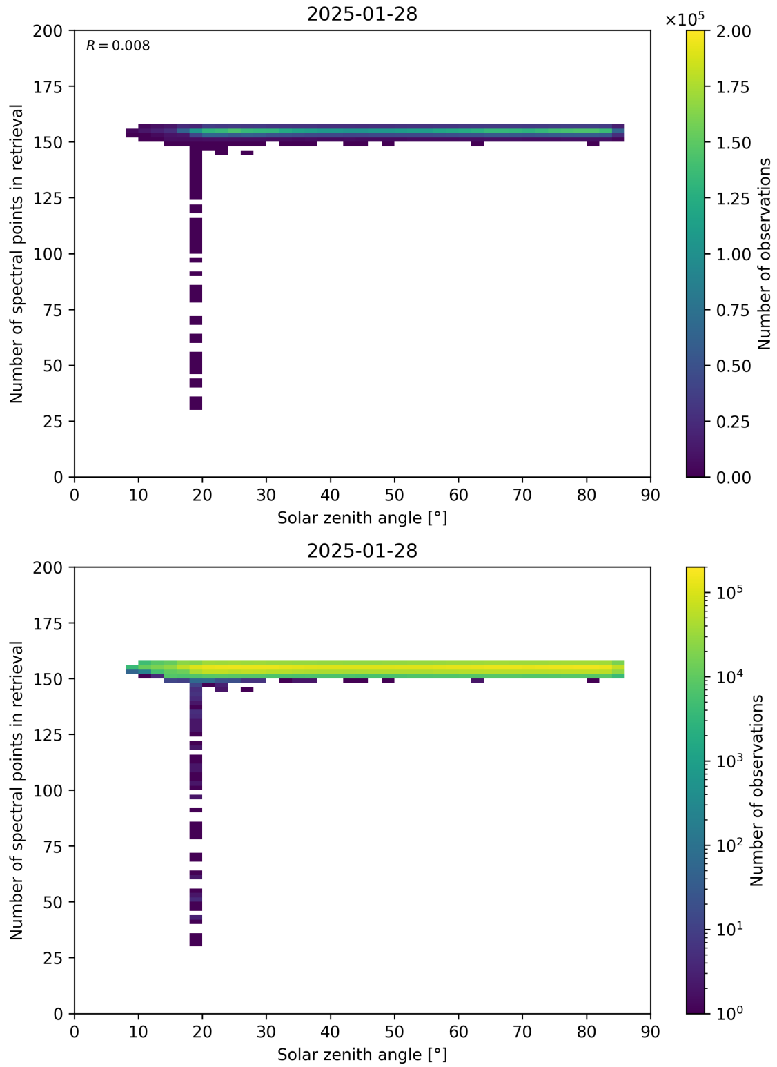
Figure 68: Scatter density plot of “Solar zenith angle” against “Number of spectral points in retrieval” for 2025-01-28 to 2025-01-29.
