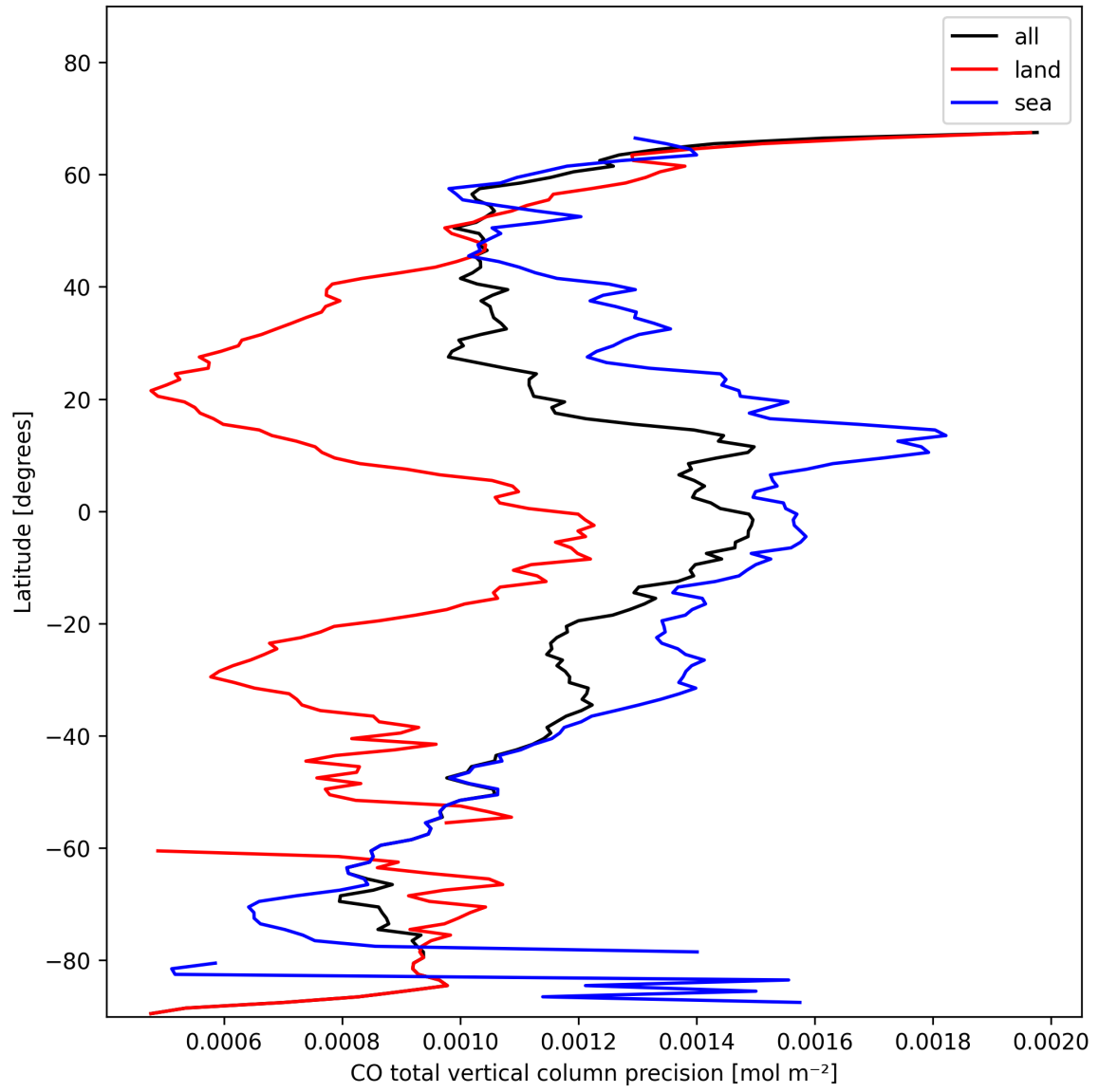
Figure 12: Zonal average of “CO total vertical column precision” for 2025-01-28 to 2025-01-29.
