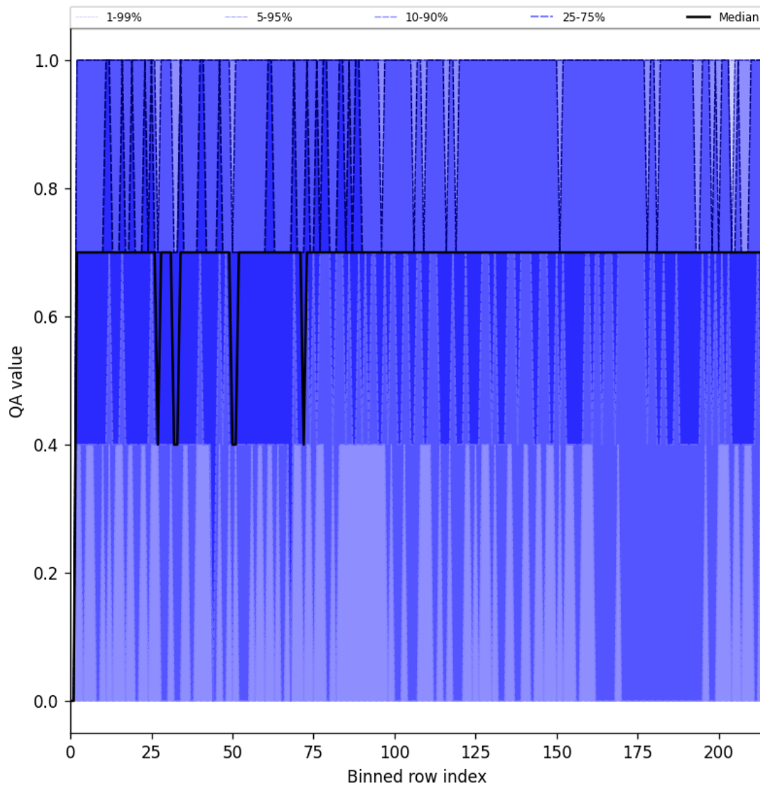
Figure 25: Along track statistics of “QA value” for 2025-01-28 to 2025-01-29
