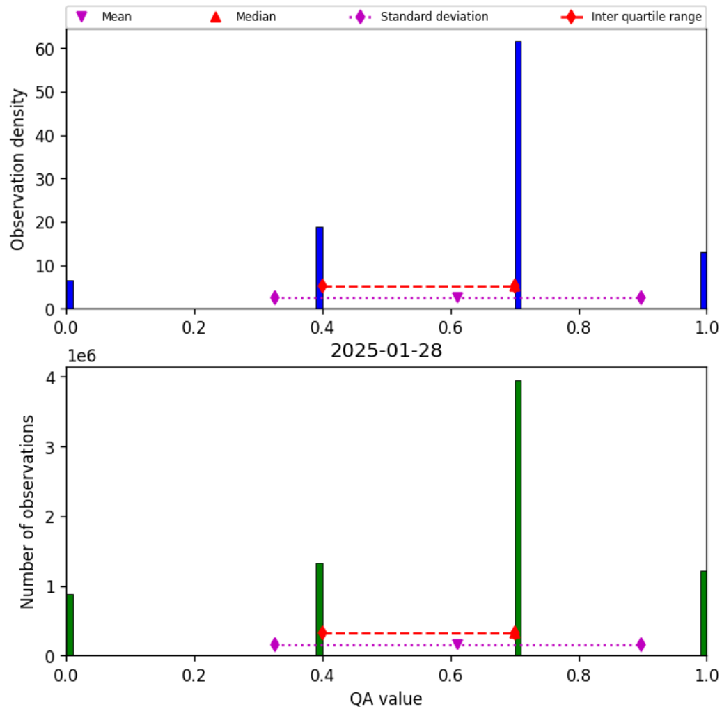
Figure 17: Histogram of “QA value” for 2025-01-28 to 2025-01-29
