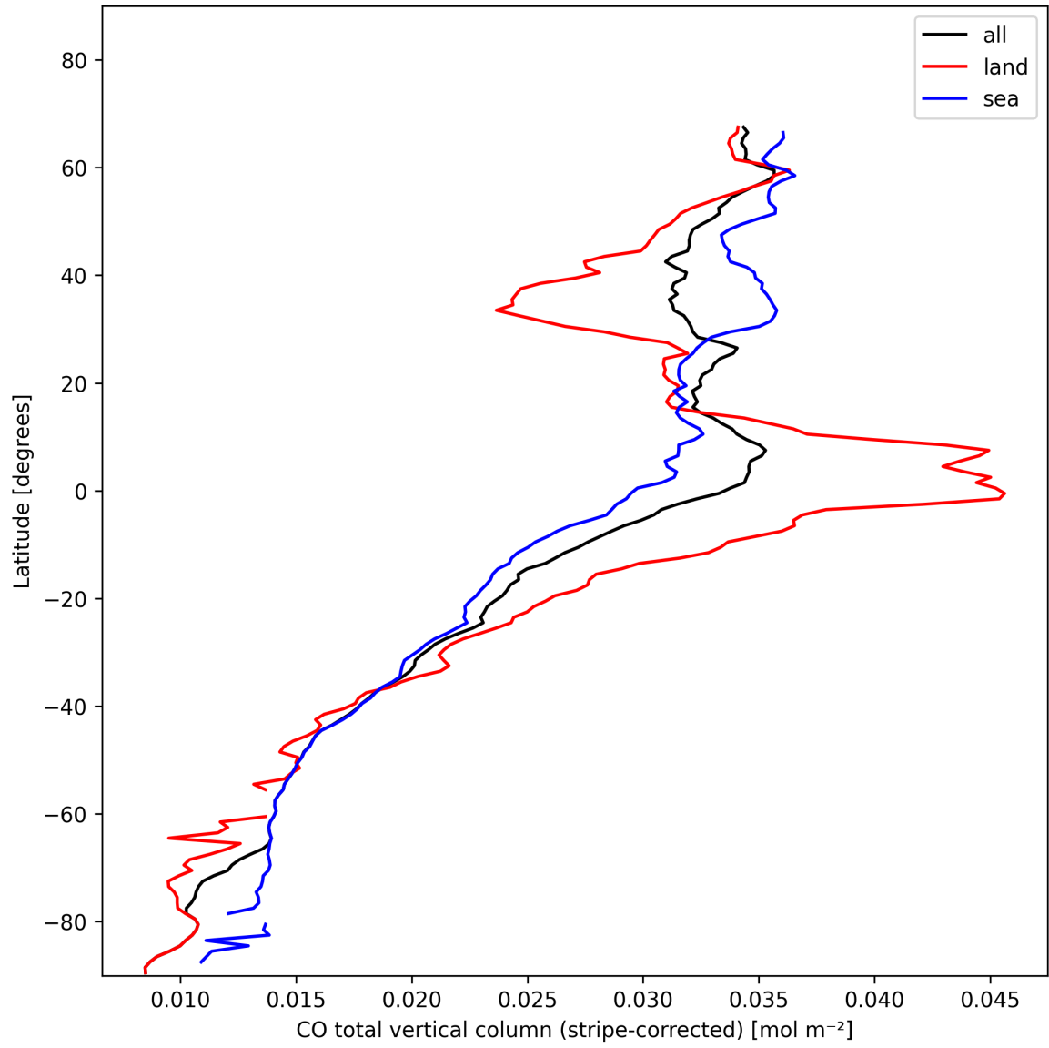
Figure 11: Zonal average of “CO total vertical column (stripe-corrected)” for 2025-01-28 to 2025-01-29.
