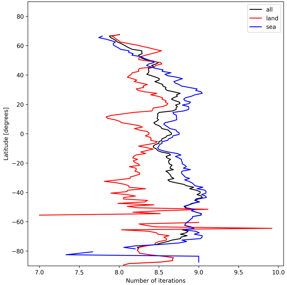
Figure 16: Zonal average of “Number of iterations” for 2025-01-28 to 2025-01-29.
