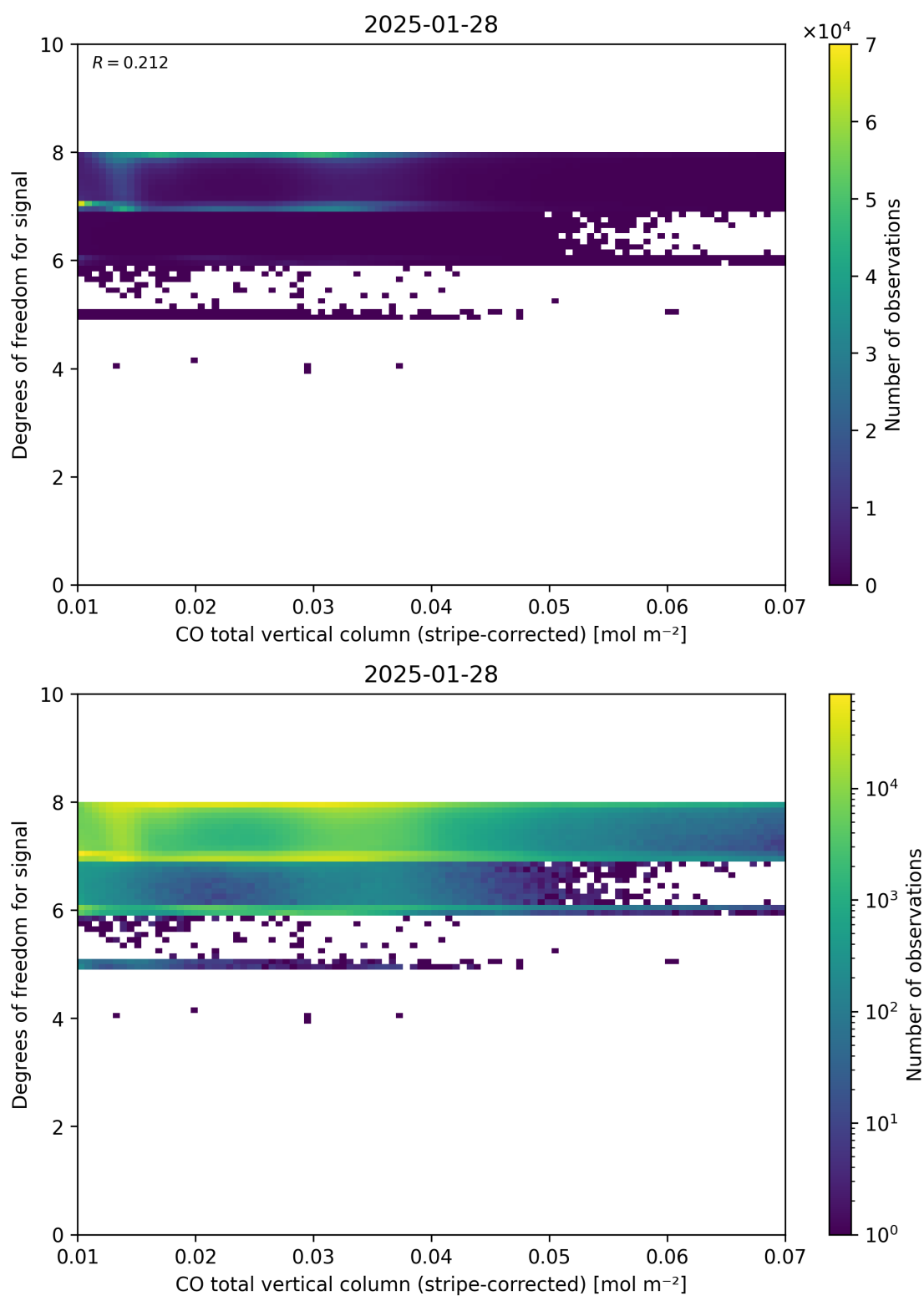
Figure 38: Scatter density plot of “CO total vertical column (stripe-corrected)” against “Degrees of freedom for signal” for 2025-01-28 to 2025-01-29.
