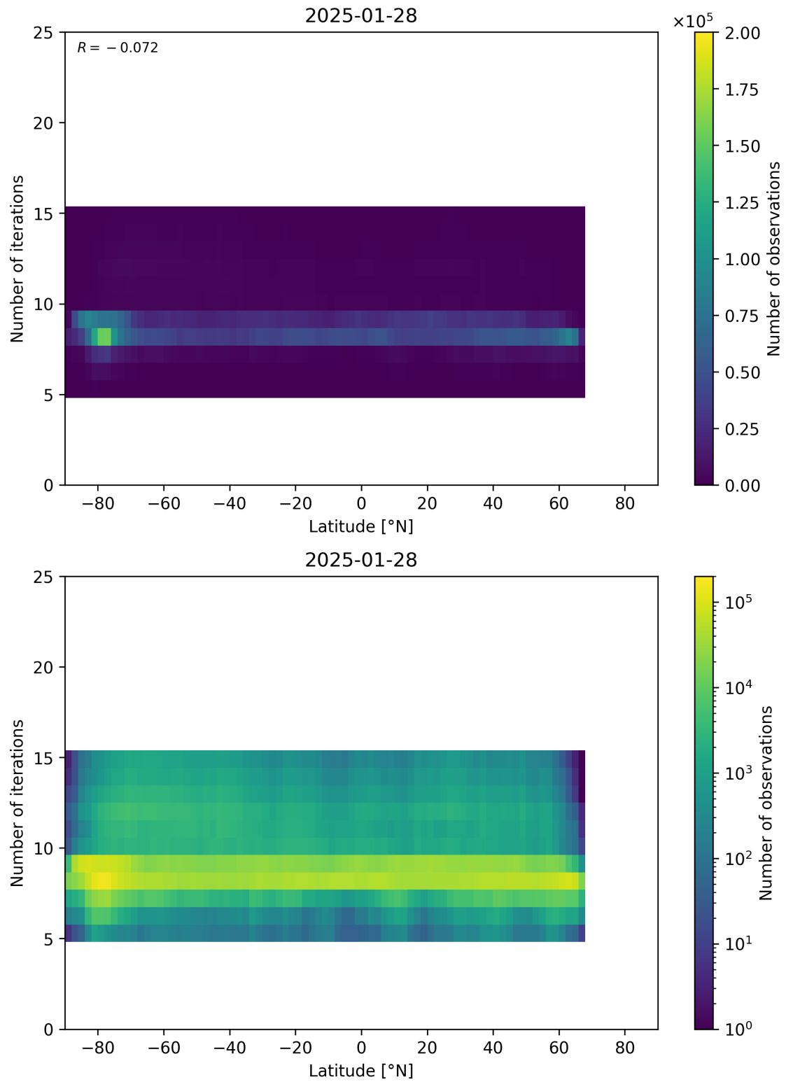
Figure 56: Scatter density plot of “Latitude” against “Number of iterations” for 2025-01-28 to 2025-01-29.
