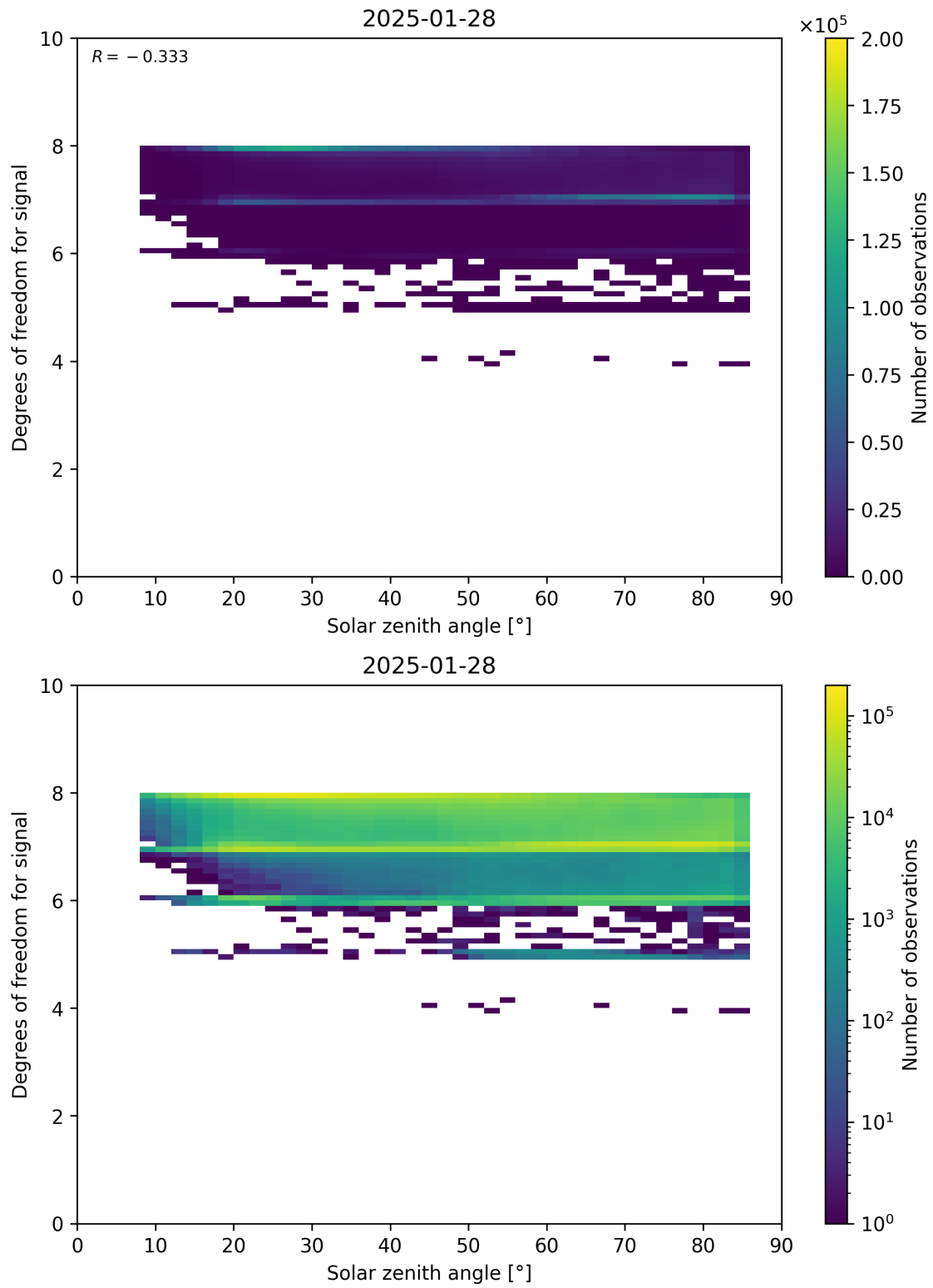
Figure 65: Scatter density plot of “Solar zenith angle” against “Degrees of freedom for signal” for 2025-01-28 to 2025-01-29.
