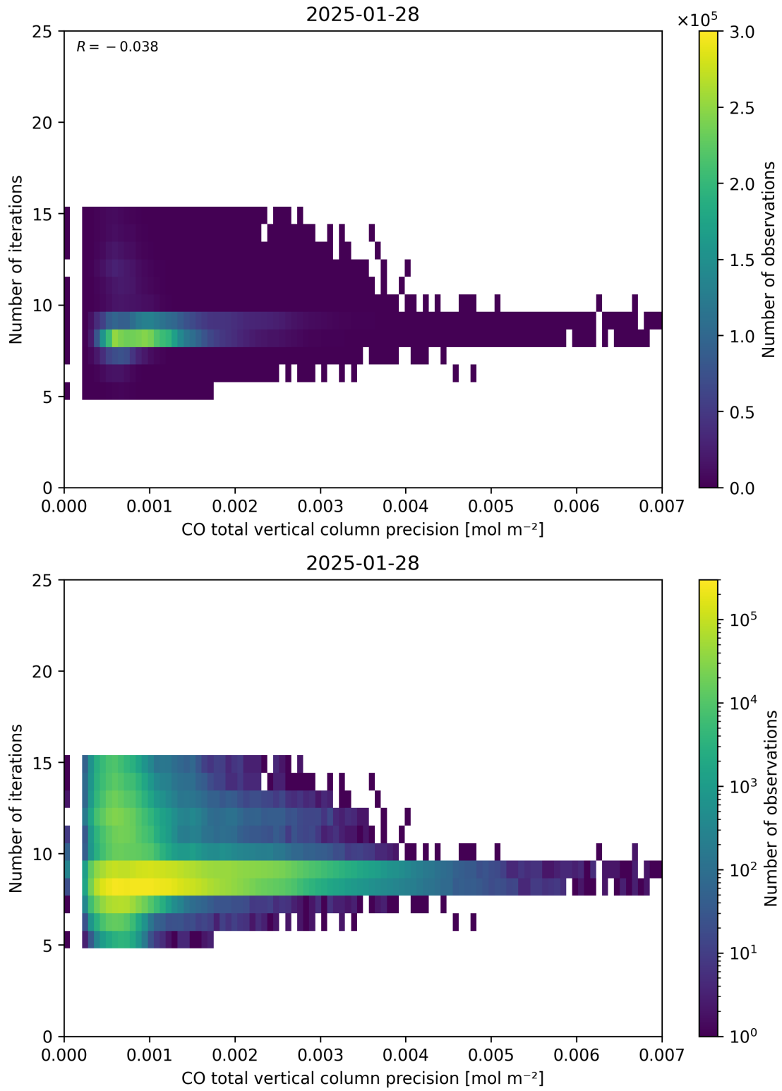
Figure 46: Scatter density plot of “CO total vertical column precision” against “Number of iterations” for 2025-01-28 to 2025-01-29.
