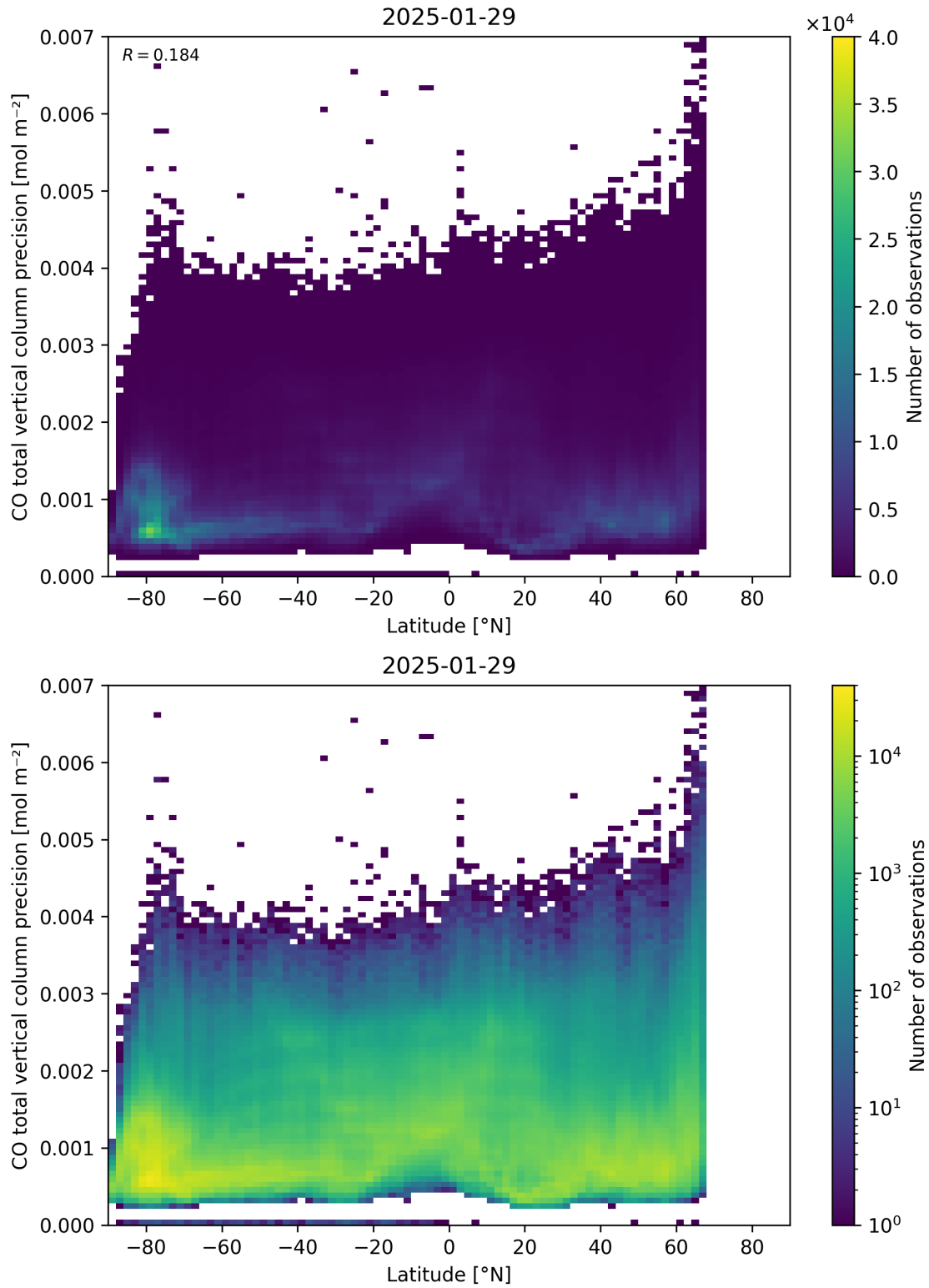
Figure 53: Scatter density plot of “Latitude” against “CO total vertical column precision” for 2025-01-28 to 2025-01-30.
