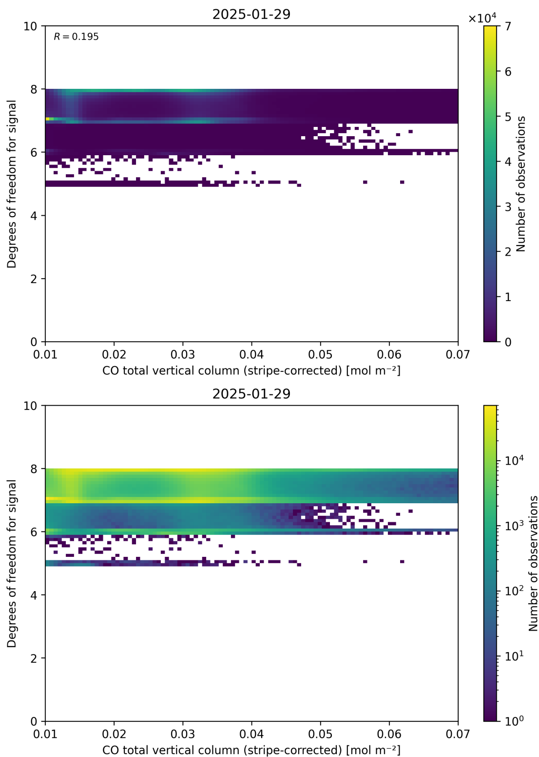
Figure 38: Scatter density plot of “CO total vertical column (stripe-corrected)” against “Degrees of freedom for signal” for 2025-01-28 to 2025-01-30.
