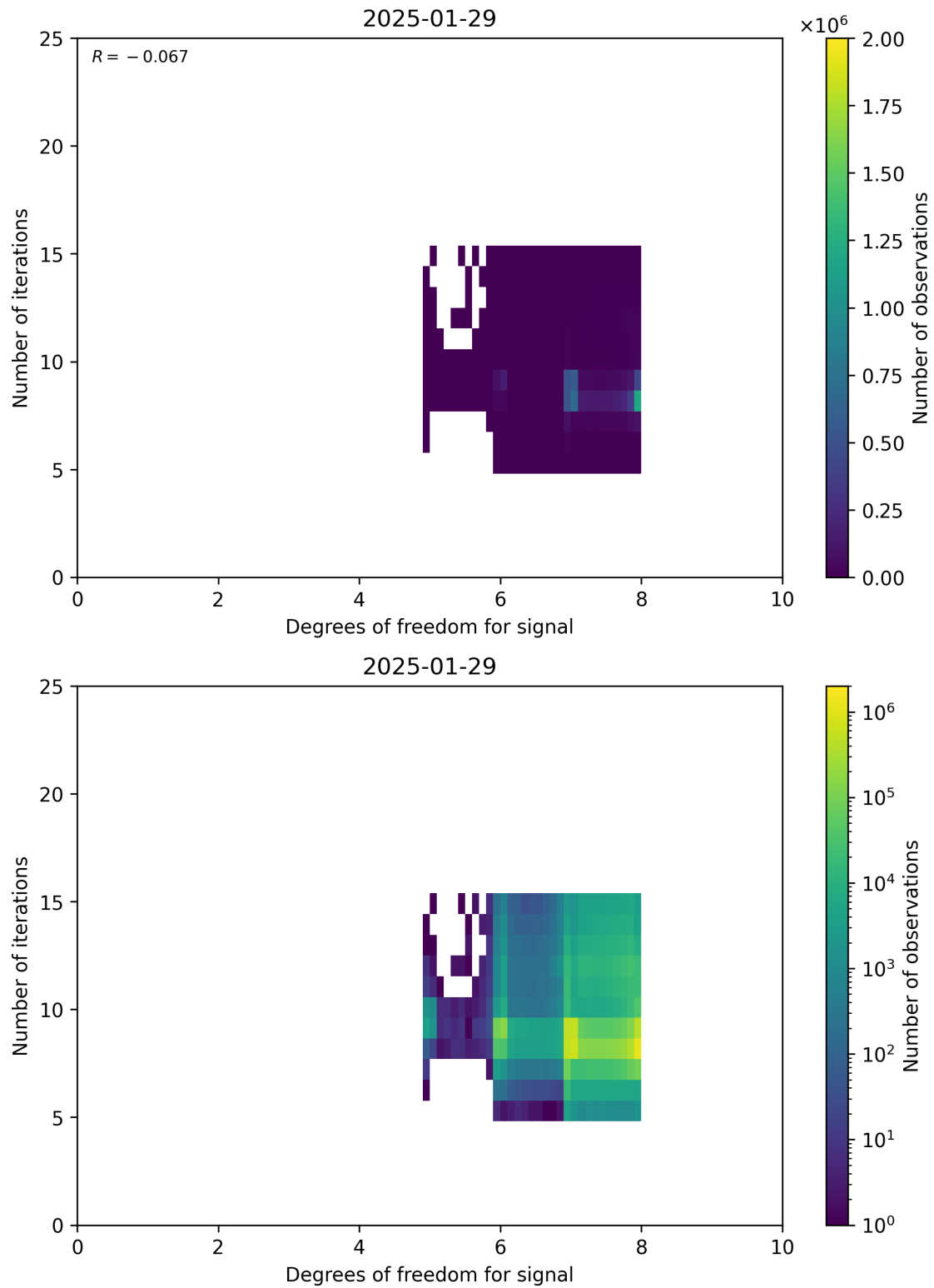
Figure 50: Scatter density plot of “Degrees of freedom for signal” against “Number of iterations” for 2025-01-28 to 2025-01-30.
