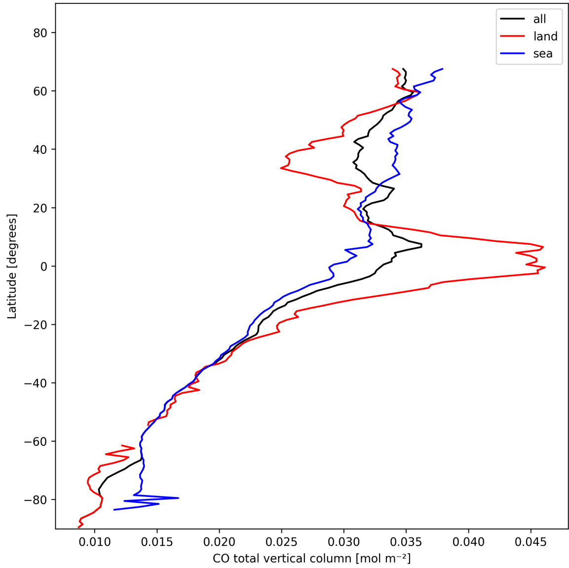
Figure 10: Zonal average of “CO total vertical column” for 2025-01-28 to 2025-01-30.
