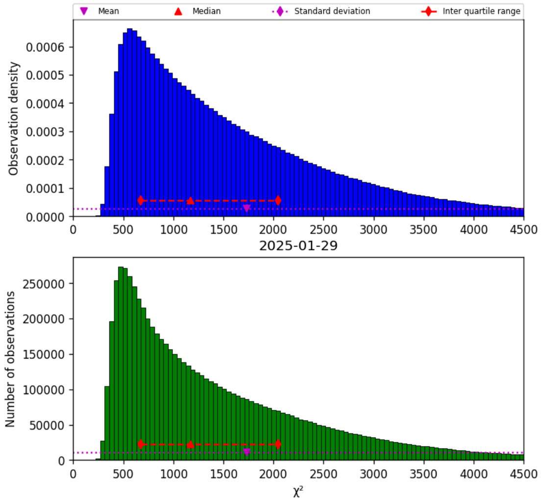
Figure 22: Histogram of “ \chi^2 ” for 2025-01-28 to 2025-01-30
