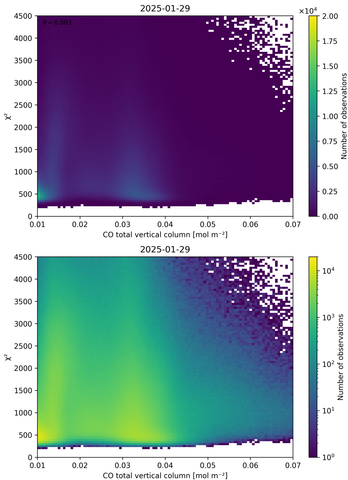
Figure 35: Scatter density plot of “CO total vertical column” against “ \chi^2 ” for 2025-01-28 to 2025-01-30.
