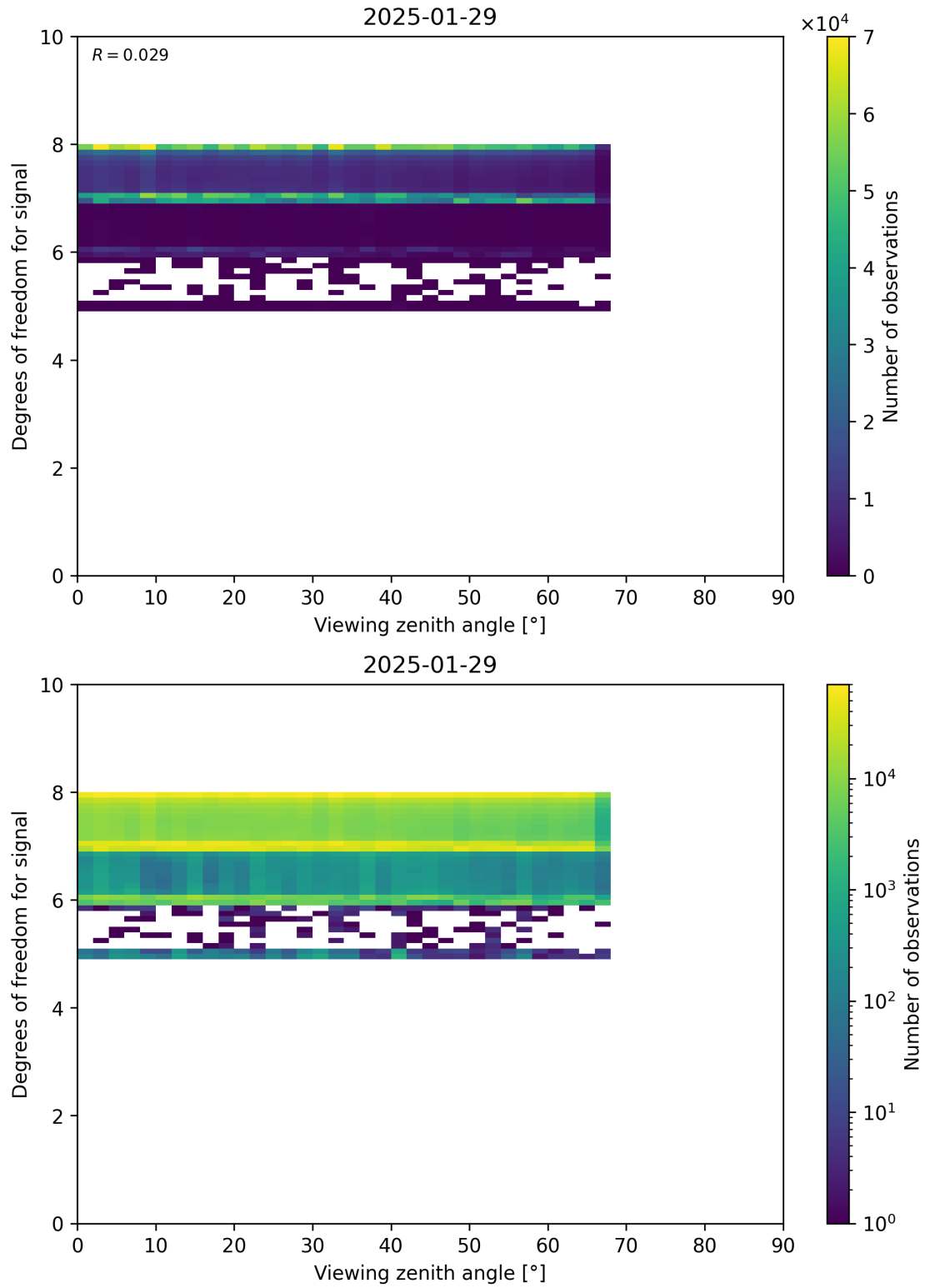
Figure 73: Scatter density plot of “Viewing zenith angle” against “Degrees of freedom for signal” for 2025-01-28 to 2025-01-30.
