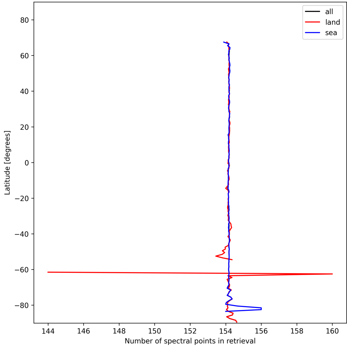
Figure 13: Zonal average of “Number of spectral points in retrieval” for 2025-01-28 to 2025-01-30.
