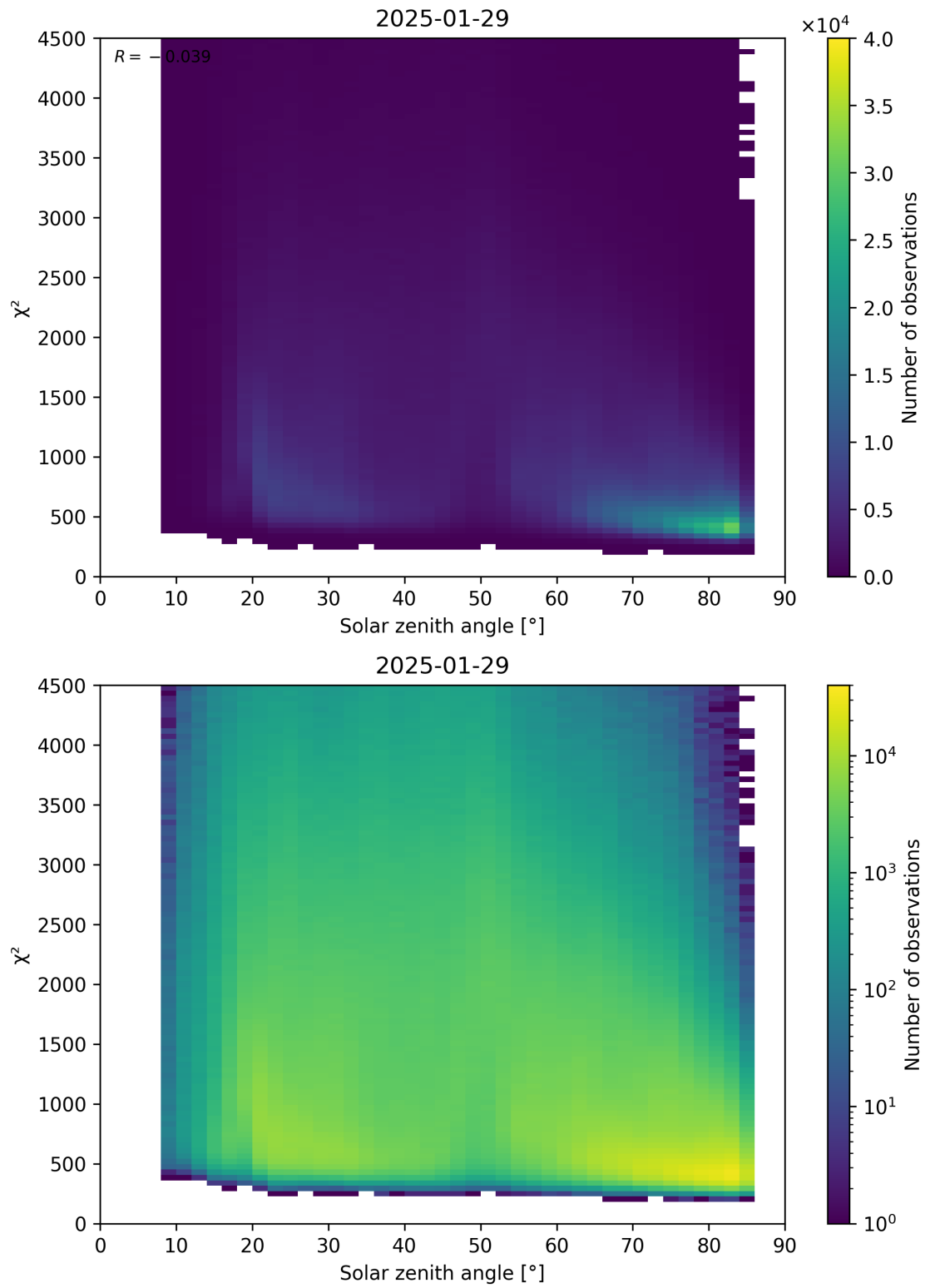
Figure 64: Scatter density plot of “Solar zenith angle” against “ \chi^2 ” for 2025-01-28 to 2025-01-30.
