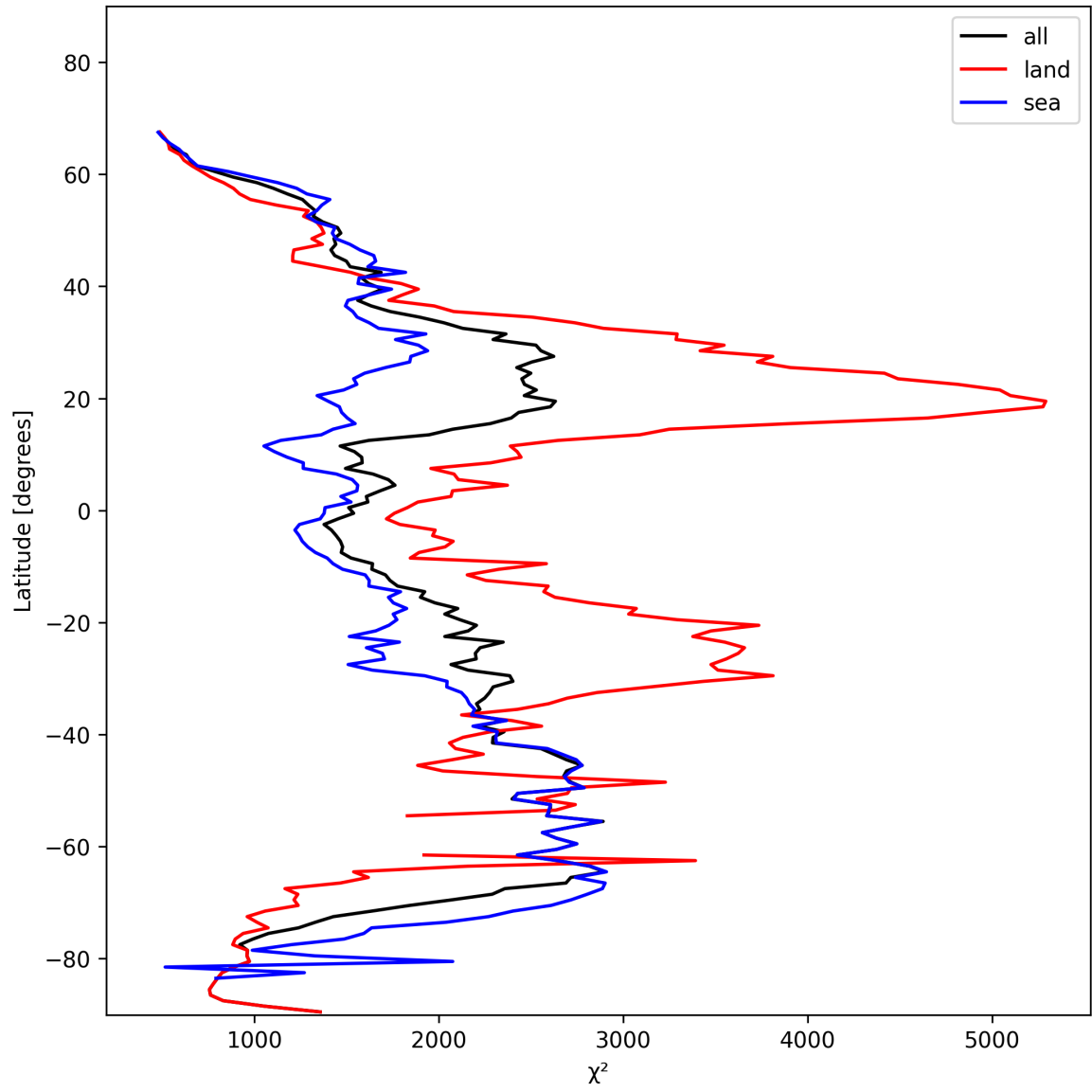
Figure 14: Zonal average of “ \chi^2 ” for 2025-01-28 to 2025-01-30.
