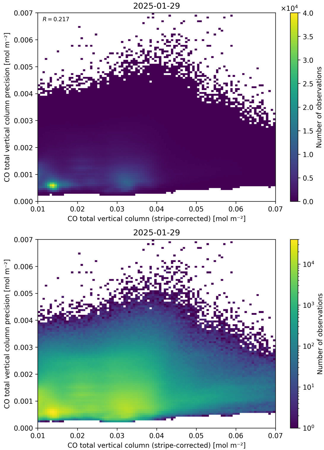
Figure 36: Scatter density plot of “CO total vertical column (stripe-corrected)” against “CO total vertical column precision” for 2025-01-28 to 2025-01-30.
