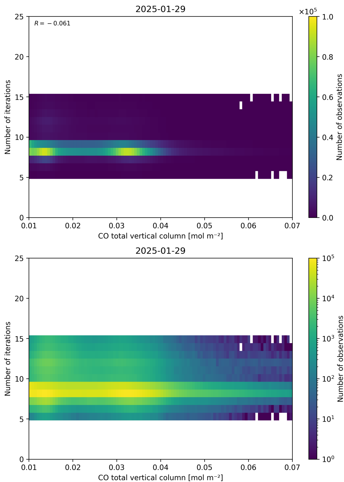
Figure 42: Scatter density plot of “CO total vertical column” against “Number of iterations” for 2025-01-28 to 2025-01-30.
