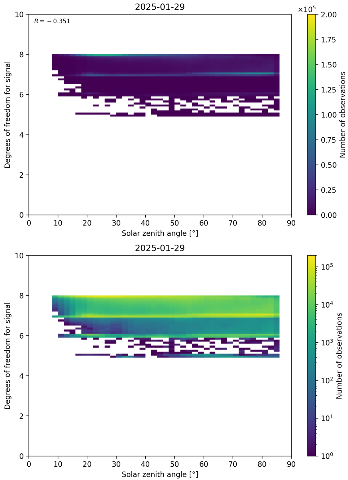
Figure 65: Scatter density plot of “Solar zenith angle” against “Degrees of freedom for signal” for 2025-01-28 to 2025-01-30.
