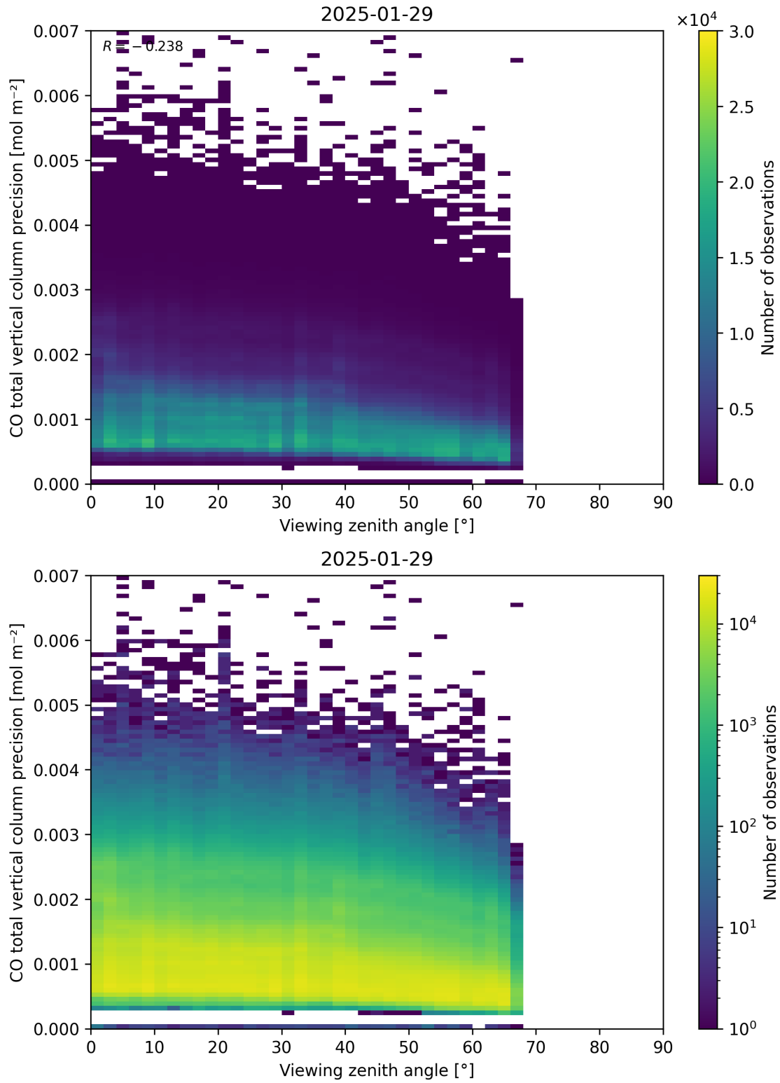
Figure 71: Scatter density plot of “Viewing zenith angle” against “CO total vertical column precision” for 2025-01-28 to 2025-01-30.
