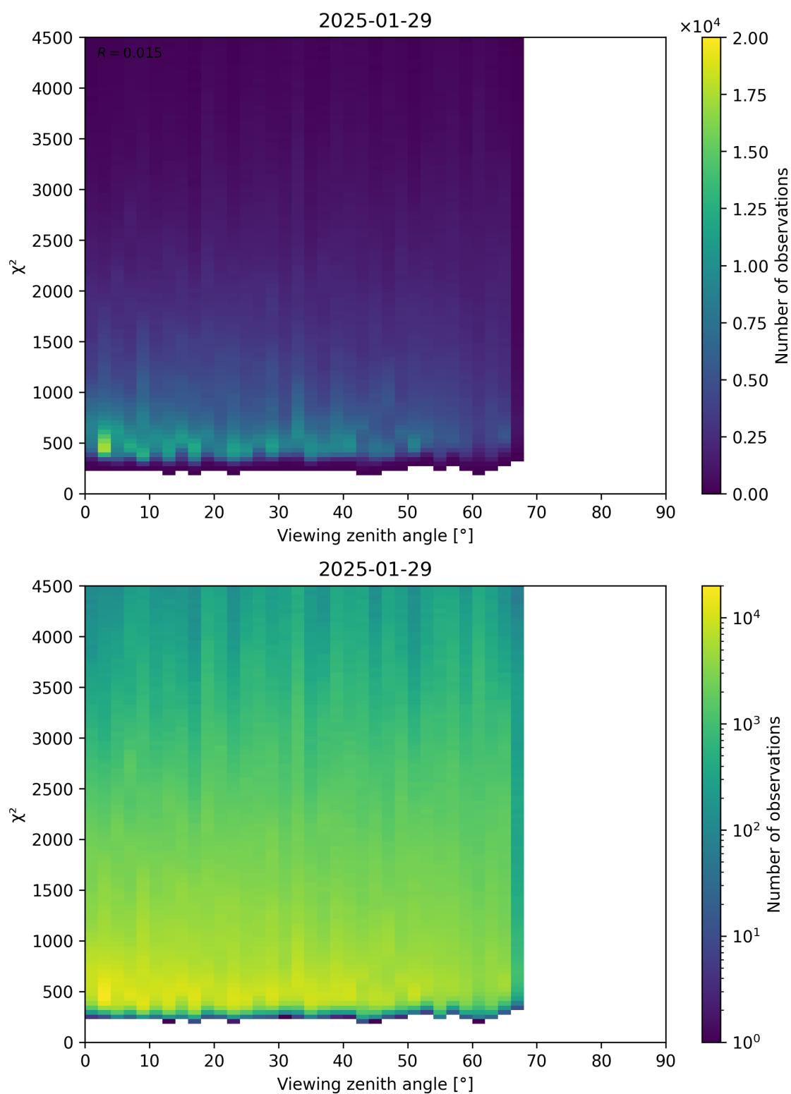
Figure 72: Scatter density plot of “Viewing zenith angle” against “ \chi^2 ” for 2025-01-28 to 2025-01-30.
