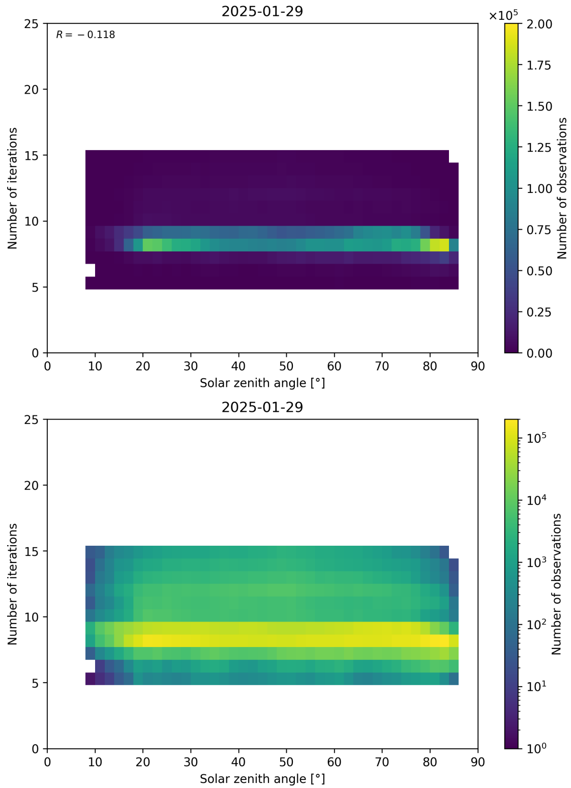
Figure 67: Scatter density plot of “Solar zenith angle” against “Number of iterations” for 2025-01-28 to 2025-01-30.
