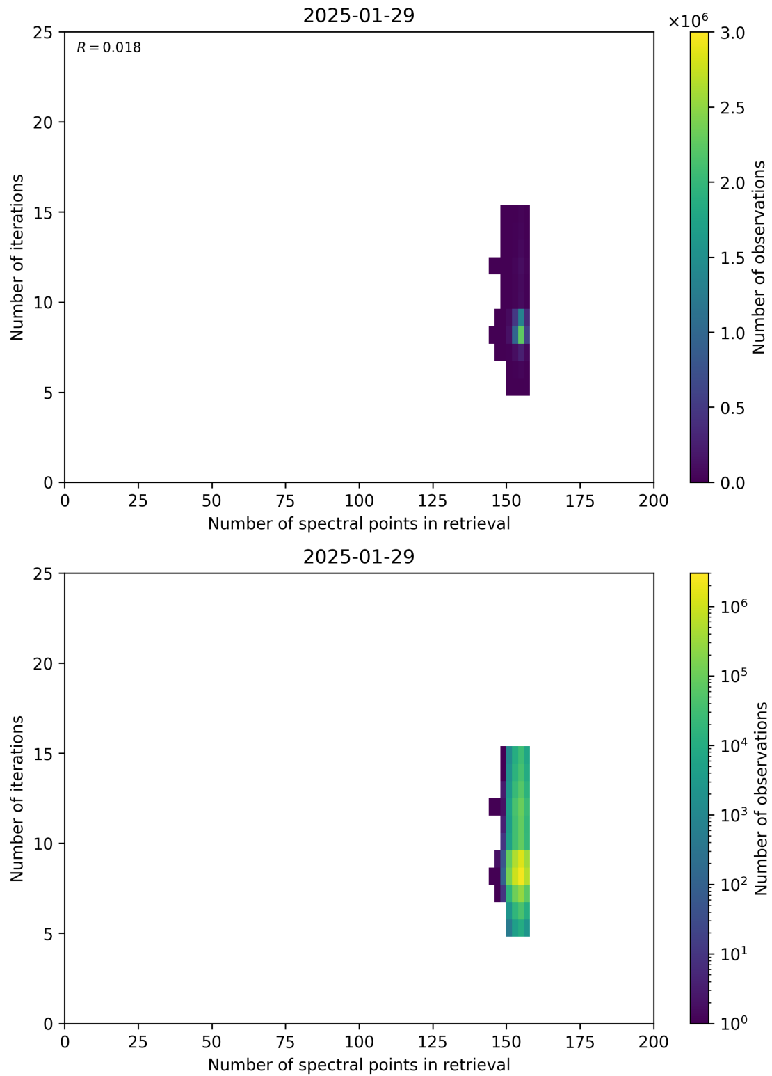
Figure 60: Scatter density plot of “Number of spectral points in retrieval” against “Number of iterations” for 2025-01-28 to 2025-01-30.
