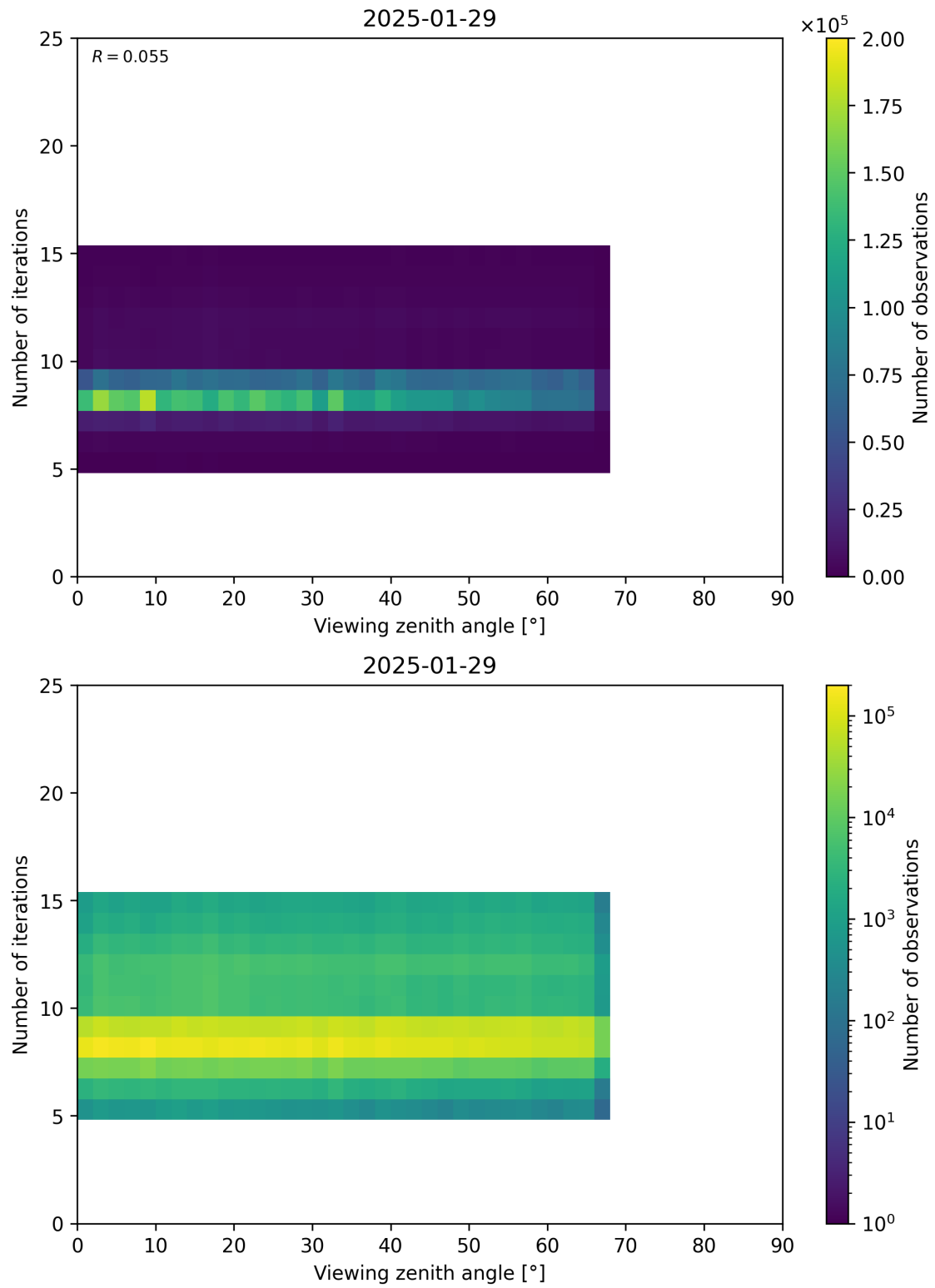
Figure 75: Scatter density plot of “Viewing zenith angle” against “Number of iterations” for 2025-01-28 to 2025-01-30.
