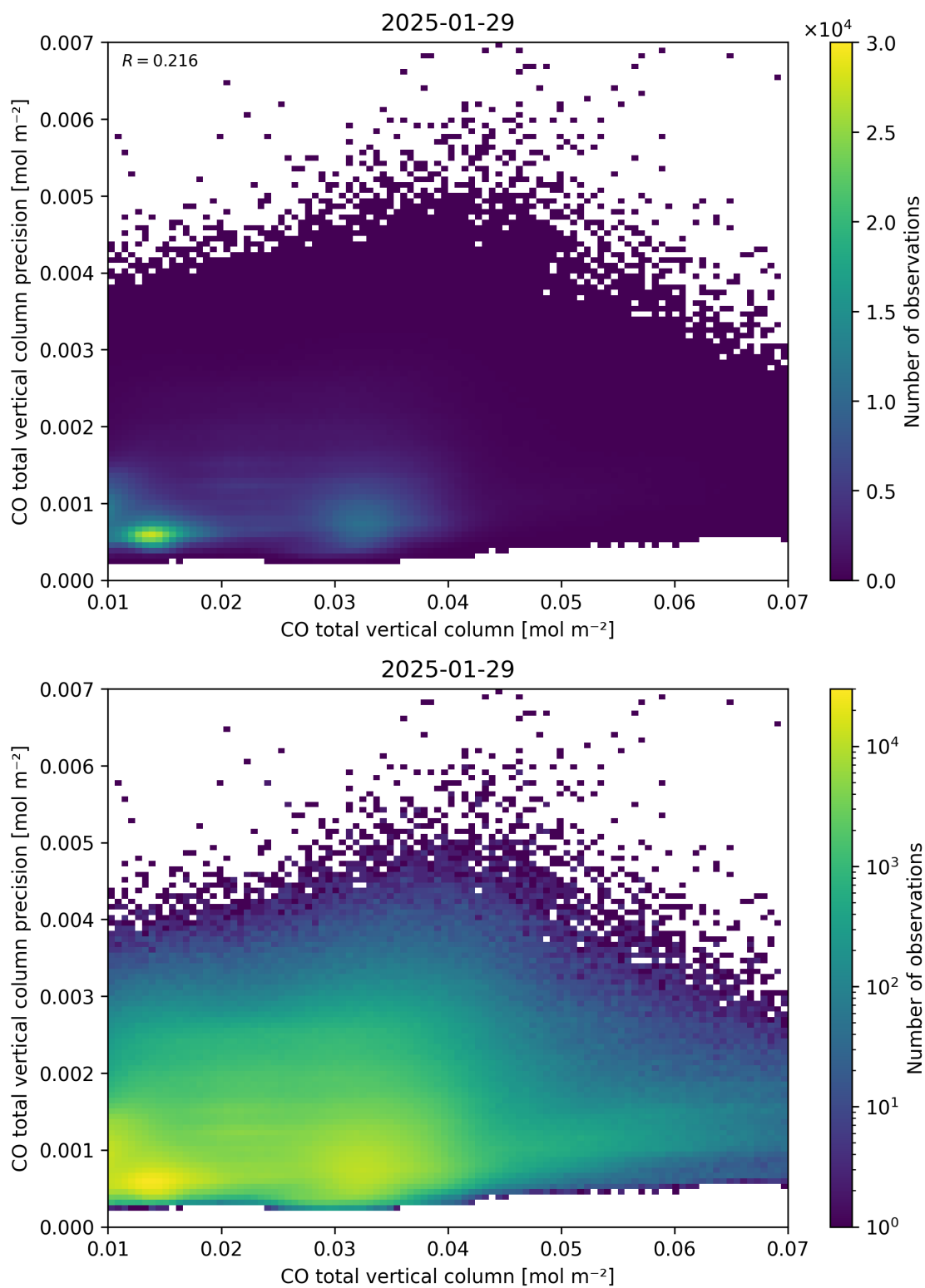
Figure 34: Scatter density plot of “CO total vertical column” against “CO total vertical column precision” for 2025-01-28 to 2025-01-30.
