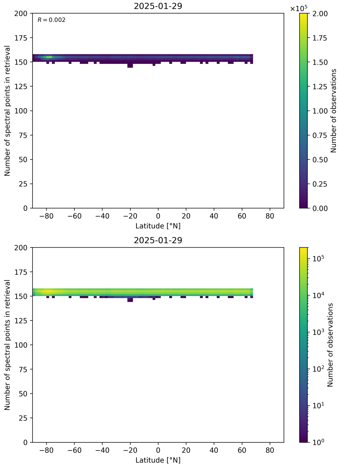
Figure 57: Scatter density plot of “Latitude” against “Number of spectral points in retrieval” for 2025-01-28 to 2025-01-30.
