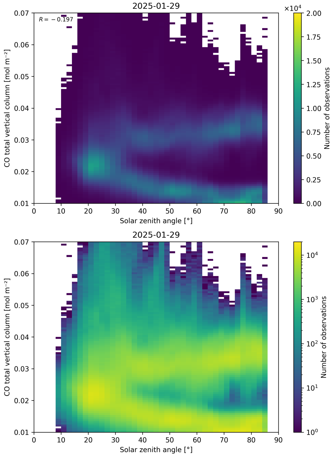
Figure 61: Scatter density plot of “Solar zenith angle” against “CO total vertical column” for 2025-01-28 to 2025-01-30.
