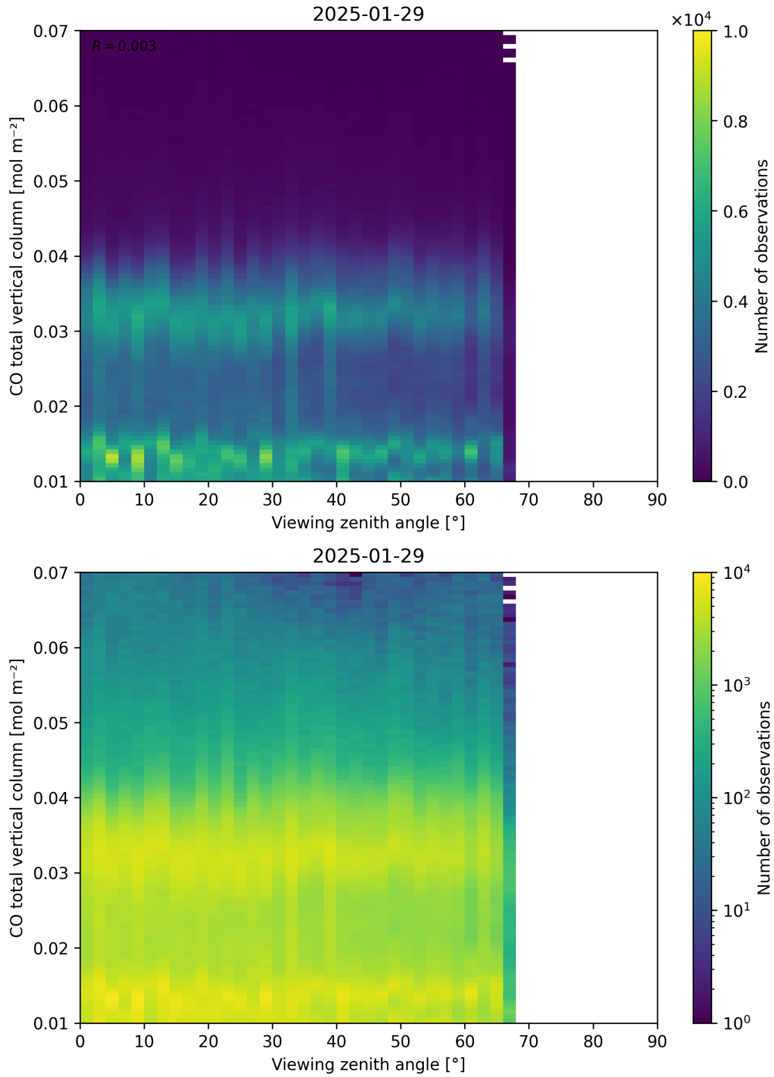
Figure 69: Scatter density plot of “Viewing zenith angle” against “CO total vertical column” for 2025-01-28 to 2025-01-30.
