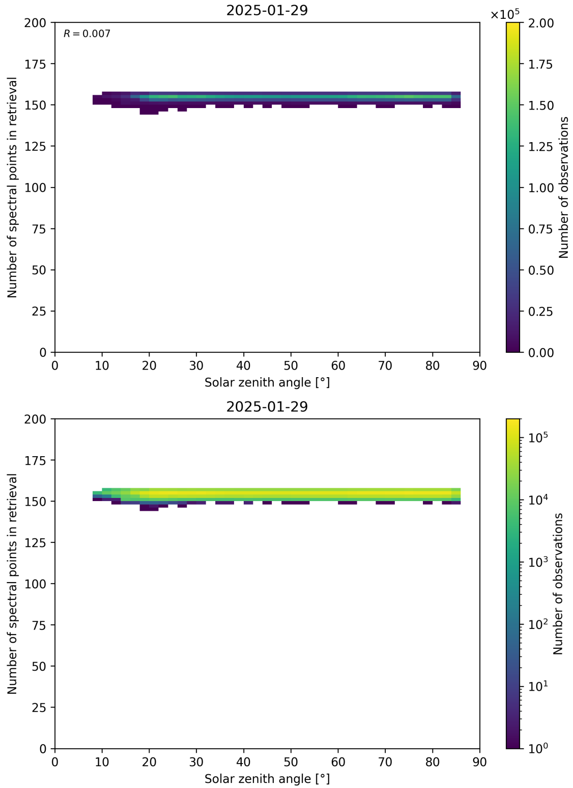
Figure 68: Scatter density plot of “Solar zenith angle” against “Number of spectral points in retrieval” for 2025-01-28 to 2025-01-30.
