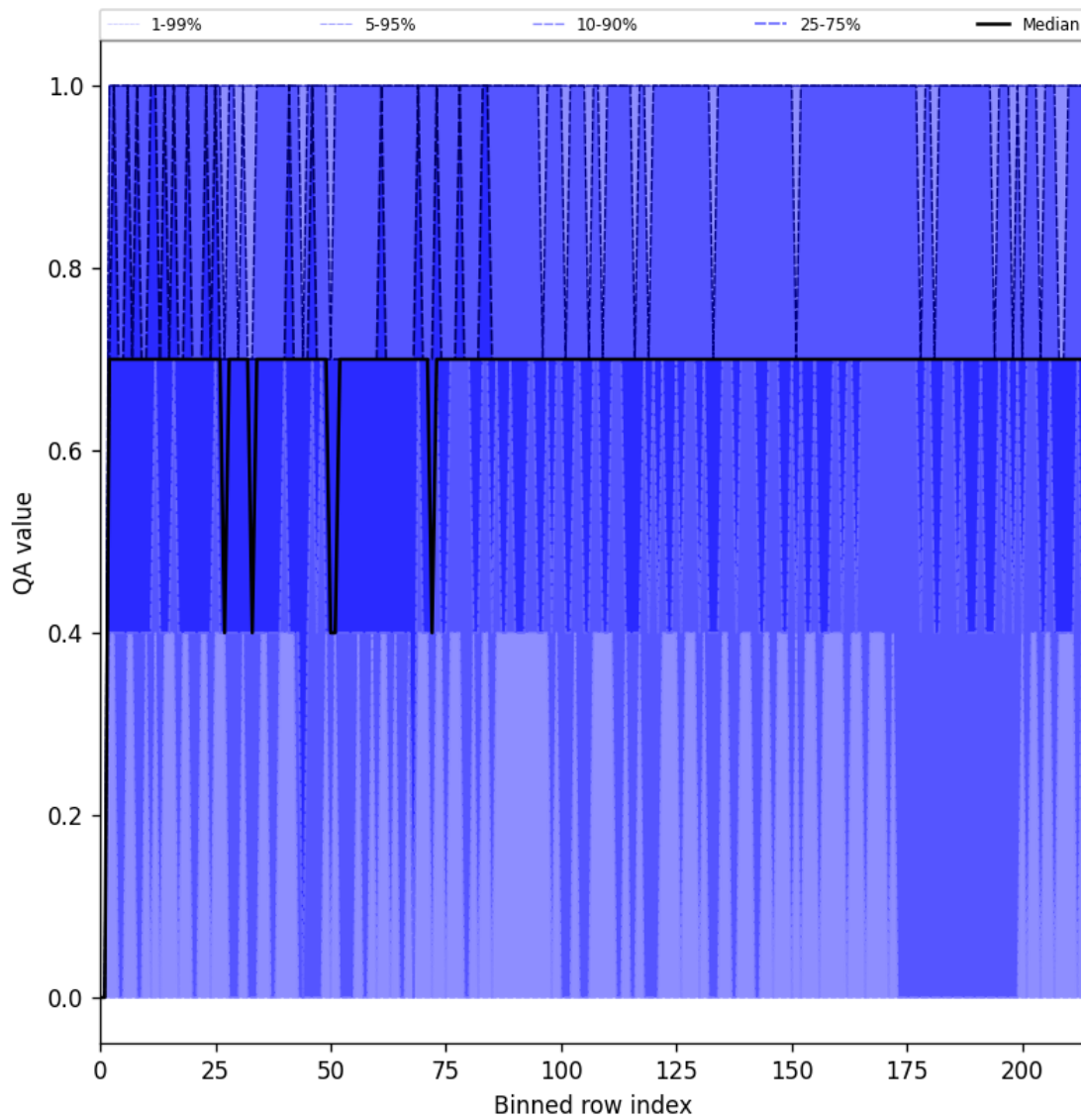
Figure 25: Along track statistics of “QA value” for 2025-01-28 to 2025-01-30
