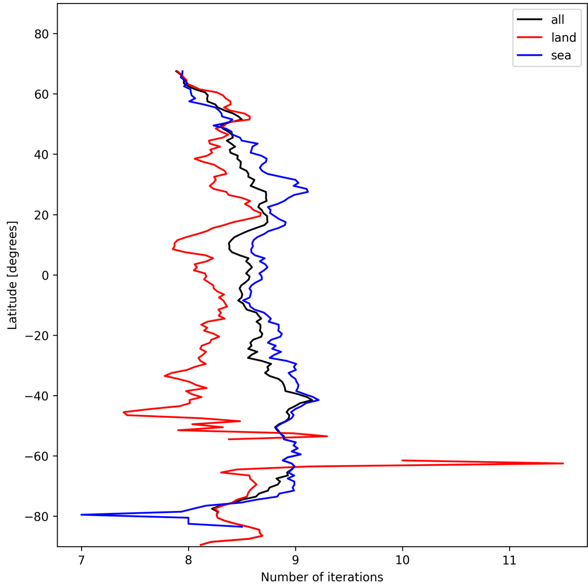
Figure 16: Zonal average of “Number of iterations” for 2025-01-28 to 2025-01-30.
