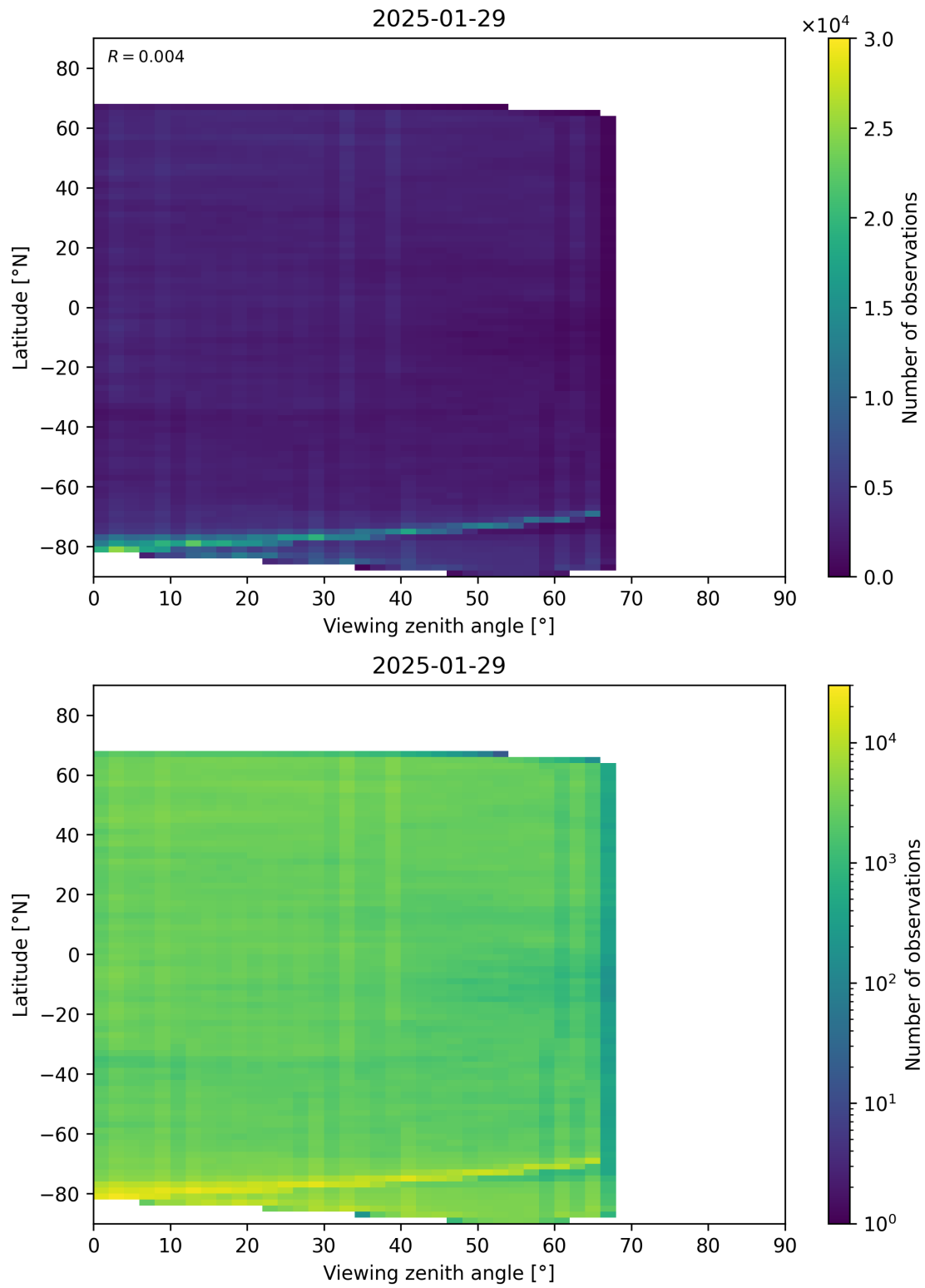
Figure 74: Scatter density plot of “Viewing zenith angle” against “Latitude” for 2025-01-28 to 2025-01-30.
