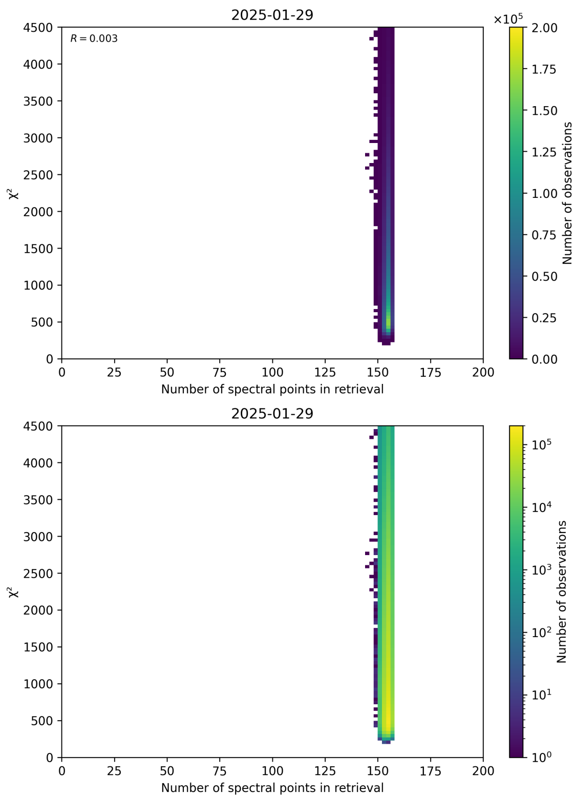
Figure 58: Scatter density plot of “Number of spectral points in retrieval” against “ \chi^2 ” for 2025-01-28 to 2025-01-30.
