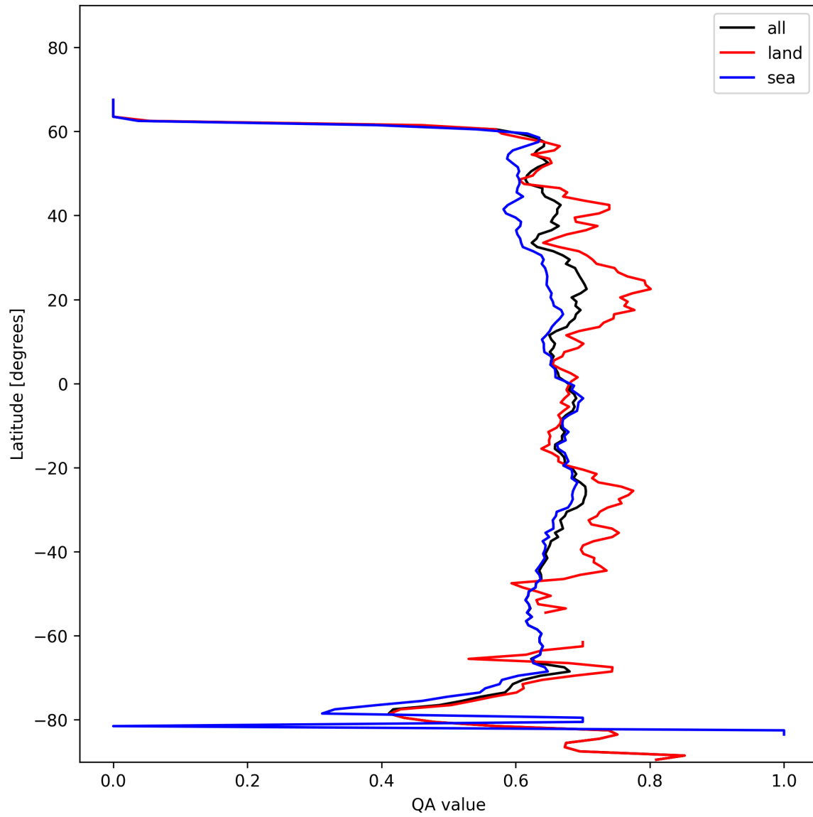
Figure 9: Zonal average of “QA value” for 2025-01-28 to 2025-01-30.
