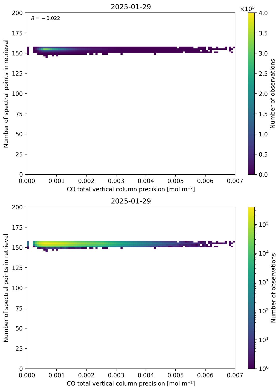
Figure 47: Scatter density plot of “CO total vertical column precision” against “Number of spectral points in retrieval” for 2025-01-28 to 2025-01-30.
