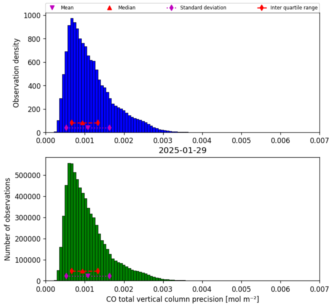
Figure 20: Histogram of “CO total vertical column precision” for 2025-01-28 to 2025-01-30
