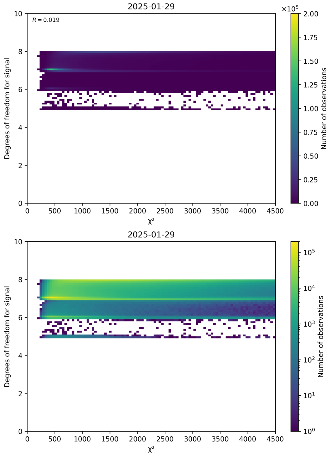
Figure 48: Scatter density plot of “ \chi^2 ” against “Degrees of freedom for signal” for 2025-01-28 to 2025-01-30.
