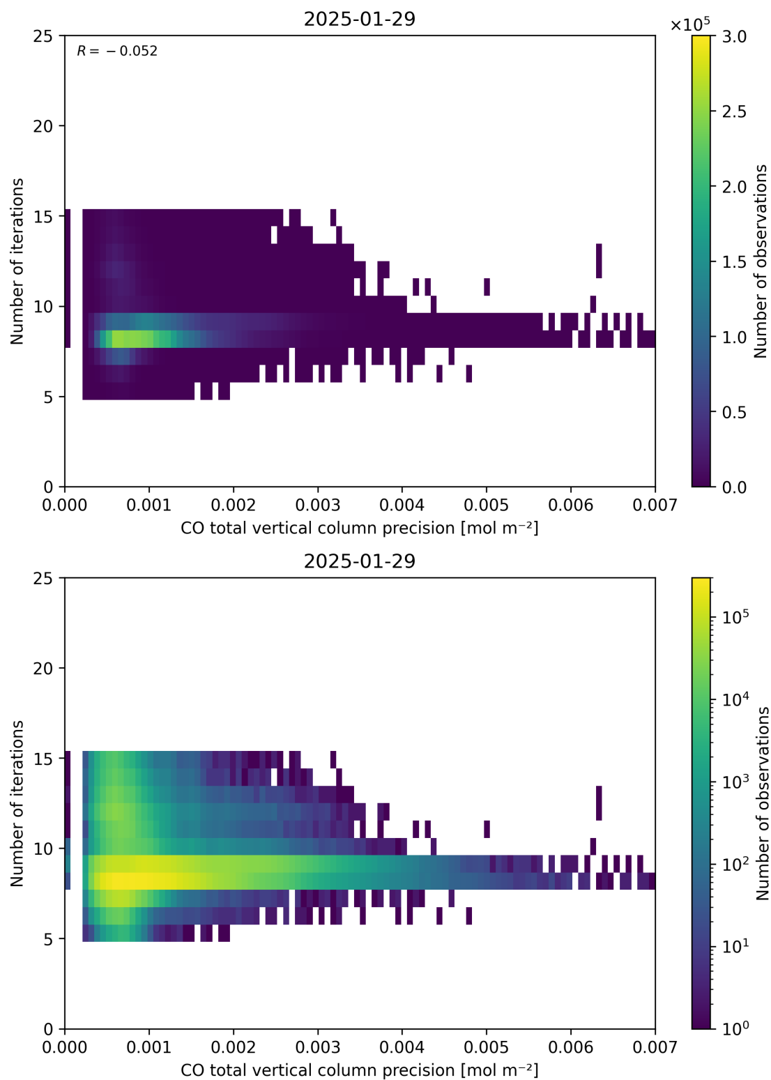
Figure 46: Scatter density plot of “CO total vertical column precision” against “Number of iterations” for 2025-01-28 to 2025-01-30.
