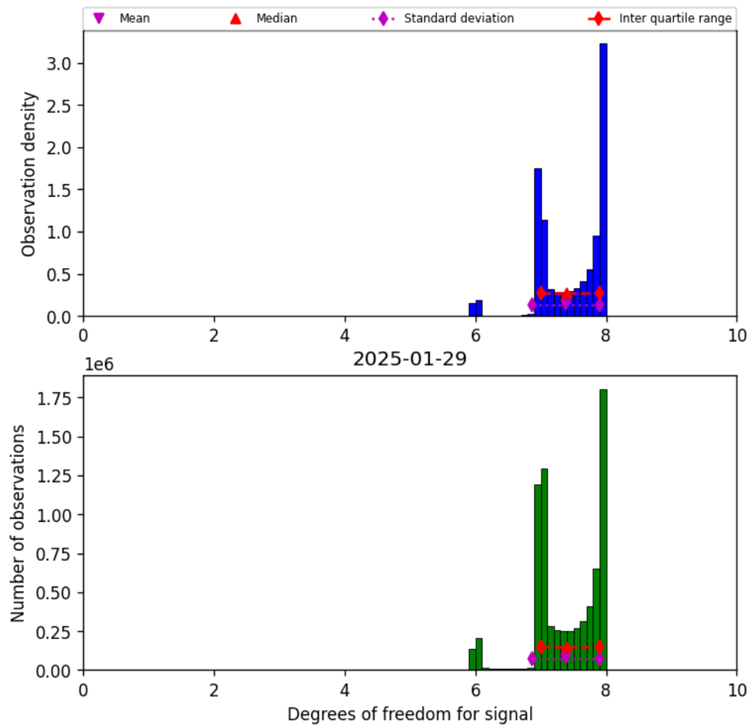
Figure 23: Histogram of “Degrees of freedom for signal” for 2025-01-28 to 2025-01-30
