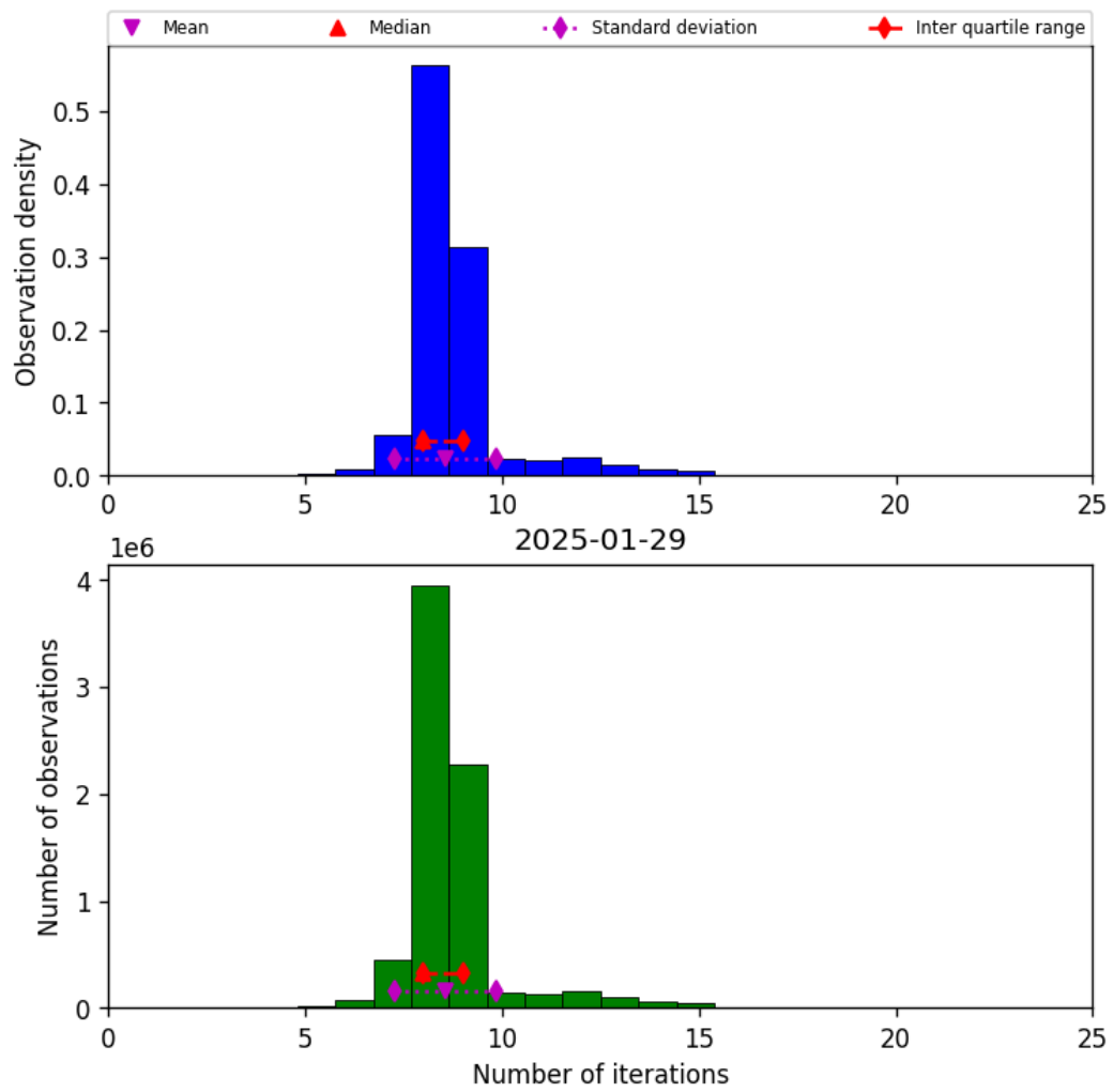
Figure 24: Histogram of “Number of iterations” for 2025-01-28 to 2025-01-30
