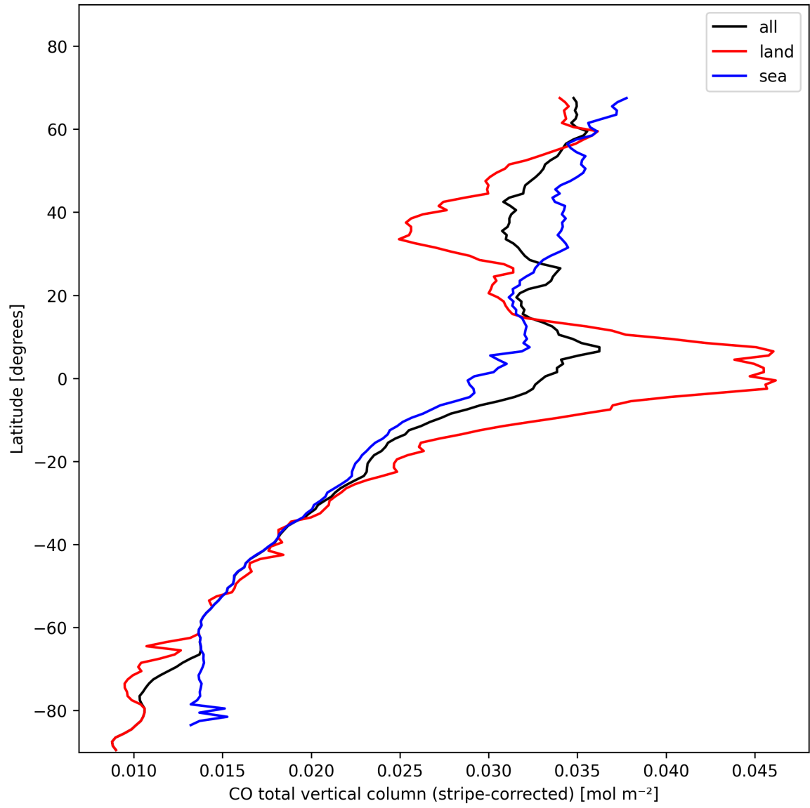
Figure 11: Zonal average of “CO total vertical column (stripe-corrected)” for 2025-01-28 to 2025-01-30.
