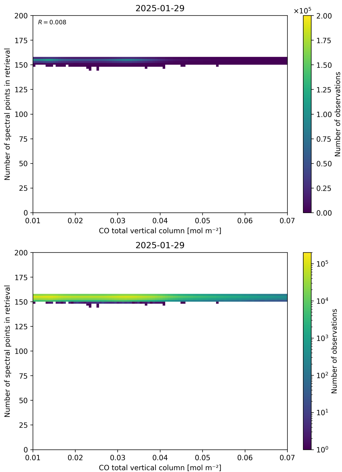
Figure 43: Scatter density plot of “CO total vertical column” against “Number of spectral points in retrieval” for 2025-01-28 to 2025-01-30.
