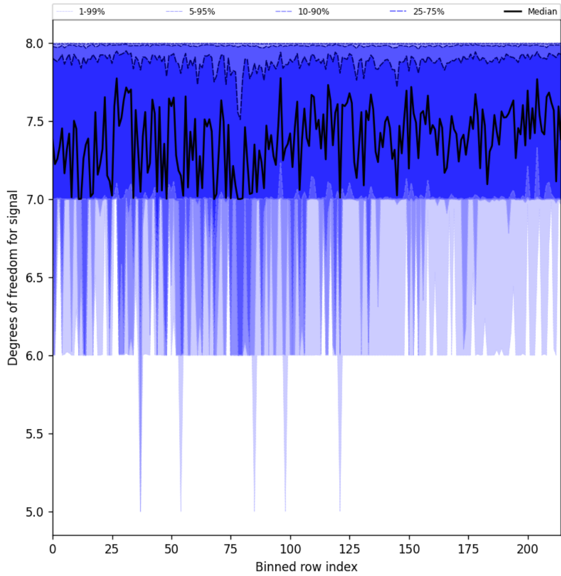
Figure 31: Along track statistics of “Degrees of freedom for signal” for 2025-01-28 to 2025-01-30
