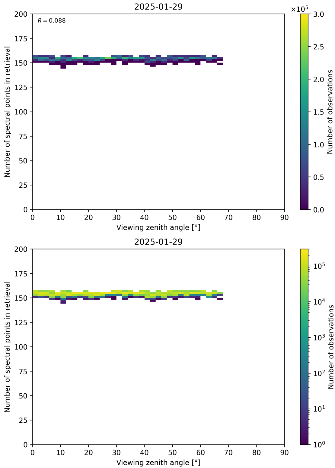
Figure 76: Scatter density plot of “Viewing zenith angle” against “Number of spectral points in retrieval” for 2025-01-28 to 2025-01-30.
