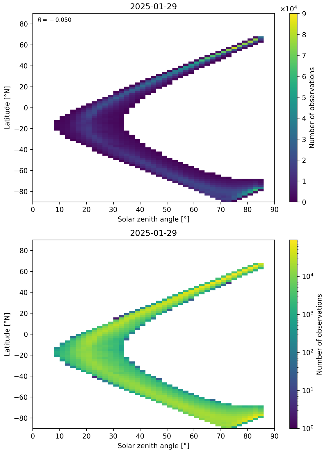
Figure 66: Scatter density plot of “Solar zenith angle” against “Latitude” for 2025-01-28 to 2025-01-30.
