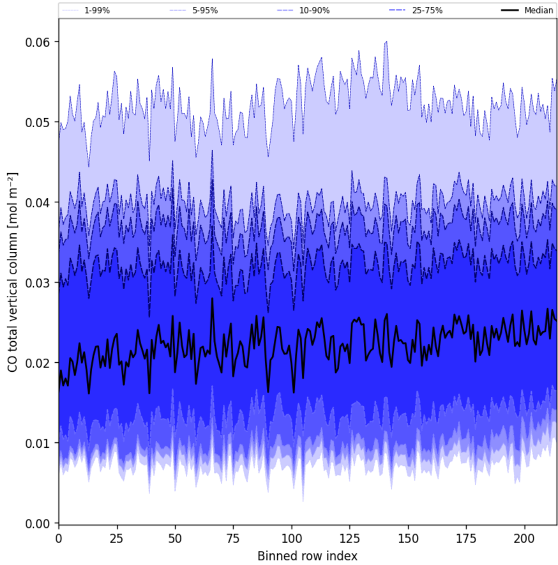
Figure 26: Along track statistics of “CO total vertical column” for 2025-01-28 to 2025-01-30
