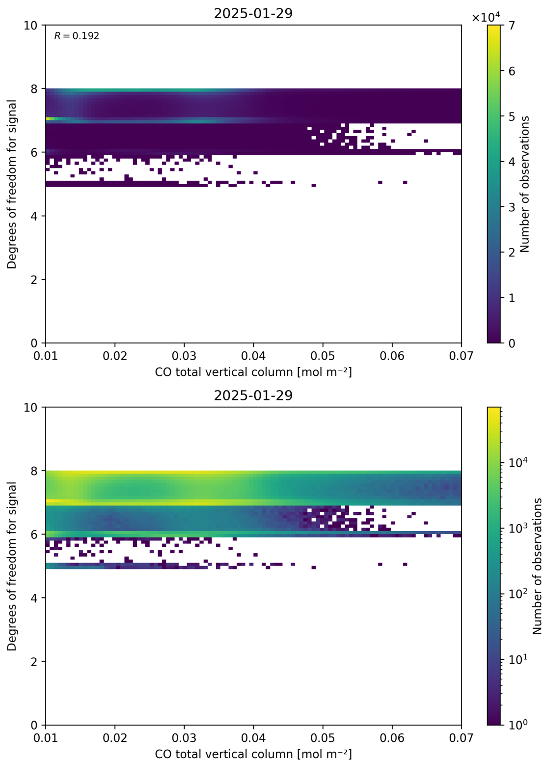
Figure 41: Scatter density plot of “CO total vertical column” against “Degrees of freedom for signal” for 2025-01-28 to 2025-01-30.
