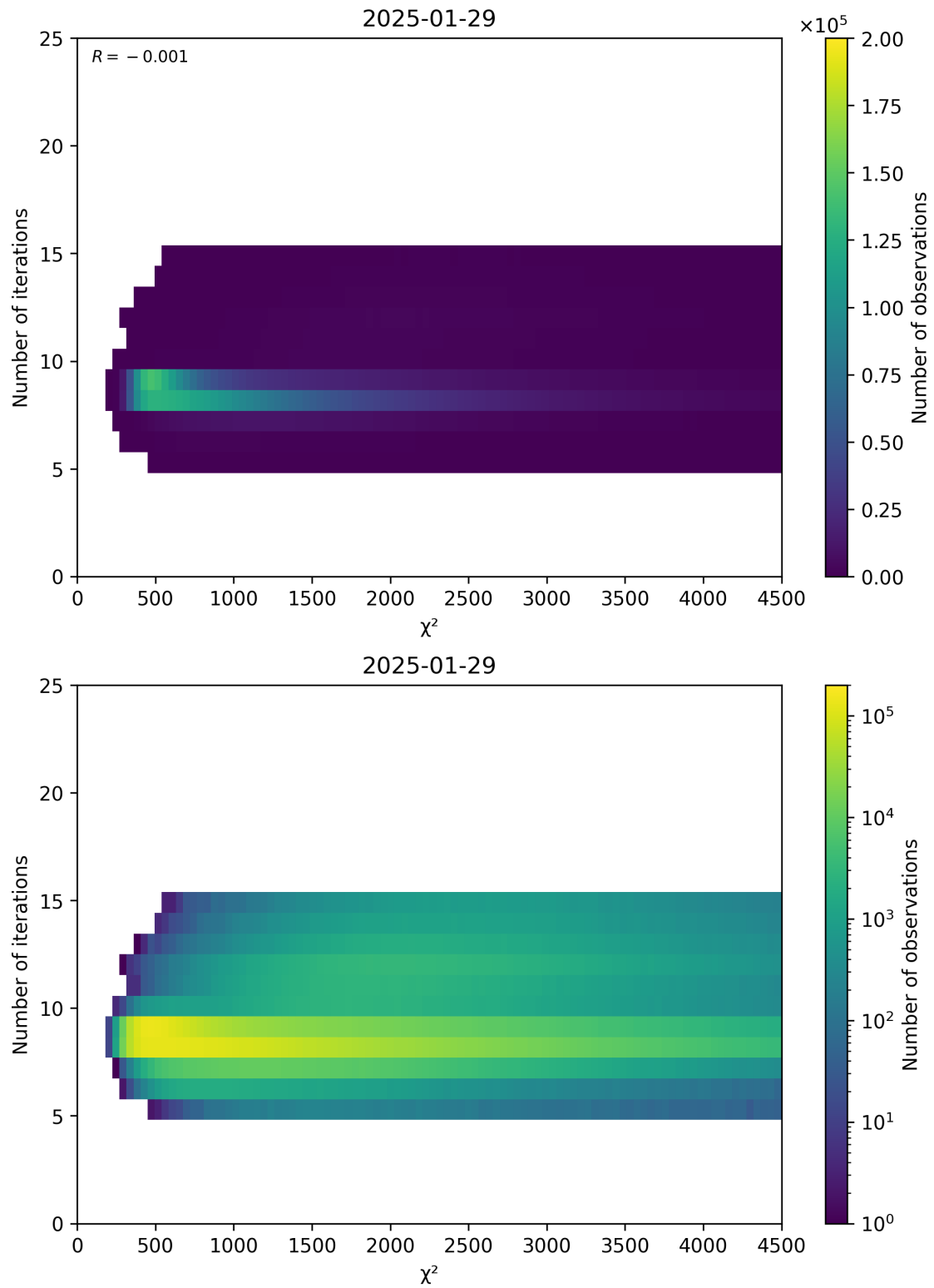
Figure 49: Scatter density plot of “ \chi^2 ” against “Number of iterations” for 2025-01-28 to 2025-01-30.
