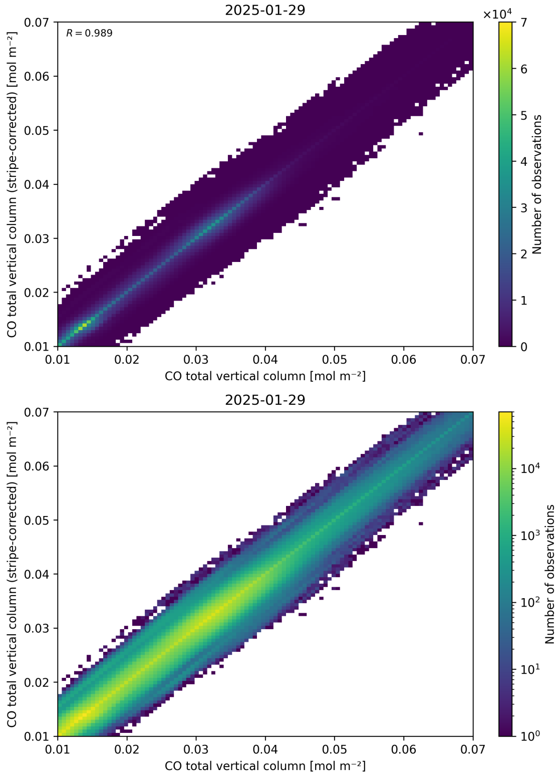
Figure 33: Scatter density plot of “CO total vertical column” against “CO total vertical column (stripe-corrected)” for 2025-01-28 to 2025-01-30.
