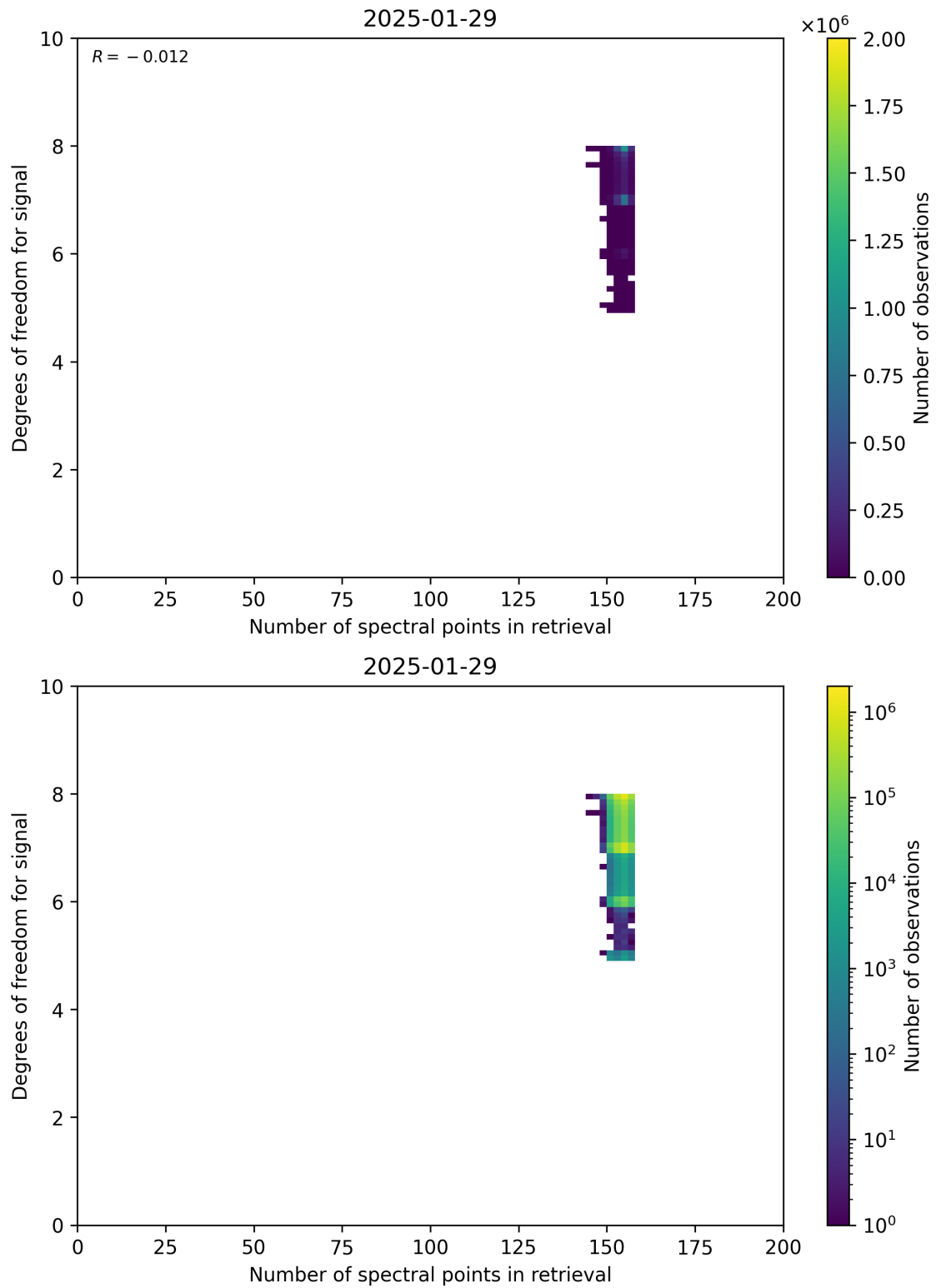
Figure 59: Scatter density plot of “Number of spectral points in retrieval” against “Degrees of freedom for signal” for 2025-01-28 to 2025-01-30.
