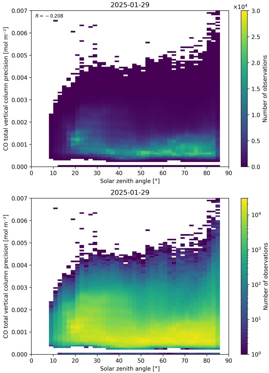
Figure 63: Scatter density plot of “Solar zenith angle” against “CO total vertical column precision” for 2025-01-28 to 2025-01-30.
