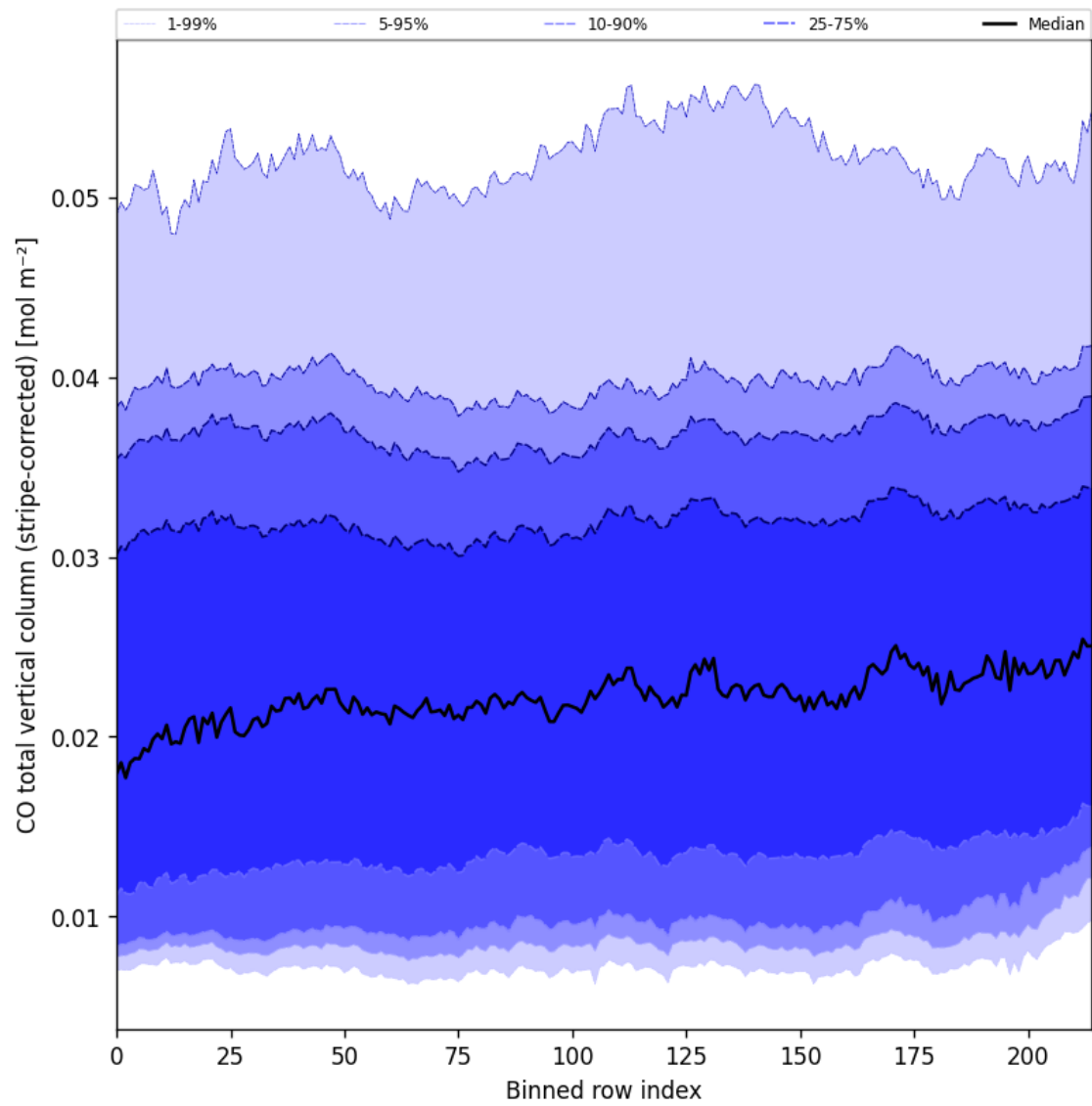
Figure 27: Along track statistics of “CO total vertical column (stripe-corrected)” for 2025-01-28 to 2025-01-30
