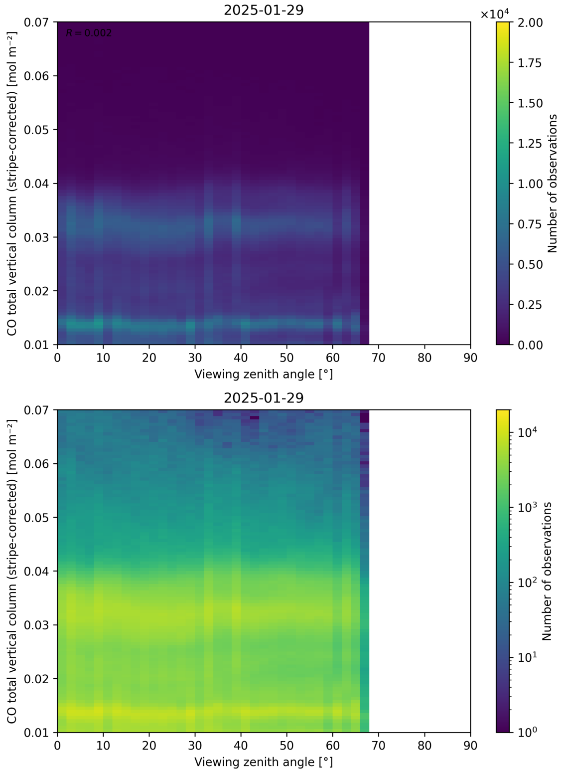
Figure 70: Scatter density plot of “Viewing zenith angle” against “CO total vertical column (stripe-corrected)” for 2025-01-28 to 2025-01-30.
