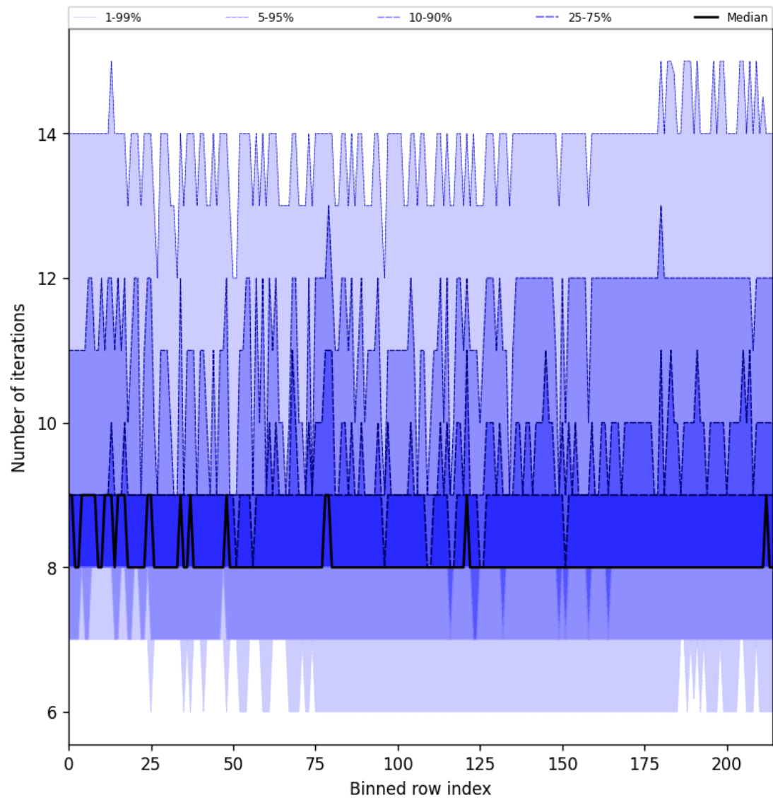
Figure 32: Along track statistics of “Number of iterations” for 2025-01-28 to 2025-01-30
