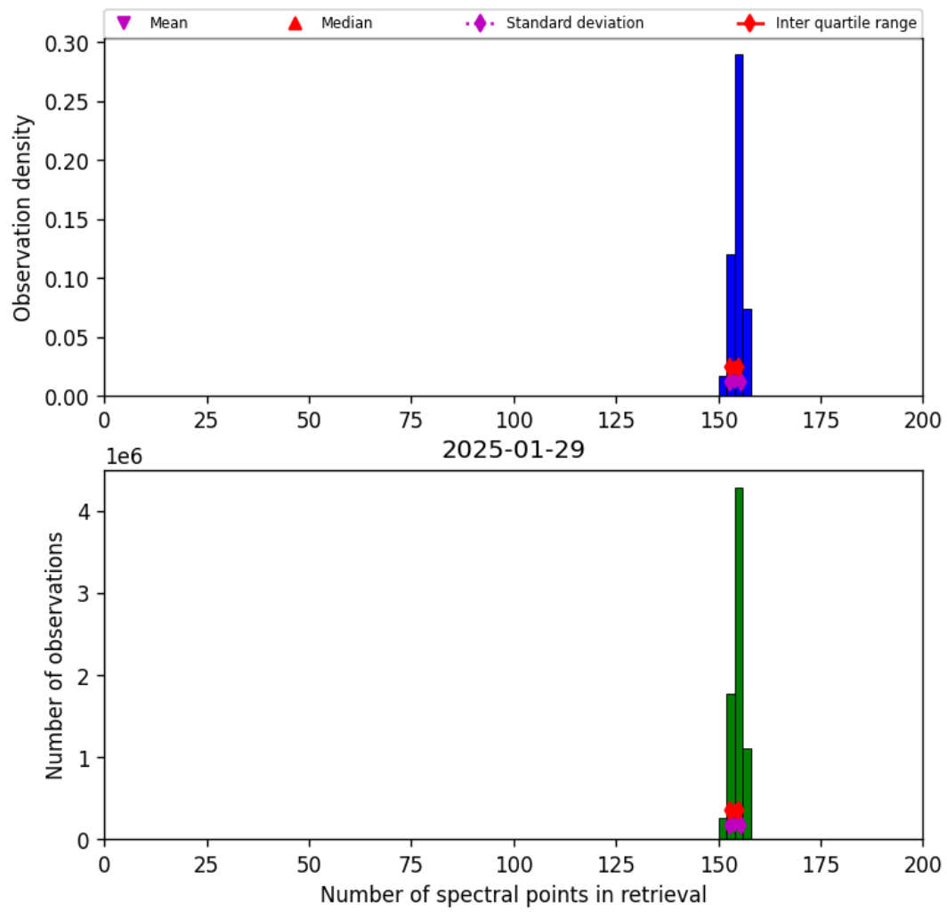
Figure 21: Histogram of “Number of spectral points in retrieval” for 2025-01-28 to 2025-01-30
