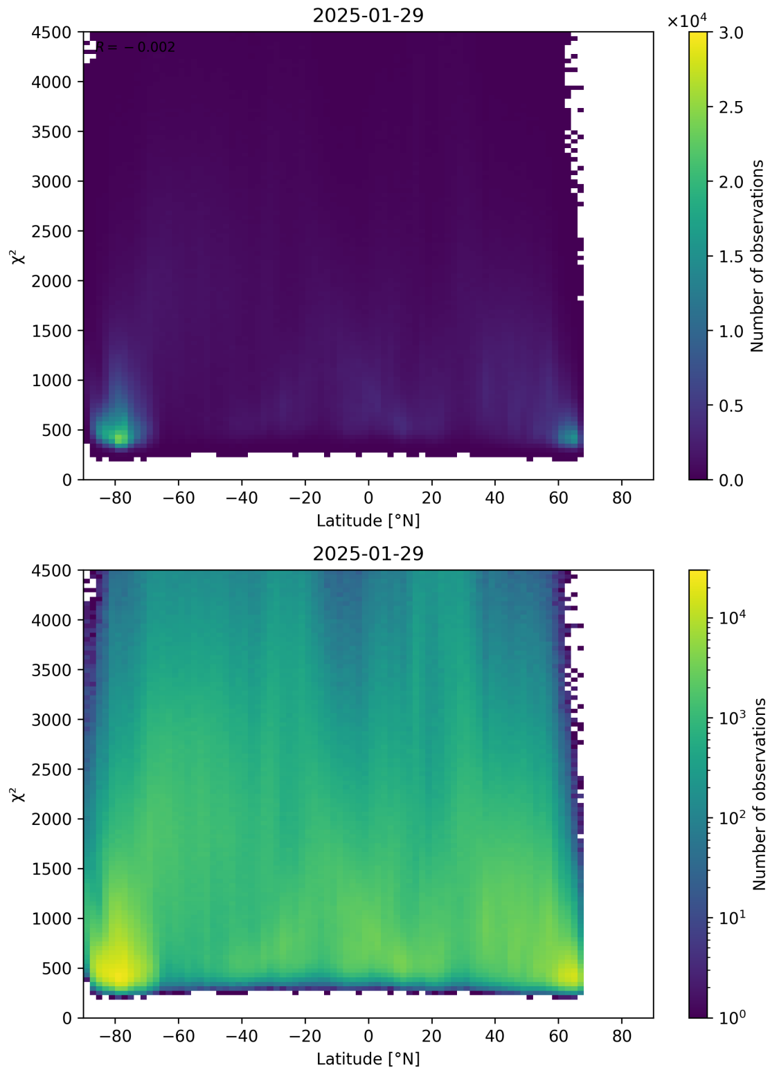
Figure 54: Scatter density plot of “Latitude” against “ \chi^2 ” for 2025-01-28 to 2025-01-30.
