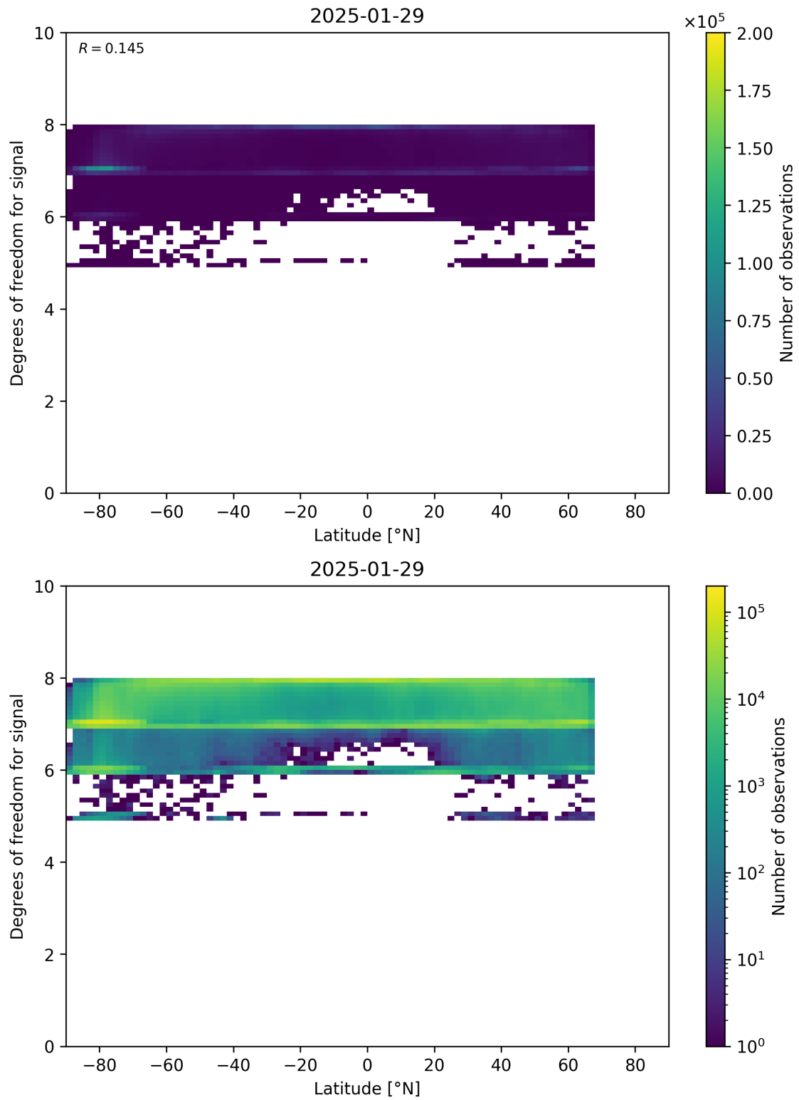
Figure 55: Scatter density plot of “Latitude” against “Degrees of freedom for signal” for 2025-01-28 to 2025-01-30.
