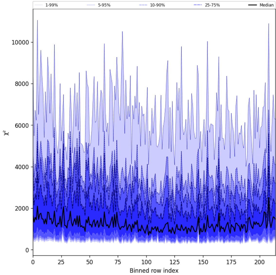
Figure 30: Along track statistics of “ \chi^2 ” for 2025-01-28 to 2025-01-30
