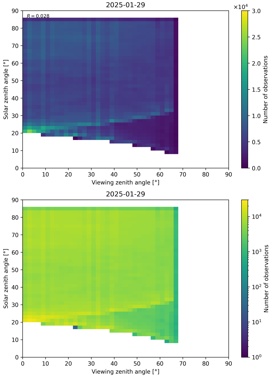
Figure 77: Scatter density plot of “Viewing zenith angle” against “Solar zenith angle” for 2025-01-28 to 2025-01-30.
