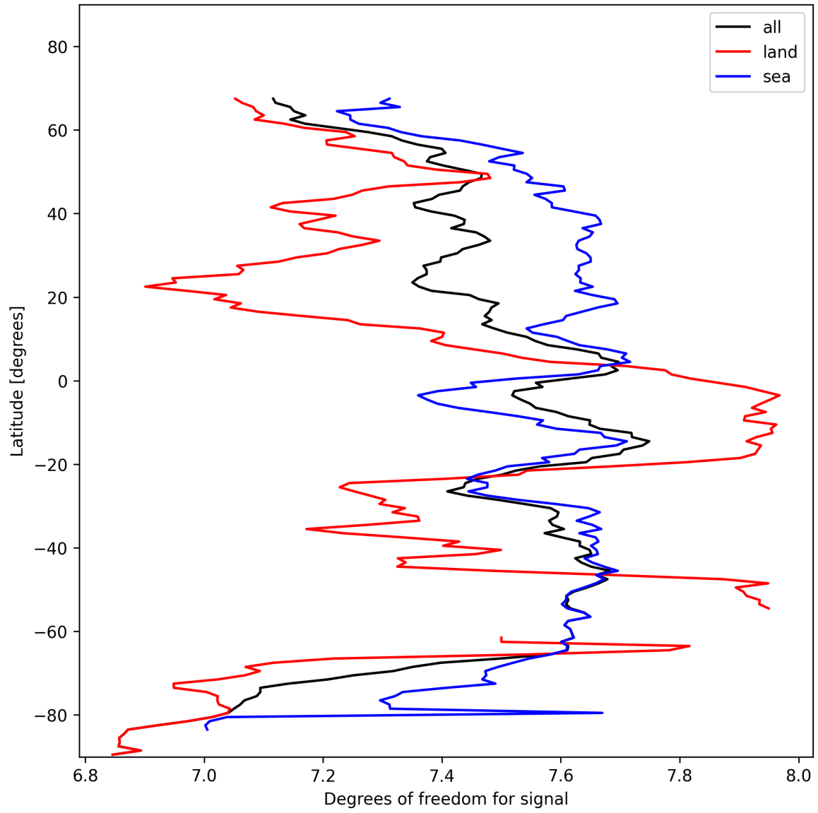
Figure 15: Zonal average of “Degrees of freedom for signal” for 2025-01-28 to 2025-01-30.
