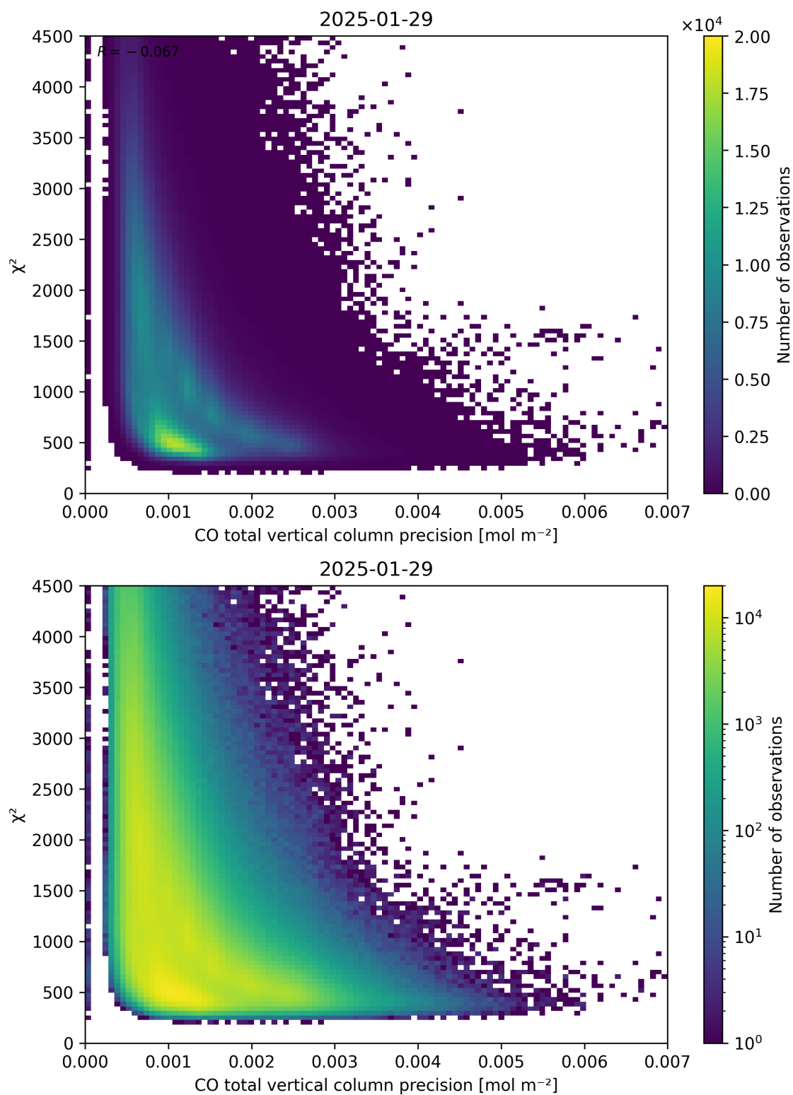
Figure 44: Scatter density plot of “CO total vertical column precision” against “ \chi^2 ” for 2025-01-28 to 2025-01-30.
