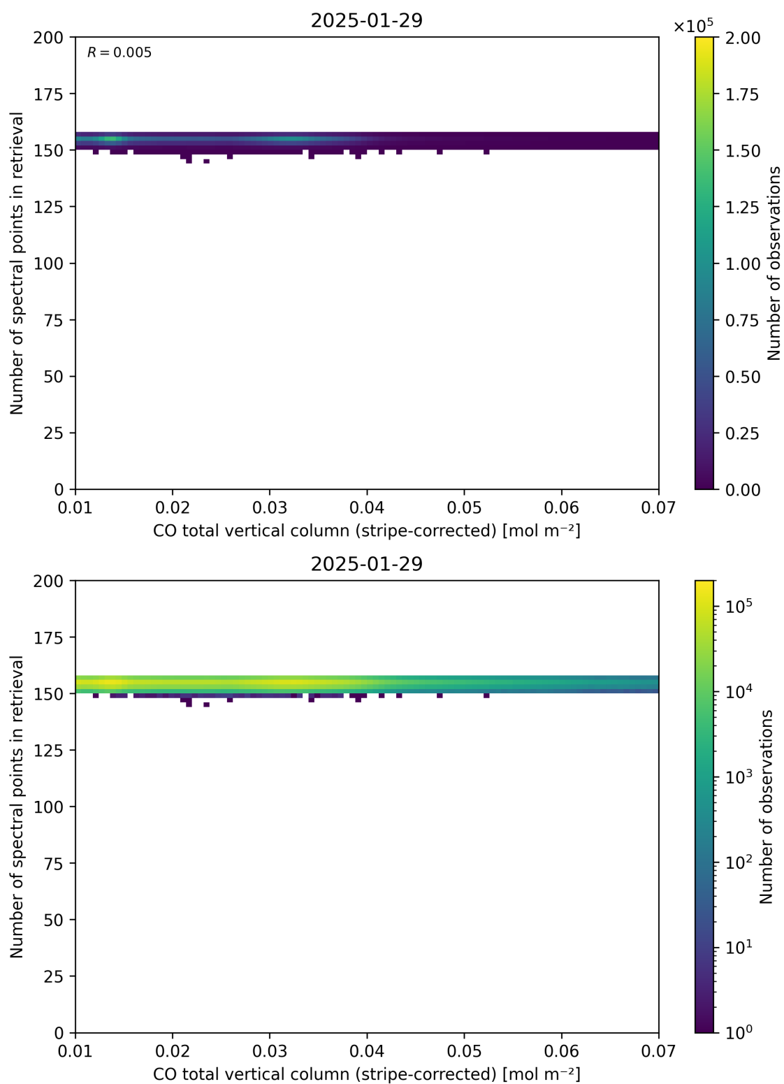
Figure 40: Scatter density plot of “CO total vertical column (stripe-corrected)” against “Number of spectral points in retrieval” for 2025-01-28 to 2025-01-30.
