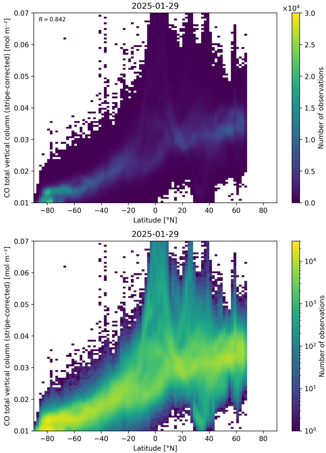
Figure 52: Scatter density plot of “Latitude” against “CO total vertical column (stripe-corrected)” for 2025-01-28 to 2025-01-30.
