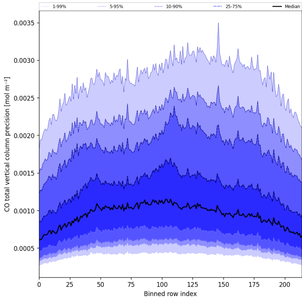
Figure 28: Along track statistics of “CO total vertical column precision” for 2025-01-28 to 2025-01-30
