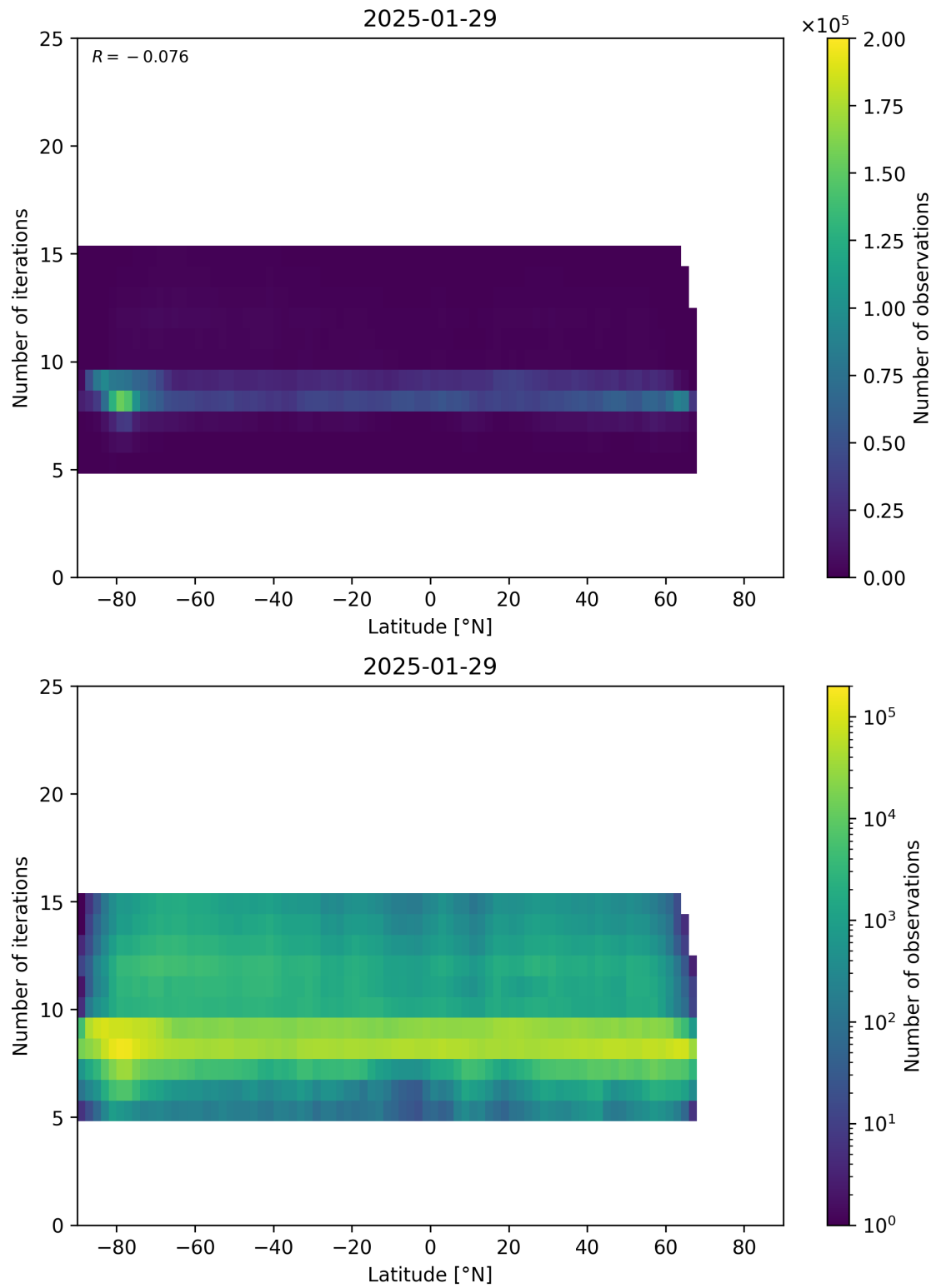
Figure 56: Scatter density plot of “Latitude” against “Number of iterations” for 2025-01-28 to 2025-01-30.
