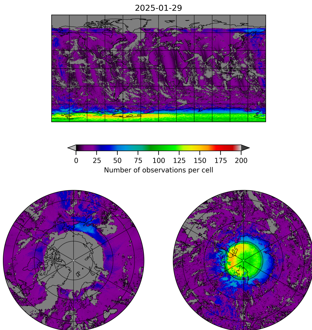
Figure 8: Map of the number of observations for 2025-01-28 to 2025-01-30
