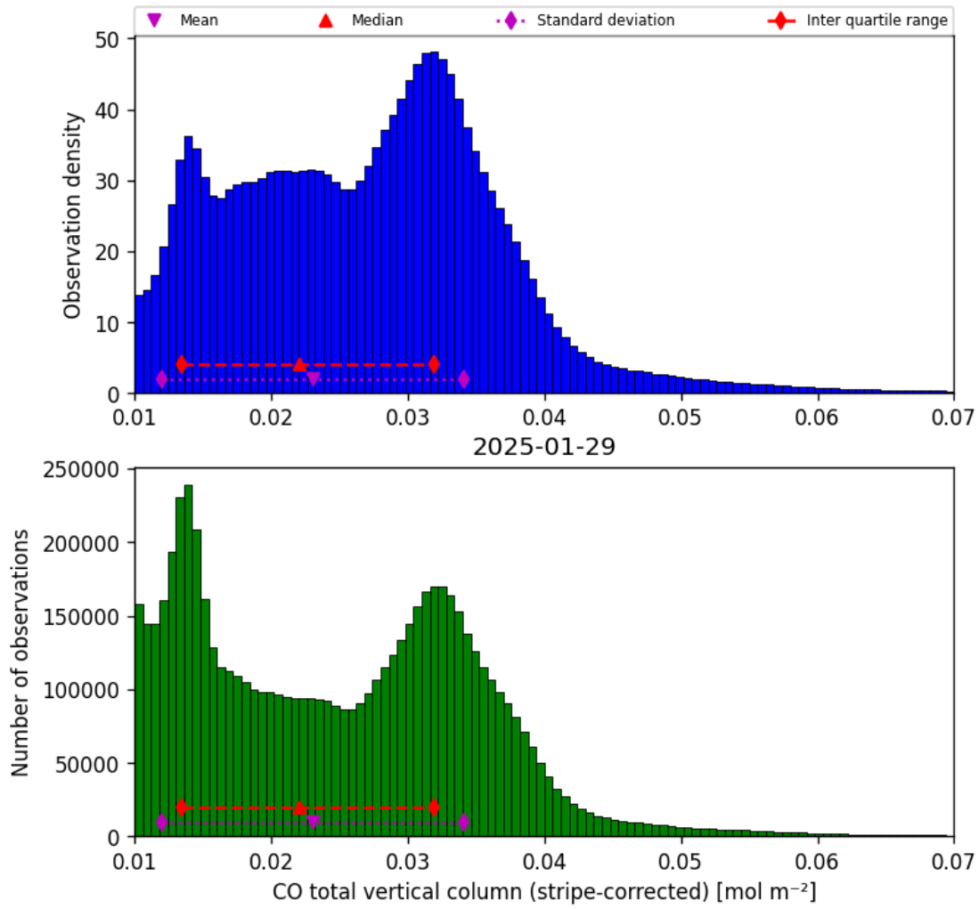
Figure 19: Histogram of “CO total vertical column (stripe-corrected)” for 2025-01-28 to 2025-01-30
