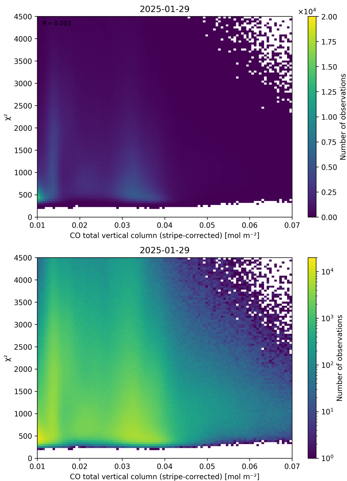
Figure 37: Scatter density plot of “CO total vertical column (stripe-corrected)” against “ \chi^2 ” for 2025-01-28 to 2025-01-30.
