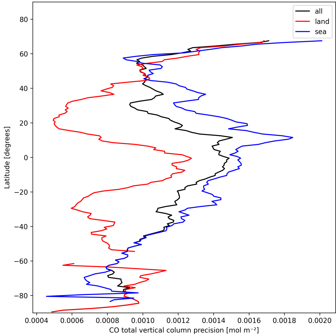
Figure 12: Zonal average of “CO total vertical column precision” for 2025-01-28 to 2025-01-30.
