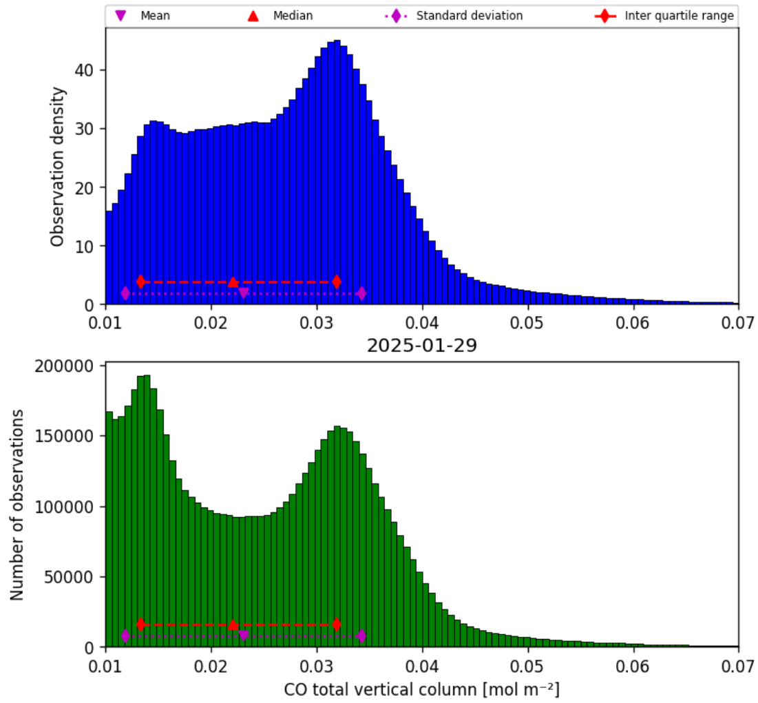
Figure 18: Histogram of “CO total vertical column” for 2025-01-28 to 2025-01-30
