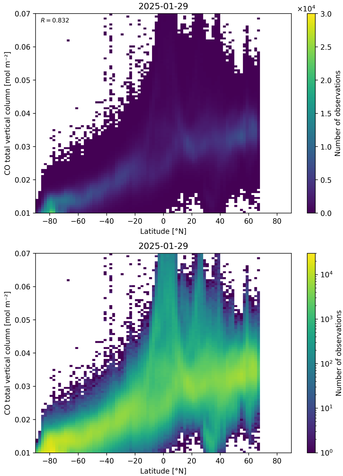
Figure 51: Scatter density plot of “Latitude” against “CO total vertical column” for 2025-01-28 to 2025-01-30.
