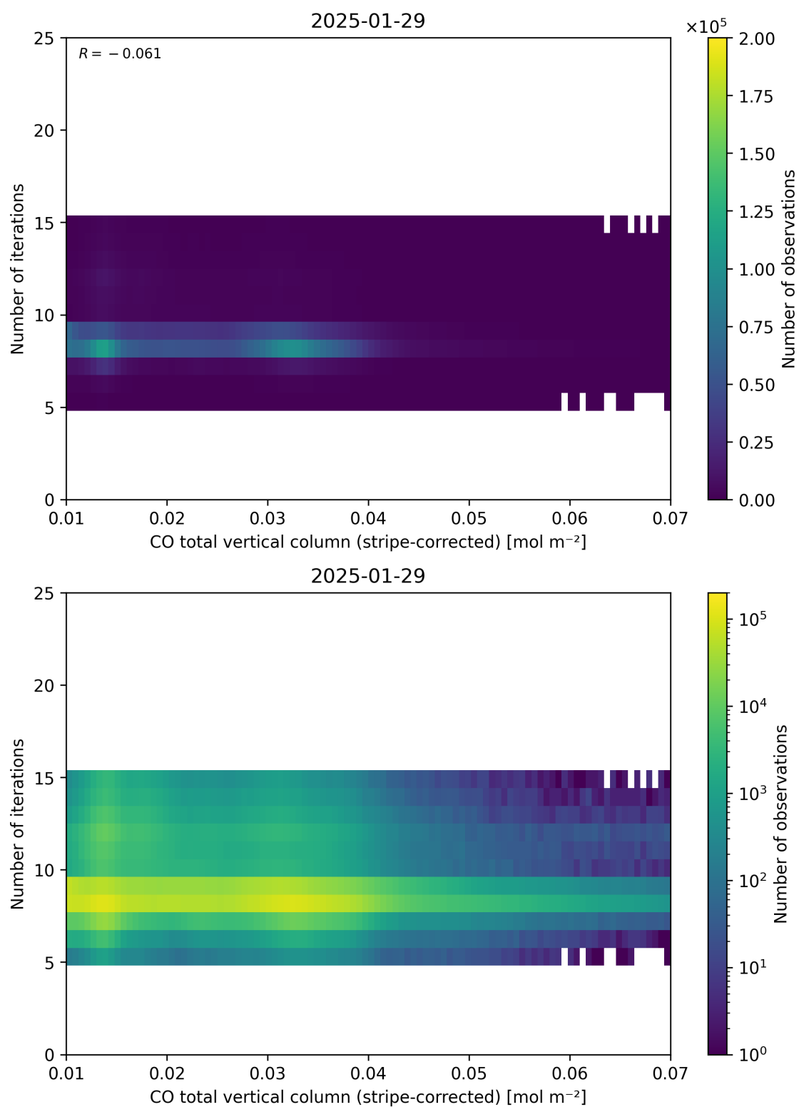
Figure 39: Scatter density plot of “CO total vertical column (stripe-corrected)” against “Number of iterations” for 2025-01-28 to 2025-01-30.
