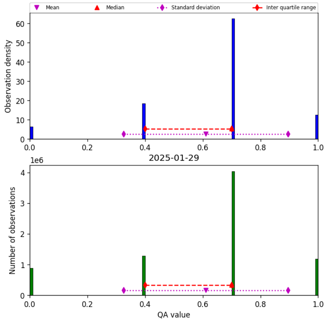
Figure 17: Histogram of “QA value” for 2025-01-28 to 2025-01-30
