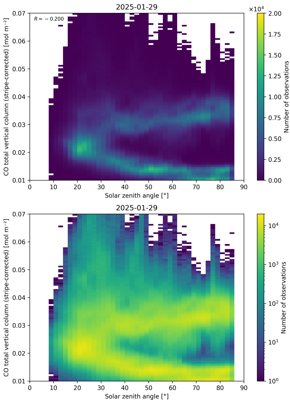
Figure 62: Scatter density plot of “Solar zenith angle” against “CO total vertical column (stripe-corrected)” for 2025-01-28 to 2025-01-30.
