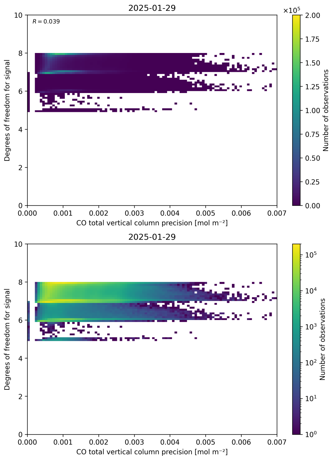
Figure 45: Scatter density plot of “CO total vertical column precision” against “Degrees of freedom for signal” for 2025-01-28 to 2025-01-30.
