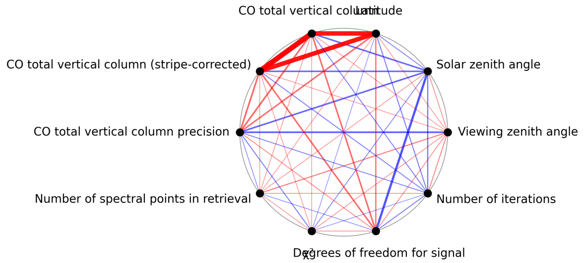
Figure 1: Map of correlation graph for 2025-01-28 to 2025-01-30.
