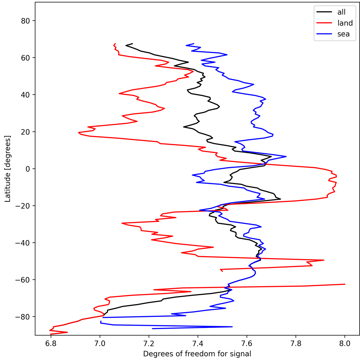
Figure 15: Zonal average of “Degrees of freedom for signal” for 2025-01-29 to 2025-01-31.
