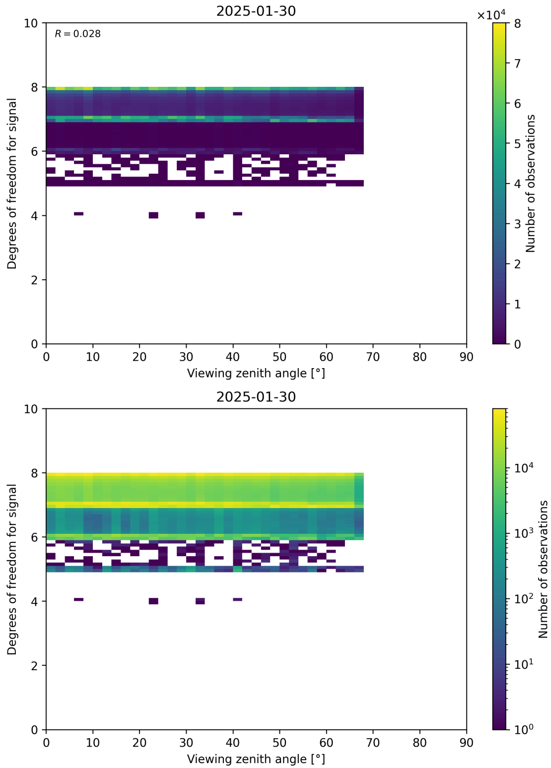
Figure 73: Scatter density plot of “Viewing zenith angle” against “Degrees of freedom for signal” for 2025-01-29 to 2025-01-31.
