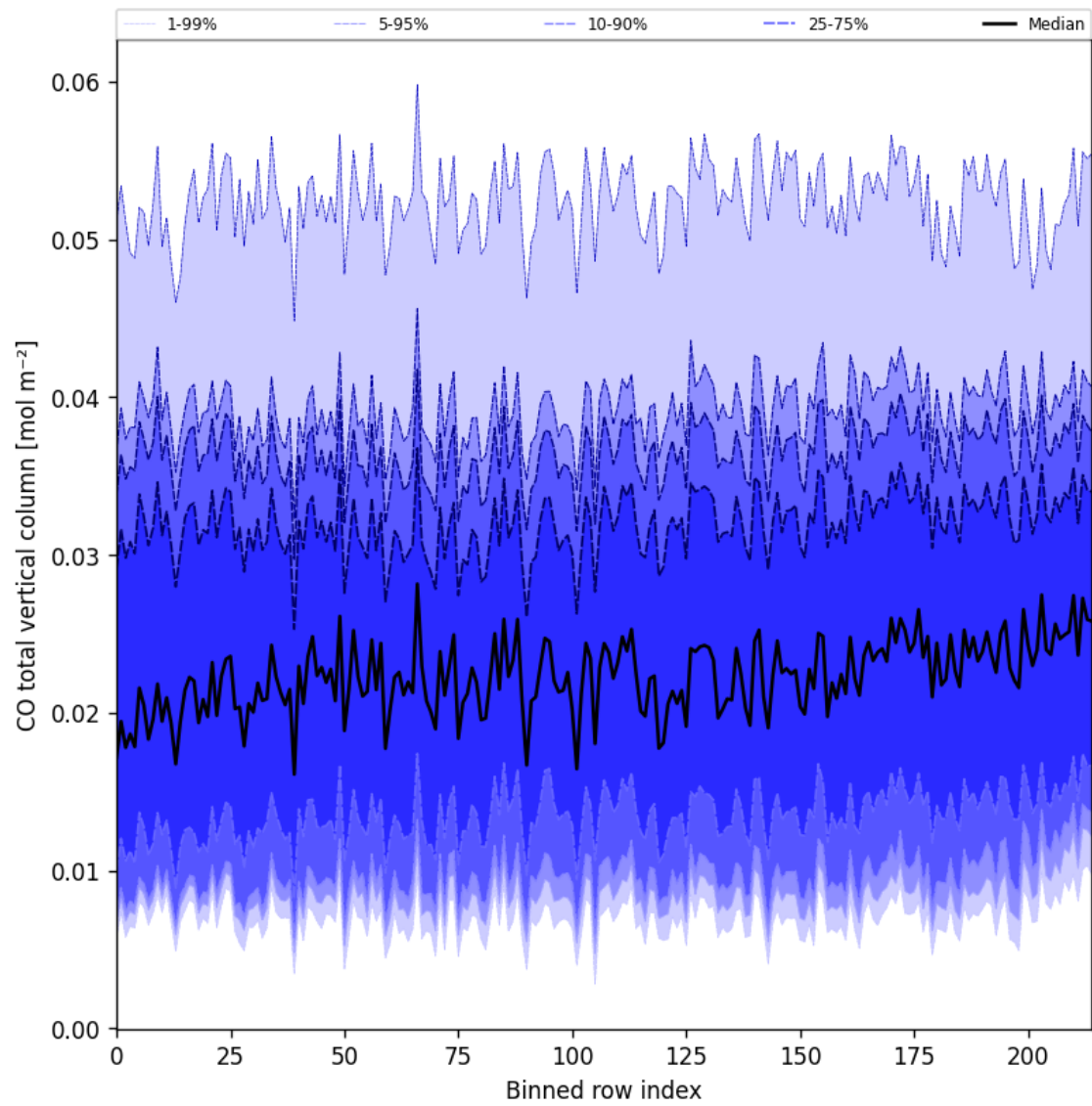
Figure 26: Along track statistics of “CO total vertical column” for 2025-01-29 to 2025-01-31
