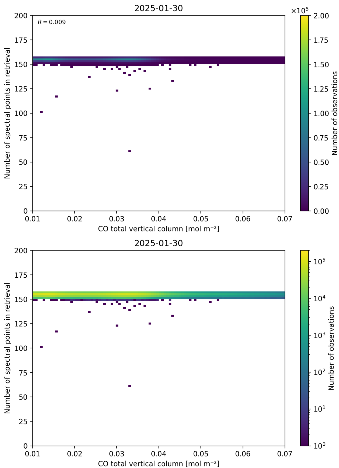
Figure 43: Scatter density plot of “CO total vertical column” against “Number of spectral points in retrieval” for 2025-01-29 to 2025-01-31.
