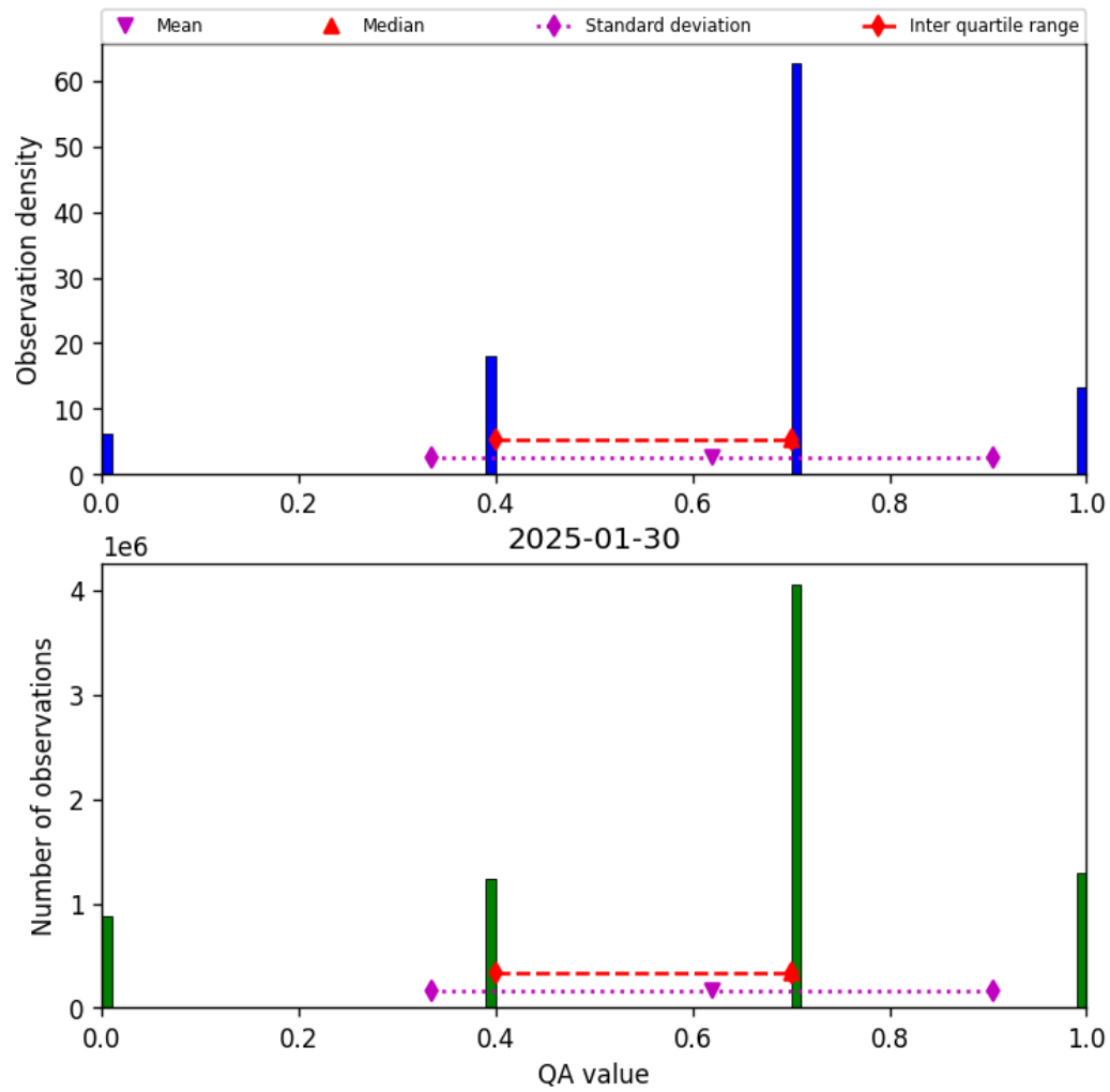
Figure 17: Histogram of “QA value” for 2025-01-29 to 2025-01-31
