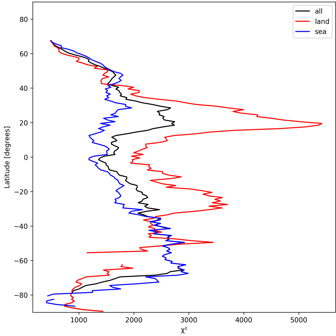
Figure 14: Zonal average of “ \chi^2 ” for 2025-01-29 to 2025-01-31.
