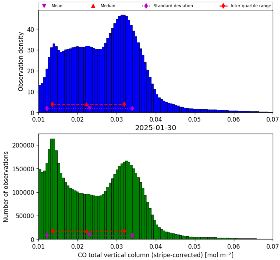
Figure 19: Histogram of “CO total vertical column (stripe-corrected)” for 2025-01-29 to 2025-01-31
