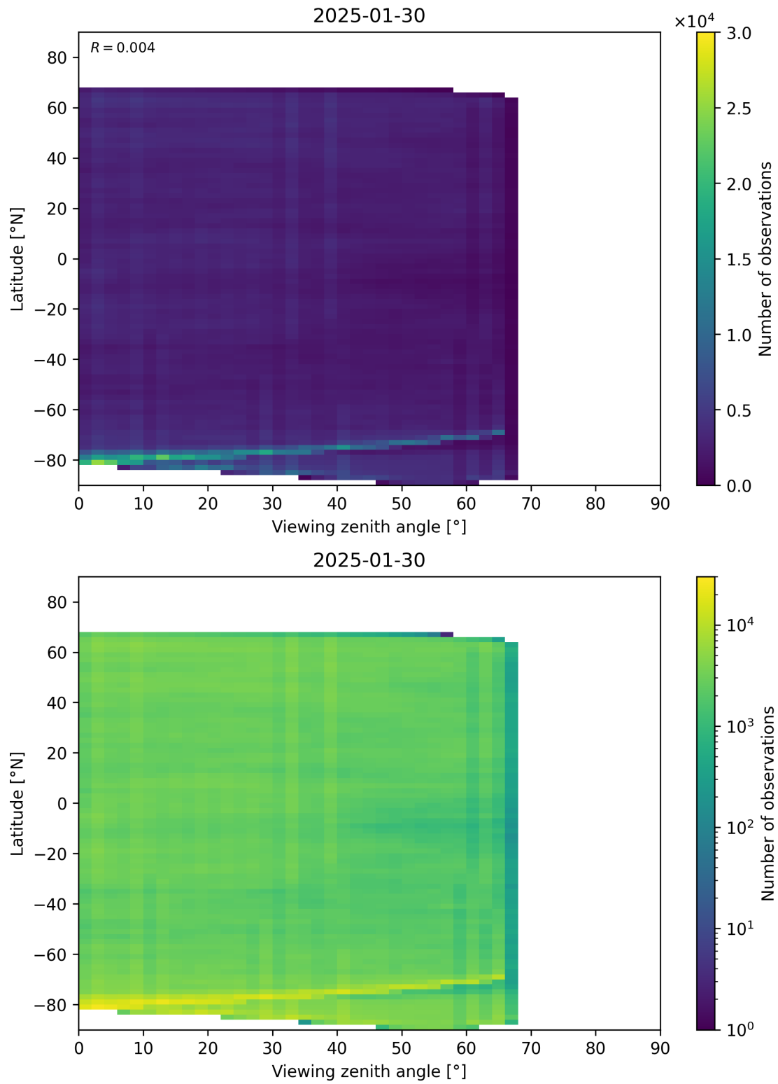
Figure 74: Scatter density plot of “Viewing zenith angle” against “Latitude” for 2025-01-29 to 2025-01-31.
