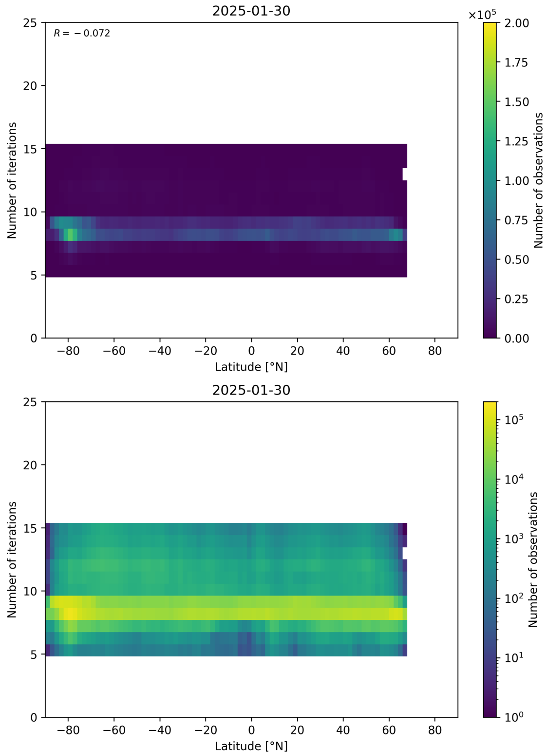
Figure 56: Scatter density plot of “Latitude” against “Number of iterations” for 2025-01-29 to 2025-01-31.
