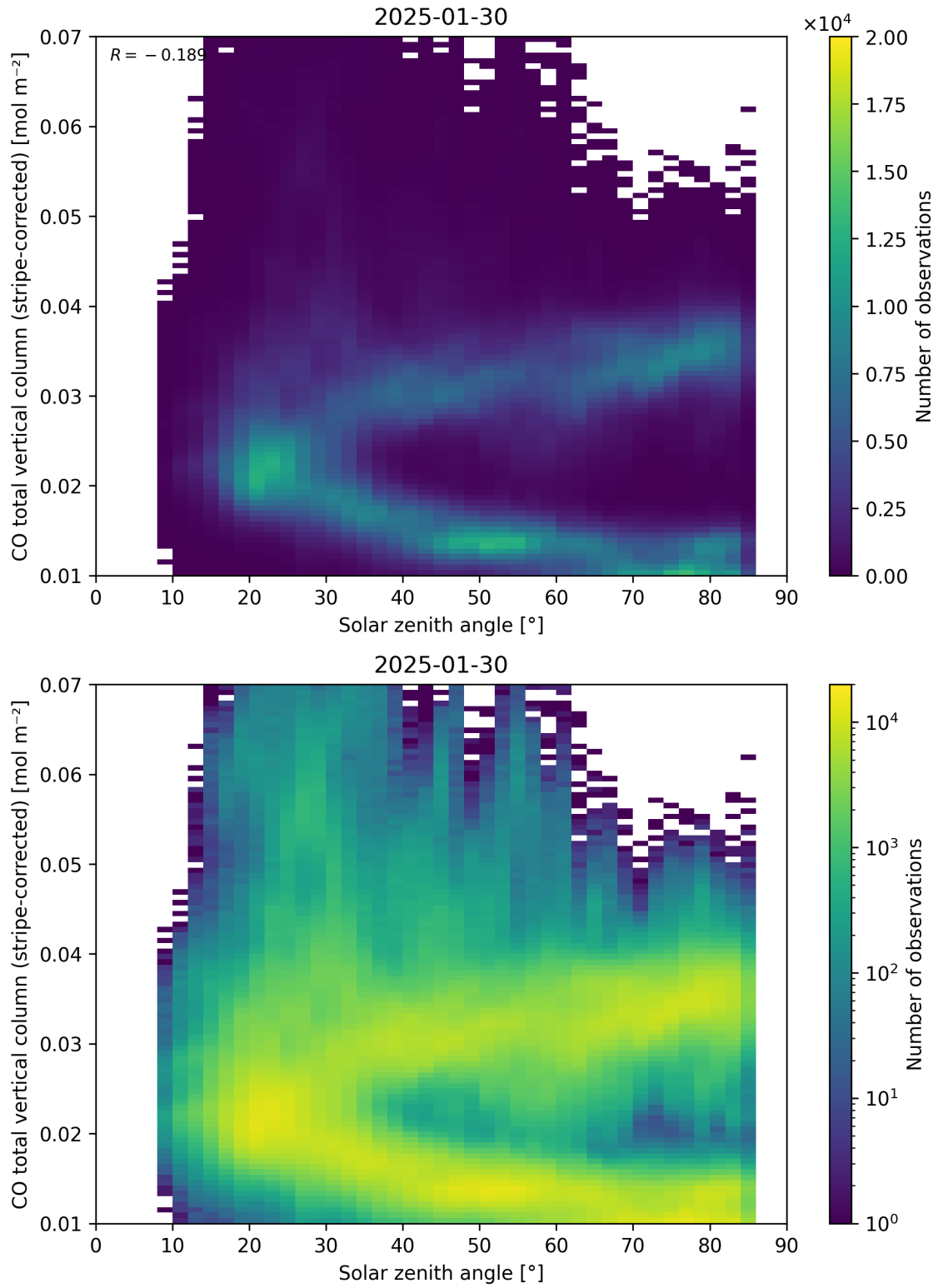
Figure 62: Scatter density plot of “Solar zenith angle” against “CO total vertical column (stripe-corrected)” for 2025-01-29 to 2025-01-31.
