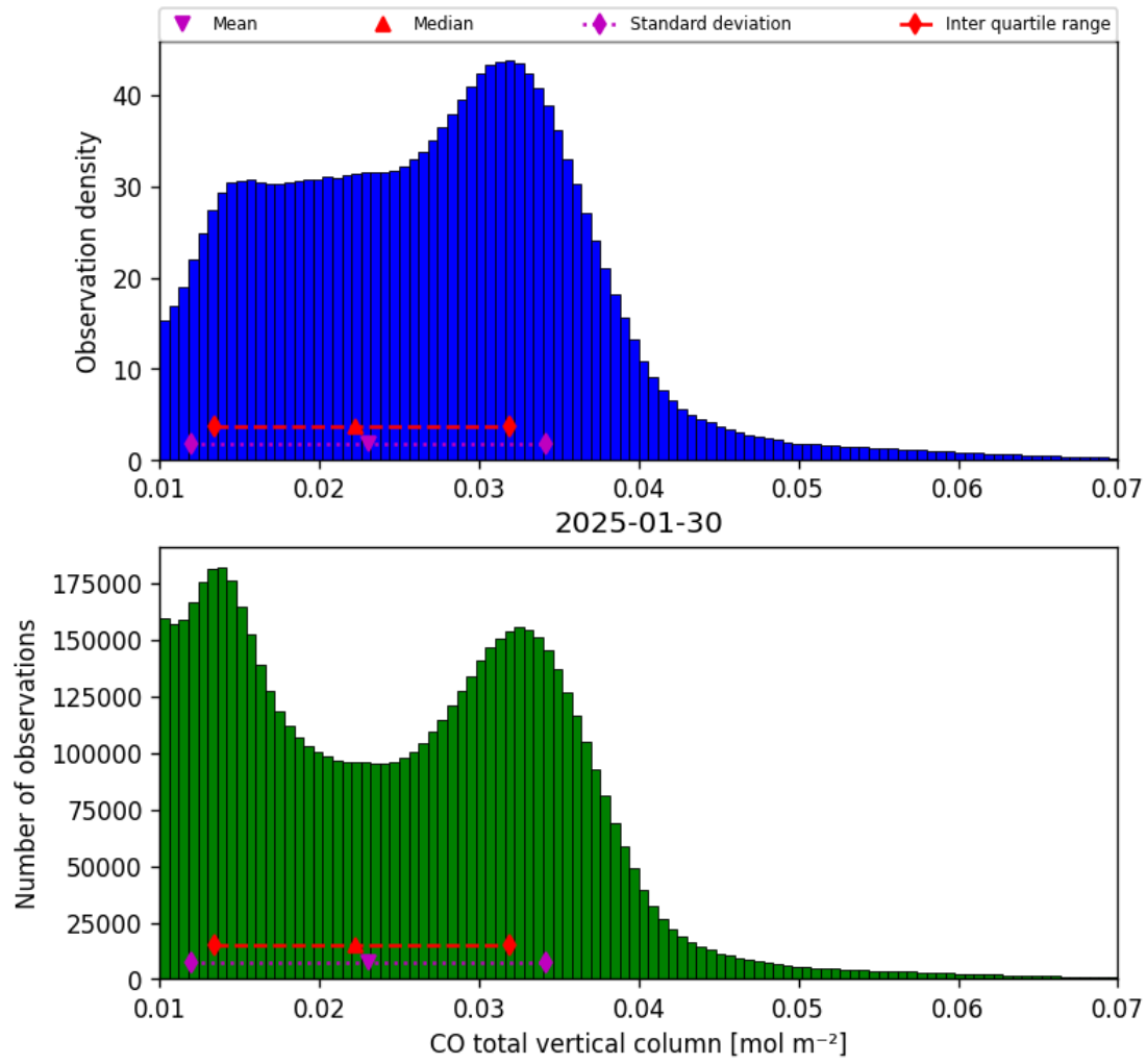
Figure 18: Histogram of “CO total vertical column” for 2025-01-29 to 2025-01-31
