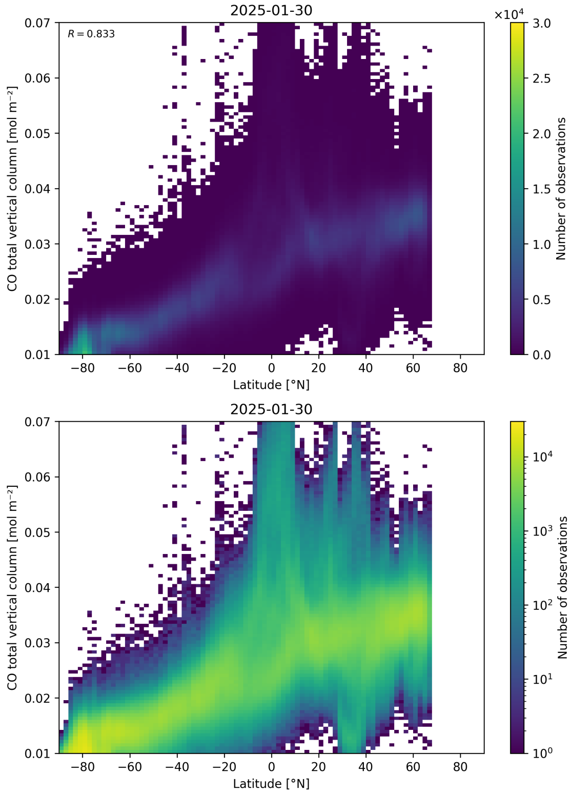
Figure 51: Scatter density plot of “Latitude” against “CO total vertical column” for 2025-01-29 to 2025-01-31.
