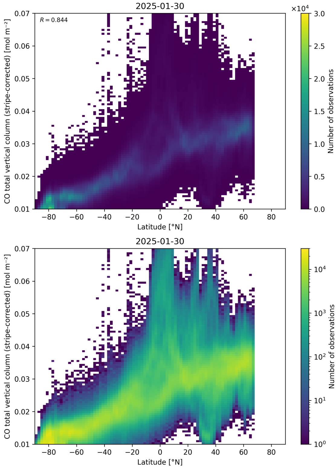
Figure 52: Scatter density plot of “Latitude” against “CO total vertical column (stripe-corrected)” for 2025-01-29 to 2025-01-31.
