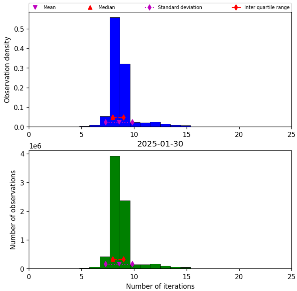
Figure 24: Histogram of “Number of iterations” for 2025-01-29 to 2025-01-31
