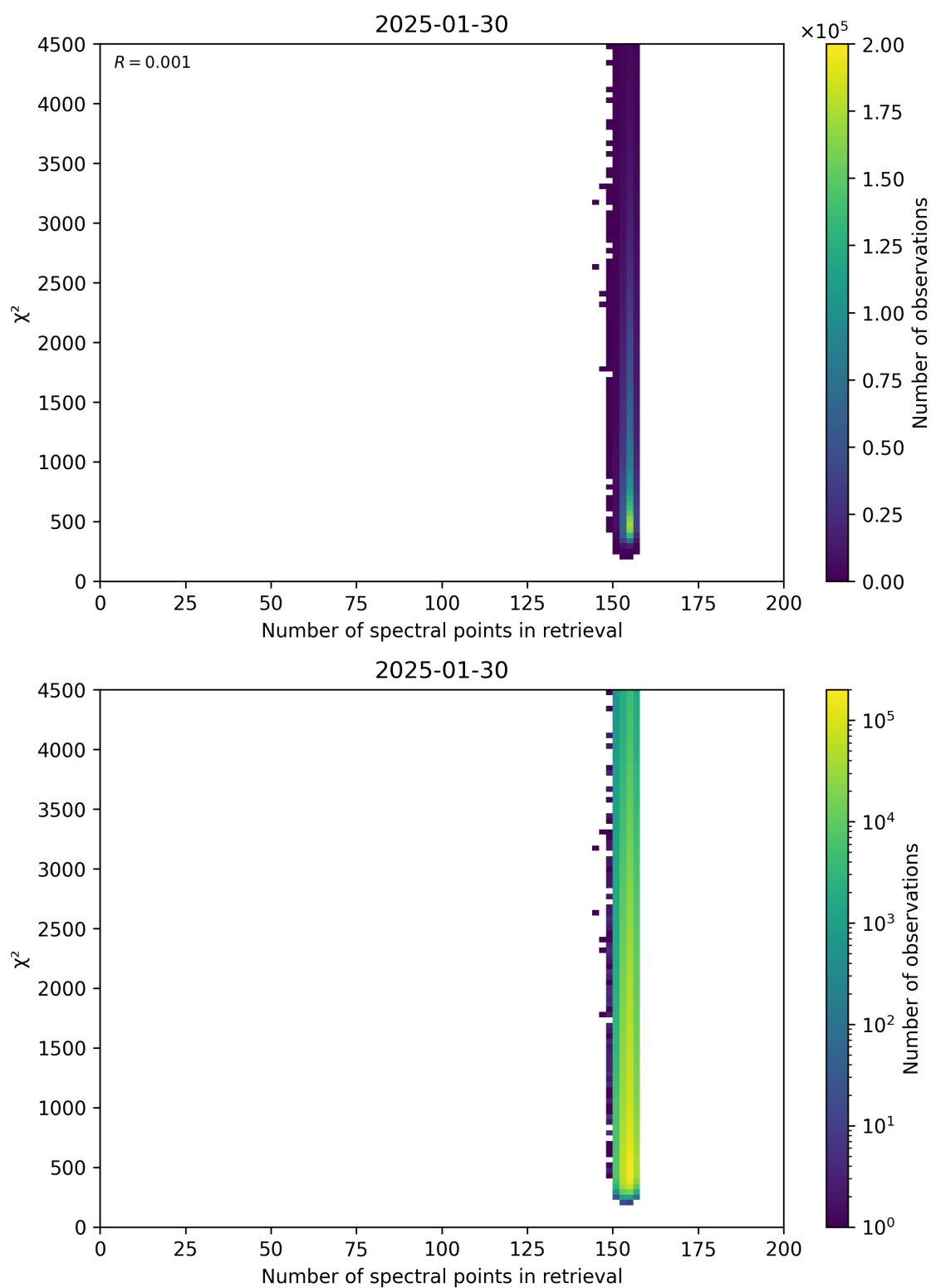
Figure 58: Scatter density plot of “Number of spectral points in retrieval” against “ \chi^2 ” for 2025-01-29 to 2025-01-31.
