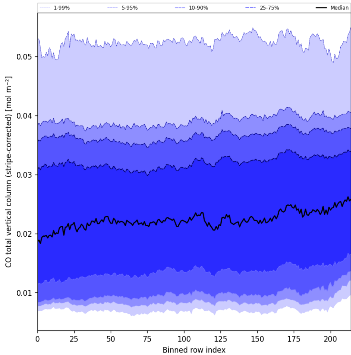
Figure 27: Along track statistics of “CO total vertical column (stripe-corrected)” for 2025-01-29 to 2025-01-31
