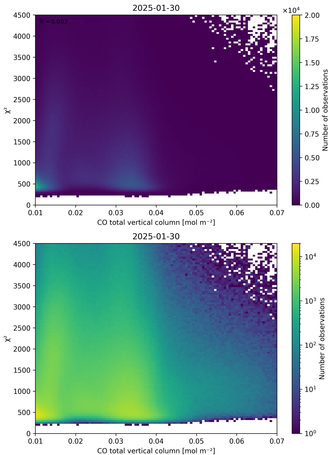
Figure 35: Scatter density plot of “CO total vertical column” against “ \chi^2 ” for 2025-01-29 to 2025-01-31.
