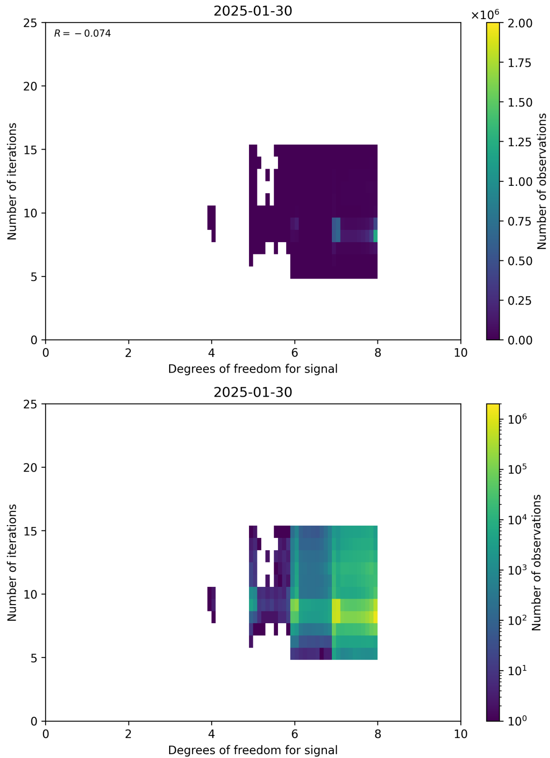
Figure 50: Scatter density plot of “Degrees of freedom for signal” against “Number of iterations” for 2025-01-29 to 2025-01-31.
