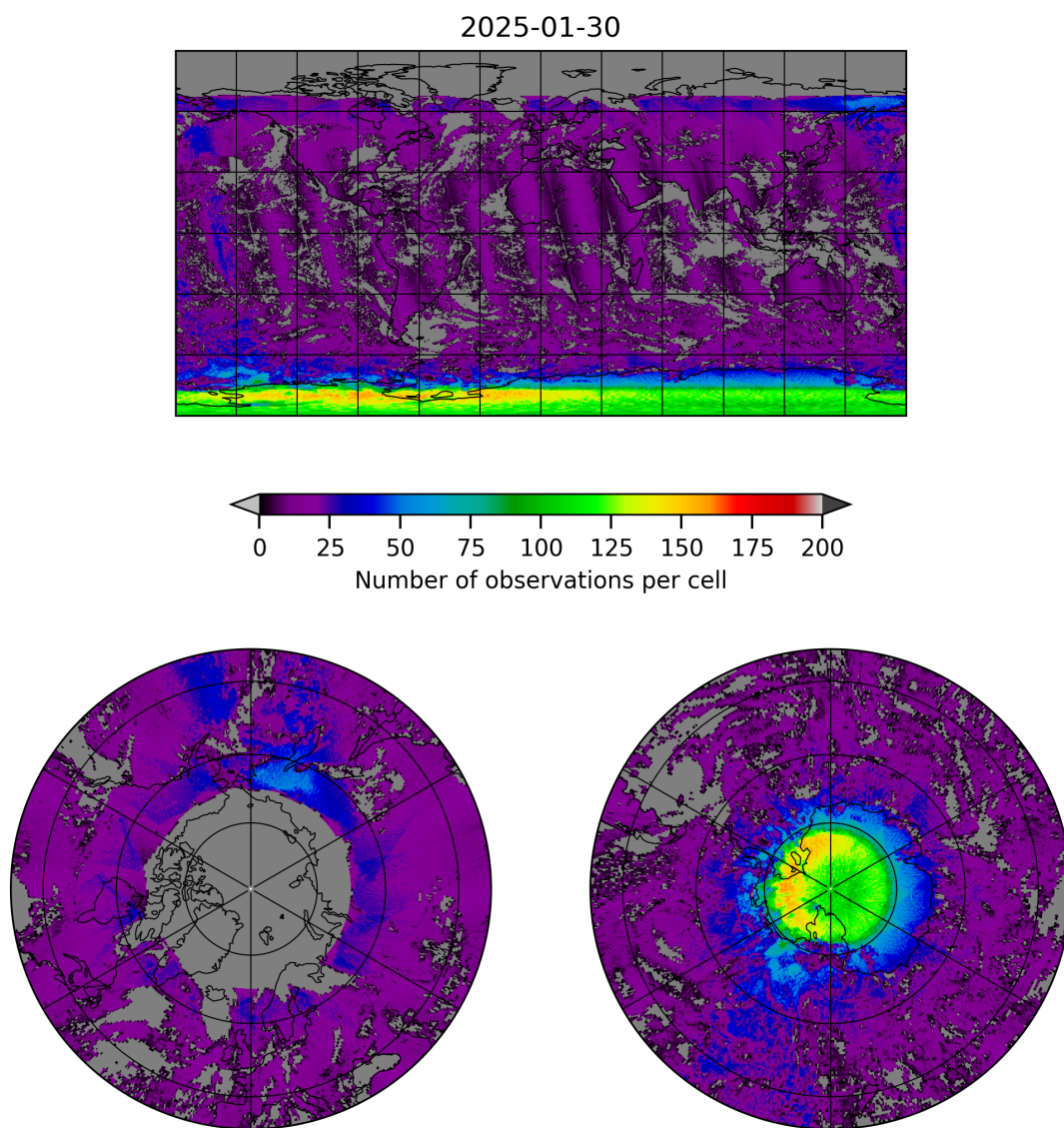
Figure 8: Map of the number of observations for 2025-01-29 to 2025-01-31
