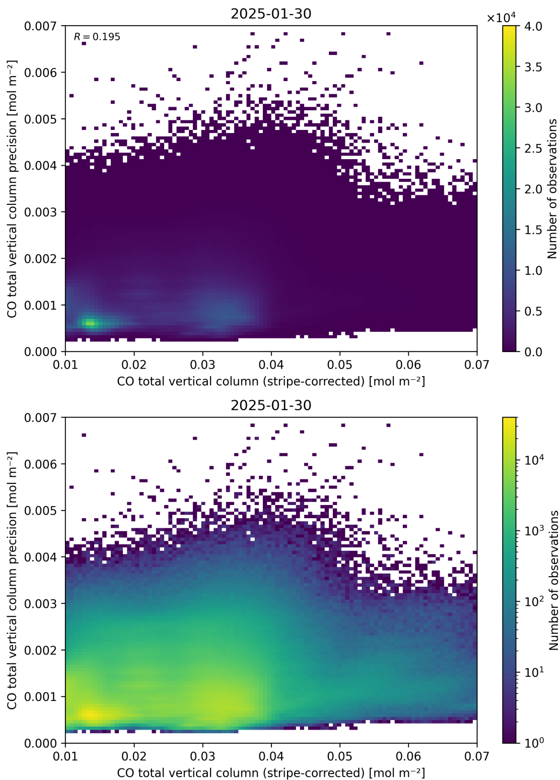
Figure 36: Scatter density plot of “CO total vertical column (stripe-corrected)” against “CO total vertical column precision” for 2025-01-29 to 2025-01-31.
