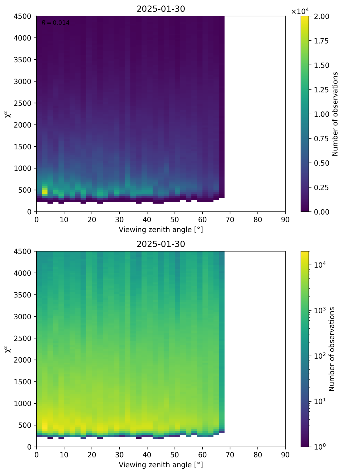
Figure 72: Scatter density plot of “Viewing zenith angle” against “ \chi^2 ” for 2025-01-29 to 2025-01-31.
