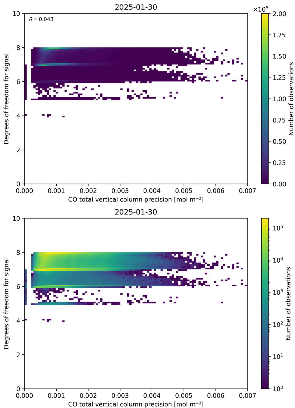
Figure 45: Scatter density plot of “CO total vertical column precision” against “Degrees of freedom for signal” for 2025-01-29 to 2025-01-31.
