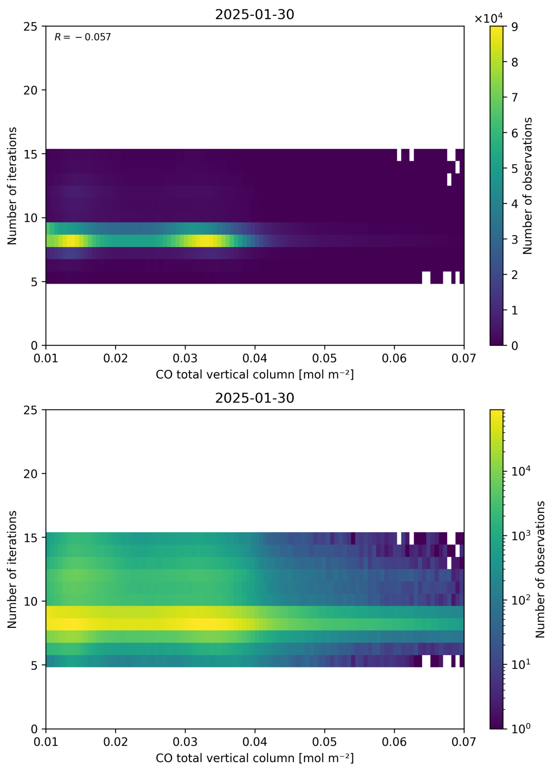
Figure 42: Scatter density plot of “CO total vertical column” against “Number of iterations” for 2025-01-29 to 2025-01-31.
