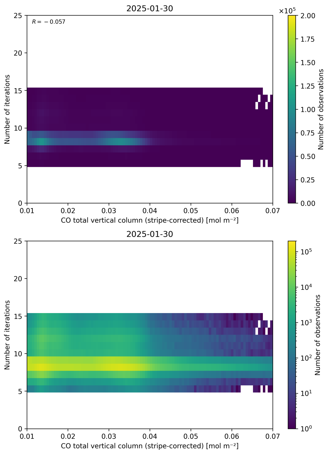
Figure 39: Scatter density plot of “CO total vertical column (stripe-corrected)” against “Number of iterations” for 2025-01-29 to 2025-01-31.
