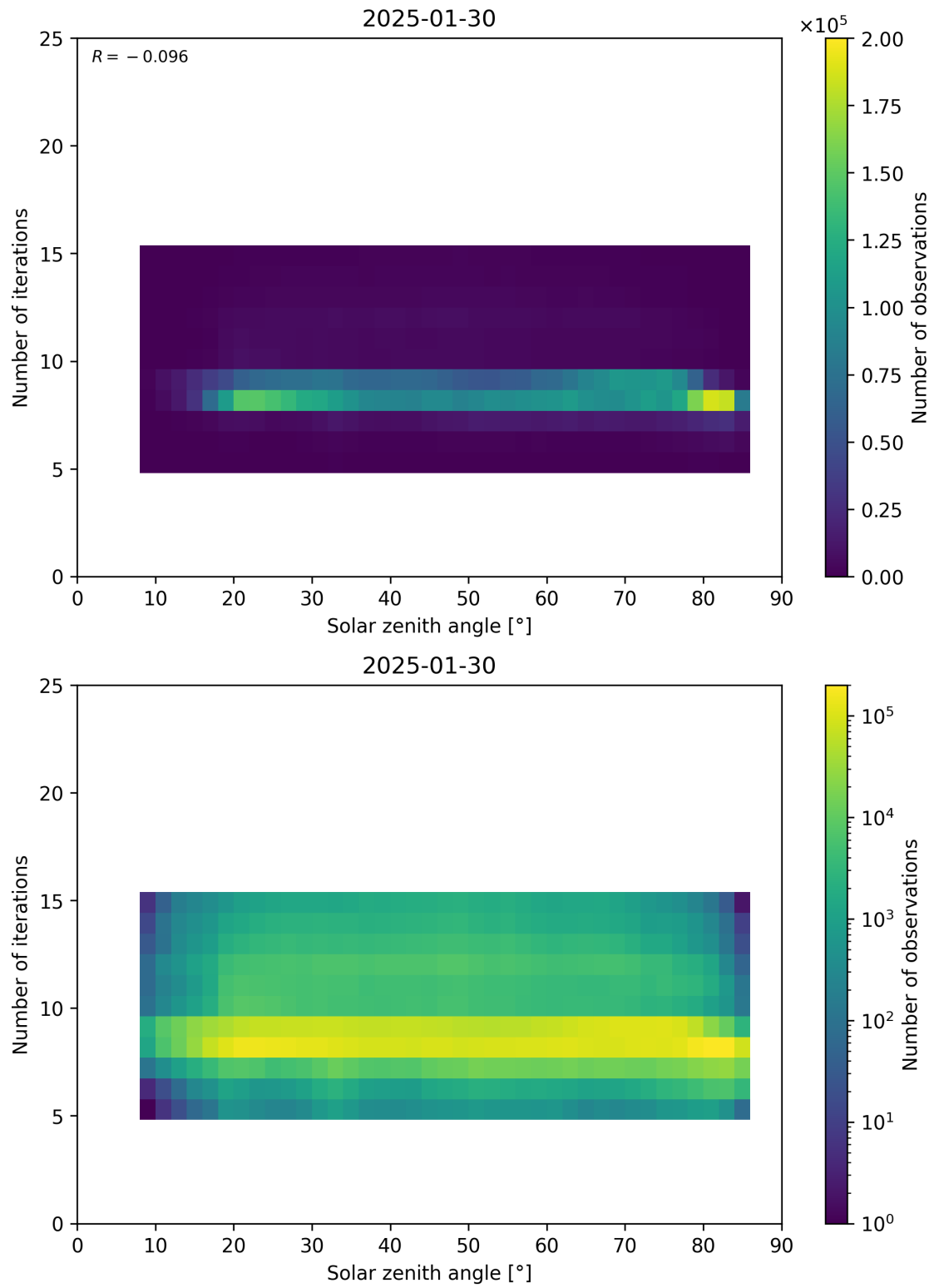
Figure 67: Scatter density plot of “Solar zenith angle” against “Number of iterations” for 2025-01-29 to 2025-01-31.
