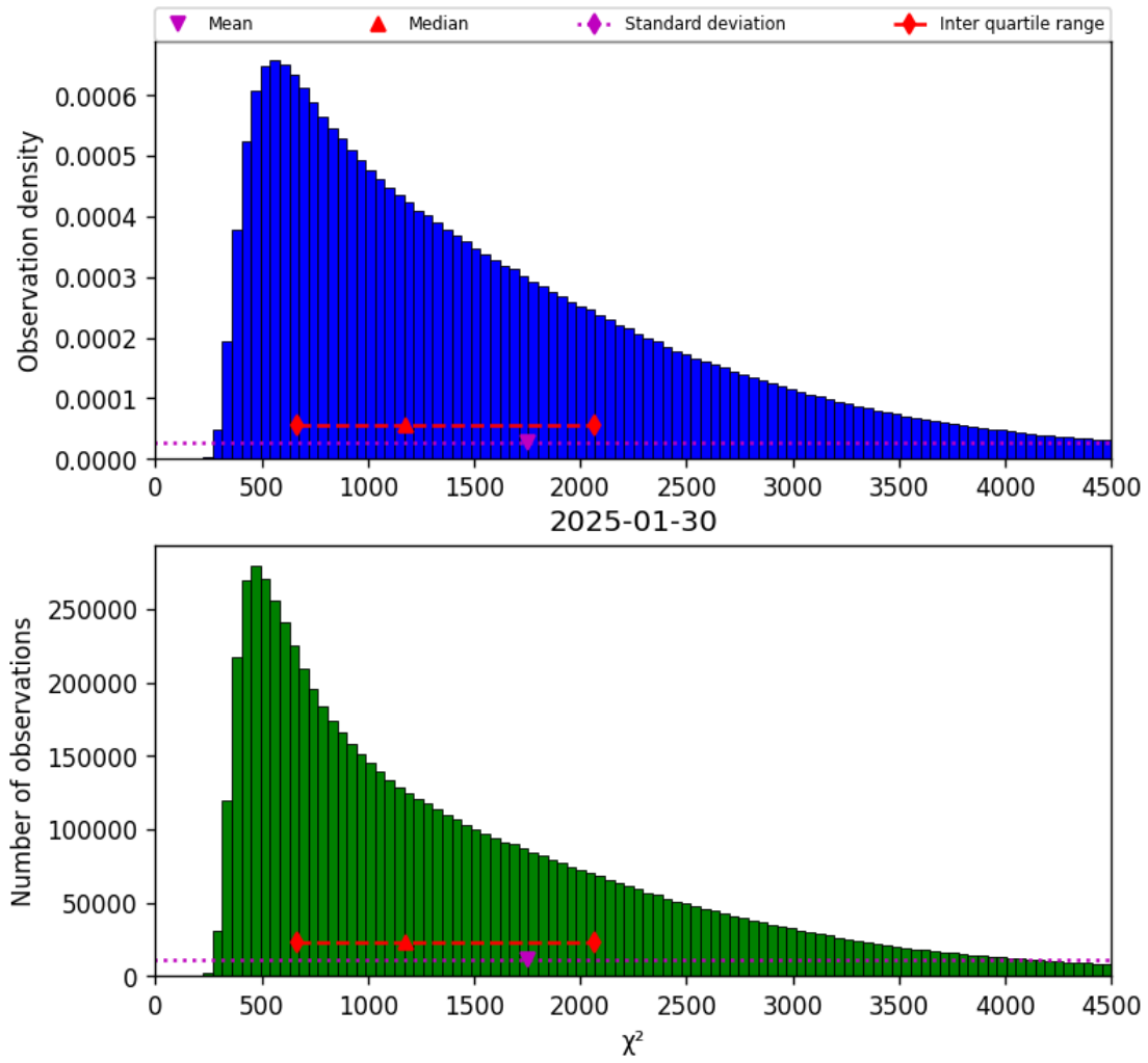
Figure 22: Histogram of “ \chi^2 ” for 2025-01-29 to 2025-01-31
