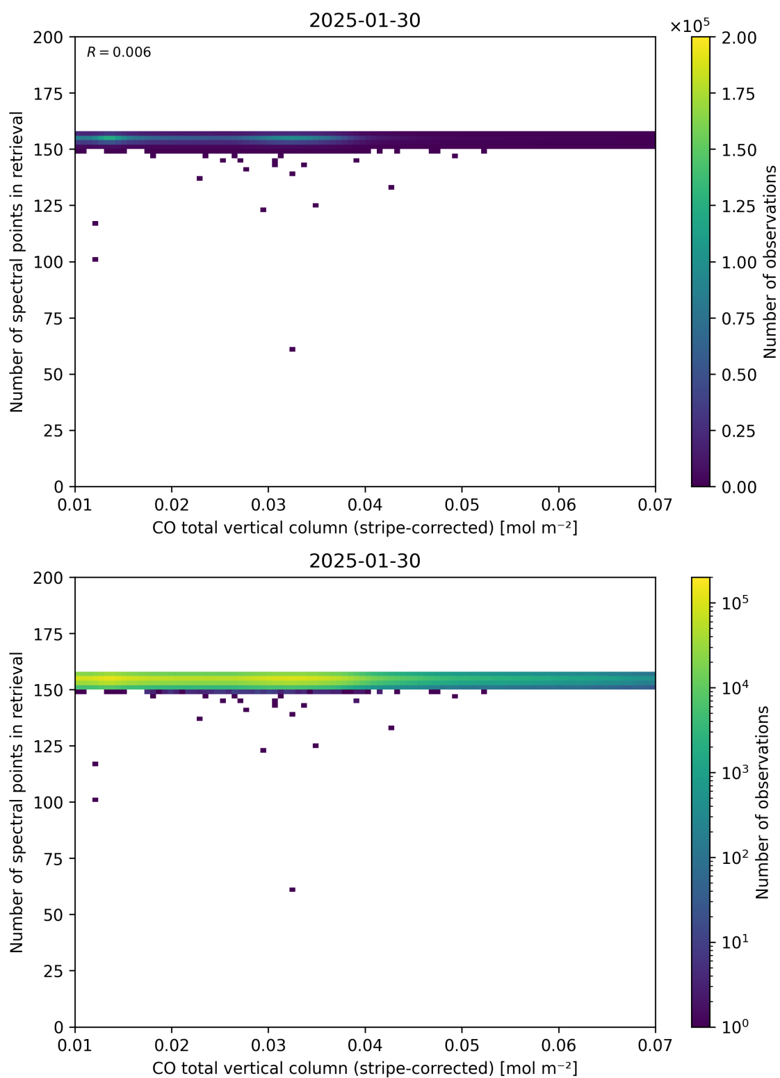
Figure 40: Scatter density plot of “CO total vertical column (stripe-corrected)” against “Number of spectral points in retrieval” for 2025-01-29 to 2025-01-31.
