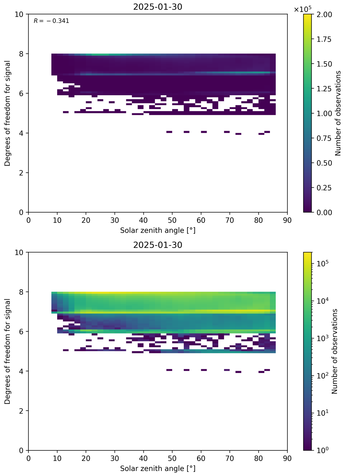
Figure 65: Scatter density plot of “Solar zenith angle” against “Degrees of freedom for signal” for 2025-01-29 to 2025-01-31.
