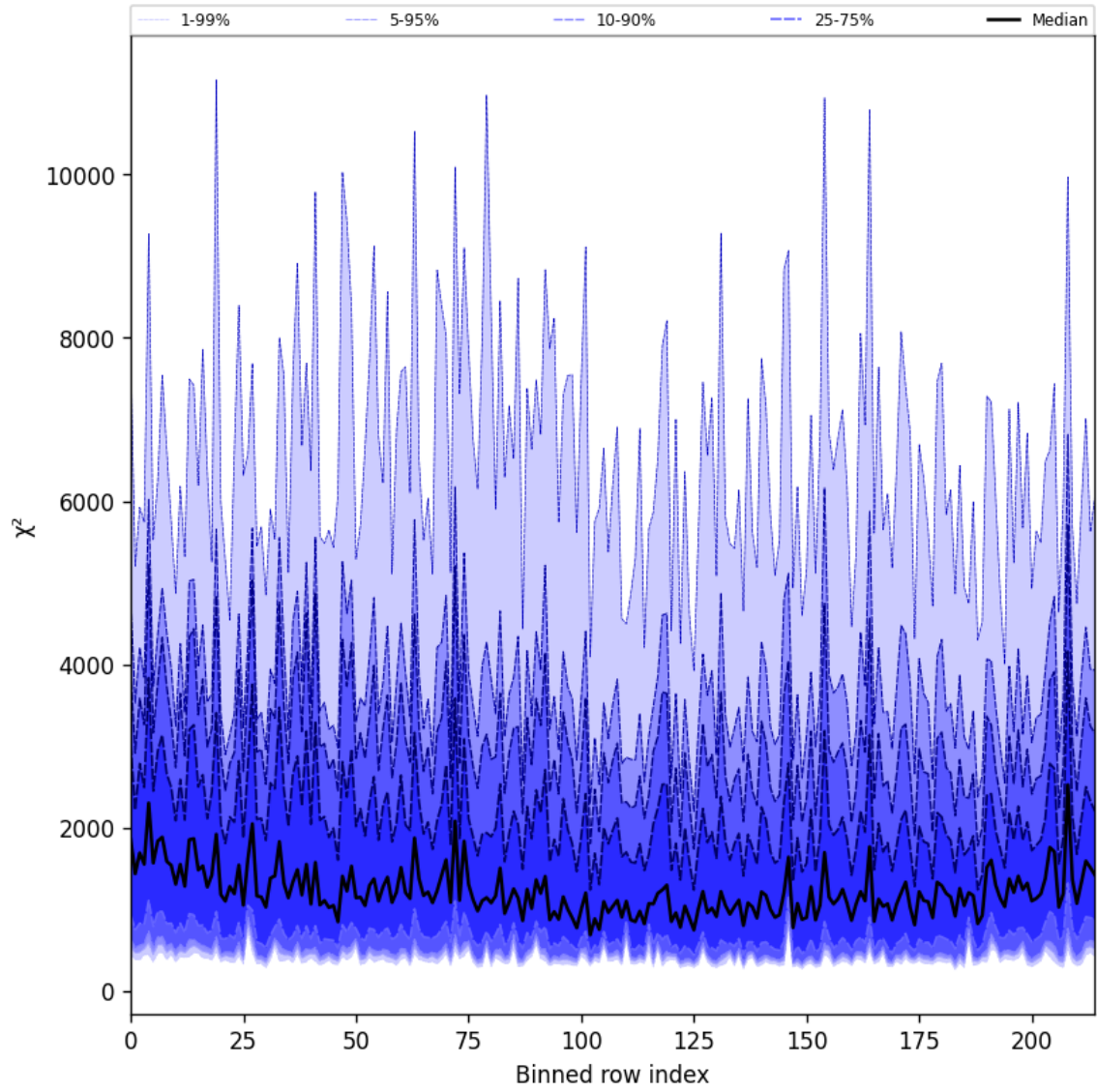
Figure 30: Along track statistics of “ \chi^2 ” for 2025-01-29 to 2025-01-31
