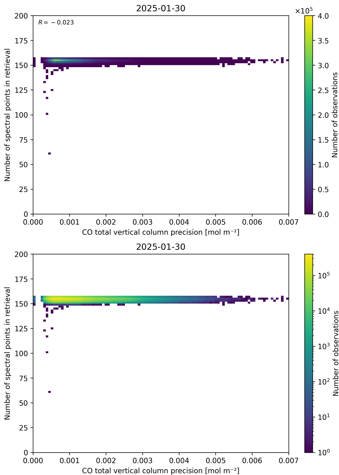
Figure 47: Scatter density plot of “CO total vertical column precision” against “Number of spectral points in retrieval” for 2025-01-29 to 2025-01-31.
