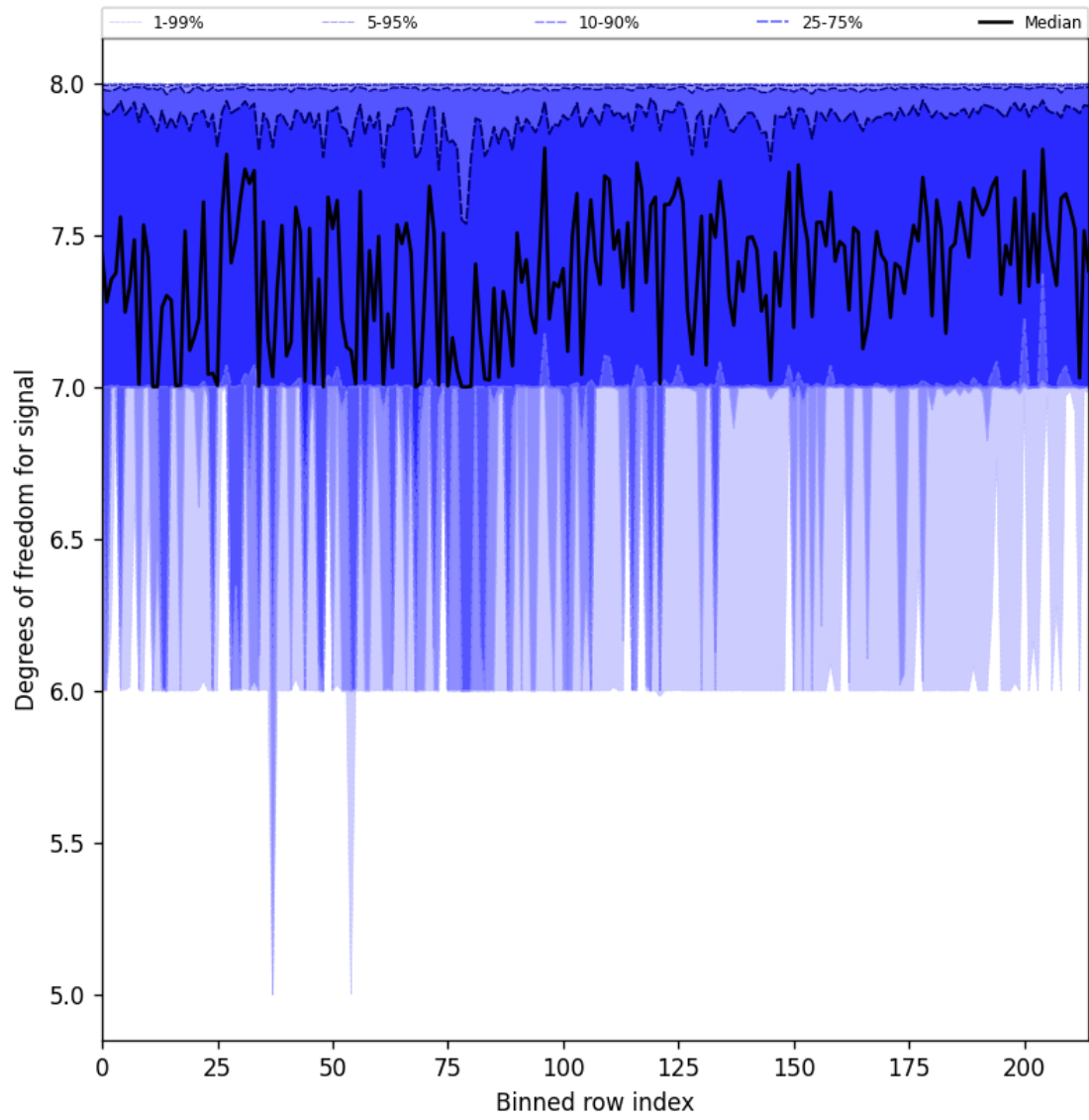
Figure 31: Along track statistics of “Degrees of freedom for signal” for 2025-01-29 to 2025-01-31
