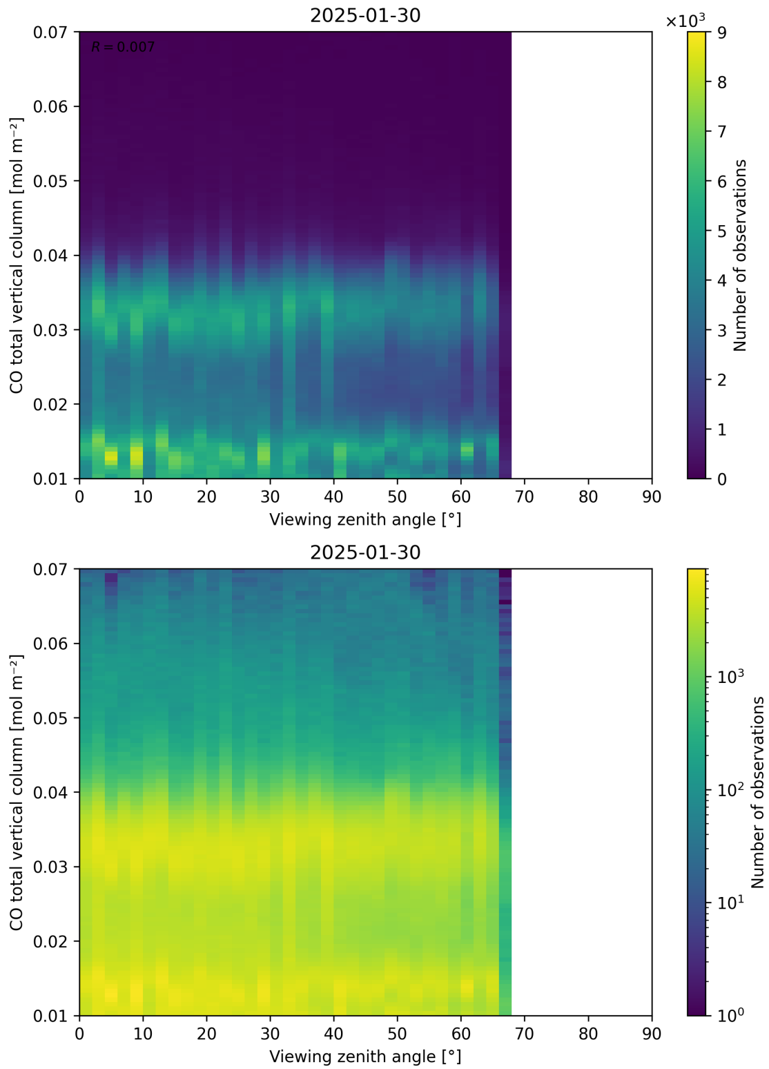
Figure 69: Scatter density plot of “Viewing zenith angle” against “CO total vertical column” for 2025-01-29 to 2025-01-31.
