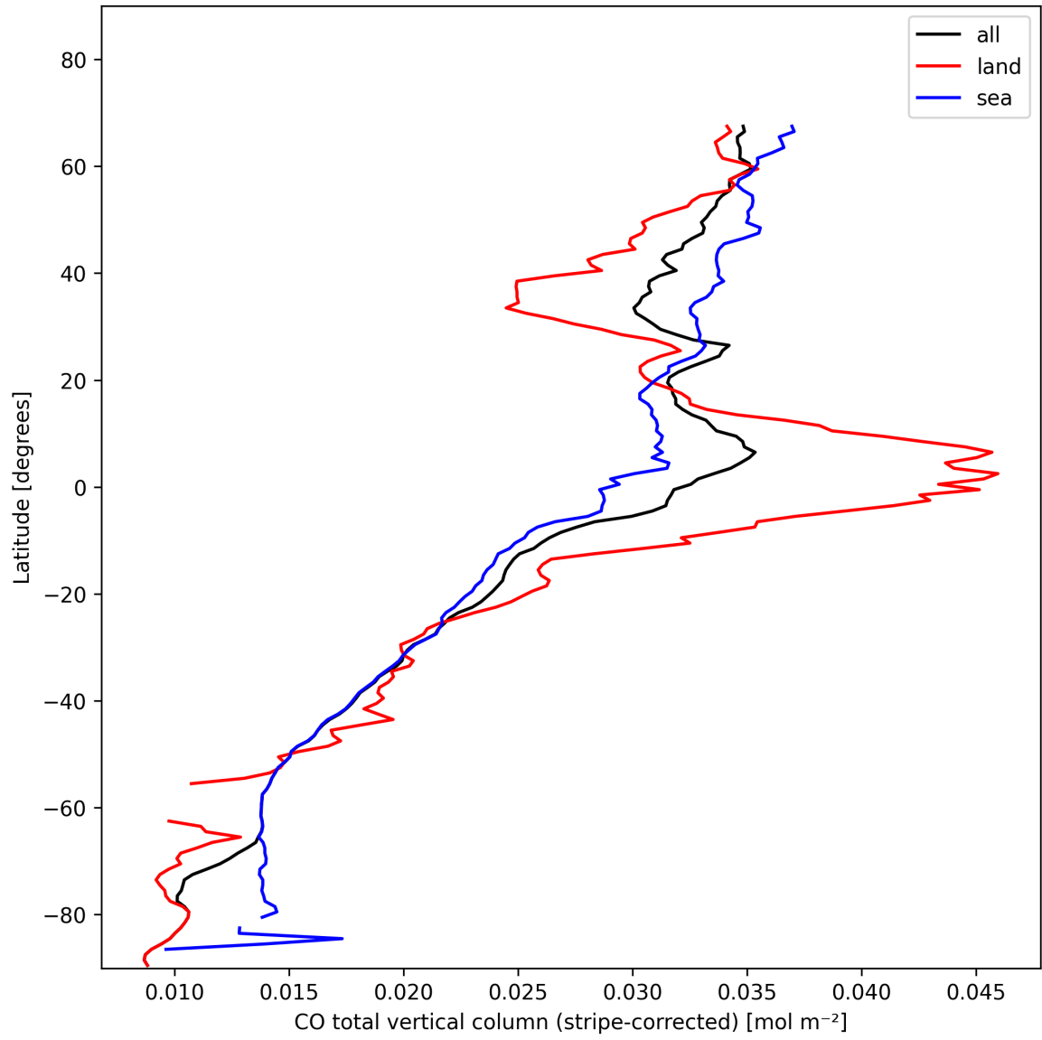
Figure 11: Zonal average of “CO total vertical column (stripe-corrected)” for 2025-01-29 to 2025-01-31.
