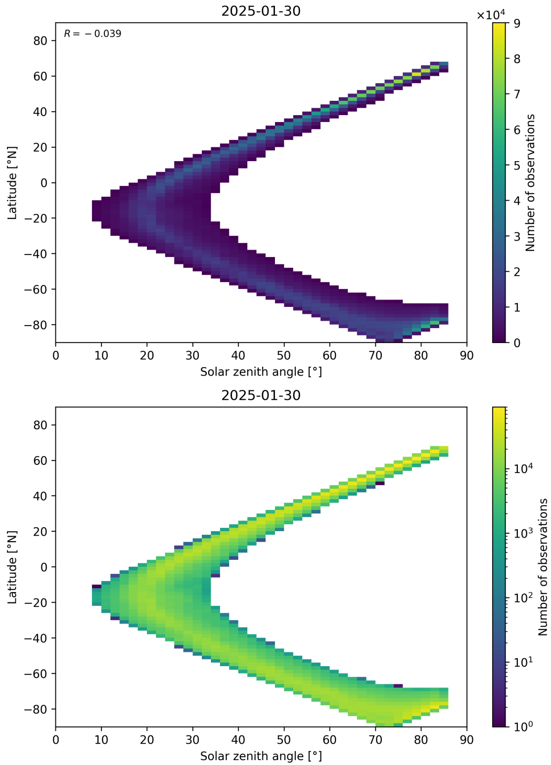
Figure 66: Scatter density plot of “Solar zenith angle” against “Latitude” for 2025-01-29 to 2025-01-31.
