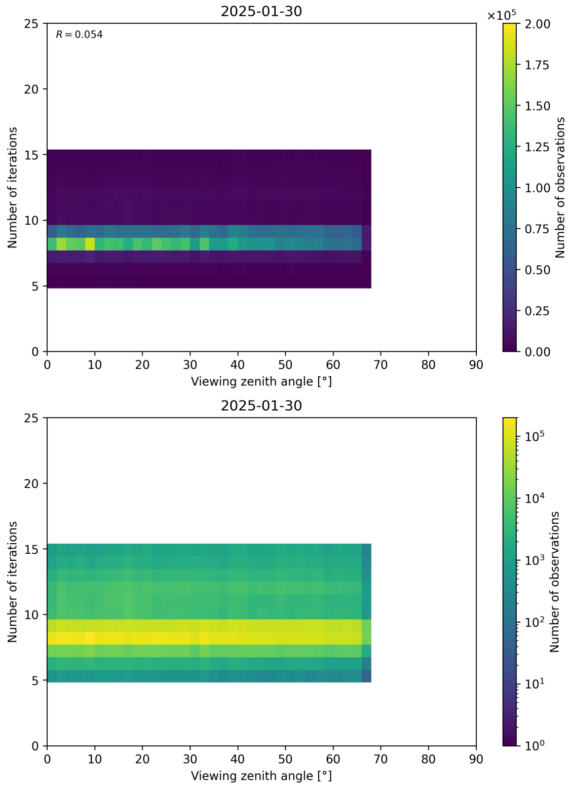
Figure 75: Scatter density plot of “Viewing zenith angle” against “Number of iterations” for 2025-01-29 to 2025-01-31.
