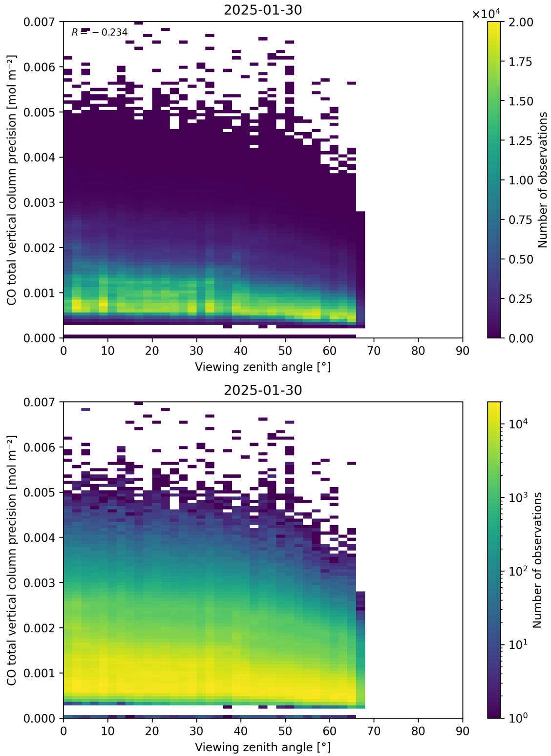
Figure 71: Scatter density plot of “Viewing zenith angle” against “CO total vertical column precision” for 2025-01-29 to 2025-01-31.
