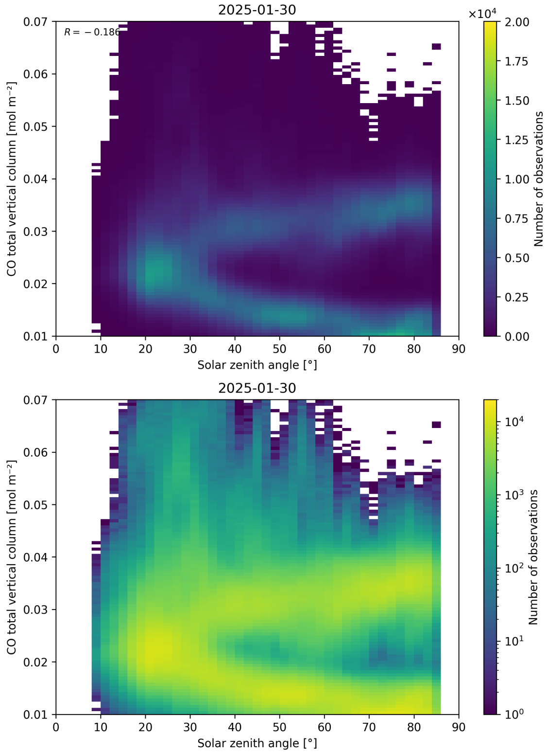
Figure 61: Scatter density plot of “Solar zenith angle” against “CO total vertical column” for 2025-01-29 to 2025-01-31.
