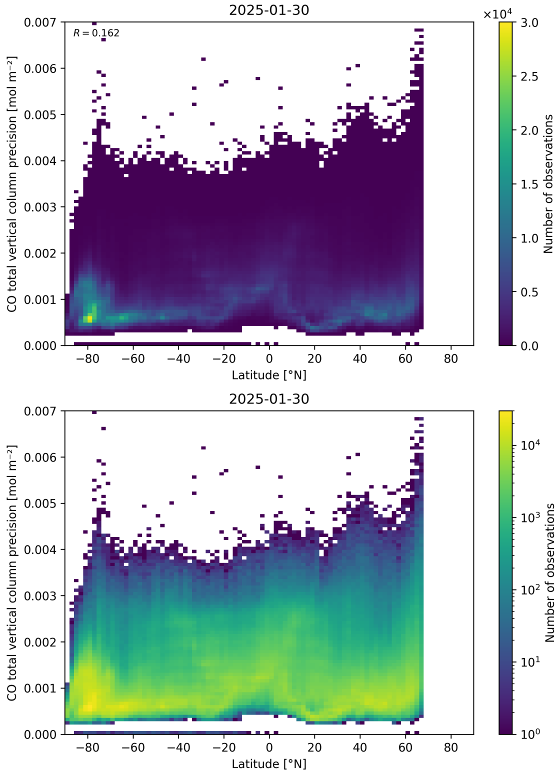
Figure 53: Scatter density plot of “Latitude” against “CO total vertical column precision” for 2025-01-29 to 2025-01-31.
