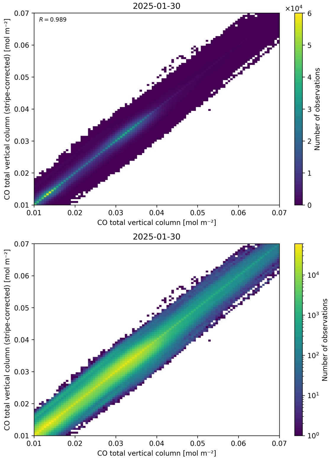
Figure 33: Scatter density plot of “CO total vertical column” against “CO total vertical column (stripe-corrected)” for 2025-01-29 to 2025-01-31.
