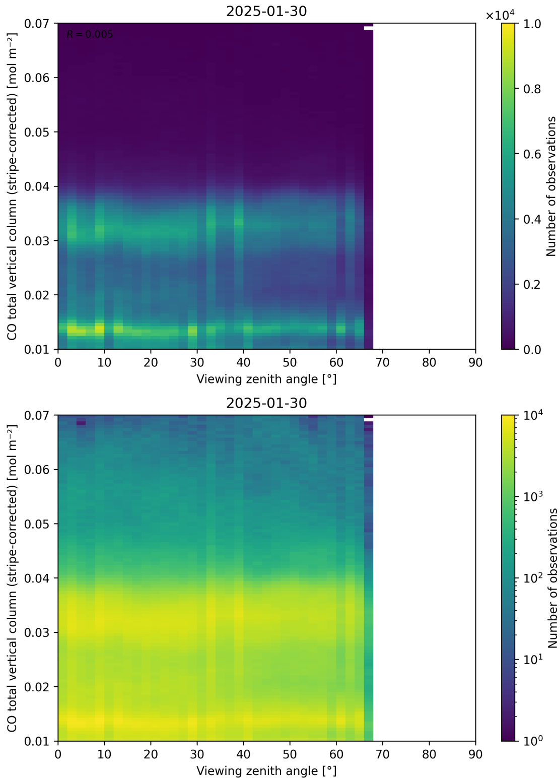
Figure 70: Scatter density plot of “Viewing zenith angle” against “CO total vertical column (stripe-corrected)” for 2025-01-29 to 2025-01-31.
