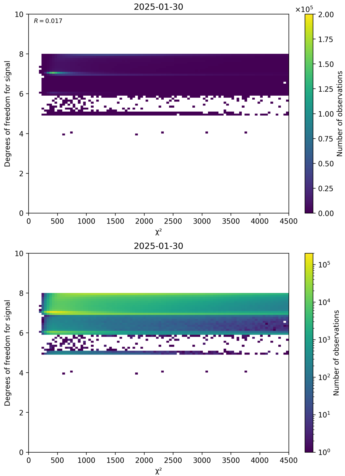
Figure 48: Scatter density plot of “ \chi^2 ” against “Degrees of freedom for signal” for 2025-01-29 to 2025-01-31.
