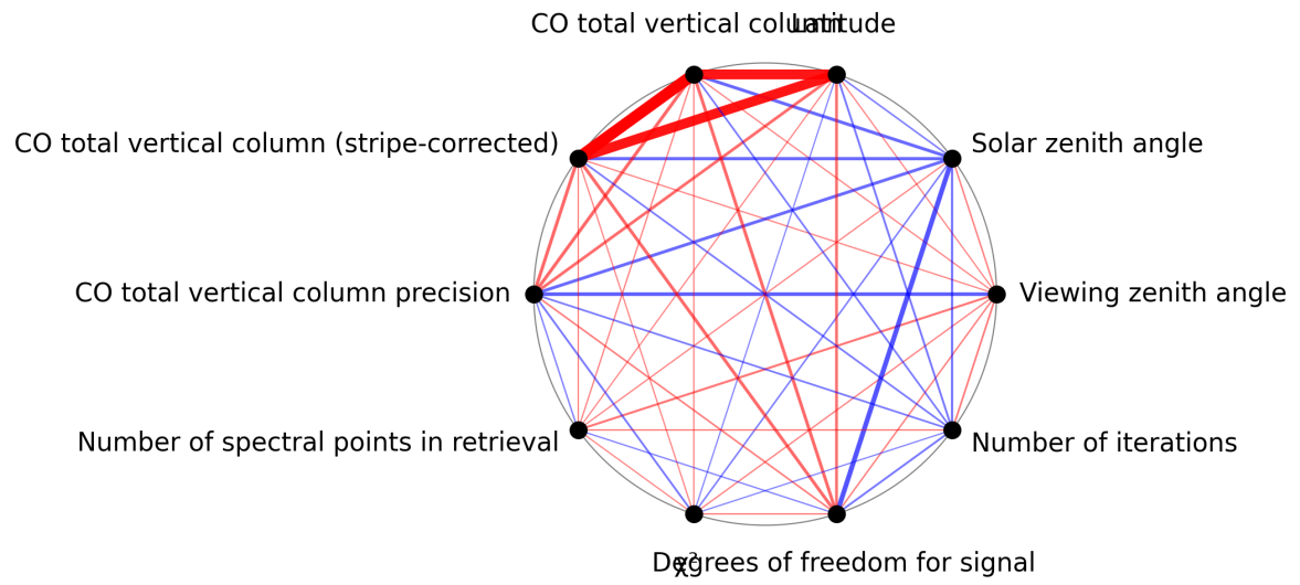
Figure 1: Map of correlation graph for 2025-01-29 to 2025-01-31.
