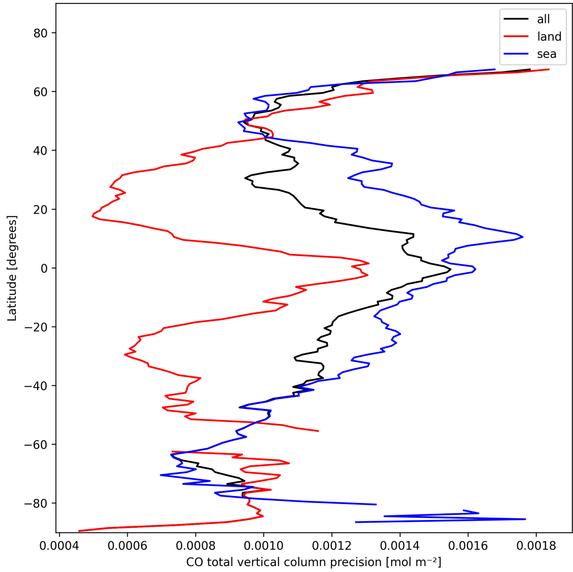
Figure 12: Zonal average of “CO total vertical column precision” for 2025-01-29 to 2025-01-31.
