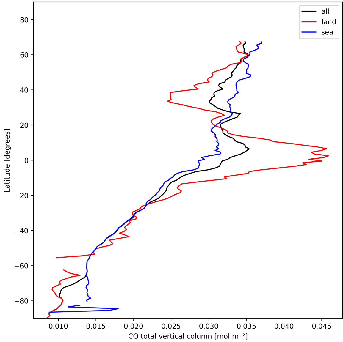
Figure 10: Zonal average of “CO total vertical column” for 2025-01-29 to 2025-01-31.
