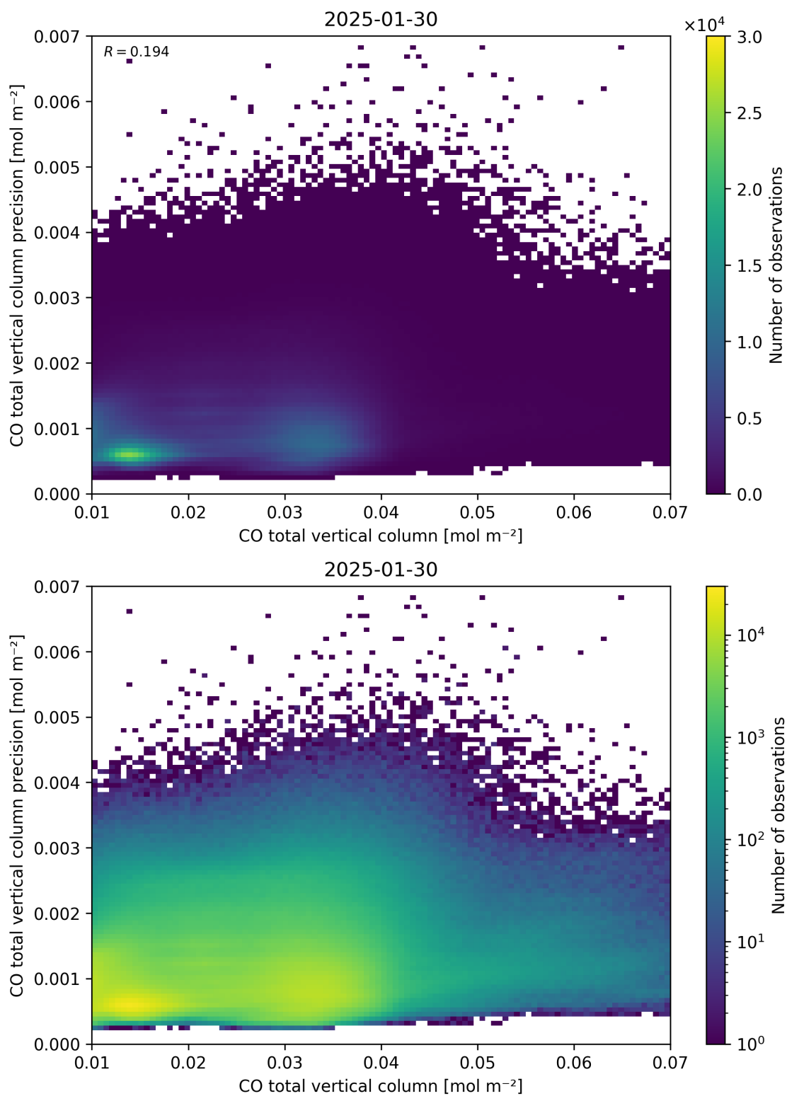
Figure 34: Scatter density plot of “CO total vertical column” against “CO total vertical column precision” for 2025-01-29 to 2025-01-31.
