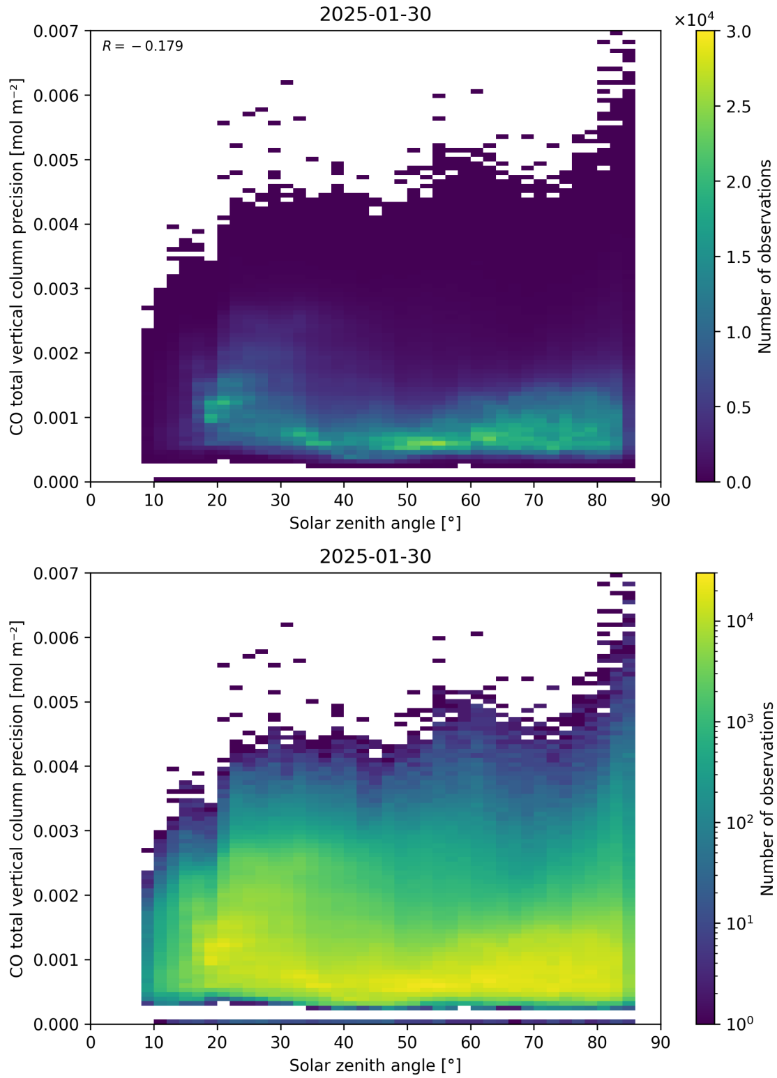
Figure 63: Scatter density plot of “Solar zenith angle” against “CO total vertical column precision” for 2025-01-29 to 2025-01-31.
