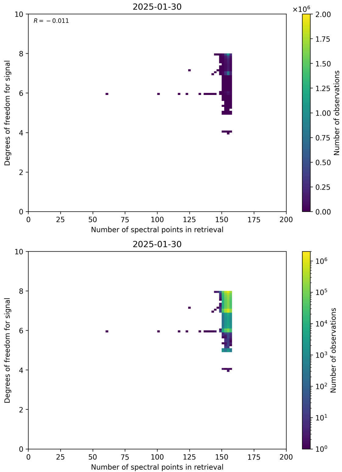
Figure 59: Scatter density plot of “Number of spectral points in retrieval” against “Degrees of freedom for signal” for 2025-01-29 to 2025-01-31.
