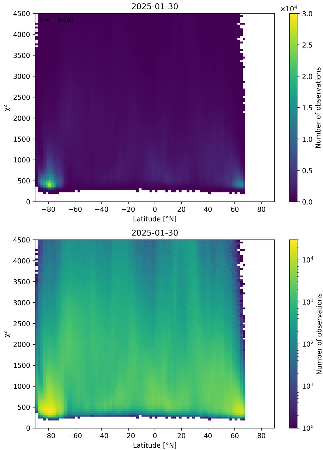
Figure 54: Scatter density plot of “Latitude” against “ \chi^2 ” for 2025-01-29 to 2025-01-31.
