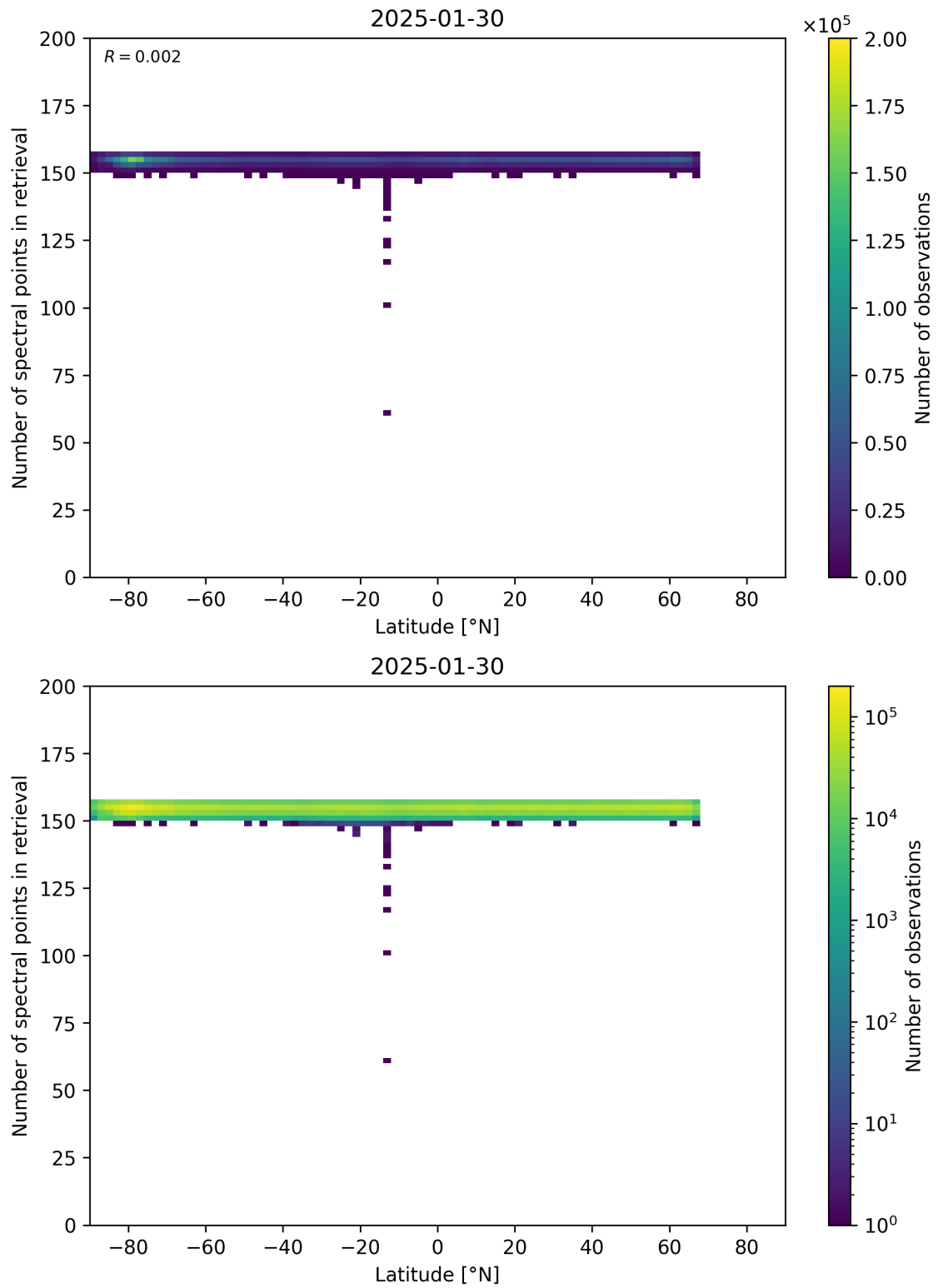
Figure 57: Scatter density plot of “Latitude” against “Number of spectral points in retrieval” for 2025-01-29 to 2025-01-31.
