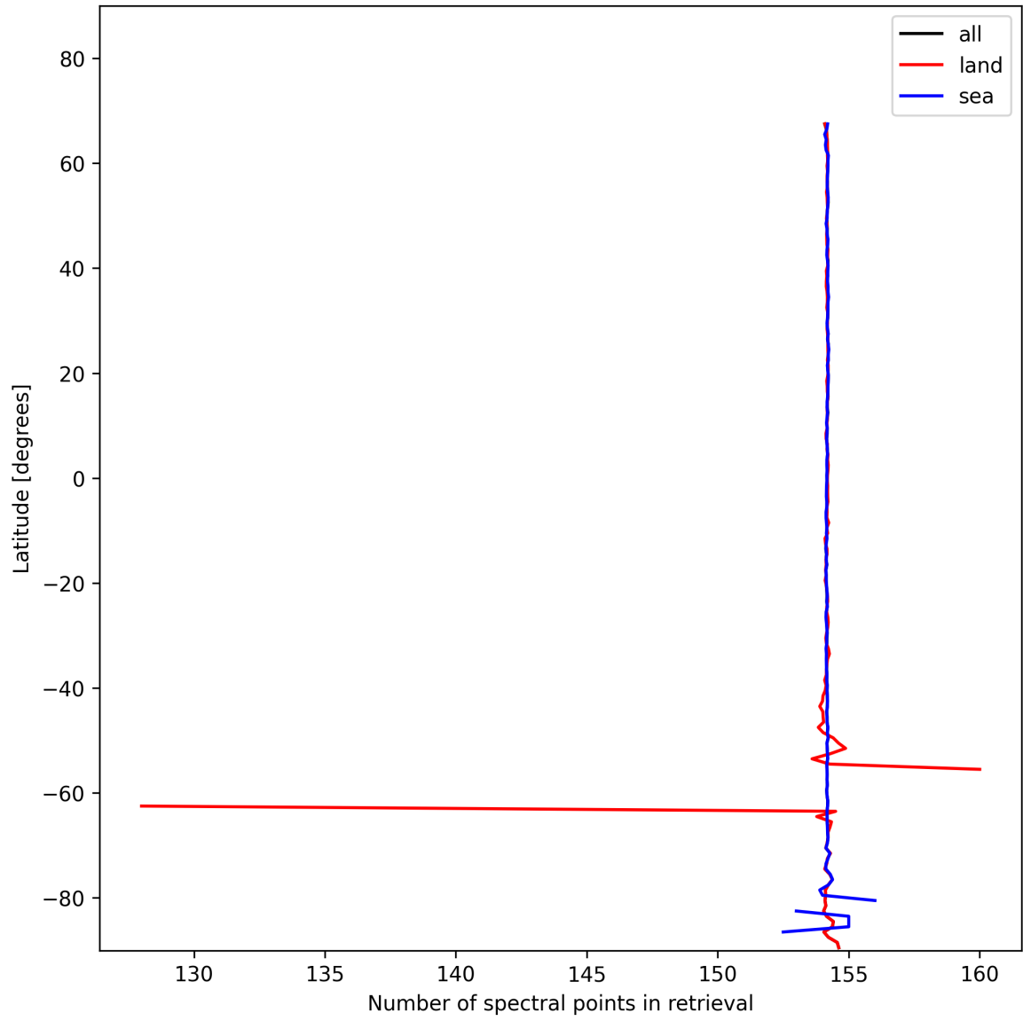
Figure 13: Zonal average of “Number of spectral points in retrieval” for 2025-01-29 to 2025-01-31.
