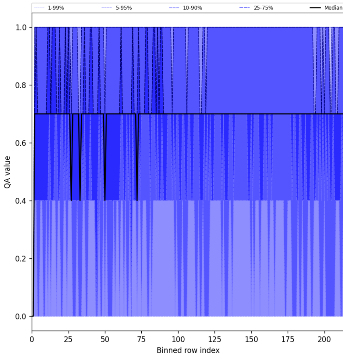
Figure 25: Along track statistics of “QA value” for 2025-01-29 to 2025-01-31
