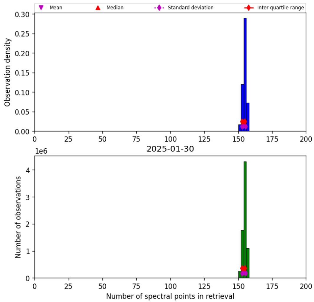
Figure 21: Histogram of “Number of spectral points in retrieval” for 2025-01-29 to 2025-01-31
