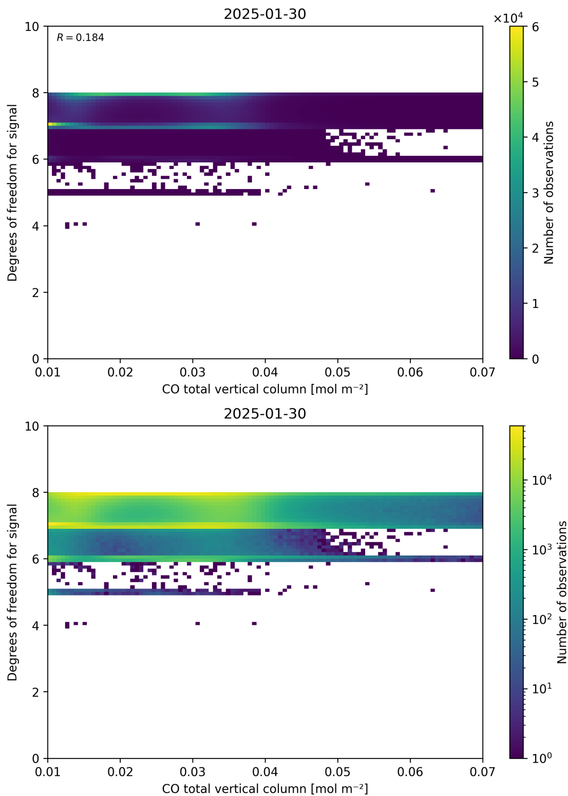
Figure 41: Scatter density plot of “CO total vertical column” against “Degrees of freedom for signal” for 2025-01-29 to 2025-01-31.
