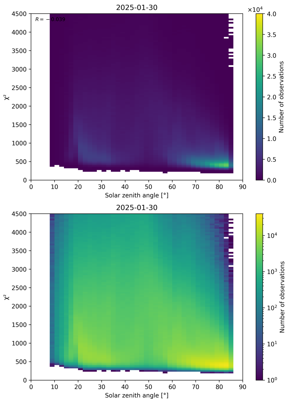
Figure 64: Scatter density plot of “Solar zenith angle” against “ \chi^2 ” for 2025-01-29 to 2025-01-31.
