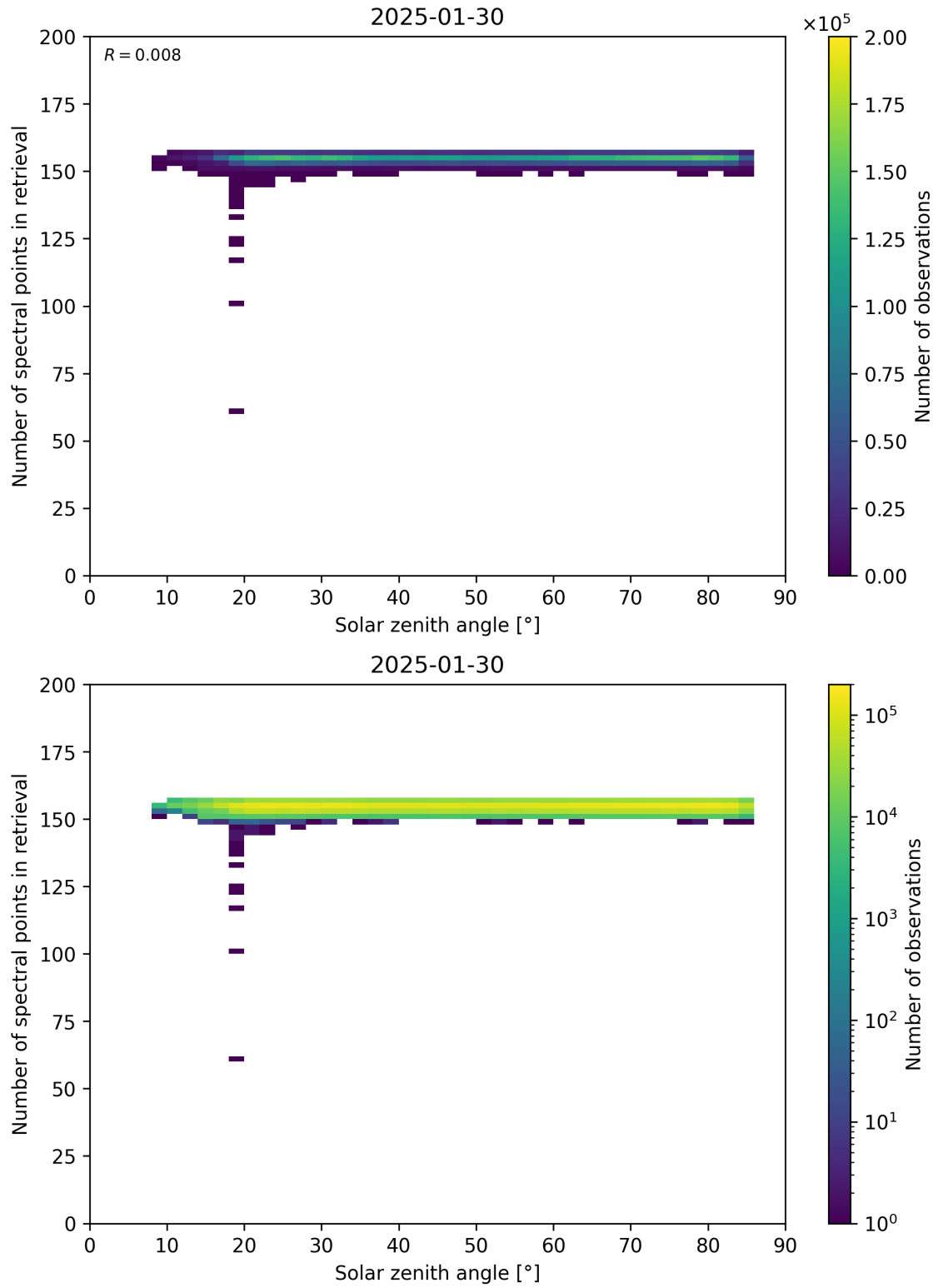
Figure 68: Scatter density plot of “Solar zenith angle” against “Number of spectral points in retrieval” for 2025-01-29 to 2025-01-31.
