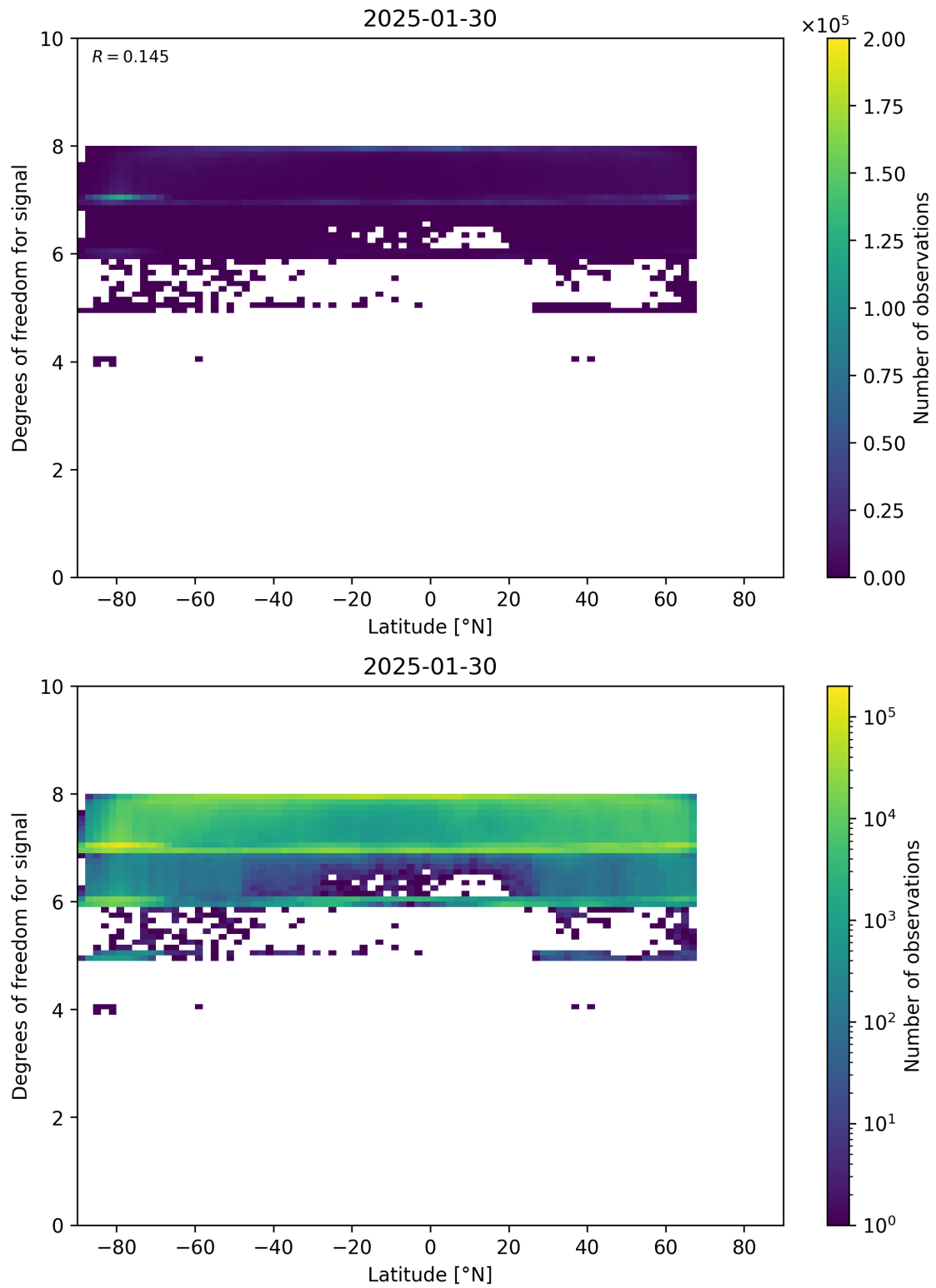
Figure 55: Scatter density plot of “Latitude” against “Degrees of freedom for signal” for 2025-01-29 to 2025-01-31.
