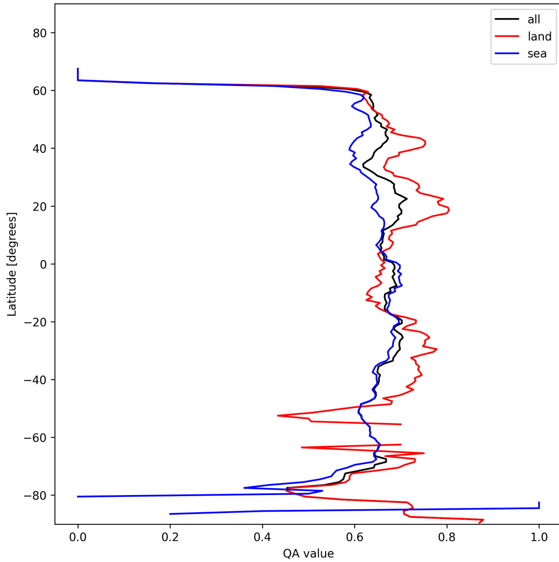
Figure 9: Zonal average of “QA value” for 2025-01-29 to 2025-01-31.
