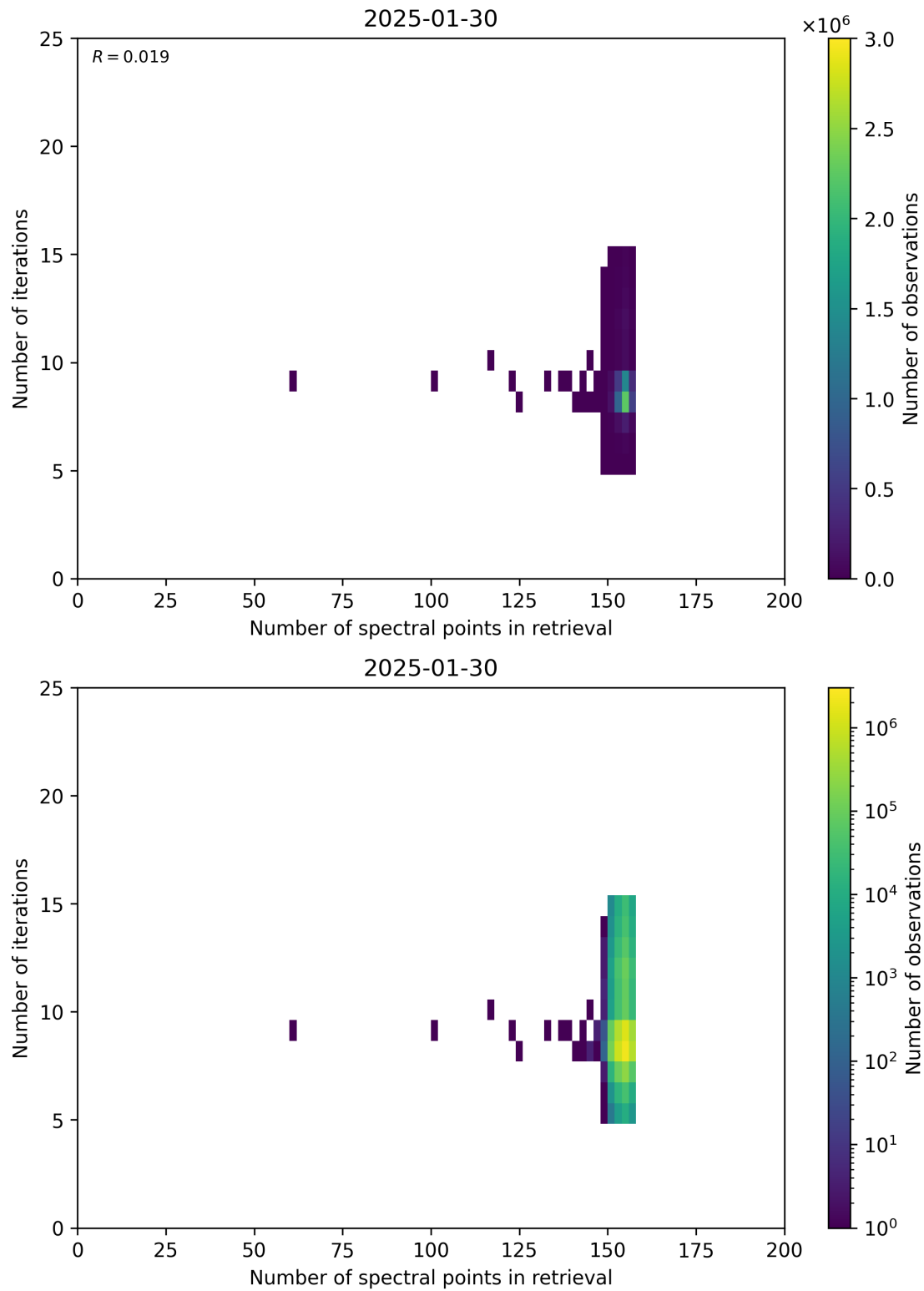
Figure 60: Scatter density plot of “Number of spectral points in retrieval” against “Number of iterations” for 2025-01-29 to 2025-01-31.
