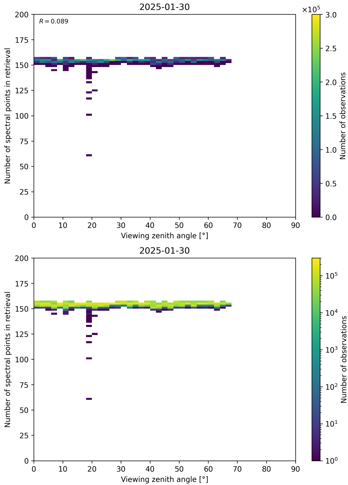
Figure 76: Scatter density plot of “Viewing zenith angle” against “Number of spectral points in retrieval” for 2025-01-29 to 2025-01-31.
