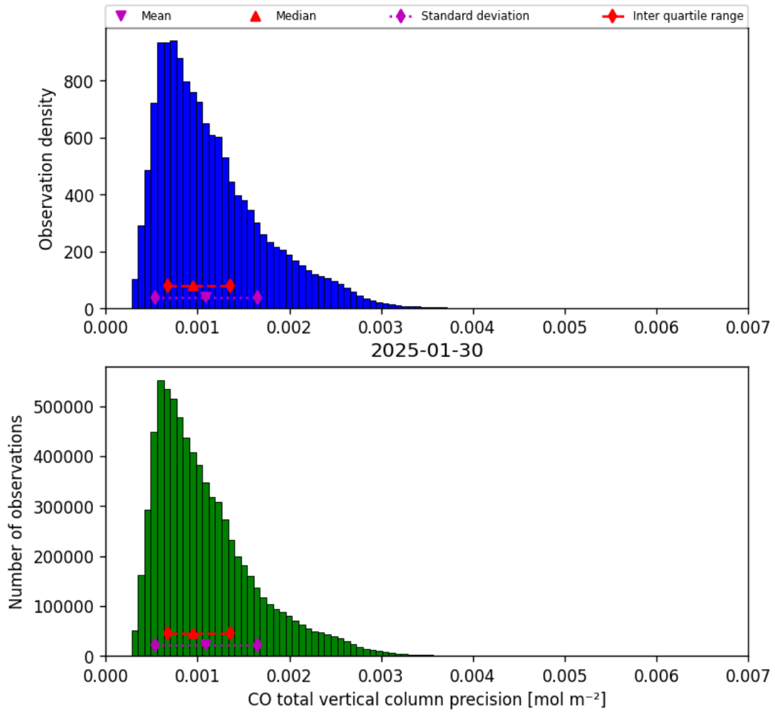
Figure 20: Histogram of “CO total vertical column precision” for 2025-01-29 to 2025-01-31
