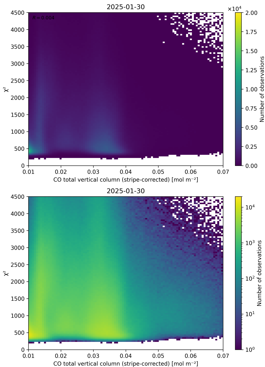
Figure 37: Scatter density plot of “CO total vertical column (stripe-corrected)” against “ \chi^2 ” for 2025-01-29 to 2025-01-31.
