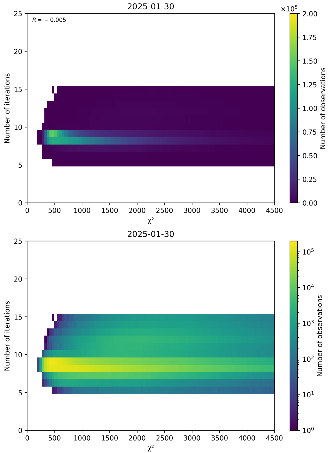
Figure 49: Scatter density plot of “ \chi^2 ” against “Number of iterations” for 2025-01-29 to 2025-01-31.
