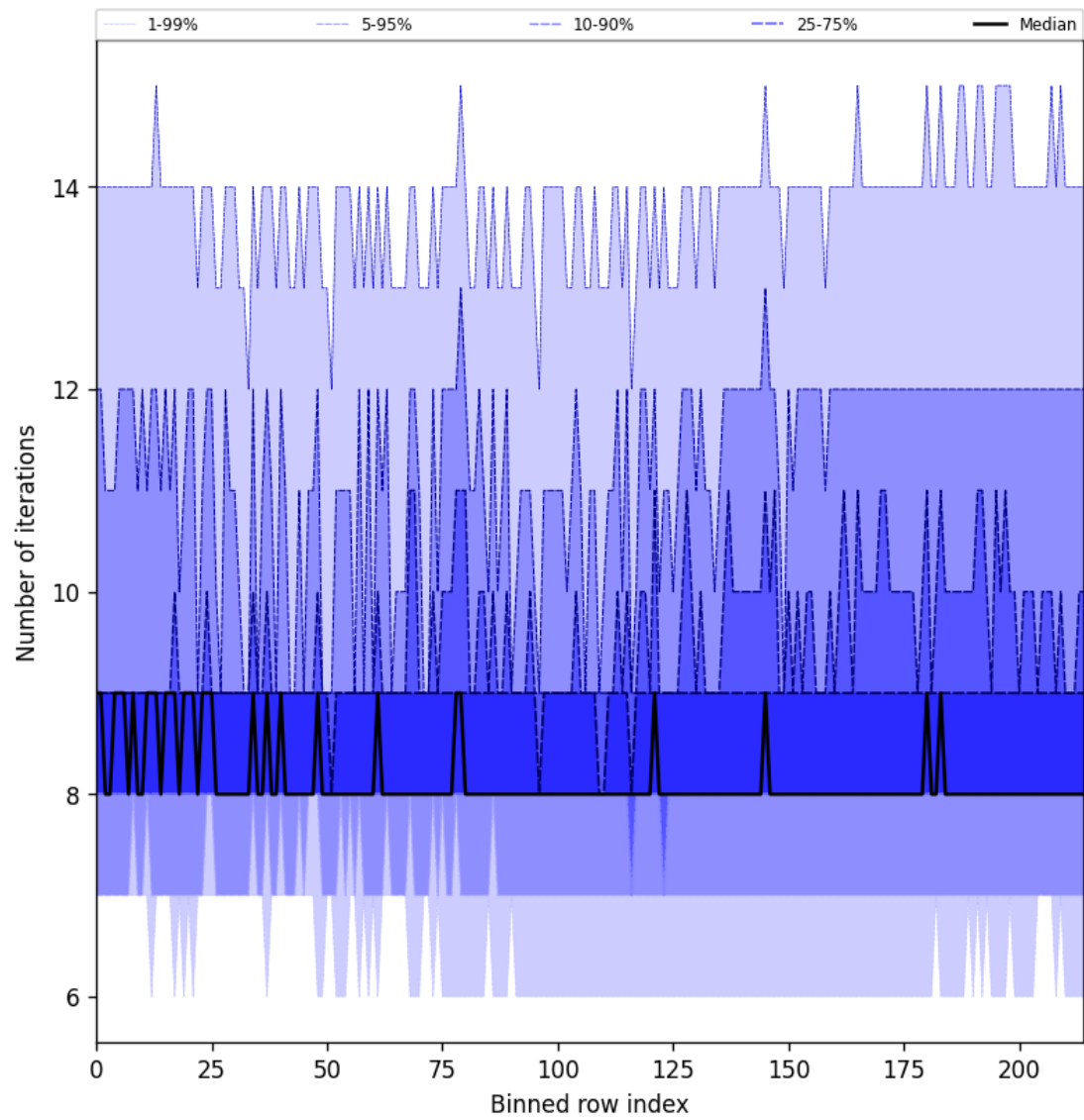
Figure 32: Along track statistics of “Number of iterations” for 2025-01-29 to 2025-01-31
