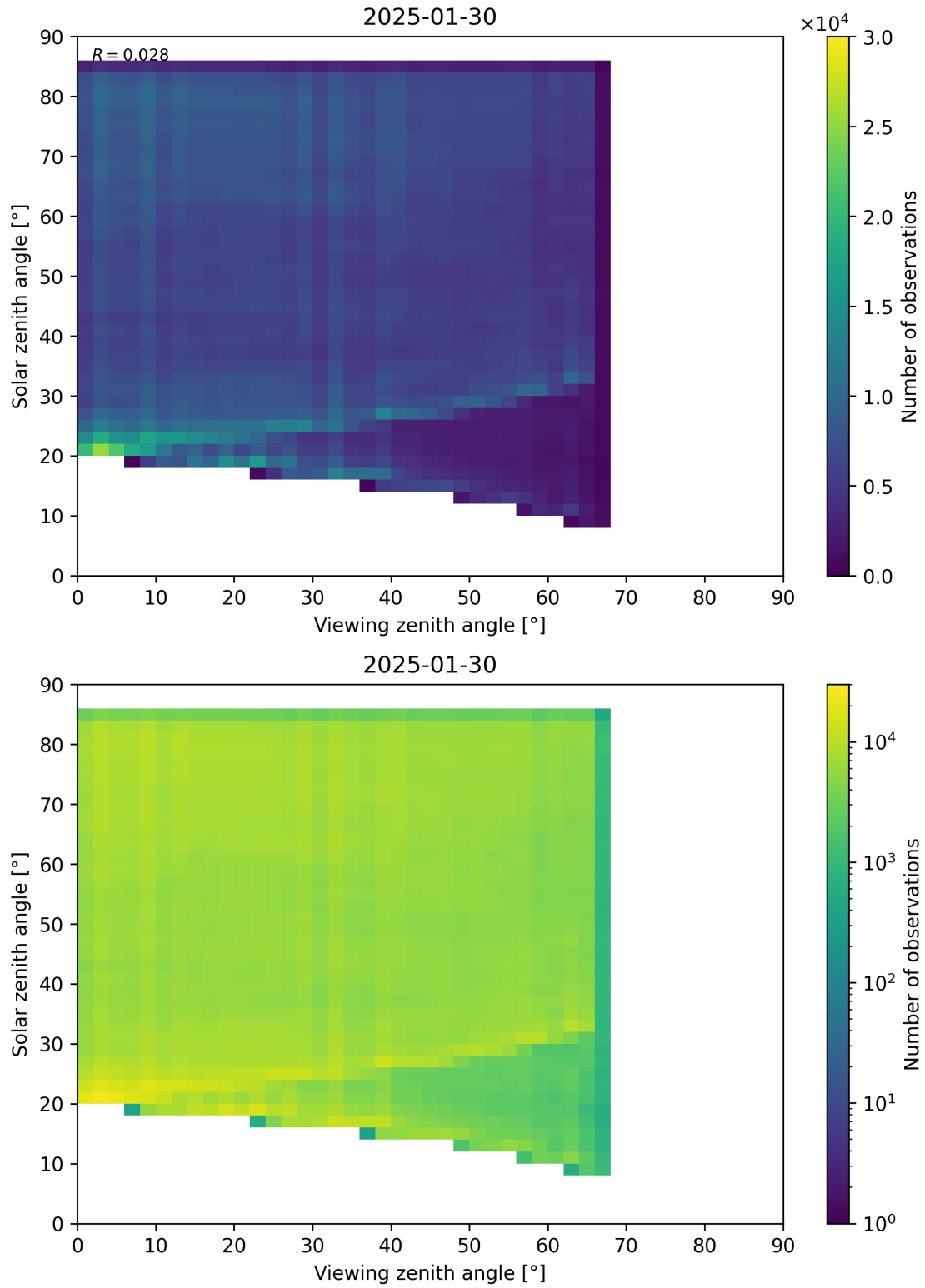
Figure 77: Scatter density plot of “Viewing zenith angle” against “Solar zenith angle” for 2025-01-29 to 2025-01-31.
