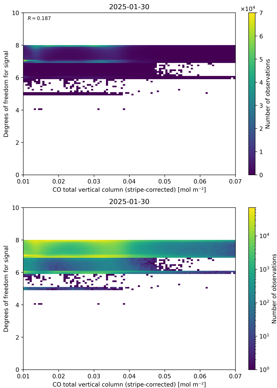
Figure 38: Scatter density plot of “CO total vertical column (stripe-corrected)” against “Degrees of freedom for signal” for 2025-01-29 to 2025-01-31.
