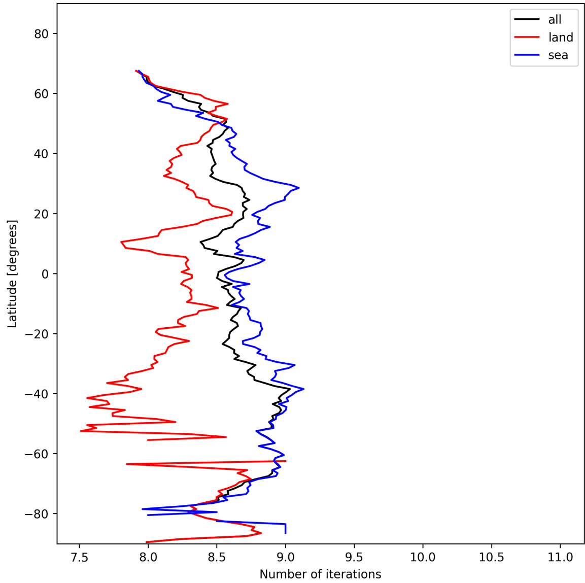
Figure 16: Zonal average of “Number of iterations” for 2025-01-29 to 2025-01-31.
