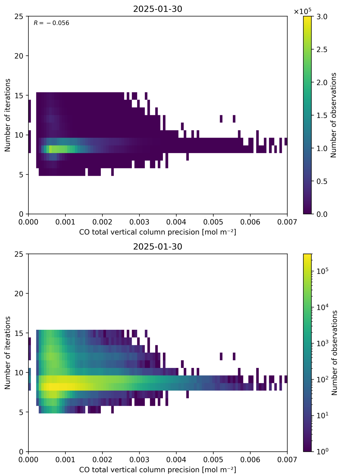
Figure 46: Scatter density plot of “CO total vertical column precision” against “Number of iterations” for 2025-01-29 to 2025-01-31.
