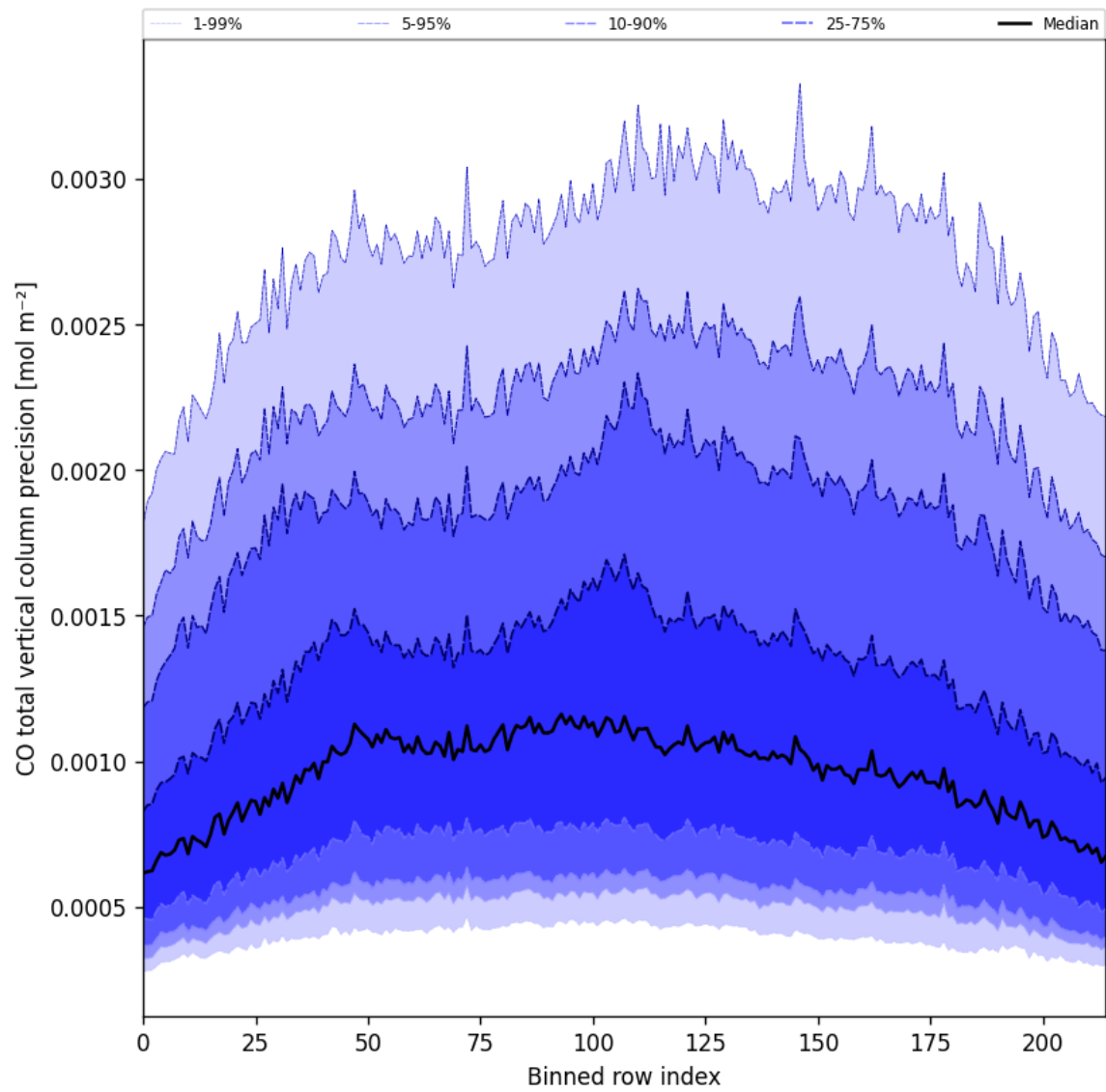
Figure 28: Along track statistics of “CO total vertical column precision” for 2025-01-29 to 2025-01-31
