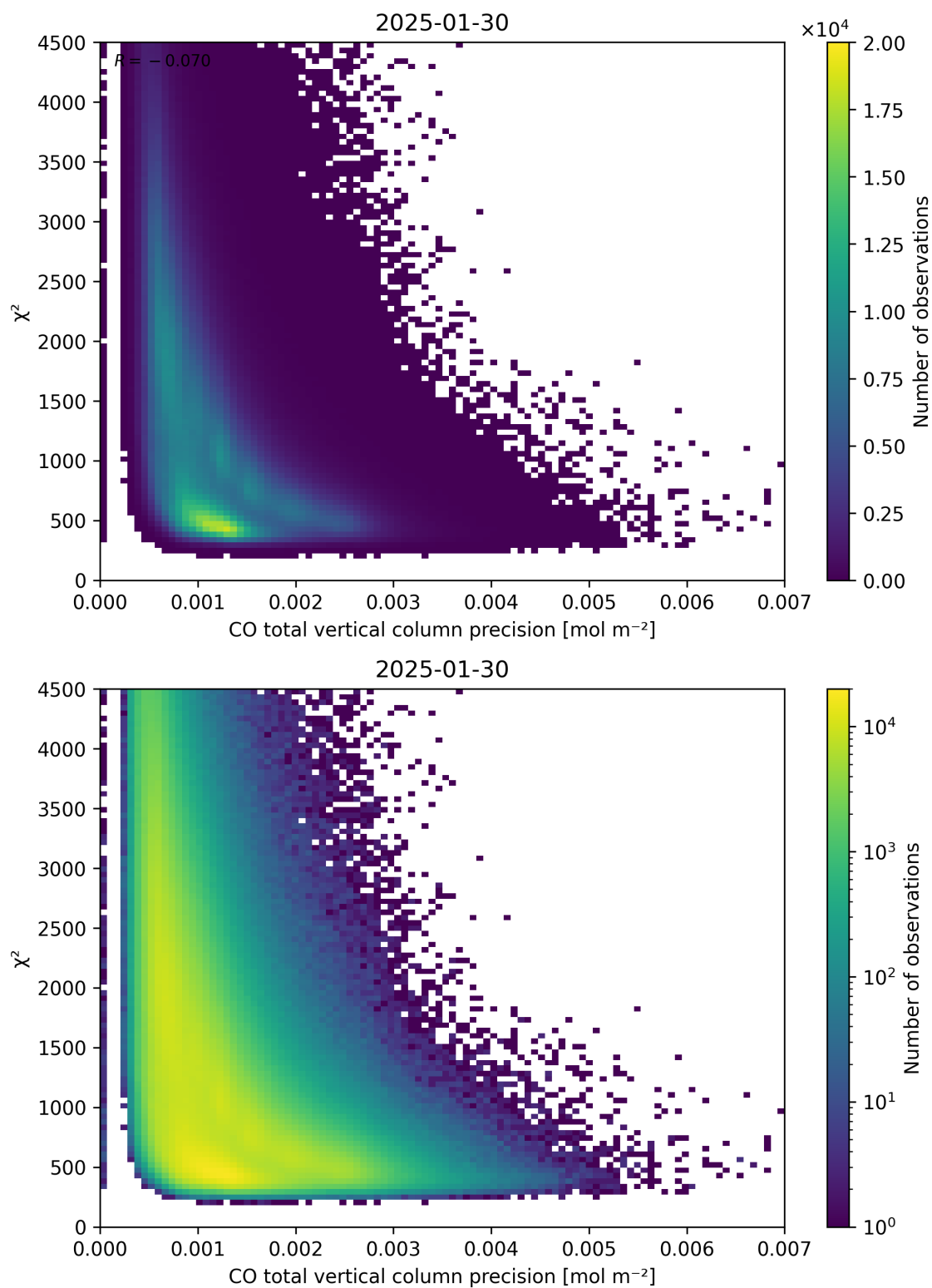
Figure 44: Scatter density plot of “CO total vertical column precision” against “ \chi^2 ” for 2025-01-29 to 2025-01-31.
