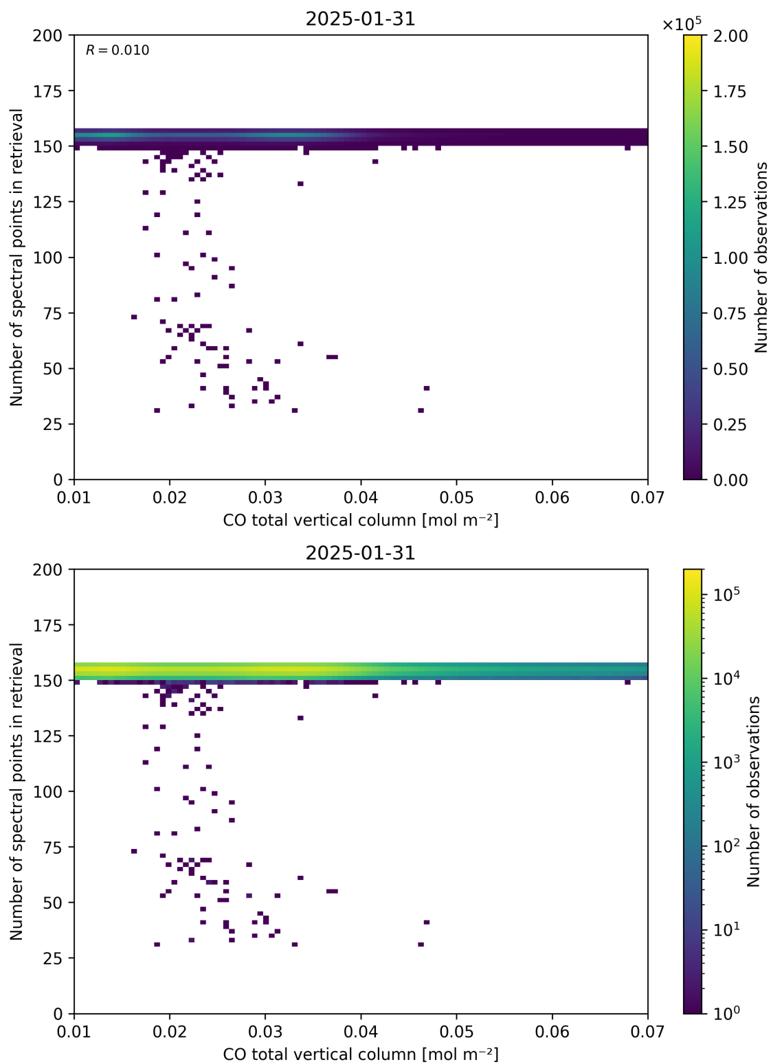
Figure 43: Scatter density plot of “CO total vertical column” against “Number of spectral points in retrieval” for 2025-01-30 to 2025-02-01.
