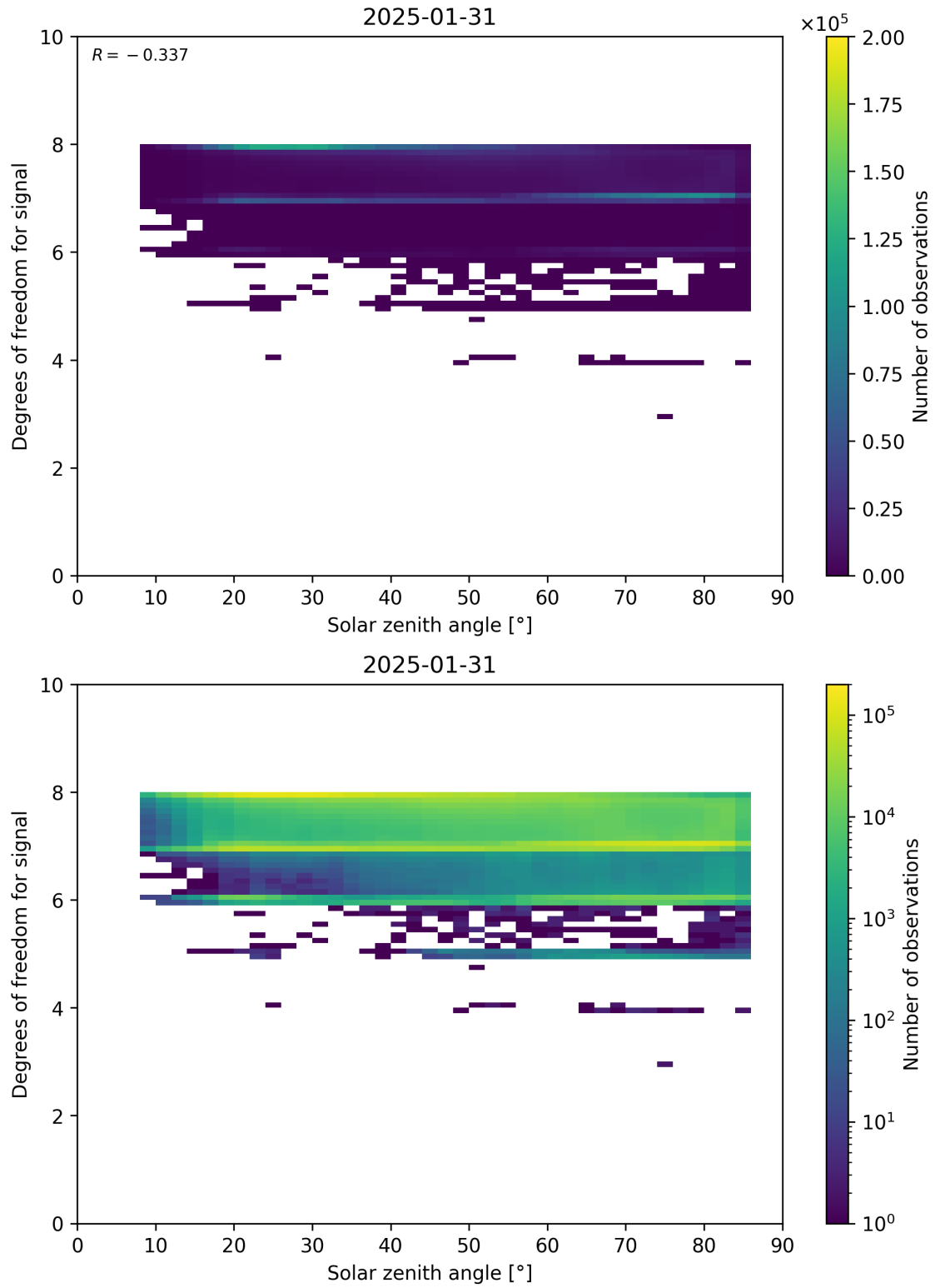
Figure 65: Scatter density plot of “Solar zenith angle” against “Degrees of freedom for signal” for 2025-01-30 to 2025-02-01.
