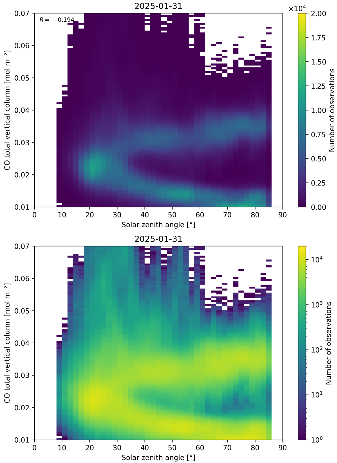
Figure 61: Scatter density plot of “Solar zenith angle” against “CO total vertical column” for 2025-01-30 to 2025-02-01.
