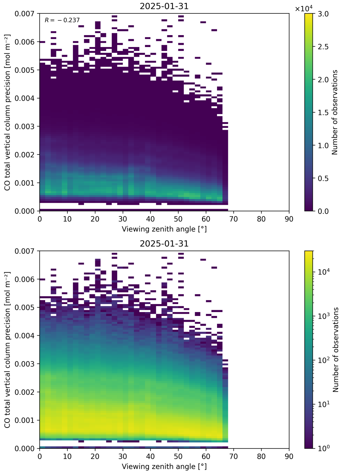
Figure 71: Scatter density plot of “Viewing zenith angle” against “CO total vertical column precision” for 2025-01-30 to 2025-02-01.
