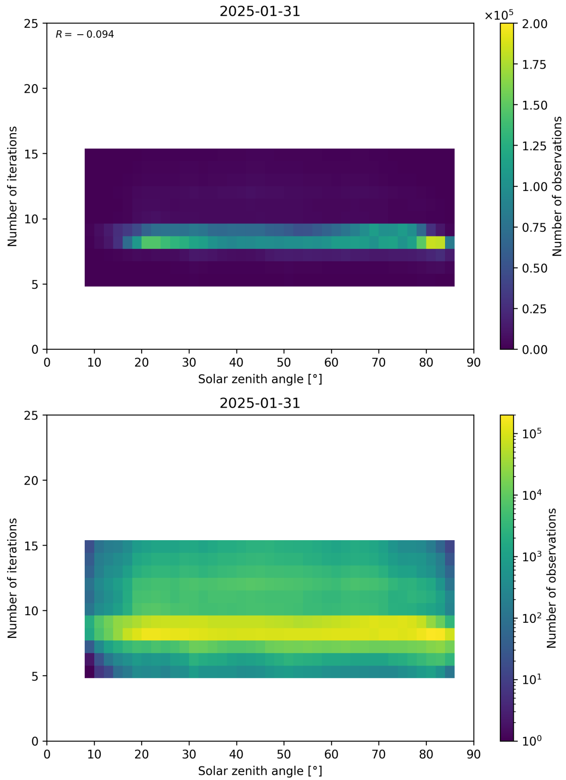
Figure 67: Scatter density plot of “Solar zenith angle” against “Number of iterations” for 2025-01-30 to 2025-02-01.
