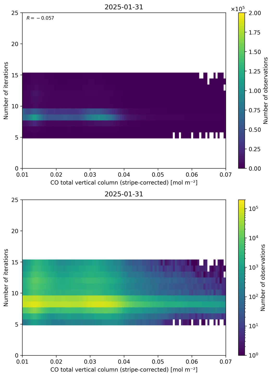
Figure 39: Scatter density plot of “CO total vertical column (stripe-corrected)” against “Number of iterations” for 2025-01-30 to 2025-02-01.
