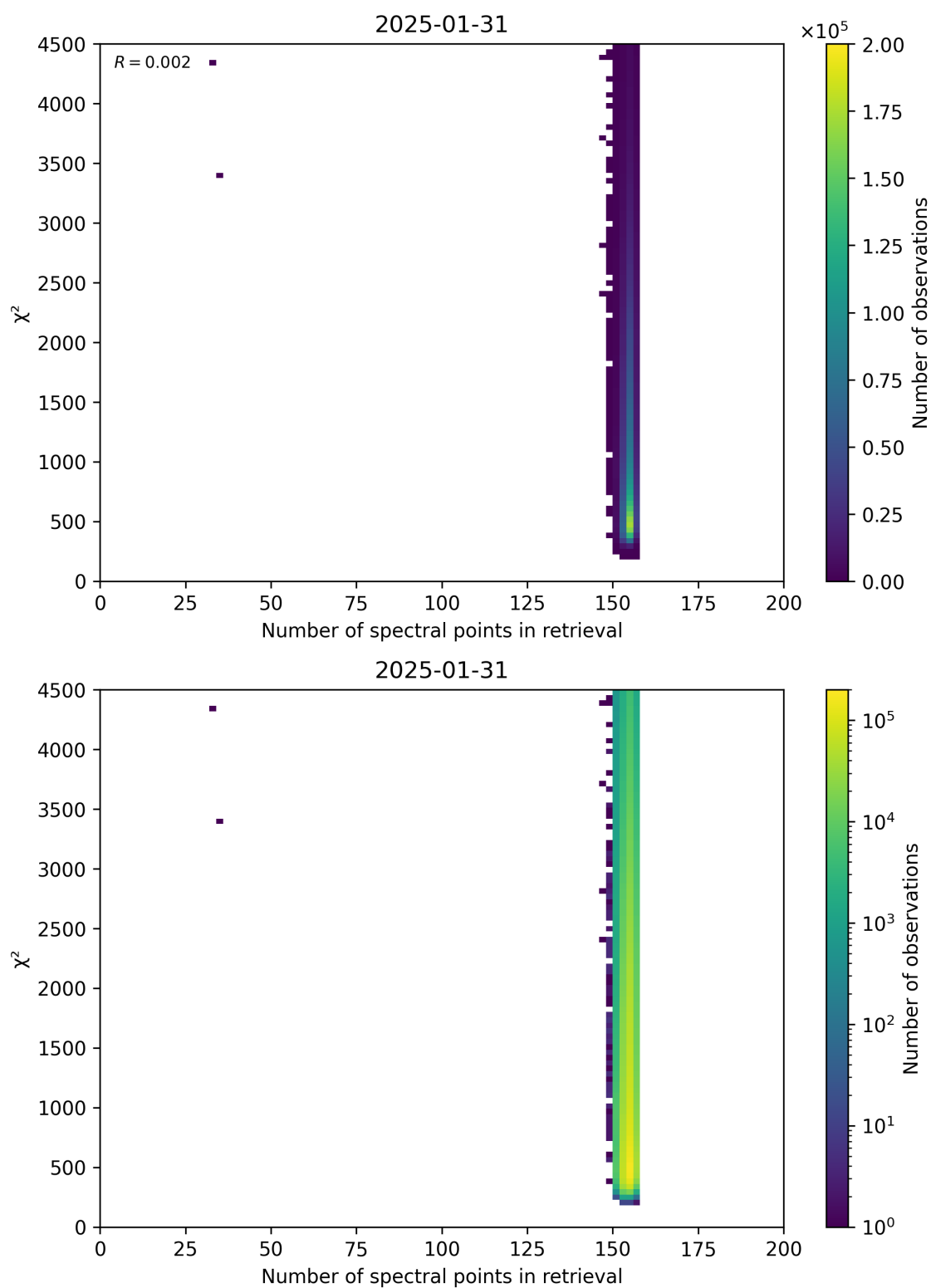
Figure 58: Scatter density plot of “Number of spectral points in retrieval” against “ \chi^2 ” for 2025-01-30 to 2025-02-01.
