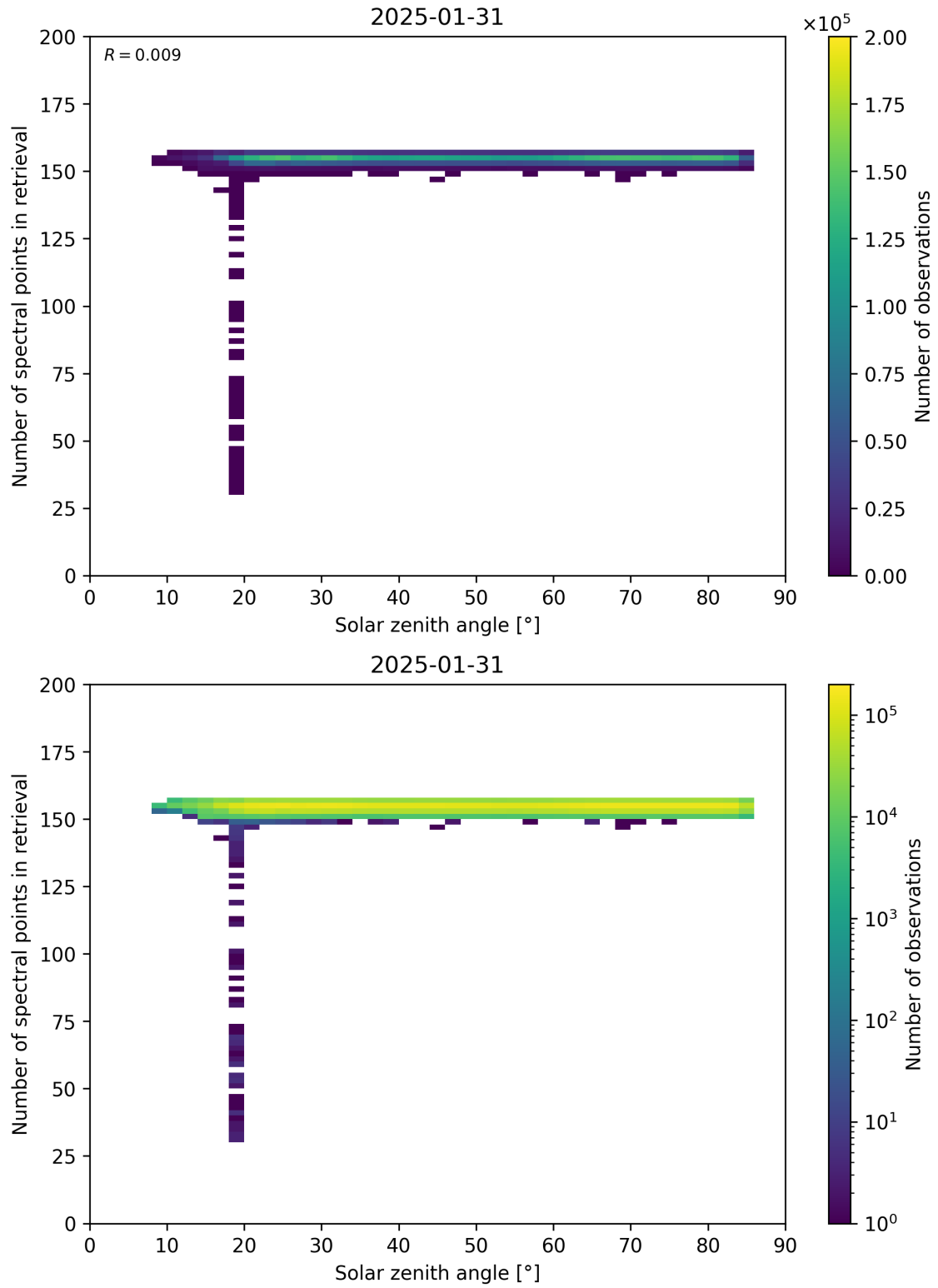
Figure 68: Scatter density plot of “Solar zenith angle” against “Number of spectral points in retrieval” for 2025-01-30 to 2025-02-01.
