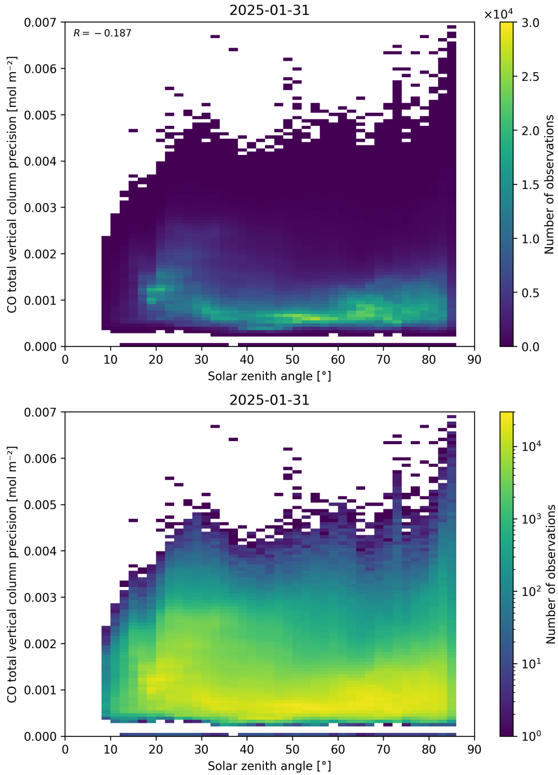
Figure 63: Scatter density plot of “Solar zenith angle” against “CO total vertical column precision” for 2025-01-30 to 2025-02-01.
