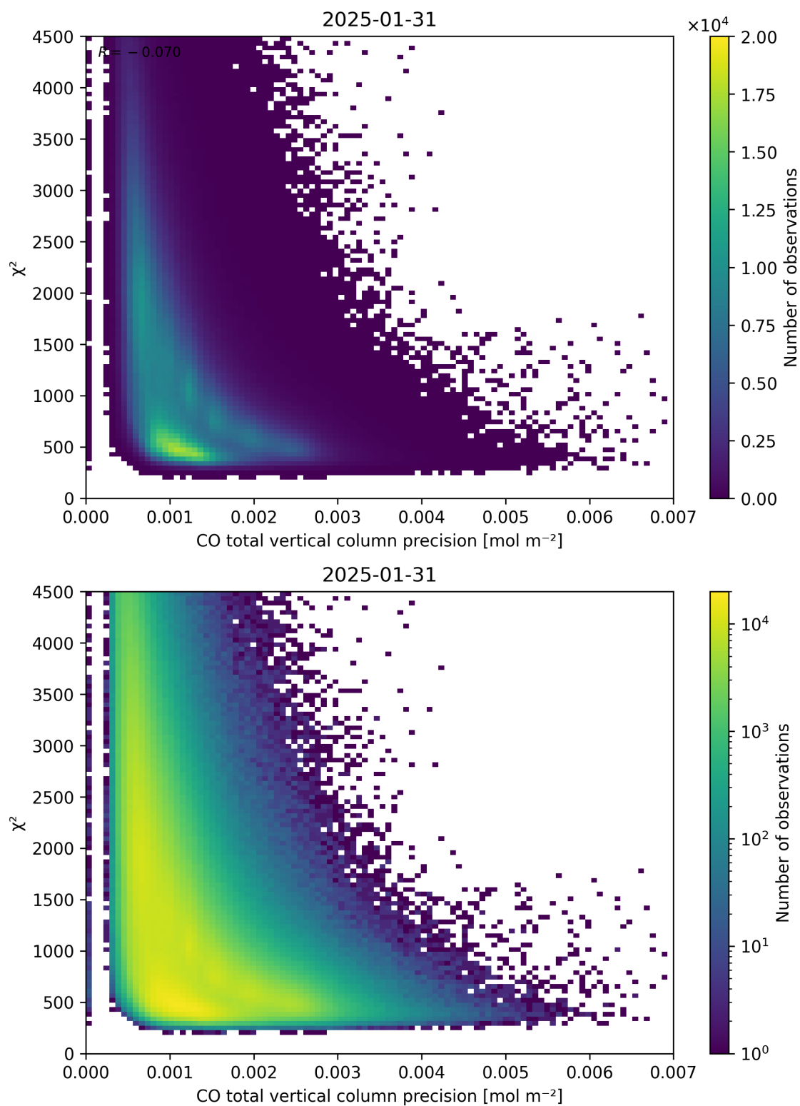
Figure 44: Scatter density plot of “CO total vertical column precision” against “ \chi^2 ” for 2025-01-30 to 2025-02-01.
