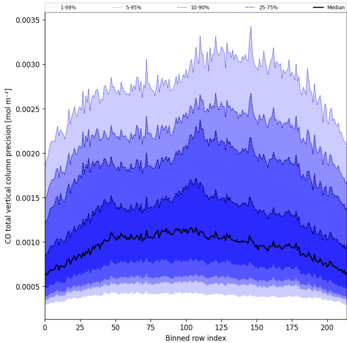
Figure 28: Along track statistics of “CO total vertical column precision” for 2025-01-30 to 2025-02-01
