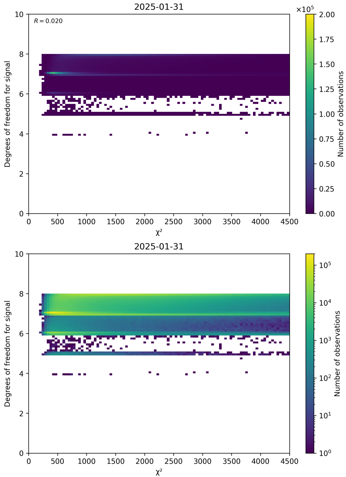
Figure 48: Scatter density plot of “ \chi^2 ” against “Degrees of freedom for signal” for 2025-01-30 to 2025-02-01.
