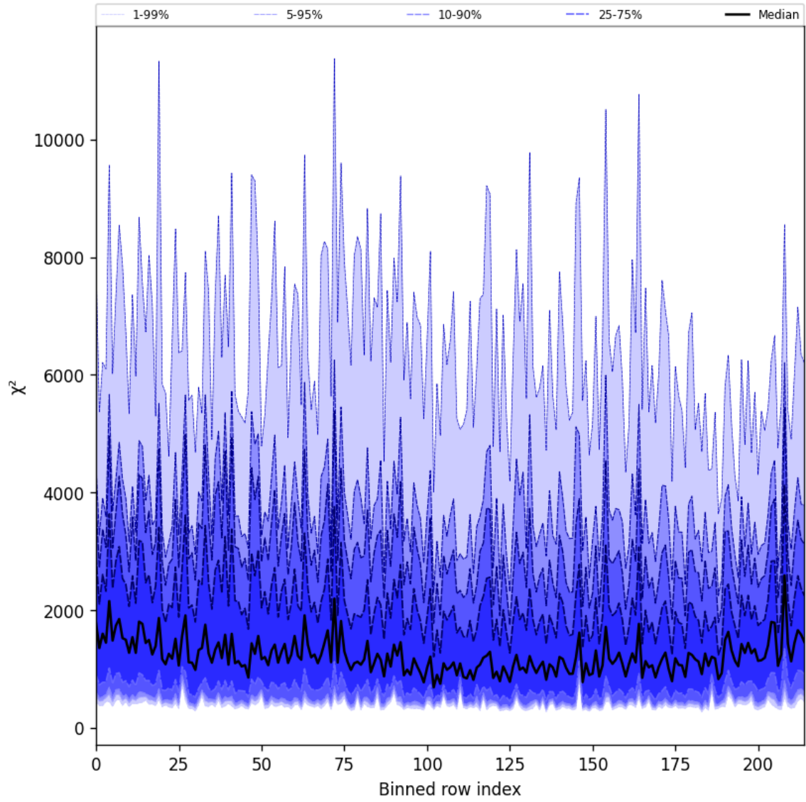
Figure 30: Along track statistics of “ \chi^2 ” for 2025-01-30 to 2025-02-01
