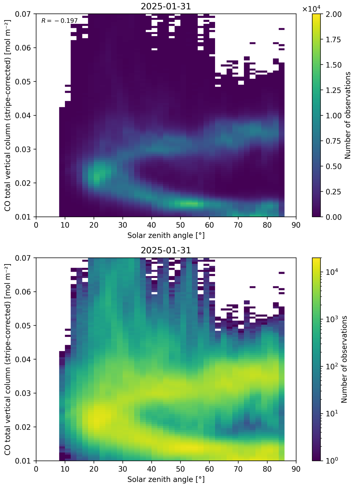
Figure 62: Scatter density plot of “Solar zenith angle” against “CO total vertical column (stripe-corrected)” for 2025-01-30 to 2025-02-01.
