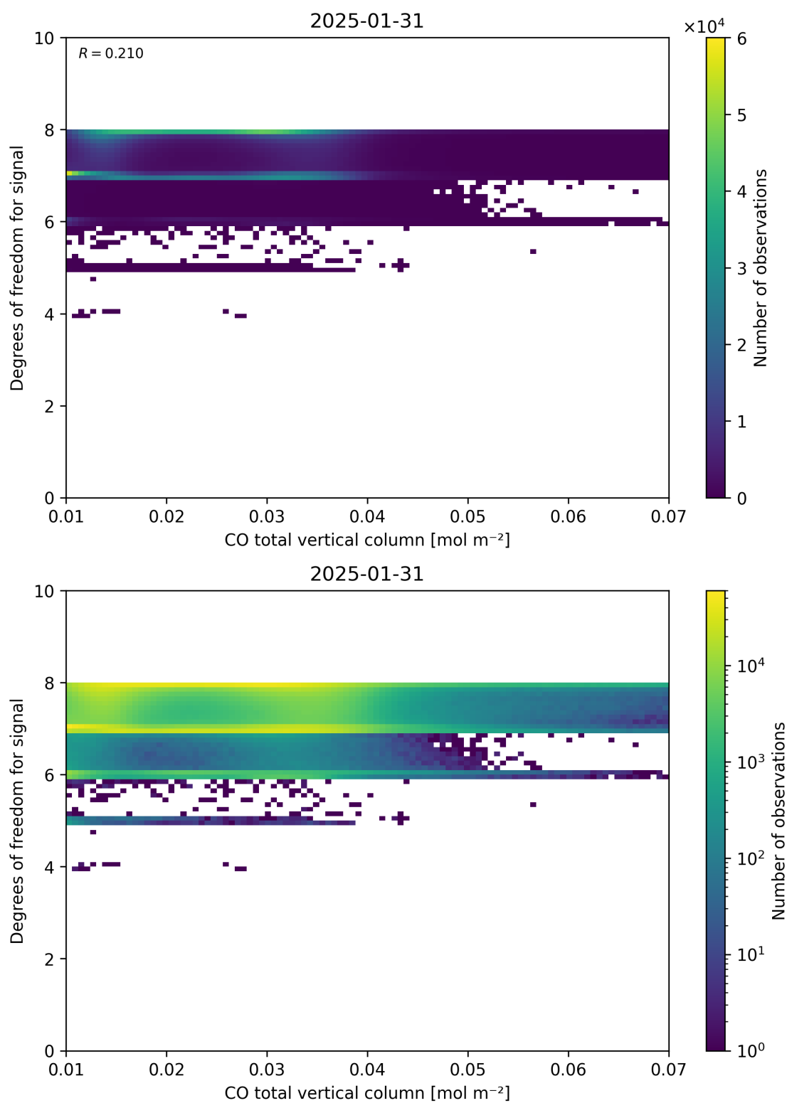
Figure 41: Scatter density plot of “CO total vertical column” against “Degrees of freedom for signal” for 2025-01-30 to 2025-02-01.
