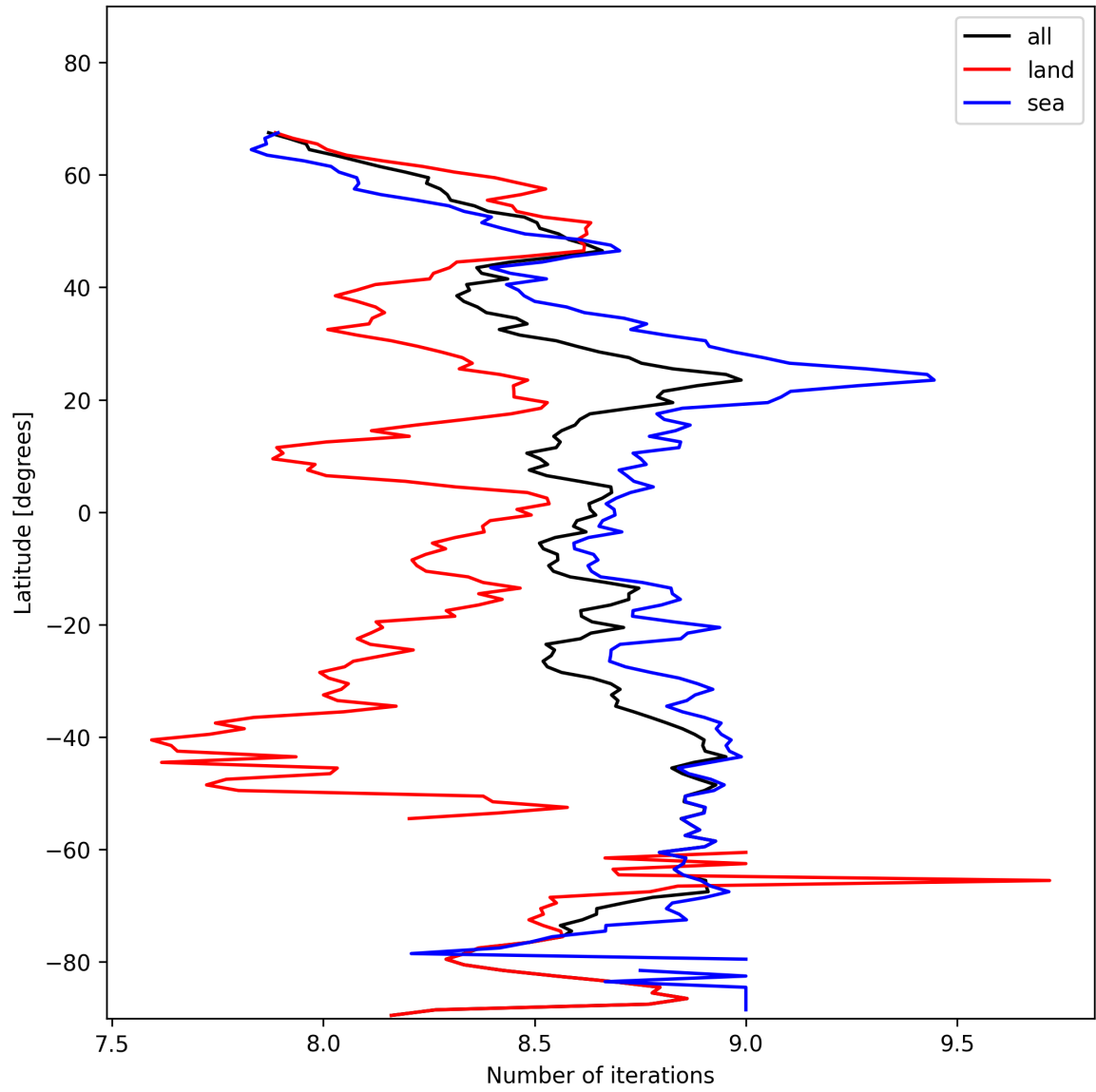
Figure 16: Zonal average of “Number of iterations” for 2025-01-30 to 2025-02-01.
