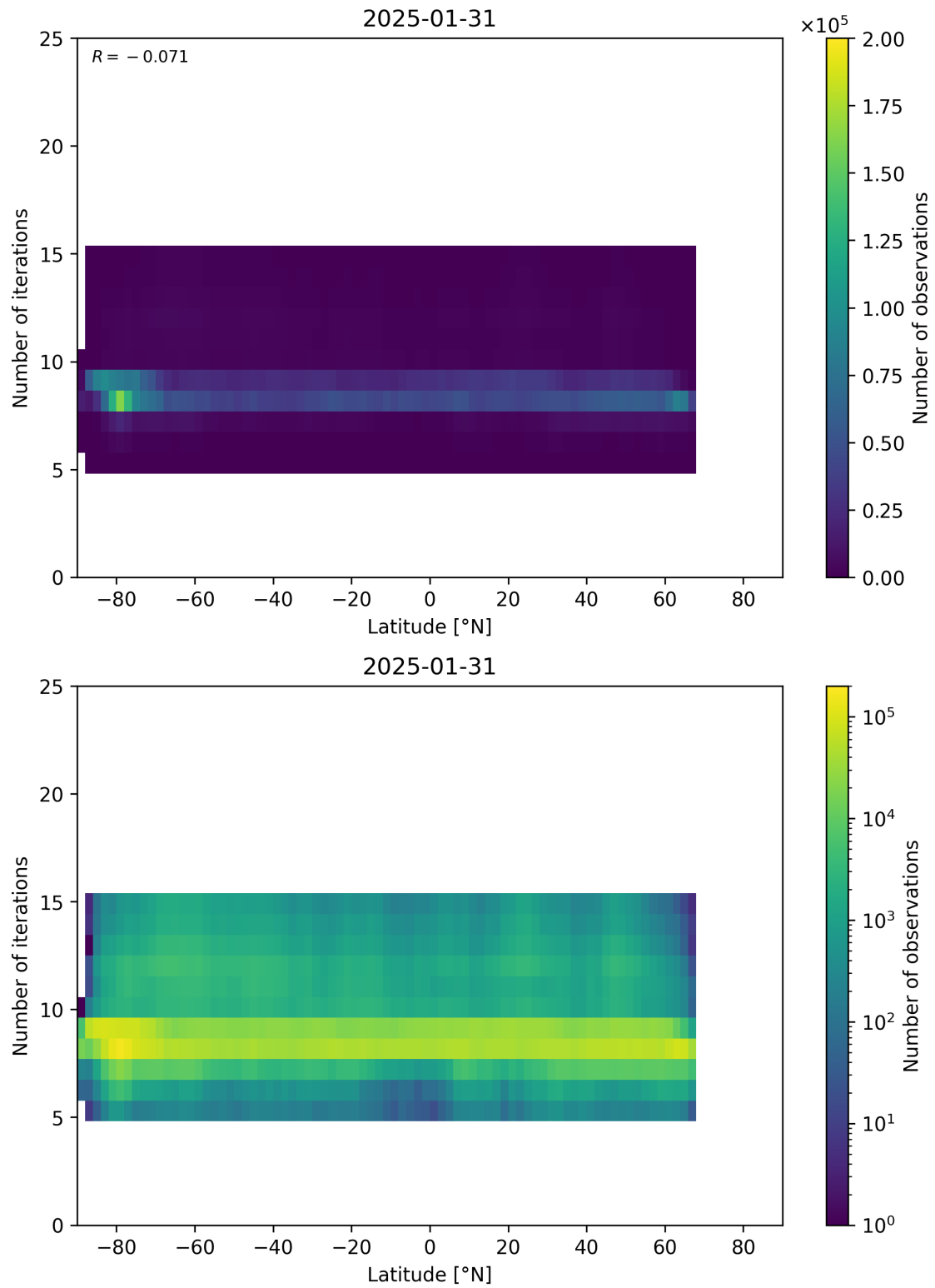
Figure 56: Scatter density plot of “Latitude” against “Number of iterations” for 2025-01-30 to 2025-02-01.
