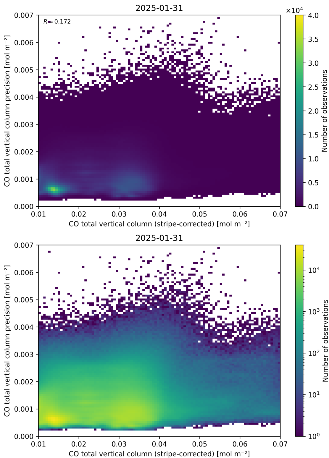
Figure 36: Scatter density plot of “CO total vertical column (stripe-corrected)” against “CO total vertical column precision” for 2025-01-30 to 2025-02-01.
