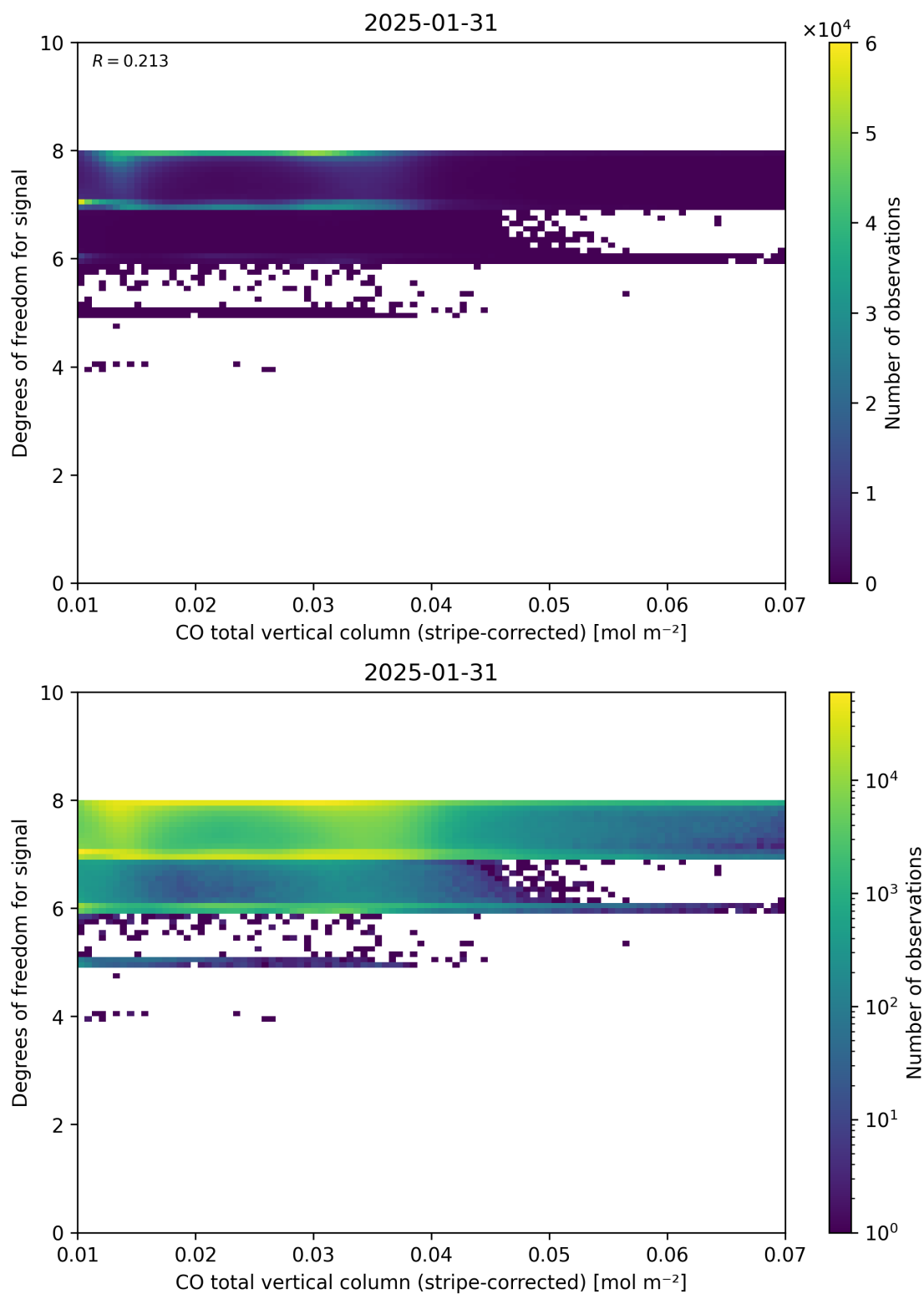
Figure 38: Scatter density plot of “CO total vertical column (stripe-corrected)” against “Degrees of freedom for signal” for 2025-01-30 to 2025-02-01.
