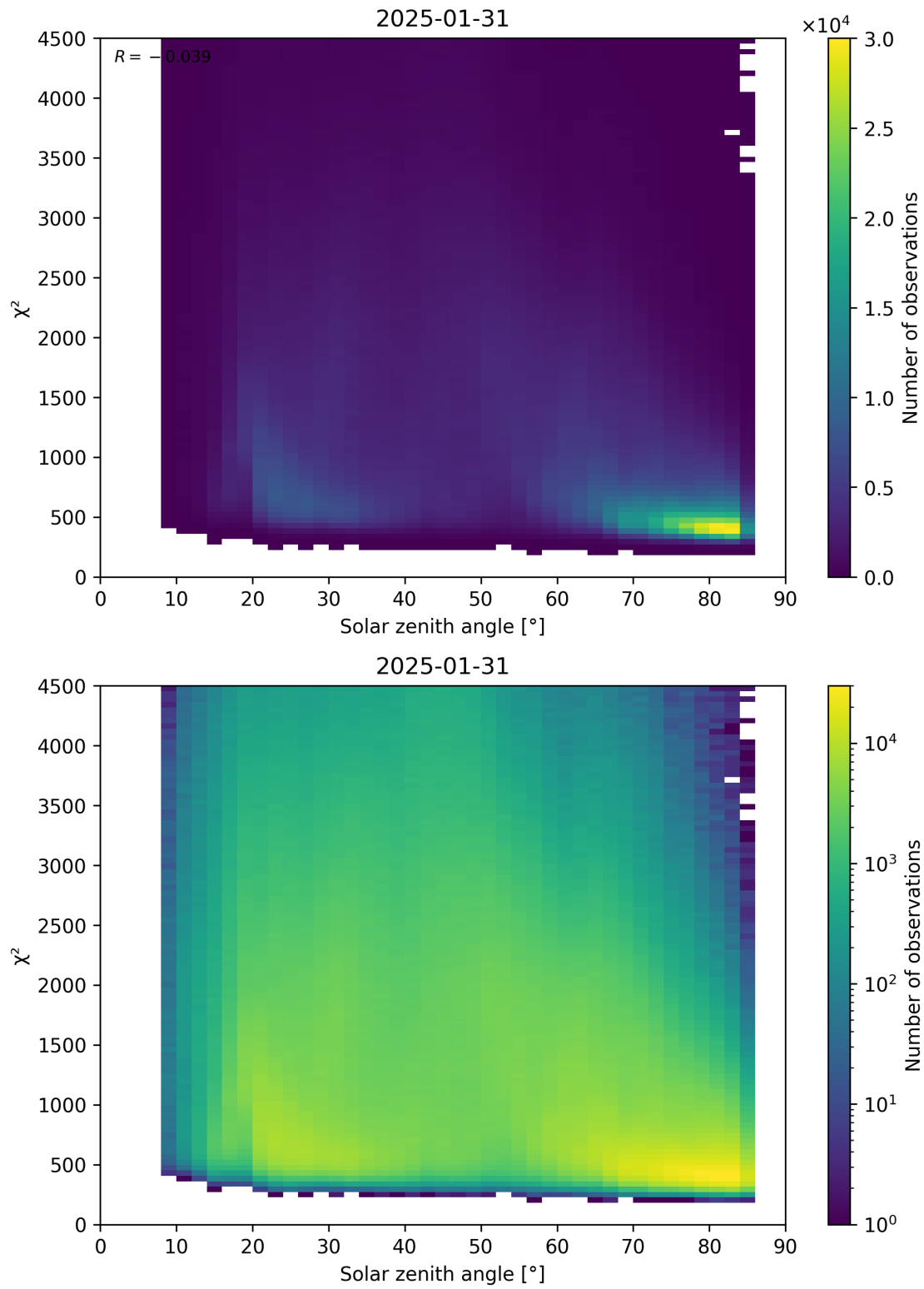
Figure 64: Scatter density plot of “Solar zenith angle” against “ \chi^2 ” for 2025-01-30 to 2025-02-01.
