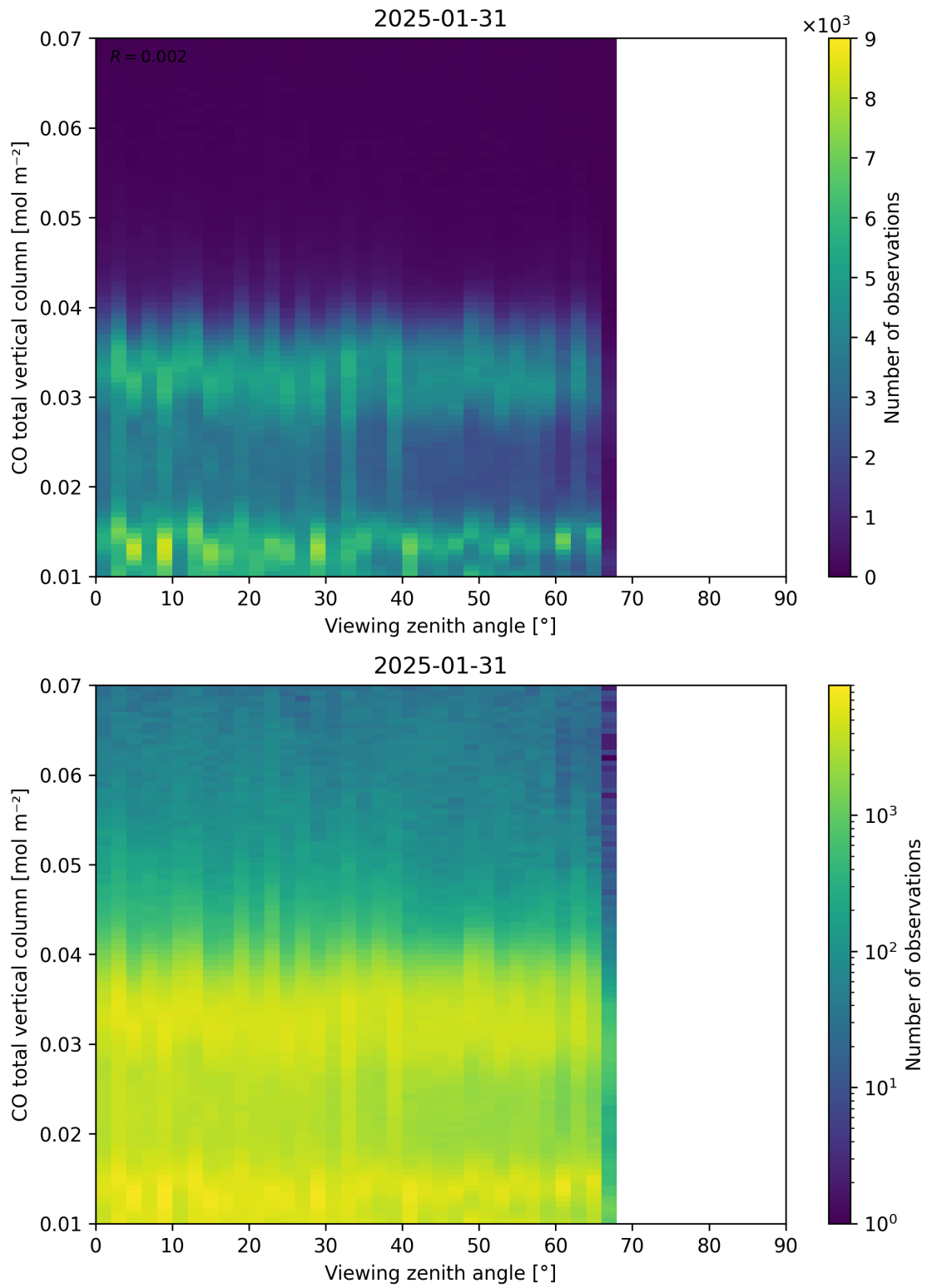
Figure 69: Scatter density plot of “Viewing zenith angle” against “CO total vertical column” for 2025-01-30 to 2025-02-01.
