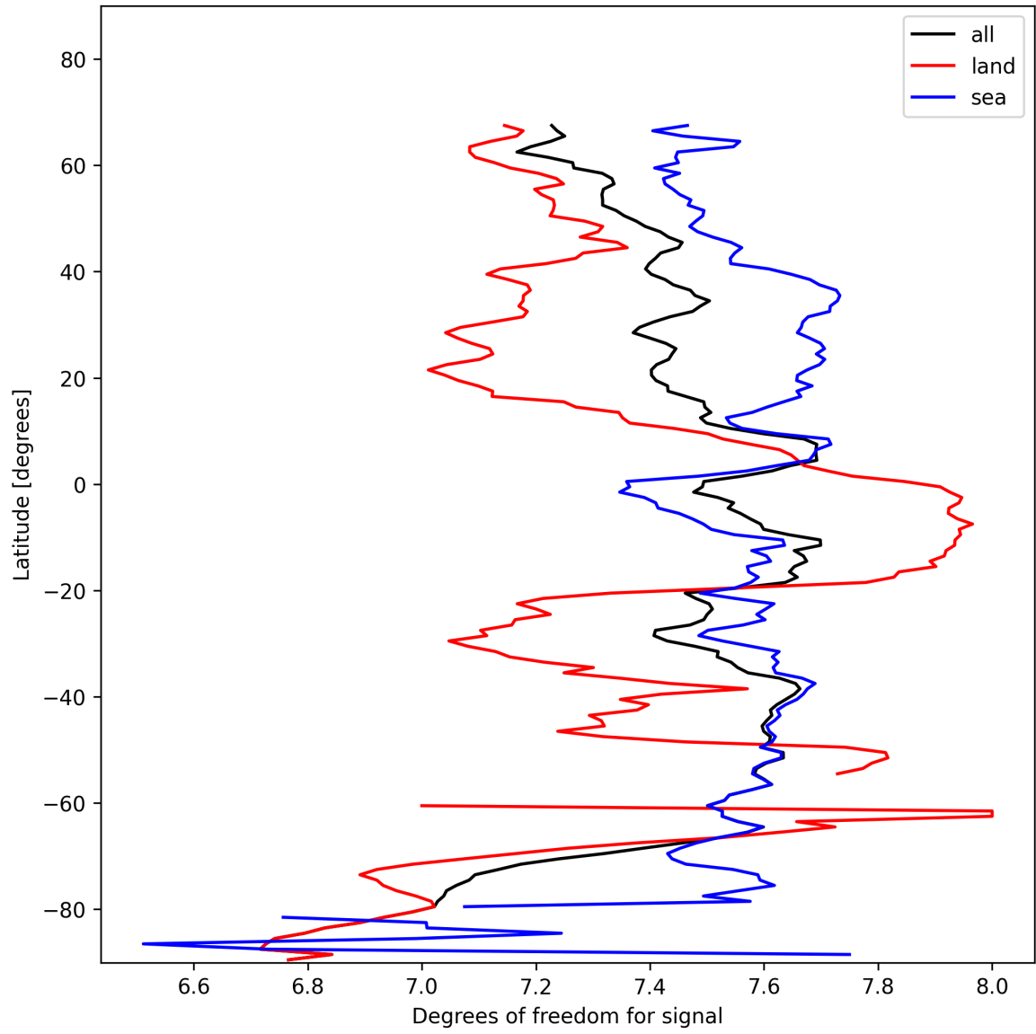
Figure 15: Zonal average of “Degrees of freedom for signal” for 2025-01-30 to 2025-02-01.
