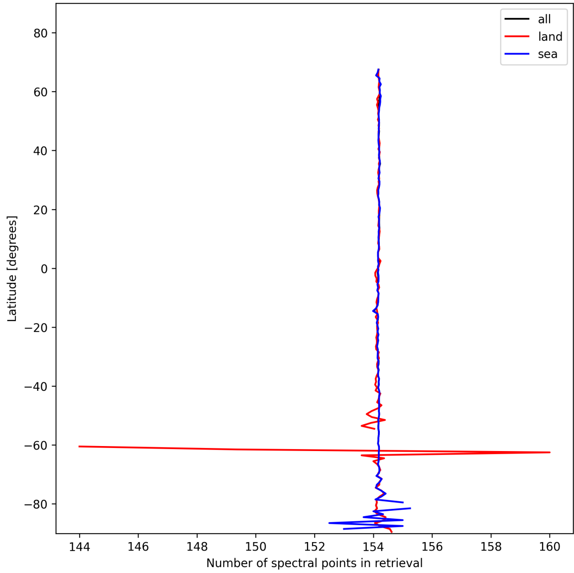
Figure 13: Zonal average of “Number of spectral points in retrieval” for 2025-01-30 to 2025-02-01.
