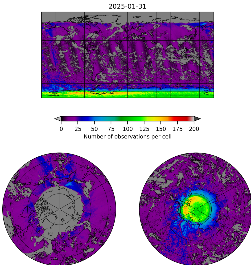
Figure 8: Map of the number of observations for 2025-01-30 to 2025-02-01
