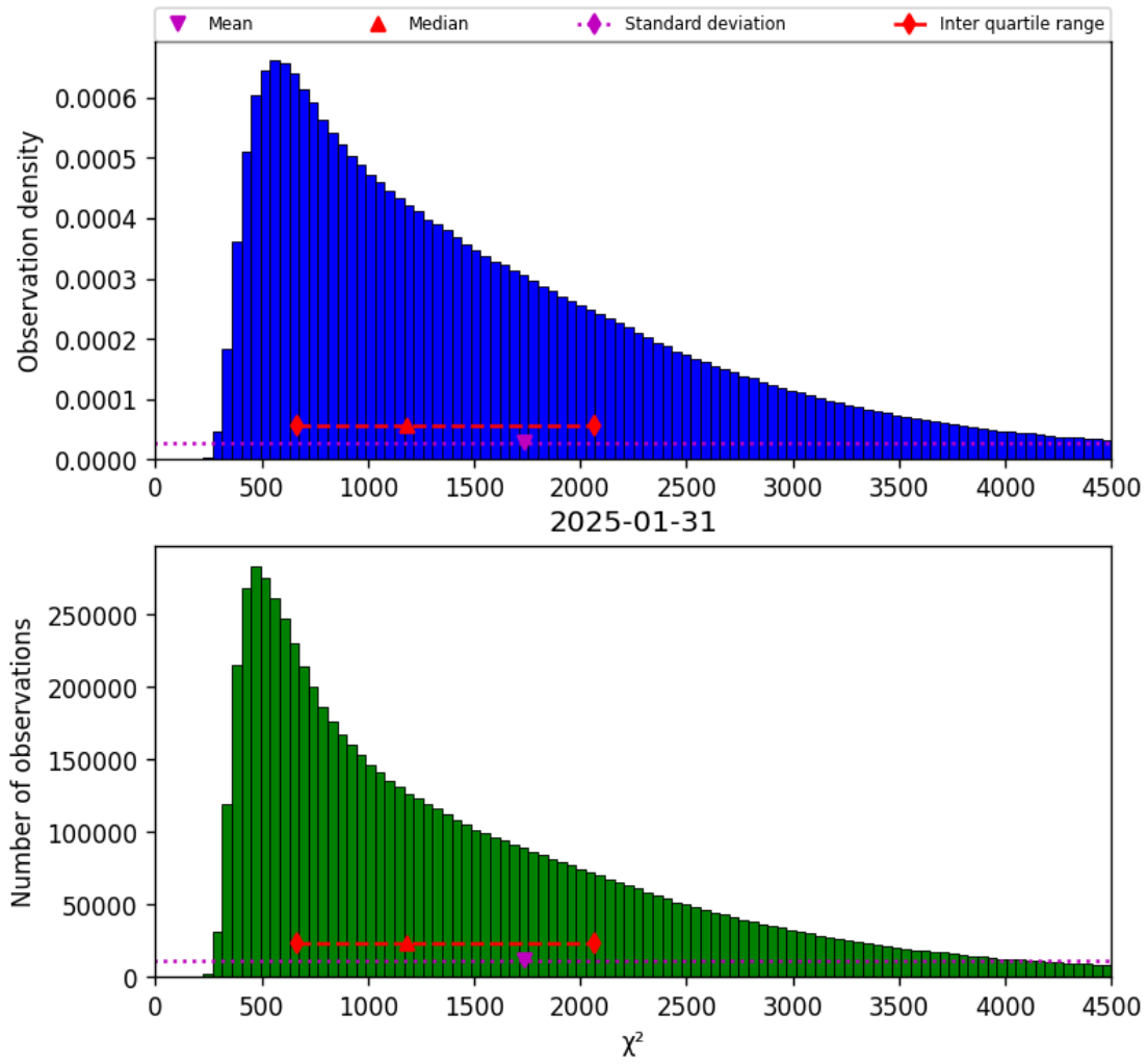
Figure 22: Histogram of " \chi^2 " for 2025-01-30 to 2025-02-01
