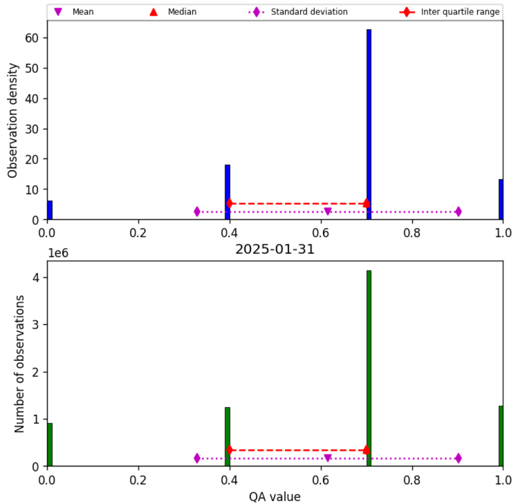
Figure 17: Histogram of “QA value” for 2025-01-30 to 2025-02-01
