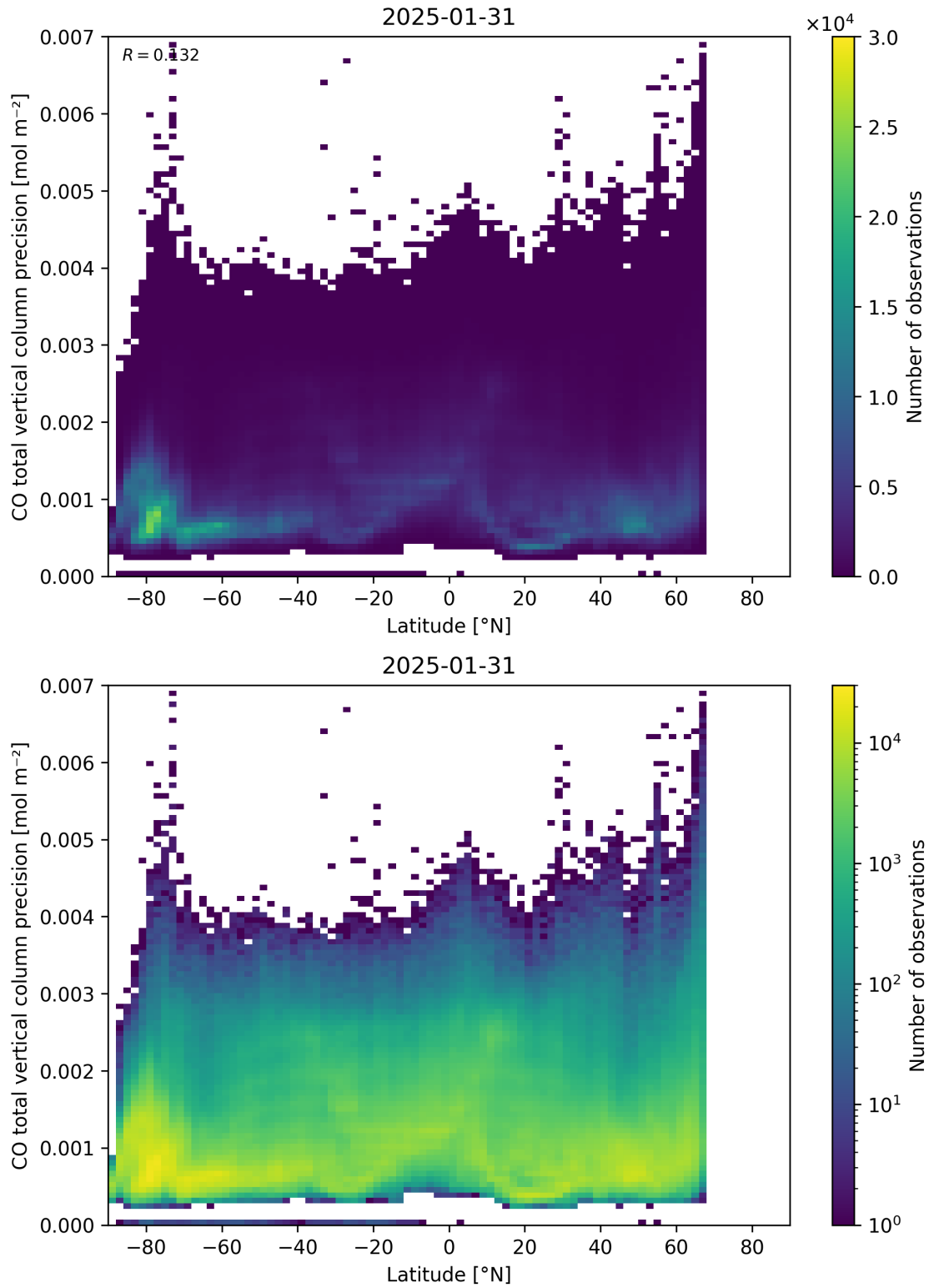
Figure 53: Scatter density plot of “Latitude” against “CO total vertical column precision” for 2025-01-30 to 2025-02-01.
