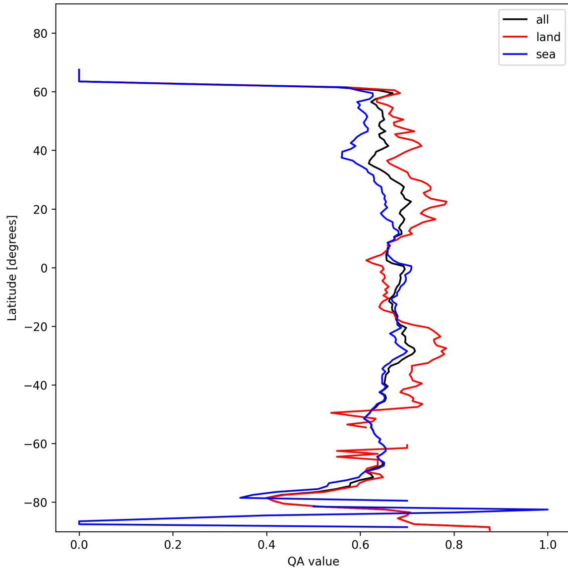
Figure 9: Zonal average of “QA value” for 2025-01-30 to 2025-02-01.
