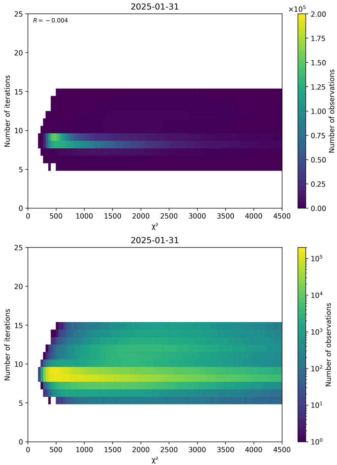
Figure 49: Scatter density plot of “ \chi^2 ” against “Number of iterations” for 2025-01-30 to 2025-02-01.
