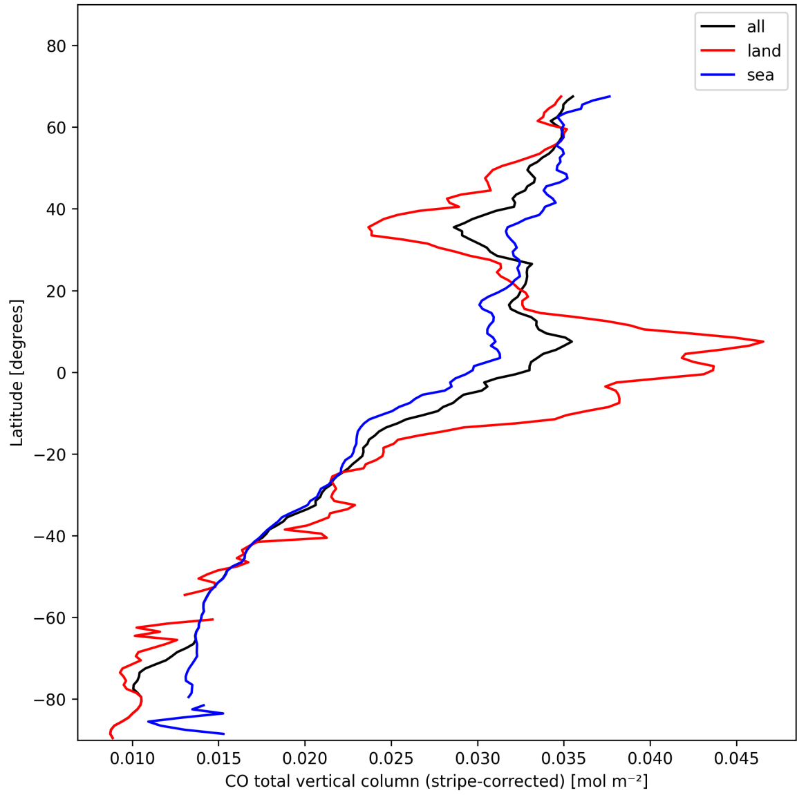
Figure 11: Zonal average of “CO total vertical column (stripe-corrected)” for 2025-01-30 to 2025-02-01.
