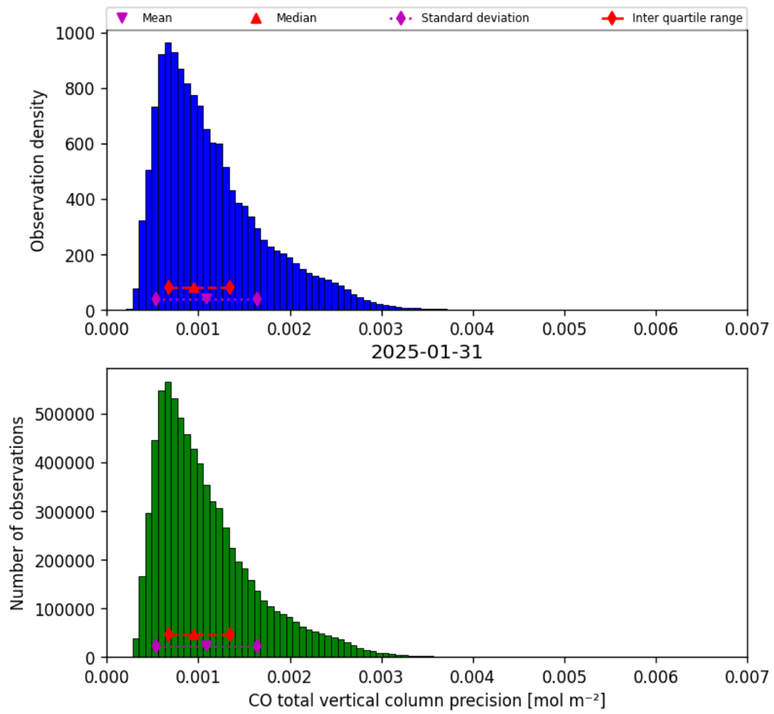
Figure 20: Histogram of “CO total vertical column precision” for 2025-01-30 to 2025-02-01
