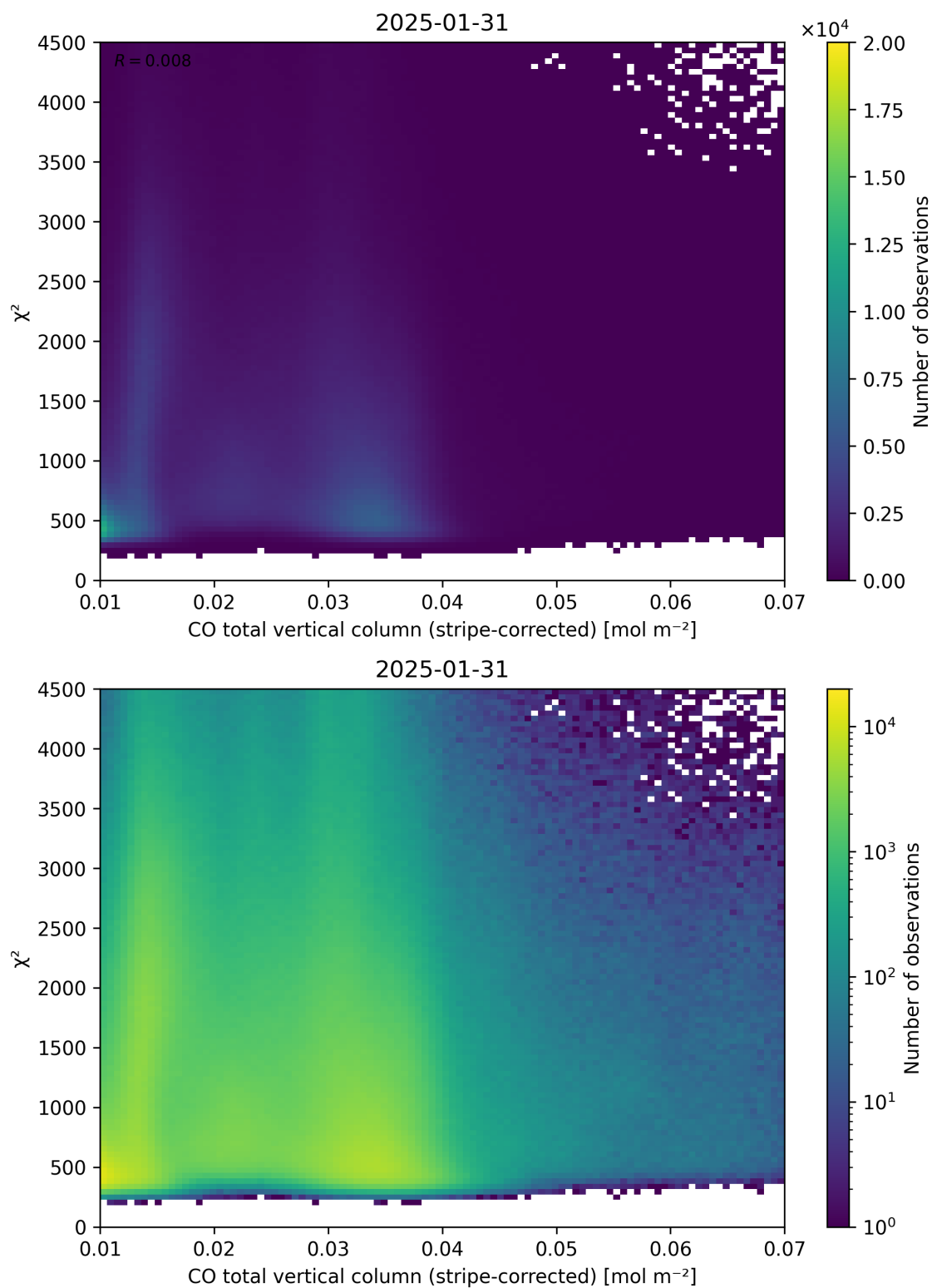
Figure 37: Scatter density plot of “CO total vertical column (stripe-corrected)” against “ \chi^2 ” for 2025-01-30 to 2025-02-01.
