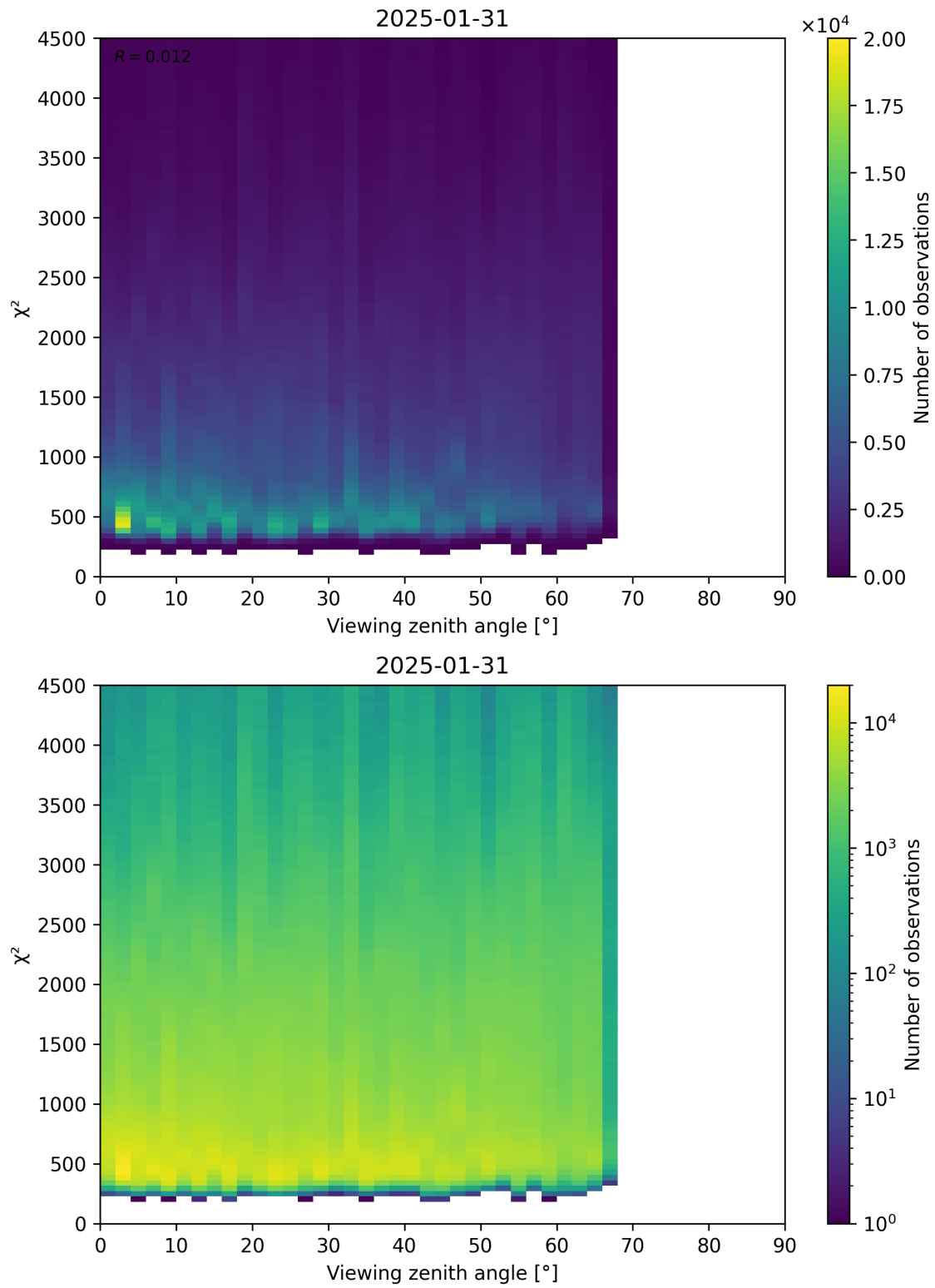
Figure 72: Scatter density plot of “Viewing zenith angle” against “ \chi^2 ” for 2025-01-30 to 2025-02-01.
