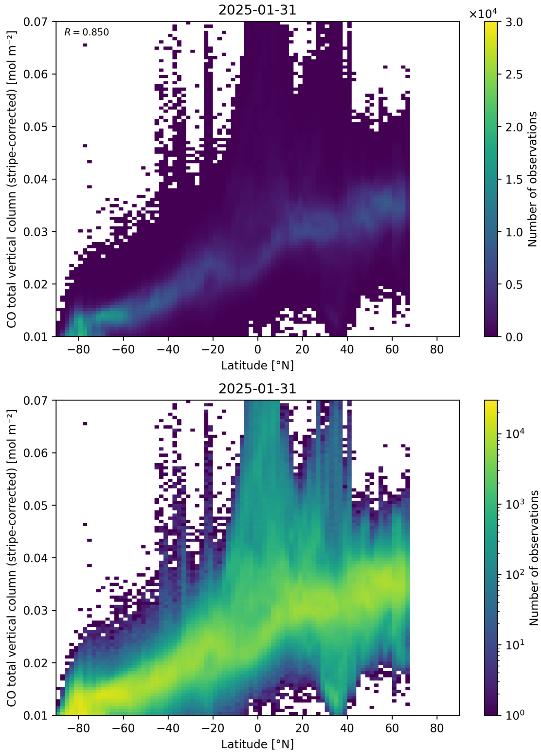
Figure 52: Scatter density plot of “Latitude” against “CO total vertical column (stripe-corrected)” for 2025-01-30 to 2025-02-01.
