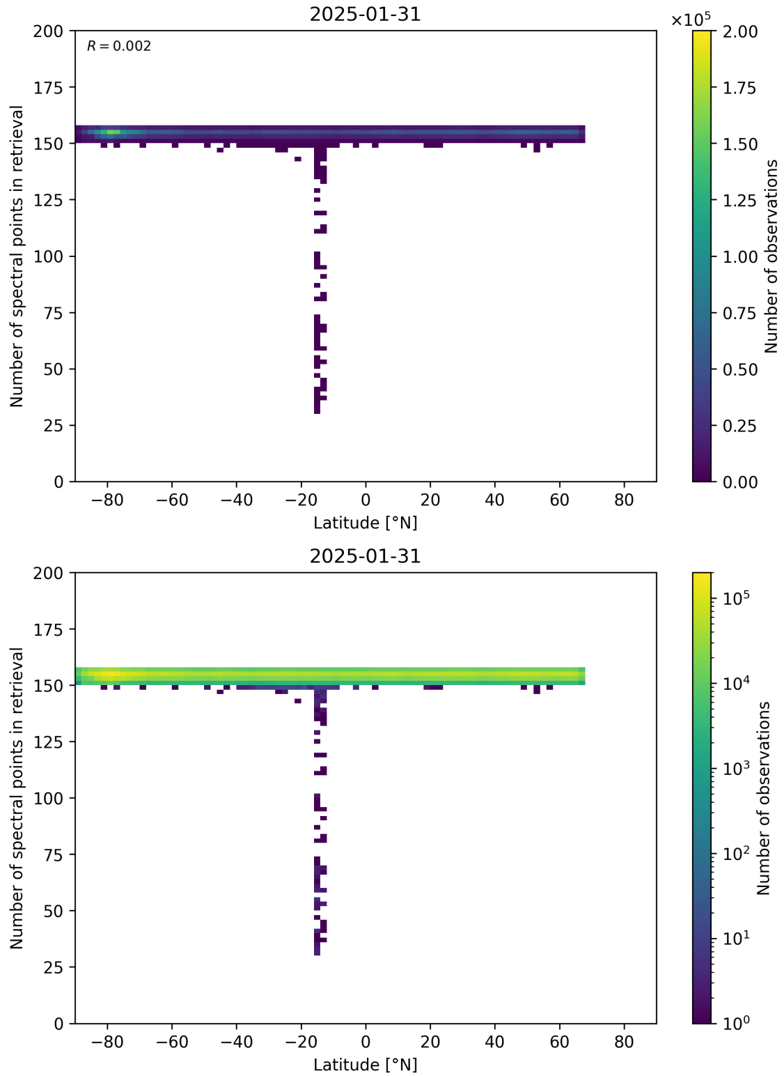
Figure 57: Scatter density plot of “Latitude” against “Number of spectral points in retrieval” for 2025-01-30 to 2025-02-01.
