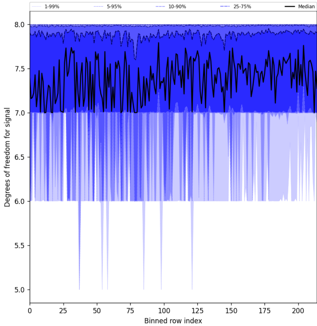
Figure 31: Along track statistics of “Degrees of freedom for signal” for 2025-01-30 to 2025-02-01
