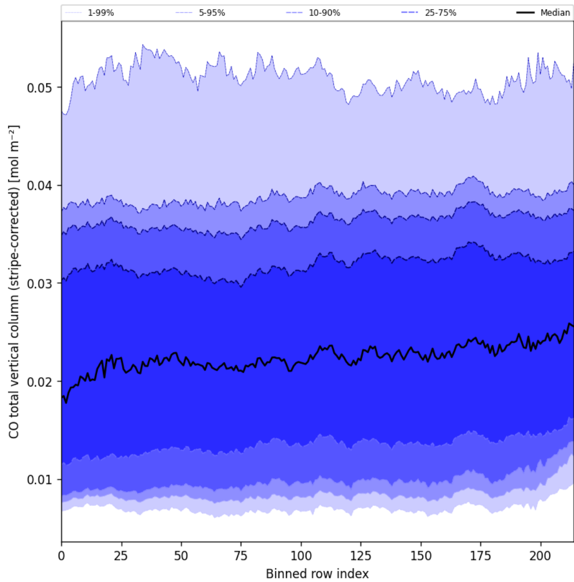
Figure 27: Along track statistics of “CO total vertical column (stripe-corrected)” for 2025-01-30 to 2025-02-01
