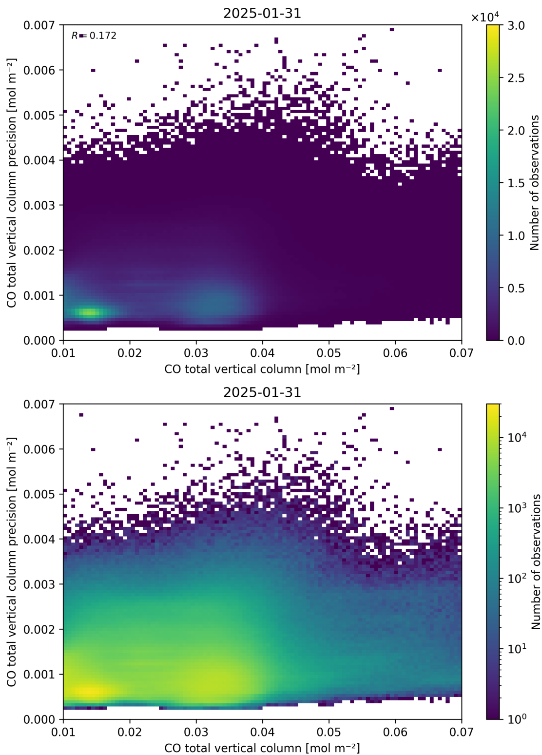
Figure 34: Scatter density plot of “CO total vertical column” against “CO total vertical column precision” for 2025-01-30 to 2025-02-01.
