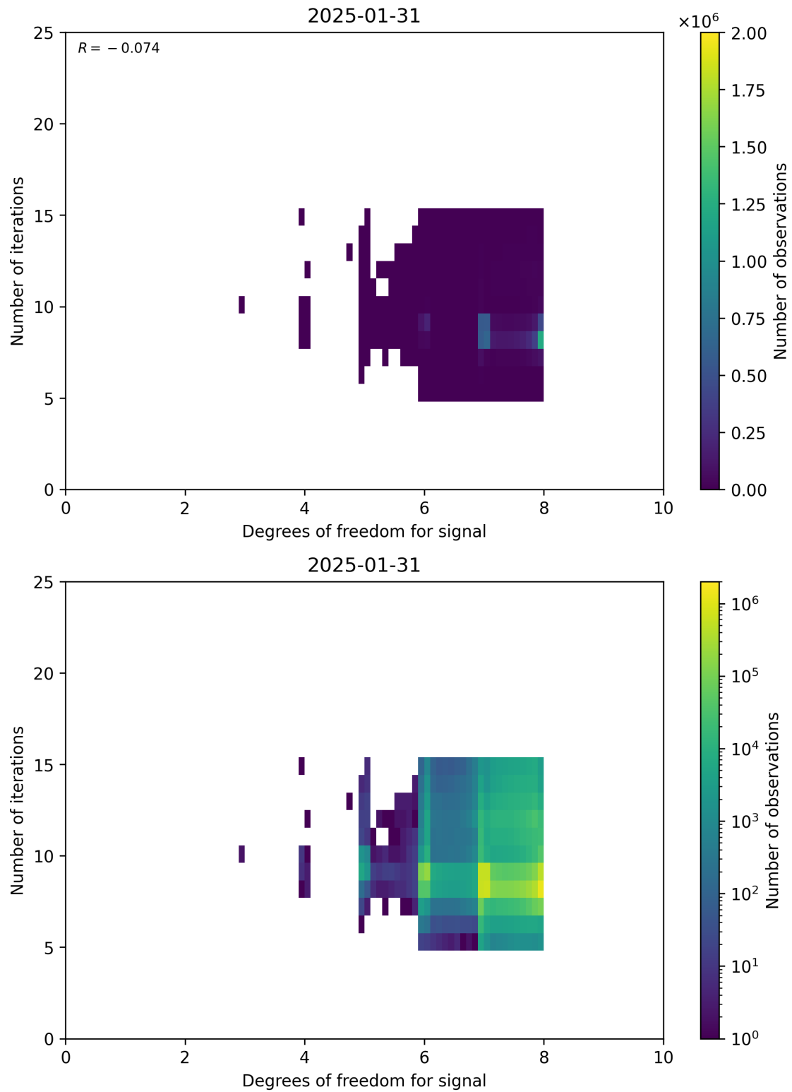
Figure 50: Scatter density plot of “Degrees of freedom for signal” against “Number of iterations” for 2025-01-30 to 2025-02-01.
