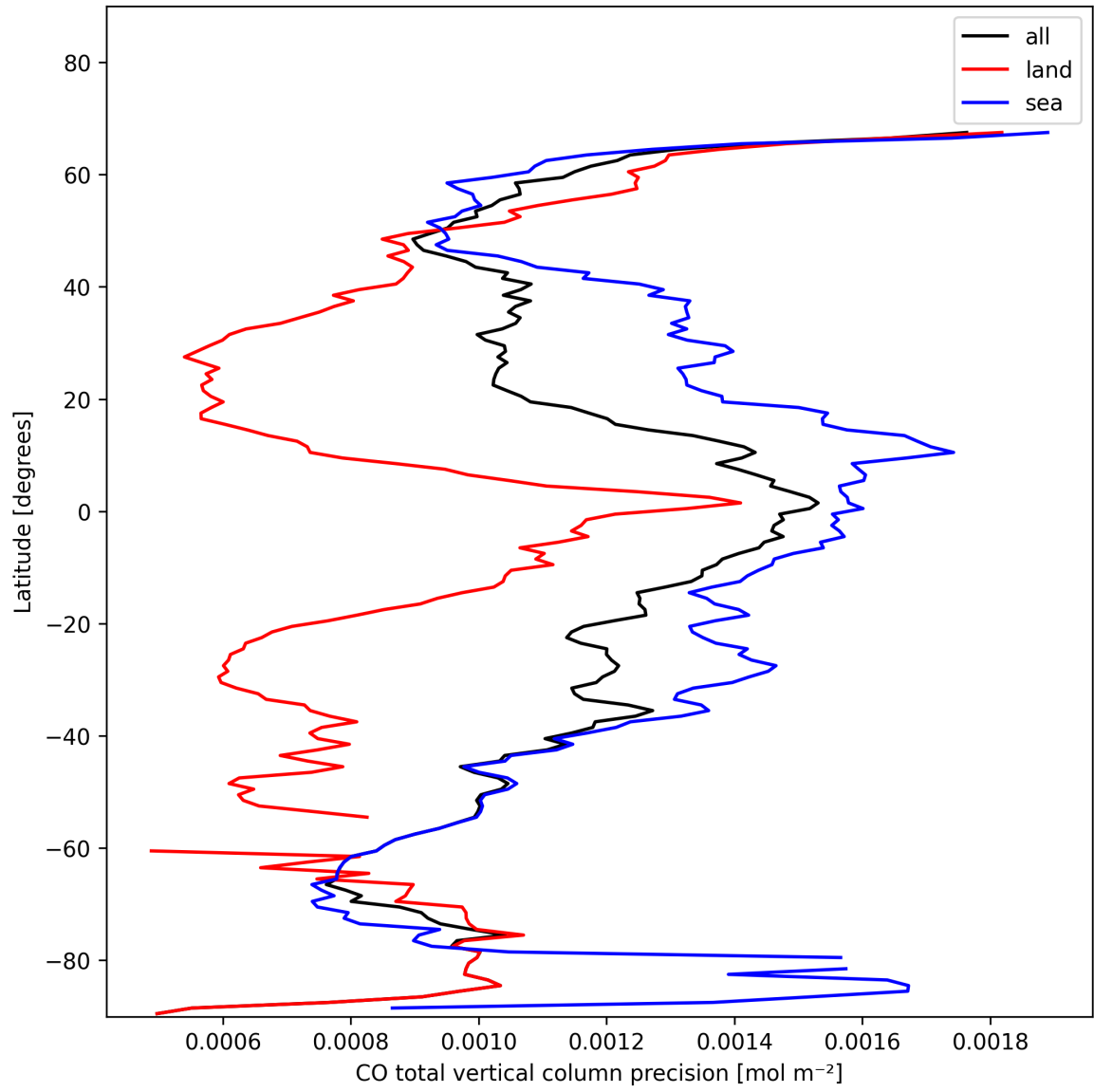
Figure 12: Zonal average of “CO total vertical column precision” for 2025-01-30 to 2025-02-01.
