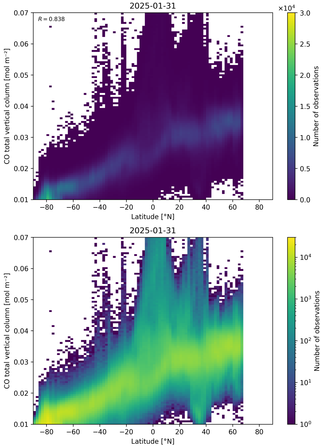
Figure 51: Scatter density plot of “Latitude” against “CO total vertical column” for 2025-01-30 to 2025-02-01.
