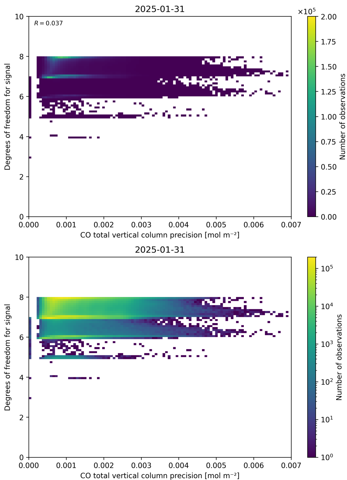
Figure 45: Scatter density plot of “CO total vertical column precision” against “Degrees of freedom for signal” for 2025-01-30 to 2025-02-01.
