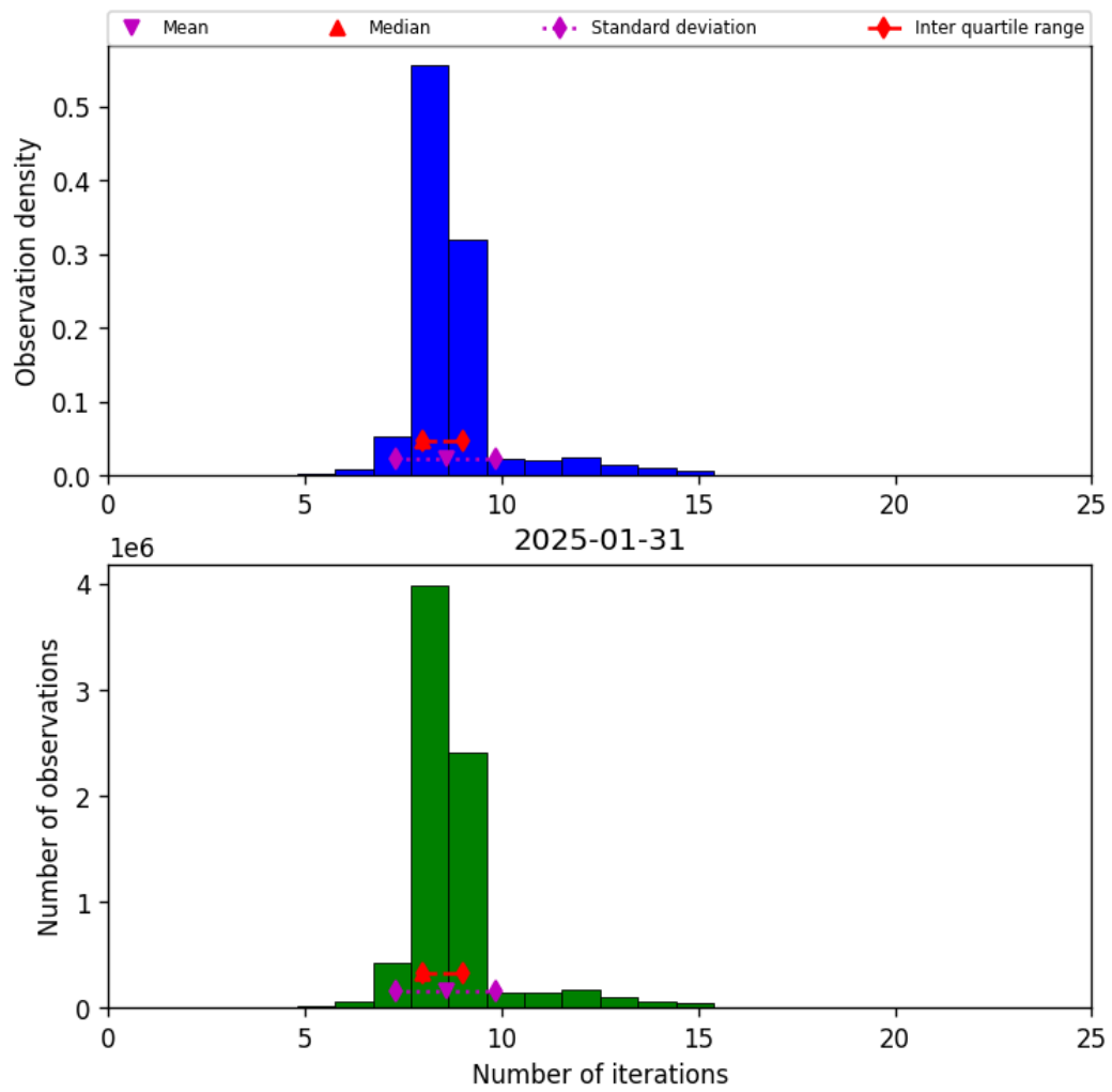
Figure 24: Histogram of “Number of iterations” for 2025-01-30 to 2025-02-01
