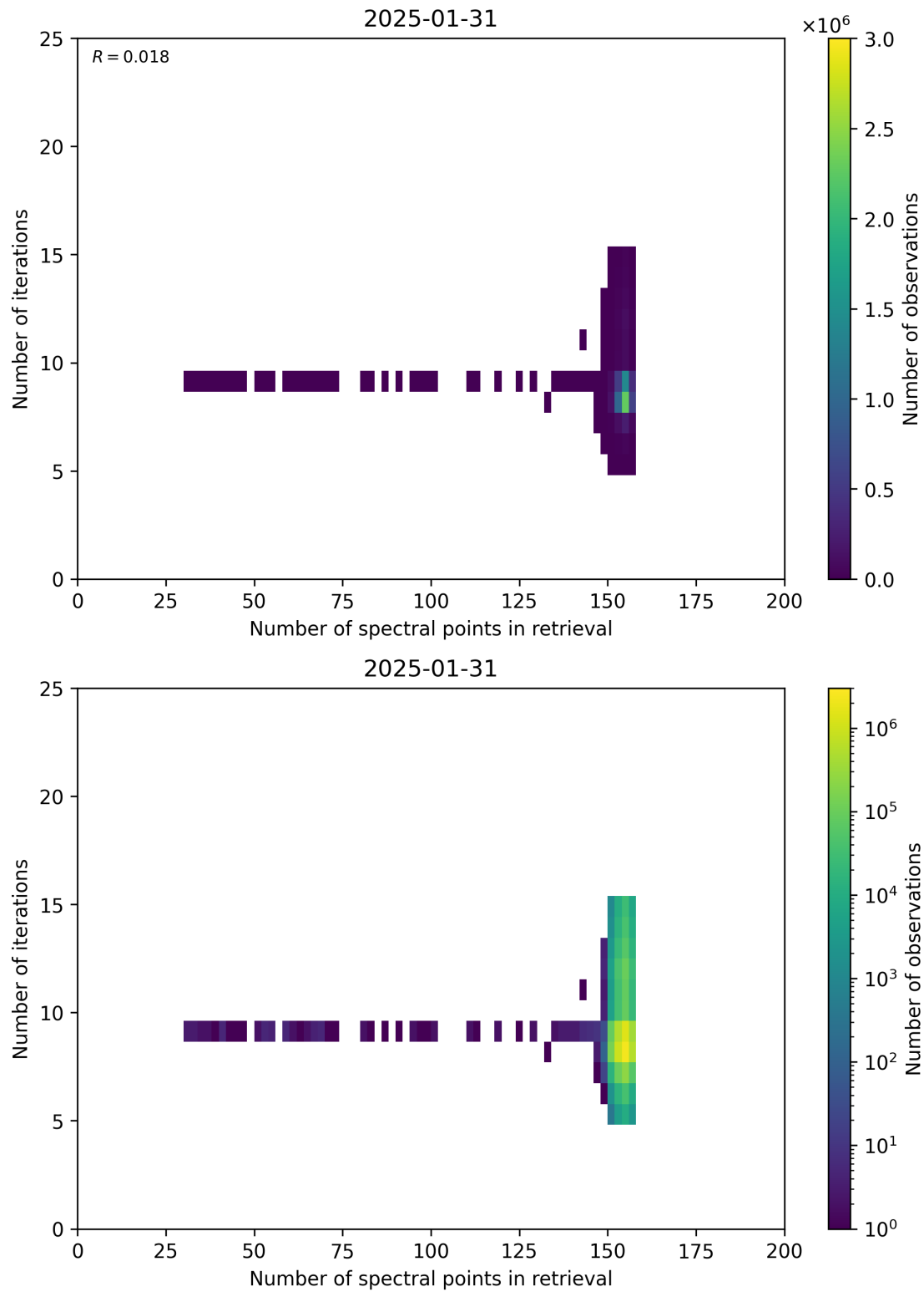
Figure 60: Scatter density plot of “Number of spectral points in retrieval” against “Number of iterations” for 2025-01-30 to 2025-02-01.
