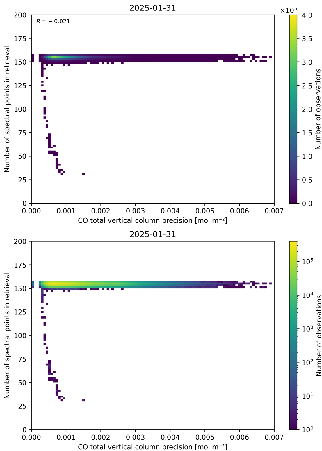
Figure 47: Scatter density plot of “CO total vertical column precision” against “Number of spectral points in retrieval” for 2025-01-30 to 2025-02-01.
