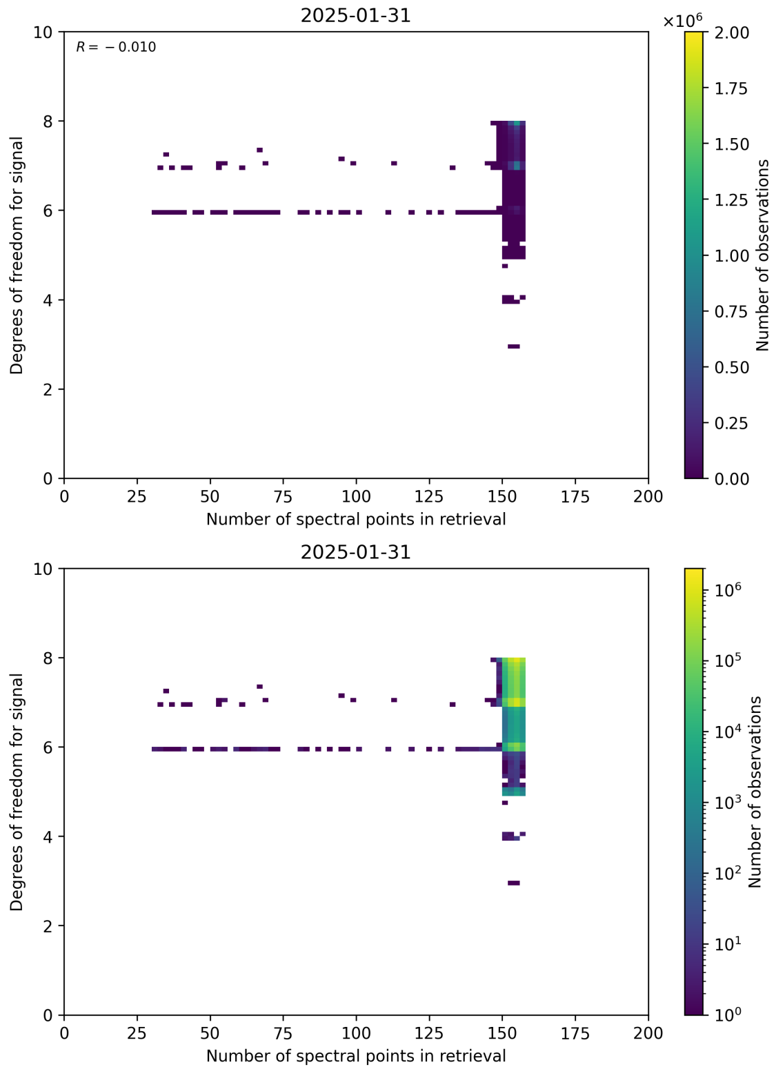
Figure 59: Scatter density plot of “Number of spectral points in retrieval” against “Degrees of freedom for signal” for 2025-01-30 to 2025-02-01.
