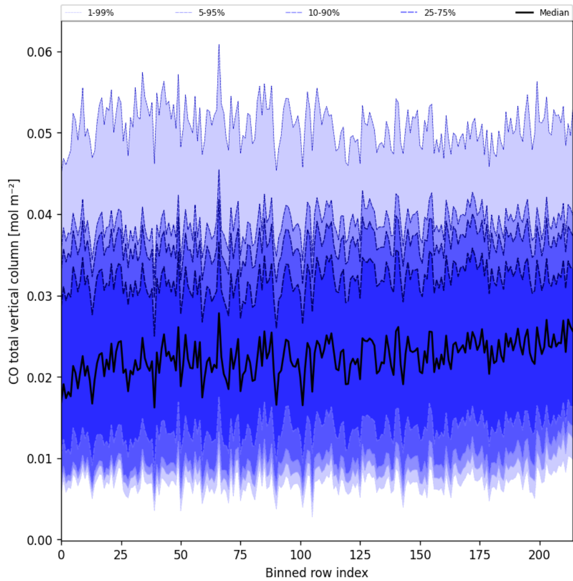
Figure 26: Along track statistics of “CO total vertical column” for 2025-01-30 to 2025-02-01
