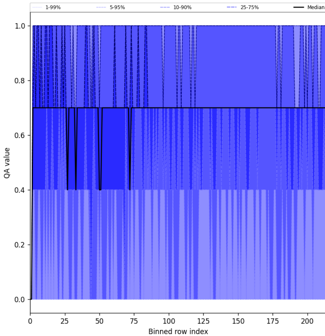
Figure 25: Along track statistics of “QA value” for 2025-01-30 to 2025-02-01
