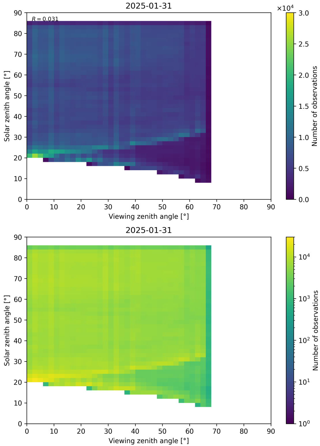
Figure 77: Scatter density plot of “Viewing zenith angle” against “Solar zenith angle” for 2025-01-30 to 2025-02-01.
