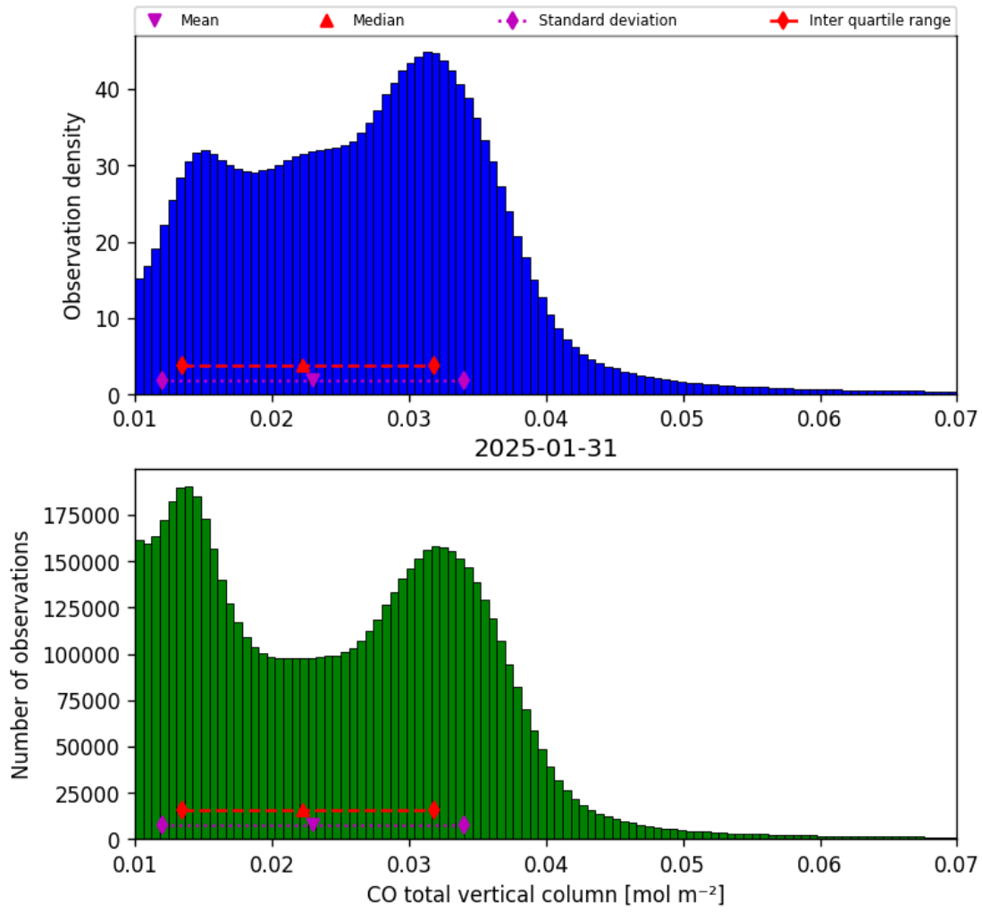
Figure 18: Histogram of “CO total vertical column” for 2025-01-30 to 2025-02-01
