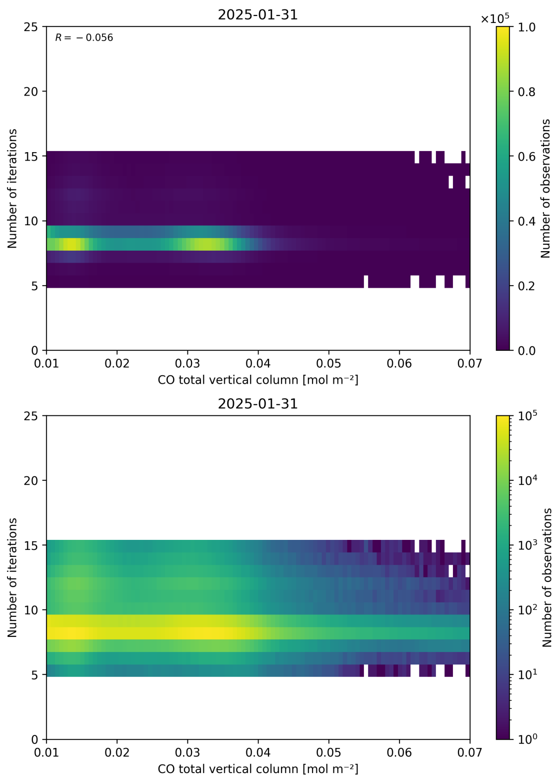
Figure 42: Scatter density plot of “CO total vertical column” against “Number of iterations” for 2025-01-30 to 2025-02-01.
