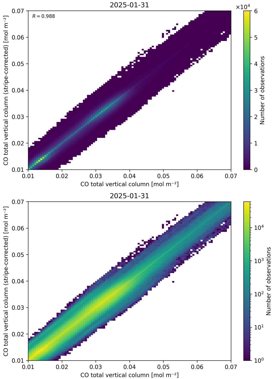
Figure 33: Scatter density plot of “CO total vertical column” against “CO total vertical column (stripe-corrected)” for 2025-01-30 to 2025-02-01.
