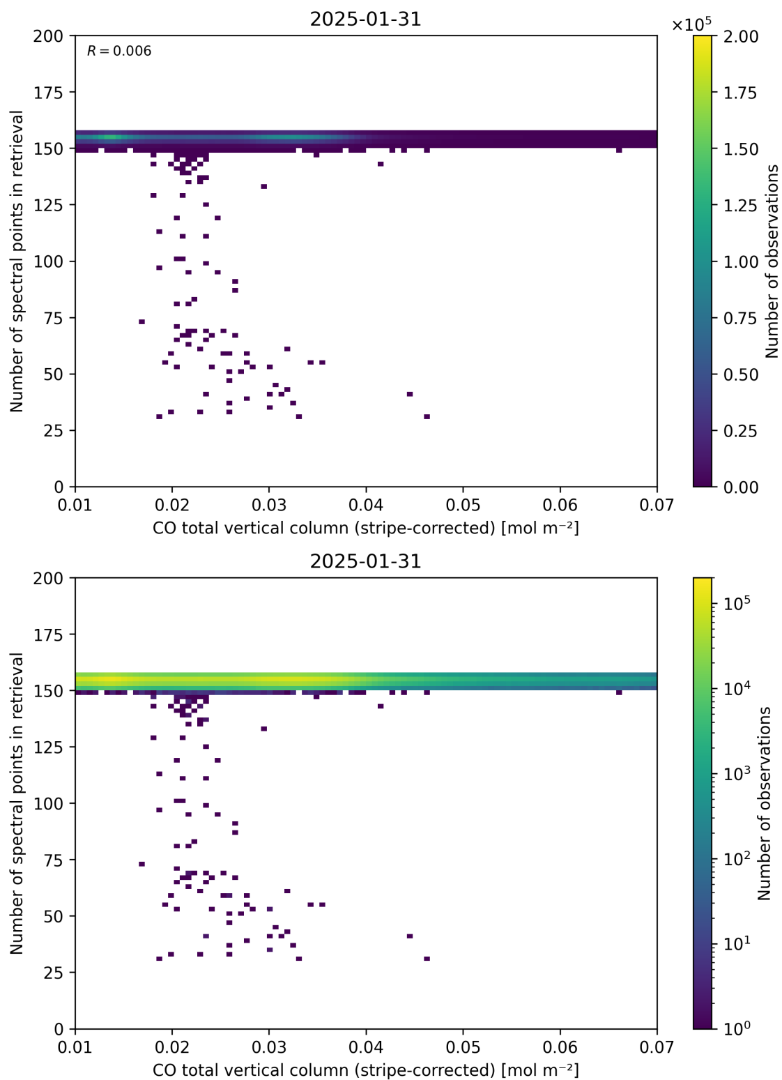
Figure 40: Scatter density plot of “CO total vertical column (stripe-corrected)” against “Number of spectral points in retrieval” for 2025-01-30 to 2025-02-01.
