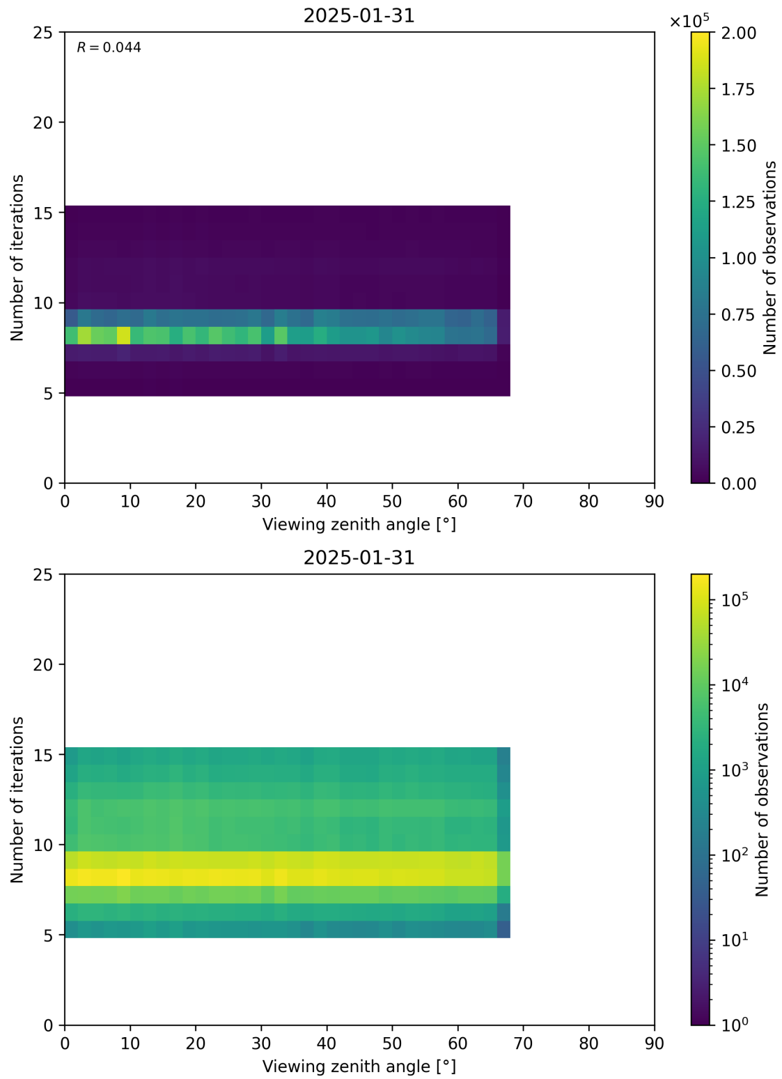
Figure 75: Scatter density plot of “Viewing zenith angle” against “Number of iterations” for 2025-01-30 to 2025-02-01.
