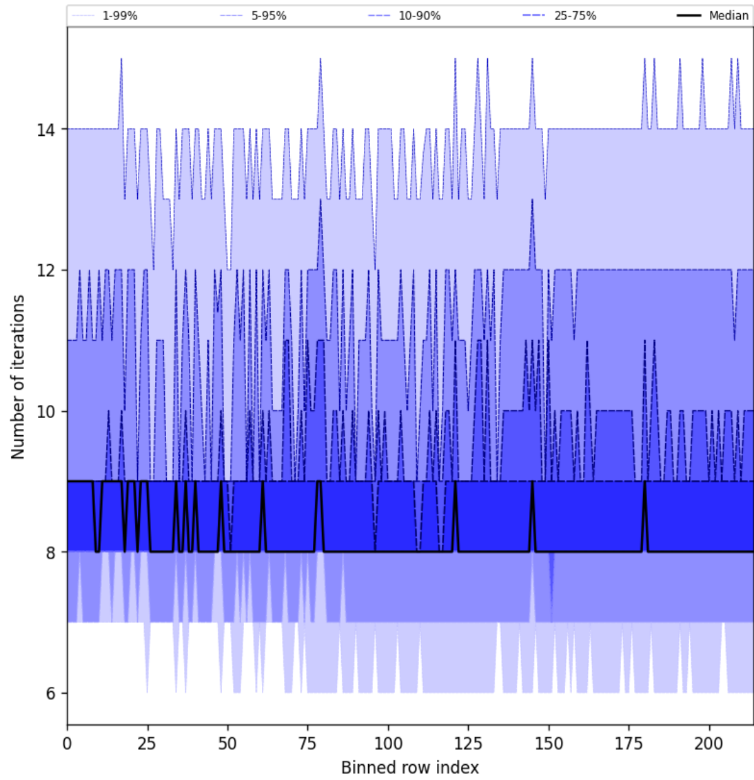
Figure 32: Along track statistics of “Number of iterations” for 2025-01-30 to 2025-02-01
