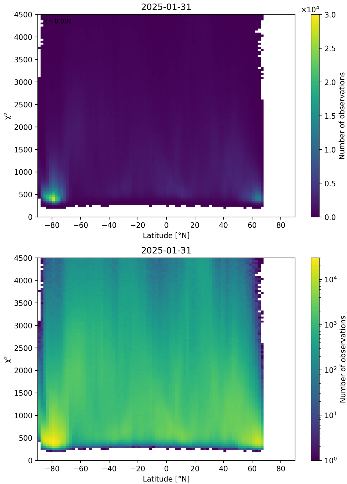
Figure 54: Scatter density plot of “Latitude” against “ \chi^2 ” for 2025-01-30 to 2025-02-01.
