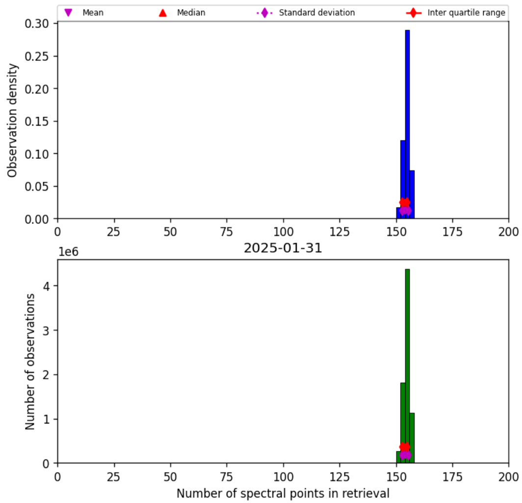
Figure 21: Histogram of “Number of spectral points in retrieval” for 2025-01-30 to 2025-02-01
