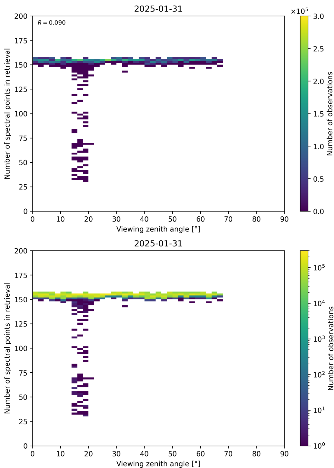
Figure 76: Scatter density plot of “Viewing zenith angle” against “Number of spectral points in retrieval” for 2025-01-30 to 2025-02-01.
