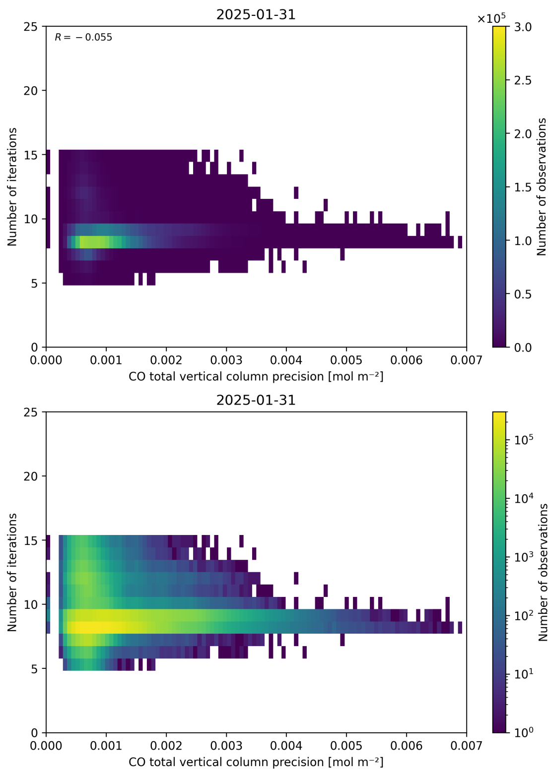
Figure 46: Scatter density plot of “CO total vertical column precision” against “Number of iterations” for 2025-01-30 to 2025-02-01.
