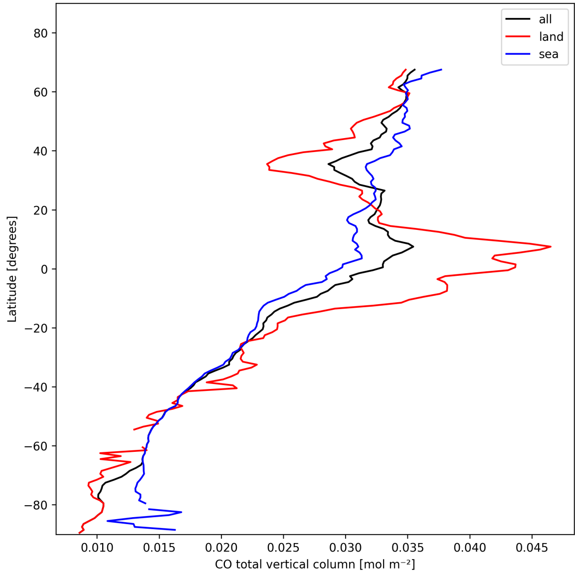
Figure 10: Zonal average of “CO total vertical column” for 2025-01-30 to 2025-02-01.
