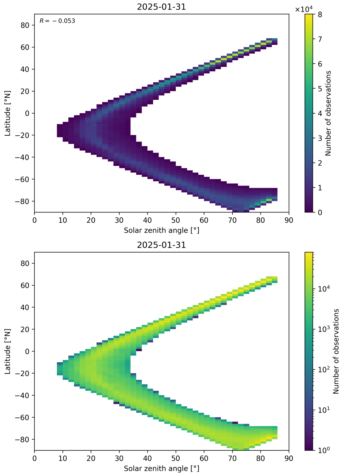
Figure 66: Scatter density plot of “Solar zenith angle” against “Latitude” for 2025-01-30 to 2025-02-01.
