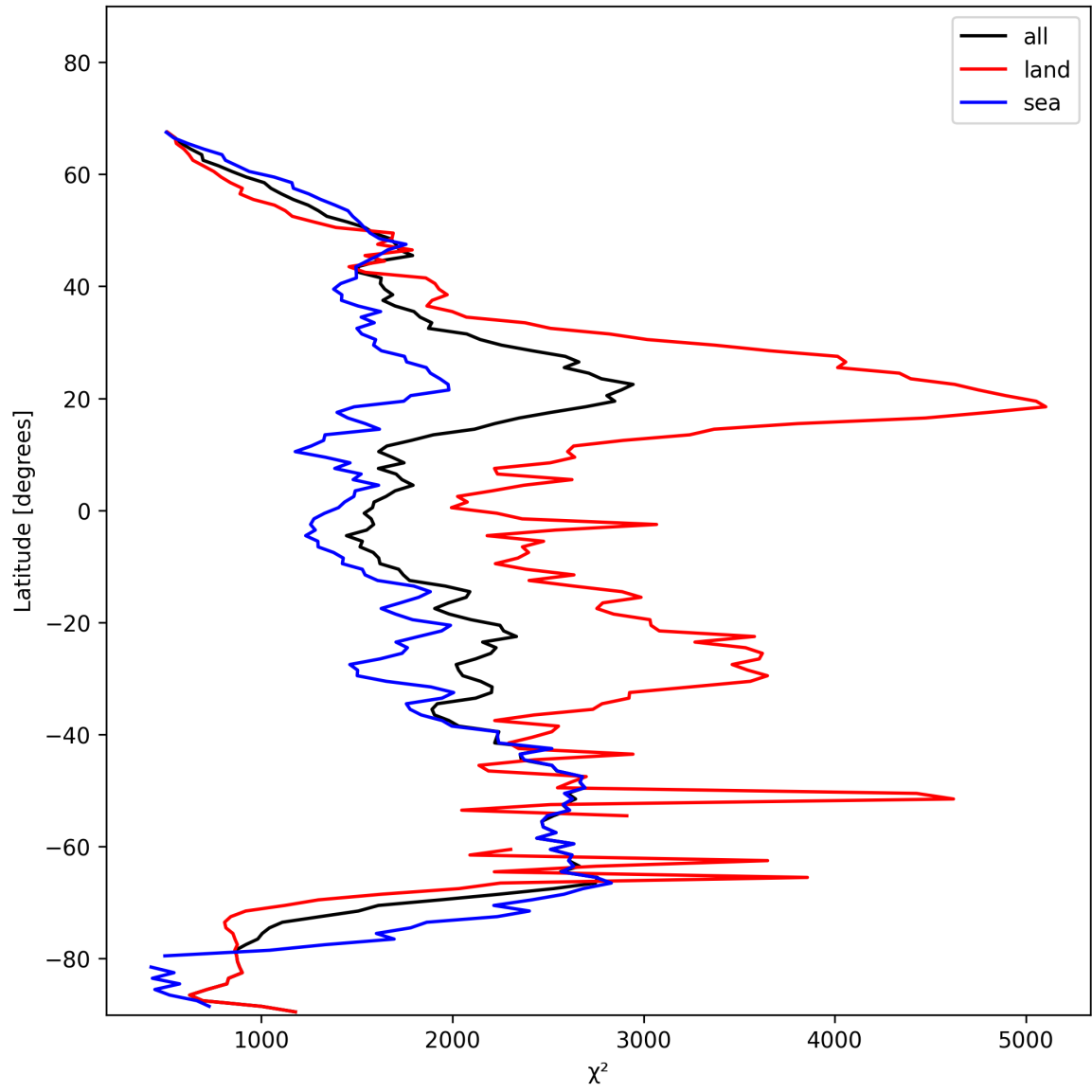
Figure 14: Zonal average of “ \chi^2 ” for 2025-01-30 to 2025-02-01.
