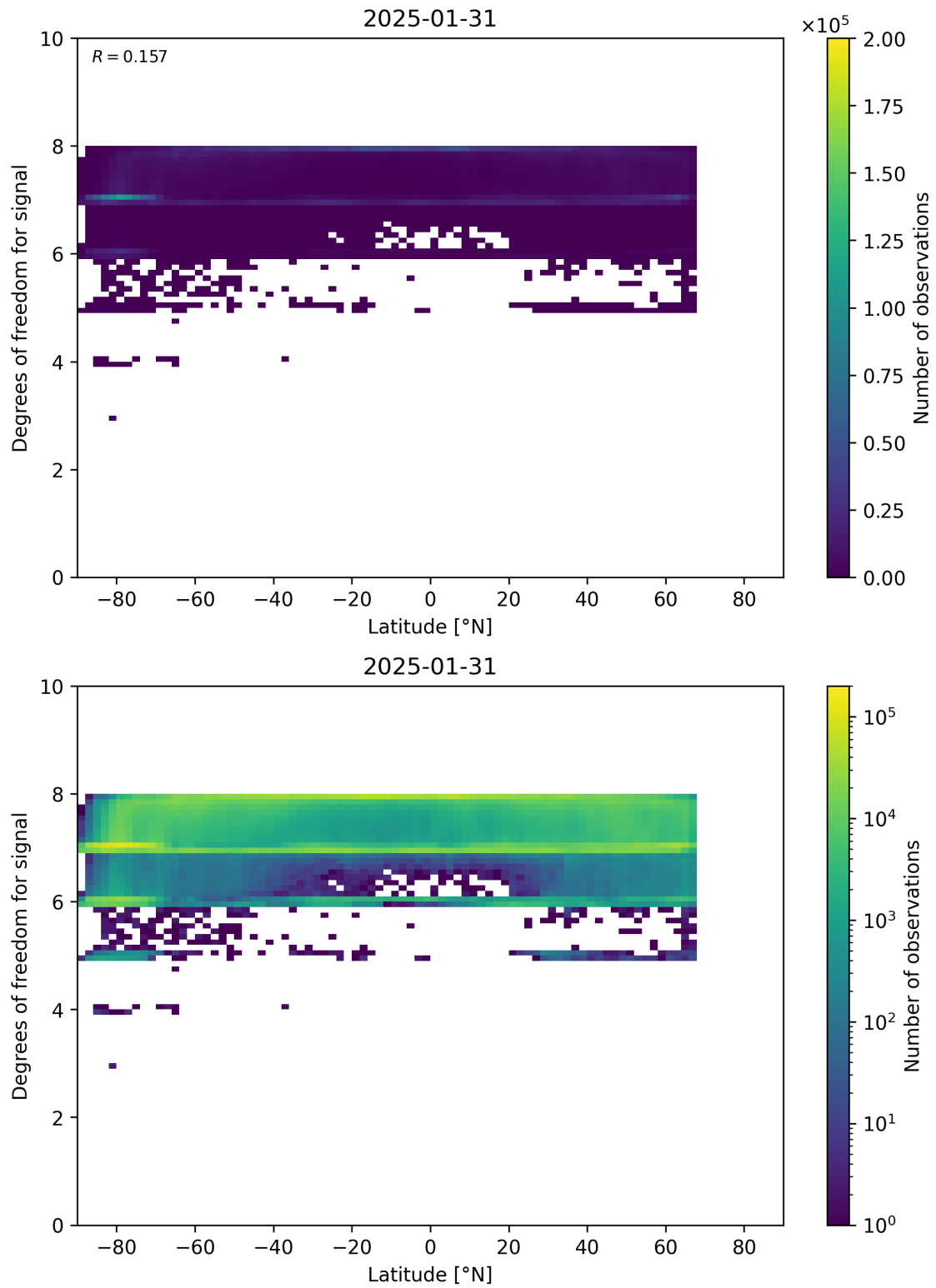
Figure 55: Scatter density plot of “Latitude” against “Degrees of freedom for signal” for 2025-01-30 to 2025-02-01.
