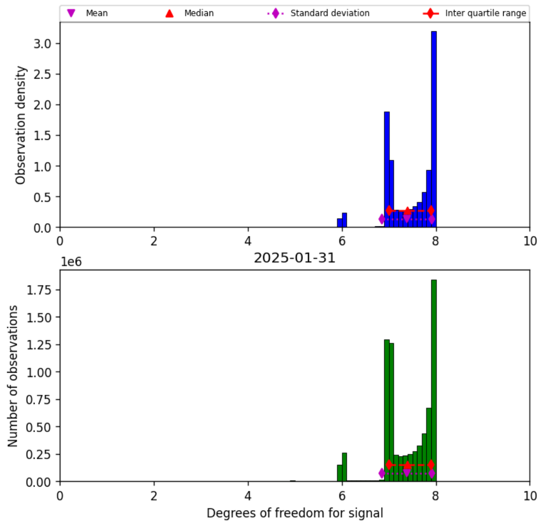
Figure 23: Histogram of “Degrees of freedom for signal” for 2025-01-30 to 2025-02-01
