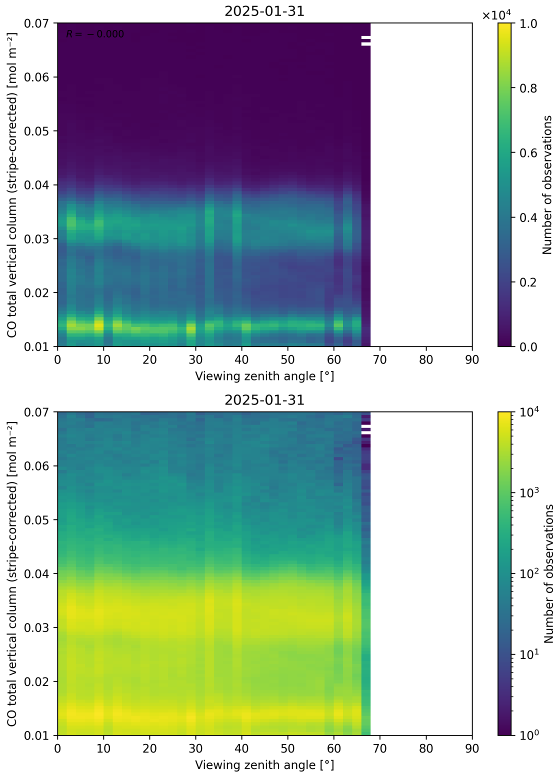
Figure 70: Scatter density plot of “Viewing zenith angle” against “CO total vertical column (stripe-corrected)” for 2025-01-30 to 2025-02-01.
