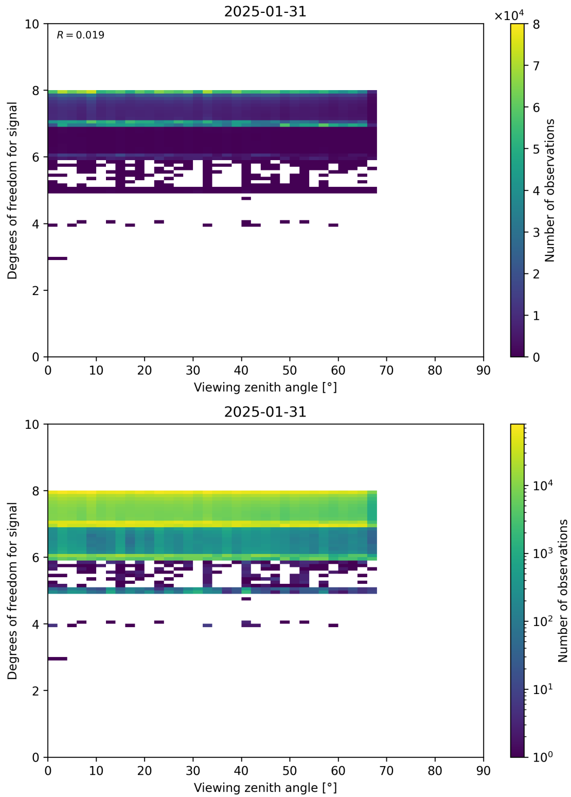
Figure 73: Scatter density plot of “Viewing zenith angle” against “Degrees of freedom for signal” for 2025-01-30 to 2025-02-01.
