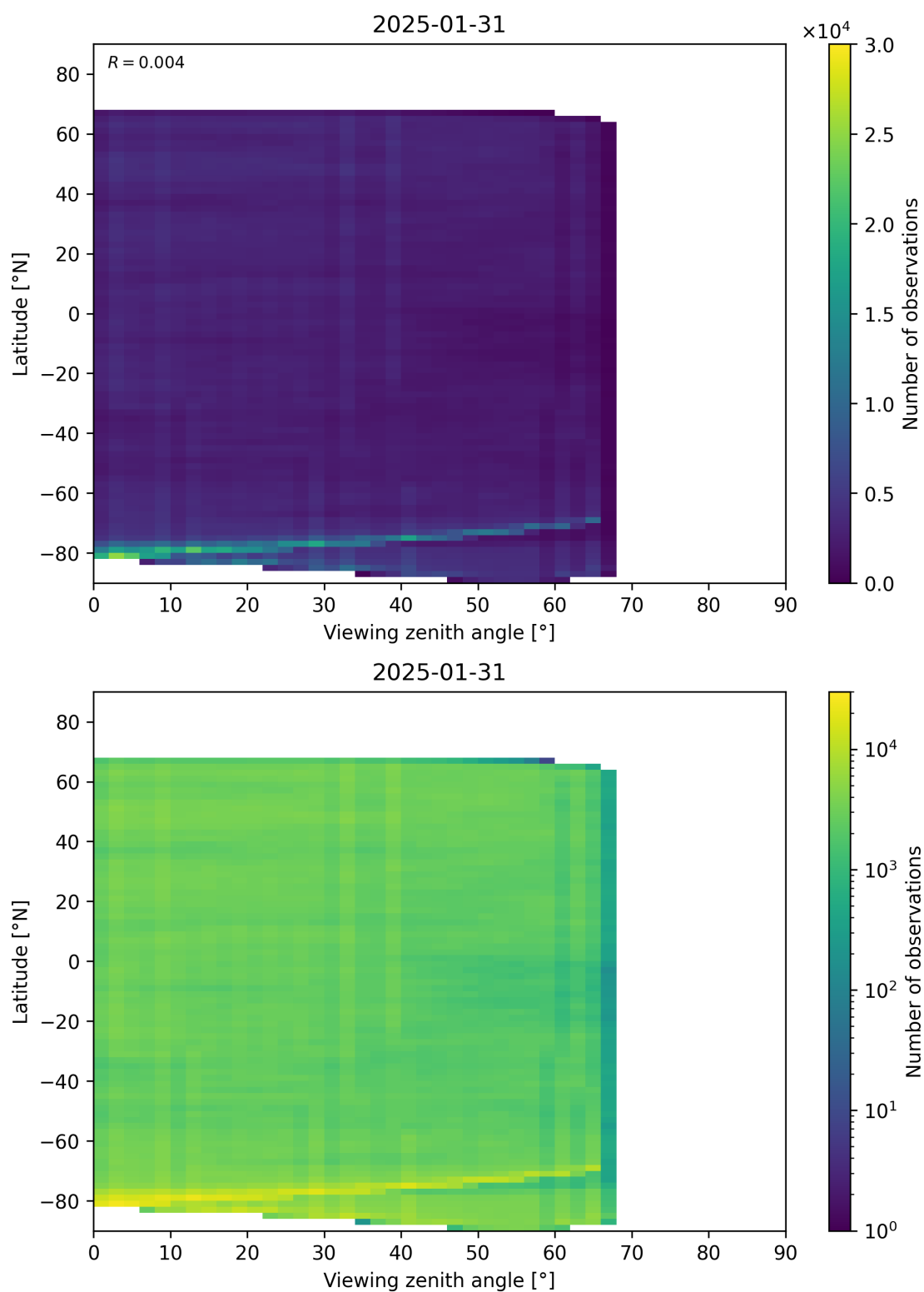
Figure 74: Scatter density plot of “Viewing zenith angle” against “Latitude” for 2025-01-30 to 2025-02-01.
