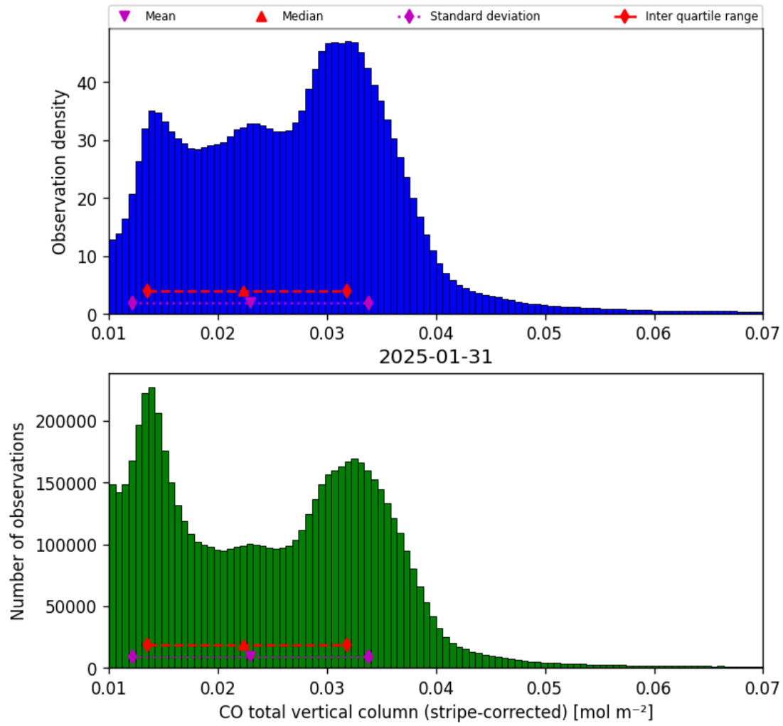
Figure 19: Histogram of “CO total vertical column (stripe-corrected)” for 2025-01-30 to 2025-02-01
