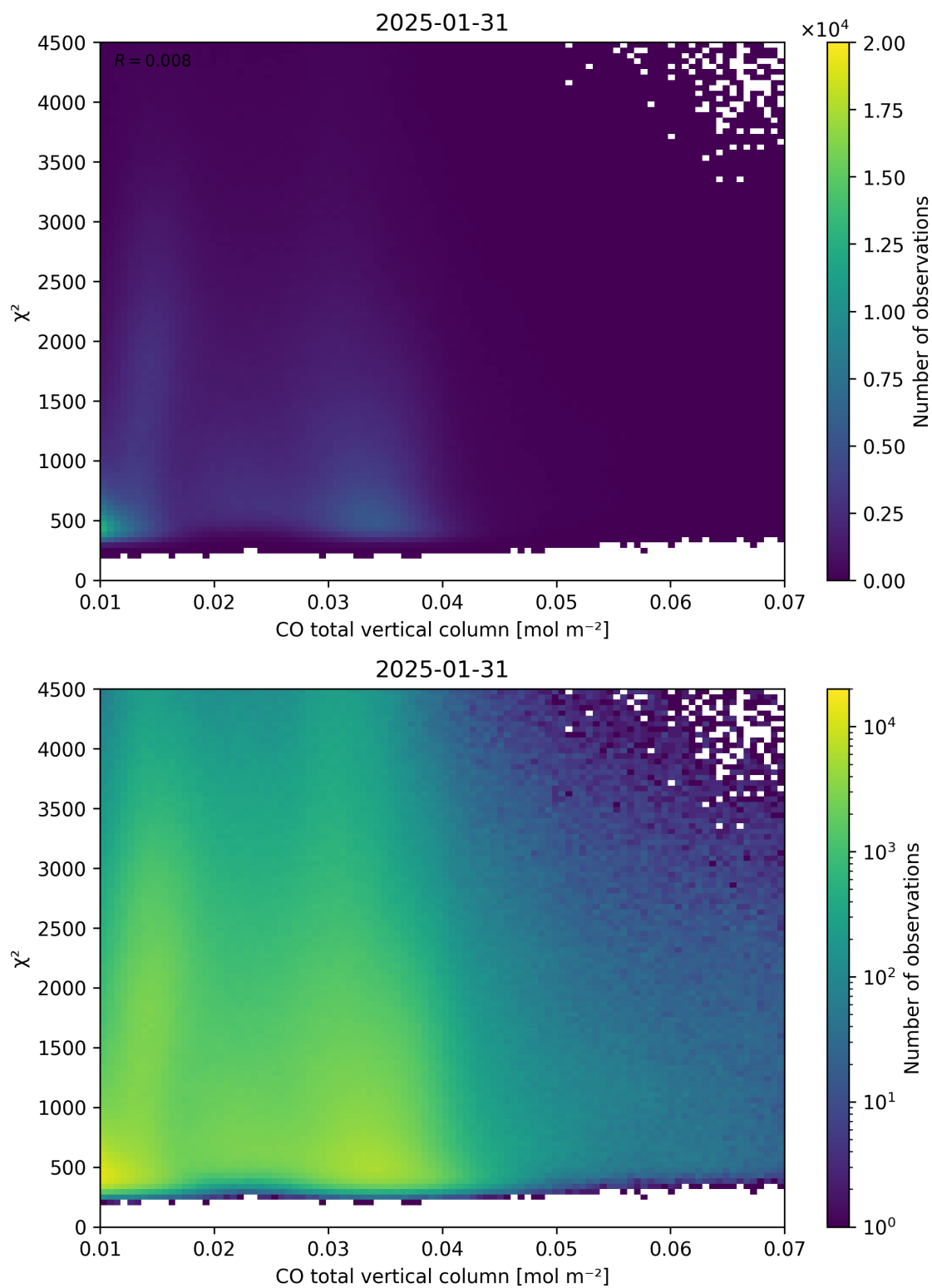
Figure 35: Scatter density plot of “CO total vertical column” against “ \chi^2 ” for 2025-01-30 to 2025-02-01.
