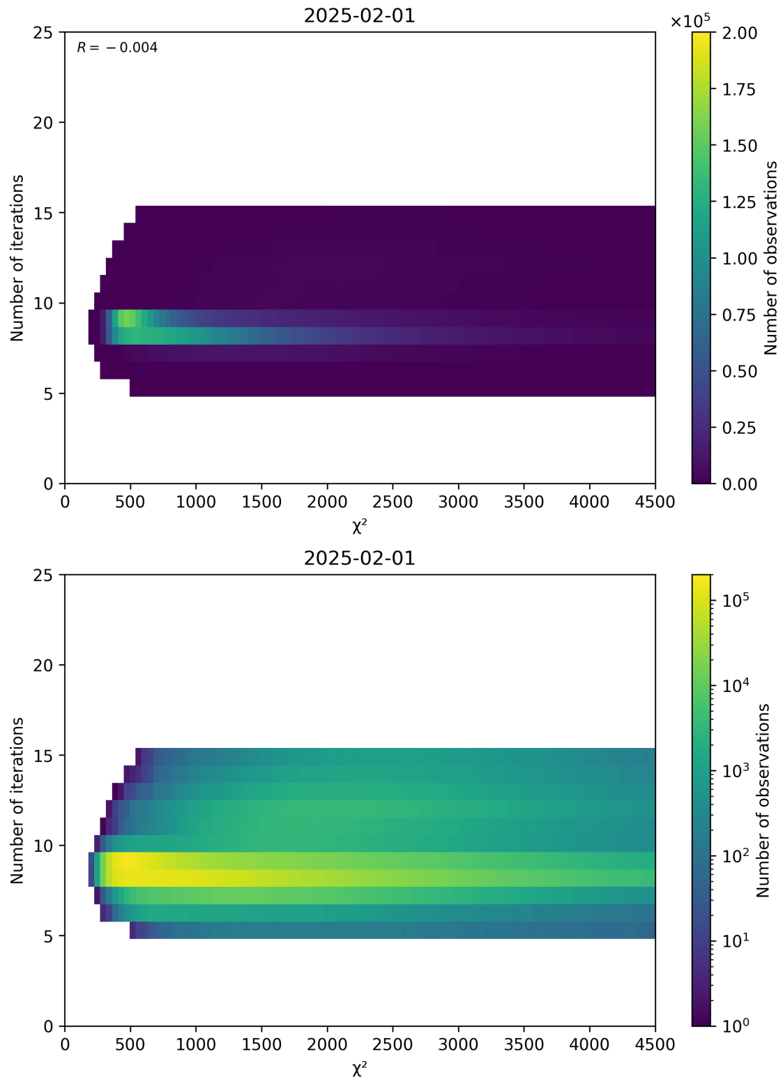
Figure 49: Scatter density plot of “ \chi^2 ” against “Number of iterations” for 2025-01-31 to 2025-02-02.
