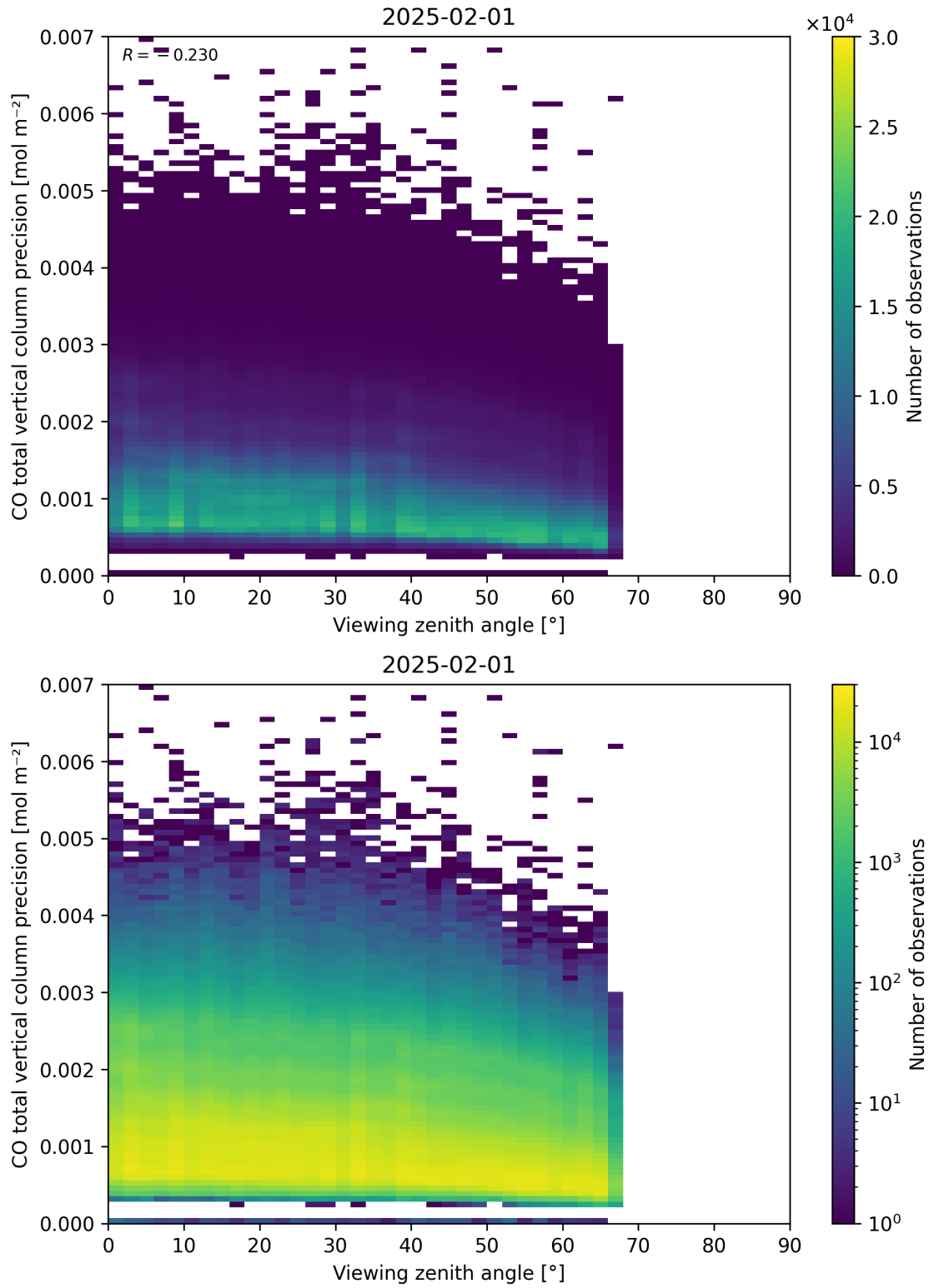
Figure 71: Scatter density plot of “Viewing zenith angle” against “CO total vertical column precision” for 2025-01-31 to 2025-02-02.
