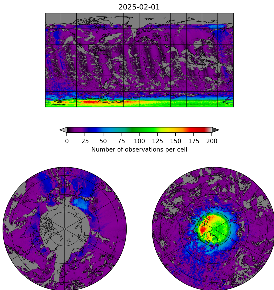
Figure 8: Map of the number of observations for 2025-01-31 to 2025-02-02
