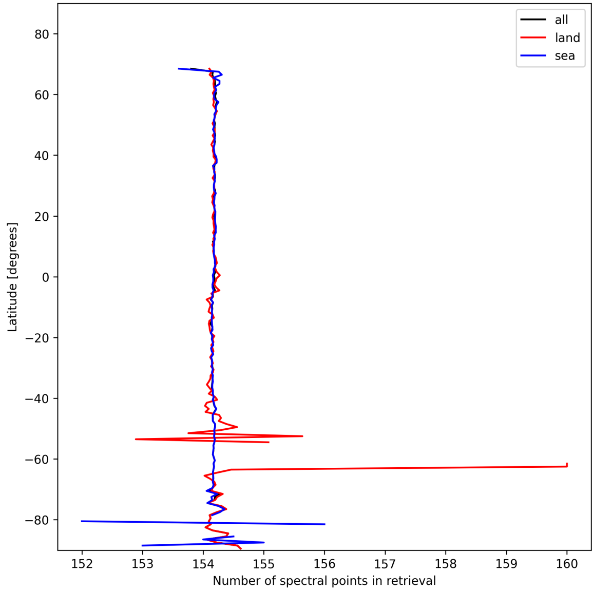
Figure 13: Zonal average of “Number of spectral points in retrieval” for 2025-01-31 to 2025-02-02.
