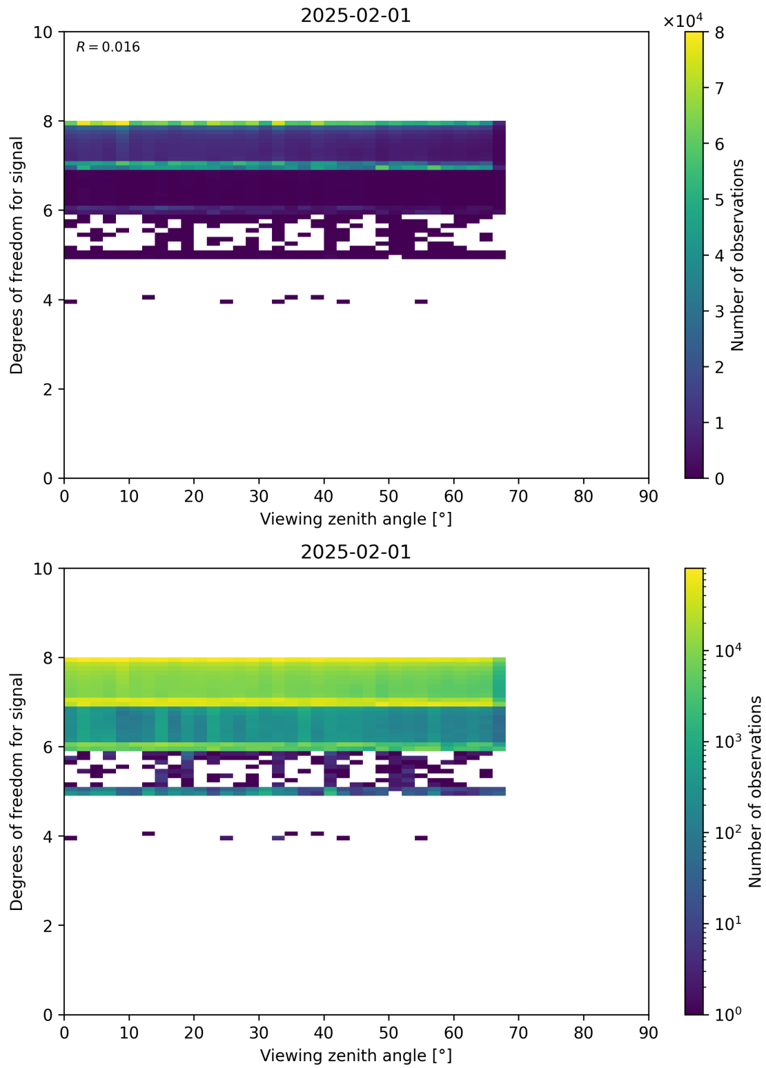
Figure 73: Scatter density plot of “Viewing zenith angle” against “Degrees of freedom for signal” for 2025-01-31 to 2025-02-02.
