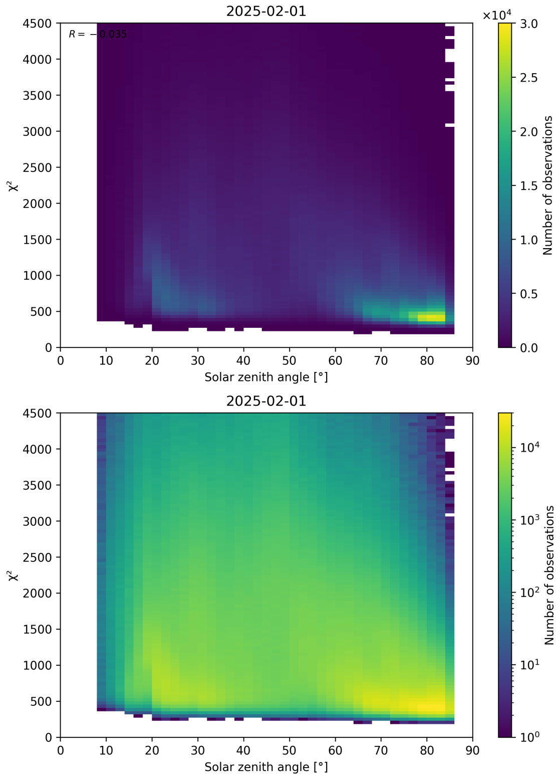
Figure 64: Scatter density plot of “Solar zenith angle” against “ \chi^2 ” for 2025-01-31 to 2025-02-02.
