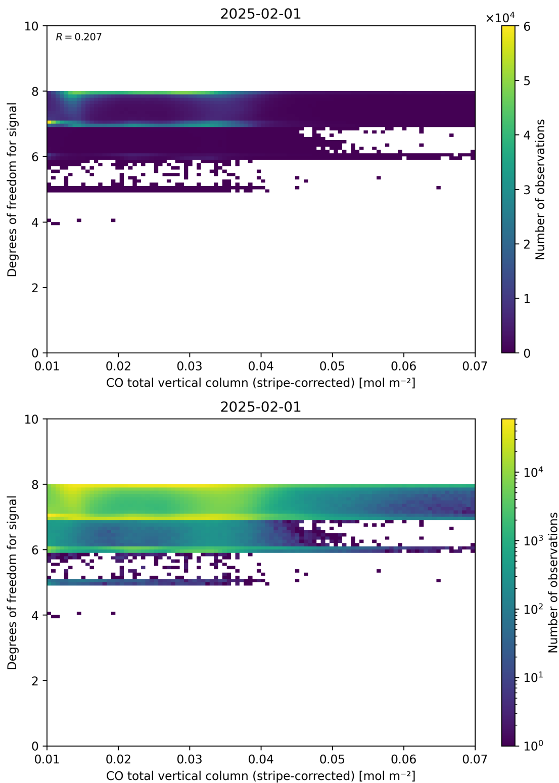
Figure 38: Scatter density plot of “CO total vertical column (stripe-corrected)” against “Degrees of freedom for signal” for 2025-01-31 to 2025-02-02.
