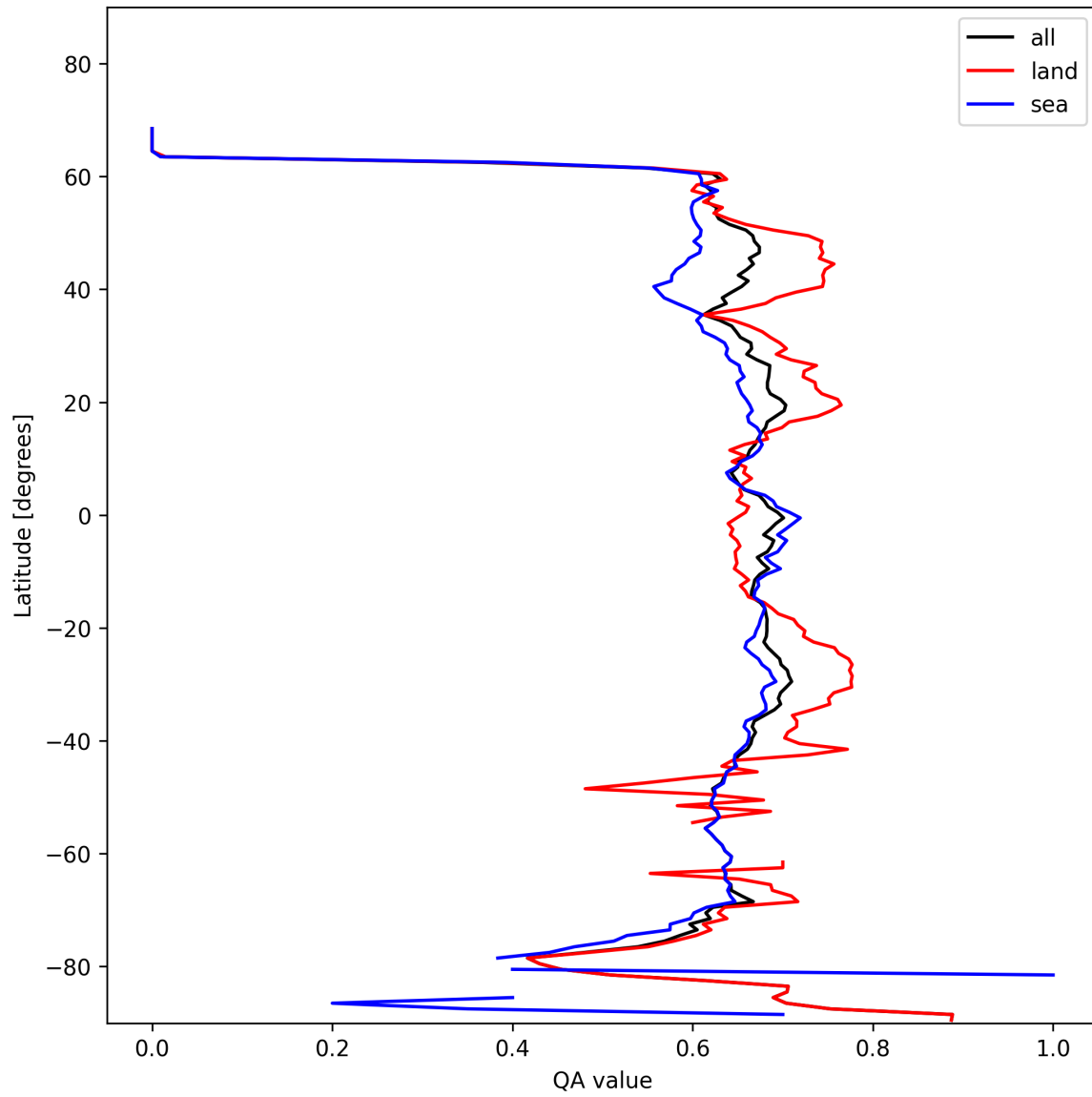
Figure 9: Zonal average of “QA value” for 2025-01-31 to 2025-02-02.
