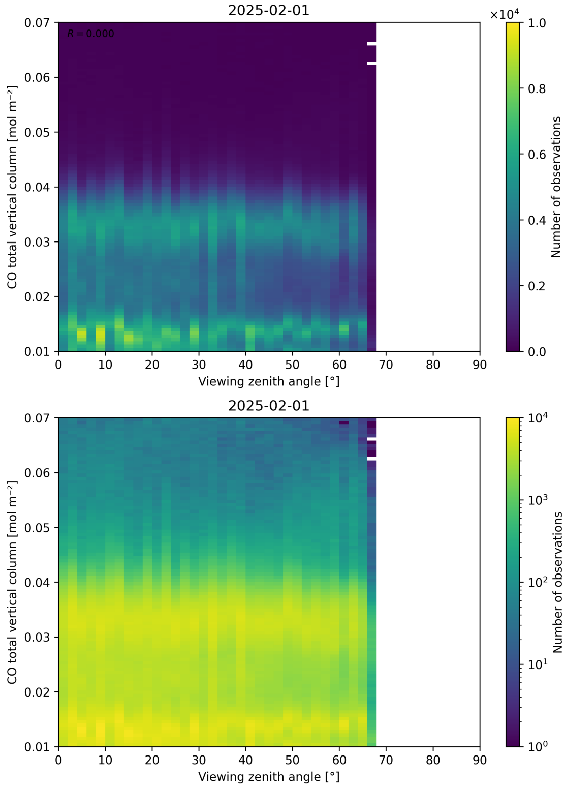
Figure 69: Scatter density plot of “Viewing zenith angle” against “CO total vertical column” for 2025-01-31 to 2025-02-02.
