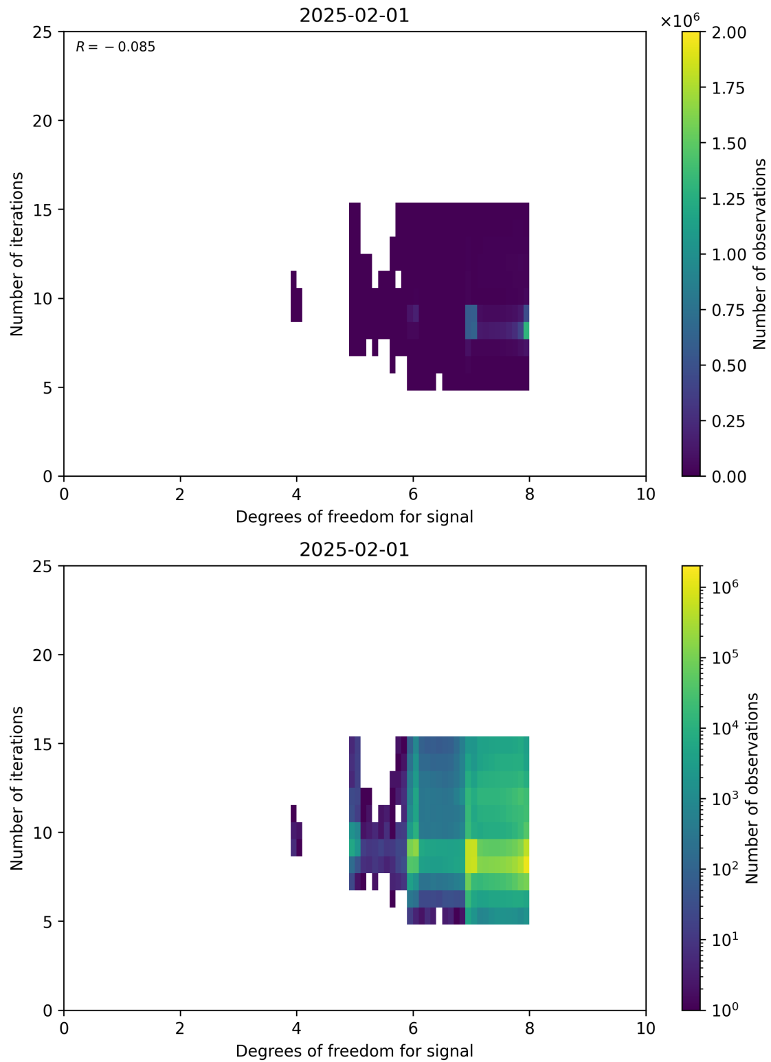
Figure 50: Scatter density plot of “Degrees of freedom for signal” against “Number of iterations” for 2025-01-31 to 2025-02-02.
