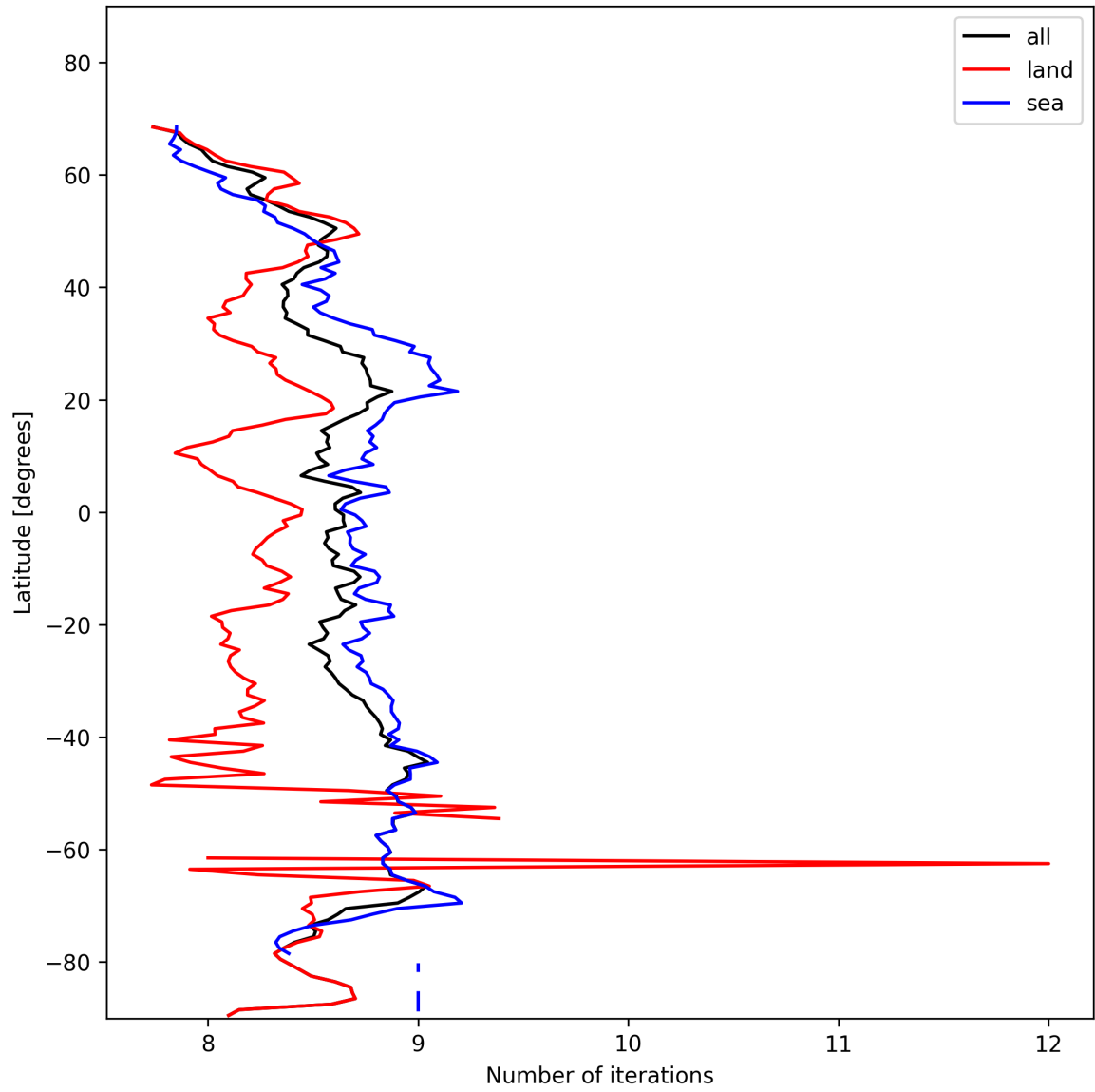
Figure 16: Zonal average of “Number of iterations” for 2025-01-31 to 2025-02-02.
