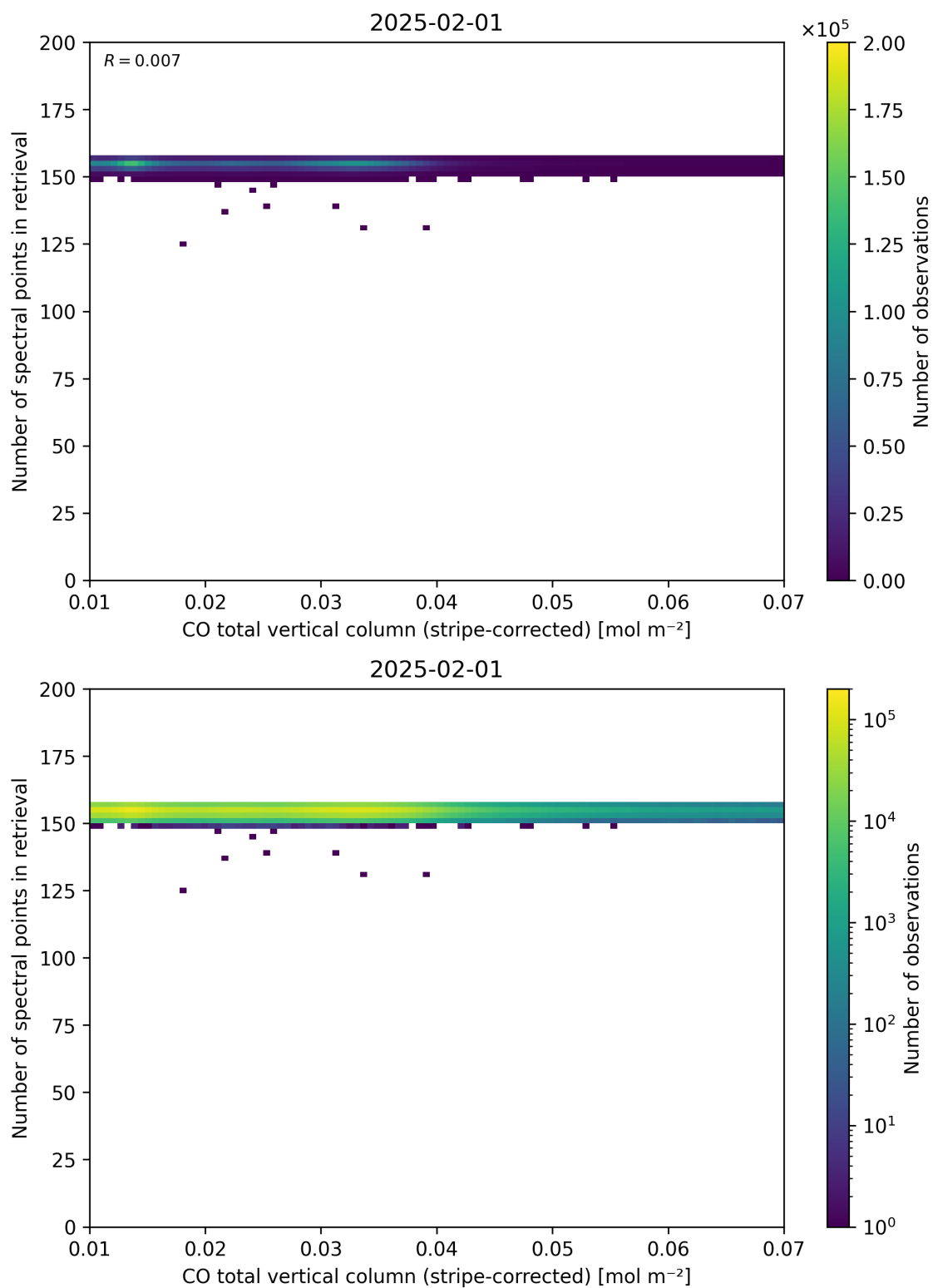
Figure 40: Scatter density plot of “CO total vertical column (stripe-corrected)” against “Number of spectral points in retrieval” for 2025-01-31 to 2025-02-02.
