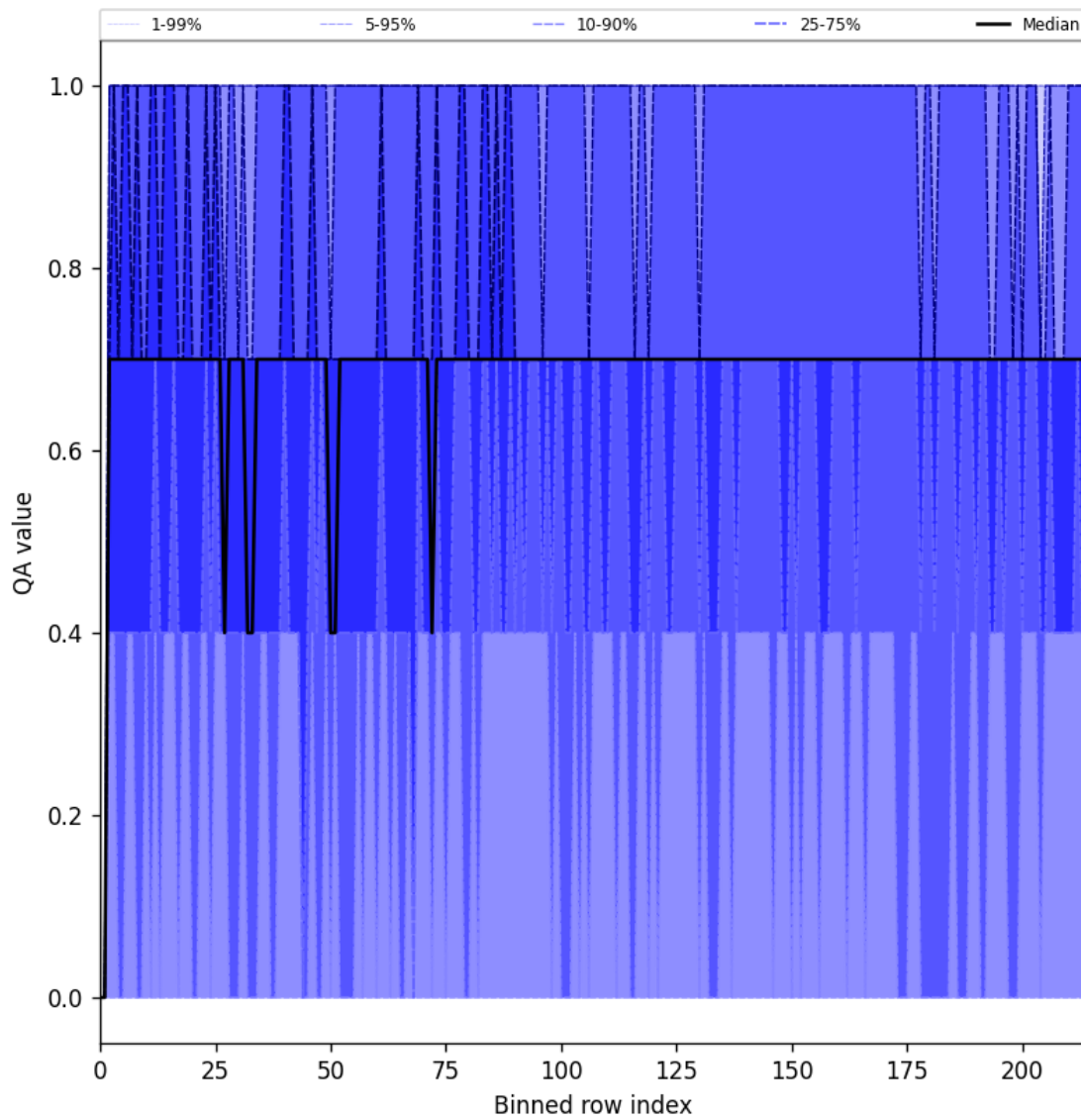
Figure 25: Along track statistics of “QA value” for 2025-01-31 to 2025-02-02
