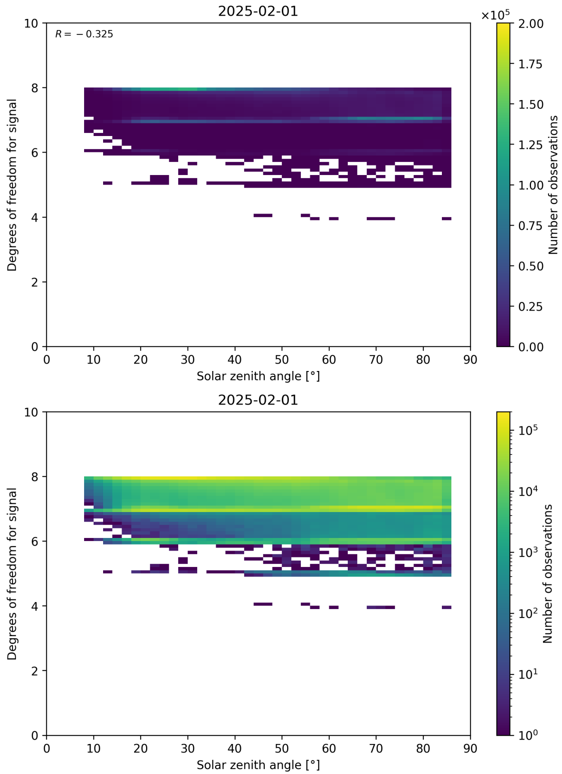
Figure 65: Scatter density plot of “Solar zenith angle” against “Degrees of freedom for signal” for 2025-01-31 to 2025-02-02.
