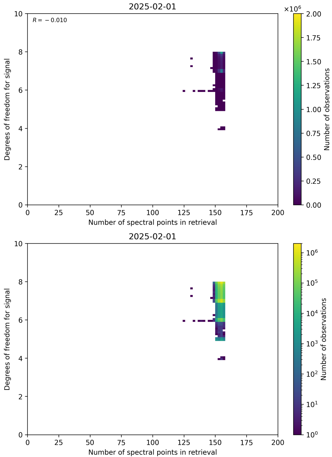
Figure 59: Scatter density plot of “Number of spectral points in retrieval” against “Degrees of freedom for signal” for 2025-01-31 to 2025-02-02.
