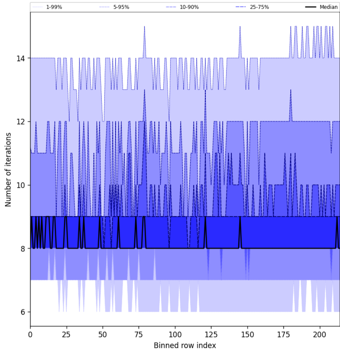
Figure 32: Along track statistics of “Number of iterations” for 2025-01-31 to 2025-02-02
