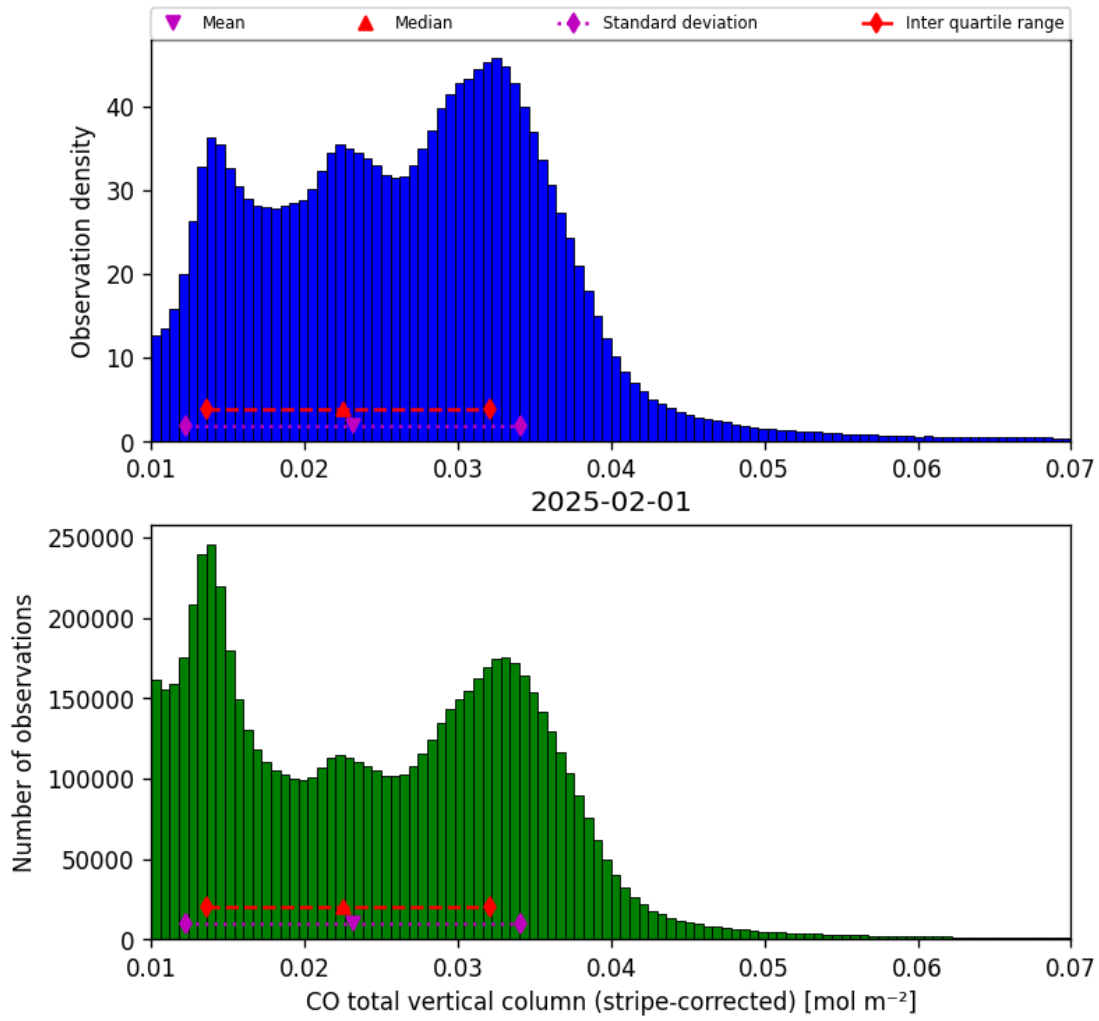
Figure 19: Histogram of “CO total vertical column (stripe-corrected)” for 2025-01-31 to 2025-02-02
