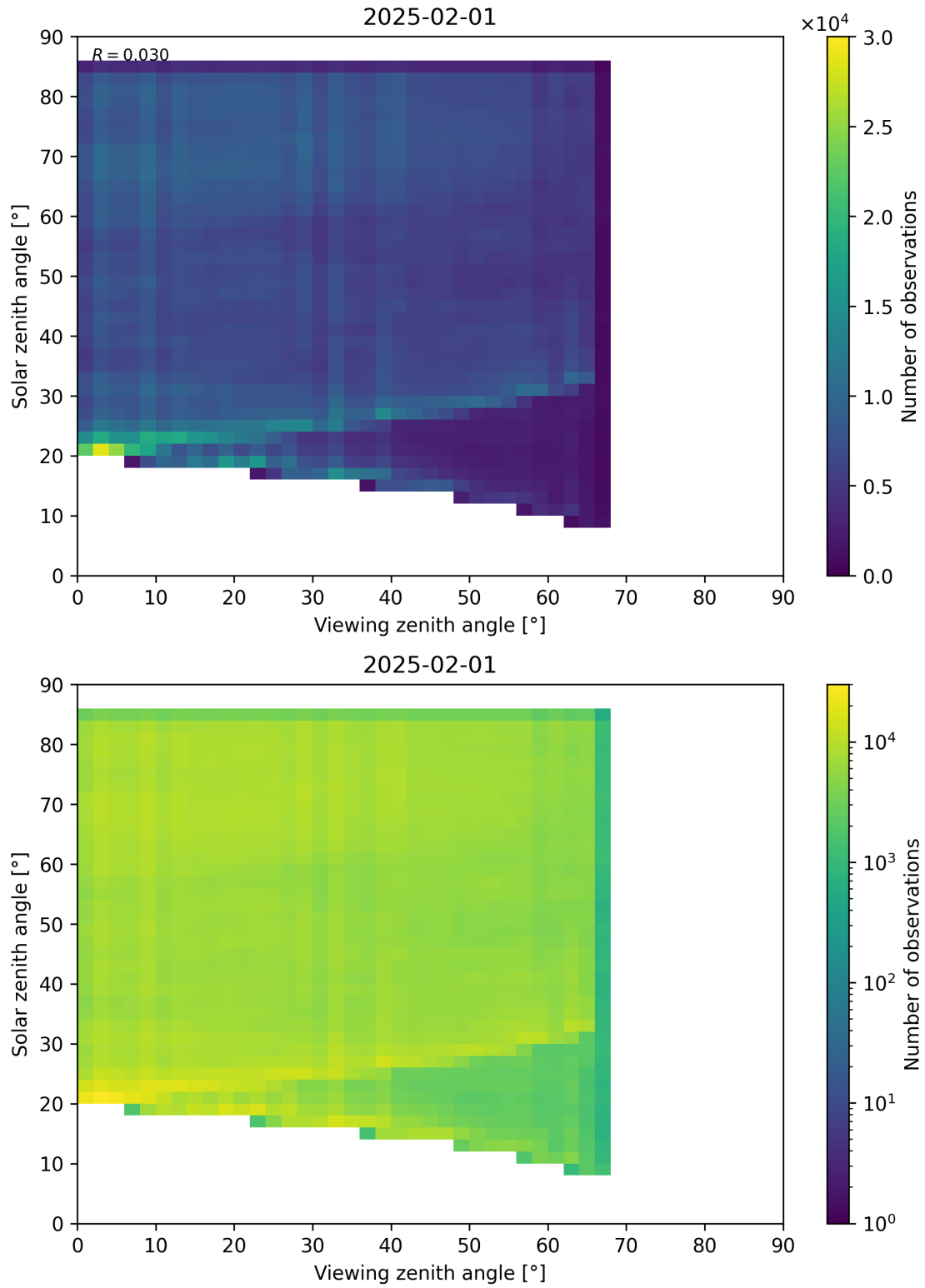
Figure 77: Scatter density plot of “Viewing zenith angle” against “Solar zenith angle” for 2025-01-31 to 2025-02-02.
