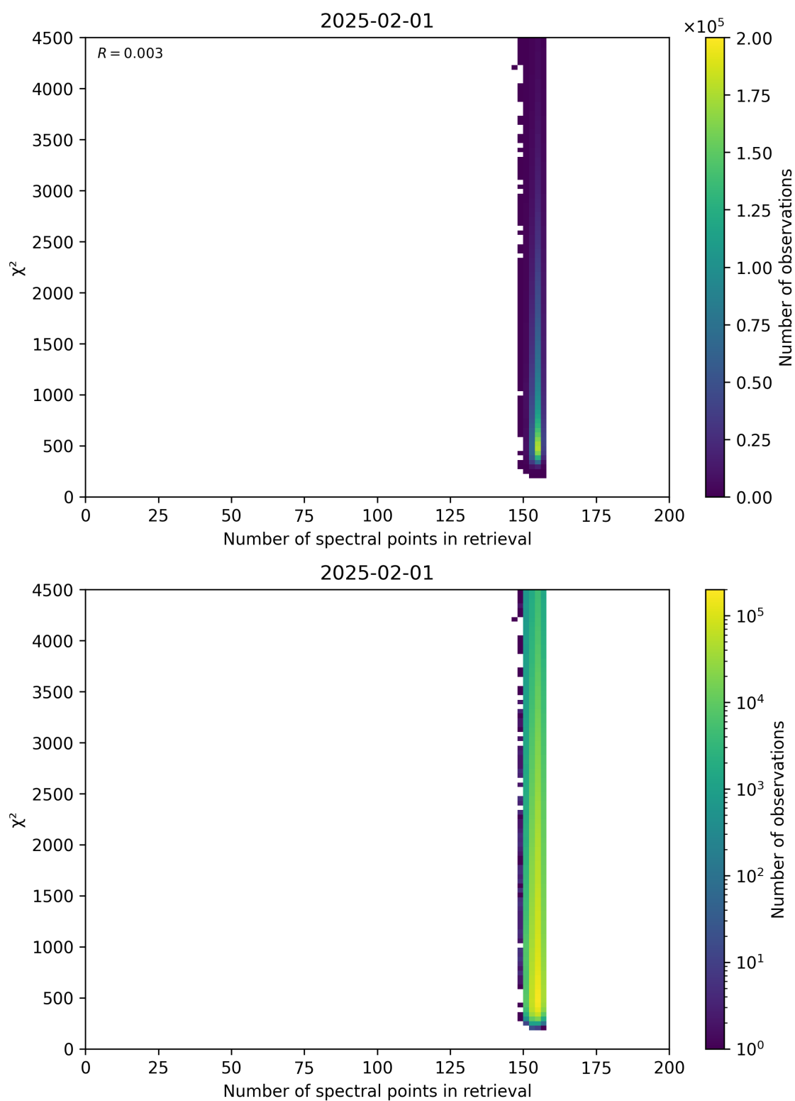
Figure 58: Scatter density plot of “Number of spectral points in retrieval” against “ \chi^2 ” for 2025-01-31 to 2025-02-02.
