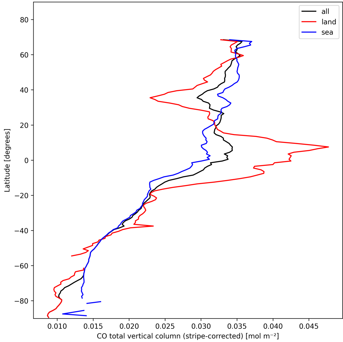
Figure 11: Zonal average of “CO total vertical column (stripe-corrected)” for 2025-01-31 to 2025-02-02.
