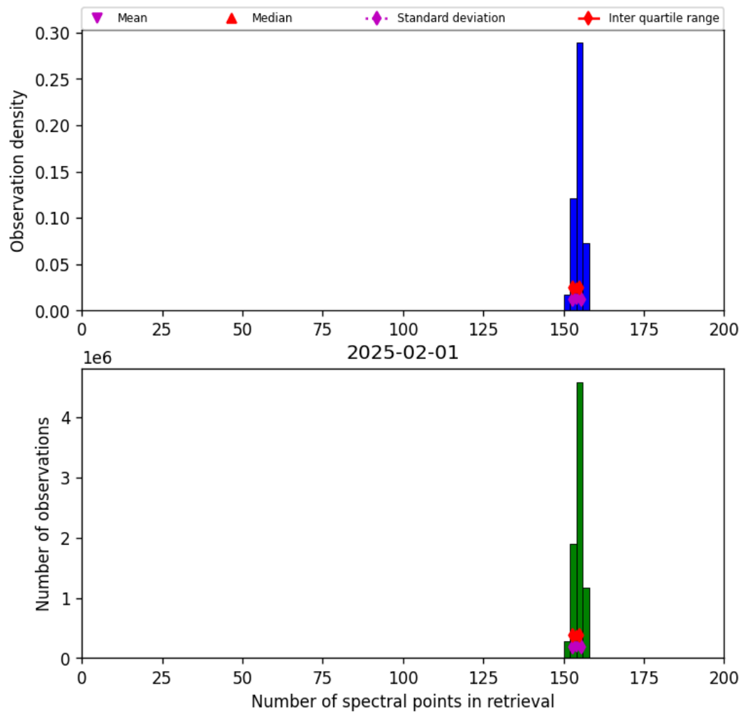
Figure 21: Histogram of “Number of spectral points in retrieval” for 2025-01-31 to 2025-02-02
