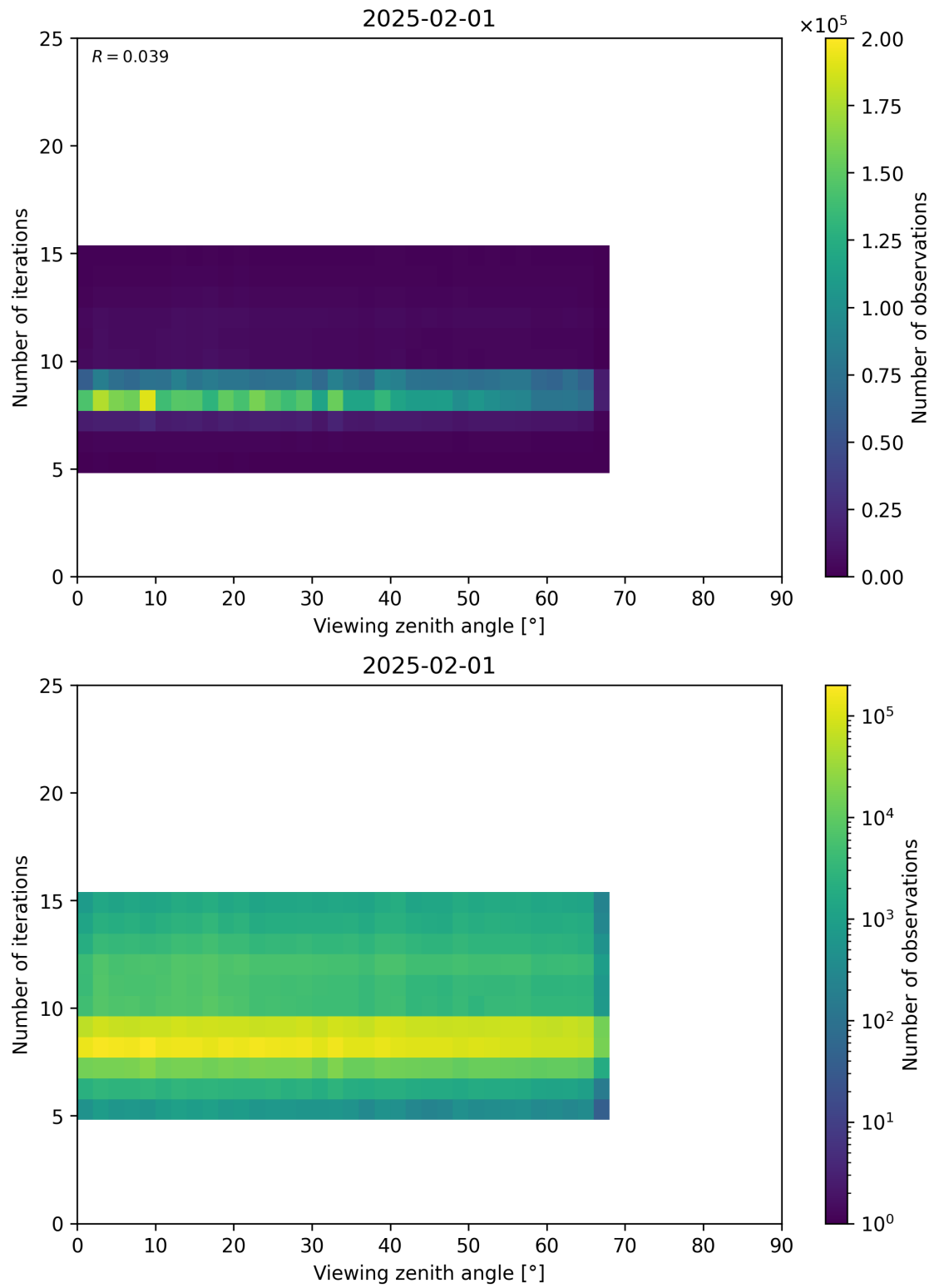
Figure 75: Scatter density plot of “Viewing zenith angle” against “Number of iterations” for 2025-01-31 to 2025-02-02.
