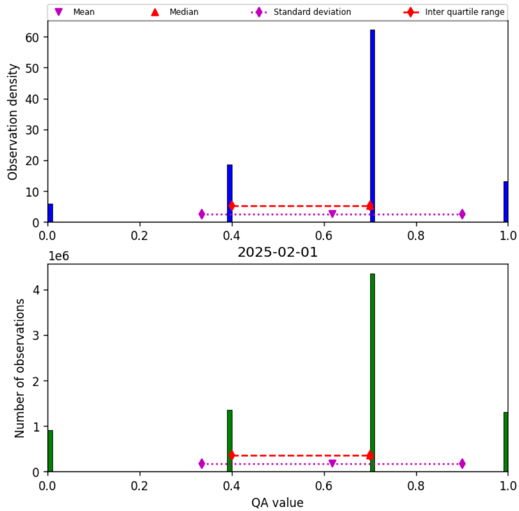
Figure 17: Histogram of “QA value” for 2025-01-31 to 2025-02-02
