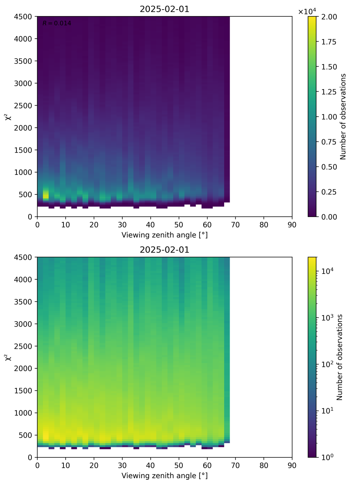
Figure 72: Scatter density plot of “Viewing zenith angle” against “ \chi^2 ” for 2025-01-31 to 2025-02-02.
