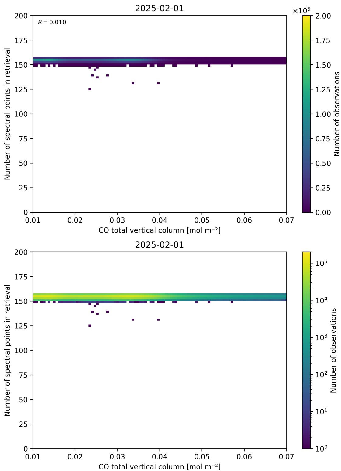
Figure 43: Scatter density plot of “CO total vertical column” against “Number of spectral points in retrieval” for 2025-01-31 to 2025-02-02.
