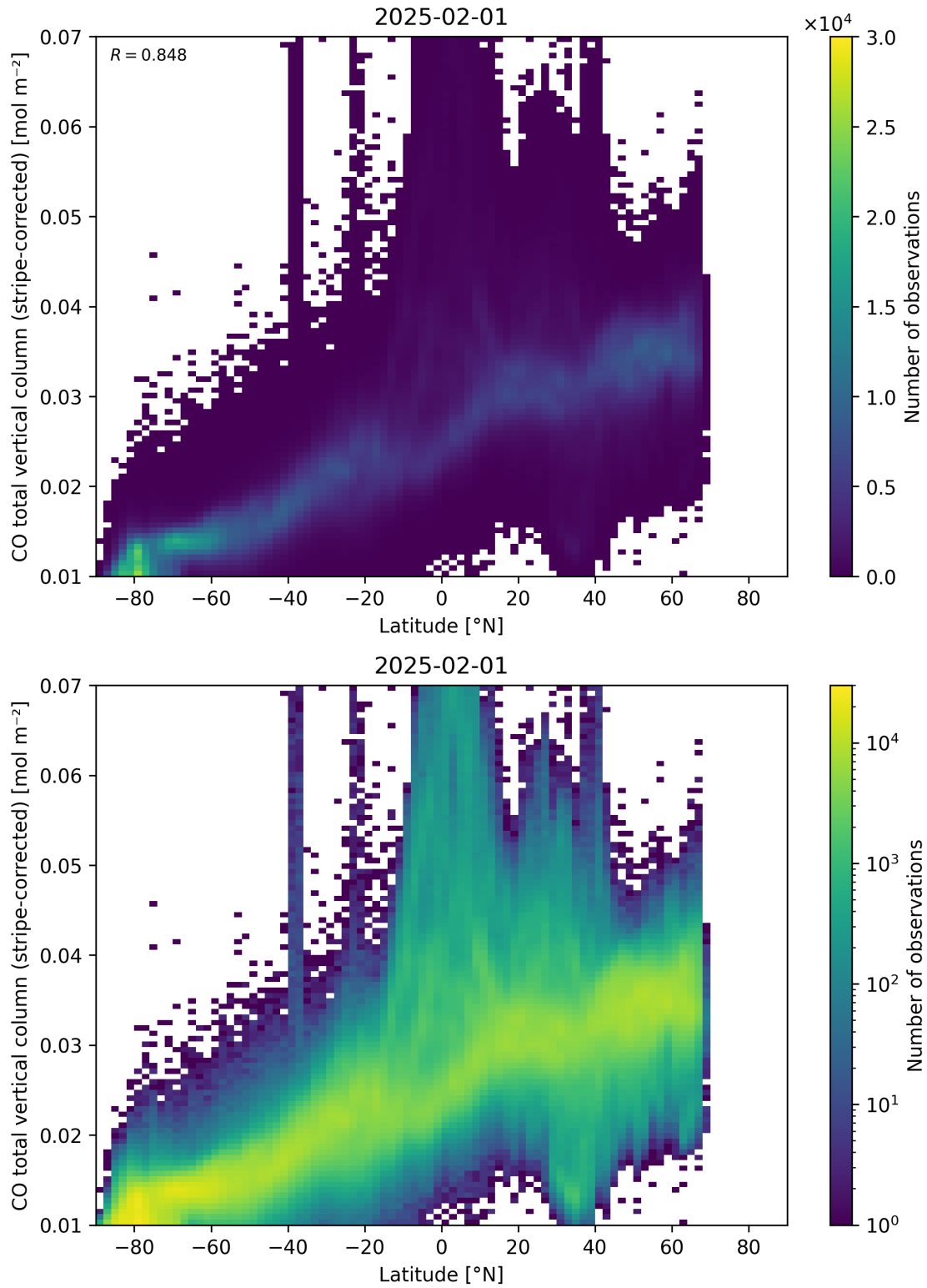
Figure 52: Scatter density plot of “Latitude” against “CO total vertical column (stripe-corrected)” for 2025-01-31 to 2025-02-02.
