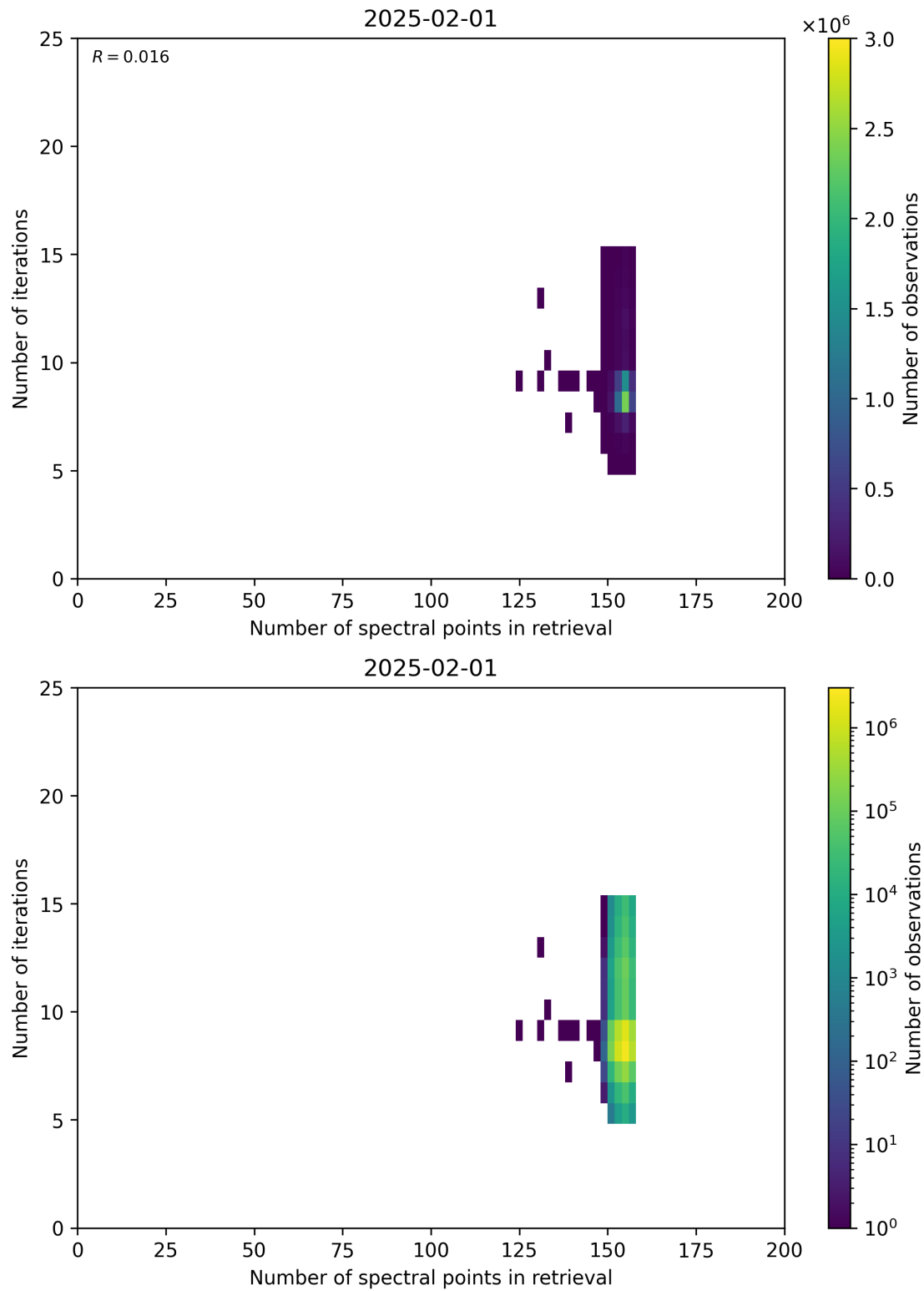
Figure 60: Scatter density plot of “Number of spectral points in retrieval” against “Number of iterations” for 2025-01-31 to 2025-02-02.
