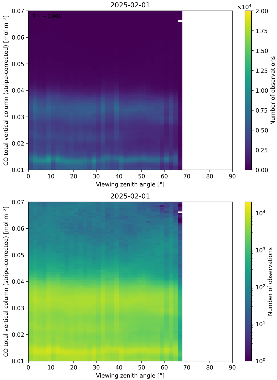
Figure 70: Scatter density plot of “Viewing zenith angle” against “CO total vertical column (stripe-corrected)” for 2025-01-31 to 2025-02-02.
