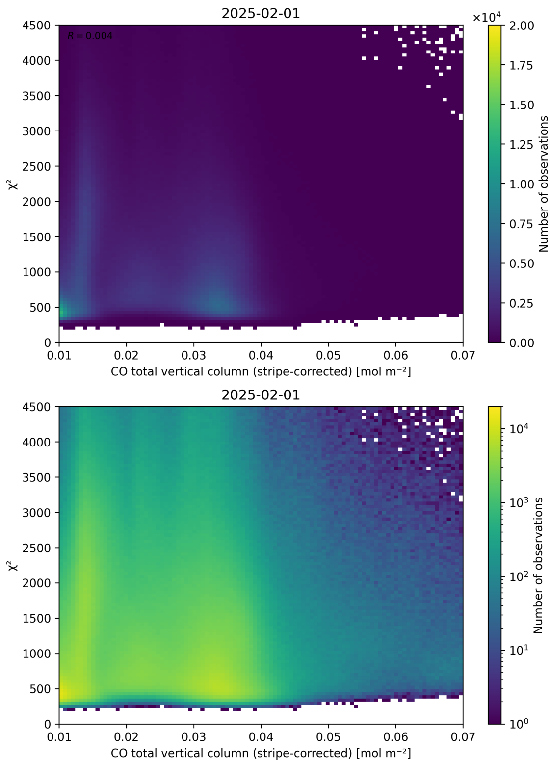
Figure 37: Scatter density plot of “CO total vertical column (stripe-corrected)” against “ \chi^2 ” for 2025-01-31 to 2025-02-02.
