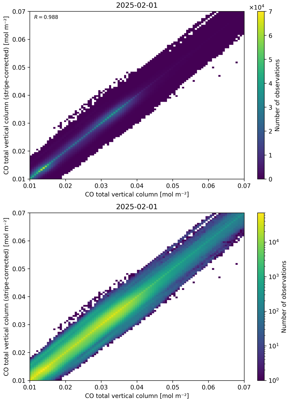
Figure 33: Scatter density plot of “CO total vertical column” against “CO total vertical column (stripe-corrected)” for 2025-01-31 to 2025-02-02.
