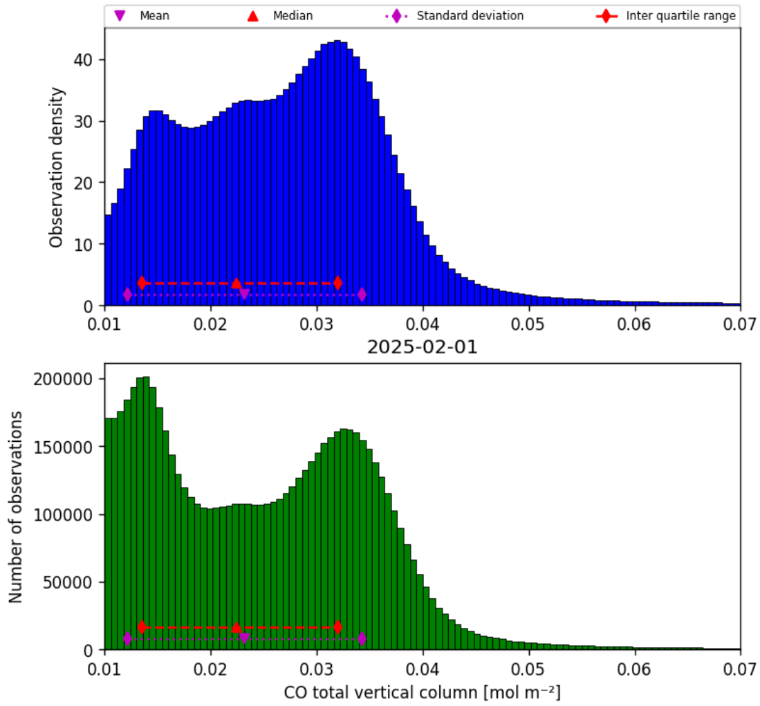
Figure 18: Histogram of “CO total vertical column” for 2025-01-31 to 2025-02-02
