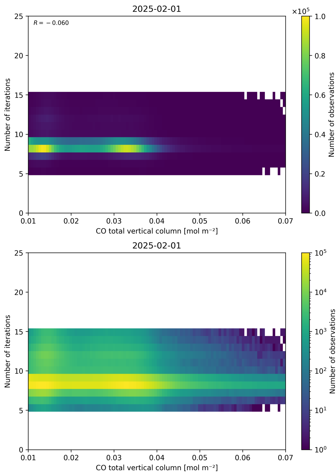
Figure 42: Scatter density plot of “CO total vertical column” against “Number of iterations” for 2025-01-31 to 2025-02-02.
