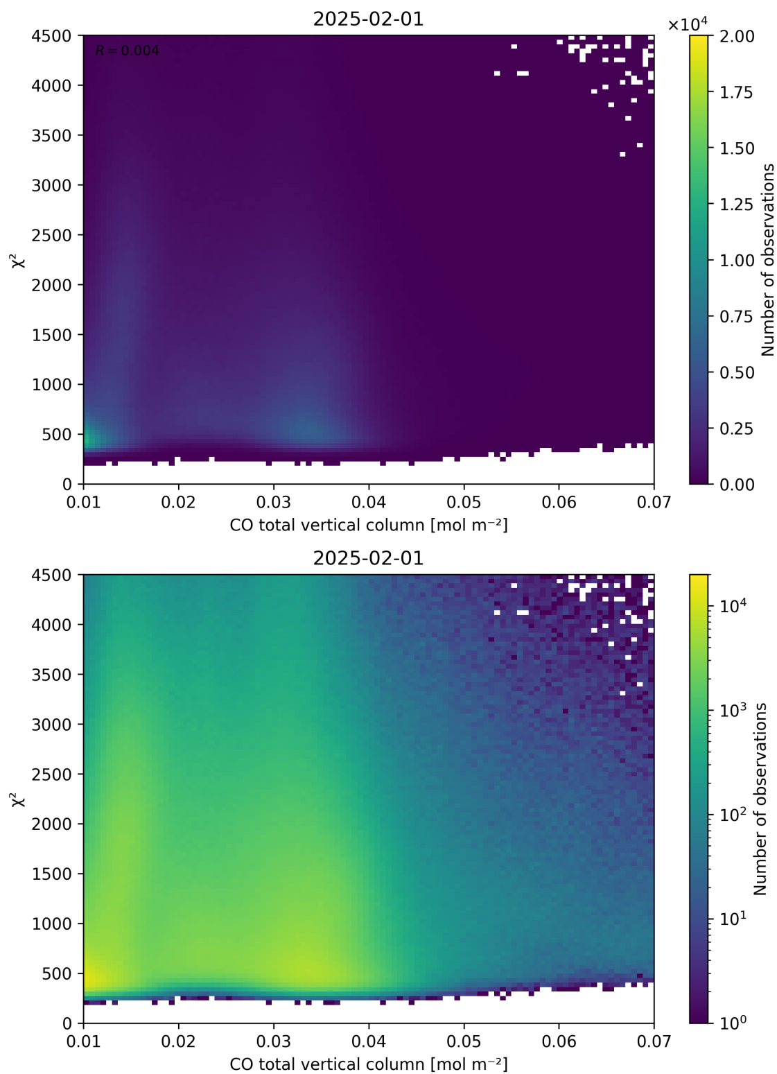
Figure 35: Scatter density plot of “CO total vertical column” against “ \chi^2 ” for 2025-01-31 to 2025-02-02.
