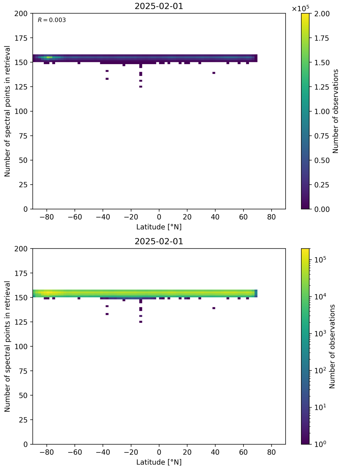
Figure 57: Scatter density plot of “Latitude” against “Number of spectral points in retrieval” for 2025-01-31 to 2025-02-02.
