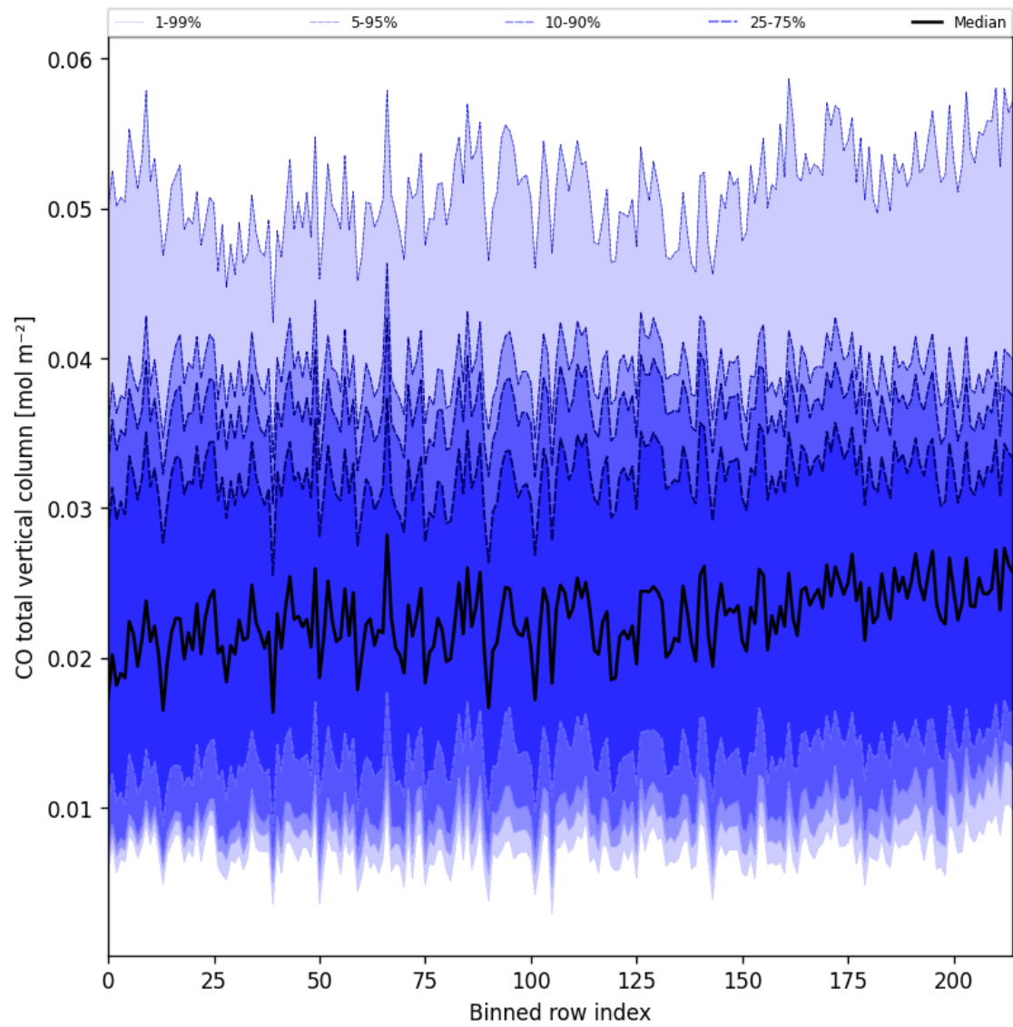
Figure 26: Along track statistics of “CO total vertical column” for 2025-01-31 to 2025-02-02
