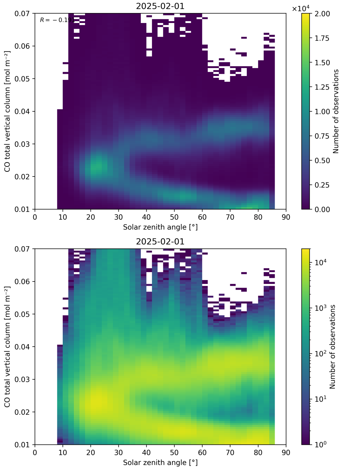
Figure 61: Scatter density plot of “Solar zenith angle” against “CO total vertical column” for 2025-01-31 to 2025-02-02.
