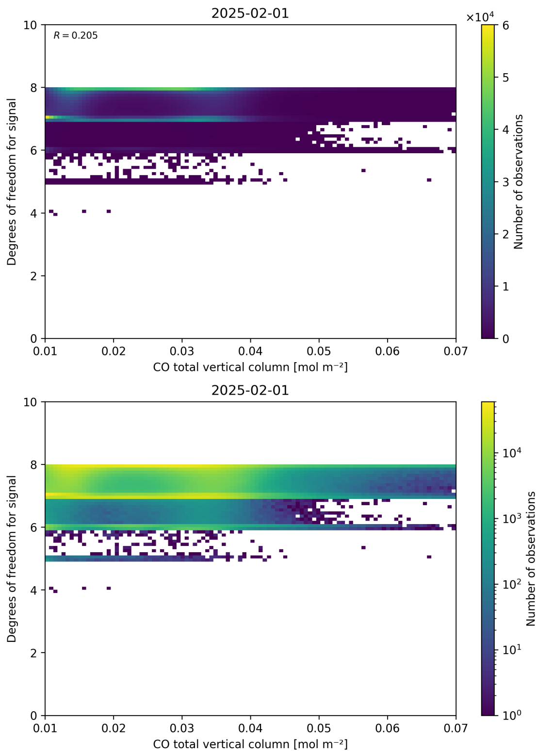
Figure 41: Scatter density plot of “CO total vertical column” against “Degrees of freedom for signal” for 2025-01-31 to 2025-02-02.
