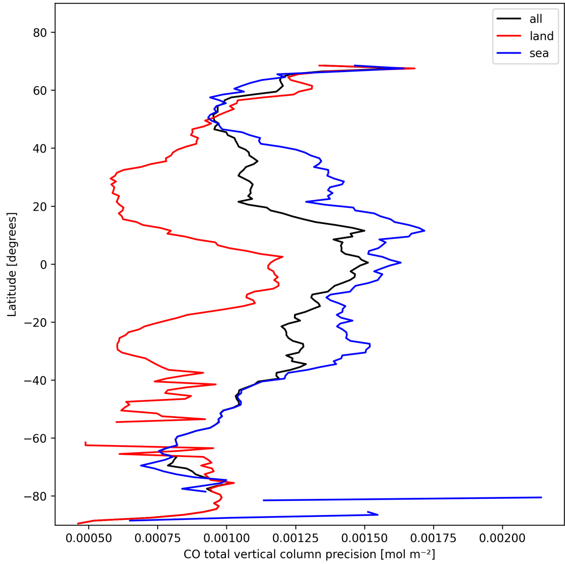
Figure 12: Zonal average of “CO total vertical column precision” for 2025-01-31 to 2025-02-02.
