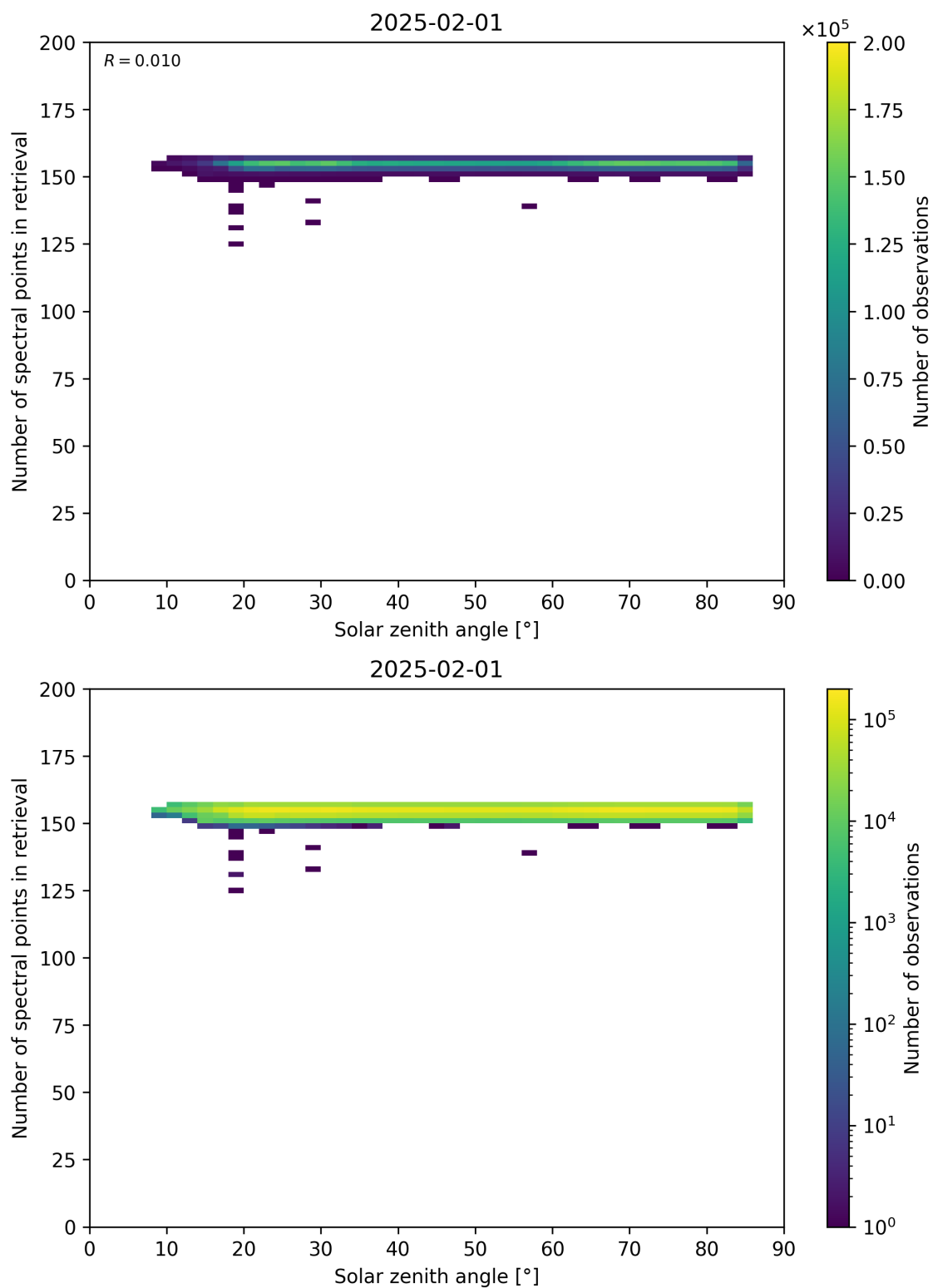
Figure 68: Scatter density plot of “Solar zenith angle” against “Number of spectral points in retrieval” for 2025-01-31 to 2025-02-02.
