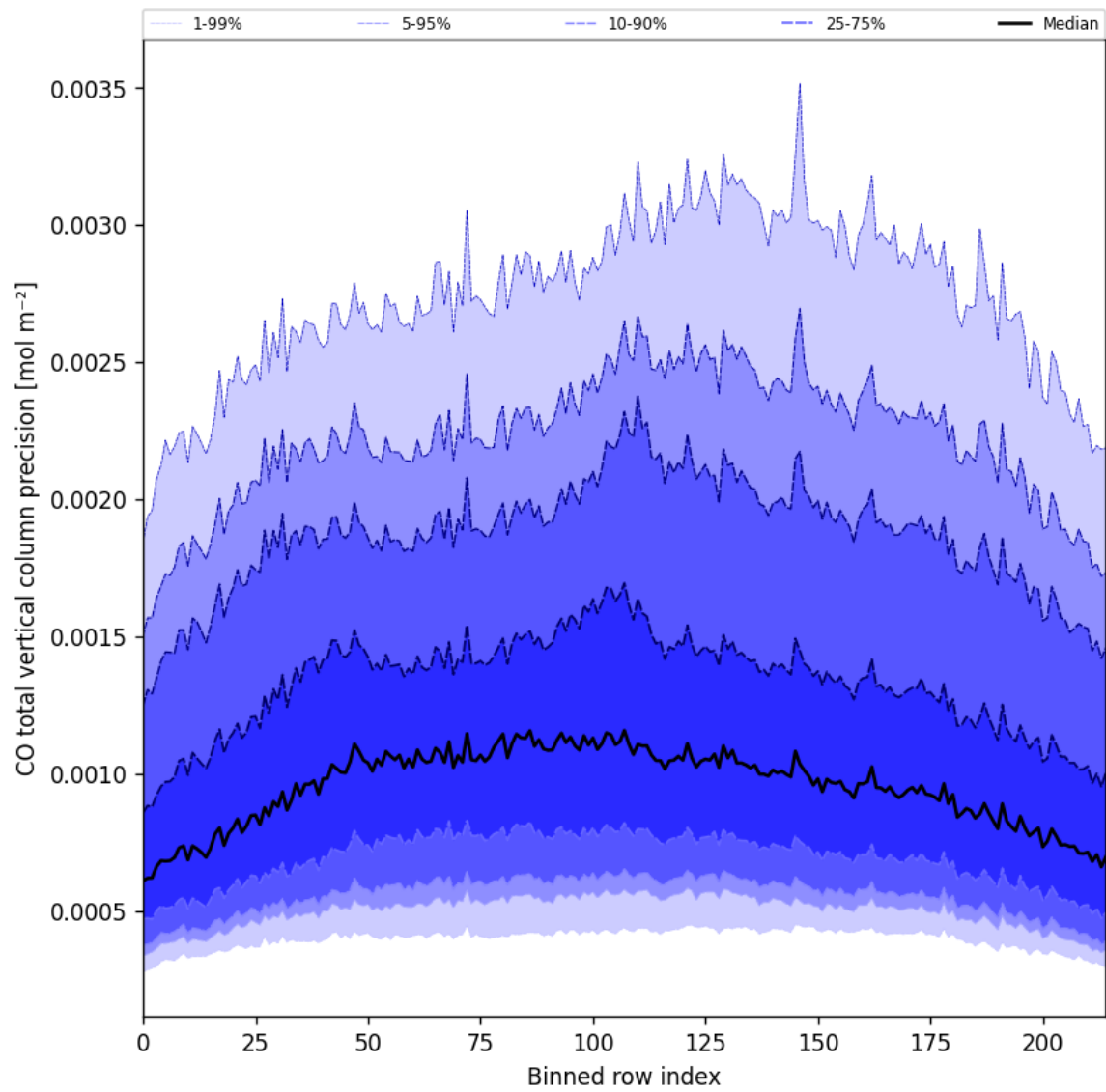
Figure 28: Along track statistics of “CO total vertical column precision” for 2025-01-31 to 2025-02-02
