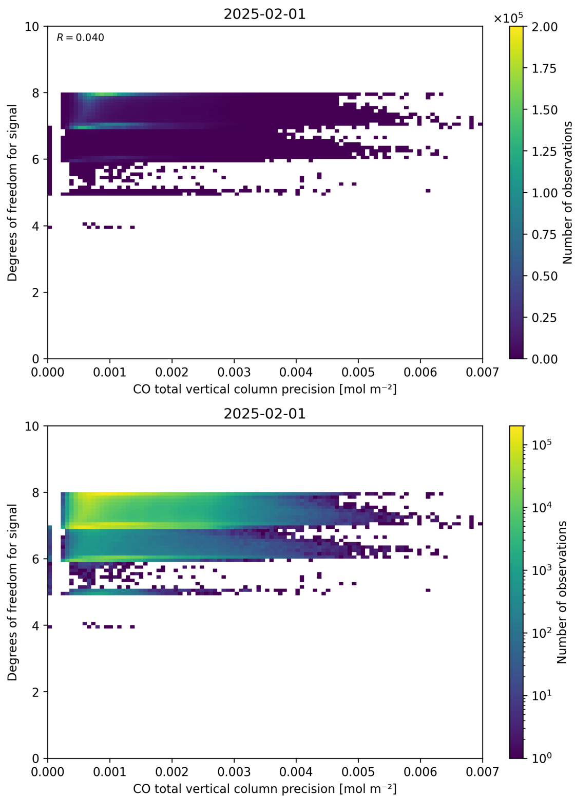
Figure 45: Scatter density plot of “CO total vertical column precision” against “Degrees of freedom for signal” for 2025-01-31 to 2025-02-02.
