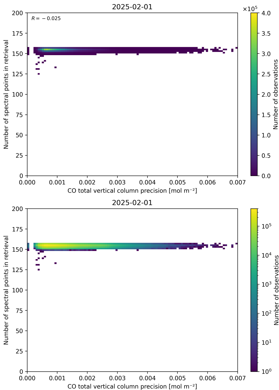
Figure 47: Scatter density plot of “CO total vertical column precision” against “Number of spectral points in retrieval” for 2025-01-31 to 2025-02-02.
