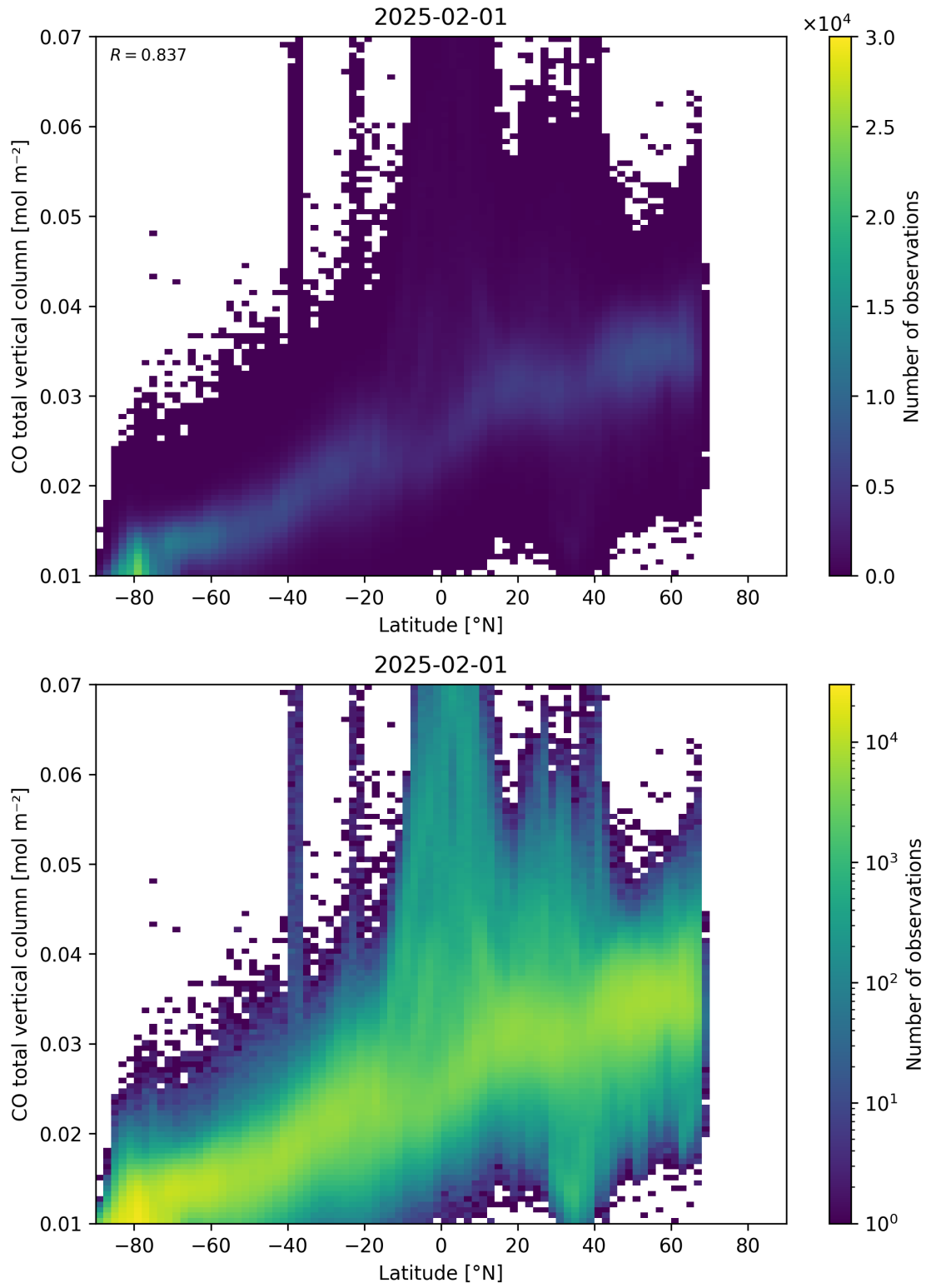
Figure 51: Scatter density plot of “Latitude” against “CO total vertical column” for 2025-01-31 to 2025-02-02.
