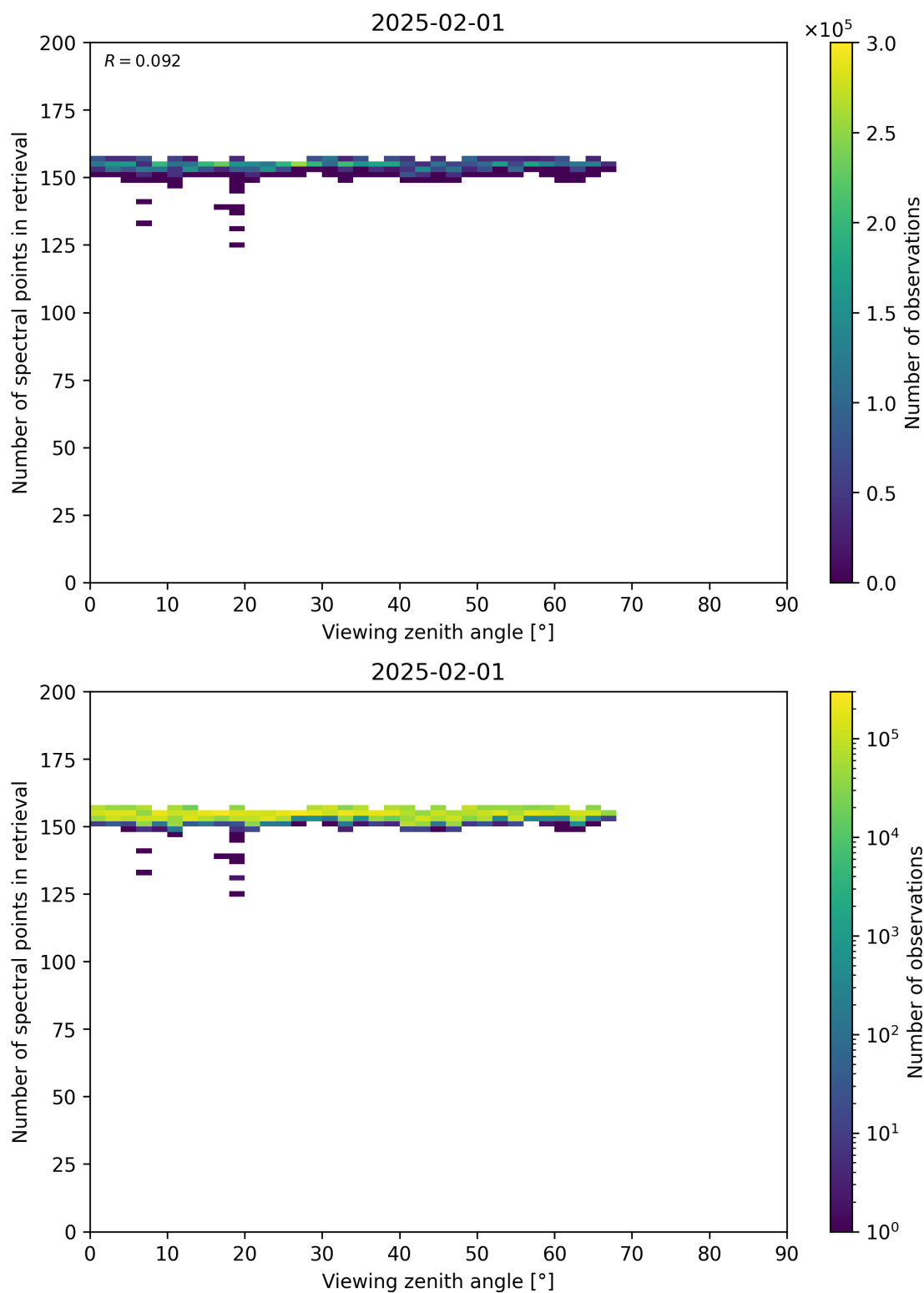
Figure 76: Scatter density plot of “Viewing zenith angle” against “Number of spectral points in retrieval” for 2025-01-31 to 2025-02-02.
