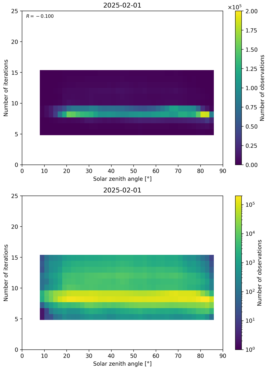
Figure 67: Scatter density plot of “Solar zenith angle” against “Number of iterations” for 2025-01-31 to 2025-02-02.
