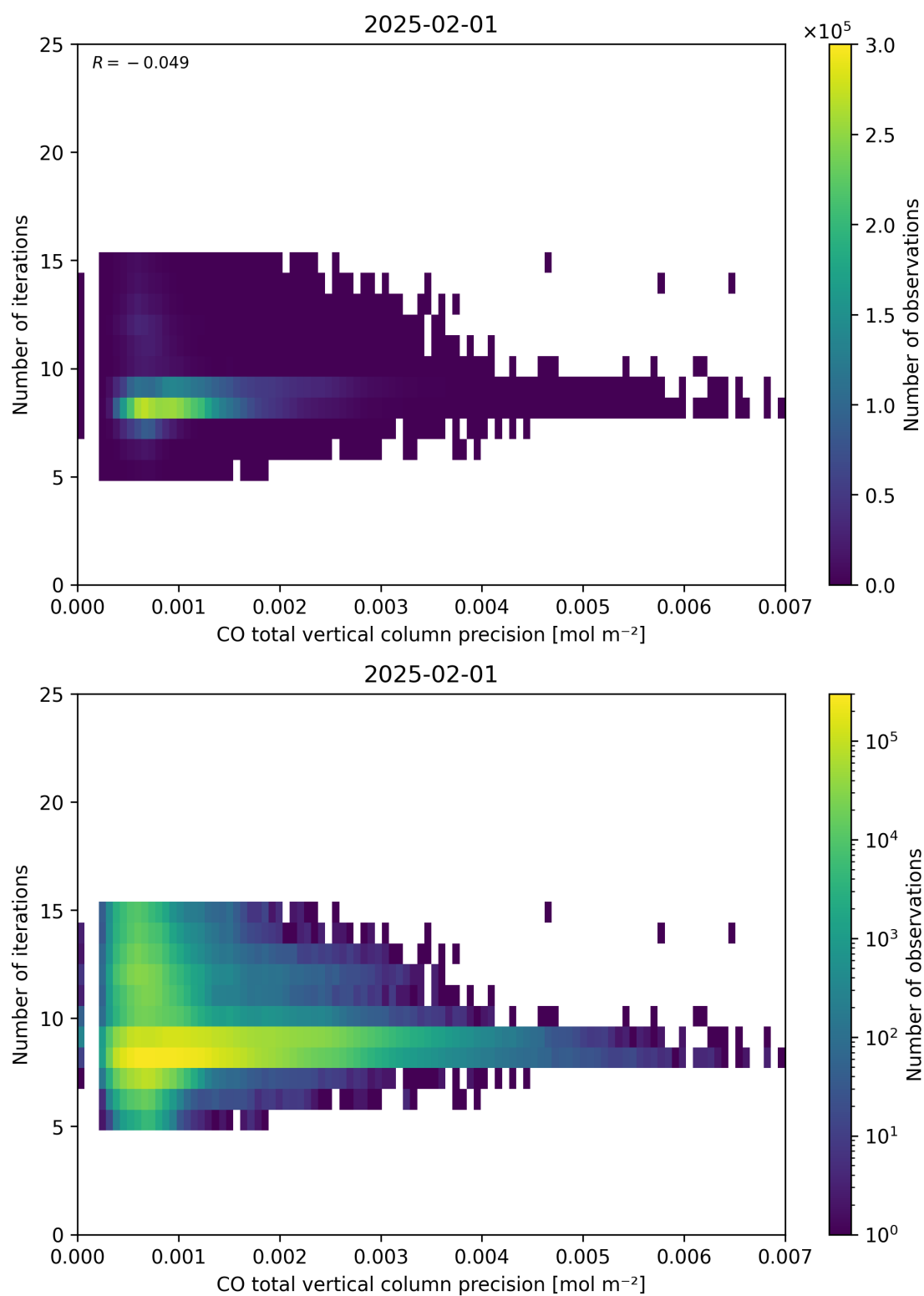
Figure 46: Scatter density plot of “CO total vertical column precision” against “Number of iterations” for 2025-01-31 to 2025-02-02.
