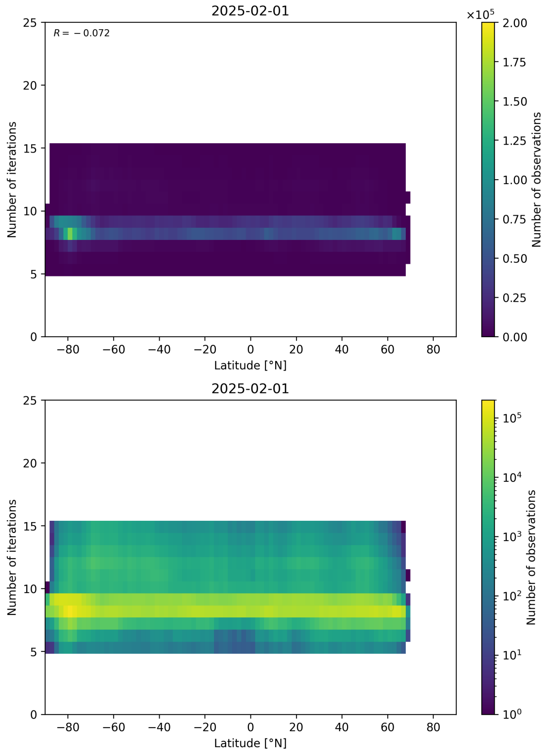
Figure 56: Scatter density plot of “Latitude” against “Number of iterations” for 2025-01-31 to 2025-02-02.
