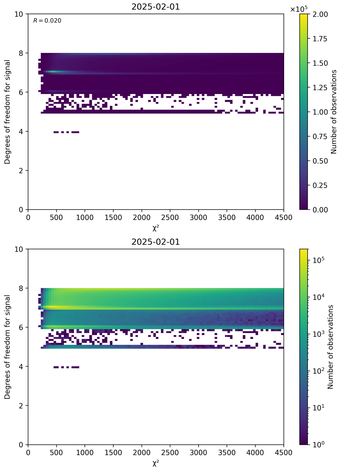
Figure 48: Scatter density plot of “ \chi^2 ” against “Degrees of freedom for signal” for 2025-01-31 to 2025-02-02.
