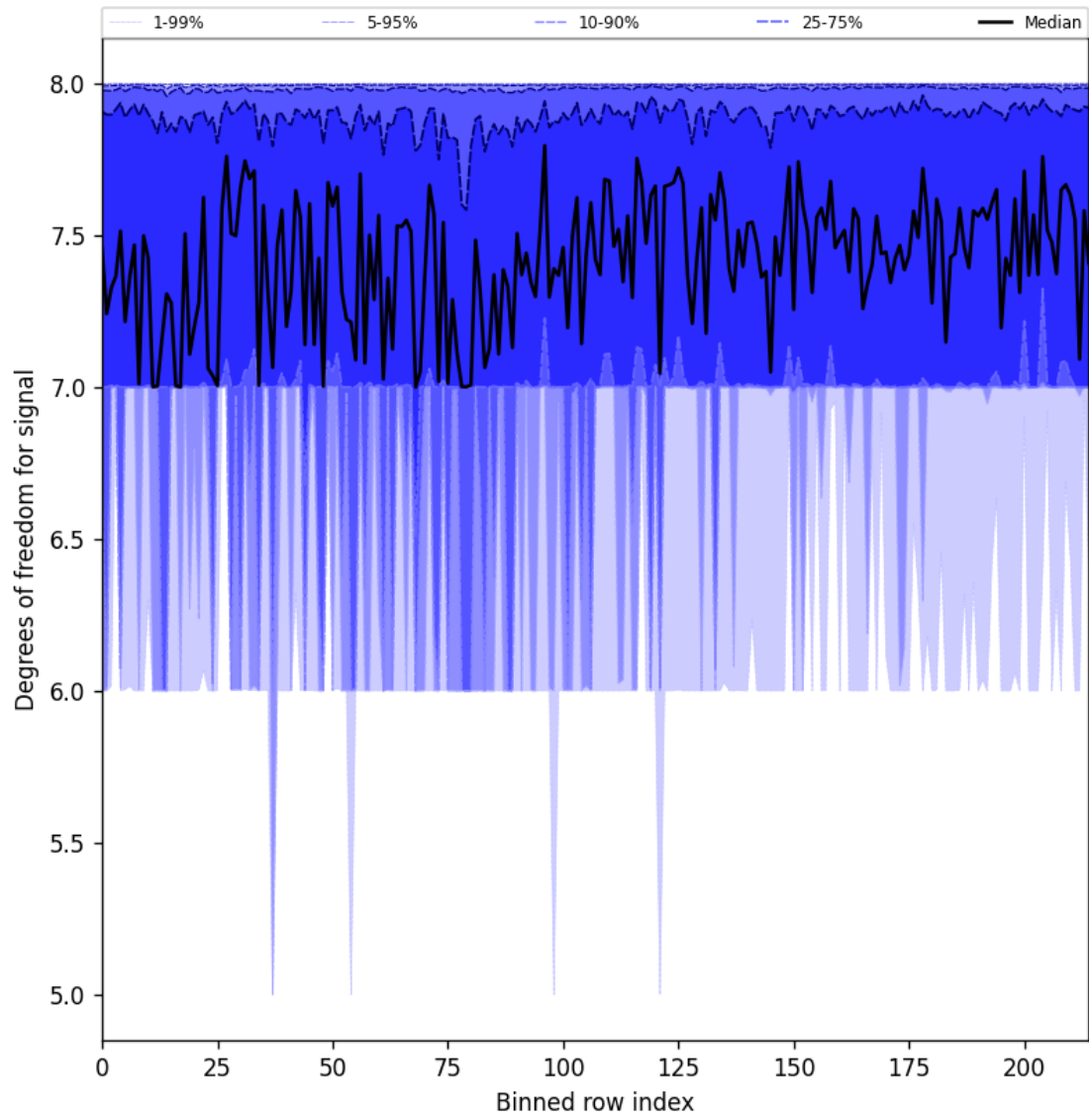
Figure 31: Along track statistics of “Degrees of freedom for signal” for 2025-01-31 to 2025-02-02
