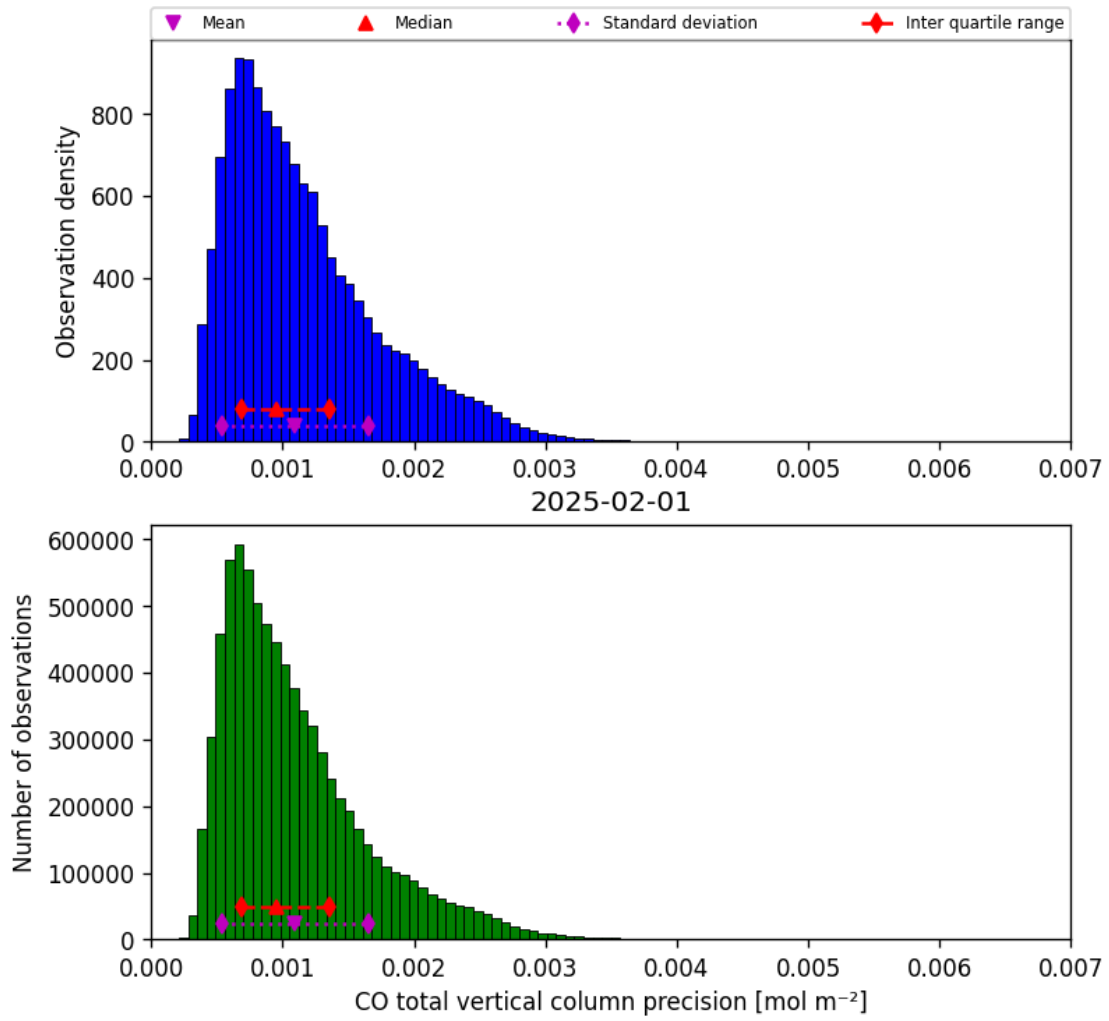
Figure 20: Histogram of “CO total vertical column precision” for 2025-01-31 to 2025-02-02
