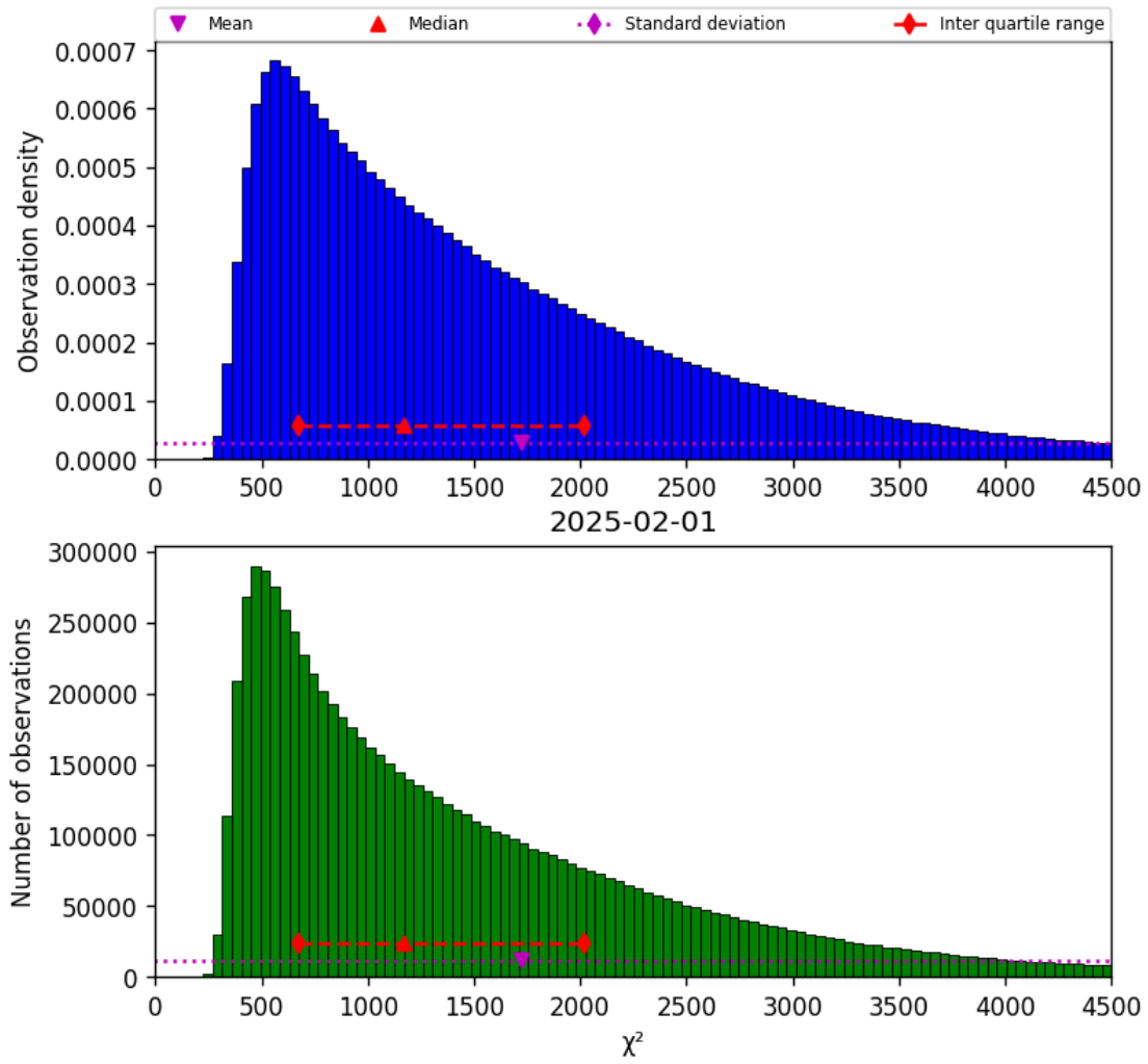
Figure 22: Histogram of " \chi^2 " for 2025-01-31 to 2025-02-02
