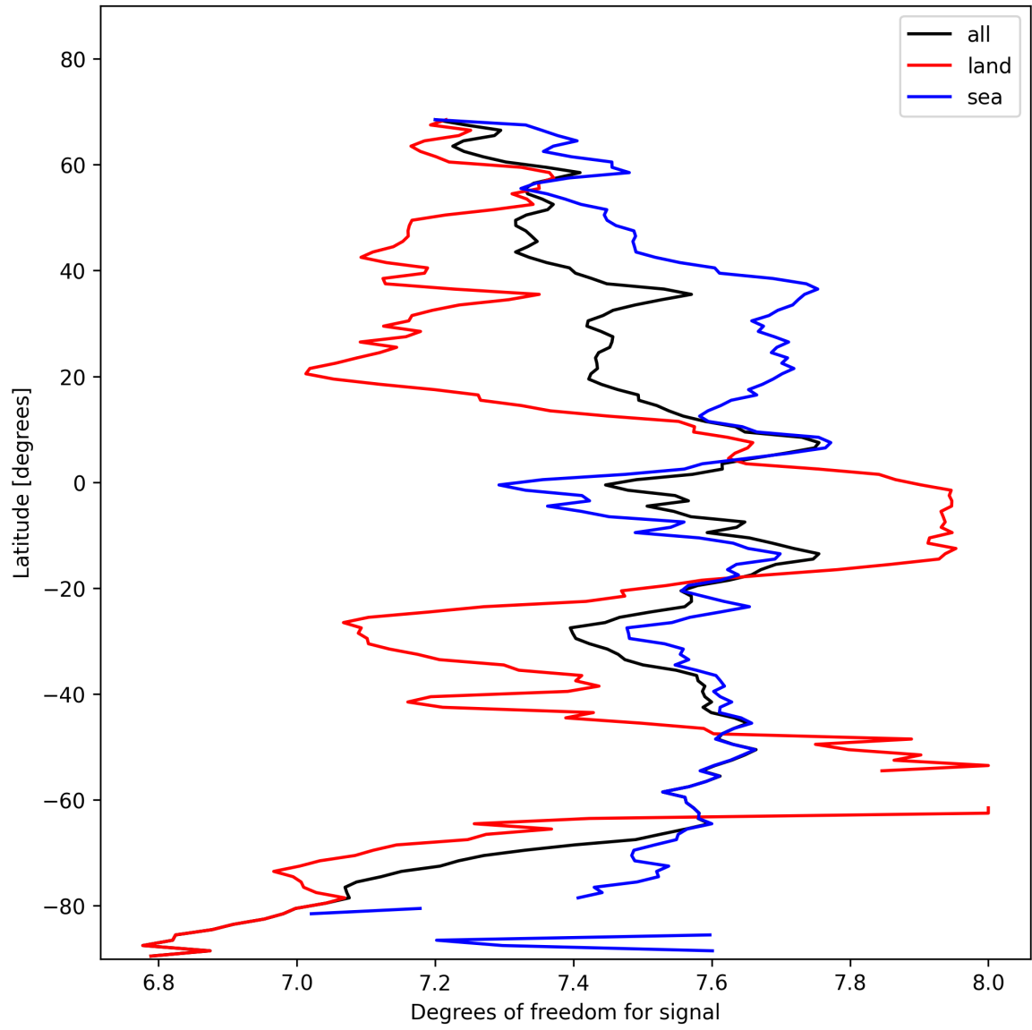
Figure 15: Zonal average of “Degrees of freedom for signal” for 2025-01-31 to 2025-02-02.
