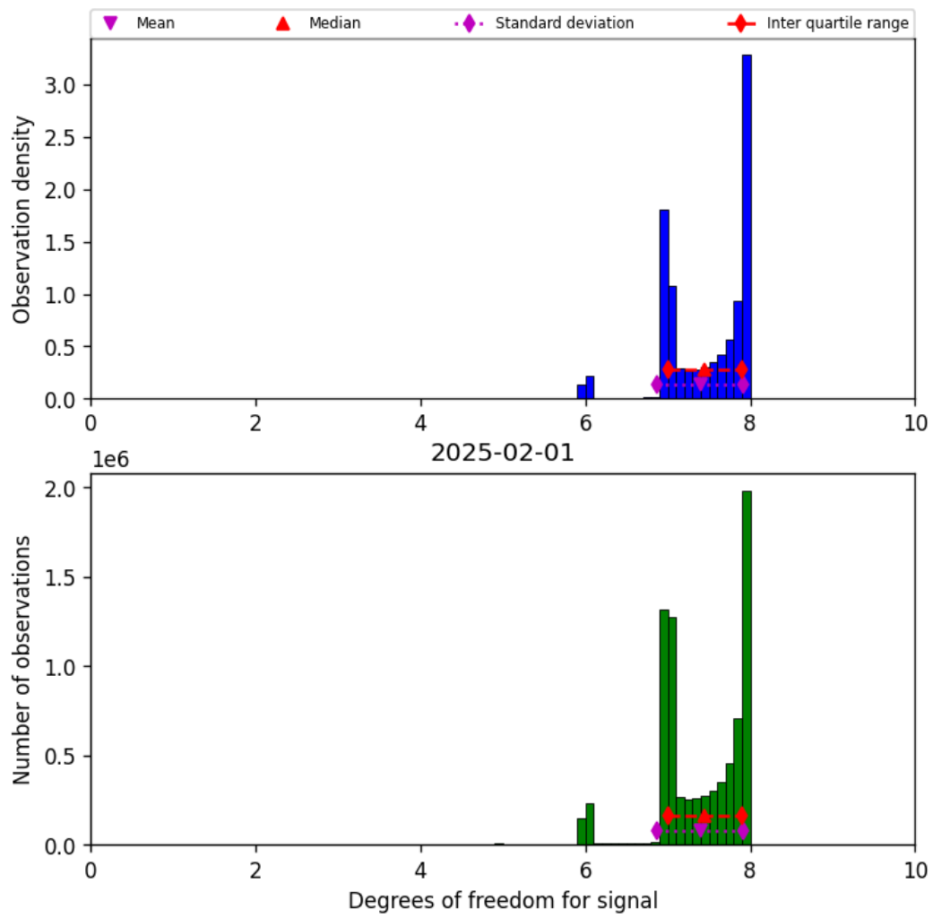
Figure 23: Histogram of “Degrees of freedom for signal” for 2025-01-31 to 2025-02-02
