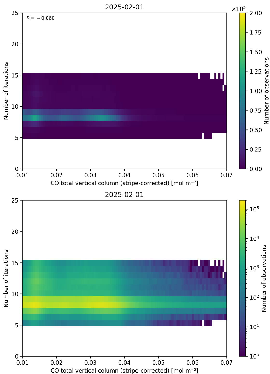
Figure 39: Scatter density plot of “CO total vertical column (stripe-corrected)” against “Number of iterations” for 2025-01-31 to 2025-02-02.
