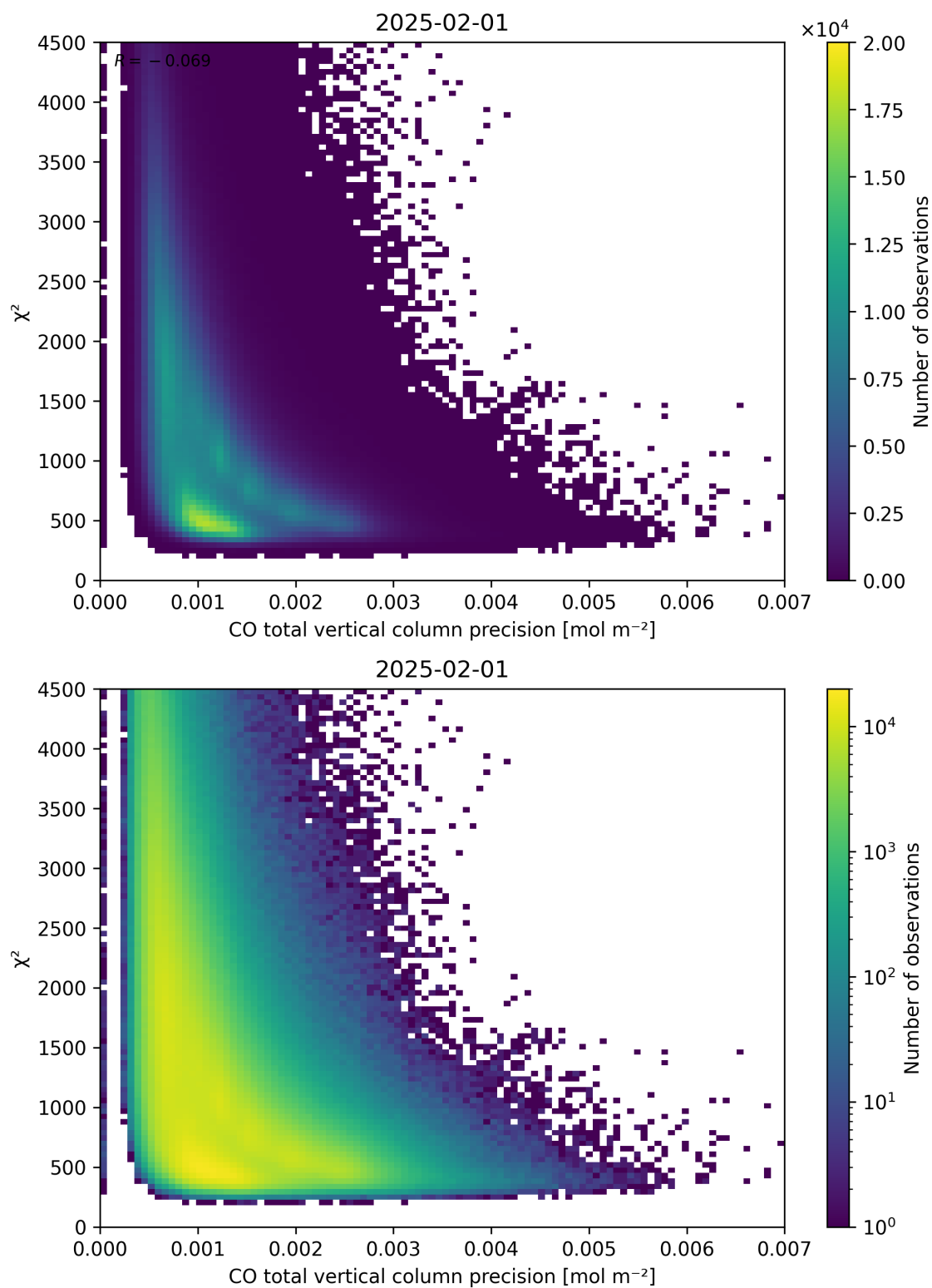
Figure 44: Scatter density plot of “CO total vertical column precision” against “ \chi^2 ” for 2025-01-31 to 2025-02-02.
