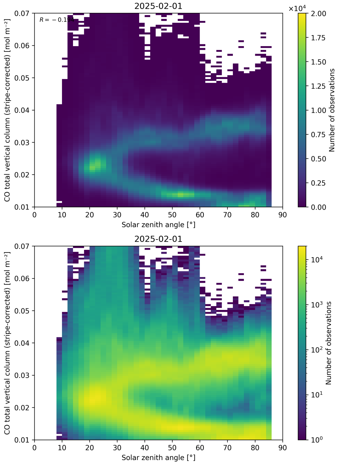
Figure 62: Scatter density plot of “Solar zenith angle” against “CO total vertical column (stripe-corrected)” for 2025-01-31 to 2025-02-02.
