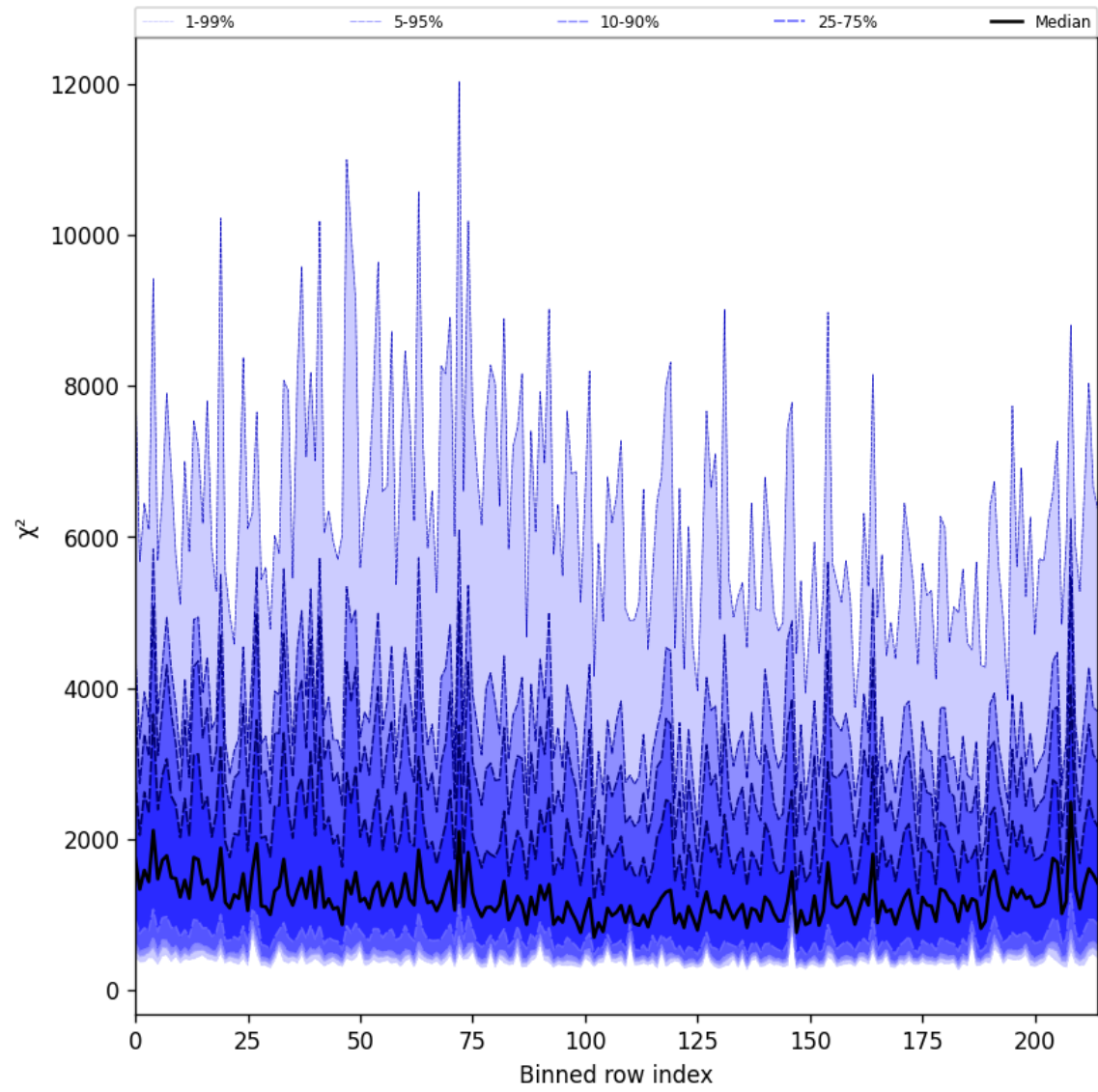
Figure 30: Along track statistics of “ \chi^2 ” for 2025-01-31 to 2025-02-02
