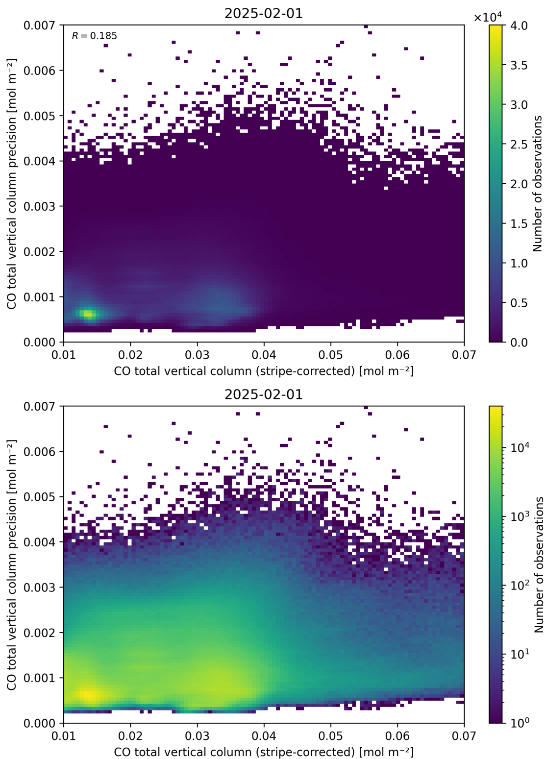
Figure 36: Scatter density plot of “CO total vertical column (stripe-corrected)” against “CO total vertical column precision” for 2025-01-31 to 2025-02-02.
