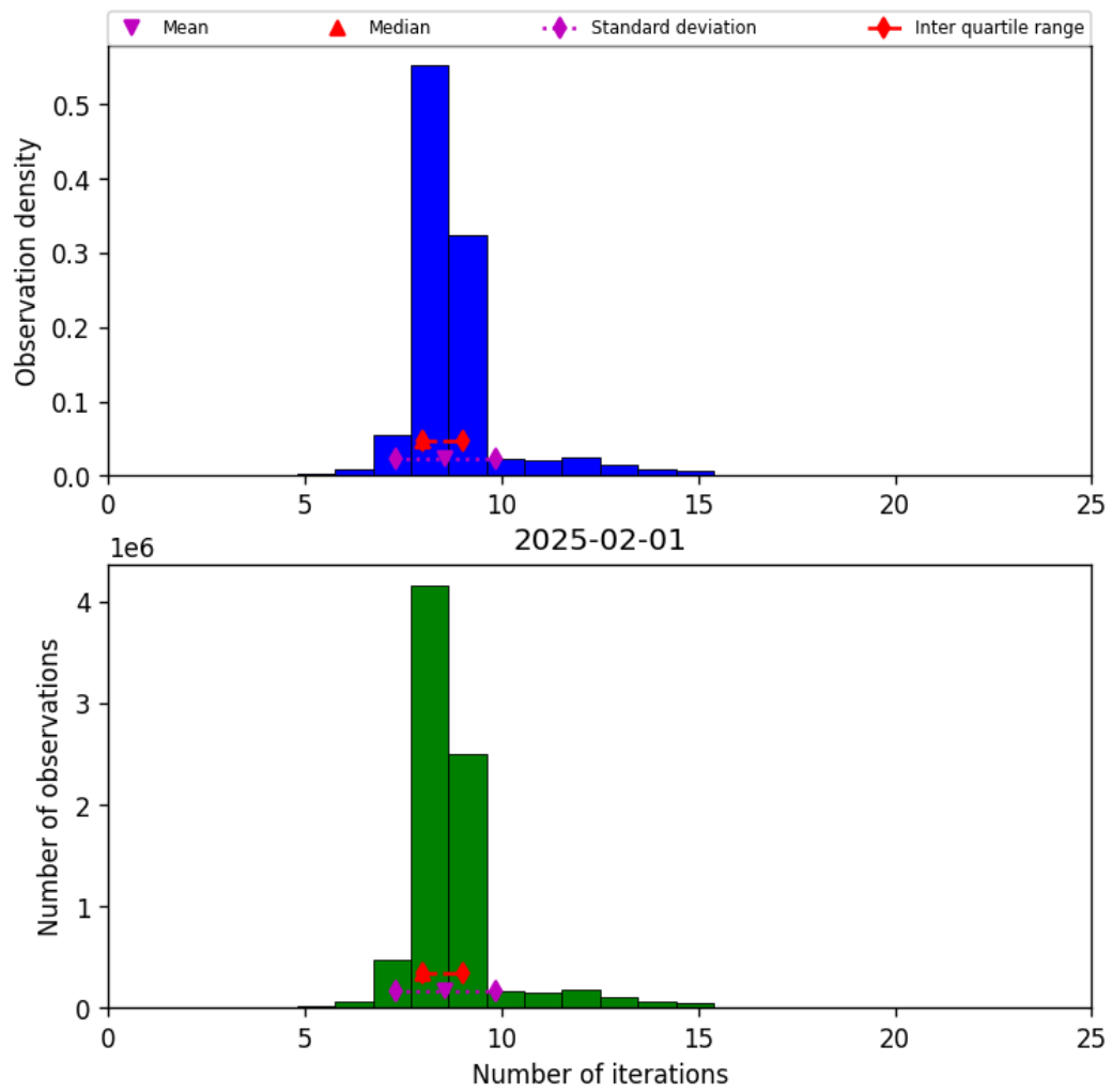
Figure 24: Histogram of “Number of iterations” for 2025-01-31 to 2025-02-02
