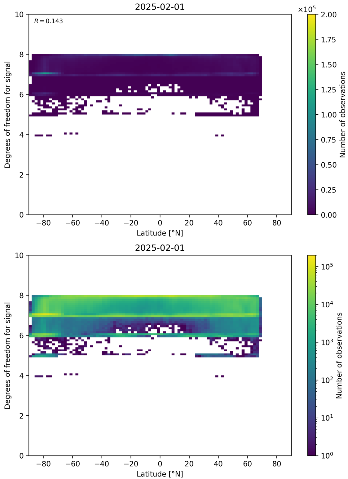
Figure 55: Scatter density plot of “Latitude” against “Degrees of freedom for signal” for 2025-01-31 to 2025-02-02.
