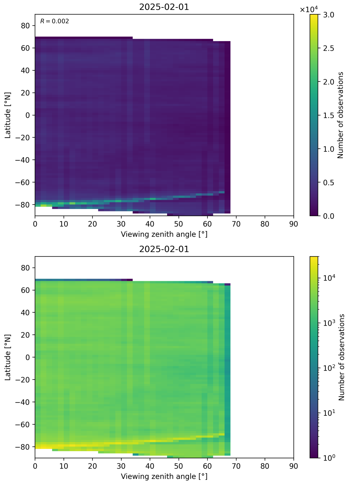
Figure 74: Scatter density plot of “Viewing zenith angle” against “Latitude” for 2025-01-31 to 2025-02-02.
