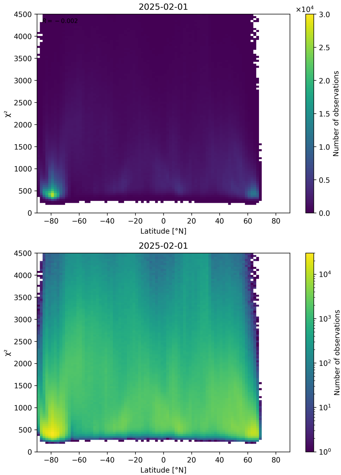
Figure 54: Scatter density plot of “Latitude” against “ \chi^2 ” for 2025-01-31 to 2025-02-02.
