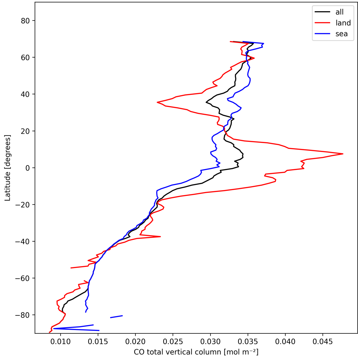
Figure 10: Zonal average of “CO total vertical column” for 2025-01-31 to 2025-02-02.
