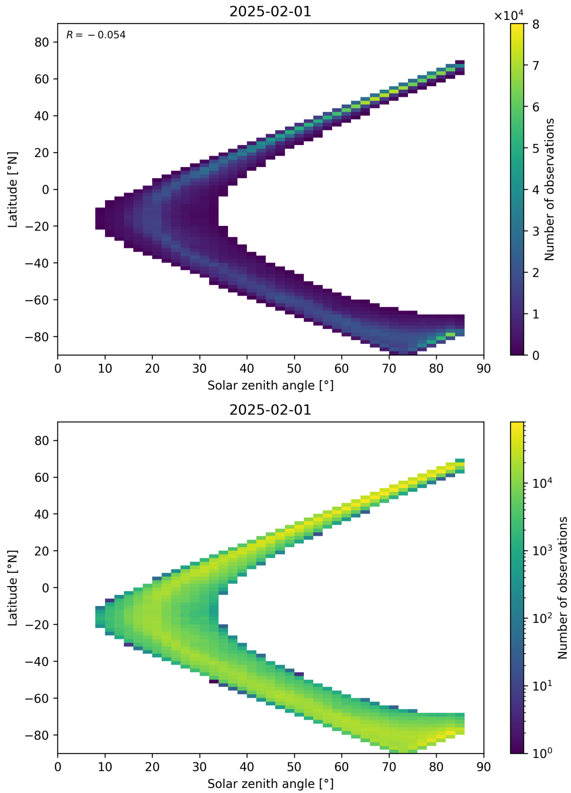
Figure 66: Scatter density plot of “Solar zenith angle” against “Latitude” for 2025-01-31 to 2025-02-02.
