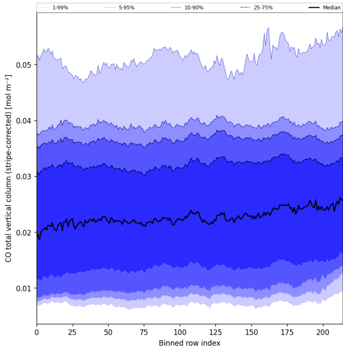
Figure 27: Along track statistics of “CO total vertical column (stripe-corrected)” for 2025-01-31 to 2025-02-02
