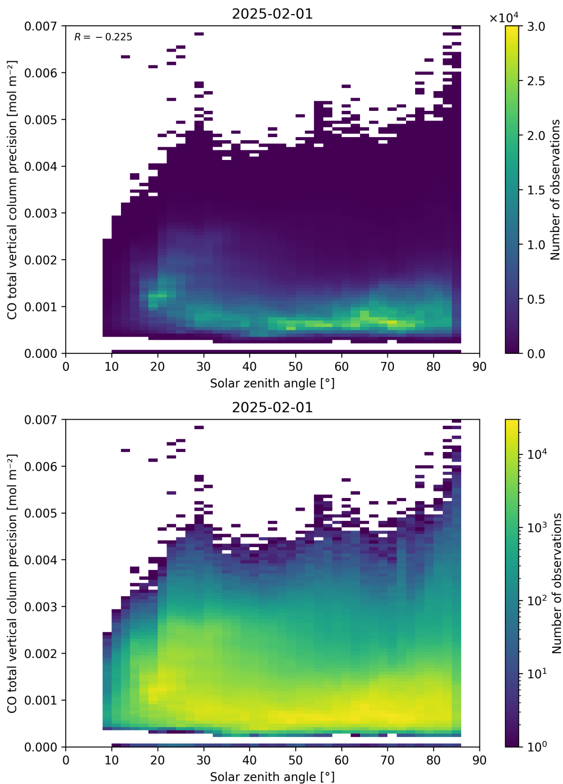
Figure 63: Scatter density plot of “Solar zenith angle” against “CO total vertical column precision” for 2025-01-31 to 2025-02-02.
