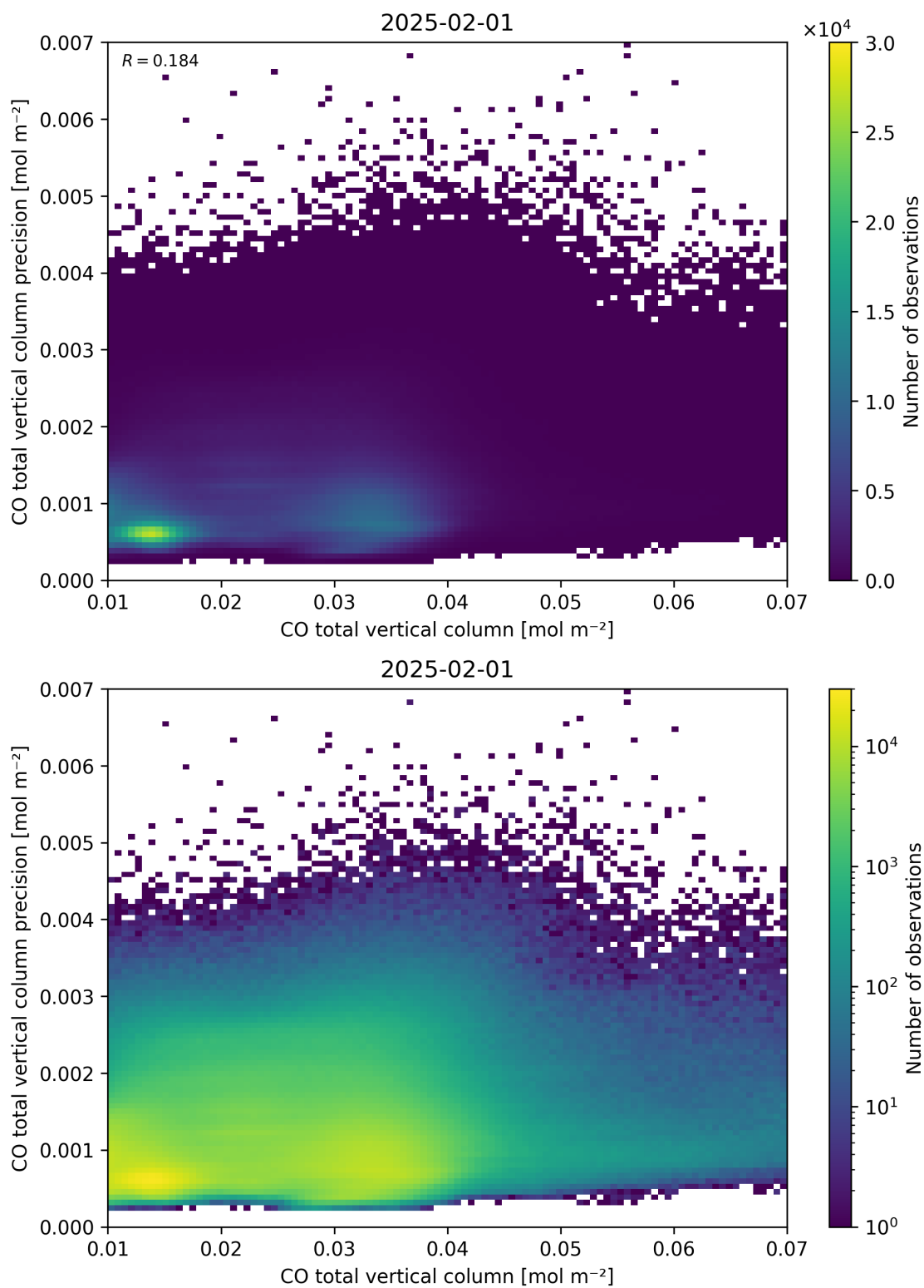
Figure 34: Scatter density plot of “CO total vertical column” against “CO total vertical column precision” for 2025-01-31 to 2025-02-02.
