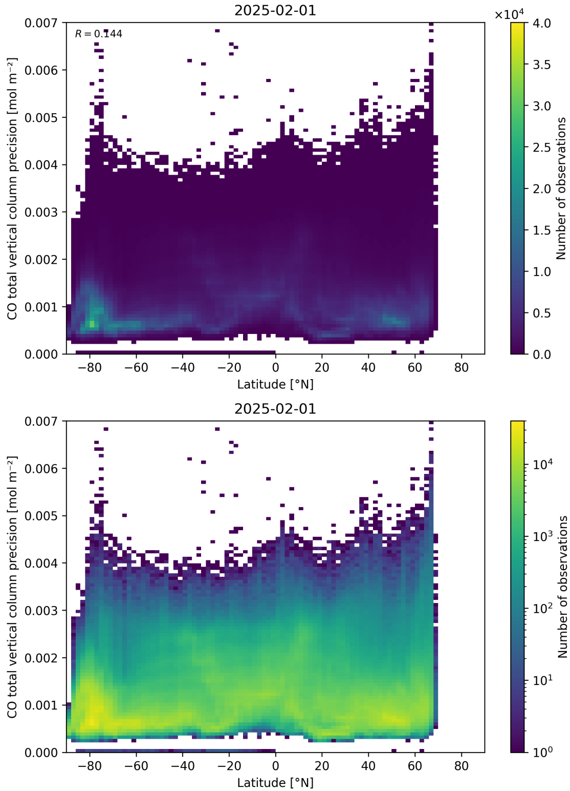
Figure 53: Scatter density plot of “Latitude” against “CO total vertical column precision” for 2025-01-31 to 2025-02-02.
