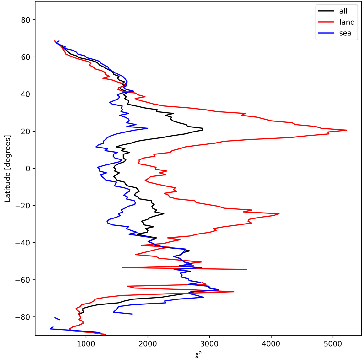
Figure 14: Zonal average of “ \chi^2 ” for 2025-01-31 to 2025-02-02.
