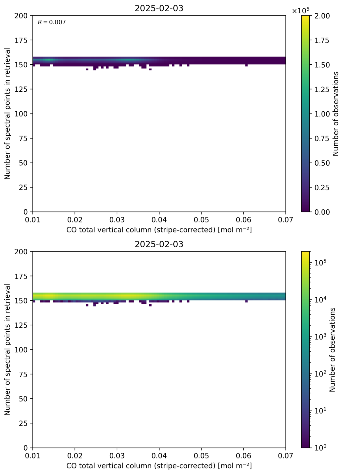
Figure 40: Scatter density plot of “CO total vertical column (stripe-corrected)” against “Number of spectral points in retrieval” for 2025-02-03 to 2025-02-04.
