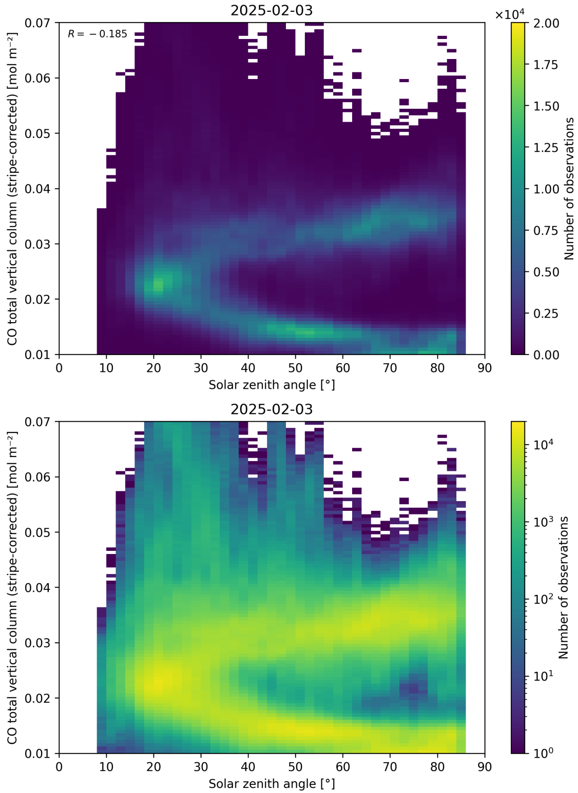
Figure 62: Scatter density plot of “Solar zenith angle” against “CO total vertical column (stripe-corrected)” for 2025-02-03 to 2025-02-04.
