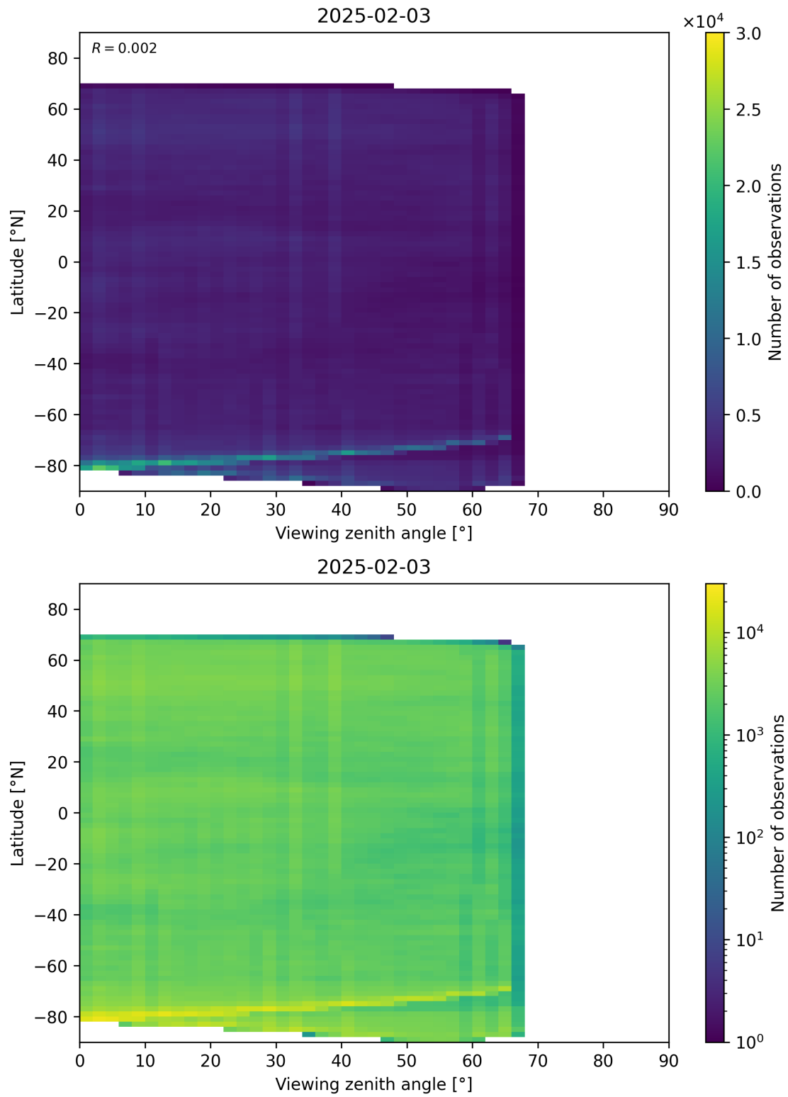
Figure 74: Scatter density plot of “Viewing zenith angle” against “Latitude” for 2025-02-03 to 2025-02-04.
