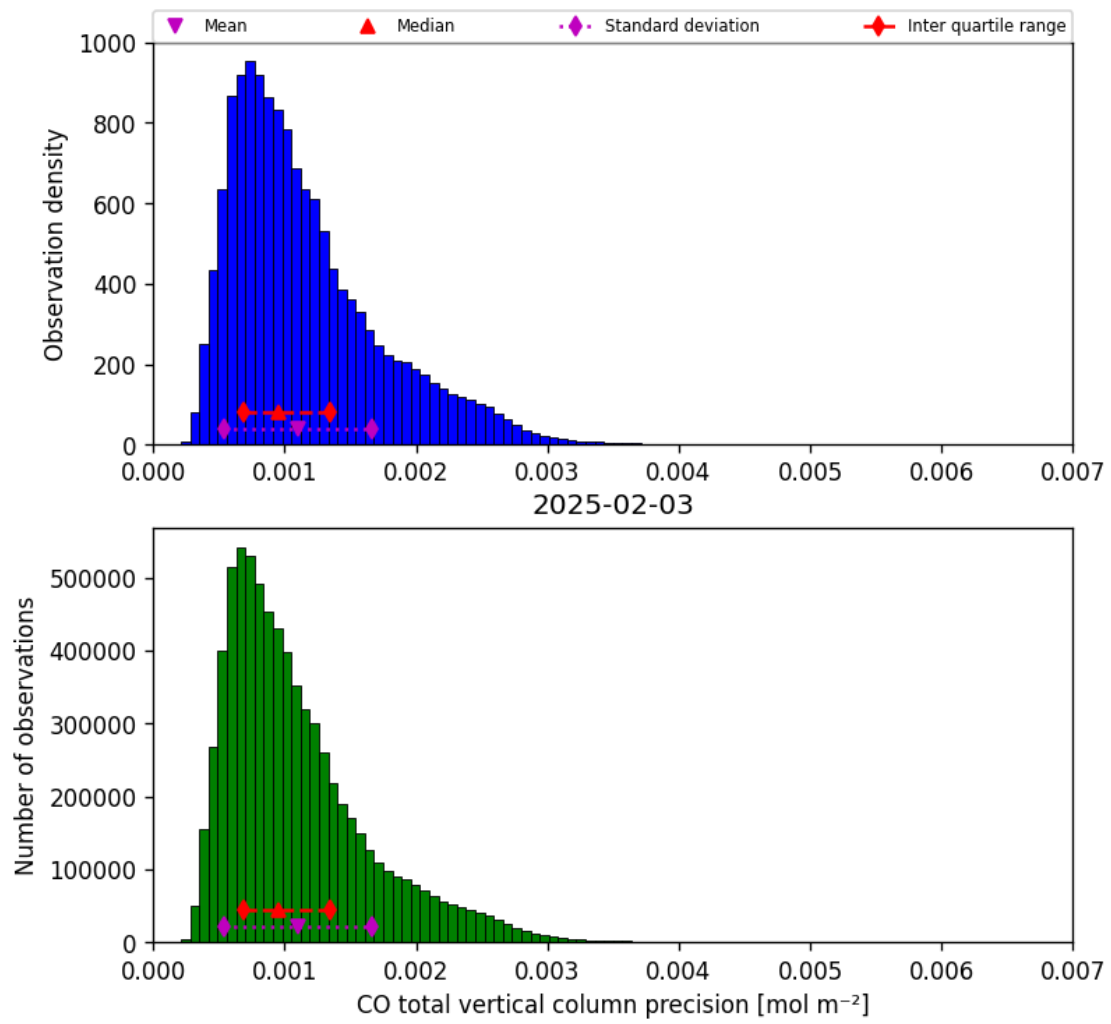
Figure 20: Histogram of “CO total vertical column precision” for 2025-02-03 to 2025-02-04
