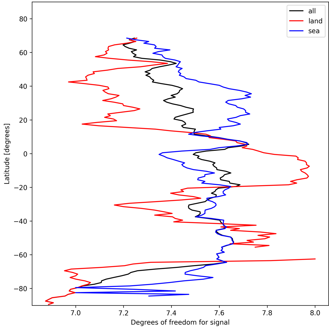
Figure 15: Zonal average of “Degrees of freedom for signal” for 2025-02-03 to 2025-02-04.
