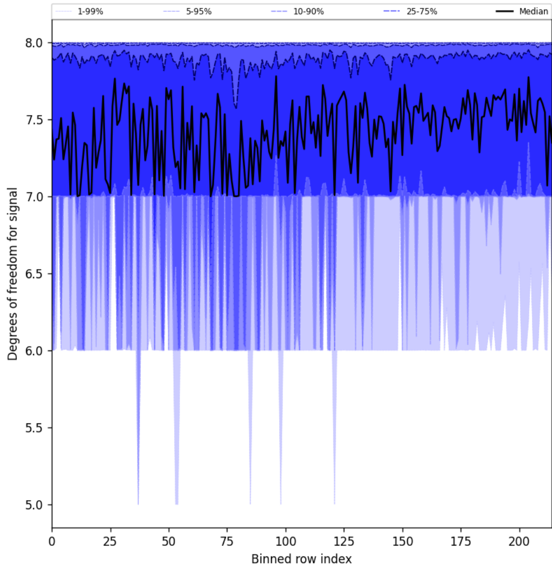
Figure 31: Along track statistics of “Degrees of freedom for signal” for 2025-02-03 to 2025-02-04
