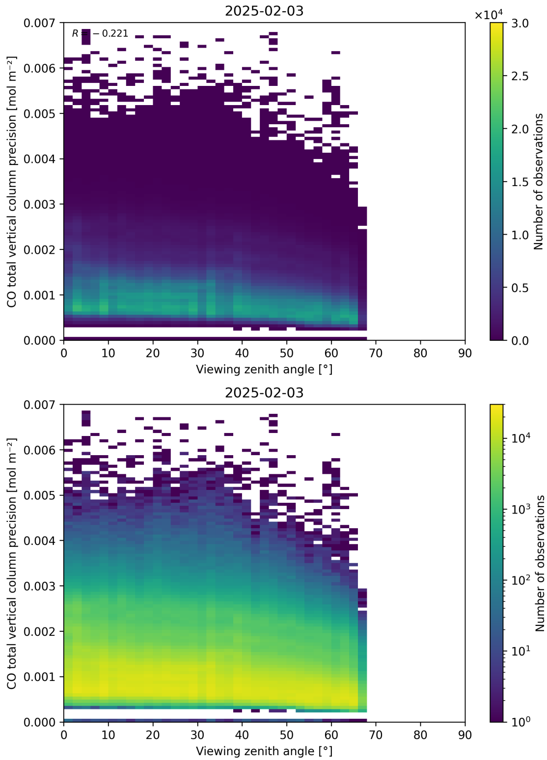
Figure 71: Scatter density plot of “Viewing zenith angle” against “CO total vertical column precision” for 2025-02-03 to 2025-02-04.
