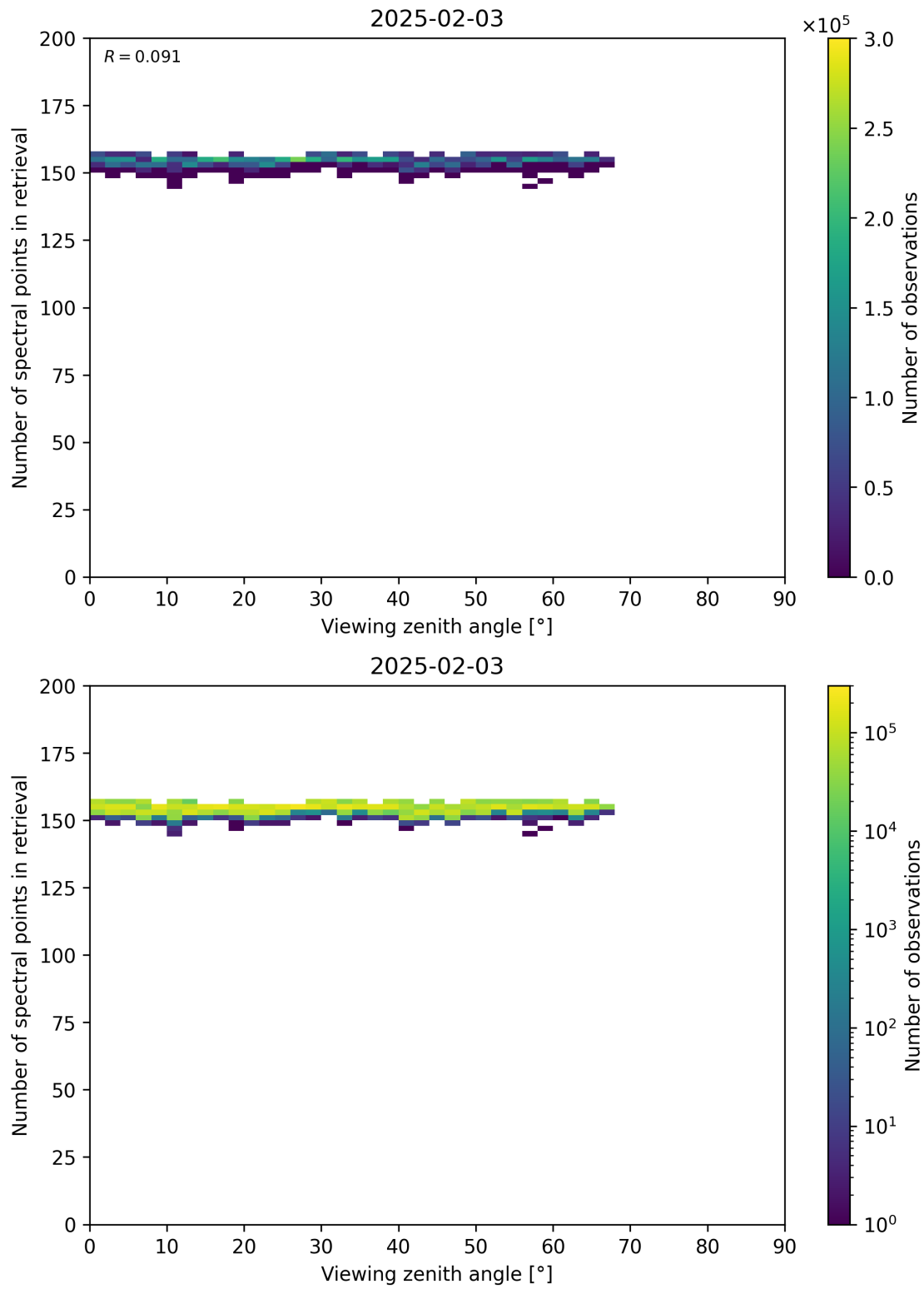
Figure 76: Scatter density plot of “Viewing zenith angle” against “Number of spectral points in retrieval” for 2025-02-03 to 2025-02-04.
