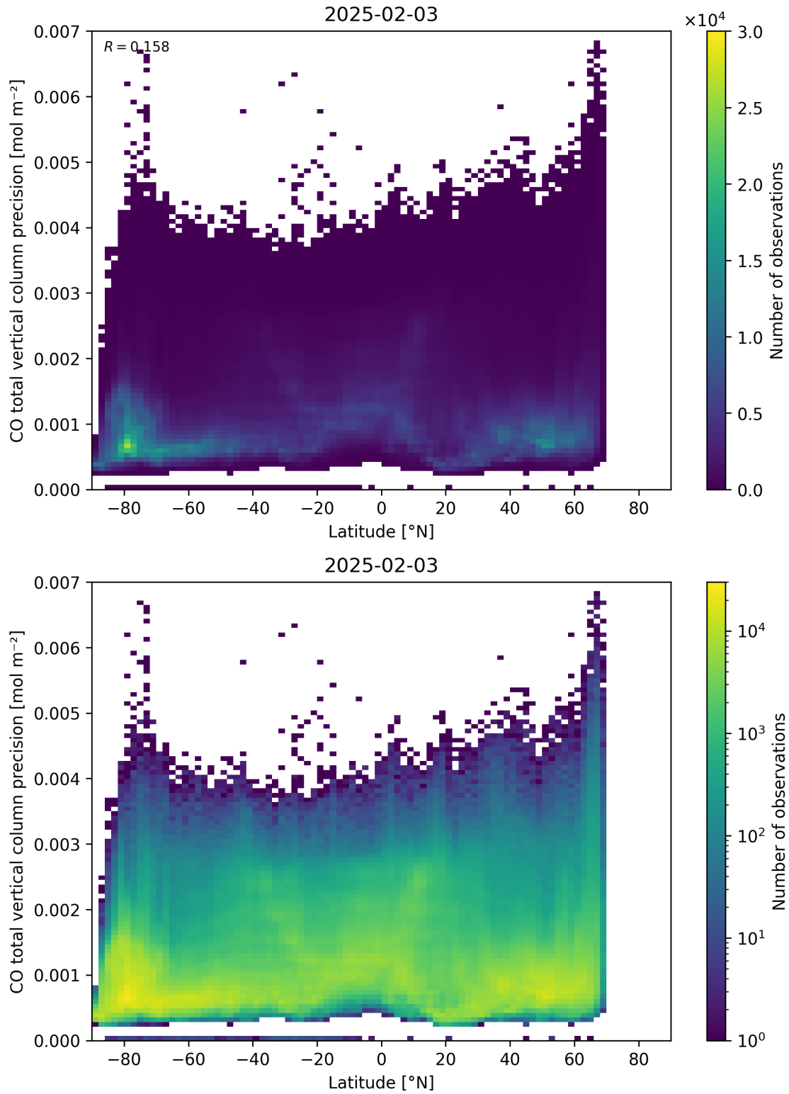
Figure 53: Scatter density plot of “Latitude” against “CO total vertical column precision” for 2025-02-03 to 2025-02-04.
