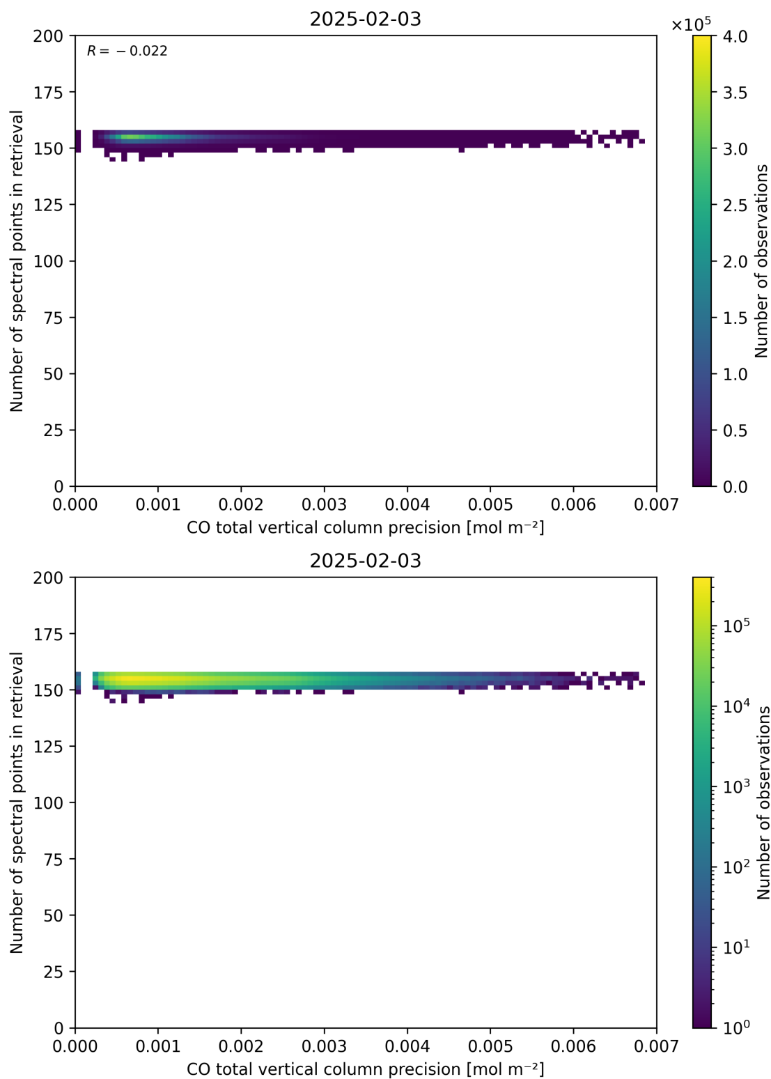
Figure 47: Scatter density plot of “CO total vertical column precision” against “Number of spectral points in retrieval” for 2025-02-03 to 2025-02-04.
