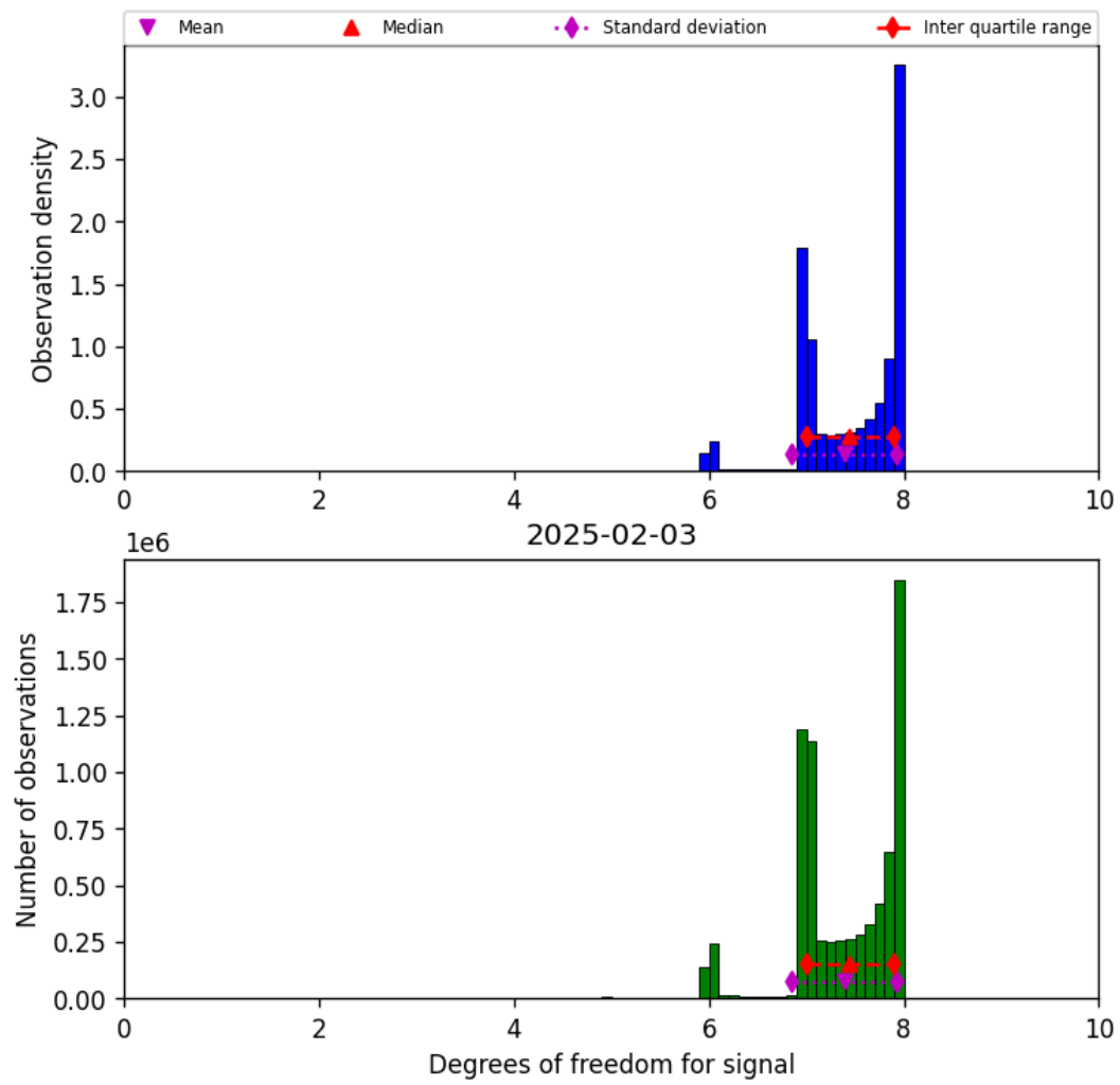
Figure 23: Histogram of “Degrees of freedom for signal” for 2025-02-03 to 2025-02-04
