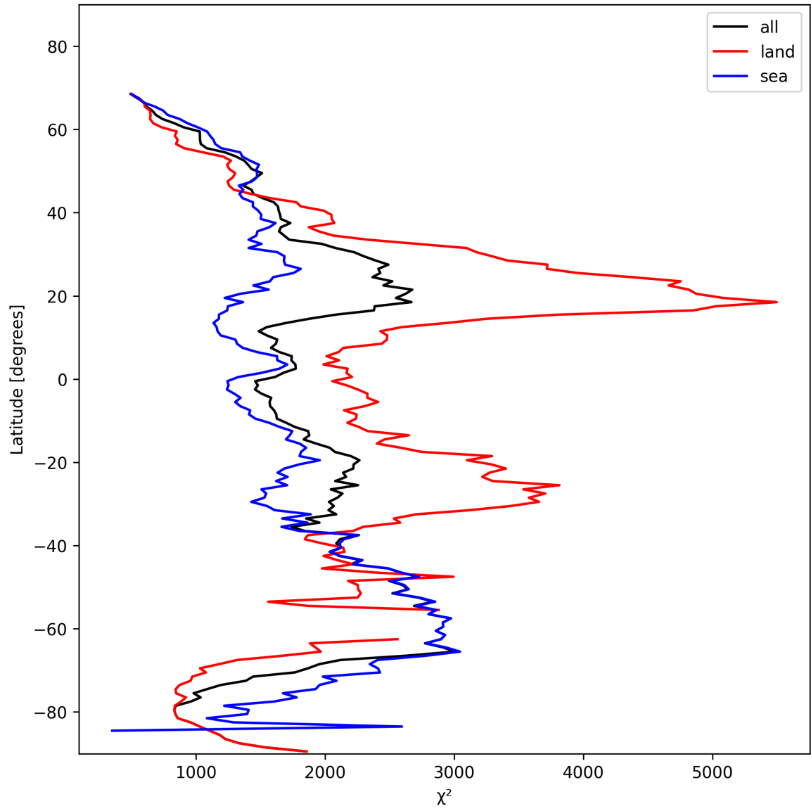
Figure 14: Zonal average of “ \chi^2 ” for 2025-02-03 to 2025-02-04.
