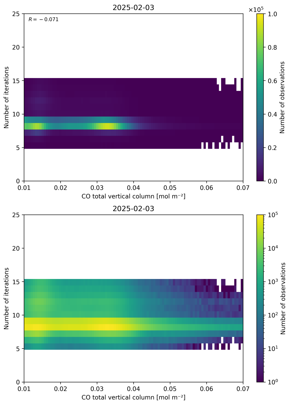
Figure 42: Scatter density plot of “CO total vertical column” against “Number of iterations” for 2025-02-03 to 2025-02-04.
