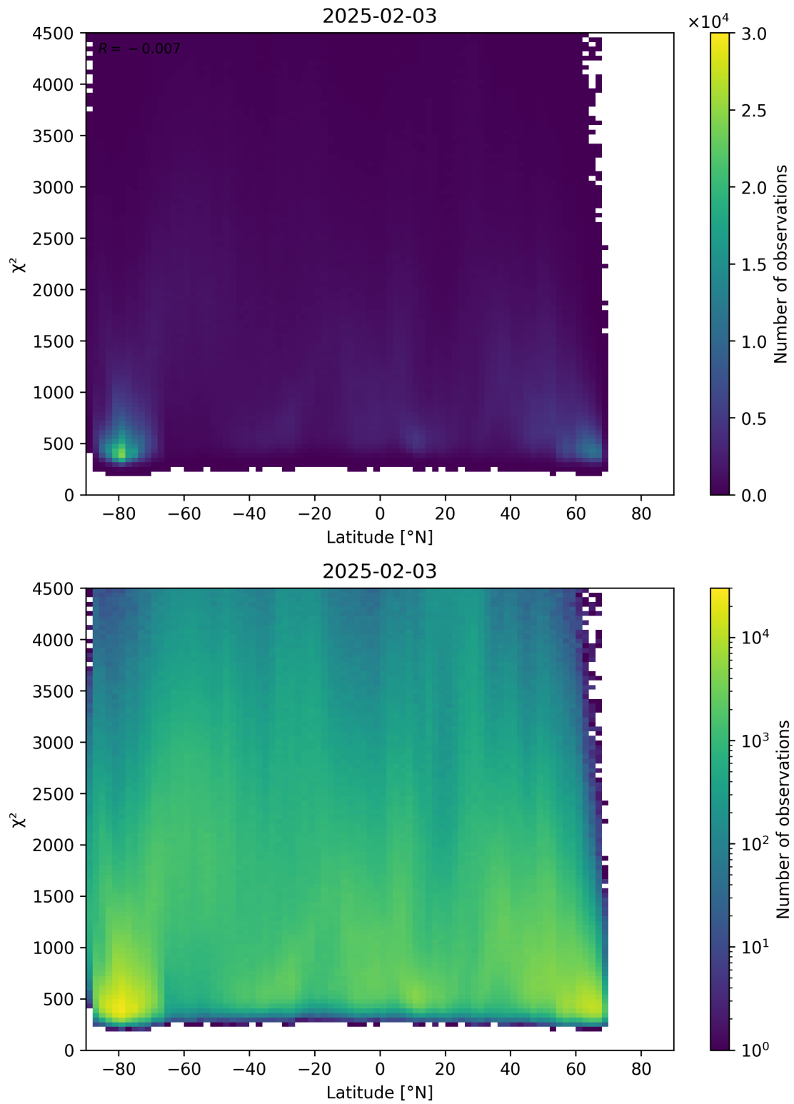
Figure 54: Scatter density plot of “Latitude” against “ \chi^2 ” for 2025-02-03 to 2025-02-04.
