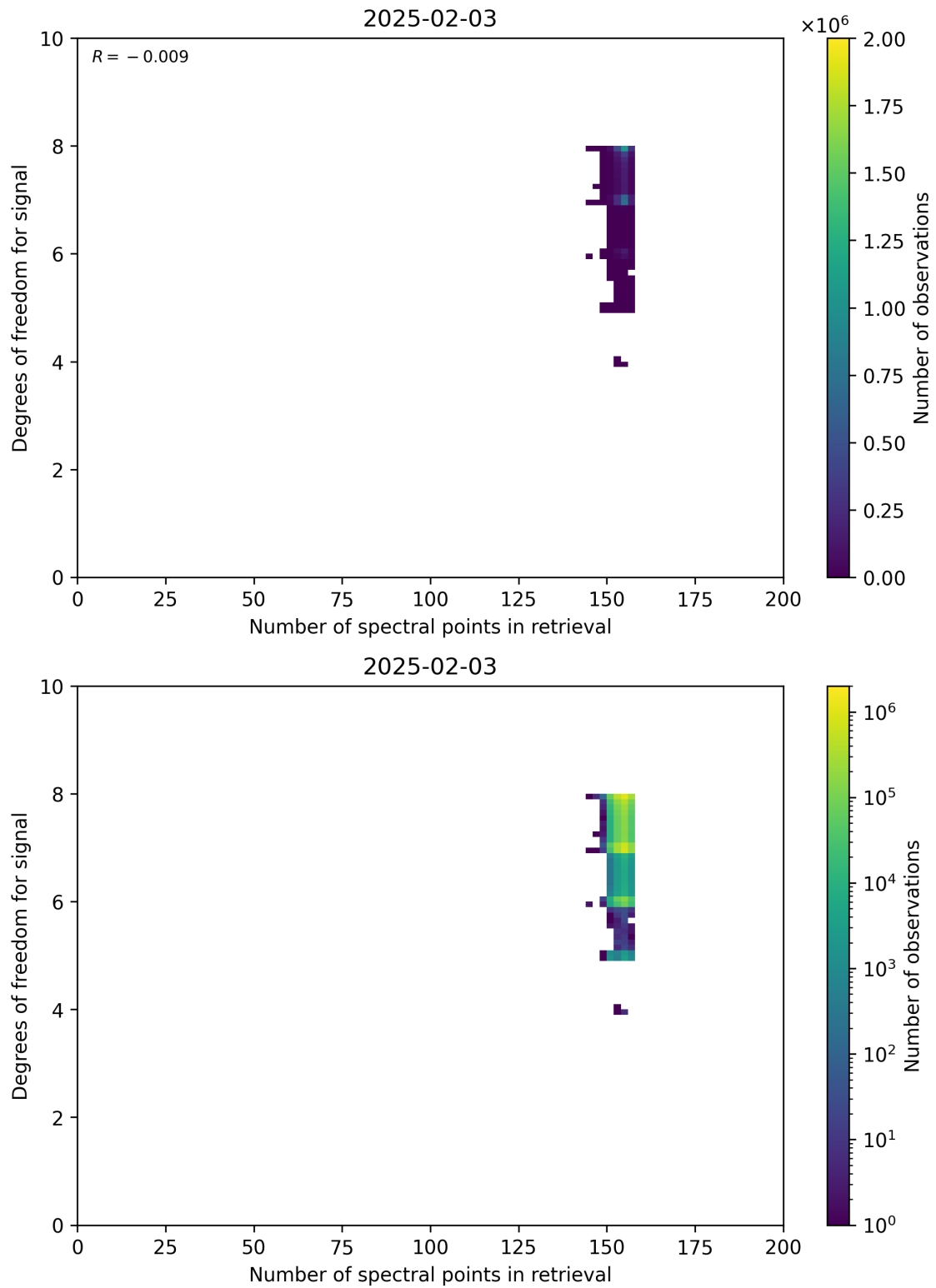
Figure 59: Scatter density plot of “Number of spectral points in retrieval” against “Degrees of freedom for signal” for 2025-02-03 to 2025-02-04.
