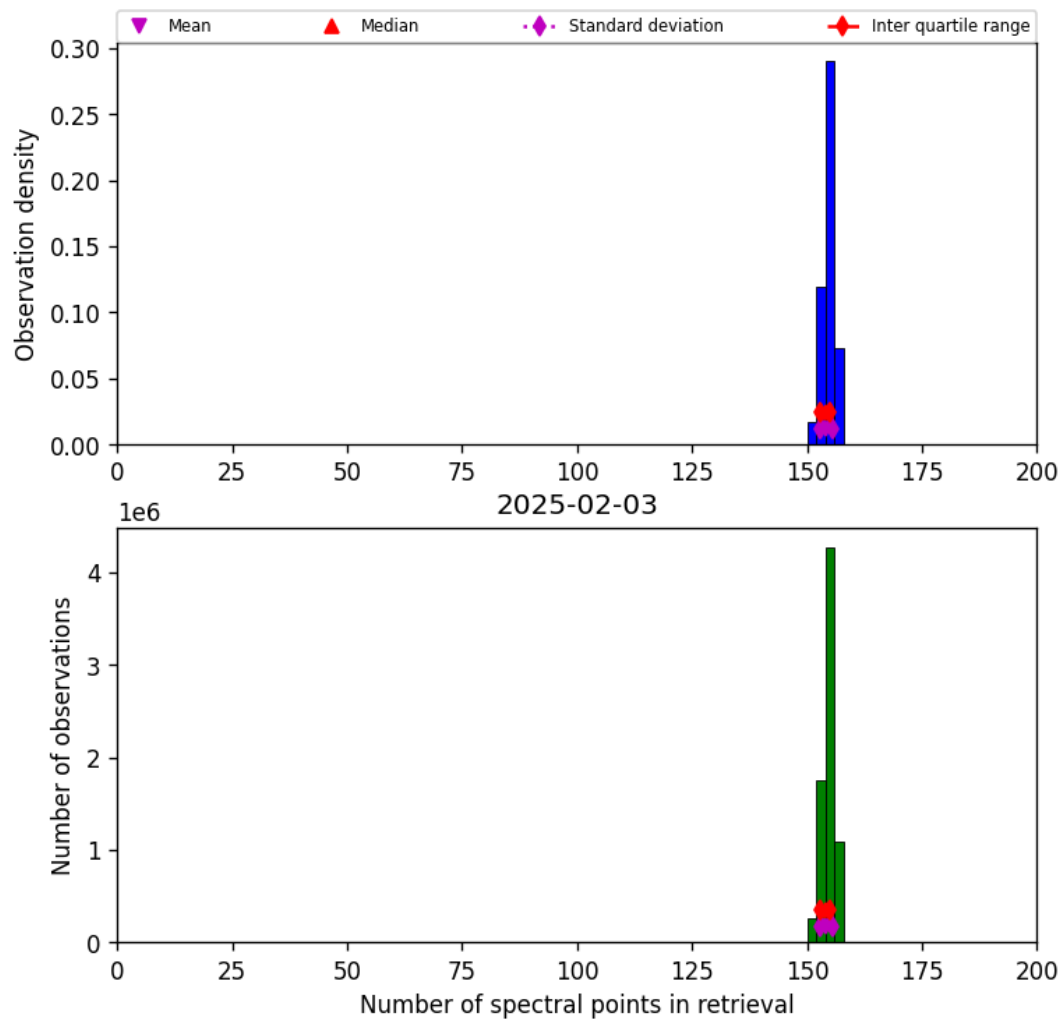
Figure 21: Histogram of “Number of spectral points in retrieval” for 2025-02-03 to 2025-02-04
