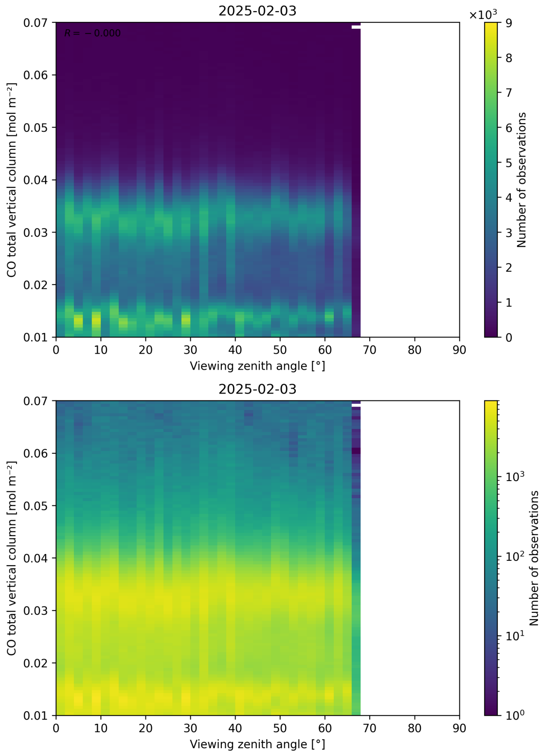
Figure 69: Scatter density plot of “Viewing zenith angle” against “CO total vertical column” for 2025-02-03 to 2025-02-04.
