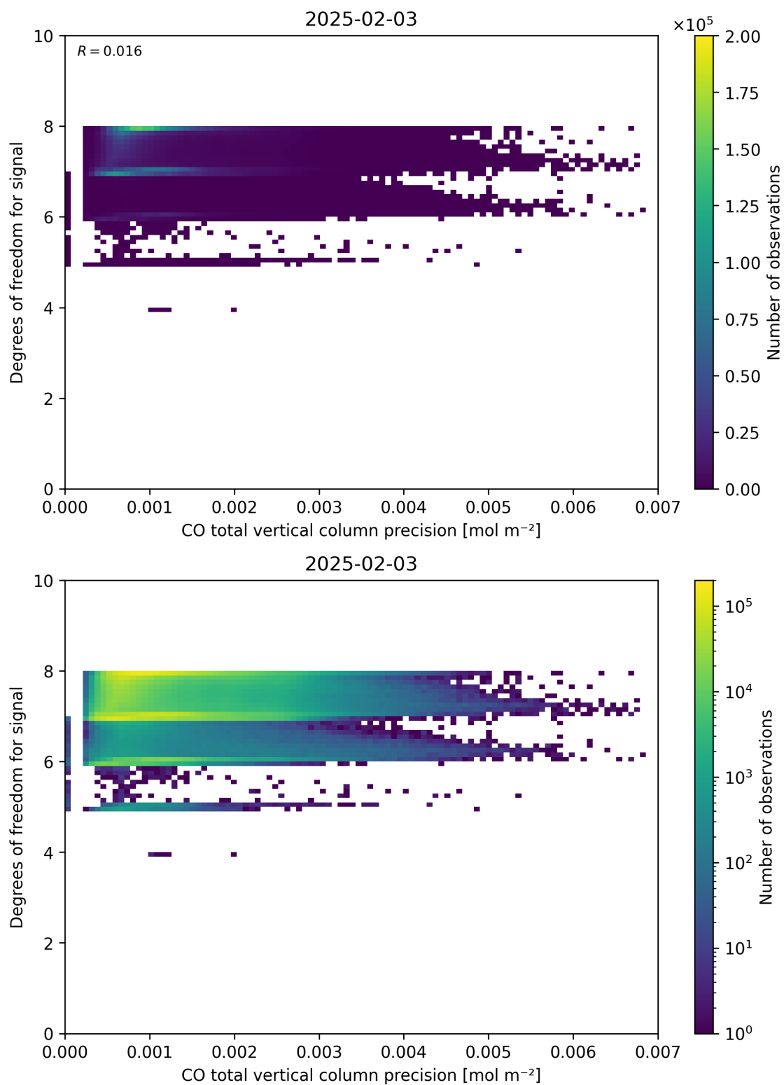
Figure 45: Scatter density plot of “CO total vertical column precision” against “Degrees of freedom for signal” for 2025-02-03 to 2025-02-04.
