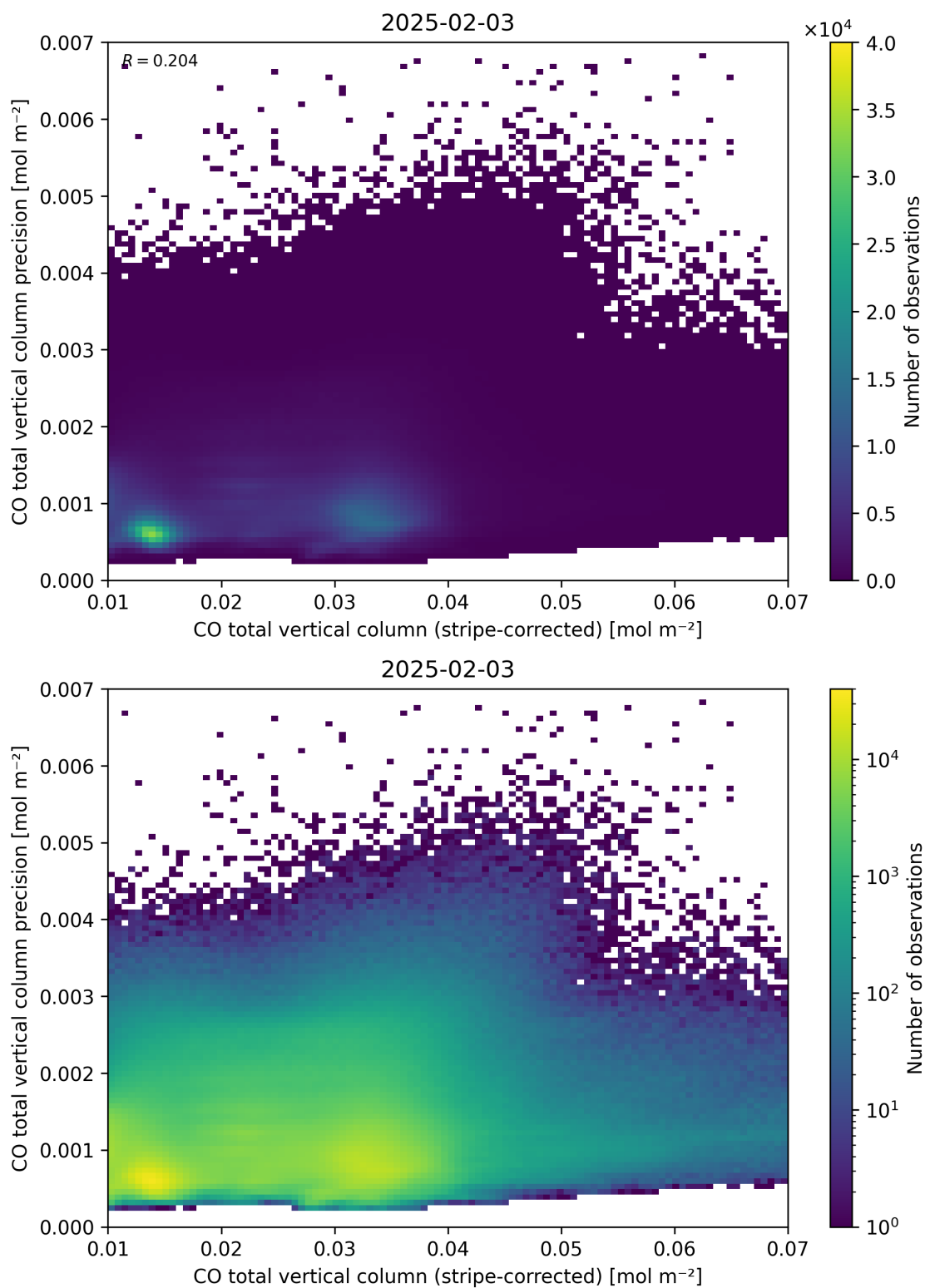
Figure 36: Scatter density plot of “CO total vertical column (stripe-corrected)” against “CO total vertical column precision” for 2025-02-03 to 2025-02-04.
