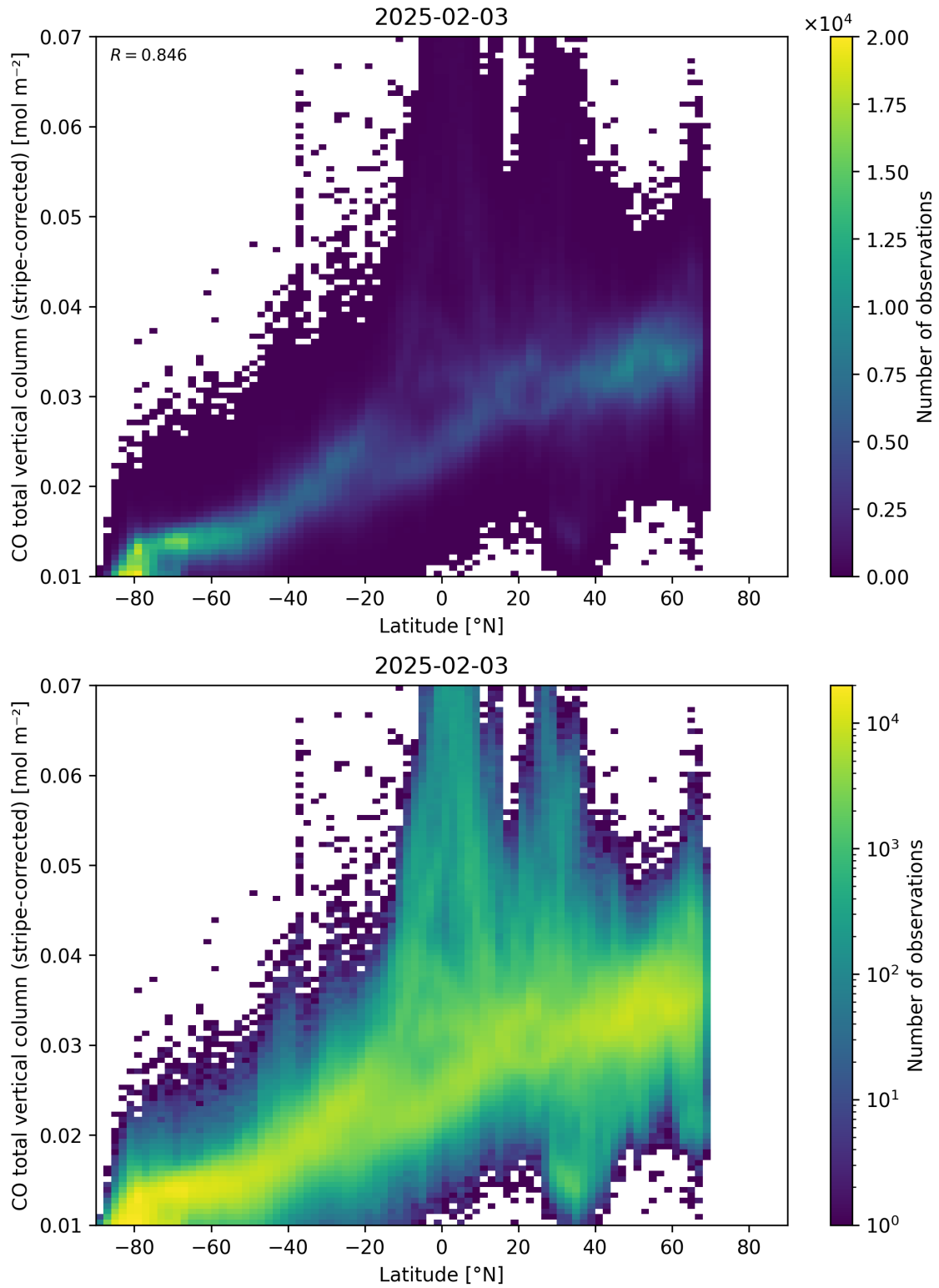
Figure 52: Scatter density plot of “Latitude” against “CO total vertical column (stripe-corrected)” for 2025-02-03 to 2025-02-04.
