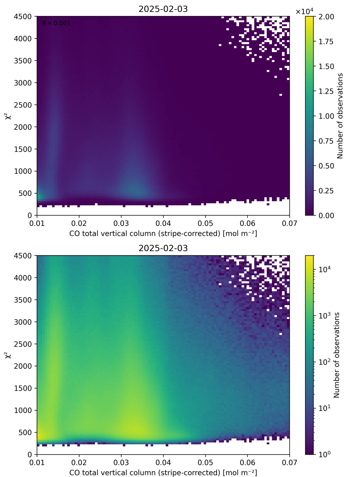
Figure 37: Scatter density plot of “CO total vertical column (stripe-corrected)” against “ \chi^2 ” for 2025-02-03 to 2025-02-04.
