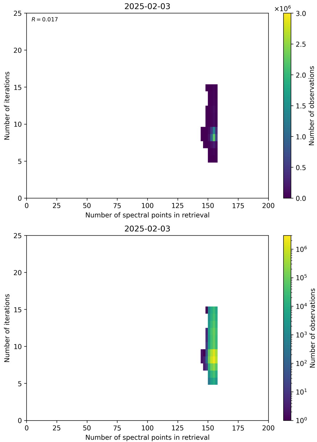
Figure 60: Scatter density plot of “Number of spectral points in retrieval” against “Number of iterations” for 2025-02-03 to 2025-02-04.
