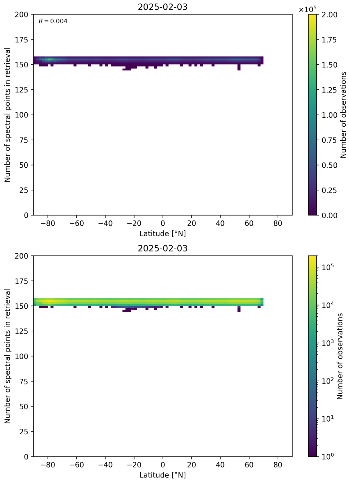
Figure 57: Scatter density plot of “Latitude” against “Number of spectral points in retrieval” for 2025-02-03 to 2025-02-04.
