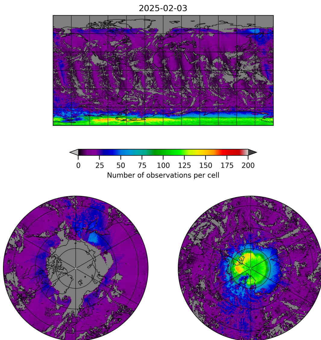
Figure 8: Map of the number of observations for 2025-02-03 to 2025-02-04
