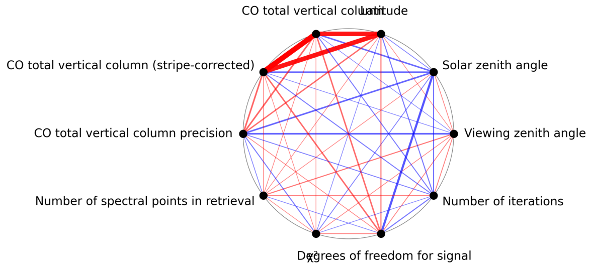
Figure 1: Map of correlation graph for 2025-02-03 to 2025-02-04.
