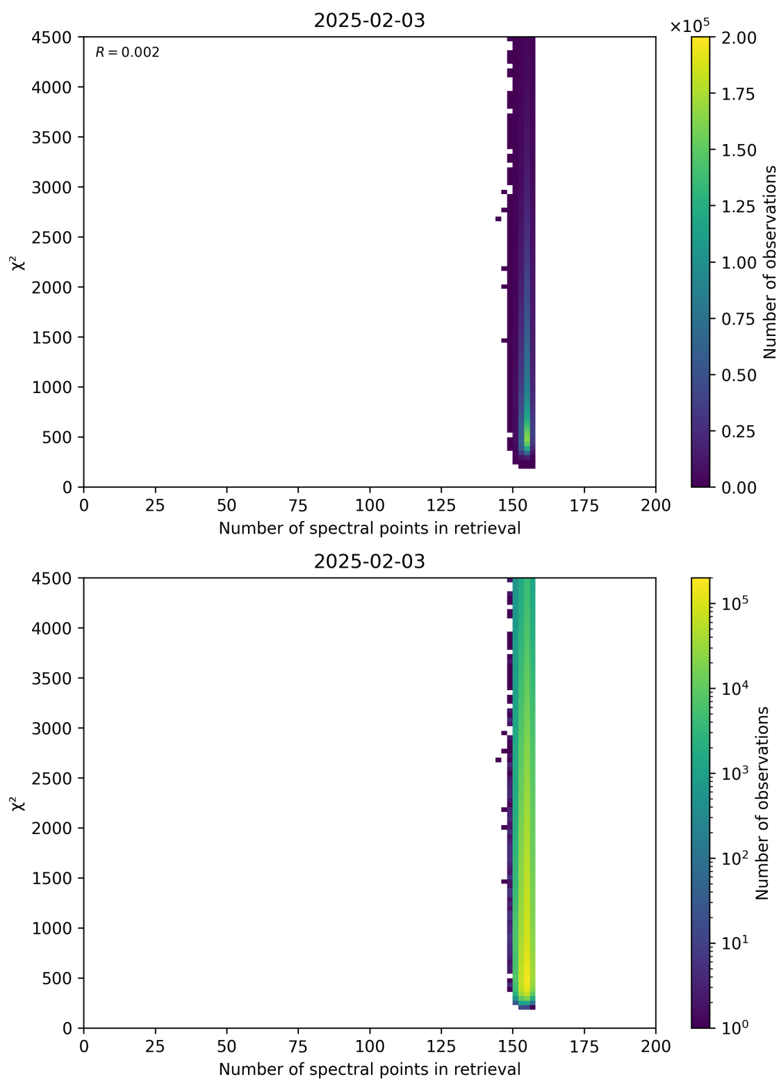
Figure 58: Scatter density plot of “Number of spectral points in retrieval” against “ \chi^2 ” for 2025-02-03 to 2025-02-04.
