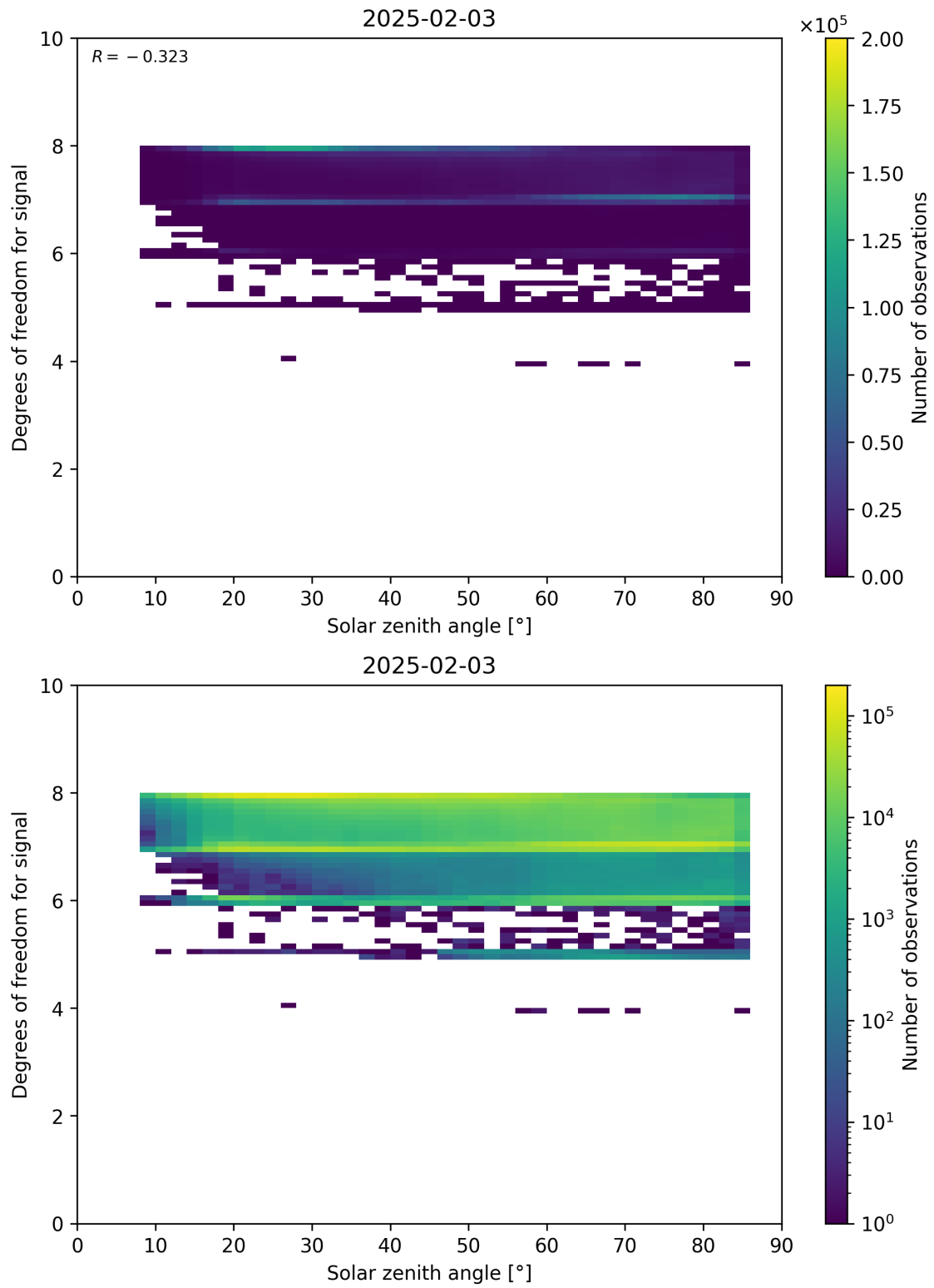
Figure 65: Scatter density plot of “Solar zenith angle” against “Degrees of freedom for signal” for 2025-02-03 to 2025-02-04.
