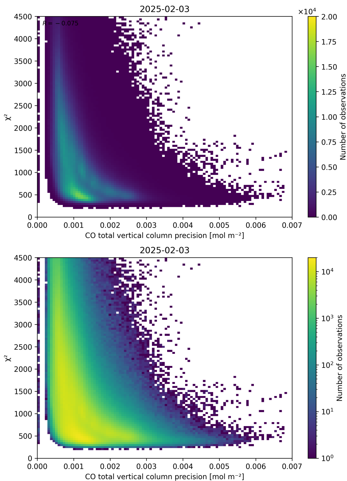
Figure 44: Scatter density plot of “CO total vertical column precision” against “ \chi^2 ” for 2025-02-03 to 2025-02-04.
