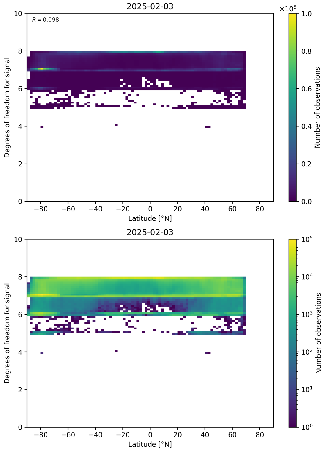
Figure 55: Scatter density plot of “Latitude” against “Degrees of freedom for signal” for 2025-02-03 to 2025-02-04.
