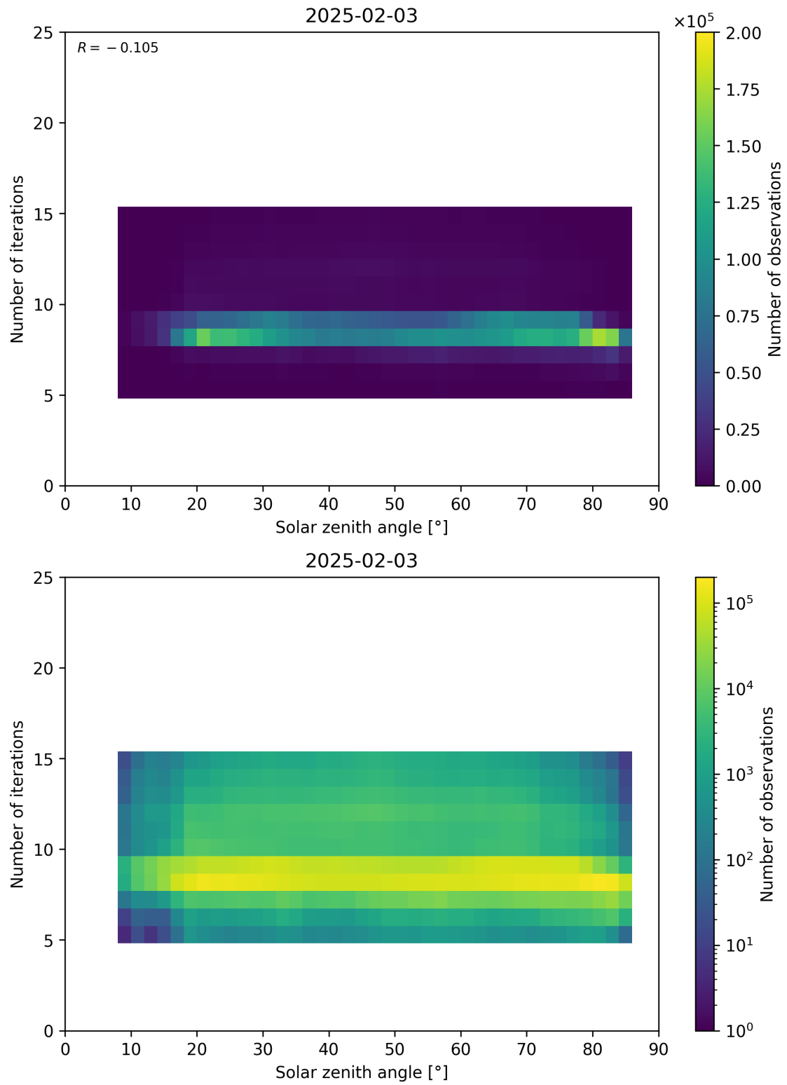
Figure 67: Scatter density plot of “Solar zenith angle” against “Number of iterations” for 2025-02-03 to 2025-02-04.
