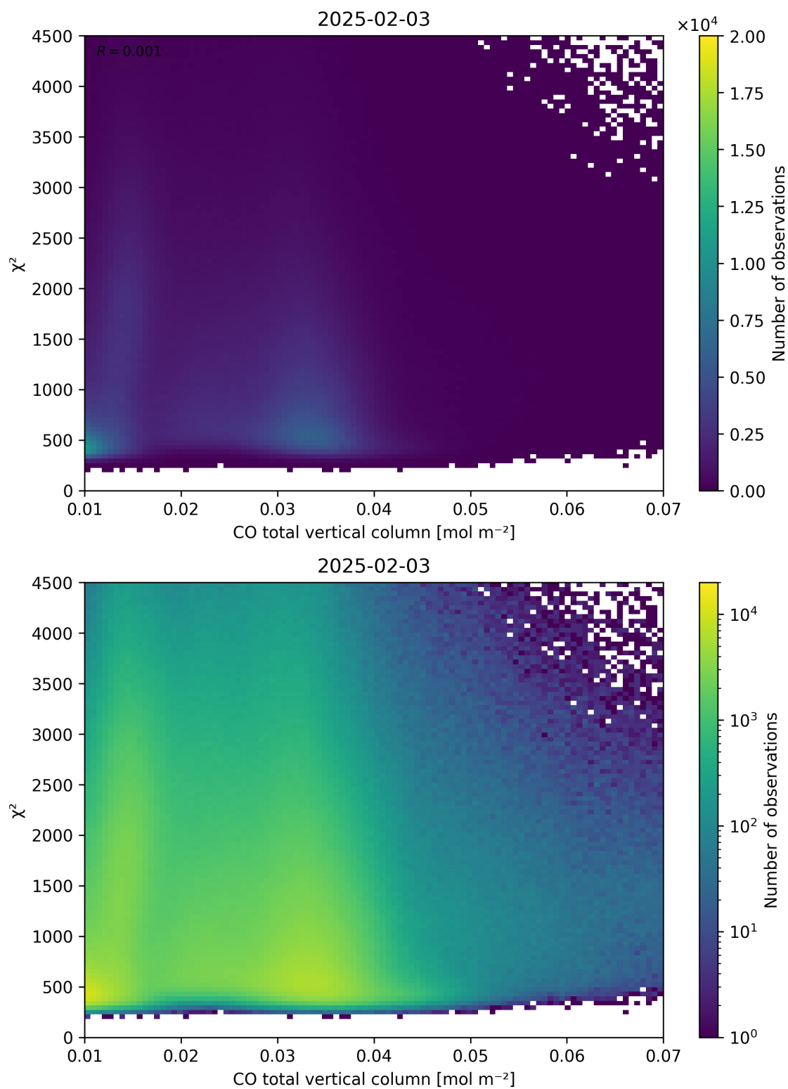
Figure 35: Scatter density plot of “CO total vertical column” against “ \chi^2 ” for 2025-02-03 to 2025-02-04.
