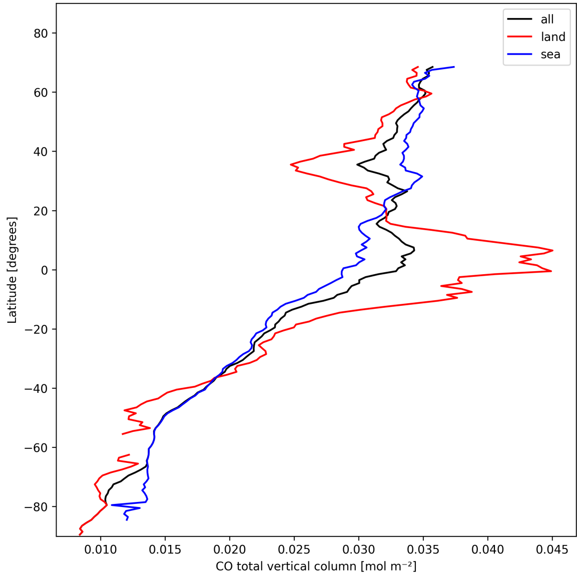
Figure 10: Zonal average of “CO total vertical column” for 2025-02-03 to 2025-02-04.
