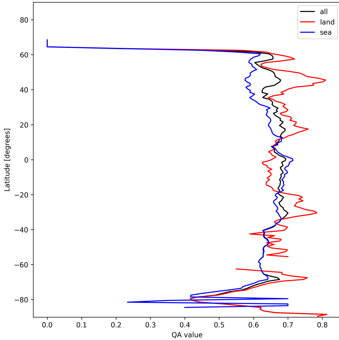
Figure 9: Zonal average of “QA value” for 2025-02-03 to 2025-02-04.
