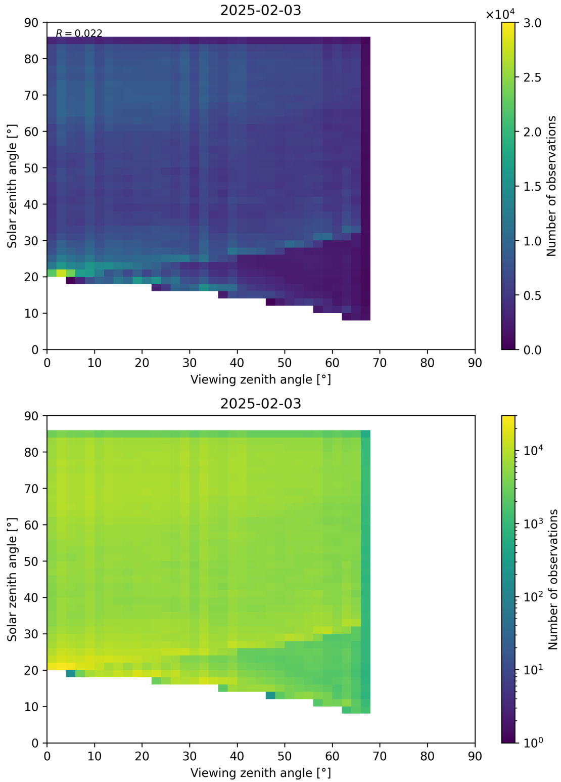
Figure 77: Scatter density plot of “Viewing zenith angle” against “Solar zenith angle” for 2025-02-03 to 2025-02-04.
