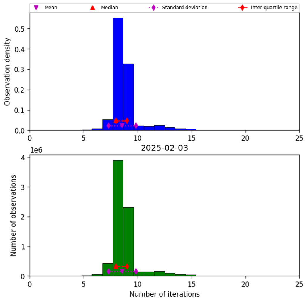
Figure 24: Histogram of “Number of iterations” for 2025-02-03 to 2025-02-04
