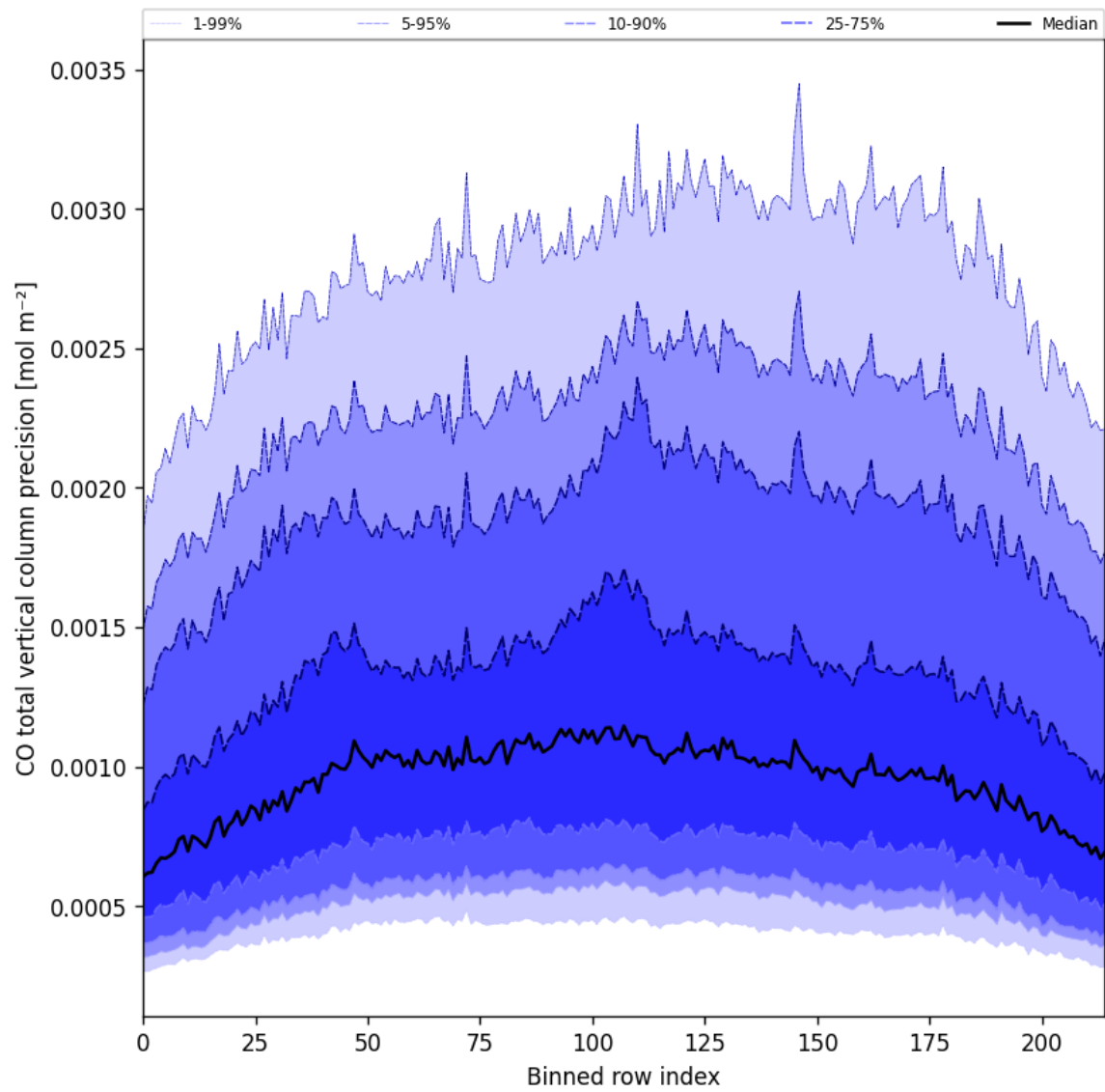
Figure 28: Along track statistics of “CO total vertical column precision” for 2025-02-03 to 2025-02-04
