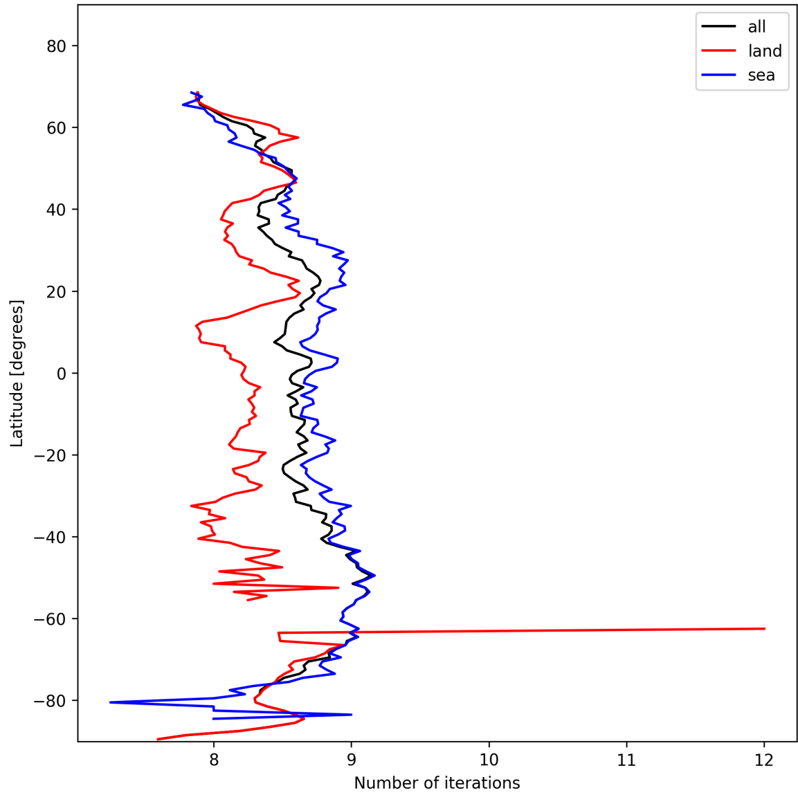
Figure 16: Zonal average of “Number of iterations” for 2025-02-03 to 2025-02-04.
