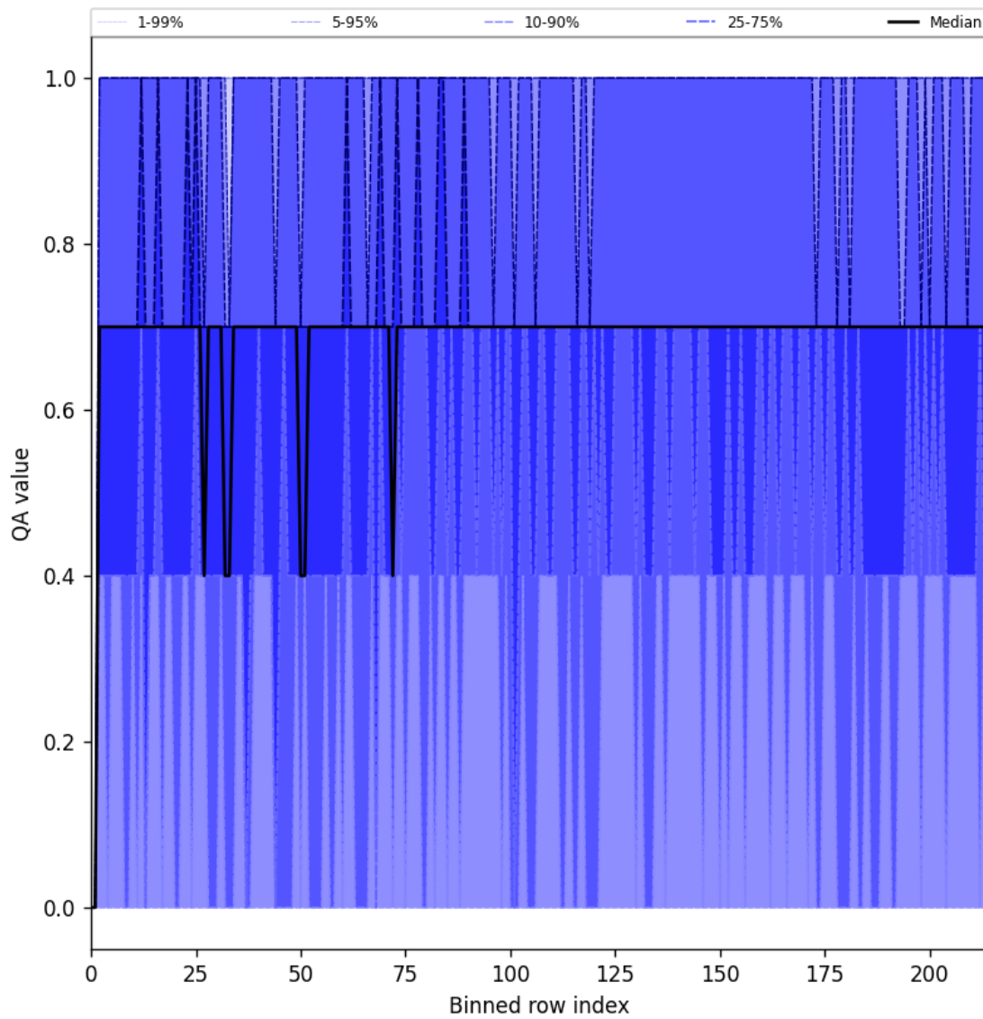
Figure 25: Along track statistics of “QA value” for 2025-02-03 to 2025-02-04
