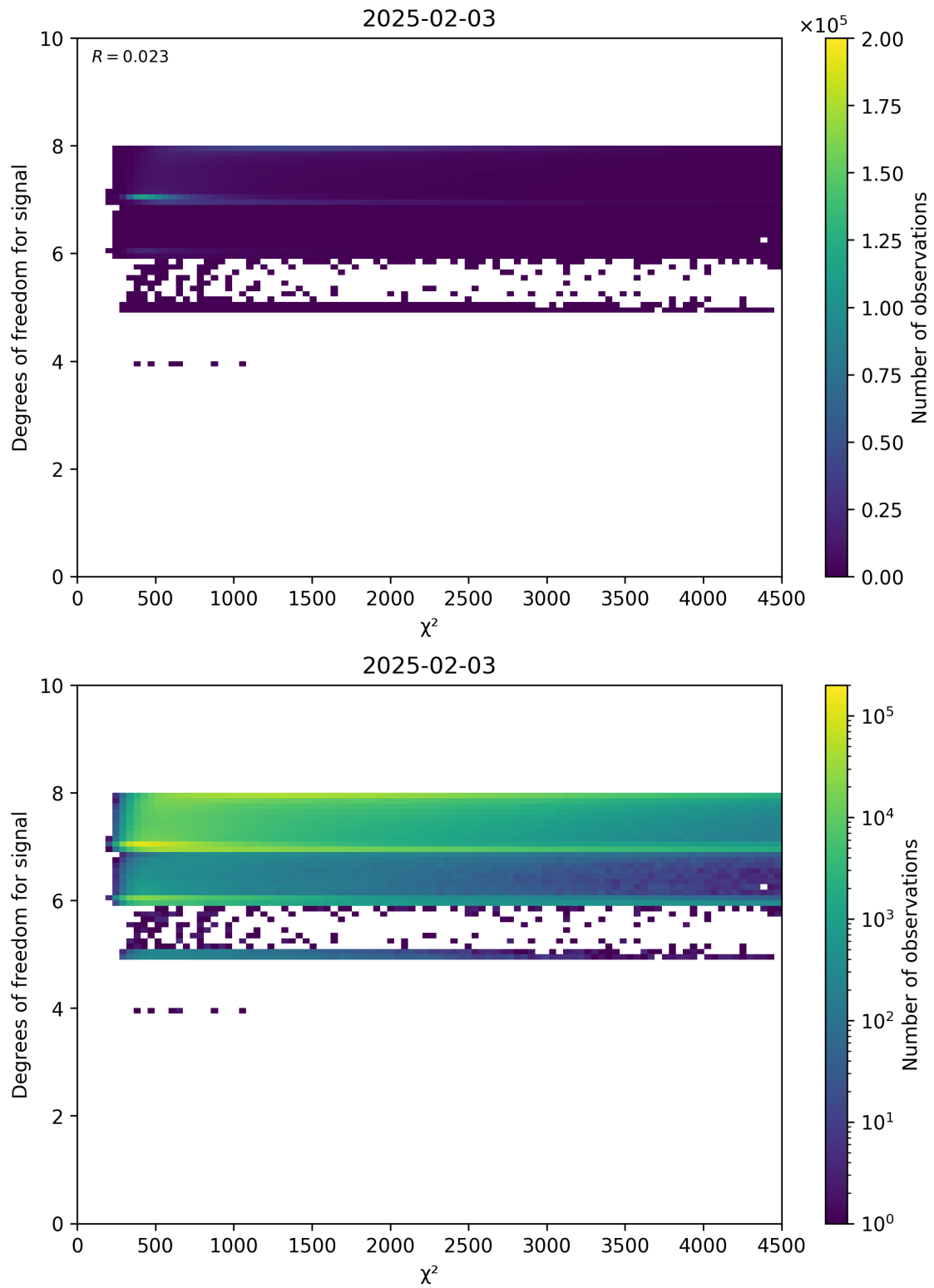
Figure 48: Scatter density plot of “ \chi^2 ” against “Degrees of freedom for signal” for 2025-02-03 to 2025-02-04.
