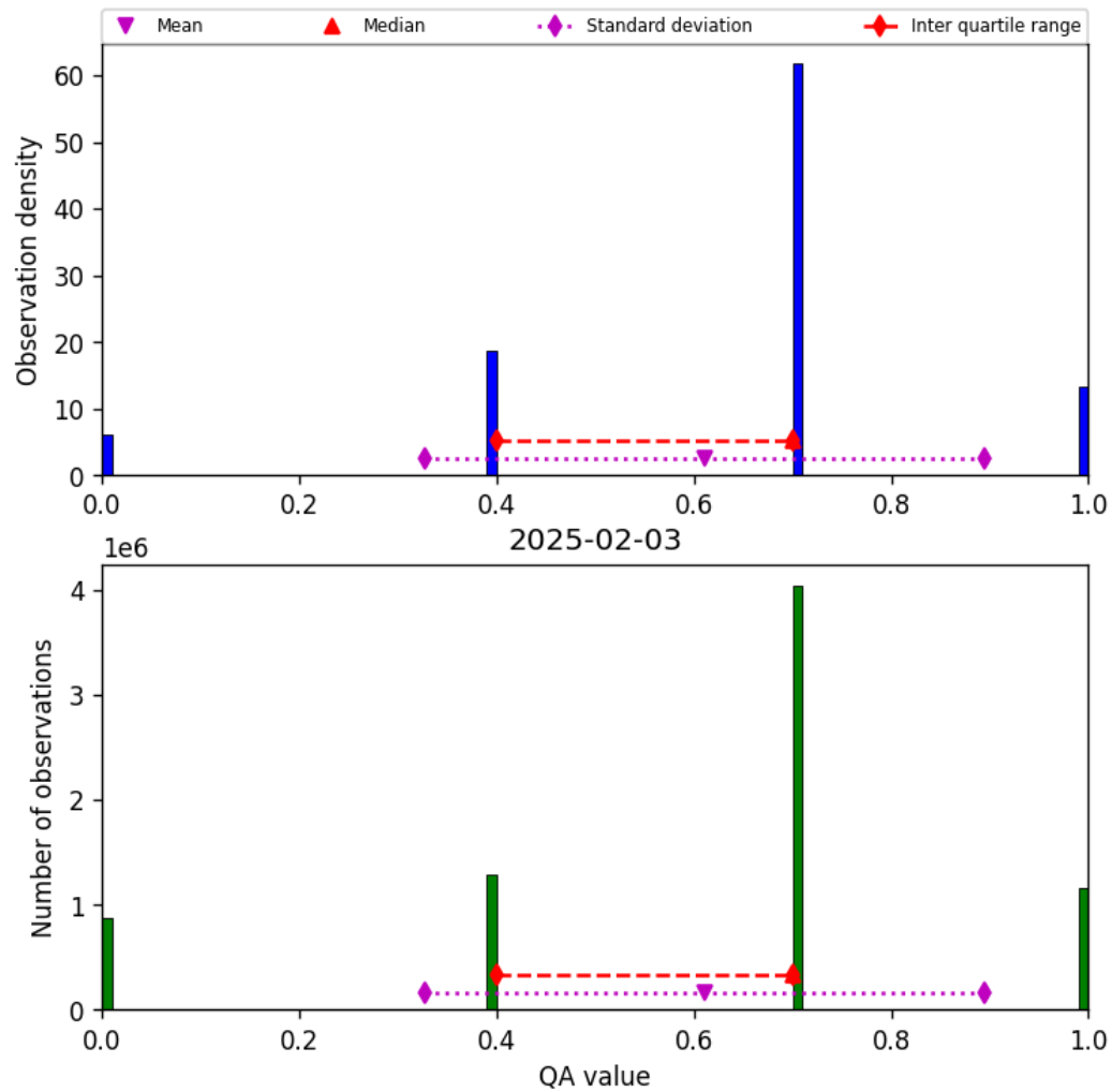
Figure 17: Histogram of “QA value” for 2025-02-03 to 2025-02-04
