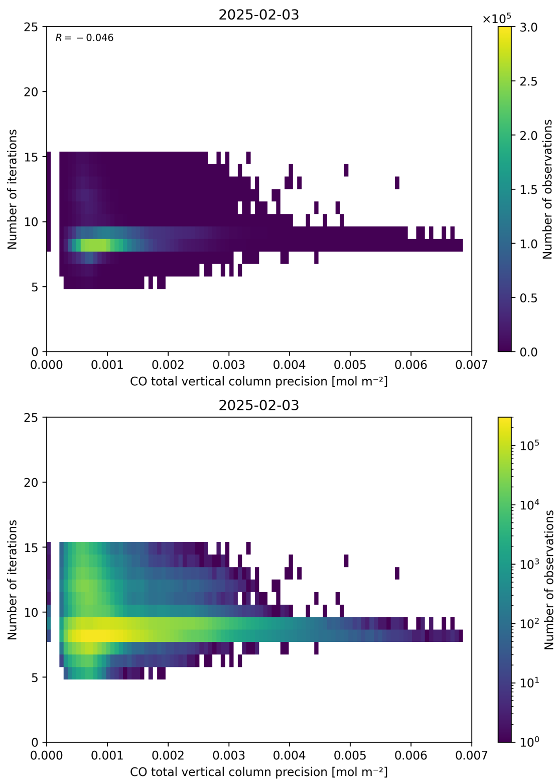
Figure 46: Scatter density plot of “CO total vertical column precision” against “Number of iterations” for 2025-02-03 to 2025-02-04.
