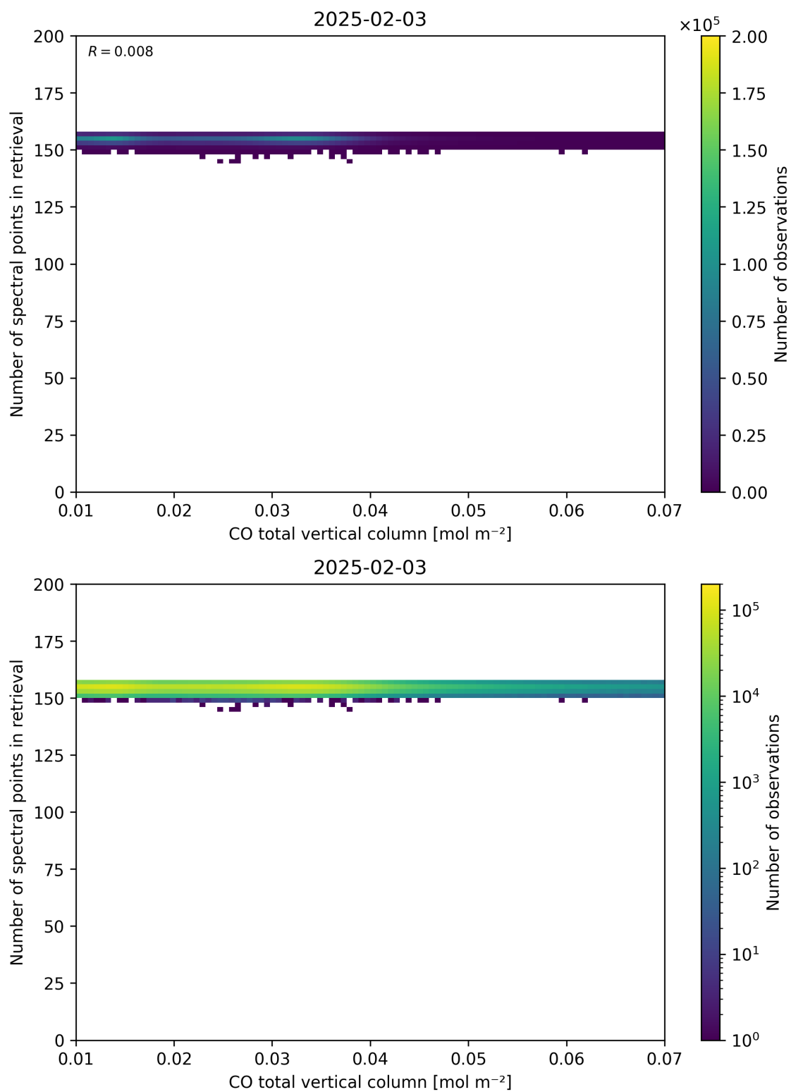
Figure 43: Scatter density plot of “CO total vertical column” against “Number of spectral points in retrieval” for 2025-02-03 to 2025-02-04.
