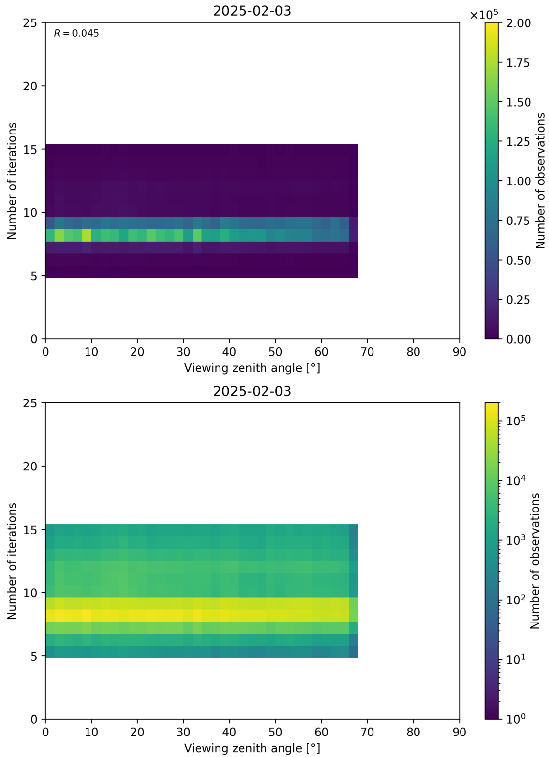
Figure 75: Scatter density plot of “Viewing zenith angle” against “Number of iterations” for 2025-02-03 to 2025-02-04.
