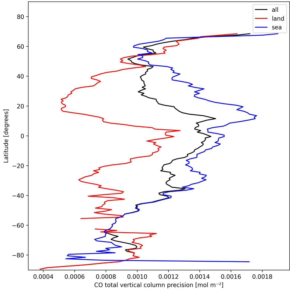
Figure 12: Zonal average of "CO total vertical column precision" for 2025-02-03 to 2025-02-04.
