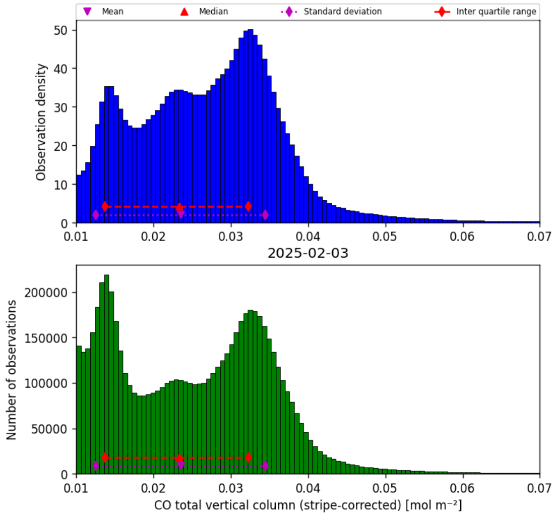
Figure 19: Histogram of “CO total vertical column (stripe-corrected)” for 2025-02-03 to 2025-02-04
