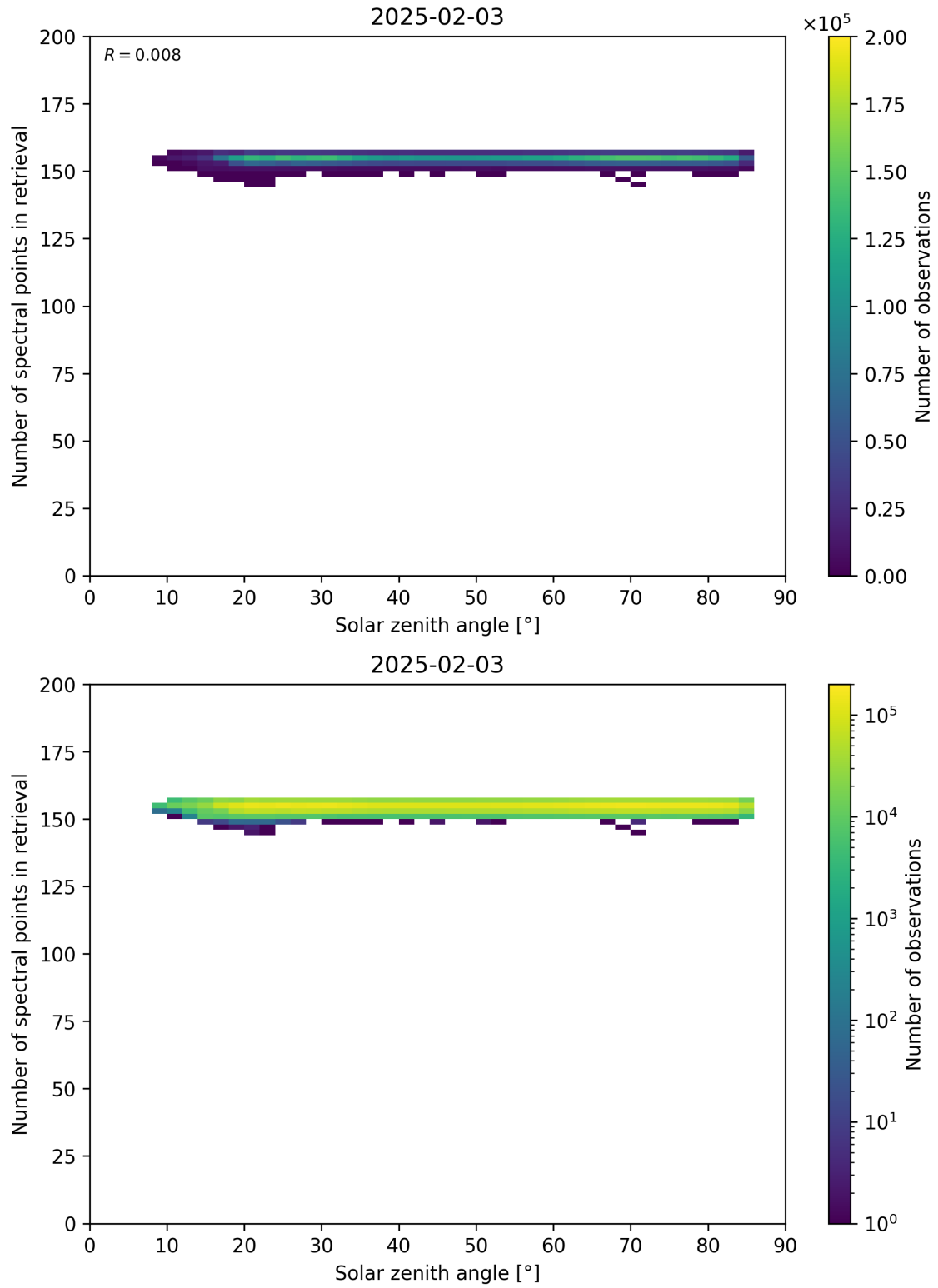
Figure 68: Scatter density plot of “Solar zenith angle” against “Number of spectral points in retrieval” for 2025-02-03 to 2025-02-04.
