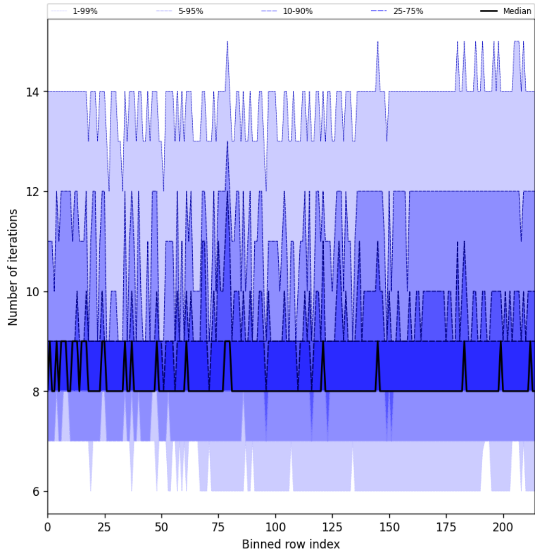
Figure 32: Along track statistics of “Number of iterations” for 2025-02-03 to 2025-02-04
