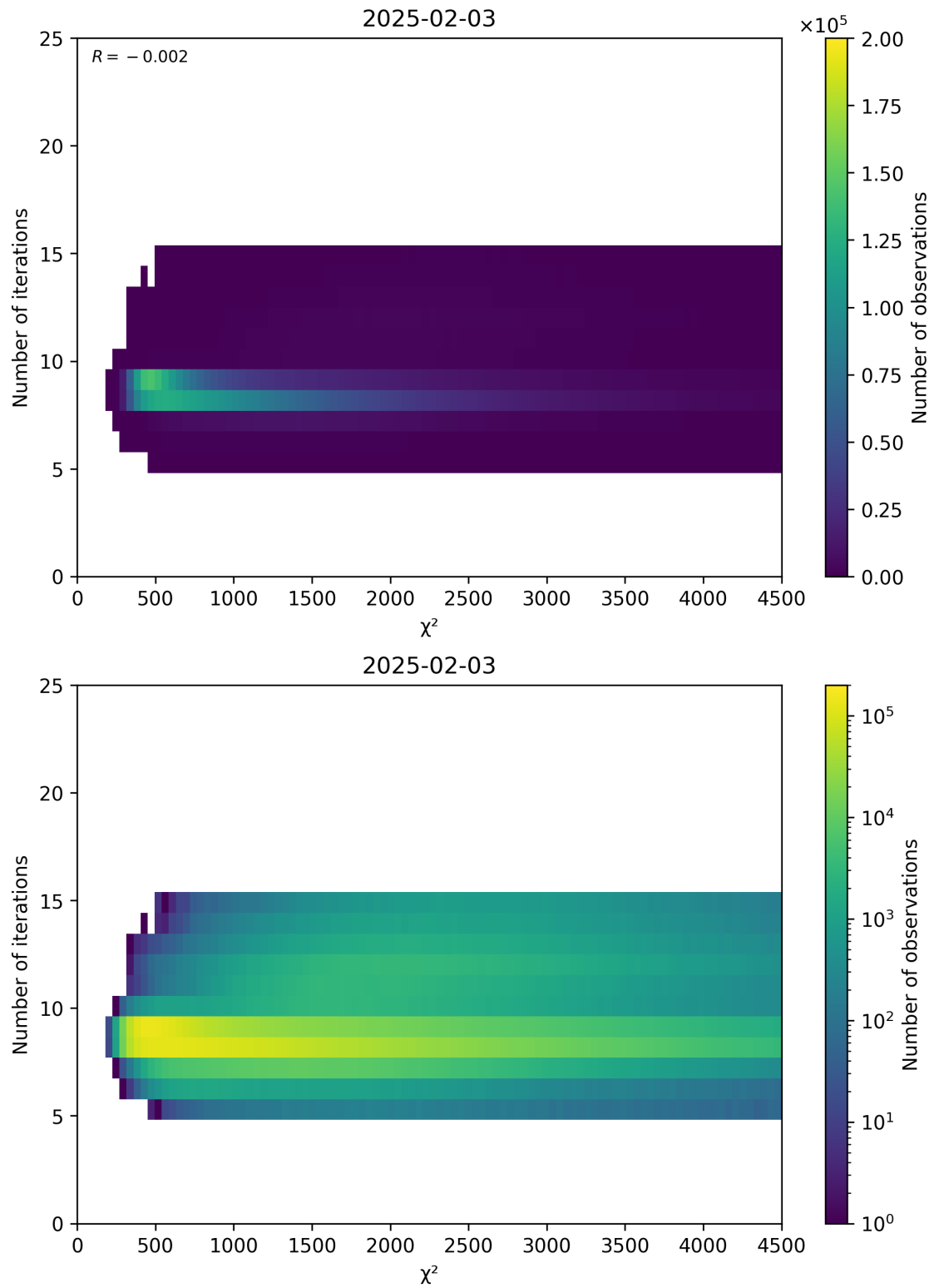
Figure 49: Scatter density plot of “ \chi^2 ” against “Number of iterations” for 2025-02-03 to 2025-02-04.
