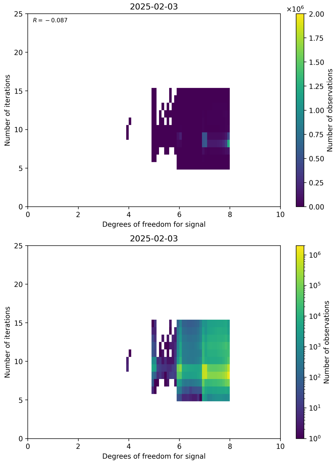
Figure 50: Scatter density plot of “Degrees of freedom for signal” against “Number of iterations” for 2025-02-03 to 2025-02-04.
