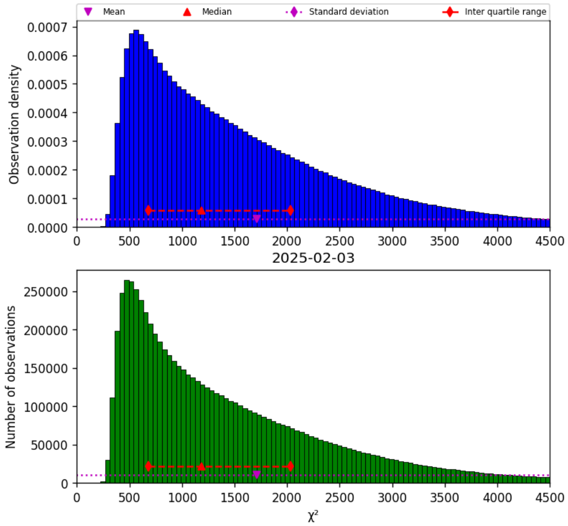
Figure 22: Histogram of “ \chi^2 ” for 2025-02-03 to 2025-02-04
