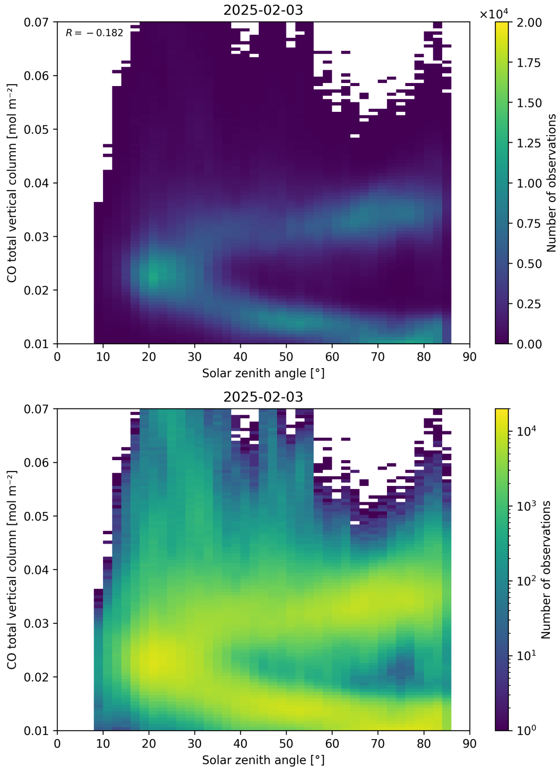
Figure 61: Scatter density plot of “Solar zenith angle” against “CO total vertical column” for 2025-02-03 to 2025-02-04.
