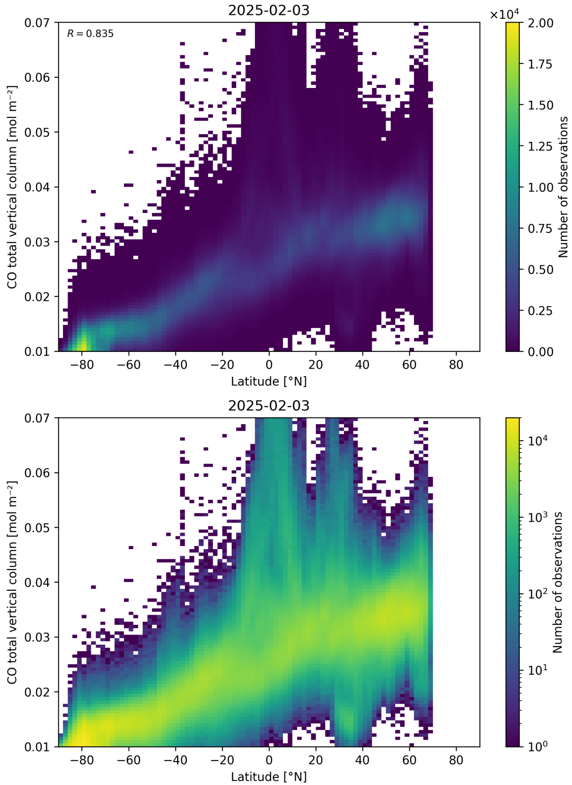
Figure 51: Scatter density plot of “Latitude” against “CO total vertical column” for 2025-02-03 to 2025-02-04.
