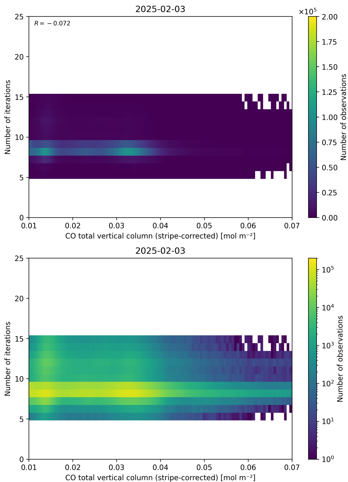
Figure 39: Scatter density plot of “CO total vertical column (stripe-corrected)” against “Number of iterations” for 2025-02-03 to 2025-02-04.
