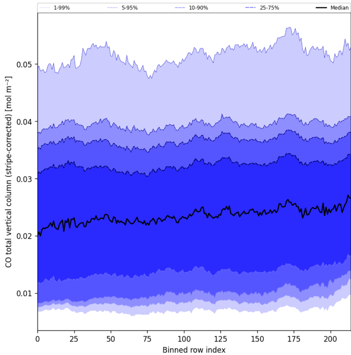
Figure 27: Along track statistics of “CO total vertical column (stripe-corrected)” for 2025-02-03 to 2025-02-04
