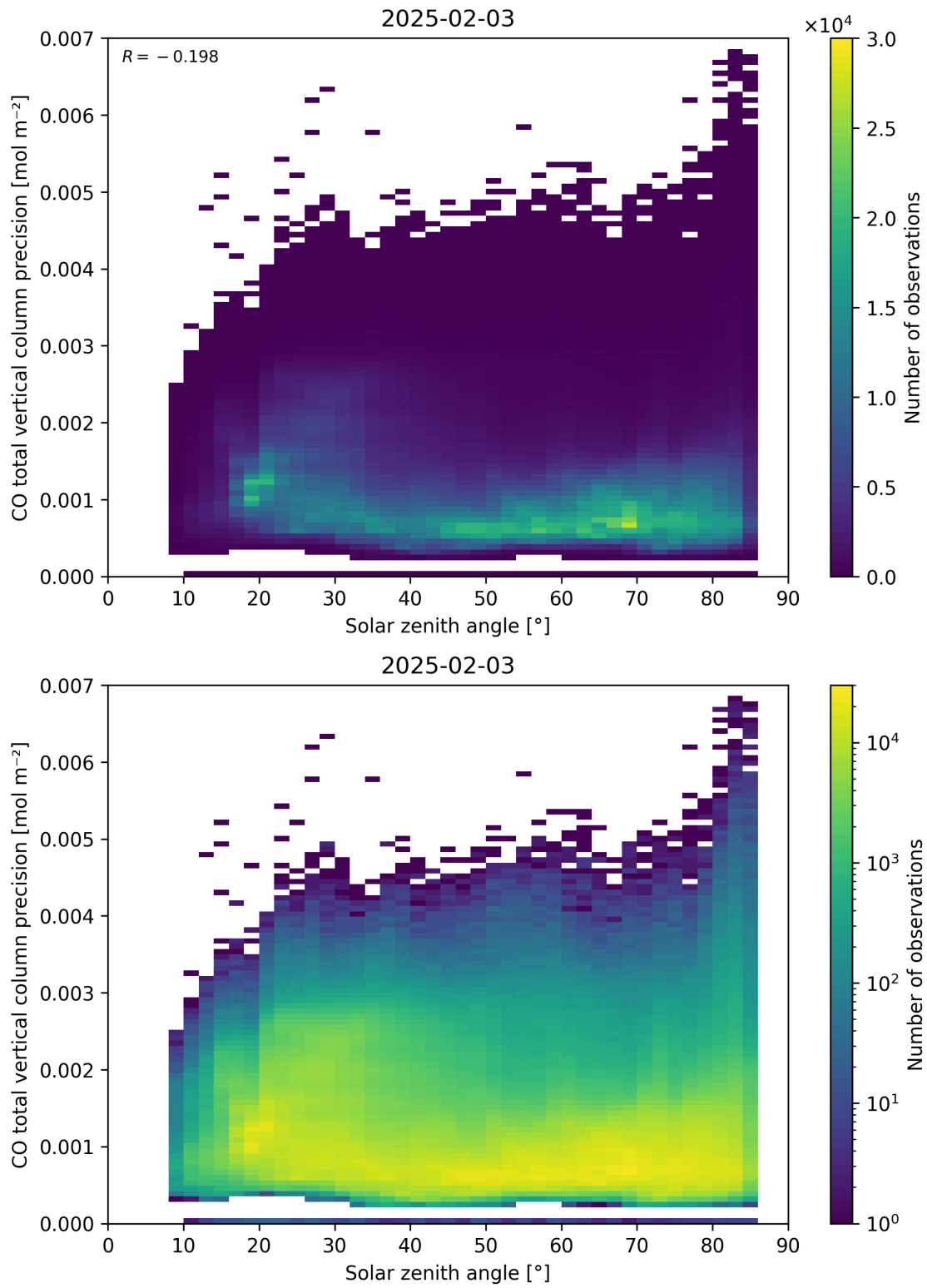
Figure 63: Scatter density plot of “Solar zenith angle” against “CO total vertical column precision” for 2025-02-03 to 2025-02-04.
