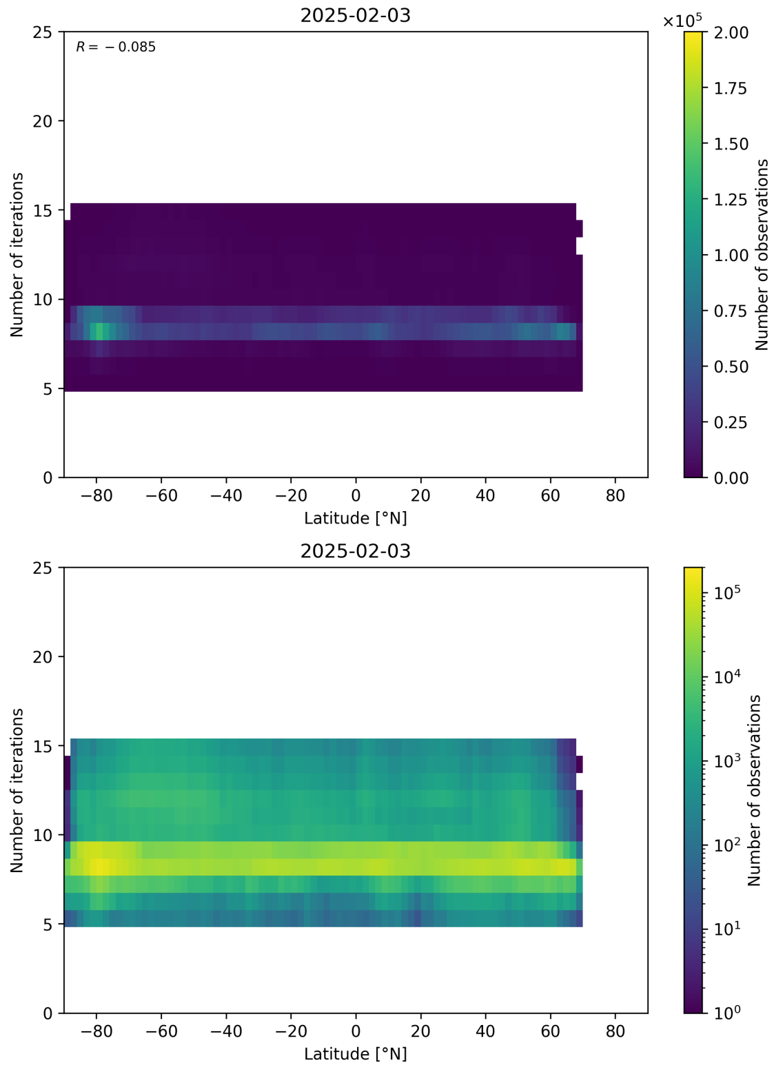
Figure 56: Scatter density plot of “Latitude” against “Number of iterations” for 2025-02-03 to 2025-02-04.
