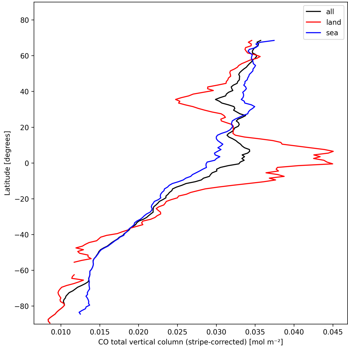
Figure 11: Zonal average of “CO total vertical column (stripe-corrected)” for 2025-02-03 to 2025-02-04.
