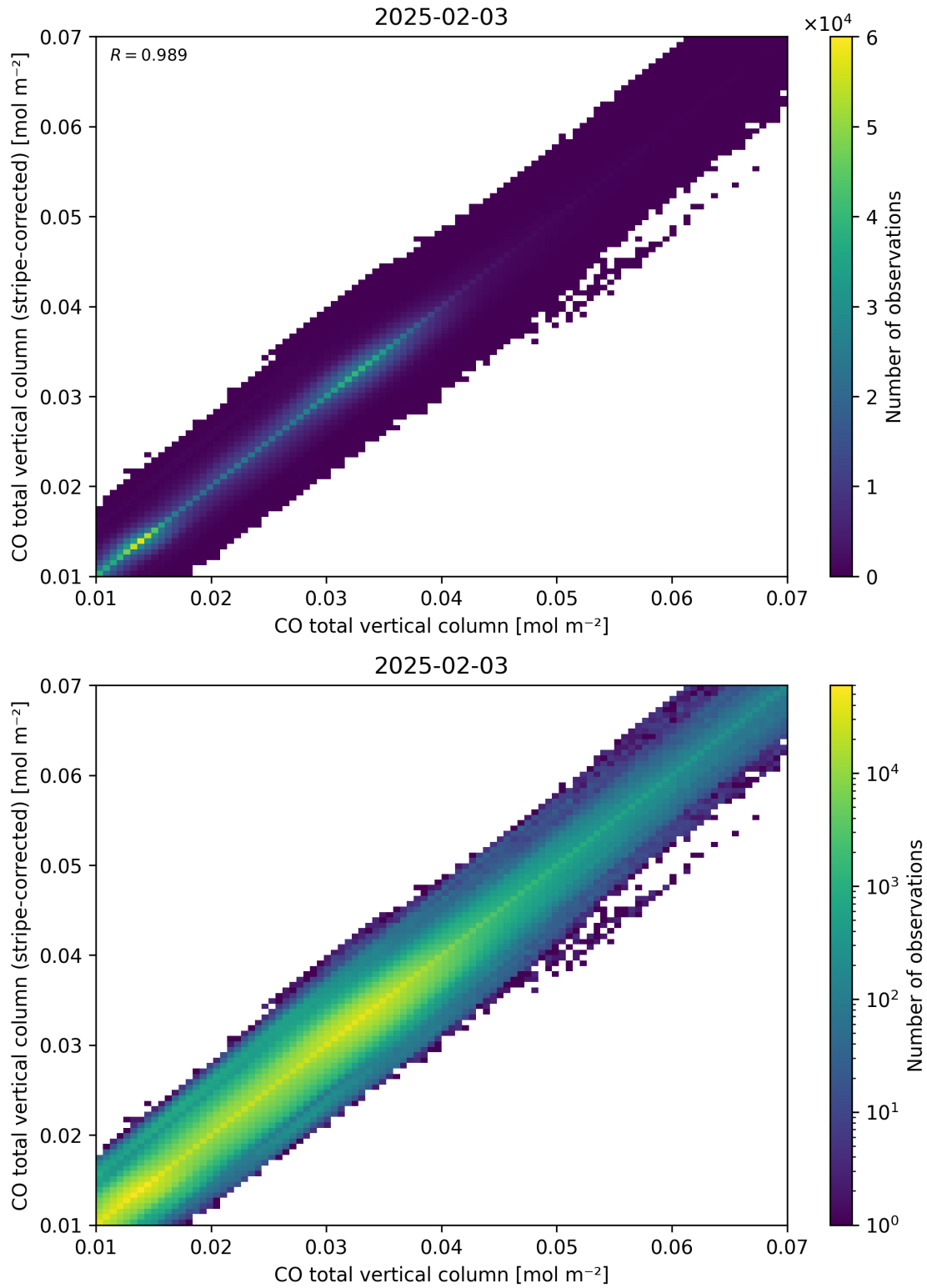
Figure 33: Scatter density plot of “CO total vertical column” against “CO total vertical column (stripe-corrected)” for 2025-02-03 to 2025-02-04.
