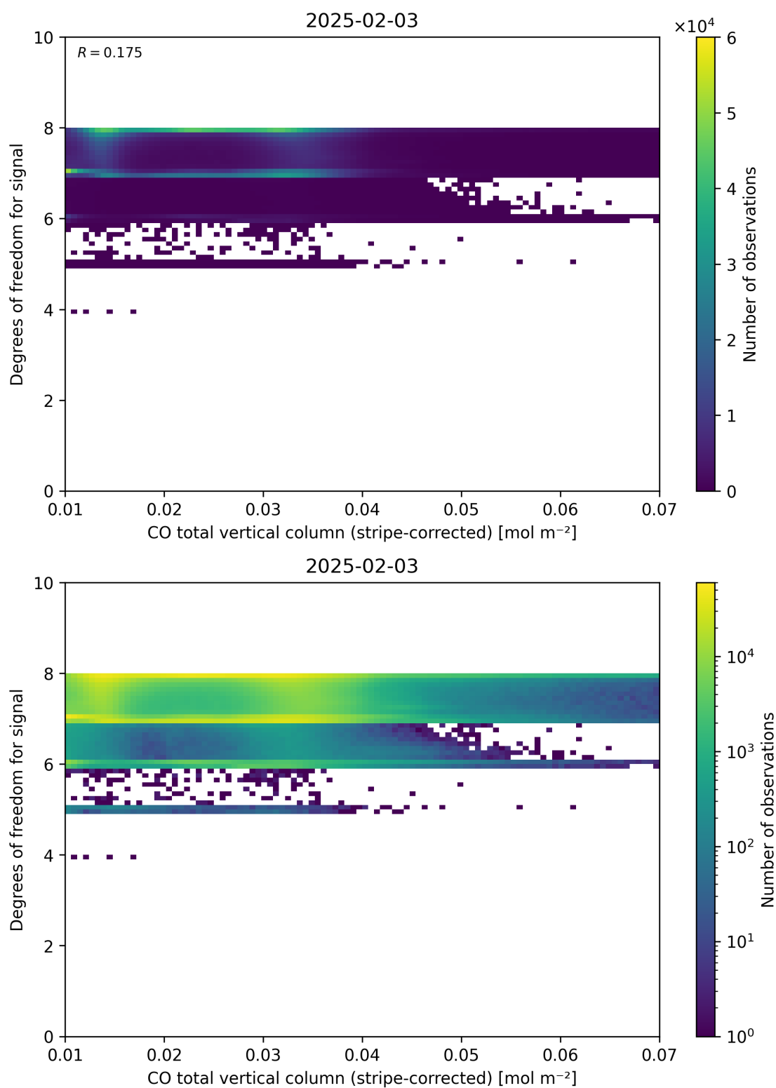
Figure 38: Scatter density plot of “CO total vertical column (stripe-corrected)” against “Degrees of freedom for signal” for 2025-02-03 to 2025-02-04.
