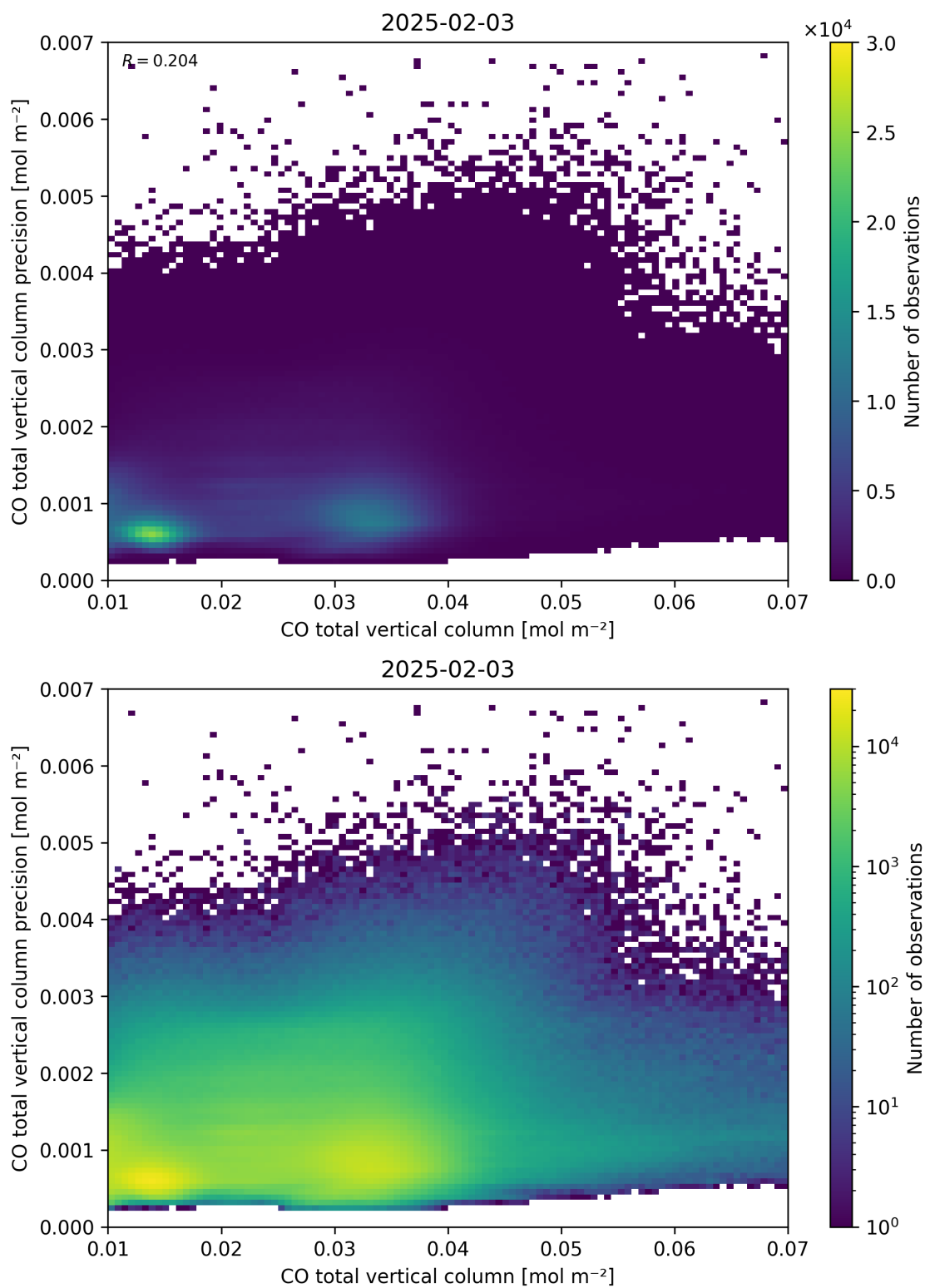
Figure 34: Scatter density plot of “CO total vertical column” against “CO total vertical column precision” for 2025-02-03 to 2025-02-04.
