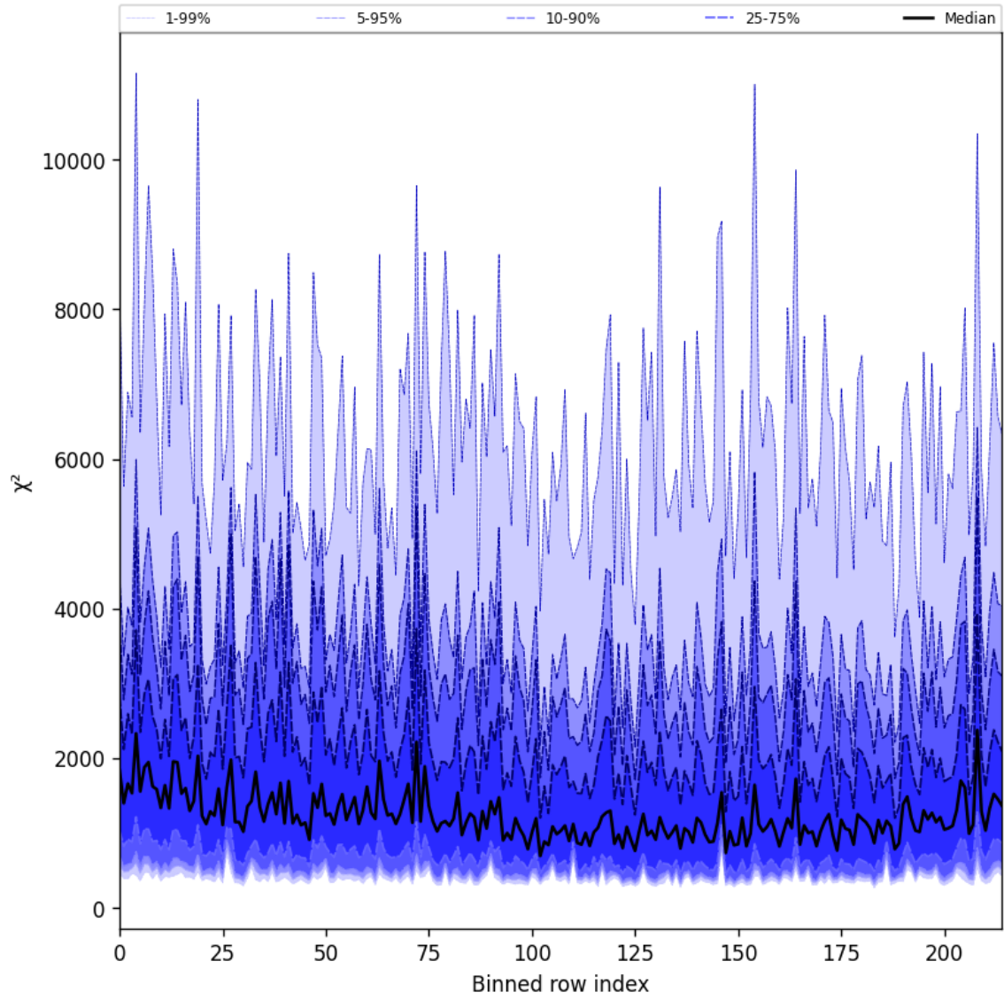
Figure 30: Along track statistics of “ \chi^2 ” for 2025-02-03 to 2025-02-04
