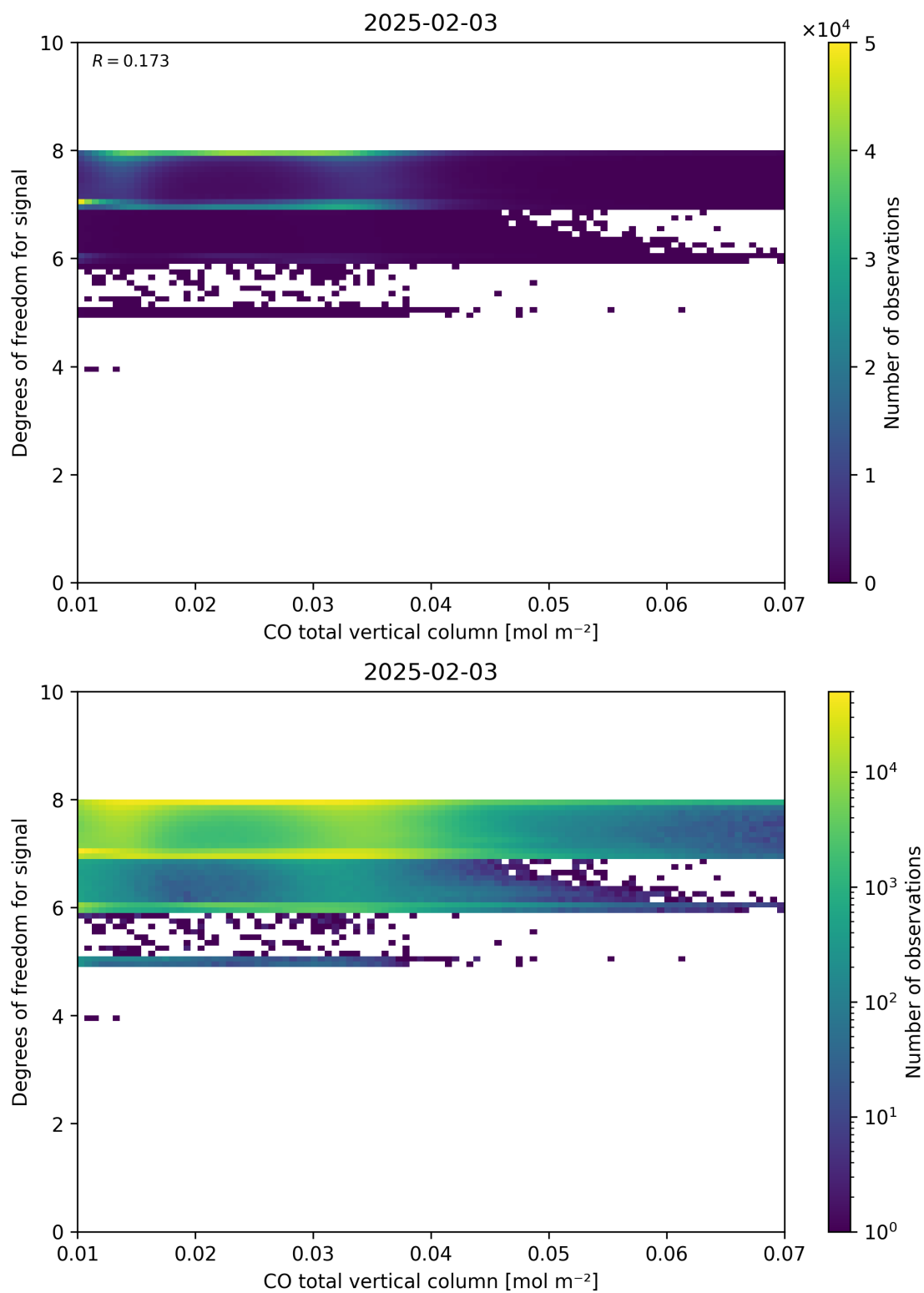
Figure 41: Scatter density plot of “CO total vertical column” against “Degrees of freedom for signal” for 2025-02-03 to 2025-02-04.
