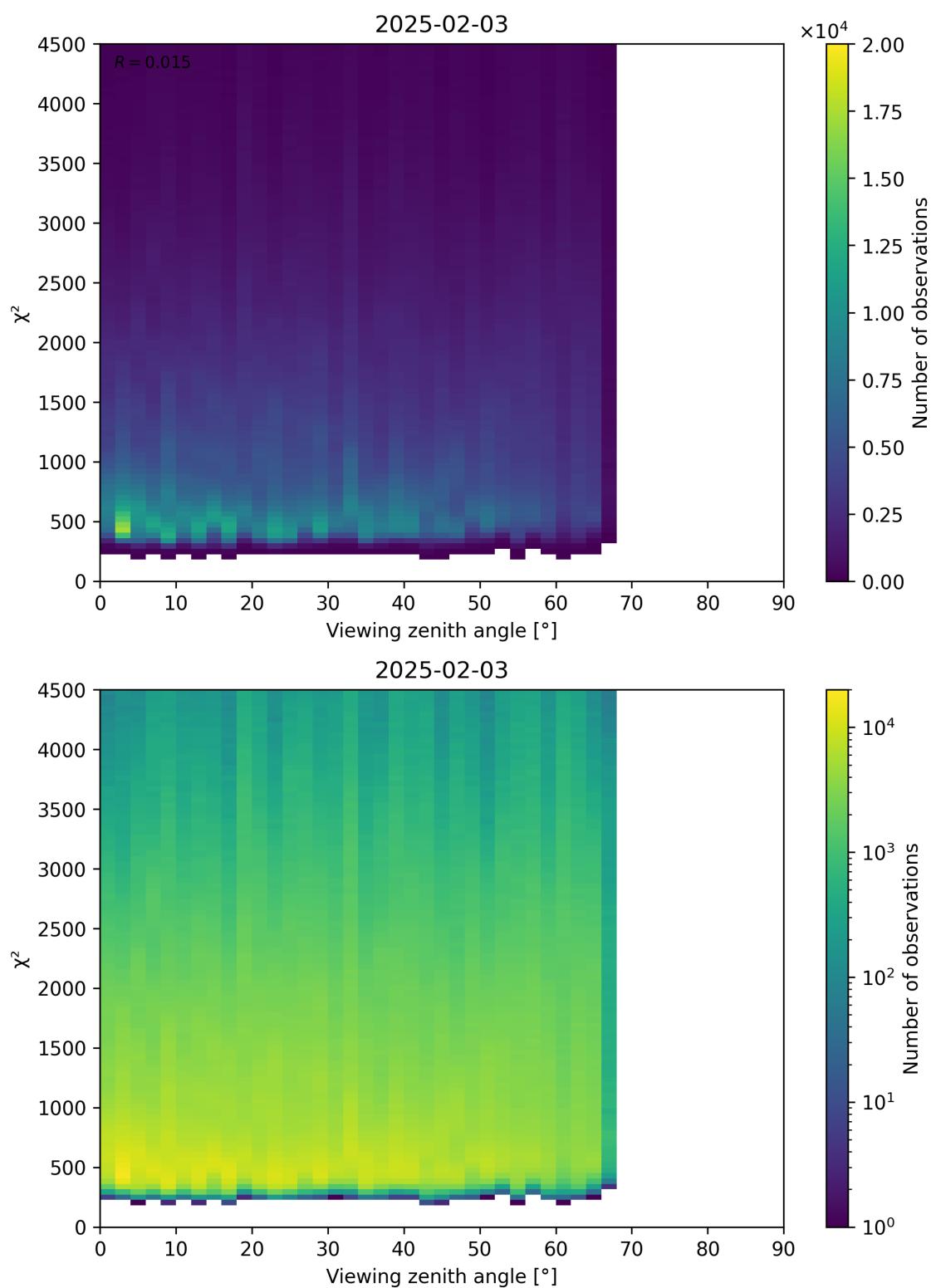
Figure 72: Scatter density plot of “Viewing zenith angle” against “ \chi^2 ” for 2025-02-03 to 2025-02-04.
