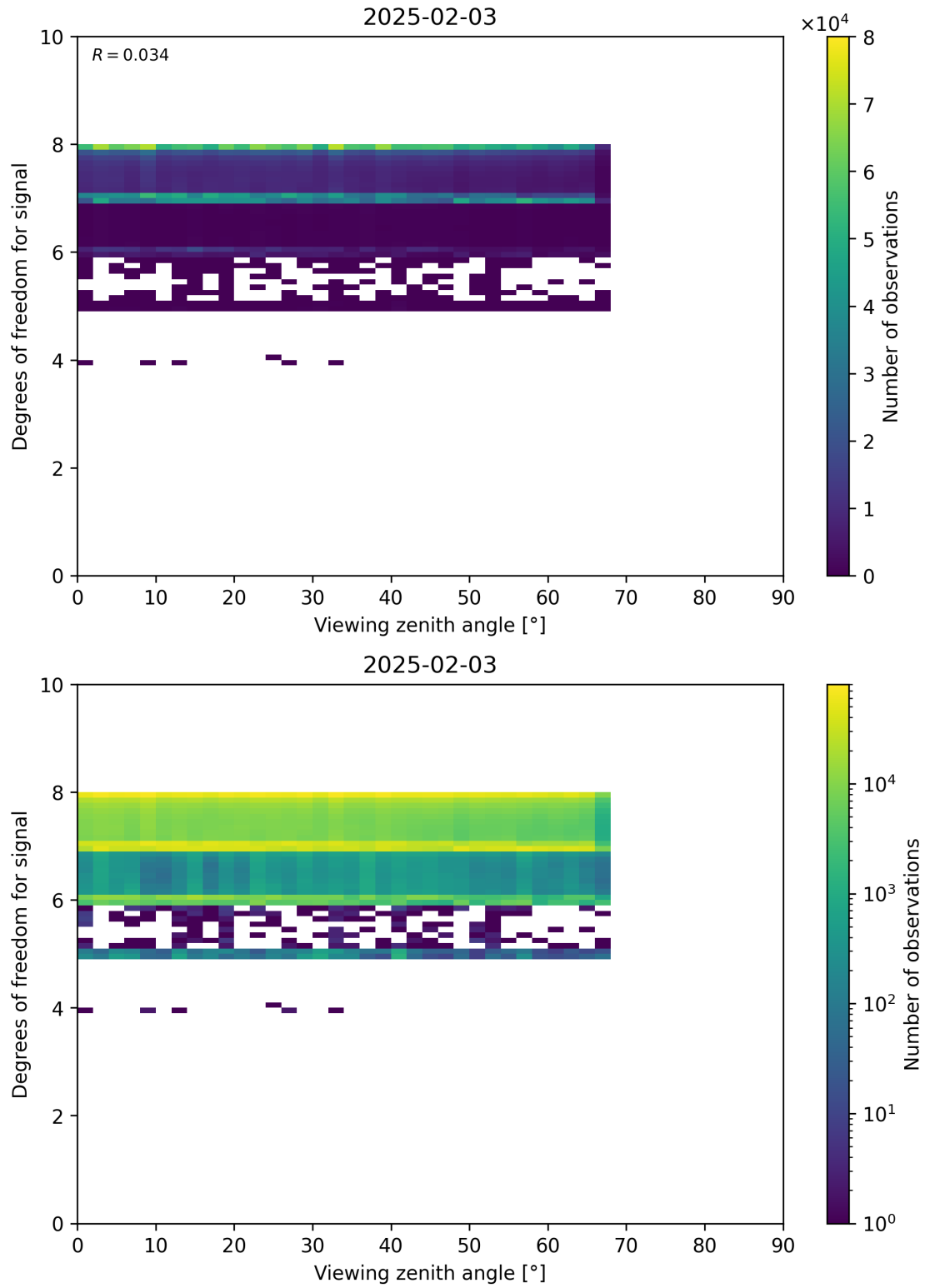
Figure 73: Scatter density plot of “Viewing zenith angle” against “Degrees of freedom for signal” for 2025-02-03 to 2025-02-04.
