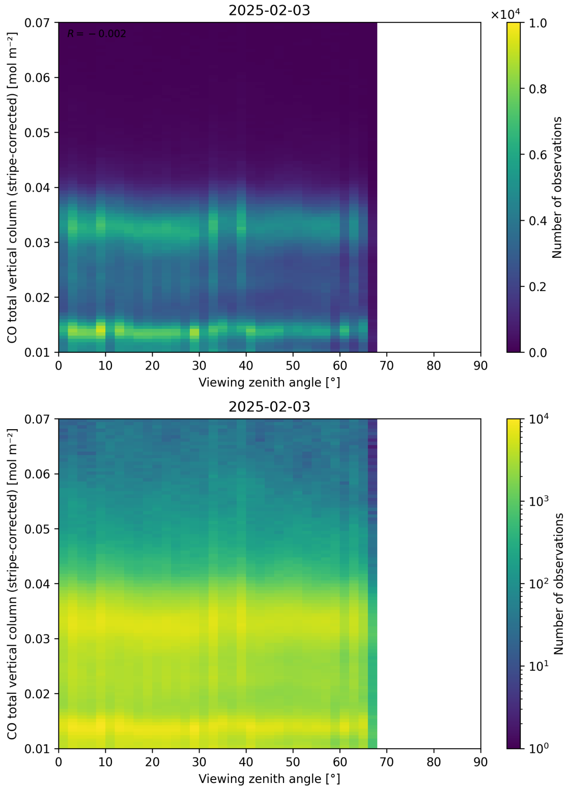
Figure 70: Scatter density plot of “Viewing zenith angle” against “CO total vertical column (stripe-corrected)” for 2025-02-03 to 2025-02-04.
