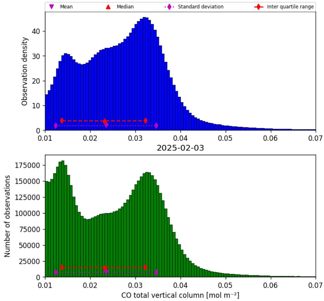
Figure 18: Histogram of “CO total vertical column” for 2025-02-03 to 2025-02-04
