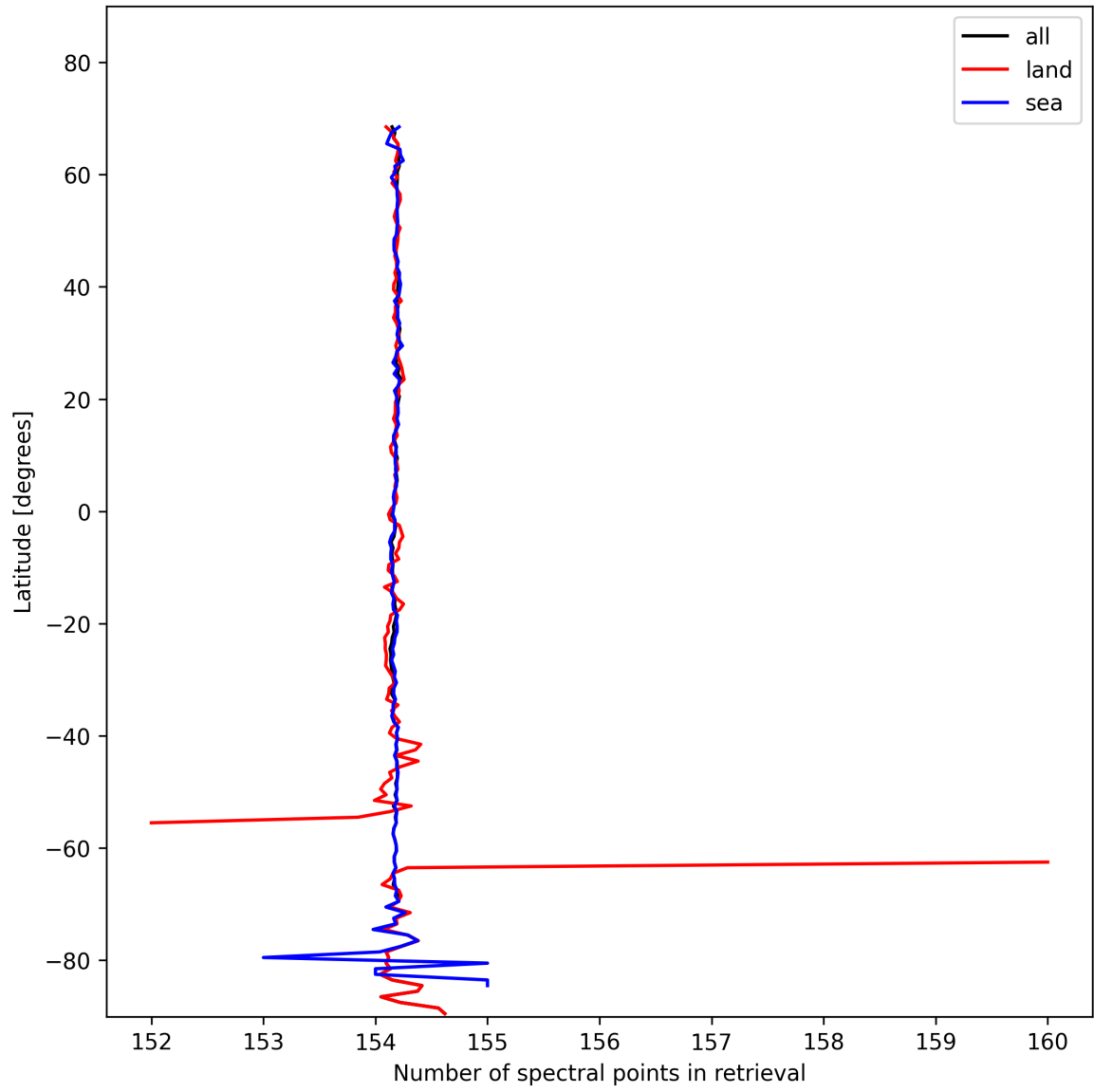
Figure 13: Zonal average of “Number of spectral points in retrieval” for 2025-02-03 to 2025-02-04.
