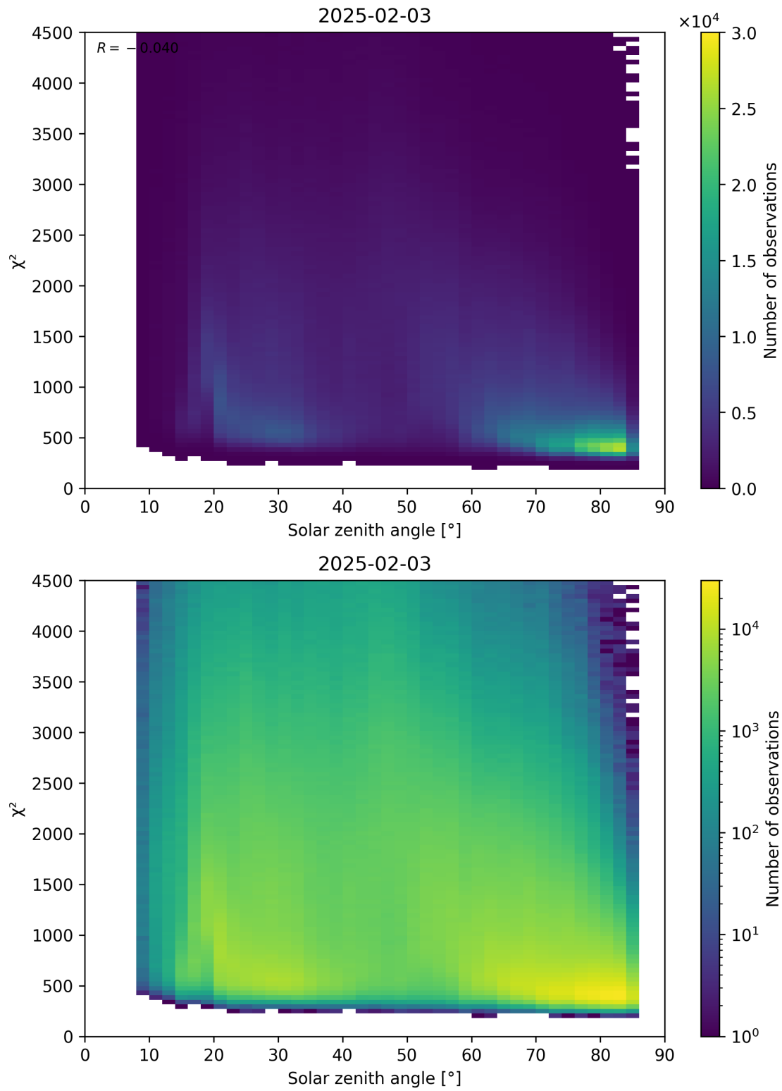
Figure 64: Scatter density plot of “Solar zenith angle” against “ \chi^2 ” for 2025-02-03 to 2025-02-04.
