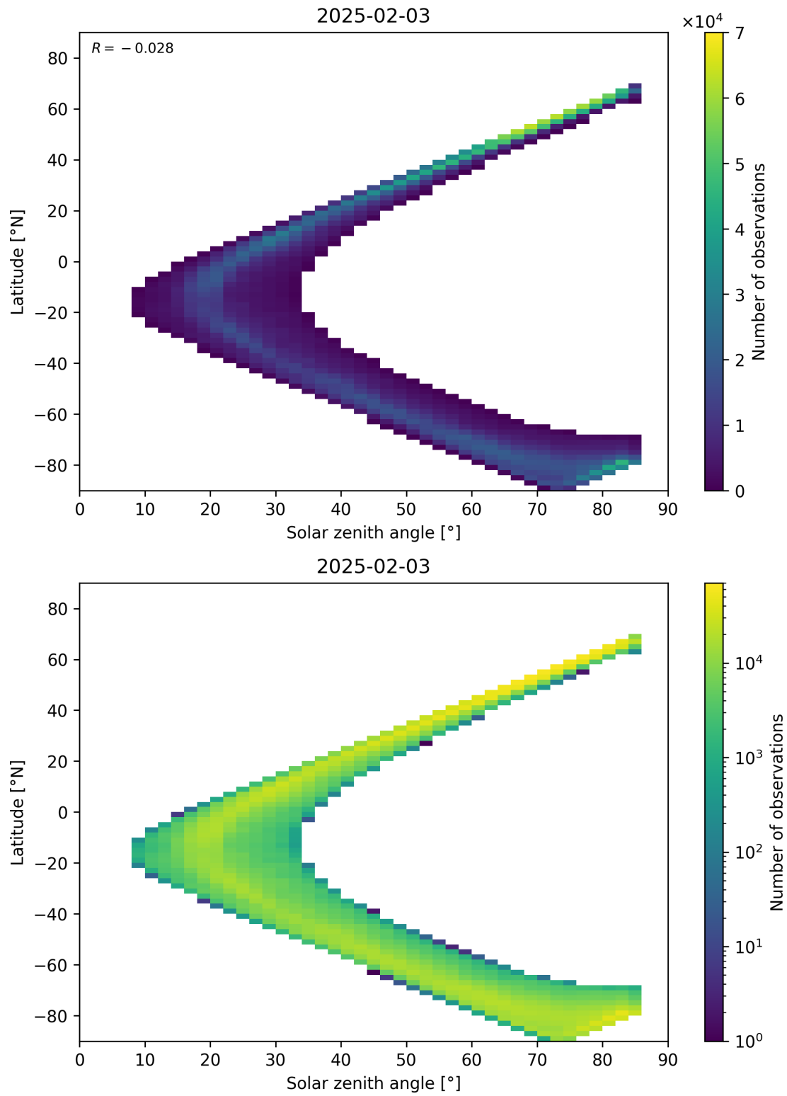
Figure 66: Scatter density plot of “Solar zenith angle” against “Latitude” for 2025-02-03 to 2025-02-04.
