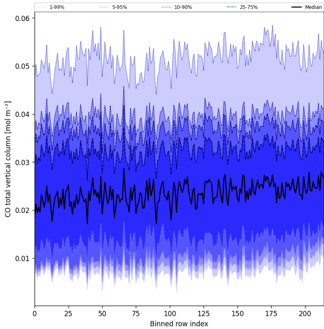
Figure 26: Along track statistics of “CO total vertical column” for 2025-02-03 to 2025-02-04
