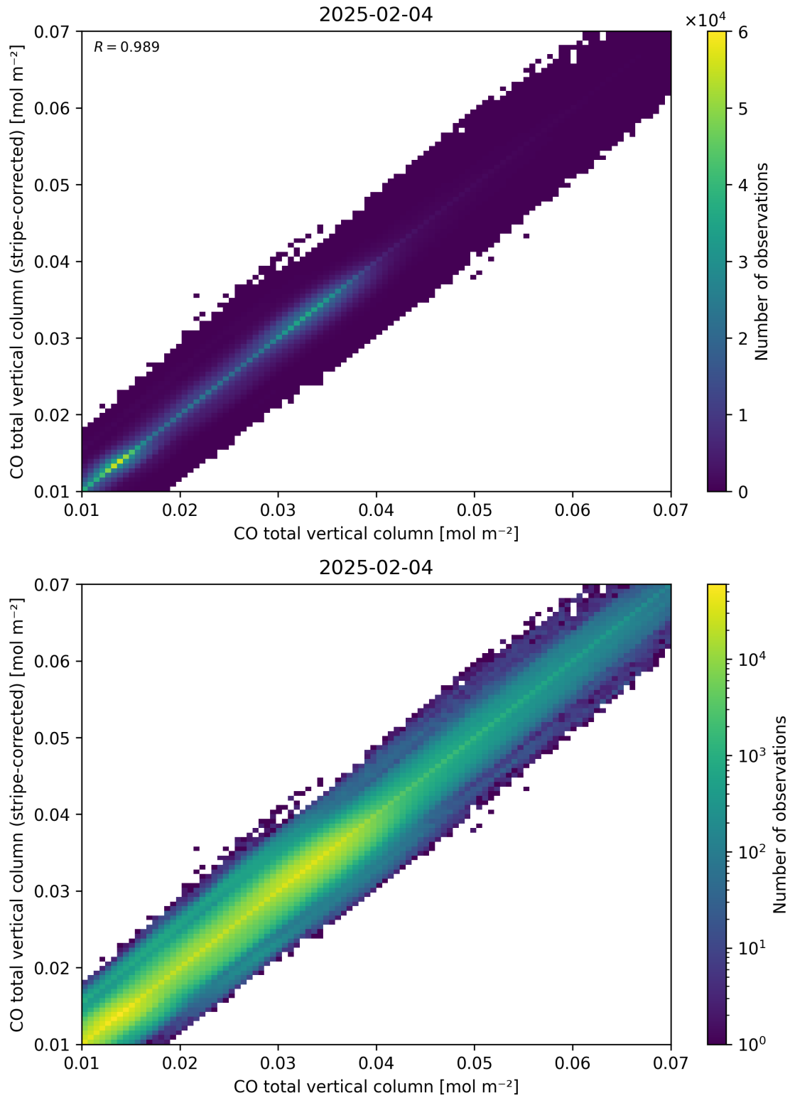
Figure 33: Scatter density plot of “CO total vertical column” against “CO total vertical column (stripe-corrected)” for 2025-02-03 to 2025-02-05.
