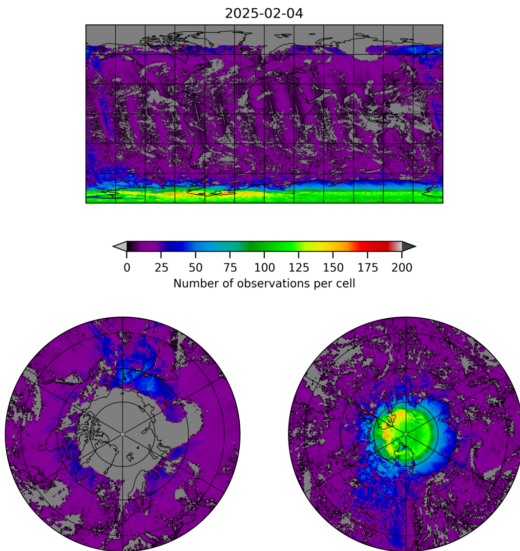
Figure 8: Map of the number of observations for 2025-02-03 to 2025-02-05
