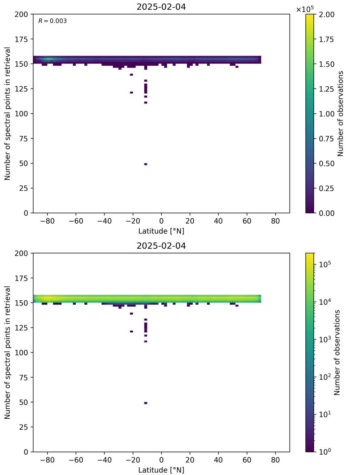
Figure 57: Scatter density plot of “Latitude” against “Number of spectral points in retrieval” for 2025-02-03 to 2025-02-05.
