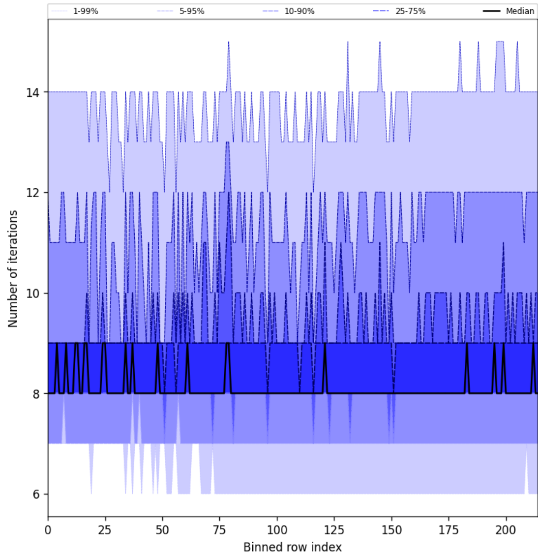
Figure 32: Along track statistics of “Number of iterations” for 2025-02-03 to 2025-02-05
