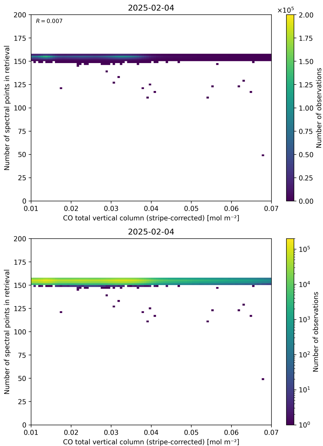
Figure 40: Scatter density plot of “CO total vertical column (stripe-corrected)” against “Number of spectral points in retrieval” for 2025-02-03 to 2025-02-05.
