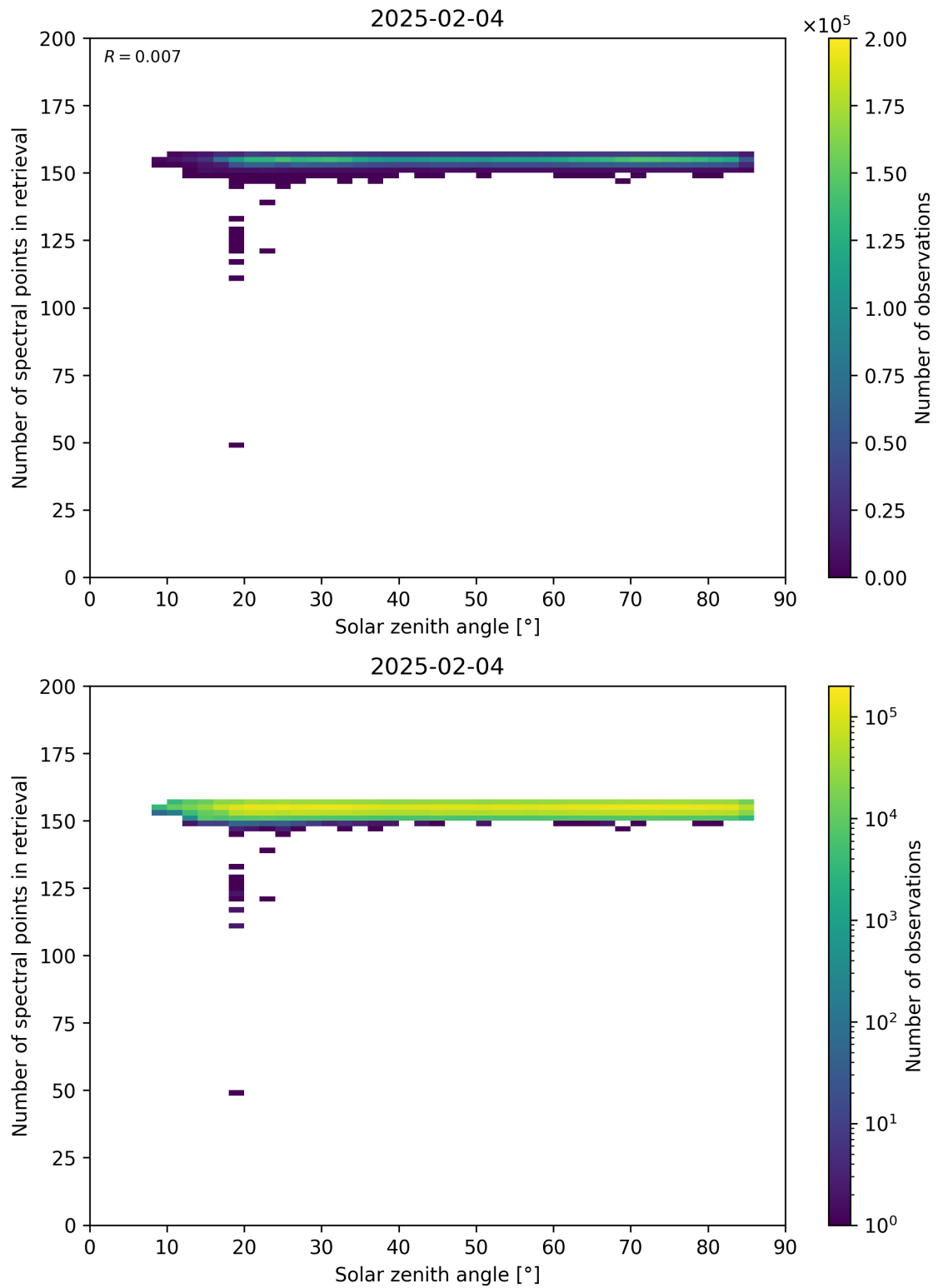
Figure 68: Scatter density plot of “Solar zenith angle” against “Number of spectral points in retrieval” for 2025-02-03 to 2025-02-05.
