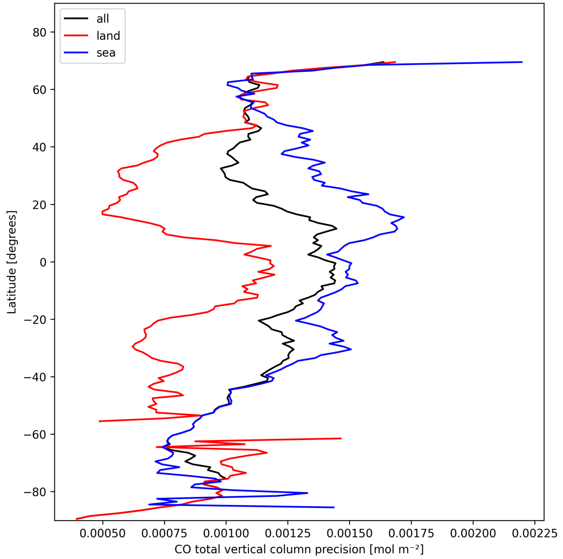
Figure 12: Zonal average of “CO total vertical column precision” for 2025-02-03 to 2025-02-05.
