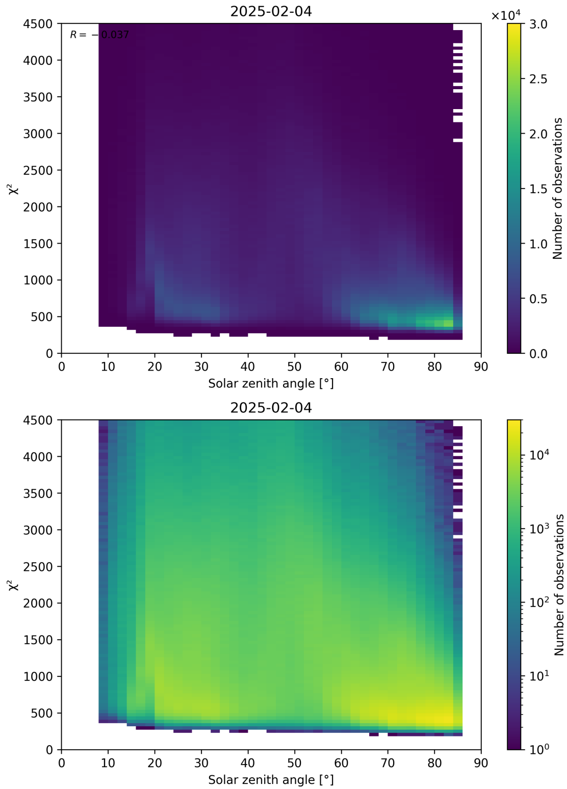
Figure 64: Scatter density plot of “Solar zenith angle” against “ \chi^2 ” for 2025-02-03 to 2025-02-05.
