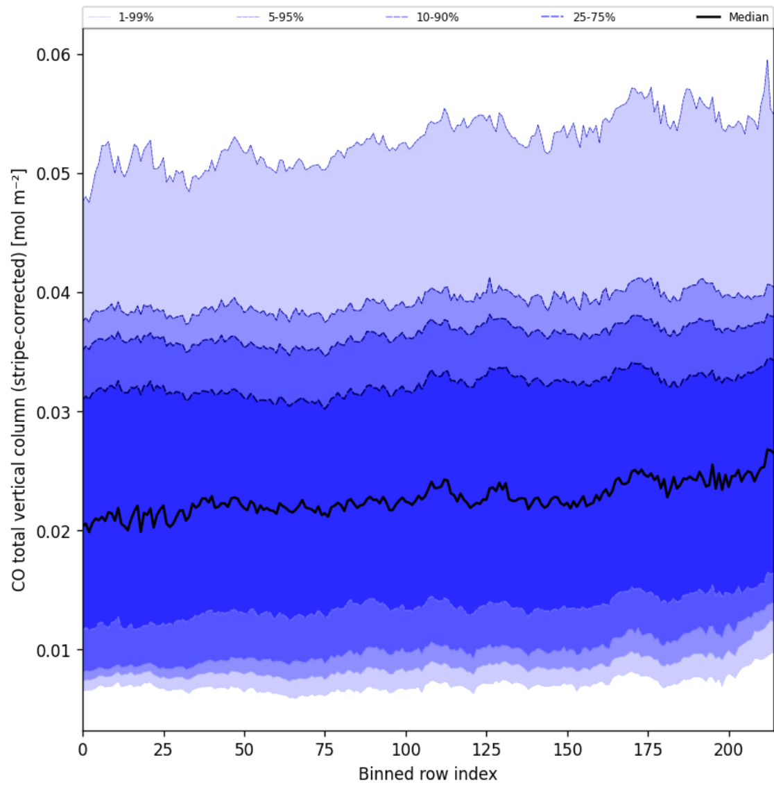
Figure 27: Along track statistics of “CO total vertical column (stripe-corrected)” for 2025-02-03 to 2025-02-05
