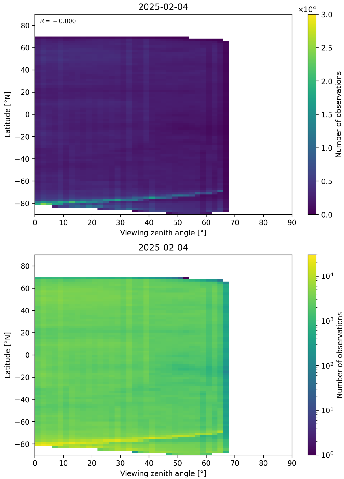
Figure 74: Scatter density plot of “Viewing zenith angle” against “Latitude” for 2025-02-03 to 2025-02-05.
