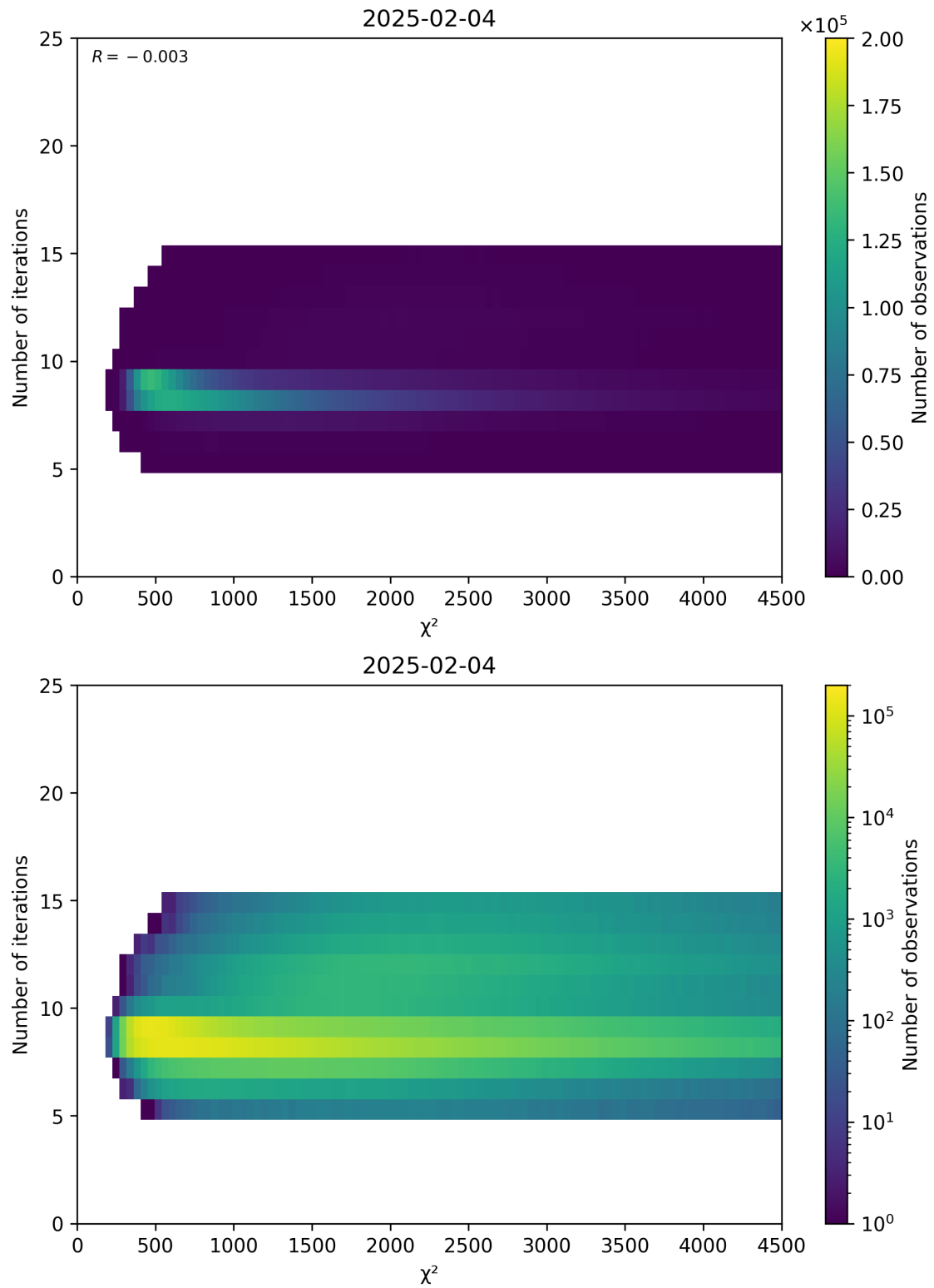
Figure 49: Scatter density plot of “ \chi^2 ” against “Number of iterations” for 2025-02-03 to 2025-02-05.
