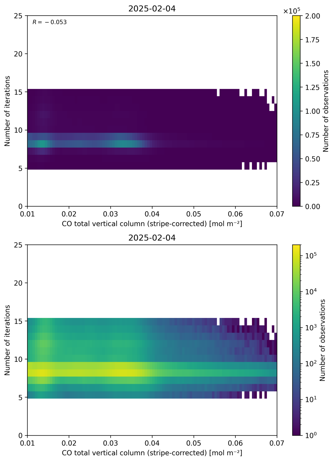
Figure 39: Scatter density plot of “CO total vertical column (stripe-corrected)” against “Number of iterations” for 2025-02-03 to 2025-02-05.
