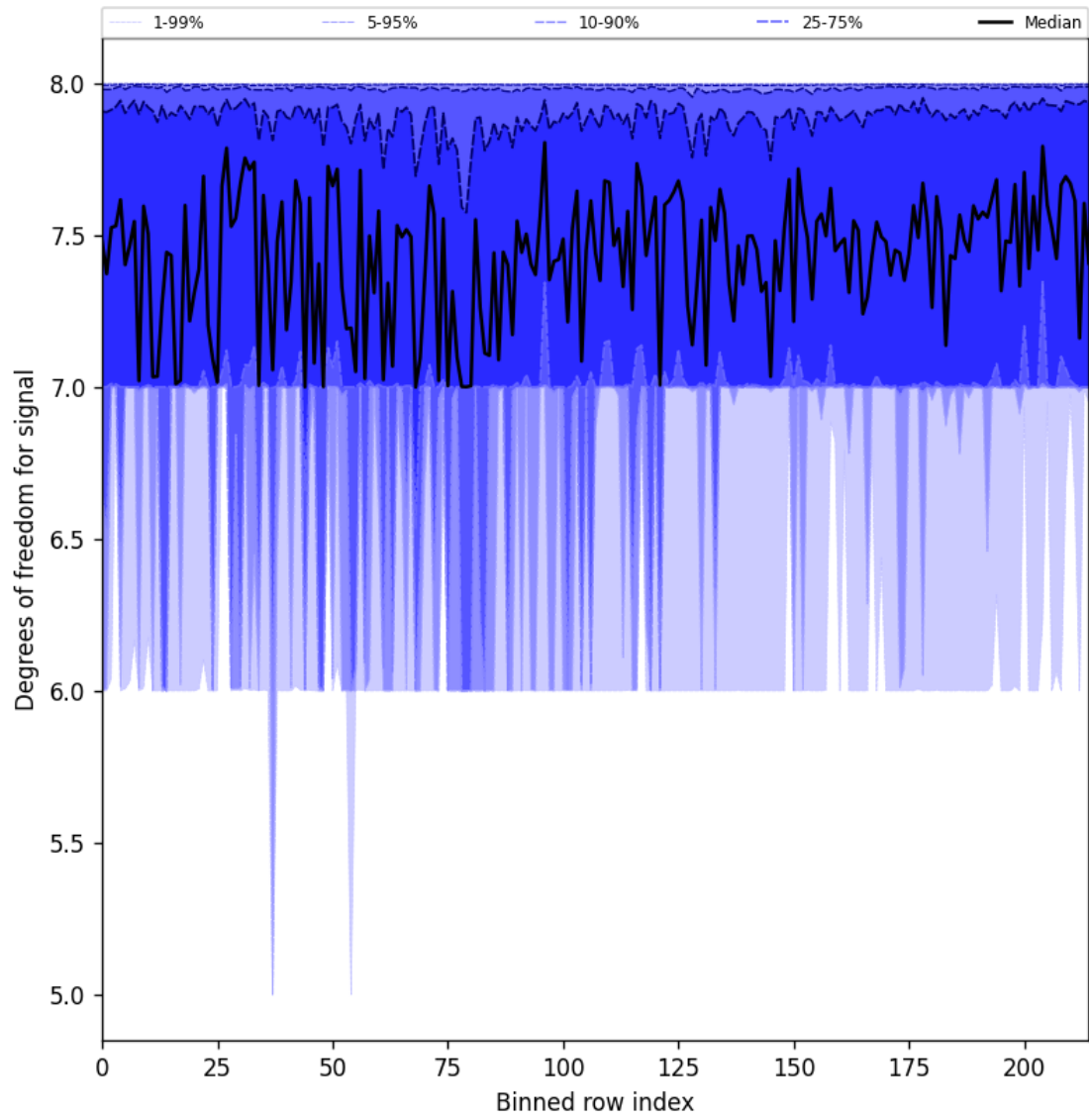
Figure 31: Along track statistics of “Degrees of freedom for signal” for 2025-02-03 to 2025-02-05
