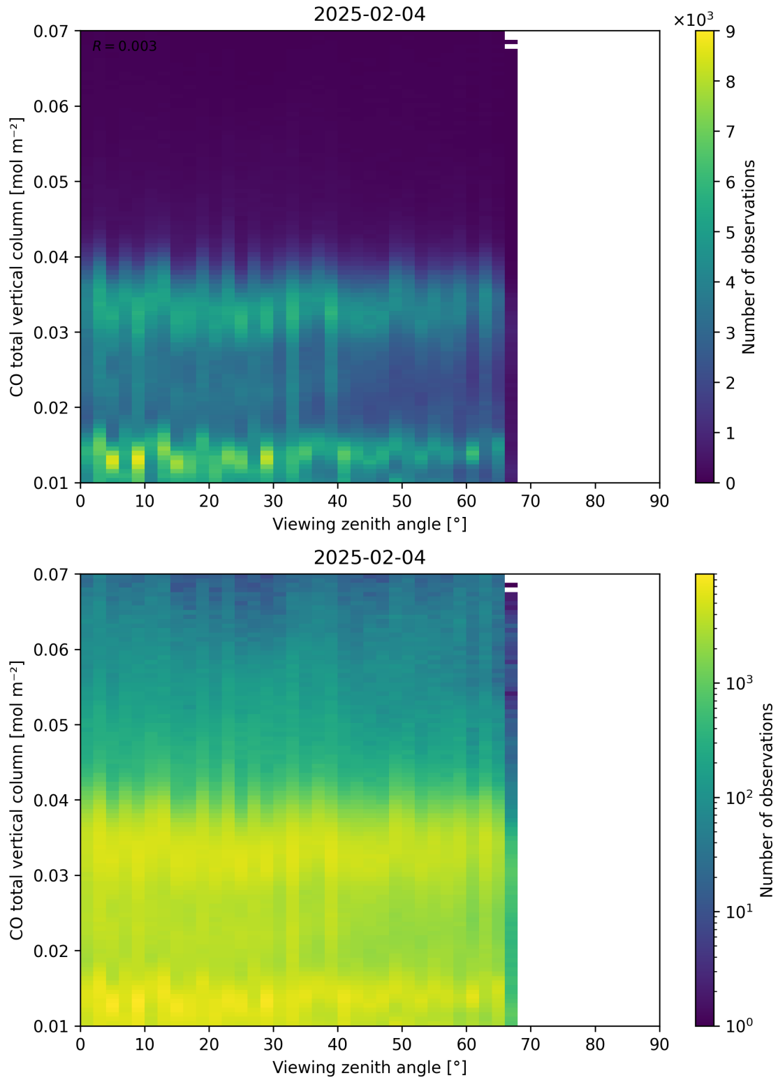
Figure 69: Scatter density plot of “Viewing zenith angle” against “CO total vertical column” for 2025-02-03 to 2025-02-05.
