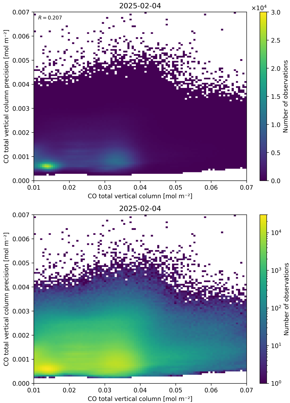
Figure 34: Scatter density plot of “CO total vertical column” against “CO total vertical column precision” for 2025-02-03 to 2025-02-05.
