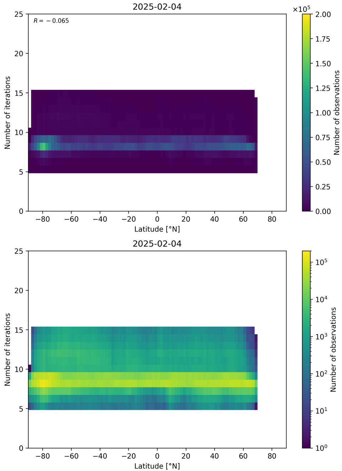
Figure 56: Scatter density plot of “Latitude” against “Number of iterations” for 2025-02-03 to 2025-02-05.
