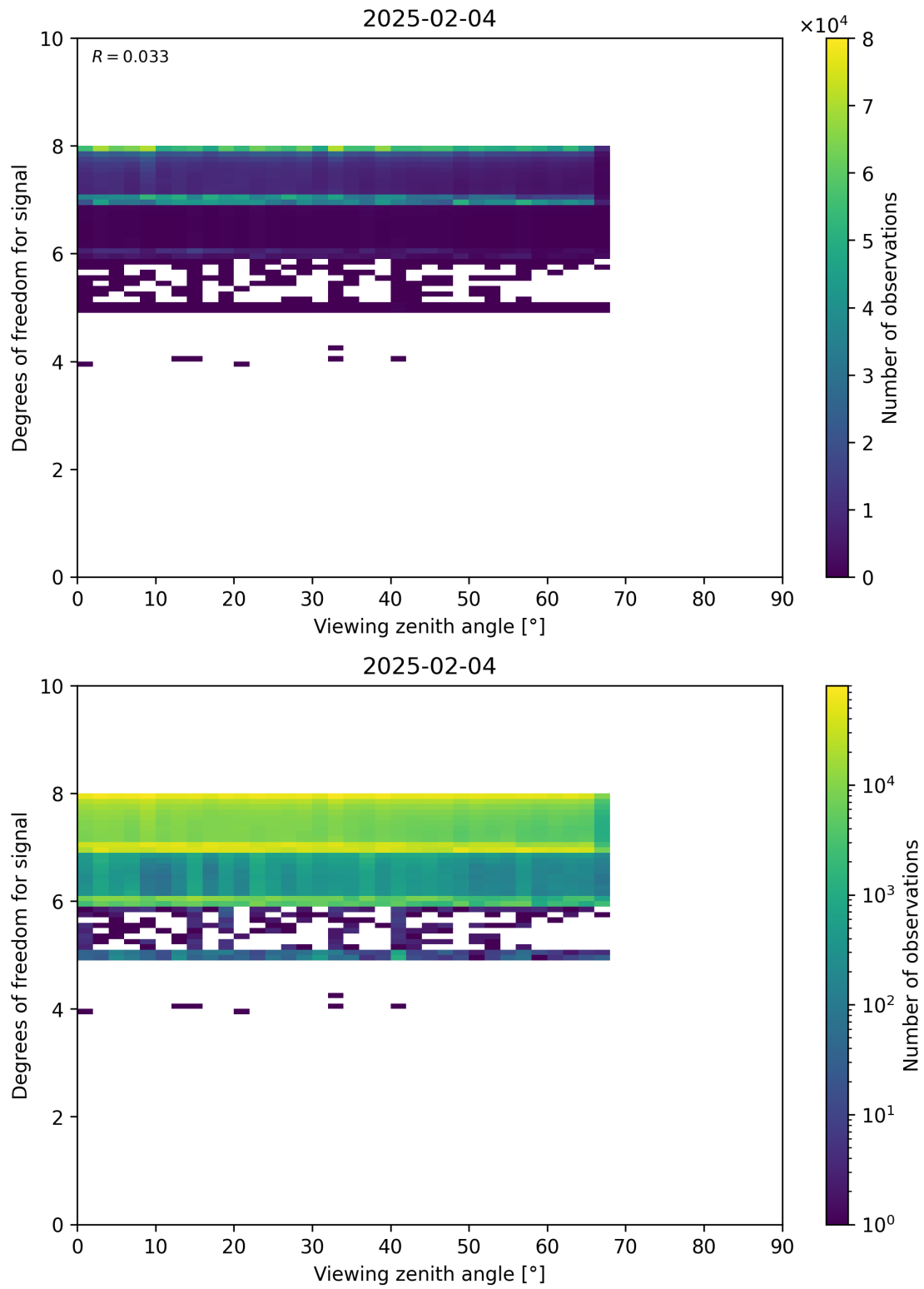
Figure 73: Scatter density plot of “Viewing zenith angle” against “Degrees of freedom for signal” for 2025-02-03 to 2025-02-05.
