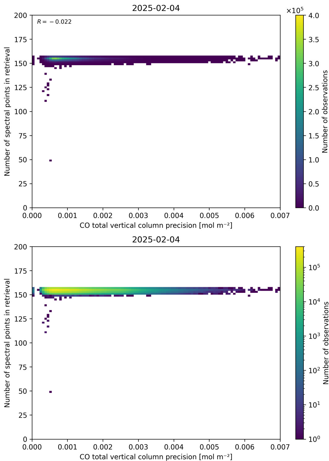
Figure 47: Scatter density plot of “CO total vertical column precision” against “Number of spectral points in retrieval” for 2025-02-03 to 2025-02-05.
