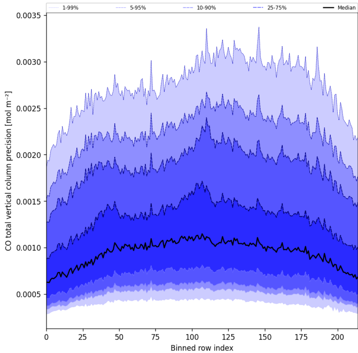
Figure 28: Along track statistics of “CO total vertical column precision” for 2025-02-03 to 2025-02-05
