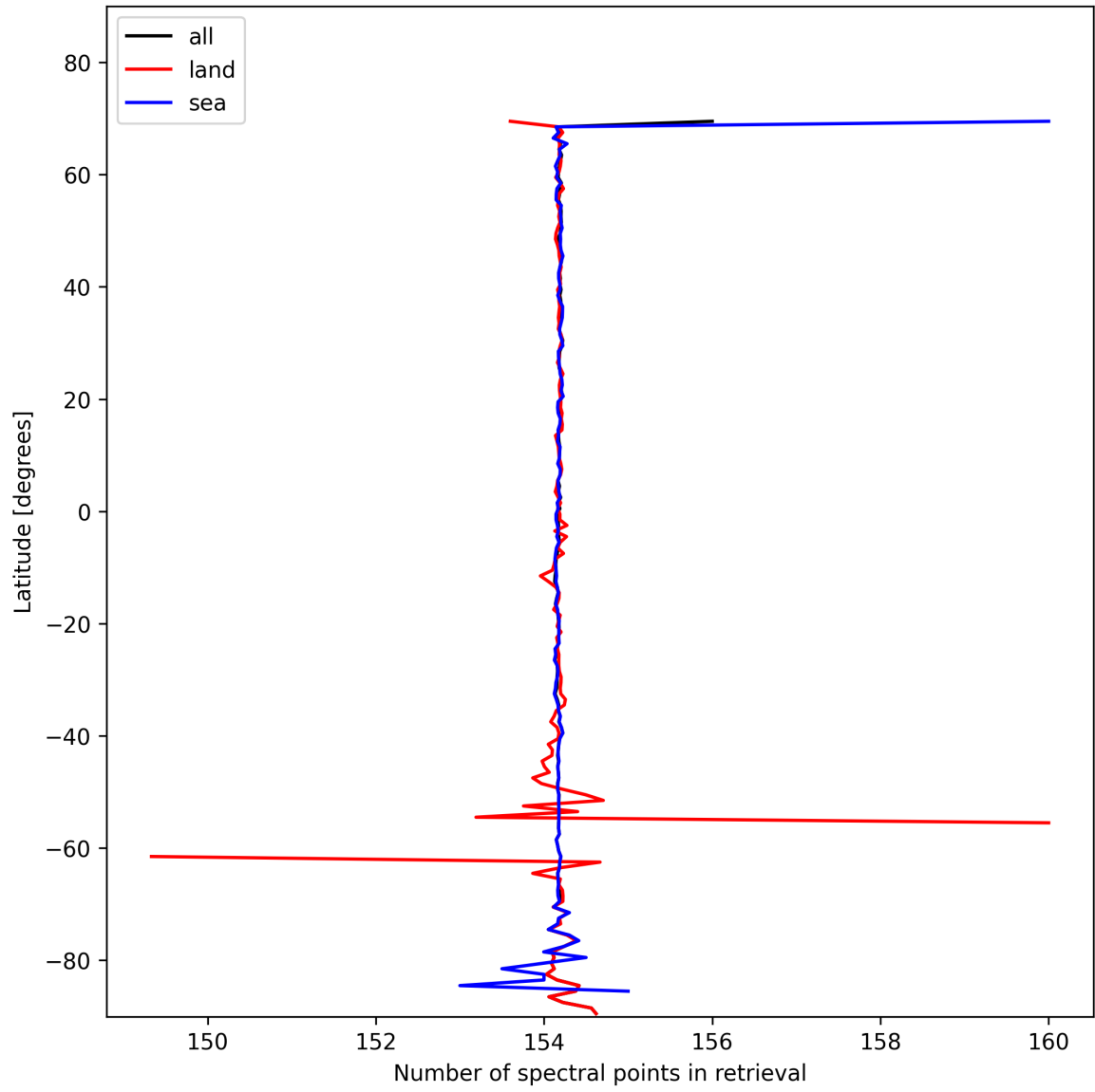
Figure 13: Zonal average of “Number of spectral points in retrieval” for 2025-02-03 to 2025-02-05.
