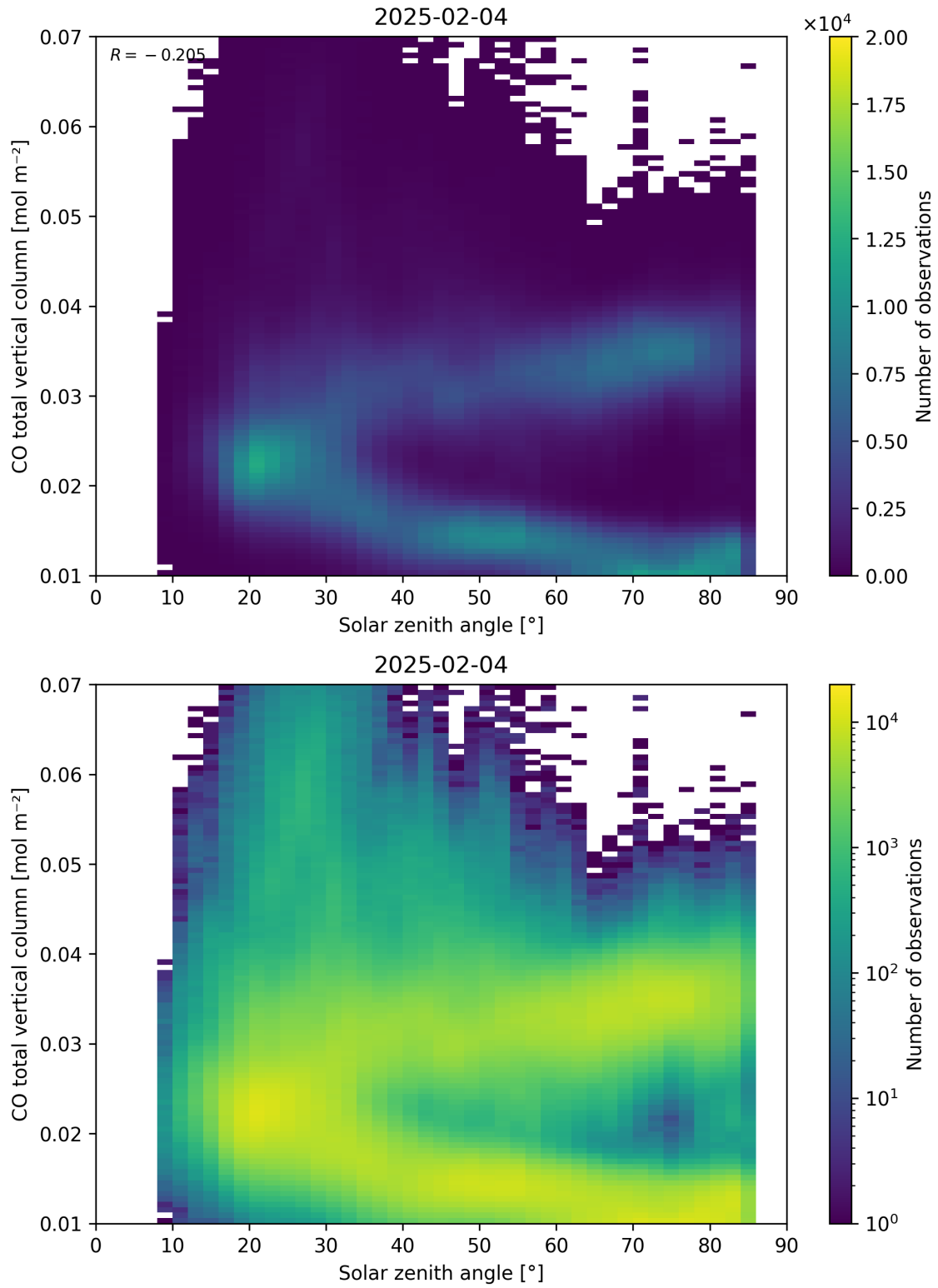
Figure 61: Scatter density plot of “Solar zenith angle” against “CO total vertical column” for 2025-02-03 to 2025-02-05.
