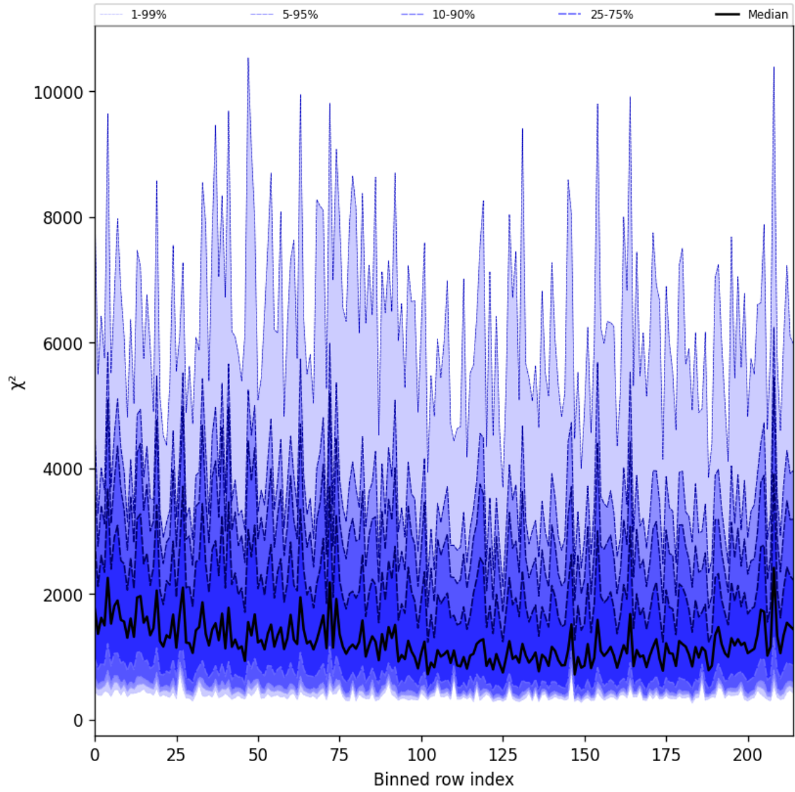
Figure 30: Along track statistics of “ \chi^2 ” for 2025-02-03 to 2025-02-05
