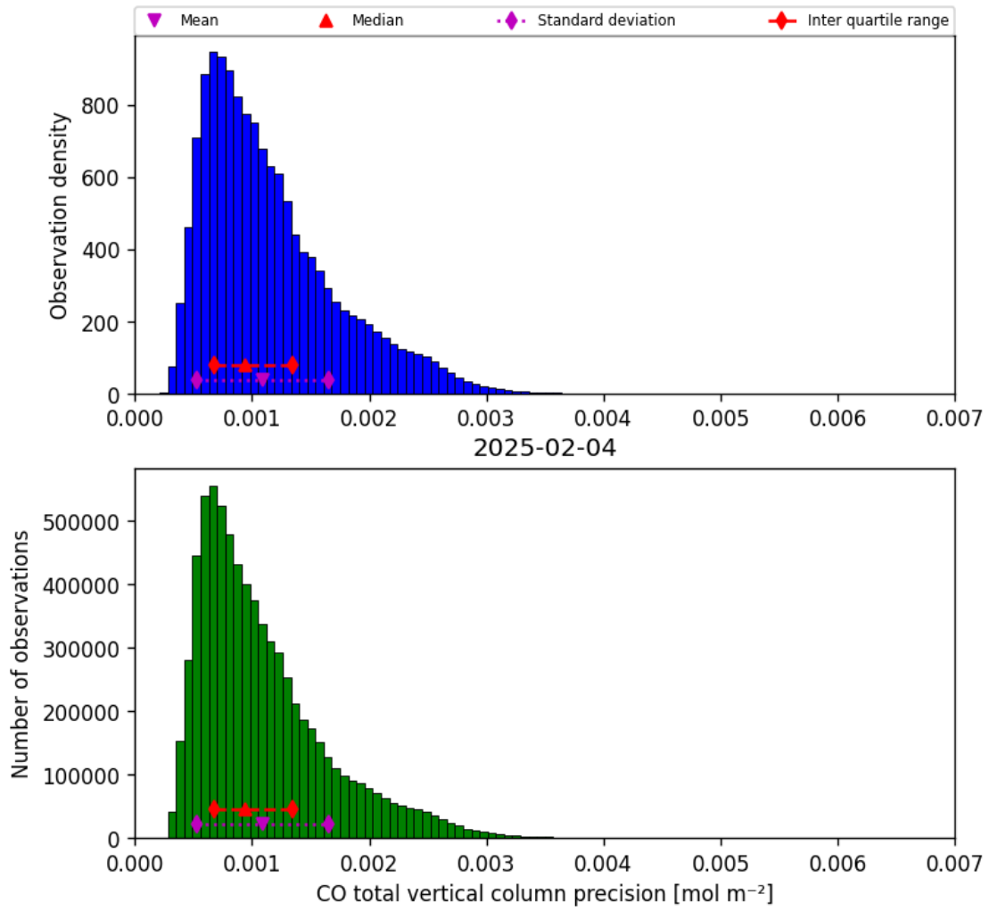
Figure 20: Histogram of “CO total vertical column precision” for 2025-02-03 to 2025-02-05
