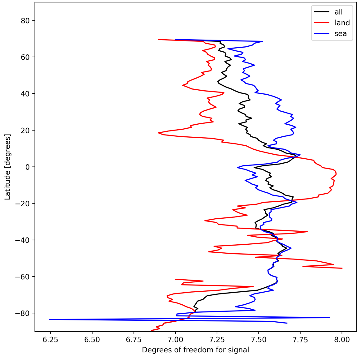
Figure 15: Zonal average of “Degrees of freedom for signal” for 2025-02-03 to 2025-02-05.
