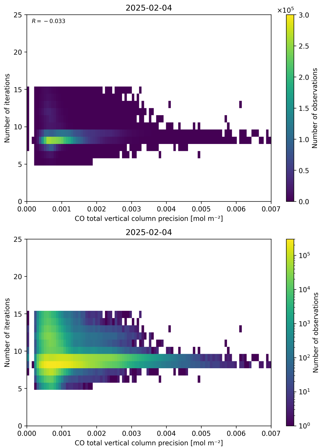
Figure 46: Scatter density plot of “CO total vertical column precision” against “Number of iterations” for 2025-02-03 to 2025-02-05.
