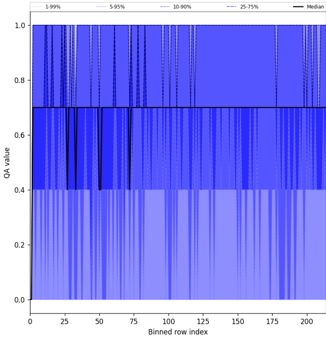
Figure 25: Along track statistics of “QA value” for 2025-02-03 to 2025-02-05
