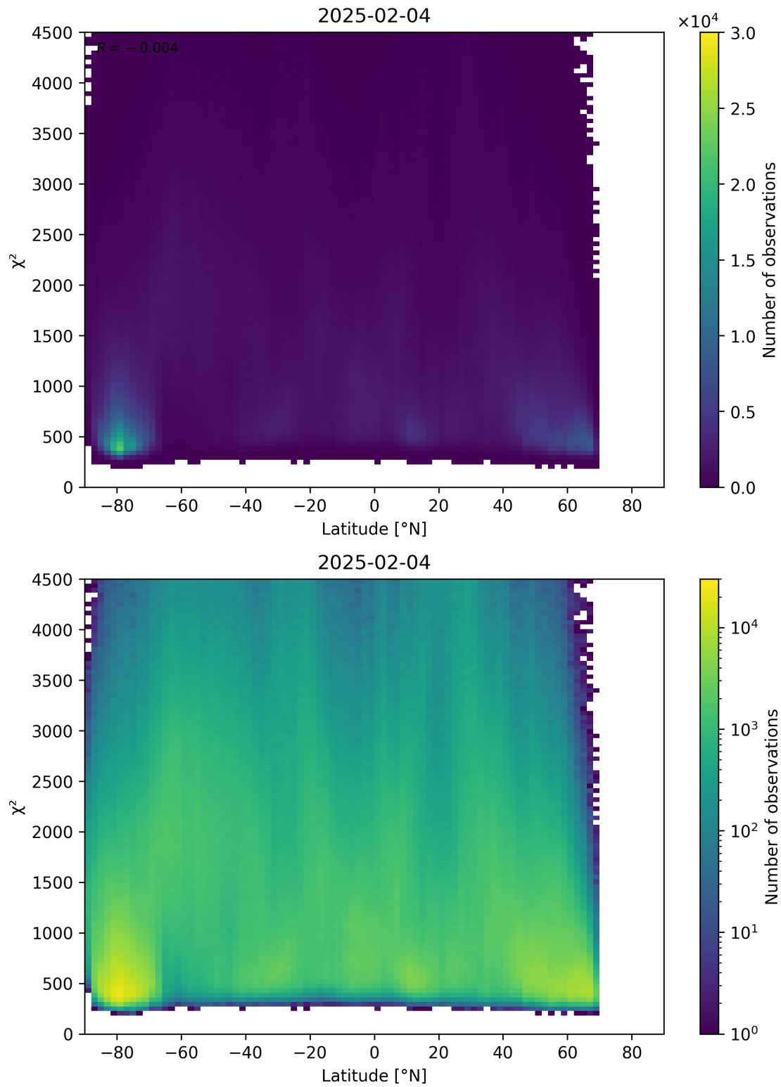
Figure 54: Scatter density plot of “Latitude” against “ \chi^2 ” for 2025-02-03 to 2025-02-05.
