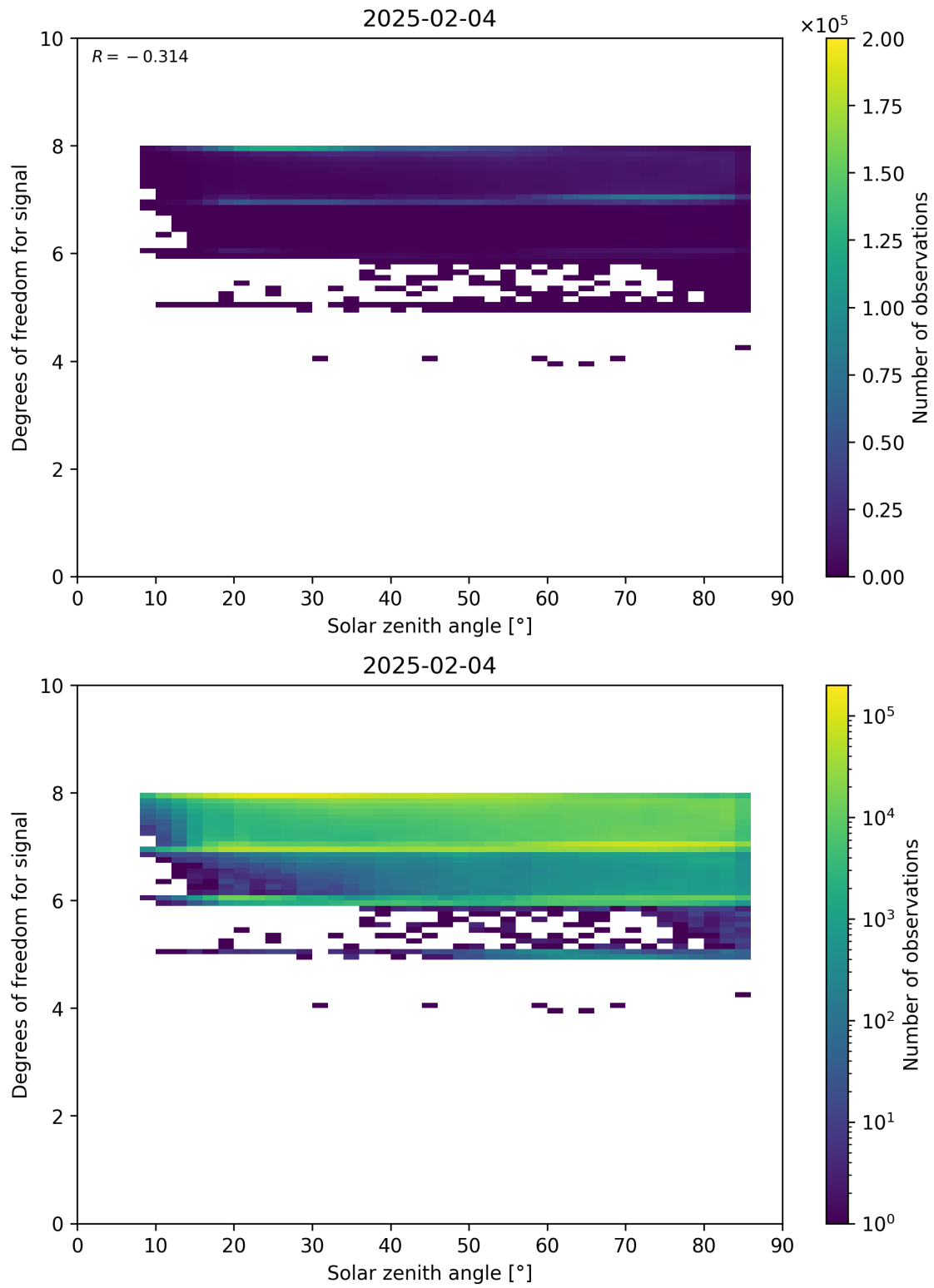
Figure 65: Scatter density plot of “Solar zenith angle” against “Degrees of freedom for signal” for 2025-02-03 to 2025-02-05.
