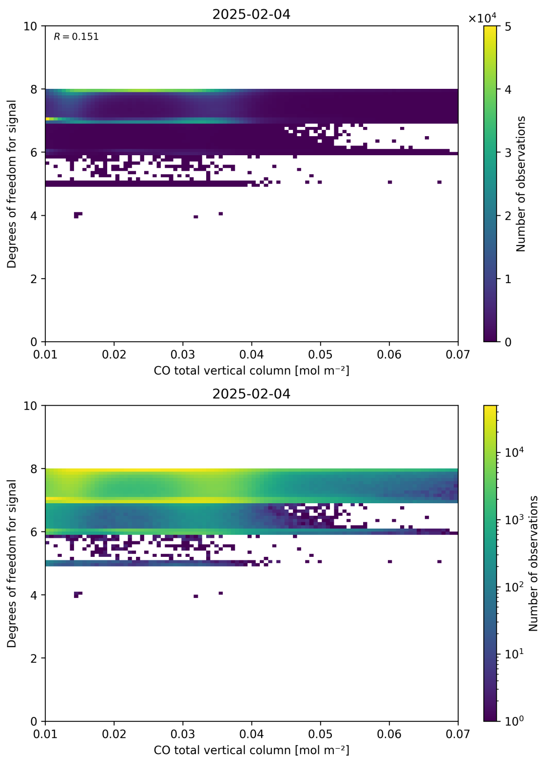
Figure 41: Scatter density plot of “CO total vertical column” against “Degrees of freedom for signal” for 2025-02-03 to 2025-02-05.
