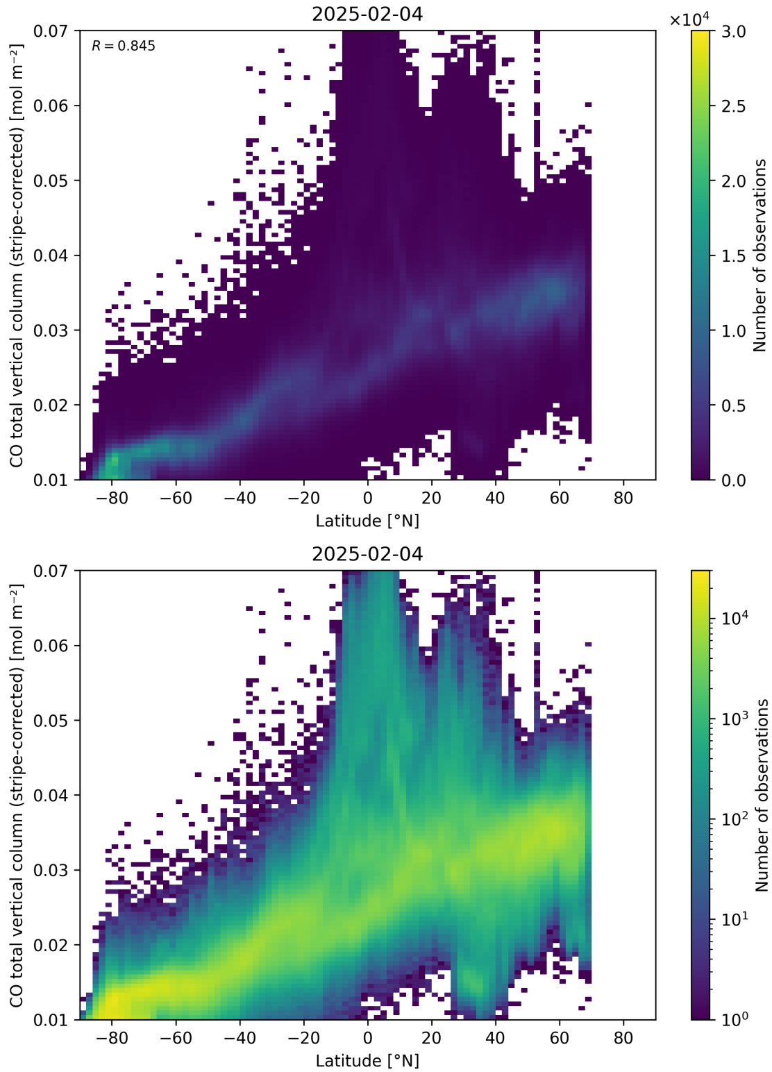
Figure 52: Scatter density plot of “Latitude” against “CO total vertical column (stripe-corrected)” for 2025-02-03 to 2025-02-05.
