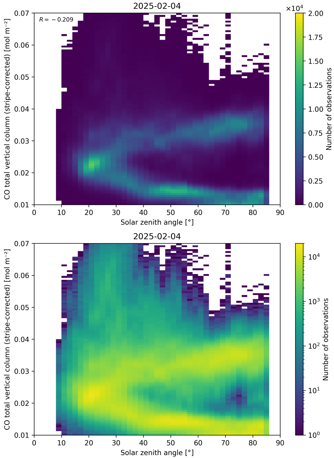
Figure 62: Scatter density plot of “Solar zenith angle” against “CO total vertical column (stripe-corrected)” for 2025-02-03 to 2025-02-05.
