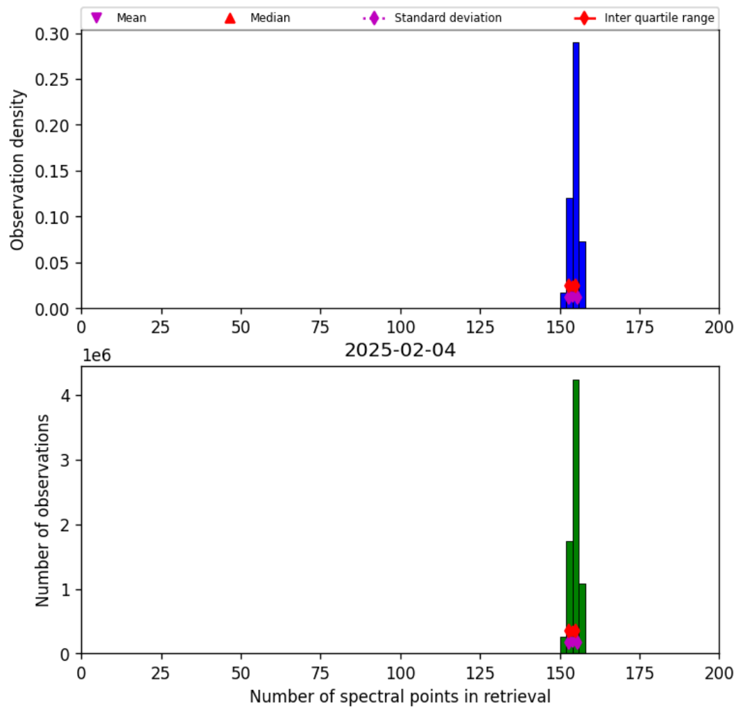
Figure 21: Histogram of “Number of spectral points in retrieval” for 2025-02-03 to 2025-02-05
