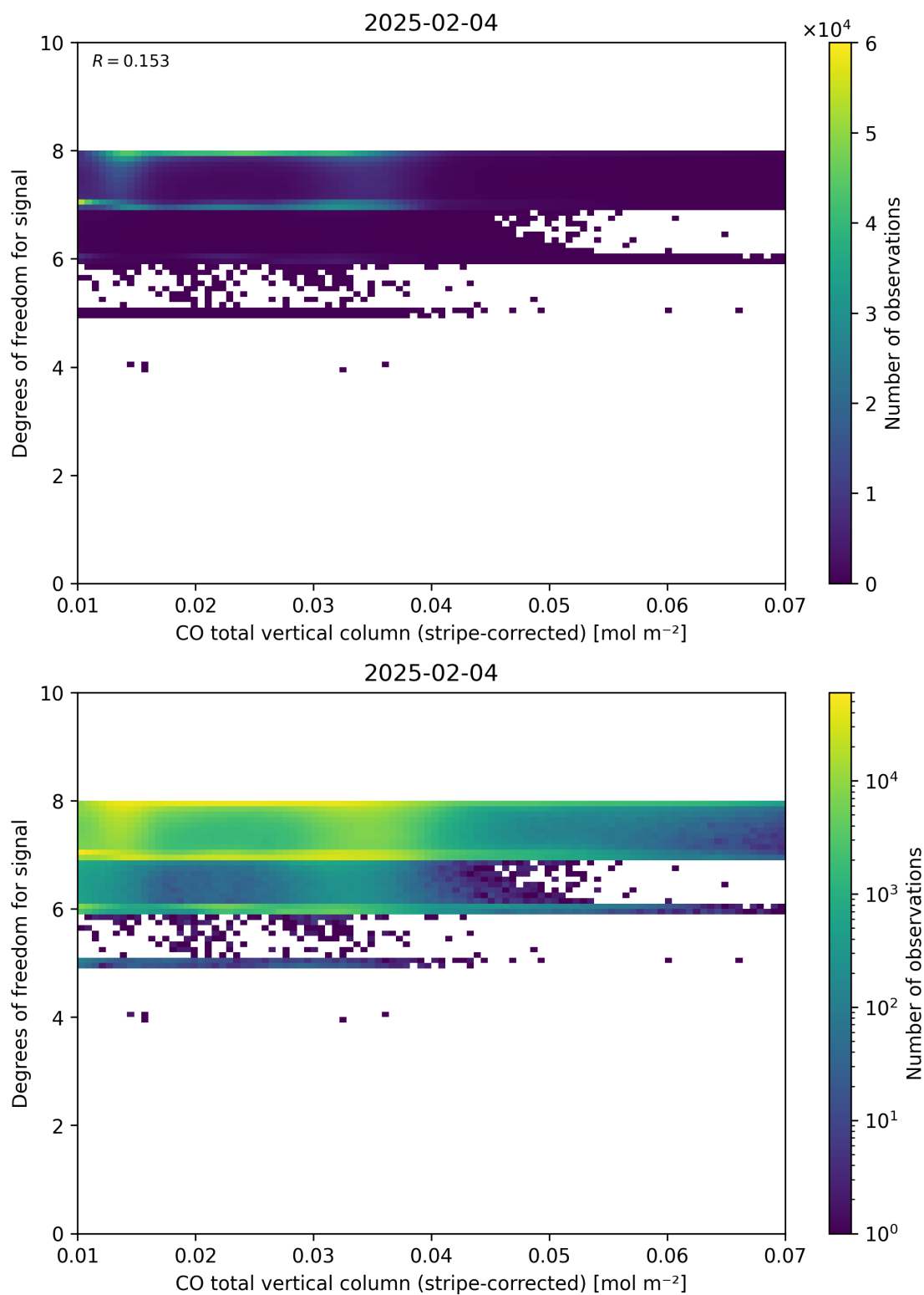
Figure 38: Scatter density plot of “CO total vertical column (stripe-corrected)” against “Degrees of freedom for signal” for 2025-02-03 to 2025-02-05.
