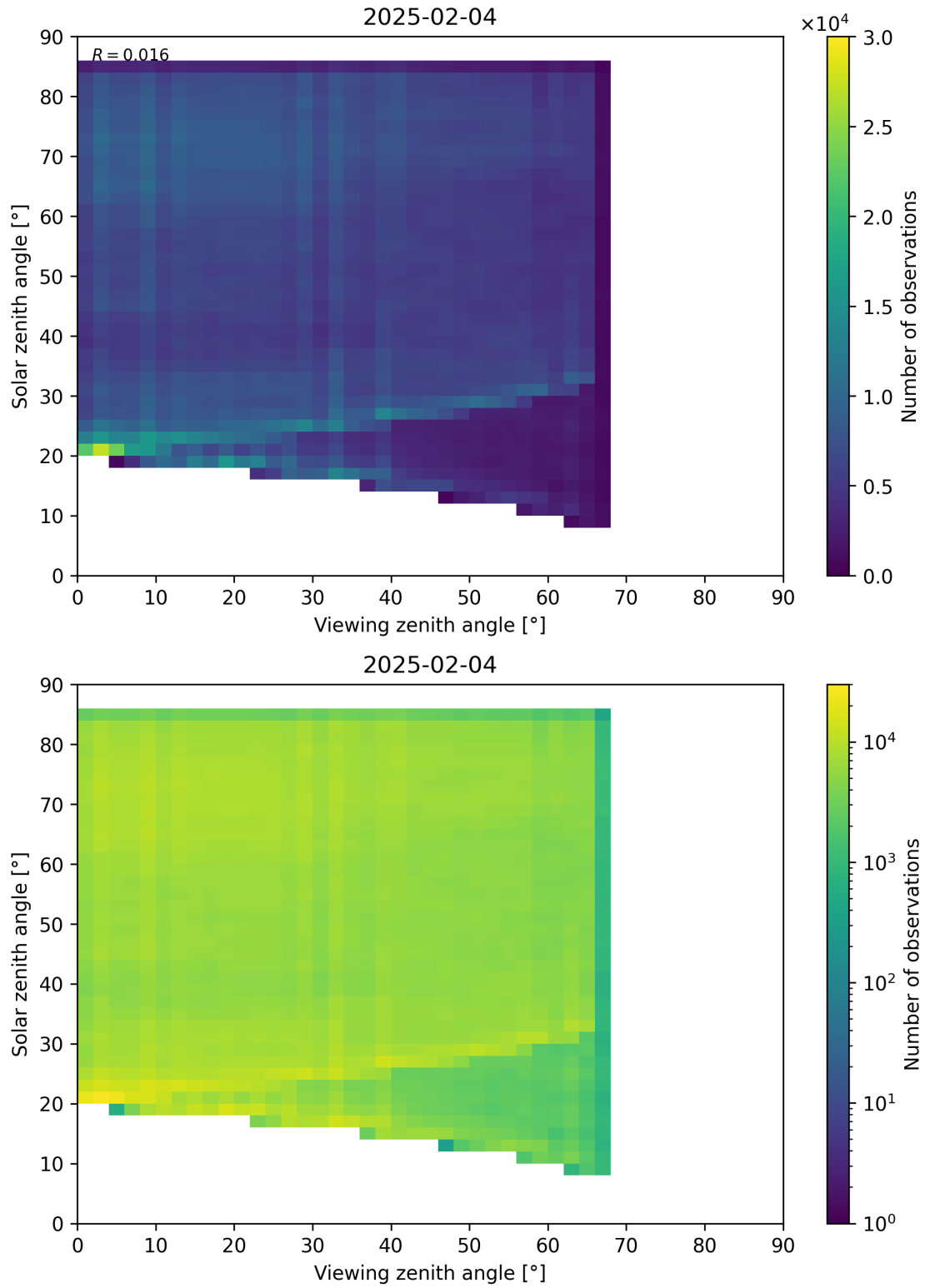
Figure 77: Scatter density plot of “Viewing zenith angle” against “Solar zenith angle” for 2025-02-03 to 2025-02-05.
