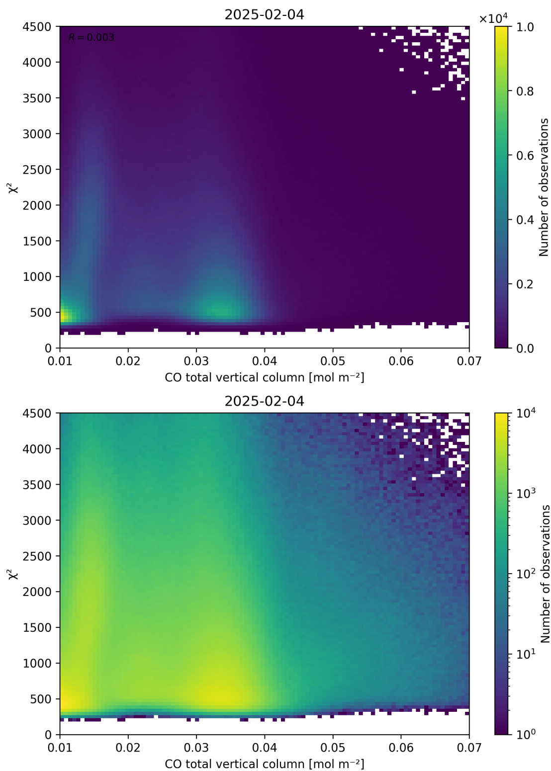
Figure 35: Scatter density plot of “CO total vertical column” against “ \chi^2 ” for 2025-02-03 to 2025-02-05.
