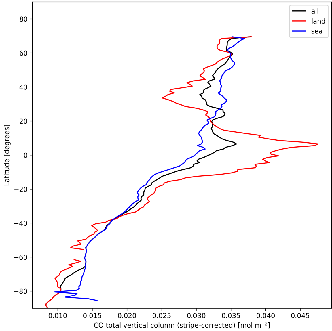
Figure 11: Zonal average of “CO total vertical column (stripe-corrected)” for 2025-02-03 to 2025-02-05.
