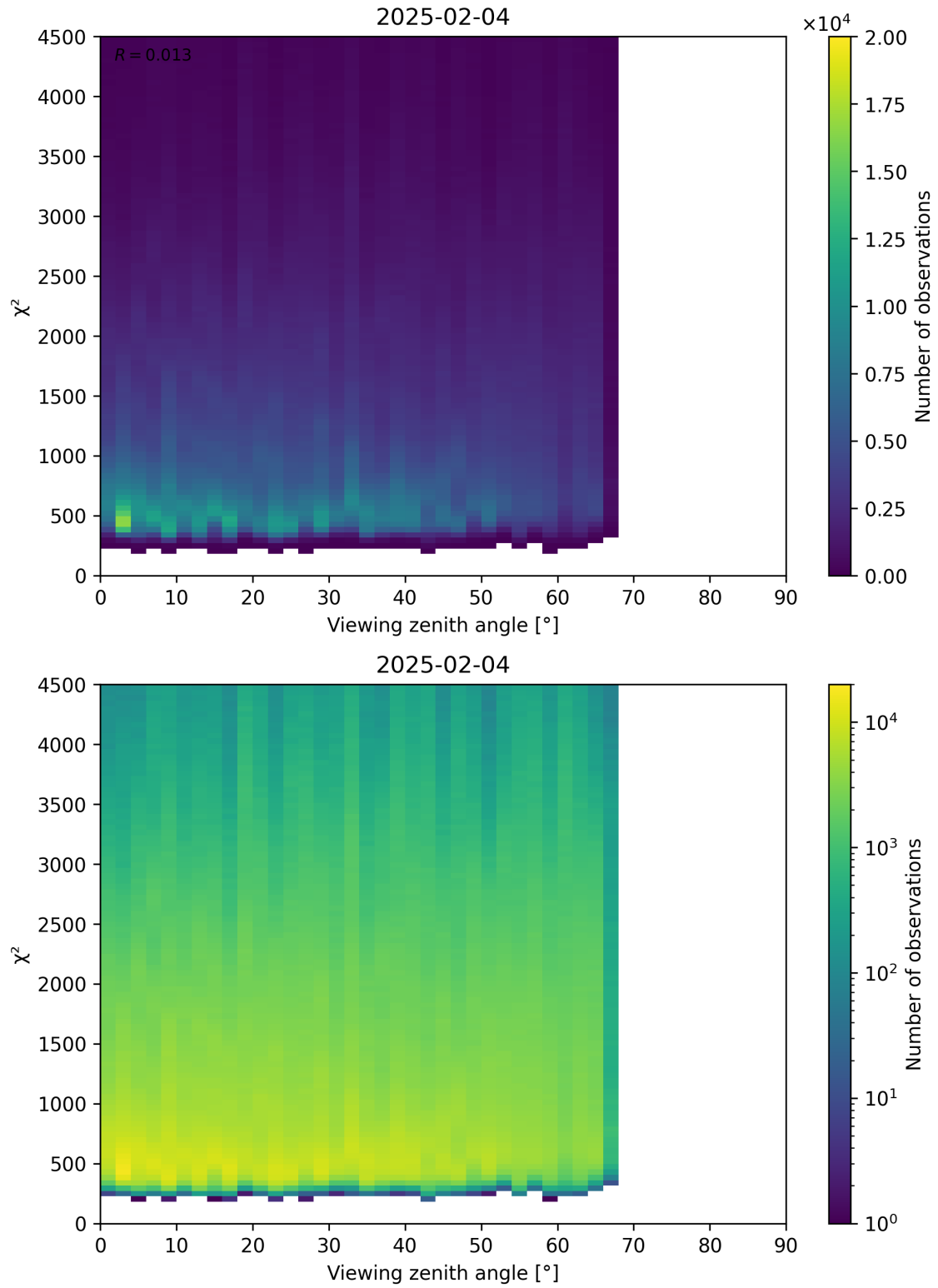
Figure 72: Scatter density plot of “Viewing zenith angle” against “ \chi^2 ” for 2025-02-03 to 2025-02-05.
