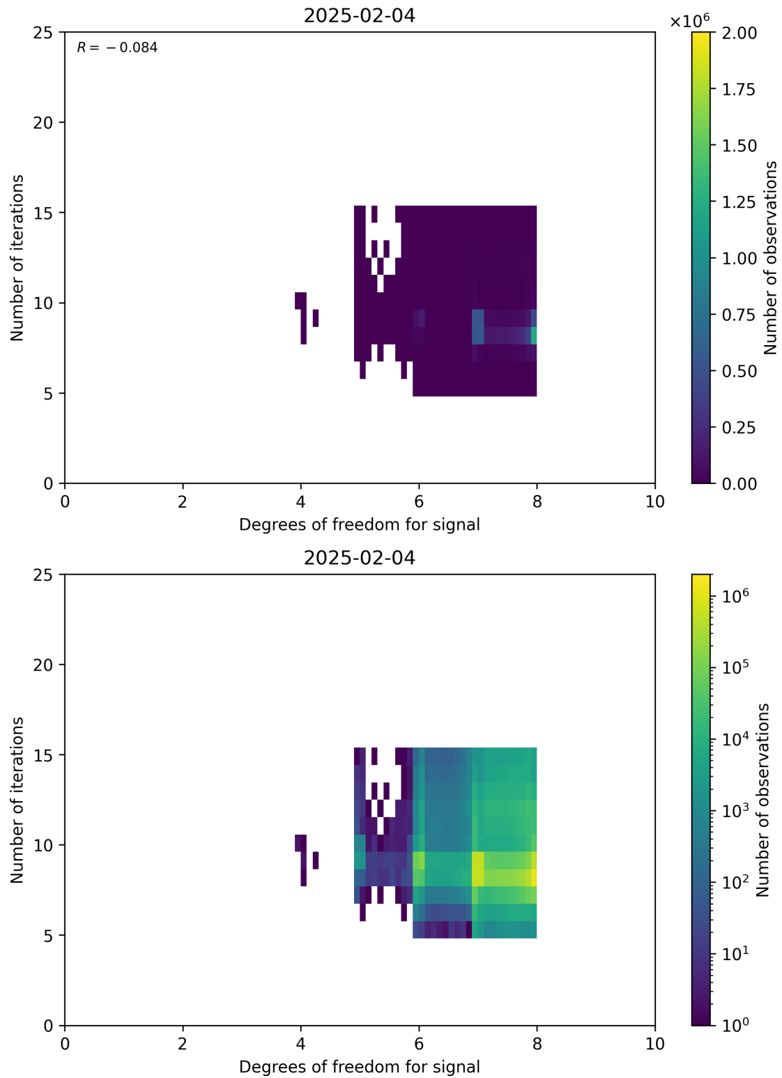
Figure 50: Scatter density plot of “Degrees of freedom for signal” against “Number of iterations” for 2025-02-03 to 2025-02-05.
