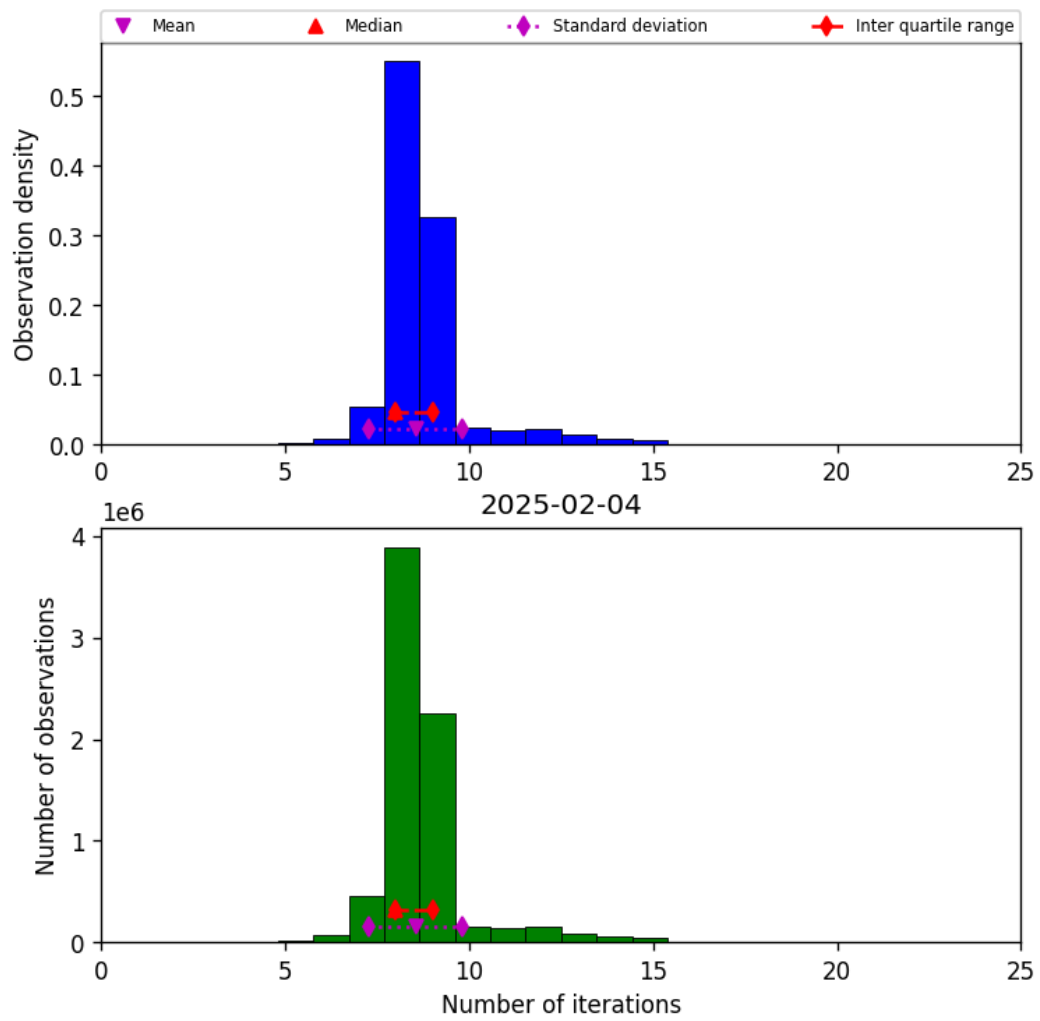
Figure 24: Histogram of “Number of iterations” for 2025-02-03 to 2025-02-05
