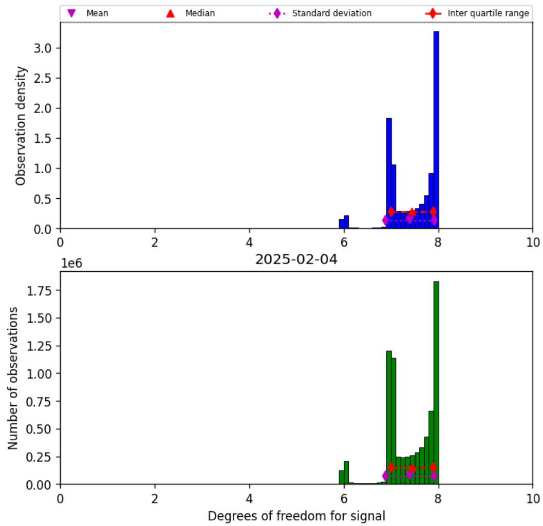
Figure 23: Histogram of “Degrees of freedom for signal” for 2025-02-03 to 2025-02-05
