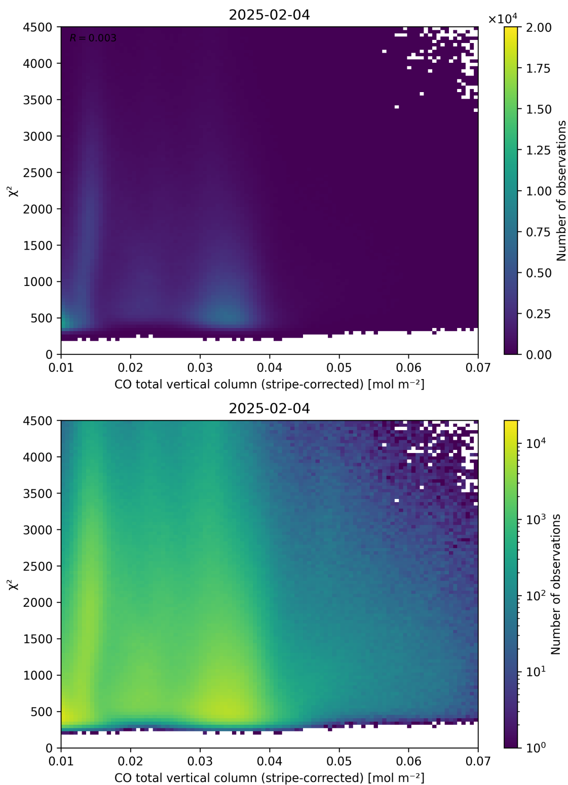
Figure 37: Scatter density plot of “CO total vertical column (stripe-corrected)” against “ \chi^2 ” for 2025-02-03 to 2025-02-05.
