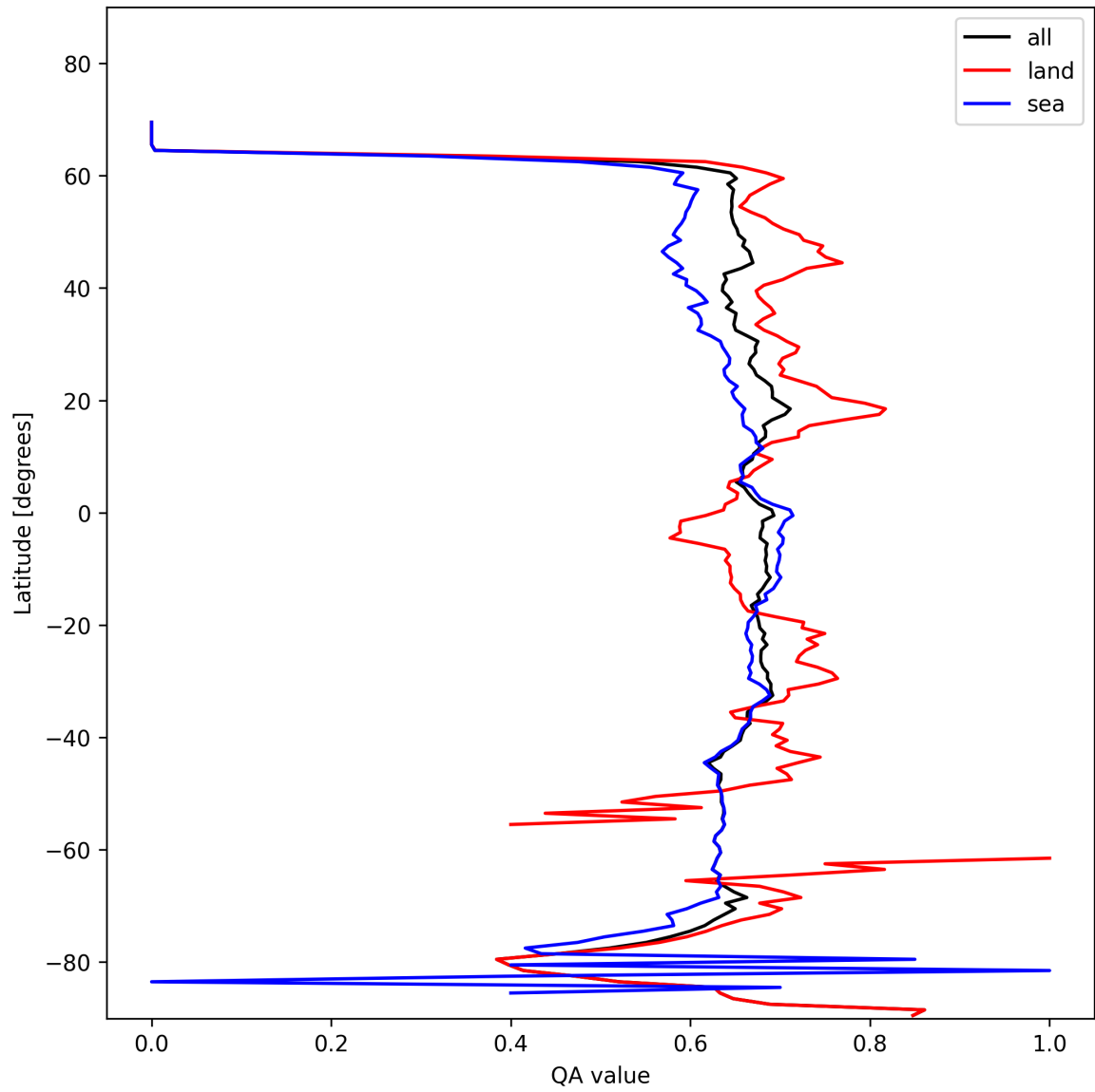
Figure 9: Zonal average of “QA value” for 2025-02-03 to 2025-02-05.
