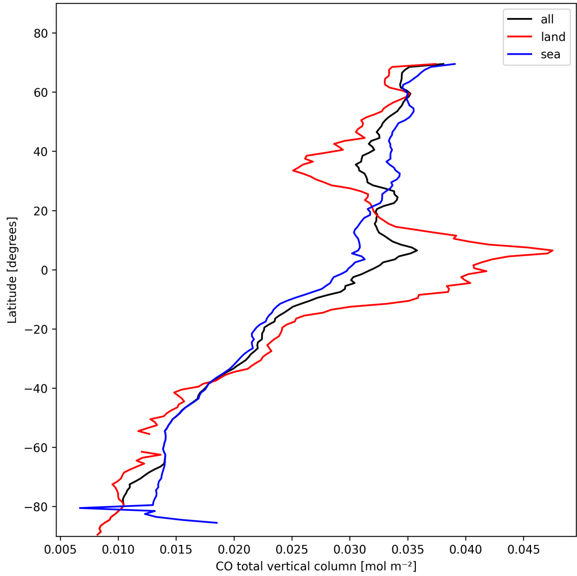
Figure 10: Zonal average of “CO total vertical column” for 2025-02-03 to 2025-02-05.
