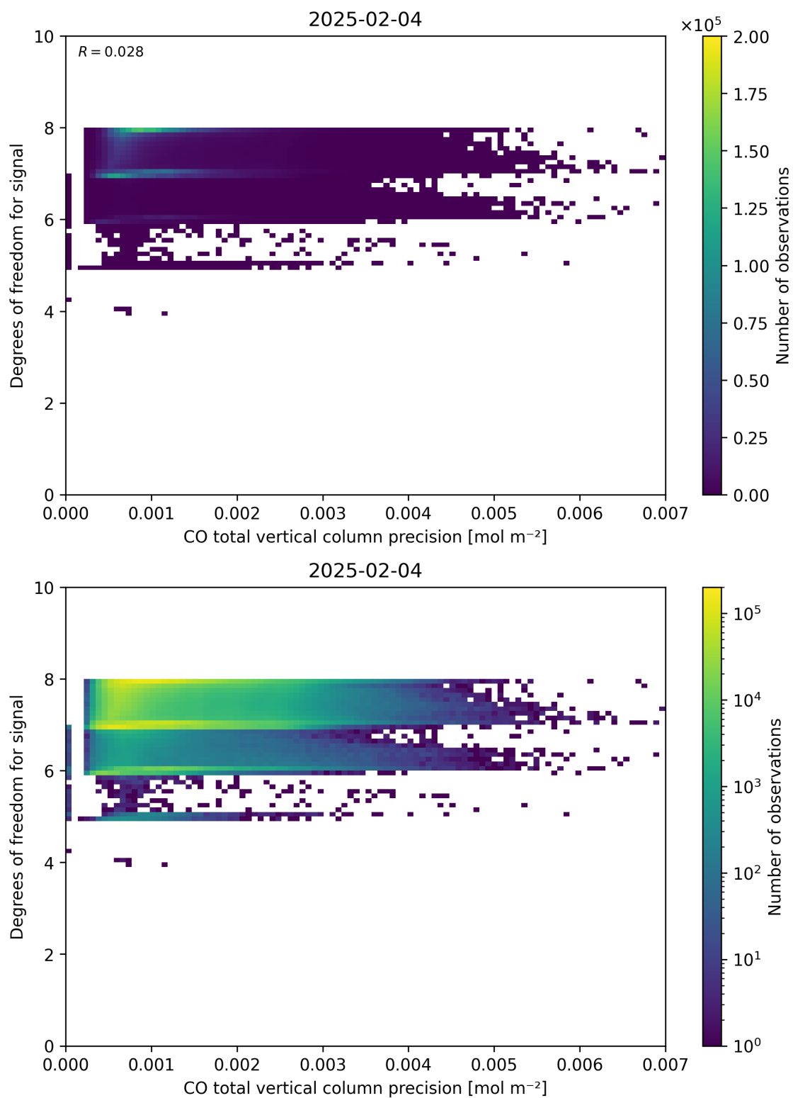
Figure 45: Scatter density plot of “CO total vertical column precision” against “Degrees of freedom for signal” for 2025-02-03 to 2025-02-05.
