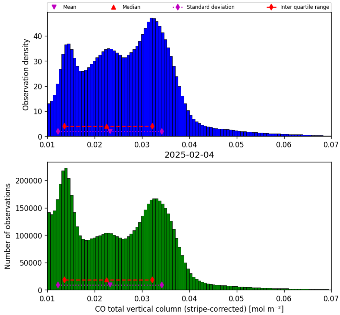
Figure 19: Histogram of “CO total vertical column (stripe-corrected)” for 2025-02-03 to 2025-02-05
