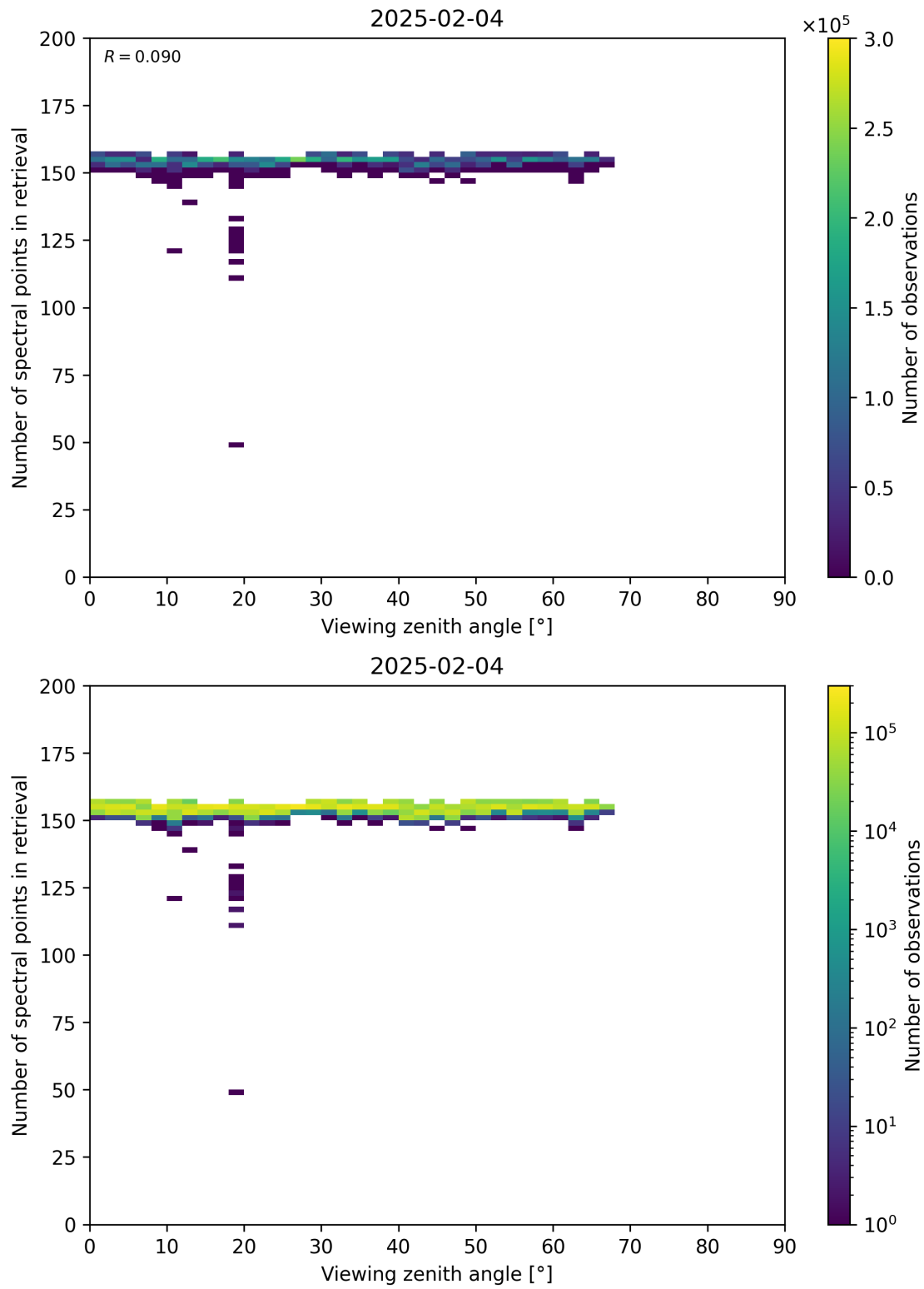
Figure 76: Scatter density plot of “Viewing zenith angle” against “Number of spectral points in retrieval” for 2025-02-03 to 2025-02-05.
