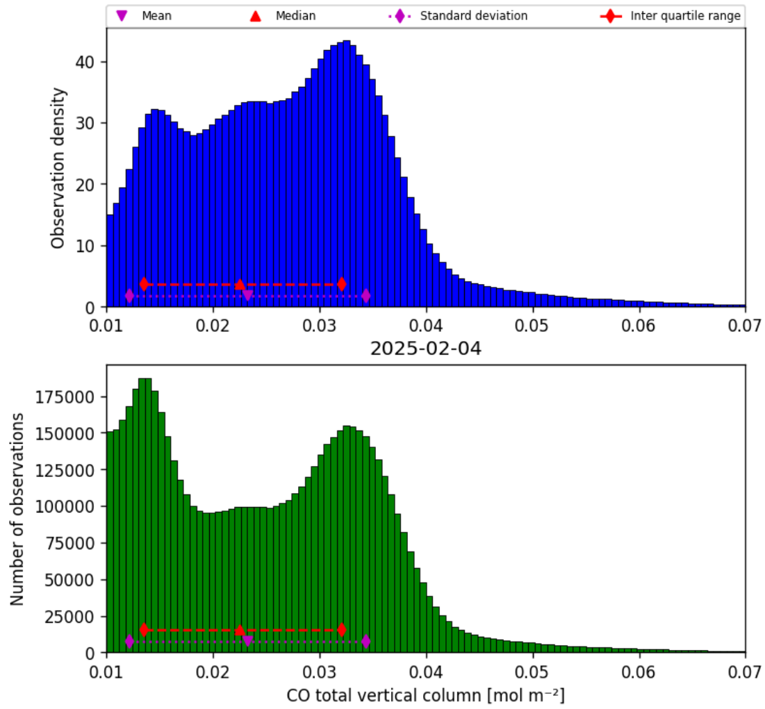
Figure 18: Histogram of “CO total vertical column” for 2025-02-03 to 2025-02-05
