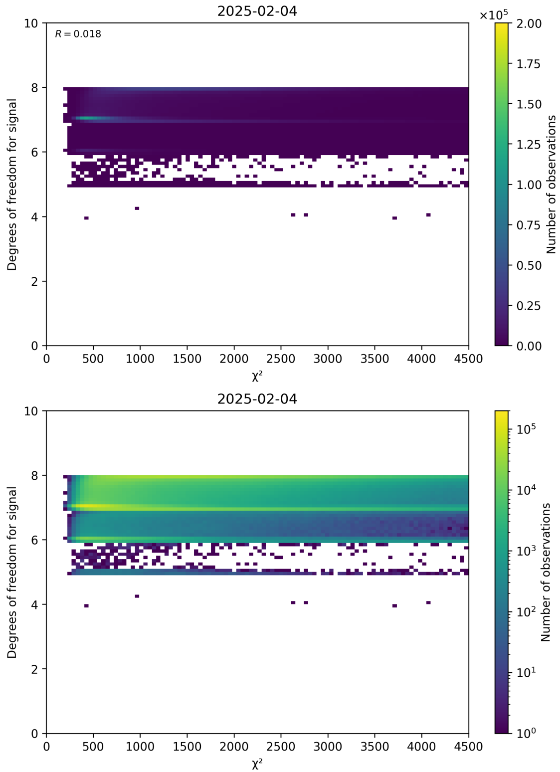
Figure 48: Scatter density plot of “ \chi^2 ” against “Degrees of freedom for signal” for 2025-02-03 to 2025-02-05.
