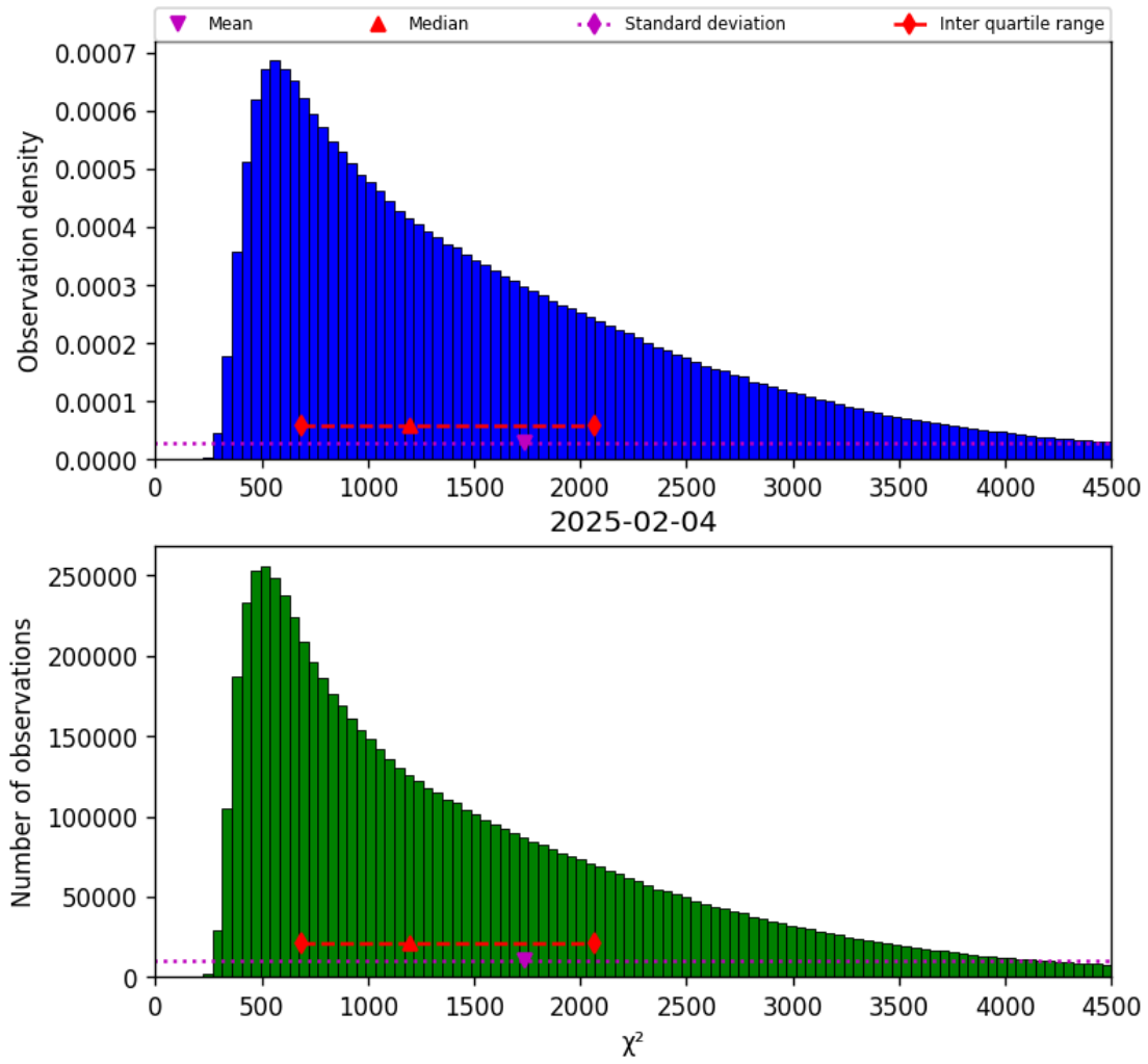
Figure 22: Histogram of " \chi^2 " for 2025-02-03 to 2025-02-05
