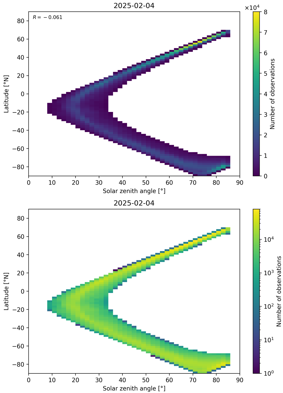
Figure 66: Scatter density plot of “Solar zenith angle” against “Latitude” for 2025-02-03 to 2025-02-05.
