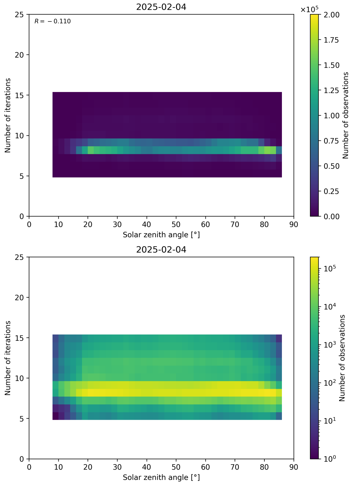
Figure 67: Scatter density plot of “Solar zenith angle” against “Number of iterations” for 2025-02-03 to 2025-02-05.
