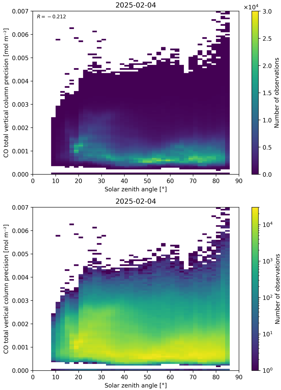
Figure 63: Scatter density plot of “Solar zenith angle” against “CO total vertical column precision” for 2025-02-03 to 2025-02-05.
