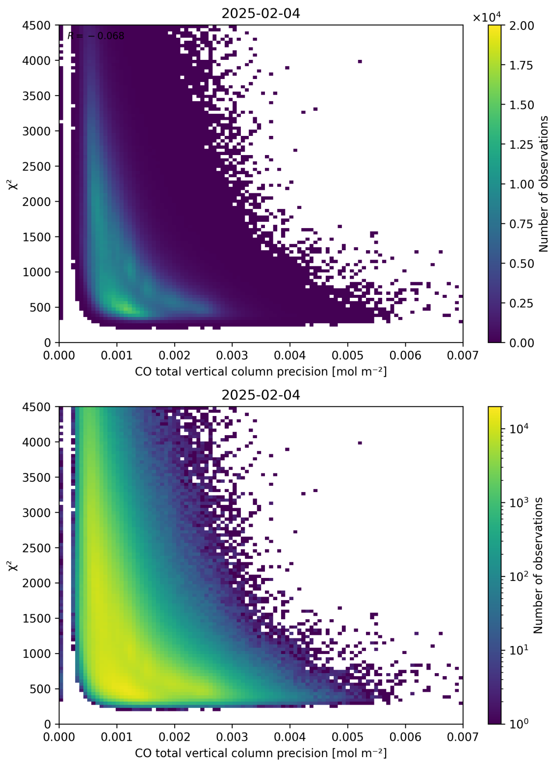
Figure 44: Scatter density plot of “CO total vertical column precision” against “ \chi^2 ” for 2025-02-03 to 2025-02-05.
