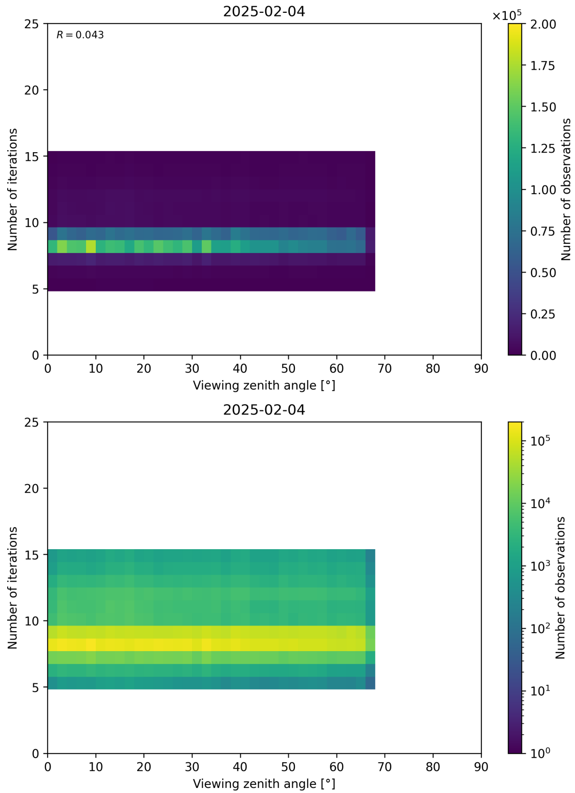
Figure 75: Scatter density plot of “Viewing zenith angle” against “Number of iterations” for 2025-02-03 to 2025-02-05.
