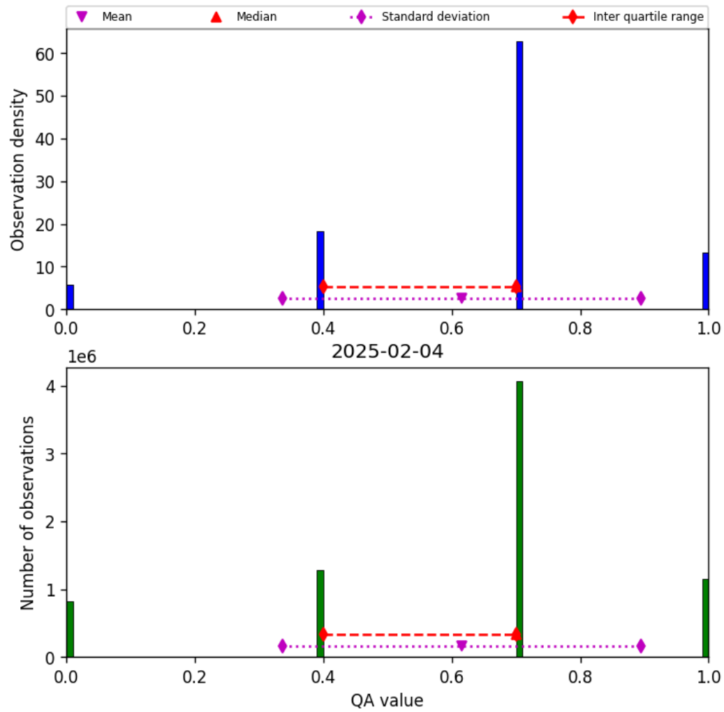
Figure 17: Histogram of “QA value” for 2025-02-03 to 2025-02-05
