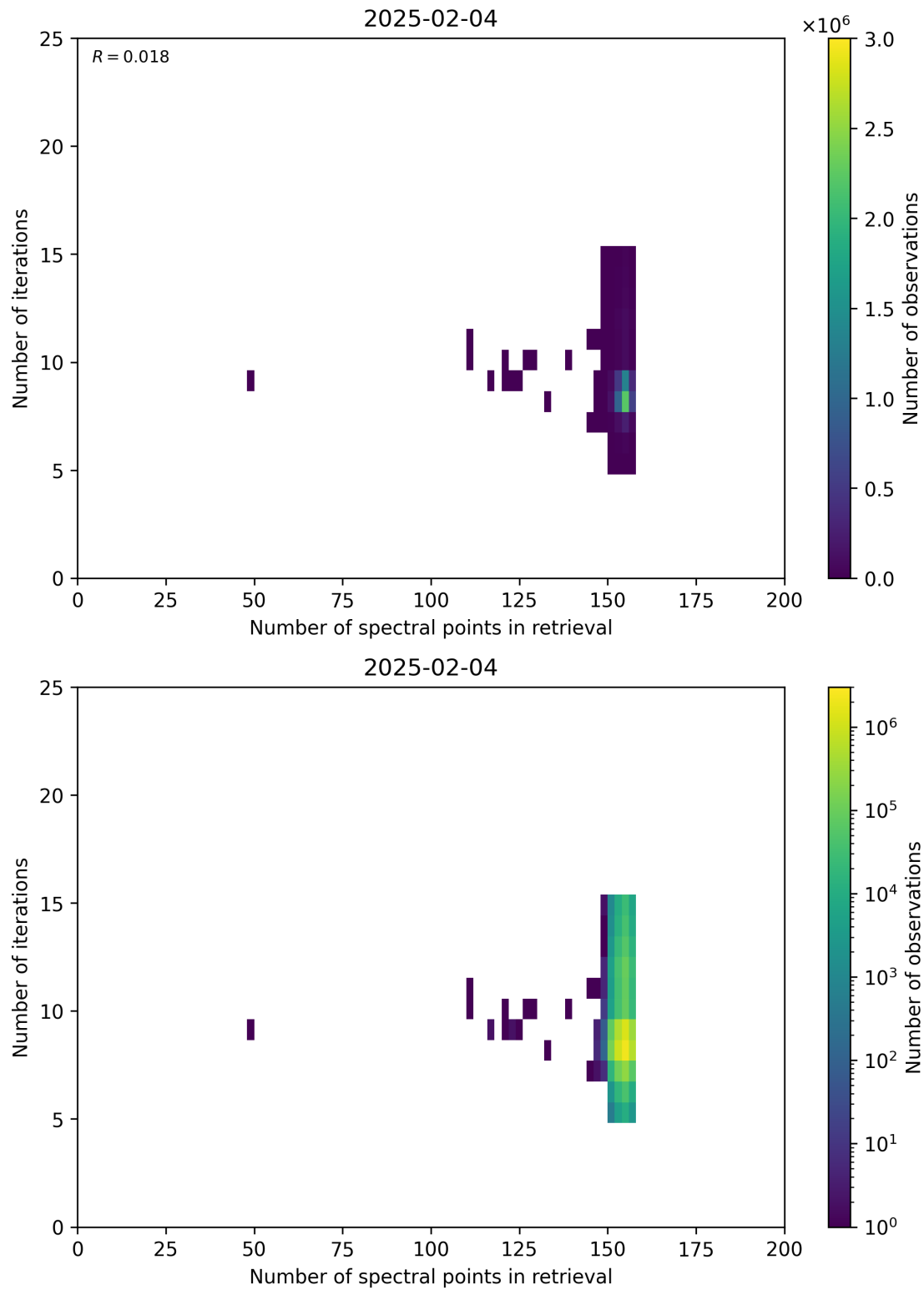
Figure 60: Scatter density plot of “Number of spectral points in retrieval” against “Number of iterations” for 2025-02-03 to 2025-02-05.
