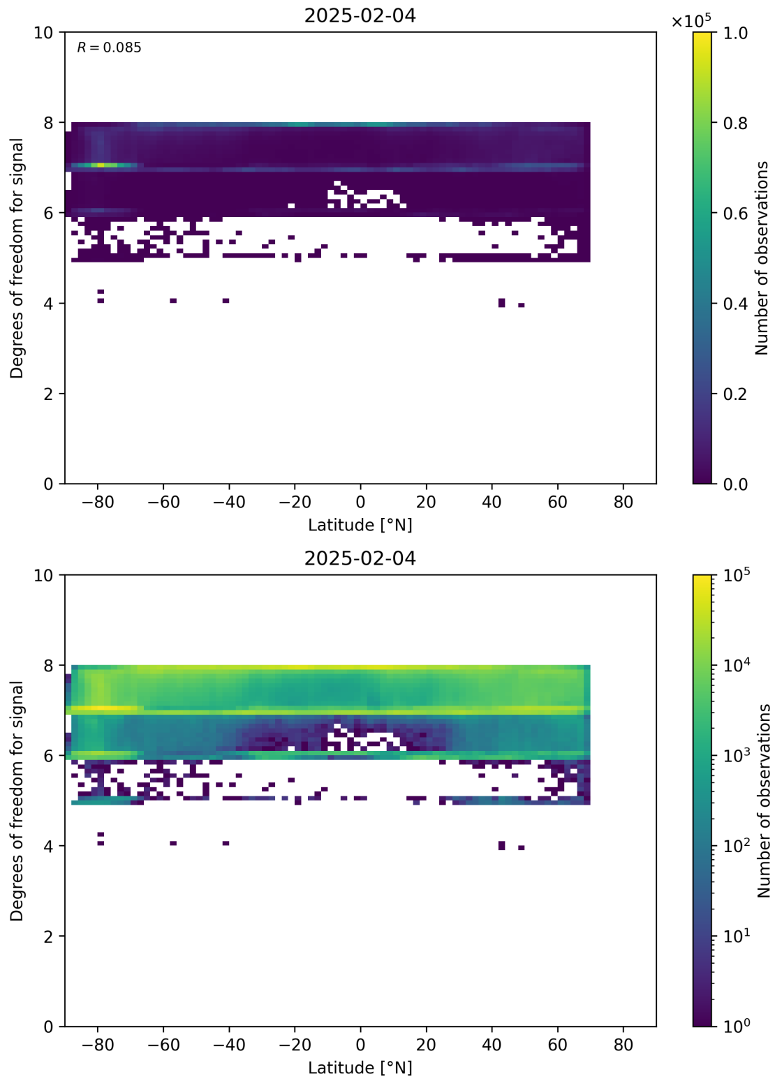
Figure 55: Scatter density plot of “Latitude” against “Degrees of freedom for signal” for 2025-02-03 to 2025-02-05.
