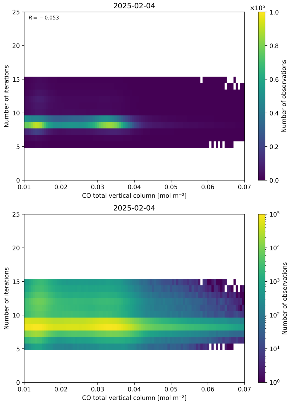
Figure 42: Scatter density plot of “CO total vertical column” against “Number of iterations” for 2025-02-03 to 2025-02-05.
