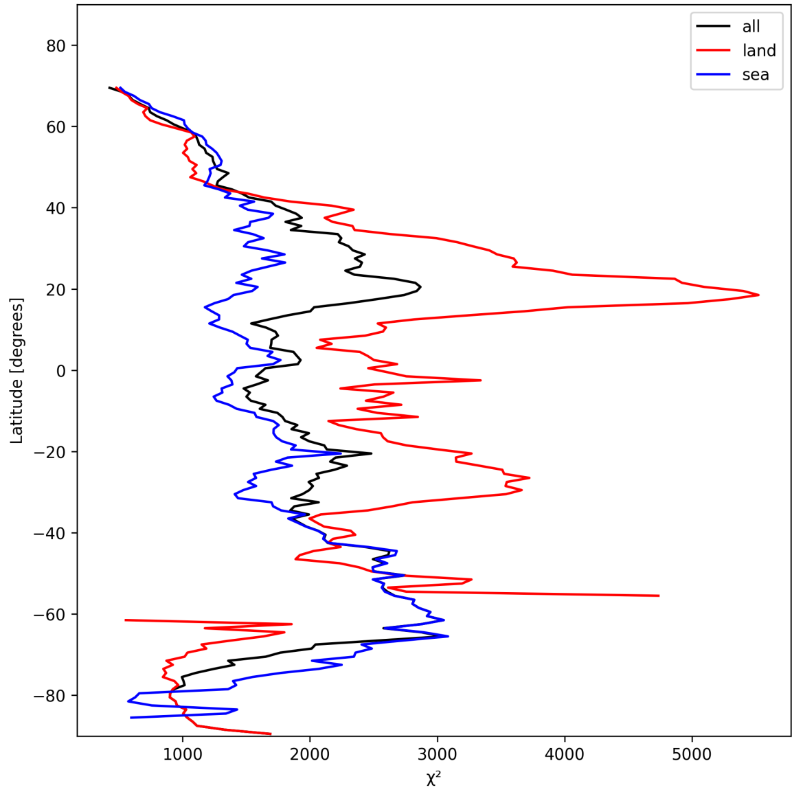
Figure 14: Zonal average of “ \chi^2 ” for 2025-02-03 to 2025-02-05.
