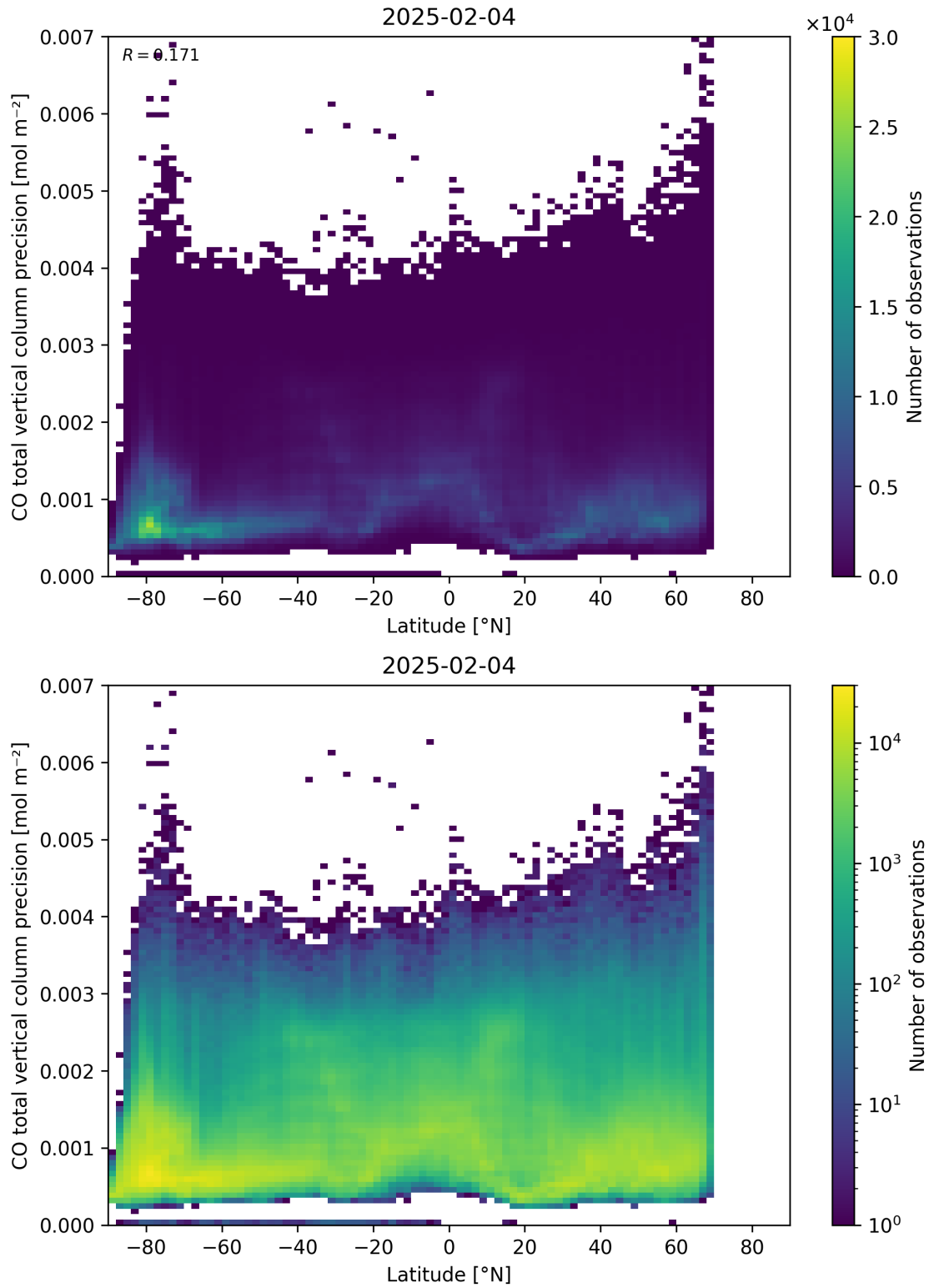
Figure 53: Scatter density plot of “Latitude” against “CO total vertical column precision” for 2025-02-03 to 2025-02-05.
