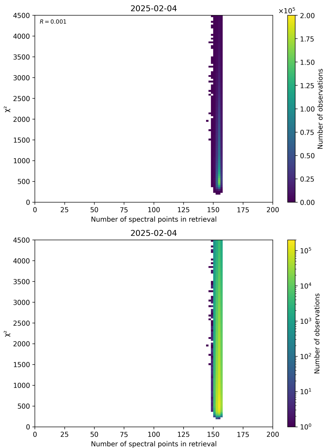
Figure 58: Scatter density plot of “Number of spectral points in retrieval” against “ \chi^2 ” for 2025-02-03 to 2025-02-05.
