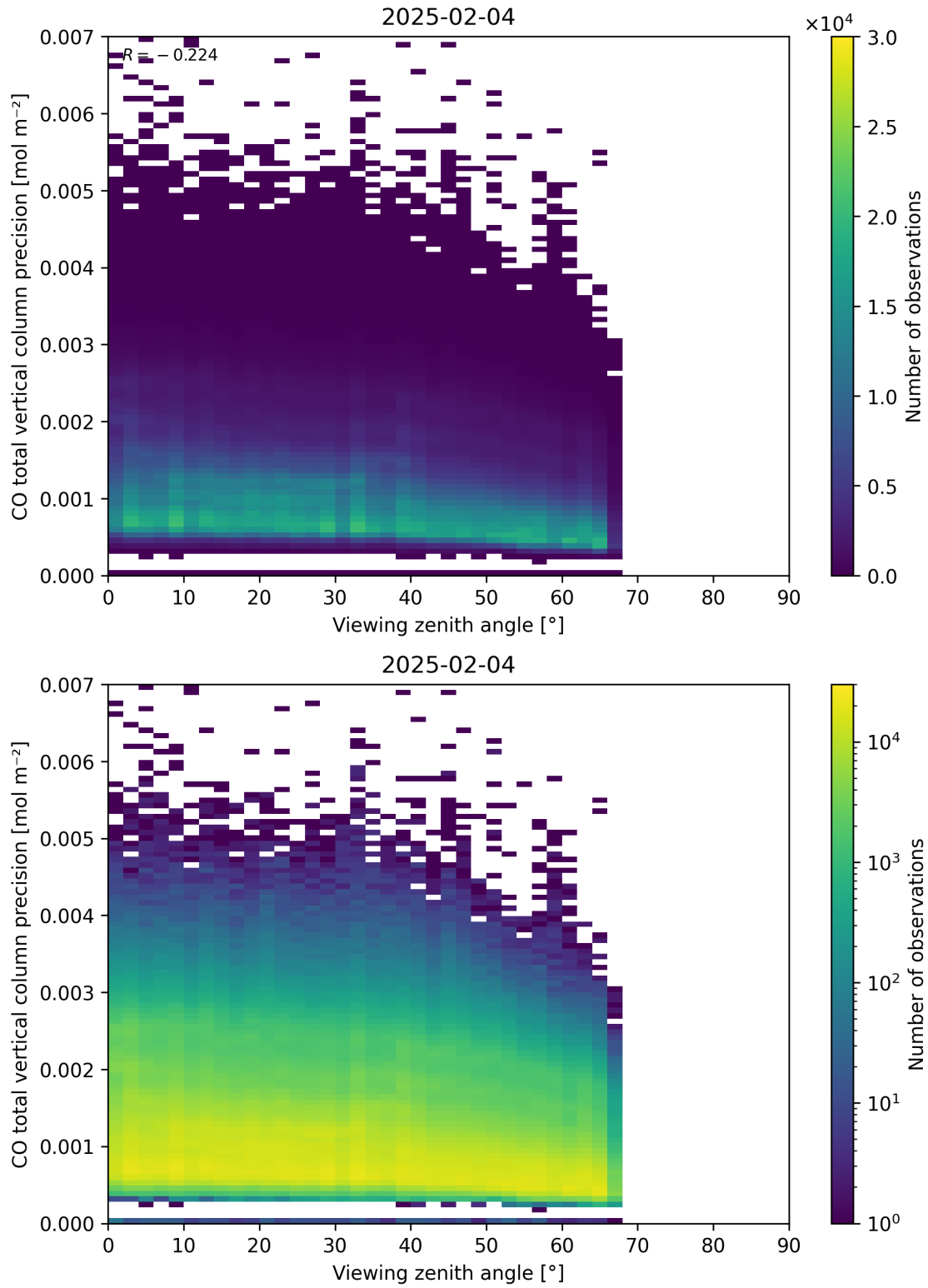
Figure 71: Scatter density plot of “Viewing zenith angle” against “CO total vertical column precision” for 2025-02-03 to 2025-02-05.
