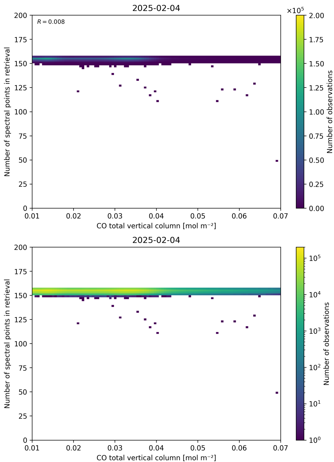
Figure 43: Scatter density plot of “CO total vertical column” against “Number of spectral points in retrieval” for 2025-02-03 to 2025-02-05.
