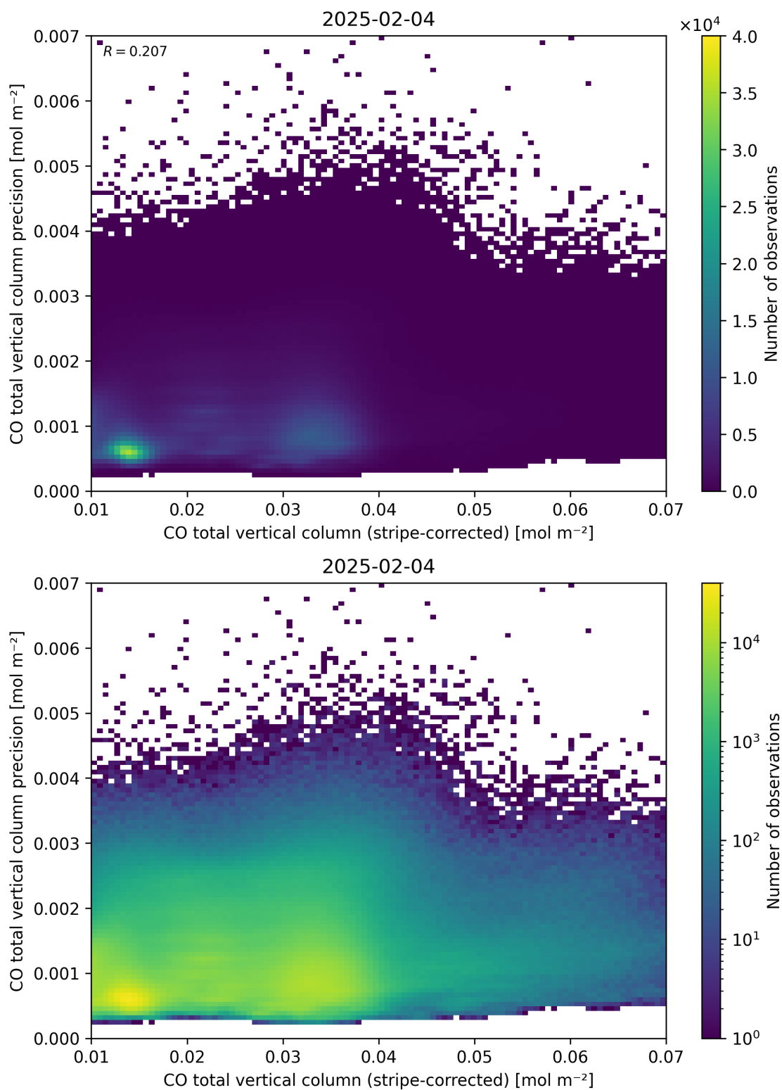
Figure 36: Scatter density plot of “CO total vertical column (stripe-corrected)” against “CO total vertical column precision” for 2025-02-03 to 2025-02-05.
