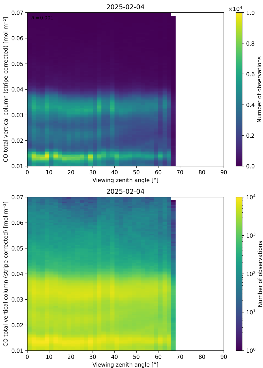
Figure 70: Scatter density plot of “Viewing zenith angle” against “CO total vertical column (stripe-corrected)” for 2025-02-03 to 2025-02-05.
