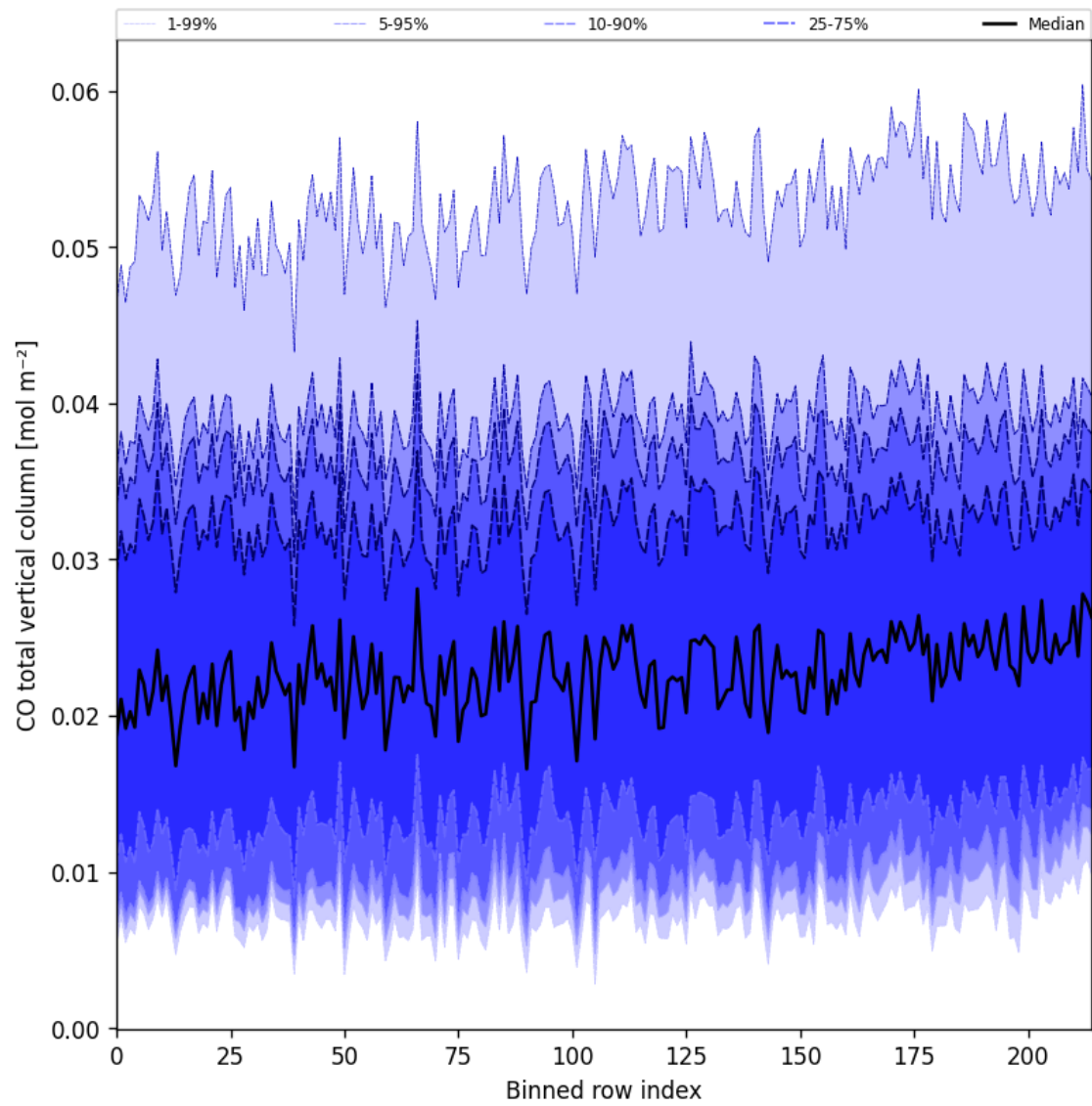
Figure 26: Along track statistics of “CO total vertical column” for 2025-02-03 to 2025-02-05
