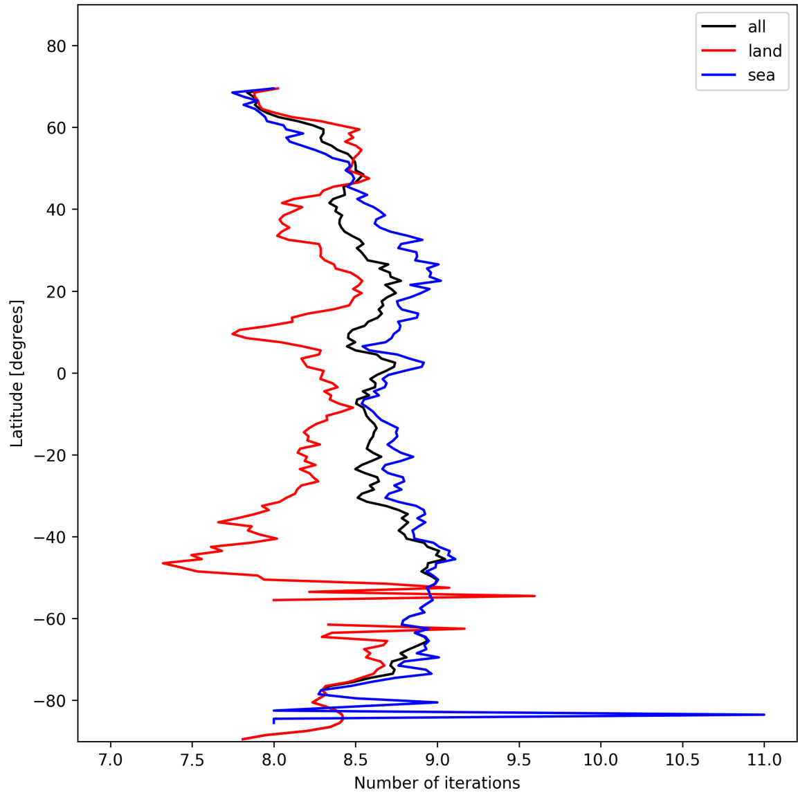
Figure 16: Zonal average of “Number of iterations” for 2025-02-03 to 2025-02-05.
