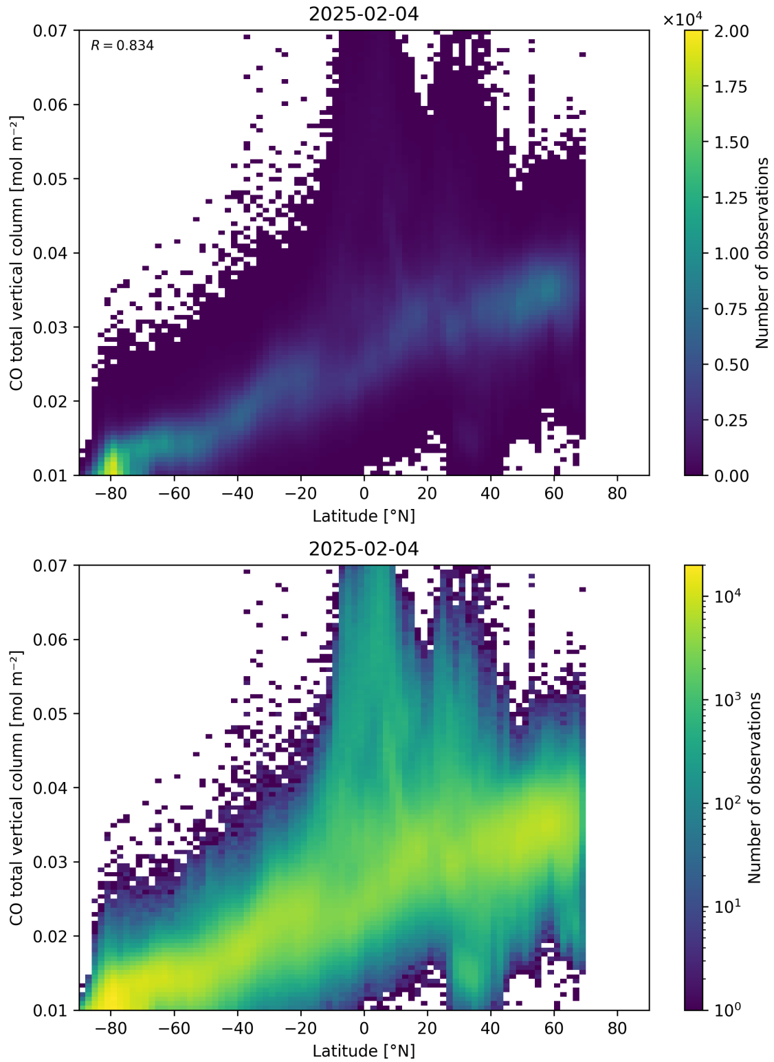
Figure 51: Scatter density plot of “Latitude” against “CO total vertical column” for 2025-02-03 to 2025-02-05.
