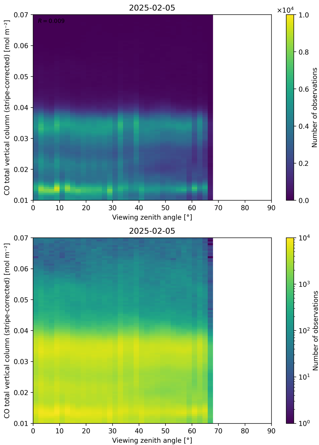
Figure 70: Scatter density plot of “Viewing zenith angle” against “CO total vertical column (stripe-corrected)” for 2025-02-04 to 2025-02-06.
