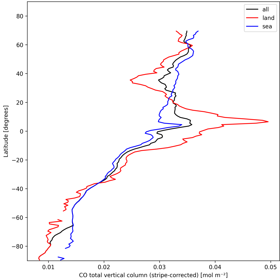
Figure 11: Zonal average of “CO total vertical column (stripe-corrected)” for 2025-02-04 to 2025-02-06.
