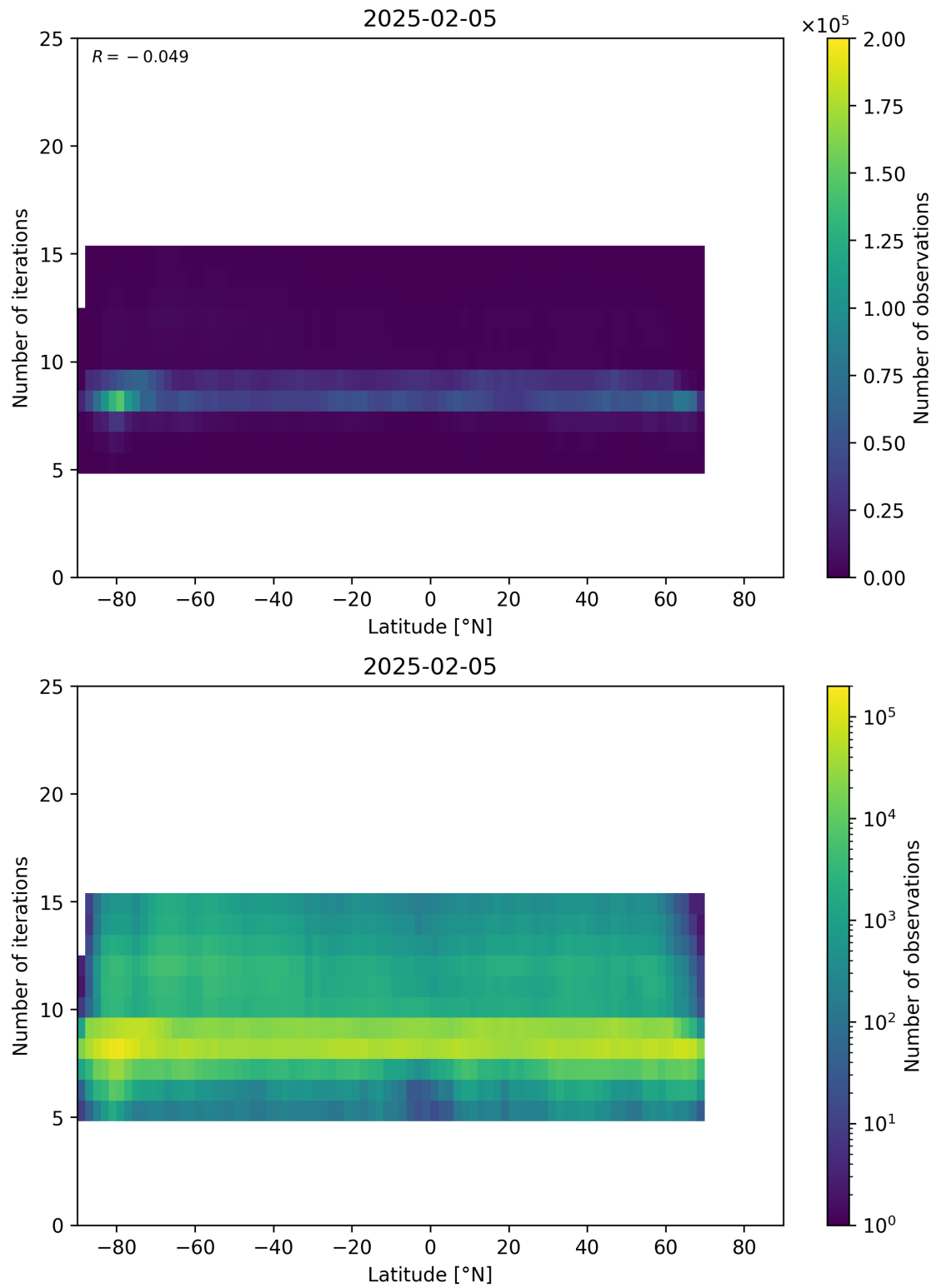
Figure 56: Scatter density plot of “Latitude” against “Number of iterations” for 2025-02-04 to 2025-02-06.
