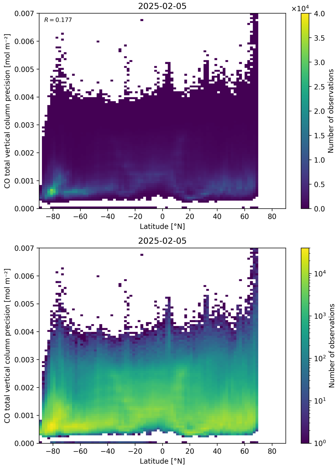
Figure 53: Scatter density plot of “Latitude” against “CO total vertical column precision” for 2025-02-04 to 2025-02-06.
