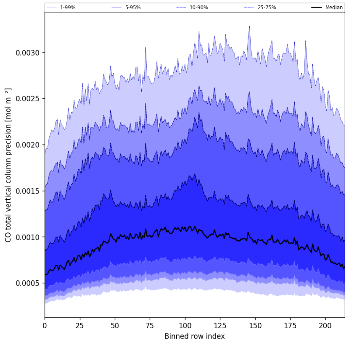
Figure 28: Along track statistics of “CO total vertical column precision” for 2025-02-04 to 2025-02-06
