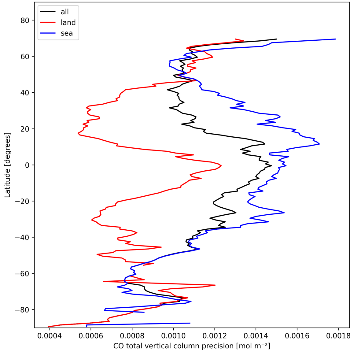
Figure 12: Zonal average of “CO total vertical column precision” for 2025-02-04 to 2025-02-06.
