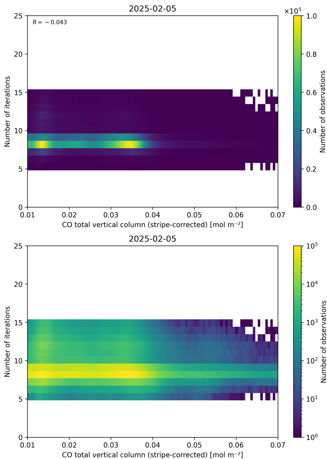
Figure 39: Scatter density plot of “CO total vertical column (stripe-corrected)” against “Number of iterations” for 2025-02-04 to 2025-02-06.
