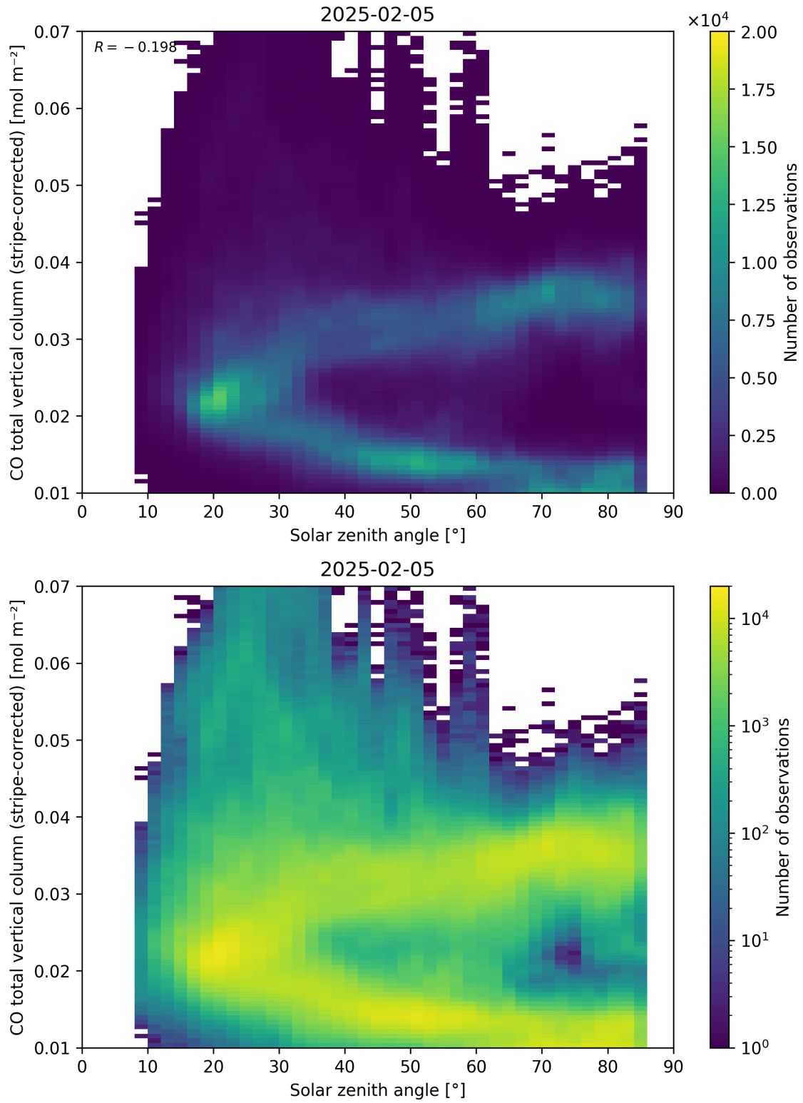
Figure 62: Scatter density plot of “Solar zenith angle” against “CO total vertical column (stripe-corrected)” for 2025-02-04 to 2025-02-06.
