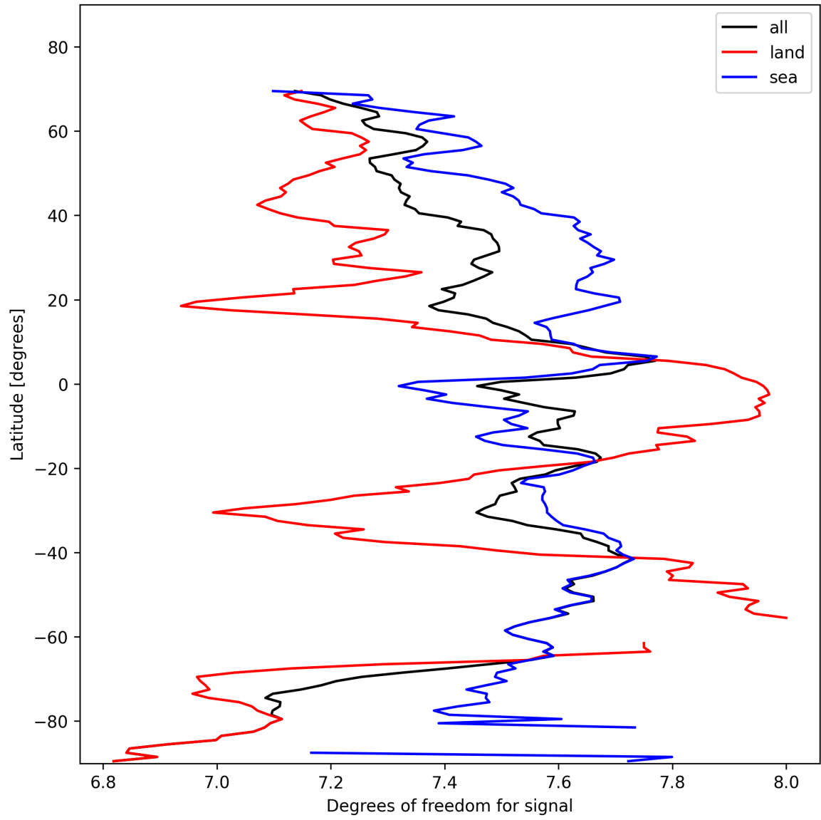
Figure 15: Zonal average of “Degrees of freedom for signal” for 2025-02-04 to 2025-02-06.
