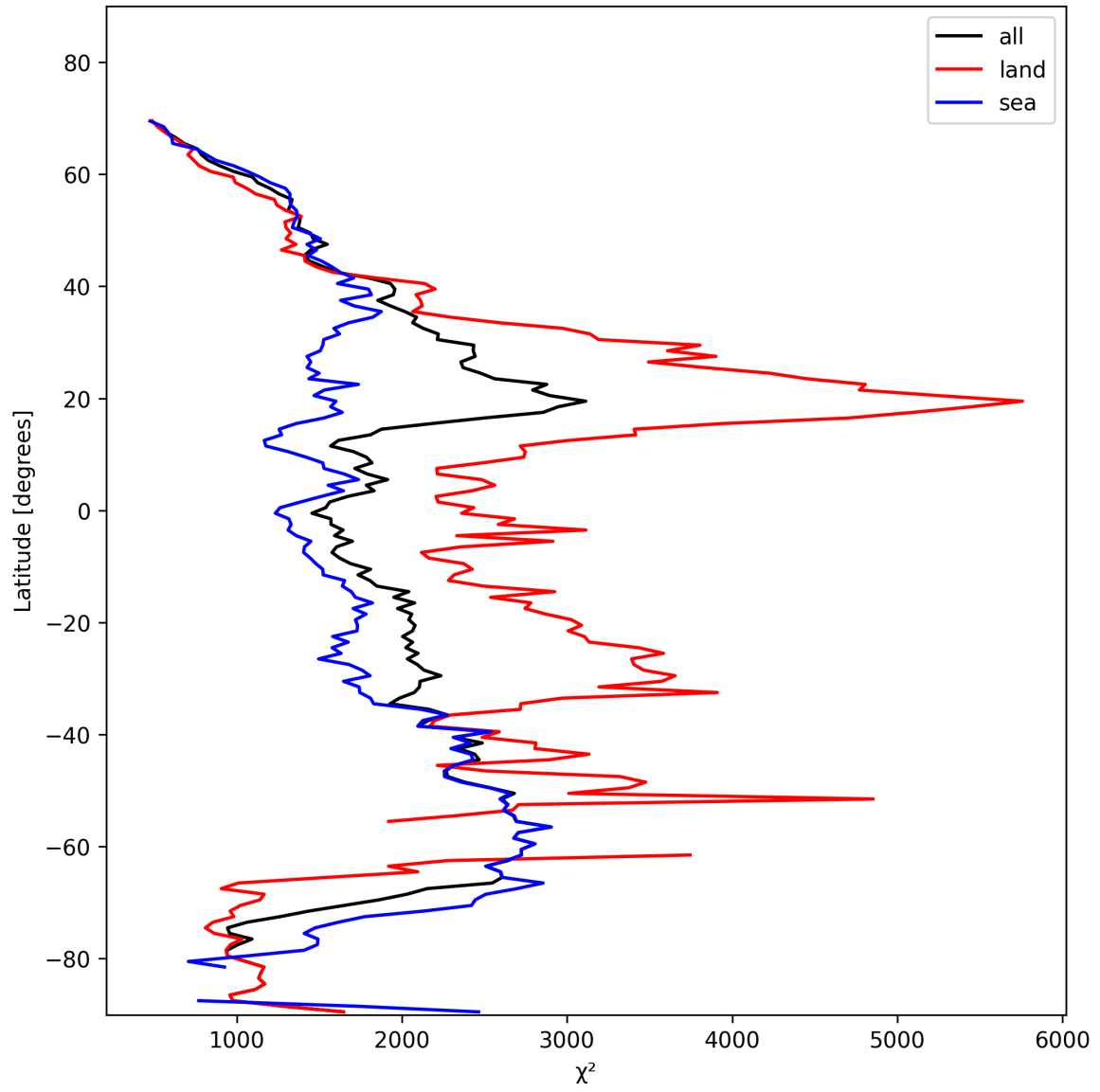
Figure 14: Zonal average of “ \chi^2 ” for 2025-02-04 to 2025-02-06.
