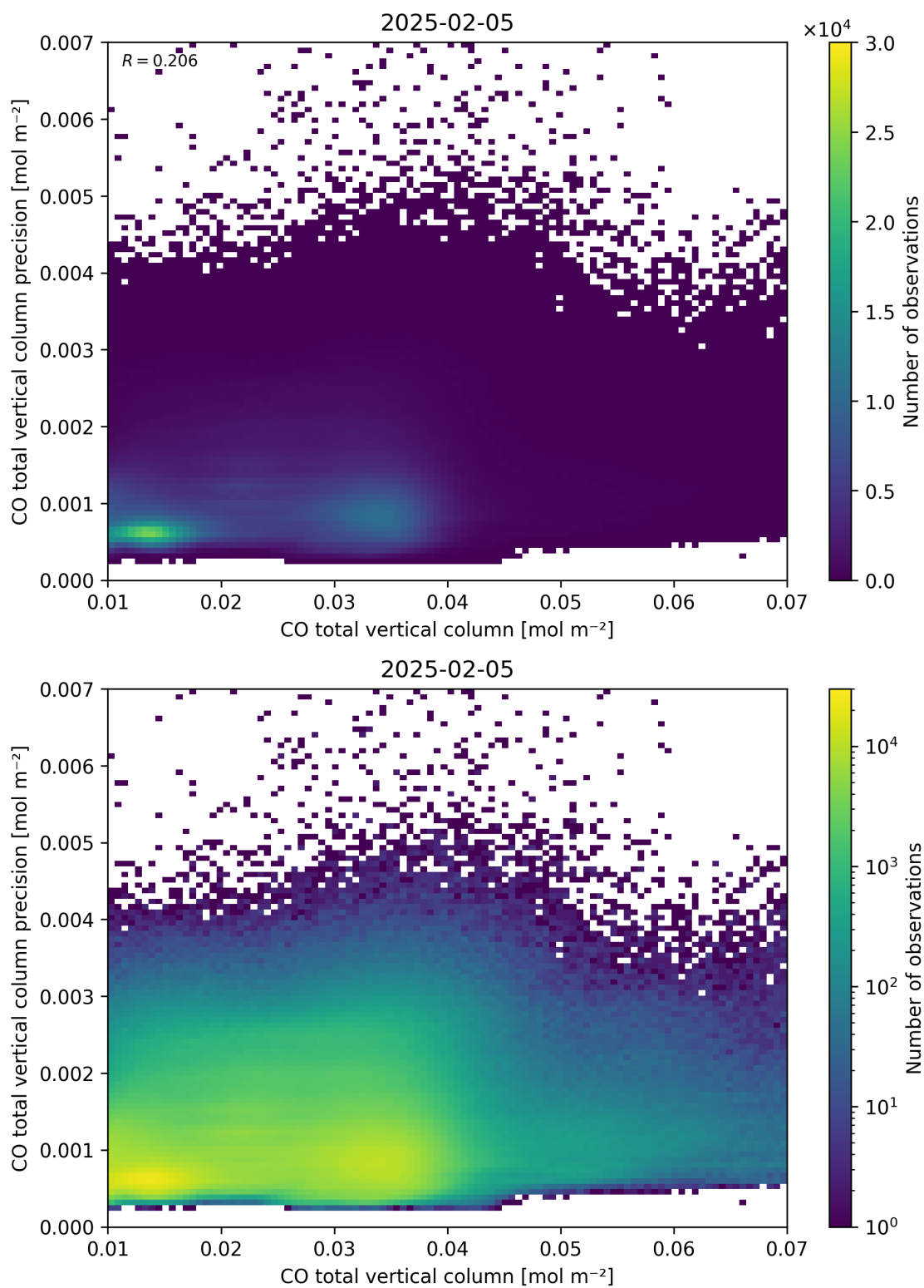
Figure 34: Scatter density plot of “CO total vertical column” against “CO total vertical column precision” for 2025-02-04 to 2025-02-06.
