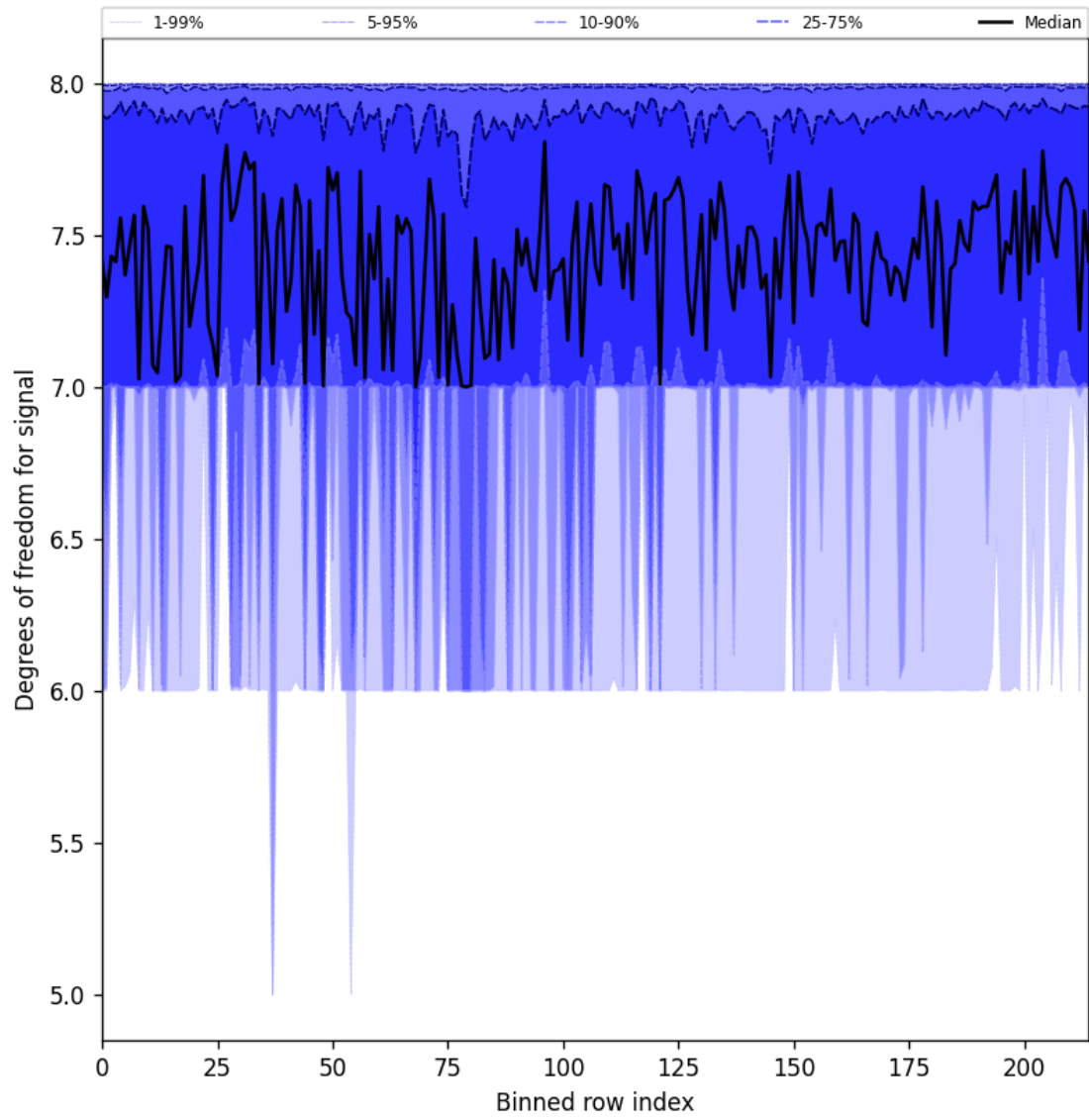
Figure 31: Along track statistics of “Degrees of freedom for signal” for 2025-02-04 to 2025-02-06
