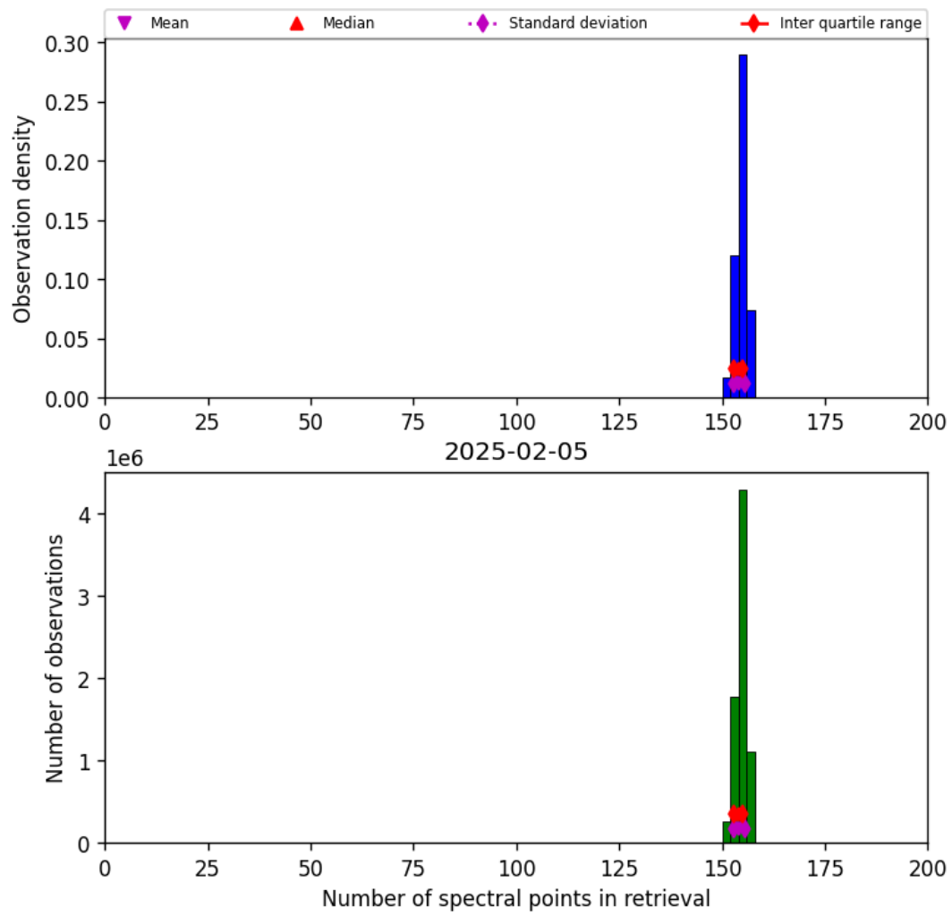
Figure 21: Histogram of “Number of spectral points in retrieval” for 2025-02-04 to 2025-02-06
