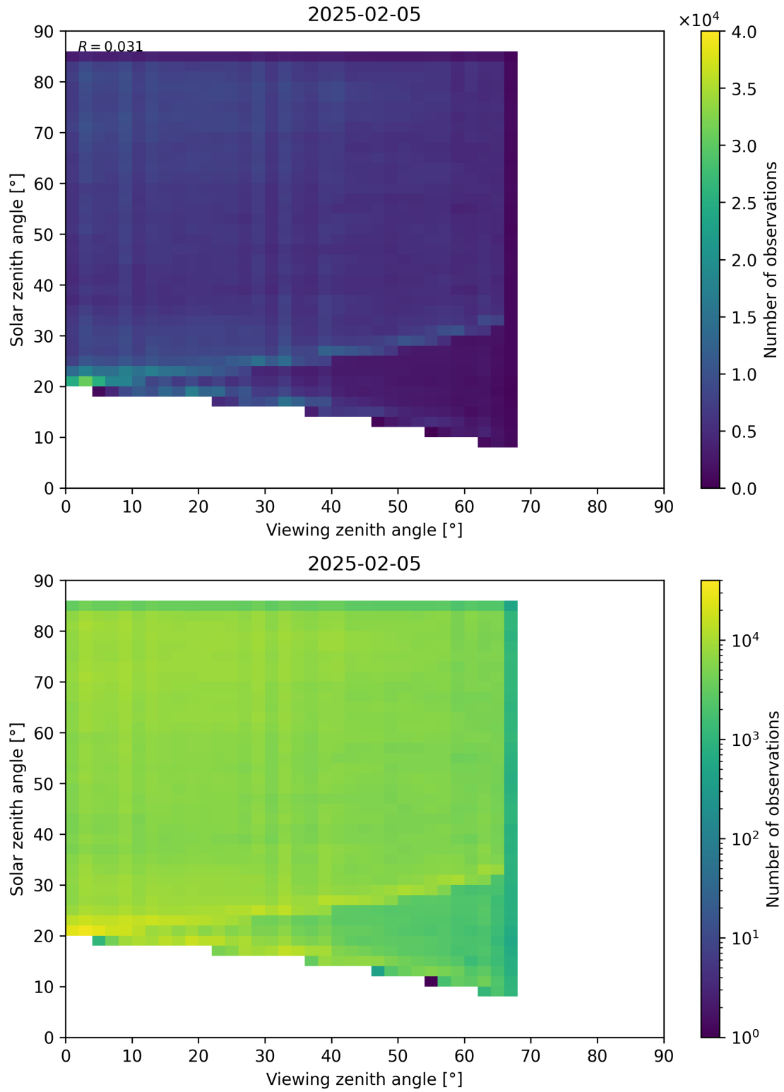
Figure 77: Scatter density plot of “Viewing zenith angle” against “Solar zenith angle” for 2025-02-04 to 2025-02-06.
