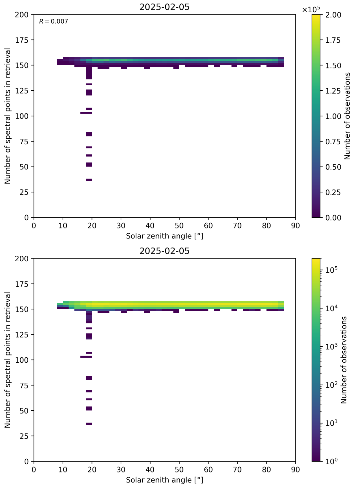
Figure 68: Scatter density plot of “Solar zenith angle” against “Number of spectral points in retrieval” for 2025-02-04 to 2025-02-06.
