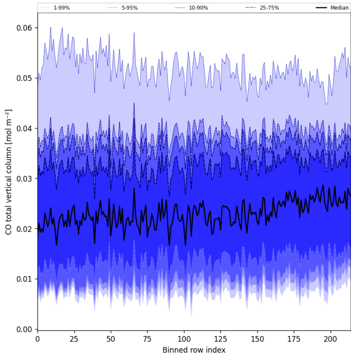
Figure 26: Along track statistics of “CO total vertical column” for 2025-02-04 to 2025-02-06
