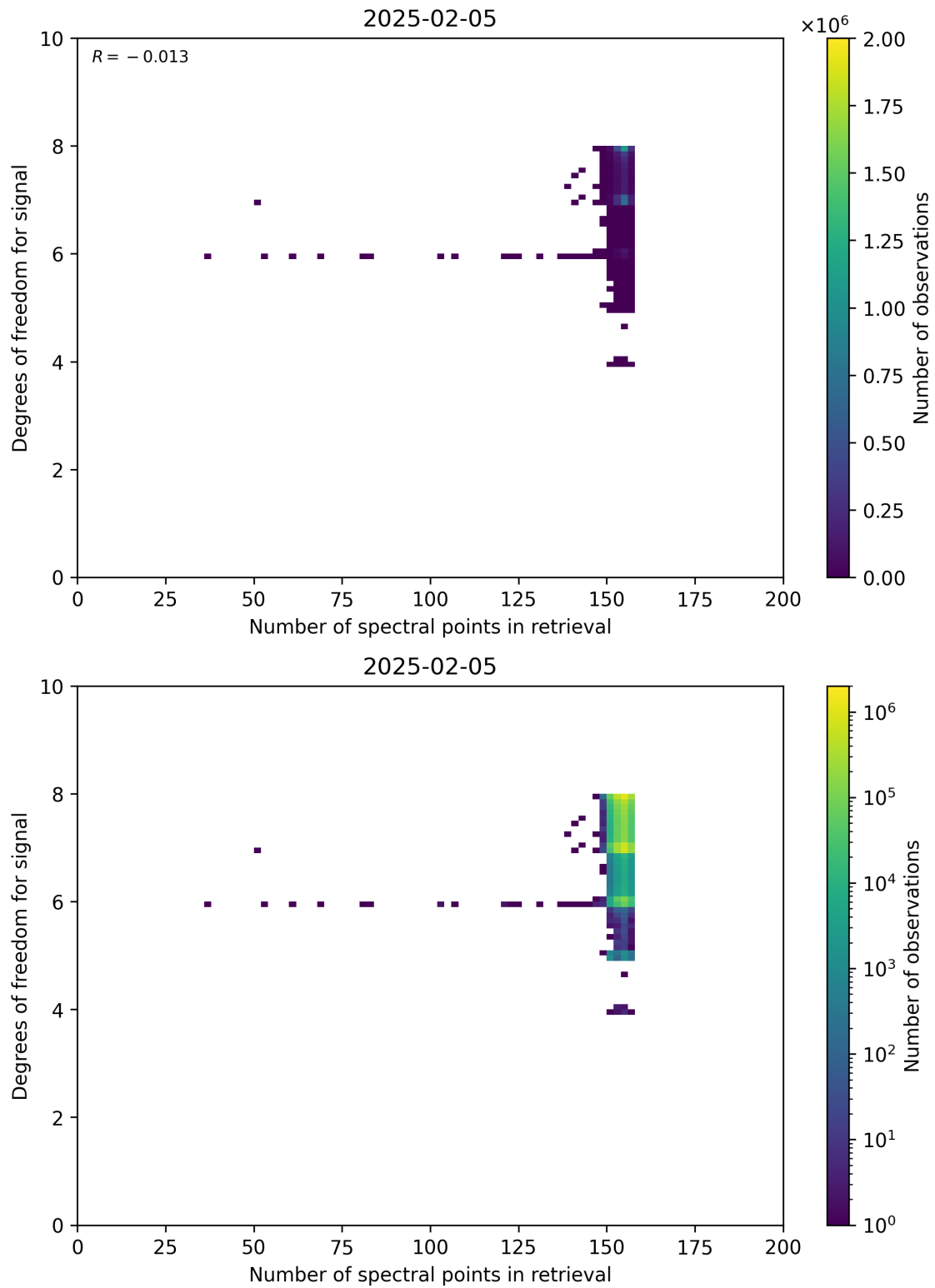
Figure 59: Scatter density plot of “Number of spectral points in retrieval” against “Degrees of freedom for signal” for 2025-02-04 to 2025-02-06.
