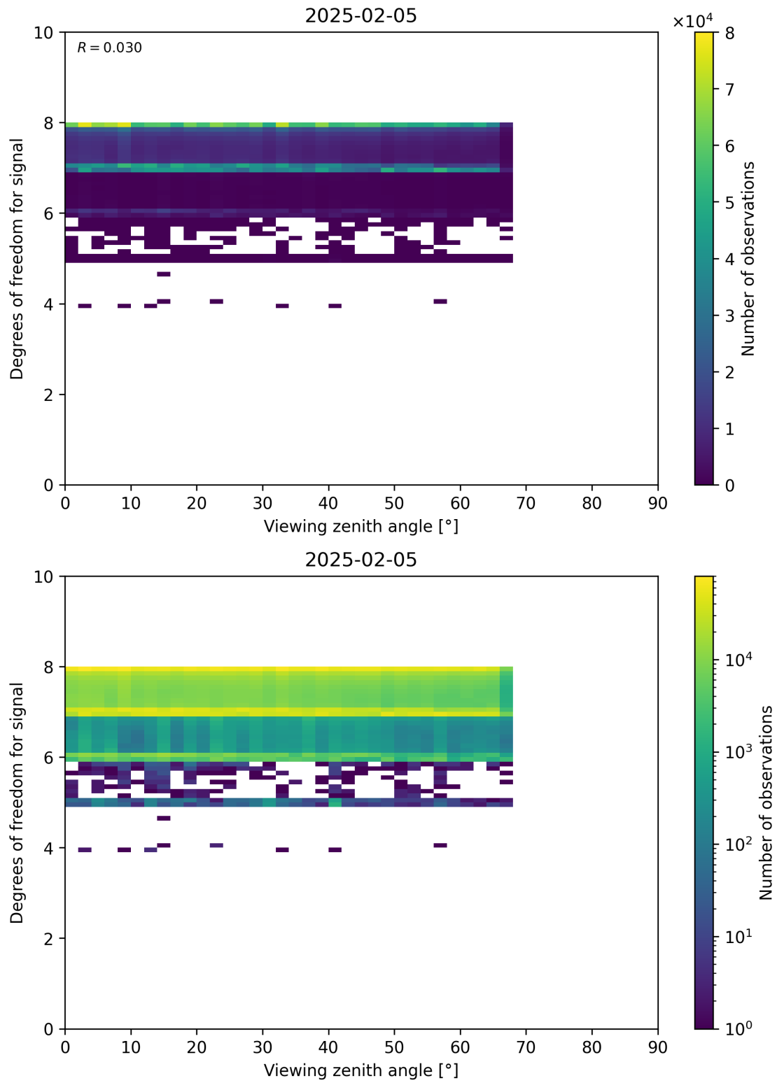
Figure 73: Scatter density plot of “Viewing zenith angle” against “Degrees of freedom for signal” for 2025-02-04 to 2025-02-06.
