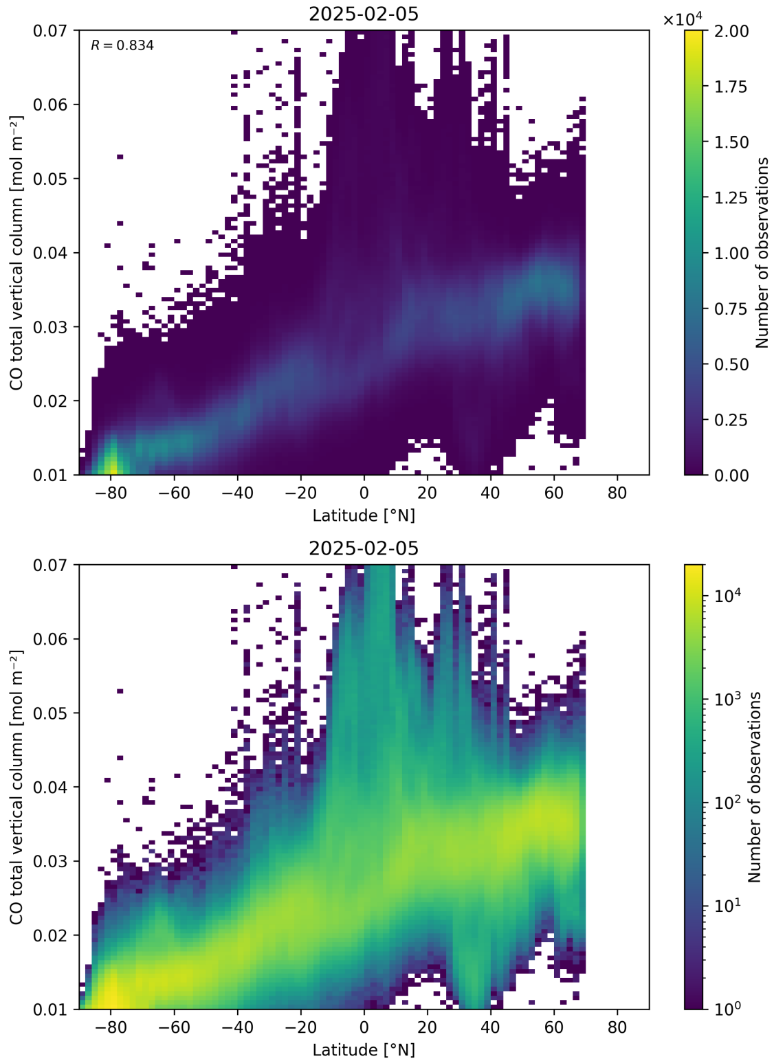
Figure 51: Scatter density plot of “Latitude” against “CO total vertical column” for 2025-02-04 to 2025-02-06.
