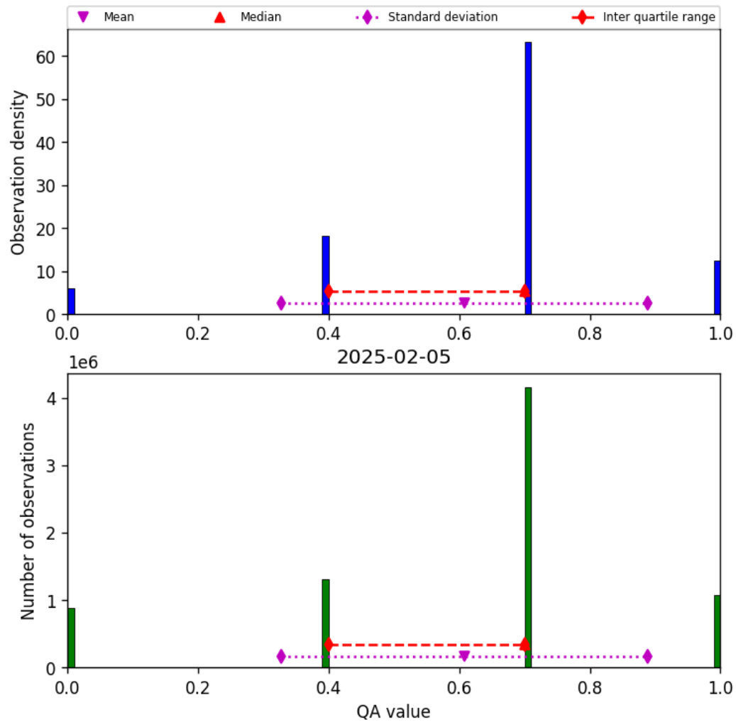
Figure 17: Histogram of “QA value” for 2025-02-04 to 2025-02-06
