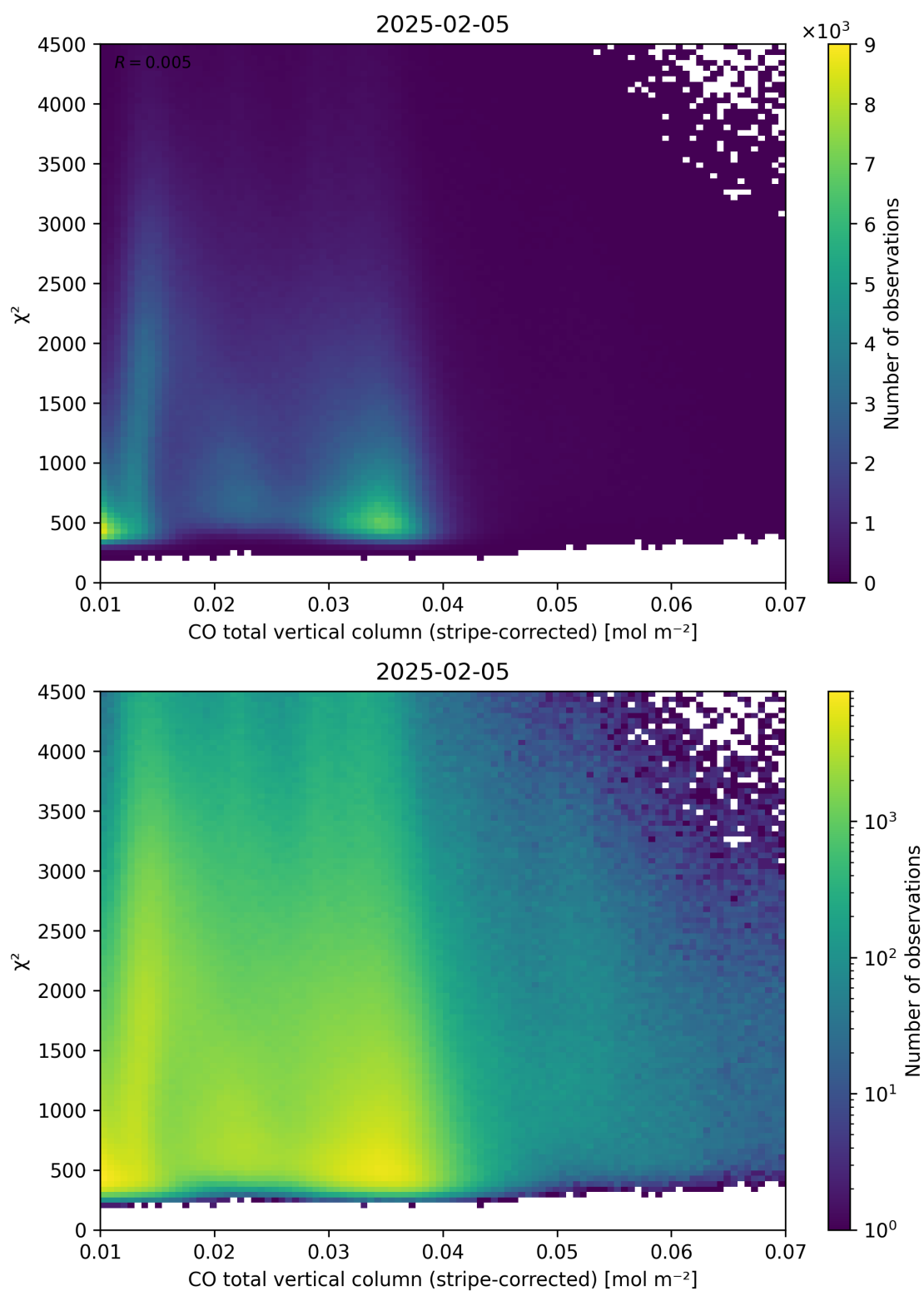
Figure 37: Scatter density plot of “CO total vertical column (stripe-corrected)” against “ \chi^2 ” for 2025-02-04 to 2025-02-06.
