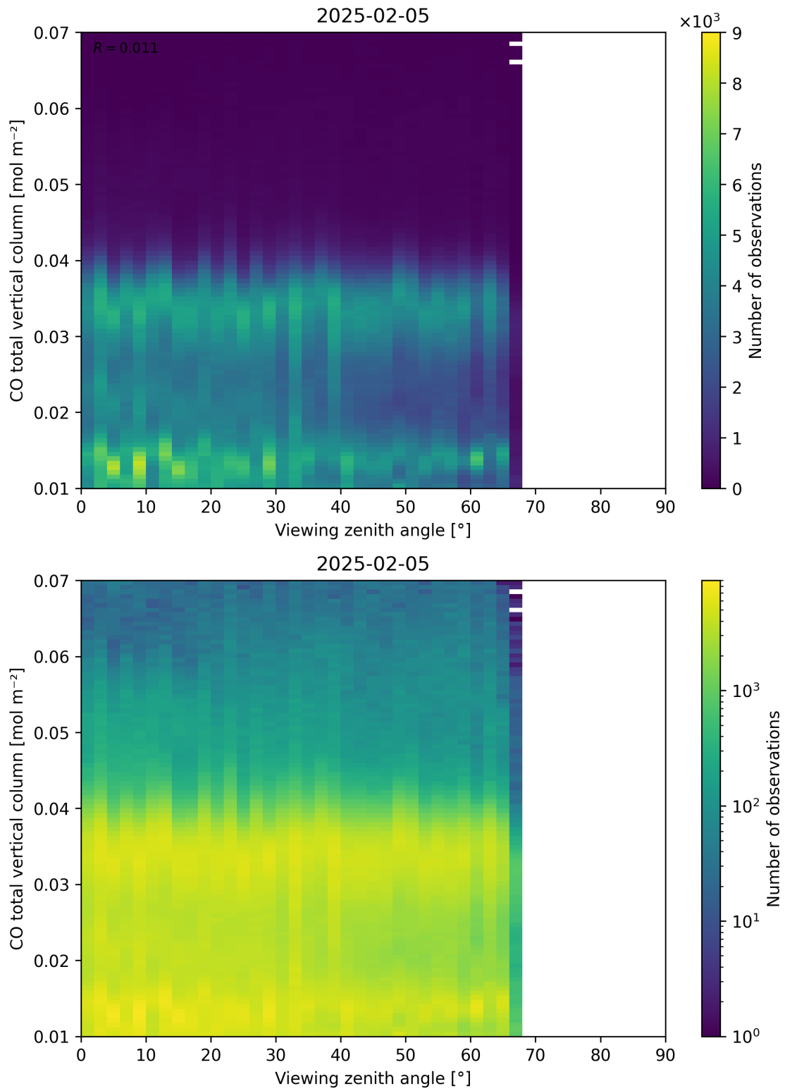
Figure 69: Scatter density plot of “Viewing zenith angle” against “CO total vertical column” for 2025-02-04 to 2025-02-06.
