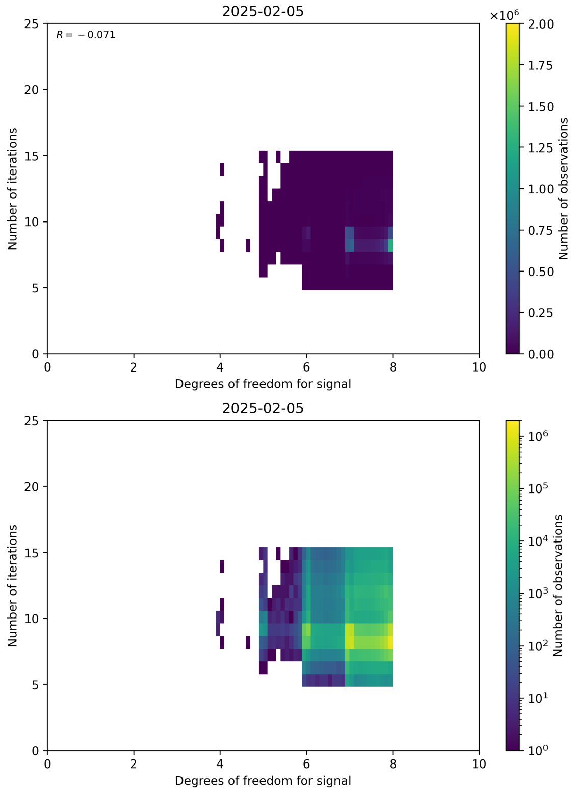
Figure 50: Scatter density plot of “Degrees of freedom for signal” against “Number of iterations” for 2025-02-04 to 2025-02-06.
