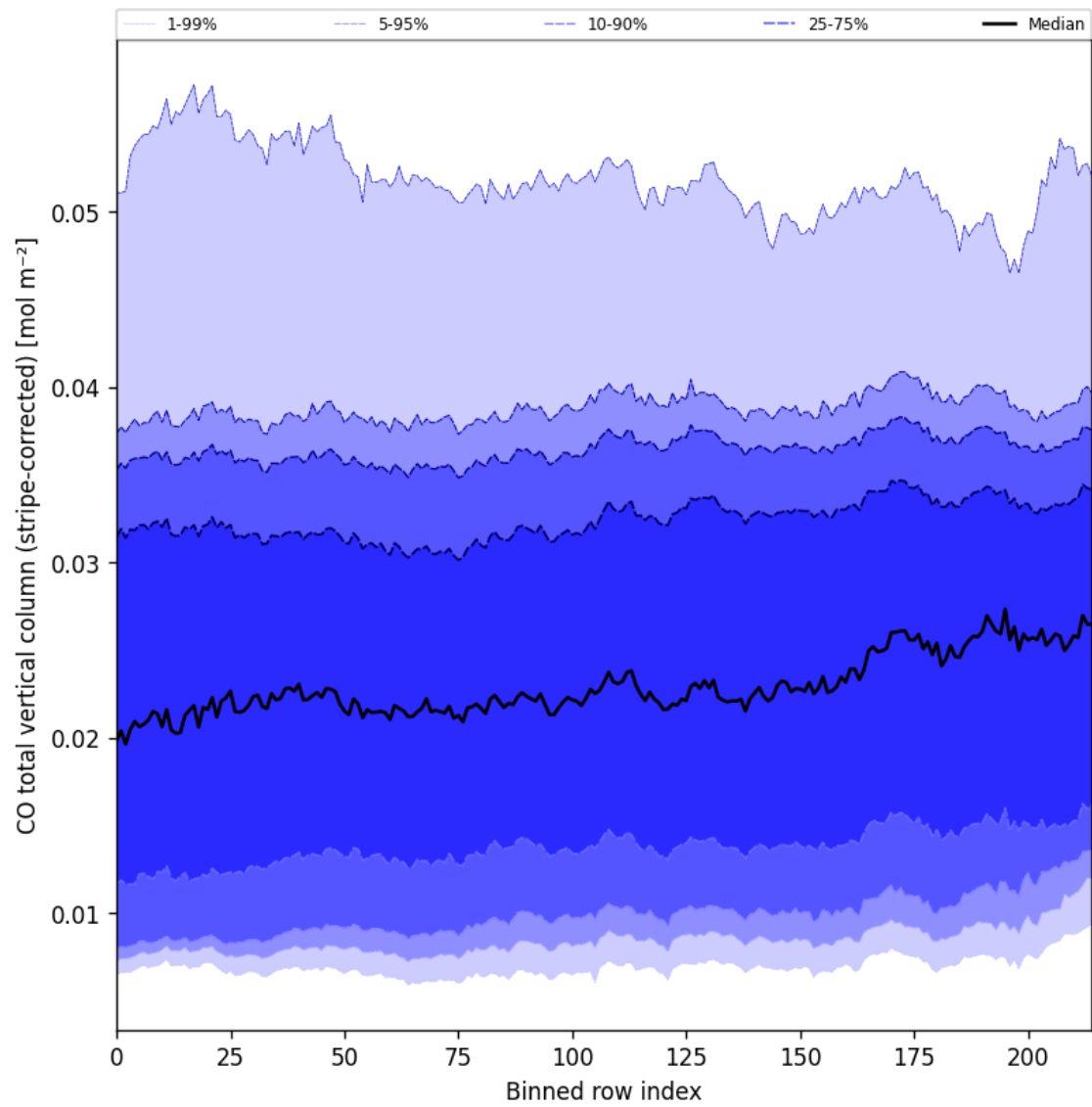
Figure 27: Along track statistics of “CO total vertical column (stripe-corrected)” for 2025-02-04 to 2025-02-06
