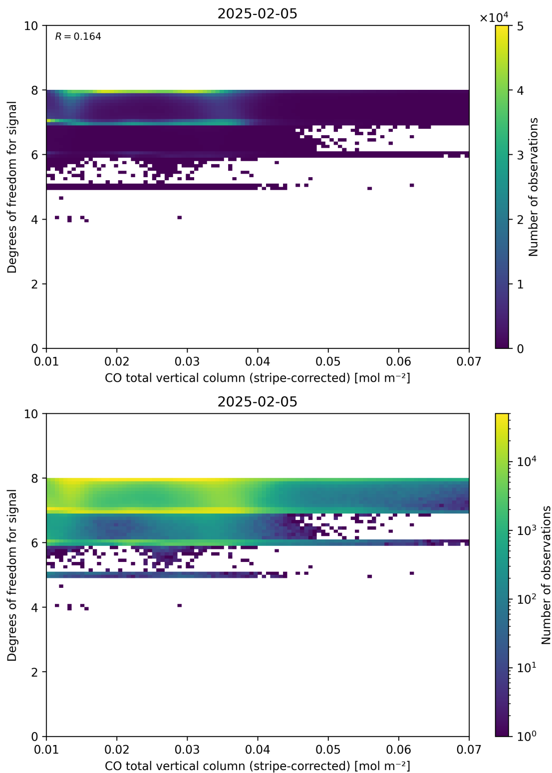
Figure 38: Scatter density plot of “CO total vertical column (stripe-corrected)” against “Degrees of freedom for signal” for 2025-02-04 to 2025-02-06.
