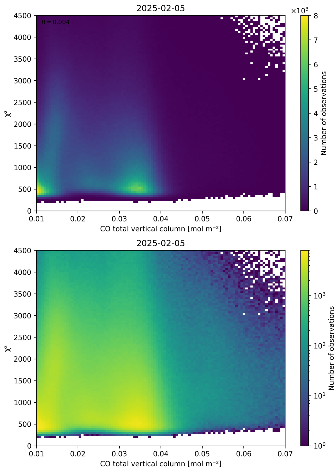
Figure 35: Scatter density plot of “CO total vertical column” against “ \chi^2 ” for 2025-02-04 to 2025-02-06.
