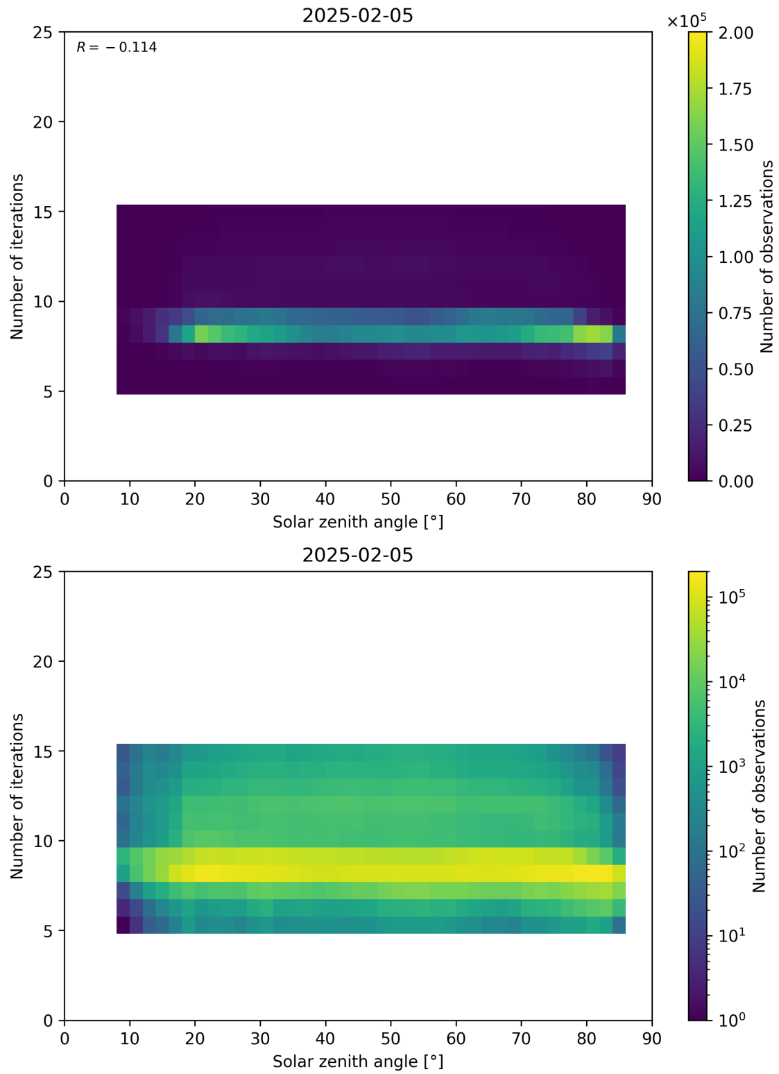
Figure 67: Scatter density plot of “Solar zenith angle” against “Number of iterations” for 2025-02-04 to 2025-02-06.
