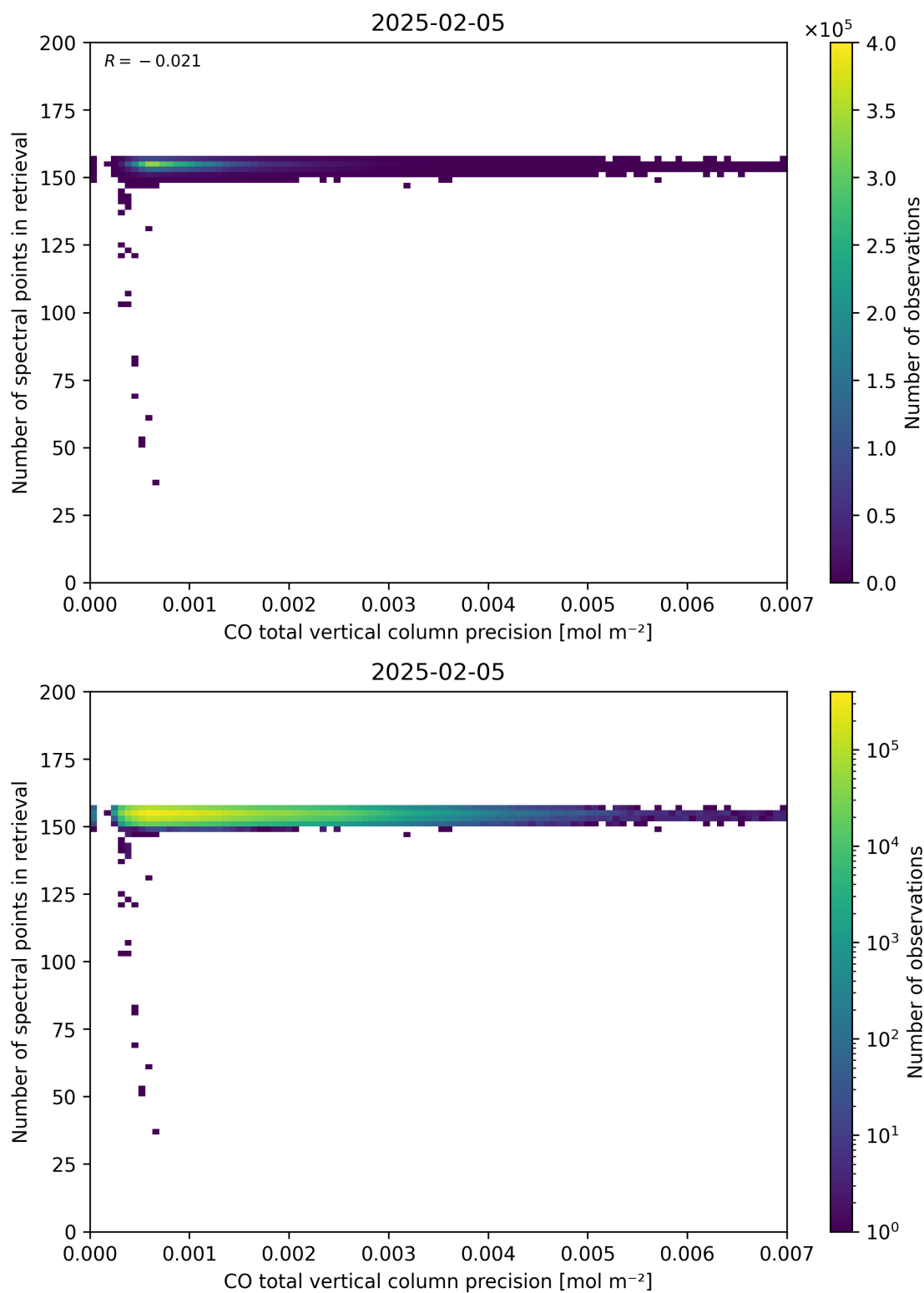
Figure 47: Scatter density plot of “CO total vertical column precision” against “Number of spectral points in retrieval” for 2025-02-04 to 2025-02-06.
