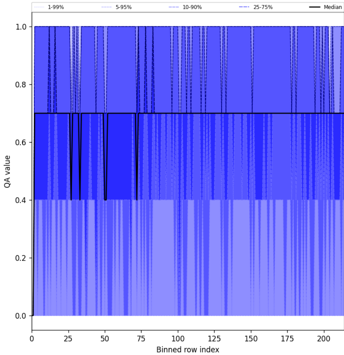
Figure 25: Along track statistics of “QA value” for 2025-02-04 to 2025-02-06
