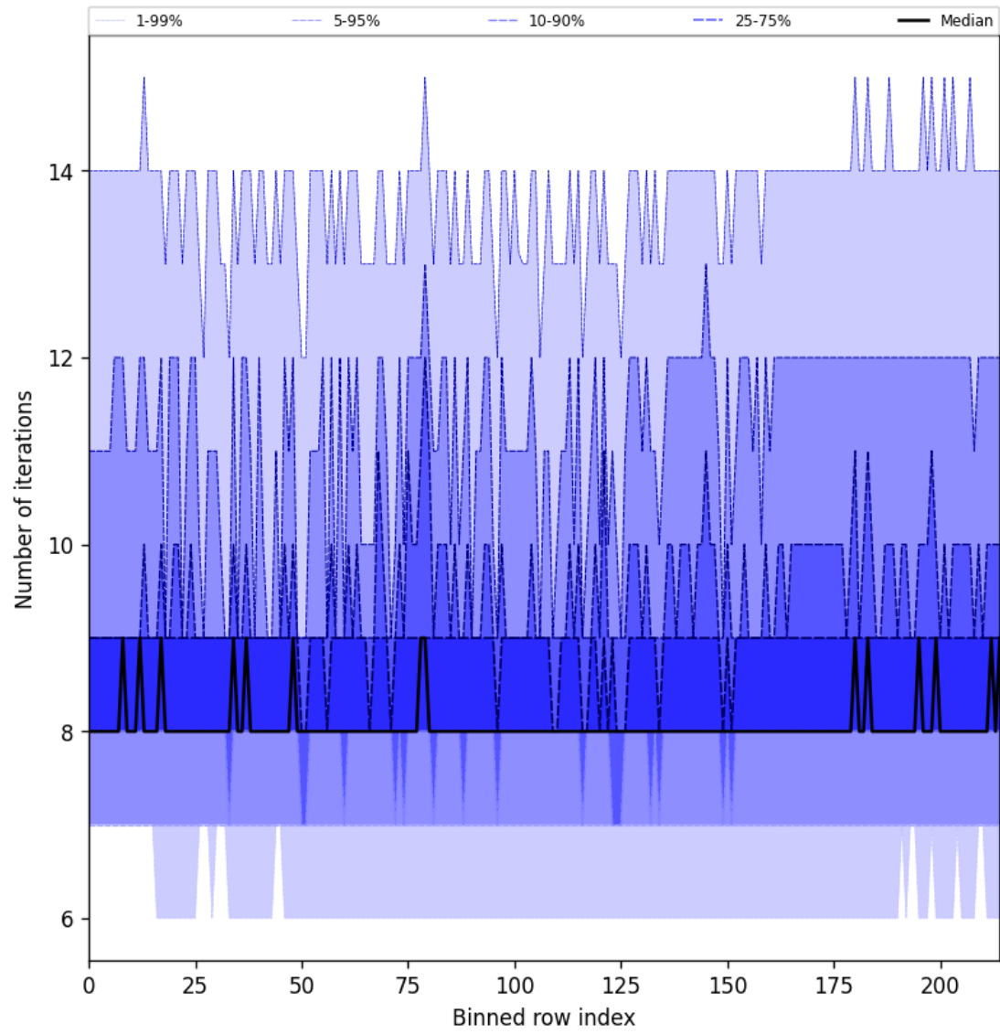
Figure 32: Along track statistics of “Number of iterations” for 2025-02-04 to 2025-02-06
