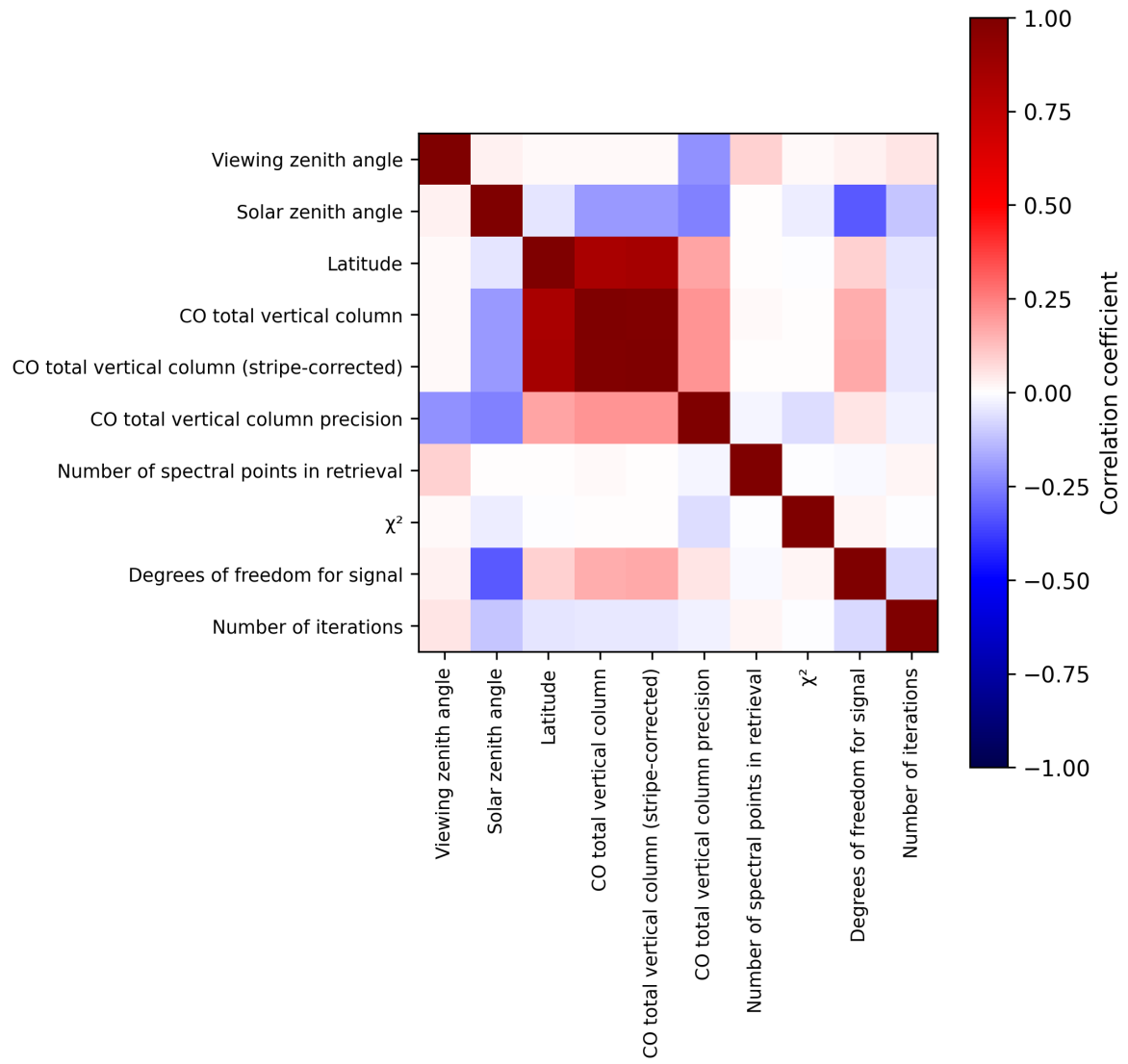
Figure 2: Map of correlation matrix for 2025-02-04 to 2025-02-06.
