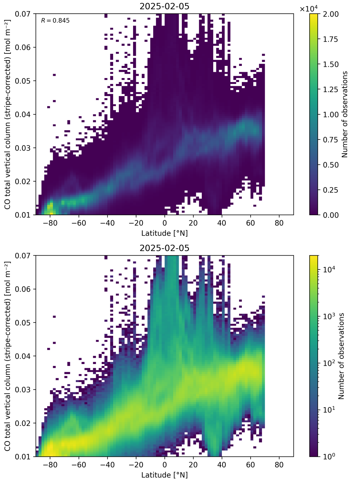
Figure 52: Scatter density plot of “Latitude” against “CO total vertical column (stripe-corrected)” for 2025-02-04 to 2025-02-06.
