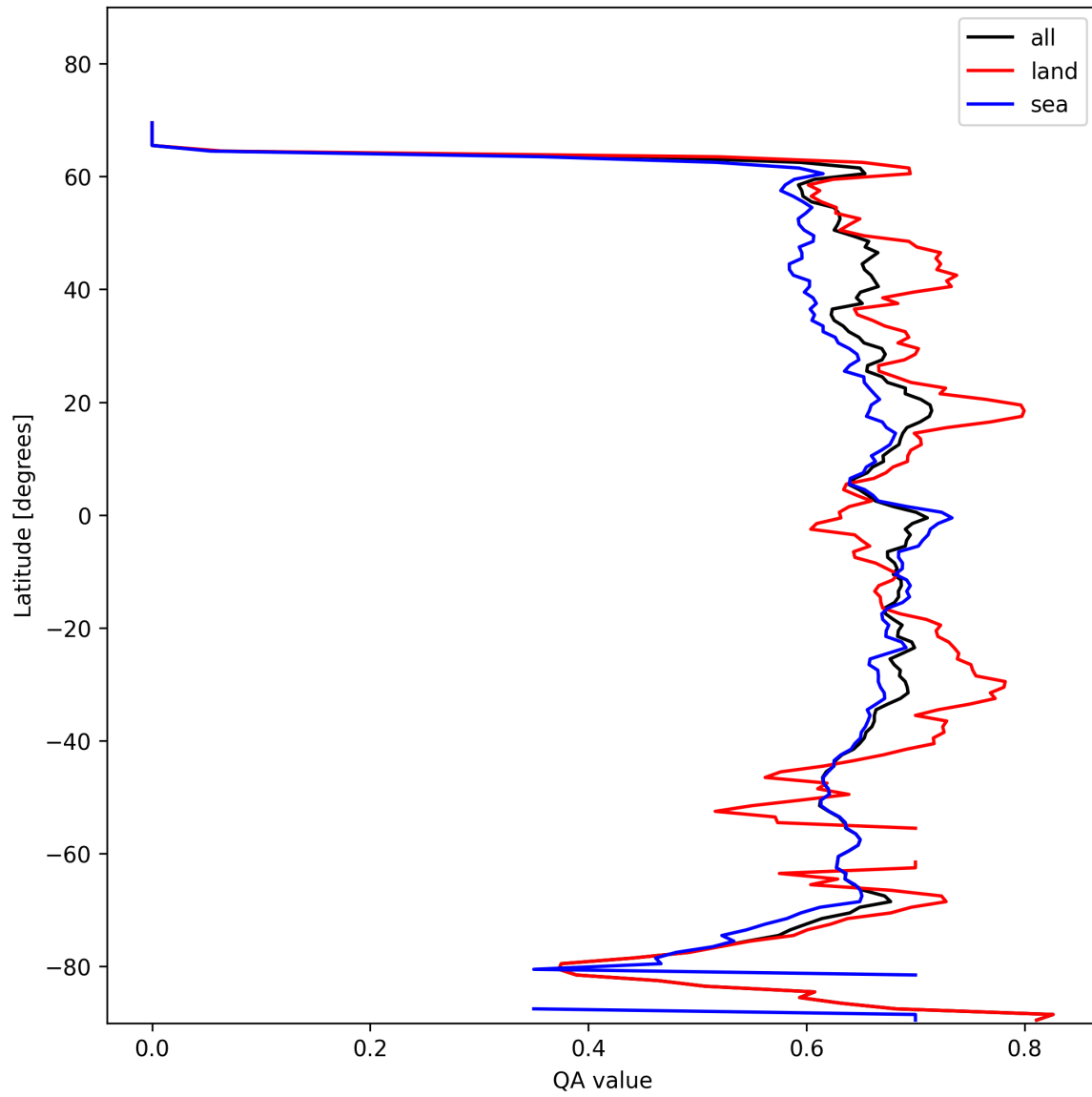
Figure 9: Zonal average of “QA value” for 2025-02-04 to 2025-02-06.
