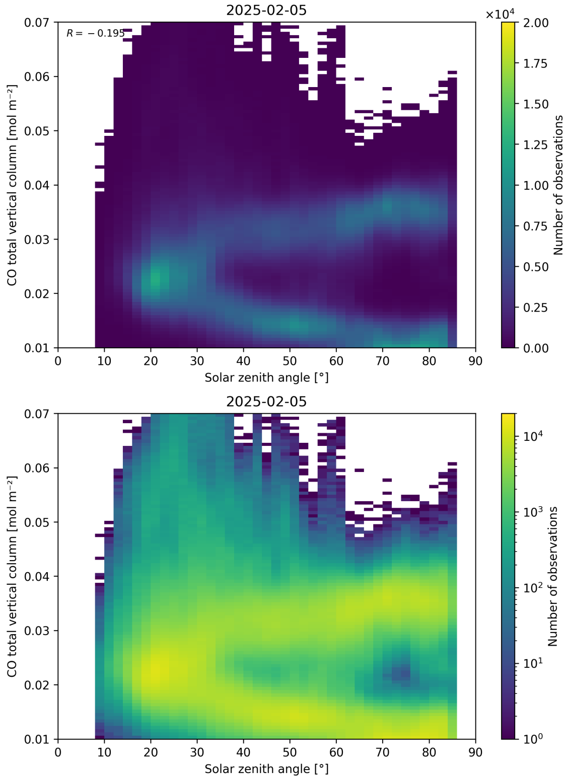
Figure 61: Scatter density plot of “Solar zenith angle” against “CO total vertical column” for 2025-02-04 to 2025-02-06.
