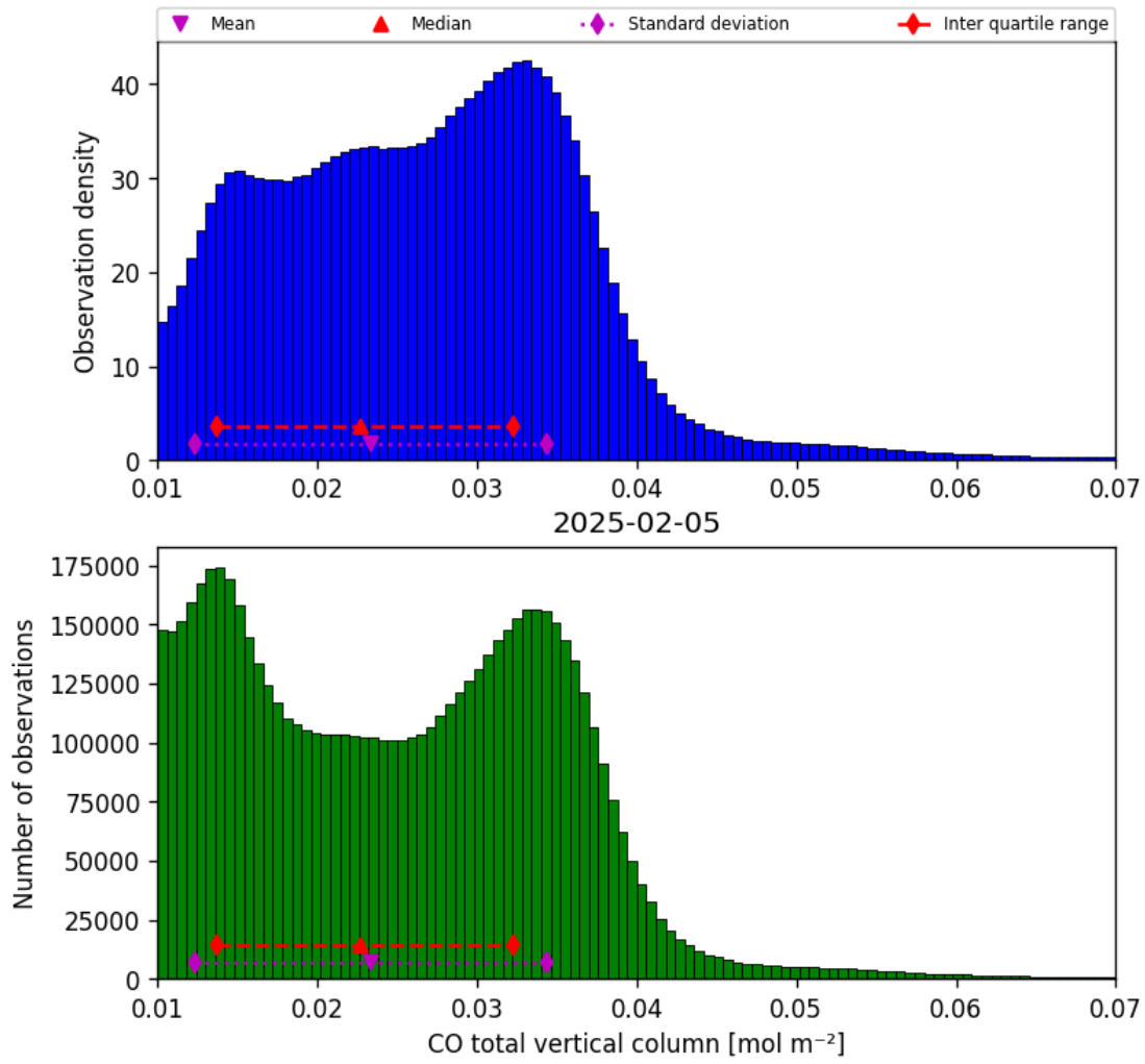
Figure 18: Histogram of “CO total vertical column” for 2025-02-04 to 2025-02-06
