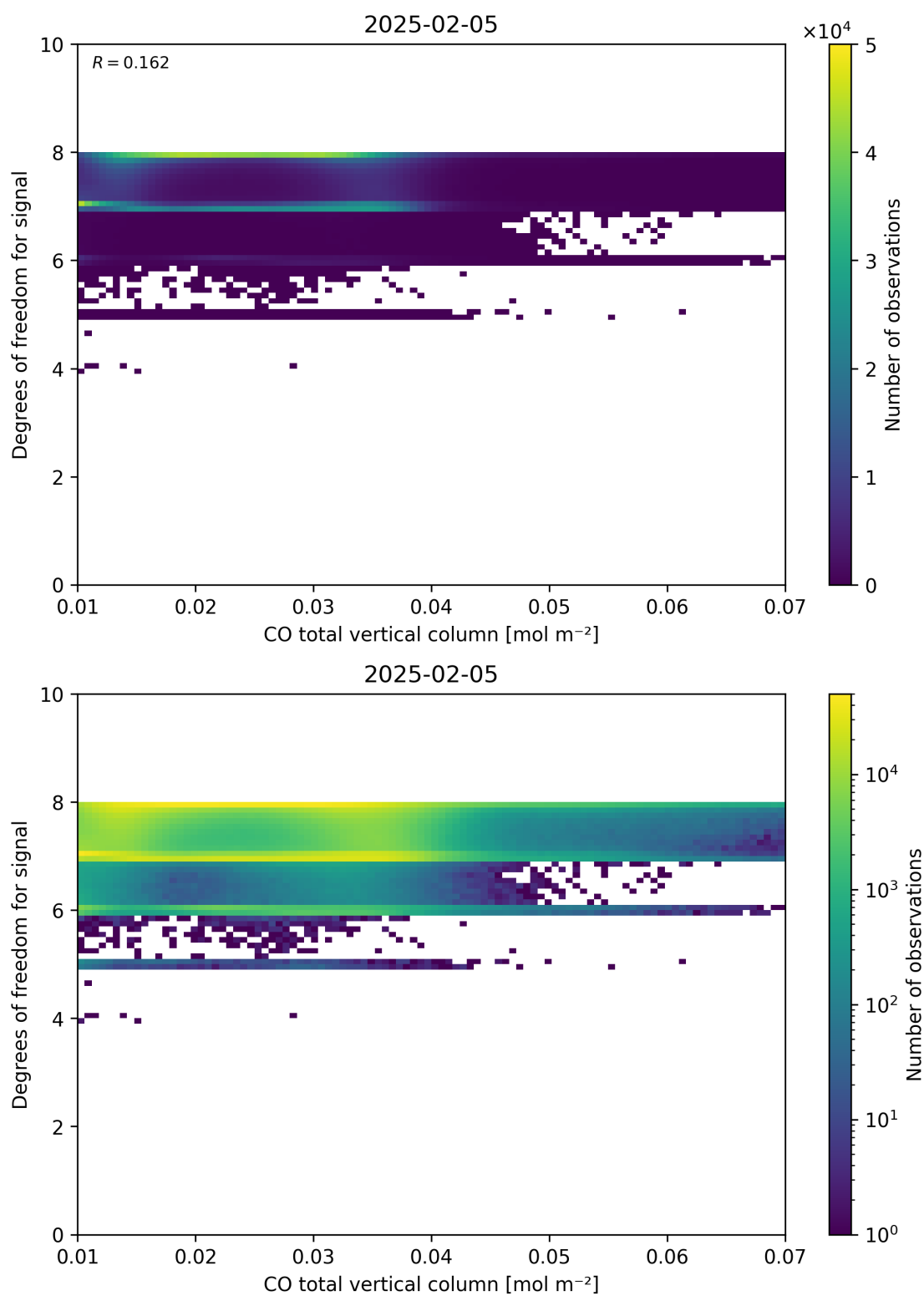
Figure 41: Scatter density plot of “CO total vertical column” against “Degrees of freedom for signal” for 2025-02-04 to 2025-02-06.
