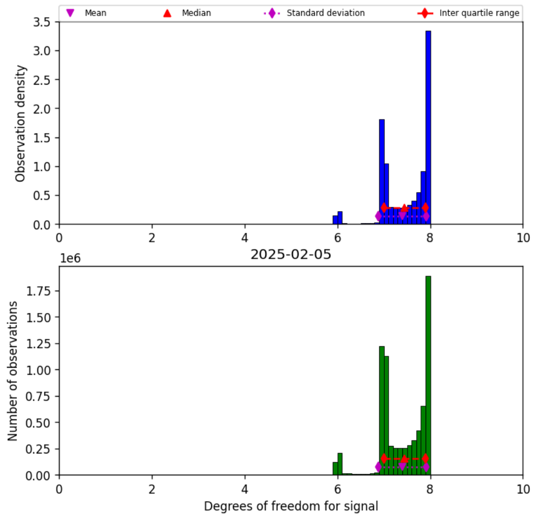
Figure 23: Histogram of “Degrees of freedom for signal” for 2025-02-04 to 2025-02-06
