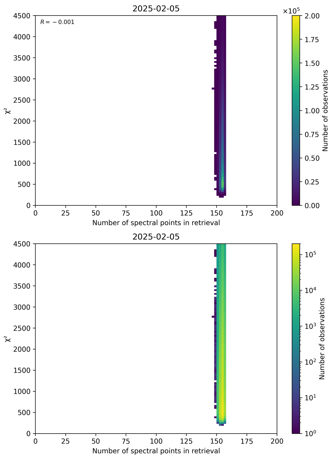
Figure 58: Scatter density plot of “Number of spectral points in retrieval” against “ \chi^2 ” for 2025-02-04 to 2025-02-06.
