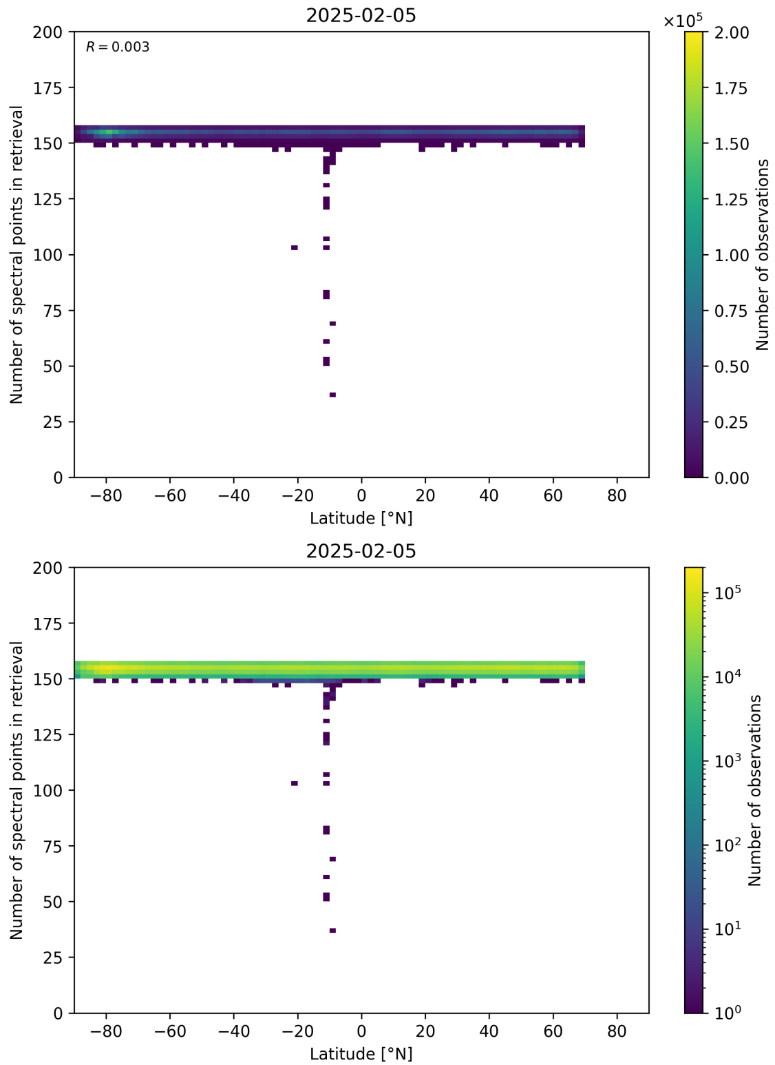
Figure 57: Scatter density plot of “Latitude” against “Number of spectral points in retrieval” for 2025-02-04 to 2025-02-06.
