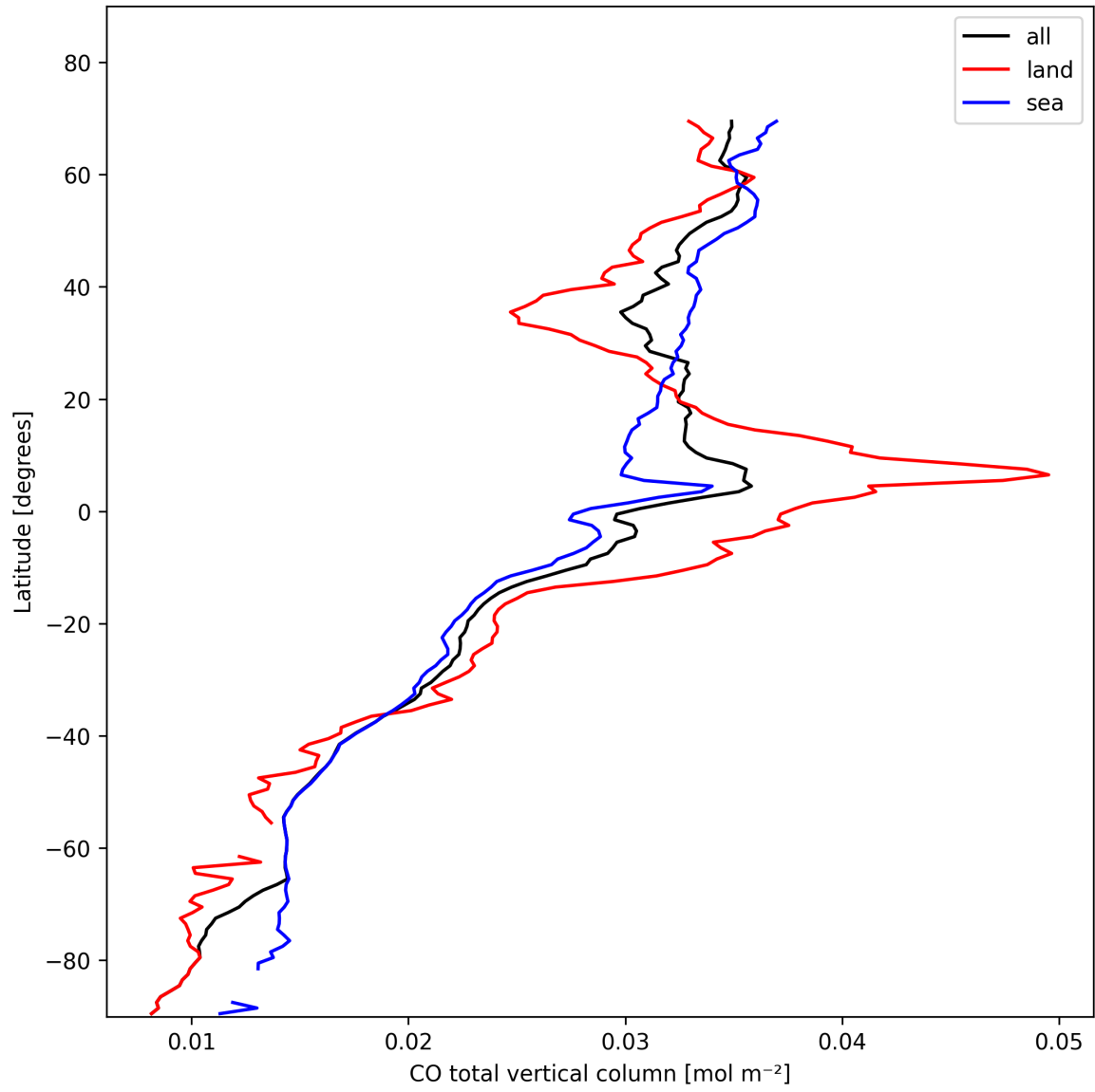
Figure 10: Zonal average of “CO total vertical column” for 2025-02-04 to 2025-02-06.
