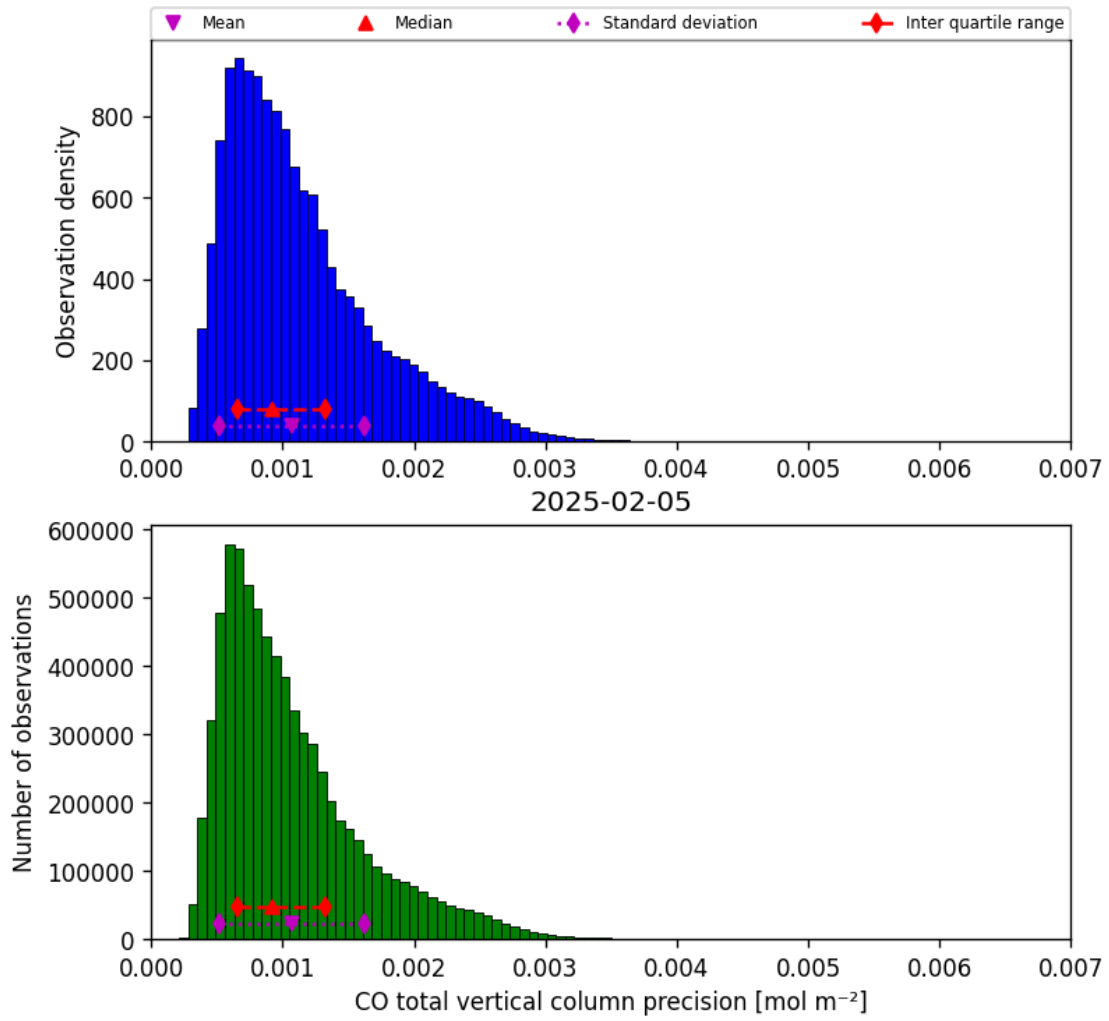
Figure 20: Histogram of “CO total vertical column precision” for 2025-02-04 to 2025-02-06
