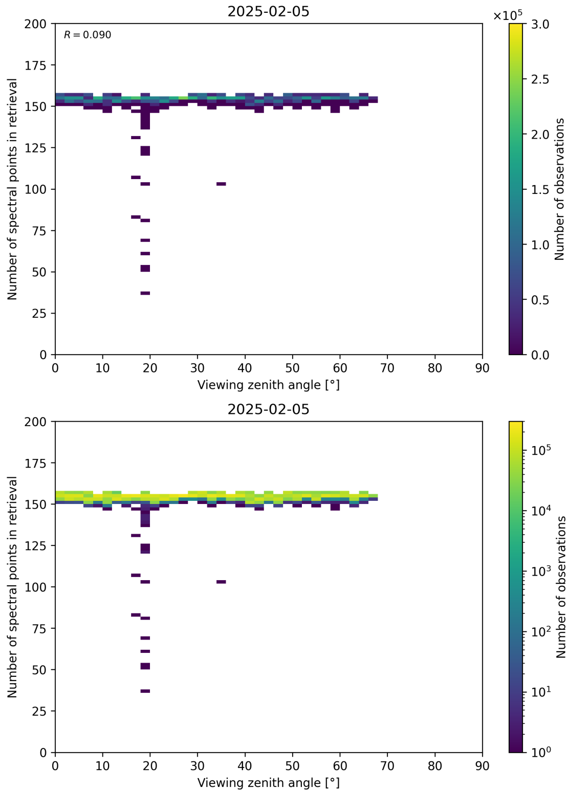
Figure 76: Scatter density plot of “Viewing zenith angle” against “Number of spectral points in retrieval” for 2025-02-04 to 2025-02-06.
