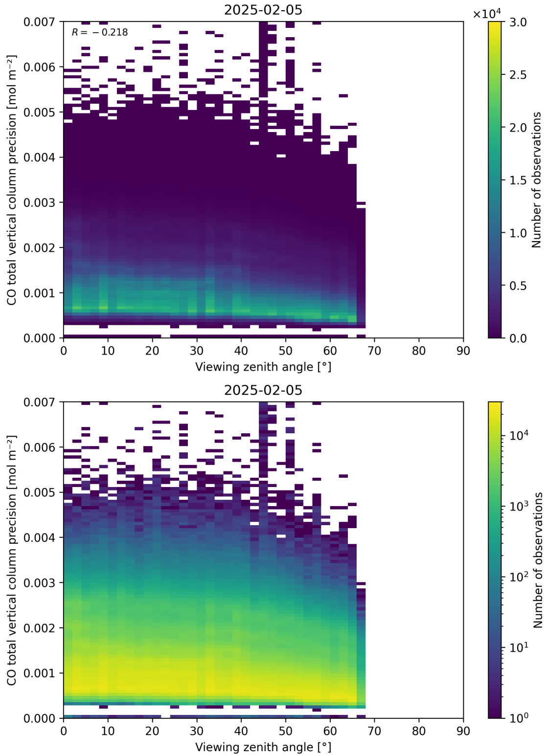
Figure 71: Scatter density plot of “Viewing zenith angle” against “CO total vertical column precision” for 2025-02-04 to 2025-02-06.
