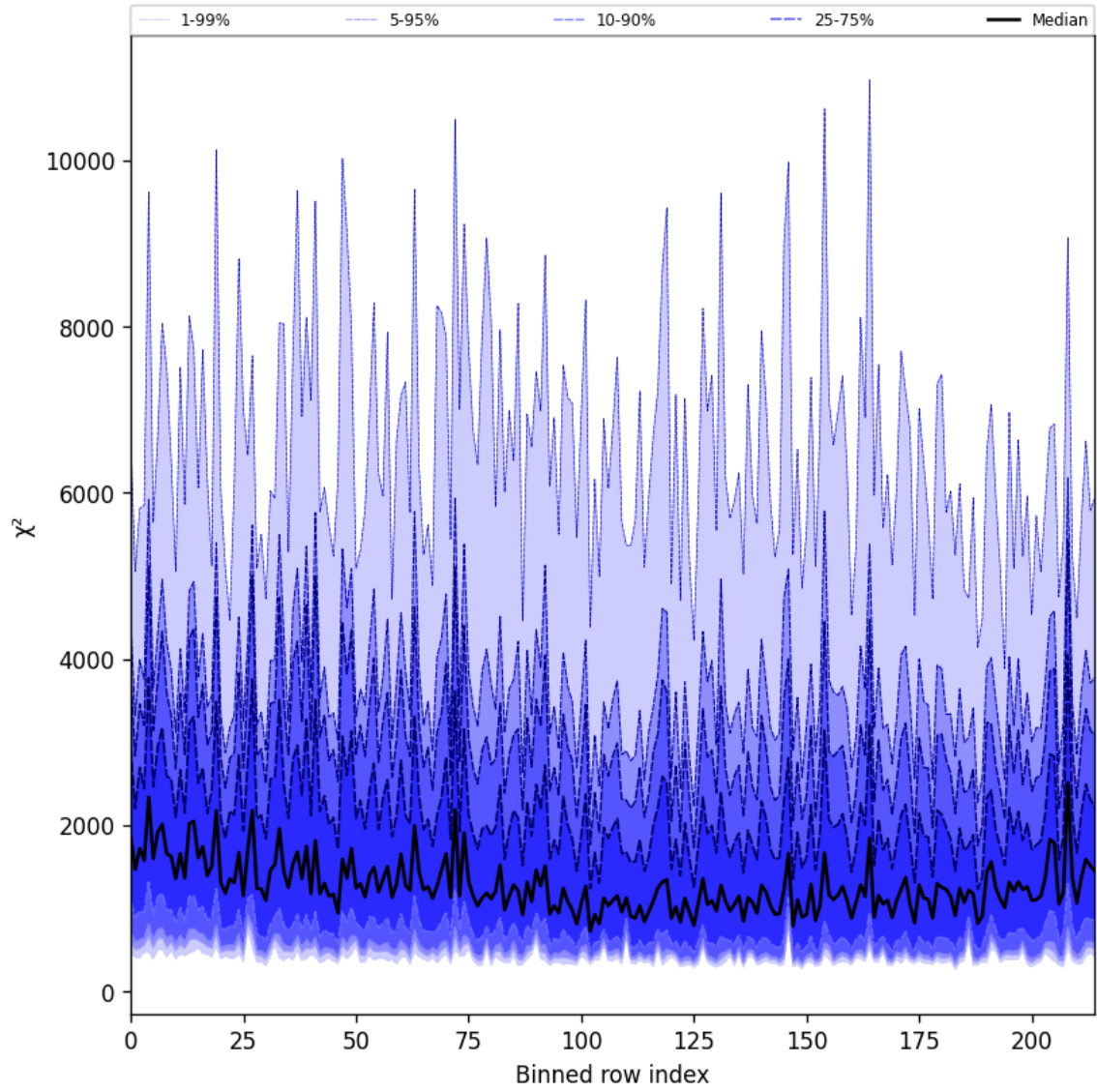
Figure 30: Along track statistics of “ \chi^2 ” for 2025-02-04 to 2025-02-06
