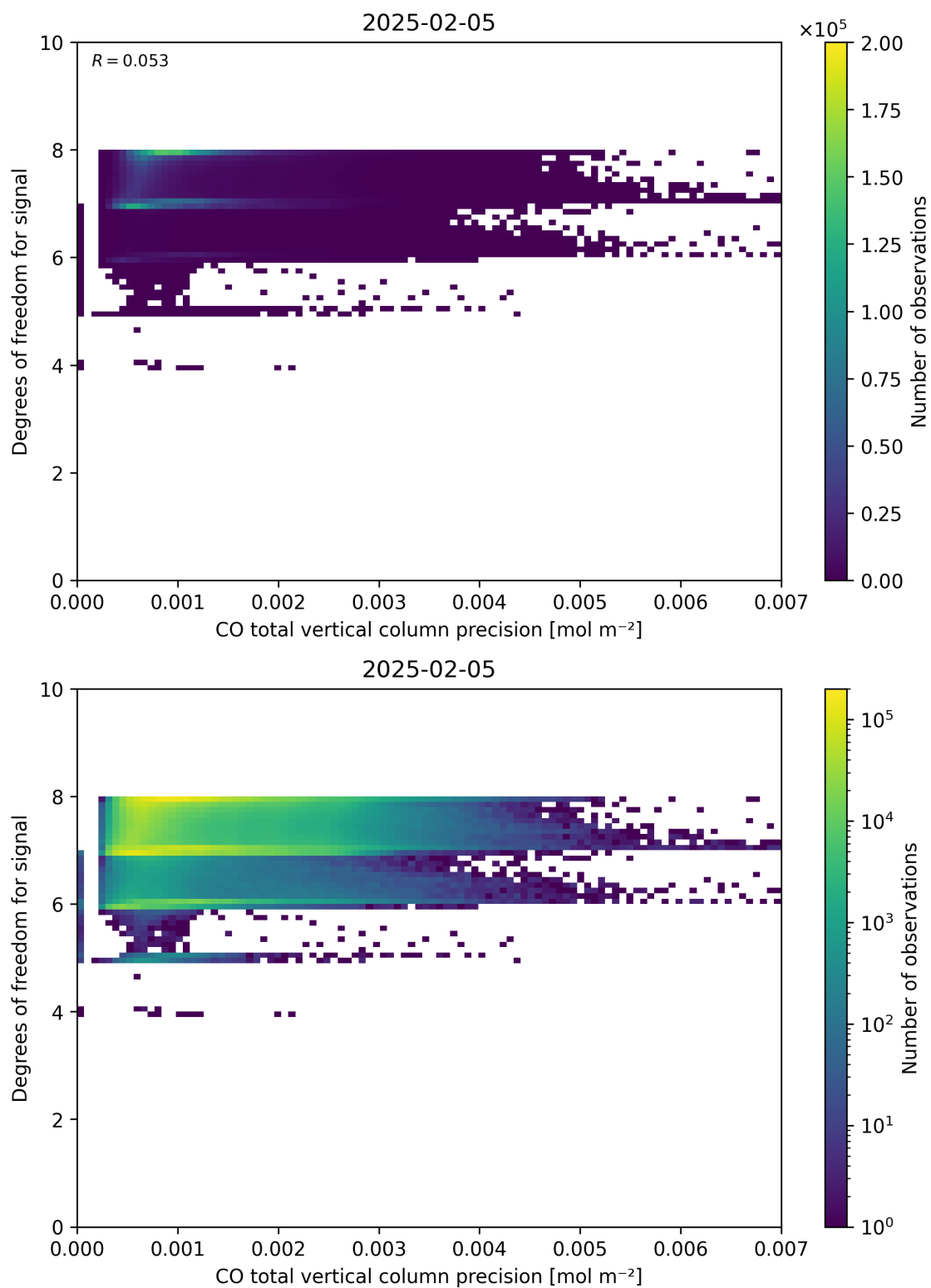
Figure 45: Scatter density plot of “CO total vertical column precision” against “Degrees of freedom for signal” for 2025-02-04 to 2025-02-06.
