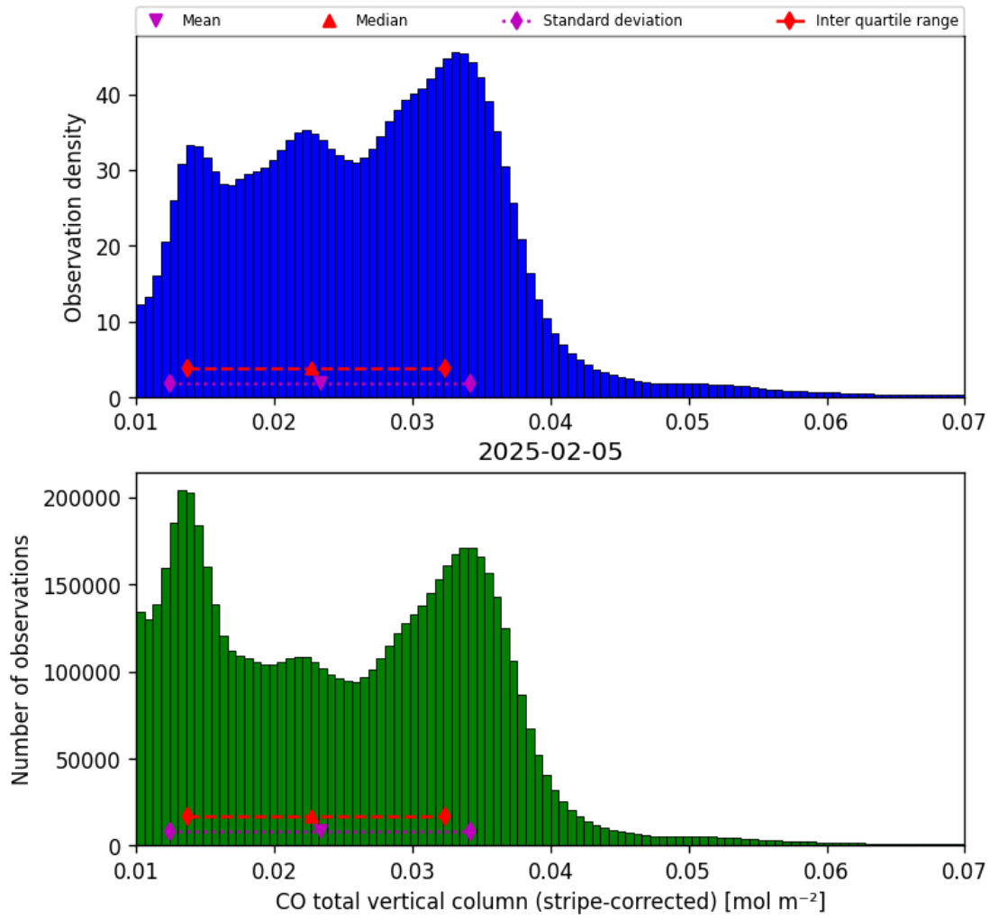
Figure 19: Histogram of “CO total vertical column (stripe-corrected)” for 2025-02-04 to 2025-02-06
