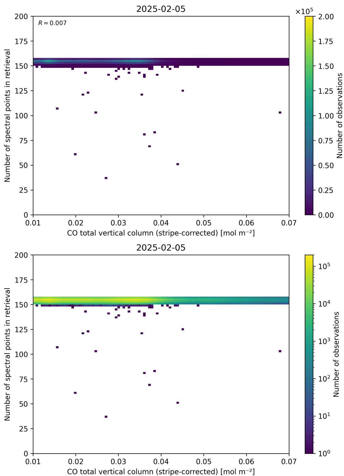
Figure 40: Scatter density plot of “CO total vertical column (stripe-corrected)” against “Number of spectral points in retrieval” for 2025-02-04 to 2025-02-06.
