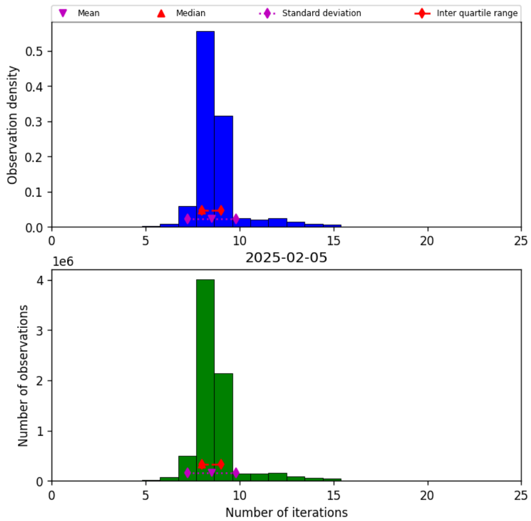
Figure 24: Histogram of “Number of iterations” for 2025-02-04 to 2025-02-06
