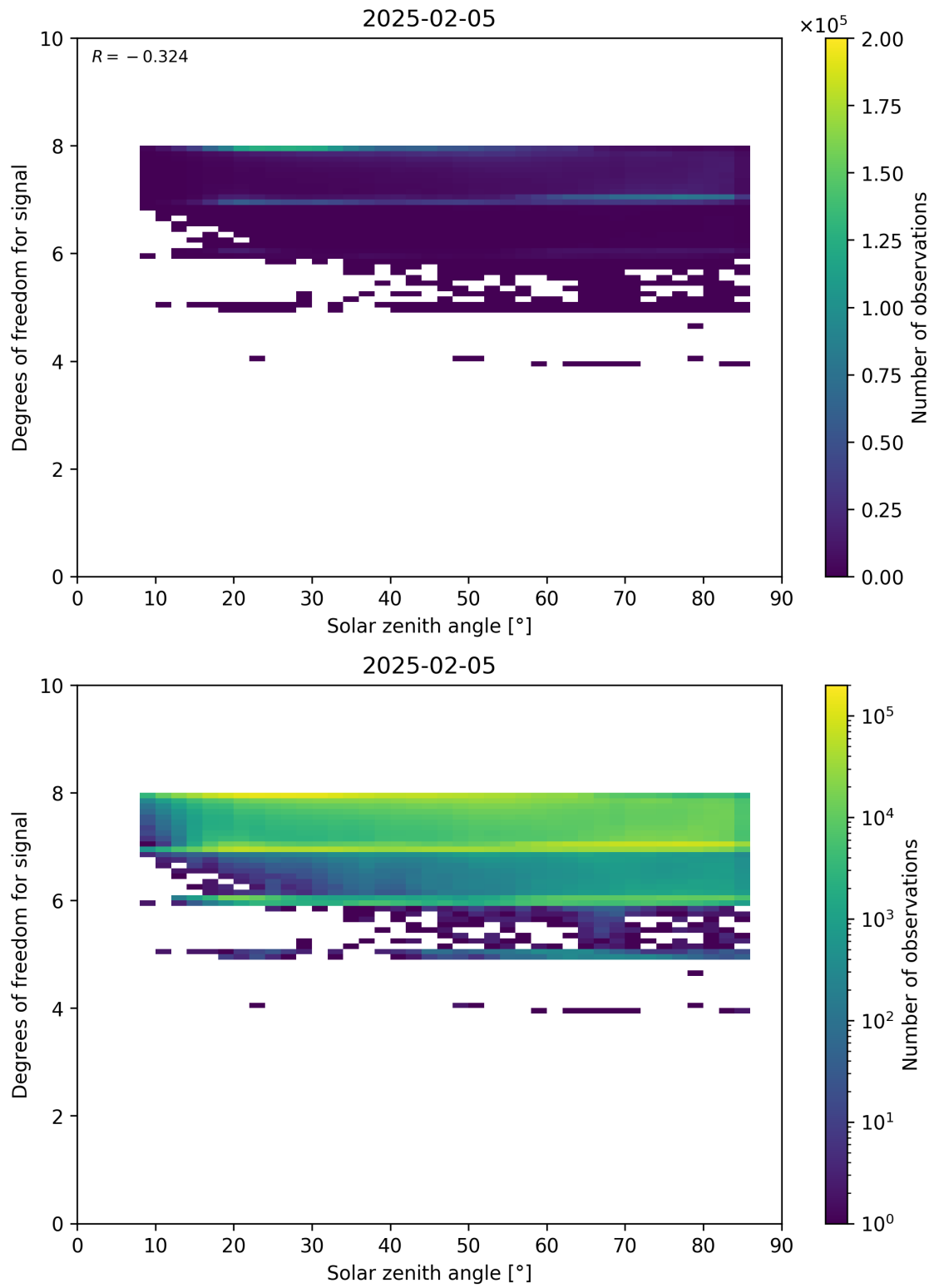
Figure 65: Scatter density plot of “Solar zenith angle” against “Degrees of freedom for signal” for 2025-02-04 to 2025-02-06.
