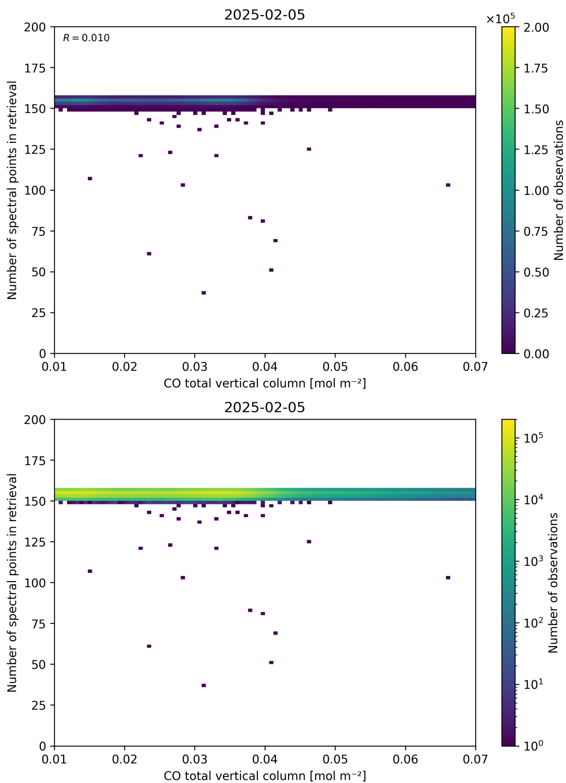
Figure 43: Scatter density plot of “CO total vertical column” against “Number of spectral points in retrieval” for 2025-02-04 to 2025-02-06.
