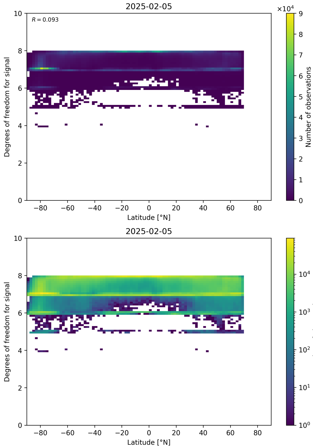
Figure 55: Scatter density plot of “Latitude” against “Degrees of freedom for signal” for 2025-02-04 to 2025-02-06.
