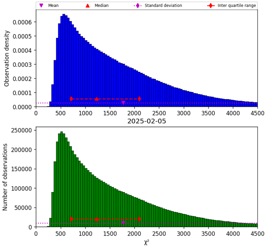
Figure 22: Histogram of “ \chi^2 ” for 2025-02-04 to 2025-02-06
