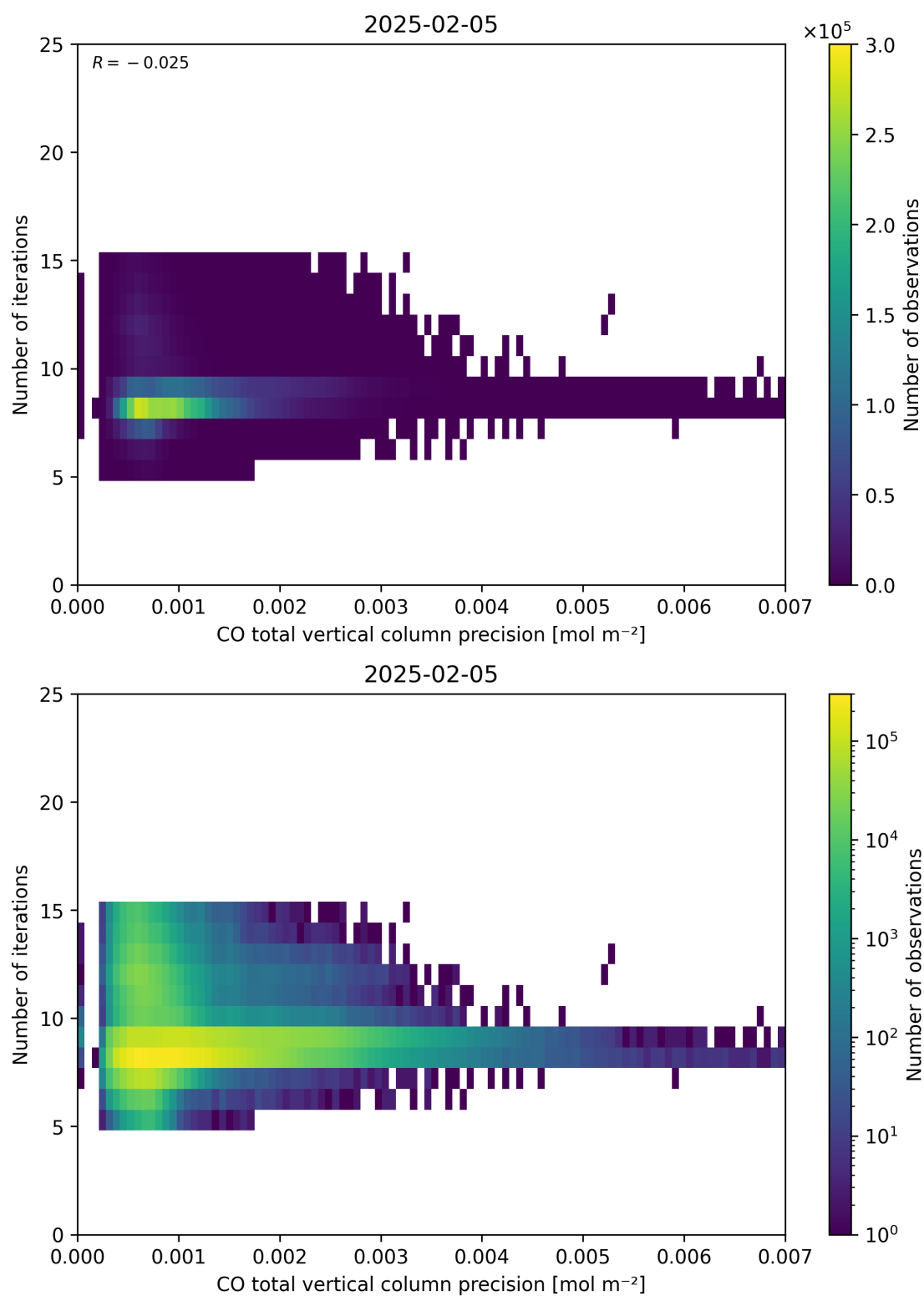
Figure 46: Scatter density plot of “CO total vertical column precision” against “Number of iterations” for 2025-02-04 to 2025-02-06.
