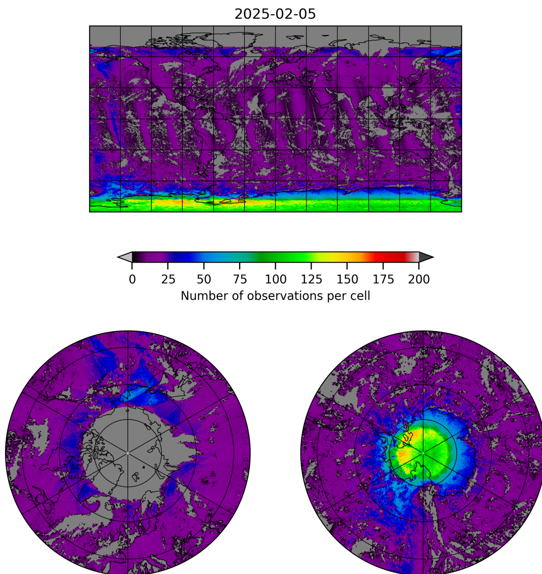
Figure 8: Map of the number of observations for 2025-02-04 to 2025-02-06
