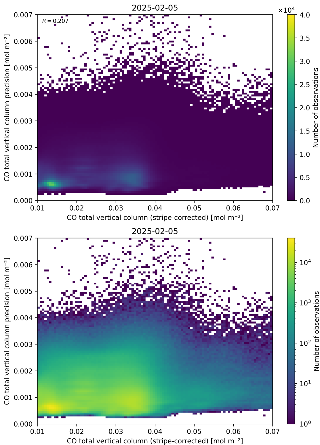
Figure 36: Scatter density plot of “CO total vertical column (stripe-corrected)” against “CO total vertical column precision” for 2025-02-04 to 2025-02-06.
