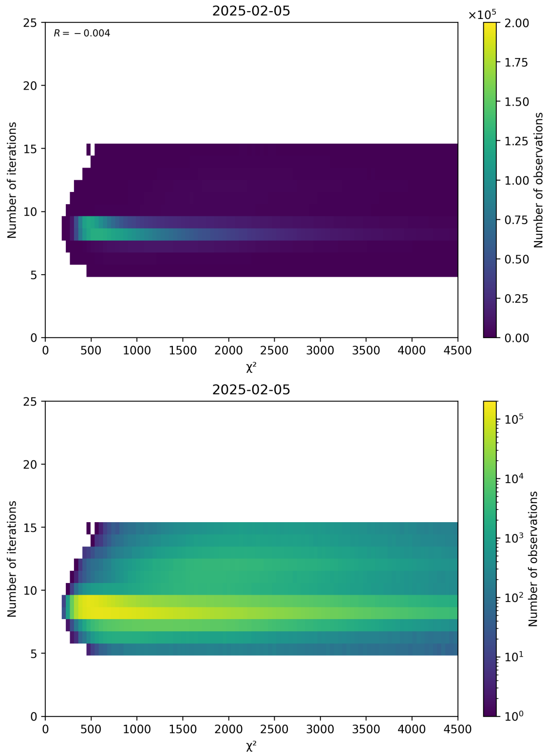
Figure 49: Scatter density plot of “ \chi^2 ” against “Number of iterations” for 2025-02-04 to 2025-02-06.
