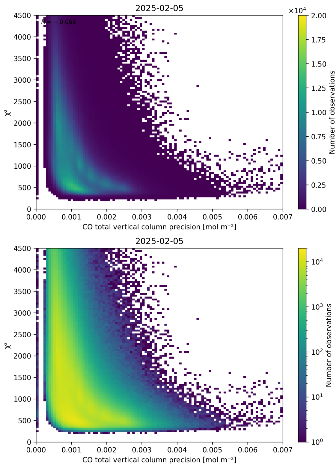
Figure 44: Scatter density plot of “CO total vertical column precision” against “ \chi^2 ” for 2025-02-04 to 2025-02-06.
