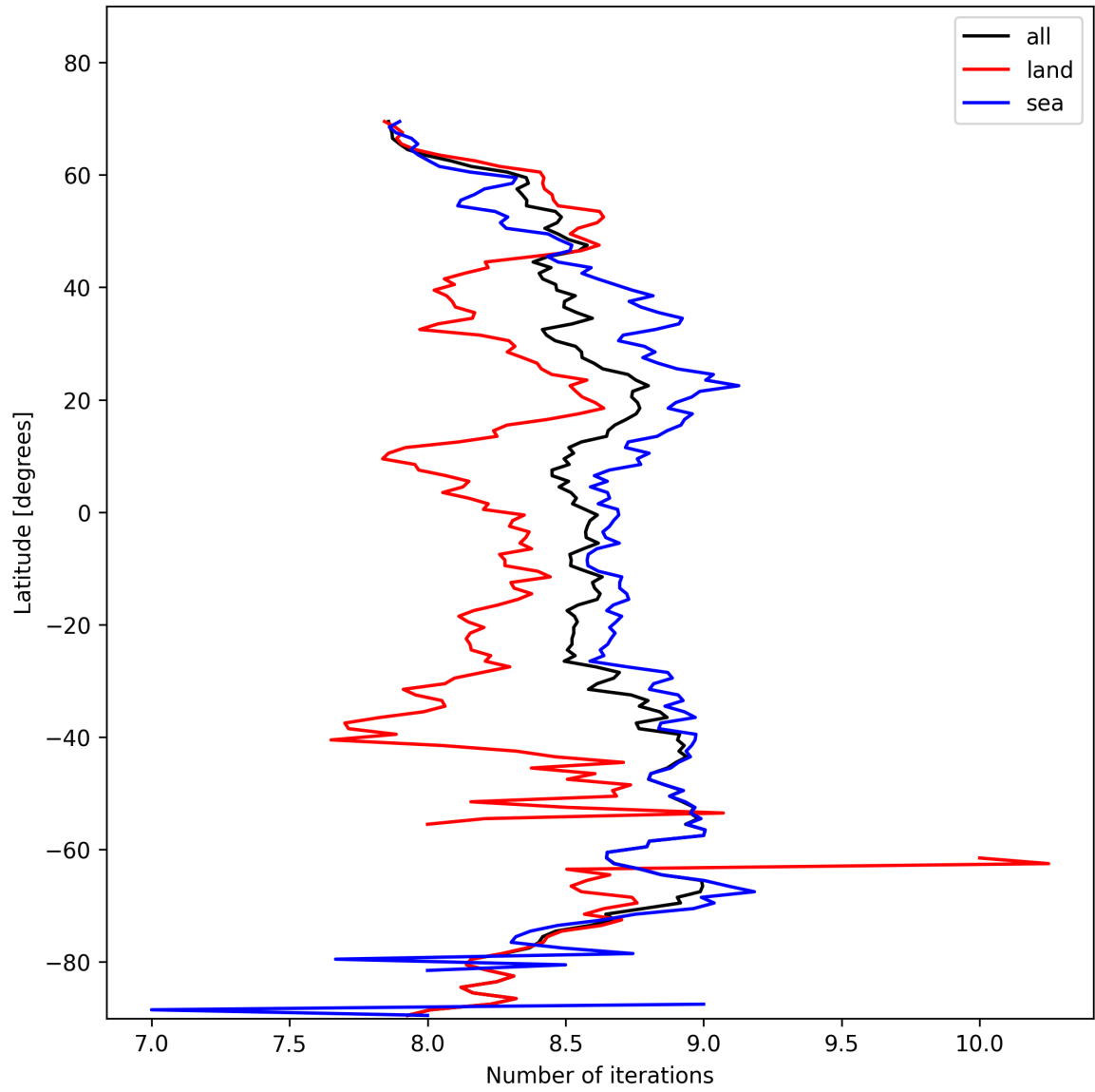
Figure 16: Zonal average of “Number of iterations” for 2025-02-04 to 2025-02-06.
