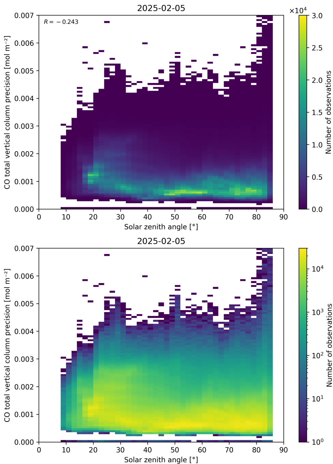
Figure 63: Scatter density plot of “Solar zenith angle” against “CO total vertical column precision” for 2025-02-04 to 2025-02-06.
