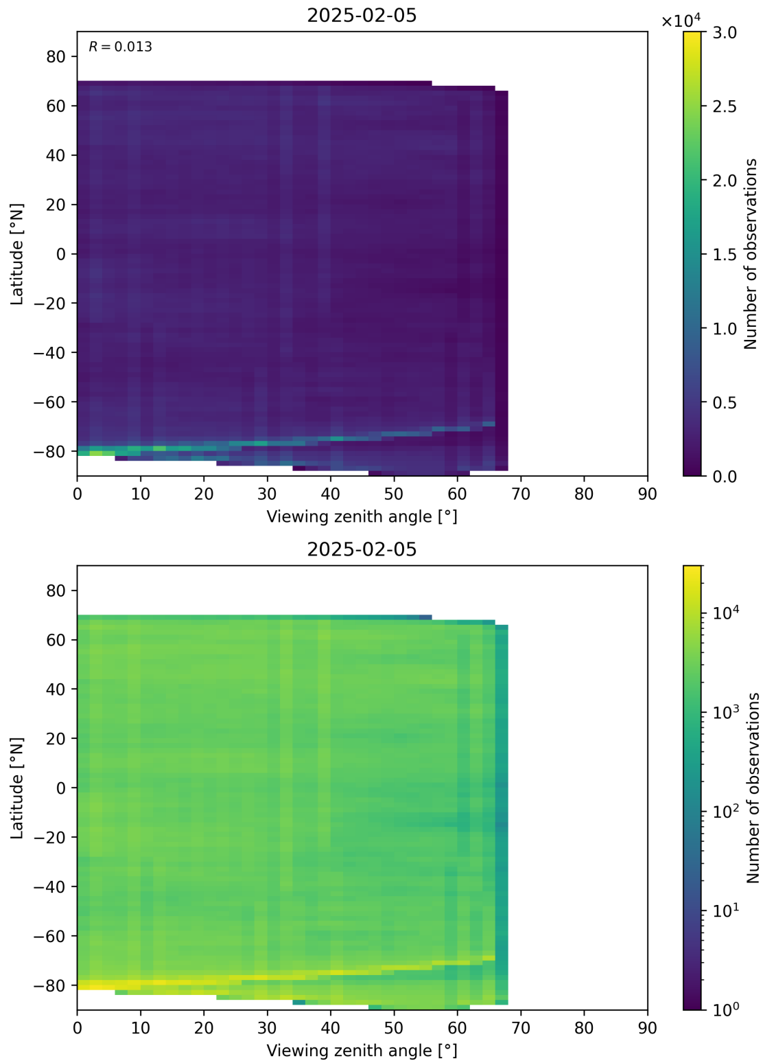
Figure 74: Scatter density plot of “Viewing zenith angle” against “Latitude” for 2025-02-04 to 2025-02-06.
