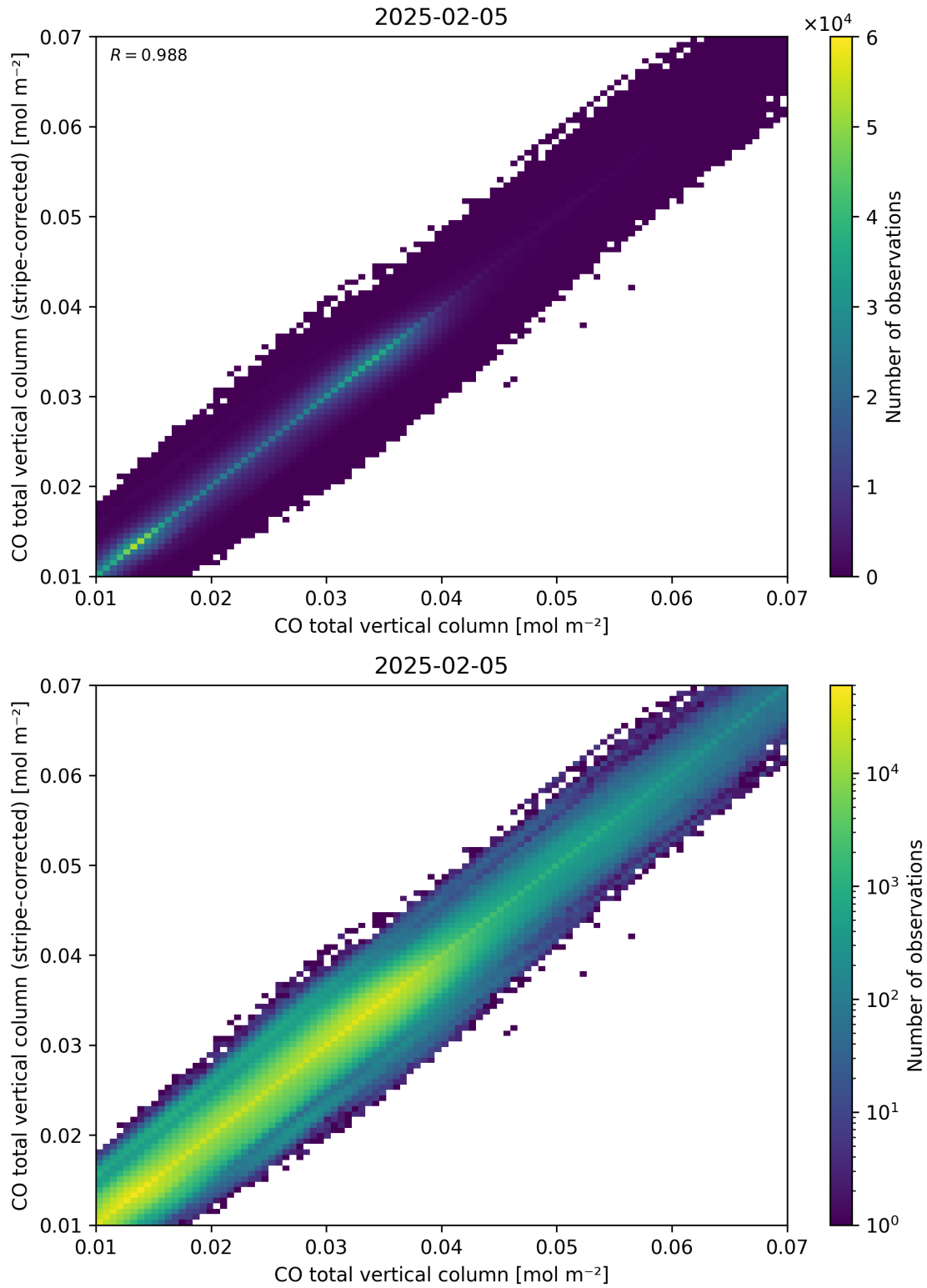
Figure 33: Scatter density plot of “CO total vertical column” against “CO total vertical column (stripe-corrected)” for 2025-02-04 to 2025-02-06.
