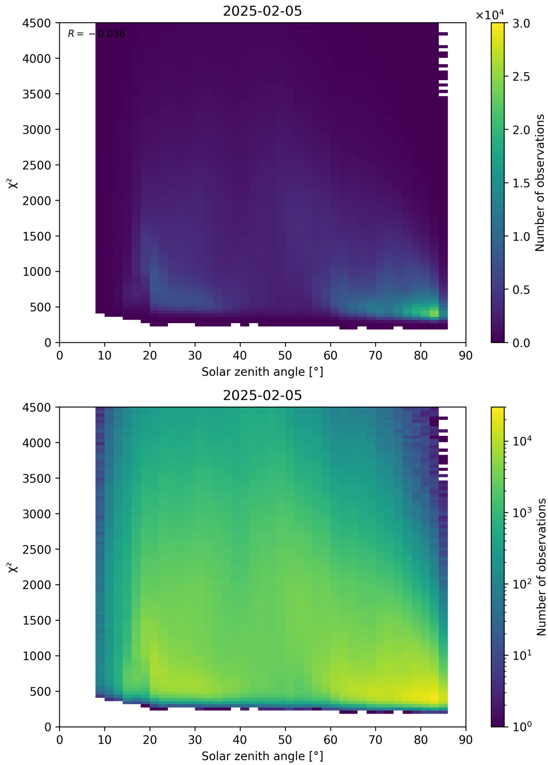
Figure 64: Scatter density plot of “Solar zenith angle” against “ \chi^2 ” for 2025-02-04 to 2025-02-06.
