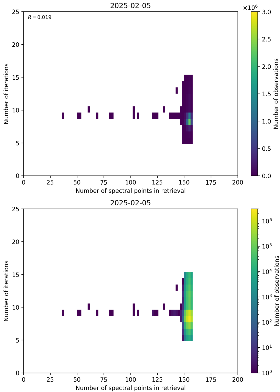
Figure 60: Scatter density plot of “Number of spectral points in retrieval” against “Number of iterations” for 2025-02-04 to 2025-02-06.
