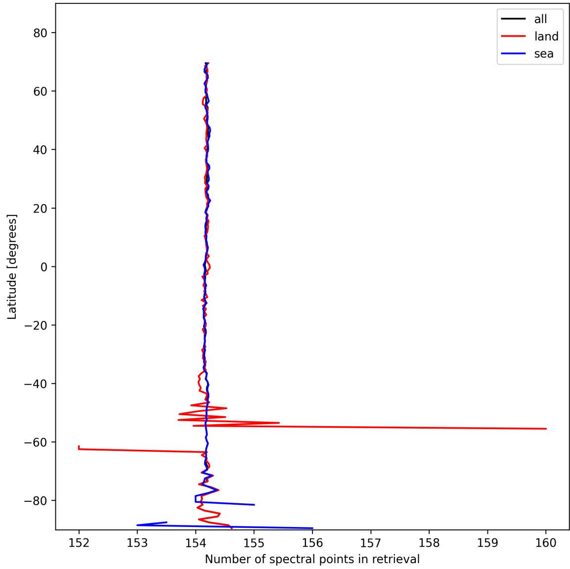
Figure 13: Zonal average of “Number of spectral points in retrieval” for 2025-02-04 to 2025-02-06.
