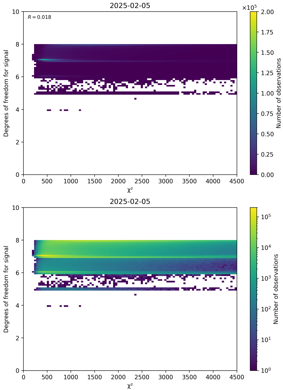
Figure 48: Scatter density plot of “ \chi^2 ” against “Degrees of freedom for signal” for 2025-02-04 to 2025-02-06.
