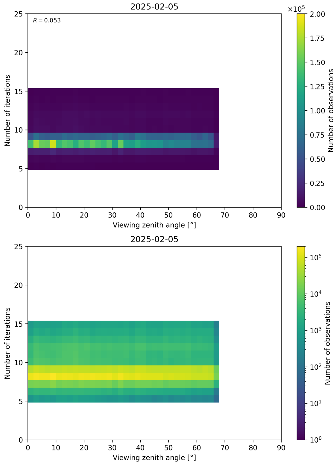
Figure 75: Scatter density plot of “Viewing zenith angle” against “Number of iterations” for 2025-02-04 to 2025-02-06.
