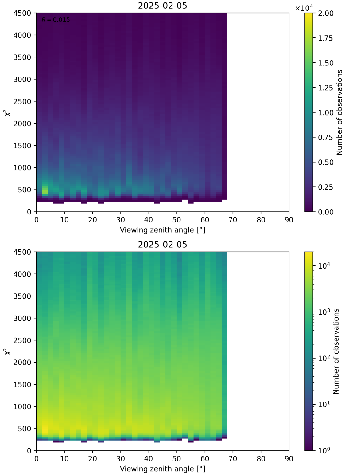
Figure 72: Scatter density plot of “Viewing zenith angle” against “ \chi^2 ” for 2025-02-04 to 2025-02-06.
