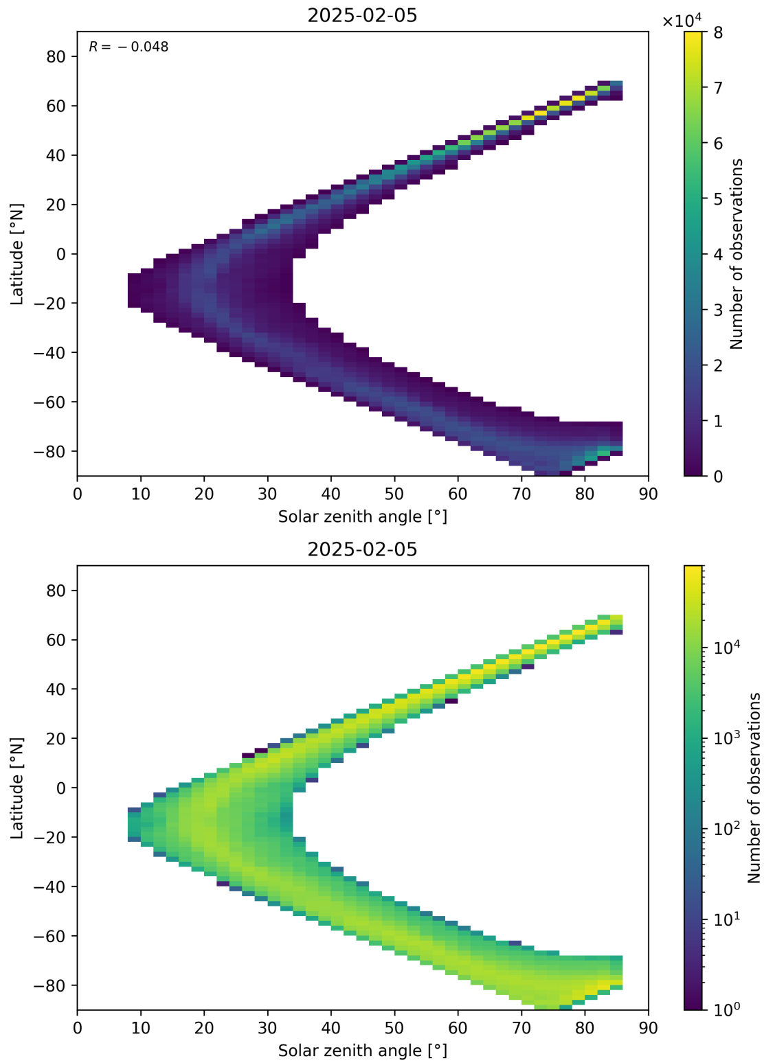
Figure 66: Scatter density plot of “Solar zenith angle” against “Latitude” for 2025-02-04 to 2025-02-06.
