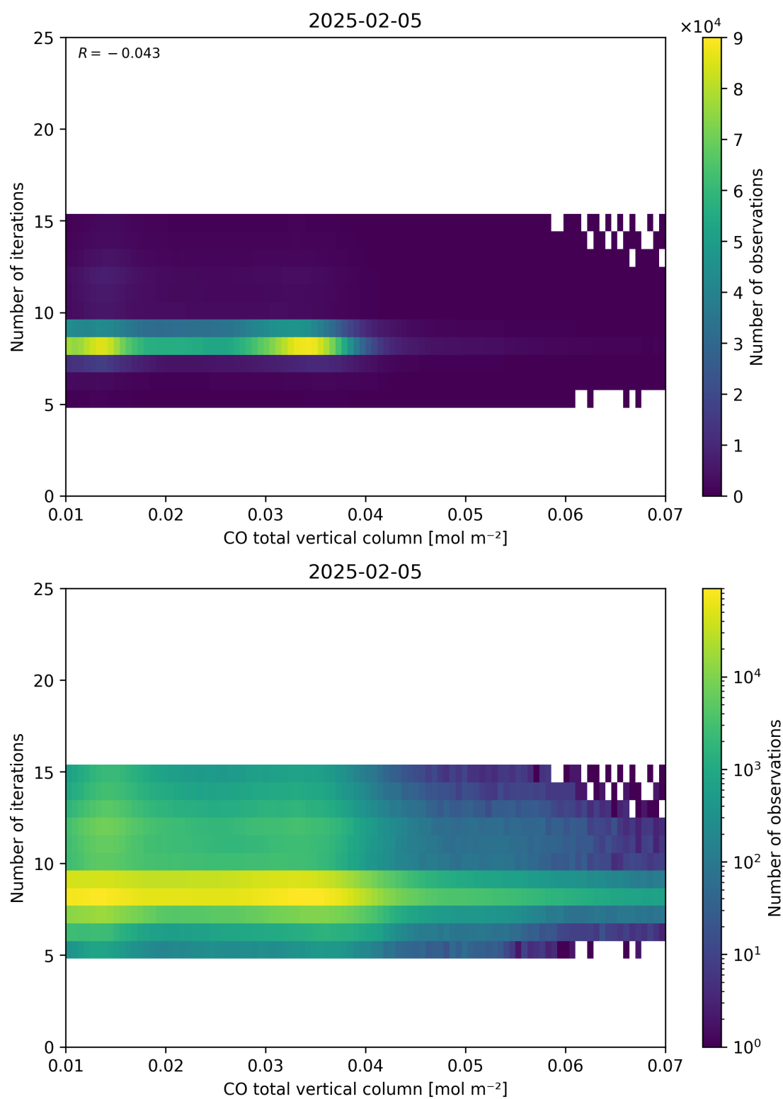
Figure 42: Scatter density plot of “CO total vertical column” against “Number of iterations” for 2025-02-04 to 2025-02-06.
