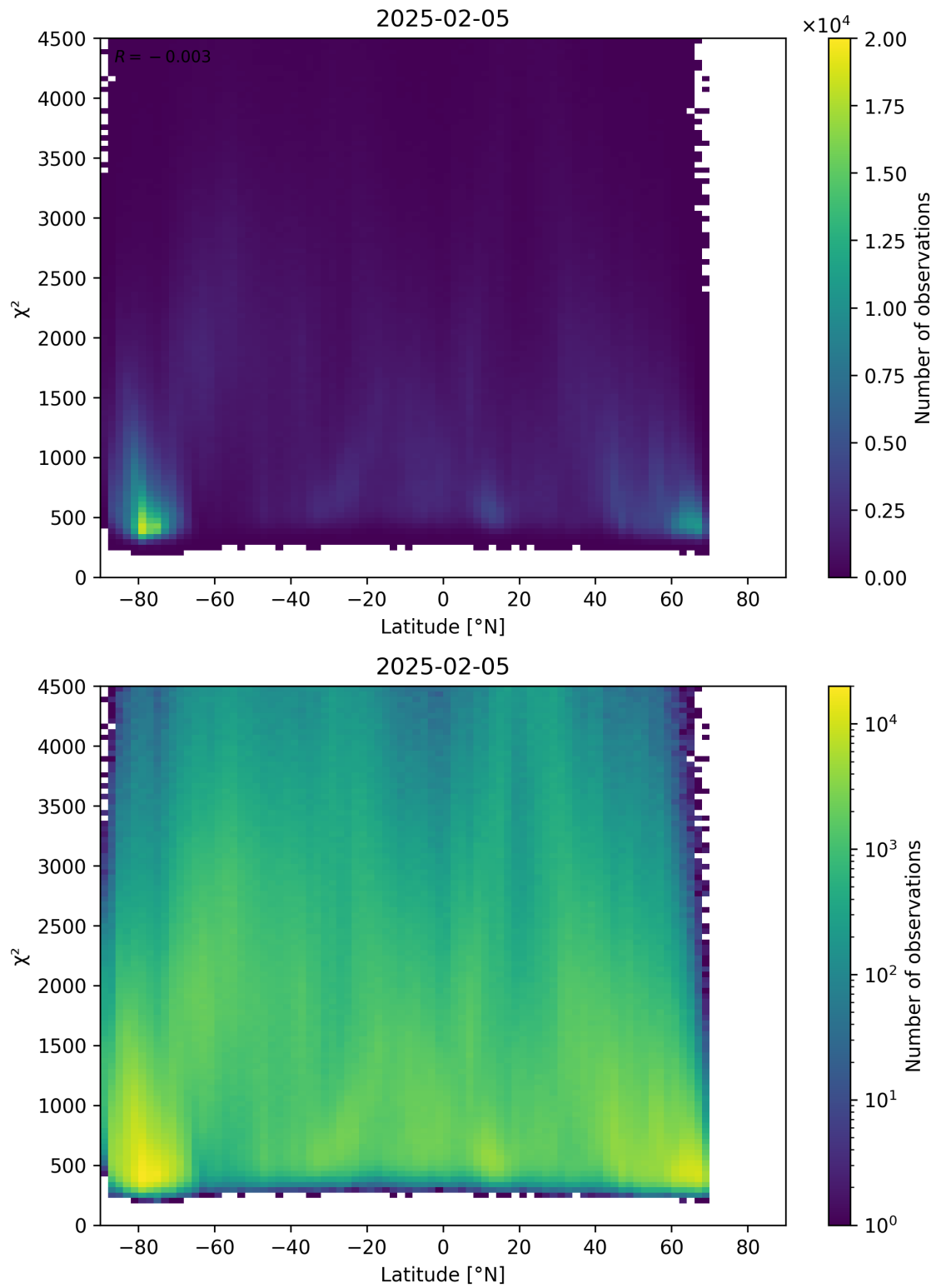
Figure 54: Scatter density plot of “Latitude” against “ \chi^2 ” for 2025-02-04 to 2025-02-06.
