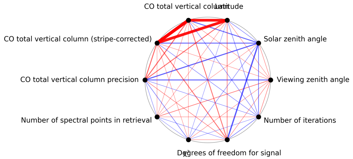
Figure 1: Map of correlation graph for 2025-02-04 to 2025-02-06.
