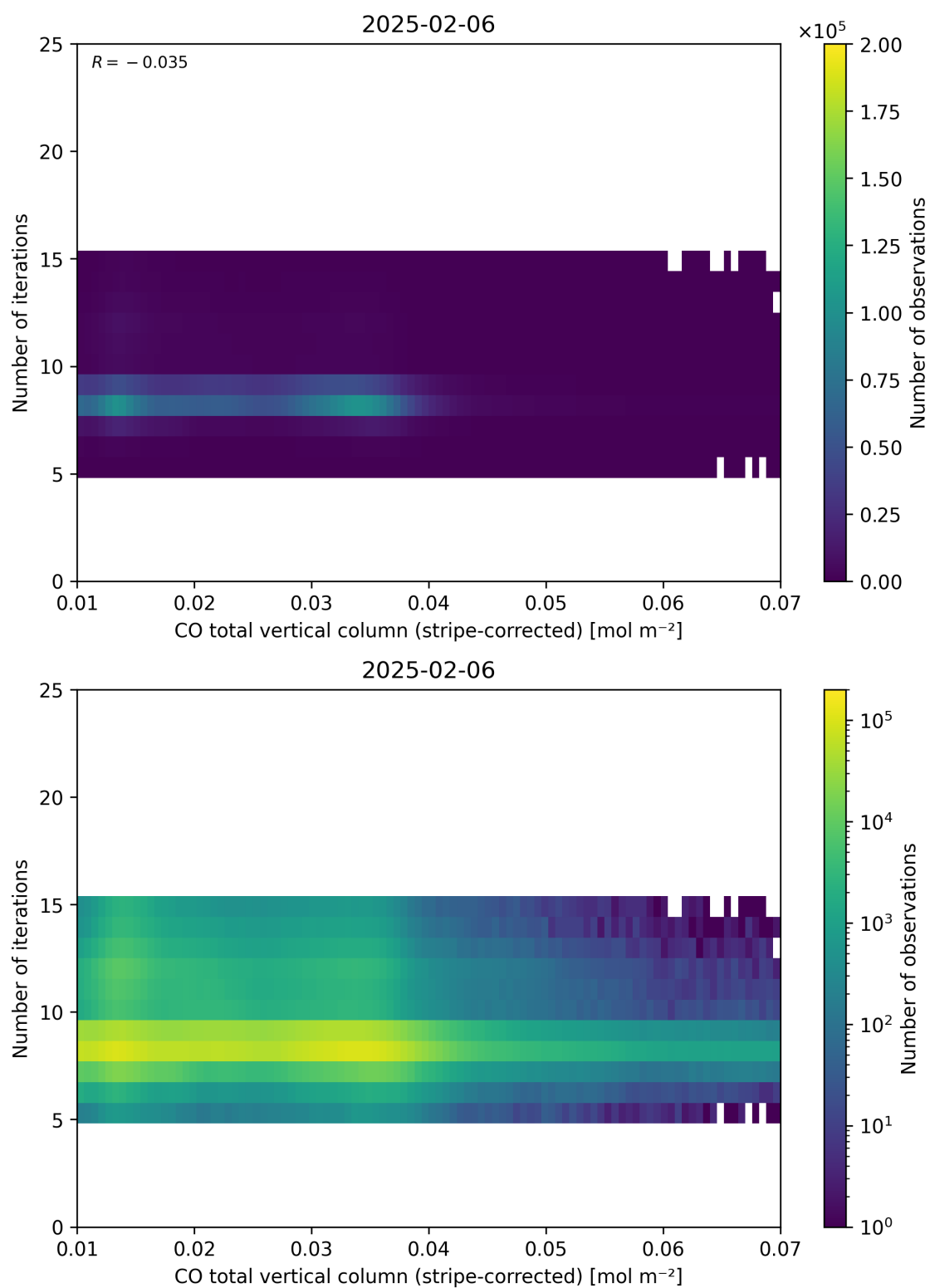
Figure 39: Scatter density plot of “CO total vertical column (stripe-corrected)” against “Number of iterations” for 2025-02-05 to 2025-02-07.
