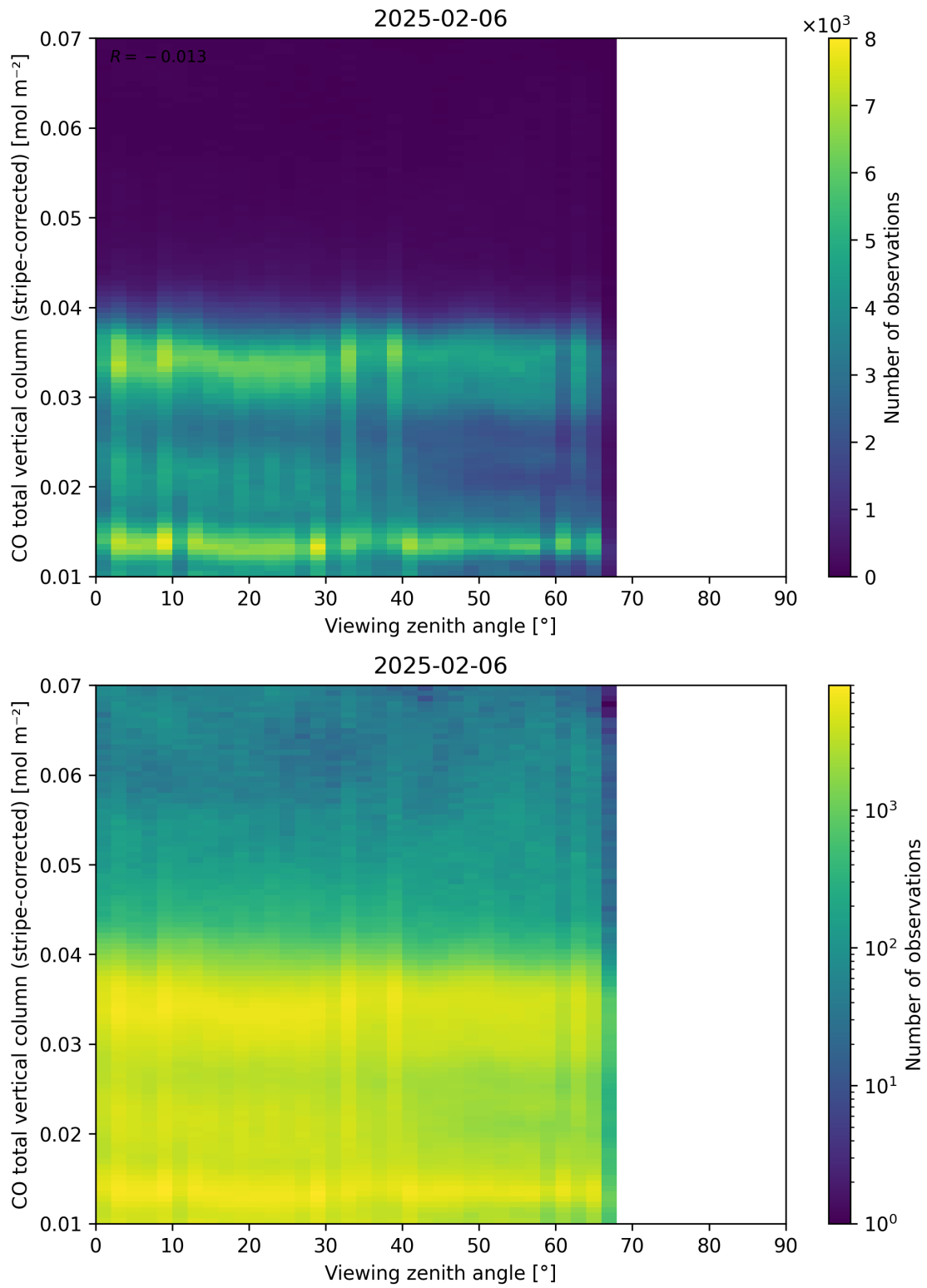
Figure 70: Scatter density plot of “Viewing zenith angle” against “CO total vertical column (stripe-corrected)” for 2025-02-05 to 2025-02-07.
