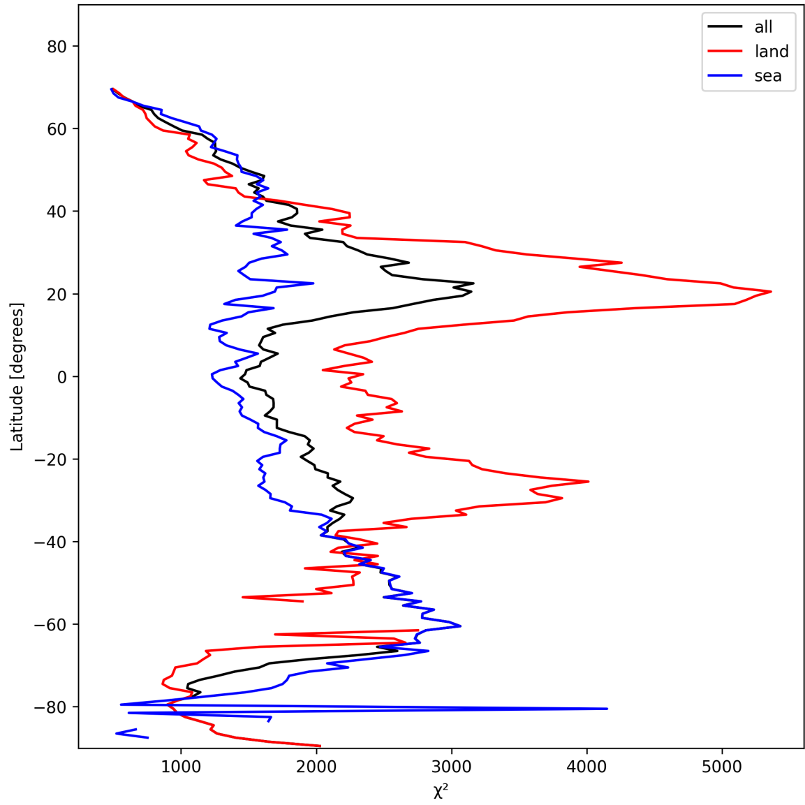
Figure 14: Zonal average of “ \chi^2 ” for 2025-02-05 to 2025-02-07.
