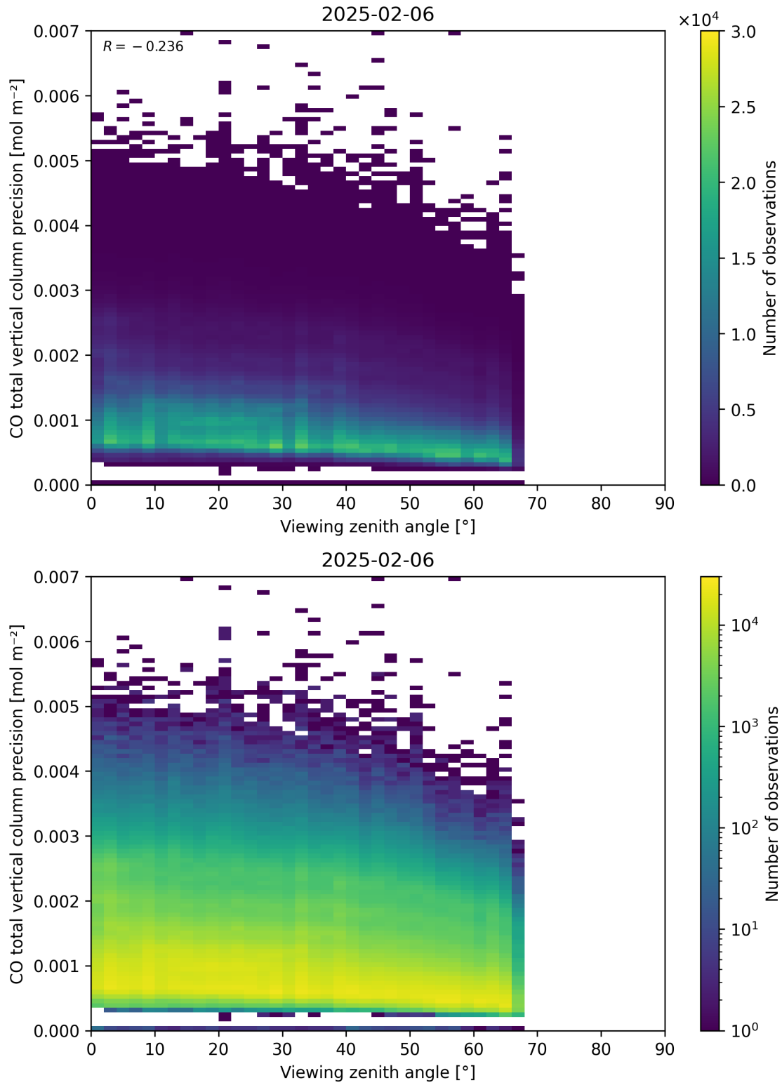
Figure 71: Scatter density plot of “Viewing zenith angle” against “CO total vertical column precision” for 2025-02-05 to 2025-02-07.
