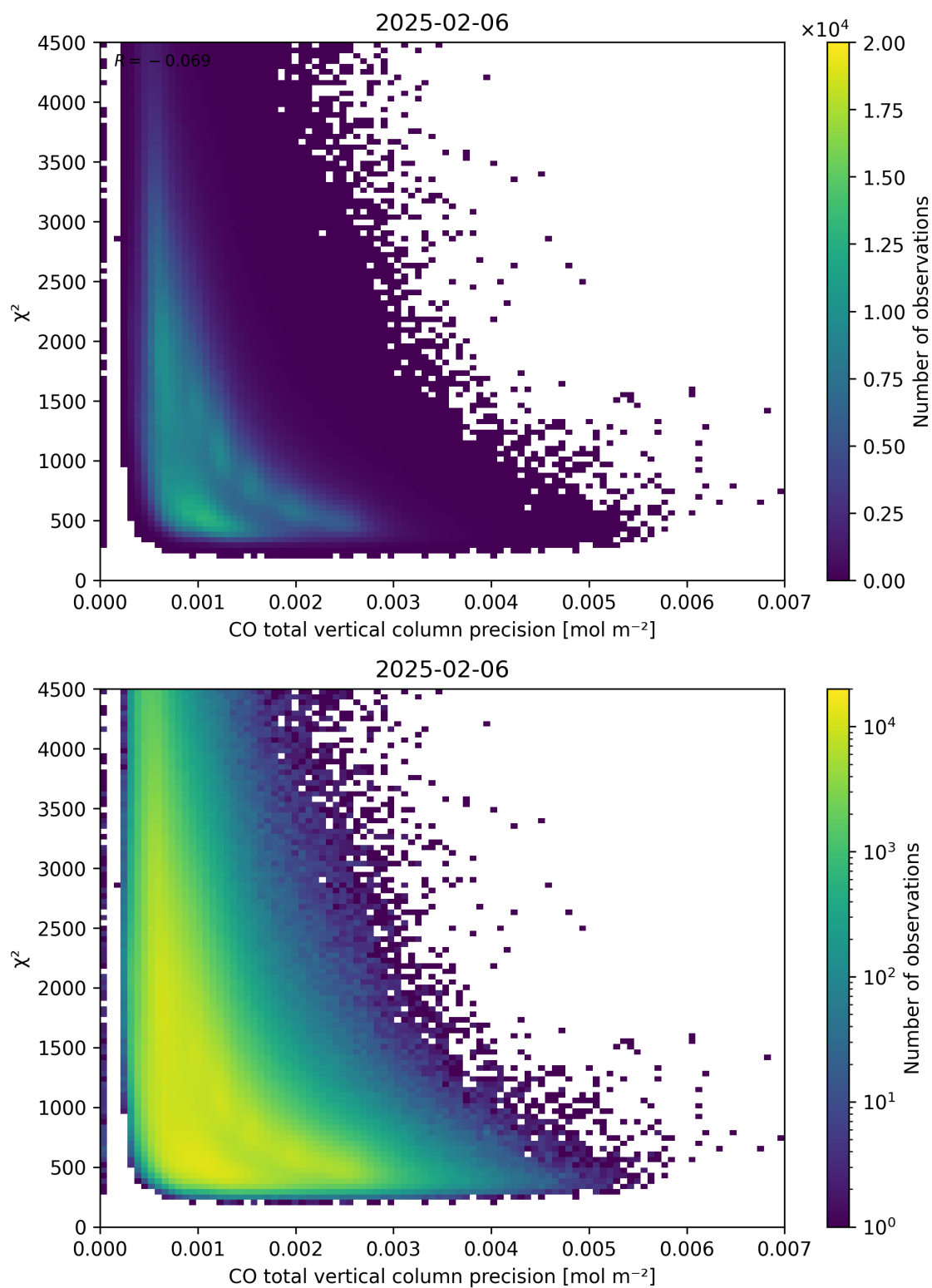
Figure 44: Scatter density plot of “CO total vertical column precision” against “ \chi^2 ” for 2025-02-05 to 2025-02-07.
