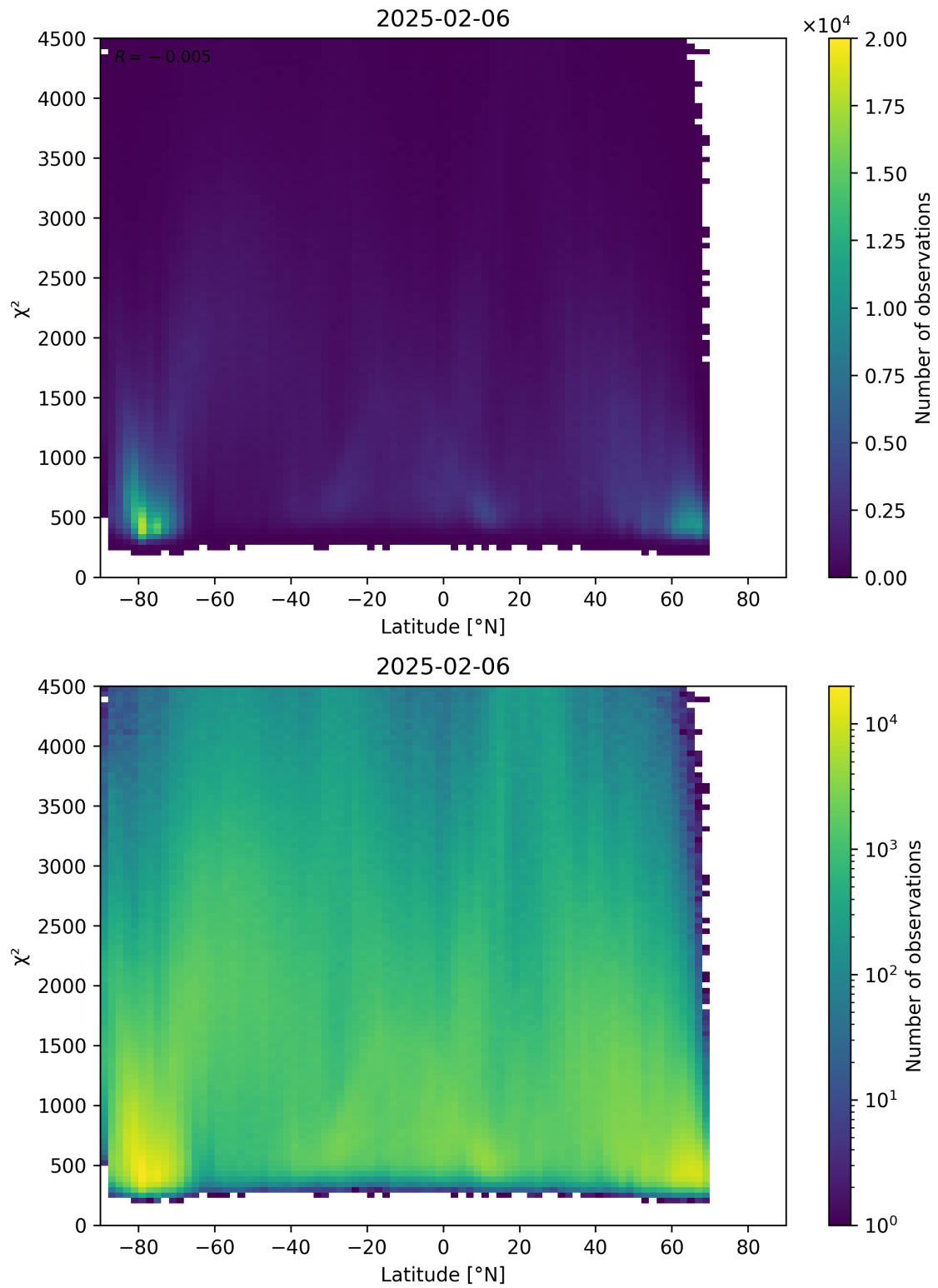
Figure 54: Scatter density plot of “Latitude” against “ \chi^2 ” for 2025-02-05 to 2025-02-07.
