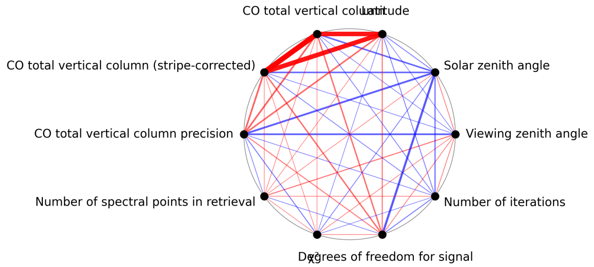
Figure 1: Map of correlation graph for 2025-02-05 to 2025-02-07.
