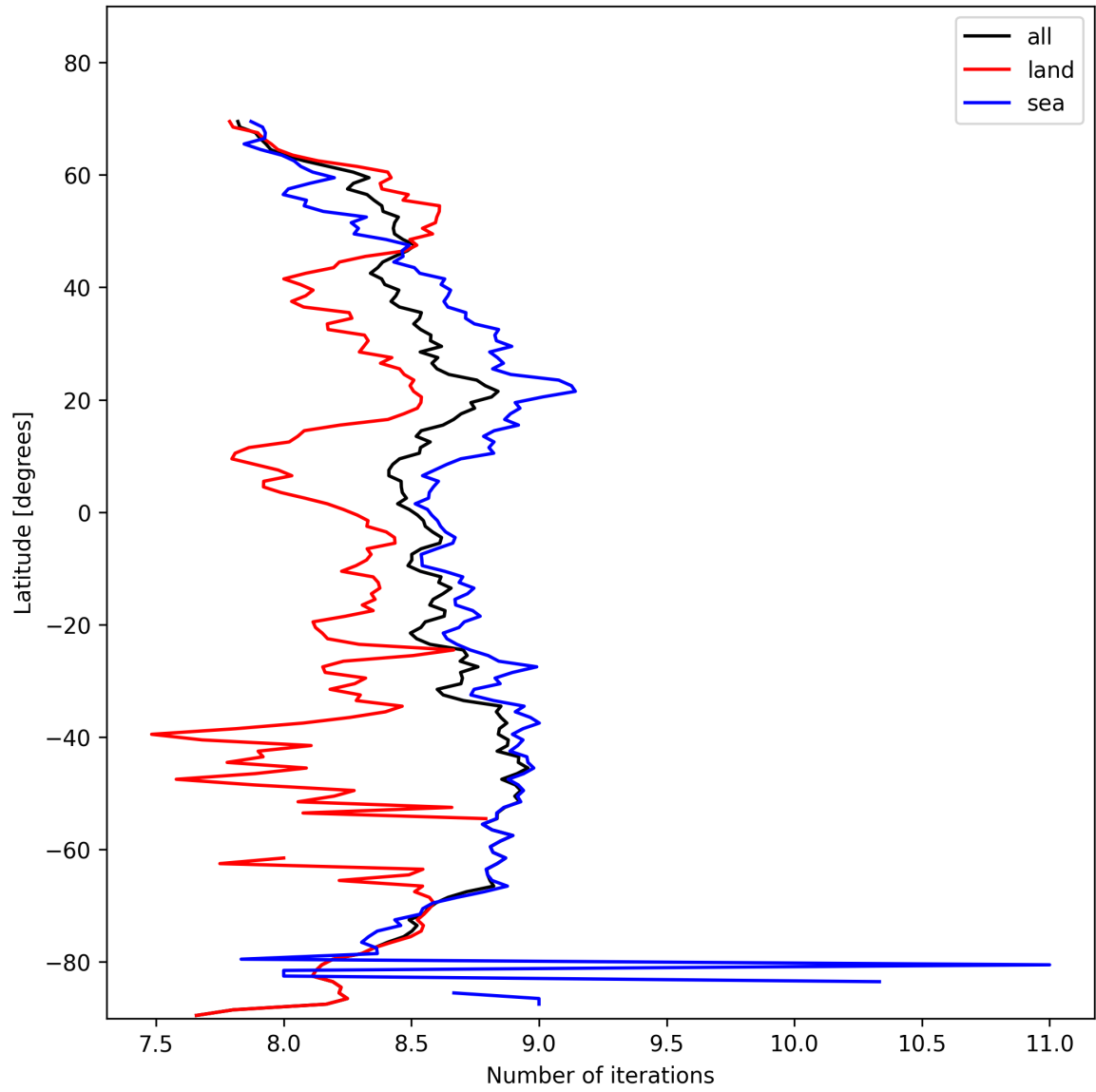
Figure 16: Zonal average of “Number of iterations” for 2025-02-05 to 2025-02-07.
