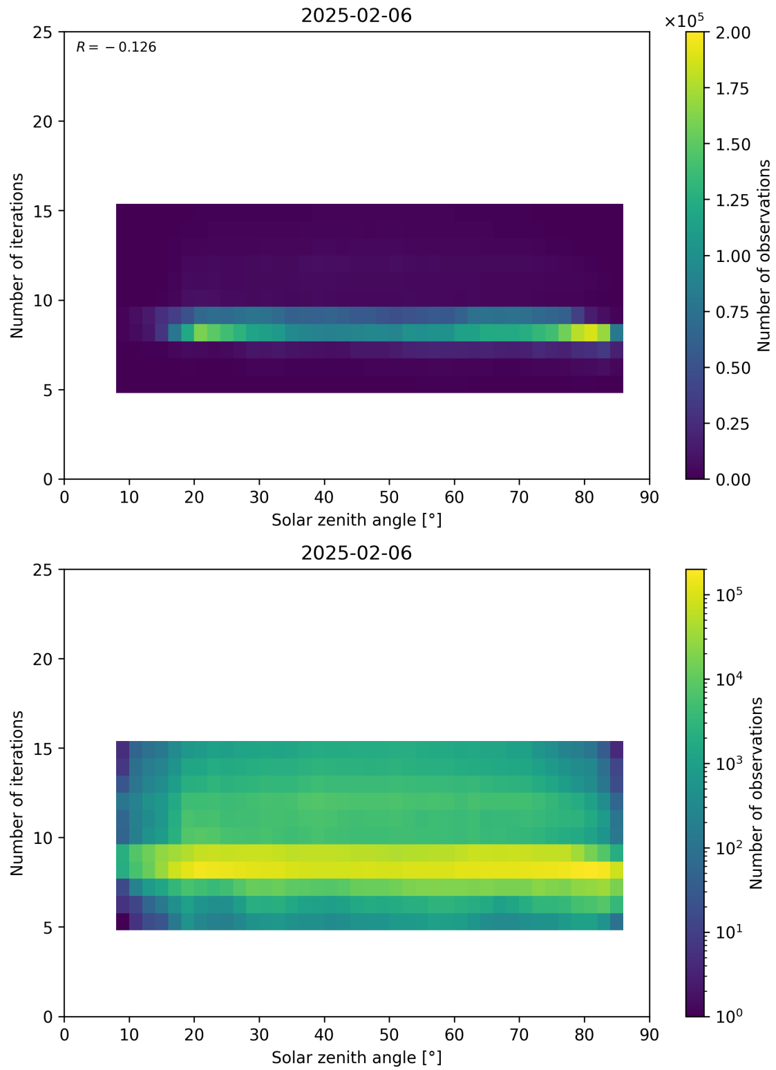
Figure 67: Scatter density plot of “Solar zenith angle” against “Number of iterations” for 2025-02-05 to 2025-02-07.
