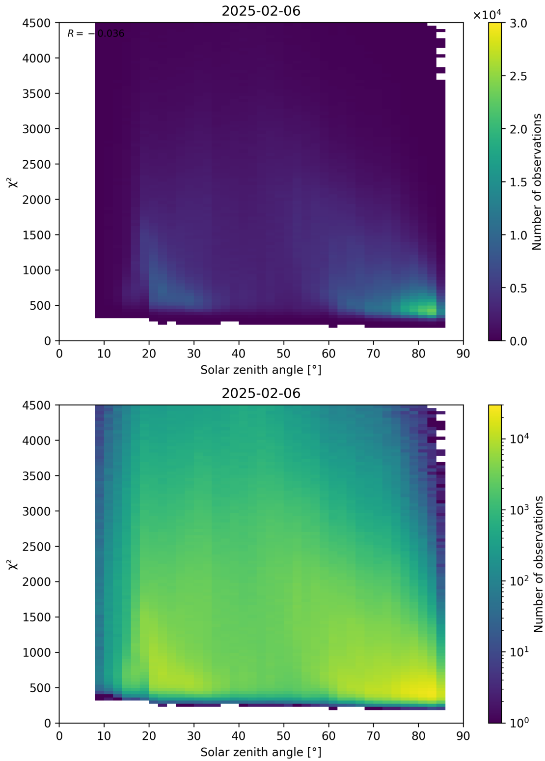
Figure 64: Scatter density plot of “Solar zenith angle” against “ \chi^2 ” for 2025-02-05 to 2025-02-07.
