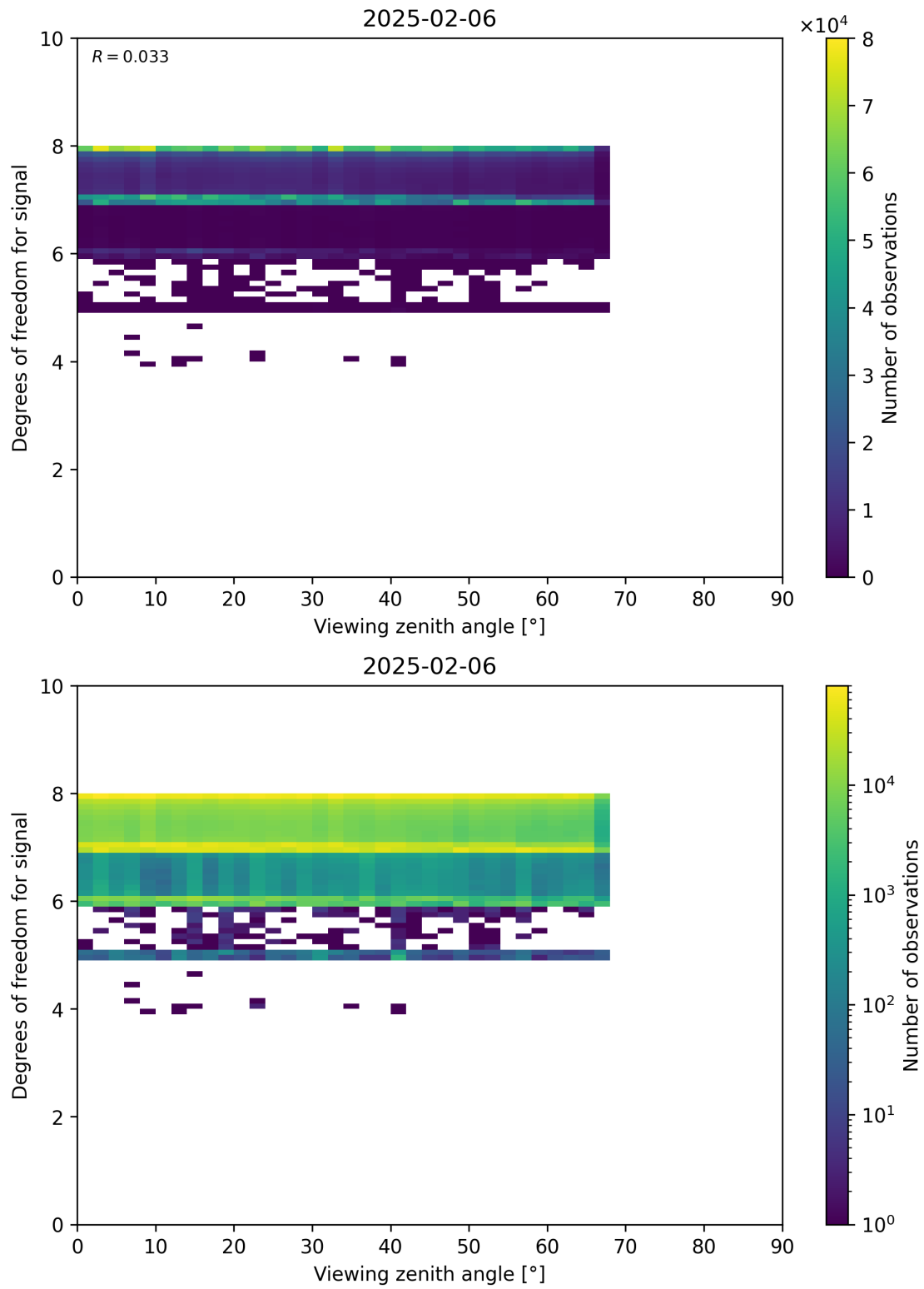
Figure 73: Scatter density plot of “Viewing zenith angle” against “Degrees of freedom for signal” for 2025-02-05 to 2025-02-07.
