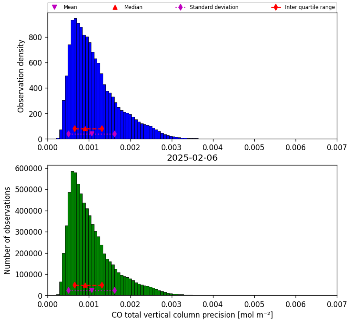
Figure 20: Histogram of “CO total vertical column precision” for 2025-02-05 to 2025-02-07
