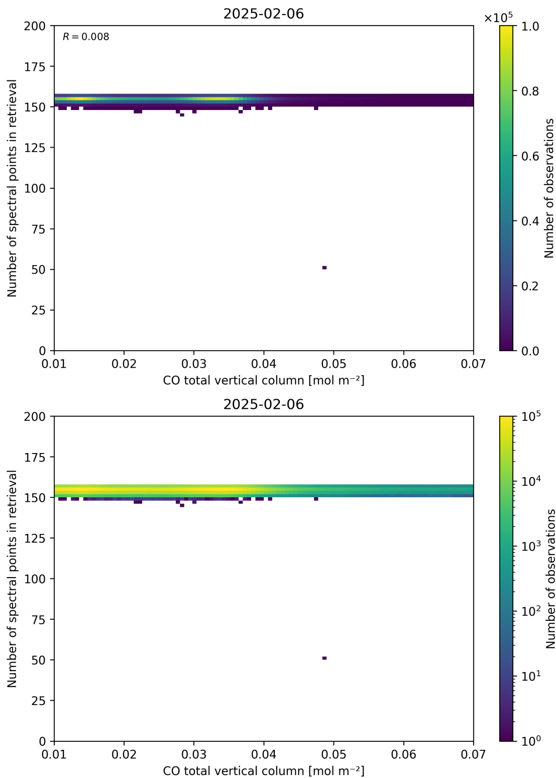
Figure 43: Scatter density plot of “CO total vertical column” against “Number of spectral points in retrieval” for 2025-02-05 to 2025-02-07.
