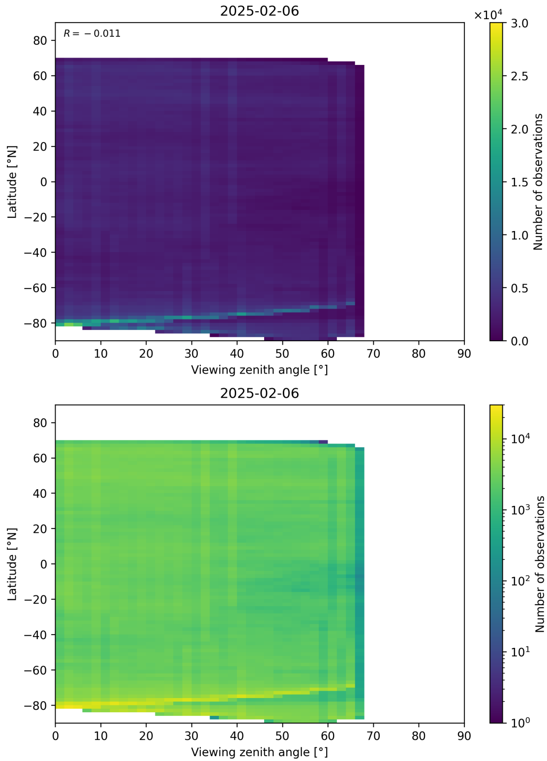
Figure 74: Scatter density plot of “Viewing zenith angle” against “Latitude” for 2025-02-05 to 2025-02-07.
