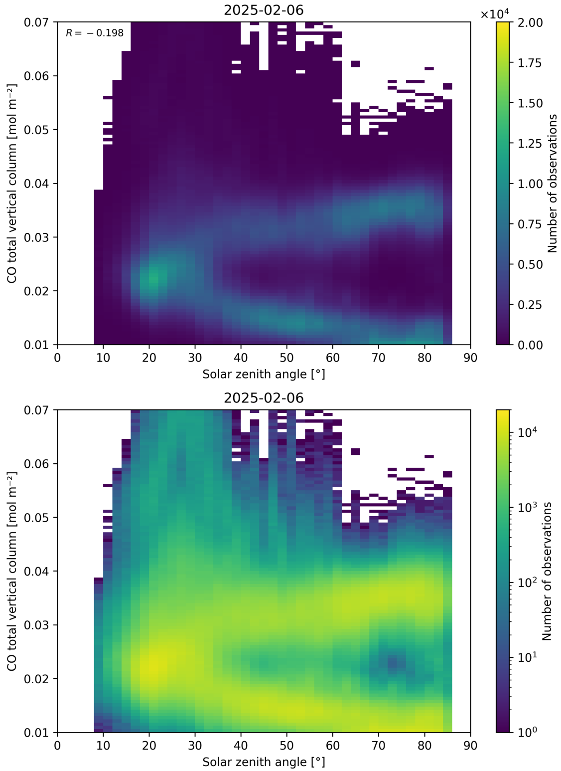
Figure 61: Scatter density plot of “Solar zenith angle” against “CO total vertical column” for 2025-02-05 to 2025-02-07.
