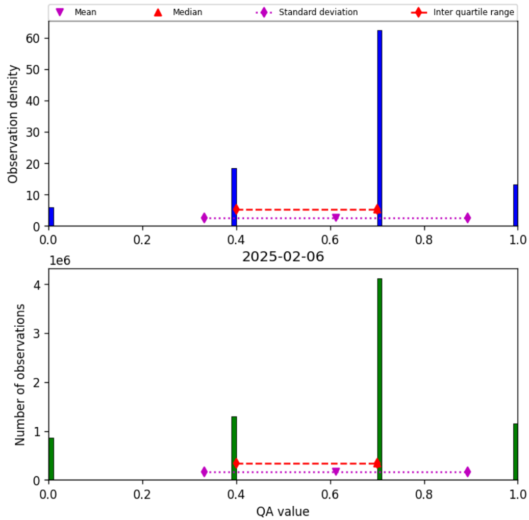
Figure 17: Histogram of “QA value” for 2025-02-05 to 2025-02-07
