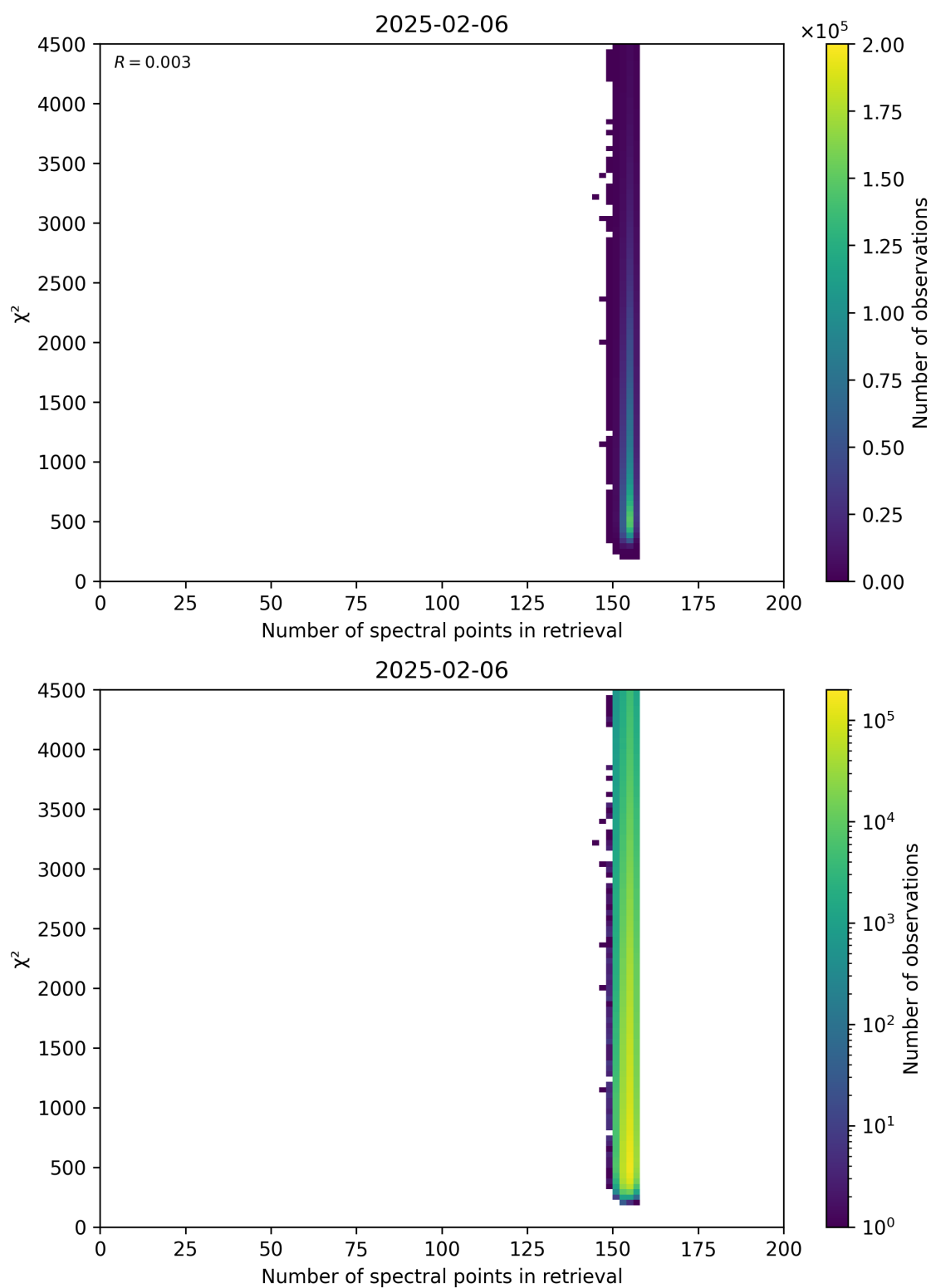
Figure 58: Scatter density plot of “Number of spectral points in retrieval” against “ \chi^2 ” for 2025-02-05 to 2025-02-07.
