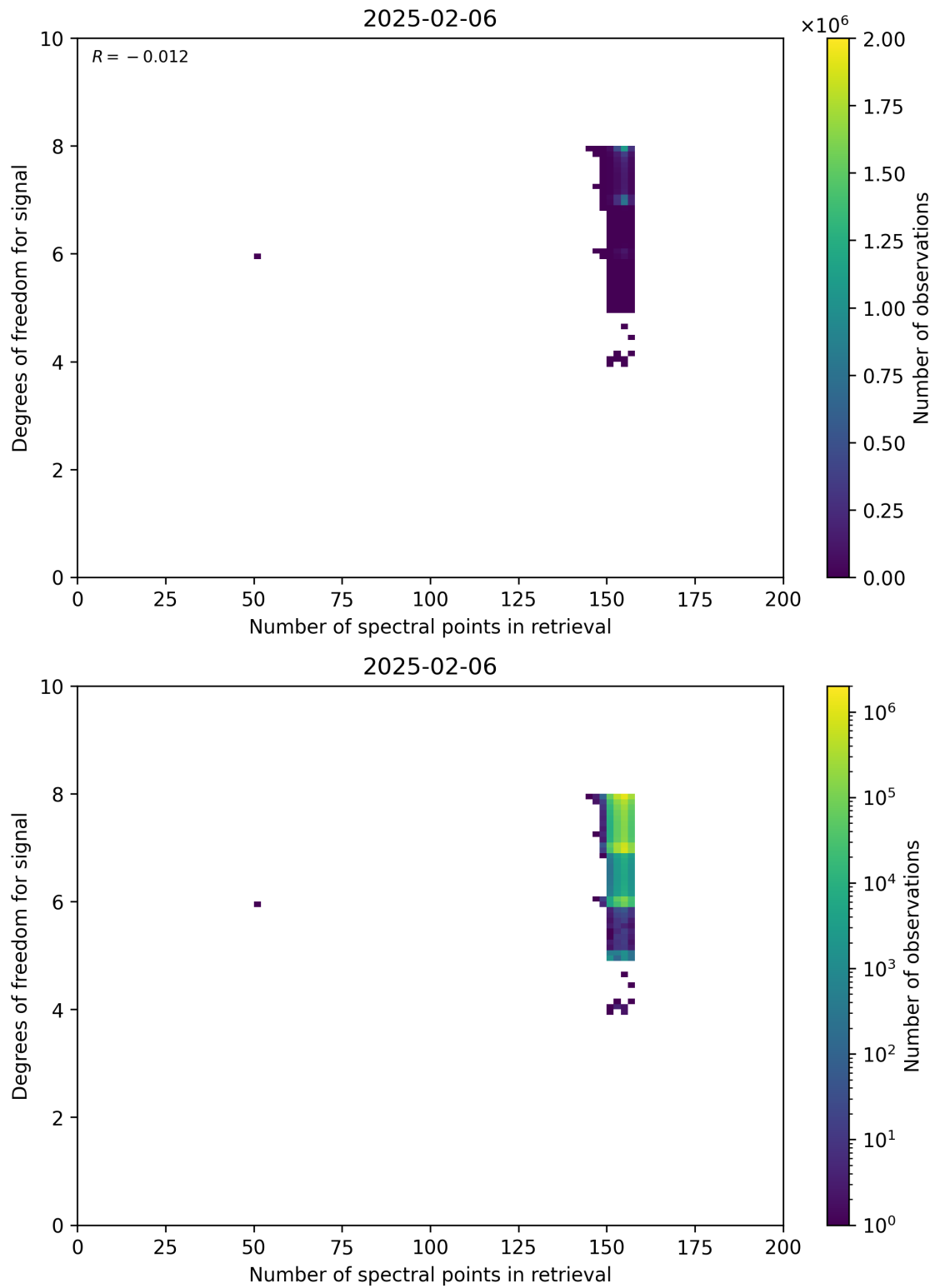
Figure 59: Scatter density plot of “Number of spectral points in retrieval” against “Degrees of freedom for signal” for 2025-02-05 to 2025-02-07.
