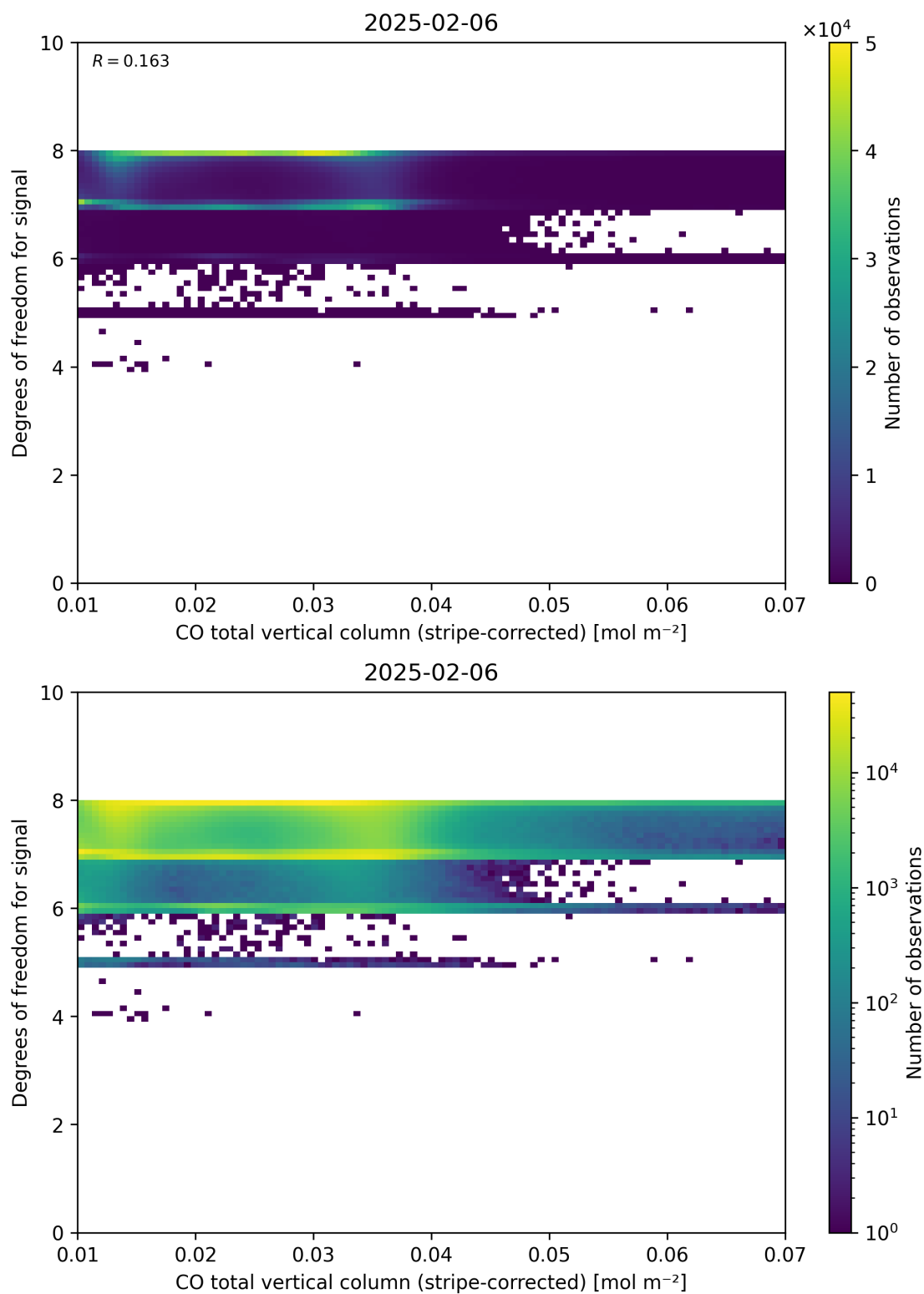
Figure 38: Scatter density plot of “CO total vertical column (stripe-corrected)” against “Degrees of freedom for signal” for 2025-02-05 to 2025-02-07.
