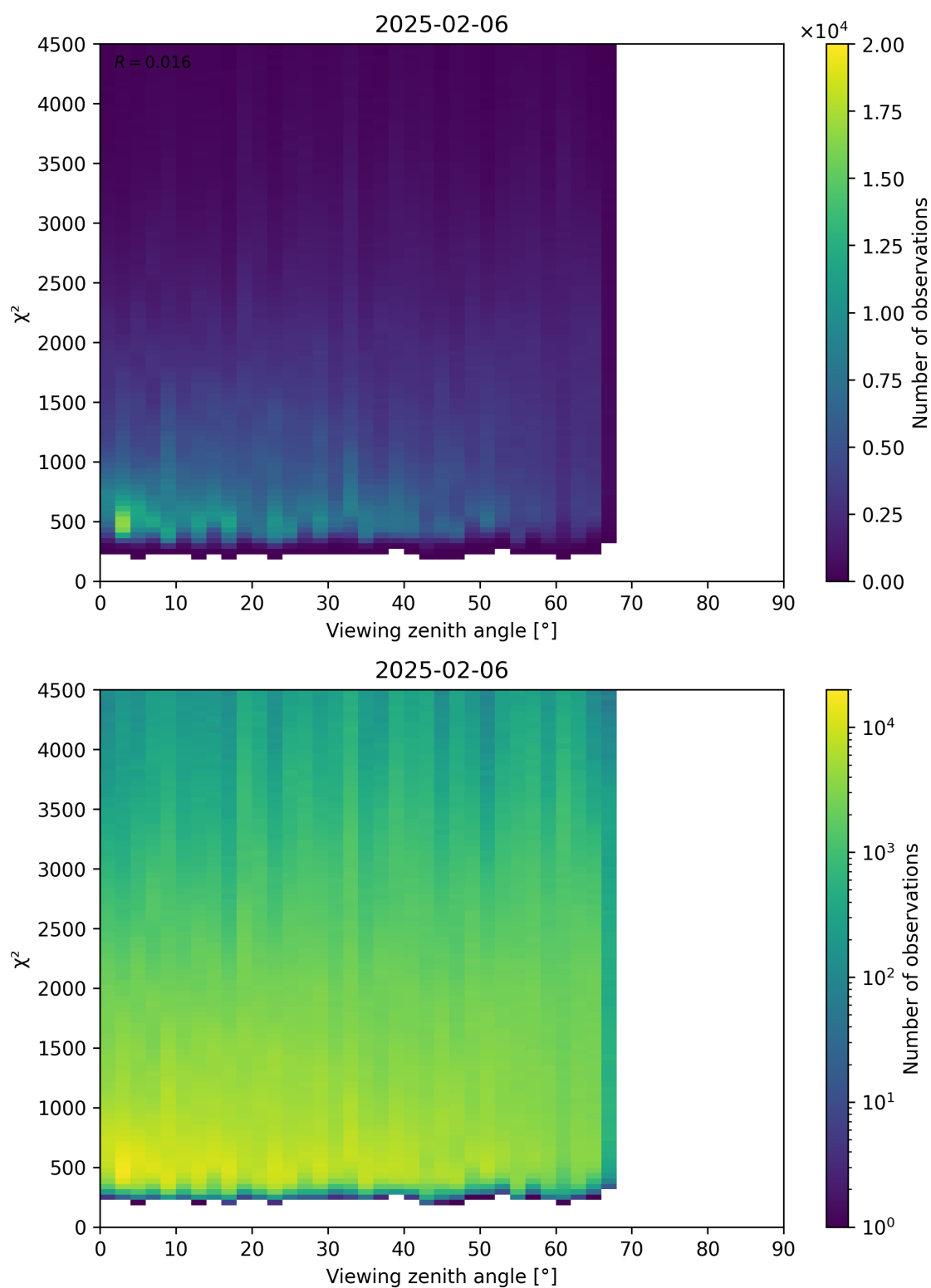
Figure 72: Scatter density plot of “Viewing zenith angle” against “ \chi^2 ” for 2025-02-05 to 2025-02-07.
