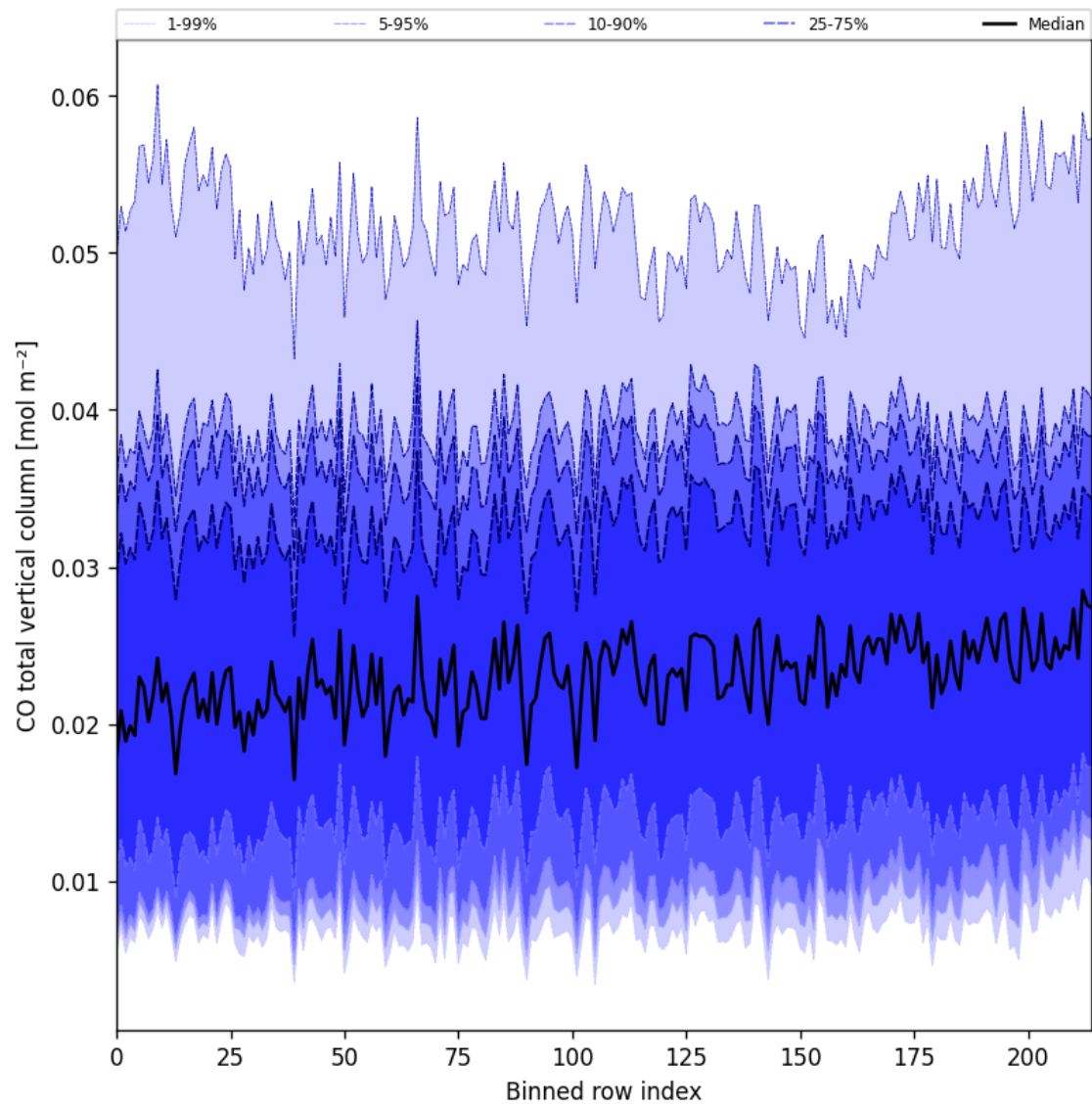
Figure 26: Along track statistics of “CO total vertical column” for 2025-02-05 to 2025-02-07
