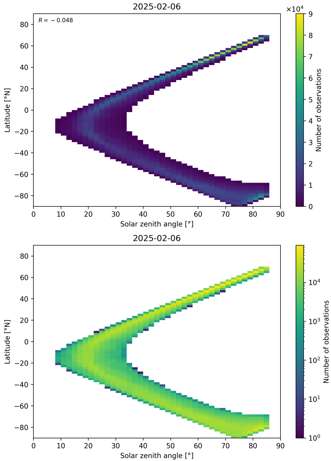
Figure 66: Scatter density plot of “Solar zenith angle” against “Latitude” for 2025-02-05 to 2025-02-07.
