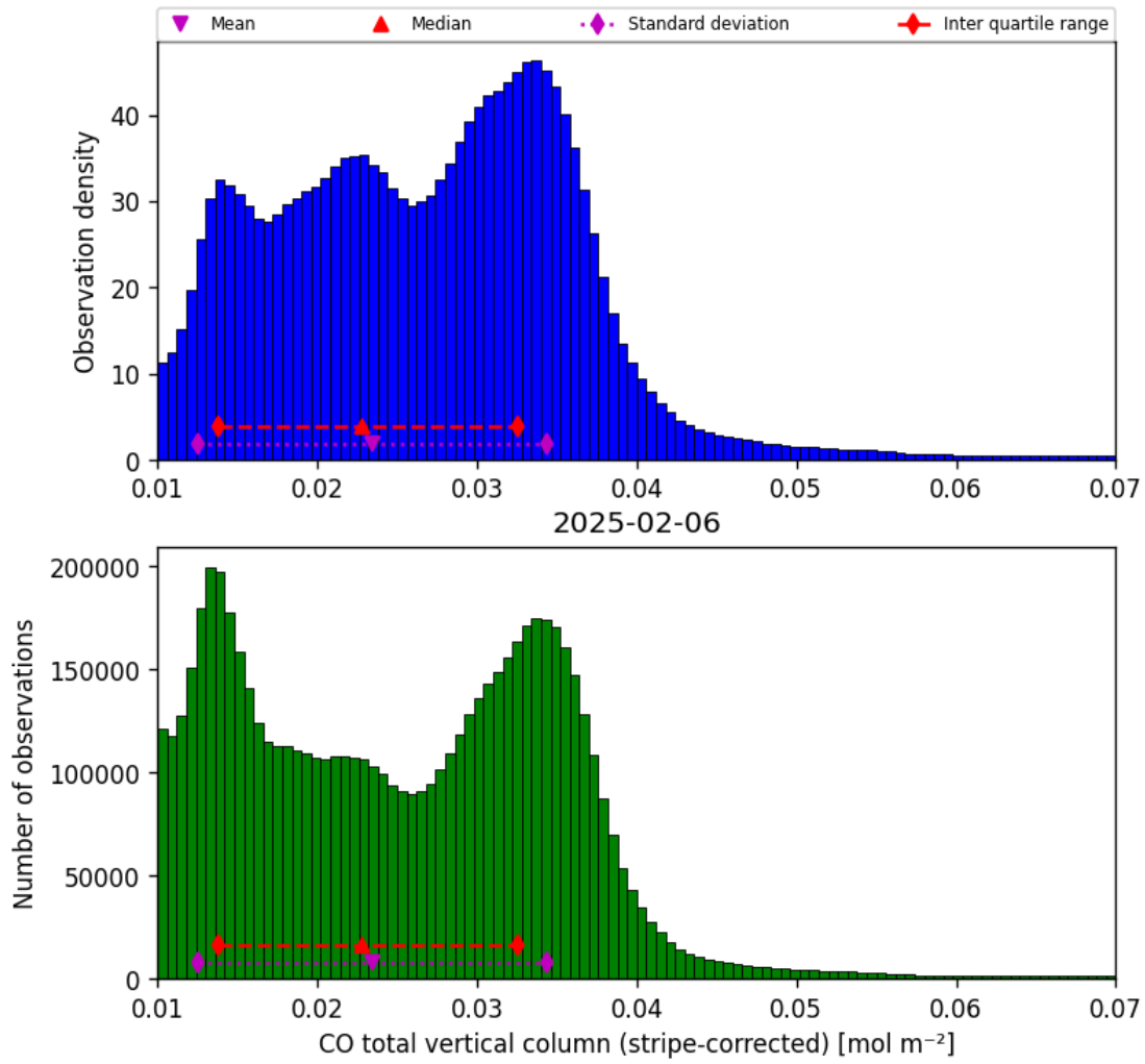
Figure 19: Histogram of “CO total vertical column (stripe-corrected)” for 2025-02-05 to 2025-02-07
