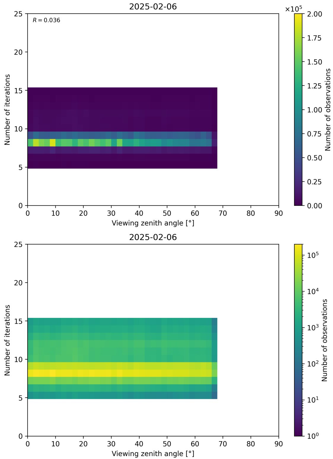
Figure 75: Scatter density plot of “Viewing zenith angle” against “Number of iterations” for 2025-02-05 to 2025-02-07.
