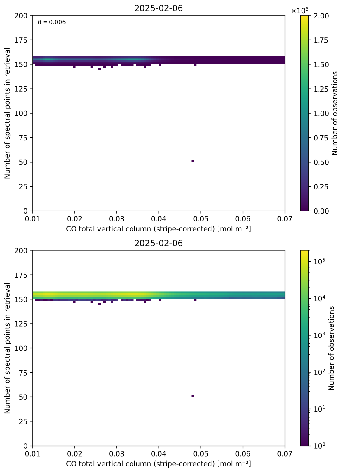
Figure 40: Scatter density plot of “CO total vertical column (stripe-corrected)” against “Number of spectral points in retrieval” for 2025-02-05 to 2025-02-07.
