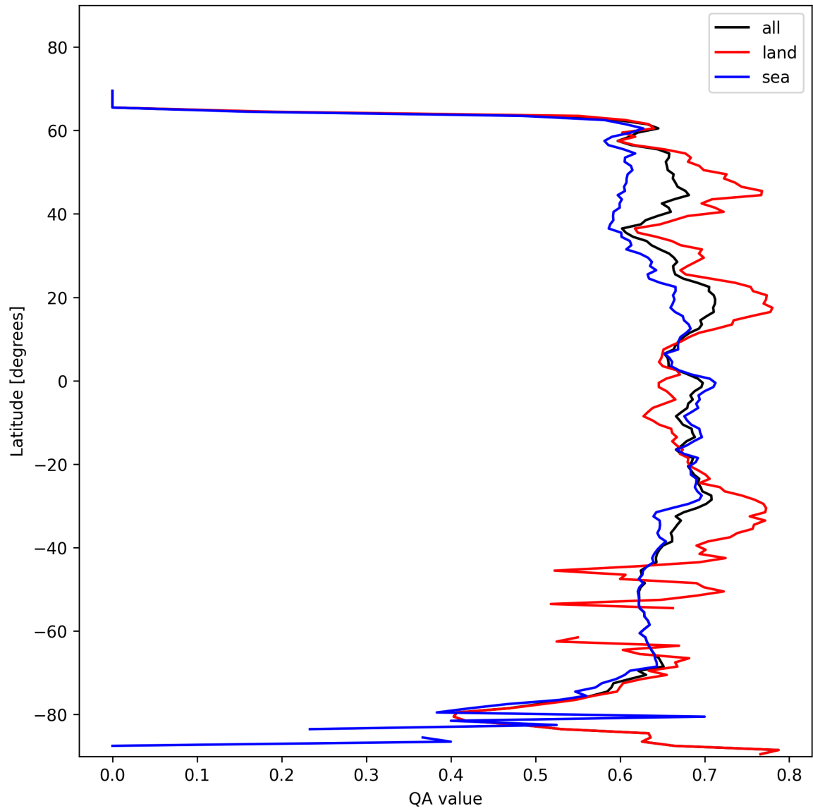
Figure 9: Zonal average of “QA value” for 2025-02-05 to 2025-02-07.
