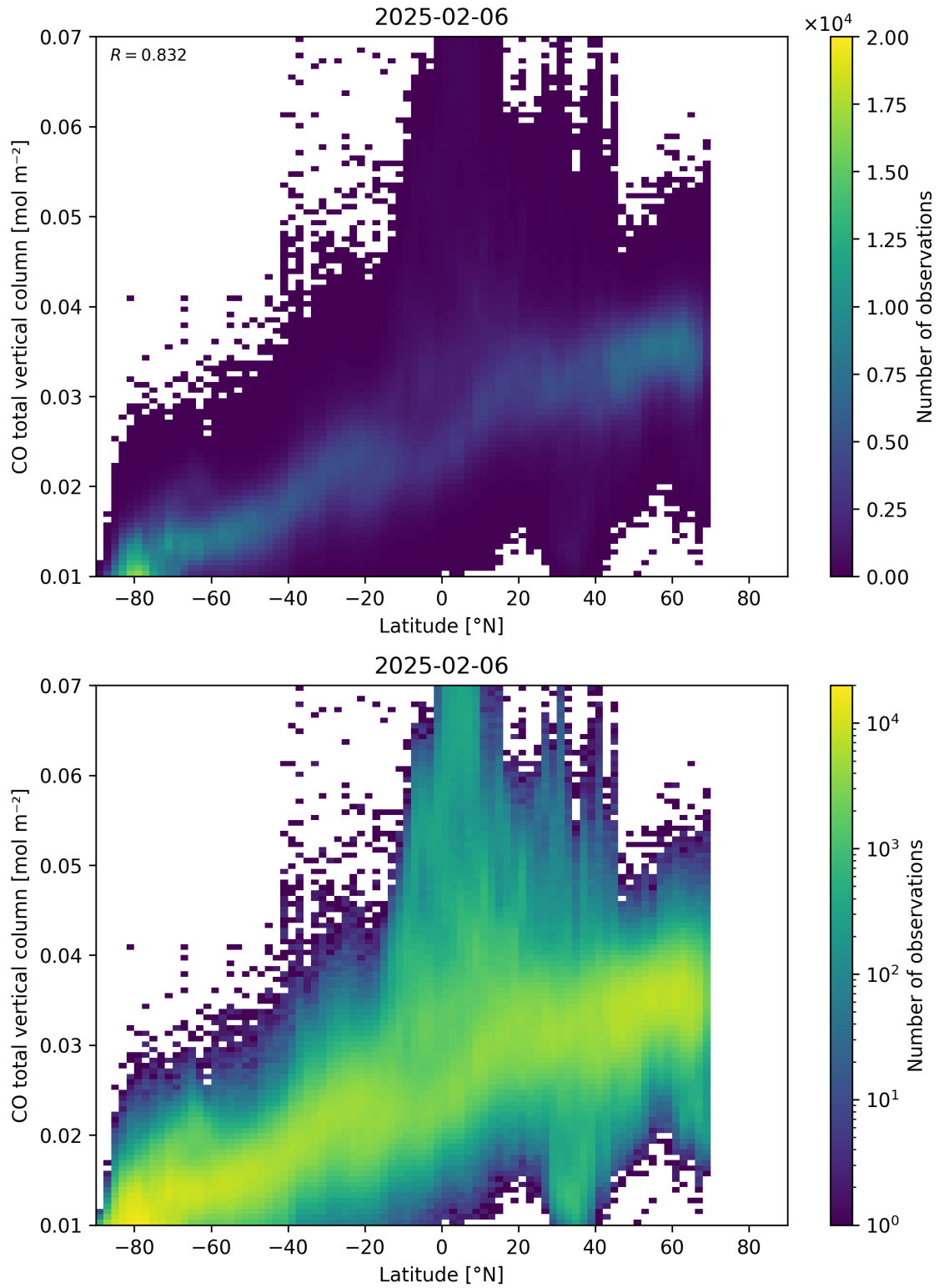
Figure 51: Scatter density plot of “Latitude” against “CO total vertical column” for 2025-02-05 to 2025-02-07.
