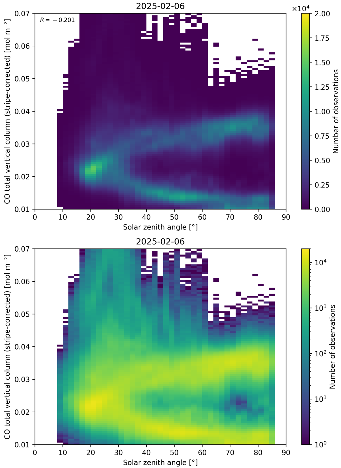
Figure 62: Scatter density plot of “Solar zenith angle” against “CO total vertical column (stripe-corrected)” for 2025-02-05 to 2025-02-07.
