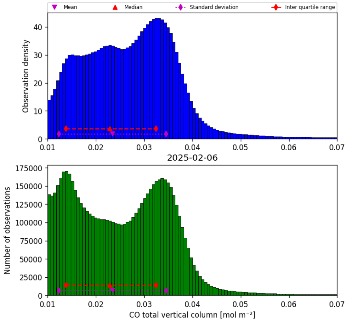
Figure 18: Histogram of “CO total vertical column” for 2025-02-05 to 2025-02-07
