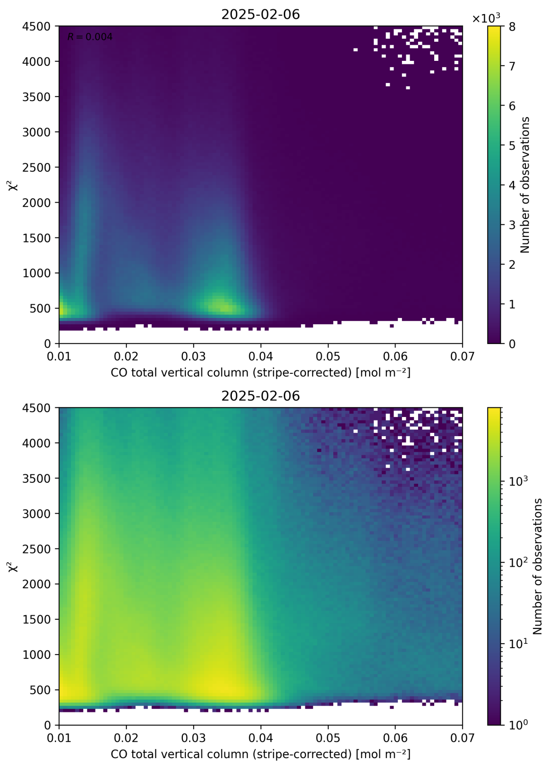
Figure 37: Scatter density plot of “CO total vertical column (stripe-corrected)” against “ \chi^2 ” for 2025-02-05 to 2025-02-07.
