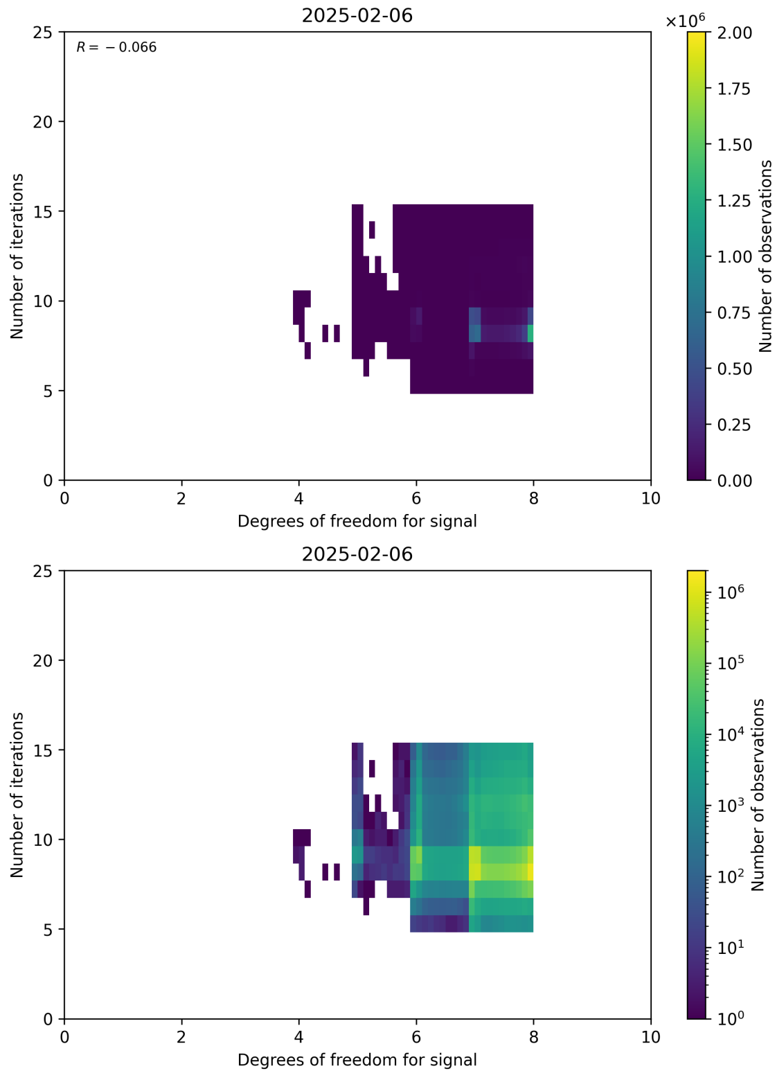
Figure 50: Scatter density plot of “Degrees of freedom for signal” against “Number of iterations” for 2025-02-05 to 2025-02-07.
