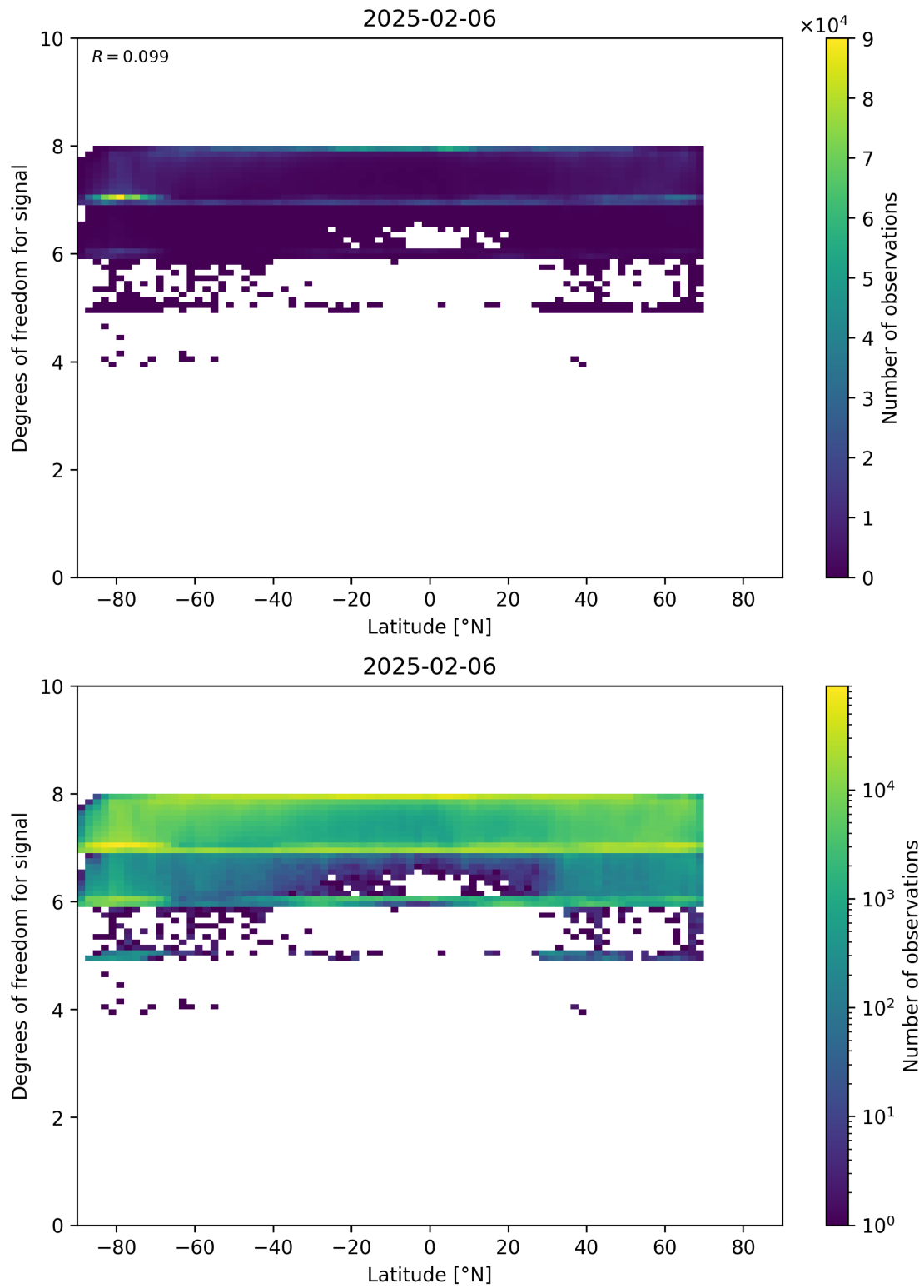
Figure 55: Scatter density plot of “Latitude” against “Degrees of freedom for signal” for 2025-02-05 to 2025-02-07.
