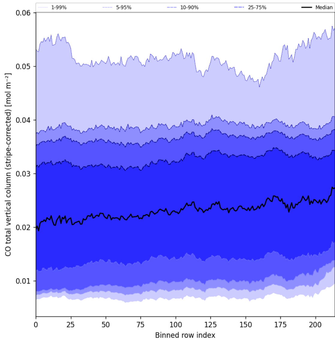
Figure 27: Along track statistics of “CO total vertical column (stripe-corrected)” for 2025-02-05 to 2025-02-07
