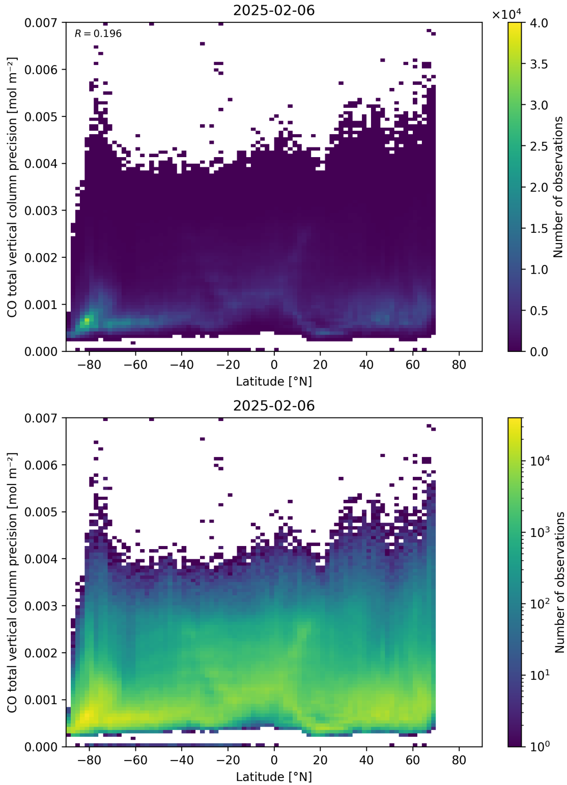
Figure 53: Scatter density plot of “Latitude” against “CO total vertical column precision” for 2025-02-05 to 2025-02-07.
