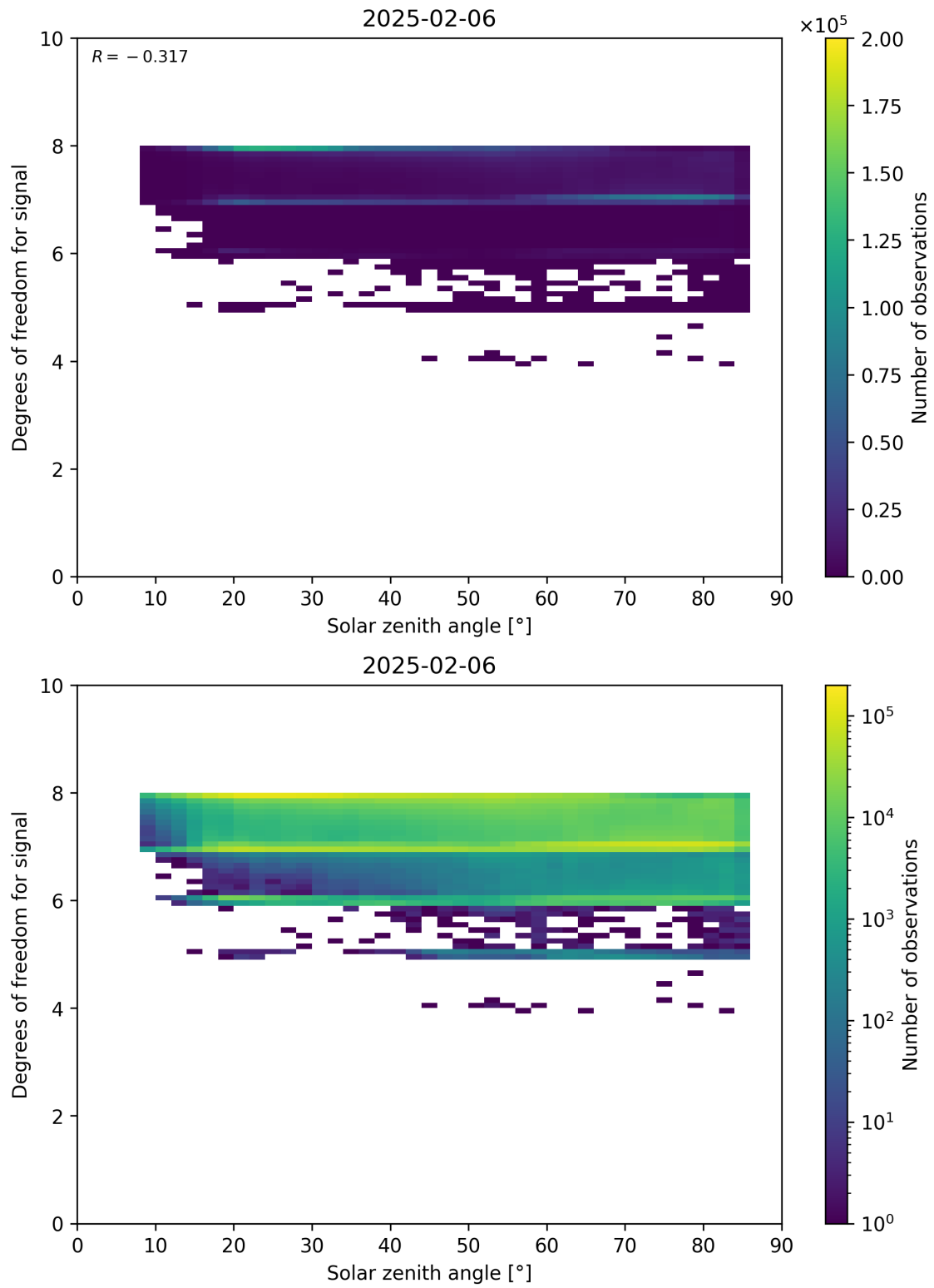
Figure 65: Scatter density plot of “Solar zenith angle” against “Degrees of freedom for signal” for 2025-02-05 to 2025-02-07.
