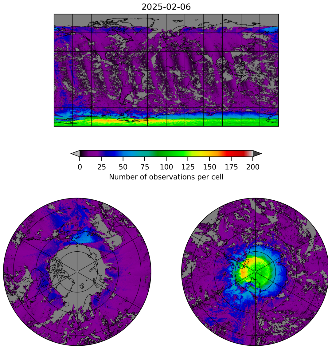
Figure 8: Map of the number of observations for 2025-02-05 to 2025-02-07
