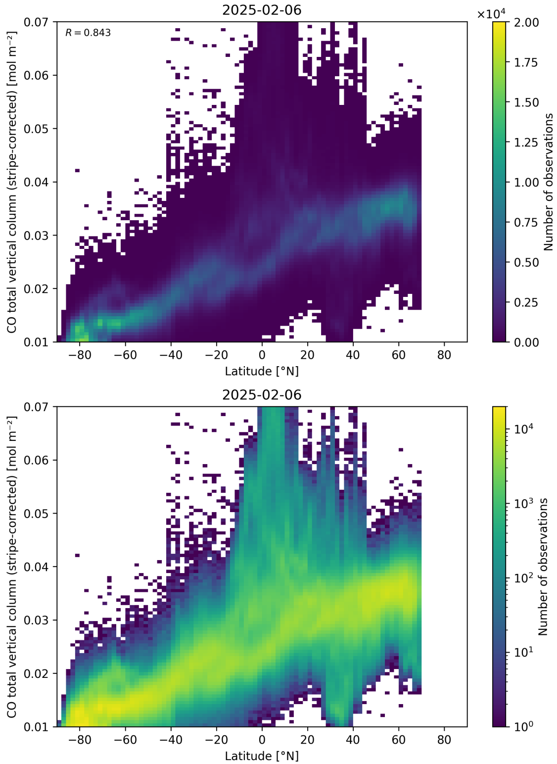
Figure 52: Scatter density plot of “Latitude” against “CO total vertical column (stripe-corrected)” for 2025-02-05 to 2025-02-07.
