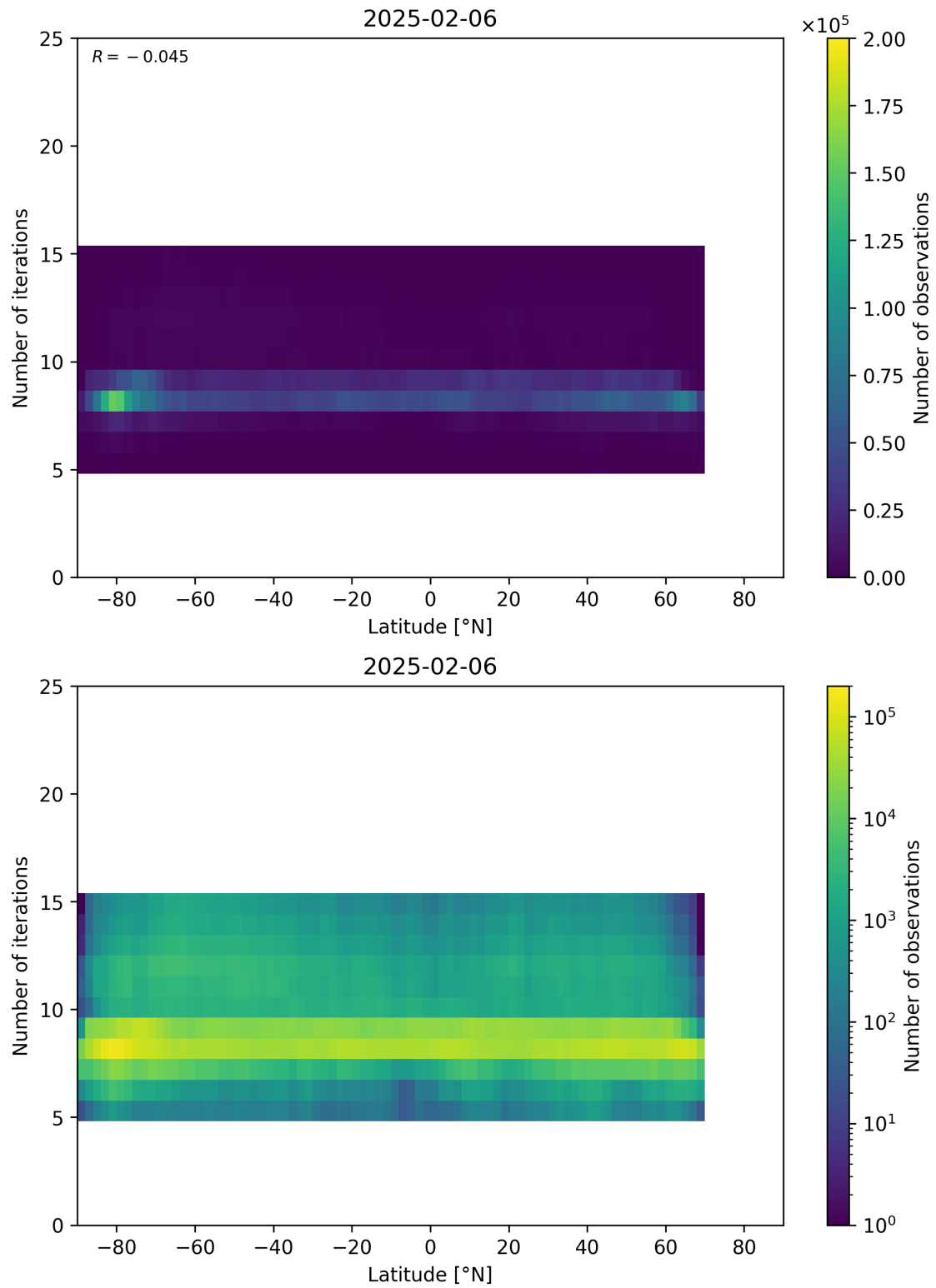
Figure 56: Scatter density plot of “Latitude” against “Number of iterations” for 2025-02-05 to 2025-02-07.
