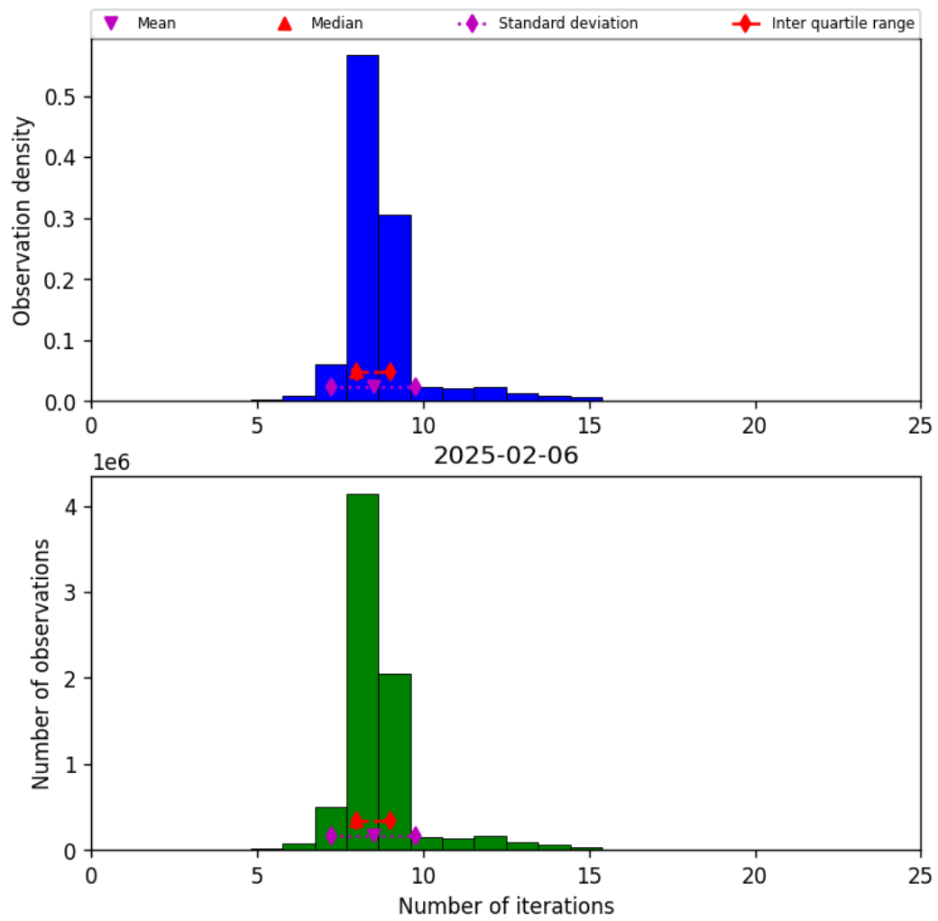
Figure 24: Histogram of “Number of iterations” for 2025-02-05 to 2025-02-07
