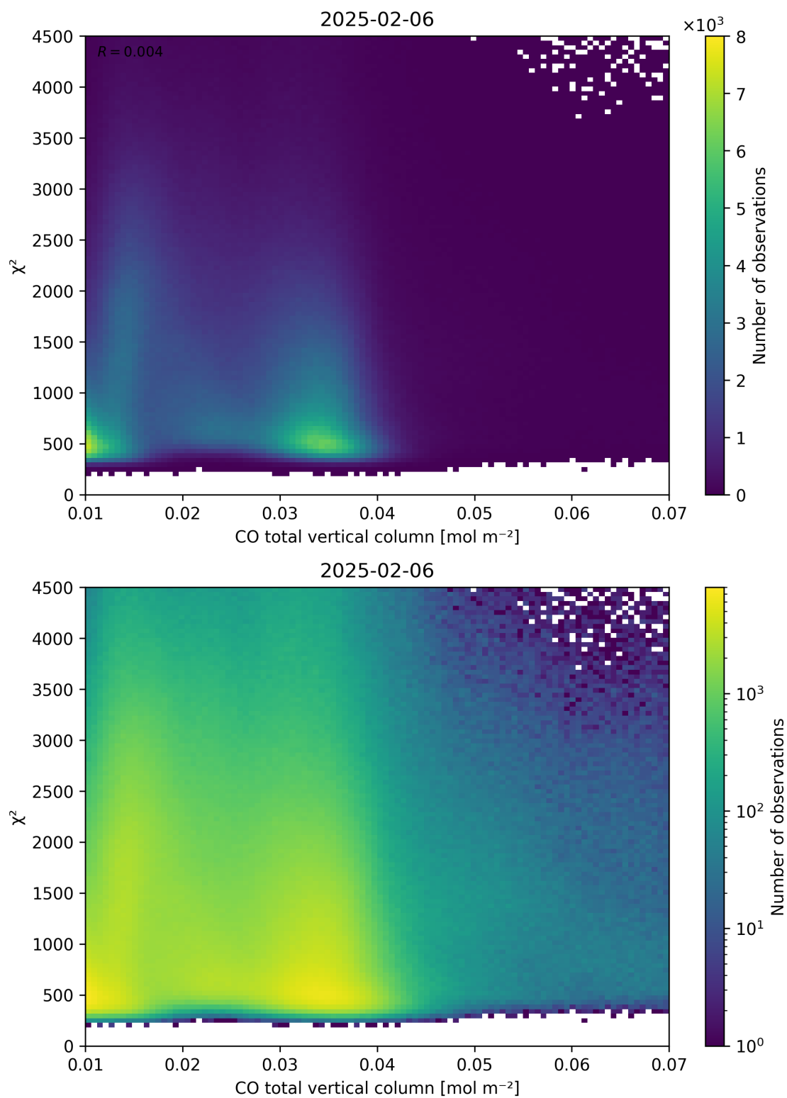
Figure 35: Scatter density plot of “CO total vertical column” against “ \chi^2 ” for 2025-02-05 to 2025-02-07.
