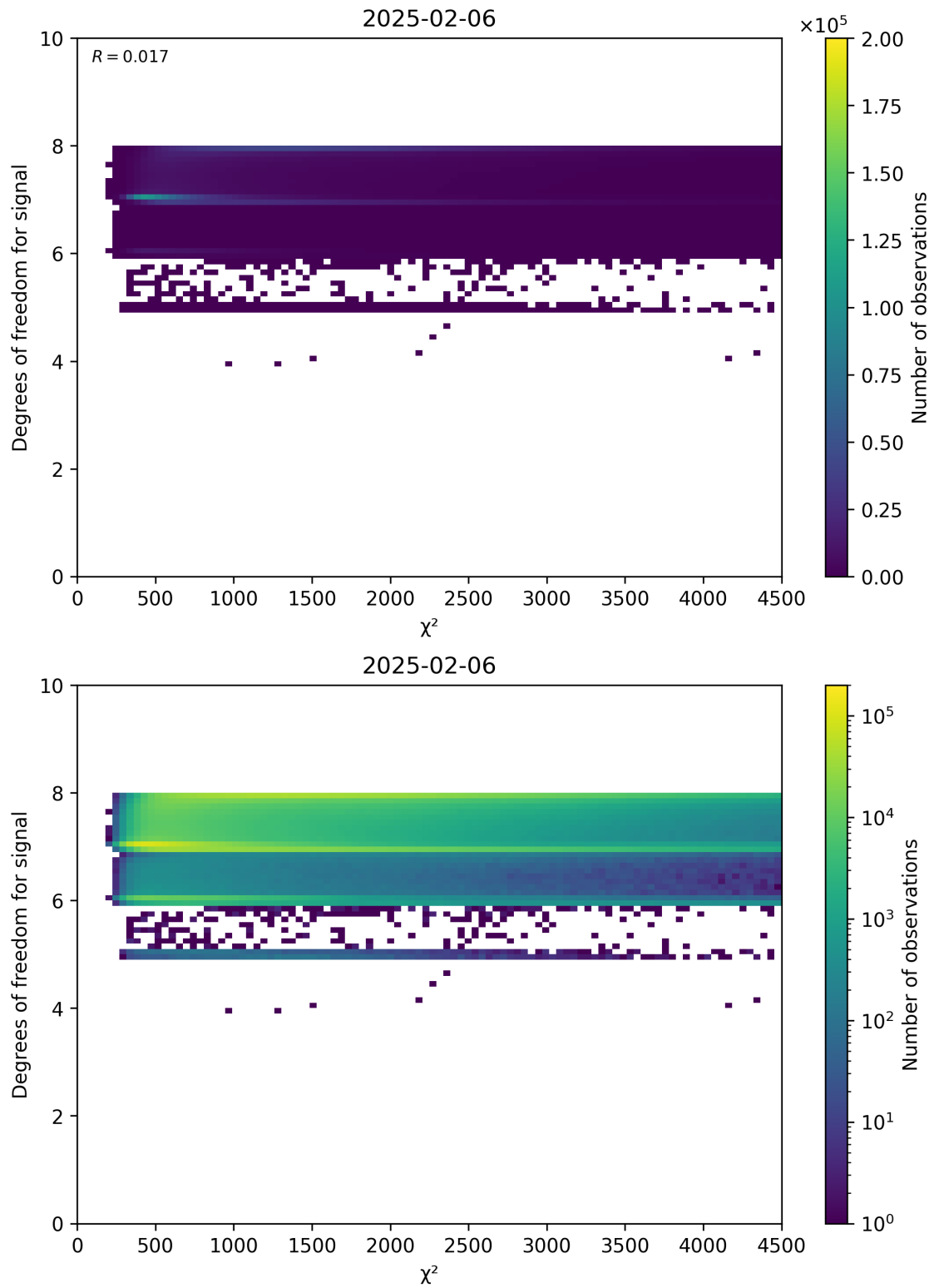
Figure 48: Scatter density plot of “ \chi^2 ” against “Degrees of freedom for signal” for 2025-02-05 to 2025-02-07.
