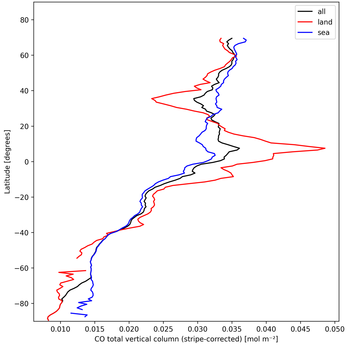
Figure 11: Zonal average of “CO total vertical column (stripe-corrected)” for 2025-02-05 to 2025-02-07.
