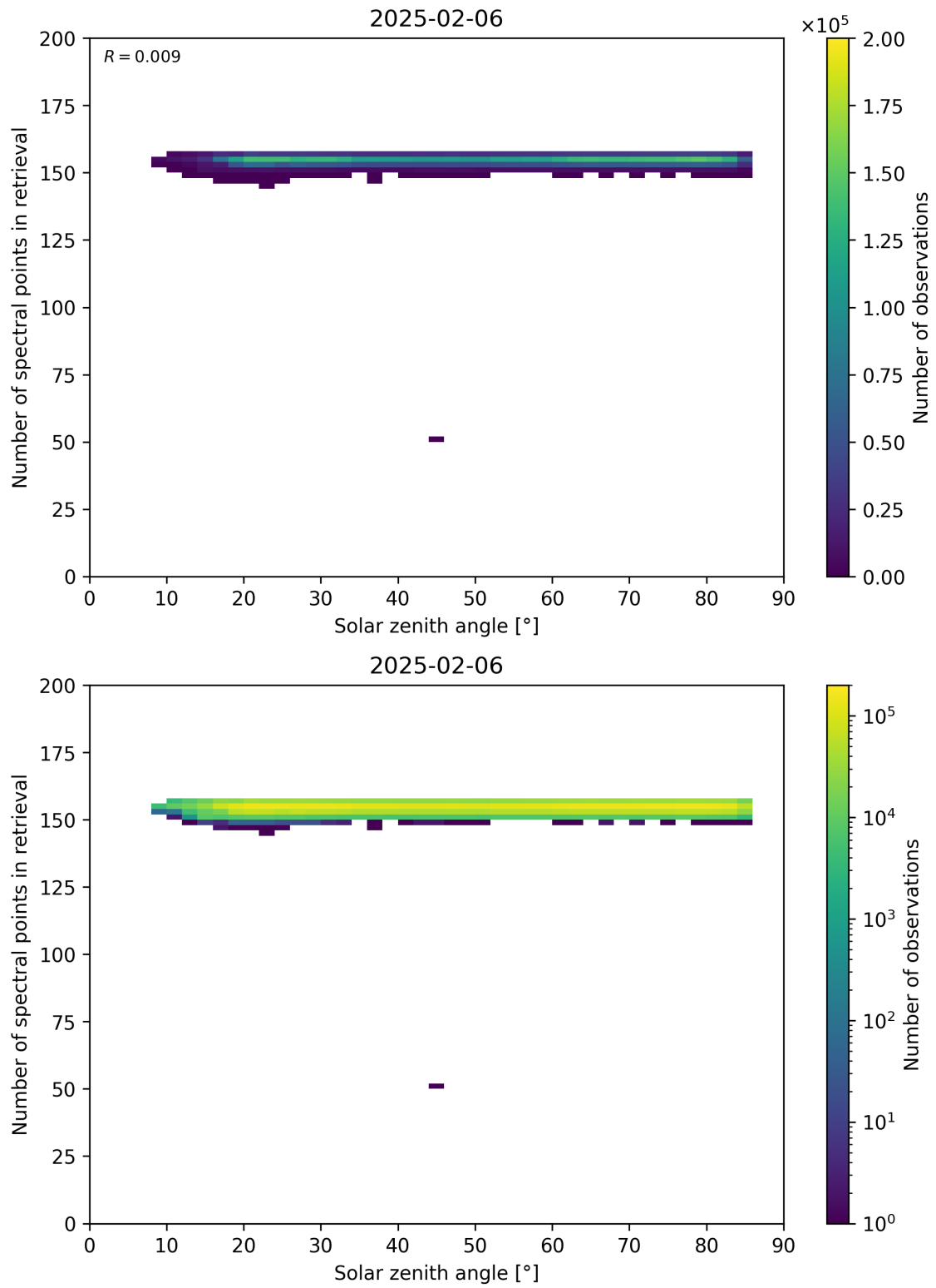
Figure 68: Scatter density plot of “Solar zenith angle” against “Number of spectral points in retrieval” for 2025-02-05 to 2025-02-07.
