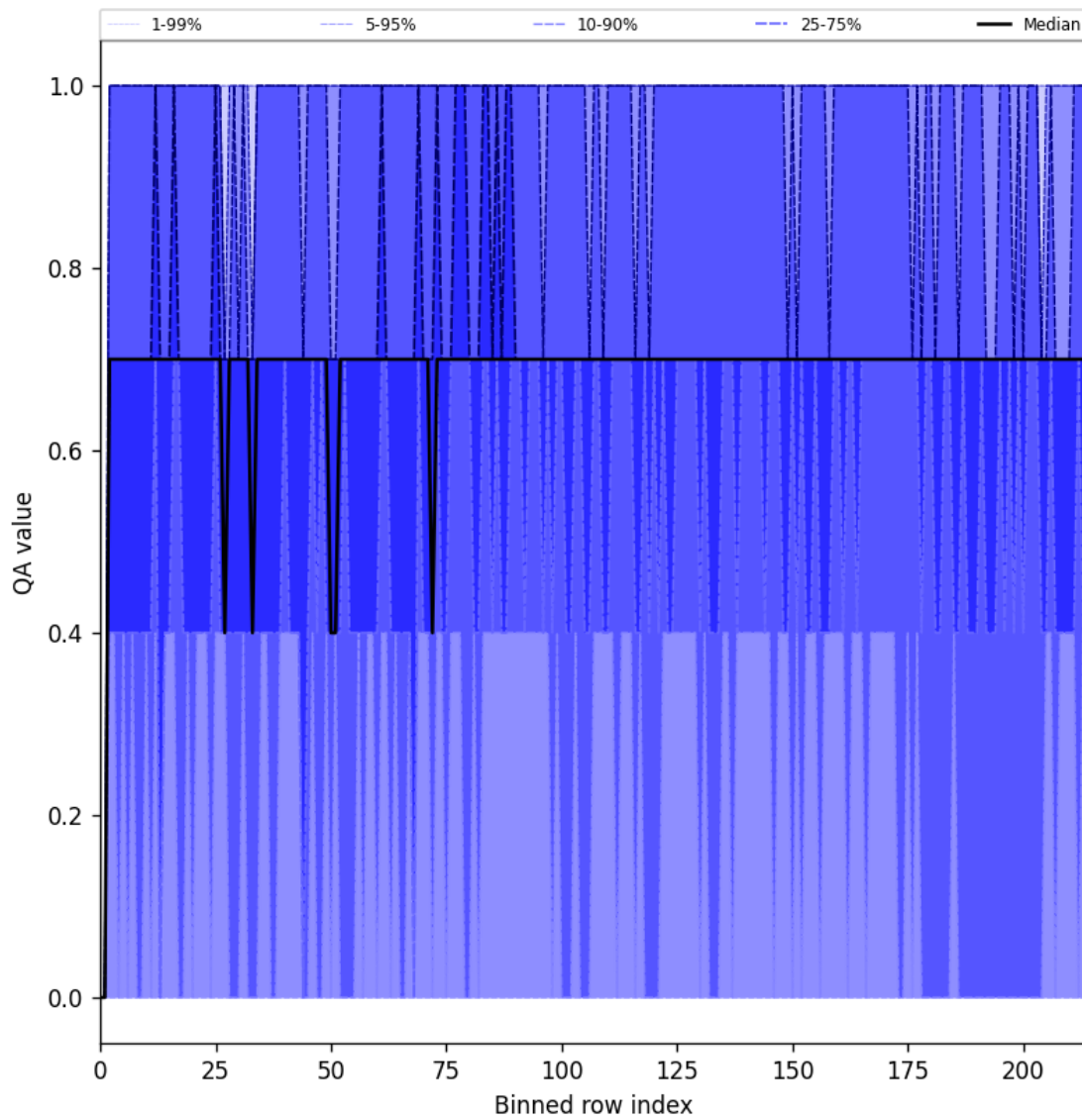
Figure 25: Along track statistics of “QA value” for 2025-02-05 to 2025-02-07
