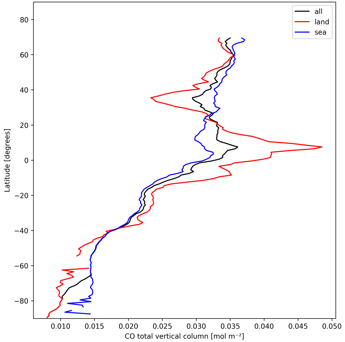
Figure 10: Zonal average of “CO total vertical column” for 2025-02-05 to 2025-02-07.
