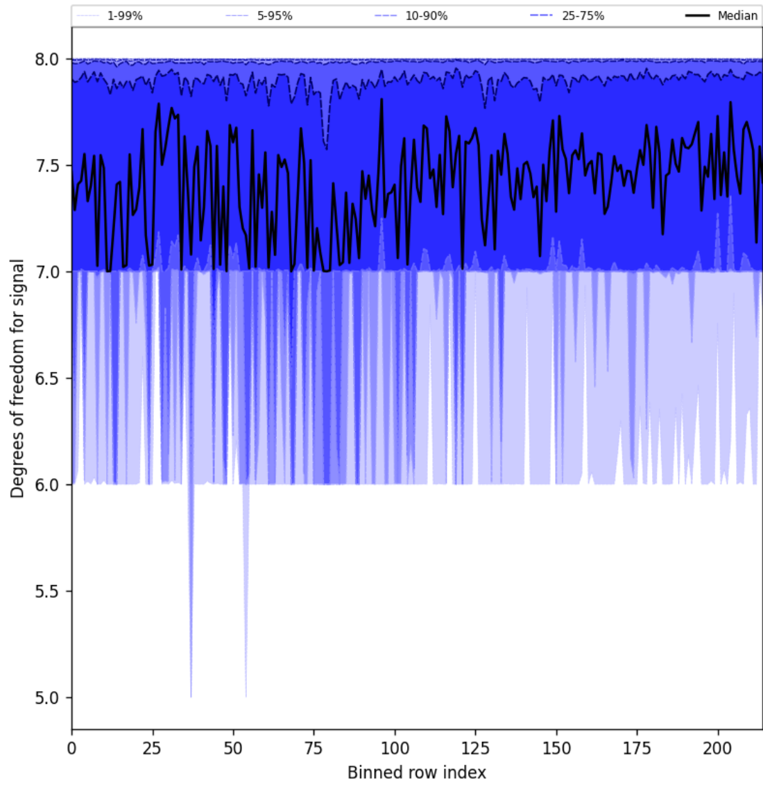
Figure 31: Along track statistics of “Degrees of freedom for signal” for 2025-02-05 to 2025-02-07
