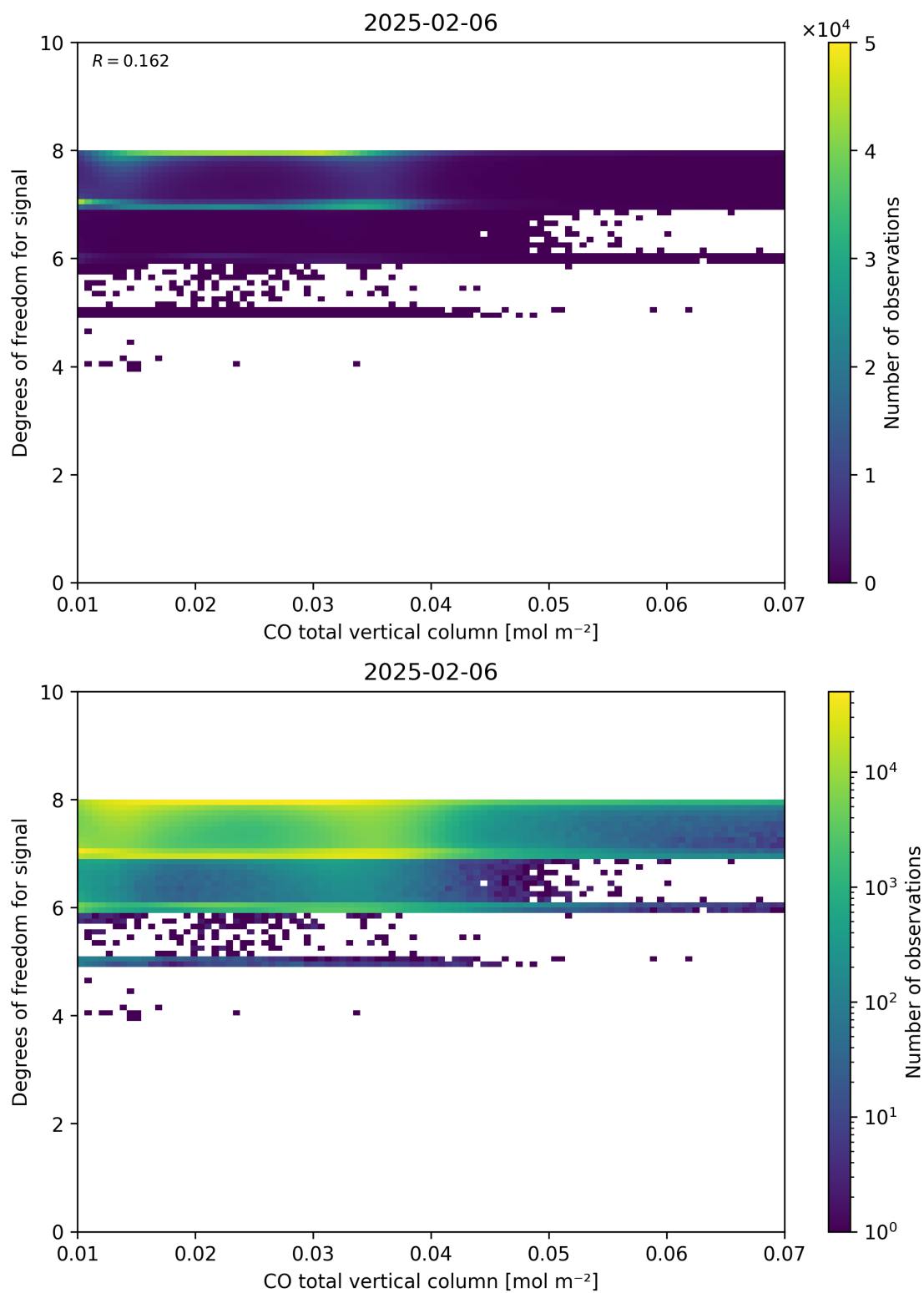
Figure 41: Scatter density plot of “CO total vertical column” against “Degrees of freedom for signal” for 2025-02-05 to 2025-02-07.
