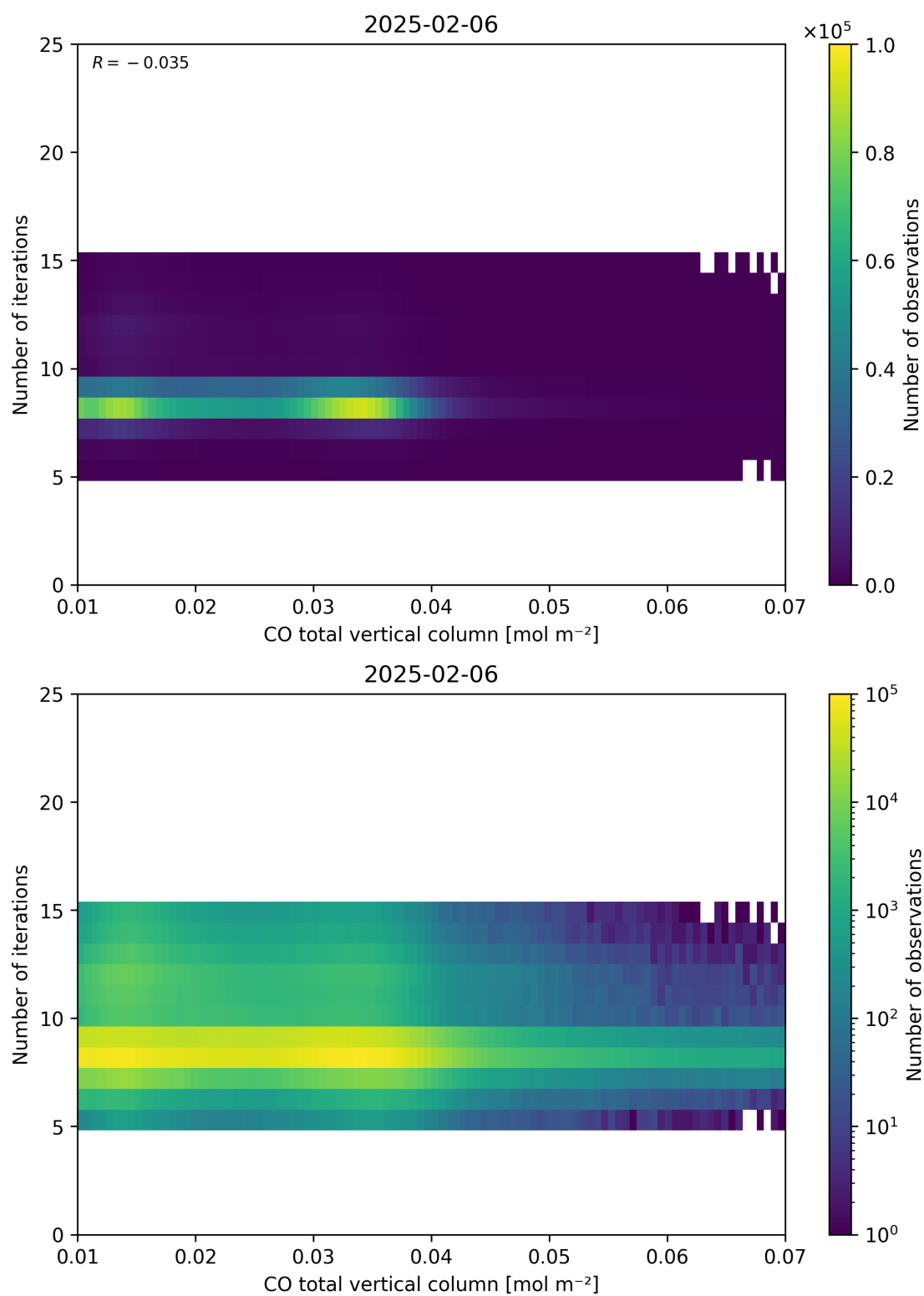
Figure 42: Scatter density plot of “CO total vertical column” against “Number of iterations” for 2025-02-05 to 2025-02-07.
