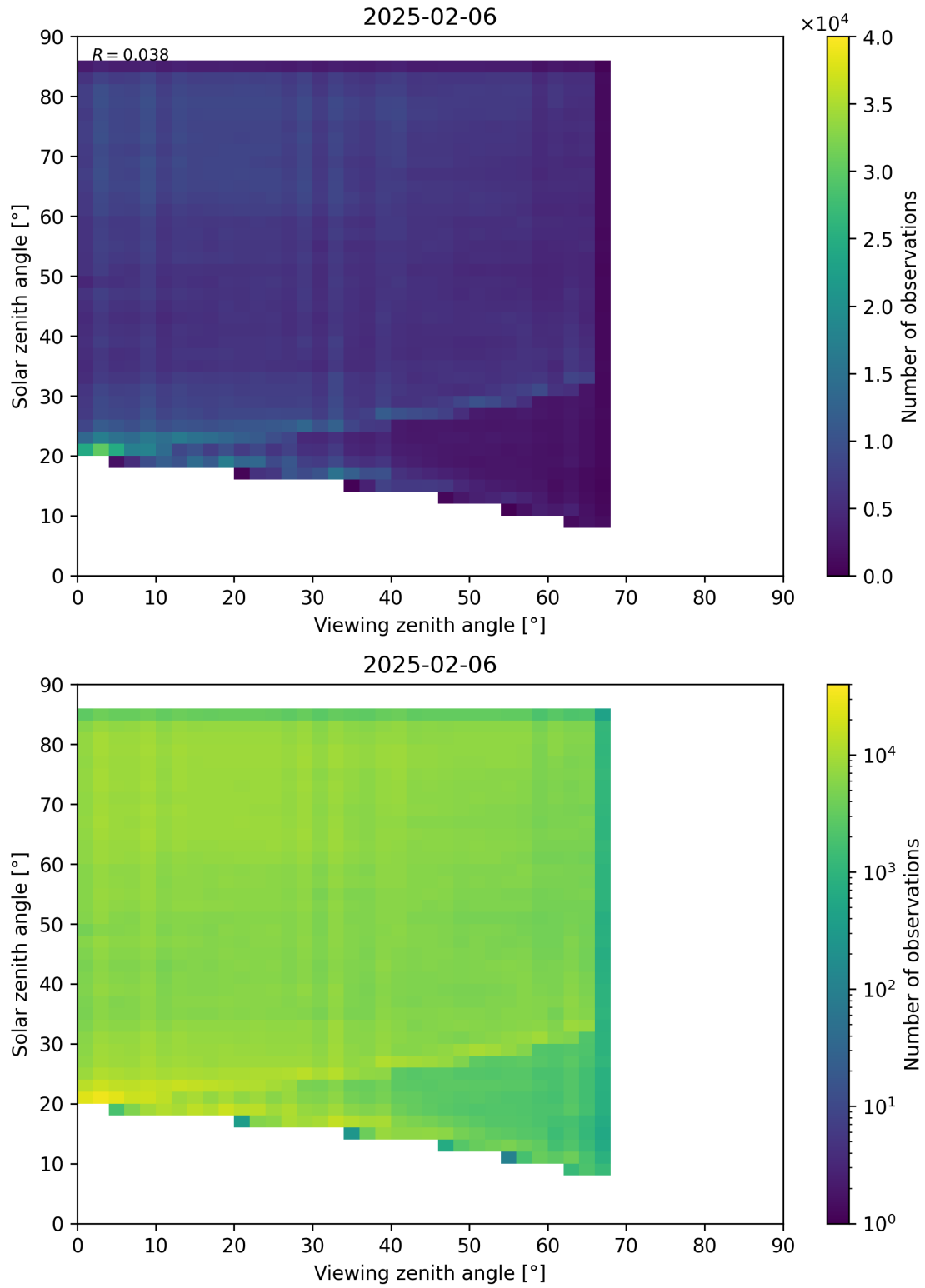
Figure 77: Scatter density plot of “Viewing zenith angle” against “Solar zenith angle” for 2025-02-05 to 2025-02-07.
