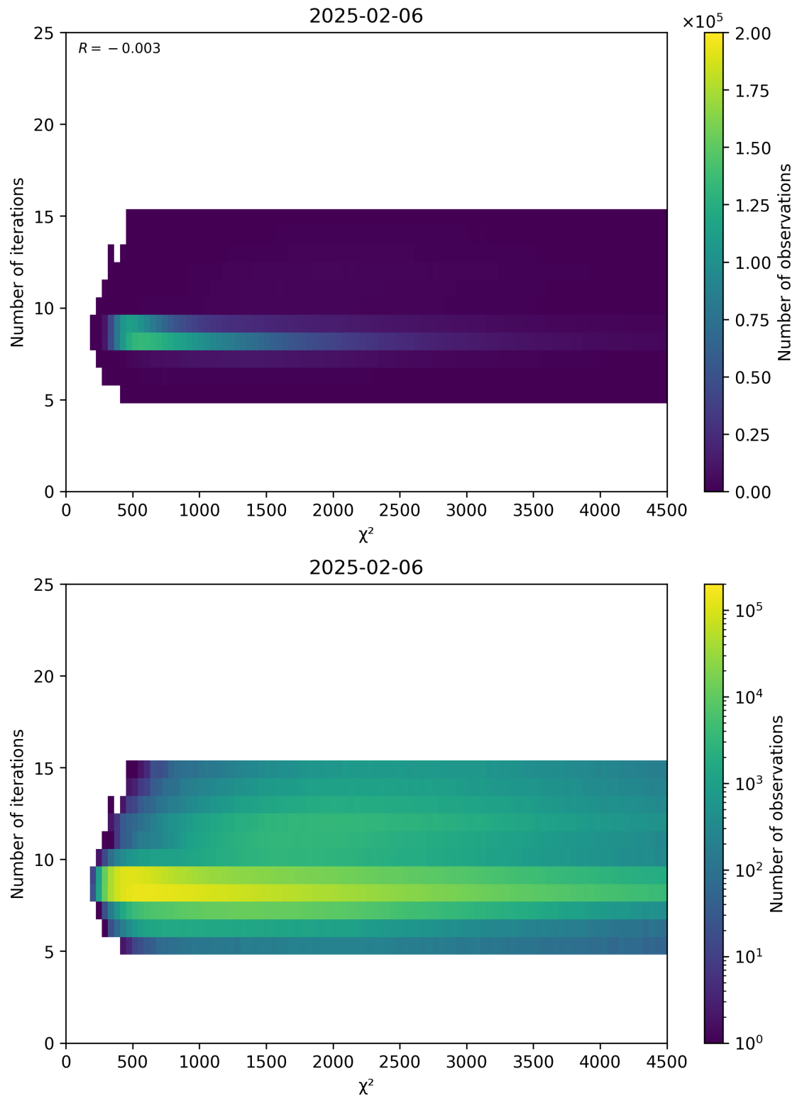
Figure 49: Scatter density plot of “ \chi^2 ” against “Number of iterations” for 2025-02-05 to 2025-02-07.
