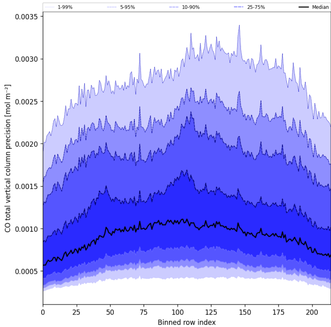
Figure 28: Along track statistics of “CO total vertical column precision” for 2025-02-05 to 2025-02-07
