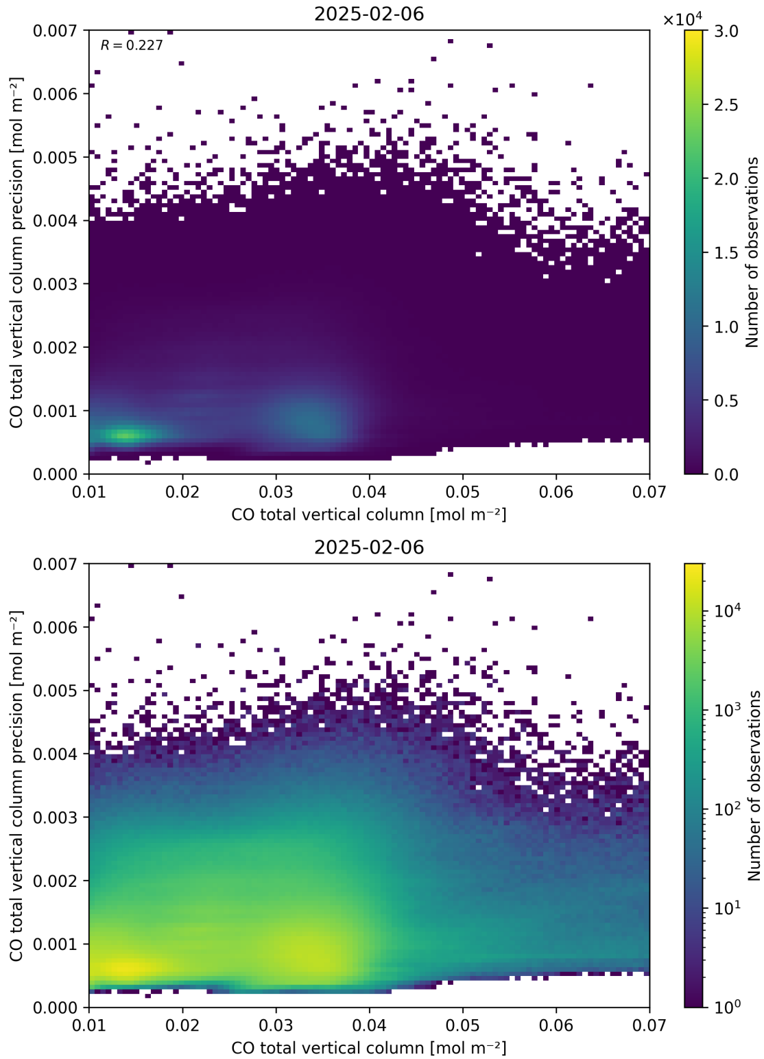
Figure 34: Scatter density plot of “CO total vertical column” against “CO total vertical column precision” for 2025-02-05 to 2025-02-07.
