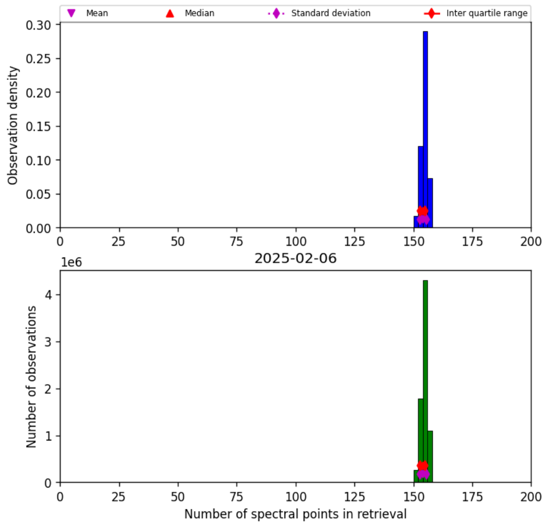
Figure 21: Histogram of “Number of spectral points in retrieval” for 2025-02-05 to 2025-02-07
