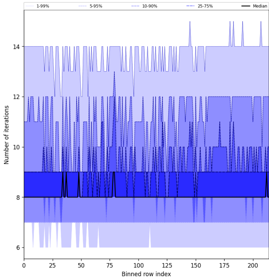
Figure 32: Along track statistics of “Number of iterations” for 2025-02-05 to 2025-02-07
