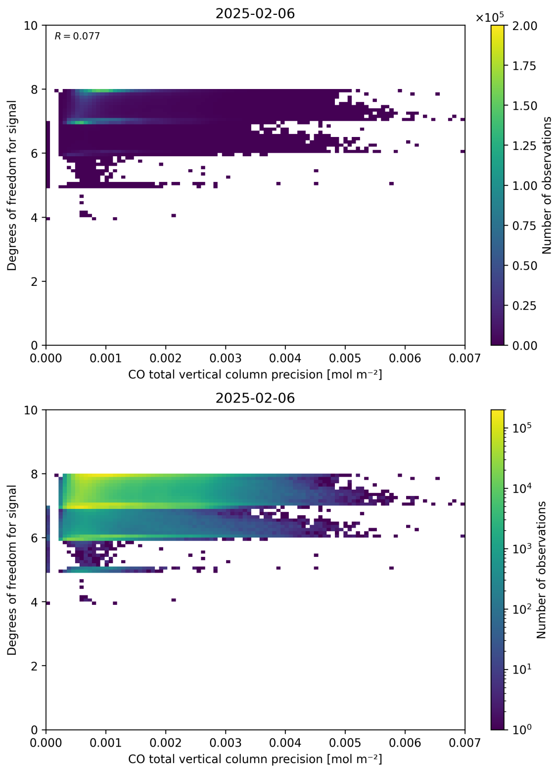
Figure 45: Scatter density plot of “CO total vertical column precision” against “Degrees of freedom for signal” for 2025-02-05 to 2025-02-07.
