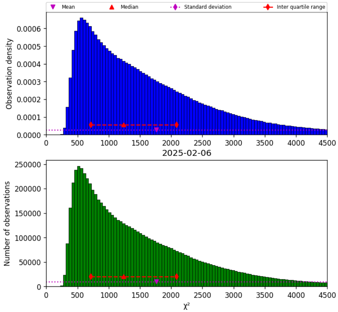
Figure 22: Histogram of “ \chi^2 ” for 2025-02-05 to 2025-02-07
