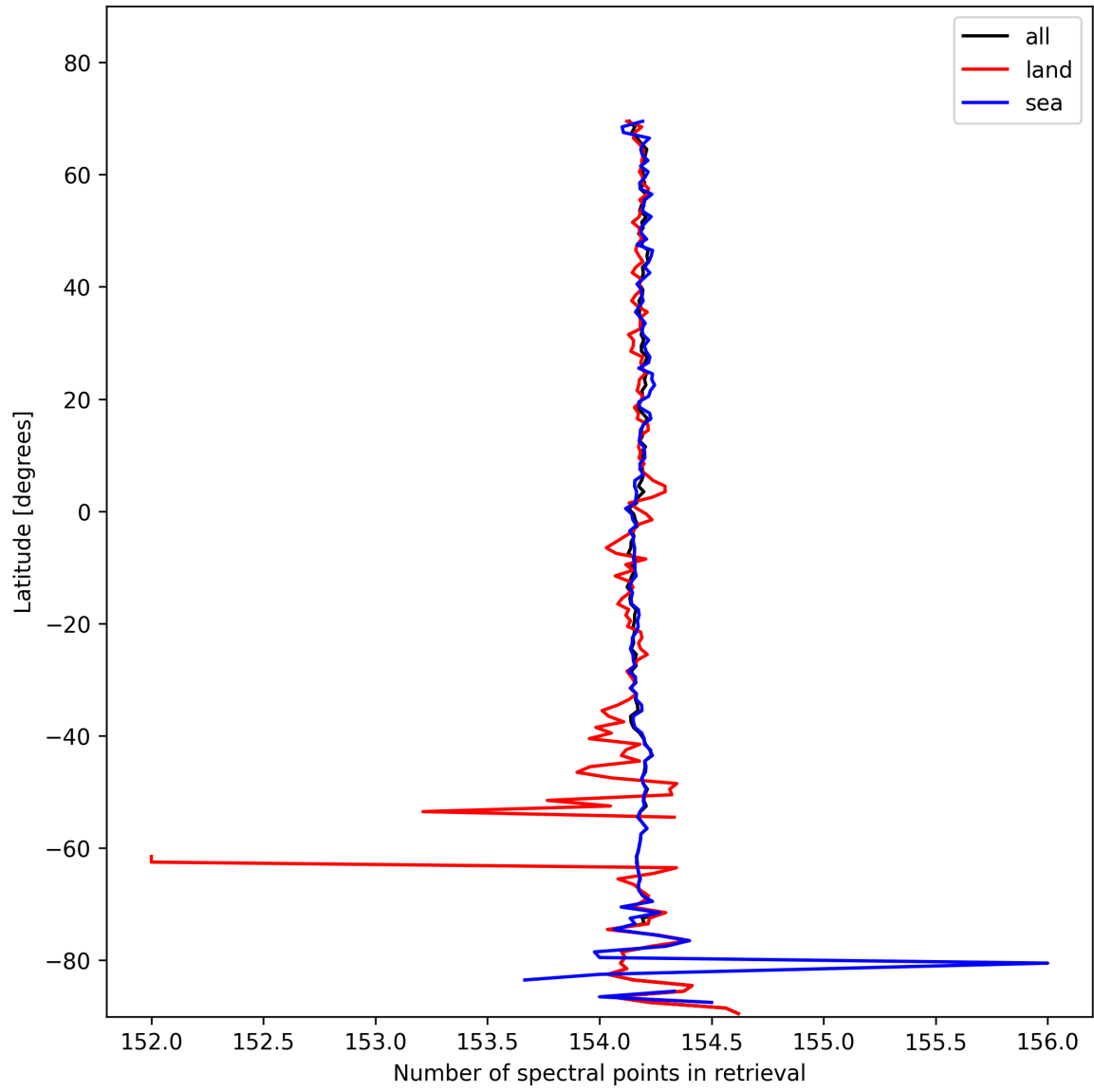
Figure 13: Zonal average of “Number of spectral points in retrieval” for 2025-02-05 to 2025-02-07.
