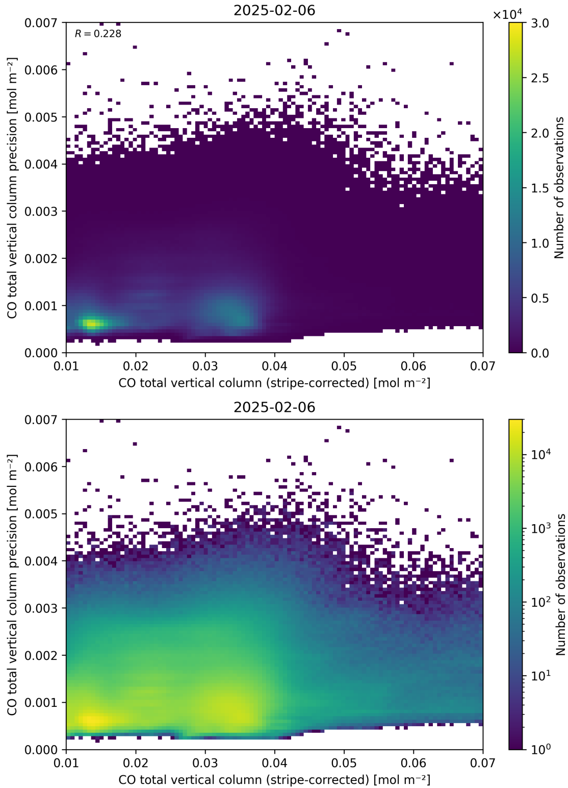
Figure 36: Scatter density plot of “CO total vertical column (stripe-corrected)” against “CO total vertical column precision” for 2025-02-05 to 2025-02-07.
