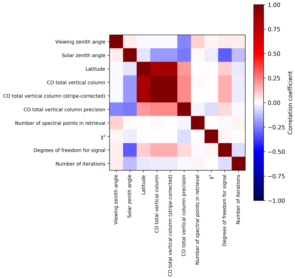
Figure 2: Map of correlation matrix for 2025-02-05 to 2025-02-07.
