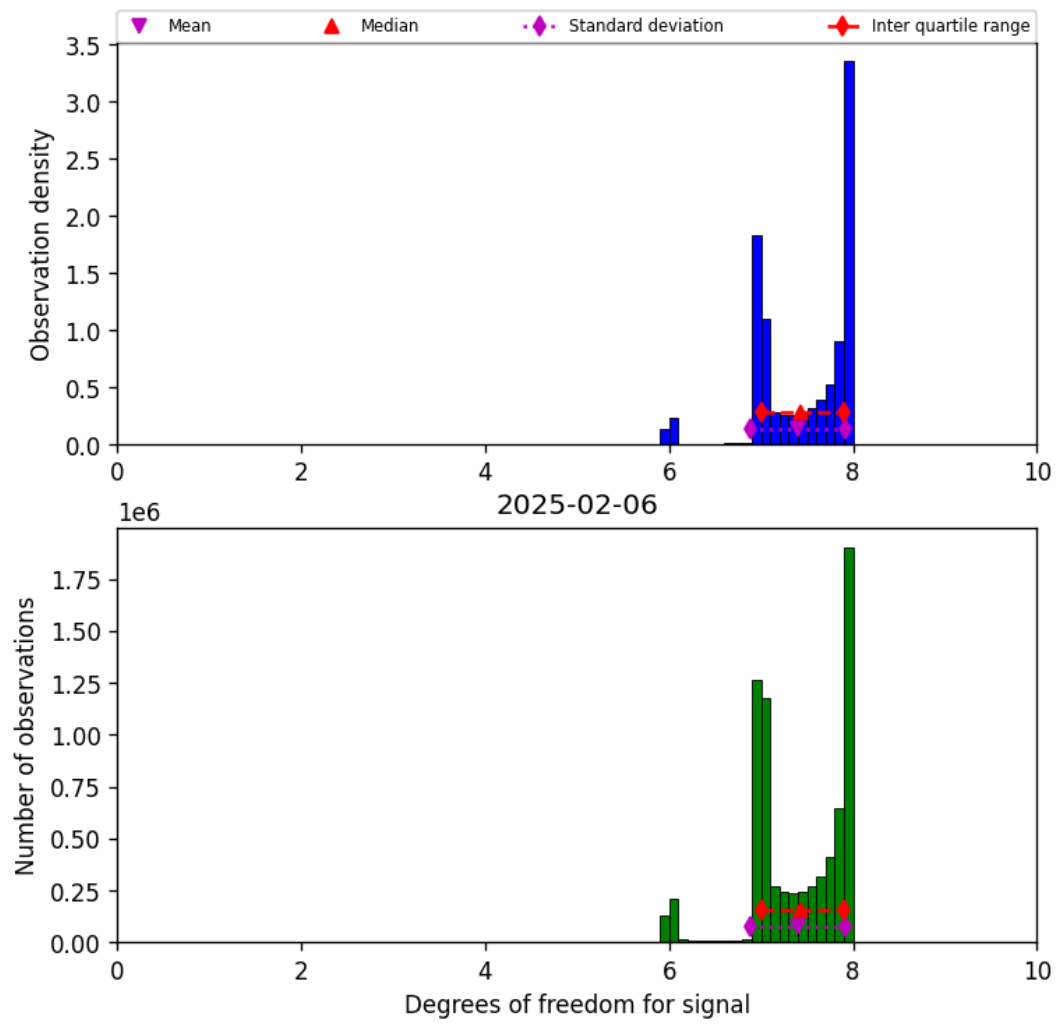
Figure 23: Histogram of “Degrees of freedom for signal” for 2025-02-05 to 2025-02-07
