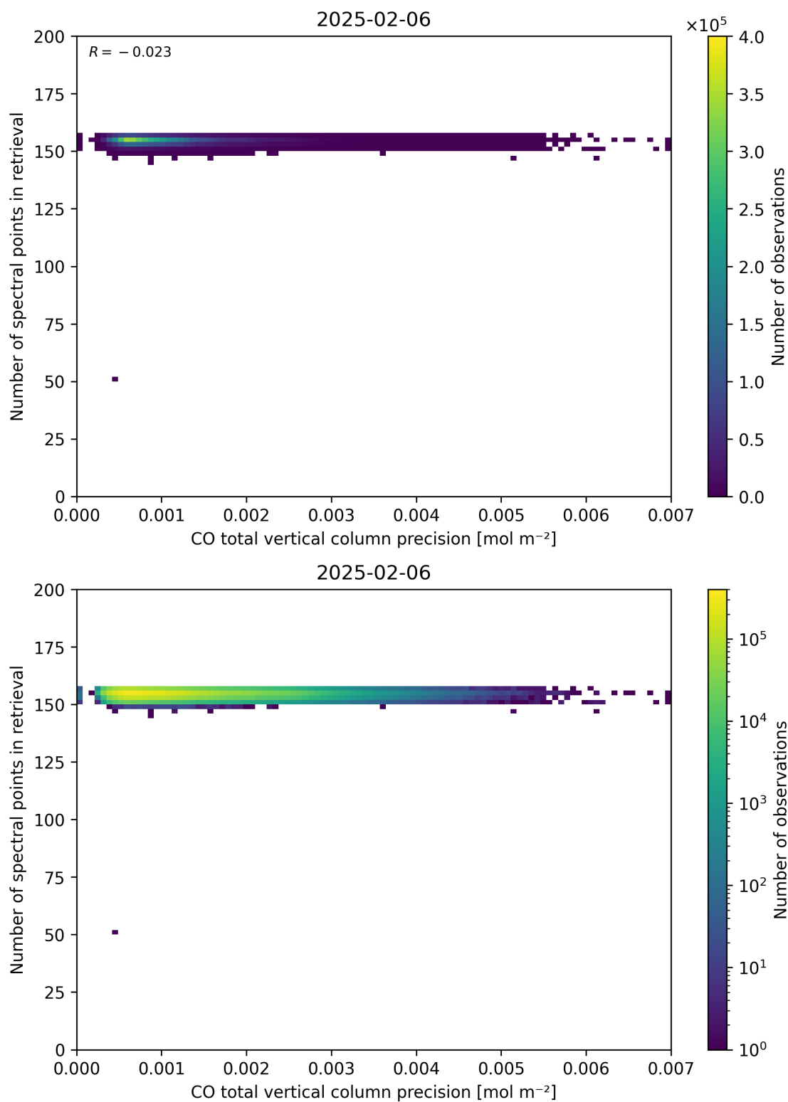
Figure 47: Scatter density plot of “CO total vertical column precision” against “Number of spectral points in retrieval” for 2025-02-05 to 2025-02-07.
