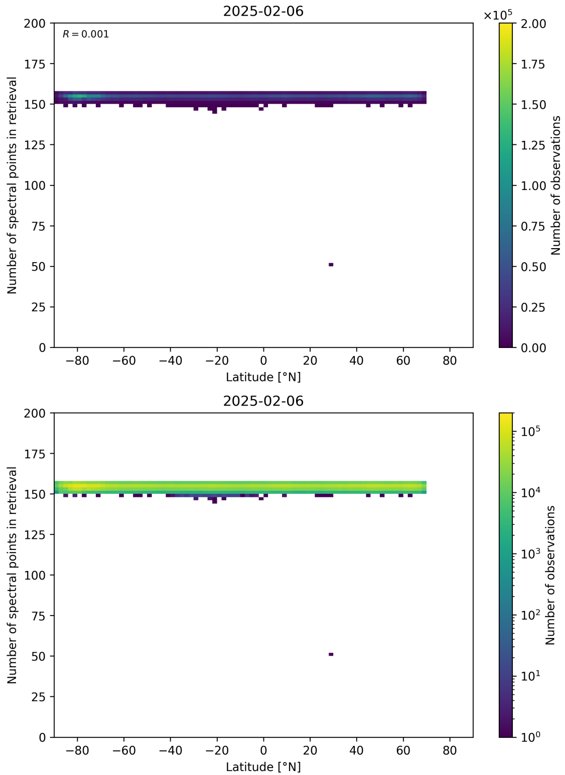
Figure 57: Scatter density plot of “Latitude” against “Number of spectral points in retrieval” for 2025-02-05 to 2025-02-07.
