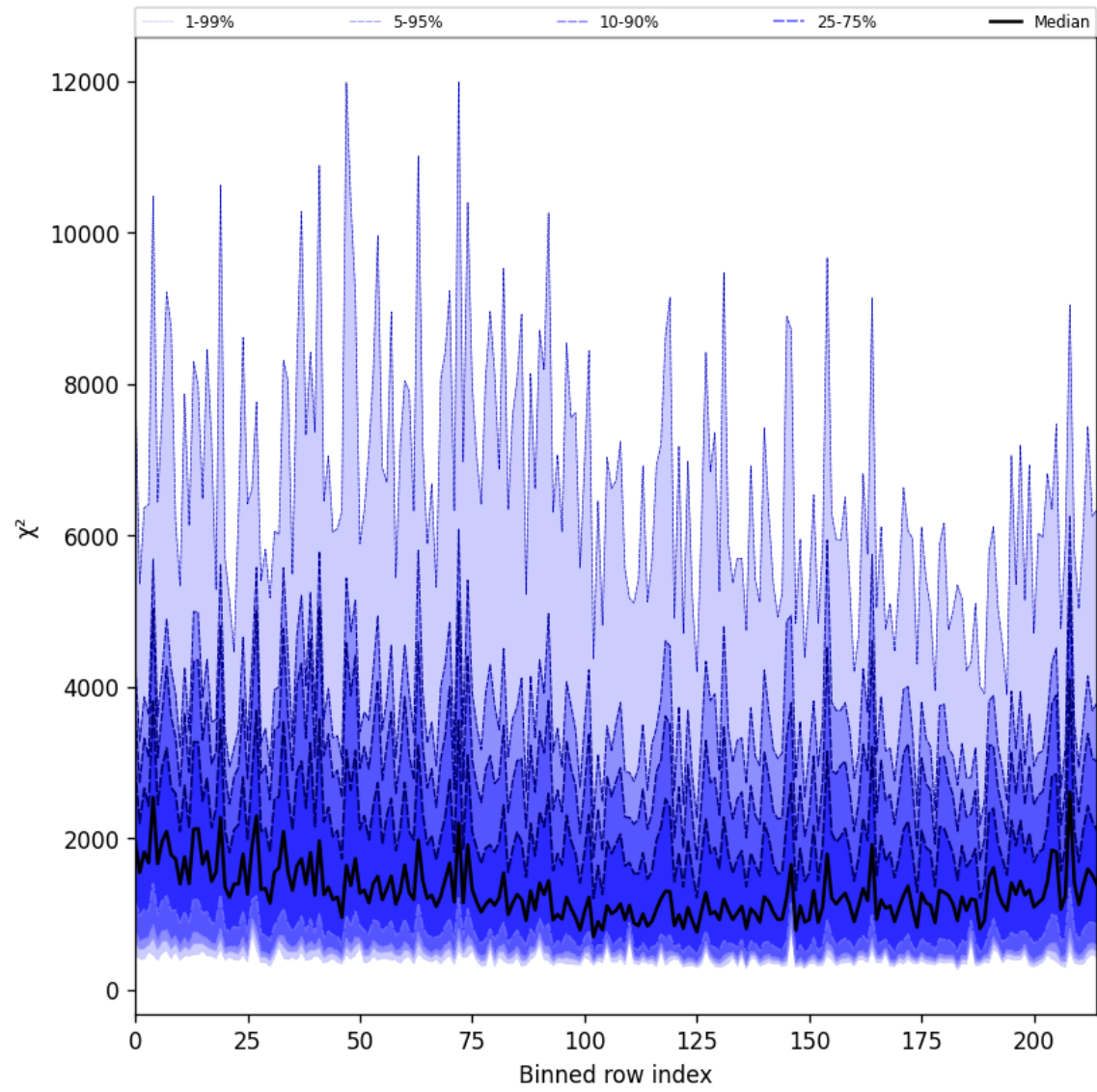
Figure 30: Along track statistics of “ \chi^2 ” for 2025-02-05 to 2025-02-07
