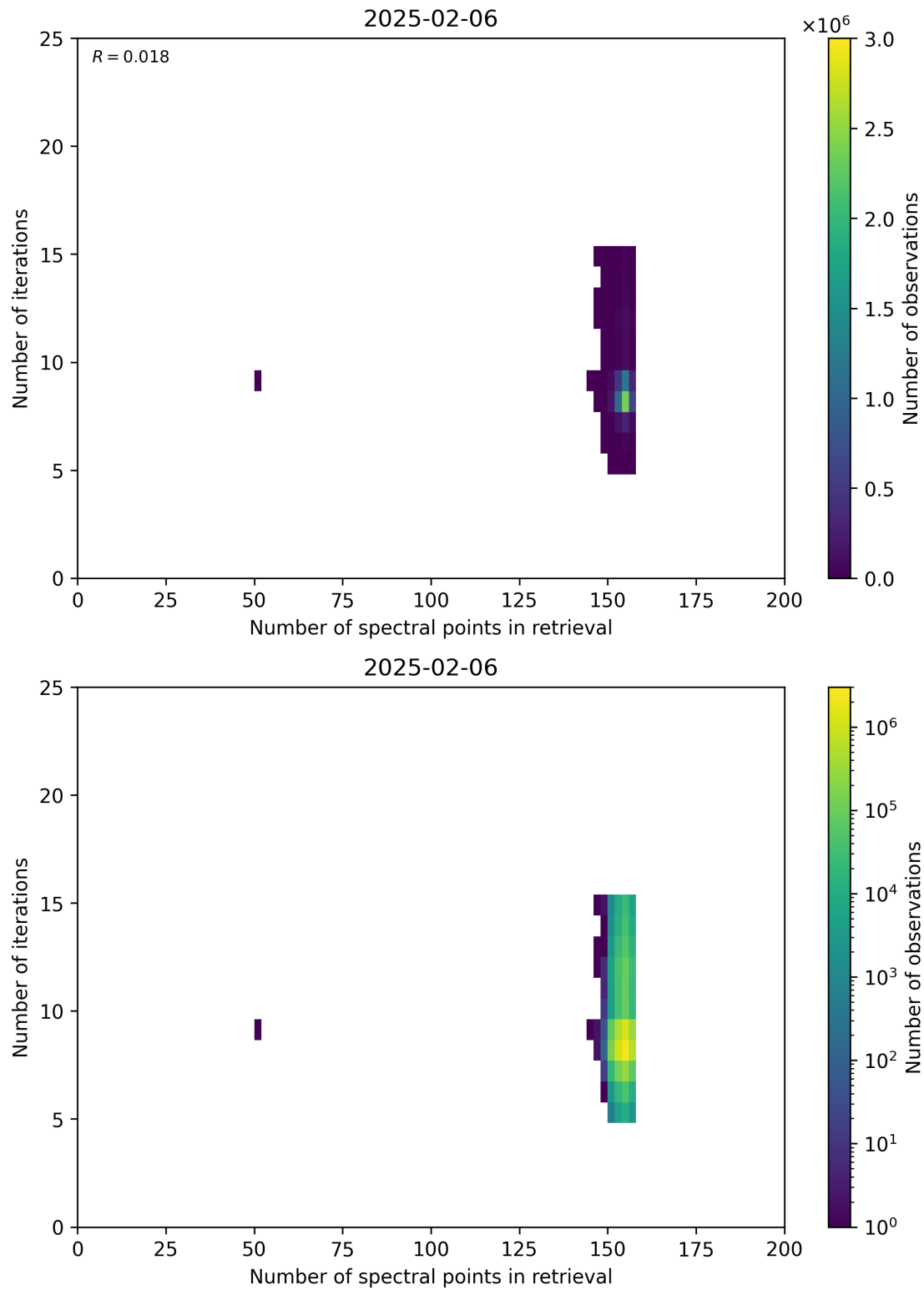
Figure 60: Scatter density plot of “Number of spectral points in retrieval” against “Number of iterations” for 2025-02-05 to 2025-02-07.
