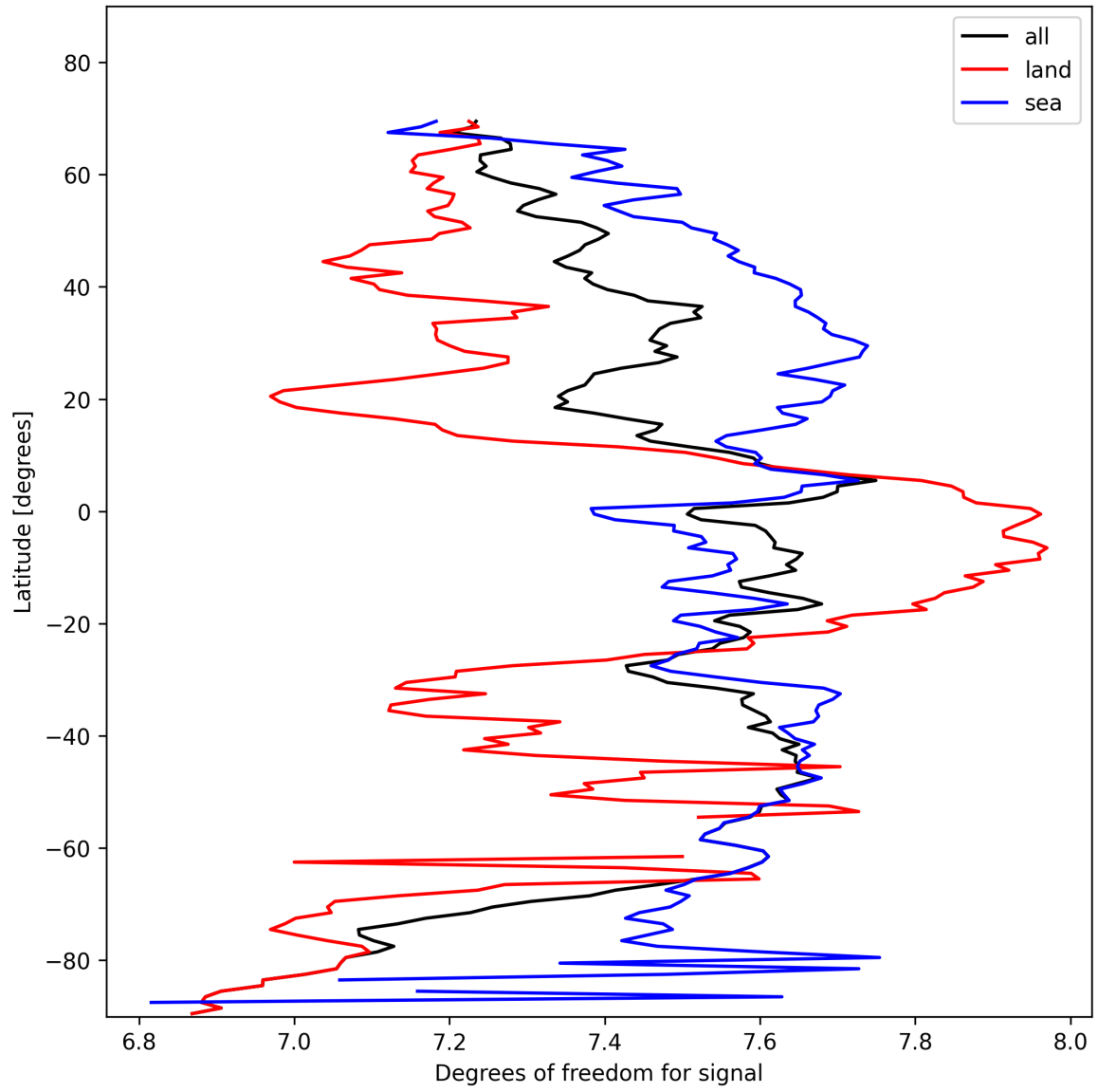
Figure 15: Zonal average of “Degrees of freedom for signal” for 2025-02-05 to 2025-02-07.
