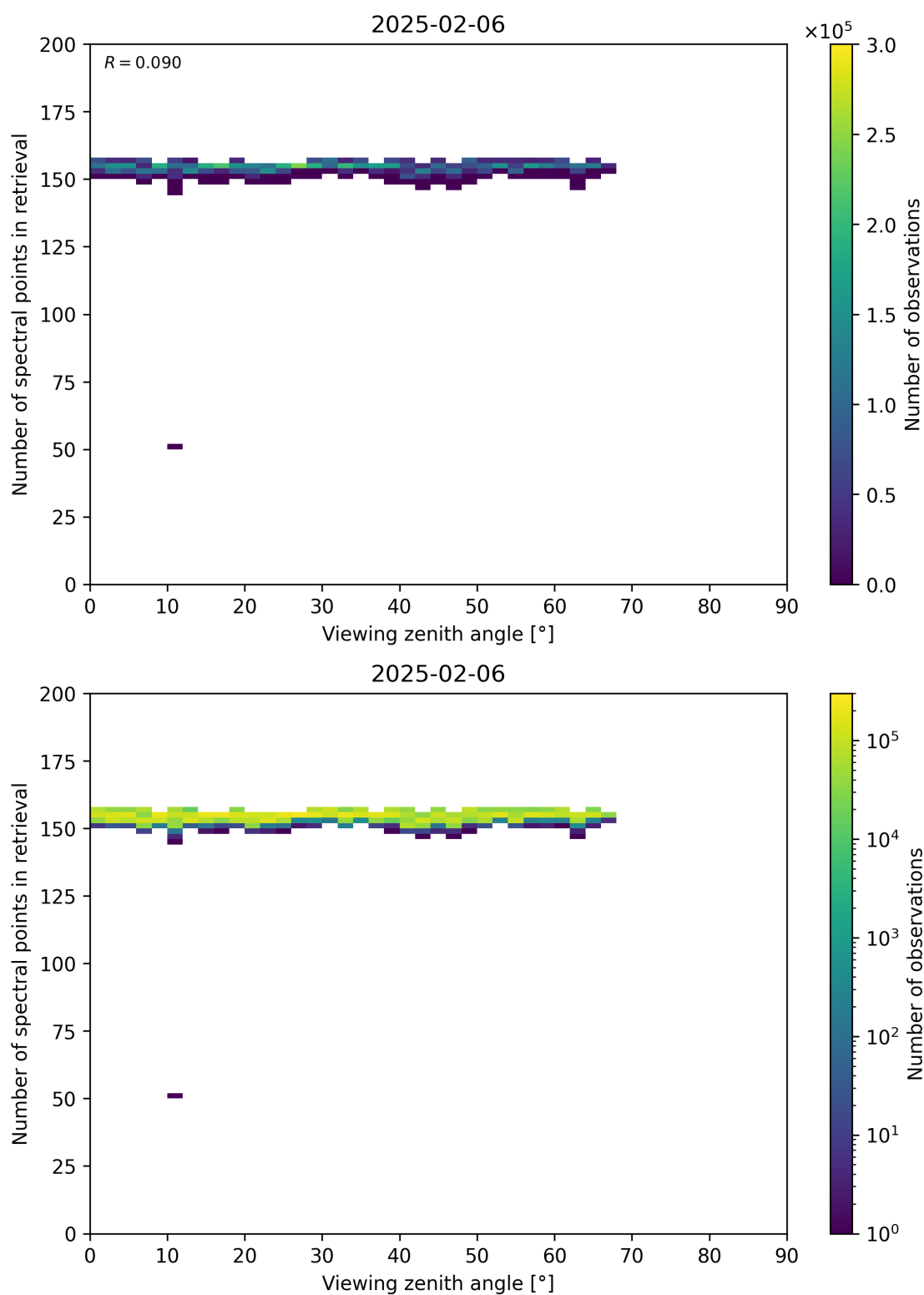
Figure 76: Scatter density plot of “Viewing zenith angle” against “Number of spectral points in retrieval” for 2025-02-05 to 2025-02-07.
