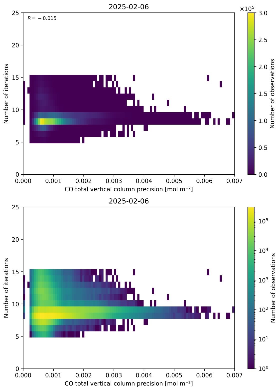
Figure 46: Scatter density plot of “CO total vertical column precision” against “Number of iterations” for 2025-02-05 to 2025-02-07.
