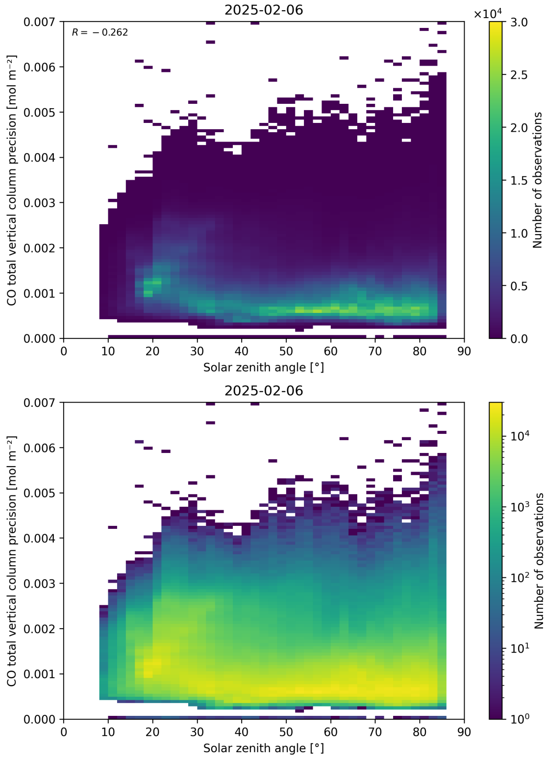
Figure 63: Scatter density plot of “Solar zenith angle” against “CO total vertical column precision” for 2025-02-05 to 2025-02-07.
