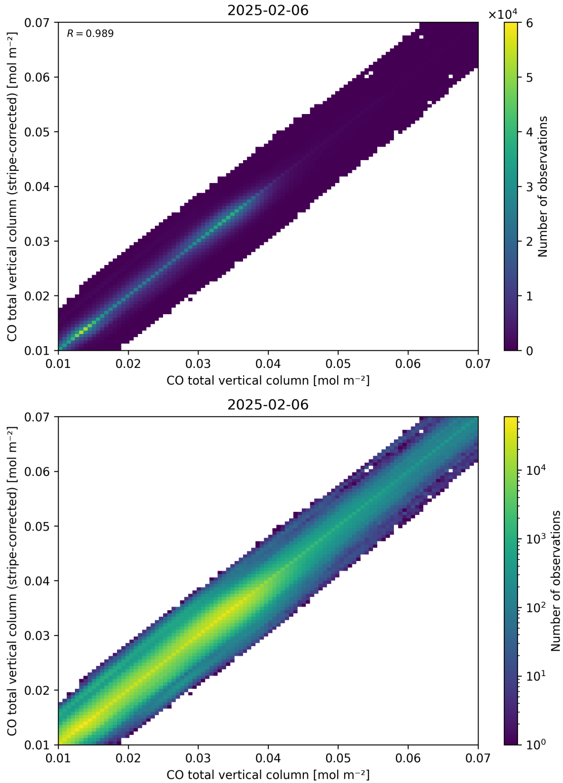
Figure 33: Scatter density plot of “CO total vertical column” against “CO total vertical column (stripe-corrected)” for 2025-02-05 to 2025-02-07.
