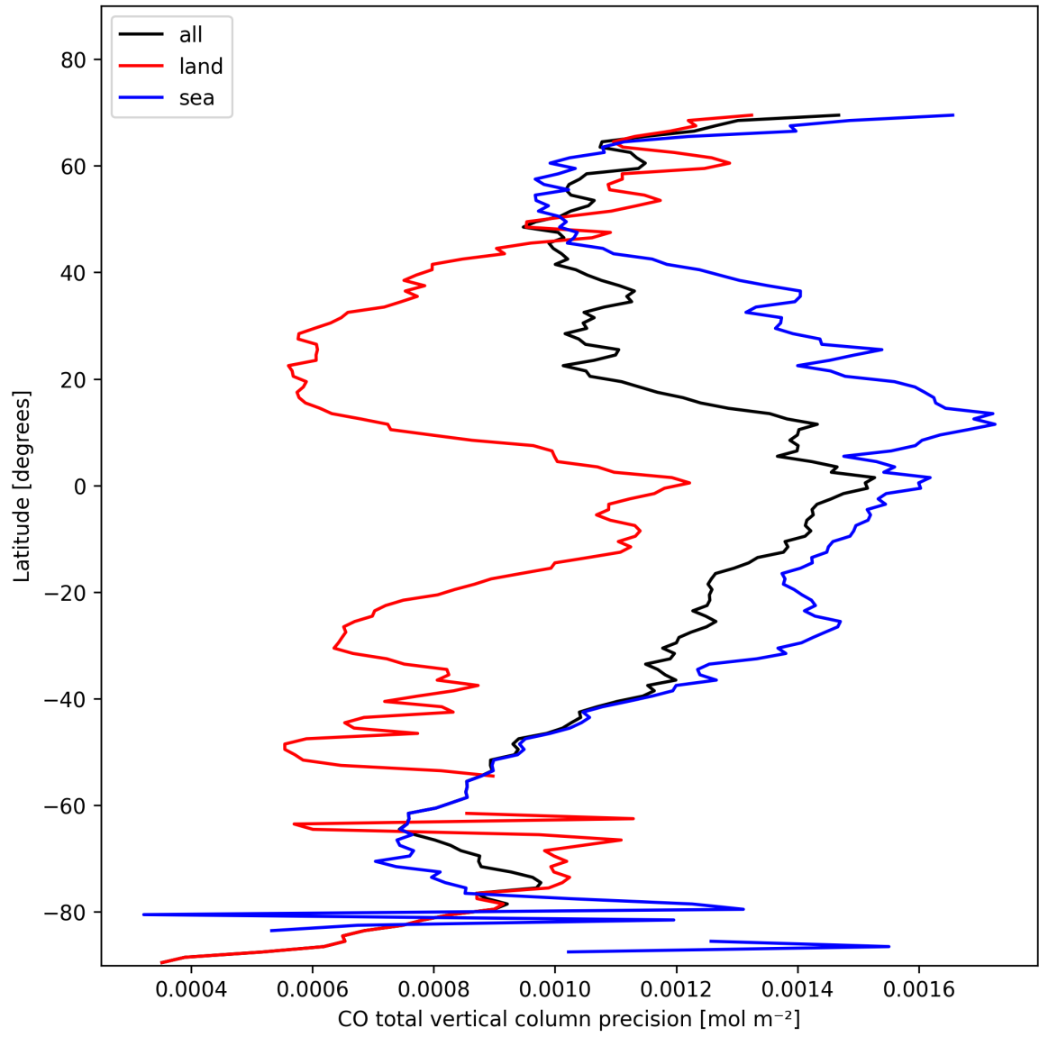
Figure 12: Zonal average of “CO total vertical column precision” for 2025-02-05 to 2025-02-07.
