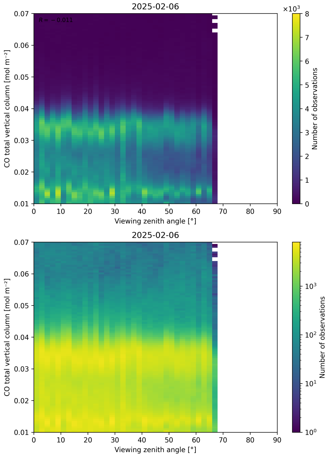
Figure 69: Scatter density plot of “Viewing zenith angle” against “CO total vertical column” for 2025-02-05 to 2025-02-07.
