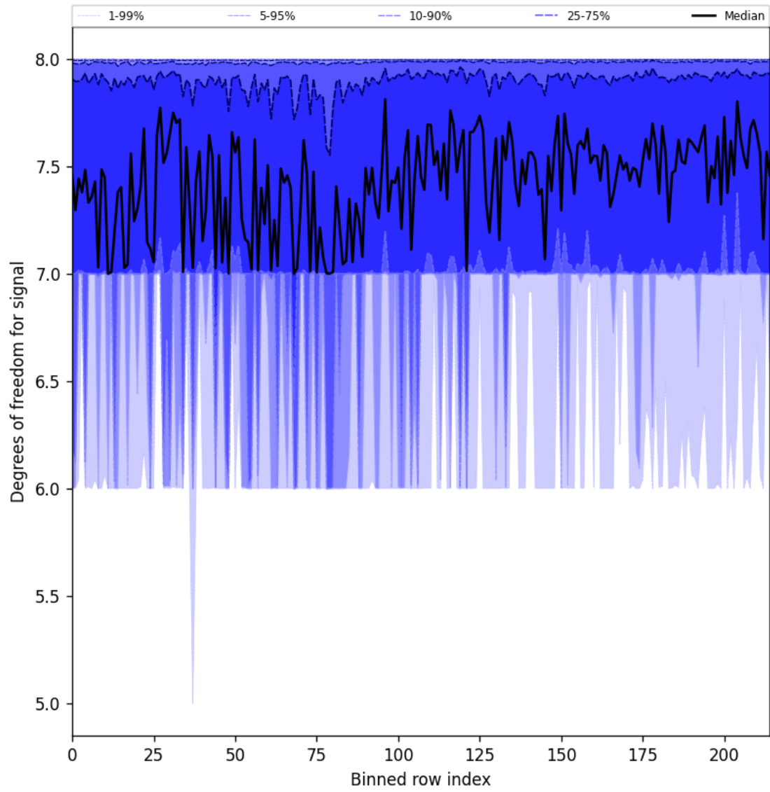
Figure 31: Along track statistics of “Degrees of freedom for signal” for 2025-02-06 to 2025-02-08
