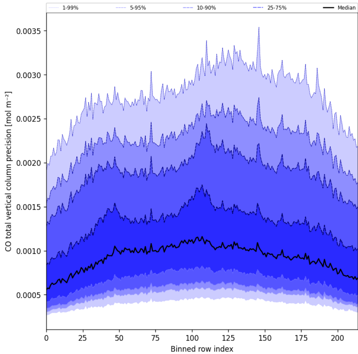
Figure 28: Along track statistics of “CO total vertical column precision” for 2025-02-06 to 2025-02-08
