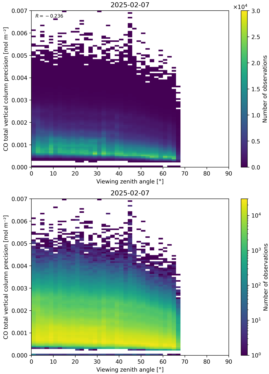
Figure 71: Scatter density plot of “Viewing zenith angle” against “CO total vertical column precision” for 2025-02-06 to 2025-02-08.
