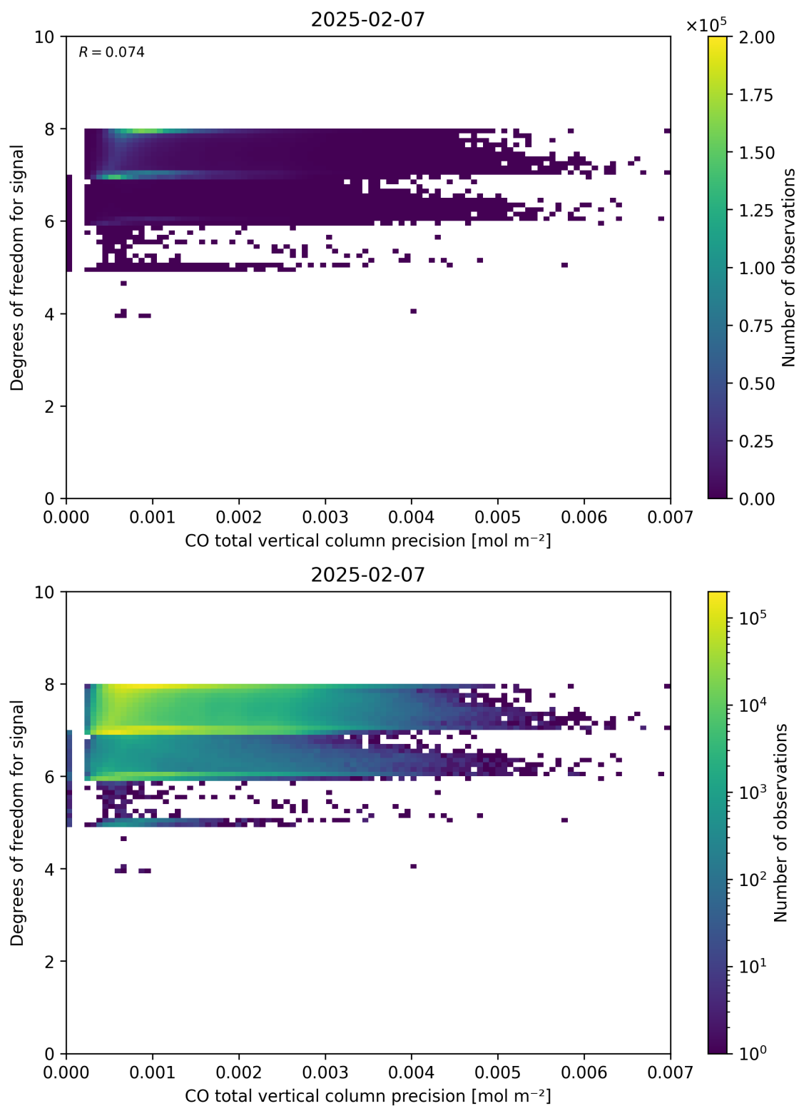
Figure 45: Scatter density plot of “CO total vertical column precision” against “Degrees of freedom for signal” for 2025-02-06 to 2025-02-08.
