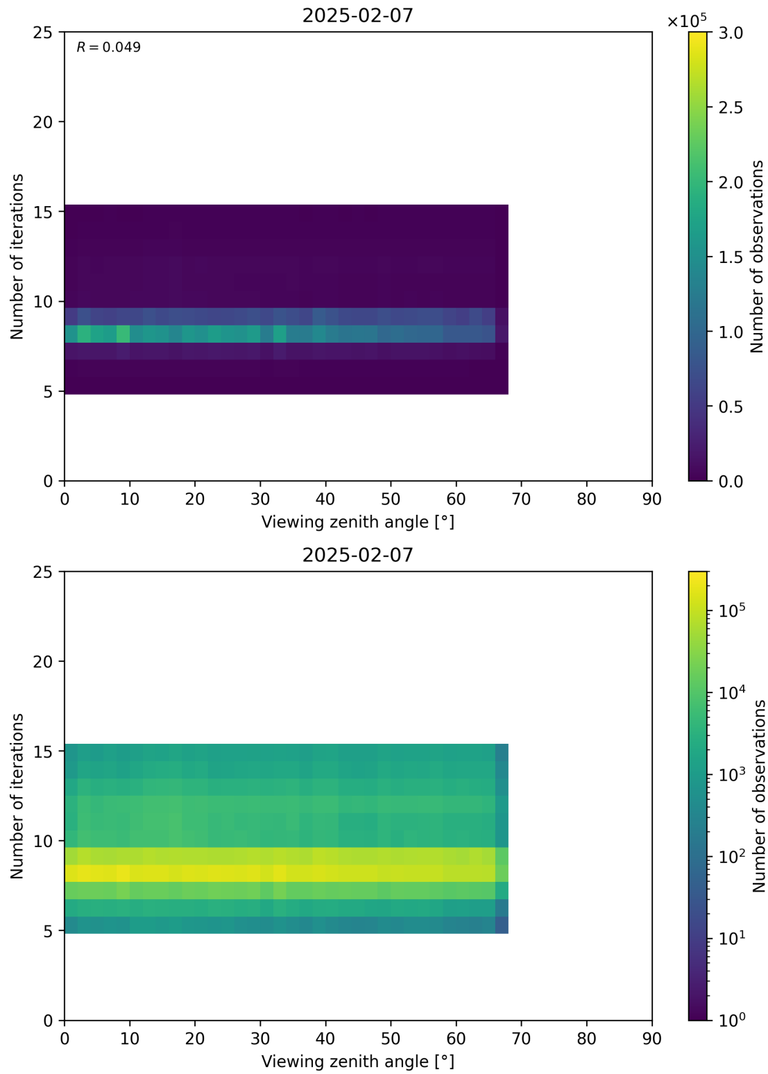
Figure 75: Scatter density plot of “Viewing zenith angle” against “Number of iterations” for 2025-02-06 to 2025-02-08.
