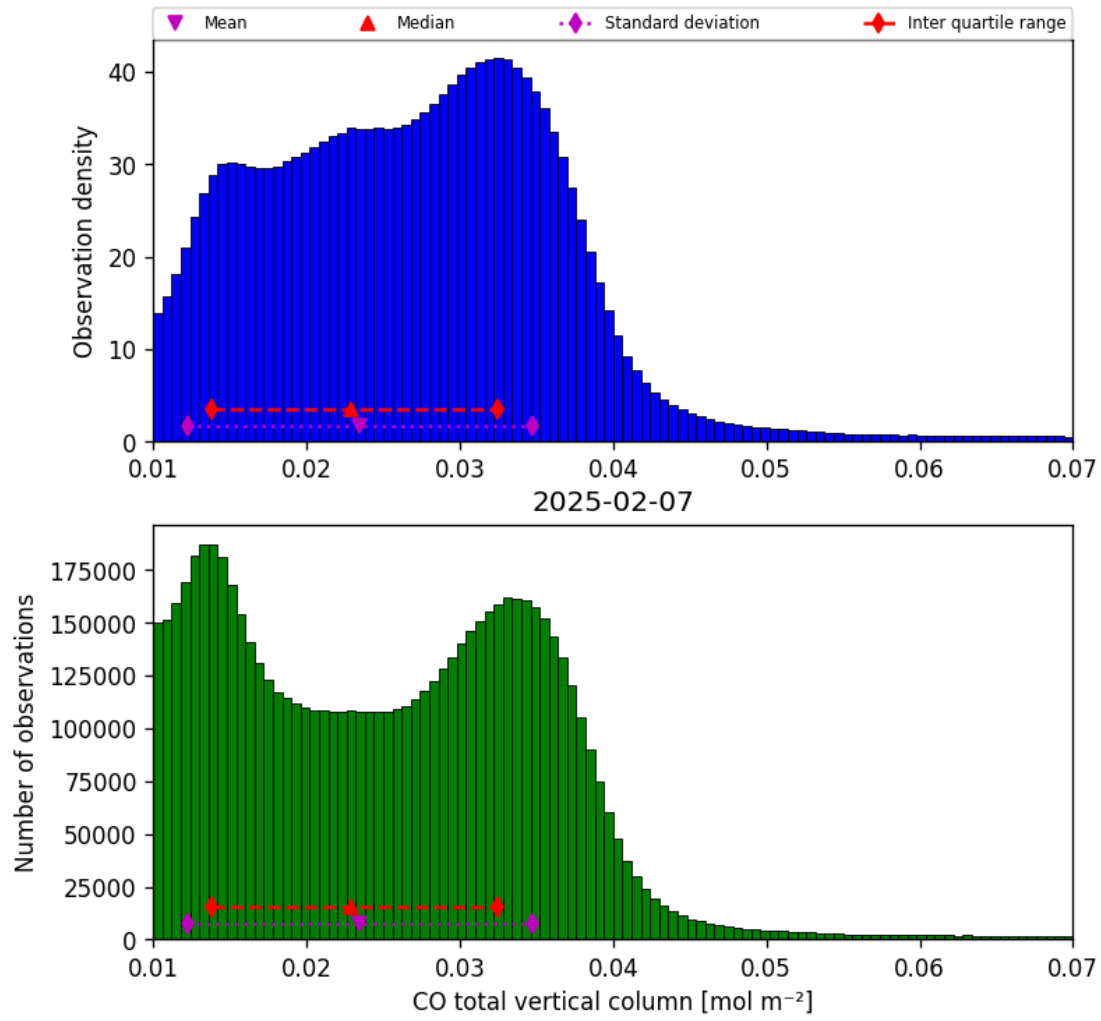
Figure 18: Histogram of “CO total vertical column” for 2025-02-06 to 2025-02-08
