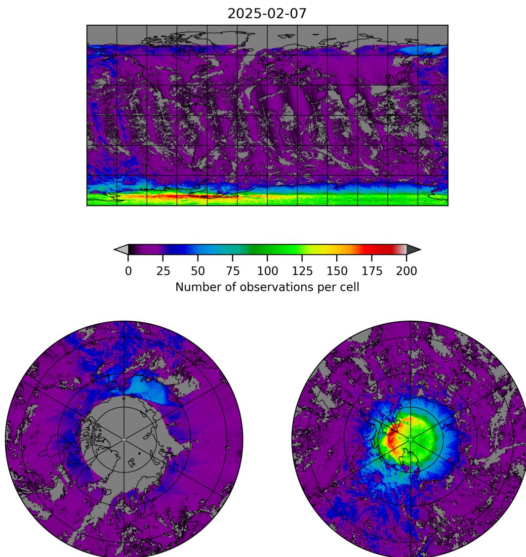
Figure 8: Map of the number of observations for 2025-02-06 to 2025-02-08
