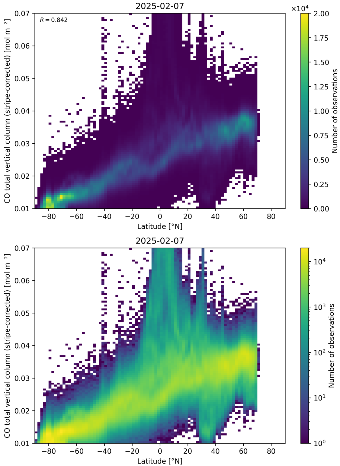
Figure 52: Scatter density plot of “Latitude” against “CO total vertical column (stripe-corrected)” for 2025-02-06 to 2025-02-08.
