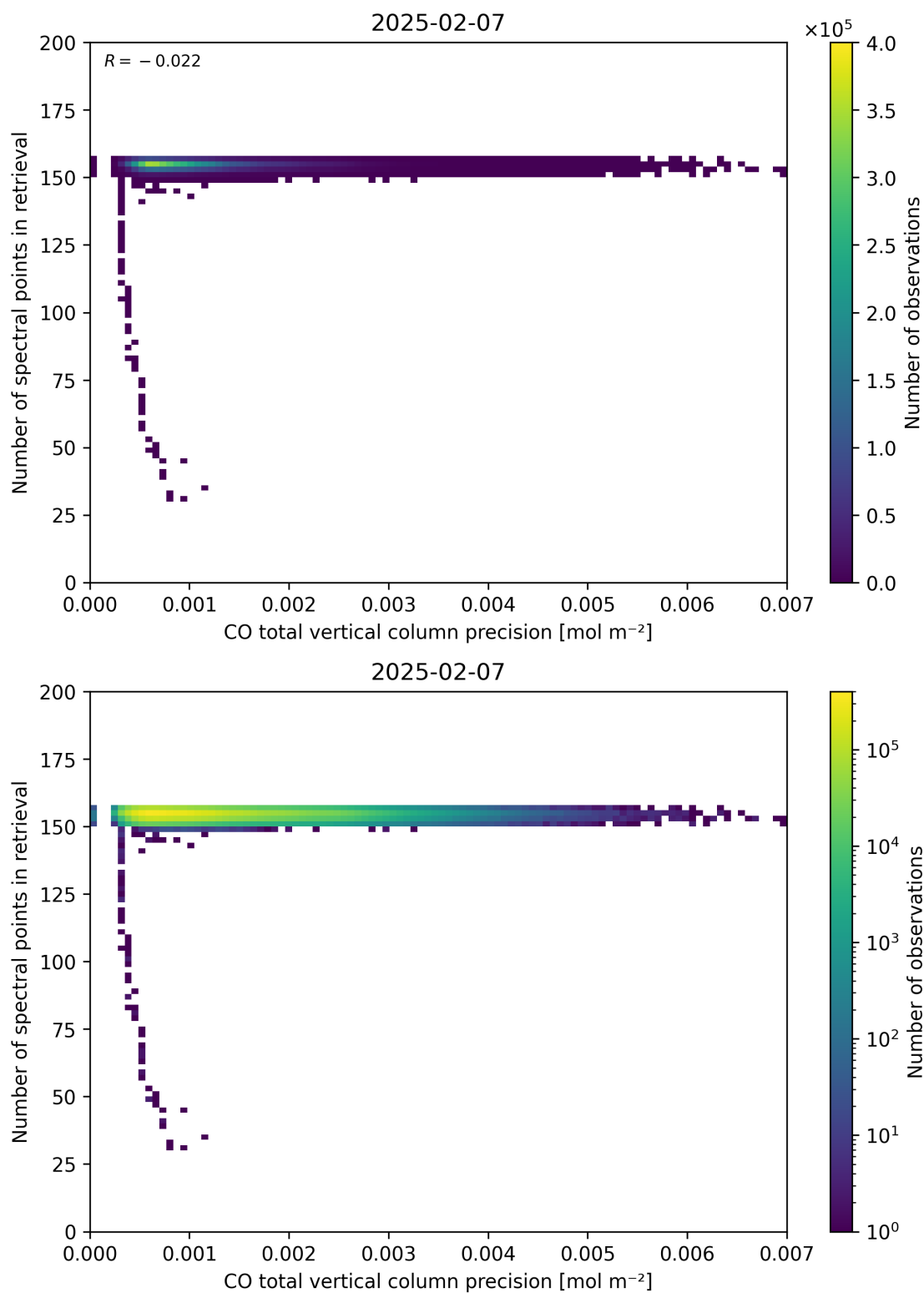
Figure 47: Scatter density plot of “CO total vertical column precision” against “Number of spectral points in retrieval” for 2025-02-06 to 2025-02-08.
