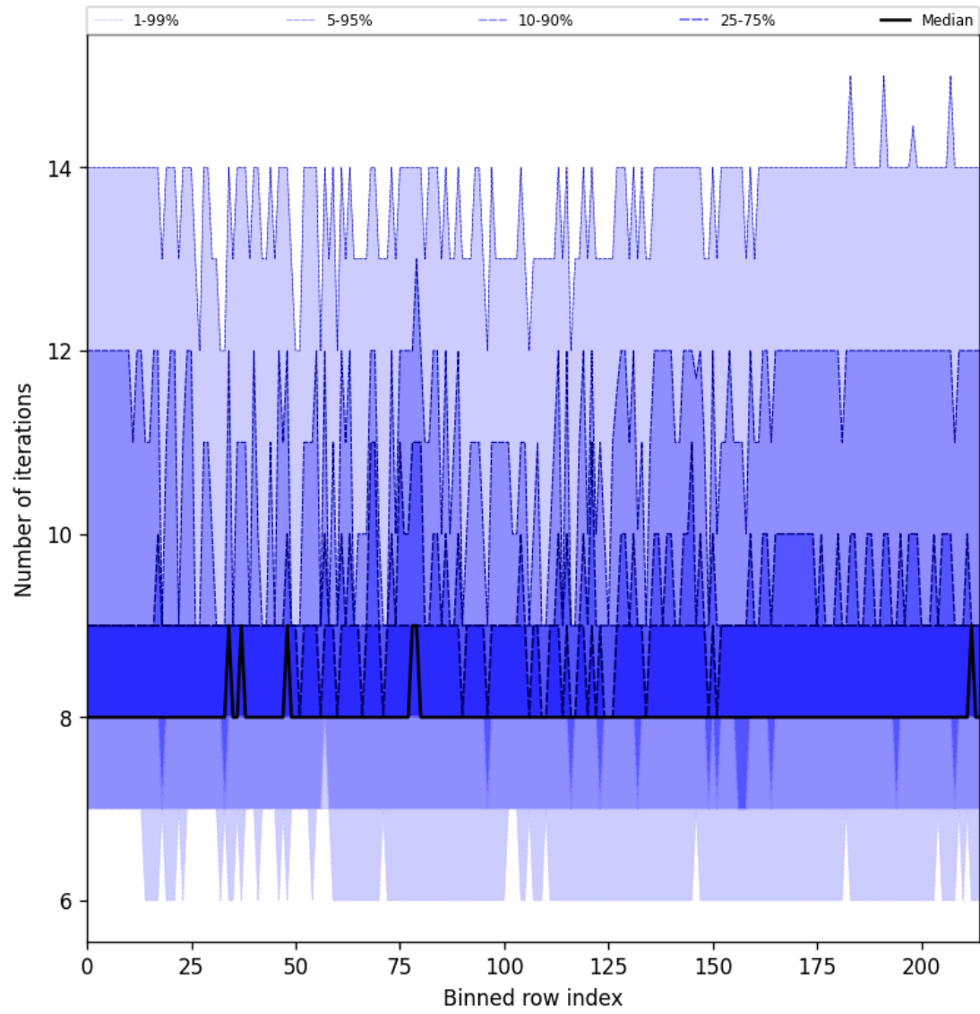
Figure 32: Along track statistics of “Number of iterations” for 2025-02-06 to 2025-02-08
