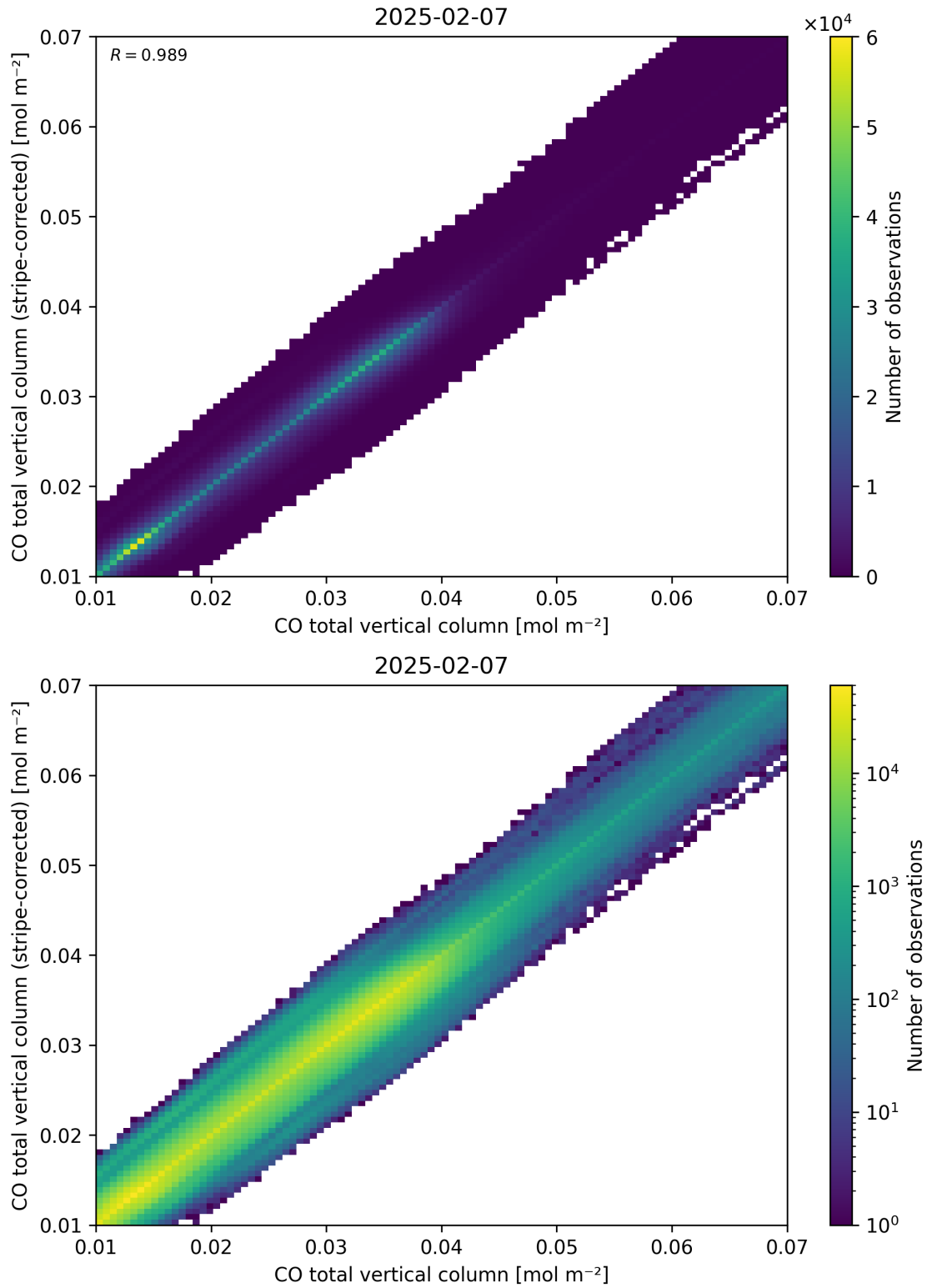
Figure 33: Scatter density plot of “CO total vertical column” against “CO total vertical column (stripe-corrected)” for 2025-02-06 to 2025-02-08.
