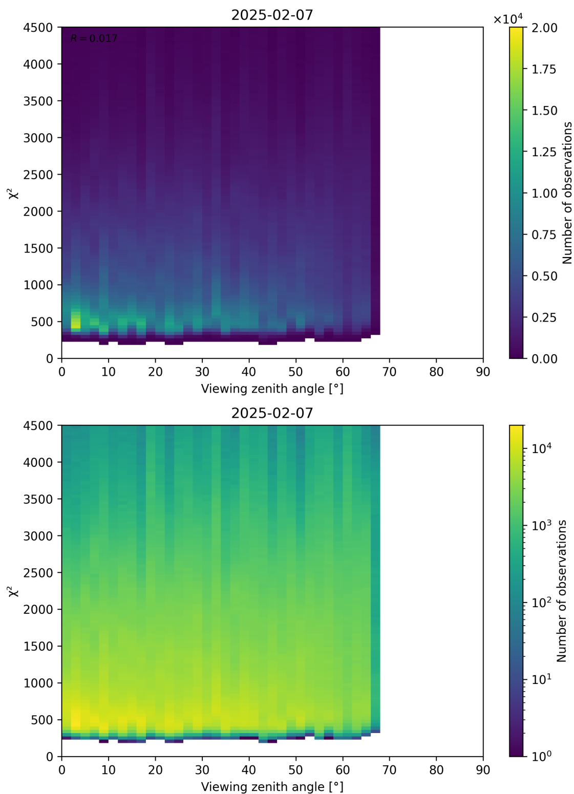
Figure 72: Scatter density plot of “Viewing zenith angle” against “ \chi^2 ” for 2025-02-06 to 2025-02-08.
