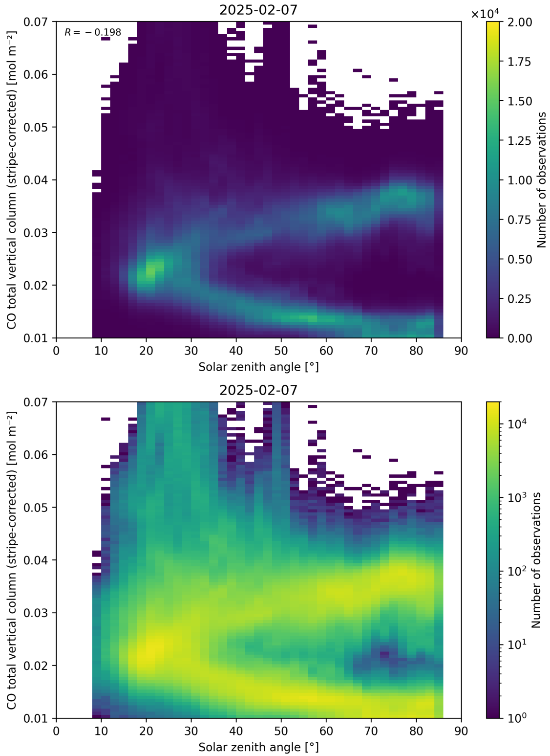
Figure 62: Scatter density plot of “Solar zenith angle” against “CO total vertical column (stripe-corrected)” for 2025-02-06 to 2025-02-08.
