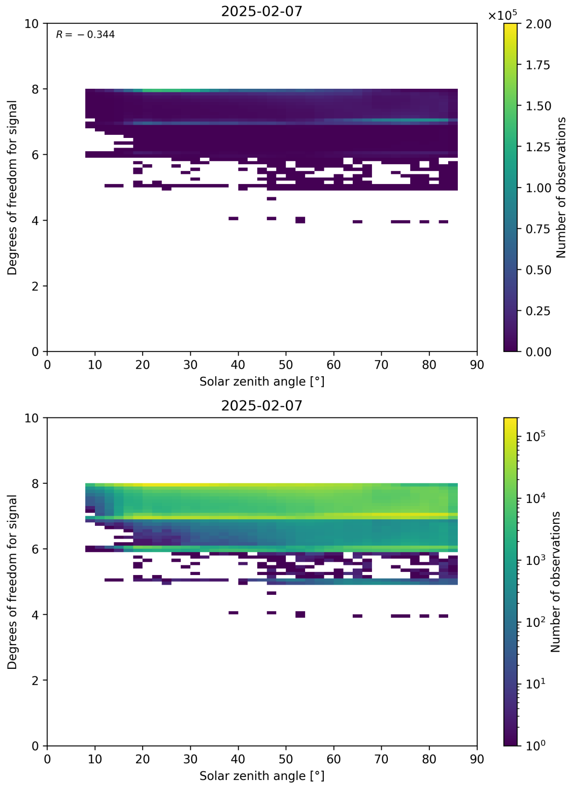
Figure 65: Scatter density plot of “Solar zenith angle” against “Degrees of freedom for signal” for 2025-02-06 to 2025-02-08.
