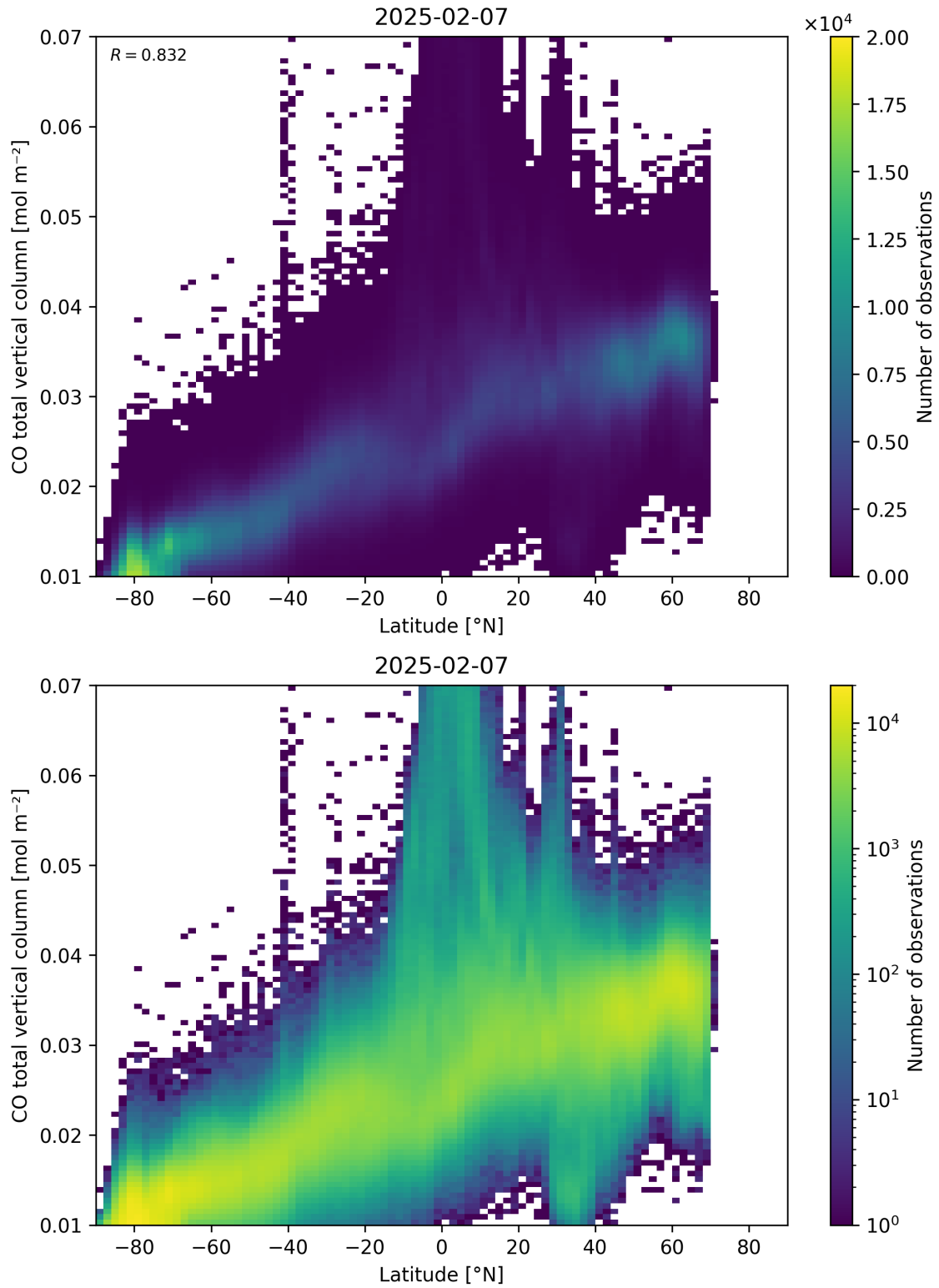
Figure 51: Scatter density plot of “Latitude” against “CO total vertical column” for 2025-02-06 to 2025-02-08.
