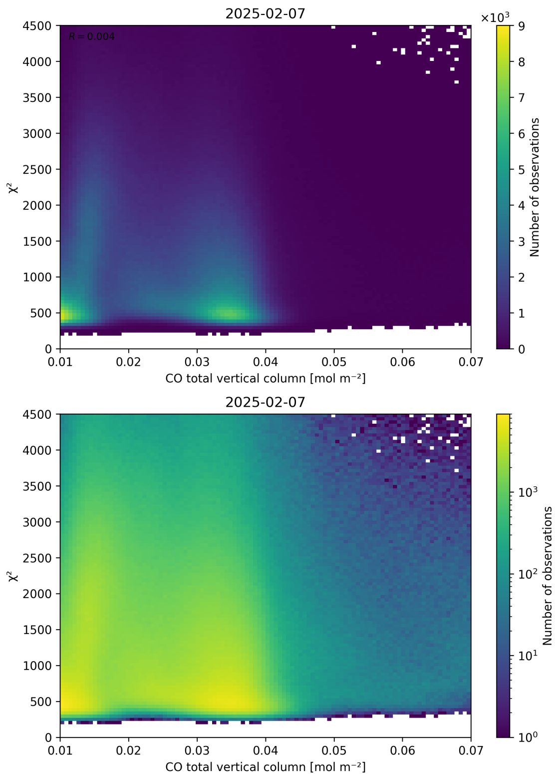
Figure 35: Scatter density plot of “CO total vertical column” against “ \chi^2 ” for 2025-02-06 to 2025-02-08.
