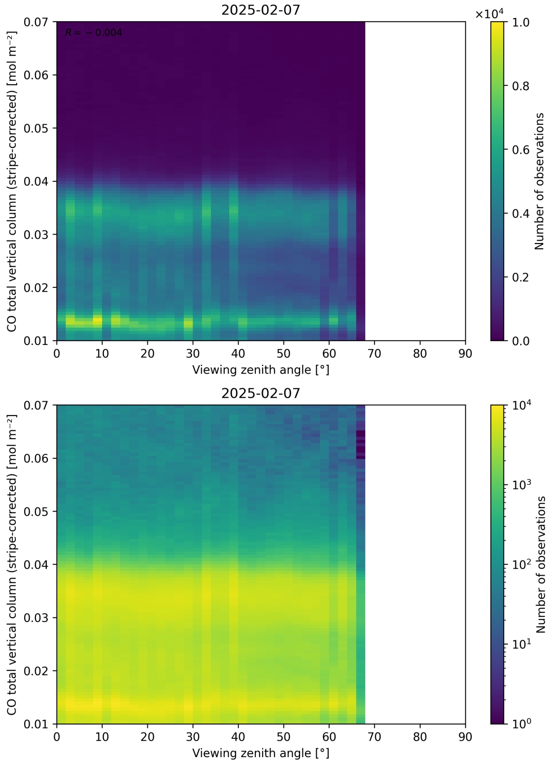
Figure 70: Scatter density plot of “Viewing zenith angle” against “CO total vertical column (stripe-corrected)” for 2025-02-06 to 2025-02-08.
