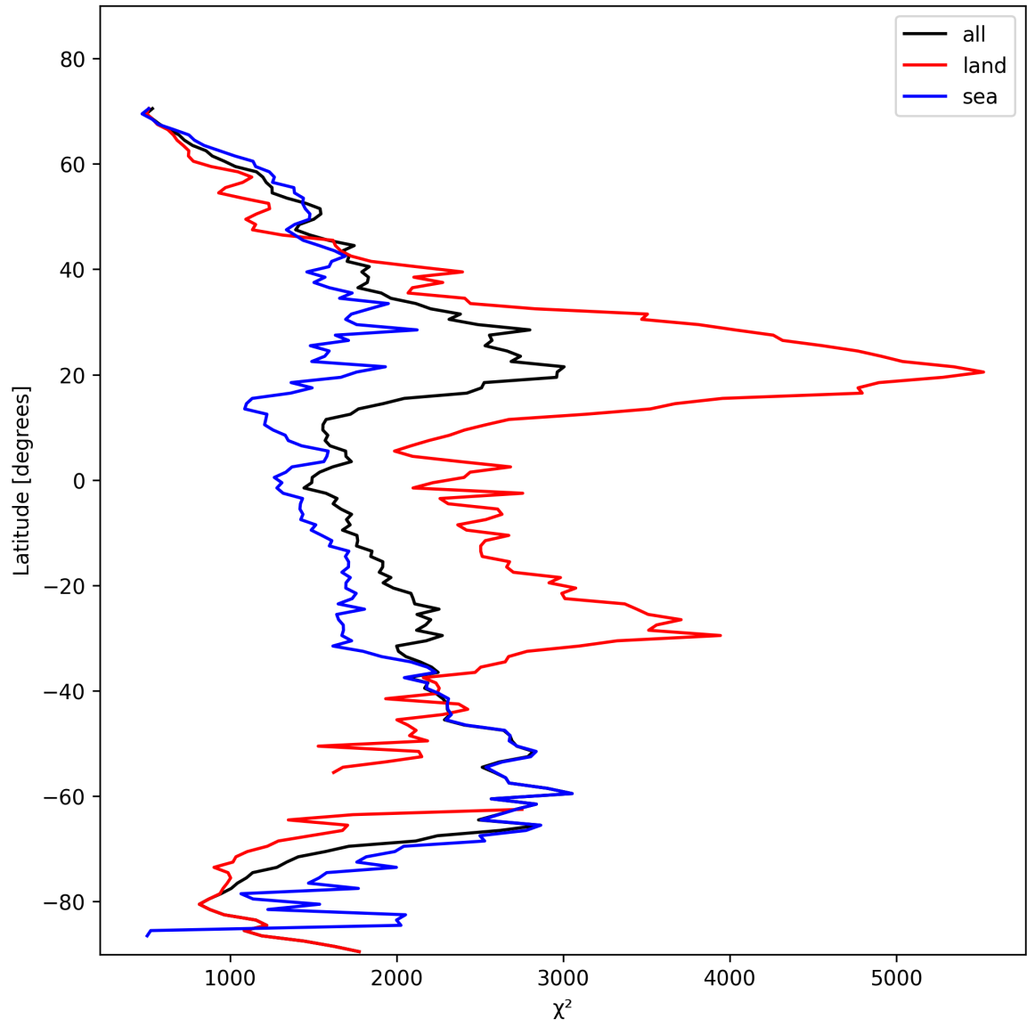
Figure 14: Zonal average of “ \chi^2 ” for 2025-02-06 to 2025-02-08.
