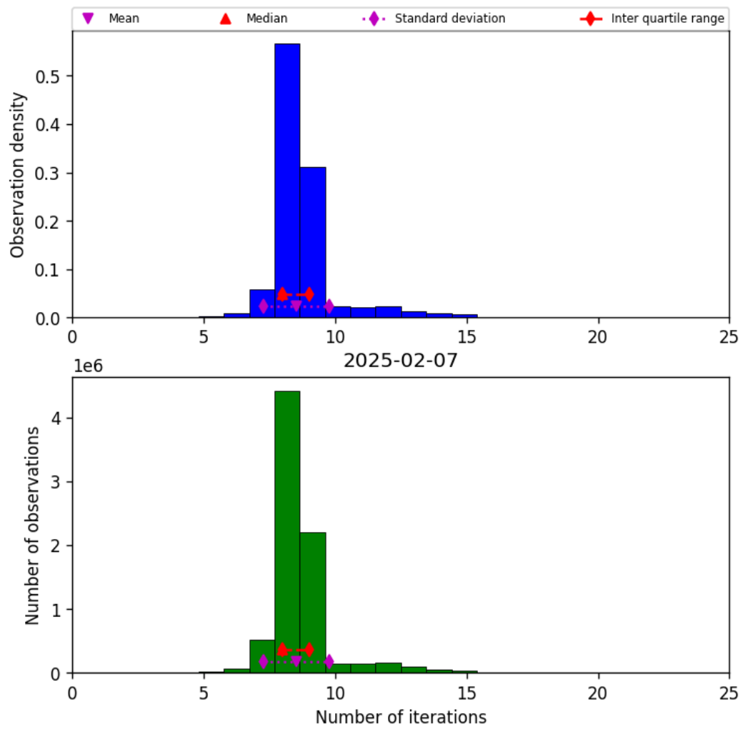
Figure 24: Histogram of “Number of iterations” for 2025-02-06 to 2025-02-08
