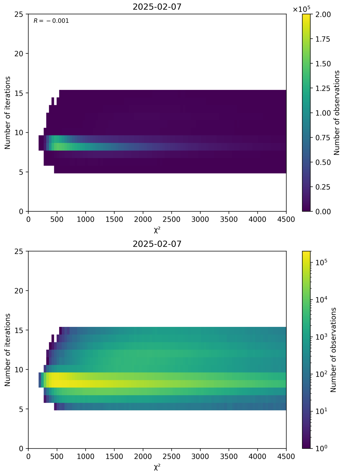
Figure 49: Scatter density plot of “ \chi^2 ” against “Number of iterations” for 2025-02-06 to 2025-02-08.
