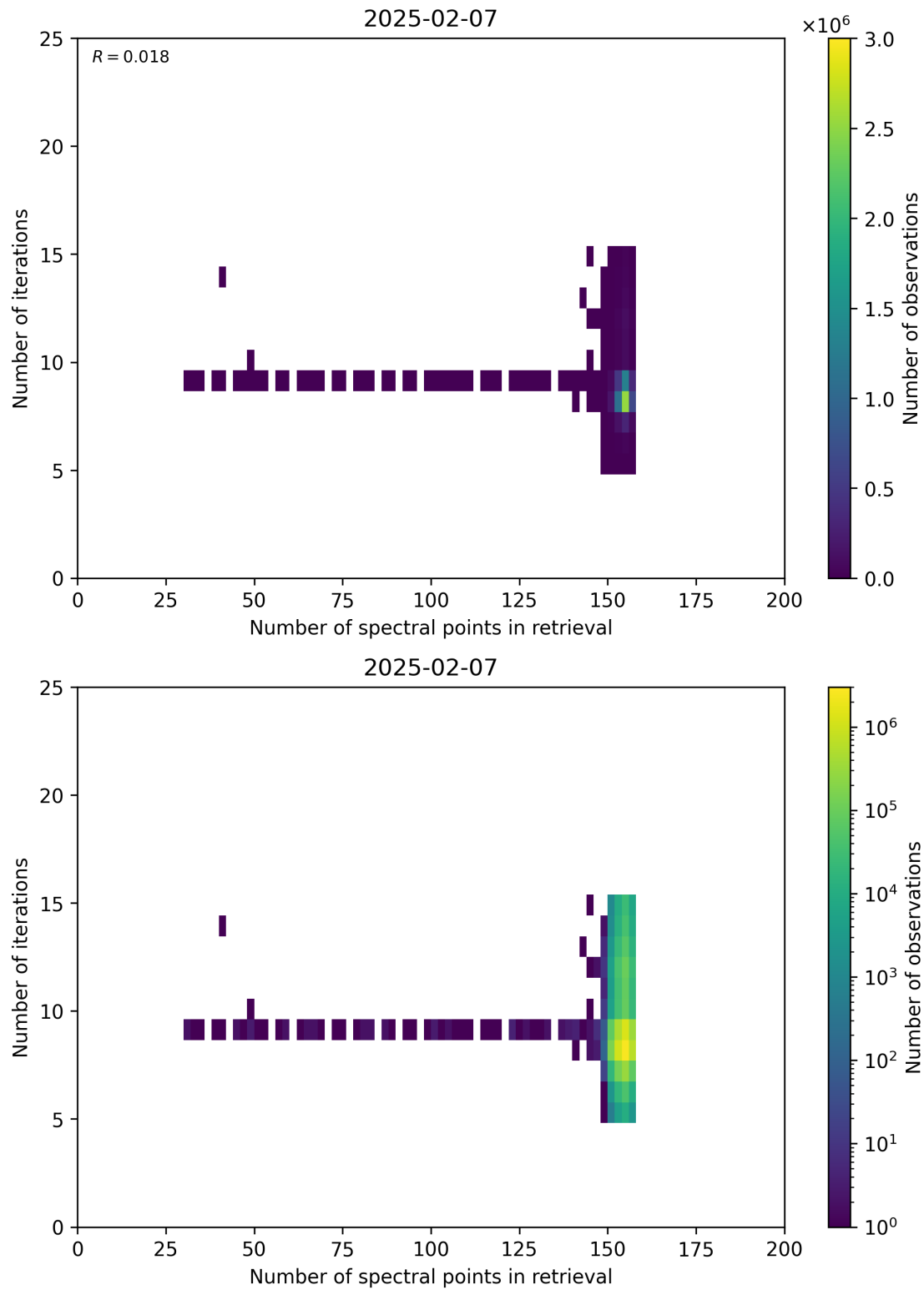
Figure 60: Scatter density plot of “Number of spectral points in retrieval” against “Number of iterations” for 2025-02-06 to 2025-02-08.
