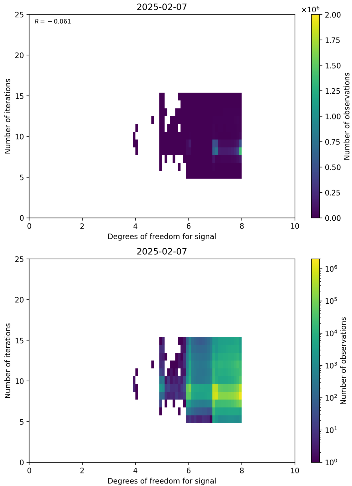
Figure 50: Scatter density plot of “Degrees of freedom for signal” against “Number of iterations” for 2025-02-06 to 2025-02-08.
