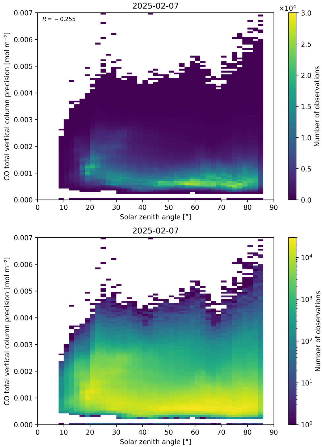
Figure 63: Scatter density plot of “Solar zenith angle” against “CO total vertical column precision” for 2025-02-06 to 2025-02-08.
