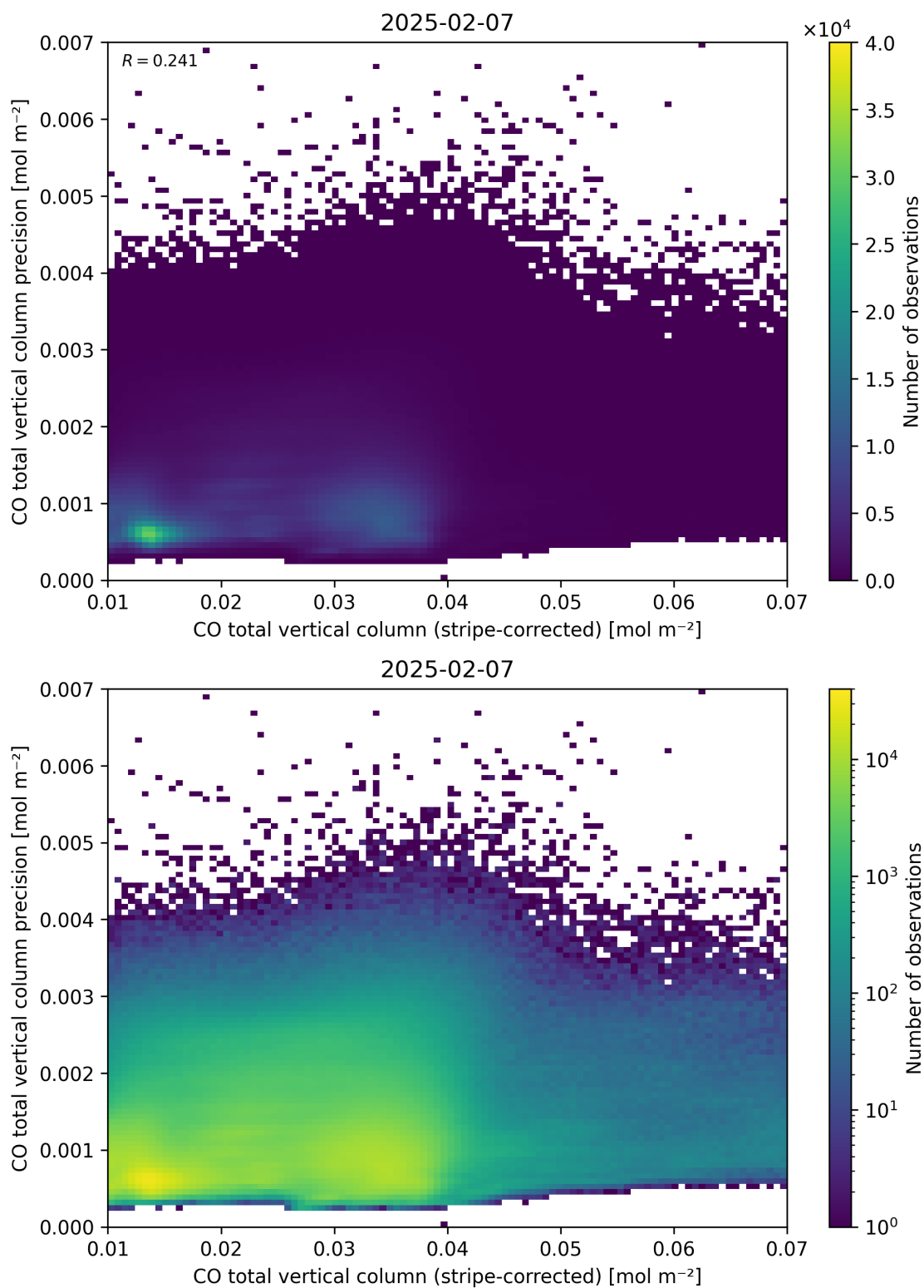
Figure 36: Scatter density plot of “CO total vertical column (stripe-corrected)” against “CO total vertical column precision” for 2025-02-06 to 2025-02-08.
