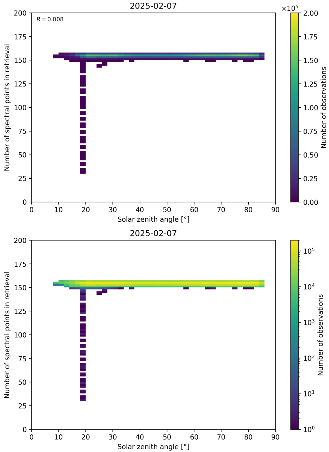
Figure 68: Scatter density plot of “Solar zenith angle” against “Number of spectral points in retrieval” for 2025-02-06 to 2025-02-08.
