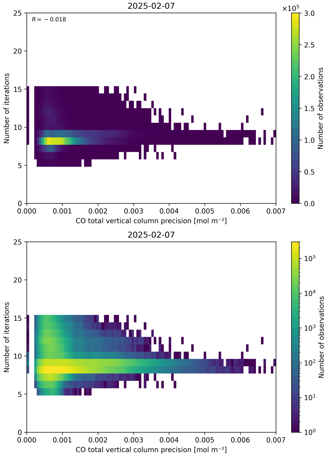
Figure 46: Scatter density plot of “CO total vertical column precision” against “Number of iterations” for 2025-02-06 to 2025-02-08.
