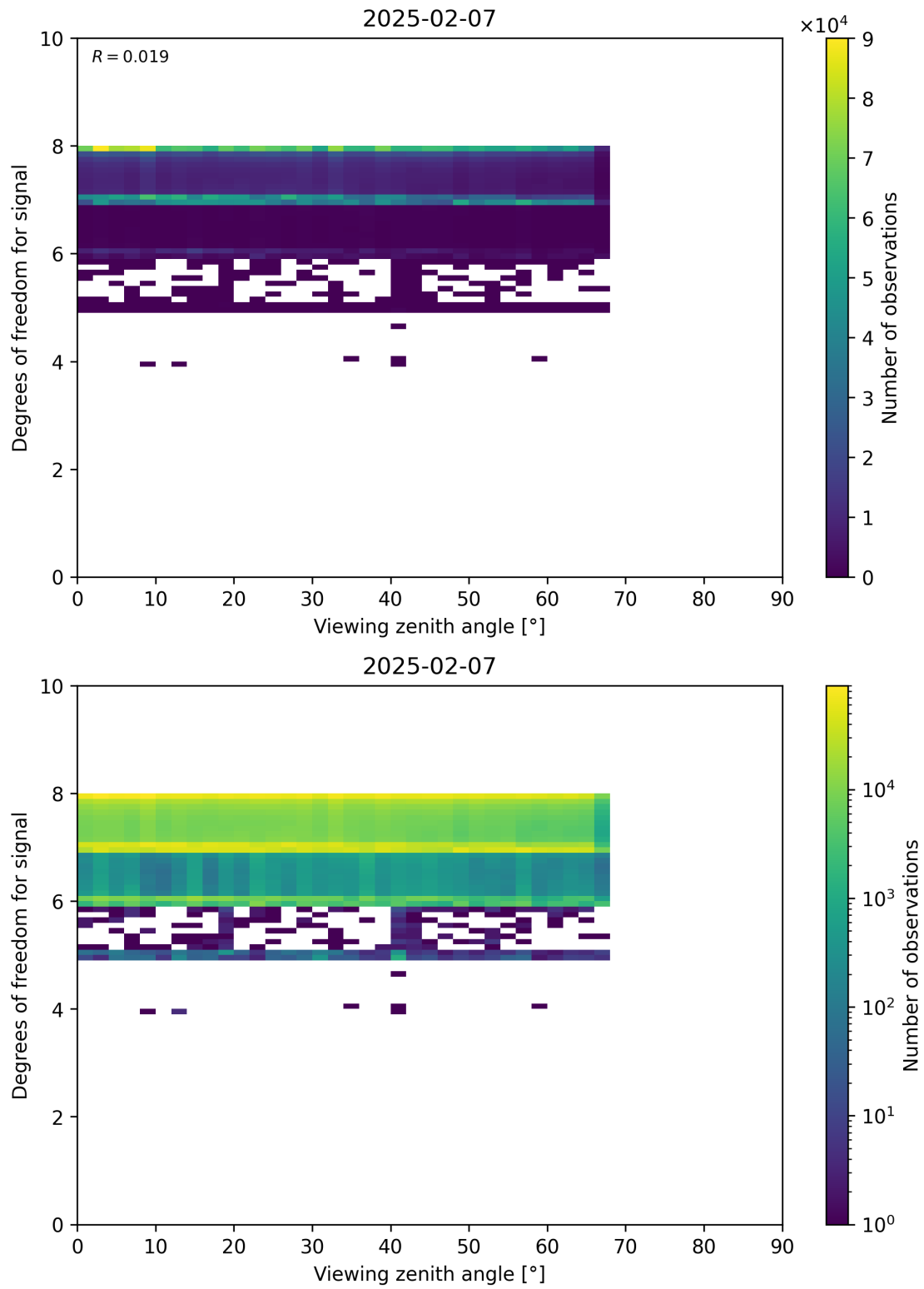
Figure 73: Scatter density plot of “Viewing zenith angle” against “Degrees of freedom for signal” for 2025-02-06 to 2025-02-08.
