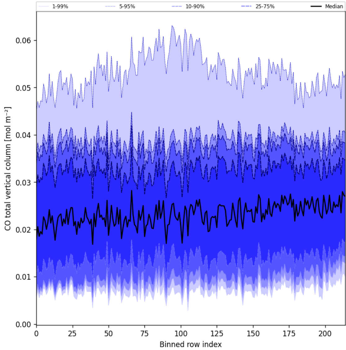
Figure 26: Along track statistics of “CO total vertical column” for 2025-02-06 to 2025-02-08
