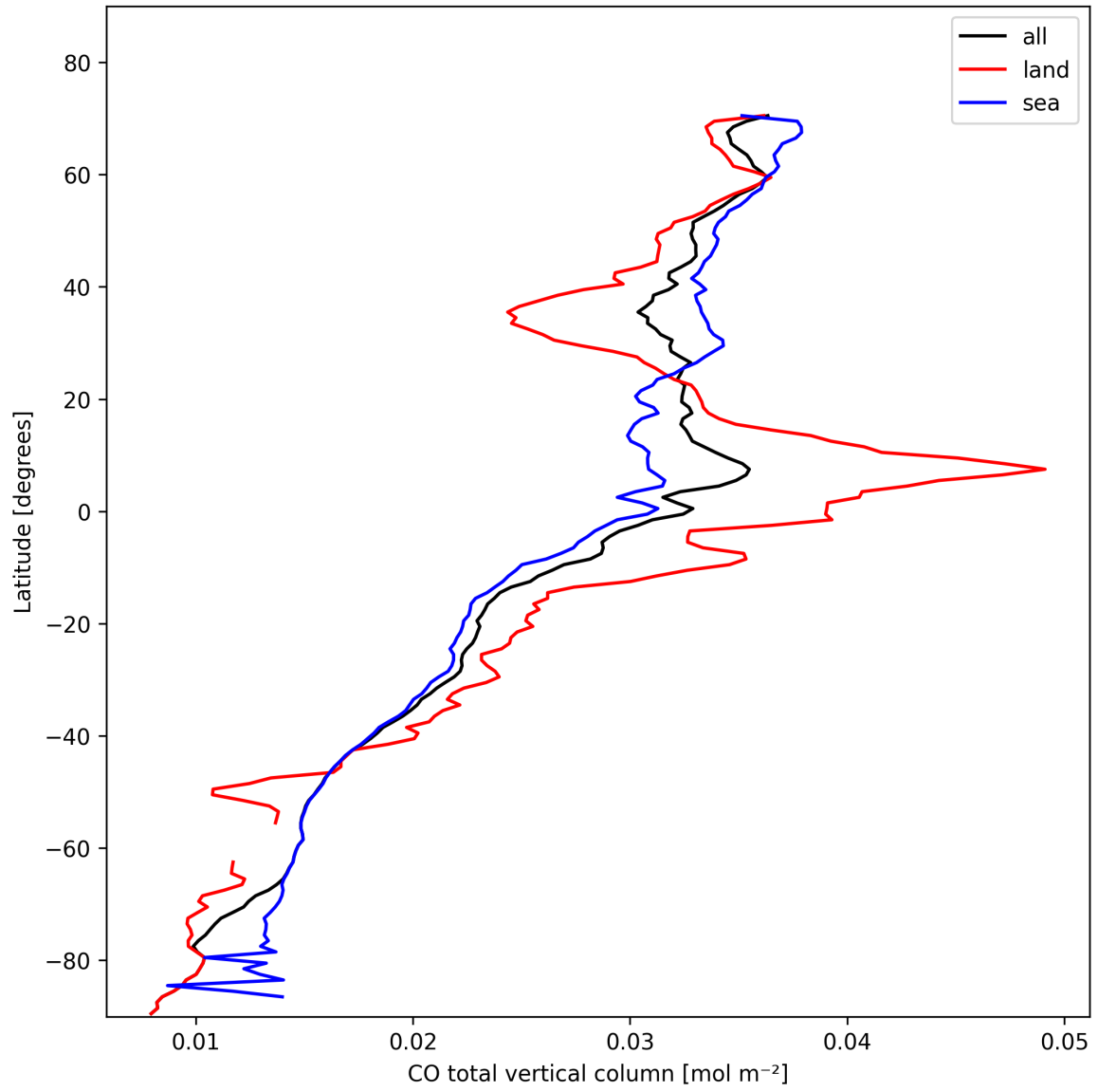
Figure 10: Zonal average of “CO total vertical column” for 2025-02-06 to 2025-02-08.
