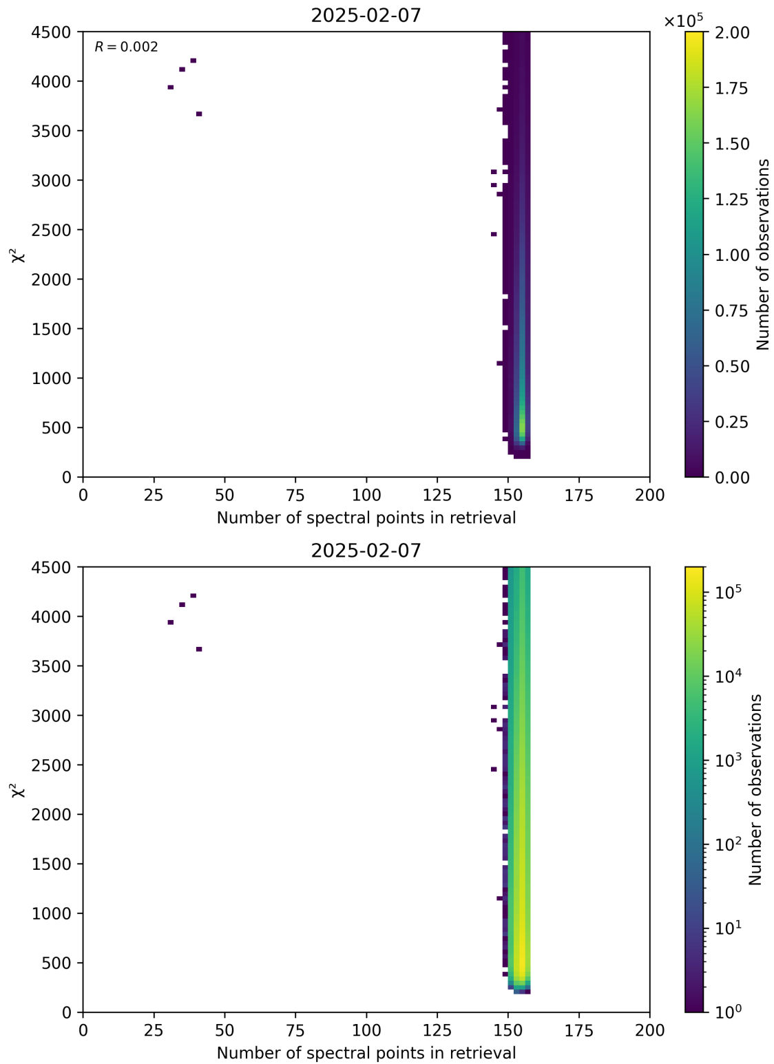
Figure 58: Scatter density plot of “Number of spectral points in retrieval” against “ \chi^2 ” for 2025-02-06 to 2025-02-08.
