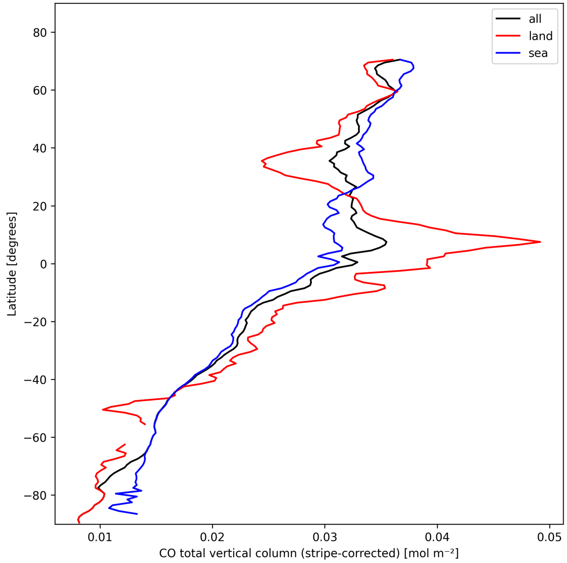
Figure 11: Zonal average of “CO total vertical column (stripe-corrected)” for 2025-02-06 to 2025-02-08.
