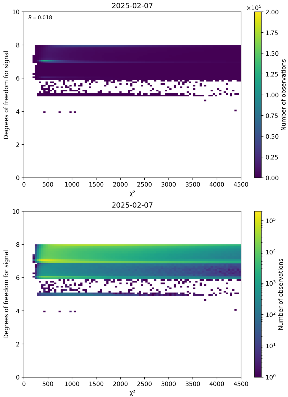
Figure 48: Scatter density plot of “ \chi^2 ” against “Degrees of freedom for signal” for 2025-02-06 to 2025-02-08.
