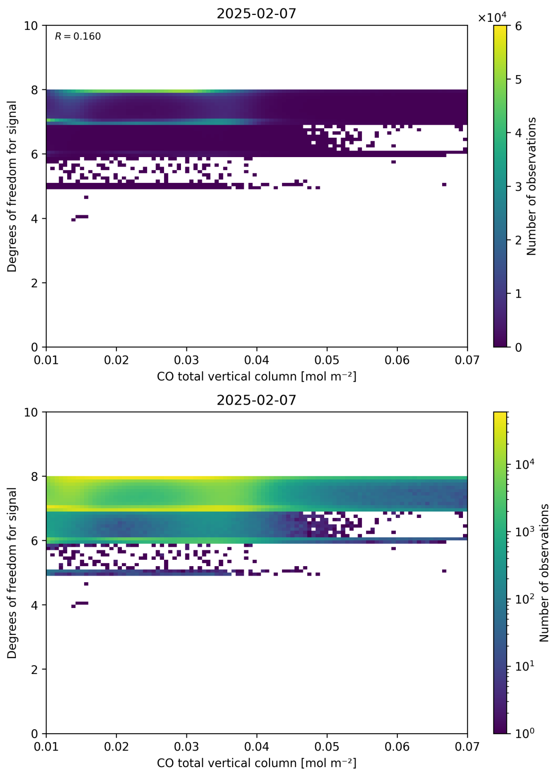
Figure 41: Scatter density plot of “CO total vertical column” against “Degrees of freedom for signal” for 2025-02-06 to 2025-02-08.
