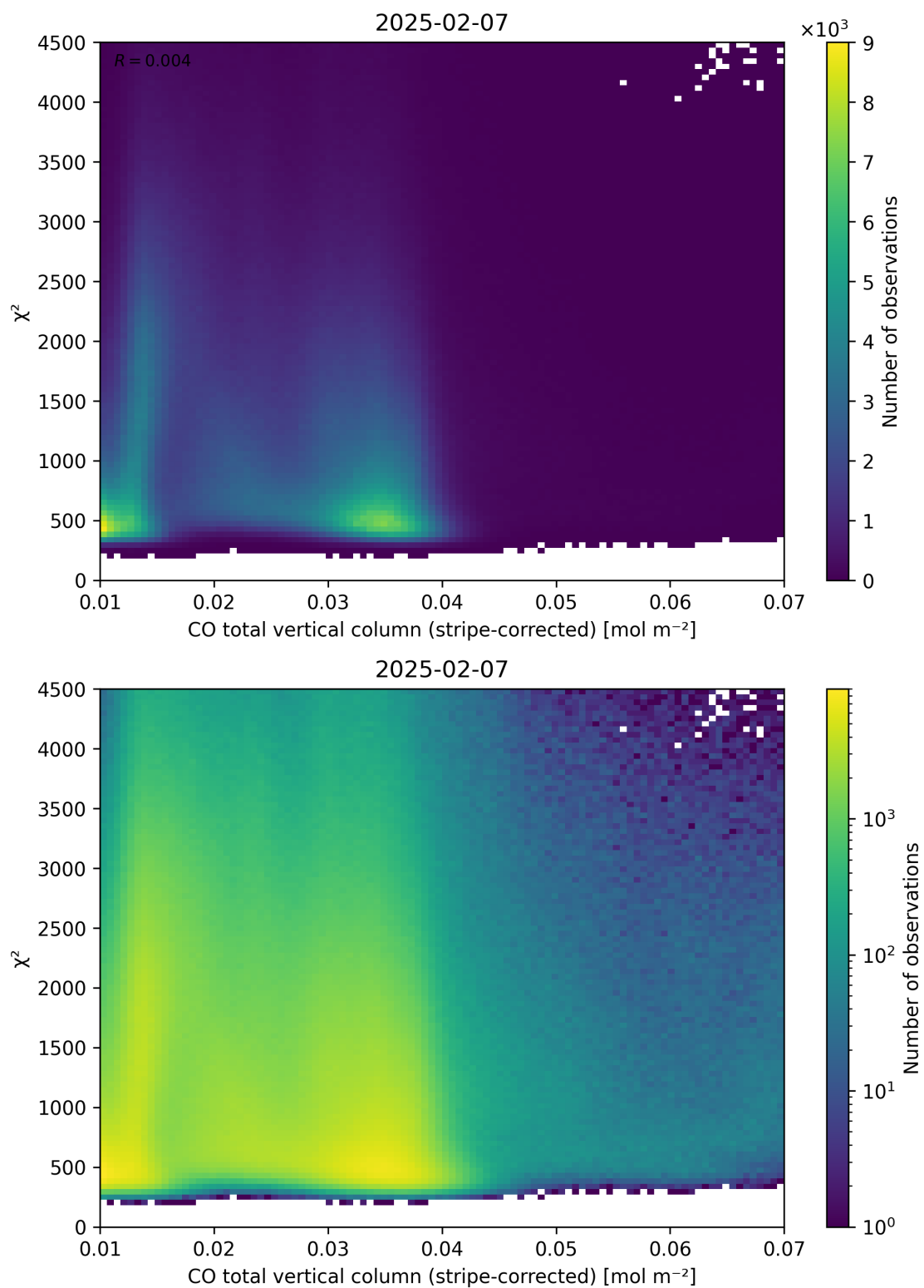
Figure 37: Scatter density plot of “CO total vertical column (stripe-corrected)” against “ \chi^2 ” for 2025-02-06 to 2025-02-08.
