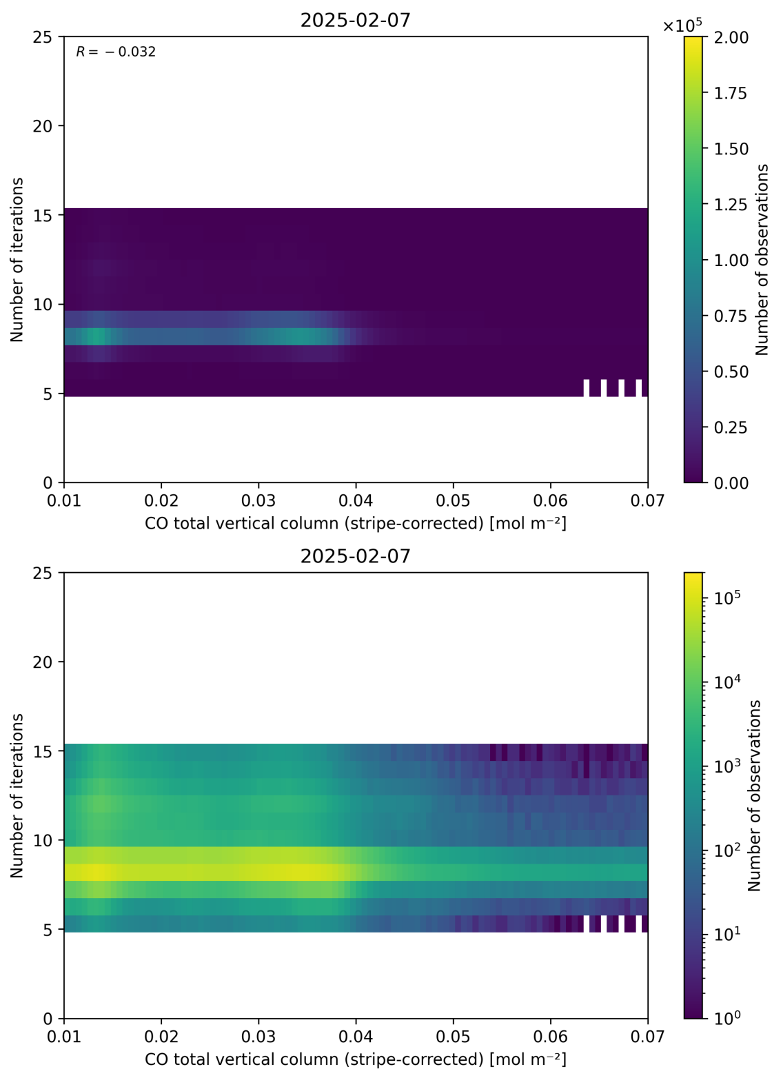
Figure 39: Scatter density plot of “CO total vertical column (stripe-corrected)” against “Number of iterations” for 2025-02-06 to 2025-02-08.
