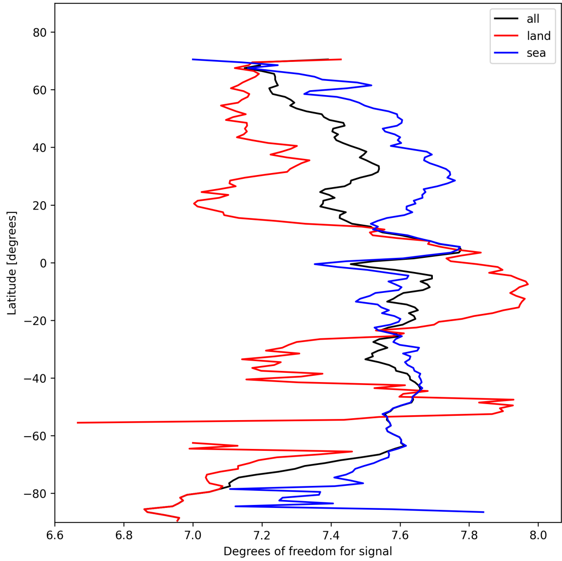
Figure 15: Zonal average of “Degrees of freedom for signal” for 2025-02-06 to 2025-02-08.
