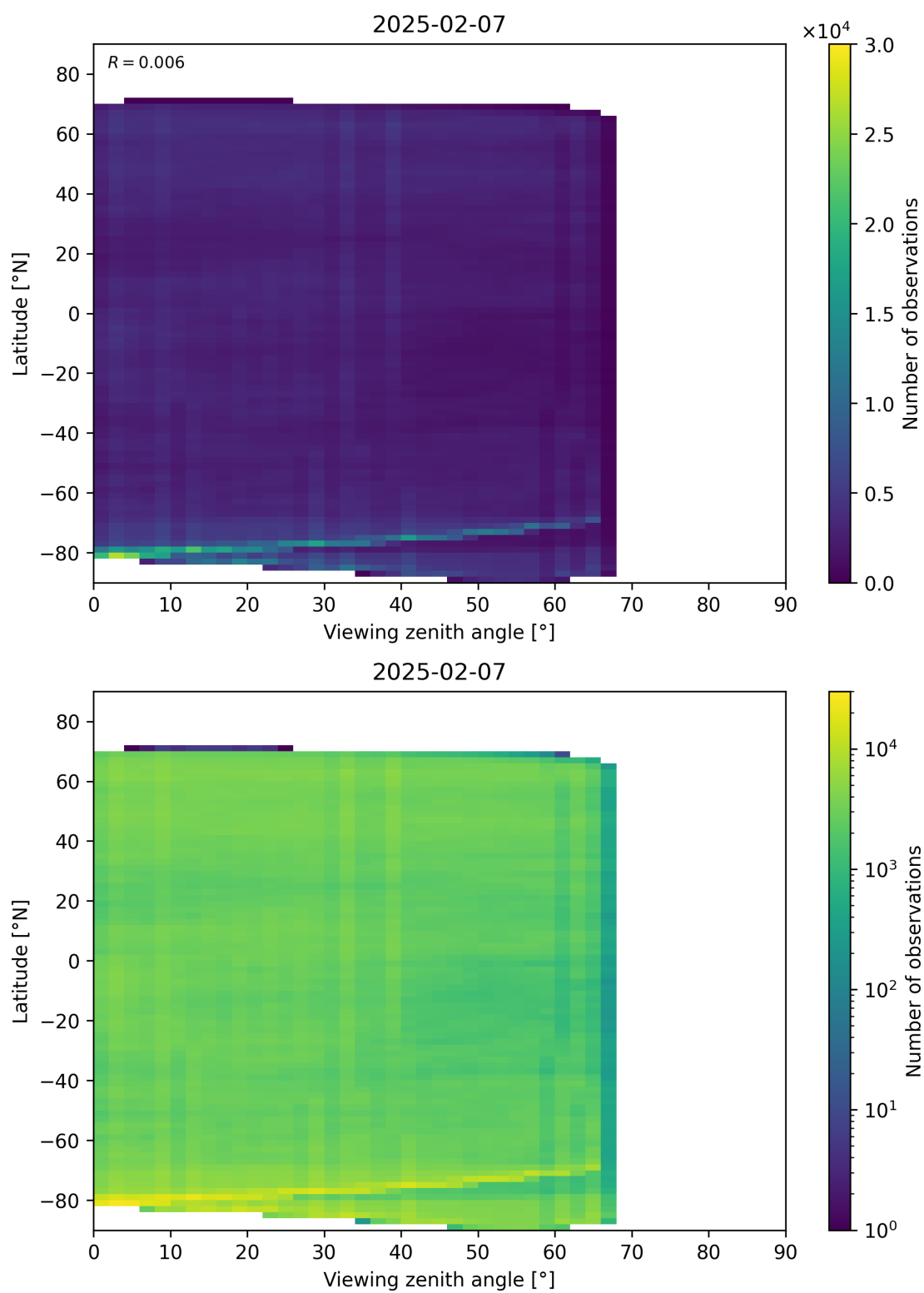
Figure 74: Scatter density plot of “Viewing zenith angle” against “Latitude” for 2025-02-06 to 2025-02-08.
