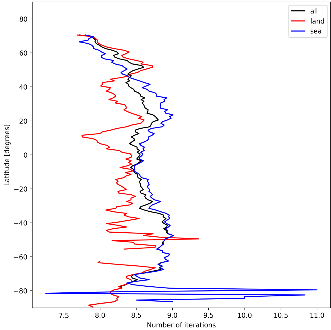
Figure 16: Zonal average of “Number of iterations” for 2025-02-06 to 2025-02-08.
