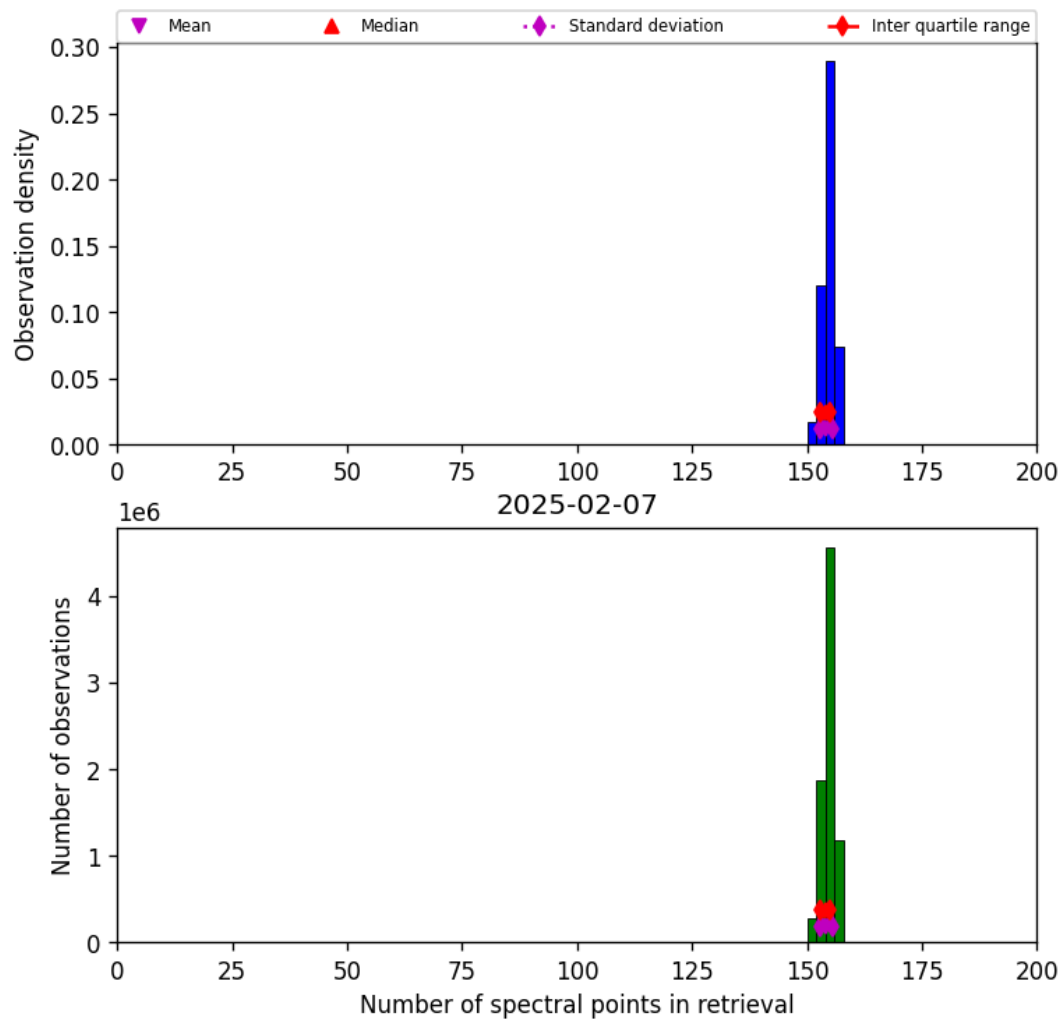
Figure 21: Histogram of “Number of spectral points in retrieval” for 2025-02-06 to 2025-02-08
