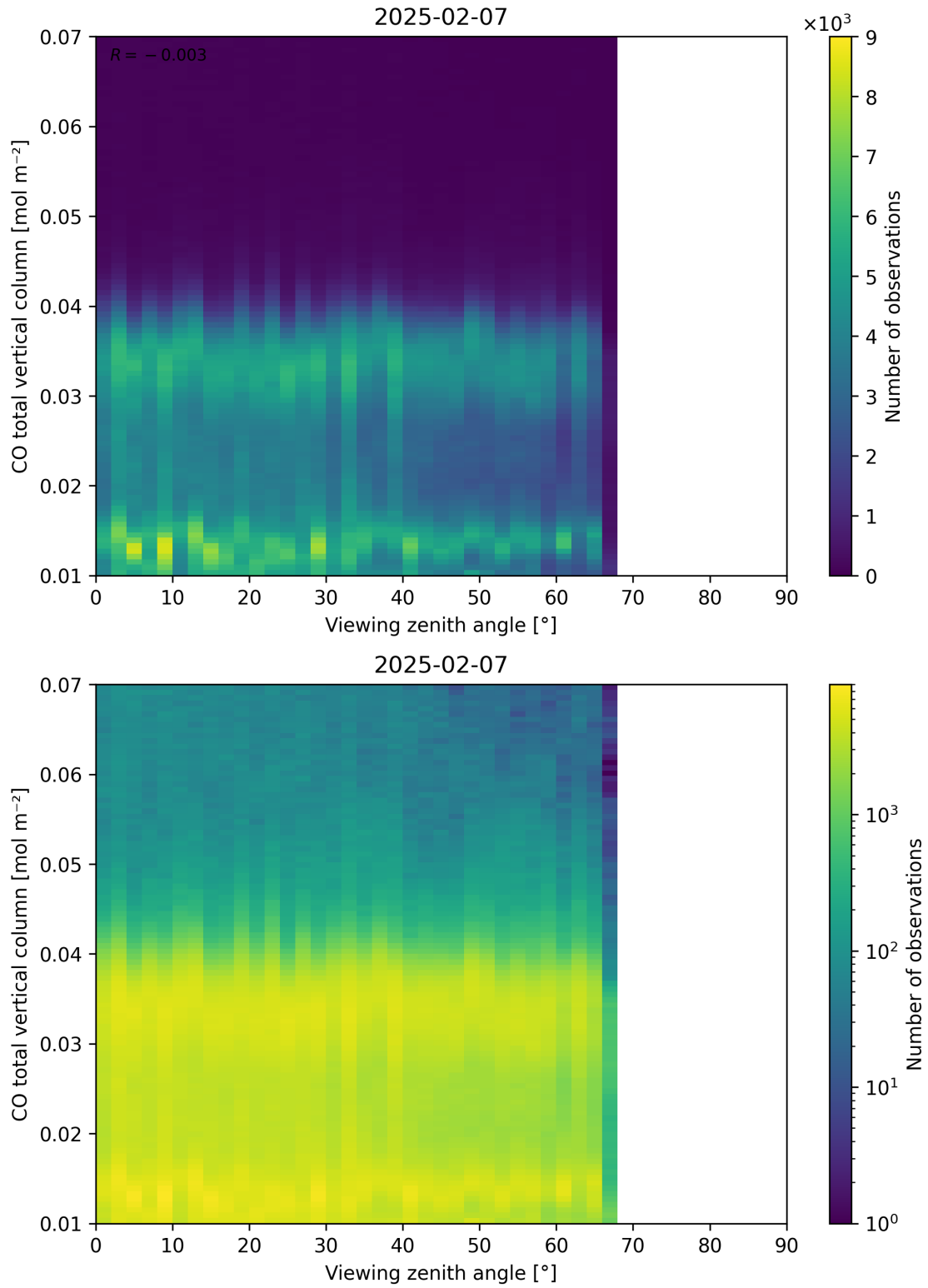
Figure 69: Scatter density plot of “Viewing zenith angle” against “CO total vertical column” for 2025-02-06 to 2025-02-08.
