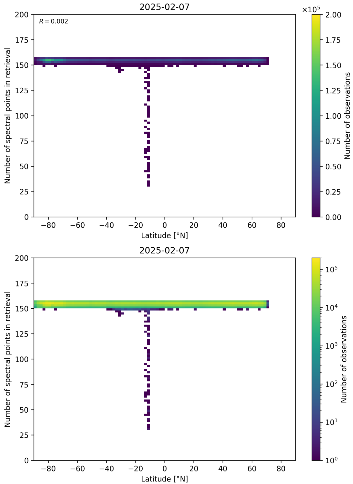
Figure 57: Scatter density plot of “Latitude” against “Number of spectral points in retrieval” for 2025-02-06 to 2025-02-08.
