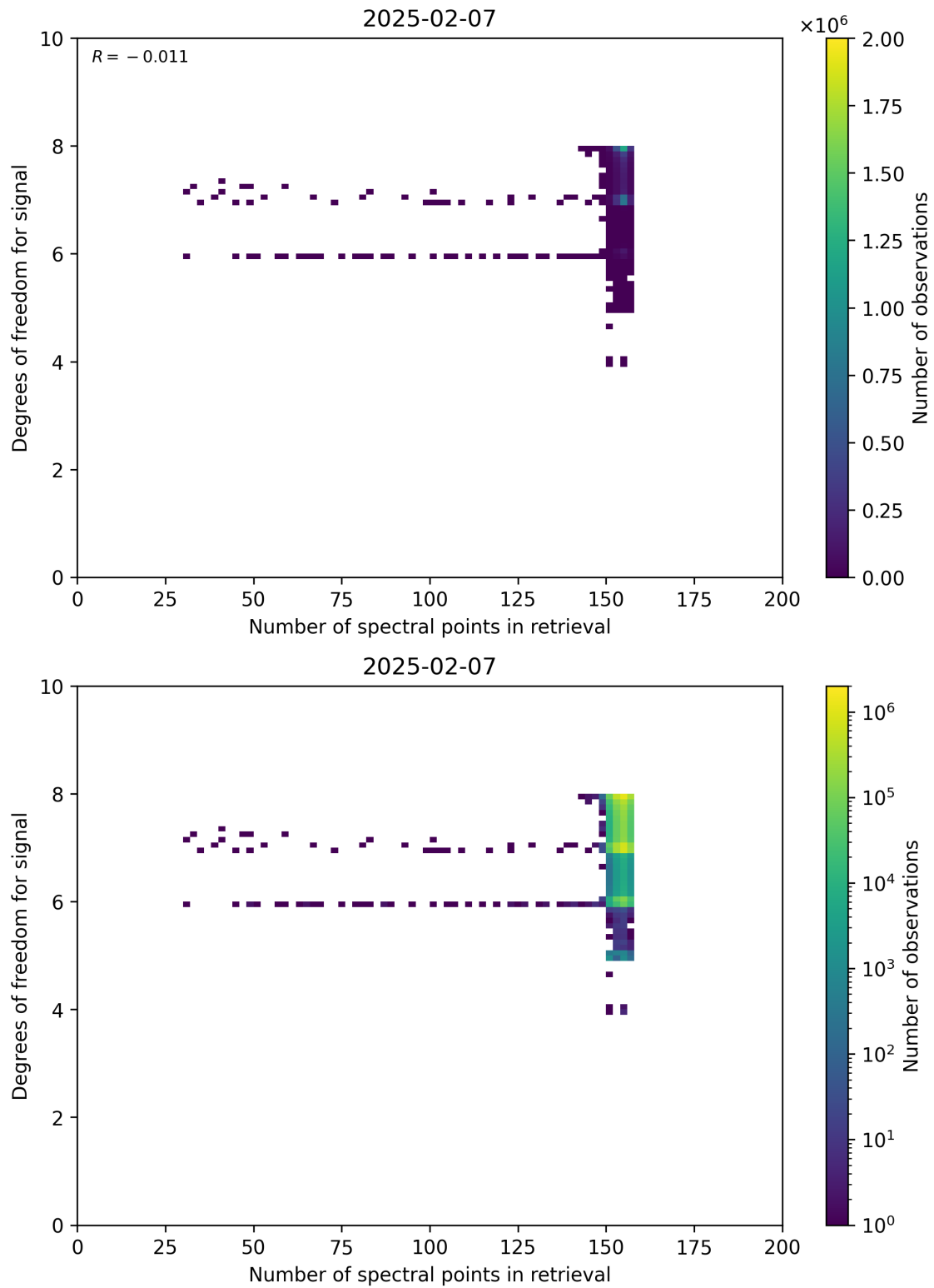
Figure 59: Scatter density plot of “Number of spectral points in retrieval” against “Degrees of freedom for signal” for 2025-02-06 to 2025-02-08.
