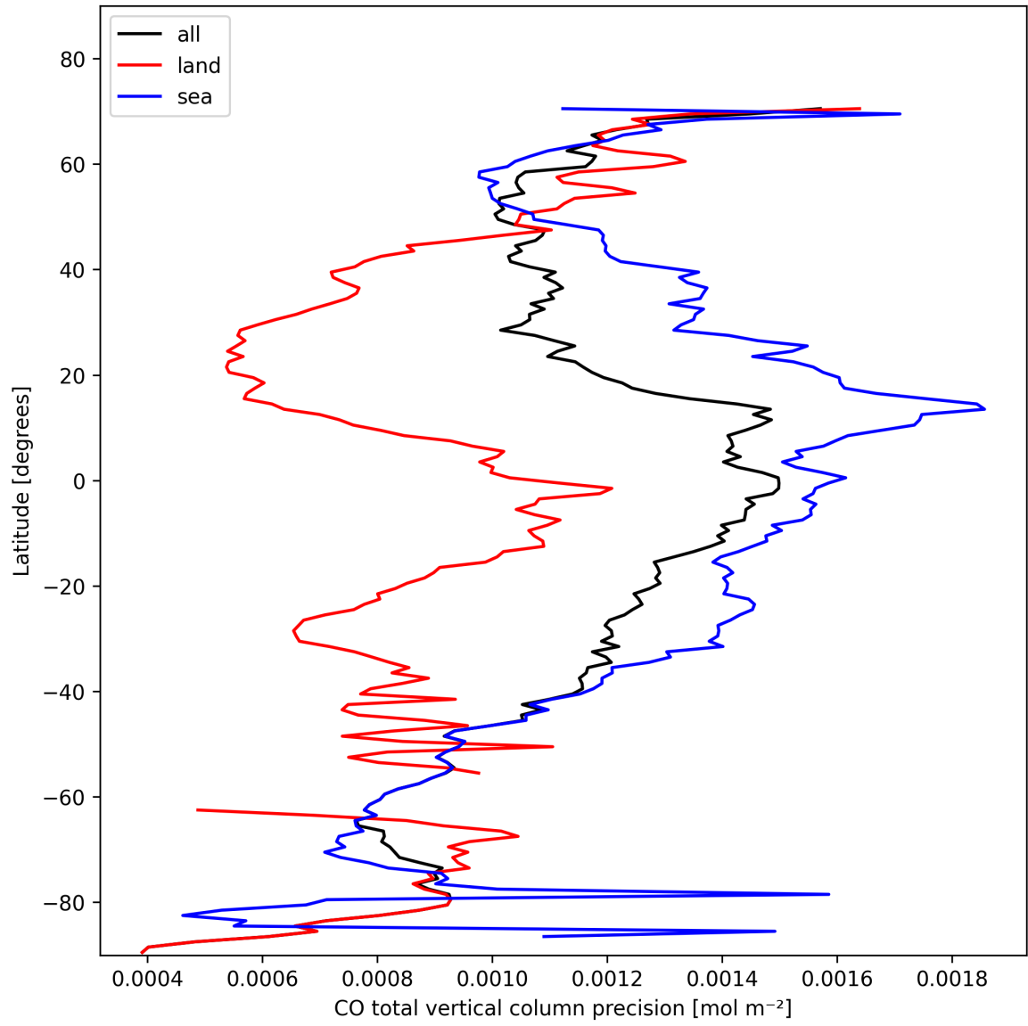
Figure 12: Zonal average of “CO total vertical column precision” for 2025-02-06 to 2025-02-08.
