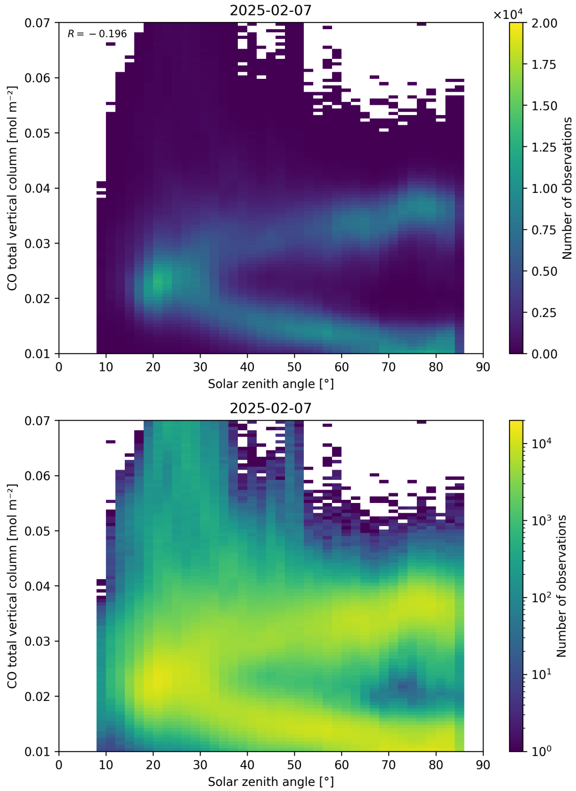
Figure 61: Scatter density plot of “Solar zenith angle” against “CO total vertical column” for 2025-02-06 to 2025-02-08.
