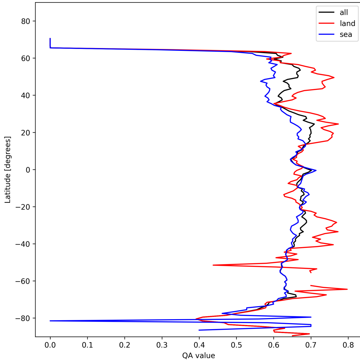
Figure 9: Zonal average of “QA value” for 2025-02-06 to 2025-02-08.
