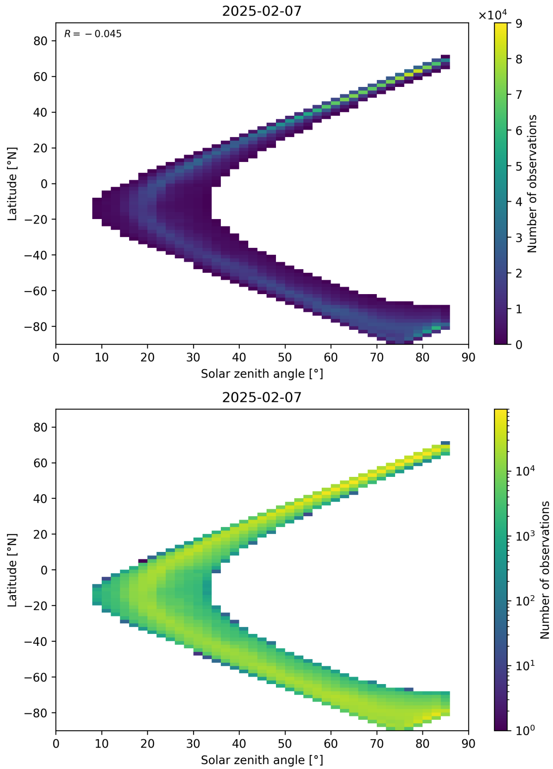
Figure 66: Scatter density plot of “Solar zenith angle” against “Latitude” for 2025-02-06 to 2025-02-08.
