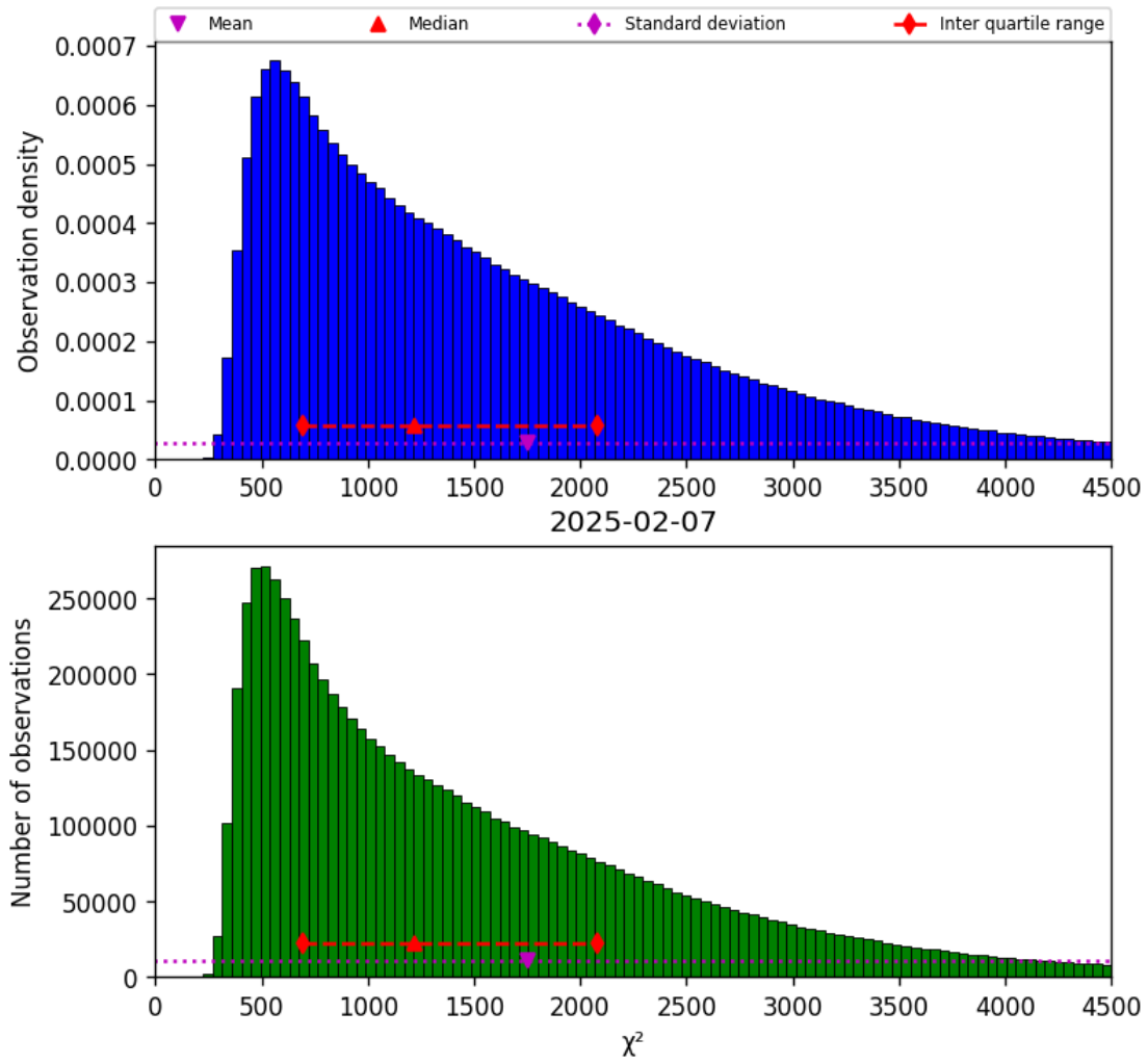
Figure 22: Histogram of " \chi^2 " for 2025-02-06 to 2025-02-08
