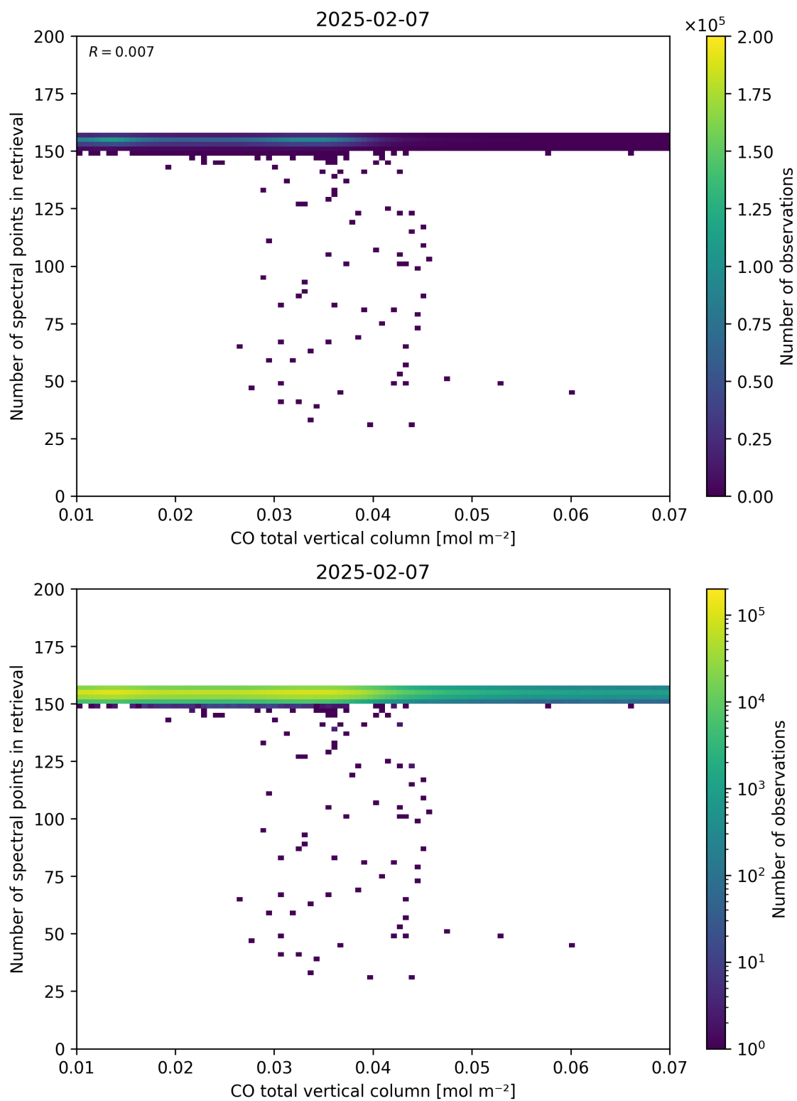
Figure 43: Scatter density plot of “CO total vertical column” against “Number of spectral points in retrieval” for 2025-02-06 to 2025-02-08.
