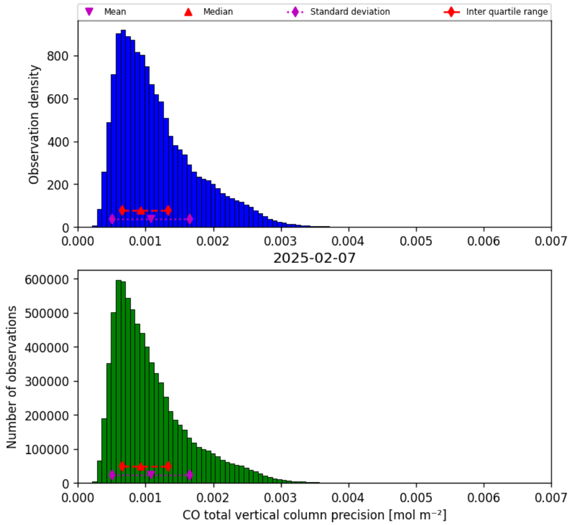
Figure 20: Histogram of “CO total vertical column precision” for 2025-02-06 to 2025-02-08
