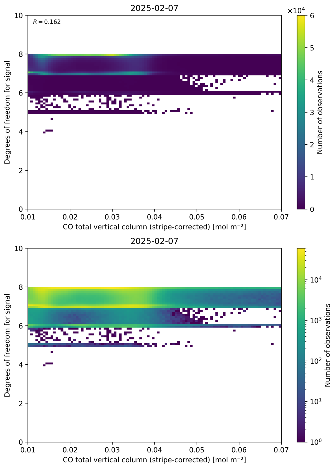
Figure 38: Scatter density plot of “CO total vertical column (stripe-corrected)” against “Degrees of freedom for signal” for 2025-02-06 to 2025-02-08.
