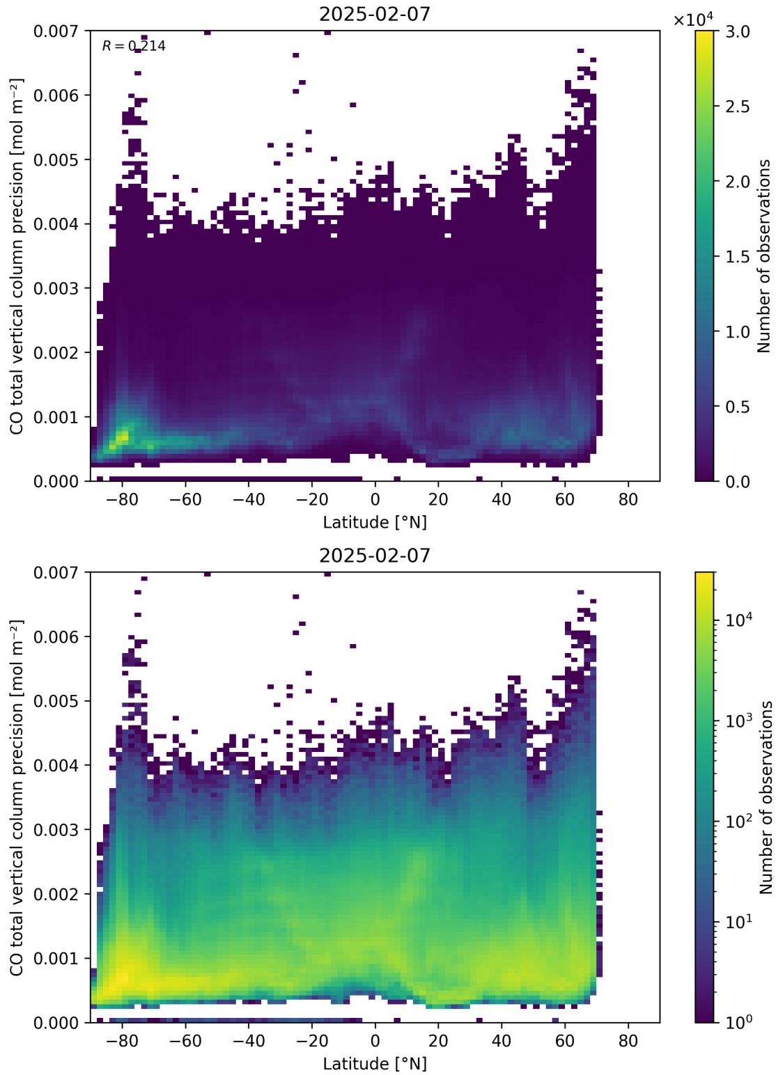
Figure 53: Scatter density plot of “Latitude” against “CO total vertical column precision” for 2025-02-06 to 2025-02-08.
