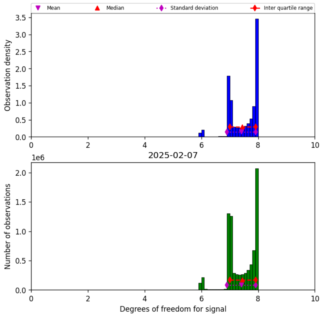
Figure 23: Histogram of “Degrees of freedom for signal” for 2025-02-06 to 2025-02-08
