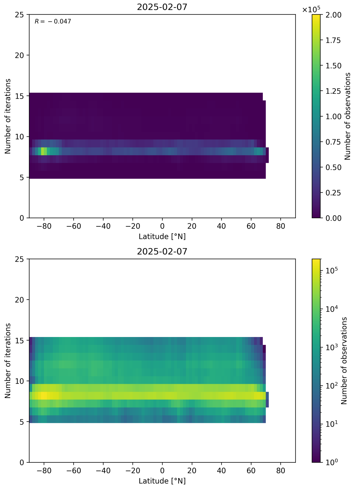
Figure 56: Scatter density plot of “Latitude” against “Number of iterations” for 2025-02-06 to 2025-02-08.
