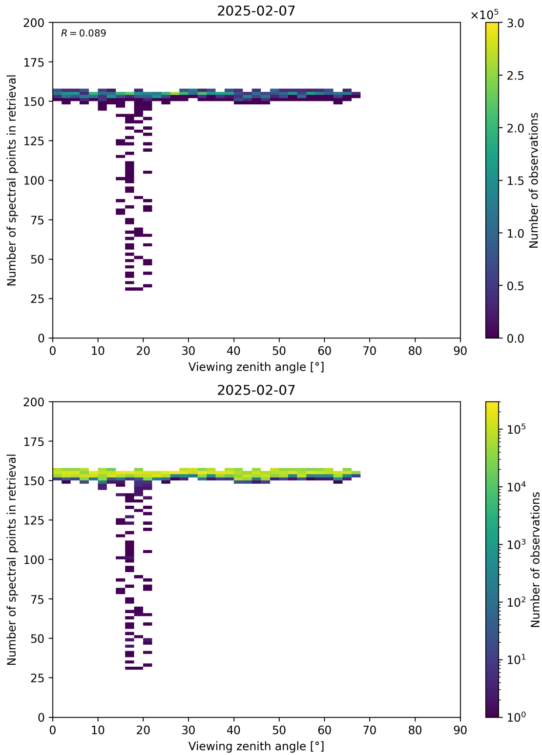
Figure 76: Scatter density plot of “Viewing zenith angle” against “Number of spectral points in retrieval” for 2025-02-06 to 2025-02-08.
