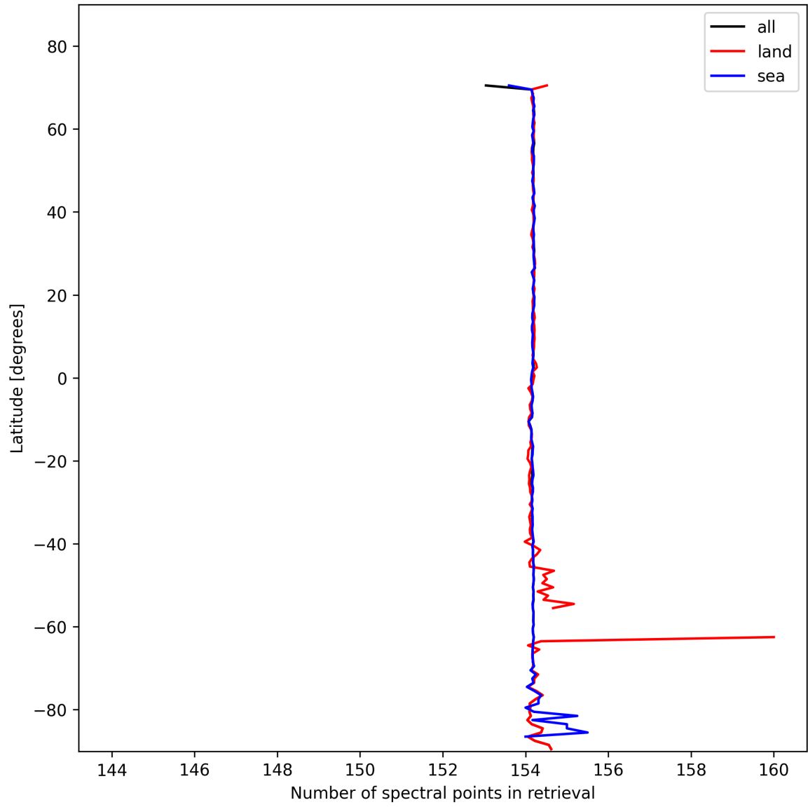
Figure 13: Zonal average of “Number of spectral points in retrieval” for 2025-02-06 to 2025-02-08.
