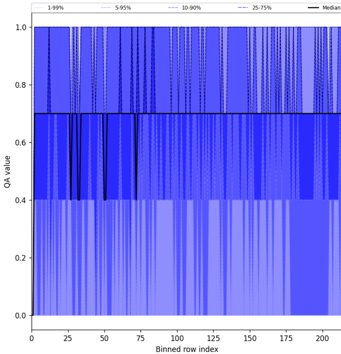
Figure 25: Along track statistics of “QA value” for 2025-02-06 to 2025-02-08
