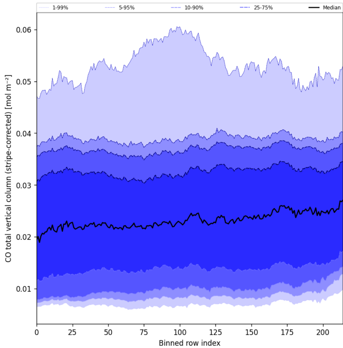
Figure 27: Along track statistics of “CO total vertical column (stripe-corrected)” for 2025-02-06 to 2025-02-08
