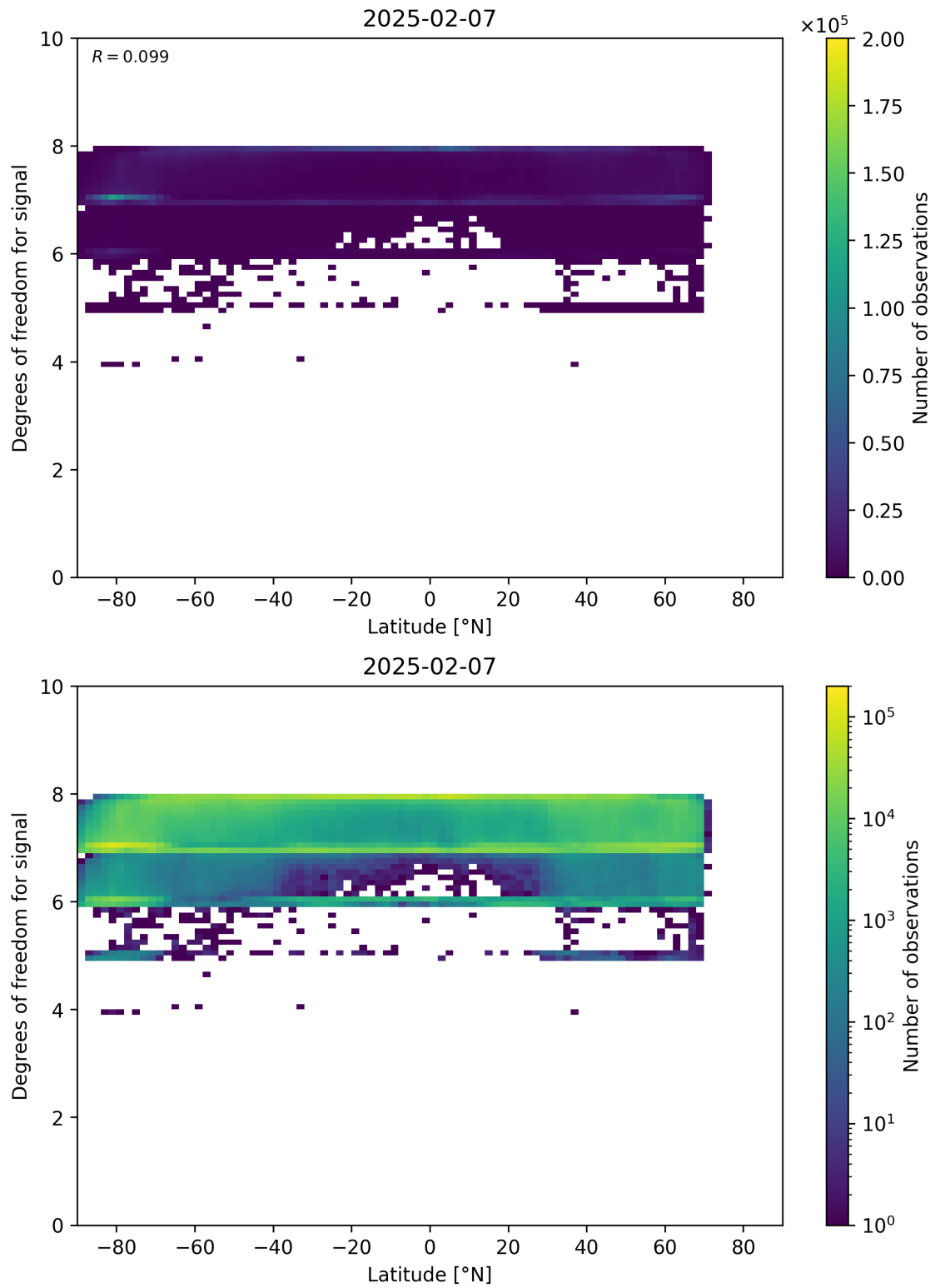
Figure 55: Scatter density plot of “Latitude” against “Degrees of freedom for signal” for 2025-02-06 to 2025-02-08.
