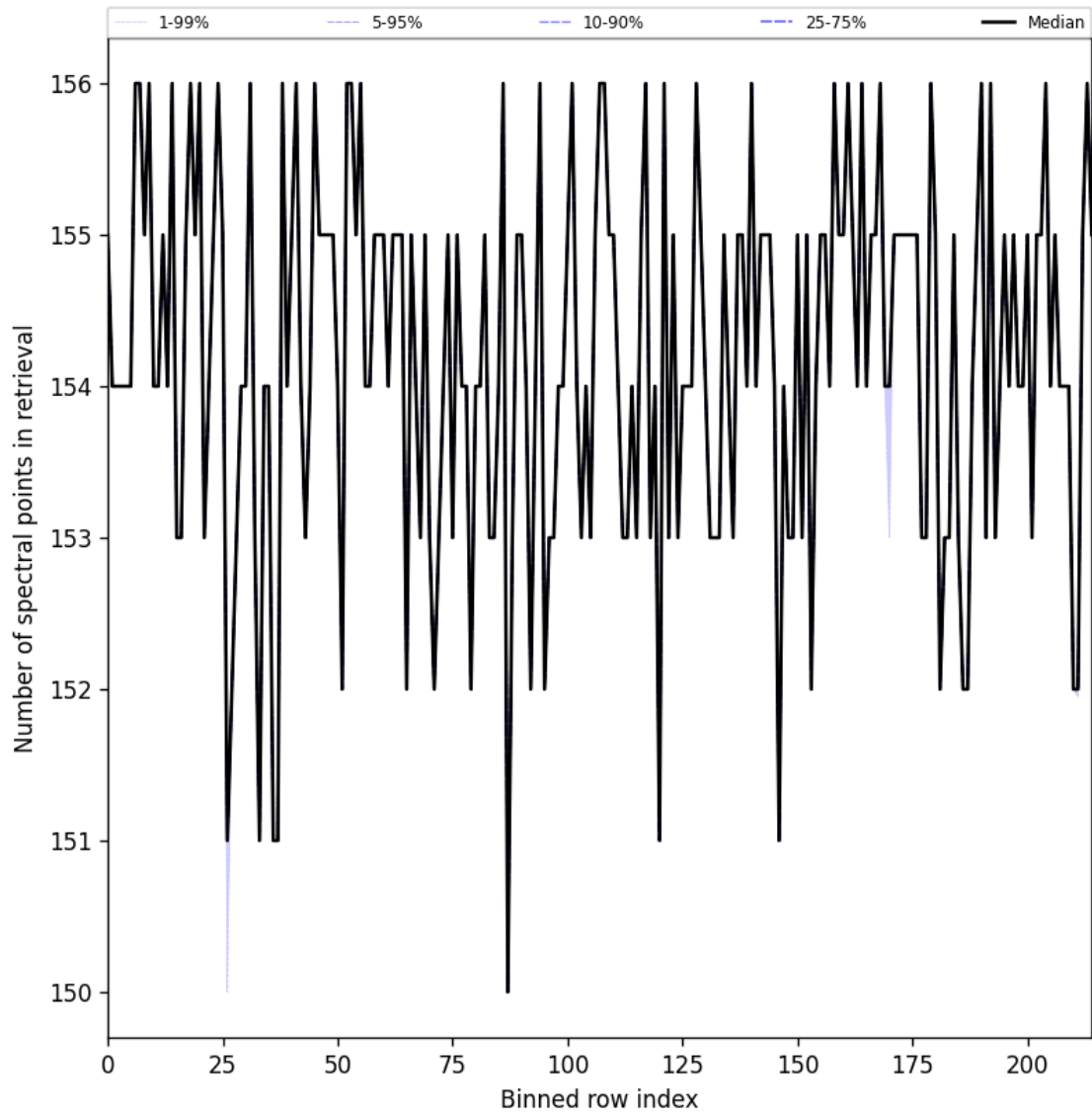
Figure 29: Along track statistics of “Number of spectral points in retrieval” for 2025-02-06 to 2025-02-08
