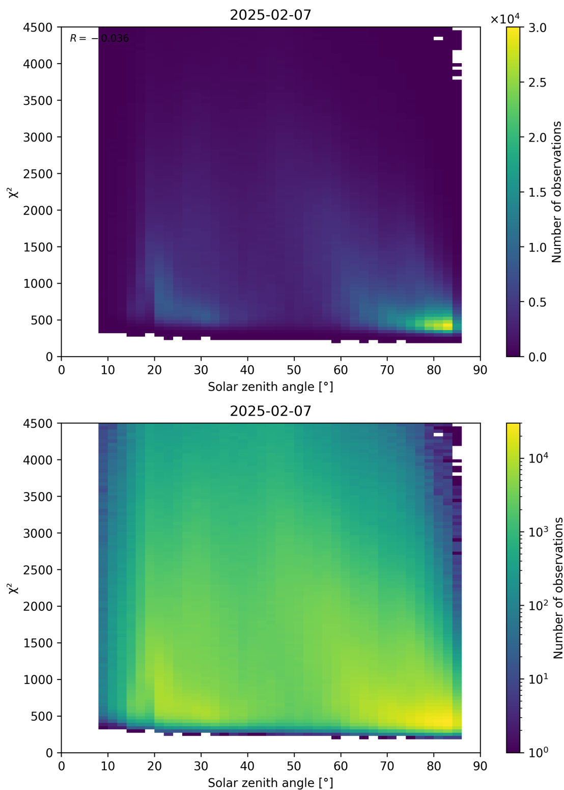
Figure 64: Scatter density plot of “Solar zenith angle” against “ \chi^2 ” for 2025-02-06 to 2025-02-08.
