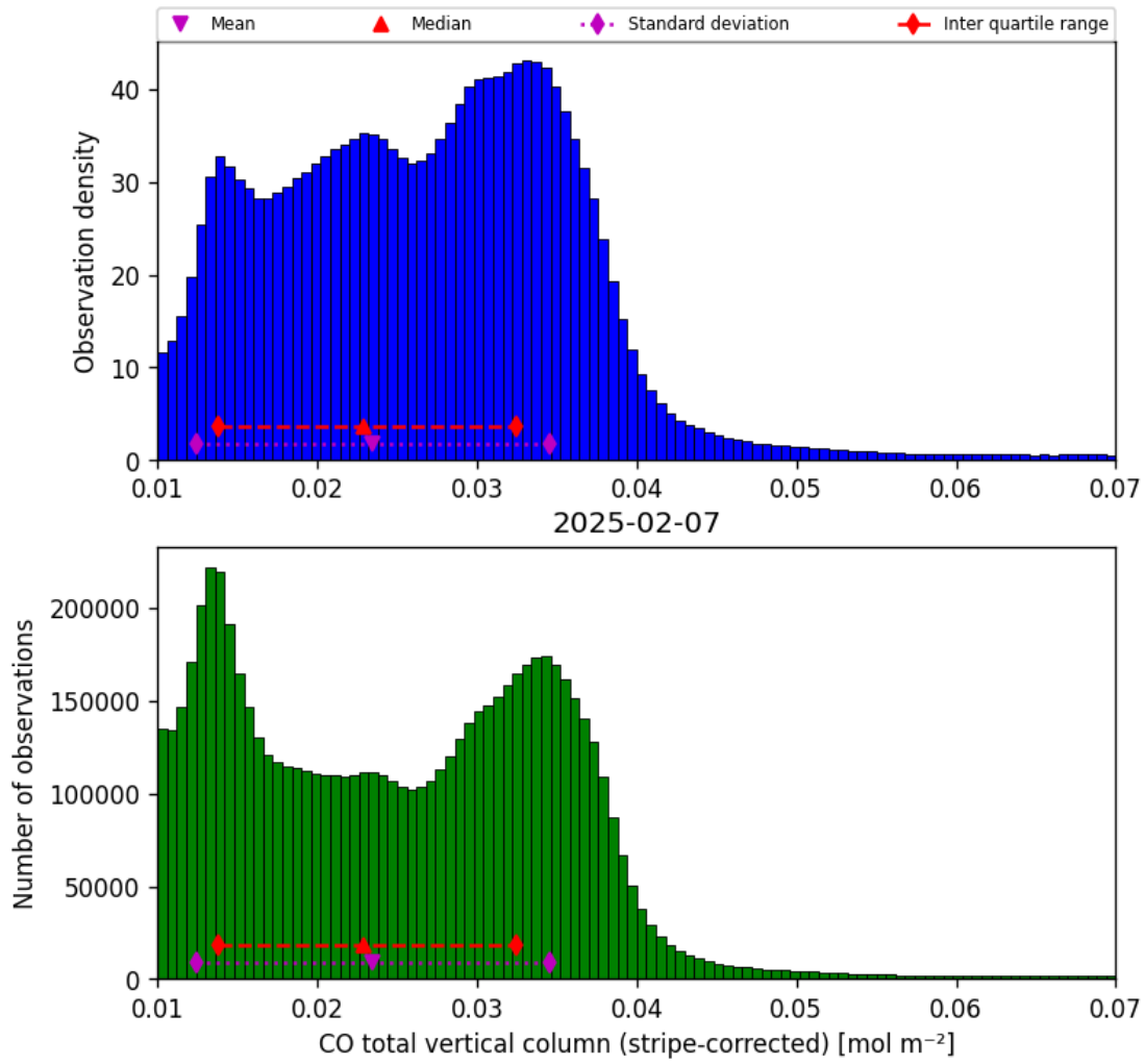
Figure 19: Histogram of “CO total vertical column (stripe-corrected)” for 2025-02-06 to 2025-02-08
