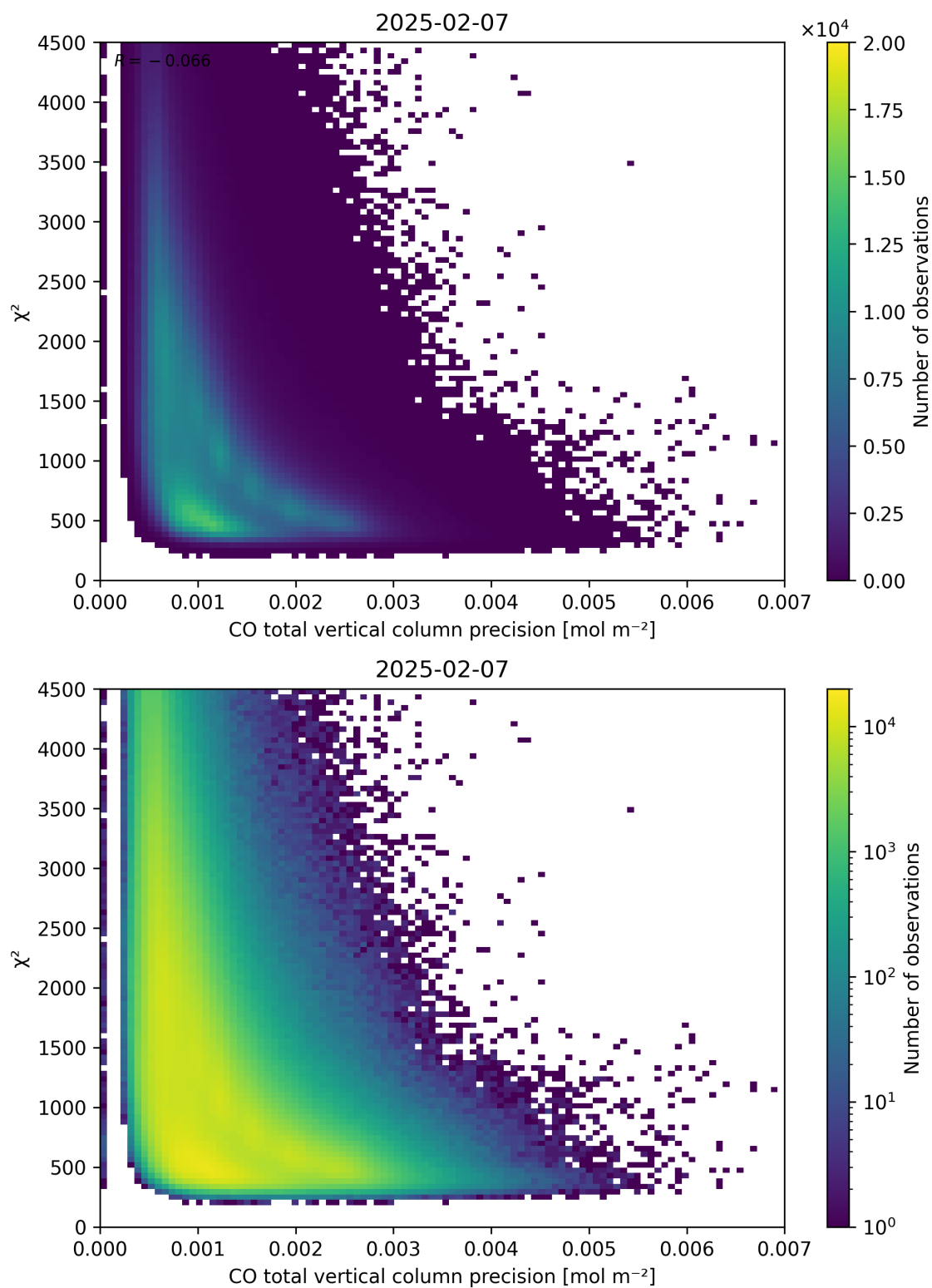
Figure 44: Scatter density plot of “CO total vertical column precision” against “ \chi^2 ” for 2025-02-06 to 2025-02-08.
