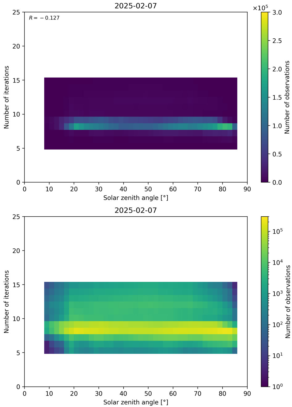
Figure 67: Scatter density plot of “Solar zenith angle” against “Number of iterations” for 2025-02-06 to 2025-02-08.
