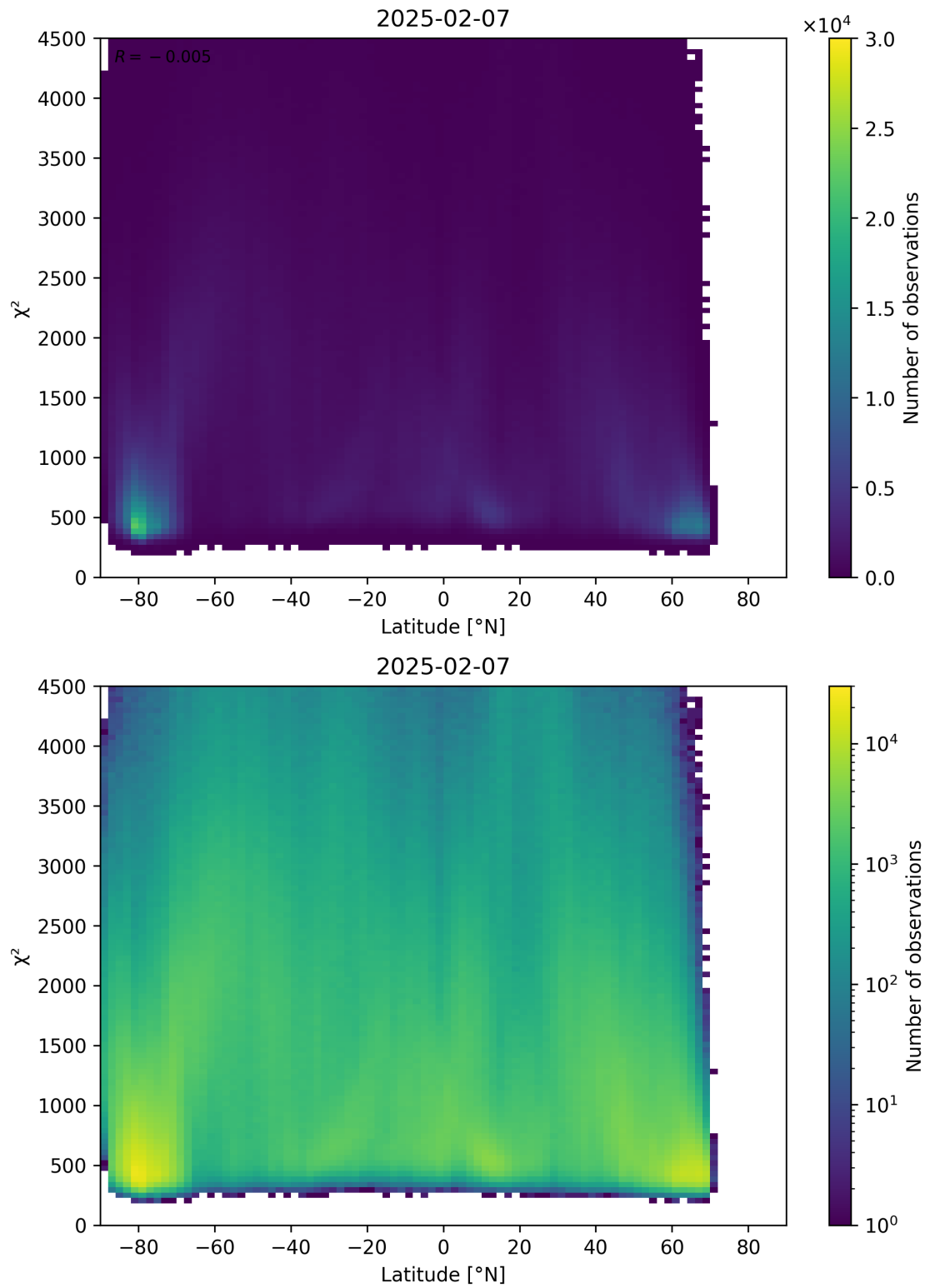
Figure 54: Scatter density plot of “Latitude” against “ \chi^2 ” for 2025-02-06 to 2025-02-08.
