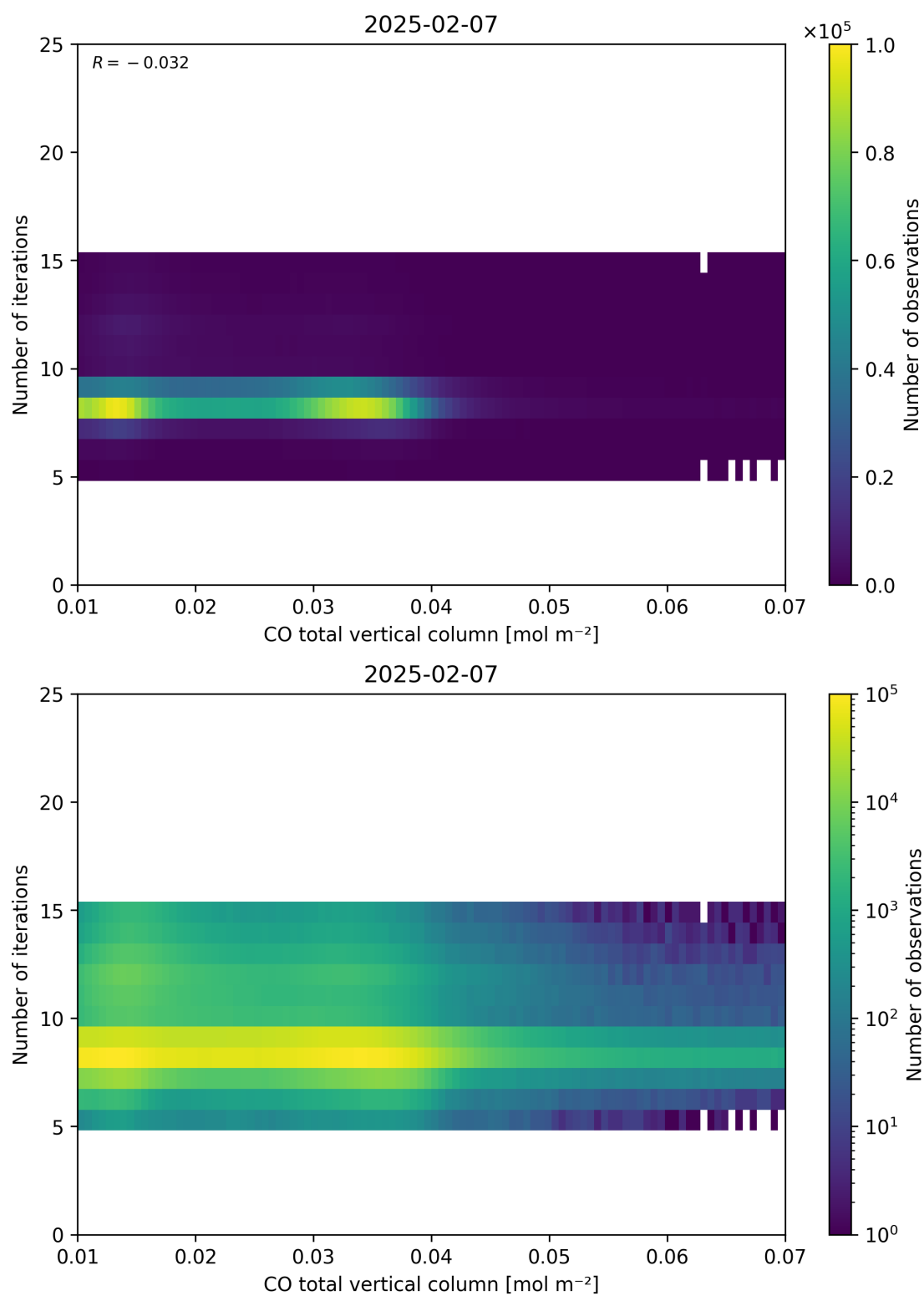
Figure 42: Scatter density plot of “CO total vertical column” against “Number of iterations” for 2025-02-06 to 2025-02-08.
