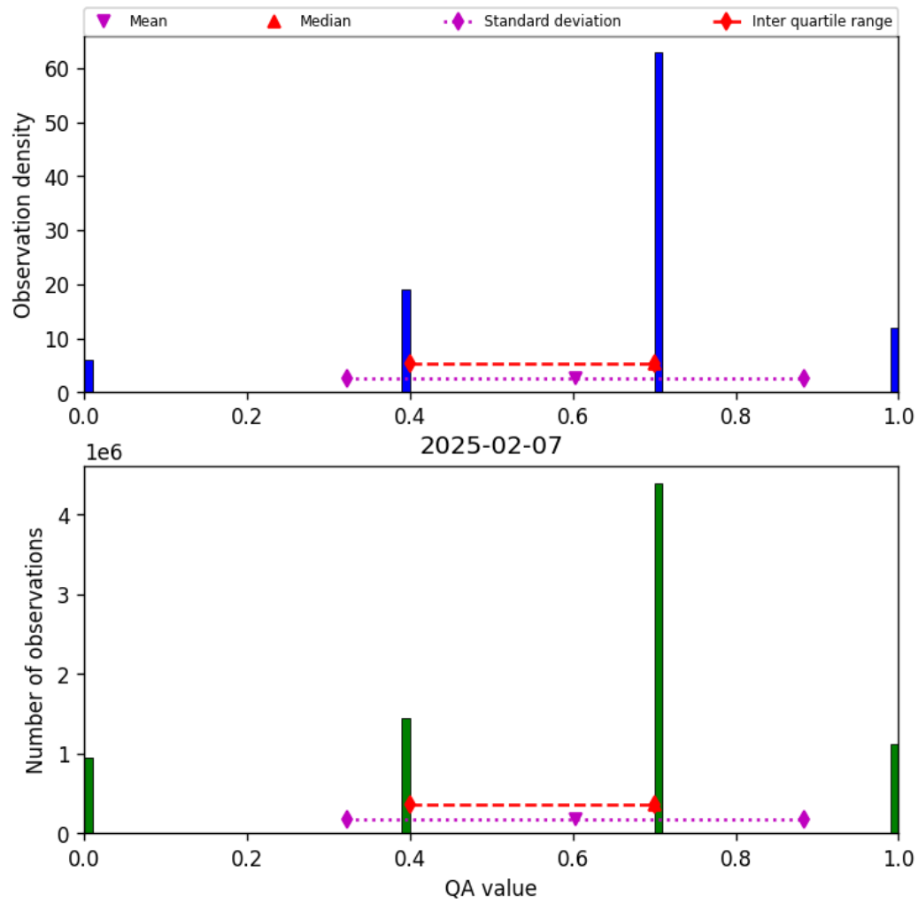
Figure 17: Histogram of “QA value” for 2025-02-06 to 2025-02-08
