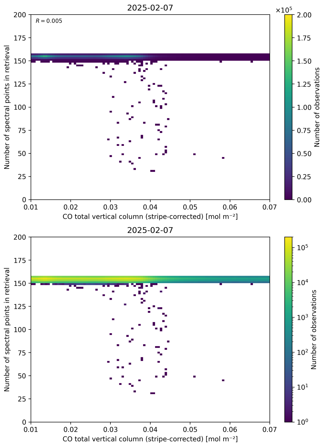
Figure 40: Scatter density plot of “CO total vertical column (stripe-corrected)” against “Number of spectral points in retrieval” for 2025-02-06 to 2025-02-08.
