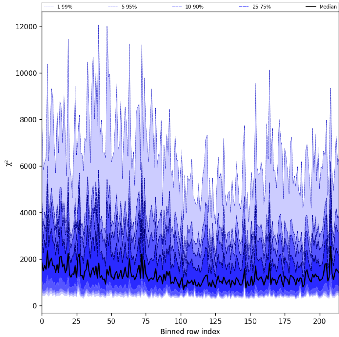
Figure 30: Along track statistics of “ \chi^2 ” for 2025-02-06 to 2025-02-08
