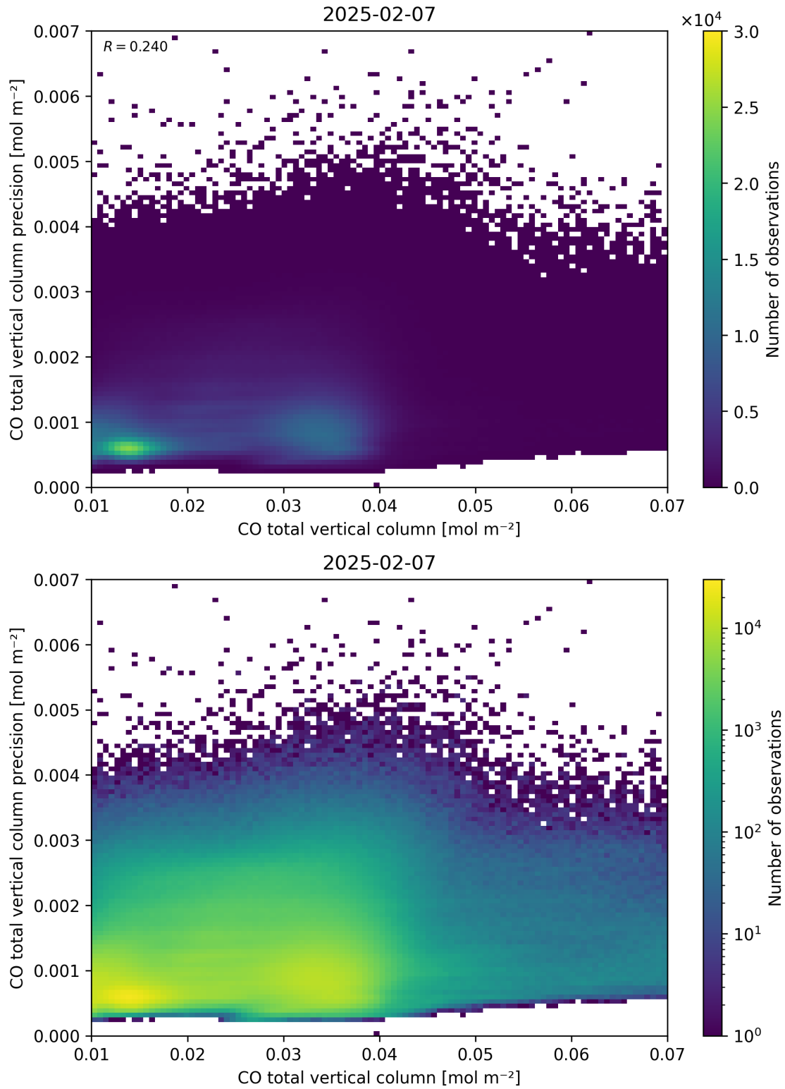
Figure 34: Scatter density plot of “CO total vertical column” against “CO total vertical column precision” for 2025-02-06 to 2025-02-08.
