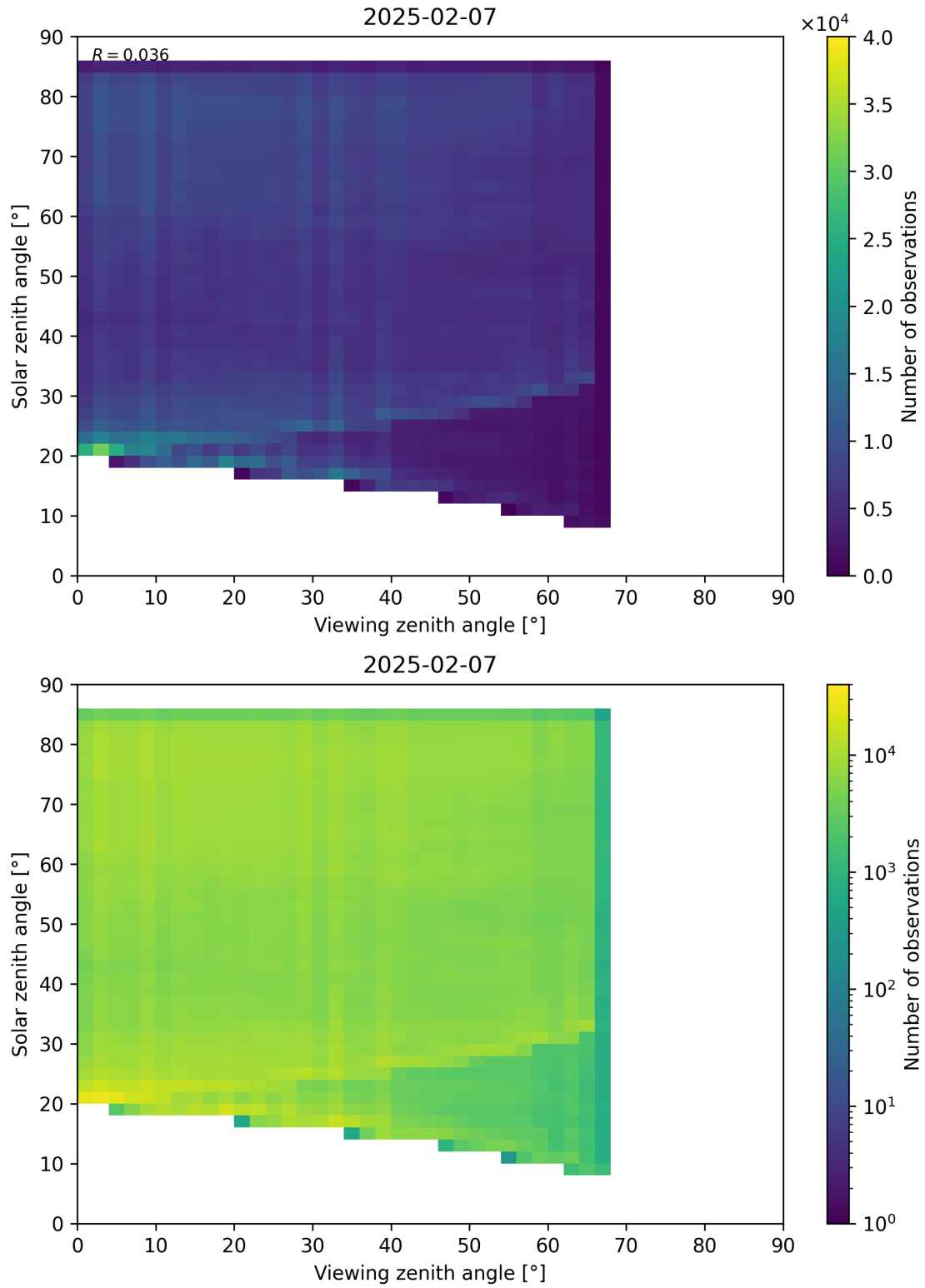
Figure 77: Scatter density plot of “Viewing zenith angle” against “Solar zenith angle” for 2025-02-06 to 2025-02-08.
