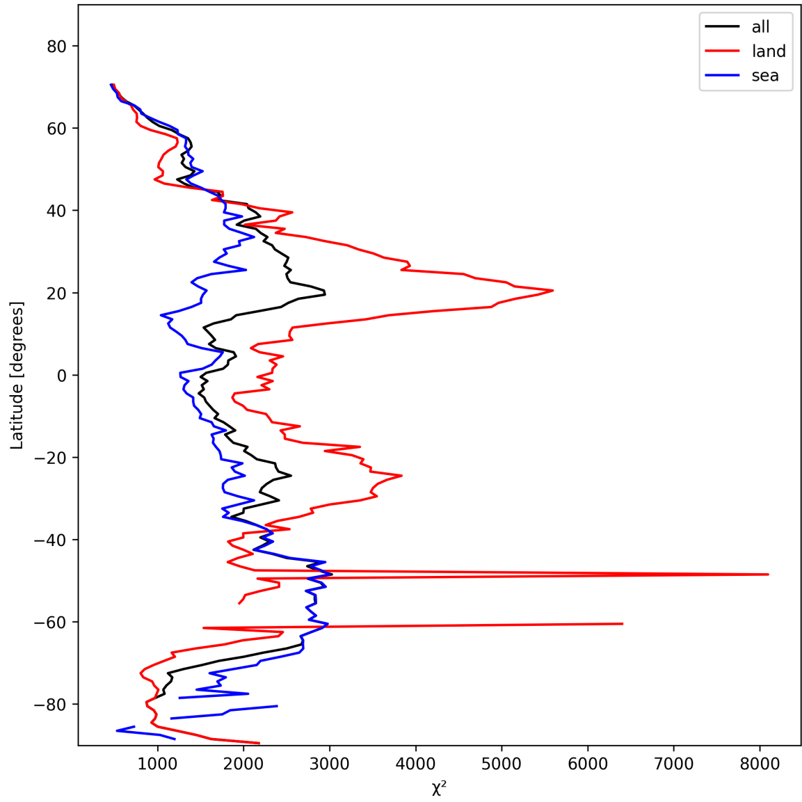
Figure 14: Zonal average of “ \chi^2 ” for 2025-02-08 to 2025-02-09.
