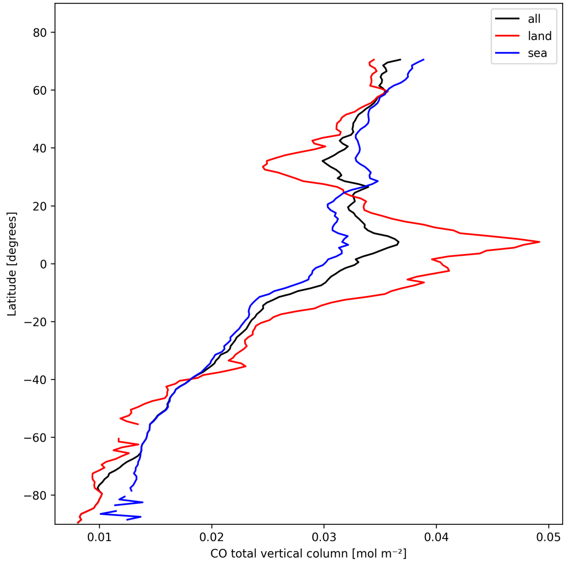
Figure 10: Zonal average of “CO total vertical column” for 2025-02-08 to 2025-02-09.
