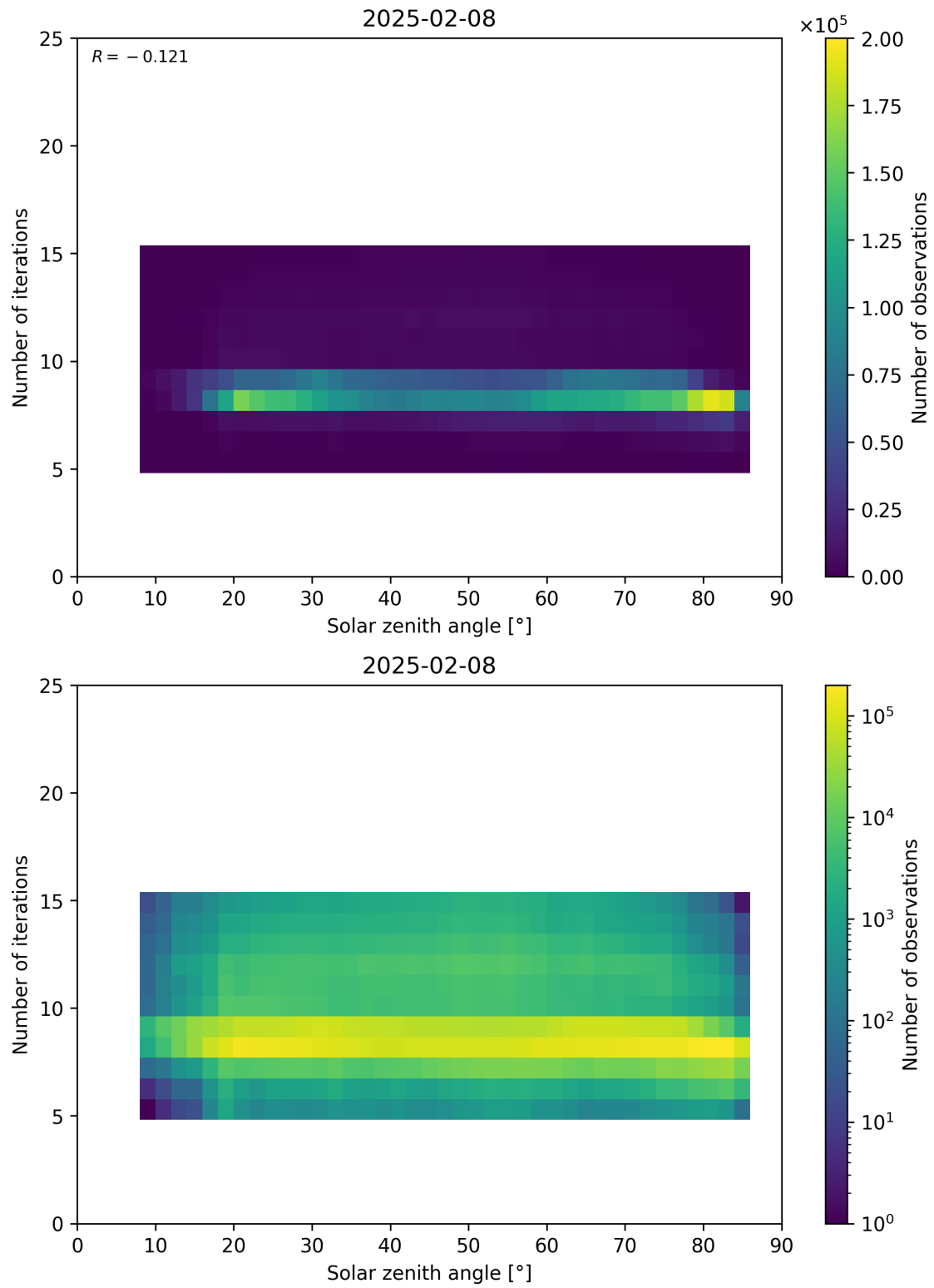
Figure 67: Scatter density plot of “Solar zenith angle” against “Number of iterations” for 2025-02-08 to 2025-02-09.
