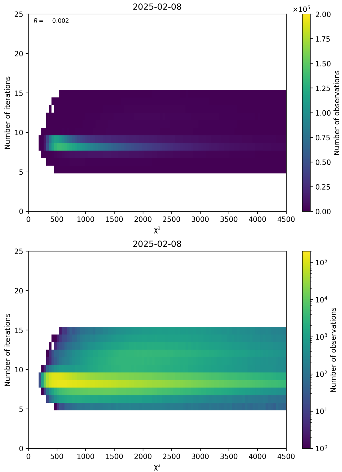
Figure 49: Scatter density plot of “ \chi^2 ” against “Number of iterations” for 2025-02-08 to 2025-02-09.
