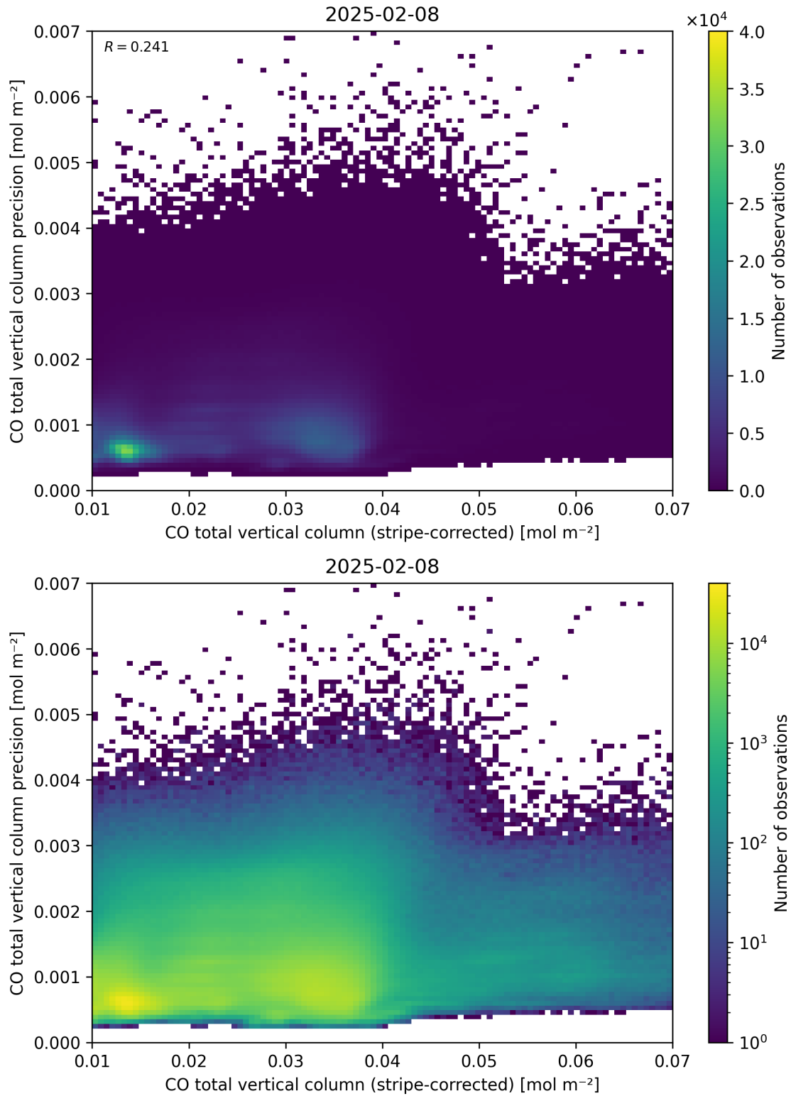
Figure 36: Scatter density plot of “CO total vertical column (stripe-corrected)” against “CO total vertical column precision” for 2025-02-08 to 2025-02-09.
