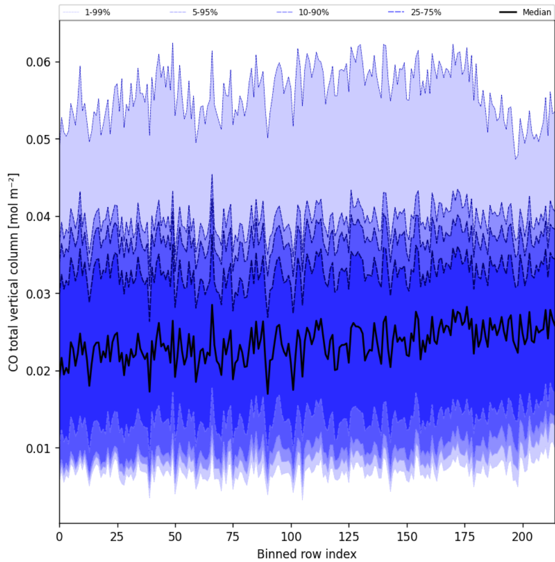
Figure 26: Along track statistics of “CO total vertical column” for 2025-02-08 to 2025-02-09
