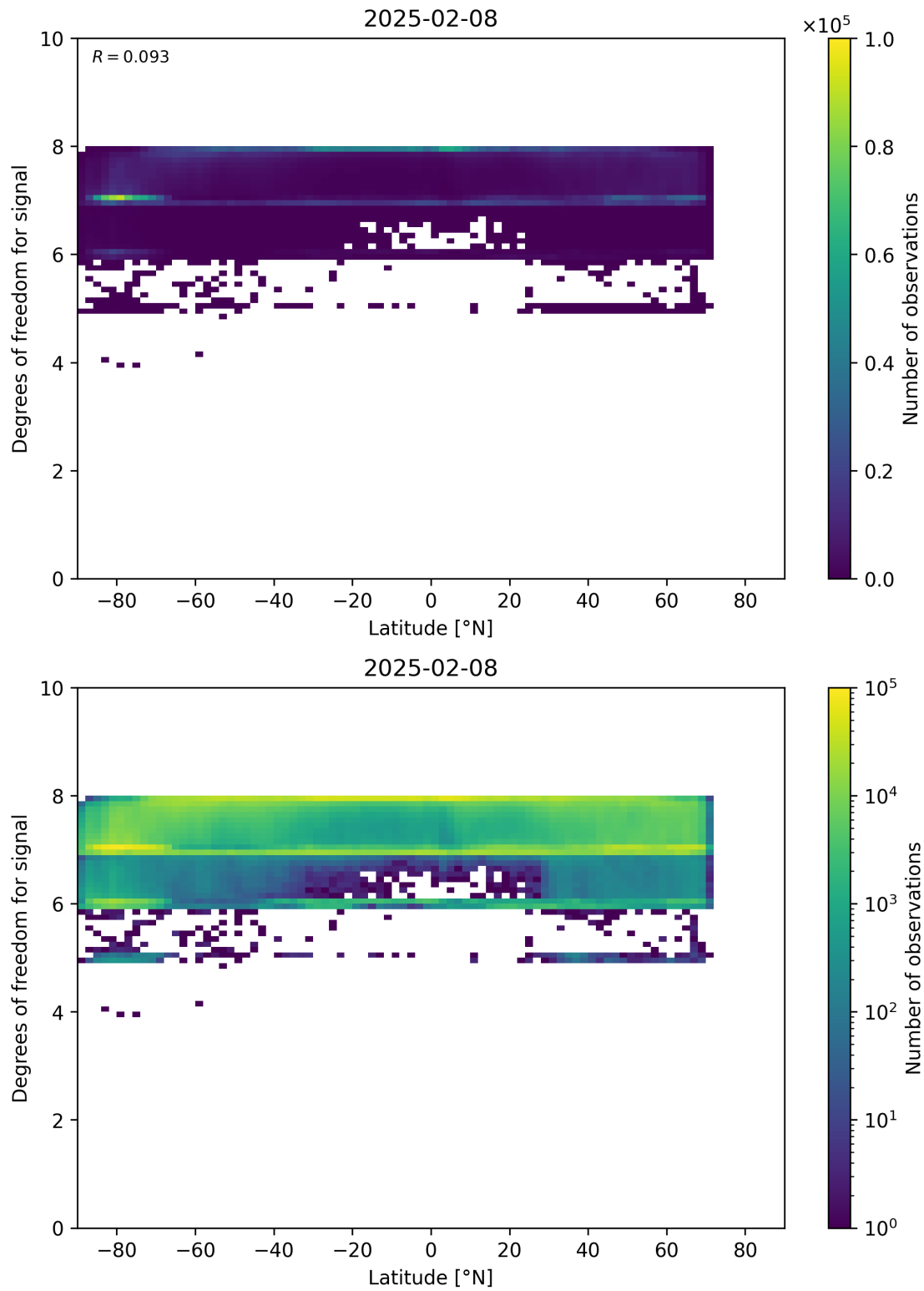
Figure 55: Scatter density plot of “Latitude” against “Degrees of freedom for signal” for 2025-02-08 to 2025-02-09.
