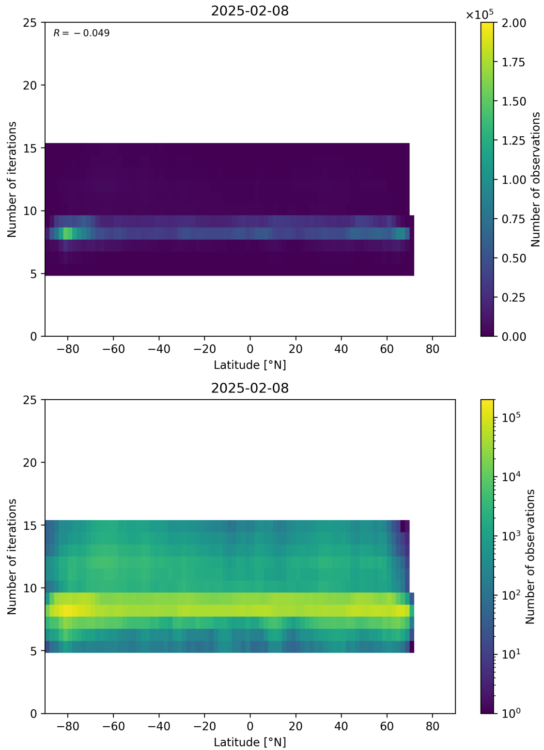
Figure 56: Scatter density plot of “Latitude” against “Number of iterations” for 2025-02-08 to 2025-02-09.
