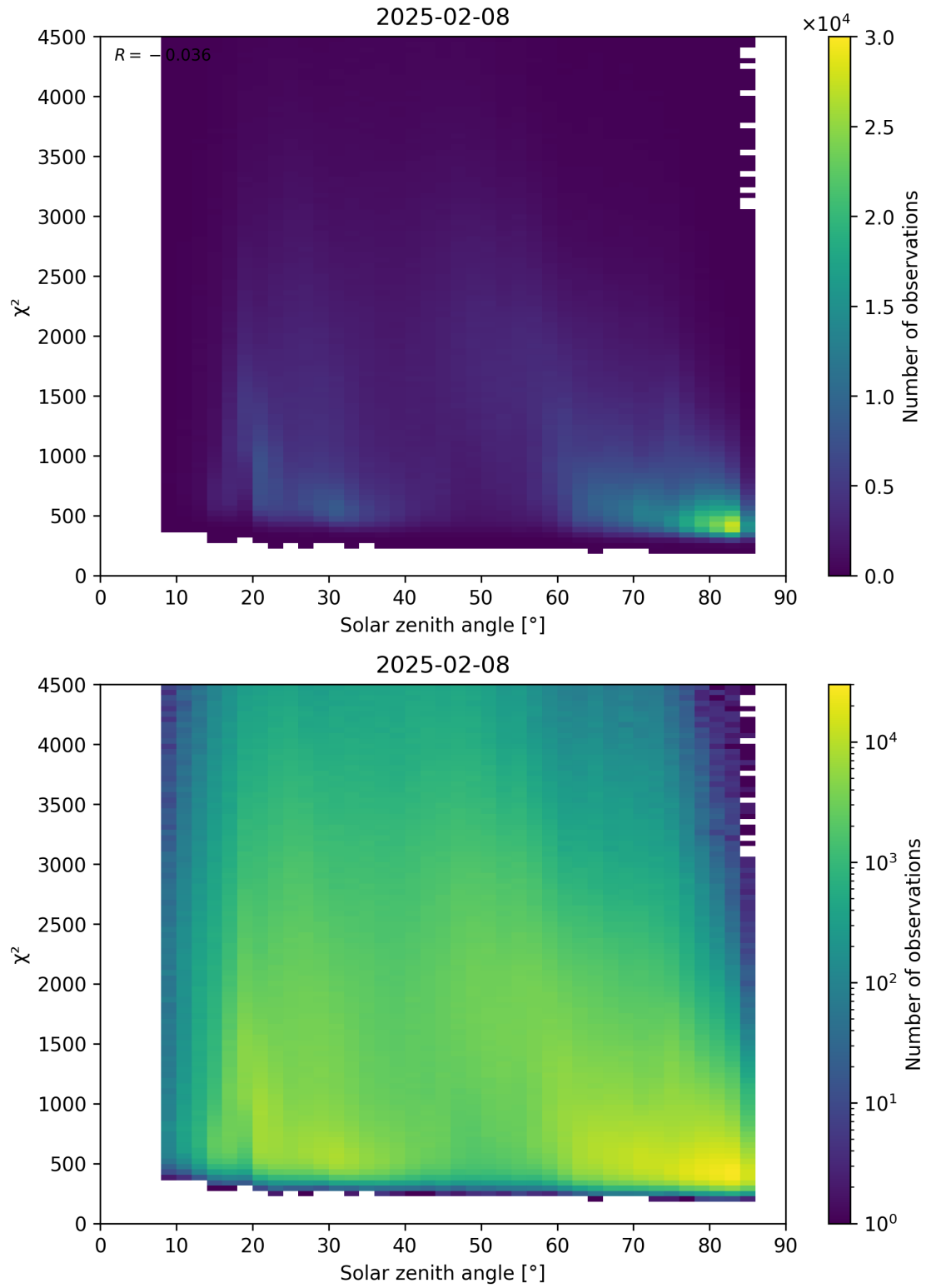
Figure 64: Scatter density plot of “Solar zenith angle” against “ \chi^2 ” for 2025-02-08 to 2025-02-09.
