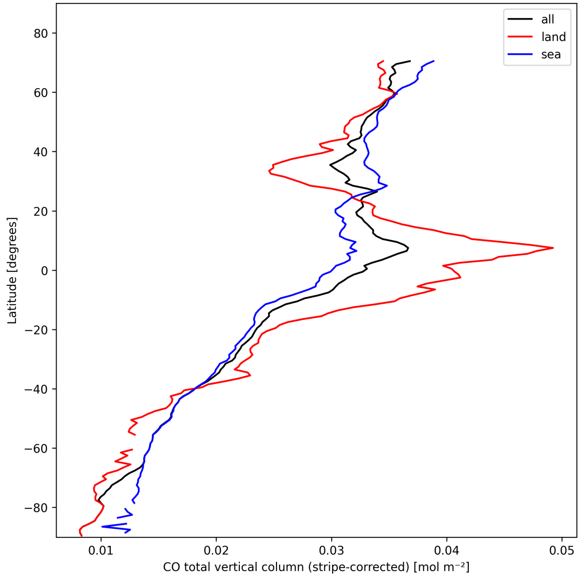
Figure 11: Zonal average of “CO total vertical column (stripe-corrected)” for 2025-02-08 to 2025-02-09.
