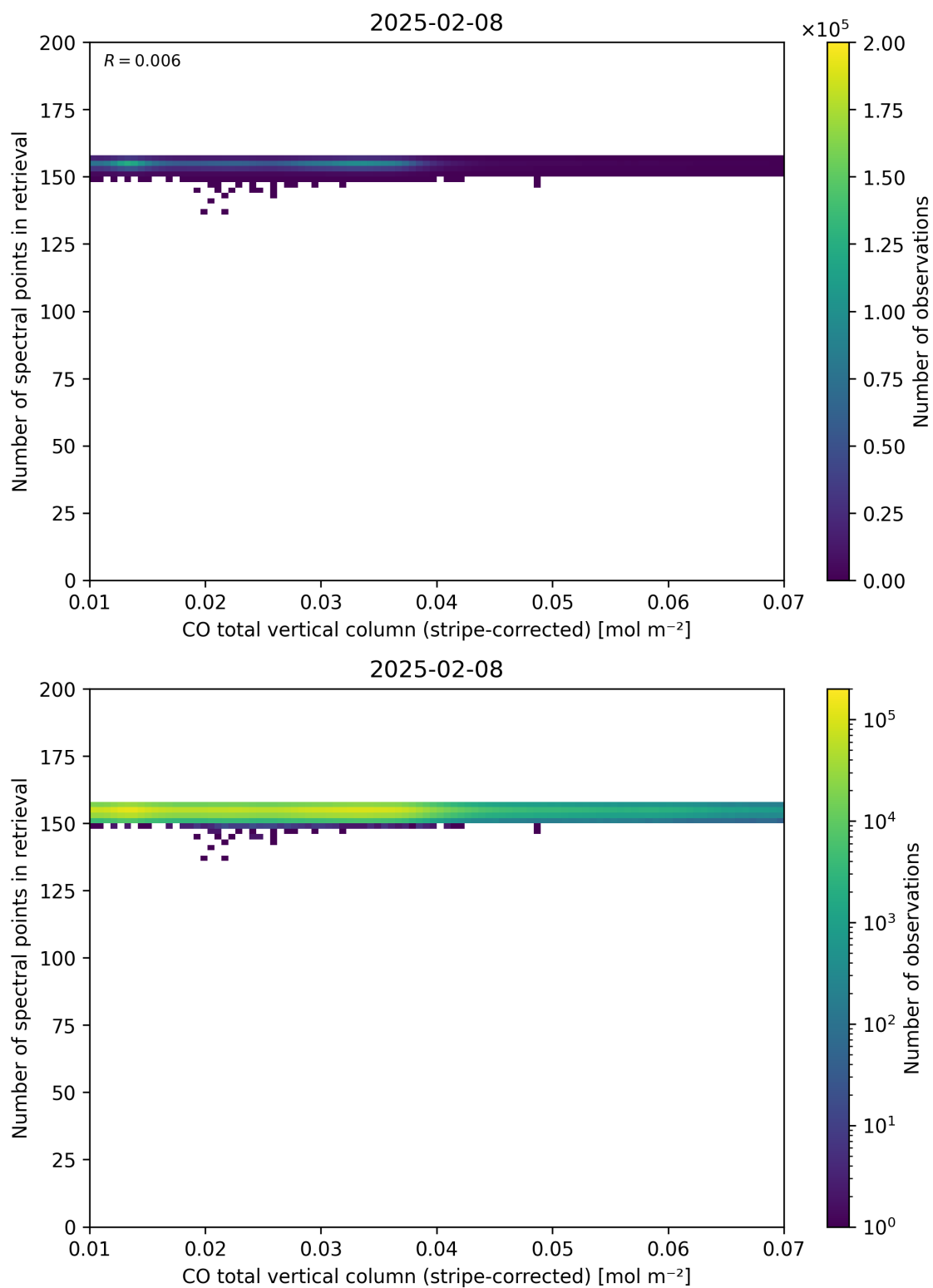
Figure 40: Scatter density plot of “CO total vertical column (stripe-corrected)” against “Number of spectral points in retrieval” for 2025-02-08 to 2025-02-09.
