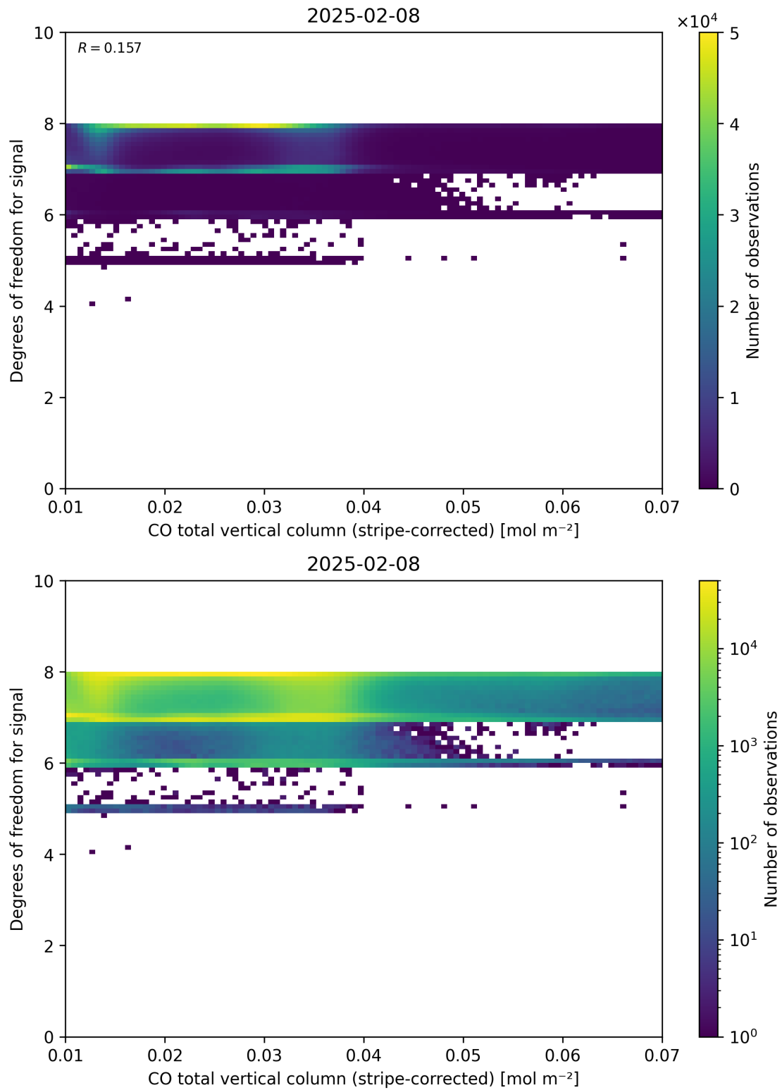
Figure 38: Scatter density plot of “CO total vertical column (stripe-corrected)” against “Degrees of freedom for signal” for 2025-02-08 to 2025-02-09.
