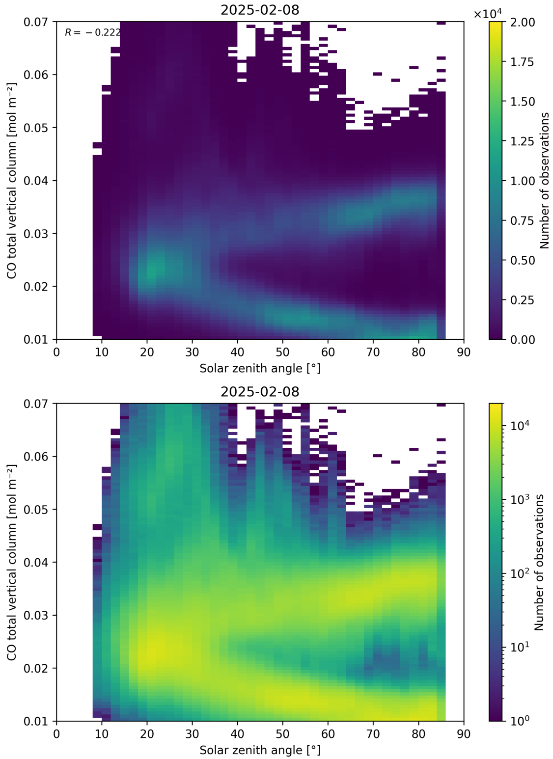
Figure 61: Scatter density plot of “Solar zenith angle” against “CO total vertical column” for 2025-02-08 to 2025-02-09.
