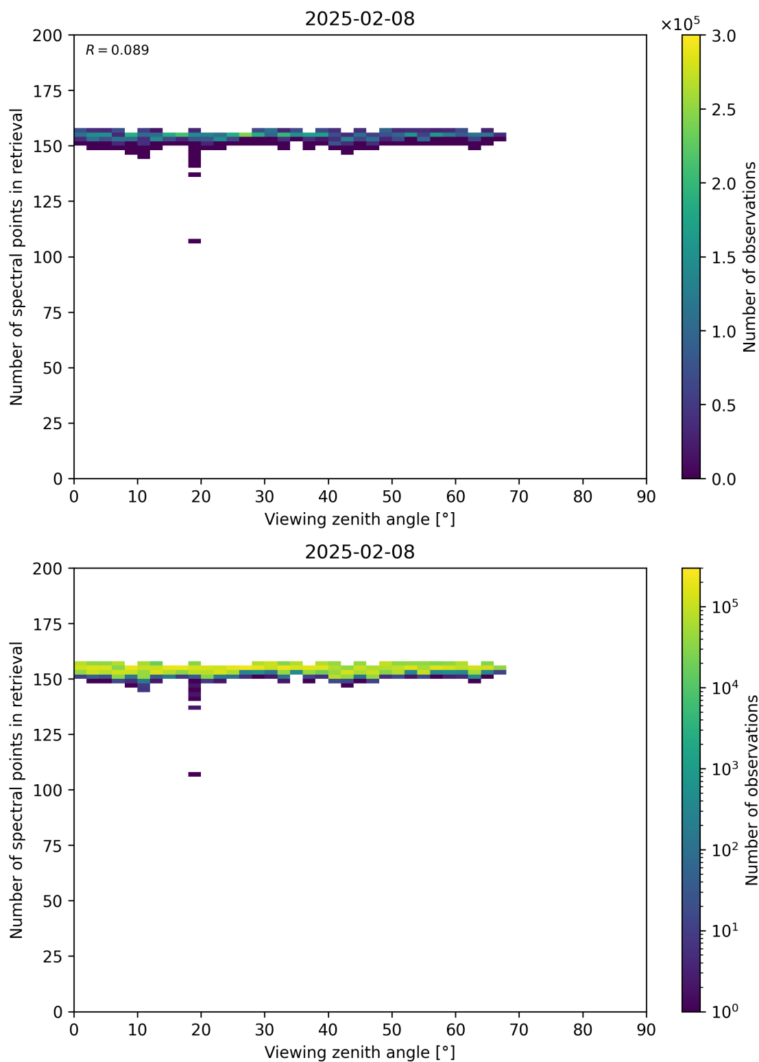
Figure 76: Scatter density plot of “Viewing zenith angle” against “Number of spectral points in retrieval” for 2025-02-08 to 2025-02-09.
