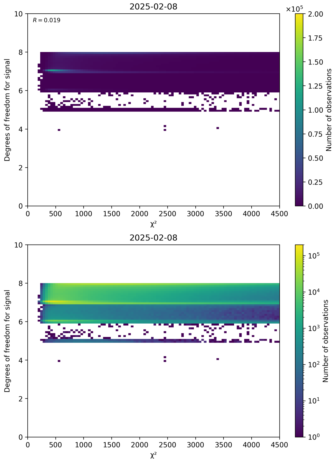
Figure 48: Scatter density plot of “ \chi^2 ” against “Degrees of freedom for signal” for 2025-02-08 to 2025-02-09.
