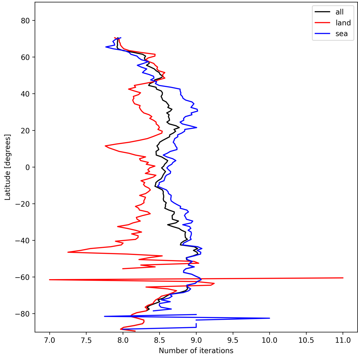
Figure 16: Zonal average of “Number of iterations” for 2025-02-08 to 2025-02-09.
