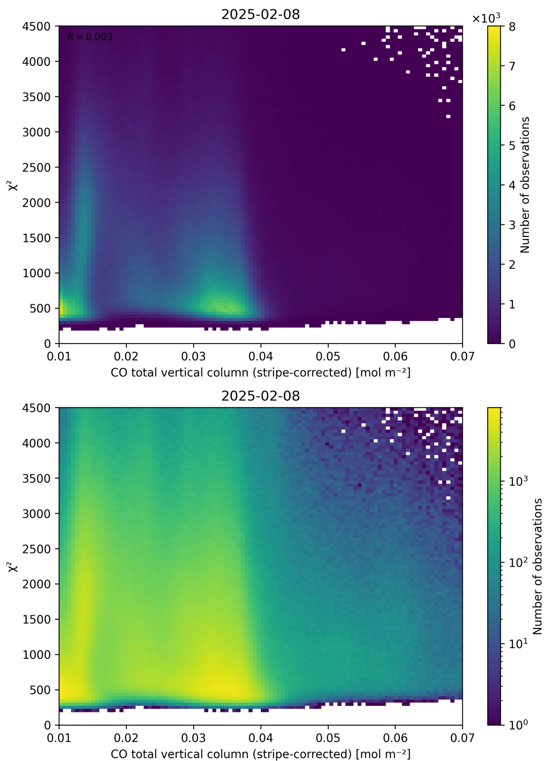
Figure 37: Scatter density plot of “CO total vertical column (stripe-corrected)” against “ \chi^2 ” for 2025-02-08 to 2025-02-09.
