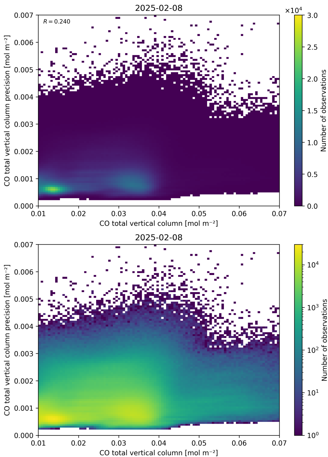
Figure 34: Scatter density plot of “CO total vertical column” against “CO total vertical column precision” for 2025-02-08 to 2025-02-09.
