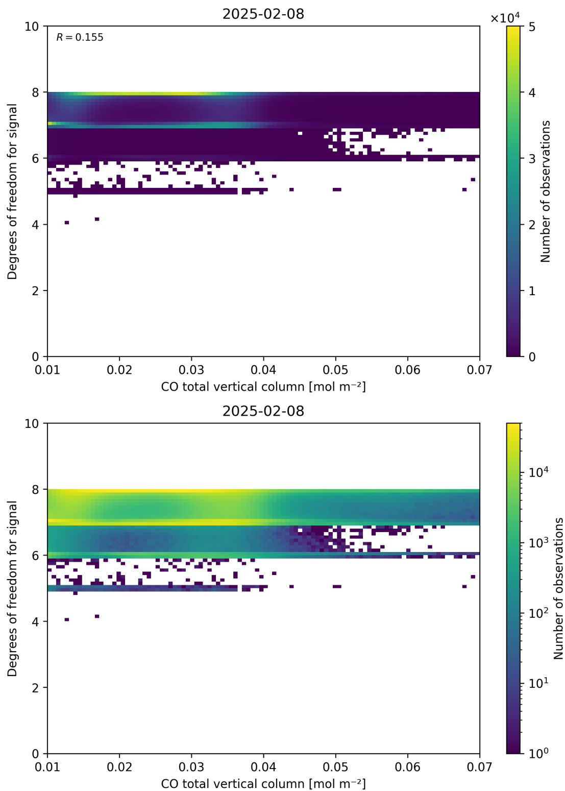
Figure 41: Scatter density plot of “CO total vertical column” against “Degrees of freedom for signal” for 2025-02-08 to 2025-02-09.
