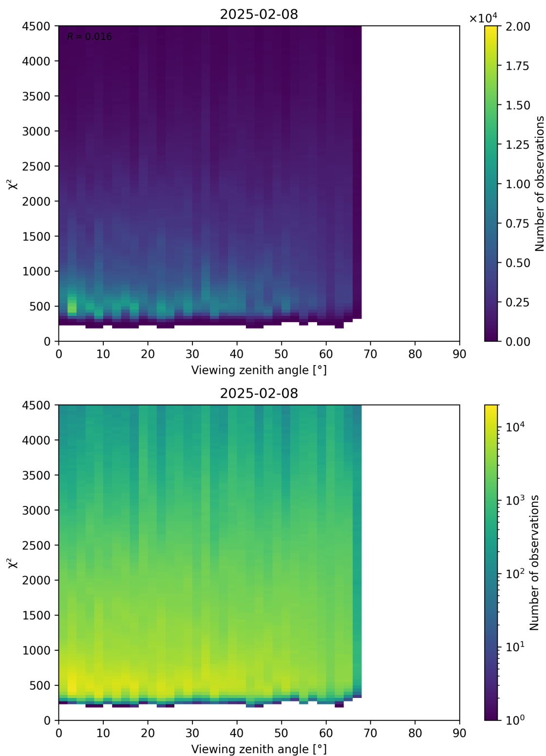
Figure 72: Scatter density plot of “Viewing zenith angle” against “ \chi^2 ” for 2025-02-08 to 2025-02-09.
