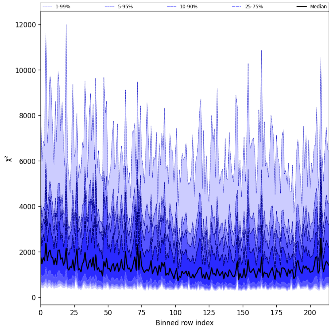
Figure 30: Along track statistics of “ \chi^2 ” for 2025-02-08 to 2025-02-09
