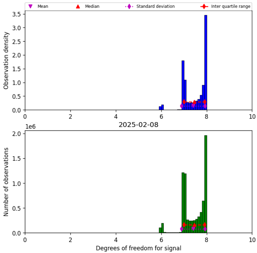
Figure 23: Histogram of “Degrees of freedom for signal” for 2025-02-08 to 2025-02-09
