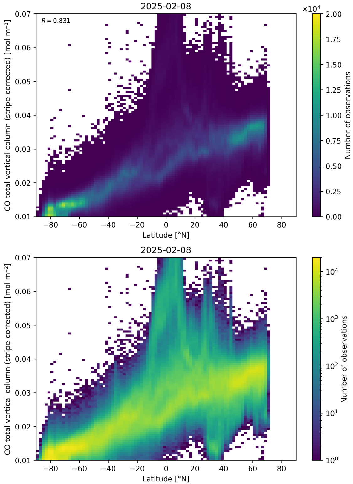
Figure 52: Scatter density plot of “Latitude” against “CO total vertical column (stripe-corrected)” for 2025-02-08 to 2025-02-09.
