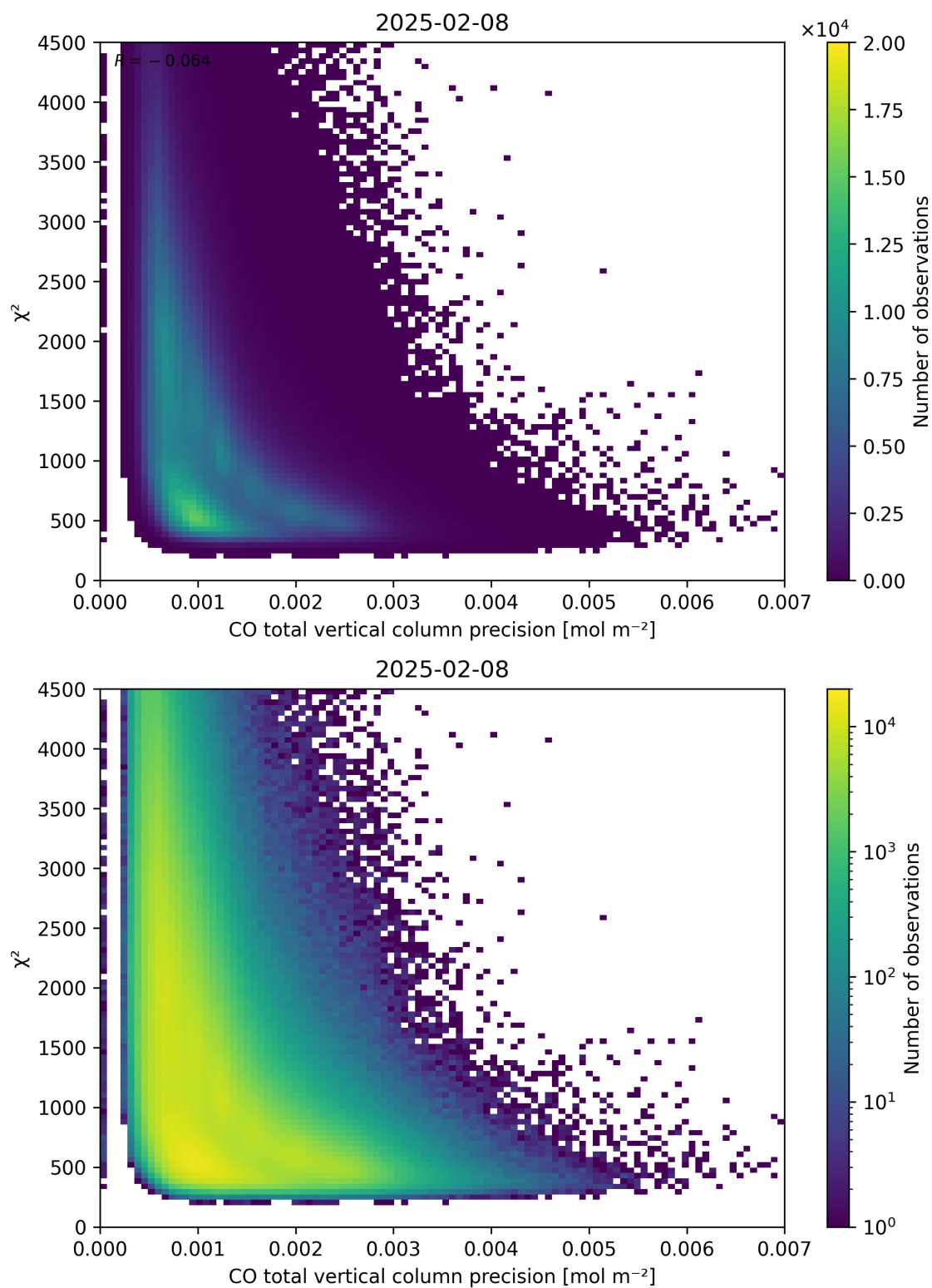
Figure 44: Scatter density plot of “CO total vertical column precision” against “ \chi^2 ” for 2025-02-08 to 2025-02-09.
