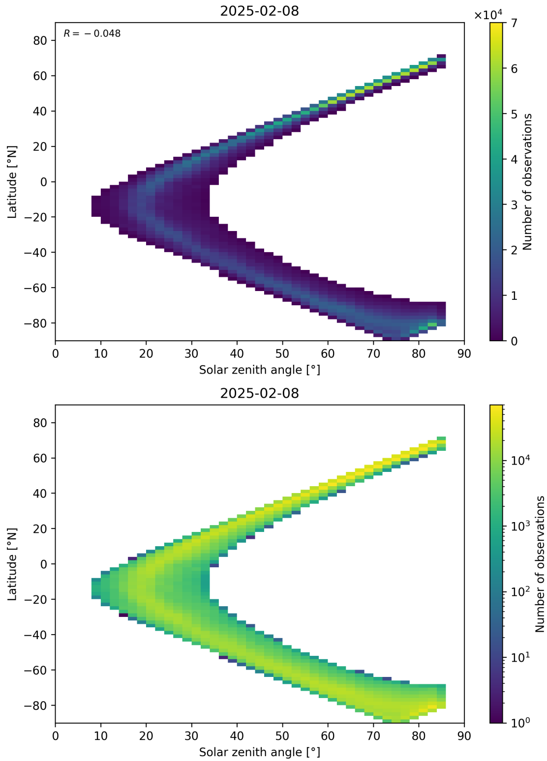
Figure 66: Scatter density plot of “Solar zenith angle” against “Latitude” for 2025-02-08 to 2025-02-09.
