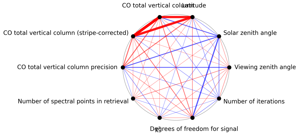
Figure 1: Map of correlation graph for 2025-02-08 to 2025-02-09.
