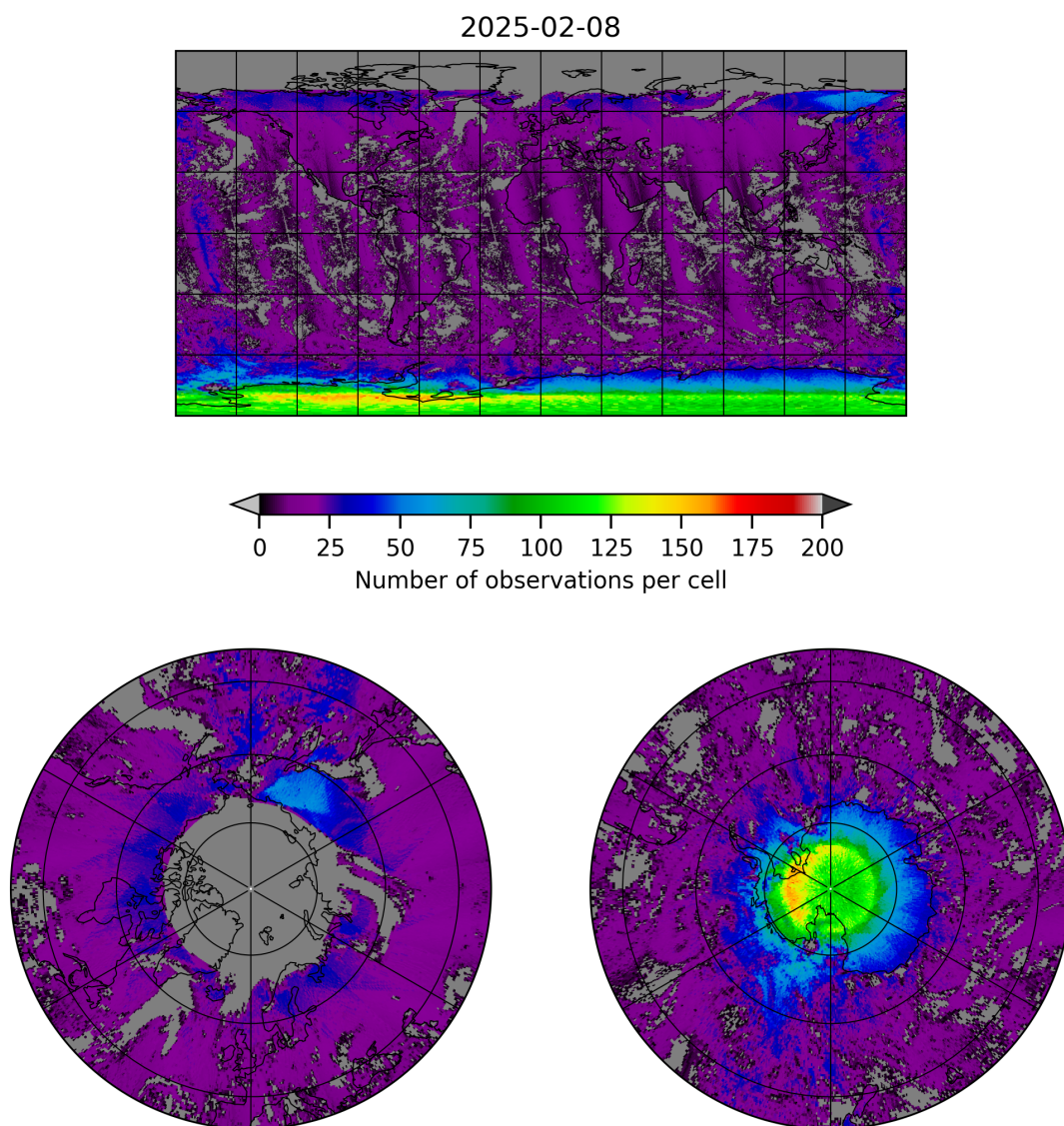
Figure 8: Map of the number of observations for 2025-02-08 to 2025-02-09
