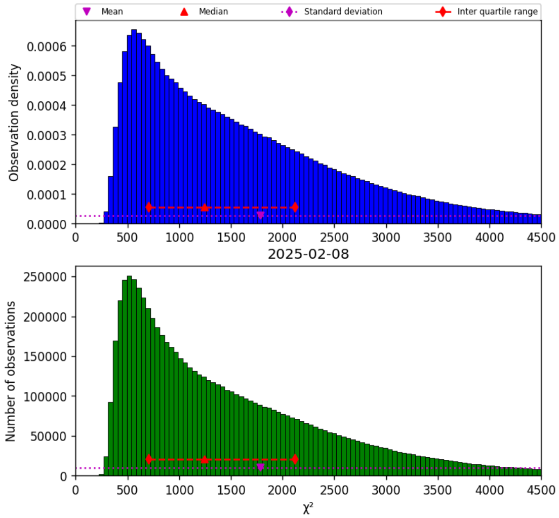
Figure 22: Histogram of “ \chi^2 ” for 2025-02-08 to 2025-02-09
