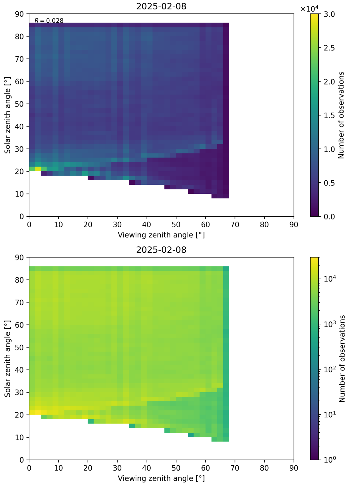
Figure 77: Scatter density plot of “Viewing zenith angle” against “Solar zenith angle” for 2025-02-08 to 2025-02-09.
