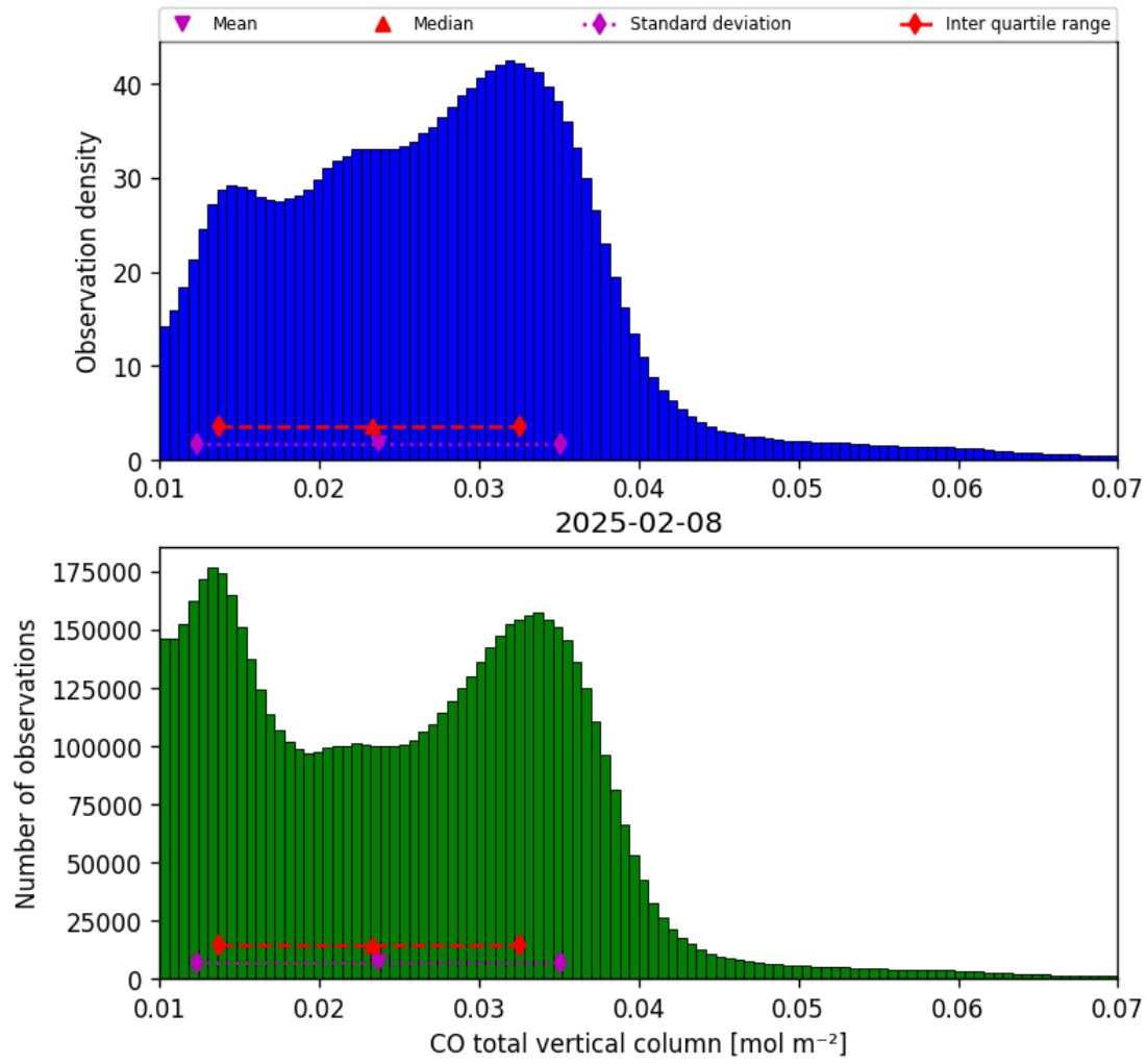
Figure 18: Histogram of “CO total vertical column” for 2025-02-08 to 2025-02-09
