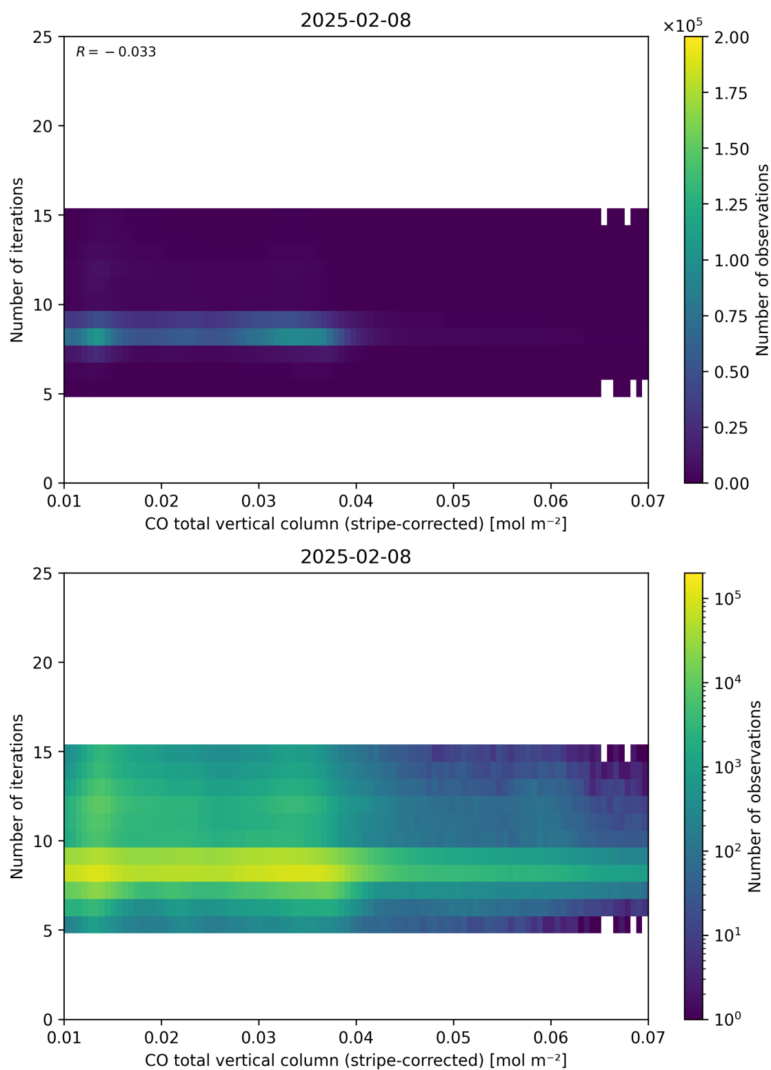
Figure 39: Scatter density plot of “CO total vertical column (stripe-corrected)” against “Number of iterations” for 2025-02-08 to 2025-02-09.
