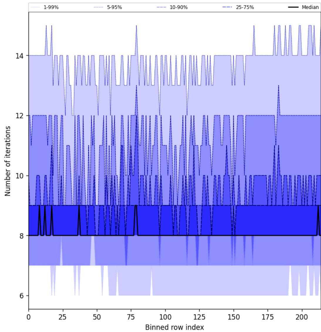
Figure 32: Along track statistics of “Number of iterations” for 2025-02-08 to 2025-02-09
