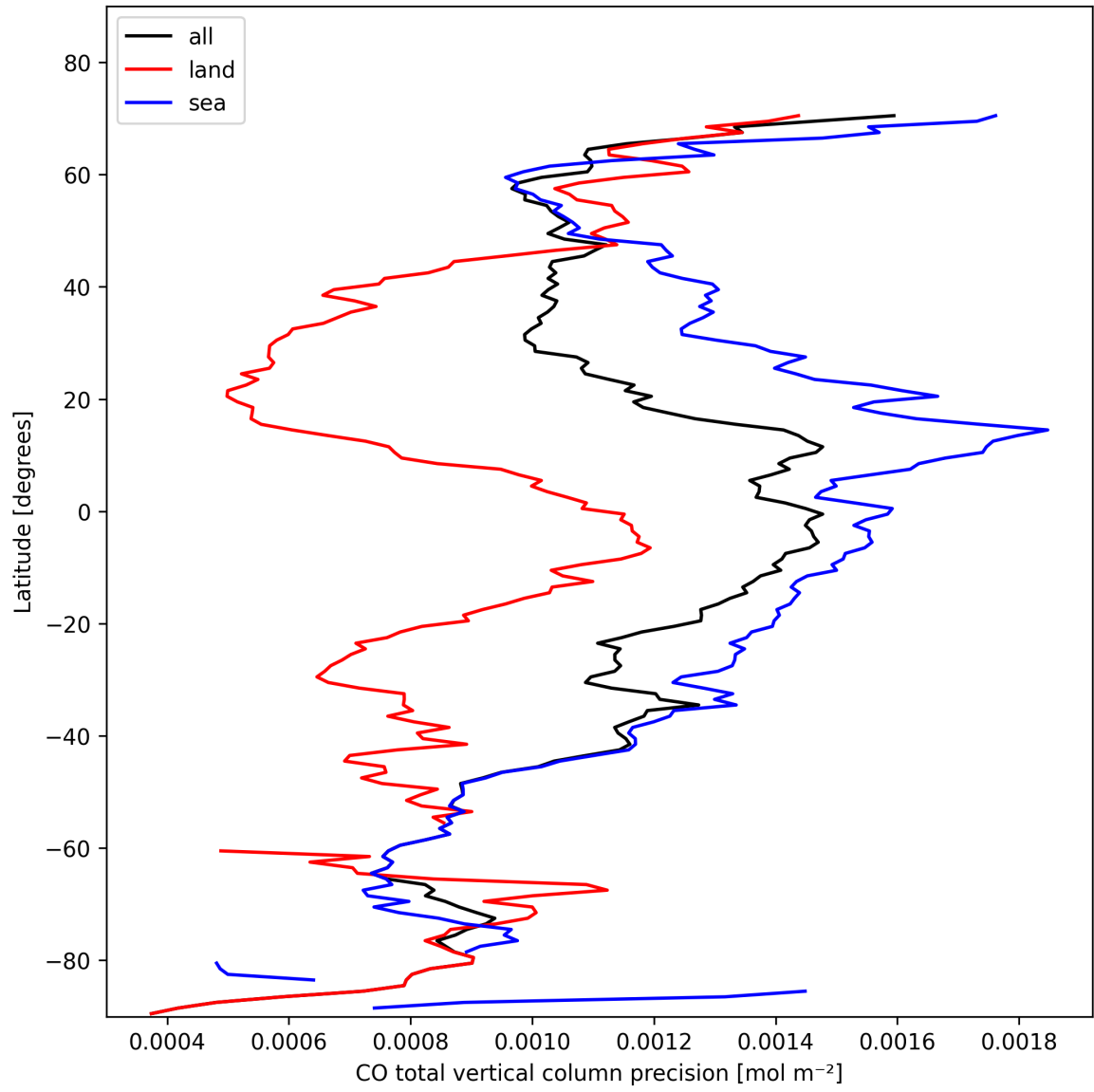
Figure 12: Zonal average of “CO total vertical column precision” for 2025-02-08 to 2025-02-09.
