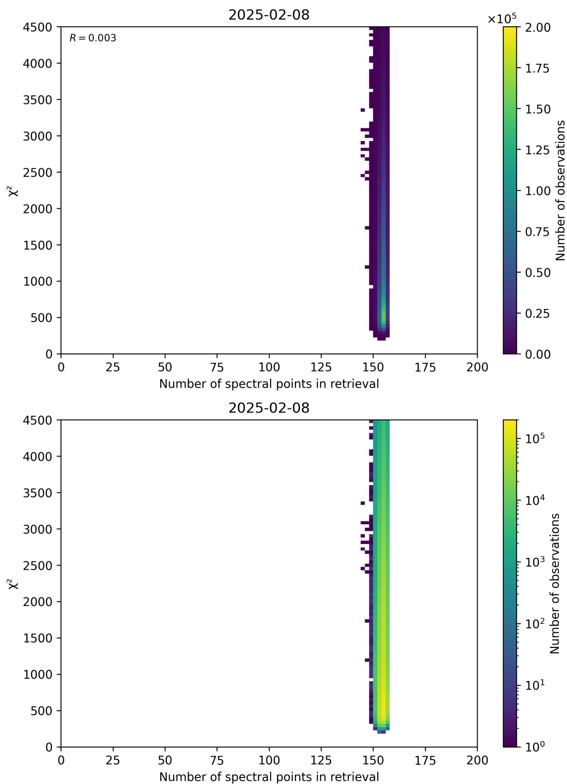
Figure 58: Scatter density plot of “Number of spectral points in retrieval” against “ \chi^2 ” for 2025-02-08 to 2025-02-09.
