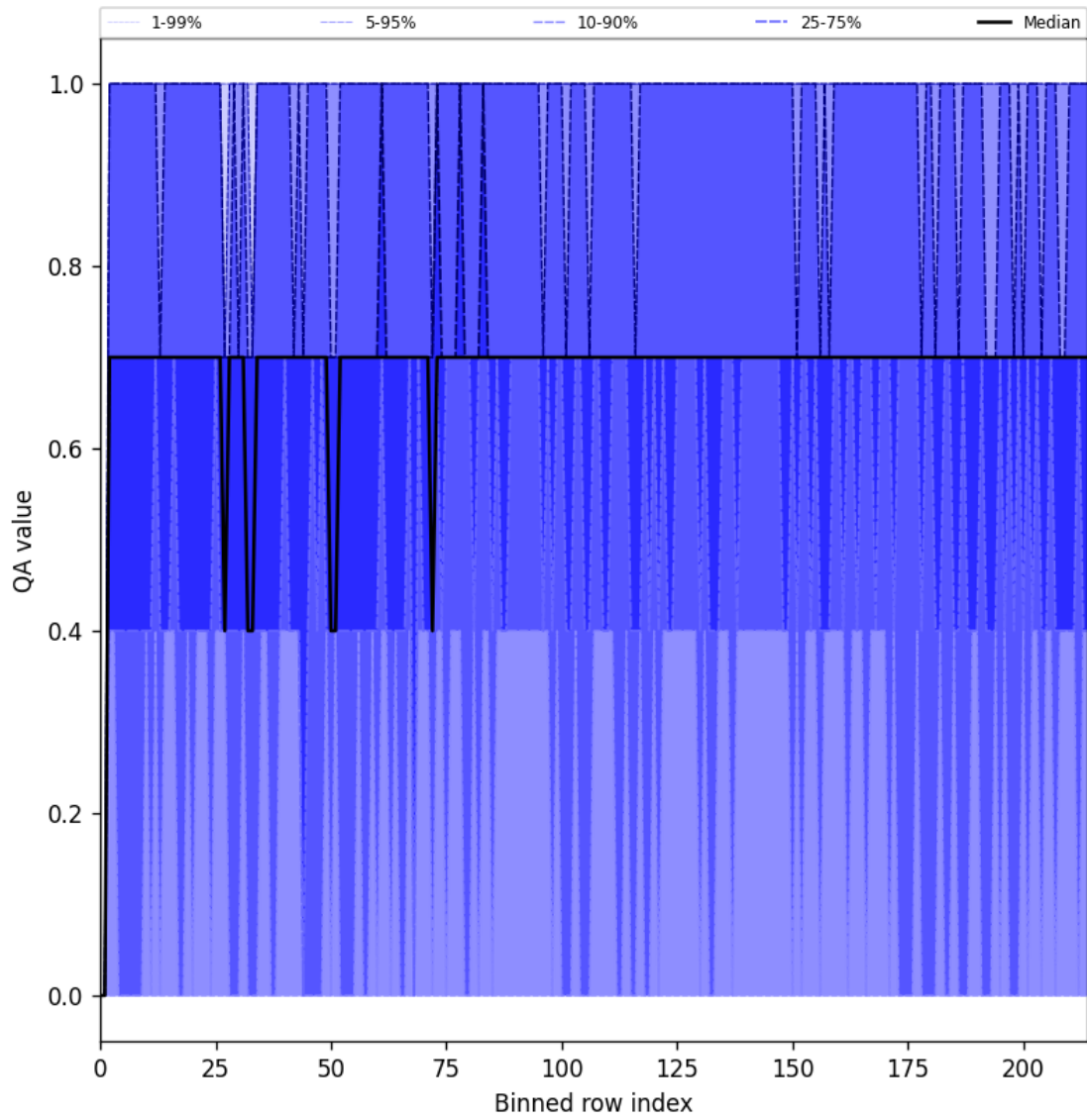
Figure 25: Along track statistics of “QA value” for 2025-02-08 to 2025-02-09
