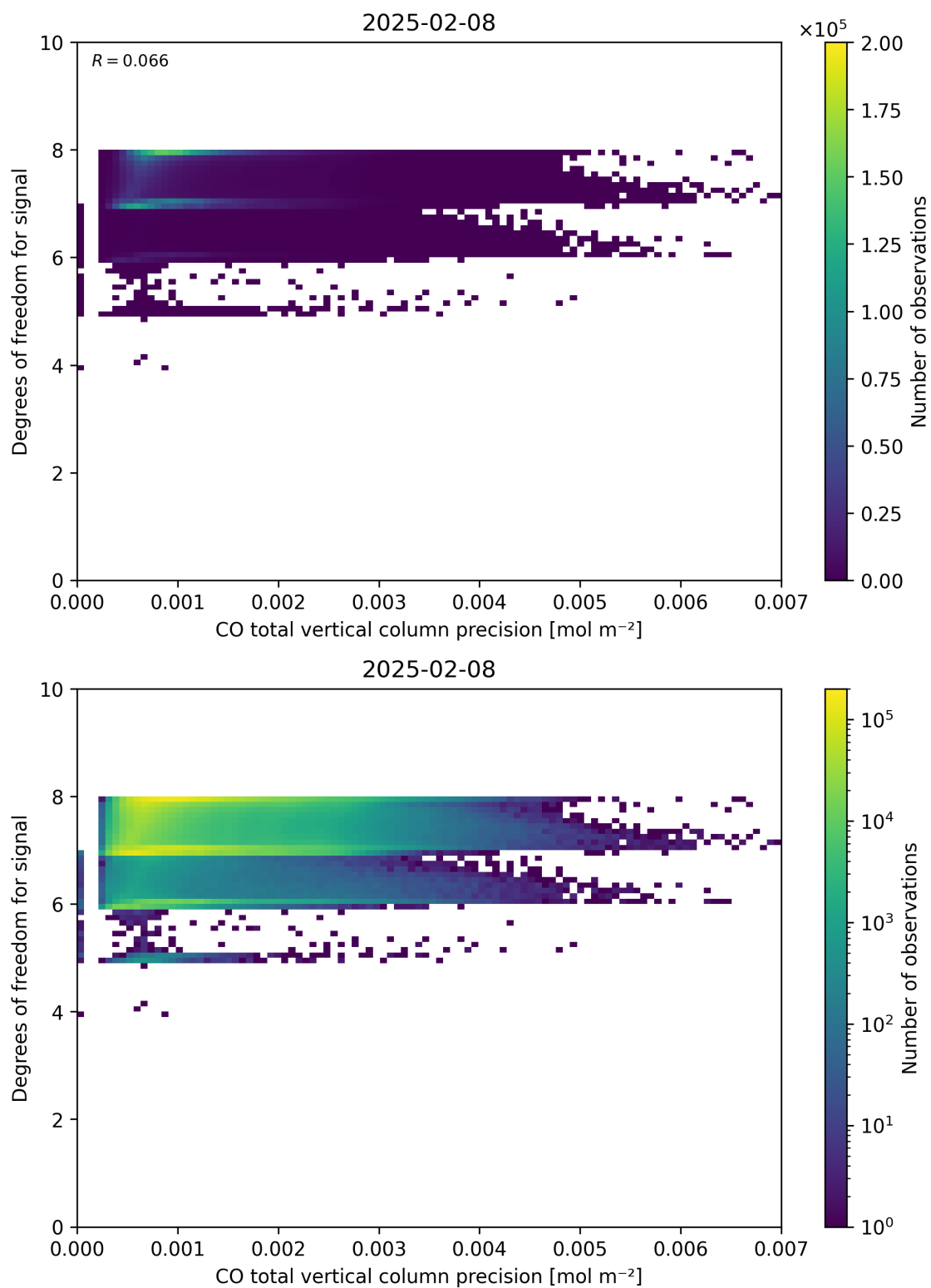
Figure 45: Scatter density plot of “CO total vertical column precision” against “Degrees of freedom for signal” for 2025-02-08 to 2025-02-09.
