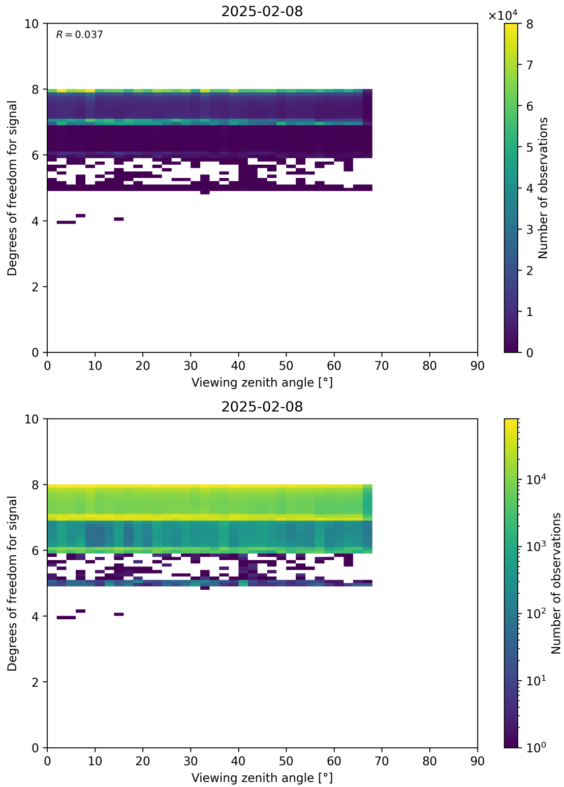
Figure 73: Scatter density plot of “Viewing zenith angle” against “Degrees of freedom for signal” for 2025-02-08 to 2025-02-09.
