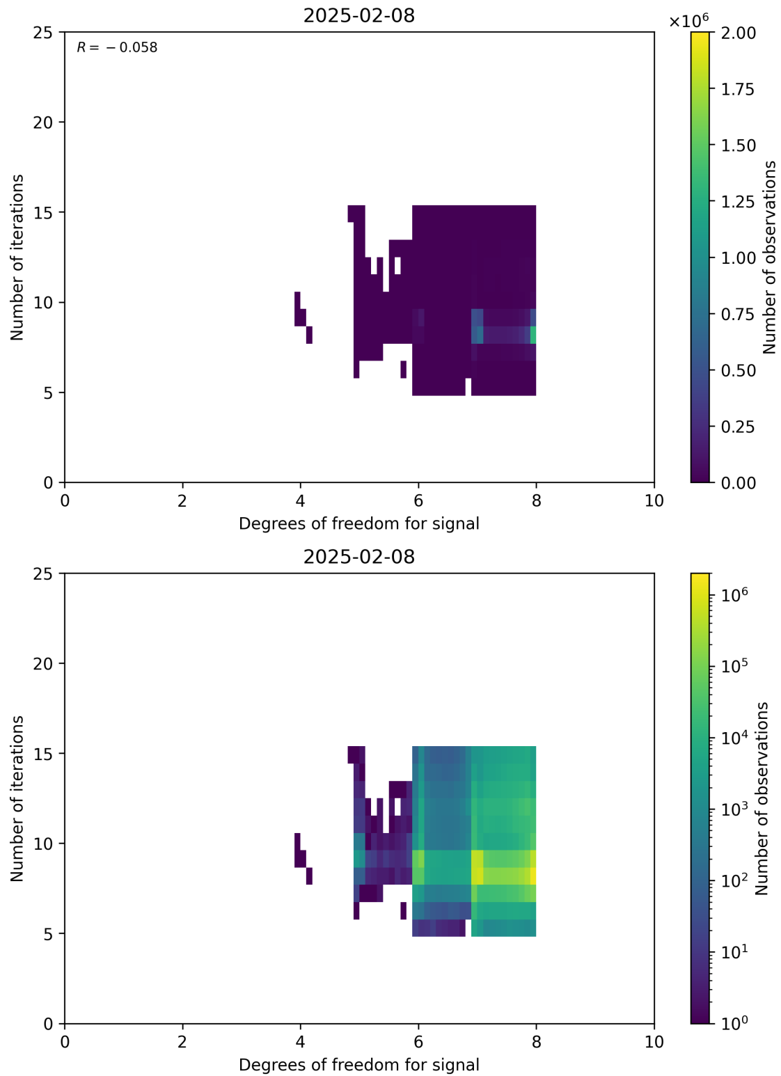
Figure 50: Scatter density plot of “Degrees of freedom for signal” against “Number of iterations” for 2025-02-08 to 2025-02-09.
