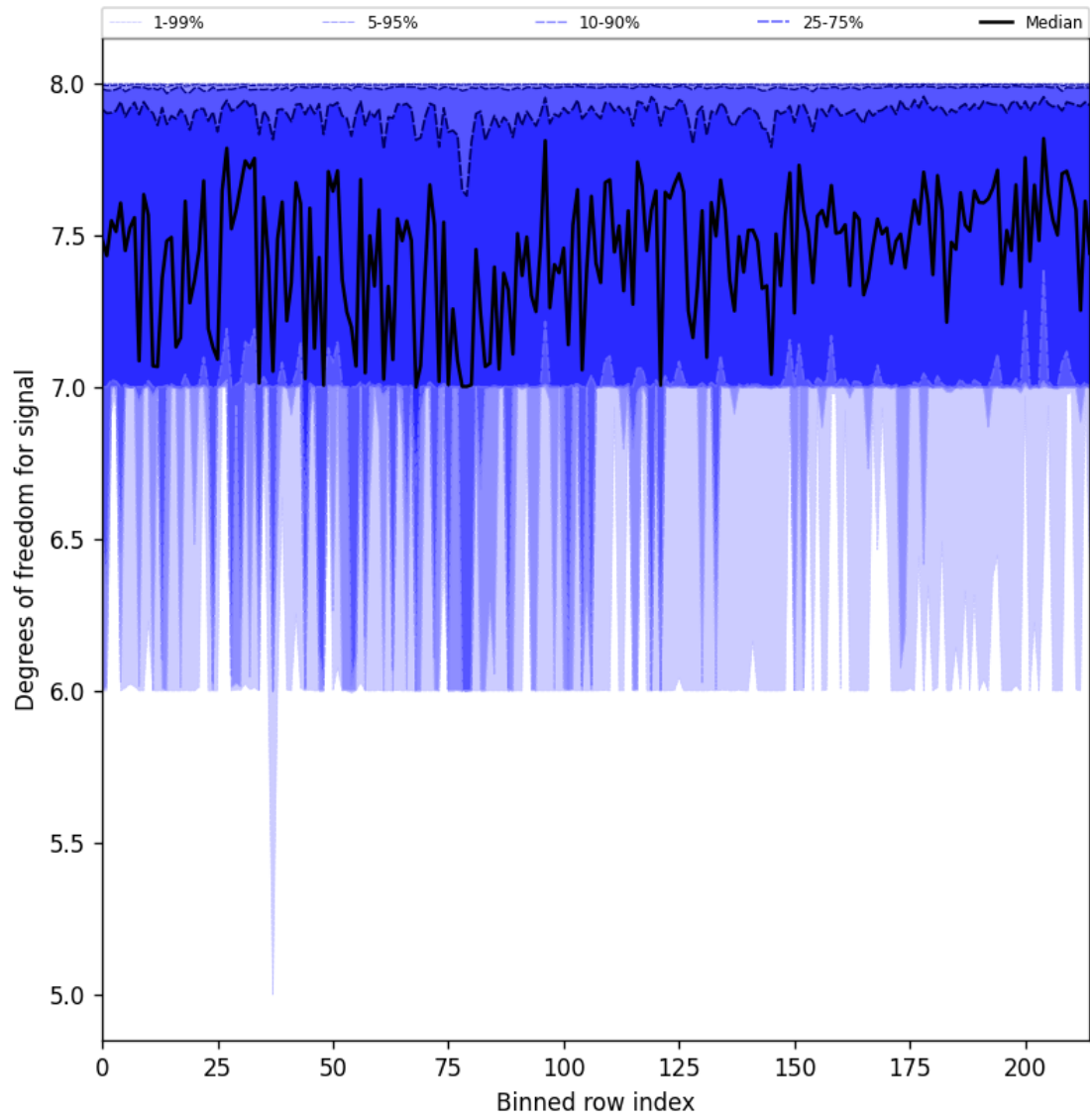
Figure 31: Along track statistics of “Degrees of freedom for signal” for 2025-02-08 to 2025-02-09
