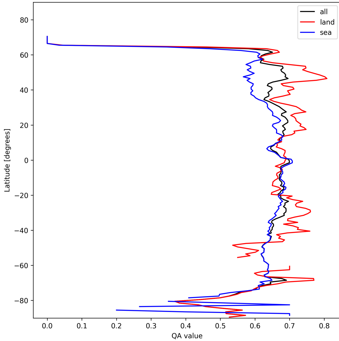
Figure 9: Zonal average of “QA value” for 2025-02-08 to 2025-02-09.
