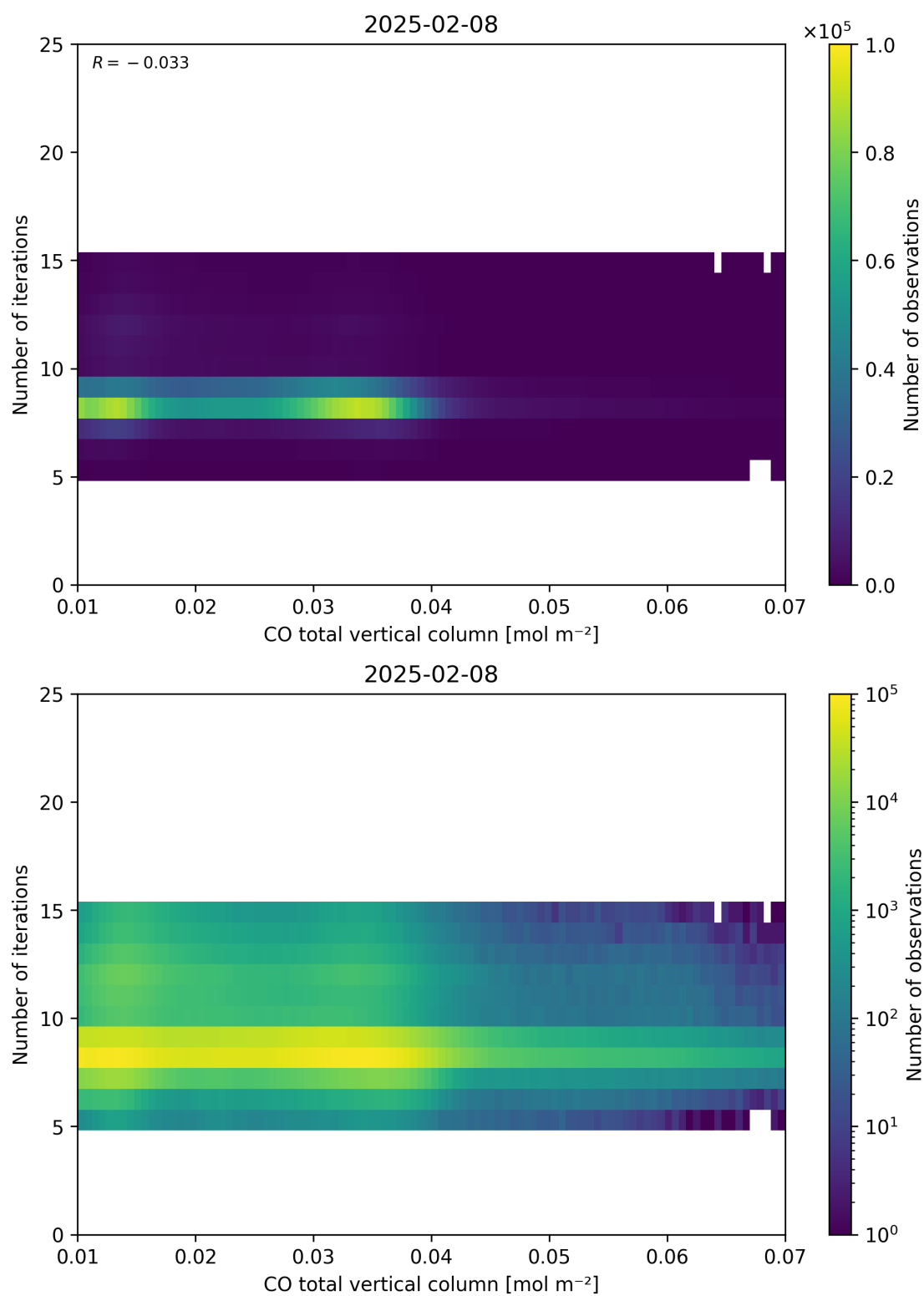
Figure 42: Scatter density plot of “CO total vertical column” against “Number of iterations” for 2025-02-08 to 2025-02-09.
