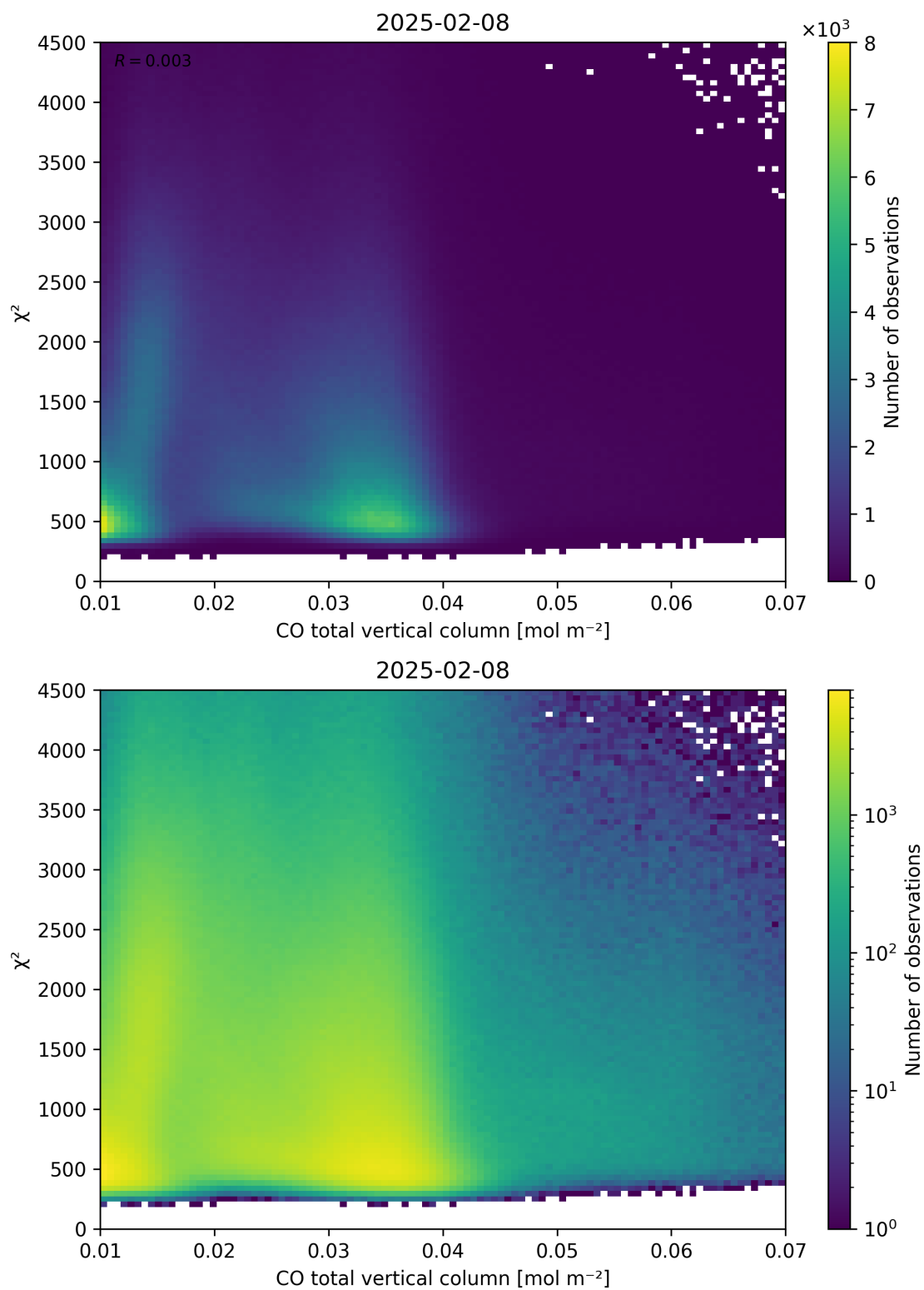
Figure 35: Scatter density plot of “CO total vertical column” against “ \chi^2 ” for 2025-02-08 to 2025-02-09.
