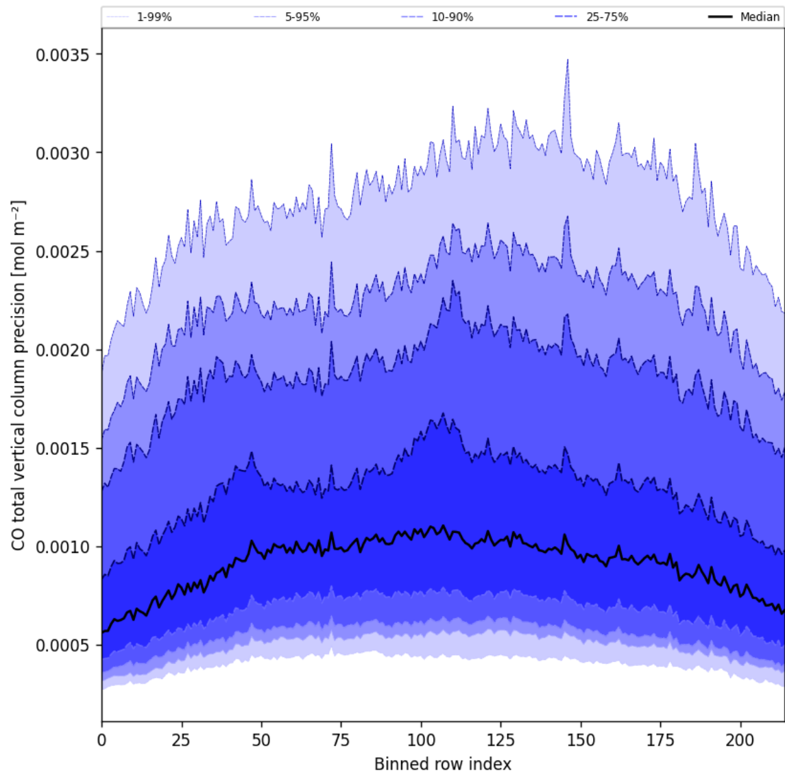
Figure 28: Along track statistics of “CO total vertical column precision” for 2025-02-08 to 2025-02-09
