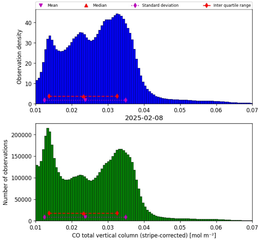
Figure 19: Histogram of “CO total vertical column (stripe-corrected)” for 2025-02-08 to 2025-02-09
