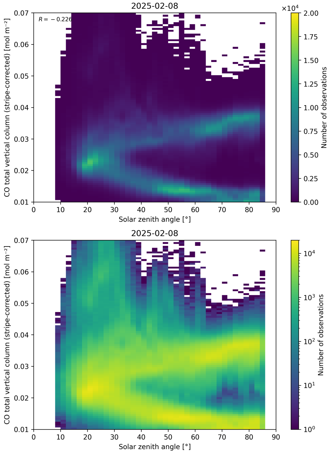
Figure 62: Scatter density plot of “Solar zenith angle” against “CO total vertical column (stripe-corrected)” for 2025-02-08 to 2025-02-09.
