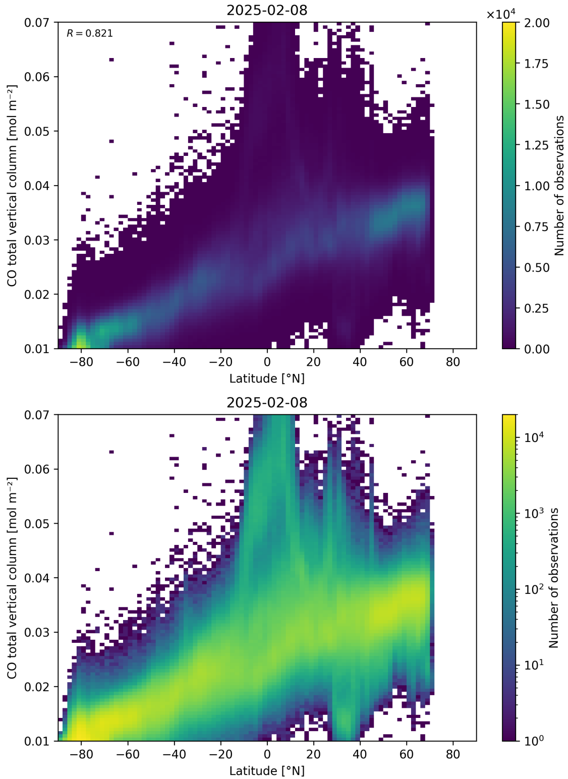
Figure 51: Scatter density plot of “Latitude” against “CO total vertical column” for 2025-02-08 to 2025-02-09.
