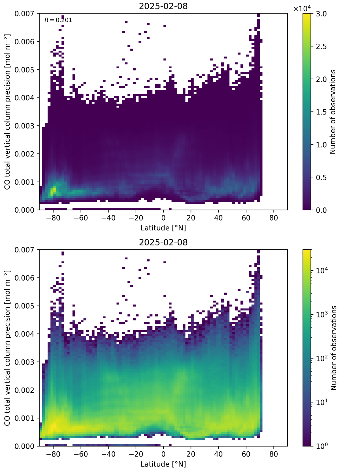
Figure 53: Scatter density plot of “Latitude” against “CO total vertical column precision” for 2025-02-08 to 2025-02-09.
