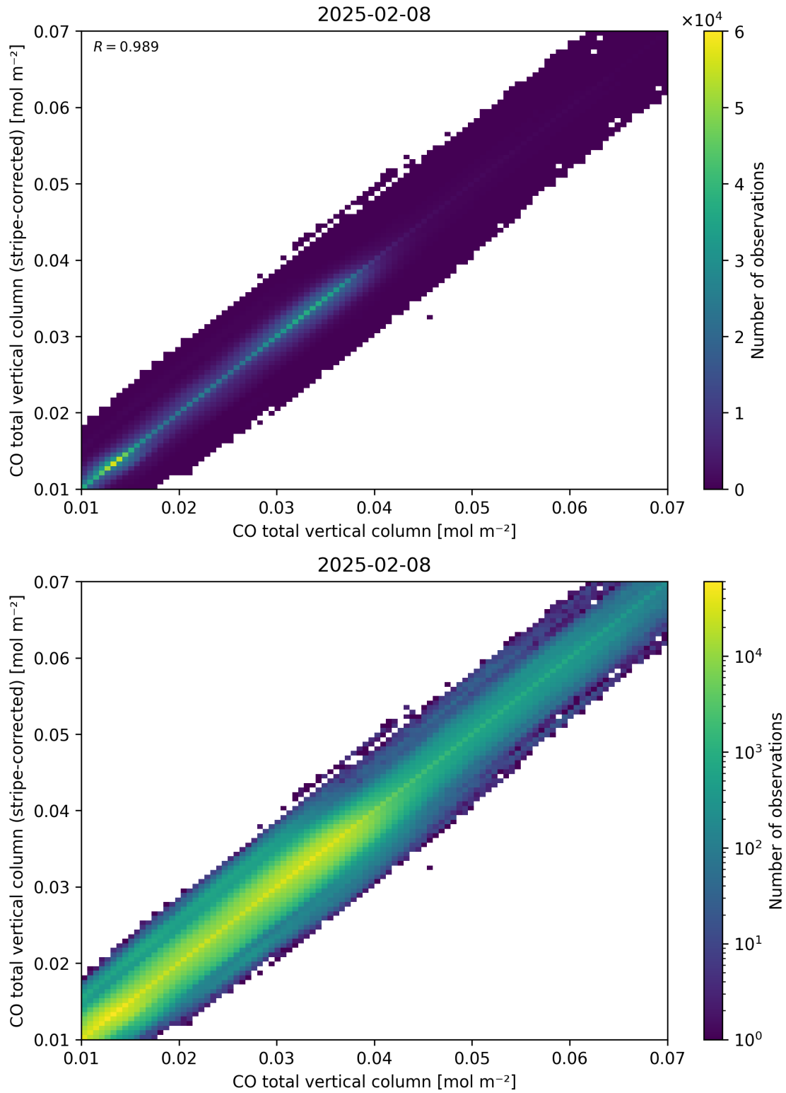
Figure 33: Scatter density plot of “CO total vertical column” against “CO total vertical column (stripe-corrected)” for 2025-02-08 to 2025-02-09.
