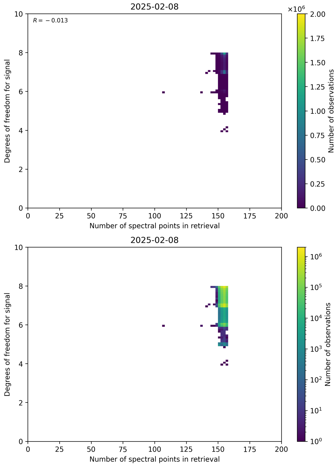
Figure 59: Scatter density plot of “Number of spectral points in retrieval” against “Degrees of freedom for signal” for 2025-02-08 to 2025-02-09.
