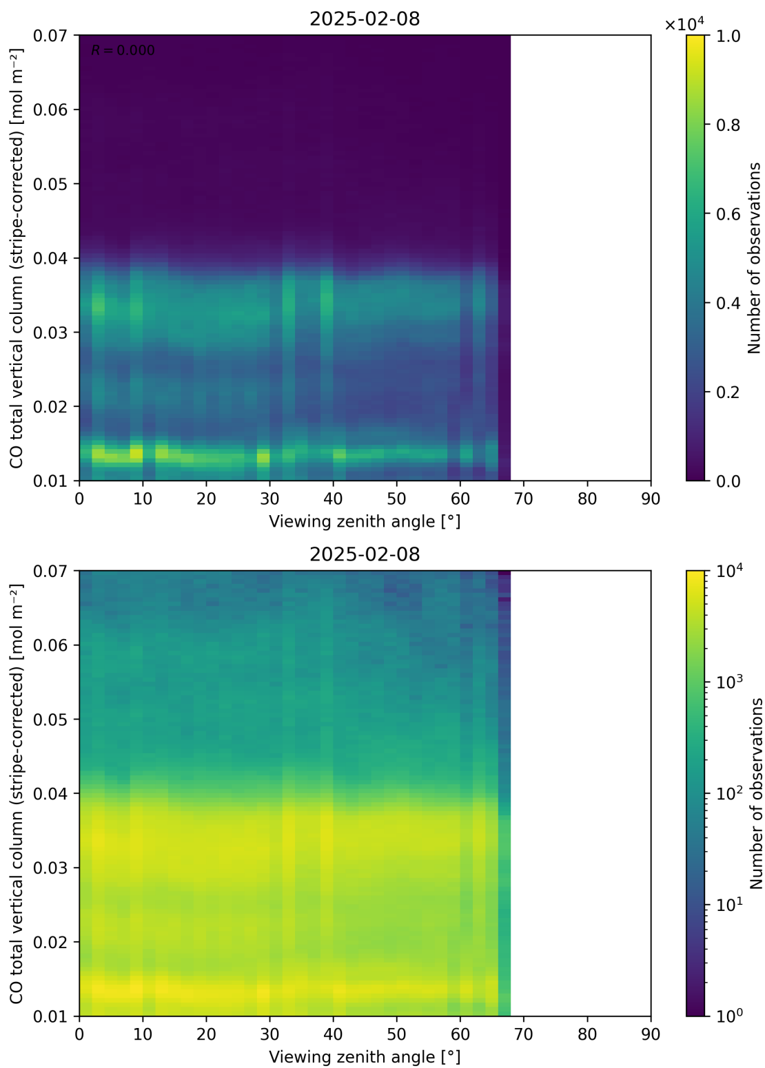
Figure 70: Scatter density plot of “Viewing zenith angle” against “CO total vertical column (stripe-corrected)” for 2025-02-08 to 2025-02-09.
