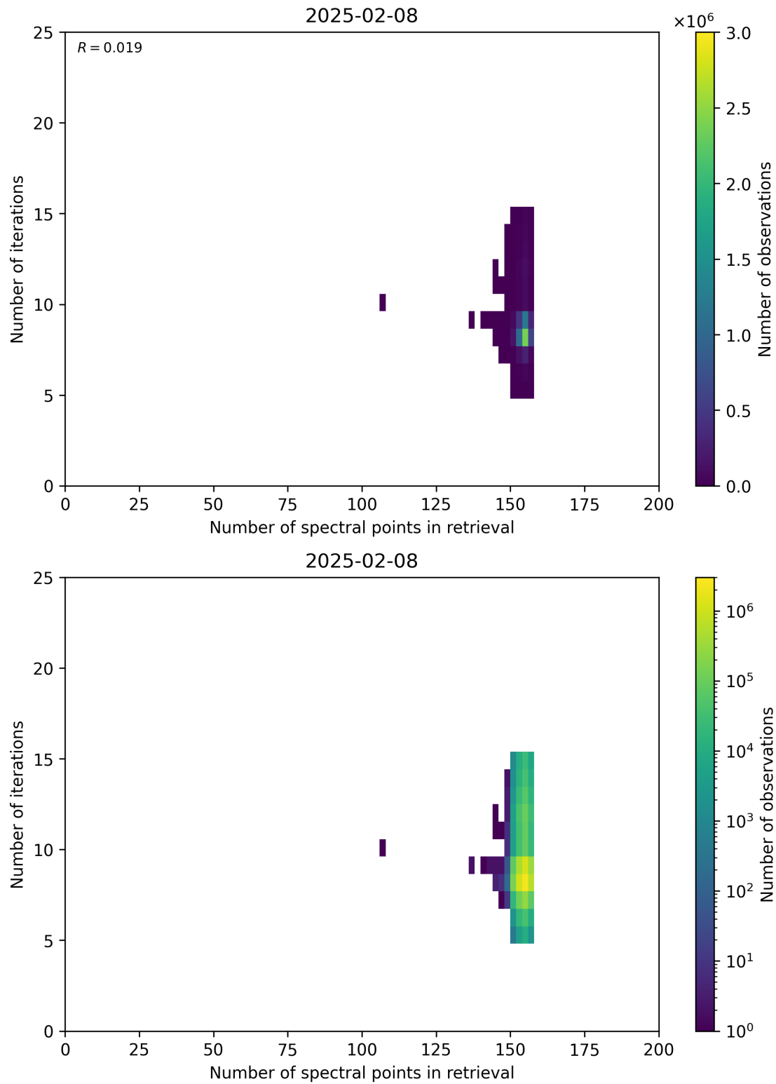
Figure 60: Scatter density plot of “Number of spectral points in retrieval” against “Number of iterations” for 2025-02-08 to 2025-02-09.
