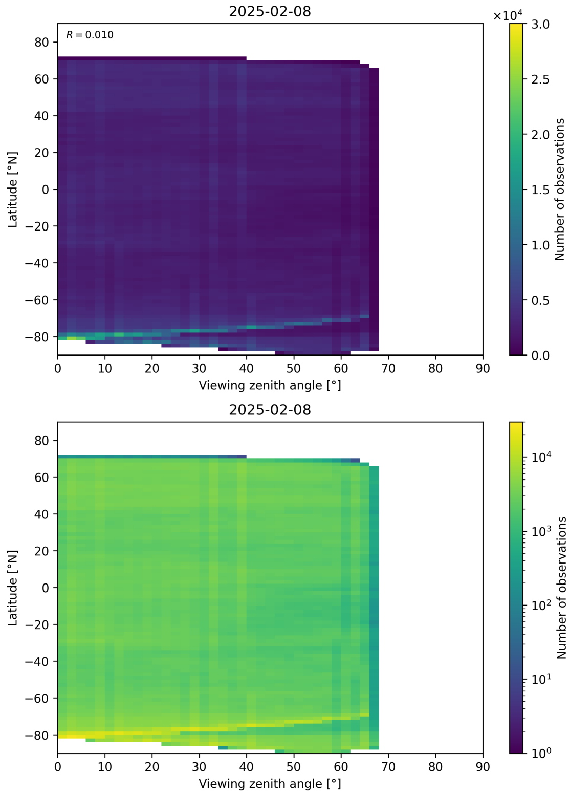
Figure 74: Scatter density plot of “Viewing zenith angle” against “Latitude” for 2025-02-08 to 2025-02-09.
