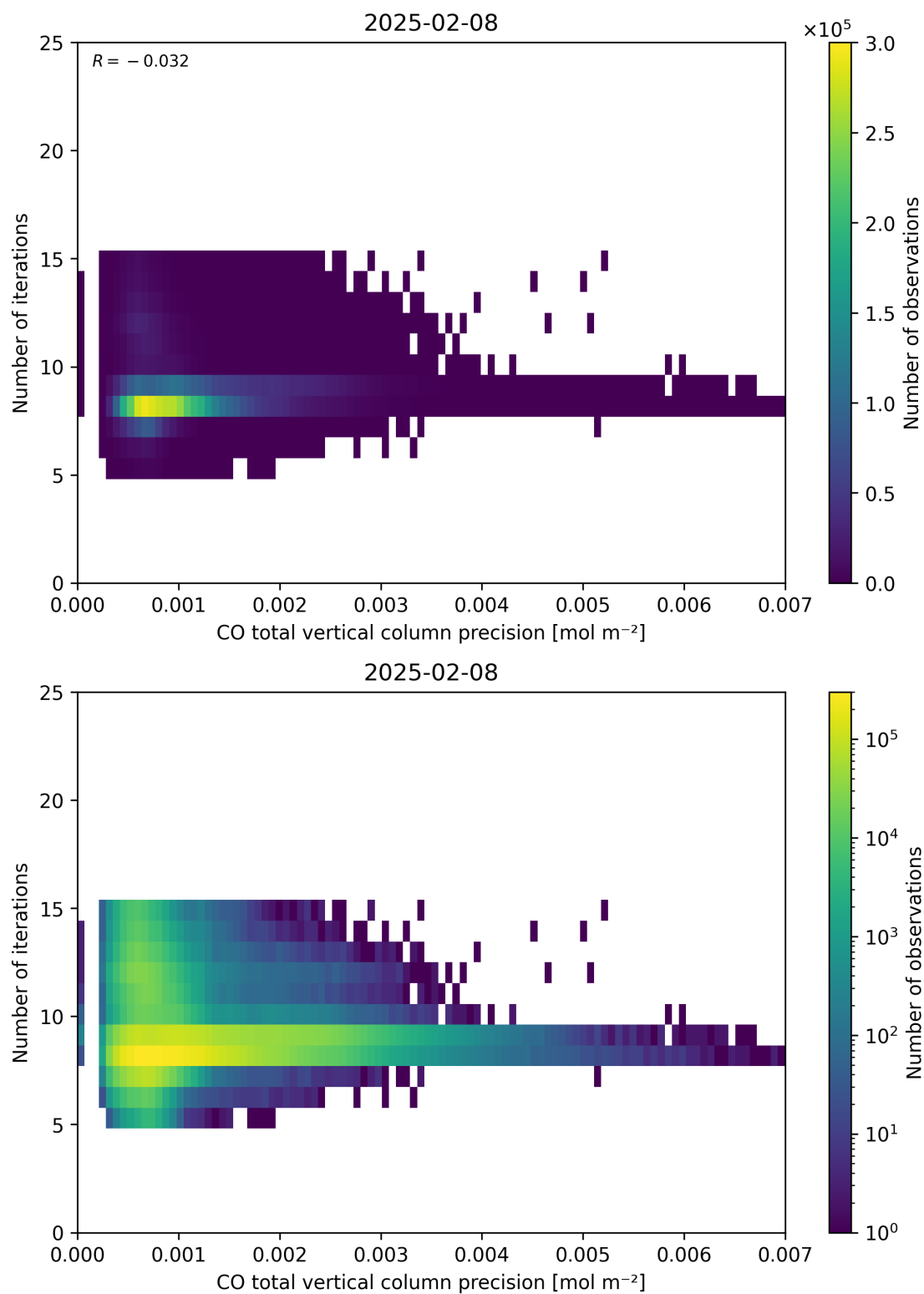
Figure 46: Scatter density plot of “CO total vertical column precision” against “Number of iterations” for 2025-02-08 to 2025-02-09.
