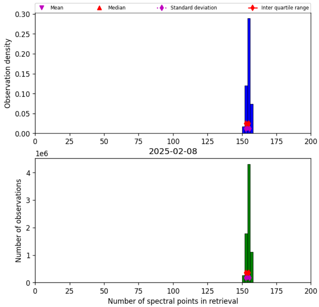
Figure 21: Histogram of “Number of spectral points in retrieval” for 2025-02-08 to 2025-02-09
