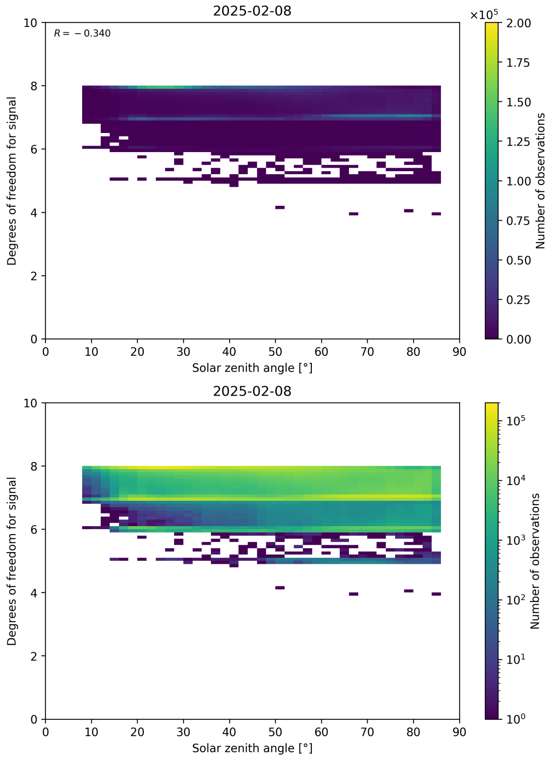
Figure 65: Scatter density plot of “Solar zenith angle” against “Degrees of freedom for signal” for 2025-02-08 to 2025-02-09.
