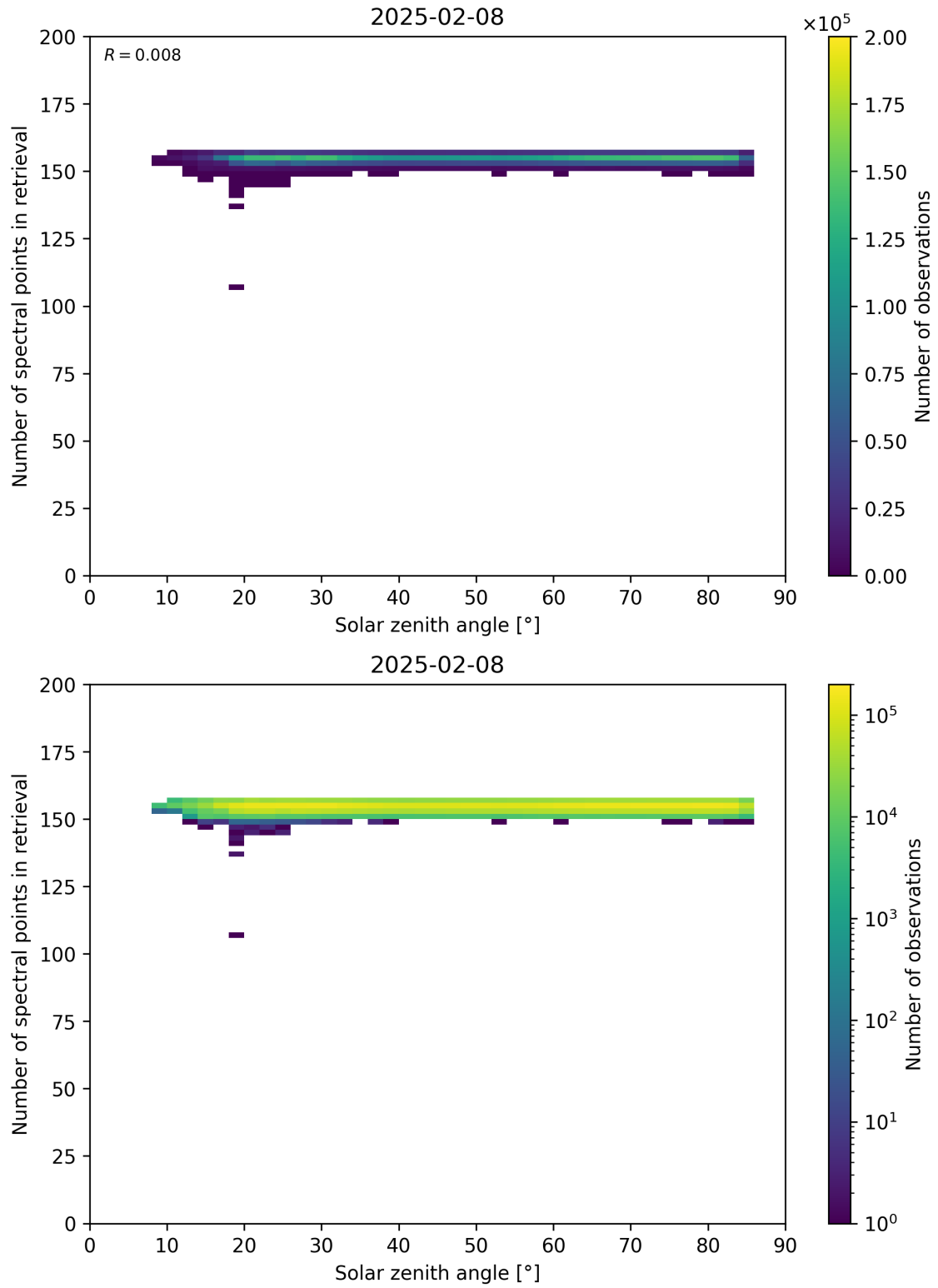
Figure 68: Scatter density plot of “Solar zenith angle” against “Number of spectral points in retrieval” for 2025-02-08 to 2025-02-09.
