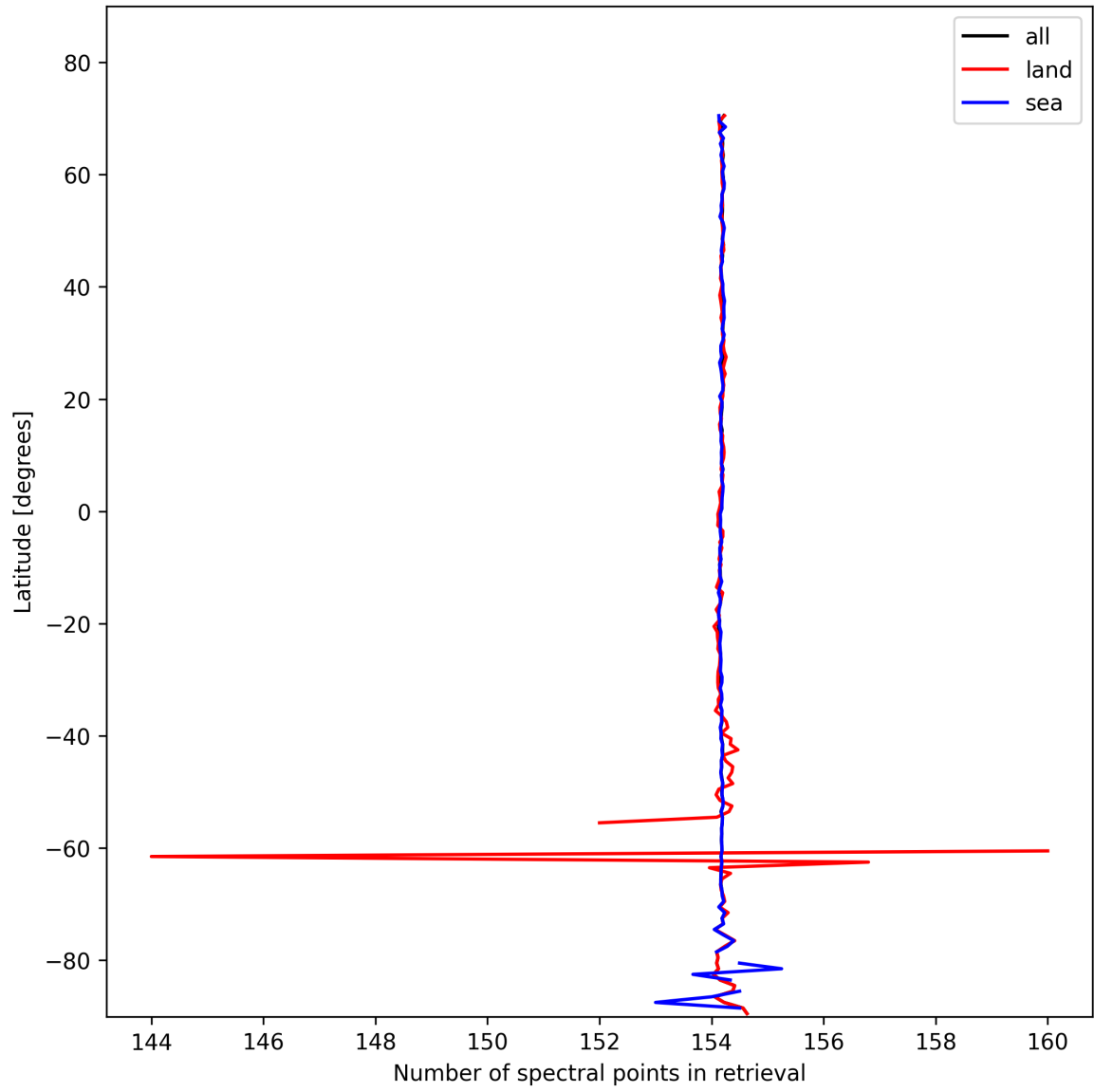
Figure 13: Zonal average of “Number of spectral points in retrieval” for 2025-02-08 to 2025-02-09.
