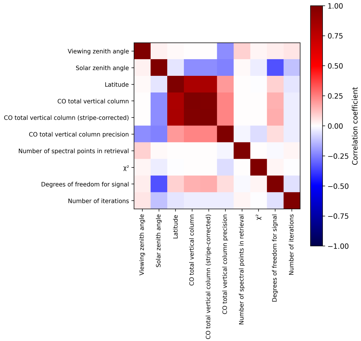
Figure 2: Map of correlation matrix for 2025-02-08 to 2025-02-09.
