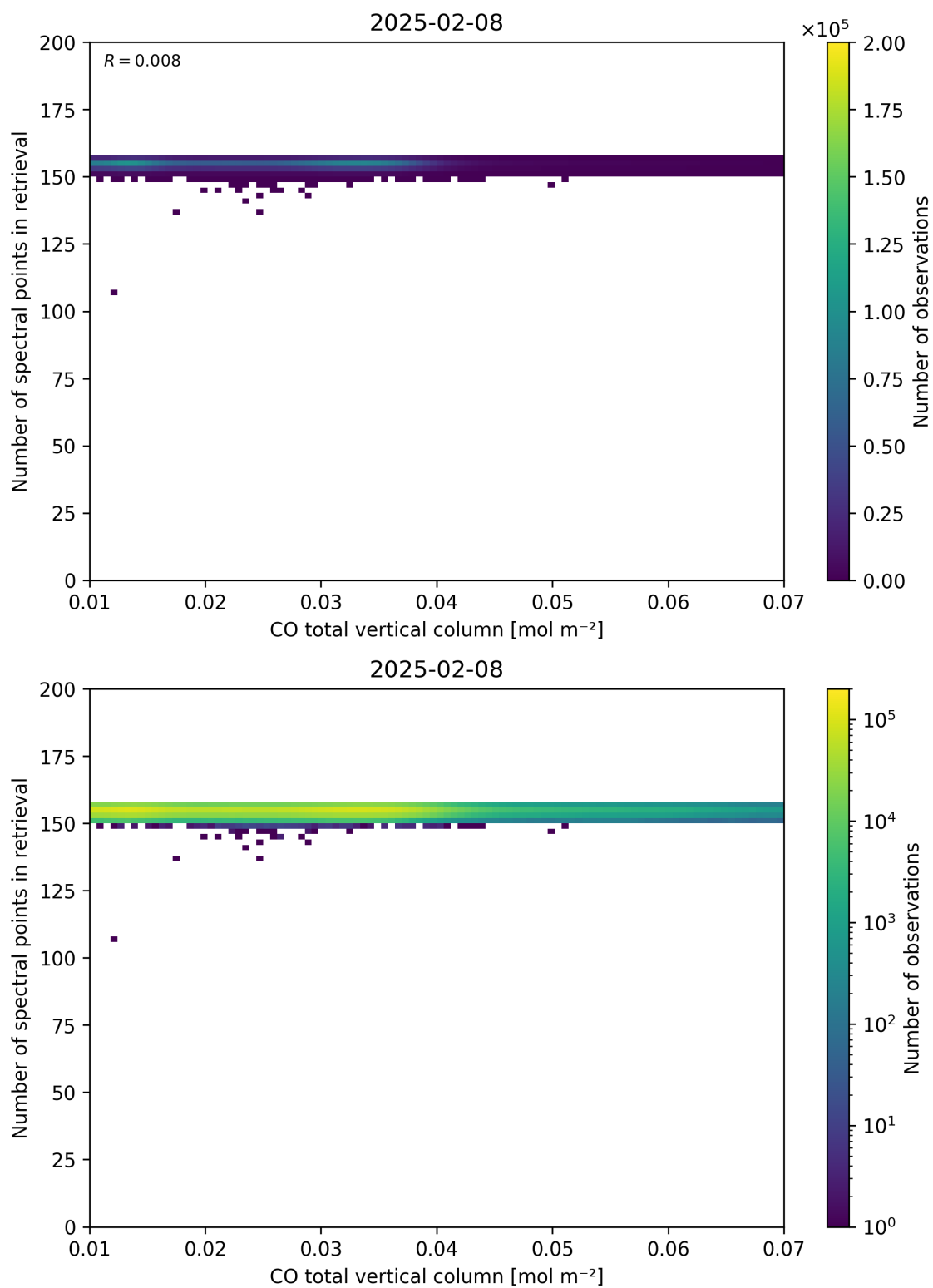
Figure 43: Scatter density plot of “CO total vertical column” against “Number of spectral points in retrieval” for 2025-02-08 to 2025-02-09.
