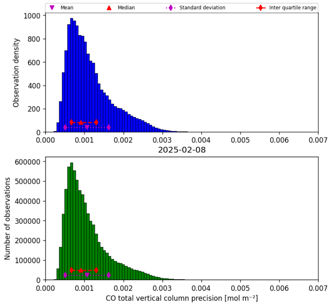
Figure 20: Histogram of “CO total vertical column precision” for 2025-02-08 to 2025-02-09
