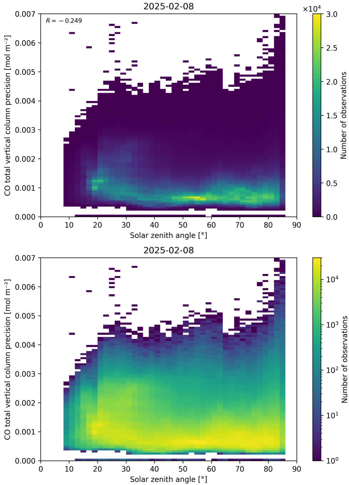
Figure 63: Scatter density plot of “Solar zenith angle” against “CO total vertical column precision” for 2025-02-08 to 2025-02-09.
