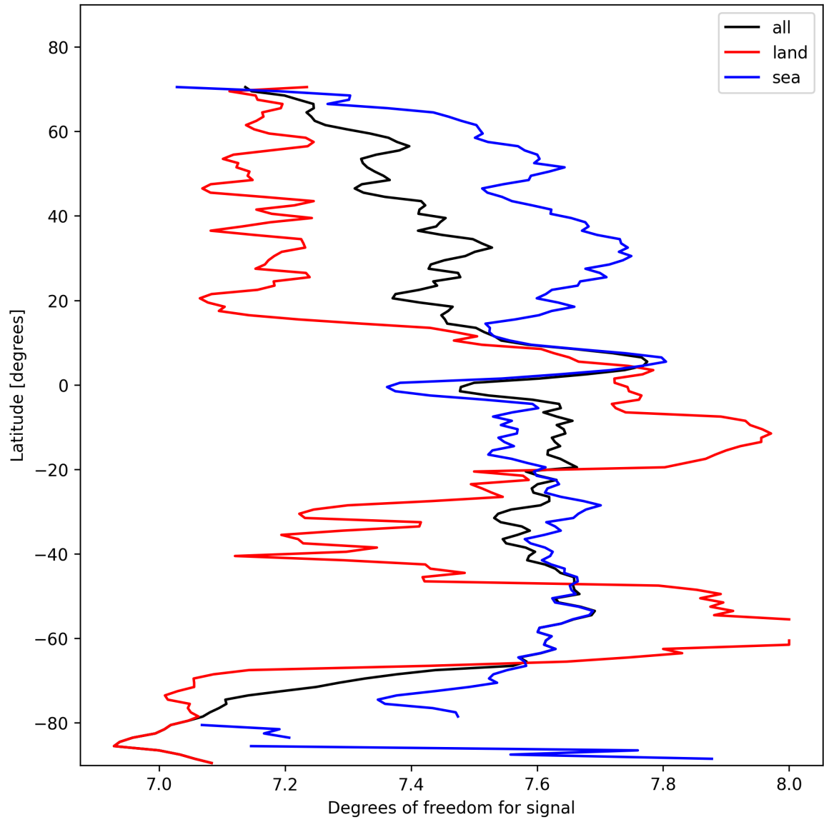
Figure 15: Zonal average of “Degrees of freedom for signal” for 2025-02-08 to 2025-02-09.
