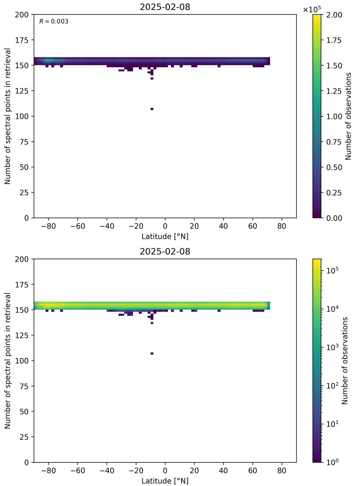
Figure 57: Scatter density plot of “Latitude” against “Number of spectral points in retrieval” for 2025-02-08 to 2025-02-09.
