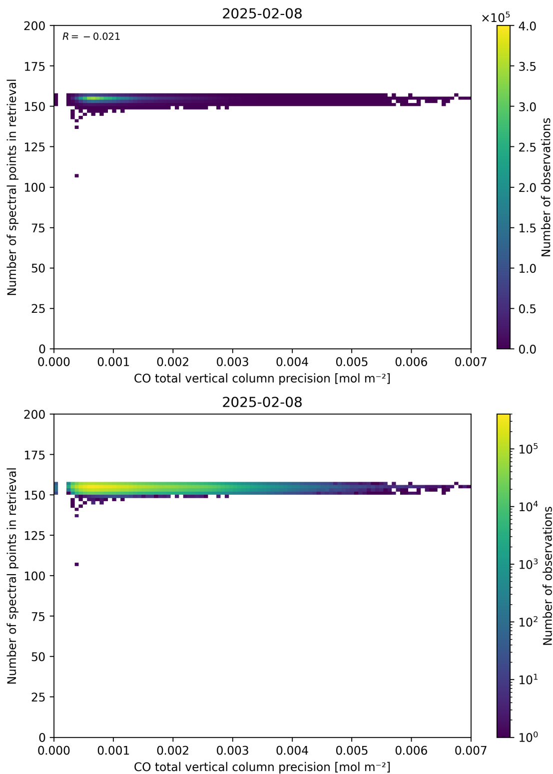
Figure 47: Scatter density plot of “CO total vertical column precision” against “Number of spectral points in retrieval” for 2025-02-08 to 2025-02-09.
