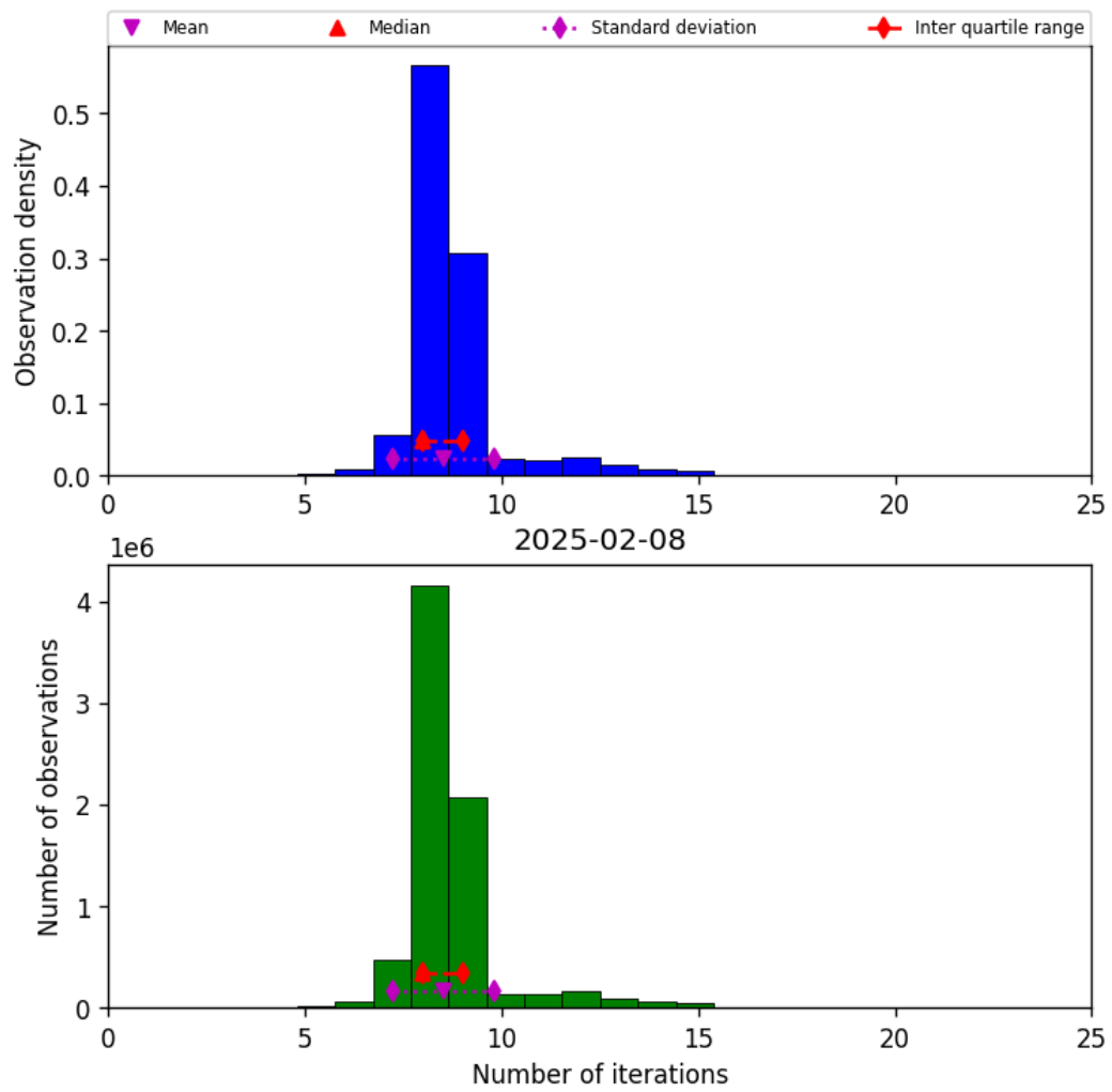
Figure 24: Histogram of “Number of iterations” for 2025-02-08 to 2025-02-09
