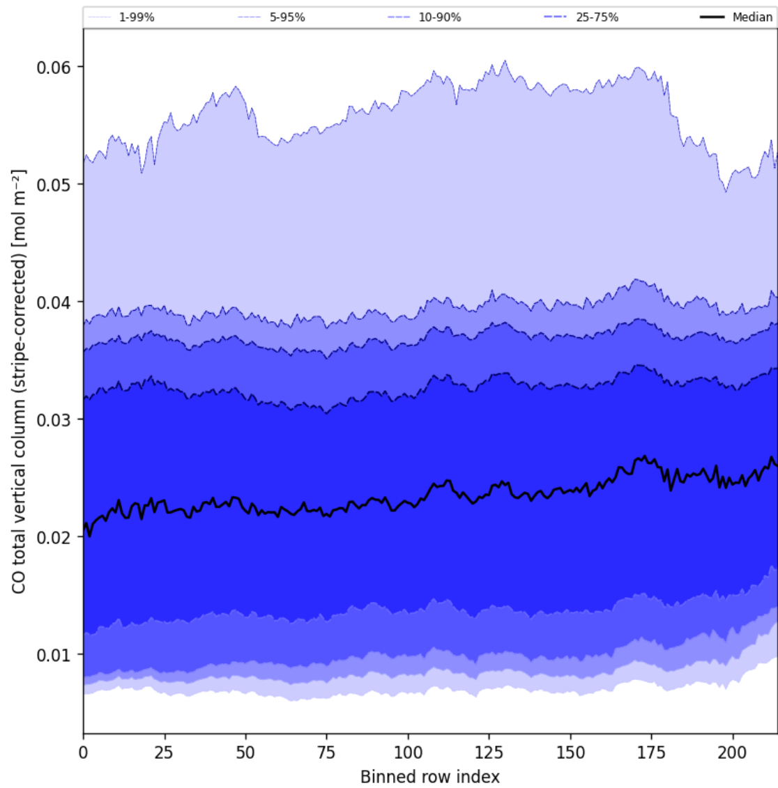
Figure 27: Along track statistics of “CO total vertical column (stripe-corrected)” for 2025-02-08 to 2025-02-09
