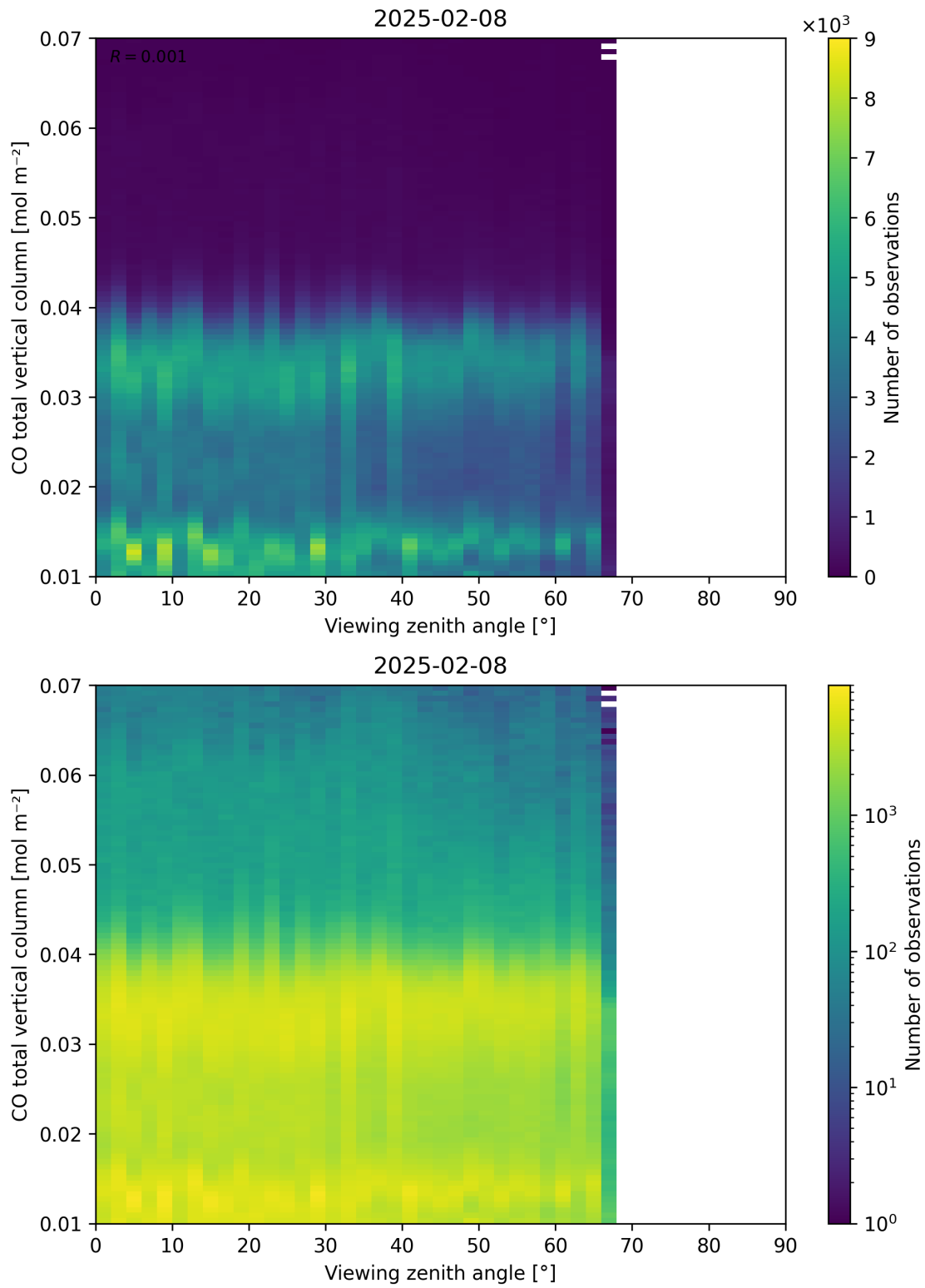
Figure 69: Scatter density plot of “Viewing zenith angle” against “CO total vertical column” for 2025-02-08 to 2025-02-09.
