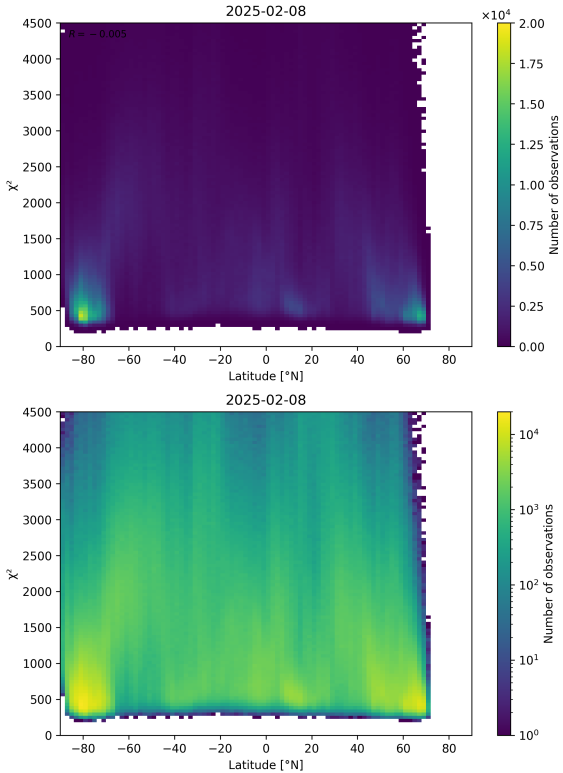
Figure 54: Scatter density plot of “Latitude” against “ \chi^2 ” for 2025-02-08 to 2025-02-09.
