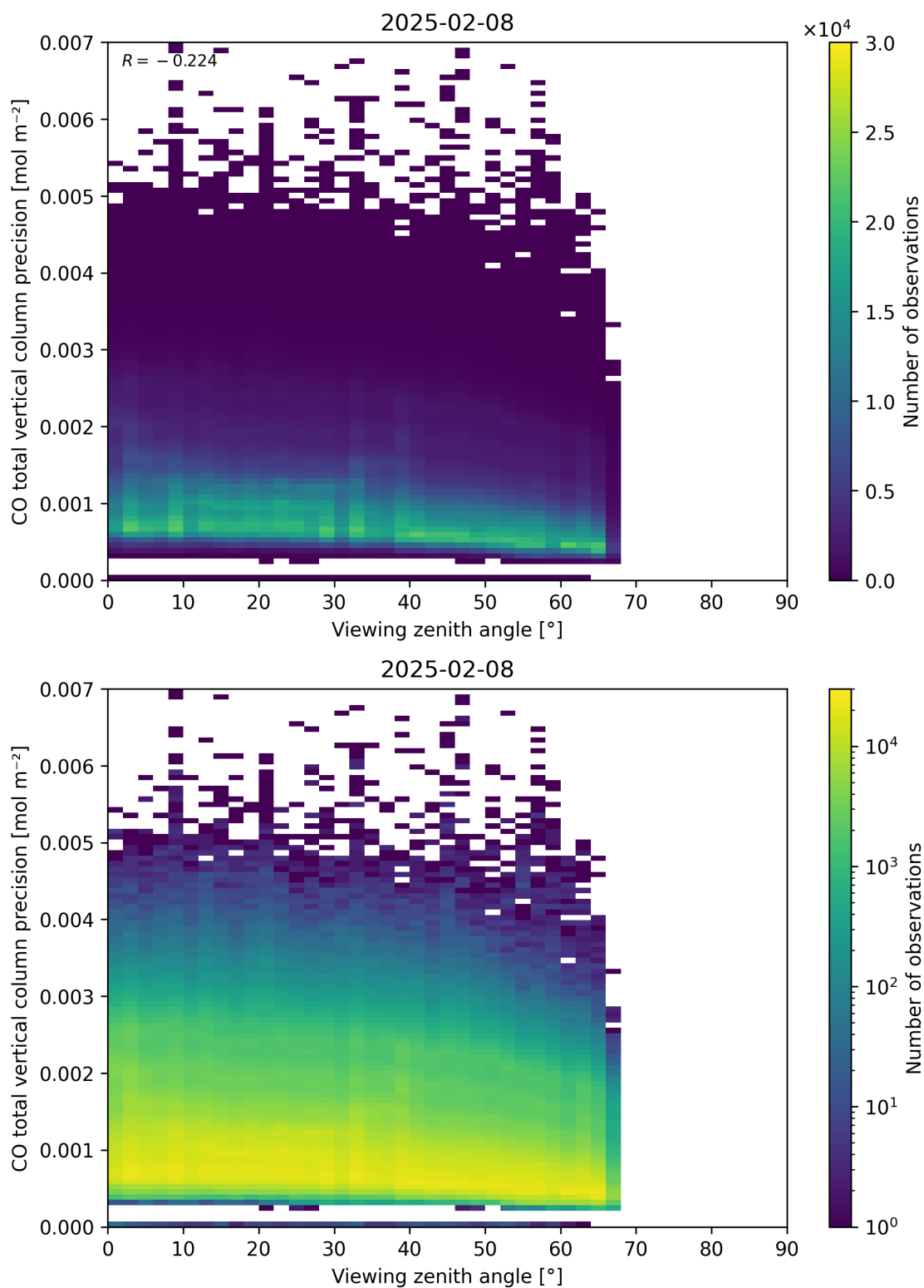
Figure 71: Scatter density plot of “Viewing zenith angle” against “CO total vertical column precision” for 2025-02-08 to 2025-02-09.
