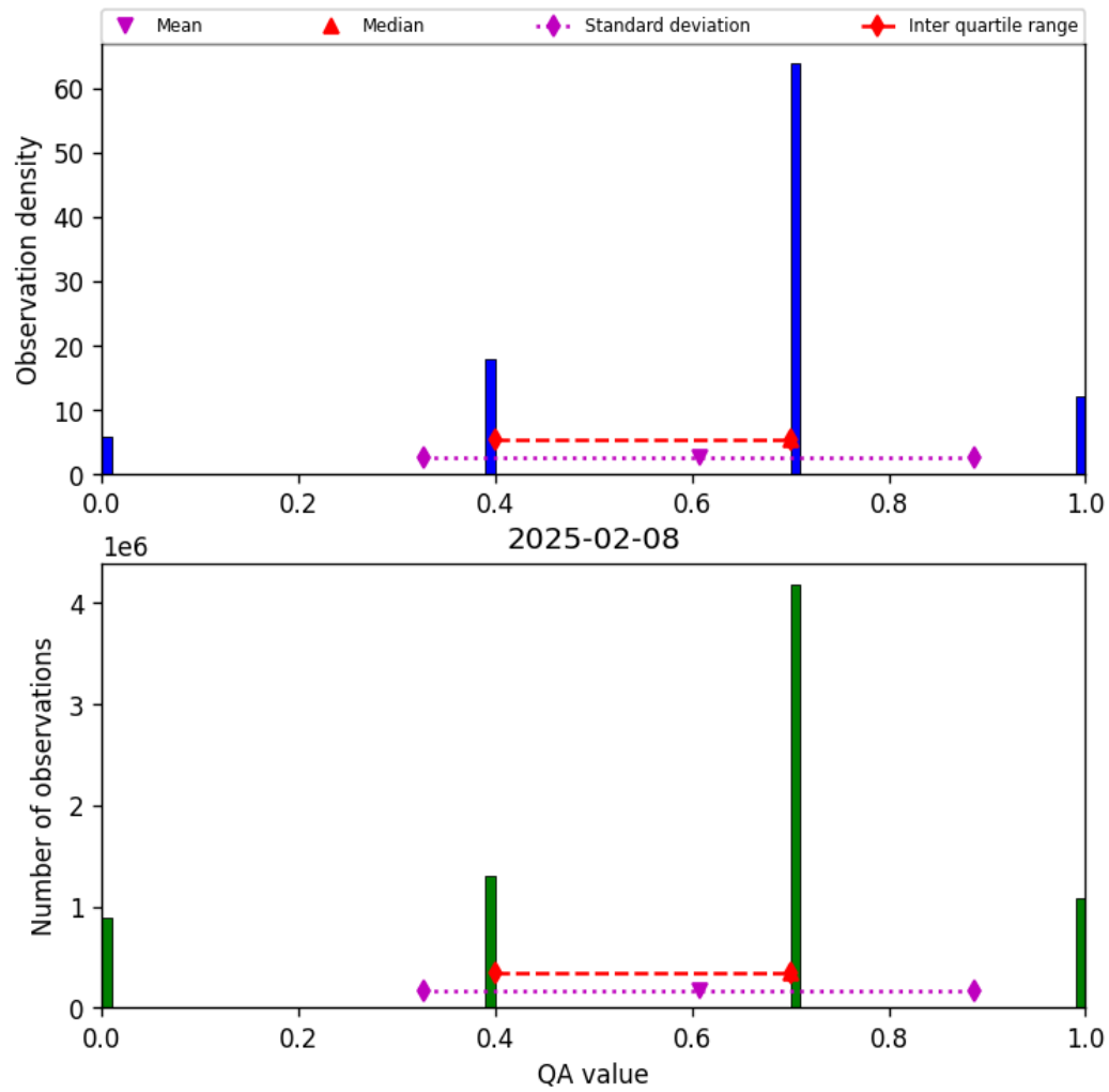
Figure 17: Histogram of “QA value” for 2025-02-08 to 2025-02-09
