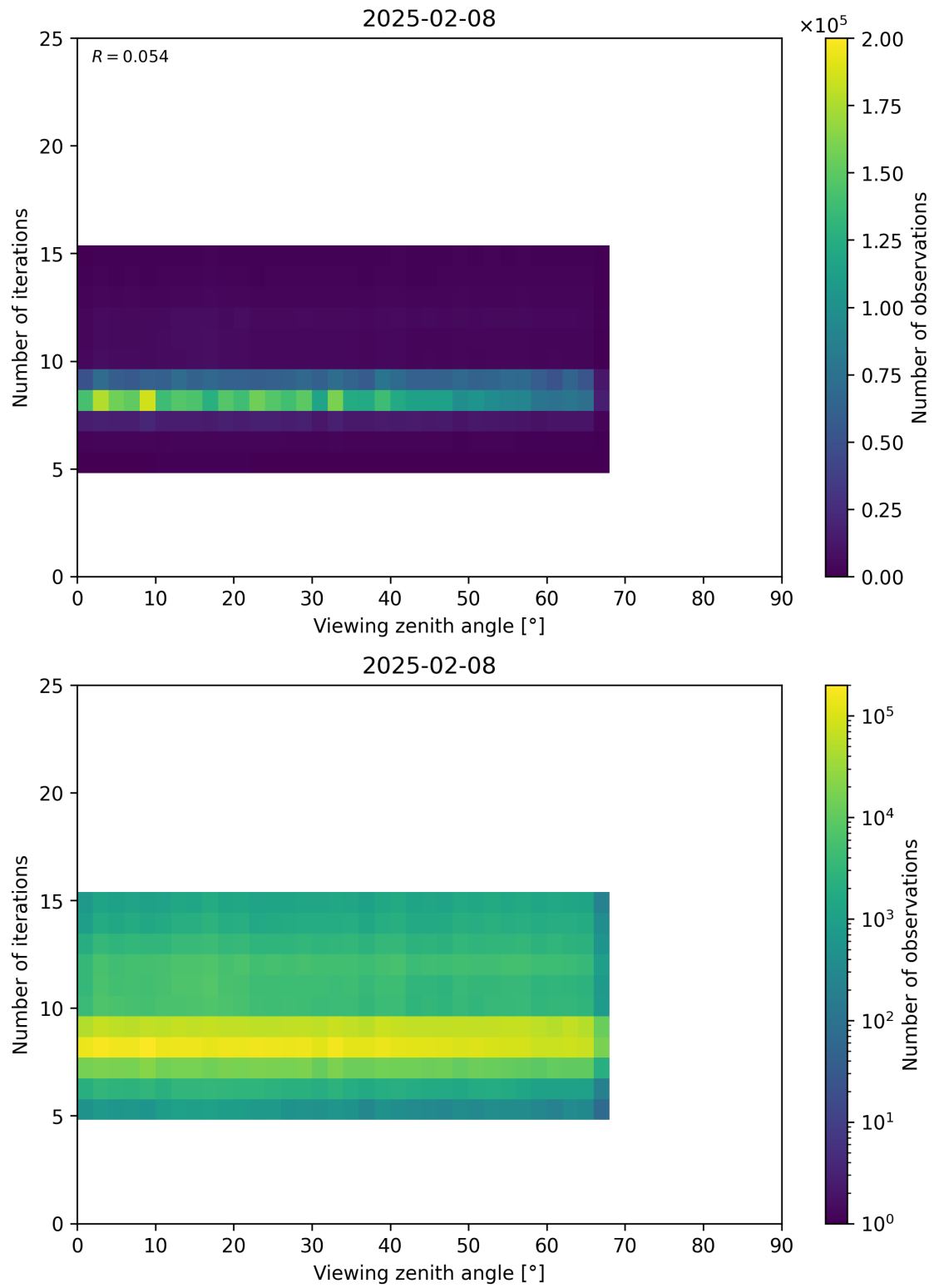
Figure 75: Scatter density plot of “Viewing zenith angle” against “Number of iterations” for 2025-02-08 to 2025-02-09.
