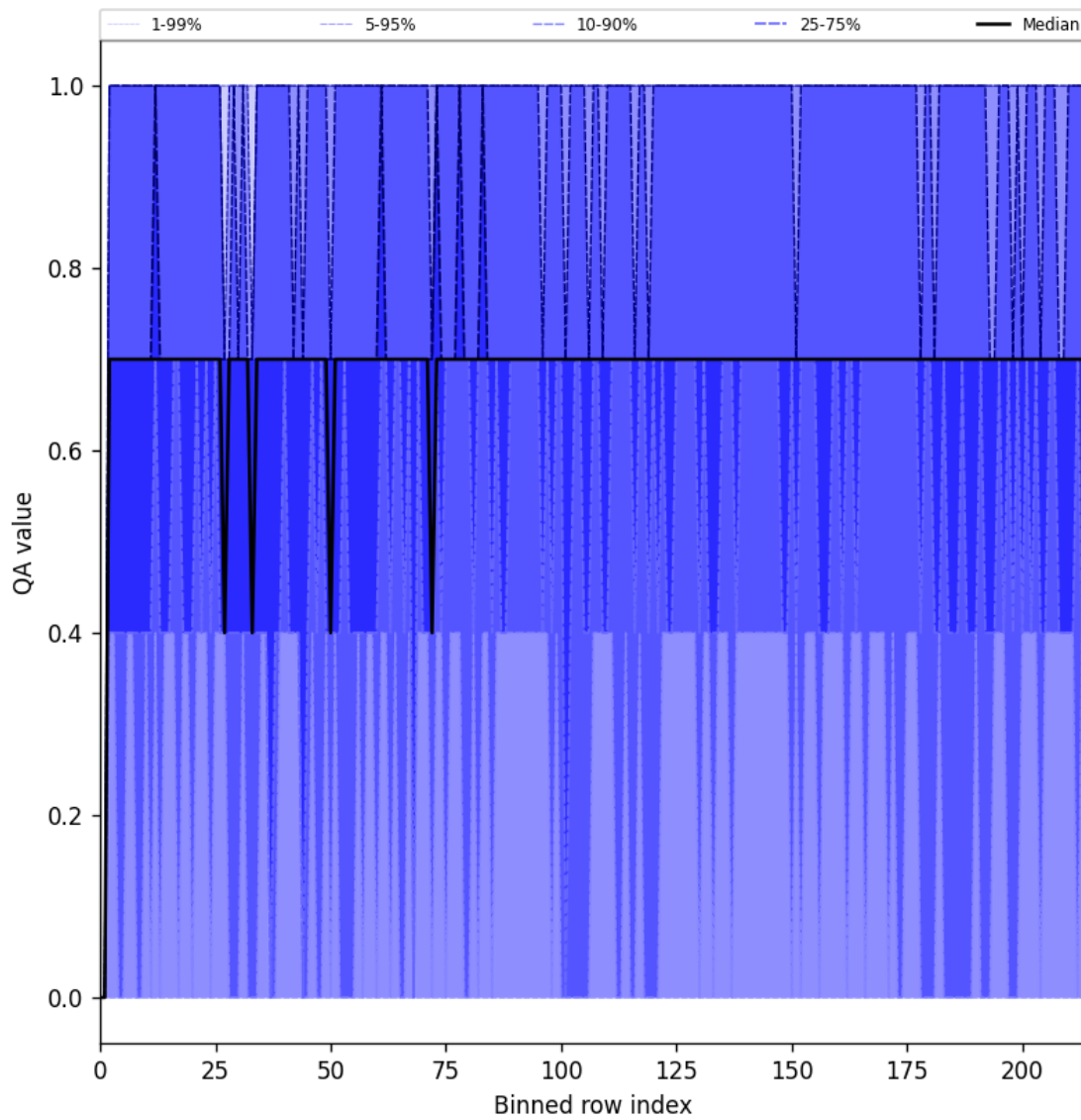
Figure 25: Along track statistics of “QA value” for 2025-02-08 to 2025-02-10
