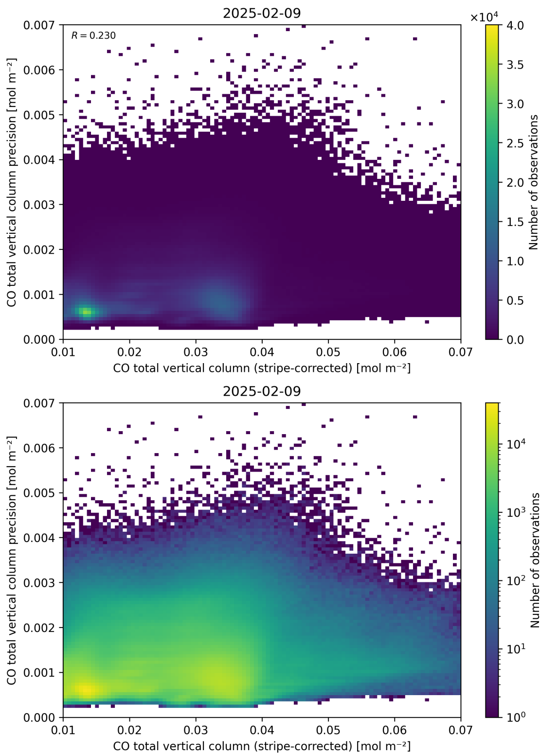
Figure 36: Scatter density plot of “CO total vertical column (stripe-corrected)” against “CO total vertical column precision” for 2025-02-08 to 2025-02-10.
