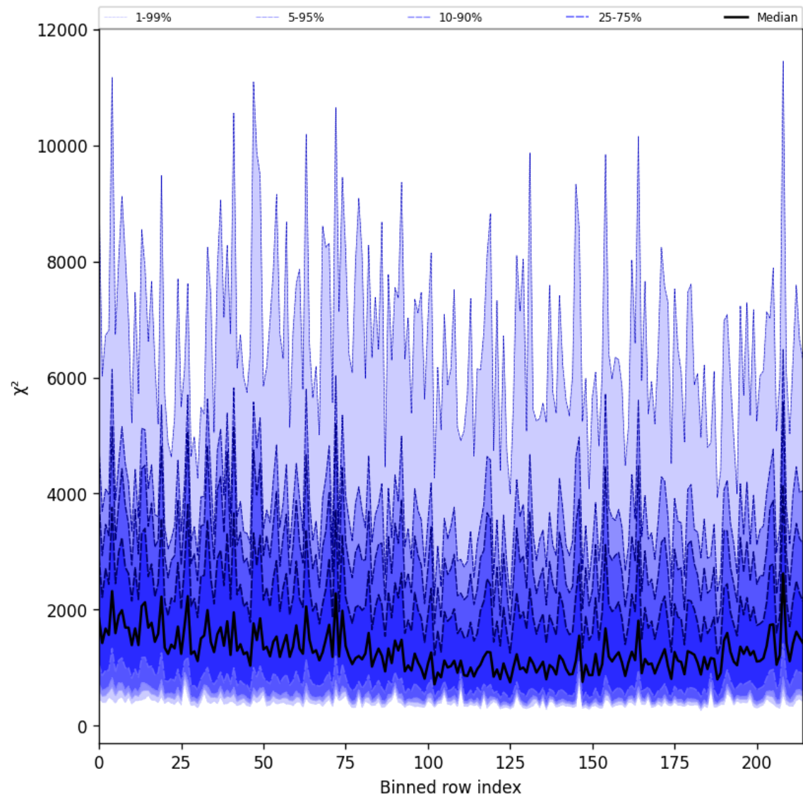
Figure 30: Along track statistics of “ \chi^2 ” for 2025-02-08 to 2025-02-10
