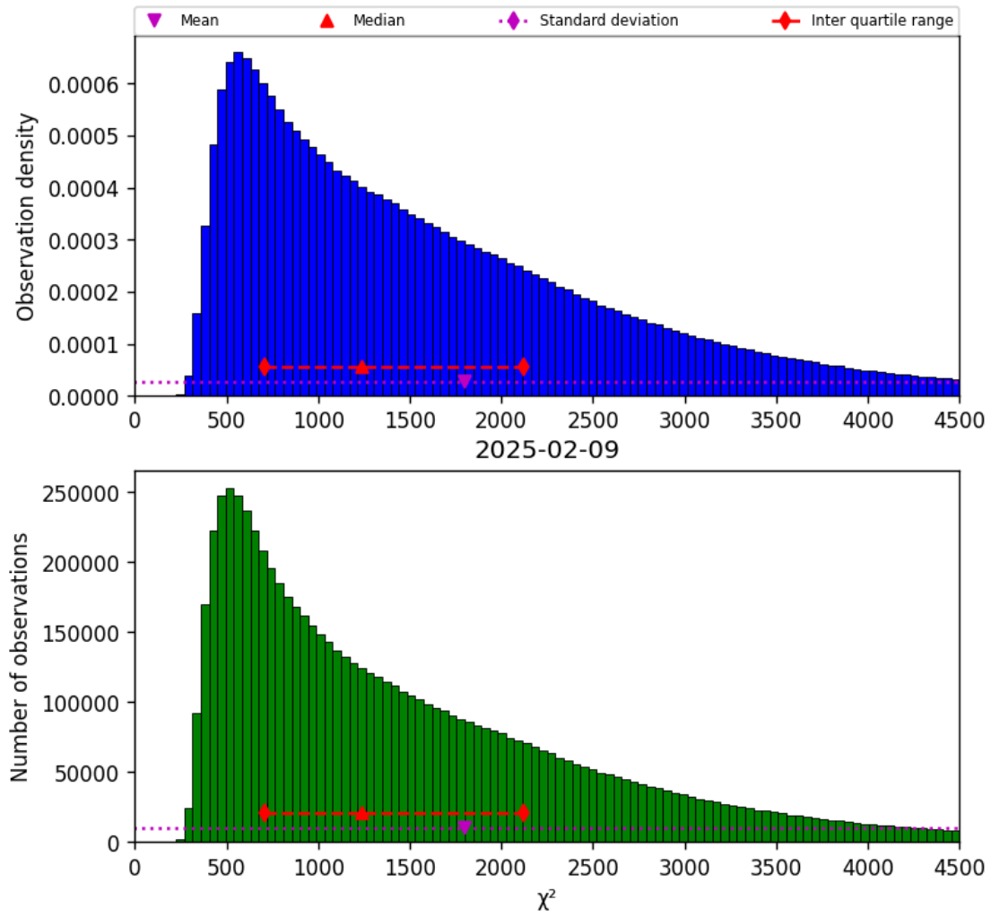
Figure 22: Histogram of “ \chi^2 ” for 2025-02-08 to 2025-02-10
