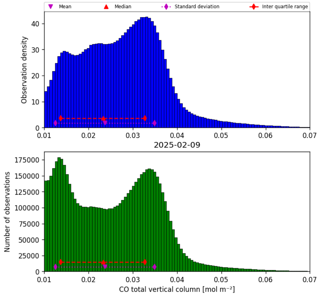
Figure 18: Histogram of “CO total vertical column” for 2025-02-08 to 2025-02-10
