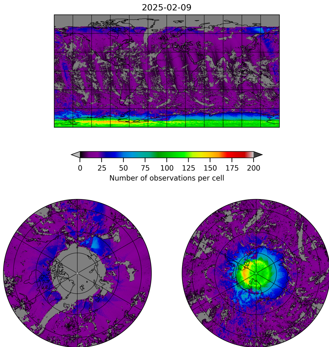
Figure 8: Map of the number of observations for 2025-02-08 to 2025-02-10
