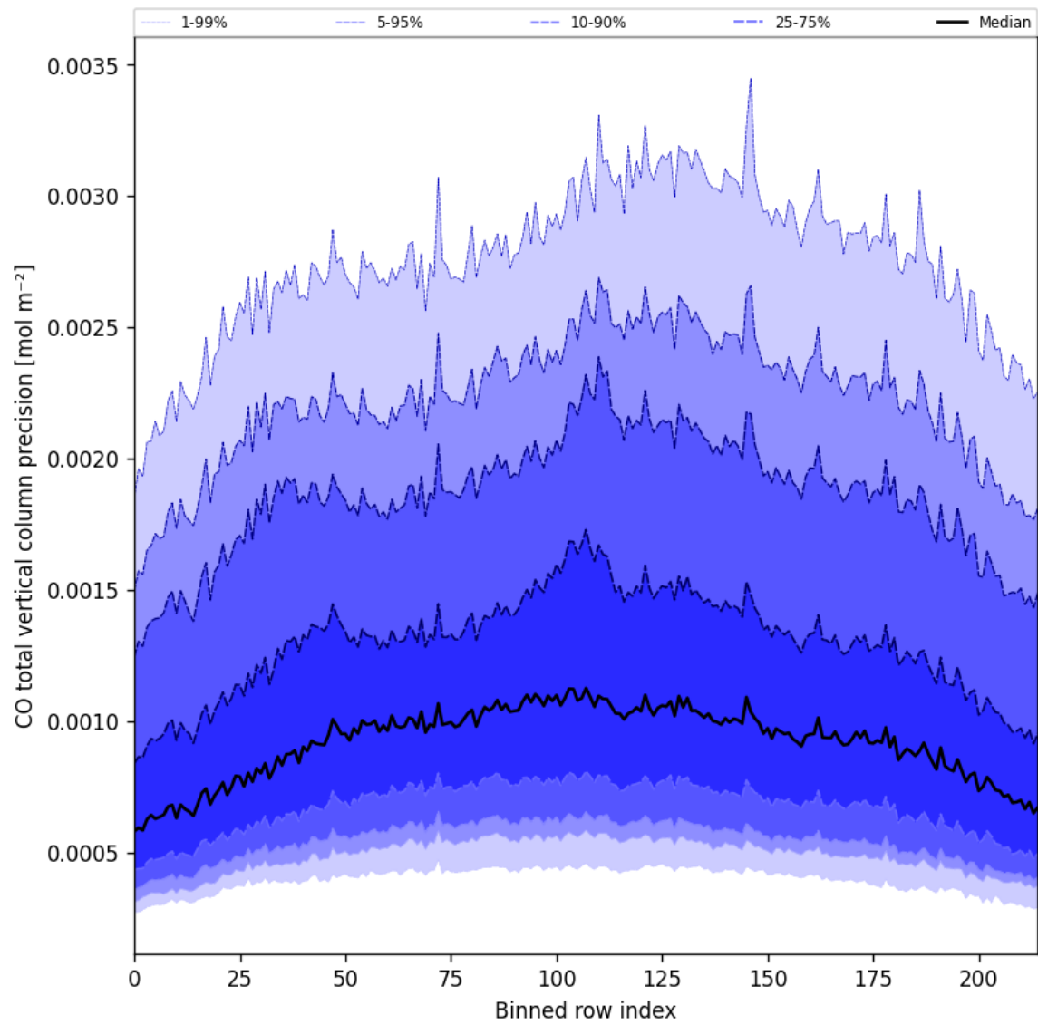
Figure 28: Along track statistics of “CO total vertical column precision” for 2025-02-08 to 2025-02-10
