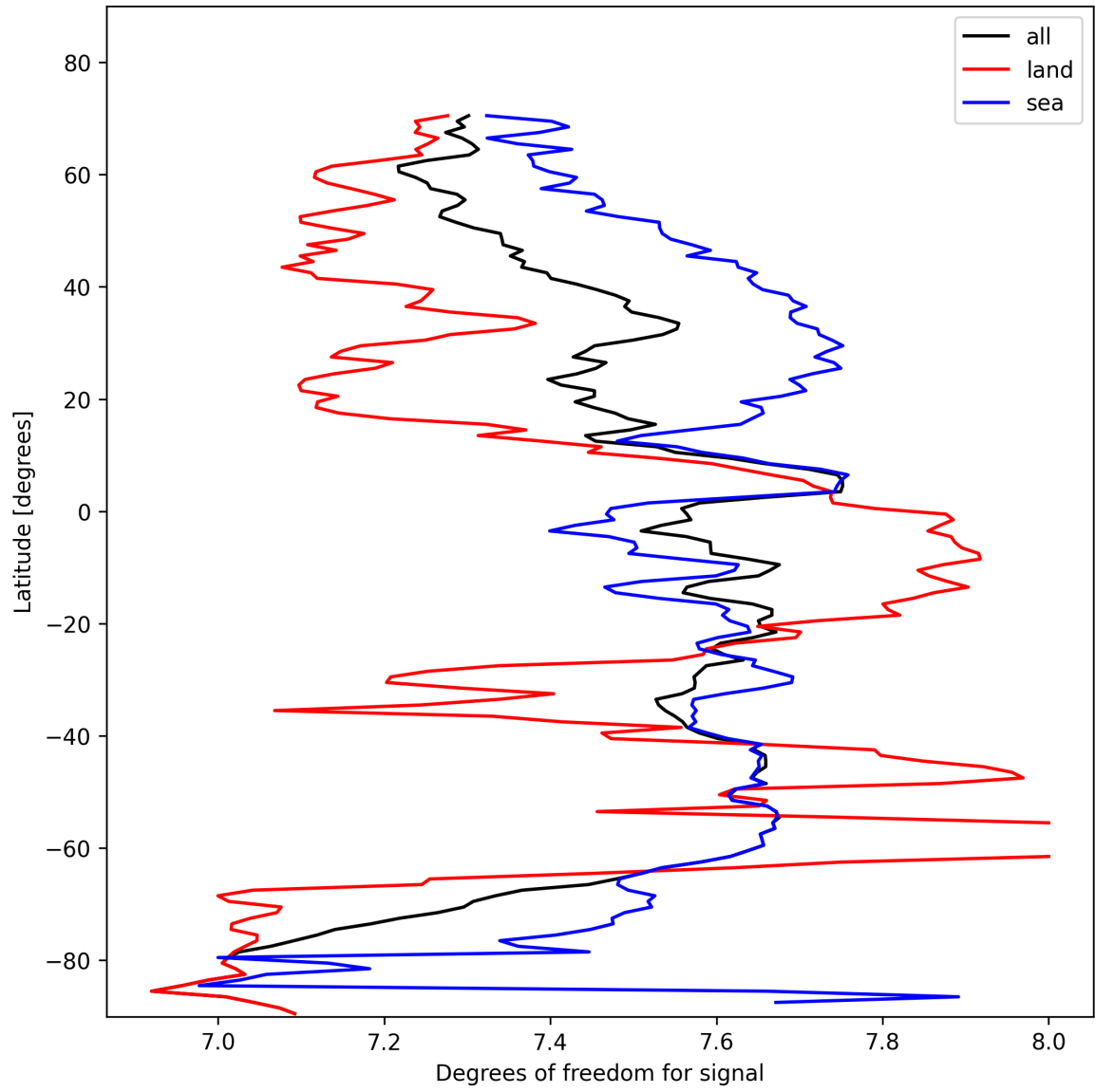
Figure 15: Zonal average of “Degrees of freedom for signal” for 2025-02-08 to 2025-02-10.
