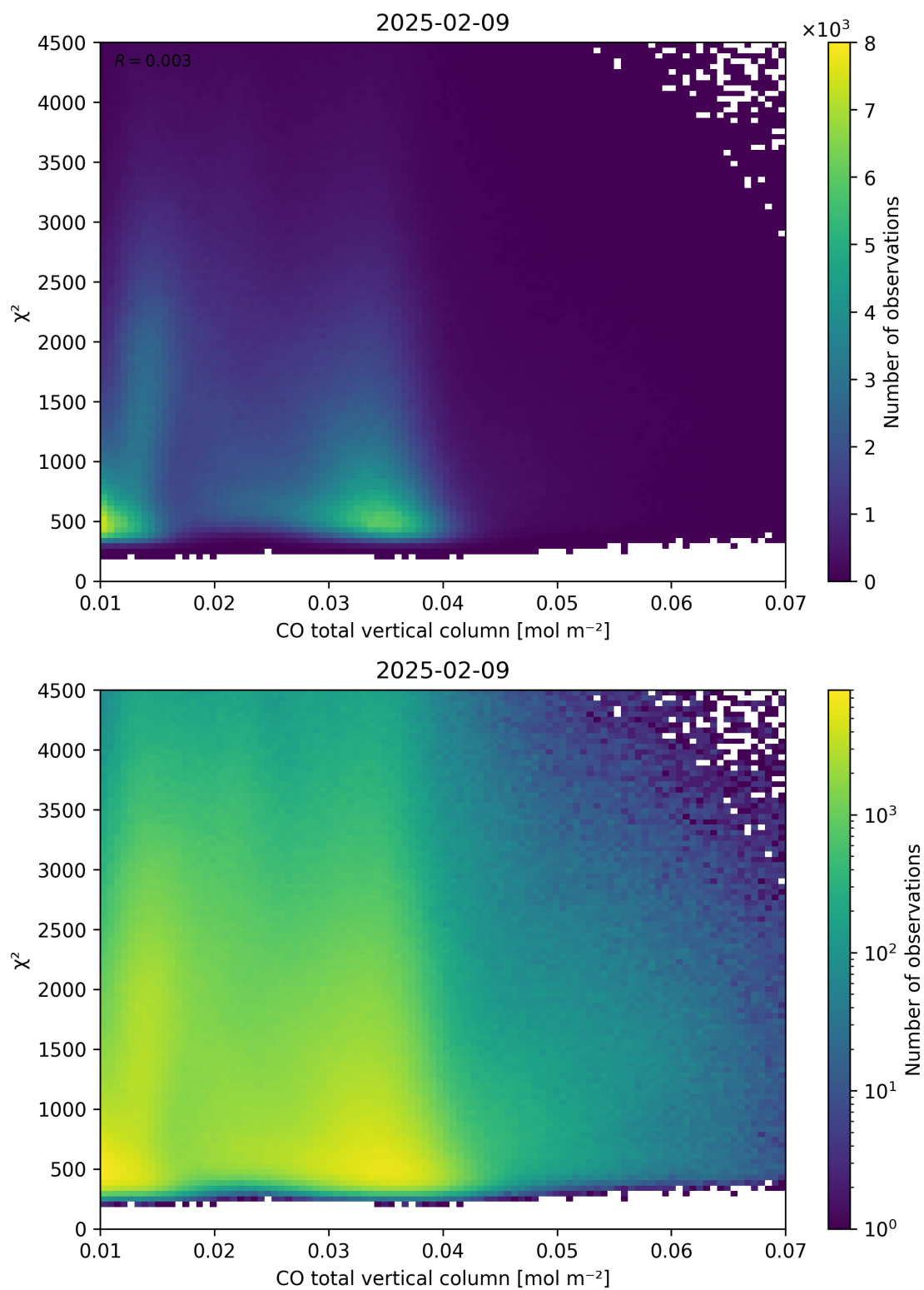
Figure 35: Scatter density plot of “CO total vertical column” against “ \chi^2 ” for 2025-02-08 to 2025-02-10.
