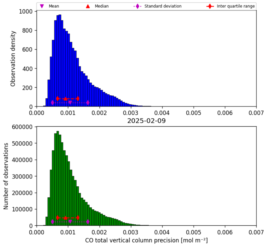
Figure 20: Histogram of “CO total vertical column precision” for 2025-02-08 to 2025-02-10
