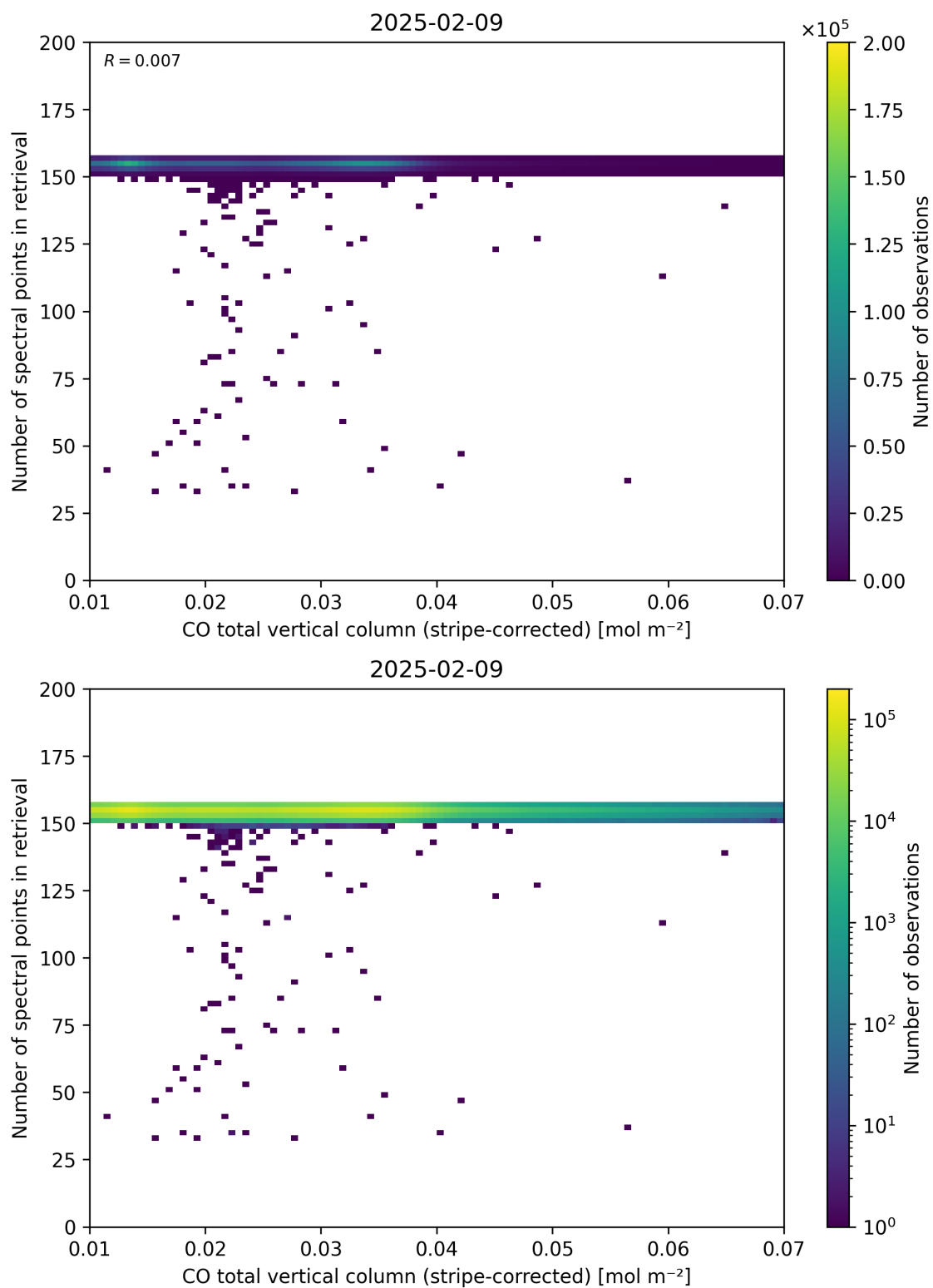
Figure 40: Scatter density plot of “CO total vertical column (stripe-corrected)” against “Number of spectral points in retrieval” for 2025-02-08 to 2025-02-10.
