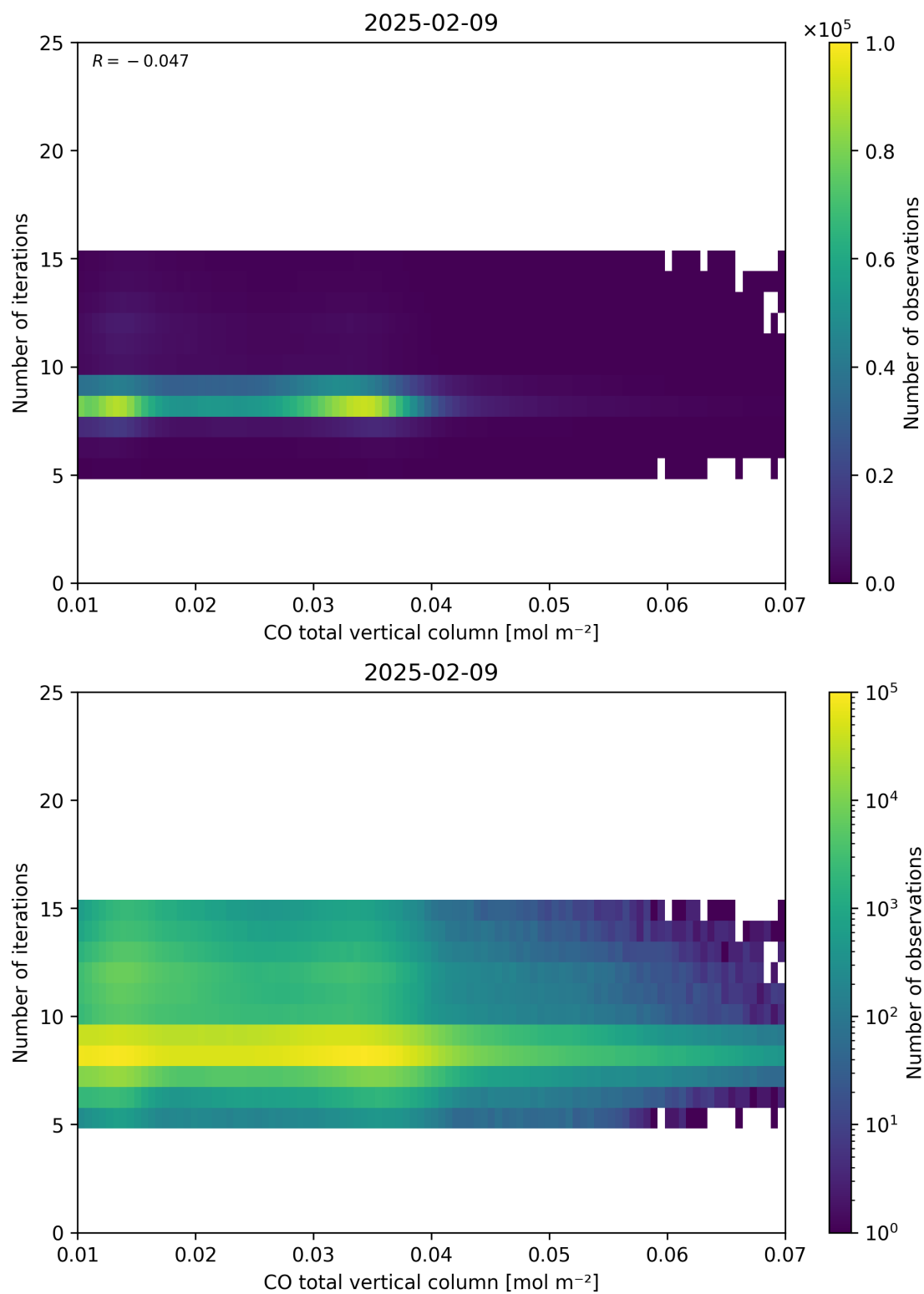
Figure 42: Scatter density plot of “CO total vertical column” against “Number of iterations” for 2025-02-08 to 2025-02-10.
