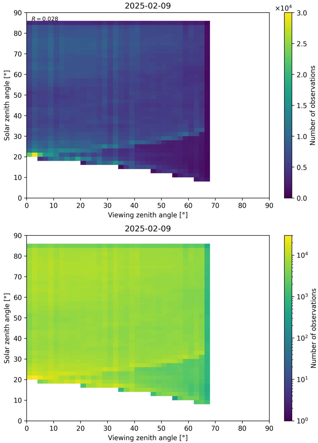
Figure 77: Scatter density plot of “Viewing zenith angle” against “Solar zenith angle” for 2025-02-08 to 2025-02-10.
