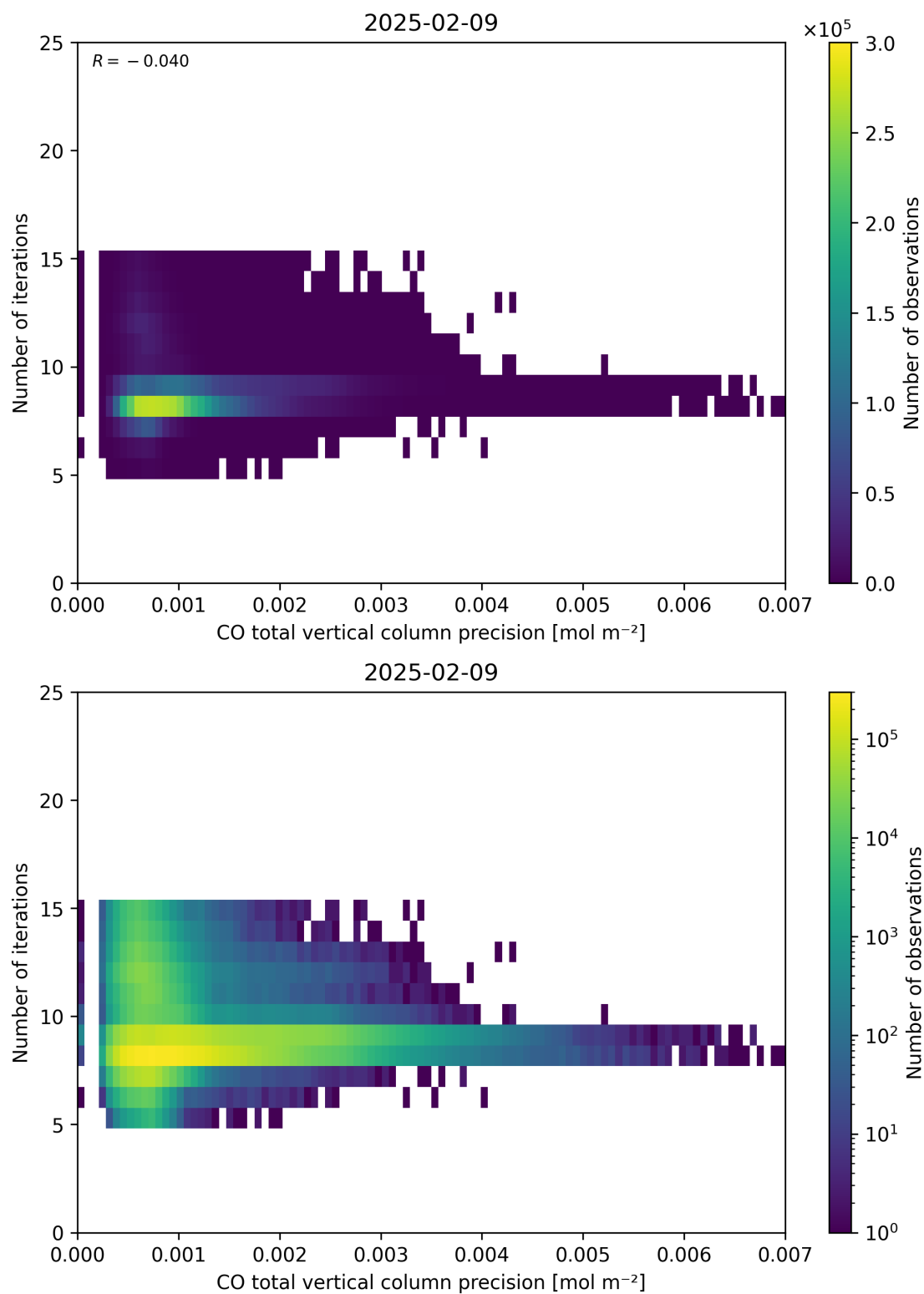
Figure 46: Scatter density plot of “CO total vertical column precision” against “Number of iterations” for 2025-02-08 to 2025-02-10.
