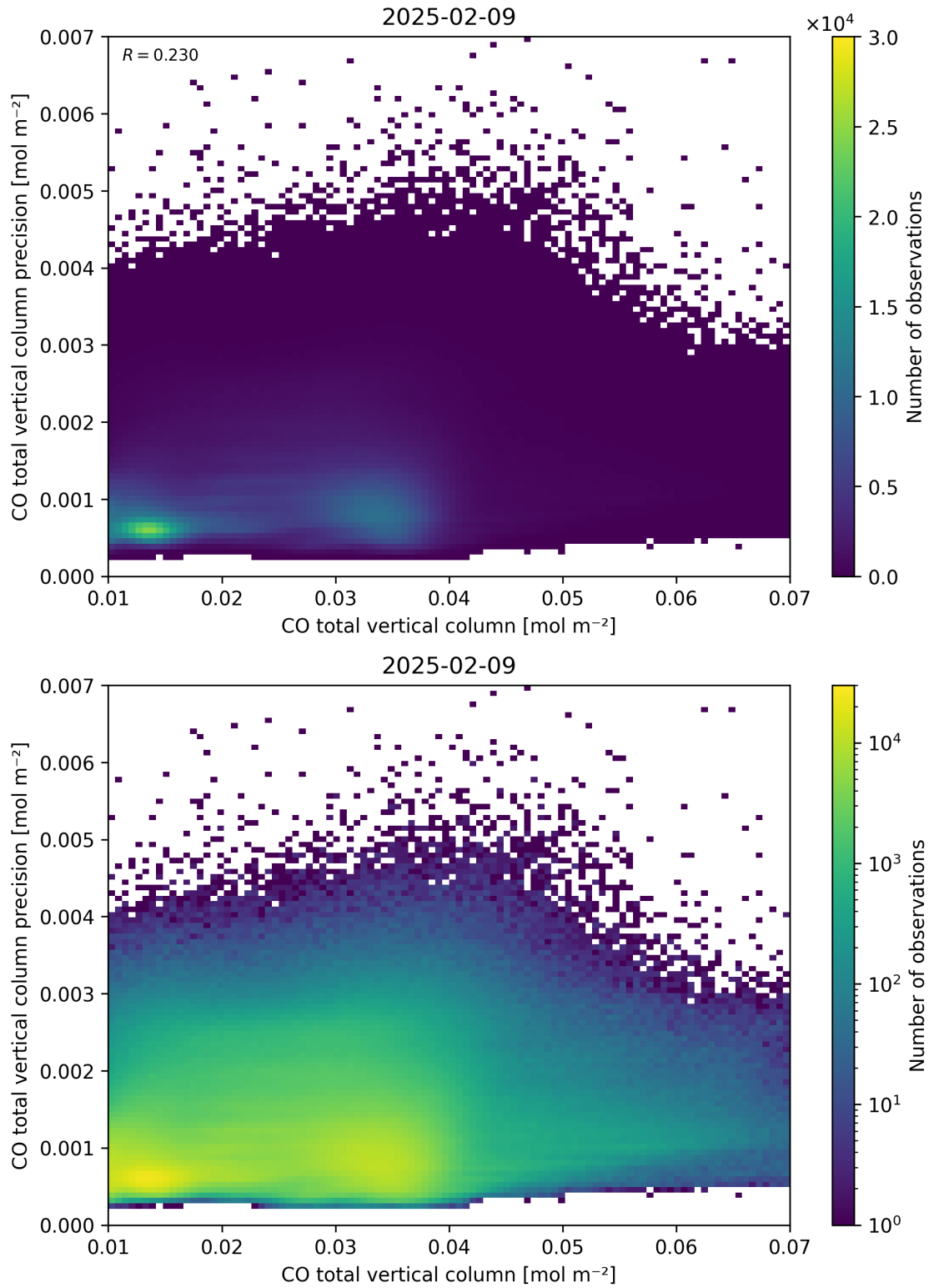
Figure 34: Scatter density plot of “CO total vertical column” against “CO total vertical column precision” for 2025-02-08 to 2025-02-10.
