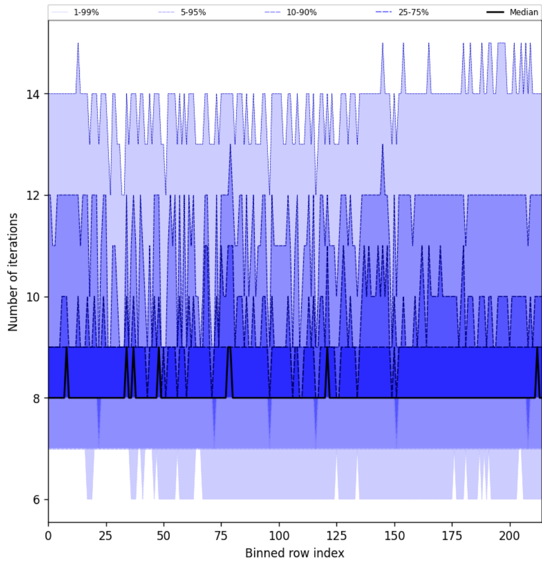
Figure 32: Along track statistics of “Number of iterations” for 2025-02-08 to 2025-02-10
