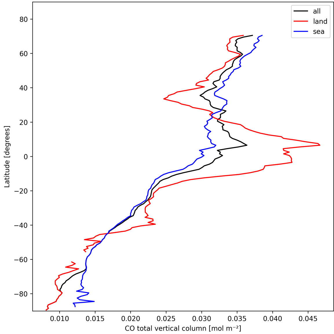
Figure 10: Zonal average of “CO total vertical column” for 2025-02-08 to 2025-02-10.
