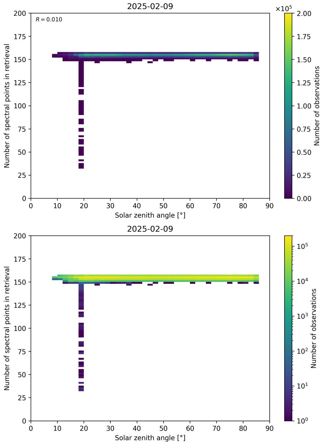
Figure 68: Scatter density plot of “Solar zenith angle” against “Number of spectral points in retrieval” for 2025-02-08 to 2025-02-10.
