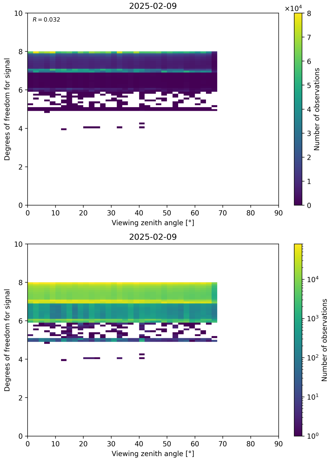
Figure 73: Scatter density plot of “Viewing zenith angle” against “Degrees of freedom for signal” for 2025-02-08 to 2025-02-10.
