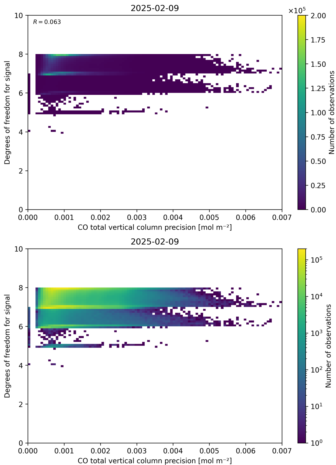
Figure 45: Scatter density plot of “CO total vertical column precision” against “Degrees of freedom for signal” for 2025-02-08 to 2025-02-10.
