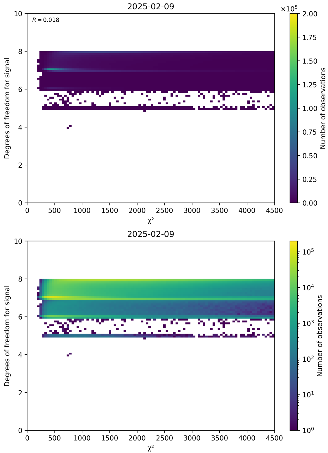
Figure 48: Scatter density plot of “ \chi^2 ” against “Degrees of freedom for signal” for 2025-02-08 to 2025-02-10.
