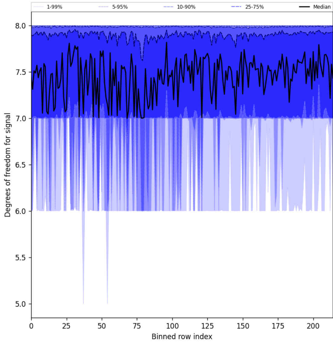
Figure 31: Along track statistics of “Degrees of freedom for signal” for 2025-02-08 to 2025-02-10
