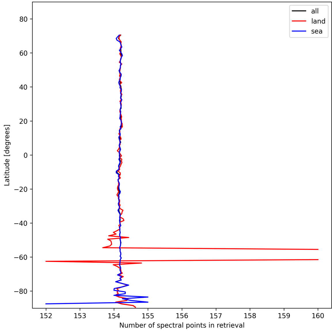
Figure 13: Zonal average of “Number of spectral points in retrieval” for 2025-02-08 to 2025-02-10.
