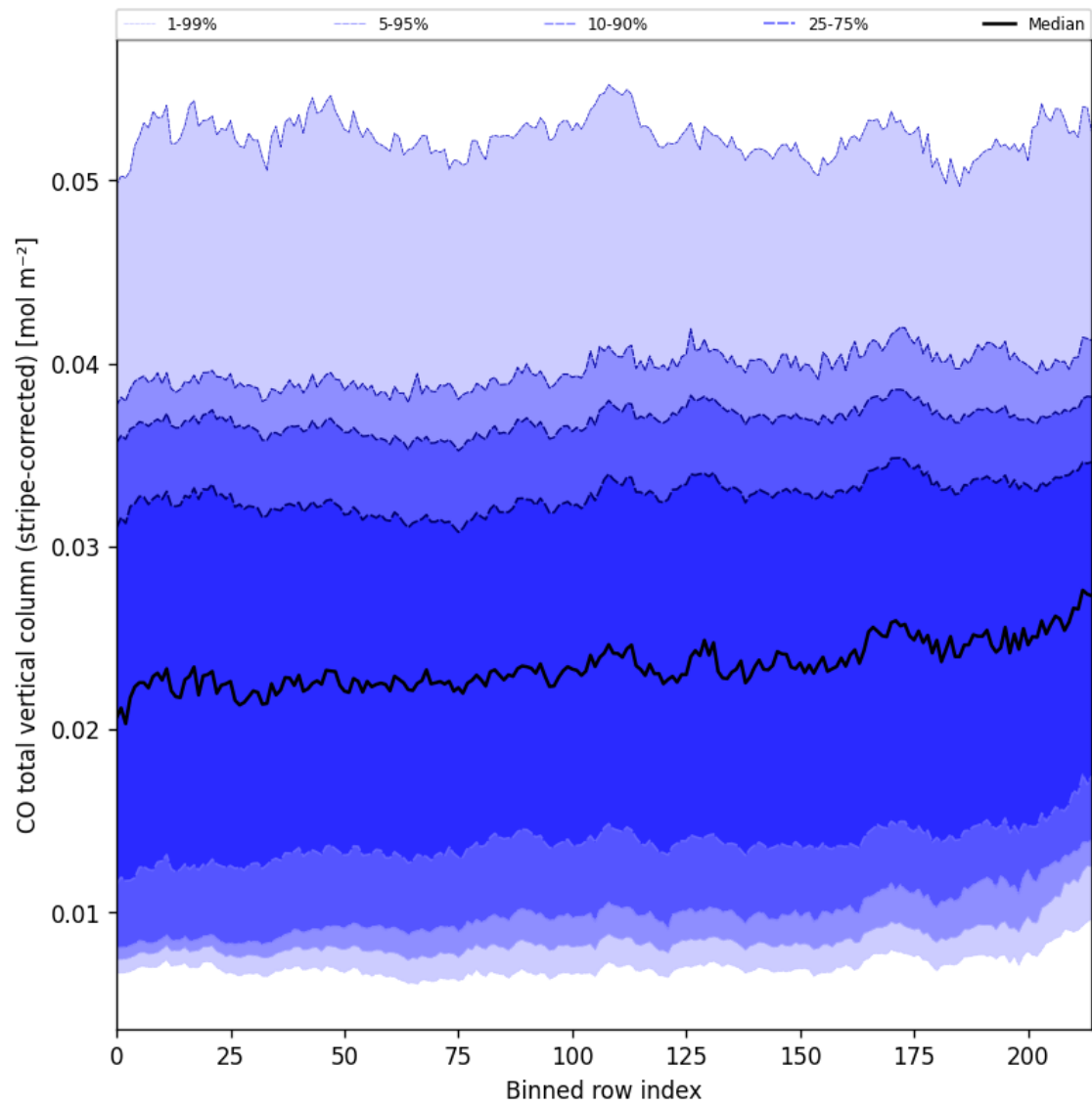
Figure 27: Along track statistics of “CO total vertical column (stripe-corrected)” for 2025-02-08 to 2025-02-10
