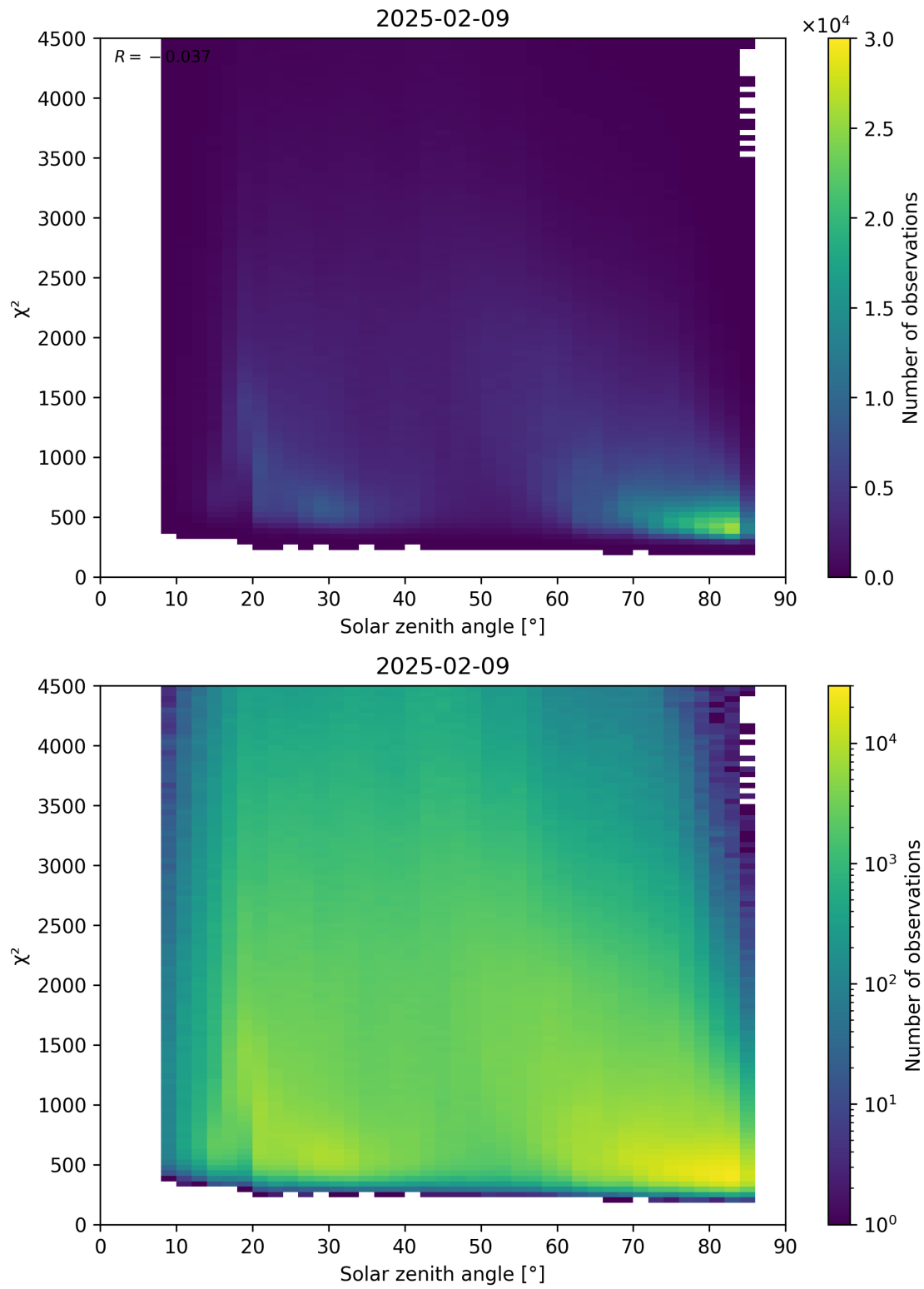
Figure 64: Scatter density plot of “Solar zenith angle” against “ \chi^2 ” for 2025-02-08 to 2025-02-10.
