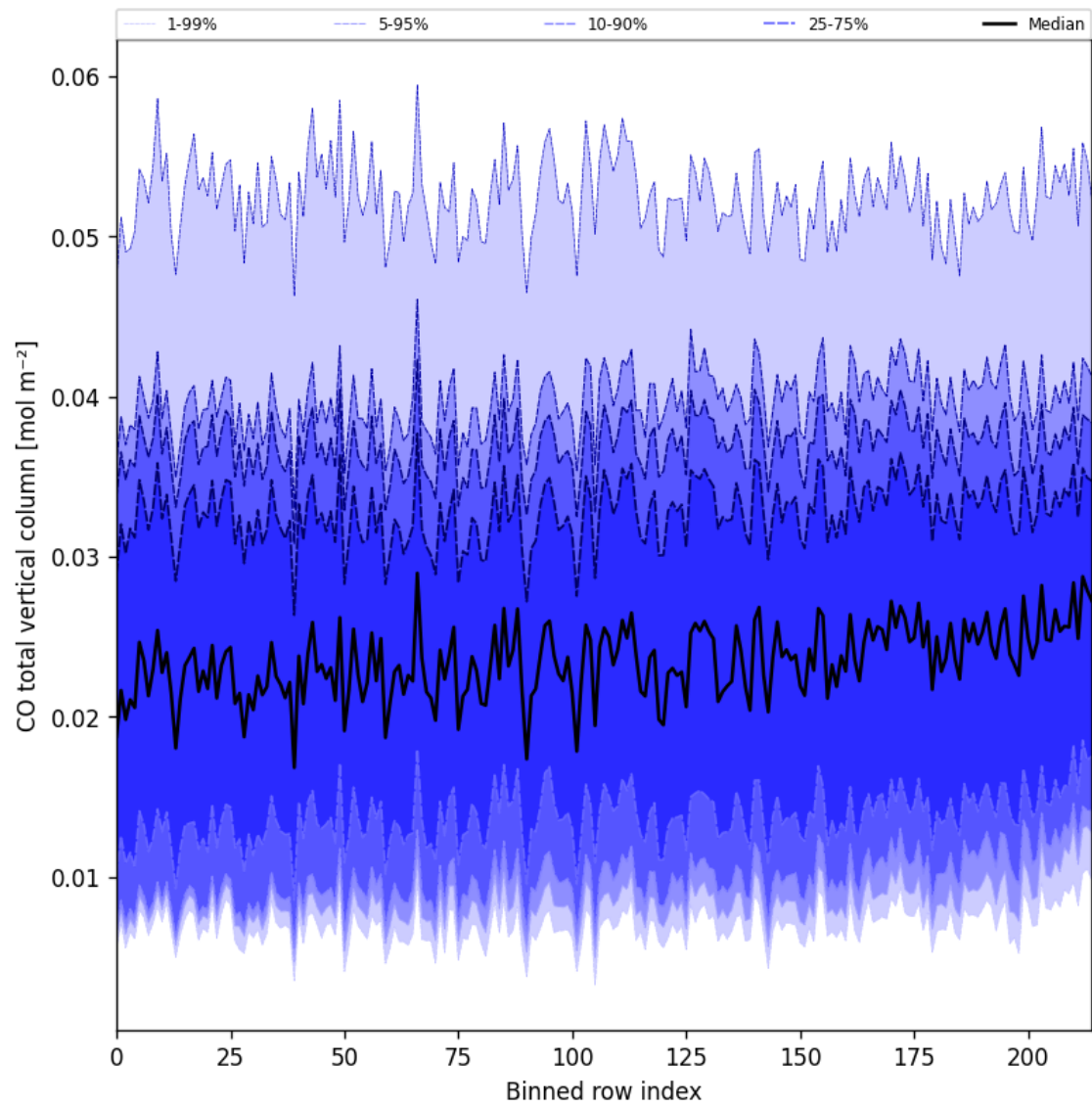
Figure 26: Along track statistics of “CO total vertical column” for 2025-02-08 to 2025-02-10
