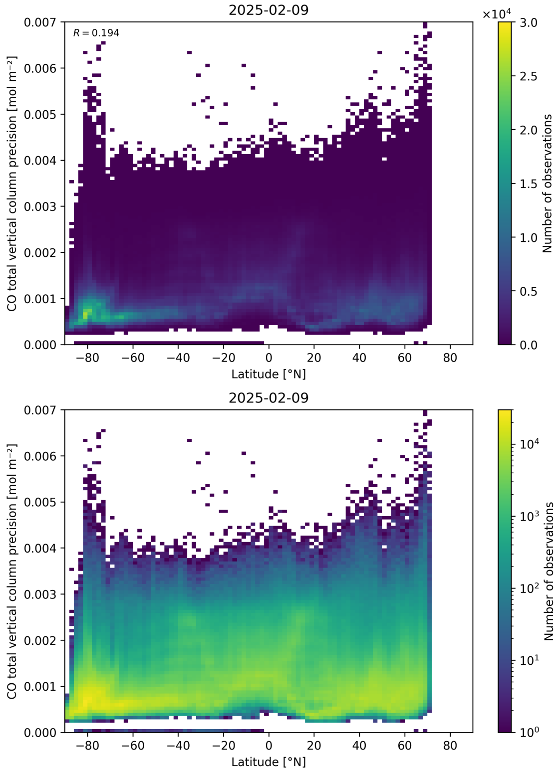
Figure 53: Scatter density plot of “Latitude” against “CO total vertical column precision” for 2025-02-08 to 2025-02-10.
