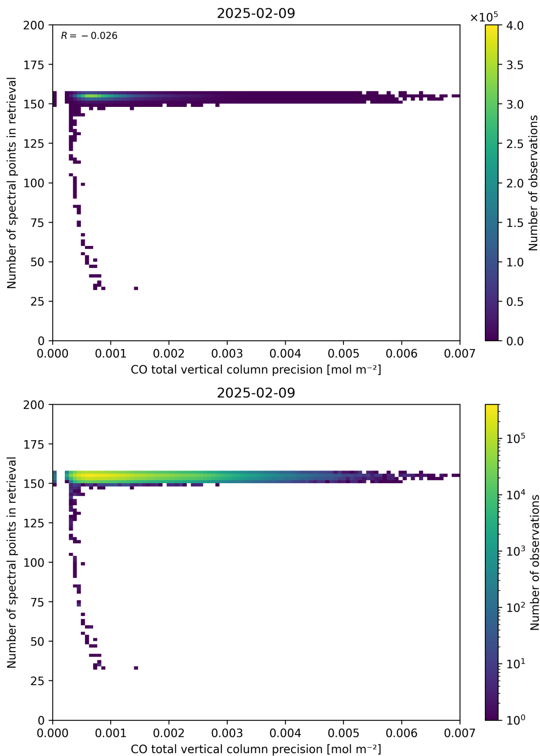
Figure 47: Scatter density plot of “CO total vertical column precision” against “Number of spectral points in retrieval” for 2025-02-08 to 2025-02-10.
