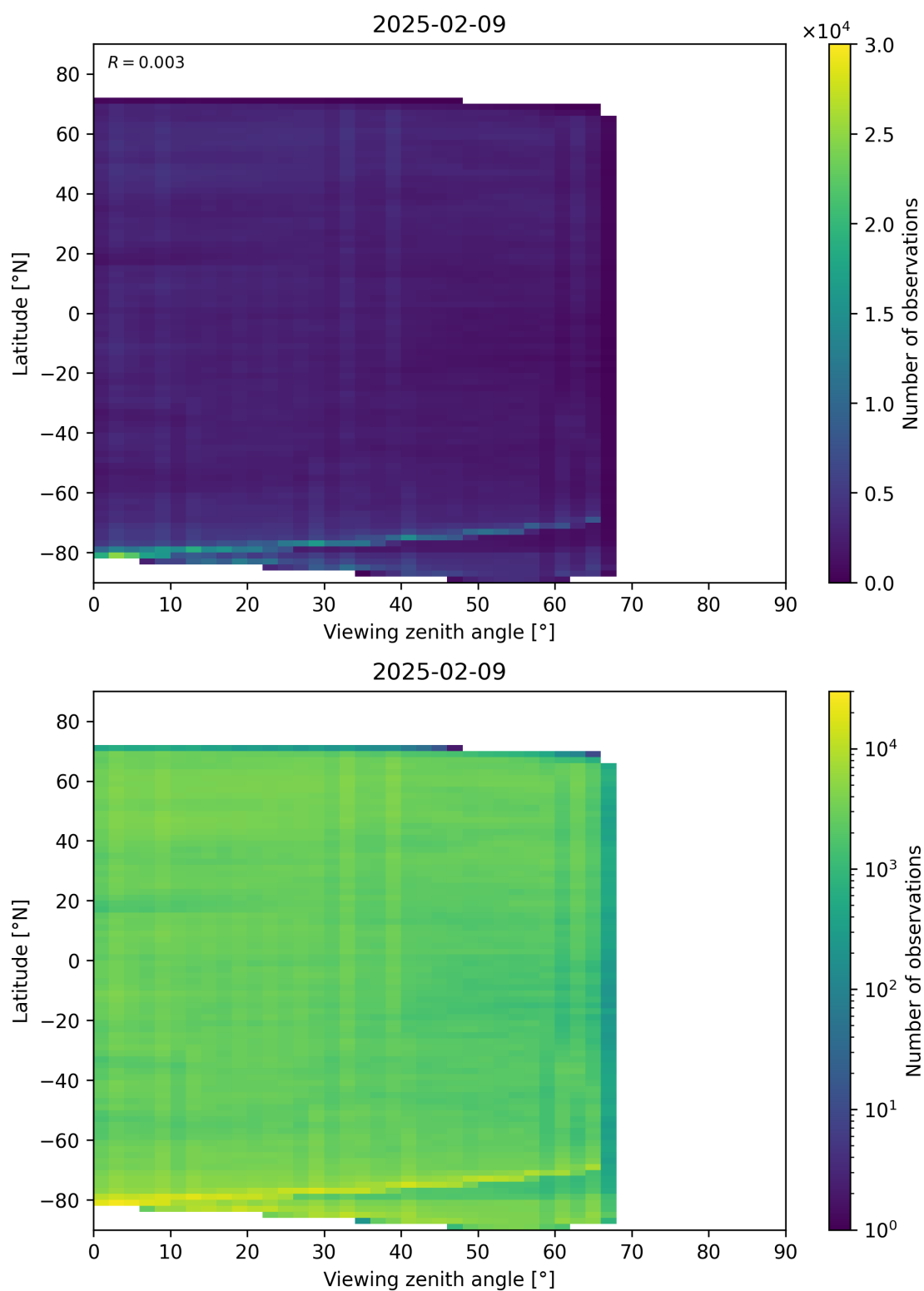
Figure 74: Scatter density plot of “Viewing zenith angle” against “Latitude” for 2025-02-08 to 2025-02-10.
