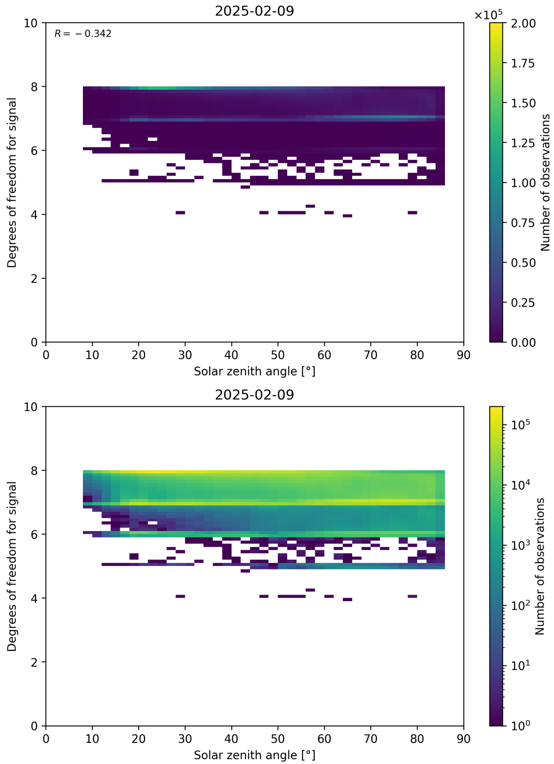
Figure 65: Scatter density plot of “Solar zenith angle” against “Degrees of freedom for signal” for 2025-02-08 to 2025-02-10.
