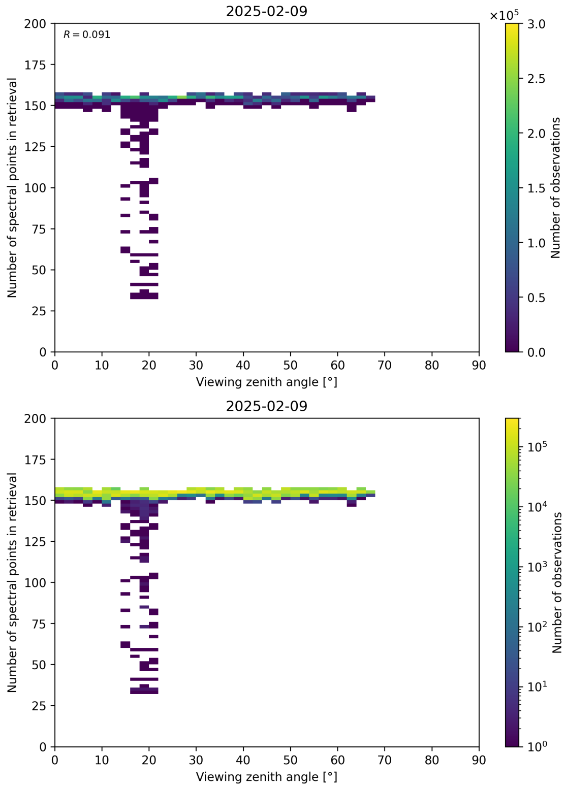
Figure 76: Scatter density plot of “Viewing zenith angle” against “Number of spectral points in retrieval” for 2025-02-08 to 2025-02-10.
