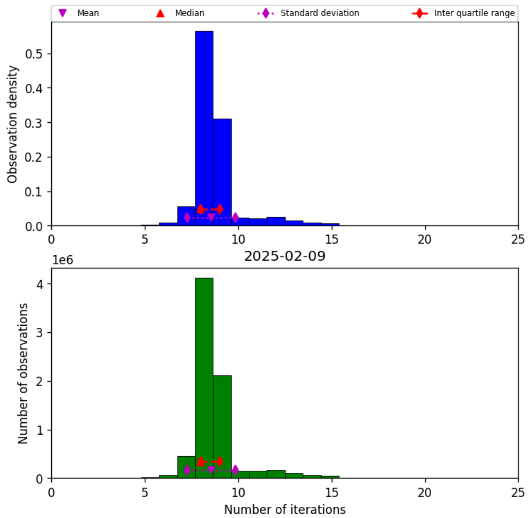
Figure 24: Histogram of “Number of iterations” for 2025-02-08 to 2025-02-10
