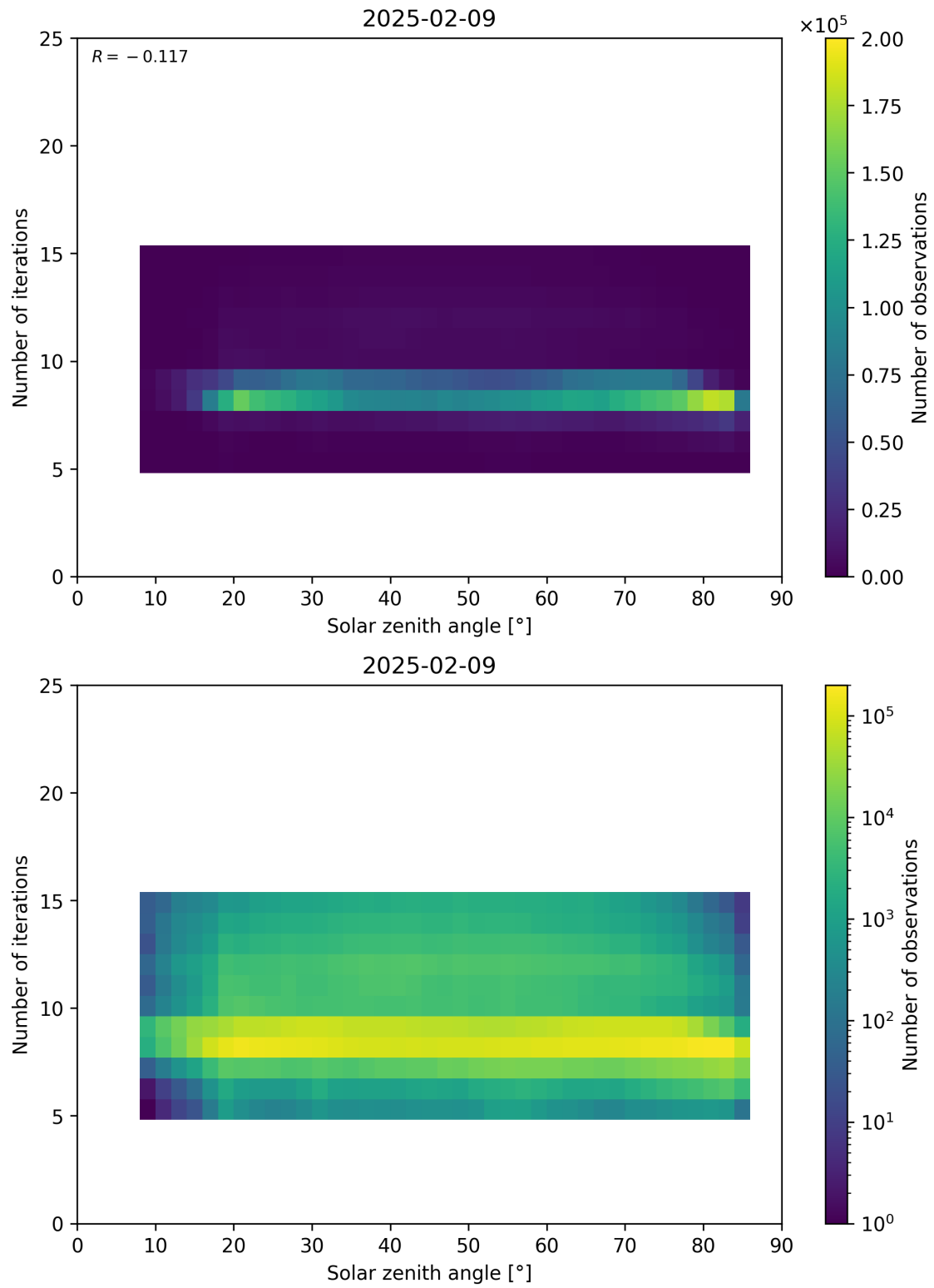
Figure 67: Scatter density plot of “Solar zenith angle” against “Number of iterations” for 2025-02-08 to 2025-02-10.
