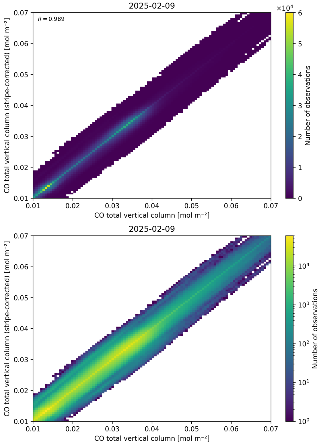
Figure 33: Scatter density plot of “CO total vertical column” against “CO total vertical column (stripe-corrected)” for 2025-02-08 to 2025-02-10.
