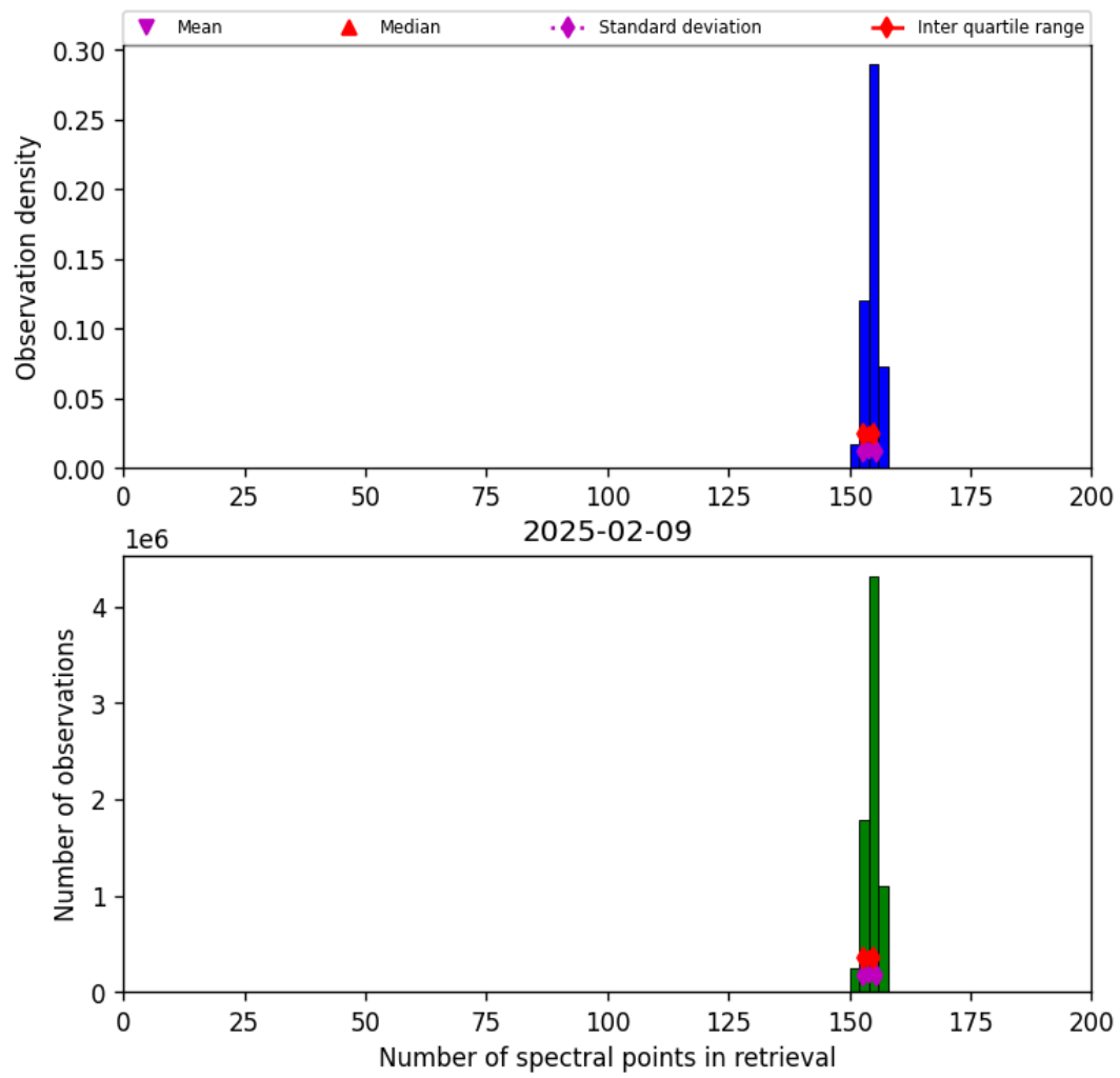
Figure 21: Histogram of “Number of spectral points in retrieval” for 2025-02-08 to 2025-02-10
