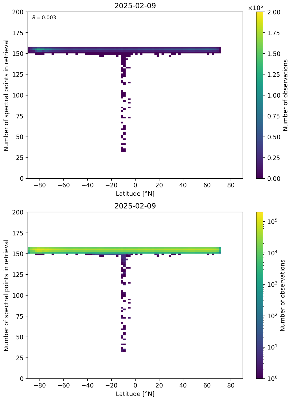
Figure 57: Scatter density plot of “Latitude” against “Number of spectral points in retrieval” for 2025-02-08 to 2025-02-10.
