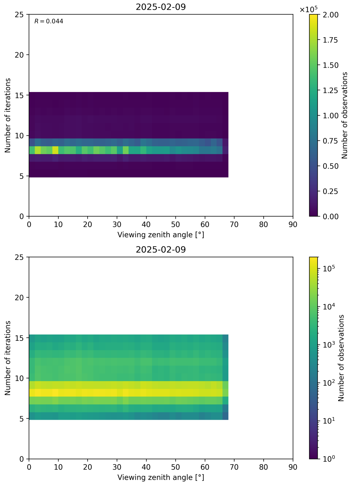
Figure 75: Scatter density plot of “Viewing zenith angle” against “Number of iterations” for 2025-02-08 to 2025-02-10.
