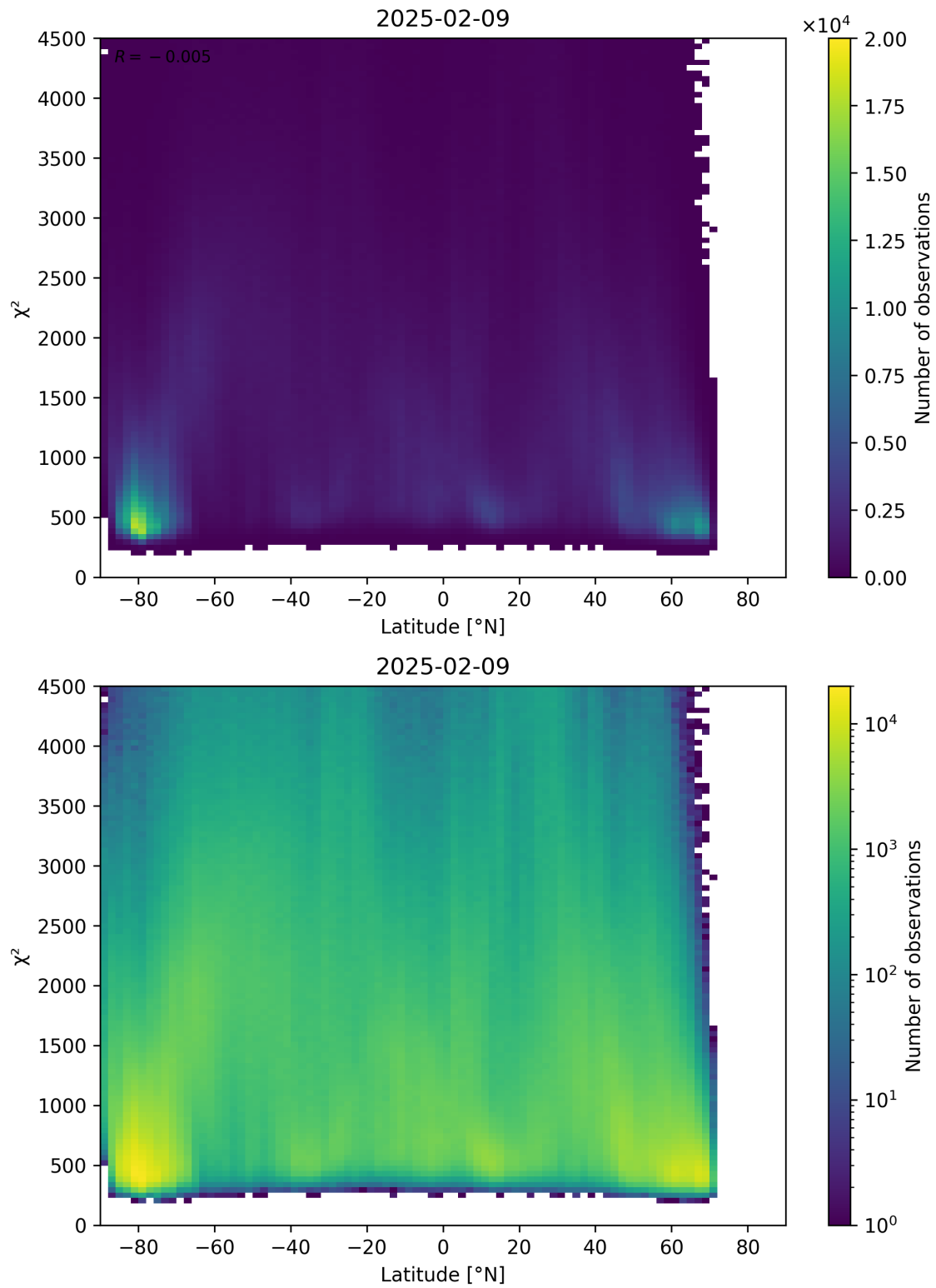
Figure 54: Scatter density plot of “Latitude” against “ \chi^2 ” for 2025-02-08 to 2025-02-10.
