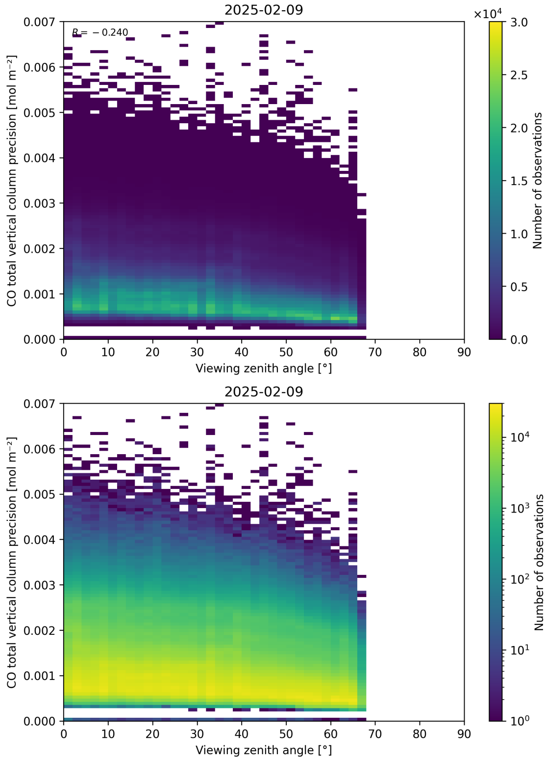
Figure 71: Scatter density plot of “Viewing zenith angle” against “CO total vertical column precision” for 2025-02-08 to 2025-02-10.
