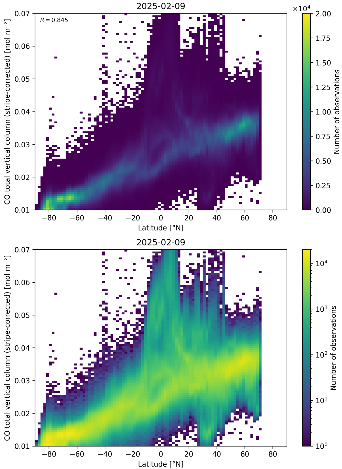
Figure 52: Scatter density plot of “Latitude” against “CO total vertical column (stripe-corrected)” for 2025-02-08 to 2025-02-10.
