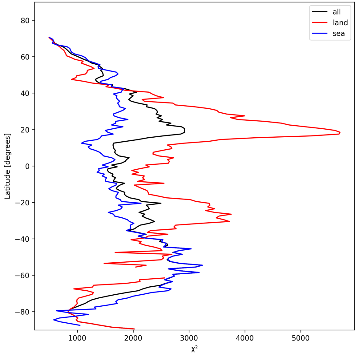
Figure 14: Zonal average of “ \chi^2 ” for 2025-02-08 to 2025-02-10.
