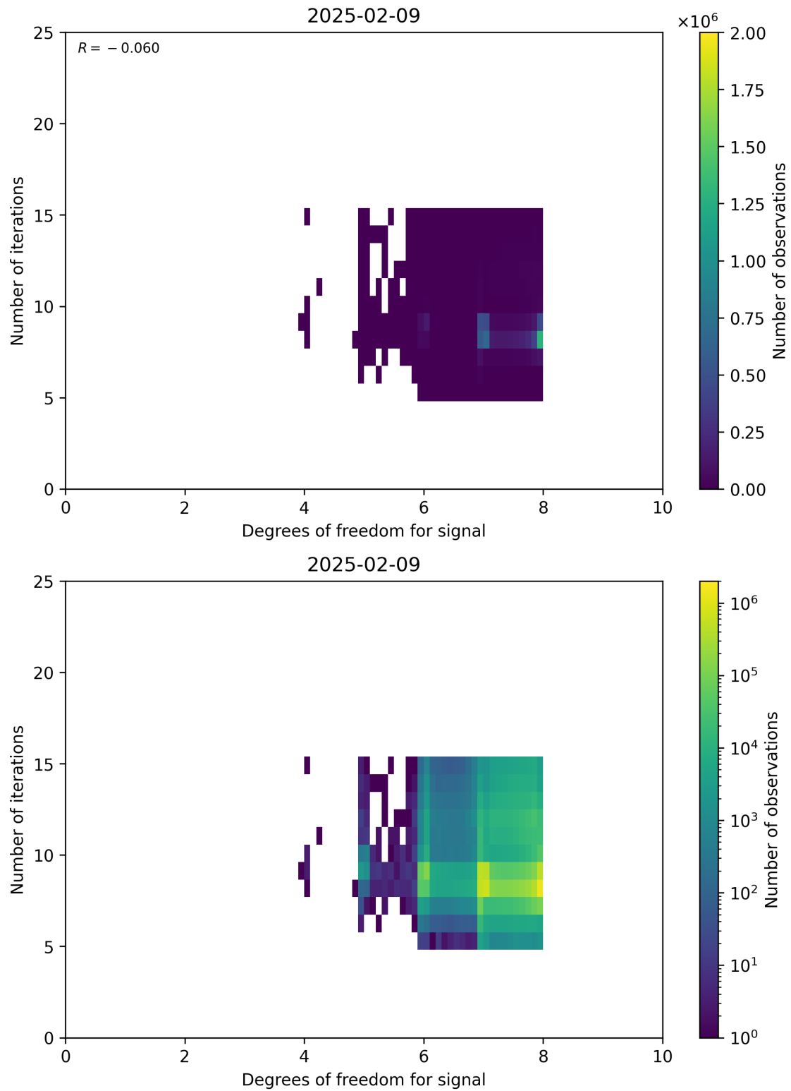
Figure 50: Scatter density plot of “Degrees of freedom for signal” against “Number of iterations” for 2025-02-08 to 2025-02-10.
