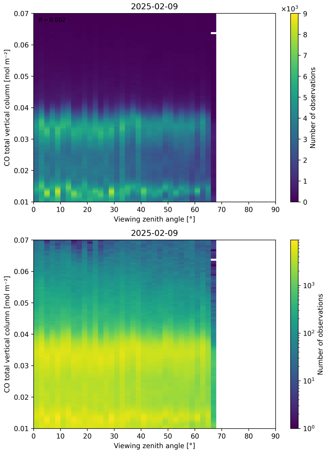
Figure 69: Scatter density plot of “Viewing zenith angle” against “CO total vertical column” for 2025-02-08 to 2025-02-10.
