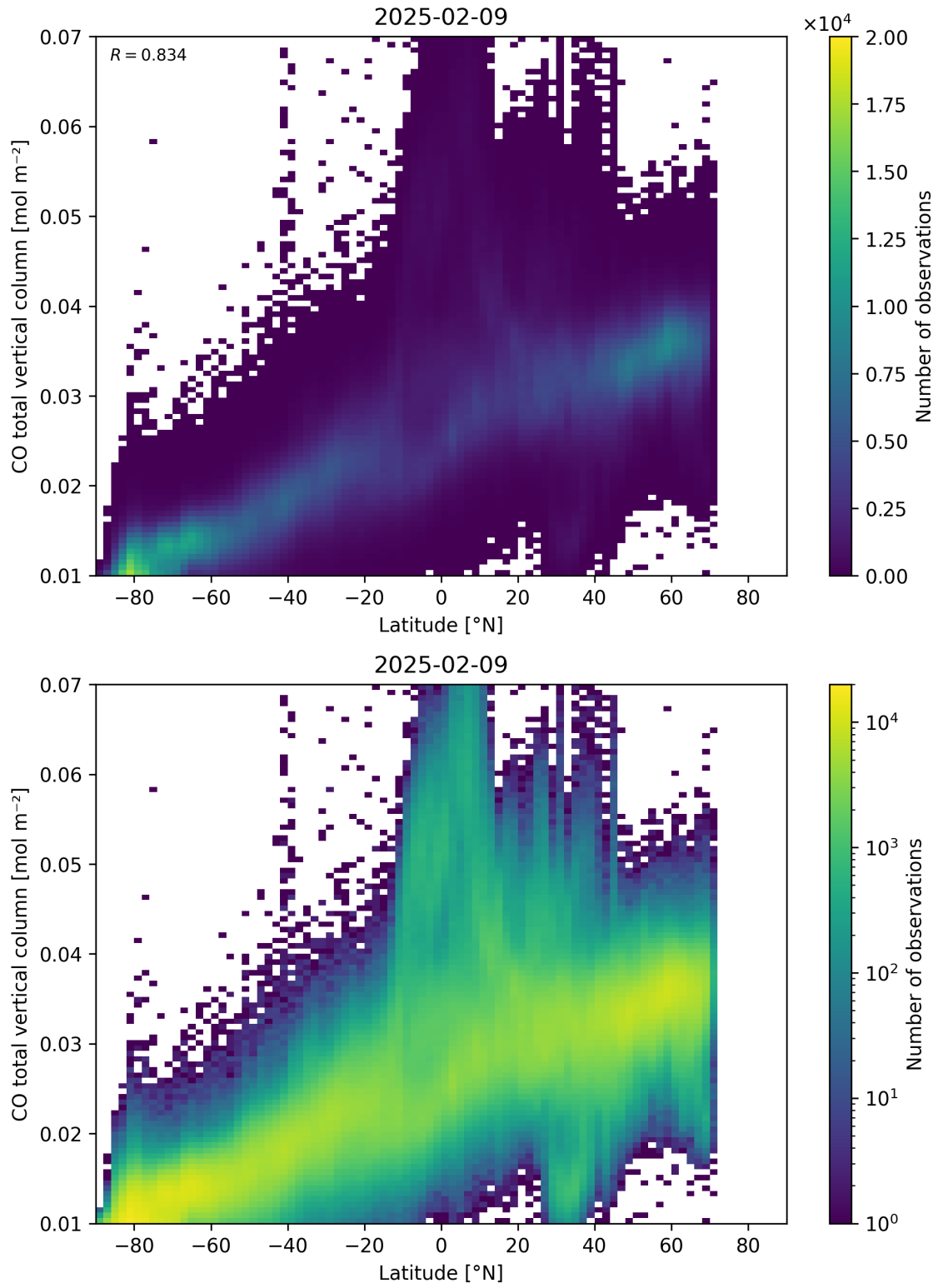
Figure 51: Scatter density plot of “Latitude” against “CO total vertical column” for 2025-02-08 to 2025-02-10.
