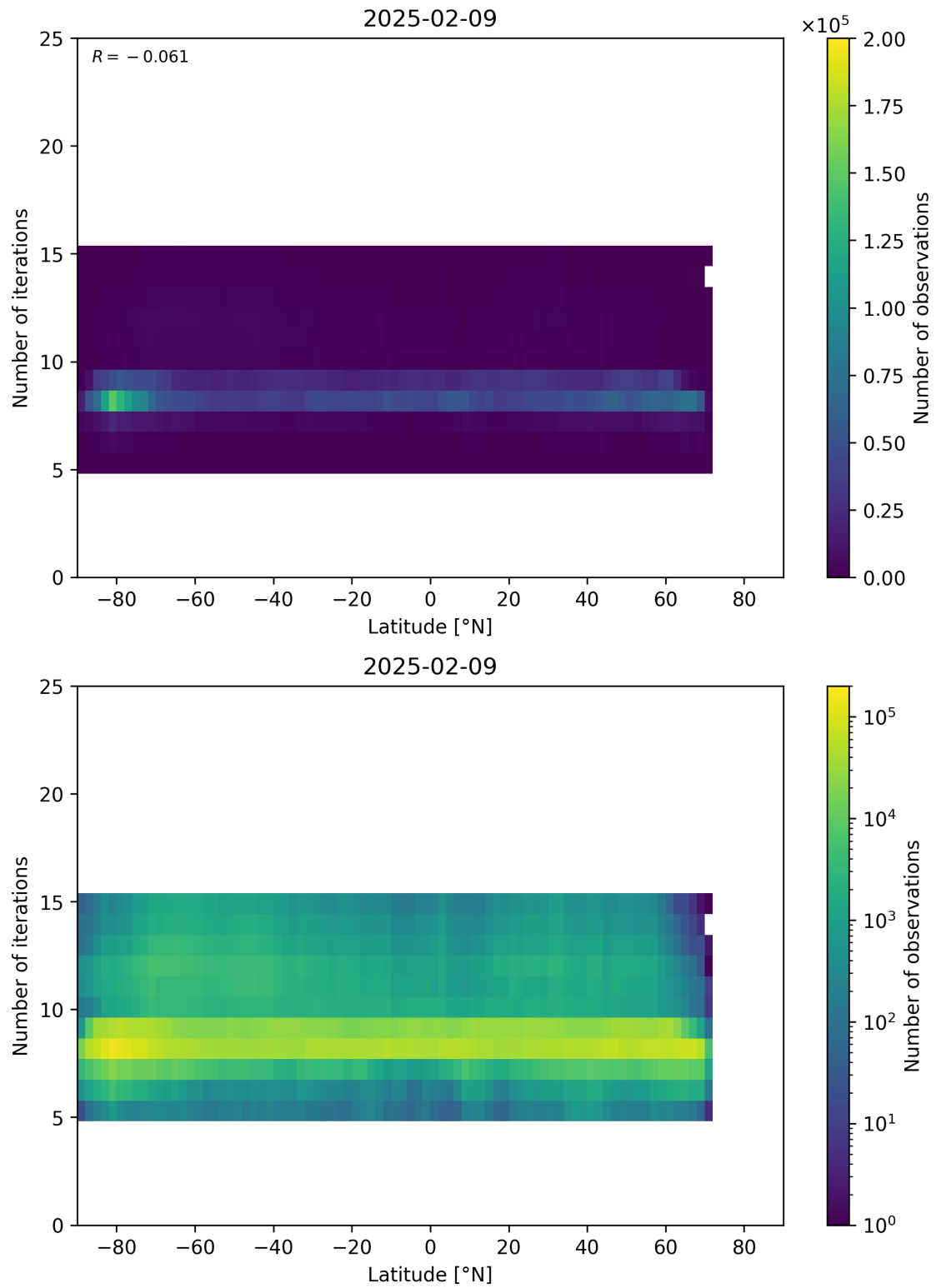
Figure 56: Scatter density plot of “Latitude” against “Number of iterations” for 2025-02-08 to 2025-02-10.
