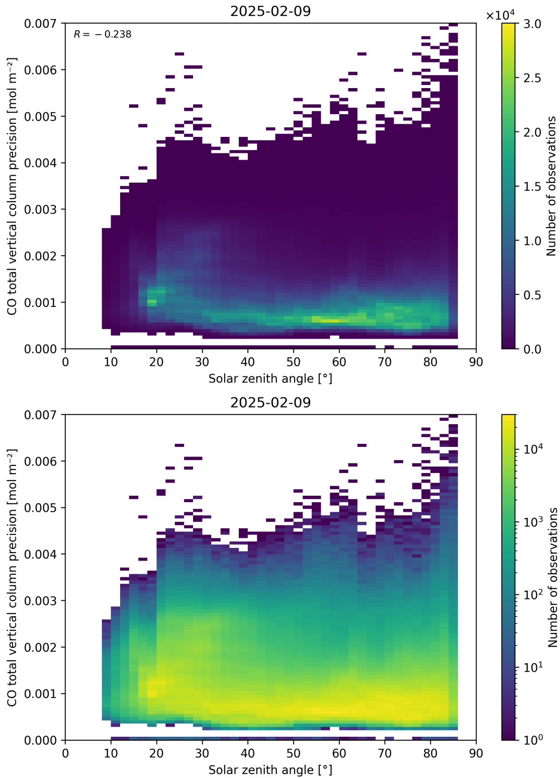
Figure 63: Scatter density plot of “Solar zenith angle” against “CO total vertical column precision” for 2025-02-08 to 2025-02-10.
