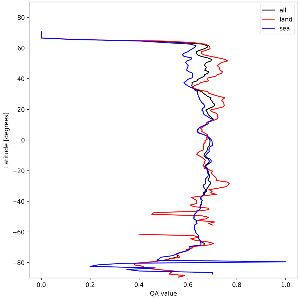
Figure 9: Zonal average of “QA value” for 2025-02-08 to 2025-02-10.
