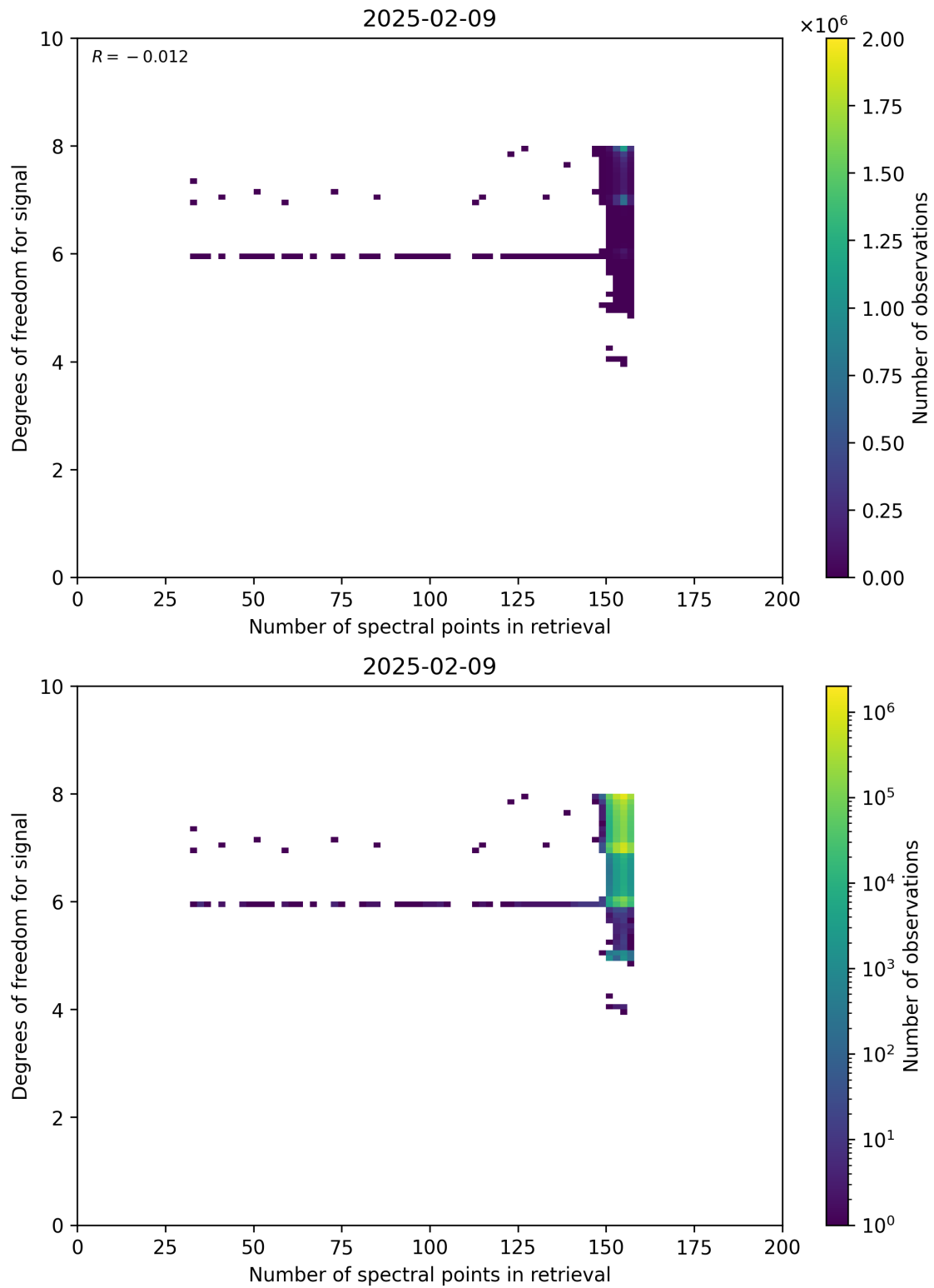
Figure 59: Scatter density plot of “Number of spectral points in retrieval” against “Degrees of freedom for signal” for 2025-02-08 to 2025-02-10.
