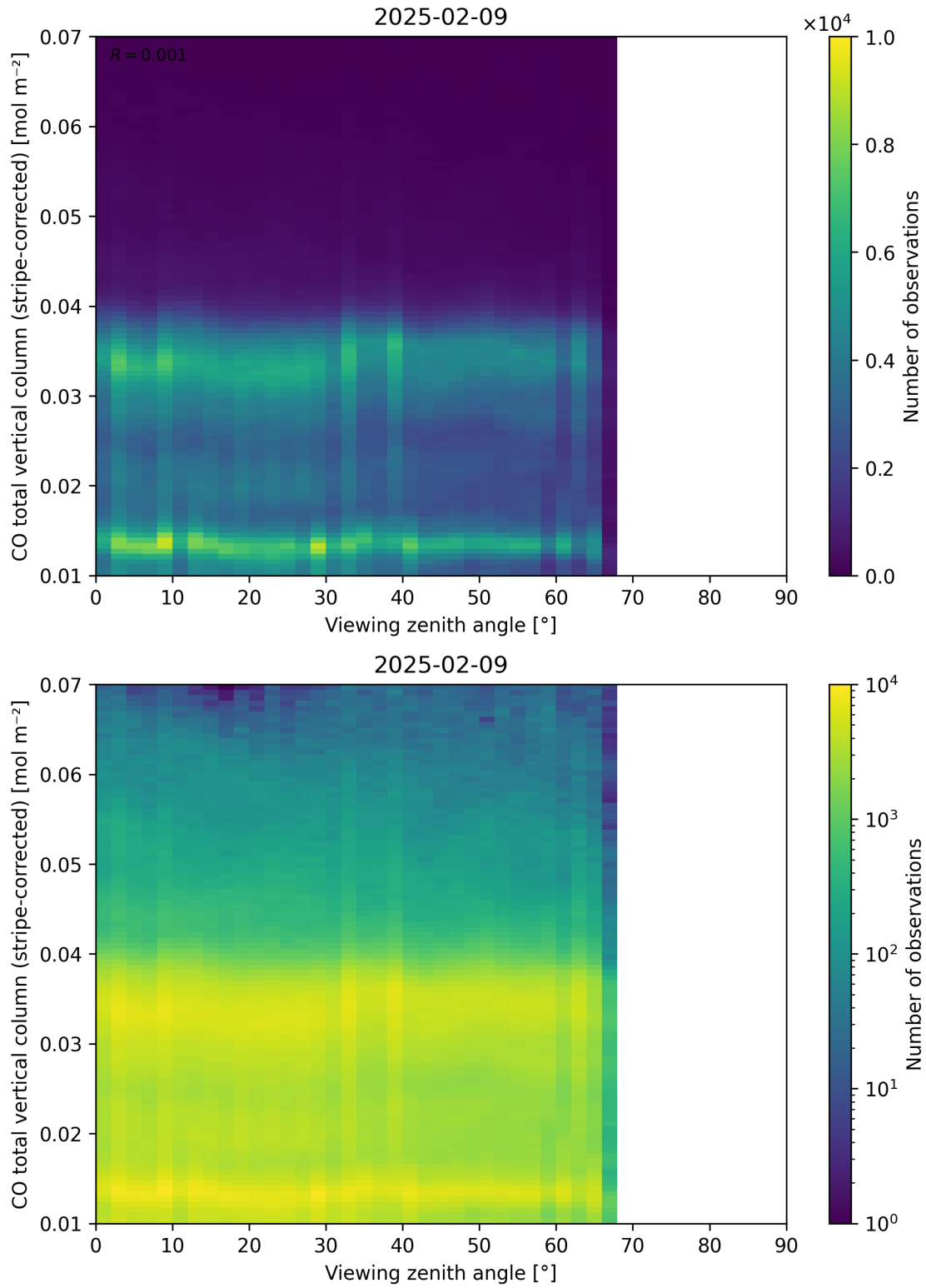
Figure 70: Scatter density plot of “Viewing zenith angle” against “CO total vertical column (stripe-corrected)” for 2025-02-08 to 2025-02-10.
