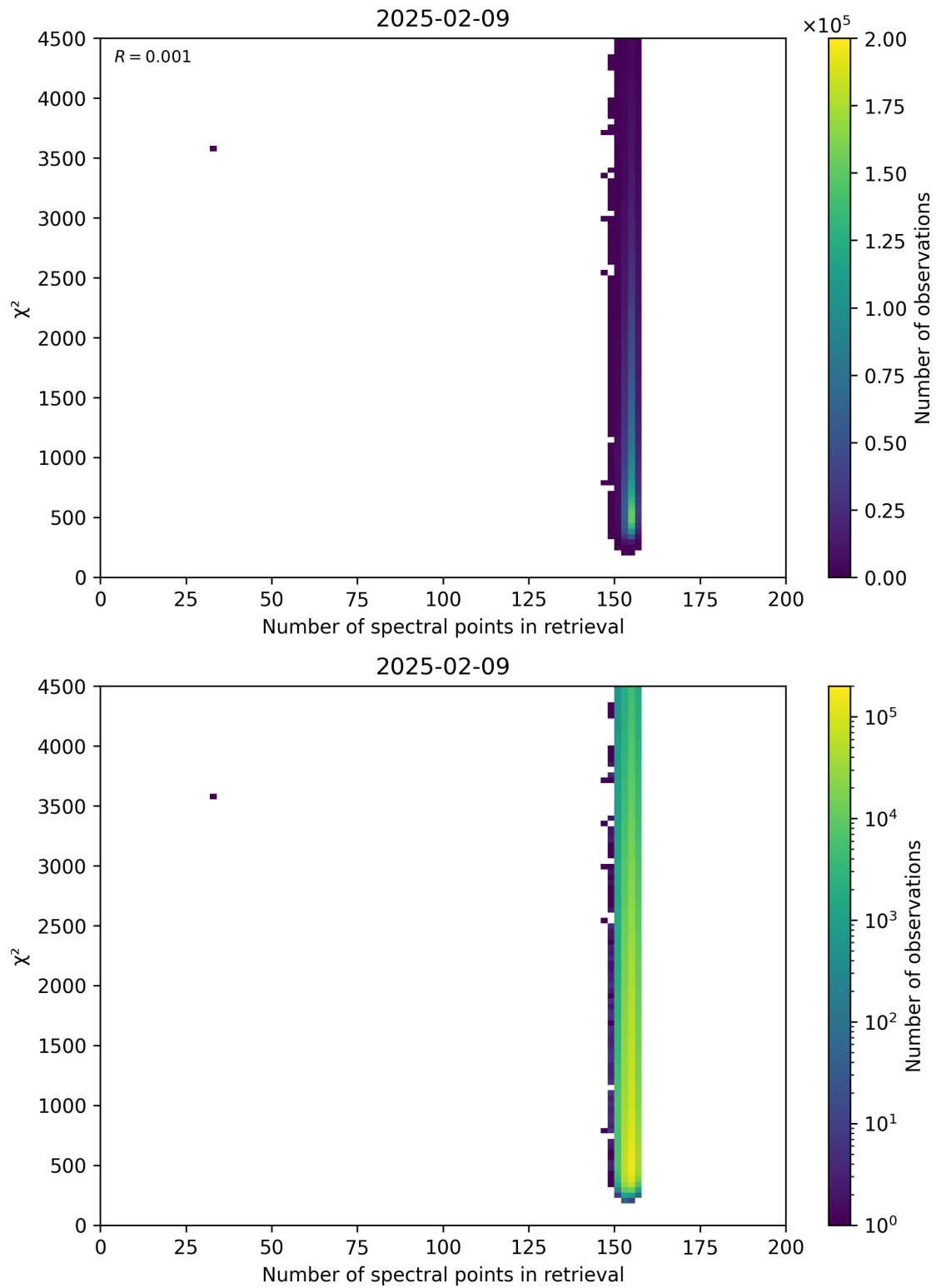
Figure 58: Scatter density plot of “Number of spectral points in retrieval” against “ \chi^2 ” for 2025-02-08 to 2025-02-10.
