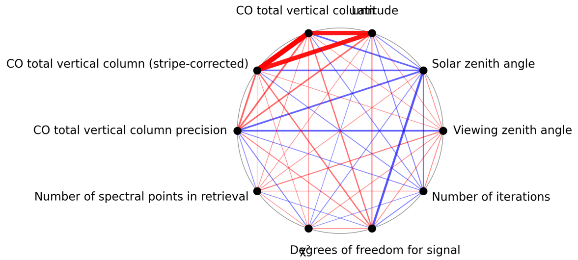
Figure 1: Map of correlation graph for 2025-02-08 to 2025-02-10.
