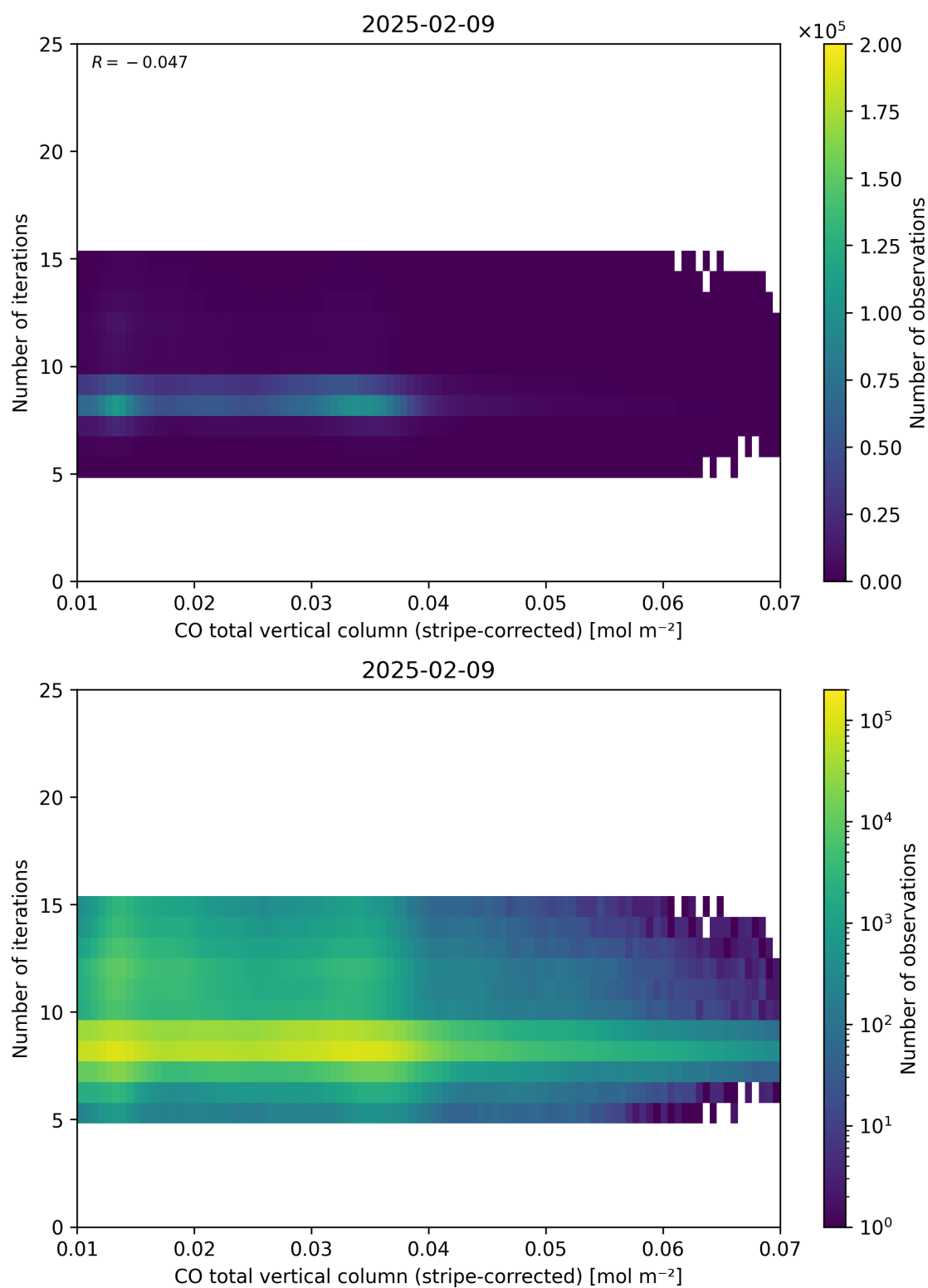
Figure 39: Scatter density plot of “CO total vertical column (stripe-corrected)” against “Number of iterations” for 2025-02-08 to 2025-02-10.
