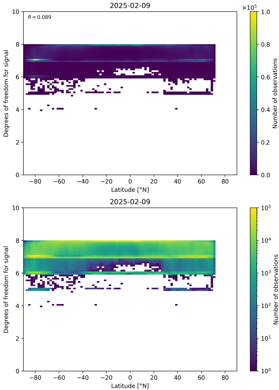
Figure 55: Scatter density plot of “Latitude” against “Degrees of freedom for signal” for 2025-02-08 to 2025-02-10.
