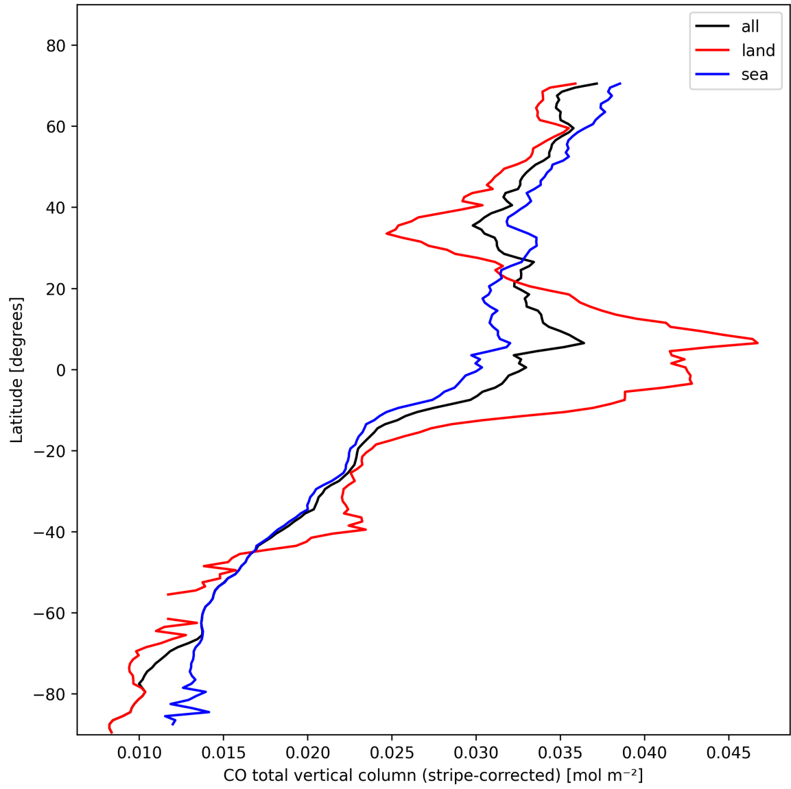
Figure 11: Zonal average of “CO total vertical column (stripe-corrected)” for 2025-02-08 to 2025-02-10.
