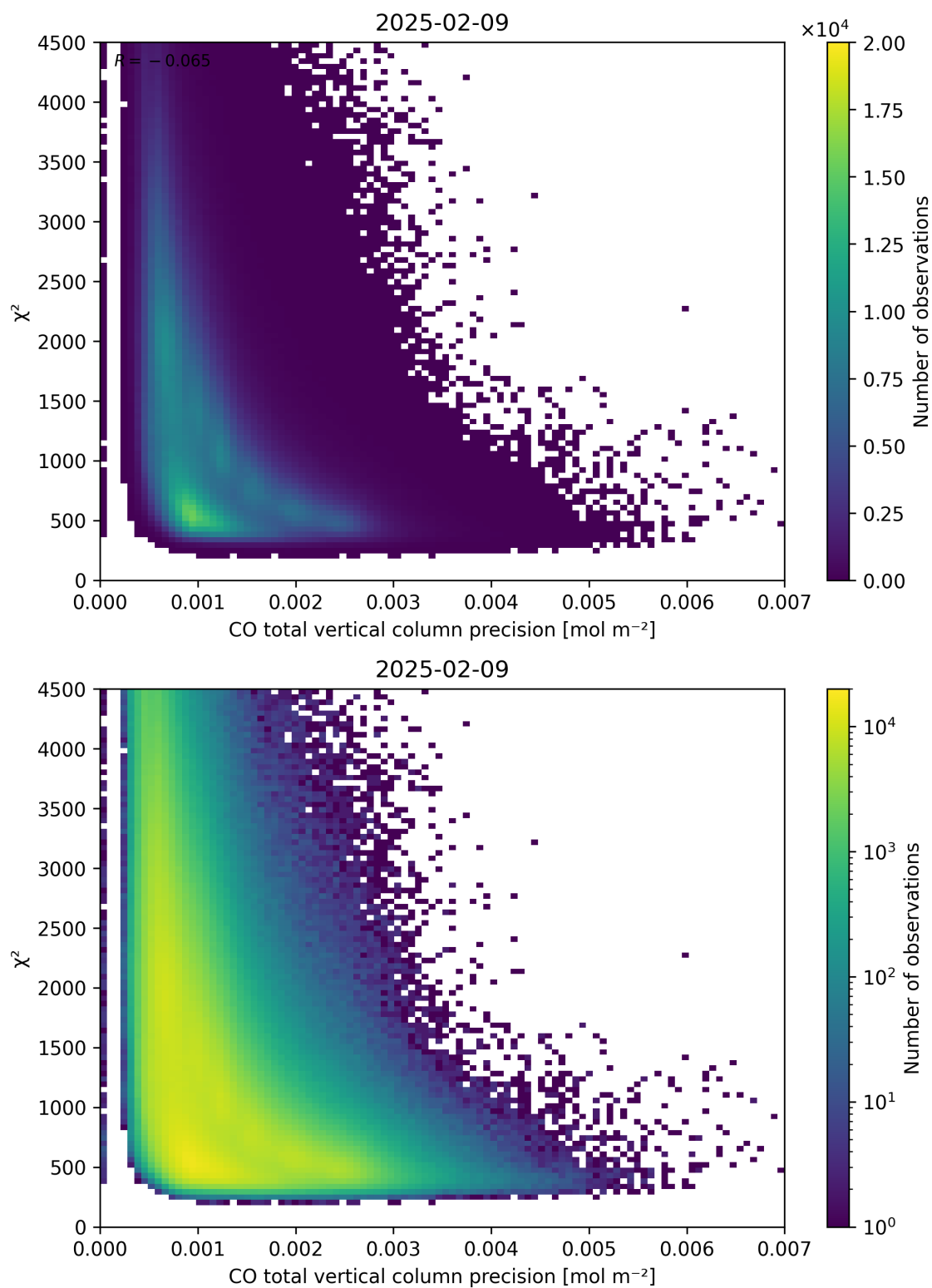
Figure 44: Scatter density plot of “CO total vertical column precision” against “ \chi^2 ” for 2025-02-08 to 2025-02-10.
