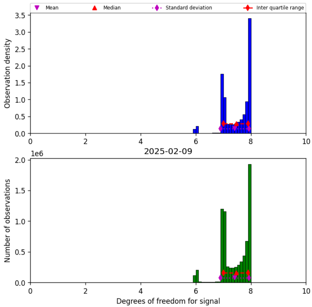
Figure 23: Histogram of “Degrees of freedom for signal” for 2025-02-08 to 2025-02-10
