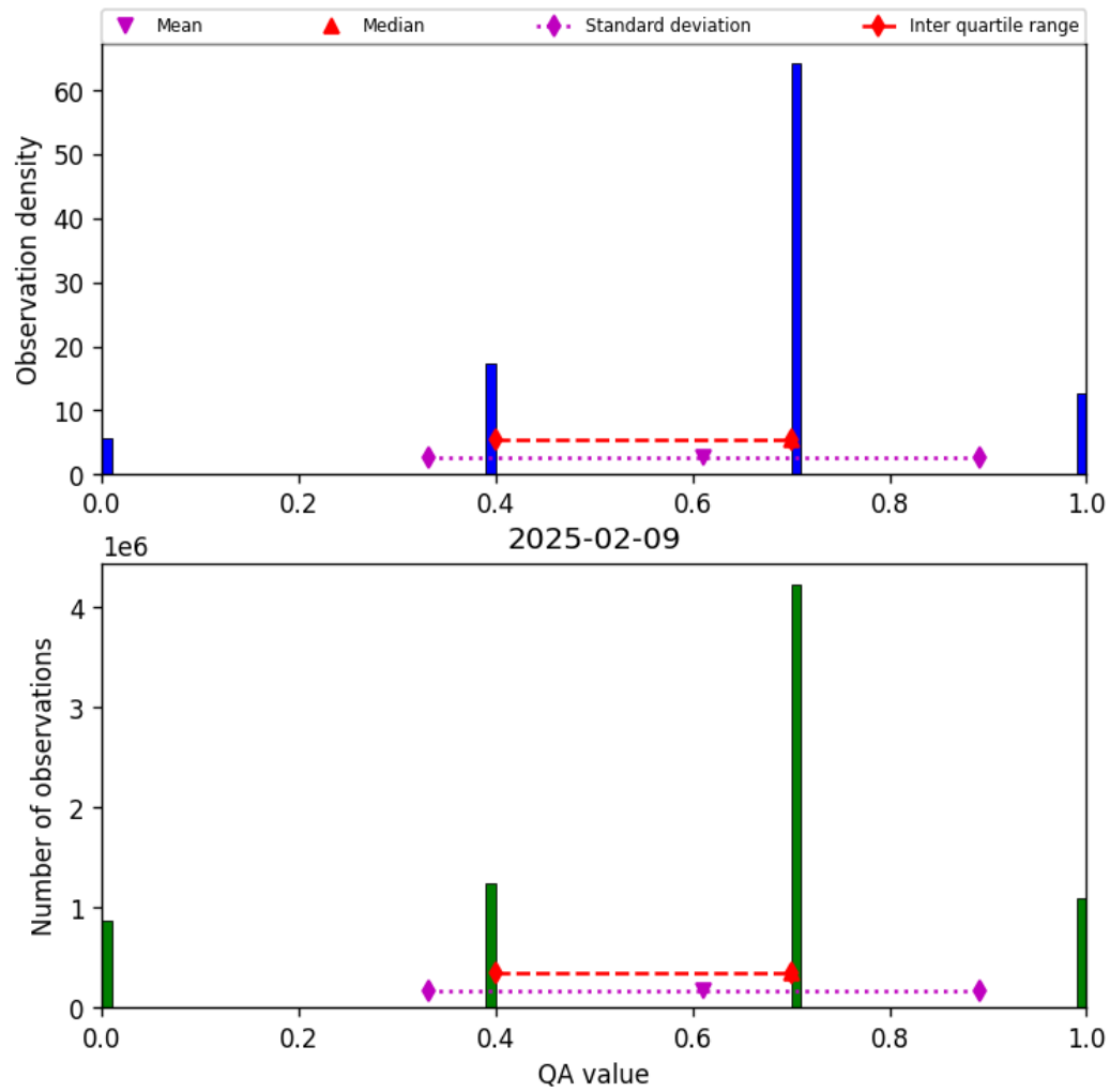
Figure 17: Histogram of “QA value” for 2025-02-08 to 2025-02-10
