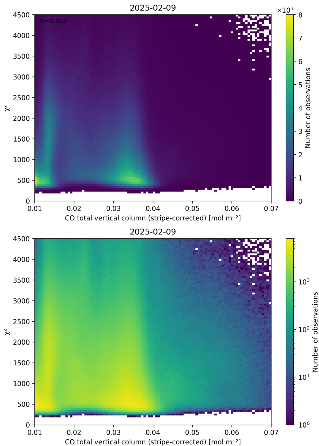
Figure 37: Scatter density plot of “CO total vertical column (stripe-corrected)” against “ \chi^2 ” for 2025-02-08 to 2025-02-10.
