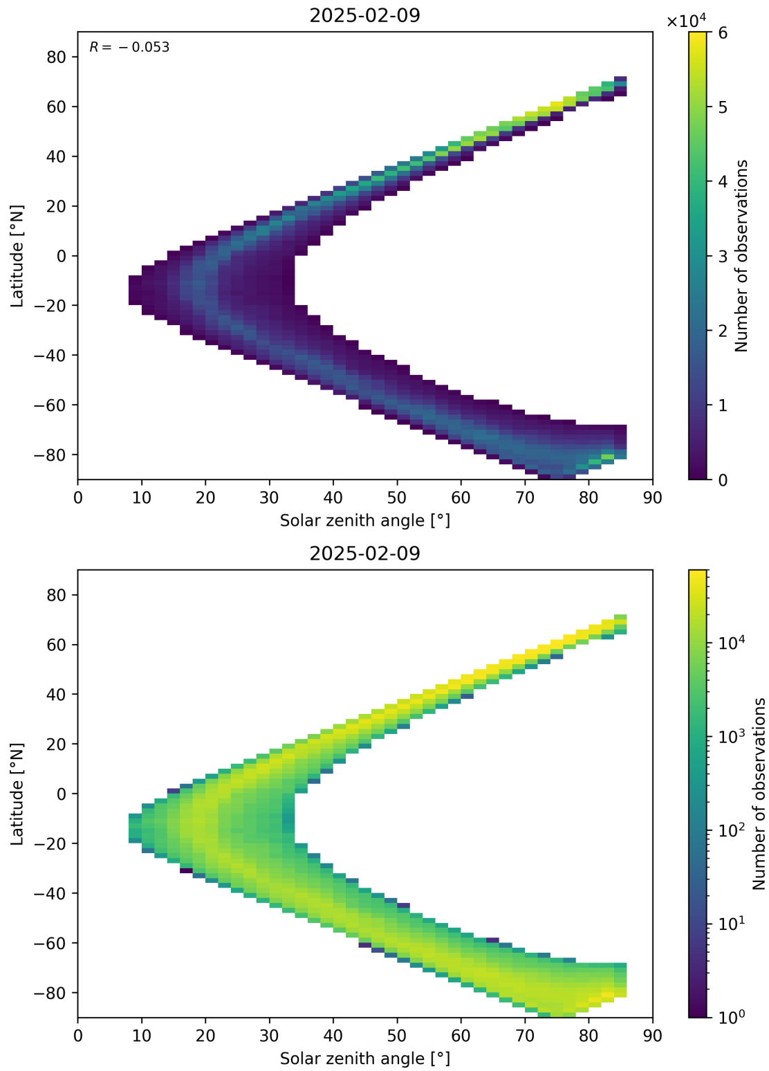
Figure 66: Scatter density plot of “Solar zenith angle” against “Latitude” for 2025-02-08 to 2025-02-10.
