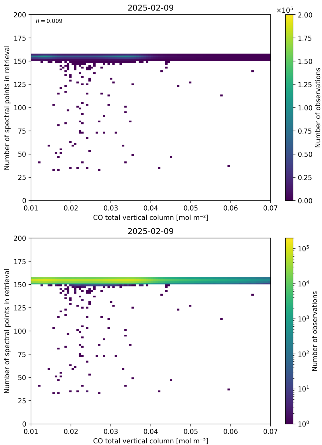
Figure 43: Scatter density plot of “CO total vertical column” against “Number of spectral points in retrieval” for 2025-02-08 to 2025-02-10.
