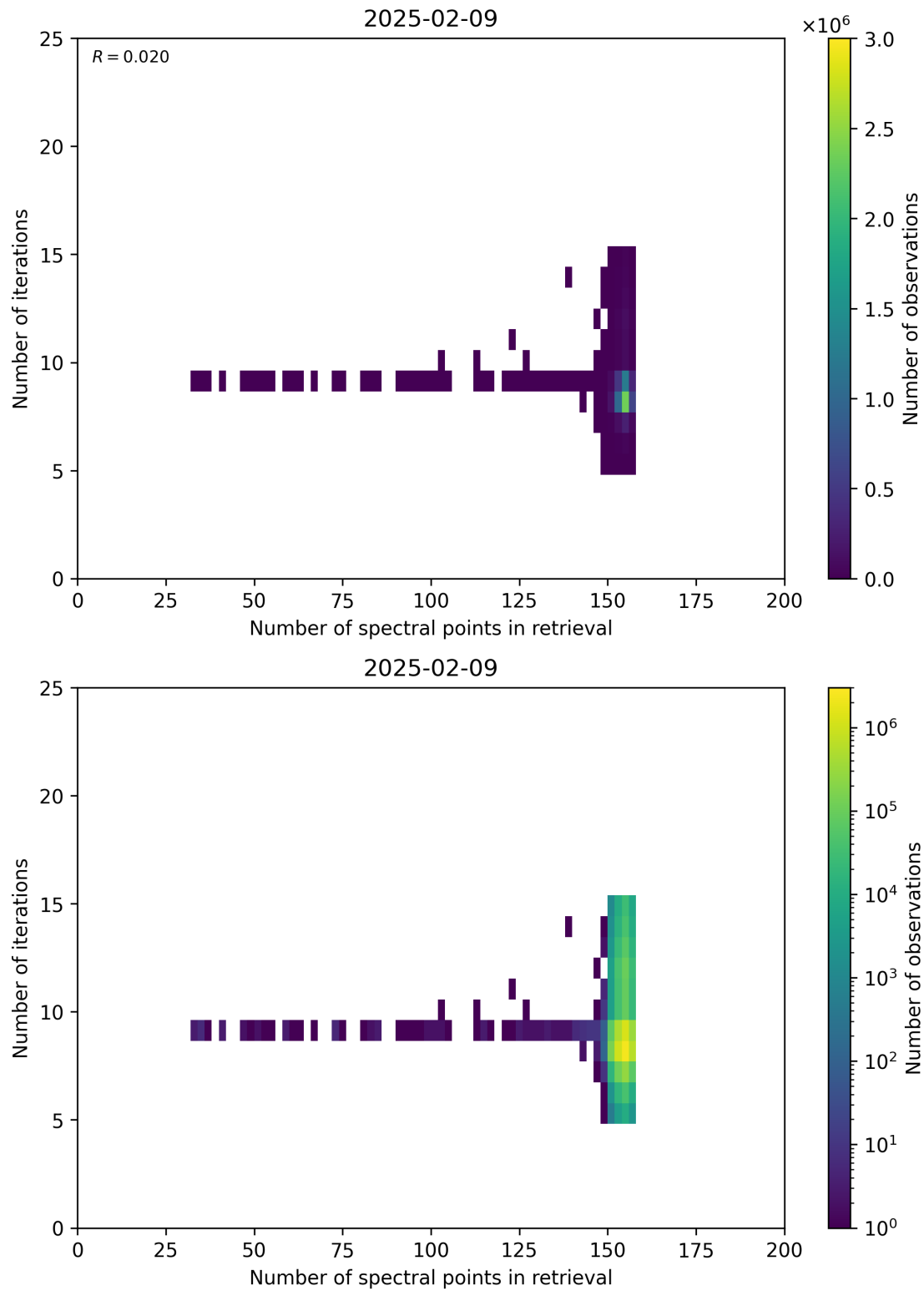
Figure 60: Scatter density plot of “Number of spectral points in retrieval” against “Number of iterations” for 2025-02-08 to 2025-02-10.
