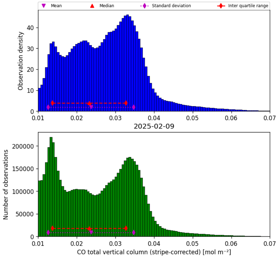
Figure 19: Histogram of “CO total vertical column (stripe-corrected)” for 2025-02-08 to 2025-02-10
