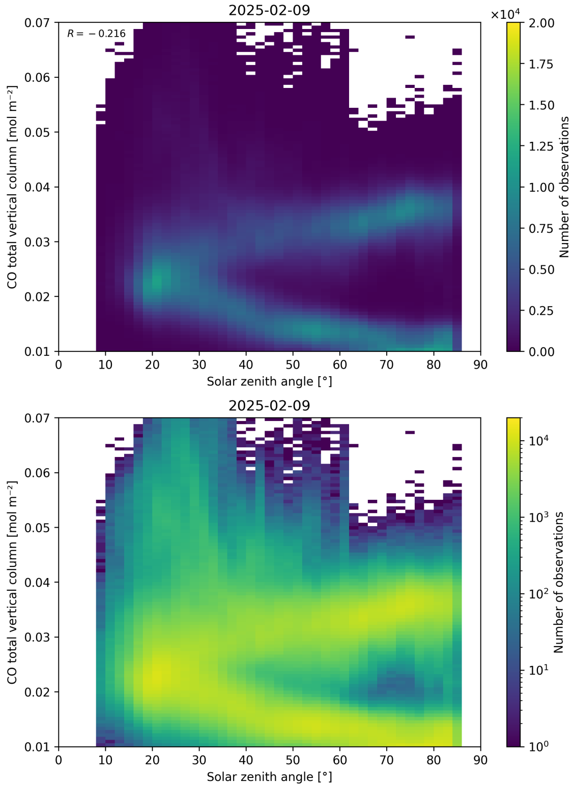
Figure 61: Scatter density plot of “Solar zenith angle” against “CO total vertical column” for 2025-02-08 to 2025-02-10.
