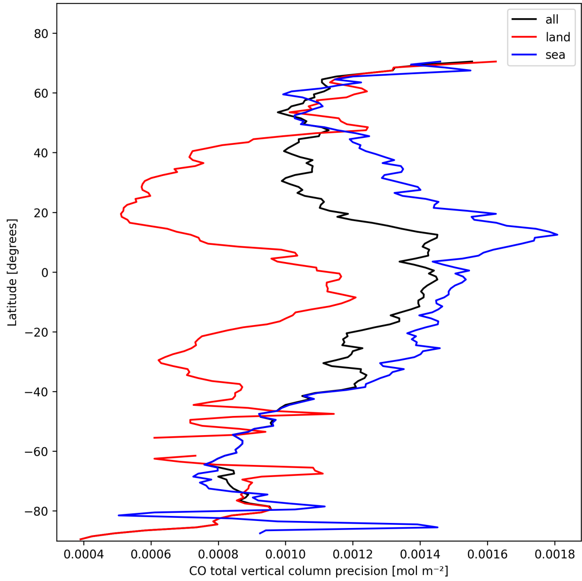
Figure 12: Zonal average of “CO total vertical column precision” for 2025-02-08 to 2025-02-10.
