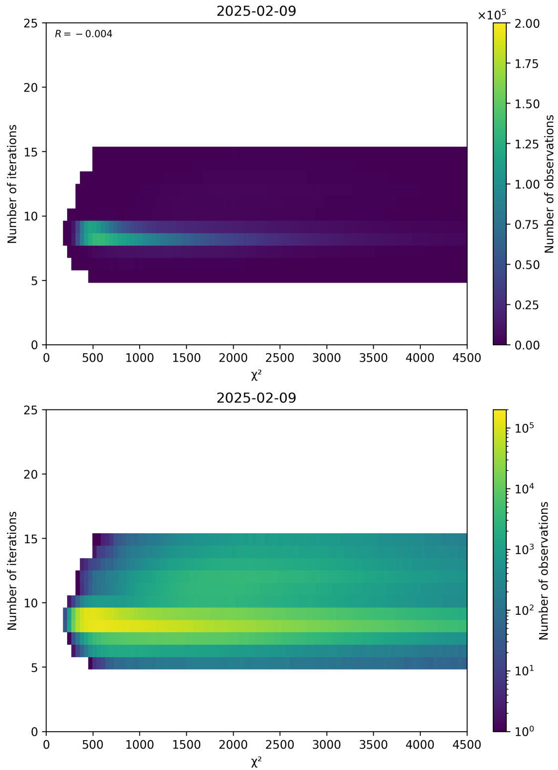
Figure 49: Scatter density plot of “ \chi^2 ” against “Number of iterations” for 2025-02-08 to 2025-02-10.
