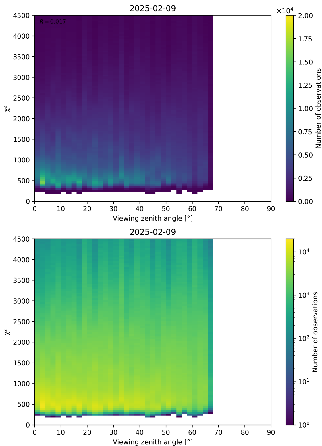
Figure 72: Scatter density plot of “Viewing zenith angle” against “ \chi^2 ” for 2025-02-08 to 2025-02-10.
