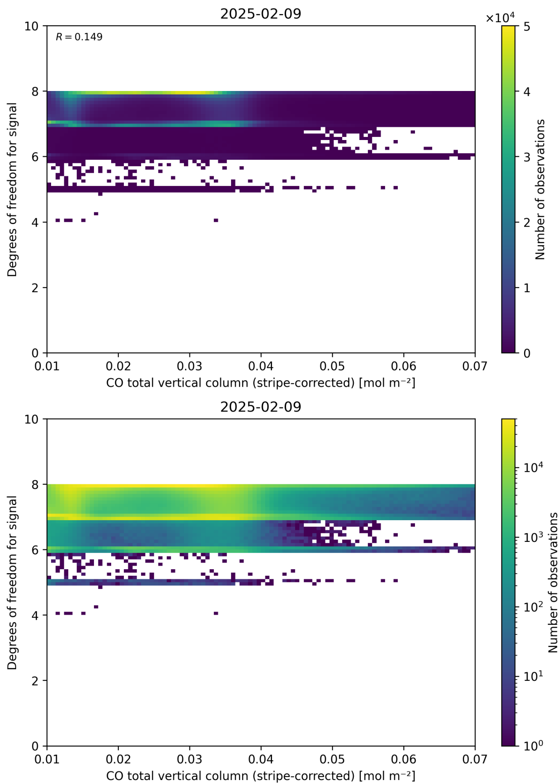
Figure 38: Scatter density plot of “CO total vertical column (stripe-corrected)” against “Degrees of freedom for signal” for 2025-02-08 to 2025-02-10.
