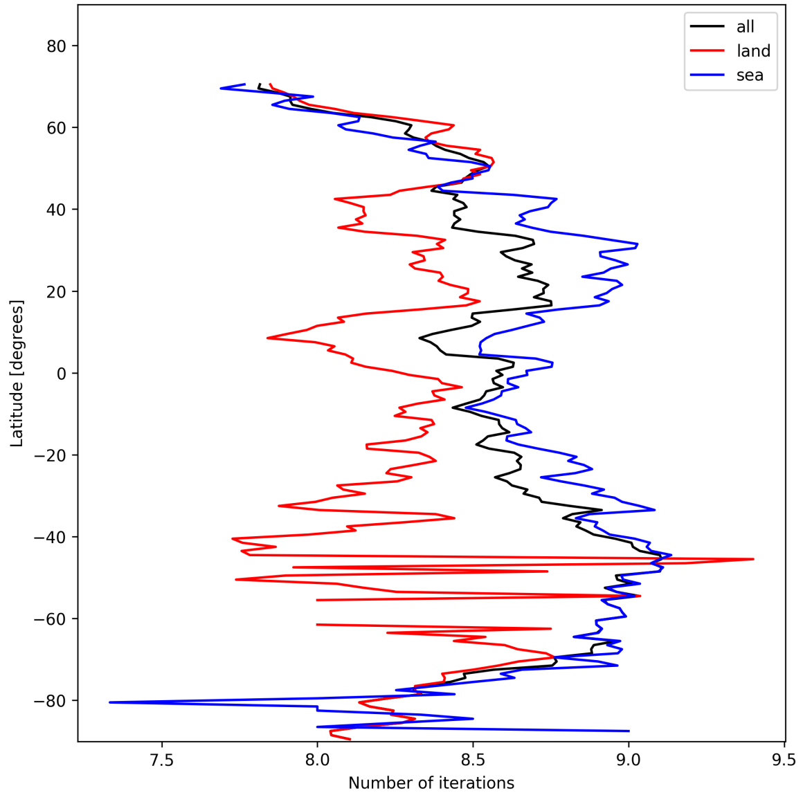
Figure 16: Zonal average of “Number of iterations” for 2025-02-08 to 2025-02-10.
