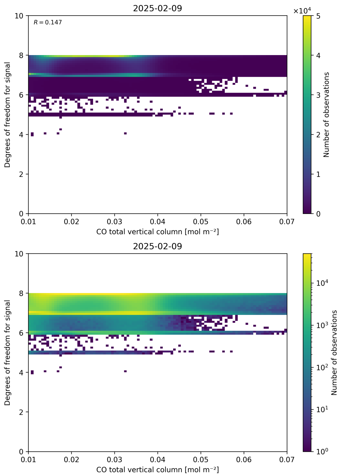
Figure 41: Scatter density plot of “CO total vertical column” against “Degrees of freedom for signal” for 2025-02-08 to 2025-02-10.
