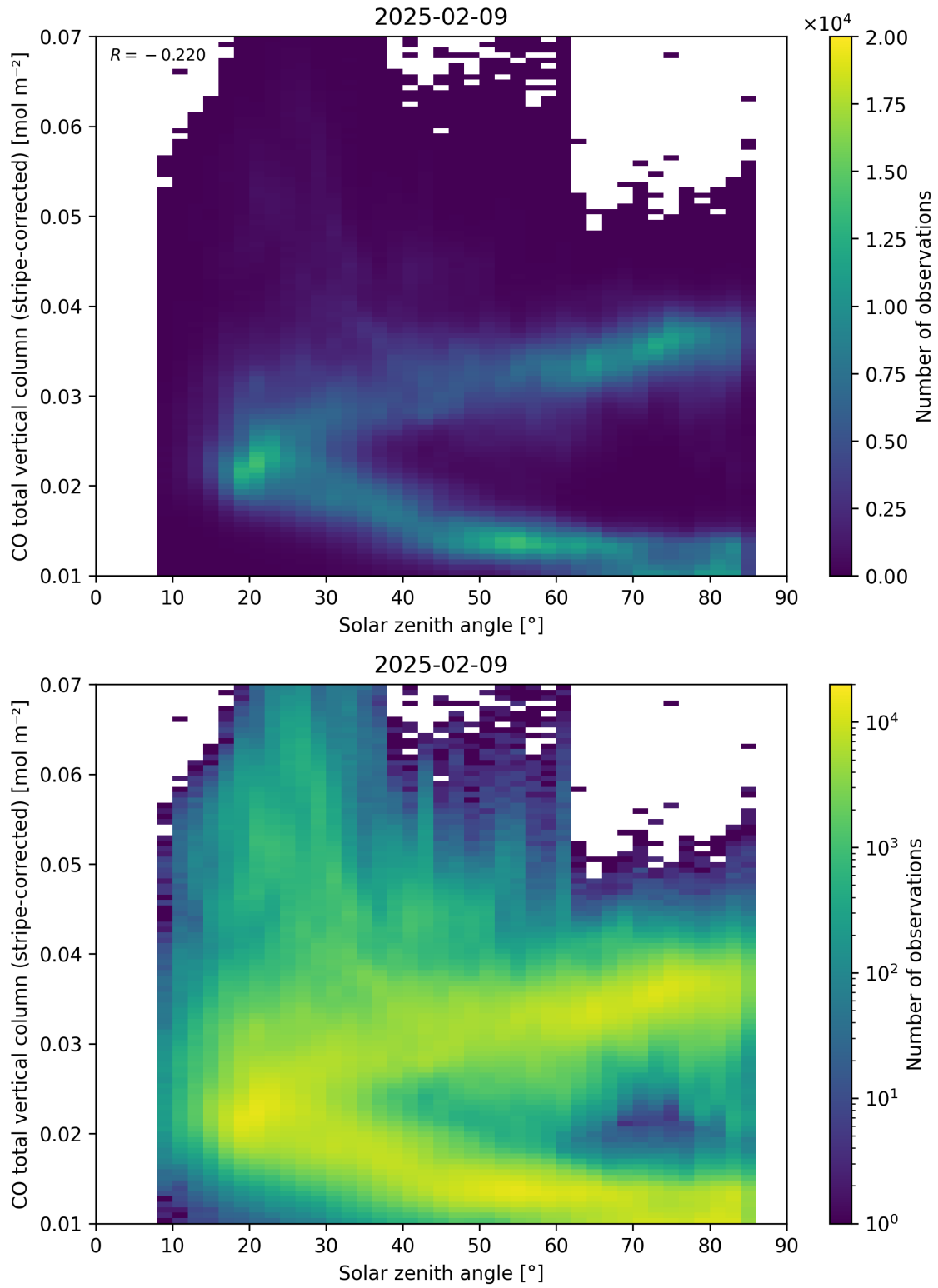
Figure 62: Scatter density plot of “Solar zenith angle” against “CO total vertical column (stripe-corrected)” for 2025-02-08 to 2025-02-10.
