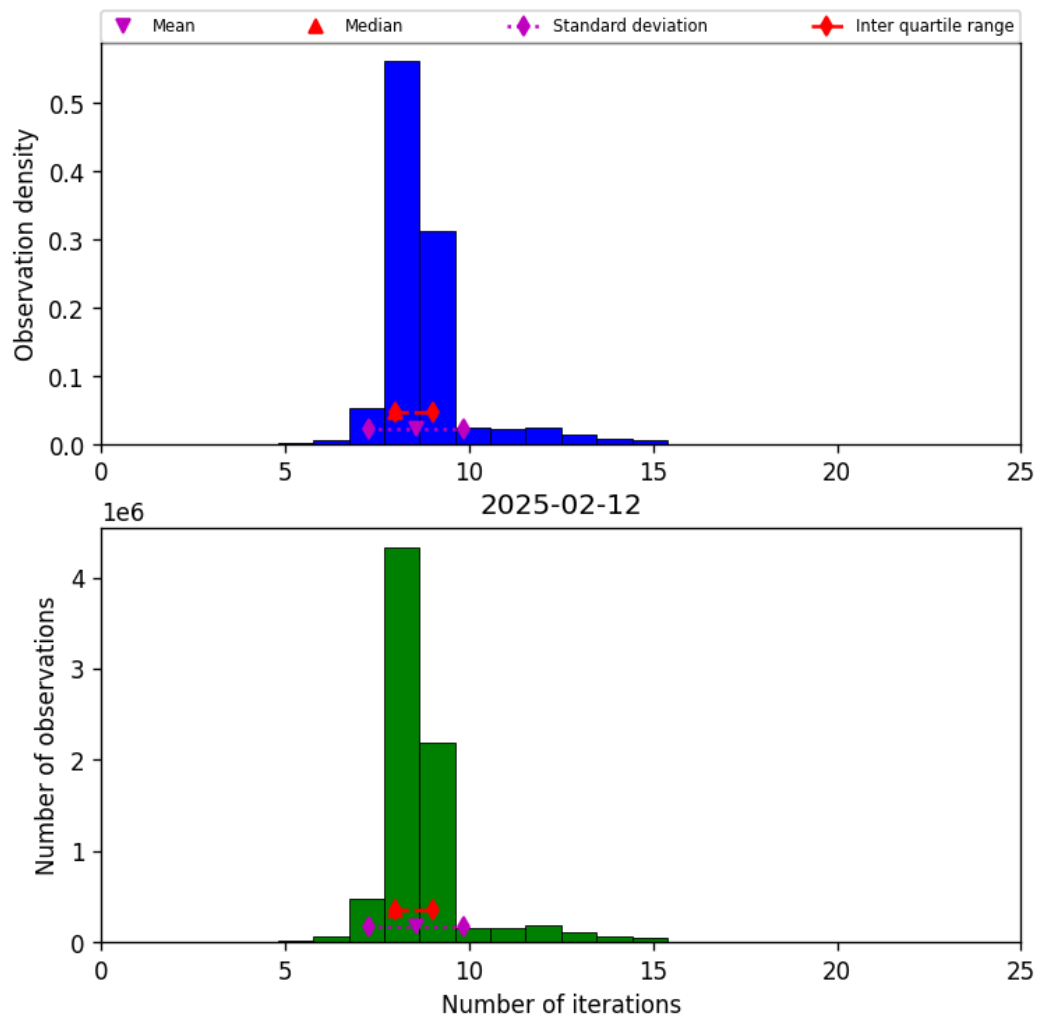
Figure 24: Histogram of “Number of iterations” for 2025-02-11 to 2025-02-13
