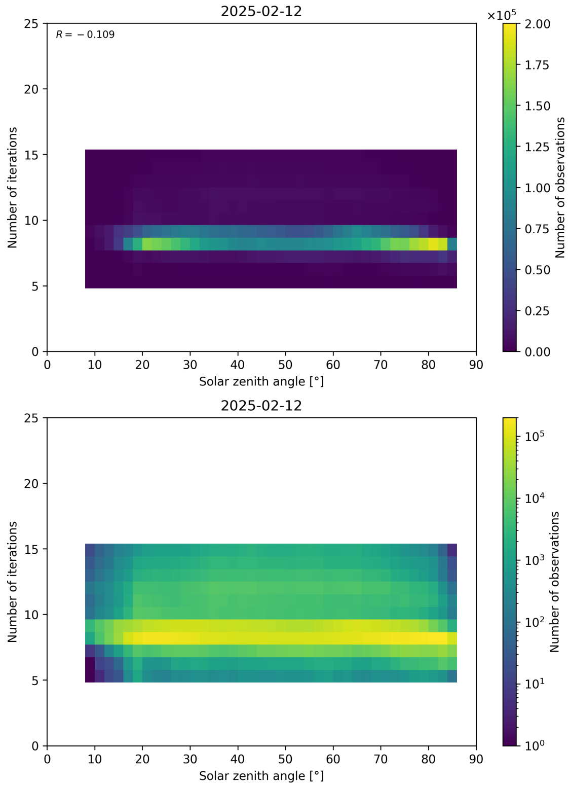
Figure 67: Scatter density plot of “Solar zenith angle” against “Number of iterations” for 2025-02-11 to 2025-02-13.
