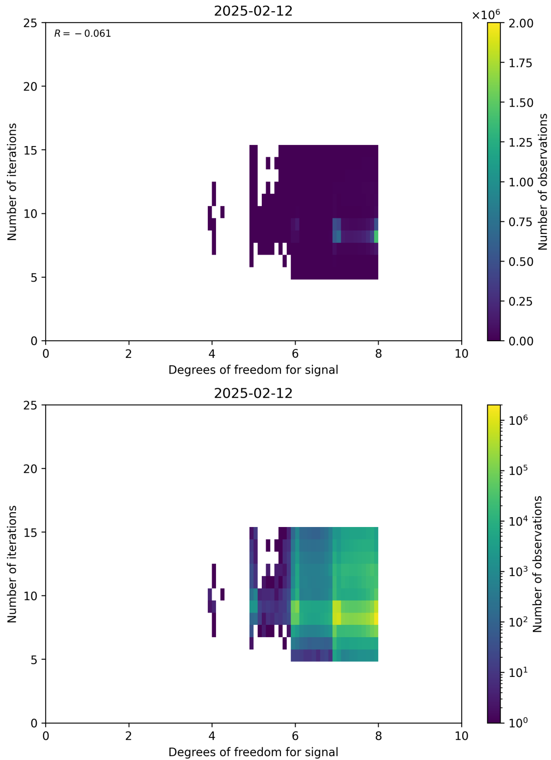
Figure 50: Scatter density plot of “Degrees of freedom for signal” against “Number of iterations” for 2025-02-11 to 2025-02-13.
