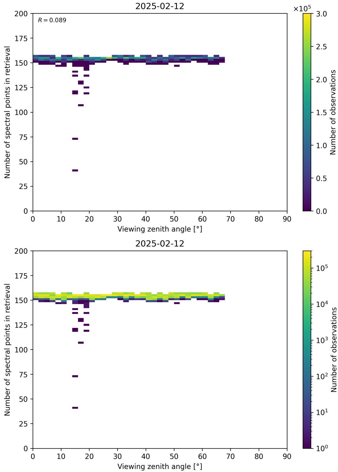
Figure 76: Scatter density plot of “Viewing zenith angle” against “Number of spectral points in retrieval” for 2025-02-11 to 2025-02-13.
