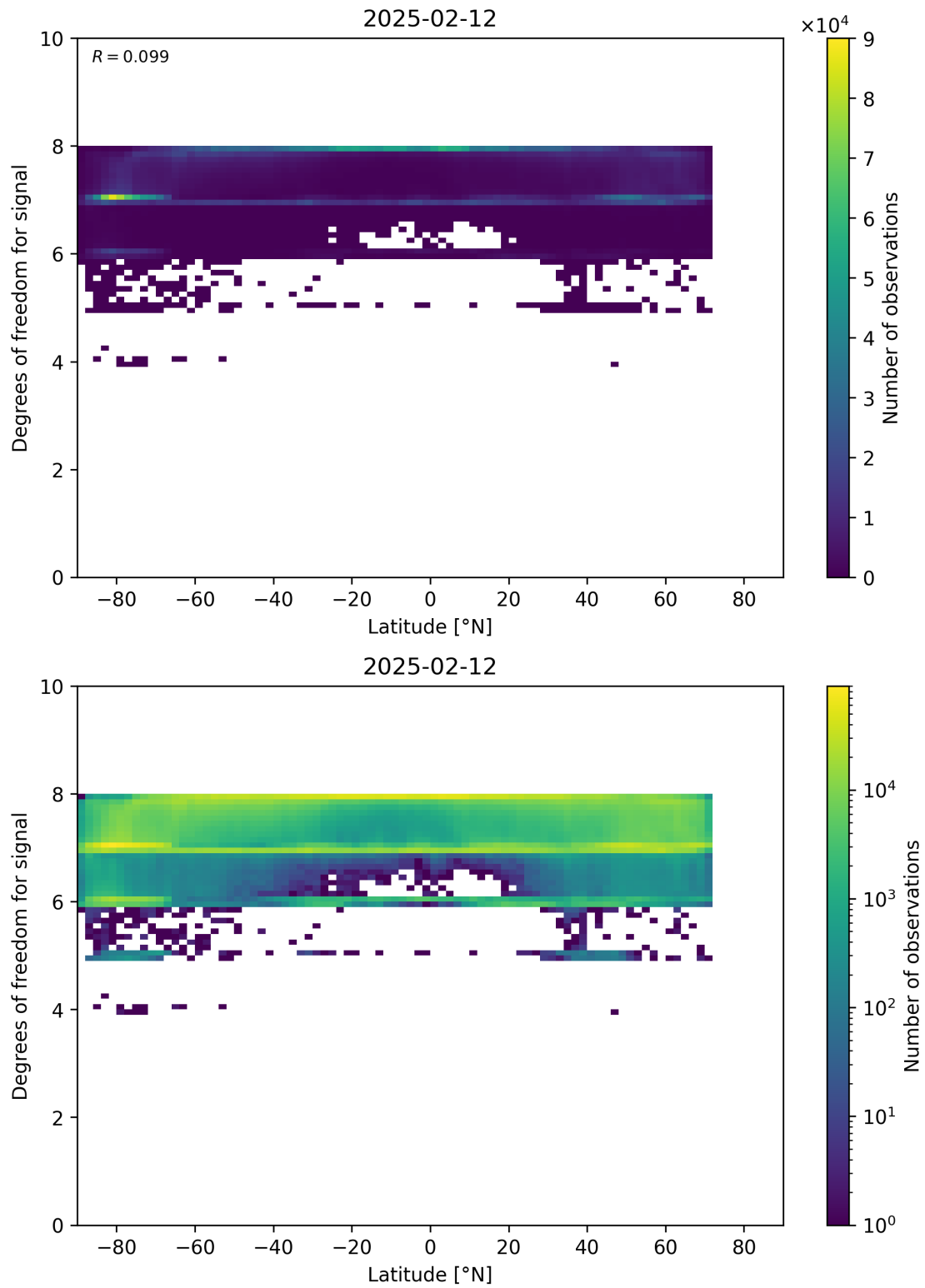
Figure 55: Scatter density plot of “Latitude” against “Degrees of freedom for signal” for 2025-02-11 to 2025-02-13.
