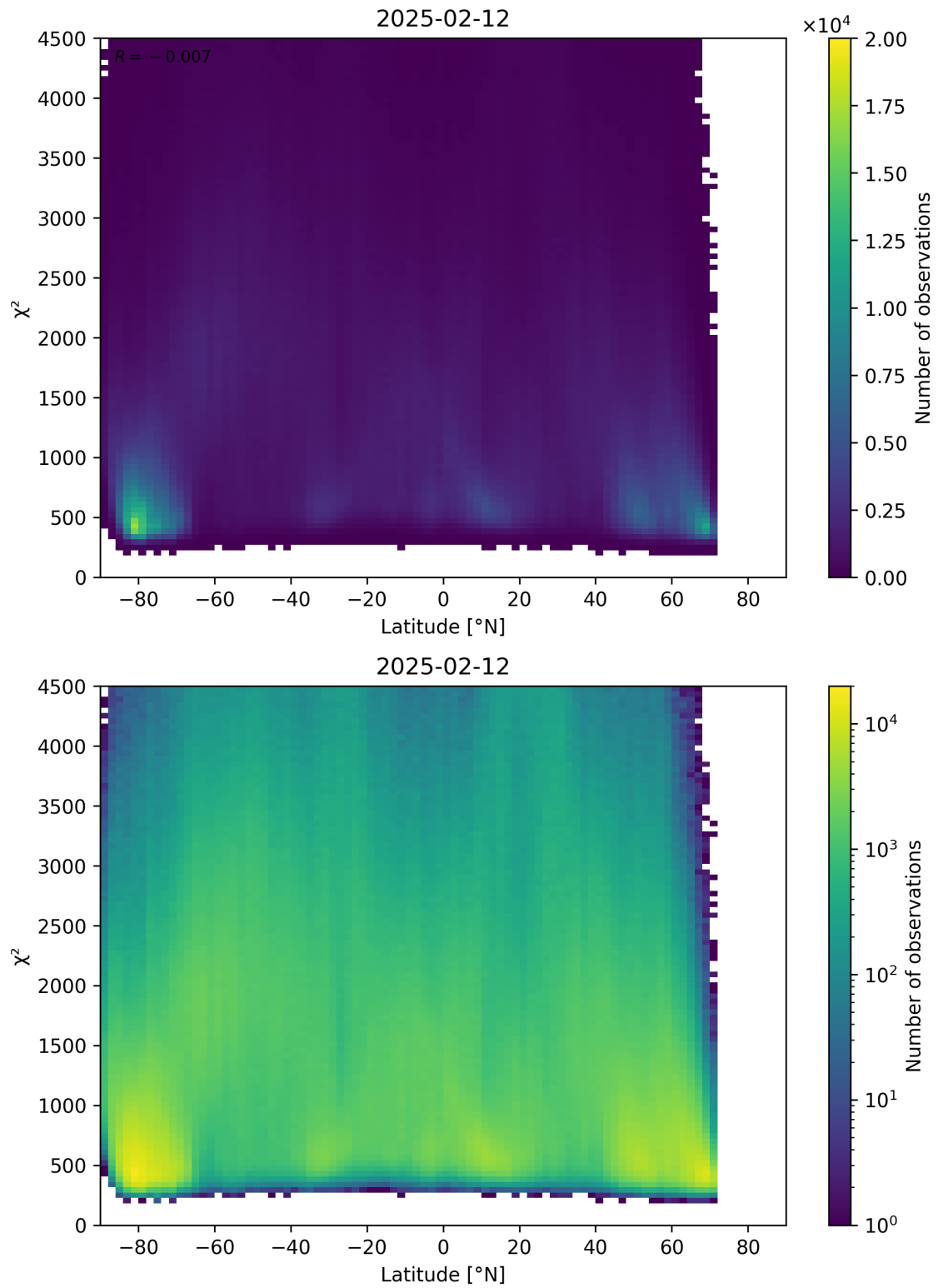
Figure 54: Scatter density plot of “Latitude” against “ \chi^2 ” for 2025-02-11 to 2025-02-13.
