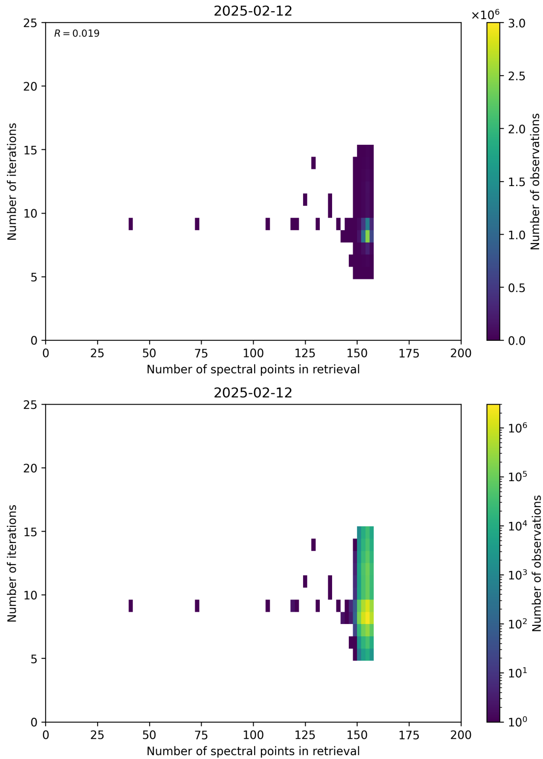
Figure 60: Scatter density plot of “Number of spectral points in retrieval” against “Number of iterations” for 2025-02-11 to 2025-02-13.
