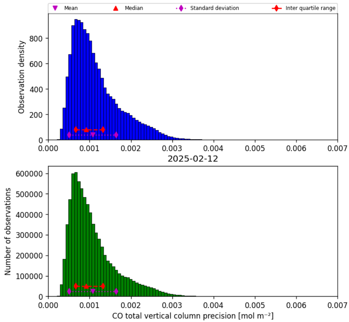
Figure 20: Histogram of “CO total vertical column precision” for 2025-02-11 to 2025-02-13
