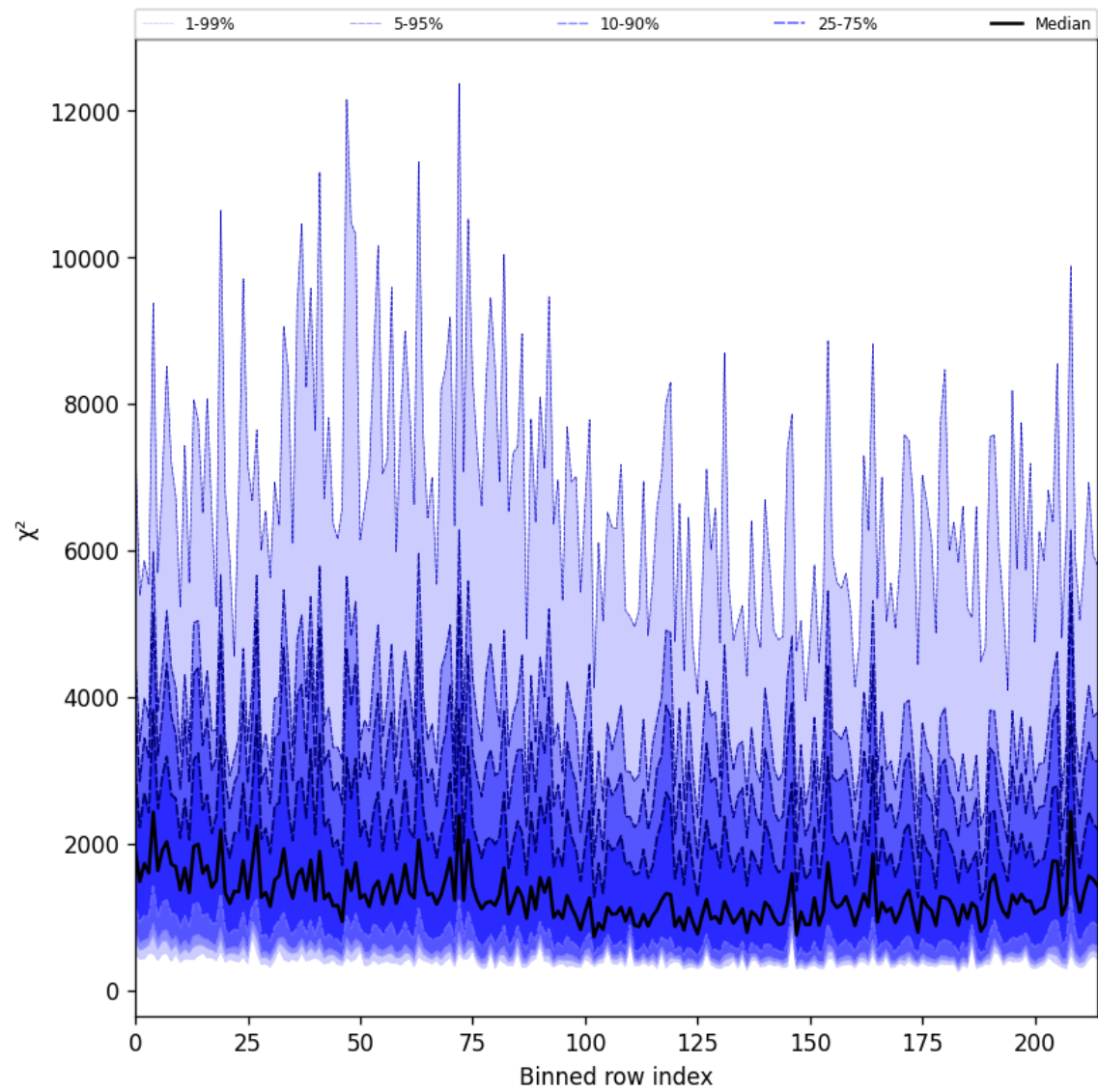
Figure 30: Along track statistics of “ \chi^2 ” for 2025-02-11 to 2025-02-13
