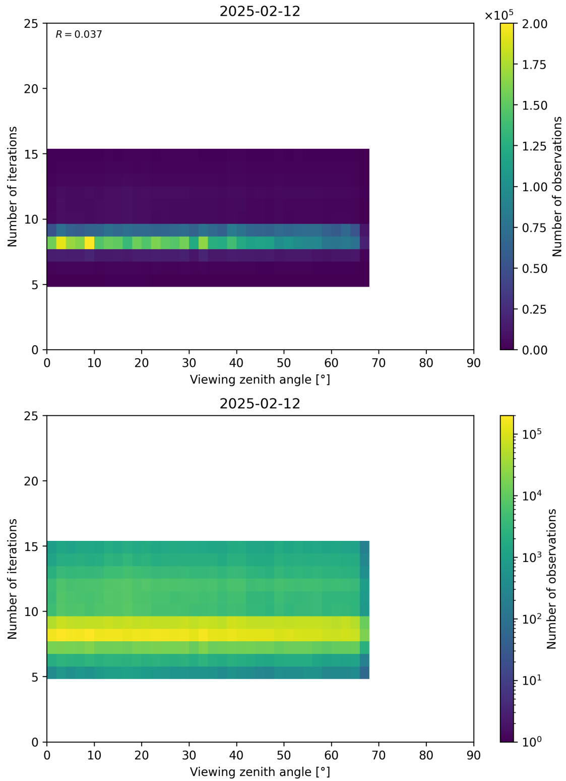
Figure 75: Scatter density plot of “Viewing zenith angle” against “Number of iterations” for 2025-02-11 to 2025-02-13.
