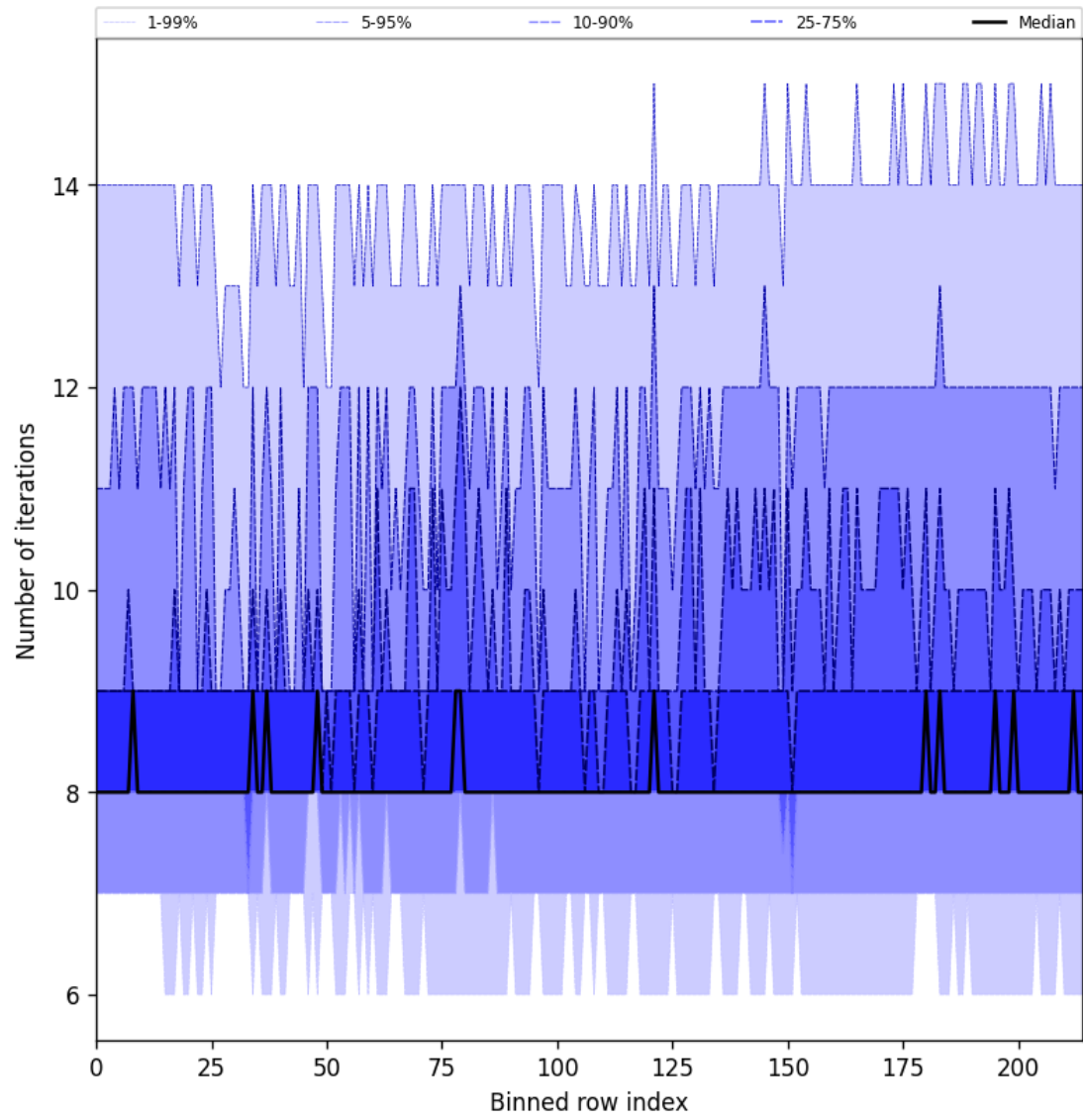
Figure 32: Along track statistics of “Number of iterations” for 2025-02-11 to 2025-02-13
