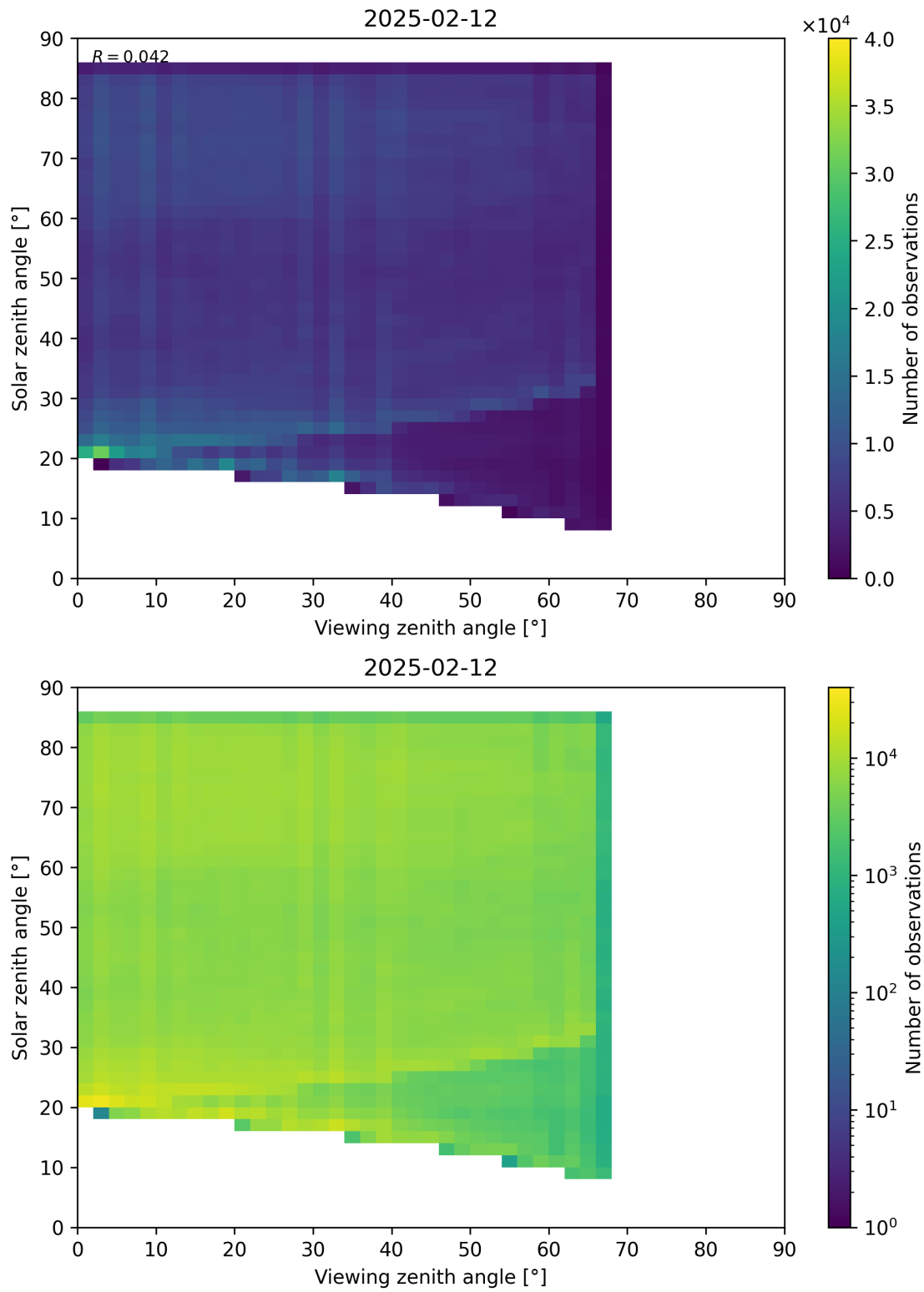
Figure 77: Scatter density plot of “Viewing zenith angle” against “Solar zenith angle” for 2025-02-11 to 2025-02-13.
