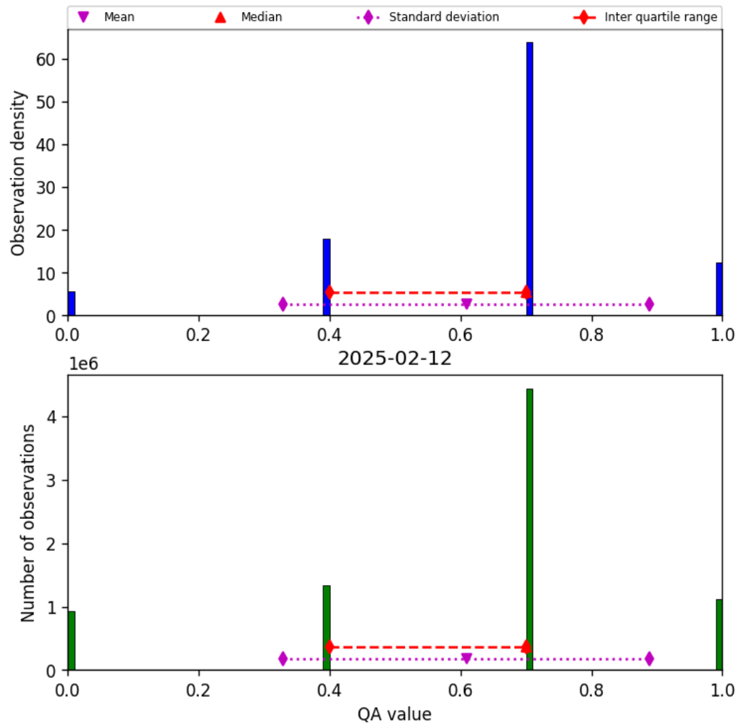
Figure 17: Histogram of “QA value” for 2025-02-11 to 2025-02-13
