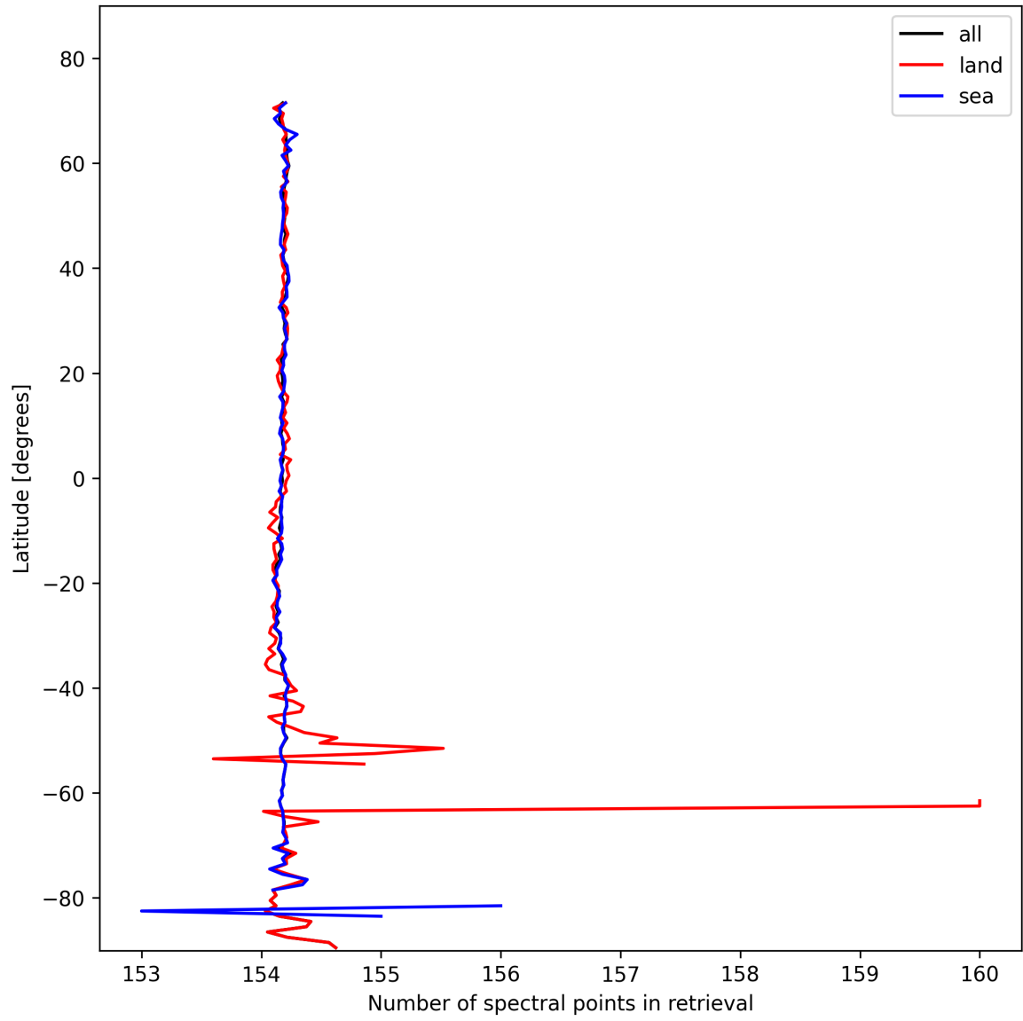
Figure 13: Zonal average of “Number of spectral points in retrieval” for 2025-02-11 to 2025-02-13.
