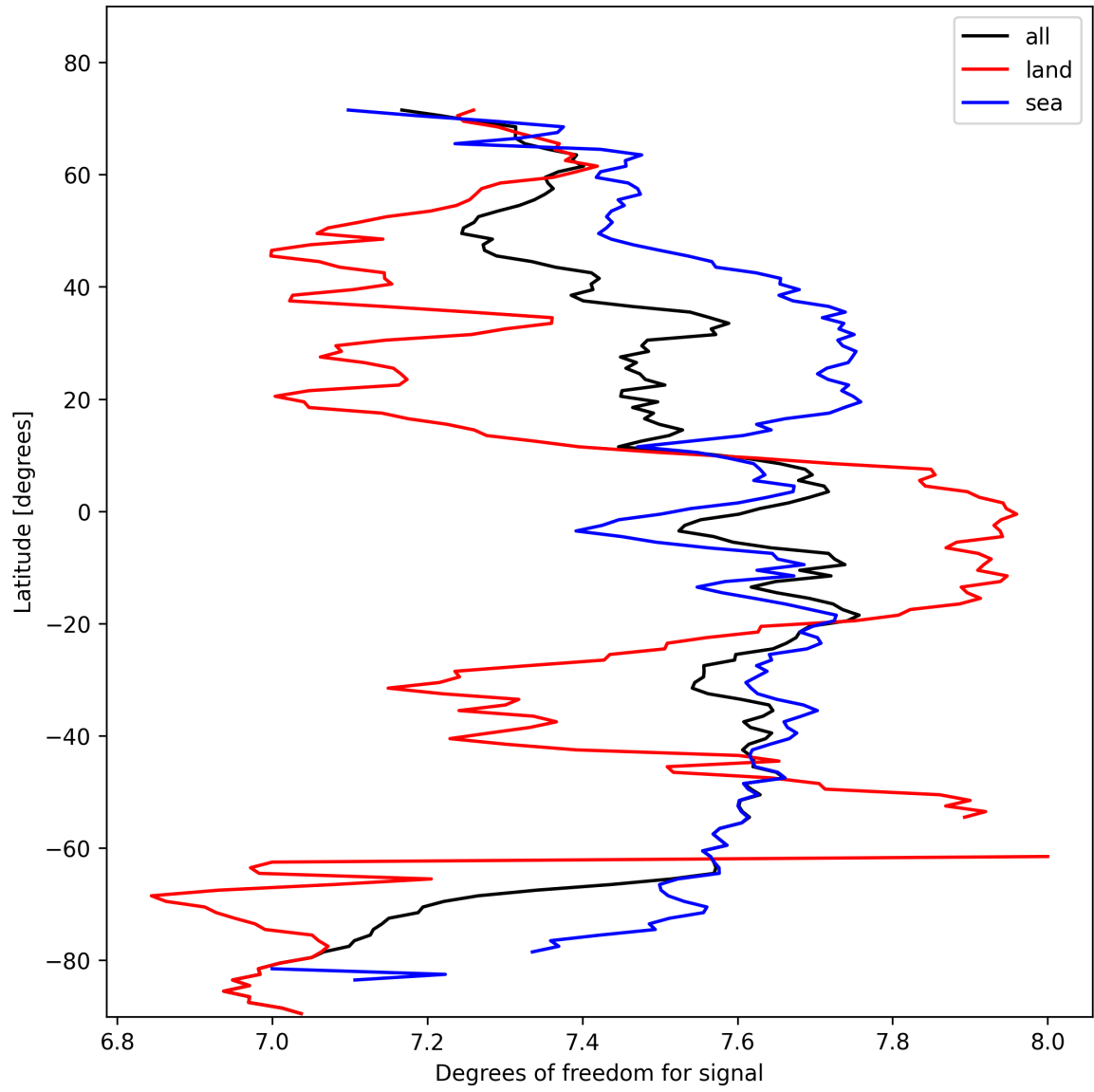
Figure 15: Zonal average of “Degrees of freedom for signal” for 2025-02-11 to 2025-02-13.
