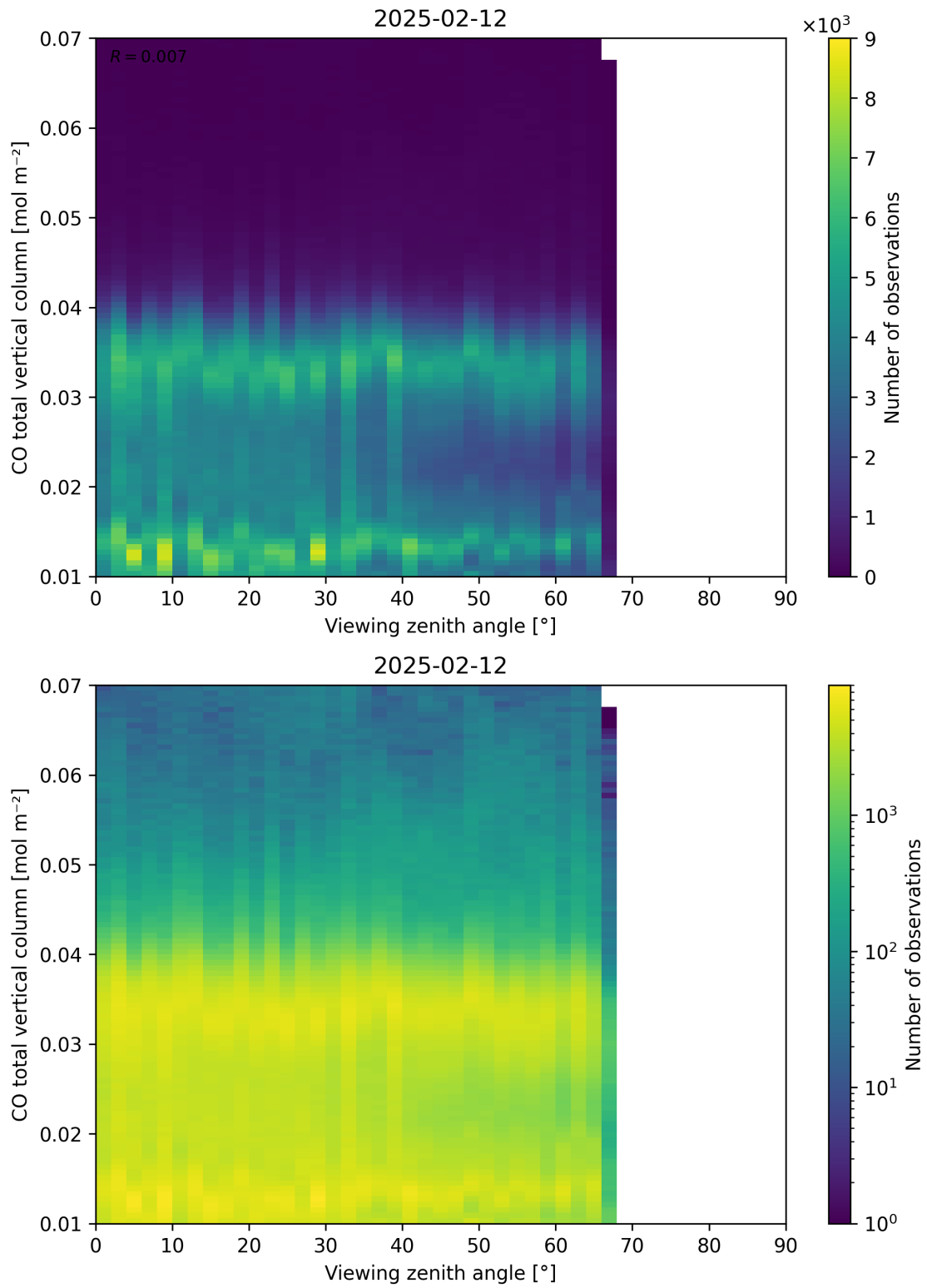
Figure 69: Scatter density plot of “Viewing zenith angle” against “CO total vertical column” for 2025-02-11 to 2025-02-13.
