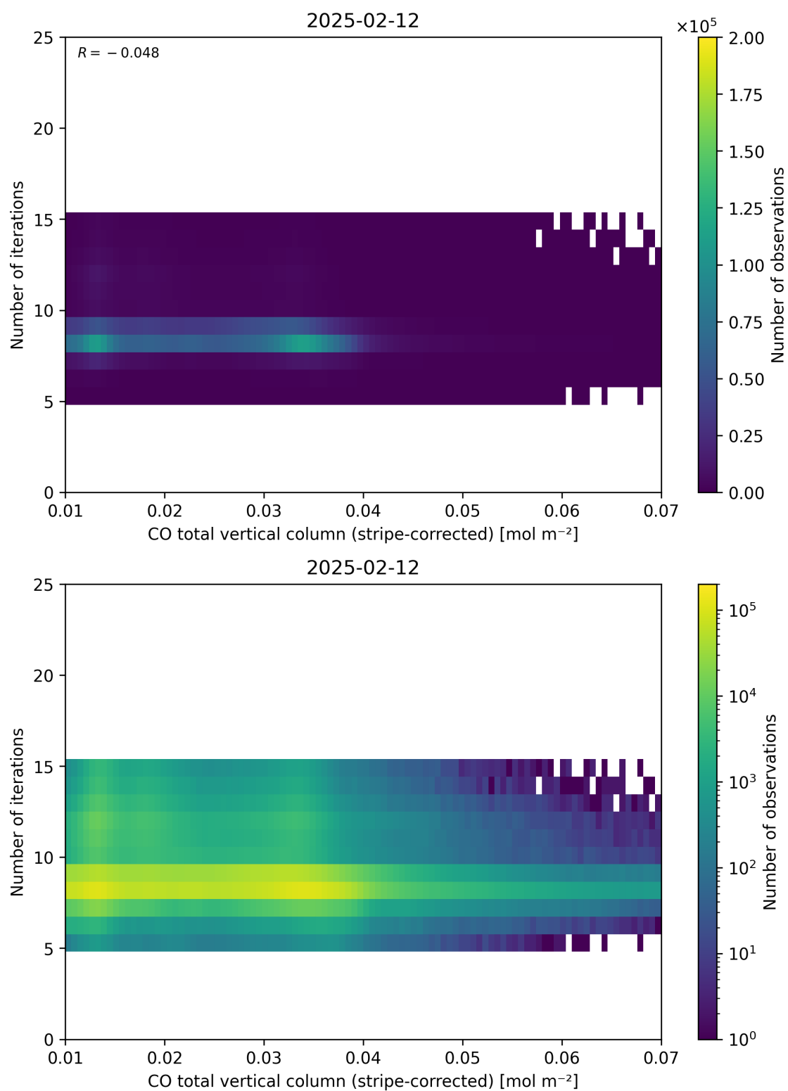
Figure 39: Scatter density plot of “CO total vertical column (stripe-corrected)” against “Number of iterations” for 2025-02-11 to 2025-02-13.
