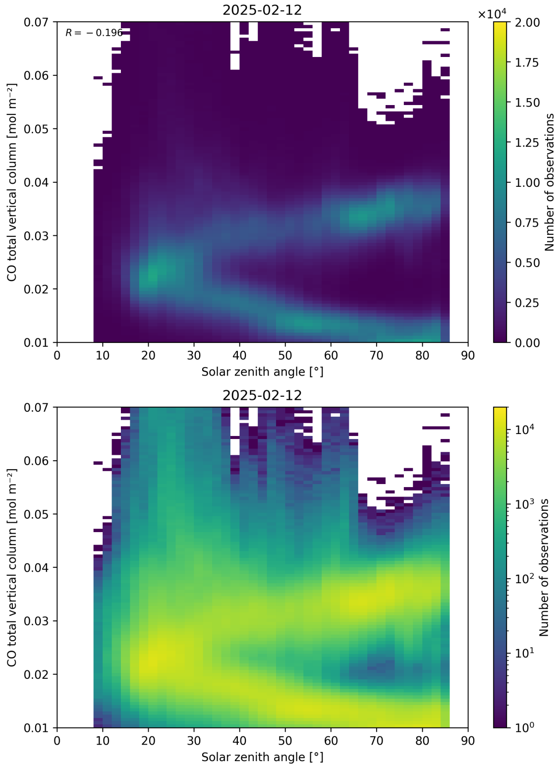
Figure 61: Scatter density plot of “Solar zenith angle” against “CO total vertical column” for 2025-02-11 to 2025-02-13.
