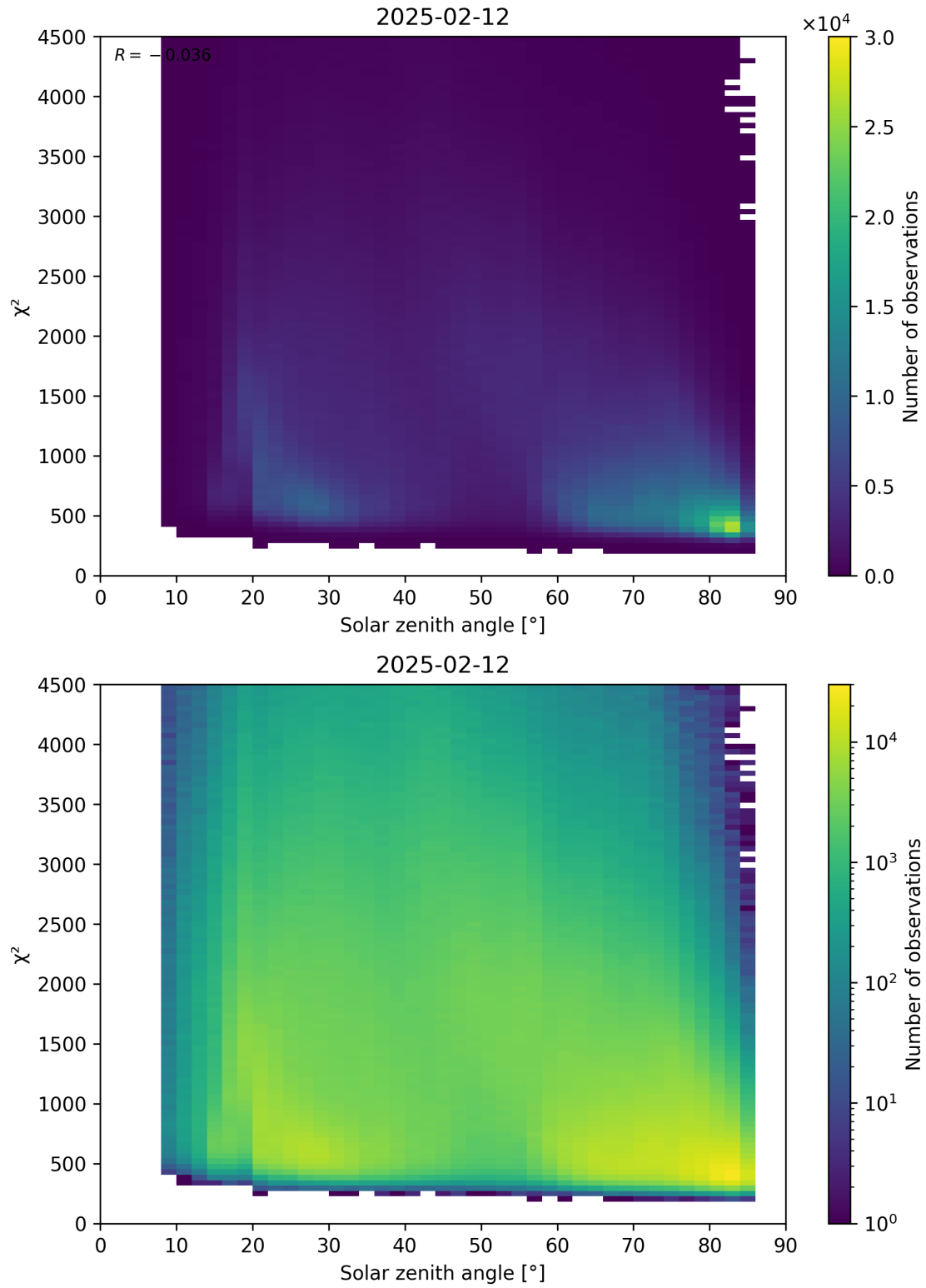
Figure 64: Scatter density plot of “Solar zenith angle” against “ \chi^2 ” for 2025-02-11 to 2025-02-13.
