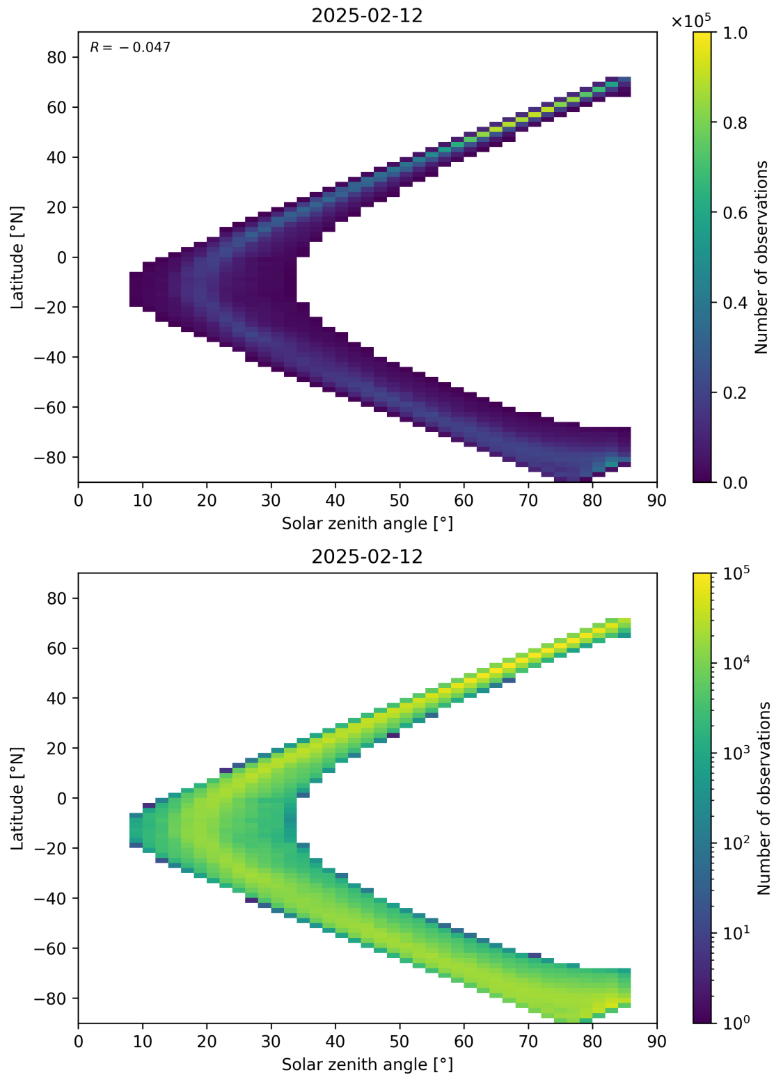
Figure 66: Scatter density plot of “Solar zenith angle” against “Latitude” for 2025-02-11 to 2025-02-13.
