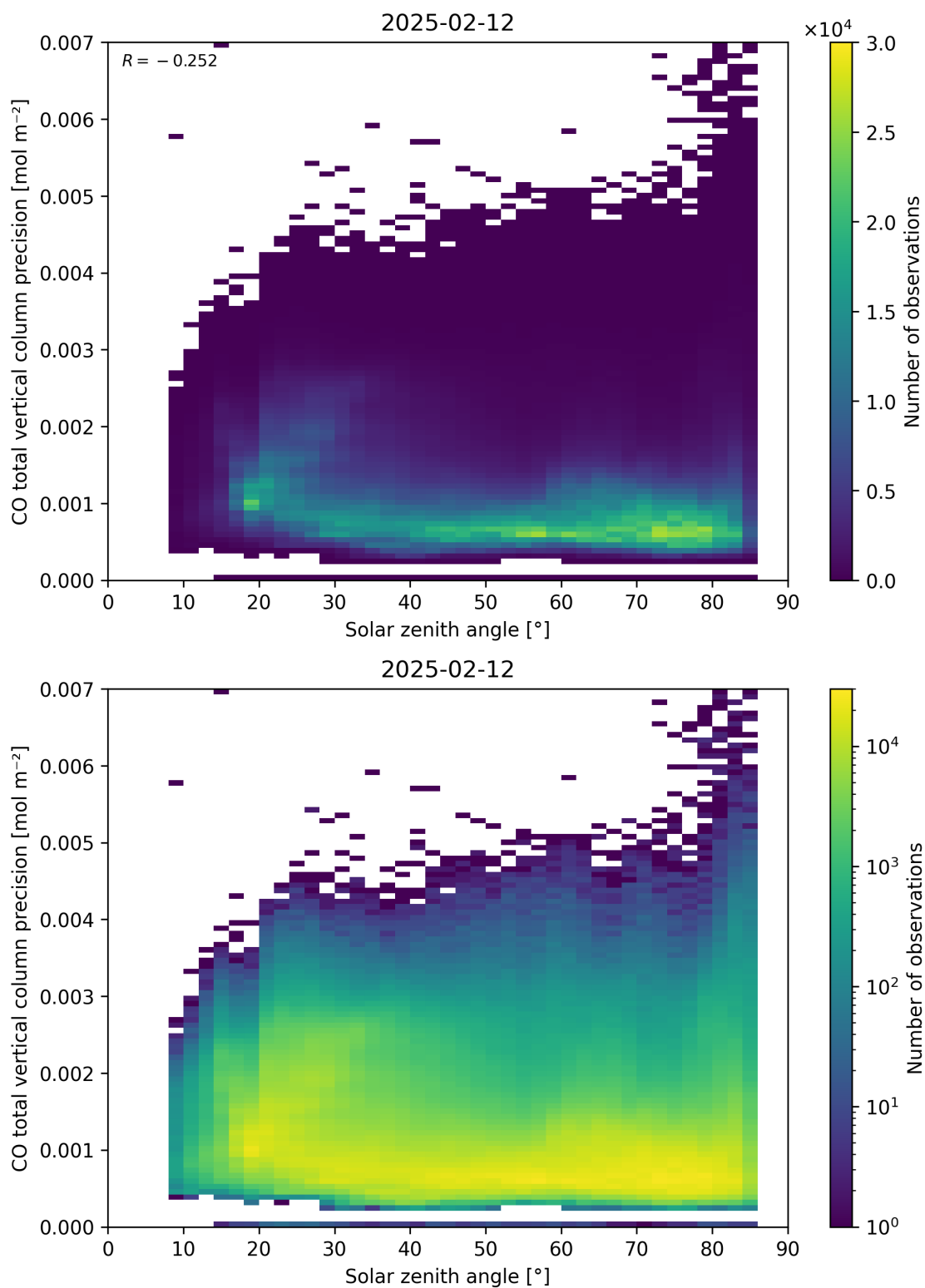
Figure 63: Scatter density plot of “Solar zenith angle” against “CO total vertical column precision” for 2025-02-11 to 2025-02-13.
