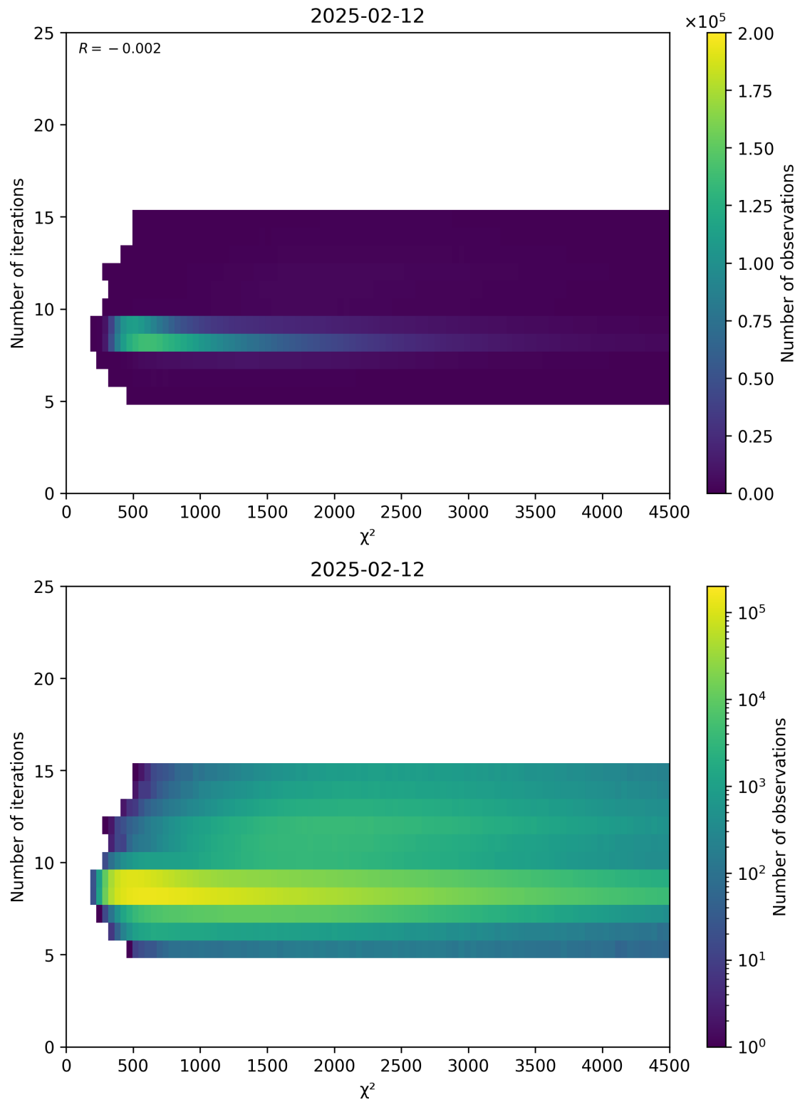
Figure 49: Scatter density plot of “ \chi^2 ” against “Number of iterations” for 2025-02-11 to 2025-02-13.
