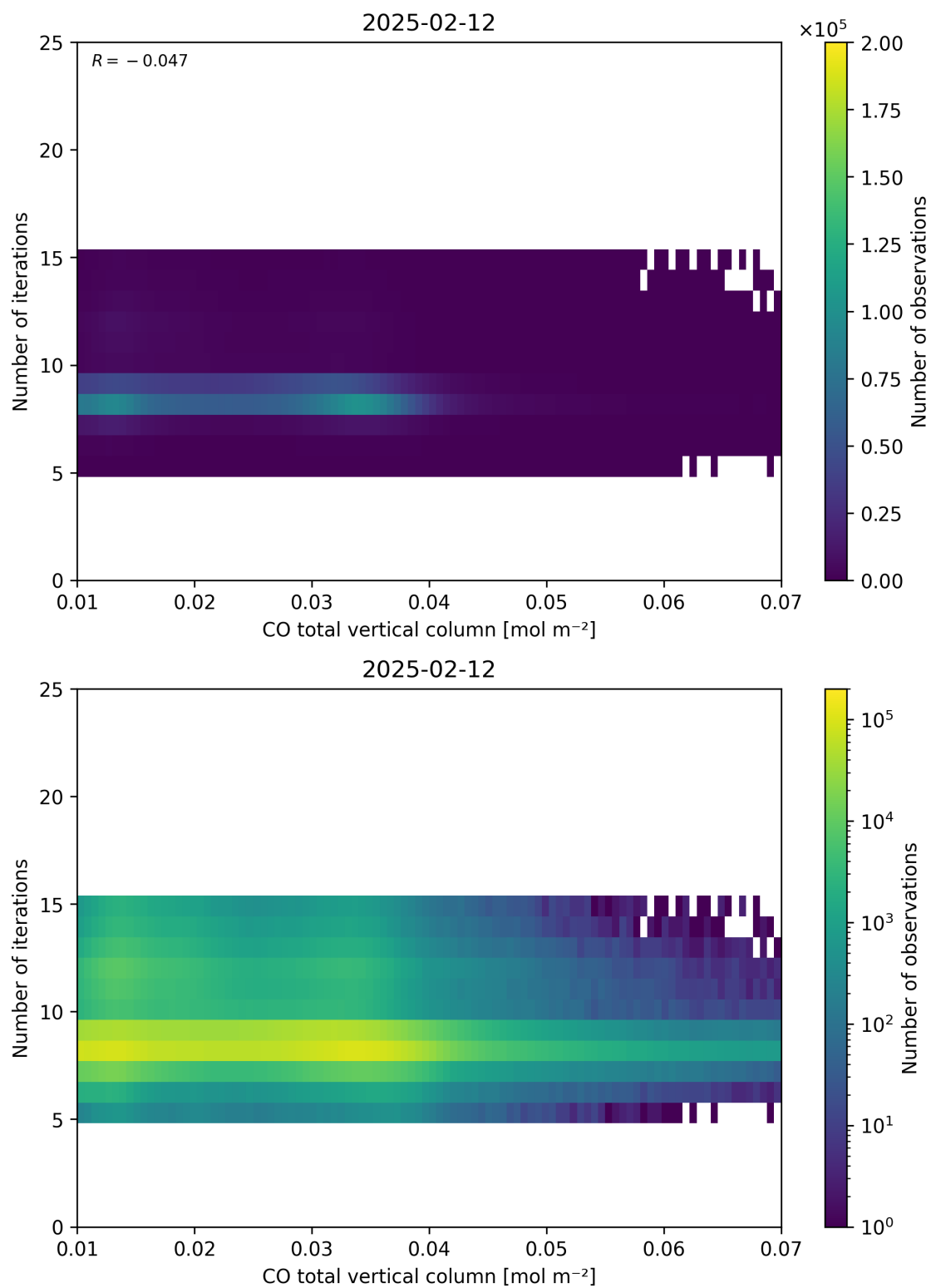
Figure 42: Scatter density plot of “CO total vertical column” against “Number of iterations” for 2025-02-11 to 2025-02-13.
