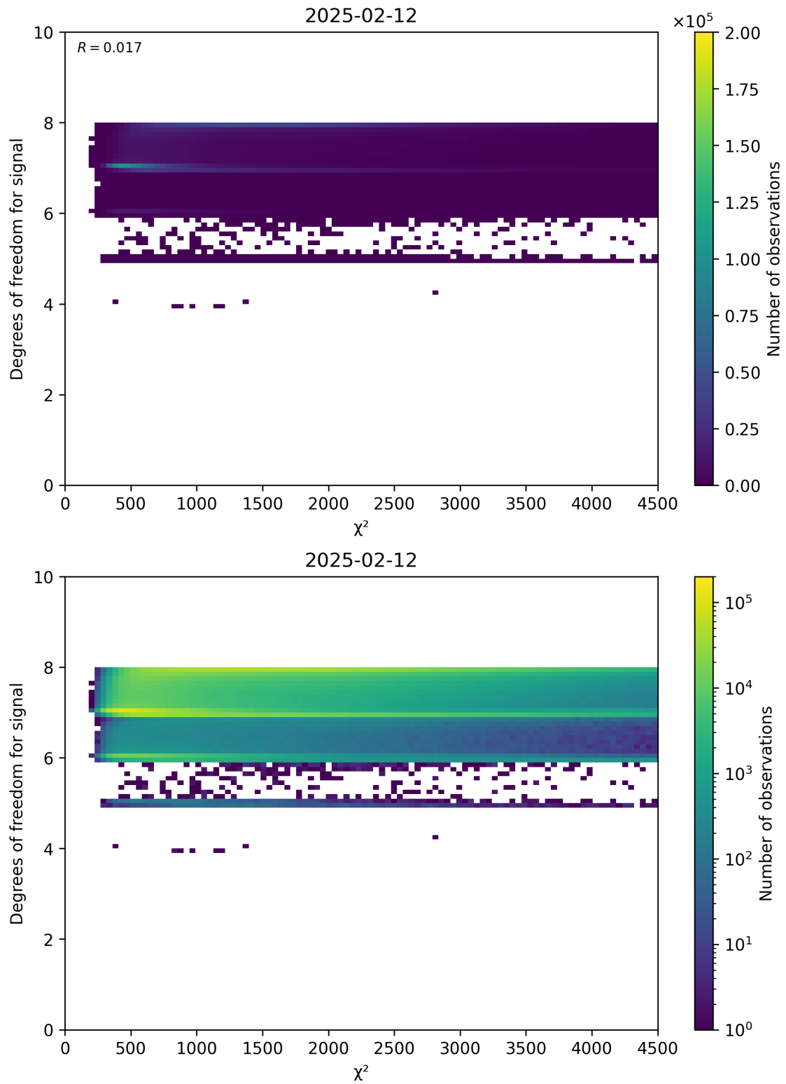
Figure 48: Scatter density plot of “ \chi^2 ” against “Degrees of freedom for signal” for 2025-02-11 to 2025-02-13.
