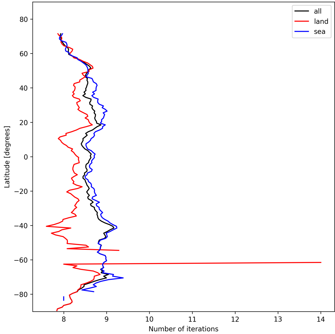
Figure 16: Zonal average of “Number of iterations” for 2025-02-11 to 2025-02-13.
