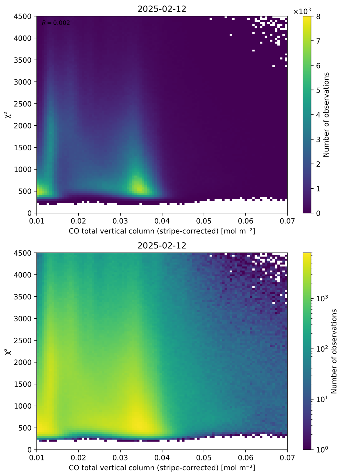
Figure 37: Scatter density plot of “CO total vertical column (stripe-corrected)” against “ \chi^2 ” for 2025-02-11 to 2025-02-13.
