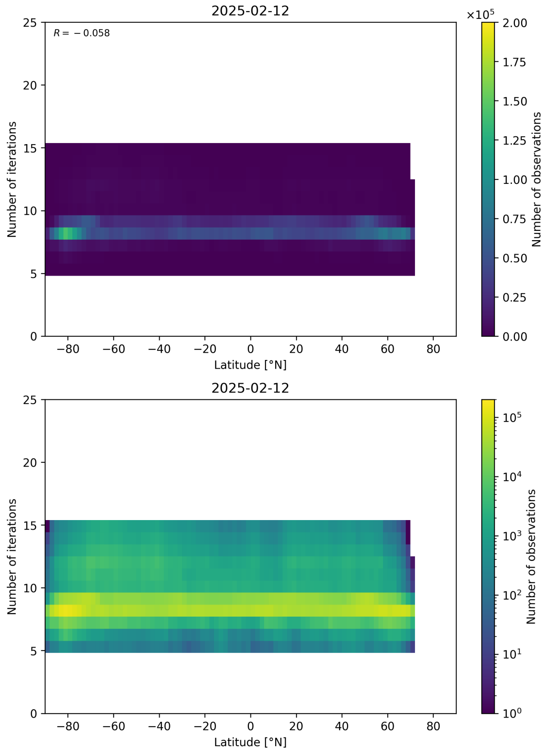
Figure 56: Scatter density plot of “Latitude” against “Number of iterations” for 2025-02-11 to 2025-02-13.
