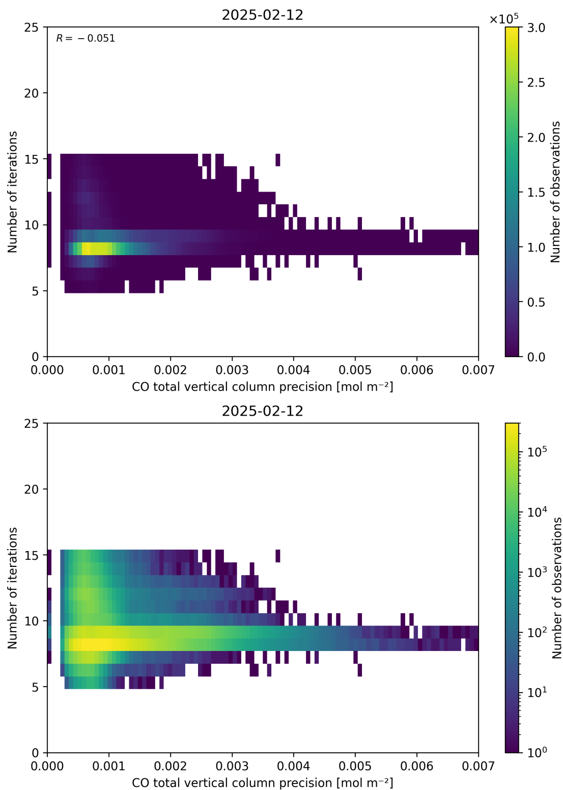
Figure 46: Scatter density plot of “CO total vertical column precision” against “Number of iterations” for 2025-02-11 to 2025-02-13.
