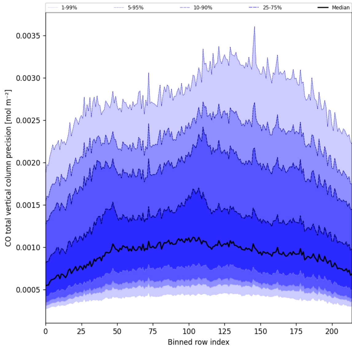
Figure 28: Along track statistics of “CO total vertical column precision” for 2025-02-11 to 2025-02-13
