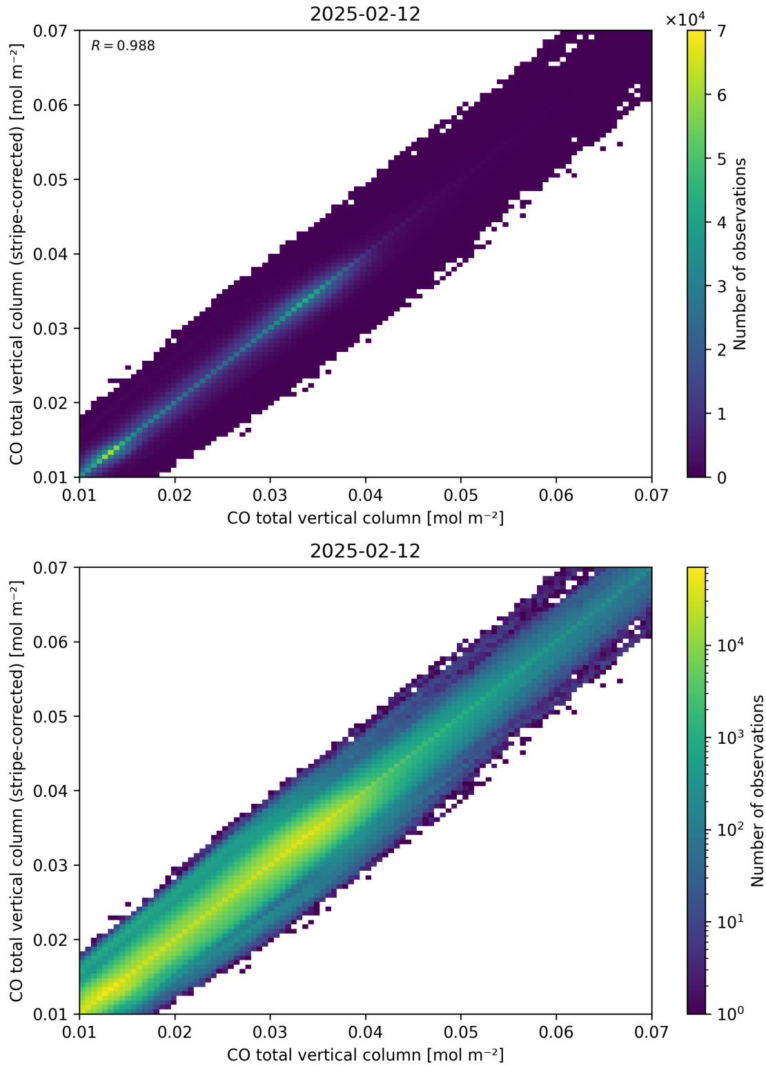
Figure 33: Scatter density plot of “CO total vertical column” against “CO total vertical column (stripe-corrected)” for 2025-02-11 to 2025-02-13.
