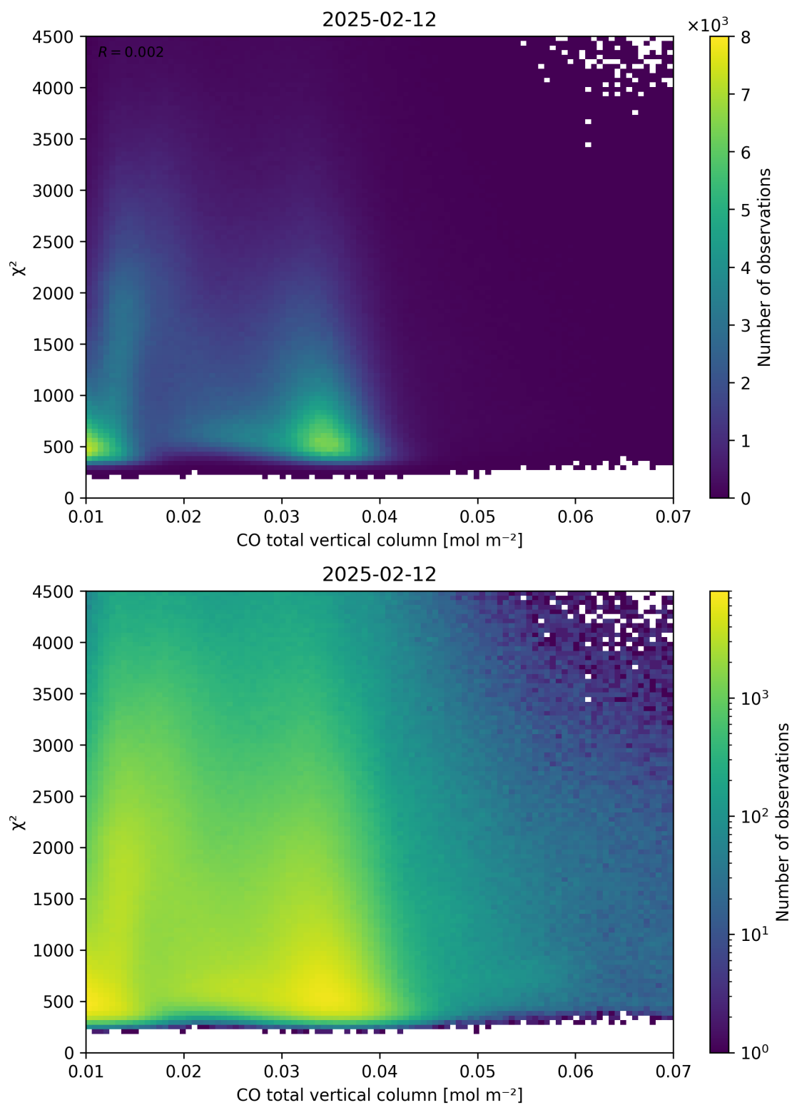
Figure 35: Scatter density plot of “CO total vertical column” against “ \chi^2 ” for 2025-02-11 to 2025-02-13.
