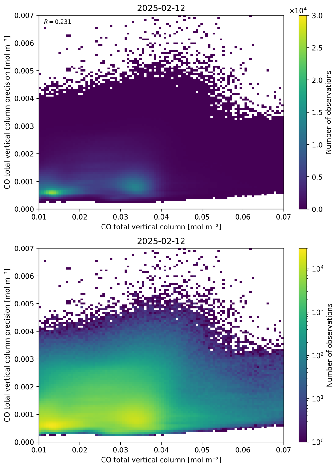
Figure 34: Scatter density plot of “CO total vertical column” against “CO total vertical column precision” for 2025-02-11 to 2025-02-13.
