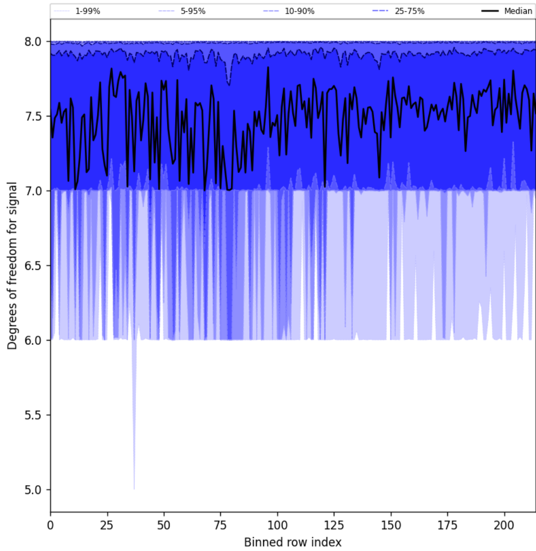
Figure 31: Along track statistics of “Degrees of freedom for signal” for 2025-02-11 to 2025-02-13
