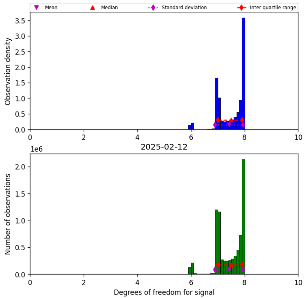
Figure 23: Histogram of “Degrees of freedom for signal” for 2025-02-11 to 2025-02-13
