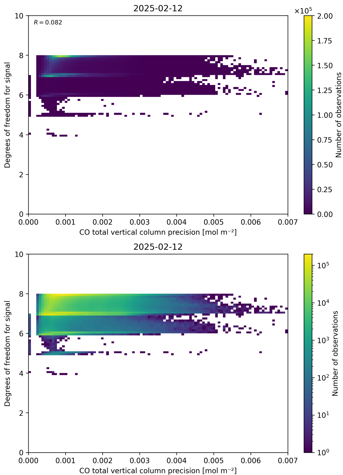
Figure 45: Scatter density plot of “CO total vertical column precision” against “Degrees of freedom for signal” for 2025-02-11 to 2025-02-13.
