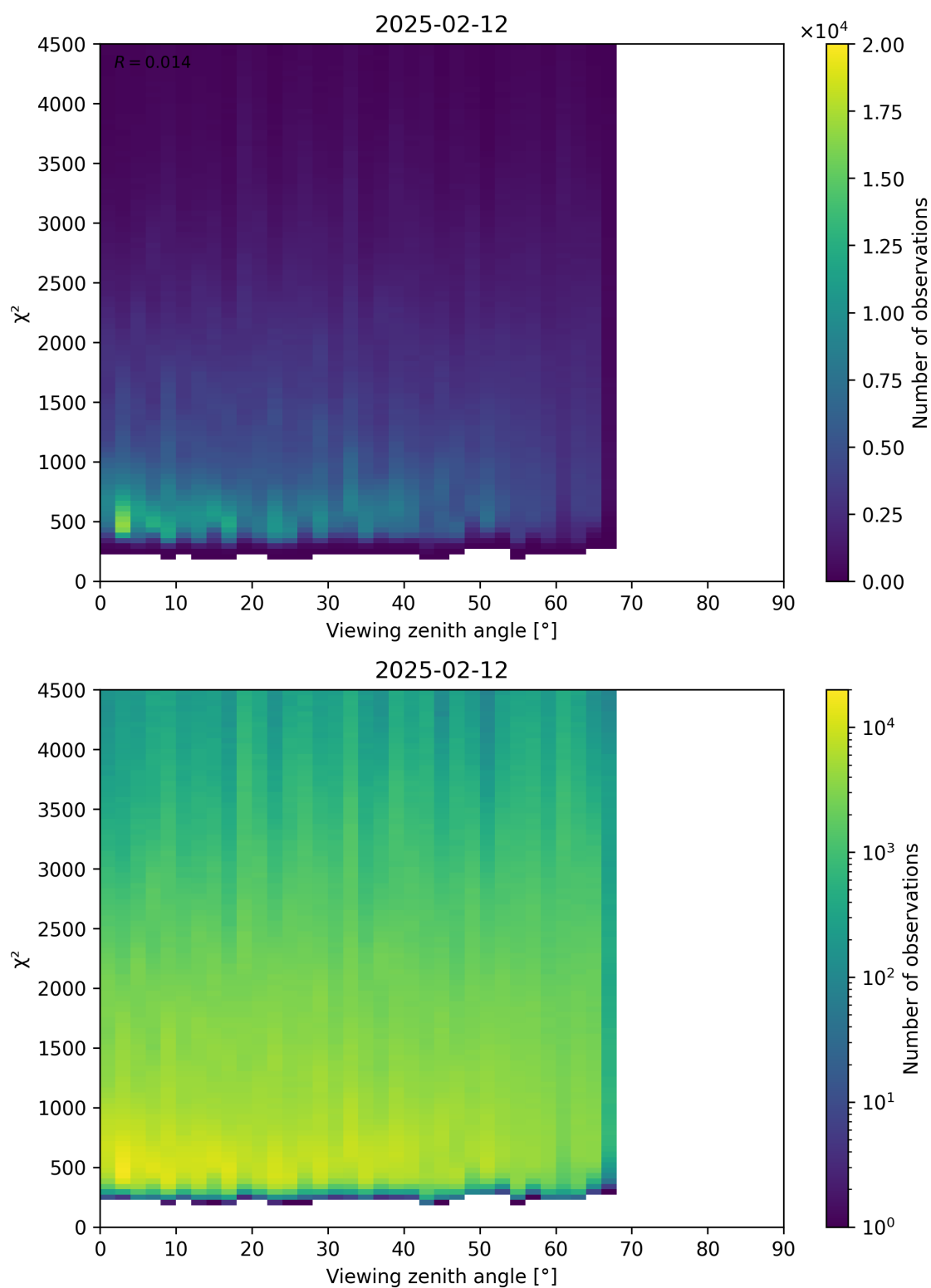
Figure 72: Scatter density plot of “Viewing zenith angle” against “ \chi^2 ” for 2025-02-11 to 2025-02-13.
