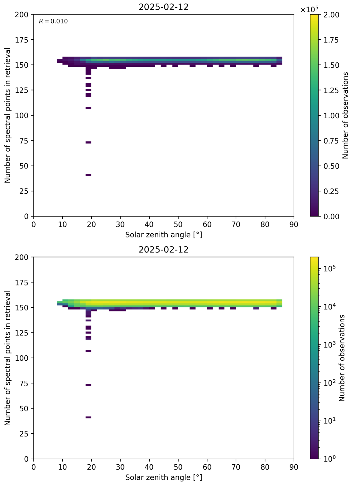
Figure 68: Scatter density plot of “Solar zenith angle” against “Number of spectral points in retrieval” for 2025-02-11 to 2025-02-13.
