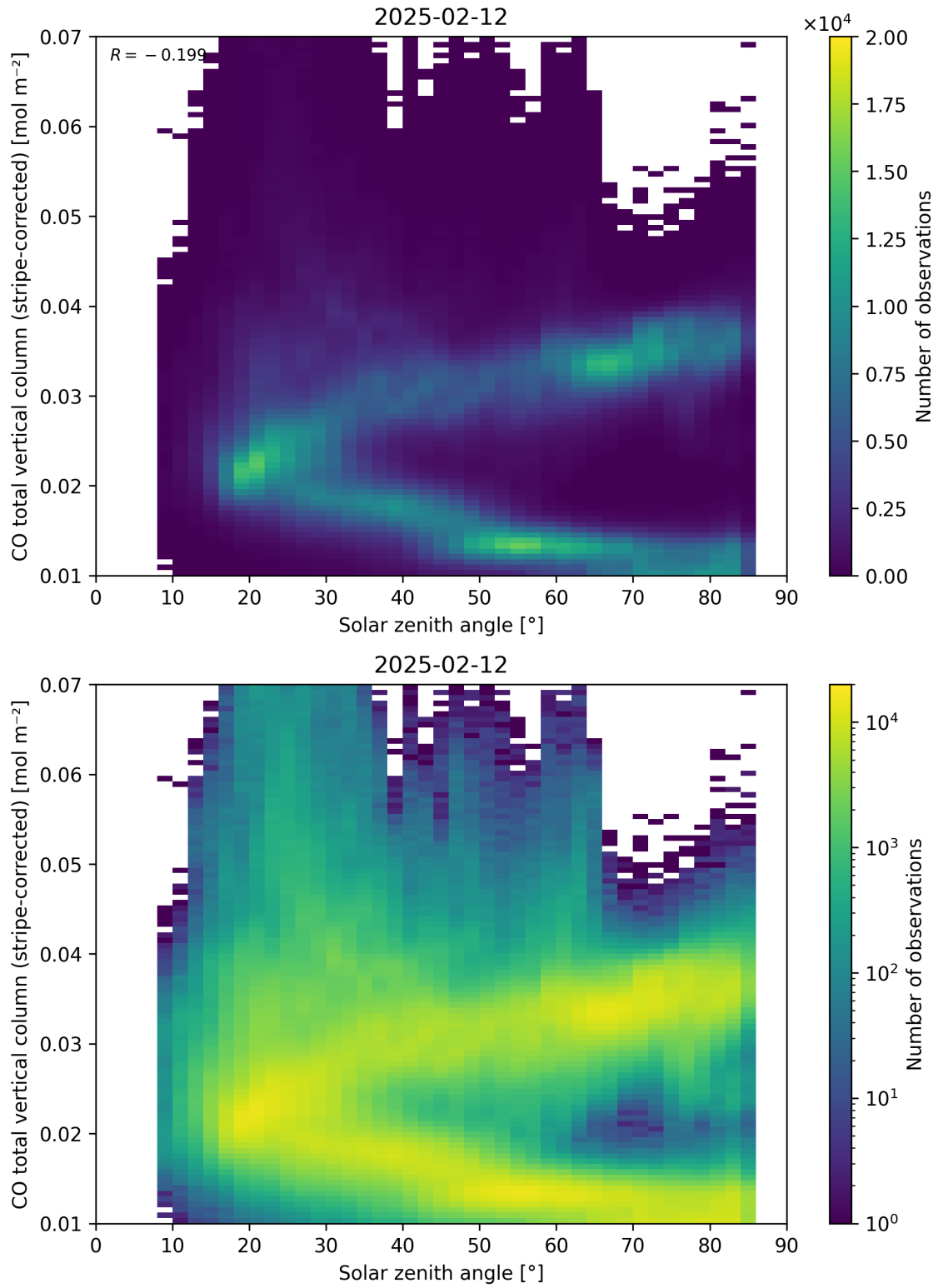
Figure 62: Scatter density plot of “Solar zenith angle” against “CO total vertical column (stripe-corrected)” for 2025-02-11 to 2025-02-13.
