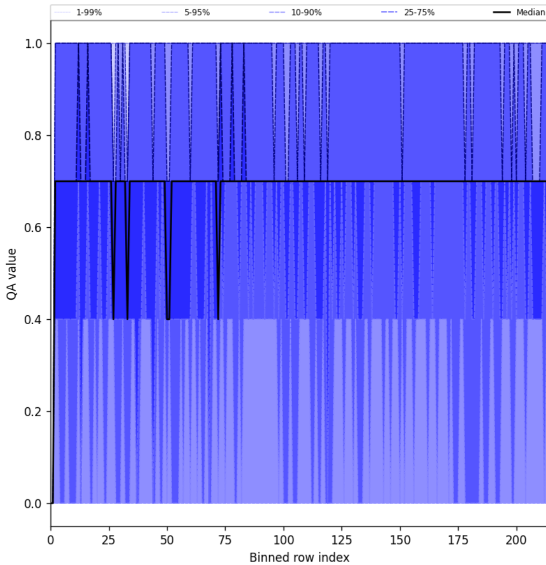
Figure 25: Along track statistics of “QA value” for 2025-02-11 to 2025-02-13
