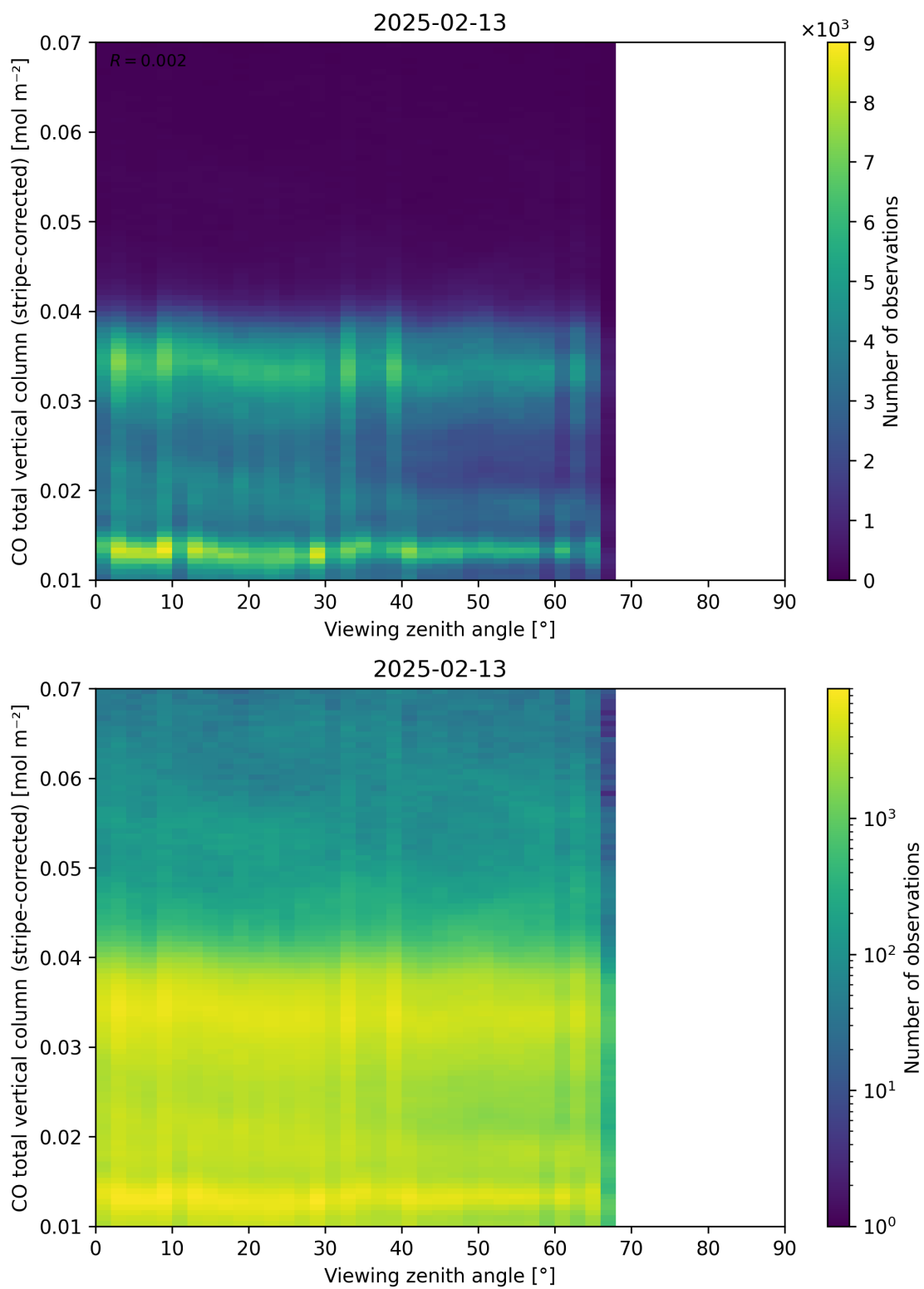
Figure 70: Scatter density plot of “Viewing zenith angle” against “CO total vertical column (stripe-corrected)” for 2025-02-13 to 2025-02-14.
