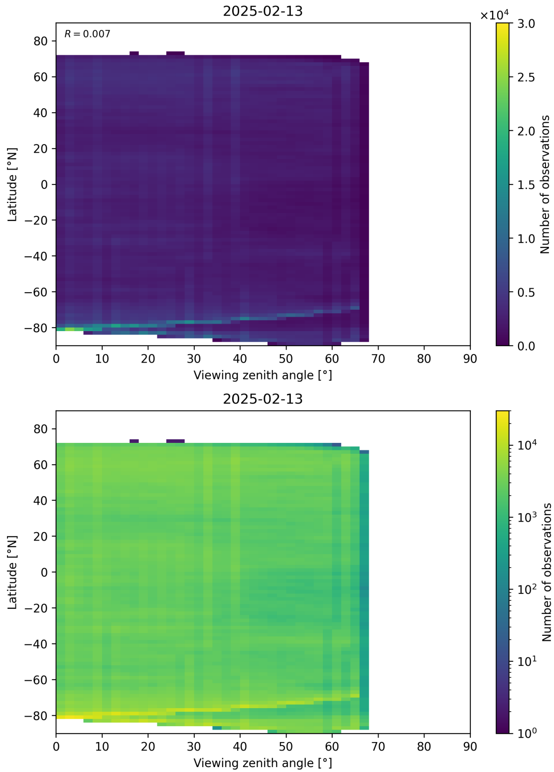
Figure 74: Scatter density plot of “Viewing zenith angle” against “Latitude” for 2025-02-13 to 2025-02-14.
