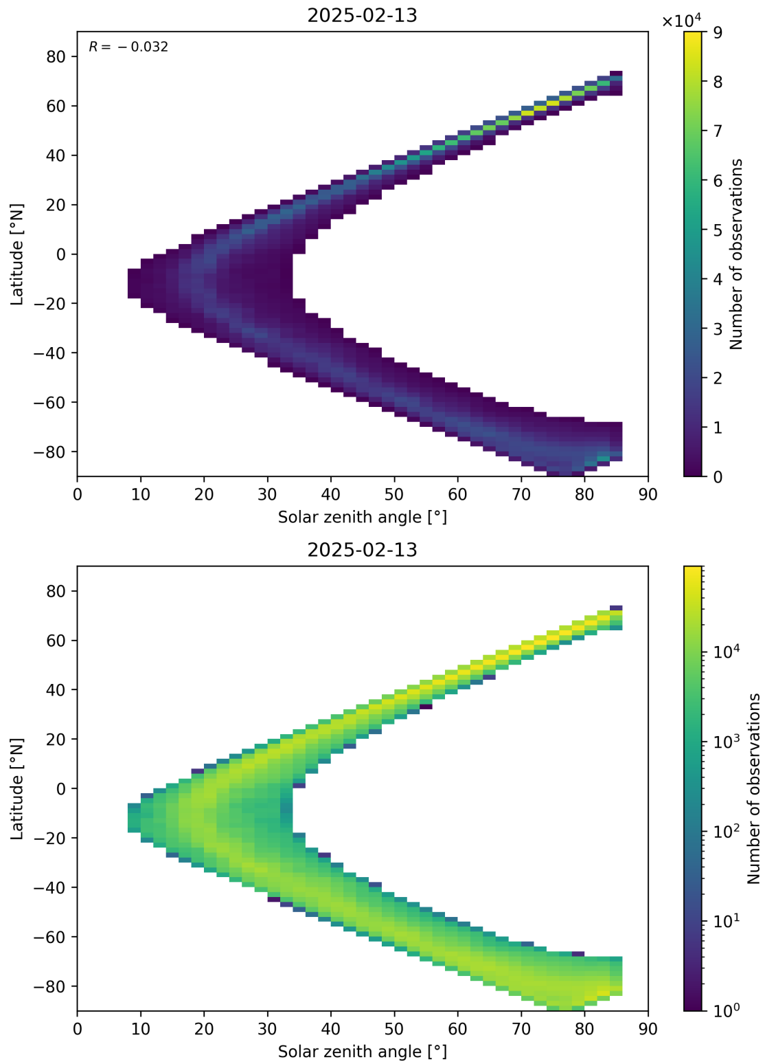
Figure 66: Scatter density plot of “Solar zenith angle” against “Latitude” for 2025-02-13 to 2025-02-14.
