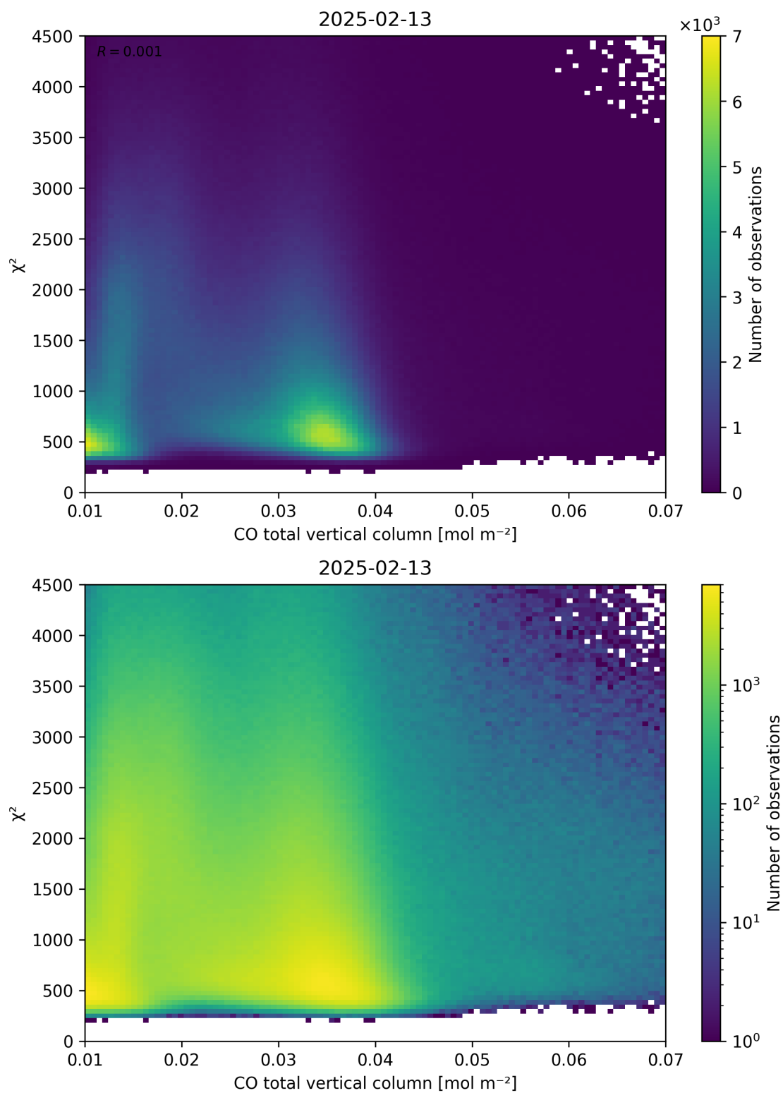
Figure 35: Scatter density plot of “CO total vertical column” against “ \chi^2 ” for 2025-02-13 to 2025-02-14.
