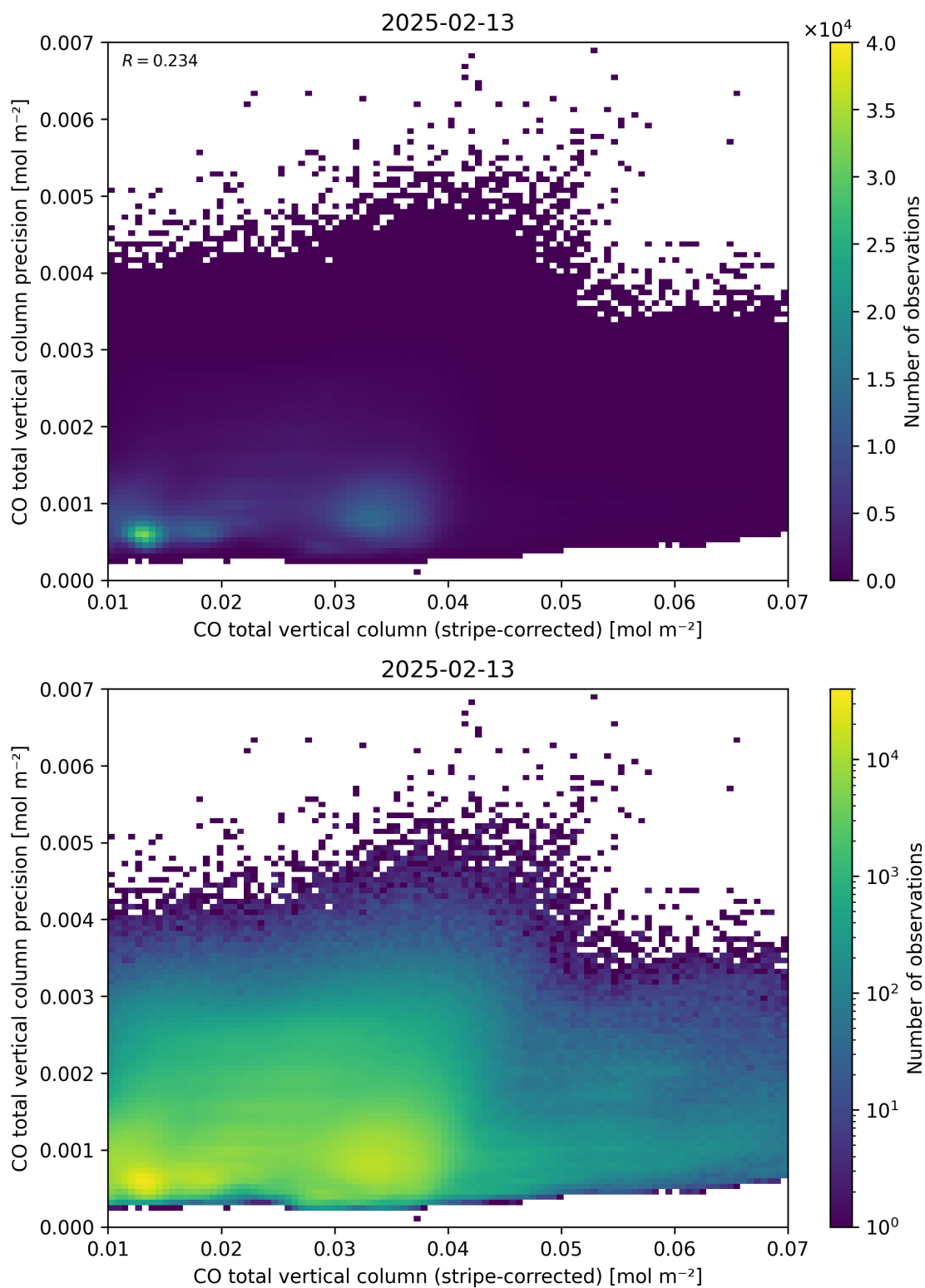
Figure 36: Scatter density plot of “CO total vertical column (stripe-corrected)” against “CO total vertical column precision” for 2025-02-13 to 2025-02-14.
