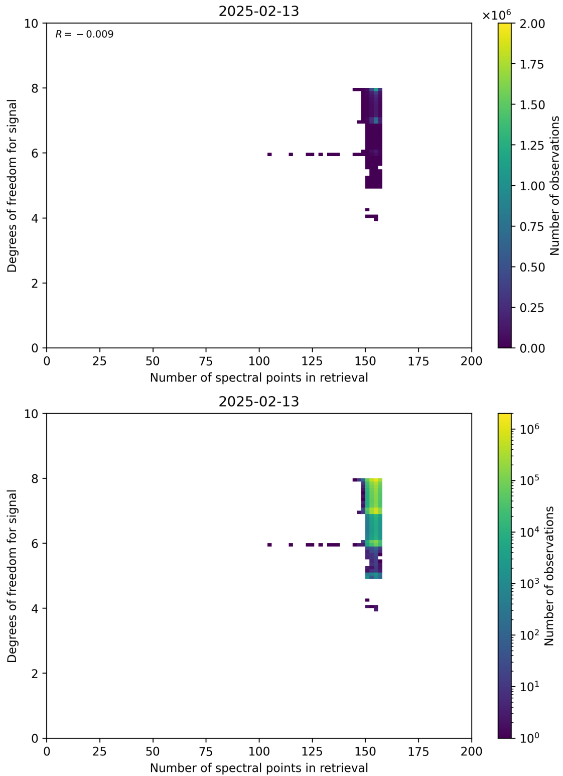
Figure 59: Scatter density plot of “Number of spectral points in retrieval” against “Degrees of freedom for signal” for 2025-02-13 to 2025-02-14.
