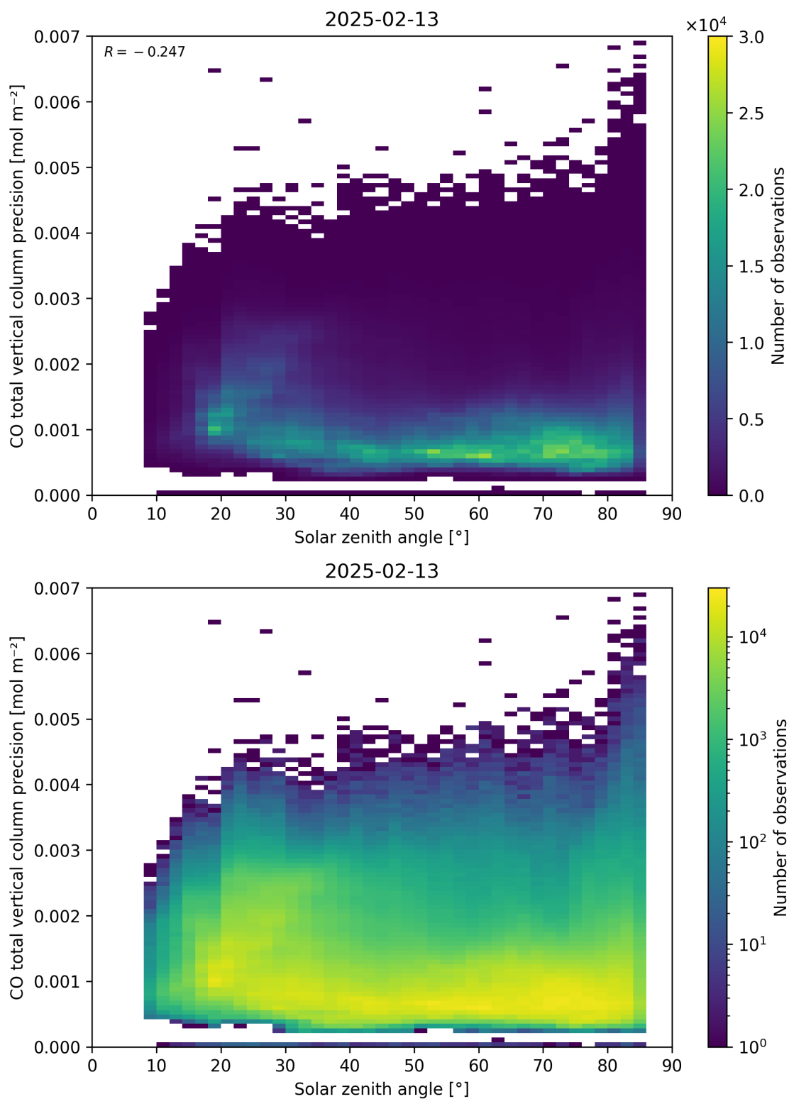
Figure 63: Scatter density plot of “Solar zenith angle” against “CO total vertical column precision” for 2025-02-13 to 2025-02-14.
