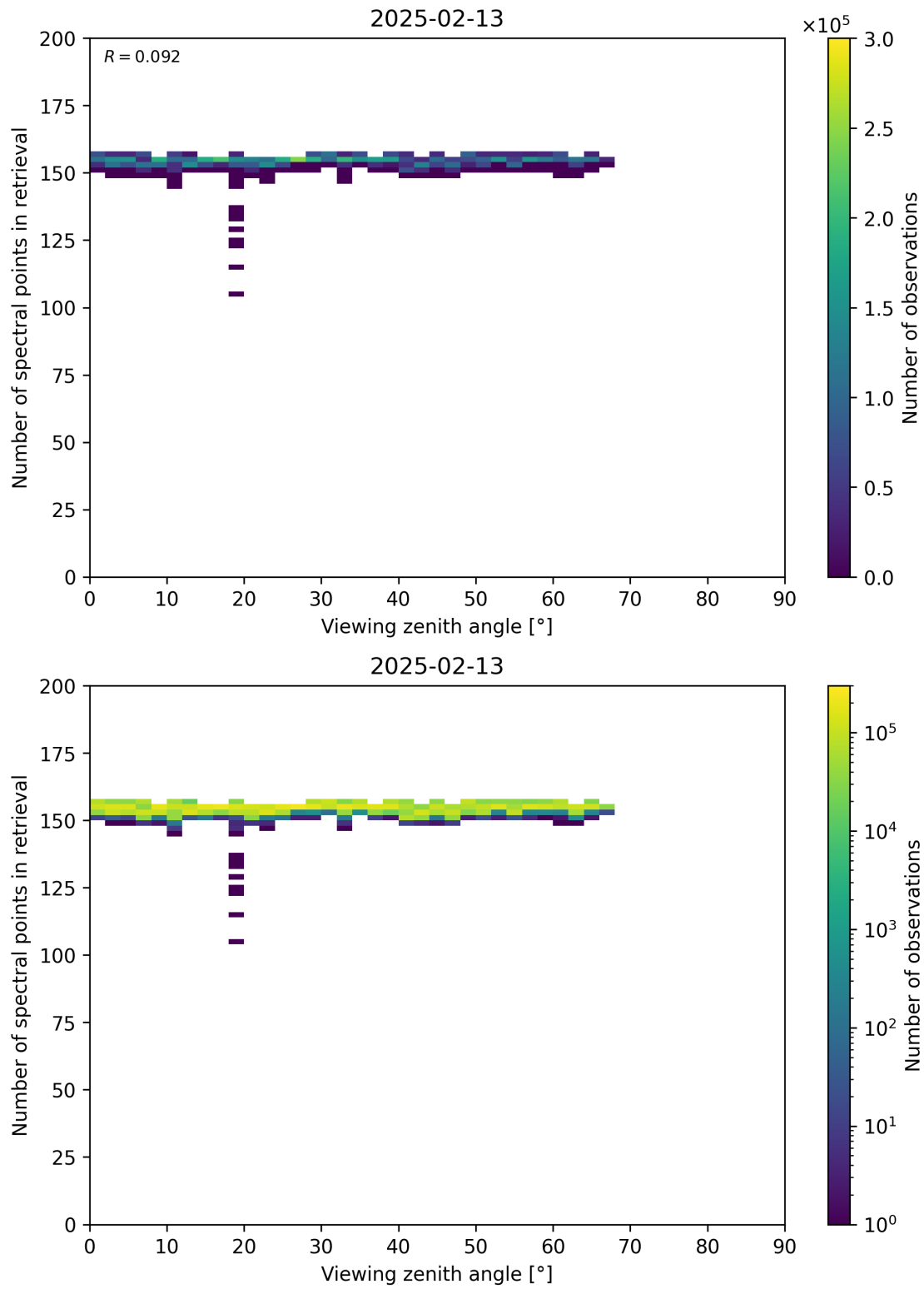
Figure 76: Scatter density plot of “Viewing zenith angle” against “Number of spectral points in retrieval” for 2025-02-13 to 2025-02-14.
