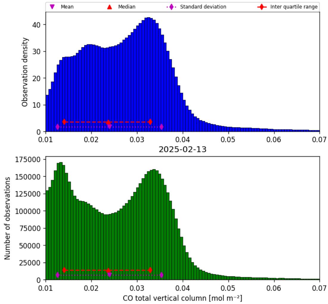
Figure 18: Histogram of “CO total vertical column” for 2025-02-13 to 2025-02-14
