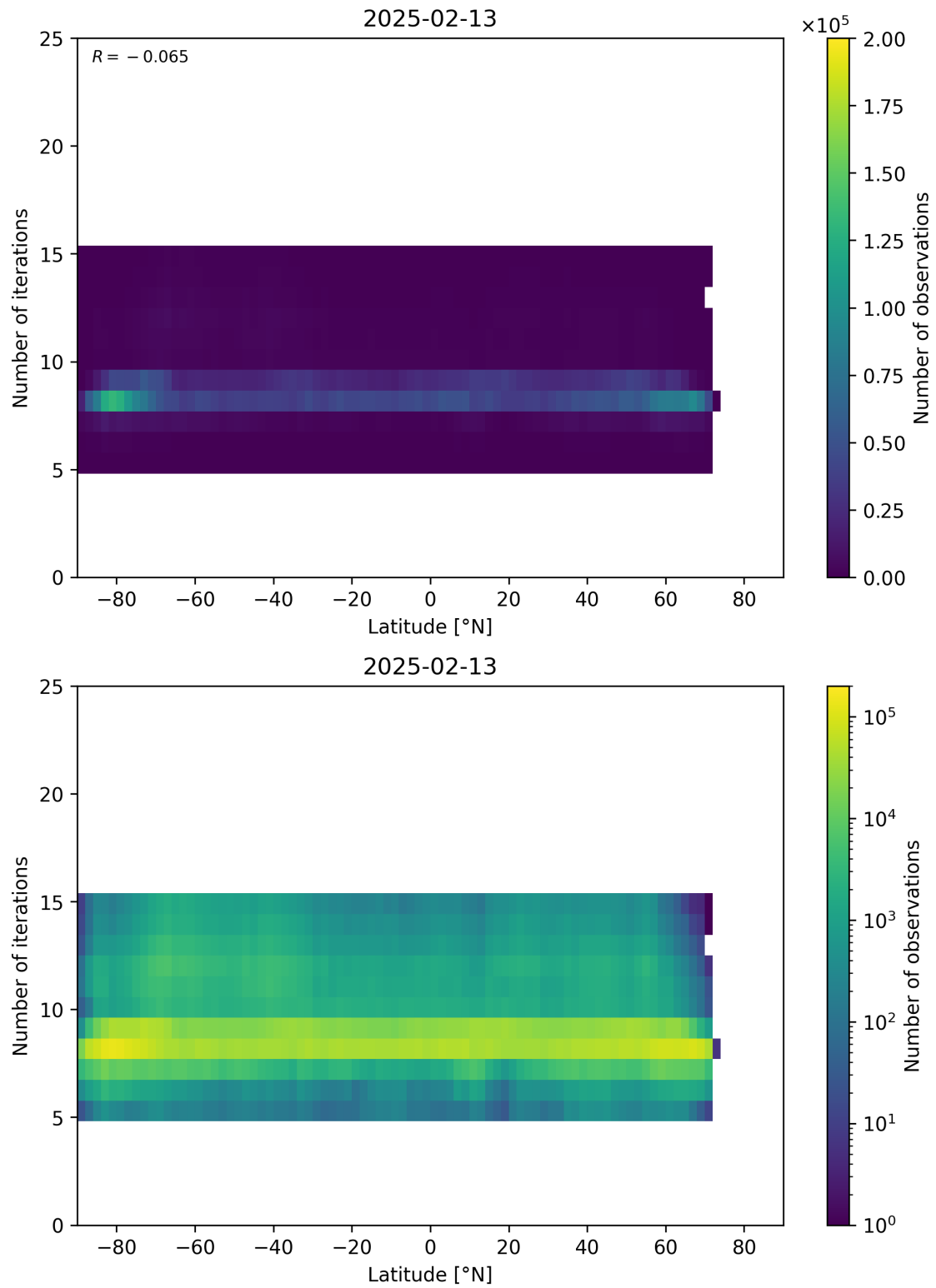
Figure 56: Scatter density plot of “Latitude” against “Number of iterations” for 2025-02-13 to 2025-02-14.
