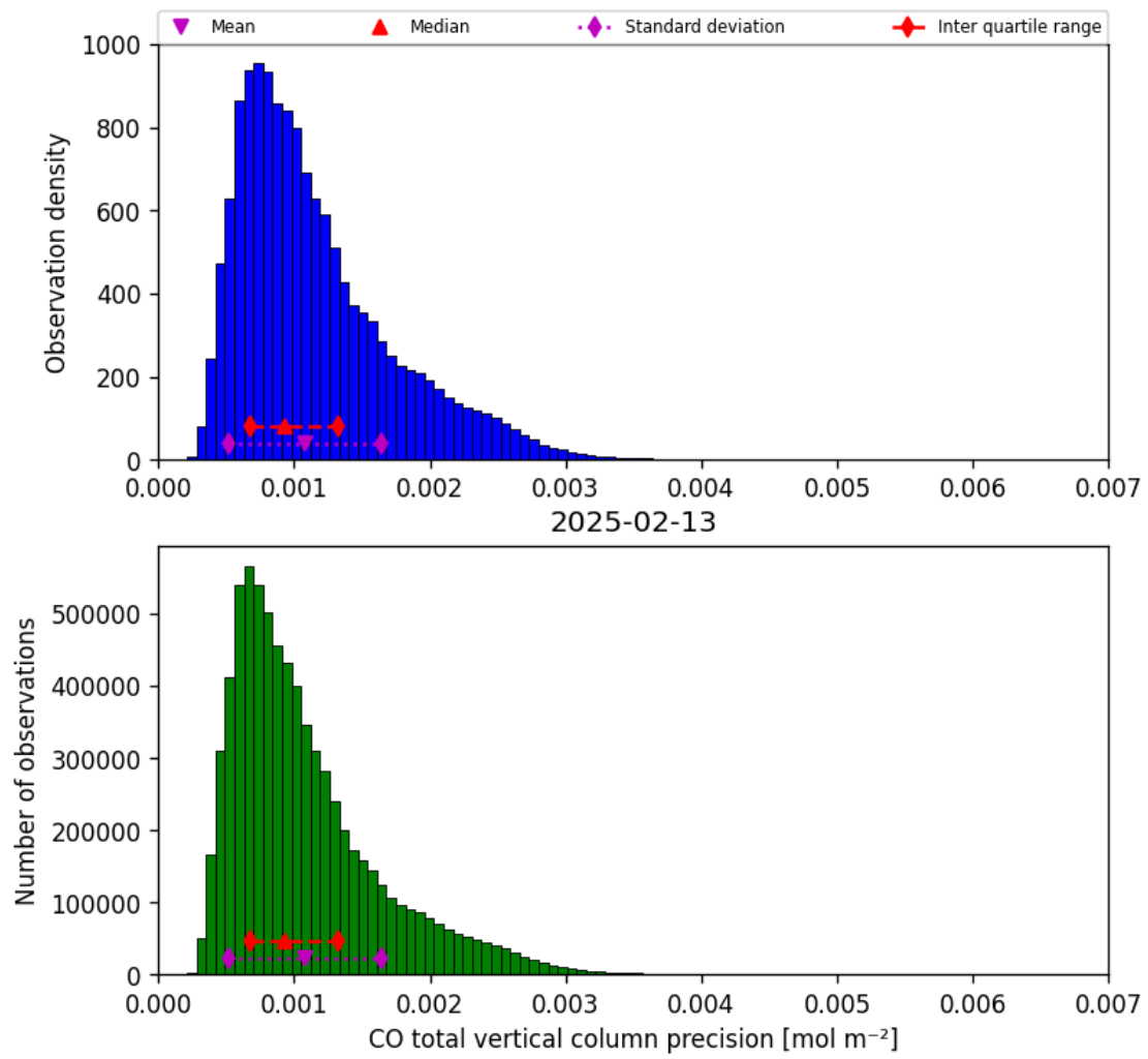
Figure 20: Histogram of “CO total vertical column precision” for 2025-02-13 to 2025-02-14
