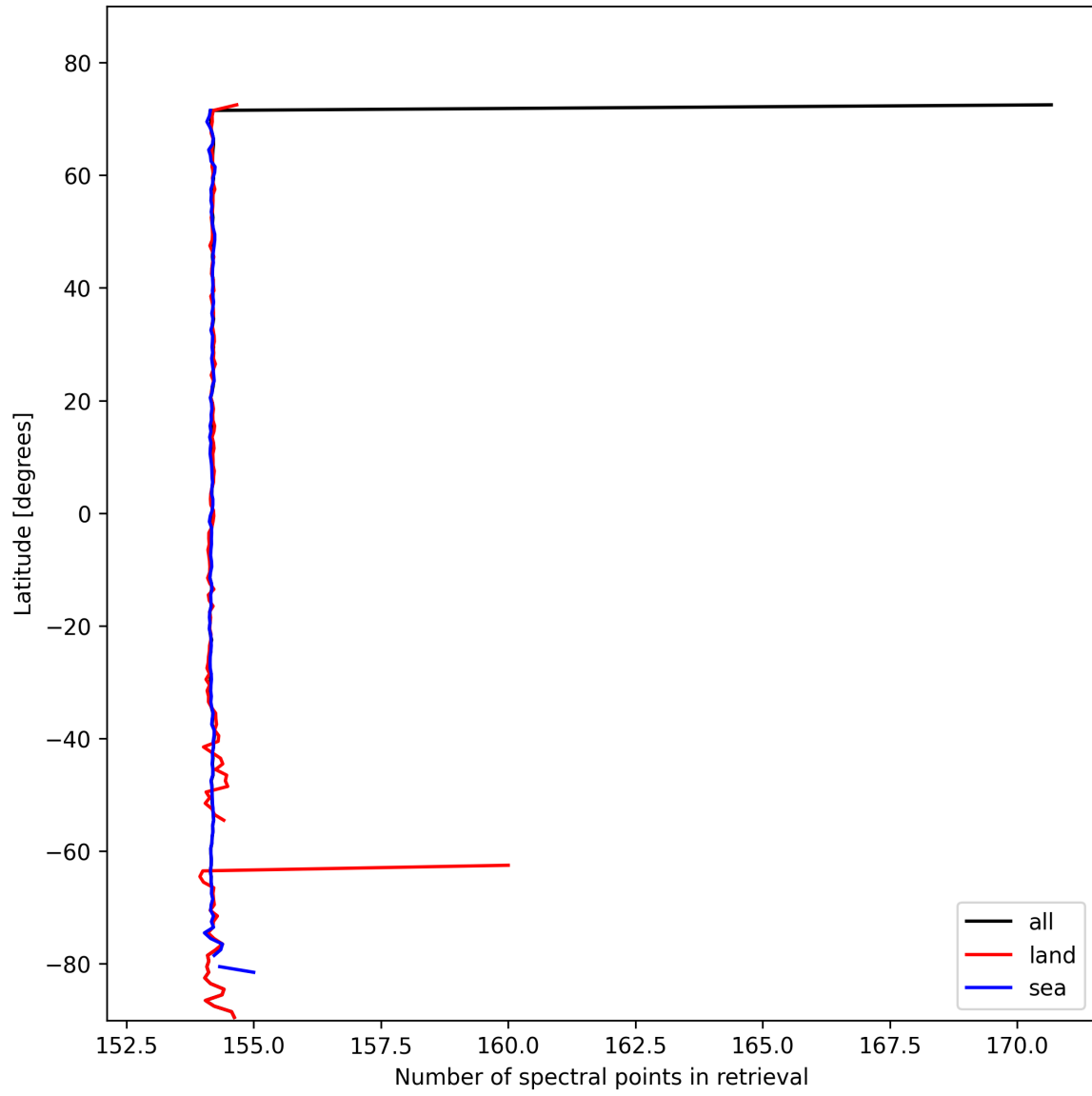
Figure 13: Zonal average of “Number of spectral points in retrieval” for 2025-02-13 to 2025-02-14.
