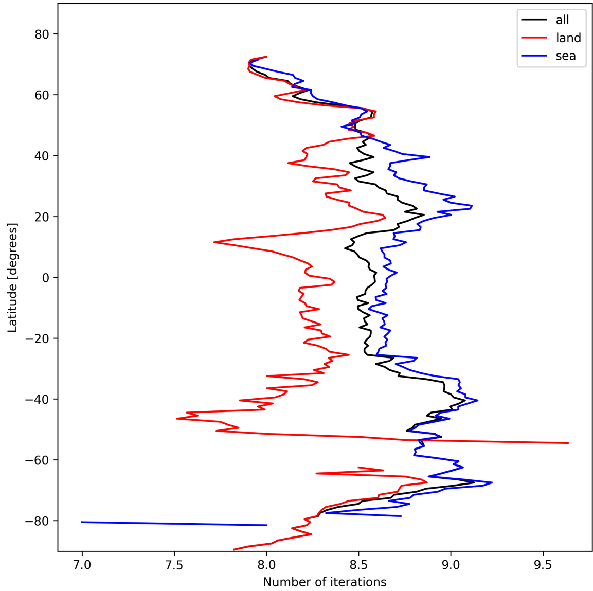
Figure 16: Zonal average of “Number of iterations” for 2025-02-13 to 2025-02-14.
