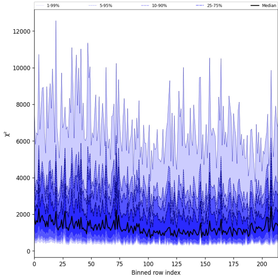
Figure 30: Along track statistics of “ \chi^2 ” for 2025-02-13 to 2025-02-14
