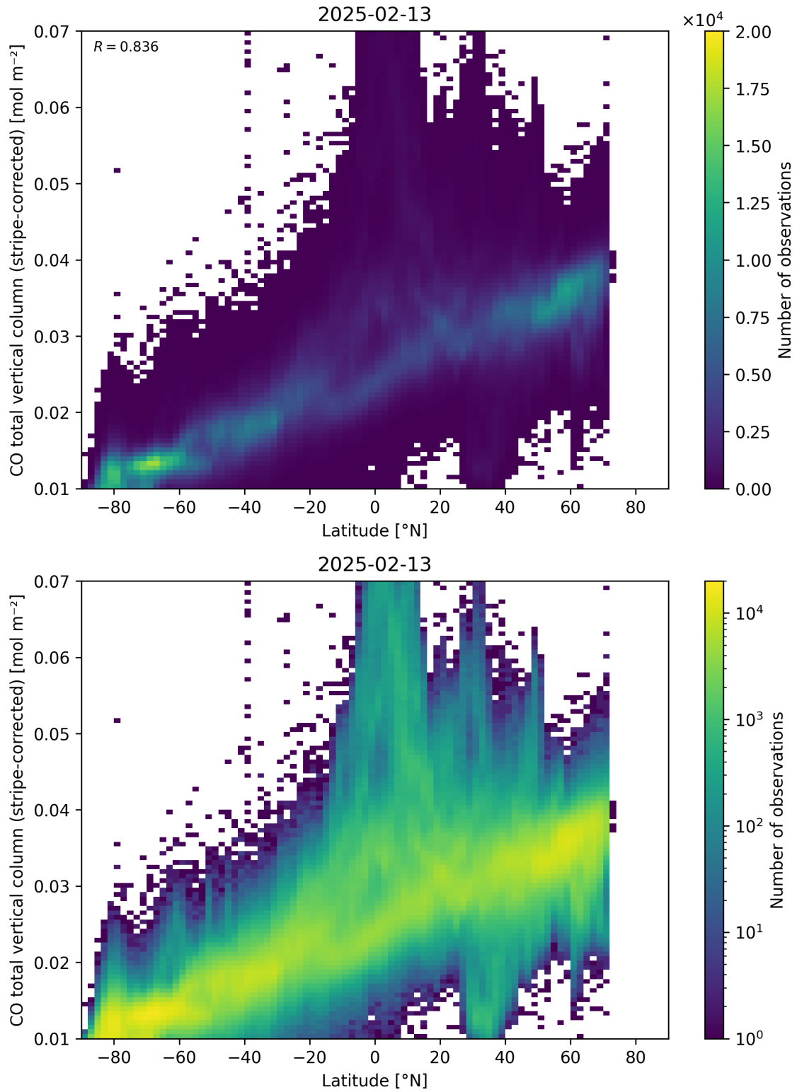
Figure 52: Scatter density plot of “Latitude” against “CO total vertical column (stripe-corrected)” for 2025-02-13 to 2025-02-14.
