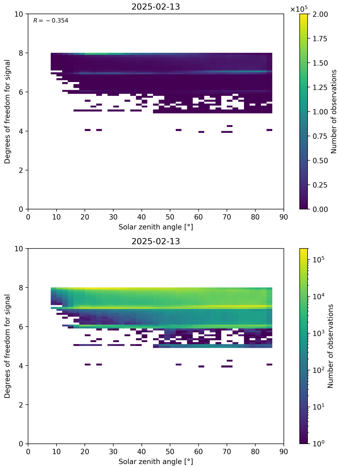
Figure 65: Scatter density plot of “Solar zenith angle” against “Degrees of freedom for signal” for 2025-02-13 to 2025-02-14.
