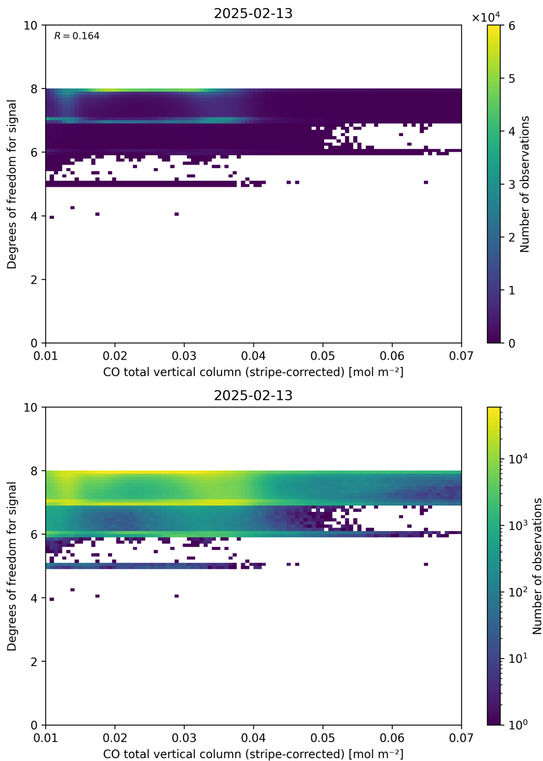
Figure 38: Scatter density plot of “CO total vertical column (stripe-corrected)” against “Degrees of freedom for signal” for 2025-02-13 to 2025-02-14.
