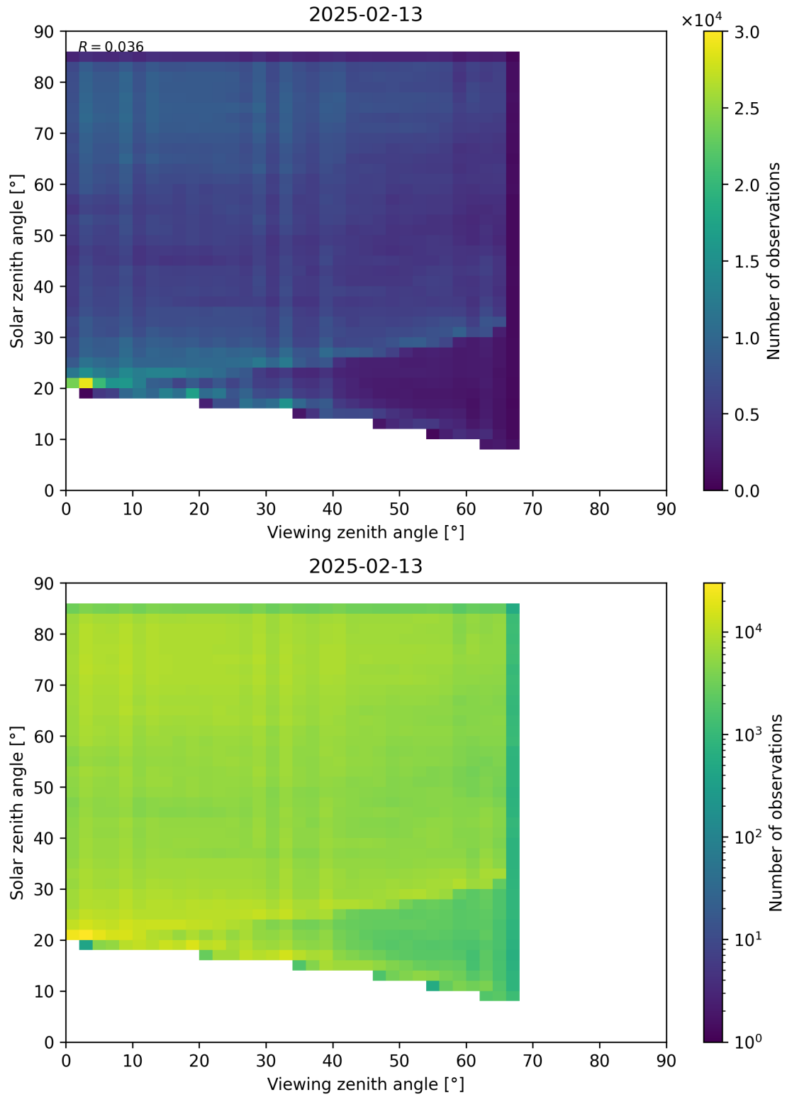
Figure 77: Scatter density plot of “Viewing zenith angle” against “Solar zenith angle” for 2025-02-13 to 2025-02-14.
