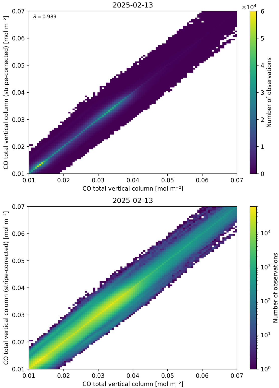
Figure 33: Scatter density plot of “CO total vertical column” against “CO total vertical column (stripe-corrected)” for 2025-02-13 to 2025-02-14.
