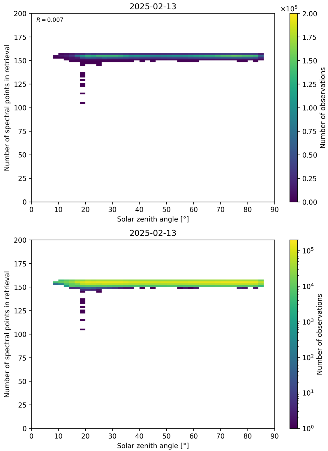
Figure 68: Scatter density plot of “Solar zenith angle” against “Number of spectral points in retrieval” for 2025-02-13 to 2025-02-14.
