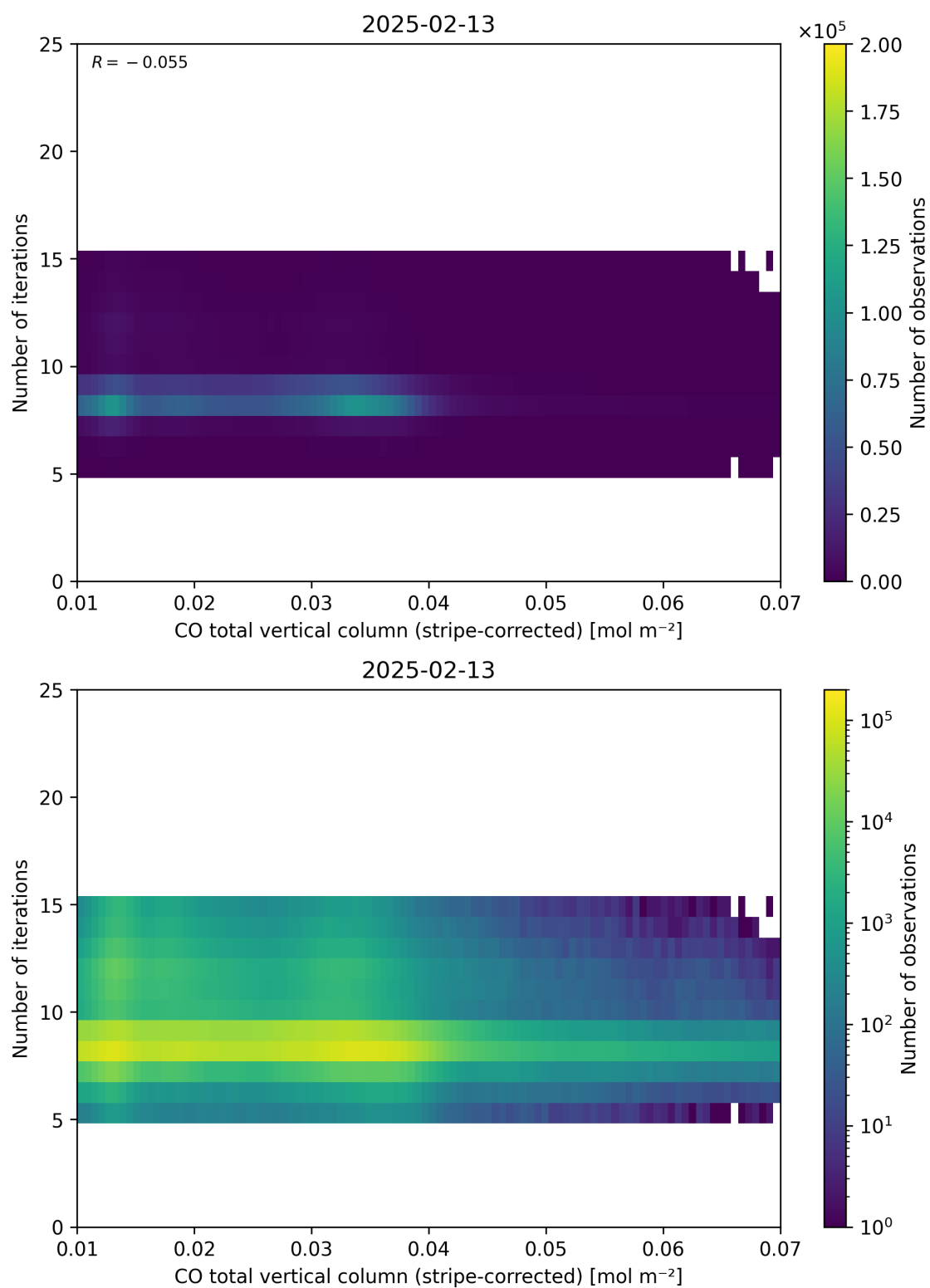
Figure 39: Scatter density plot of “CO total vertical column (stripe-corrected)” against “Number of iterations” for 2025-02-13 to 2025-02-14.
