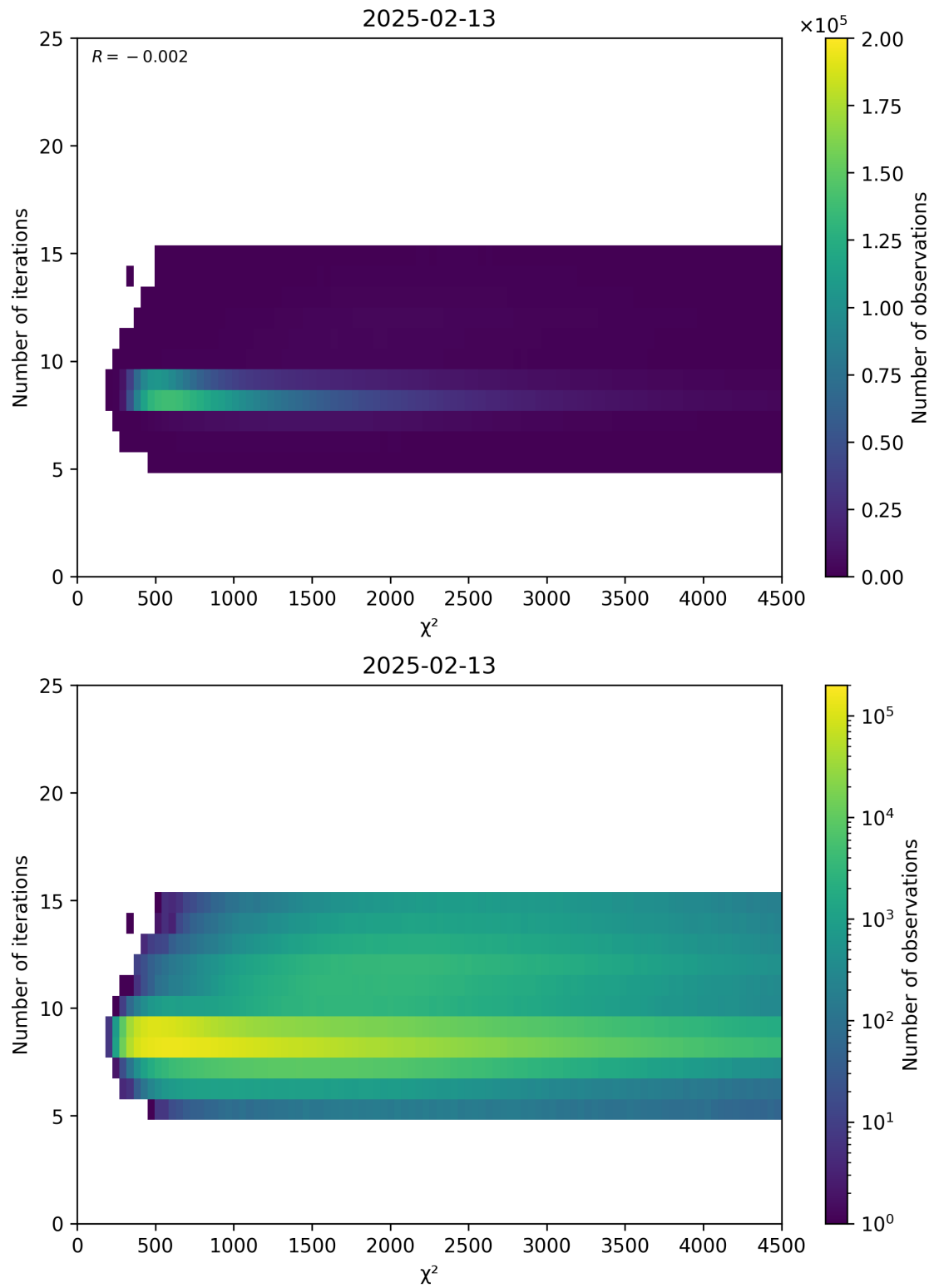
Figure 49: Scatter density plot of “ \chi^2 ” against “Number of iterations” for 2025-02-13 to 2025-02-14.
