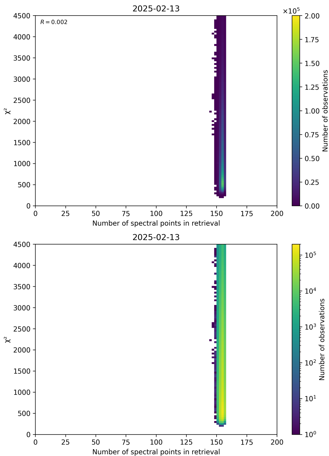
Figure 58: Scatter density plot of “Number of spectral points in retrieval” against “ \chi^2 ” for 2025-02-13 to 2025-02-14.
