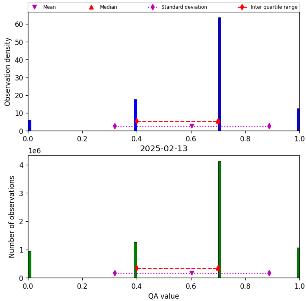
Figure 17: Histogram of “QA value” for 2025-02-13 to 2025-02-14
