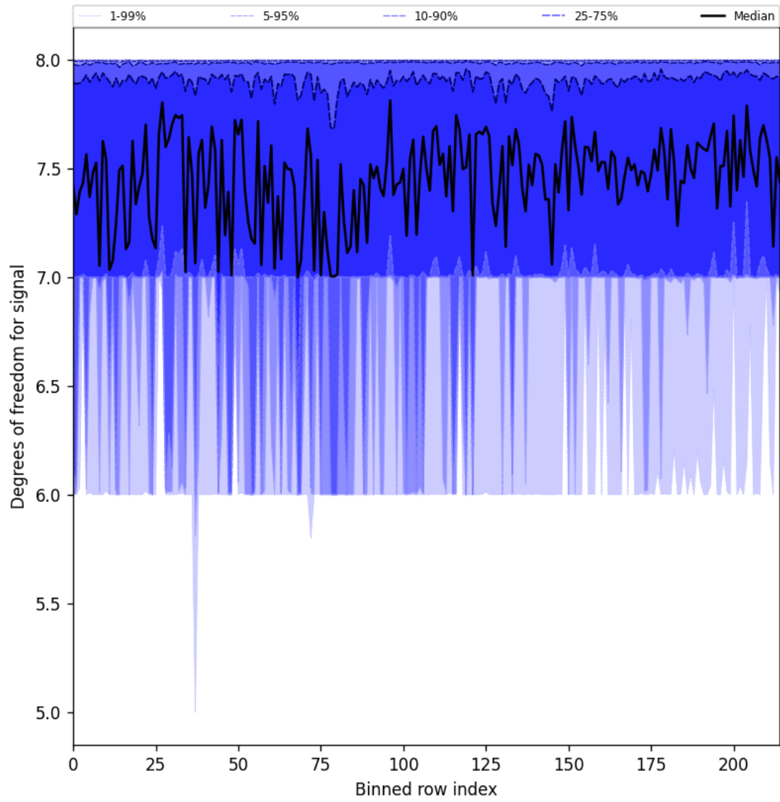
Figure 31: Along track statistics of “Degrees of freedom for signal” for 2025-02-13 to 2025-02-14
