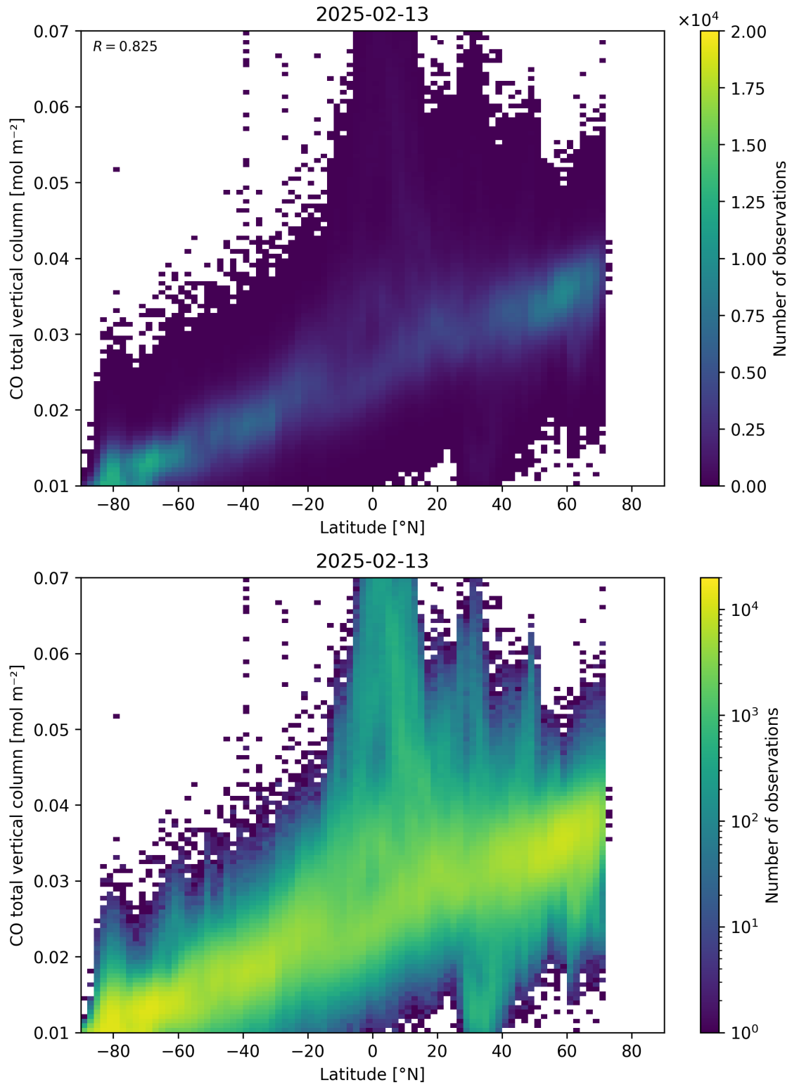
Figure 51: Scatter density plot of “Latitude” against “CO total vertical column” for 2025-02-13 to 2025-02-14.
