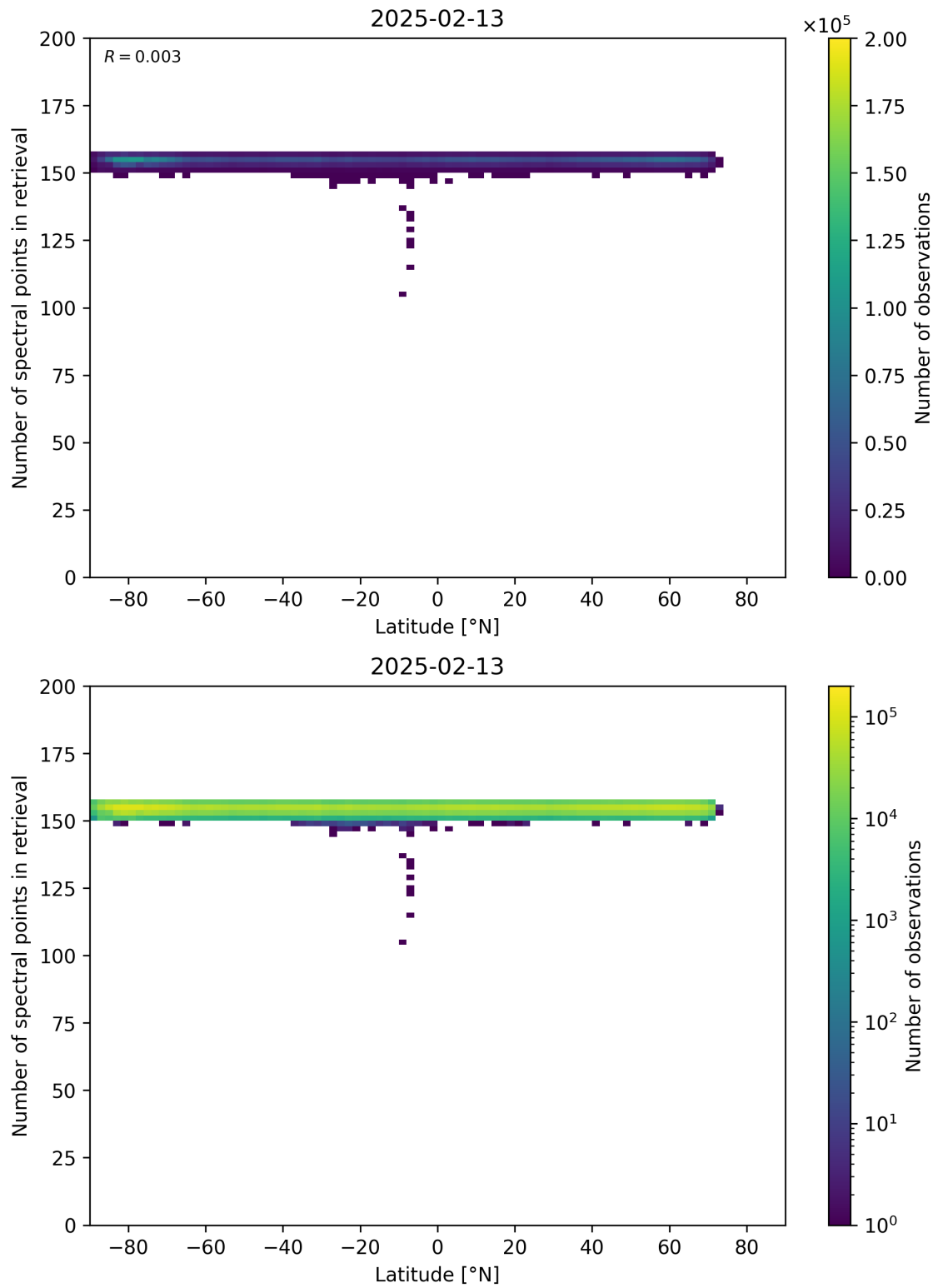
Figure 57: Scatter density plot of “Latitude” against “Number of spectral points in retrieval” for 2025-02-13 to 2025-02-14.
