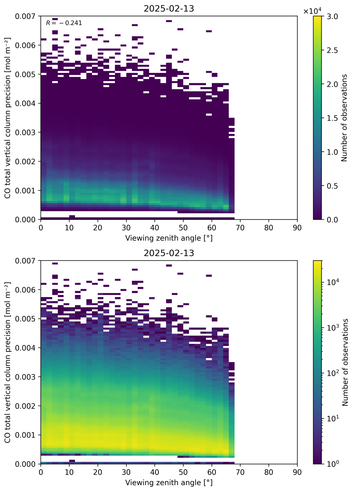
Figure 71: Scatter density plot of “Viewing zenith angle” against “CO total vertical column precision” for 2025-02-13 to 2025-02-14.
