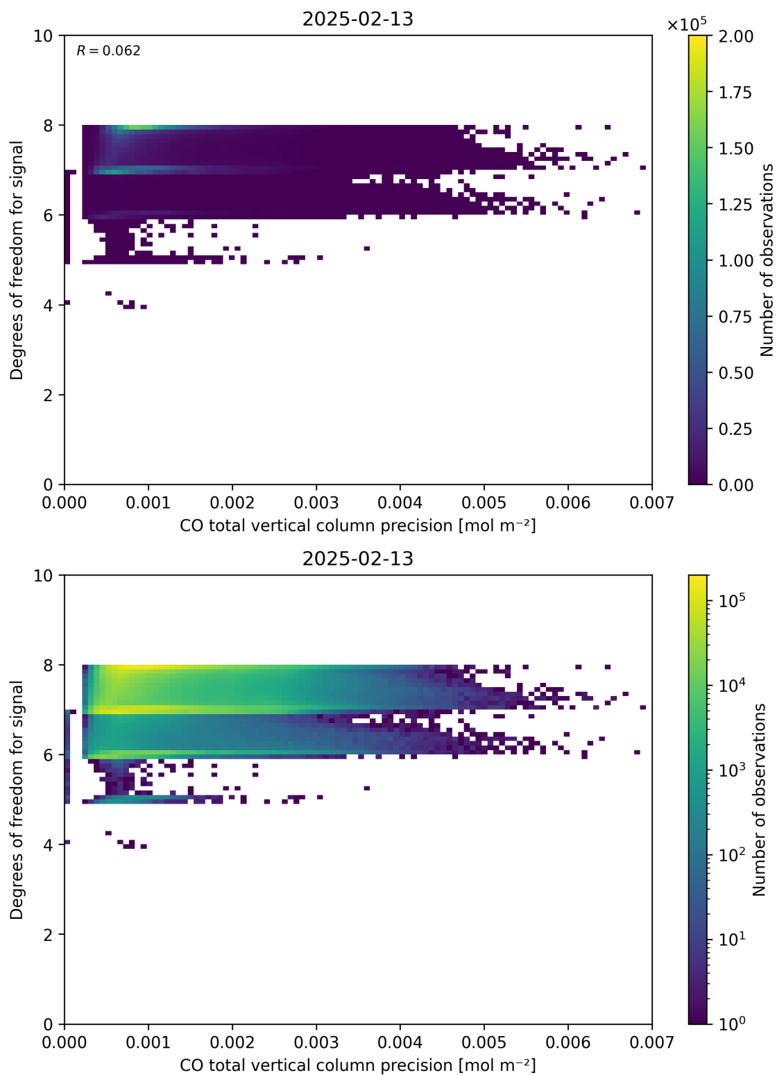
Figure 45: Scatter density plot of “CO total vertical column precision” against “Degrees of freedom for signal” for 2025-02-13 to 2025-02-14.
