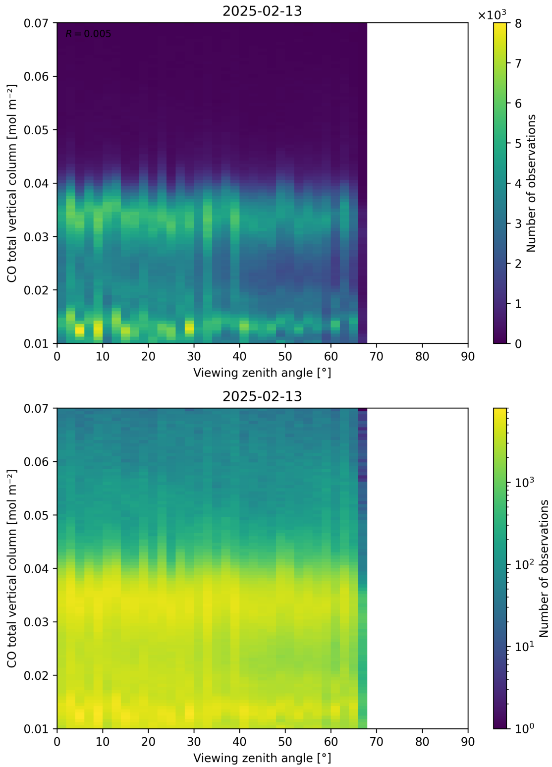
Figure 69: Scatter density plot of “Viewing zenith angle” against “CO total vertical column” for 2025-02-13 to 2025-02-14.
