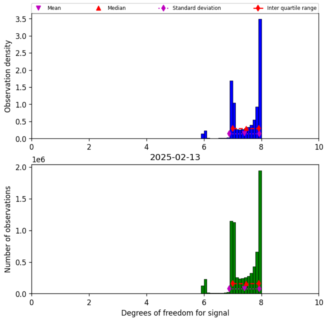
Figure 23: Histogram of “Degrees of freedom for signal” for 2025-02-13 to 2025-02-14
