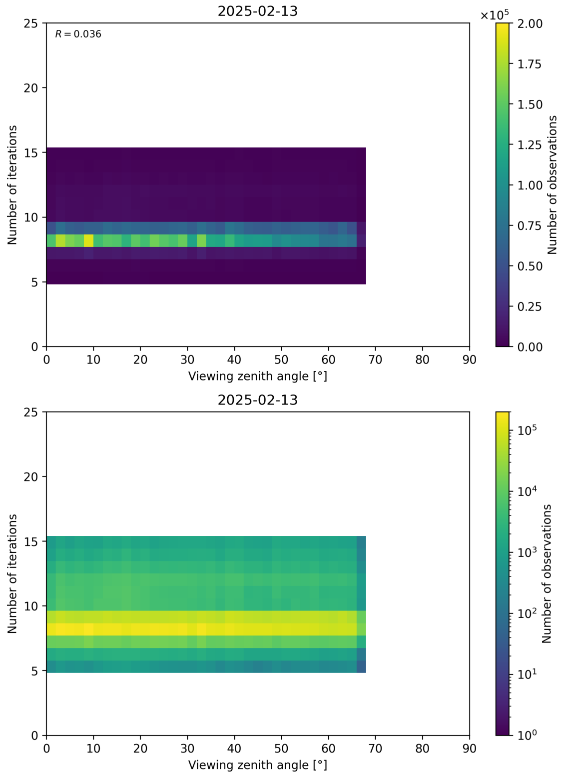
Figure 75: Scatter density plot of “Viewing zenith angle” against “Number of iterations” for 2025-02-13 to 2025-02-14.
