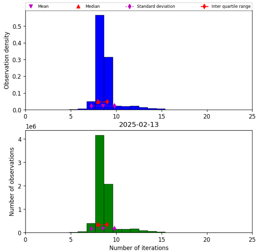
Figure 24: Histogram of “Number of iterations” for 2025-02-13 to 2025-02-14
