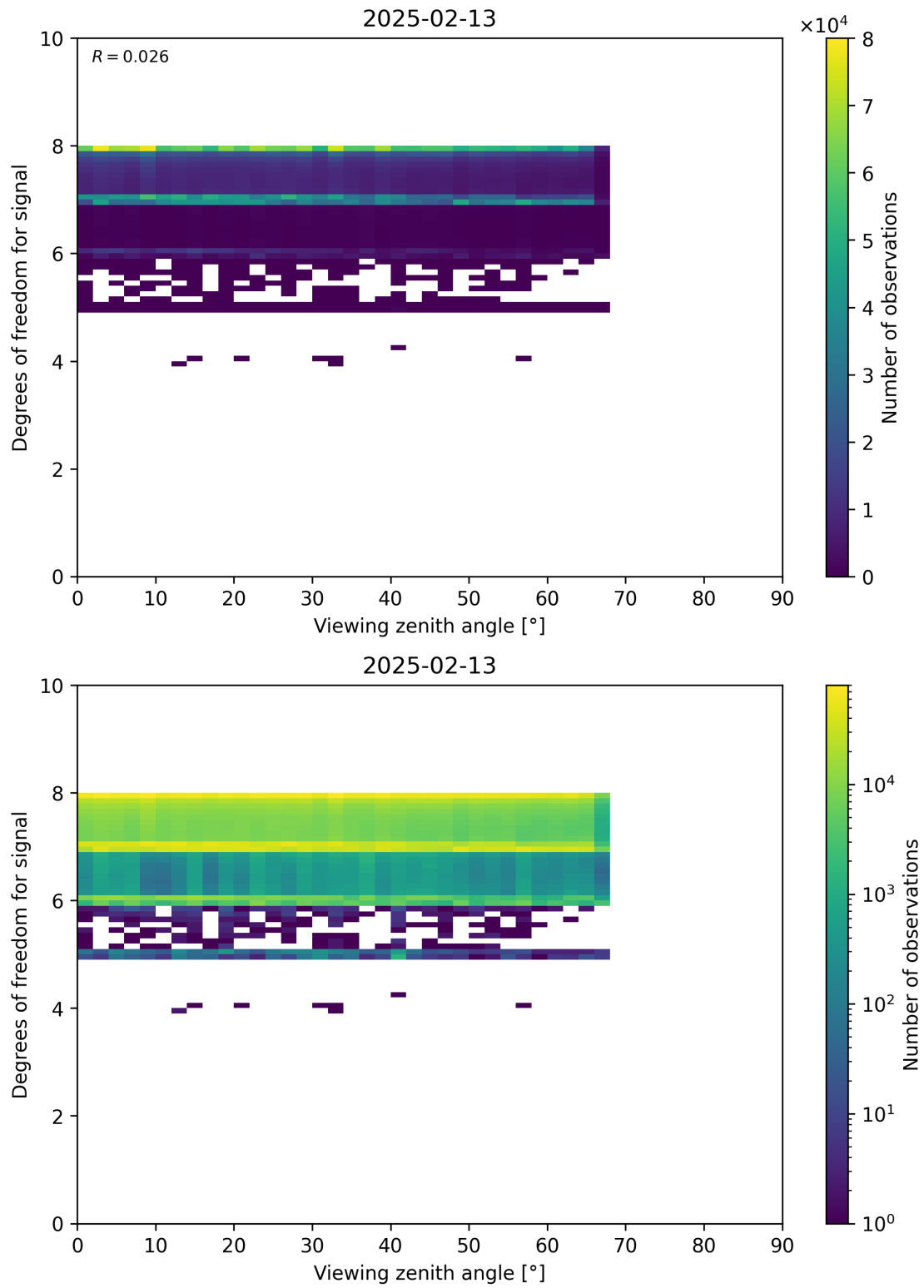
Figure 73: Scatter density plot of “Viewing zenith angle” against “Degrees of freedom for signal” for 2025-02-13 to 2025-02-14.
