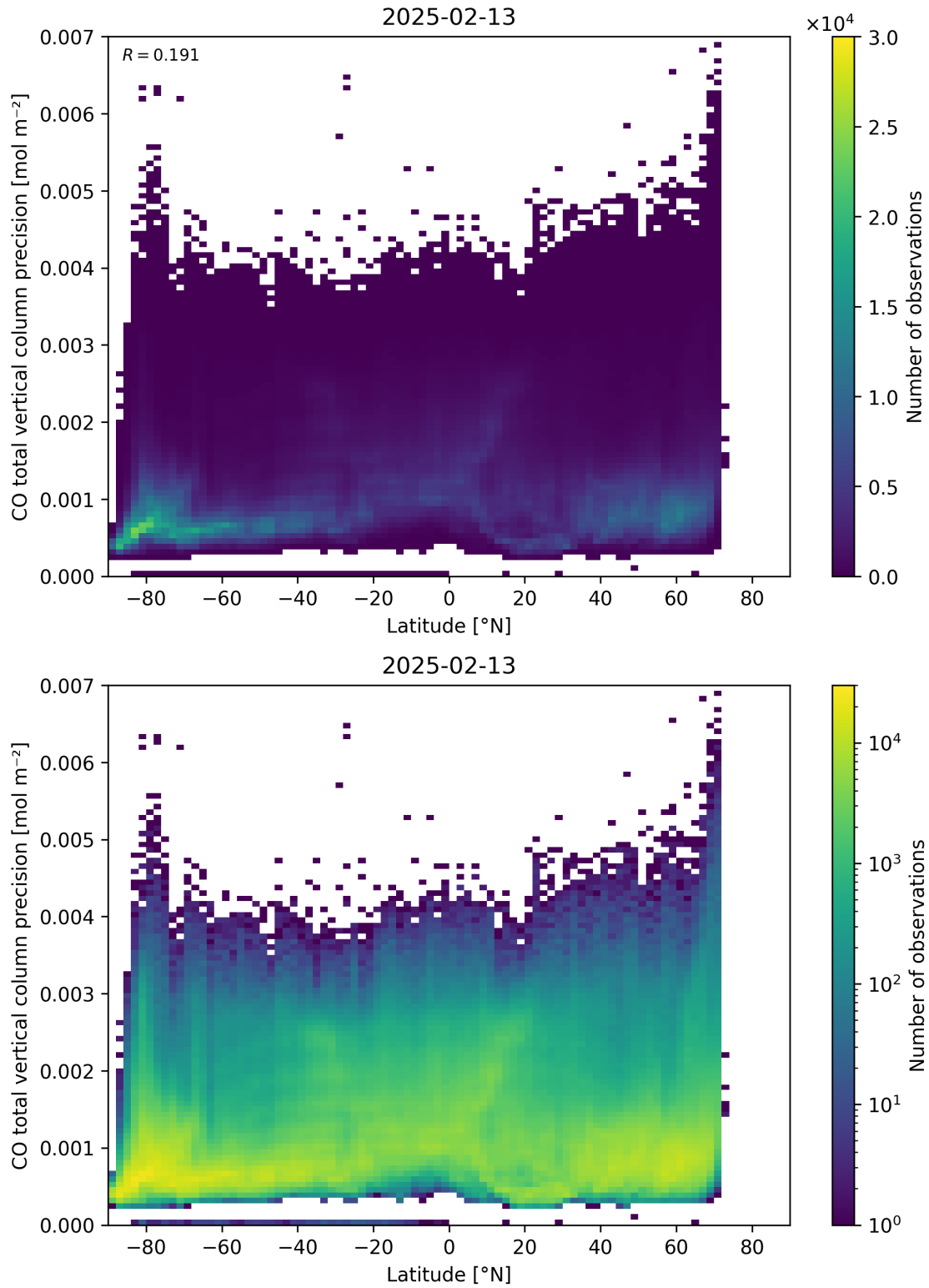
Figure 53: Scatter density plot of “Latitude” against “CO total vertical column precision” for 2025-02-13 to 2025-02-14.
