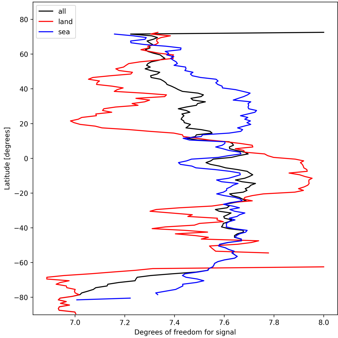
Figure 15: Zonal average of “Degrees of freedom for signal” for 2025-02-13 to 2025-02-14.
