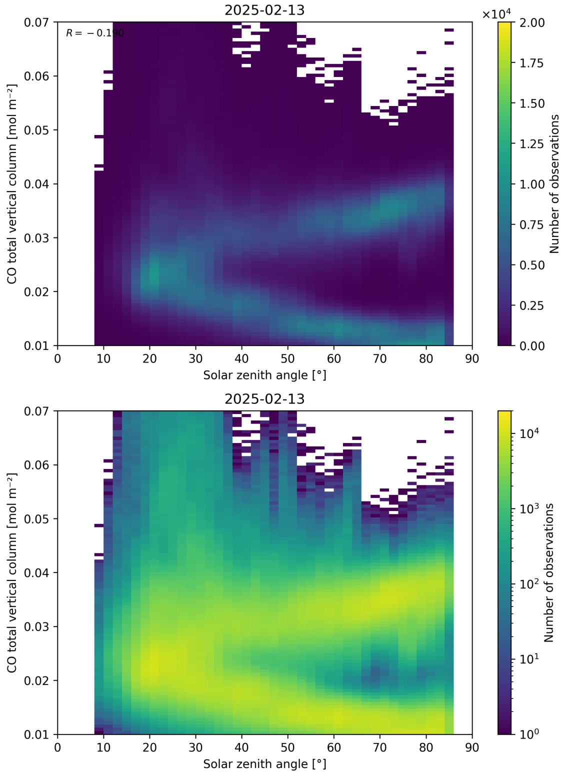
Figure 61: Scatter density plot of “Solar zenith angle” against “CO total vertical column” for 2025-02-13 to 2025-02-14.
