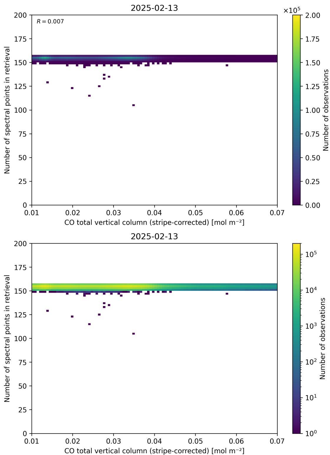
Figure 40: Scatter density plot of “CO total vertical column (stripe-corrected)” against “Number of spectral points in retrieval” for 2025-02-13 to 2025-02-14.
