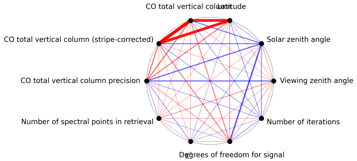
Figure 1: Map of correlation graph for 2025-02-13 to 2025-02-14.
