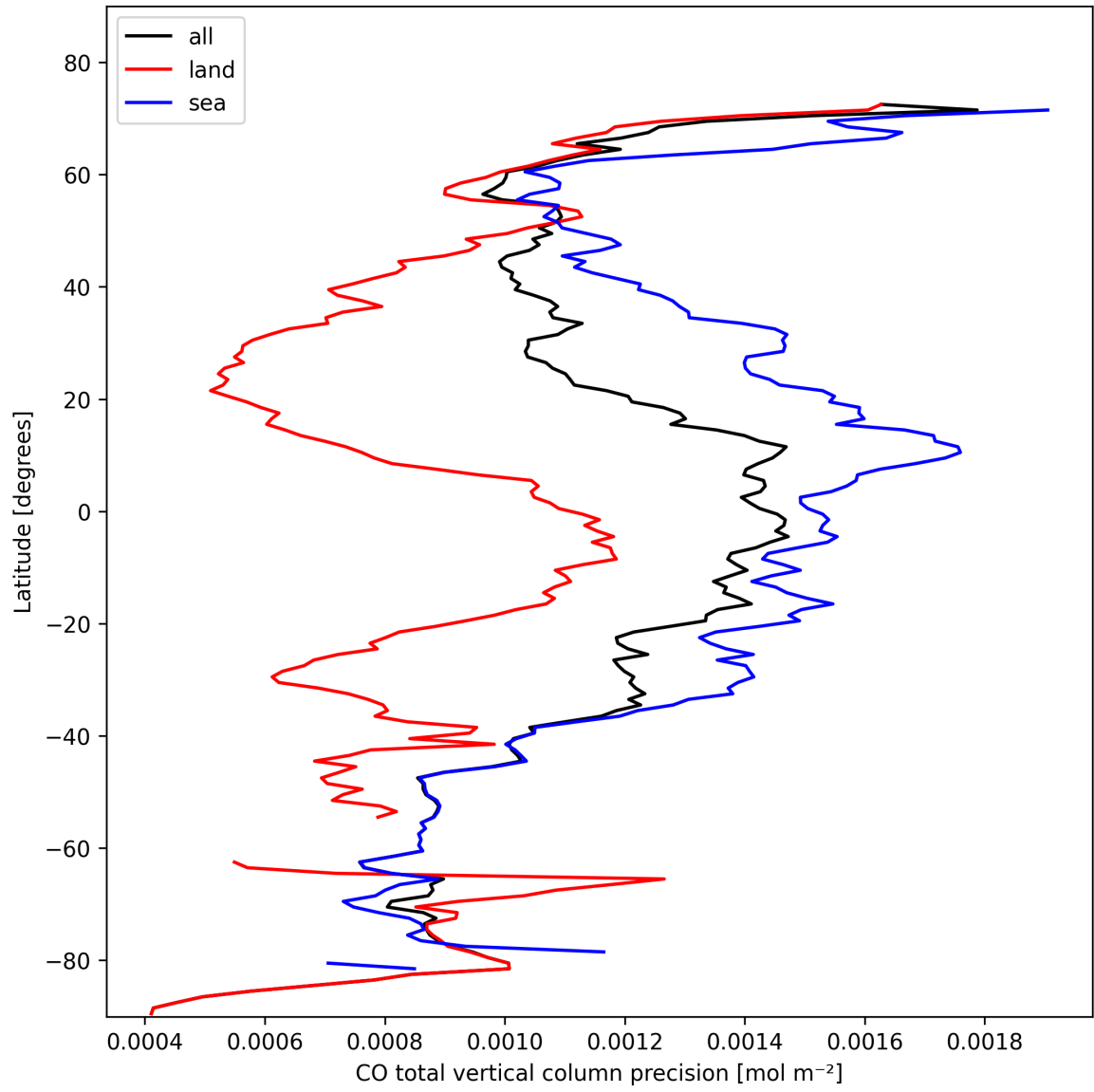
Figure 12: Zonal average of “CO total vertical column precision” for 2025-02-13 to 2025-02-14.
