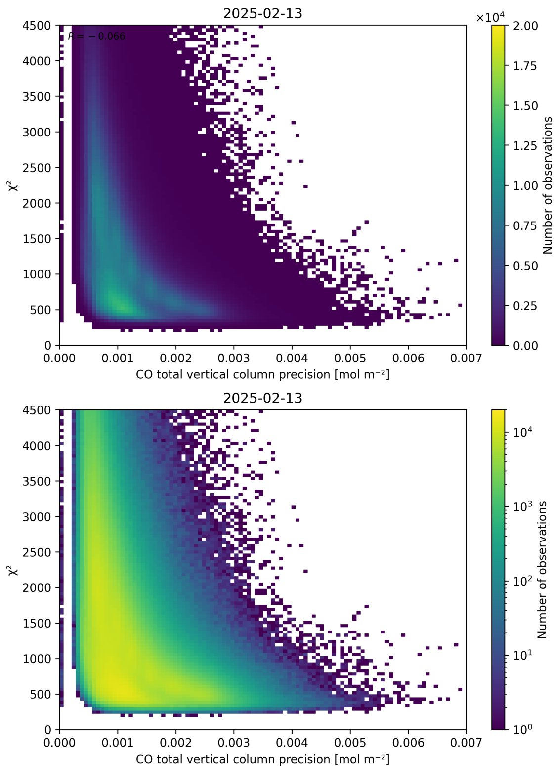
Figure 44: Scatter density plot of “CO total vertical column precision” against “ \chi^2 ” for 2025-02-13 to 2025-02-14.
