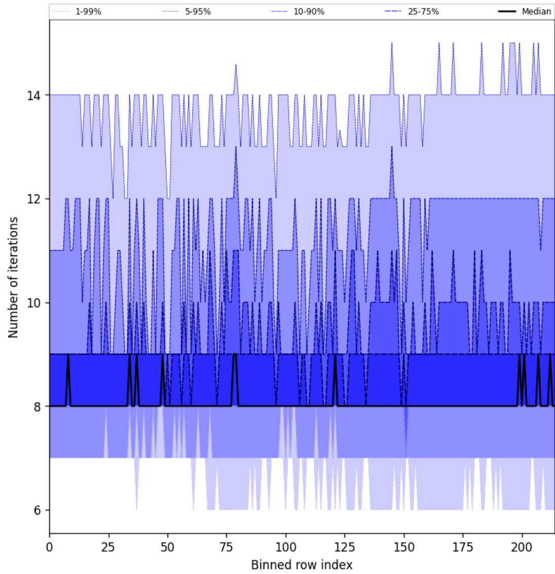
Figure 32: Along track statistics of “Number of iterations” for 2025-02-13 to 2025-02-14
