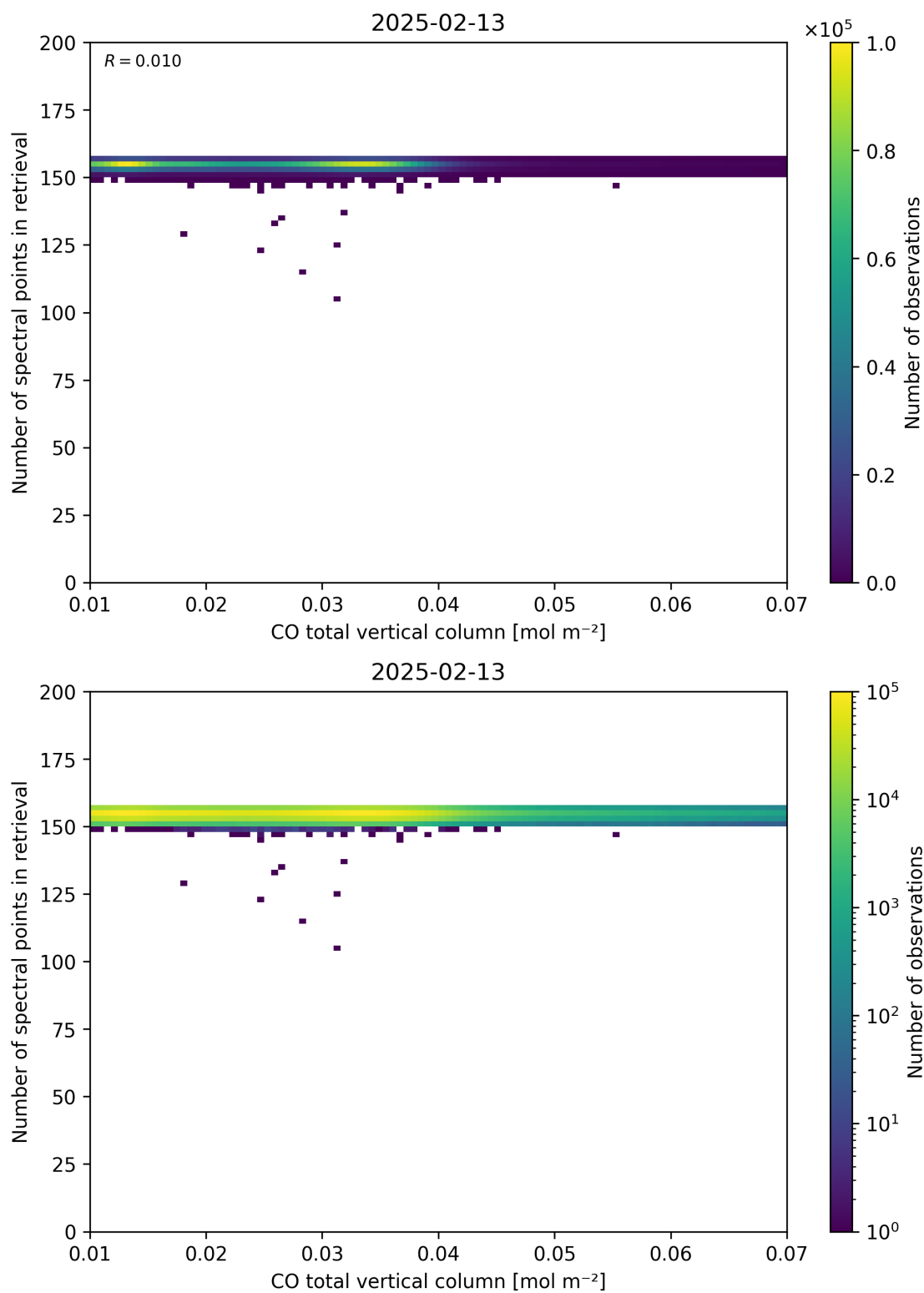
Figure 43: Scatter density plot of “CO total vertical column” against “Number of spectral points in retrieval” for 2025-02-13 to 2025-02-14.
