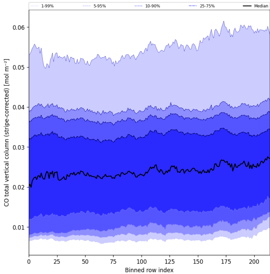
Figure 27: Along track statistics of “CO total vertical column (stripe-corrected)” for 2025-02-13 to 2025-02-14
