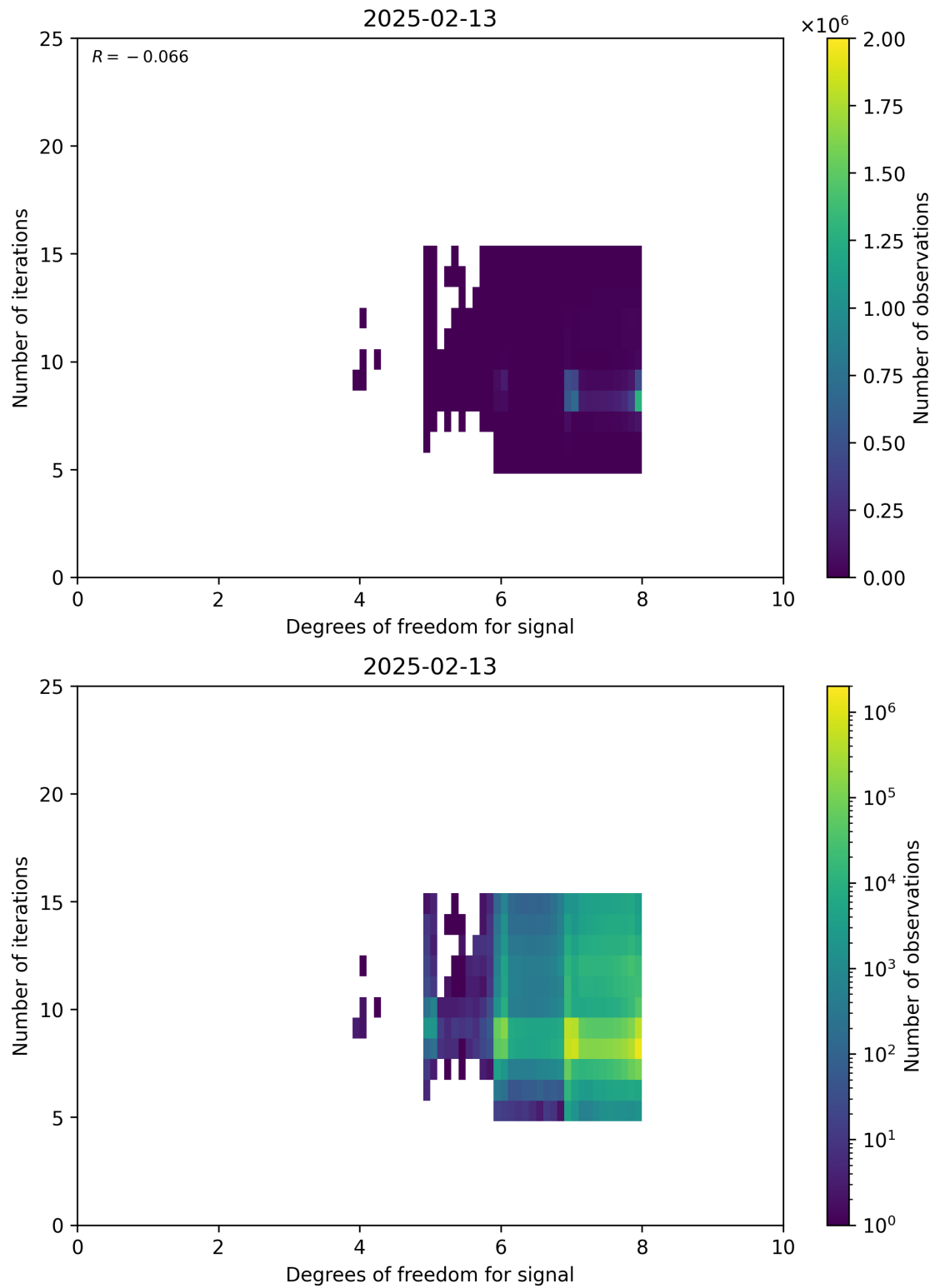
Figure 50: Scatter density plot of “Degrees of freedom for signal” against “Number of iterations” for 2025-02-13 to 2025-02-14.
