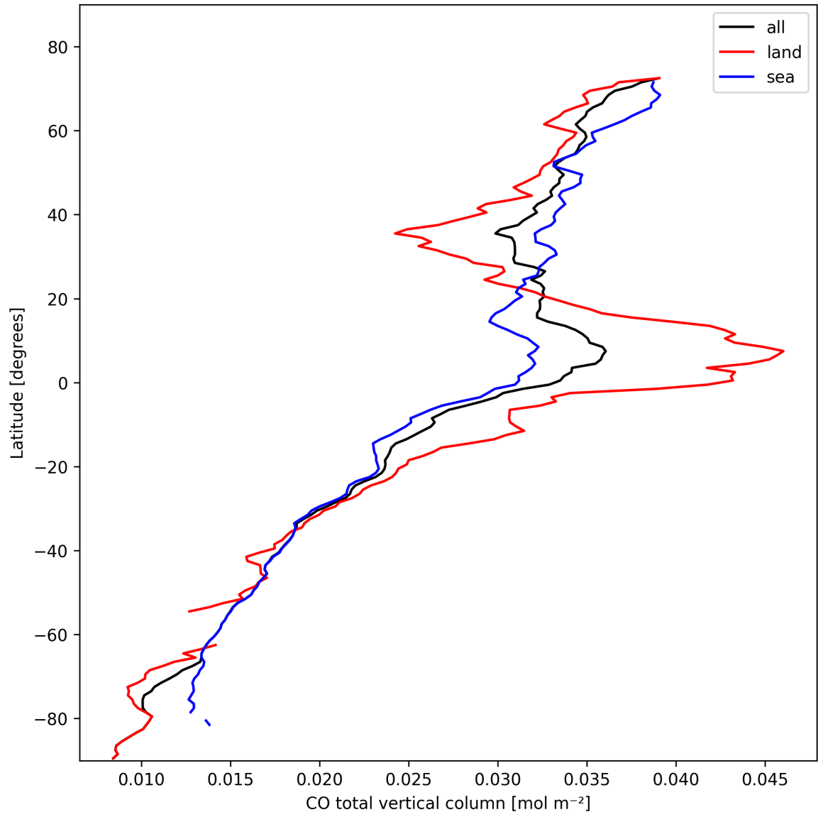
Figure 10: Zonal average of “CO total vertical column” for 2025-02-13 to 2025-02-14.
