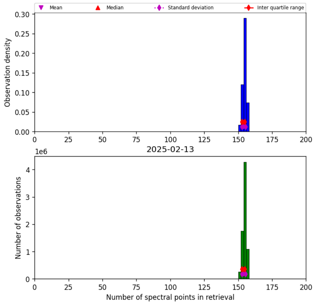
Figure 21: Histogram of “Number of spectral points in retrieval” for 2025-02-13 to 2025-02-14
