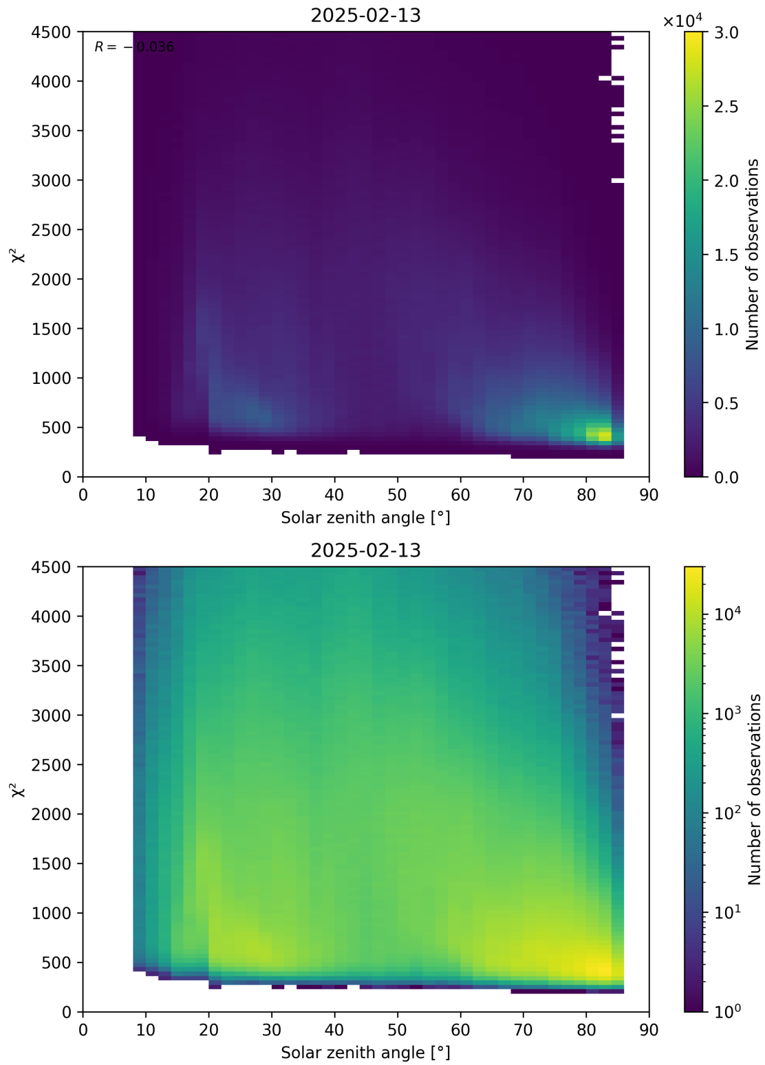
Figure 64: Scatter density plot of “Solar zenith angle” against “ \chi^2 ” for 2025-02-13 to 2025-02-14.
