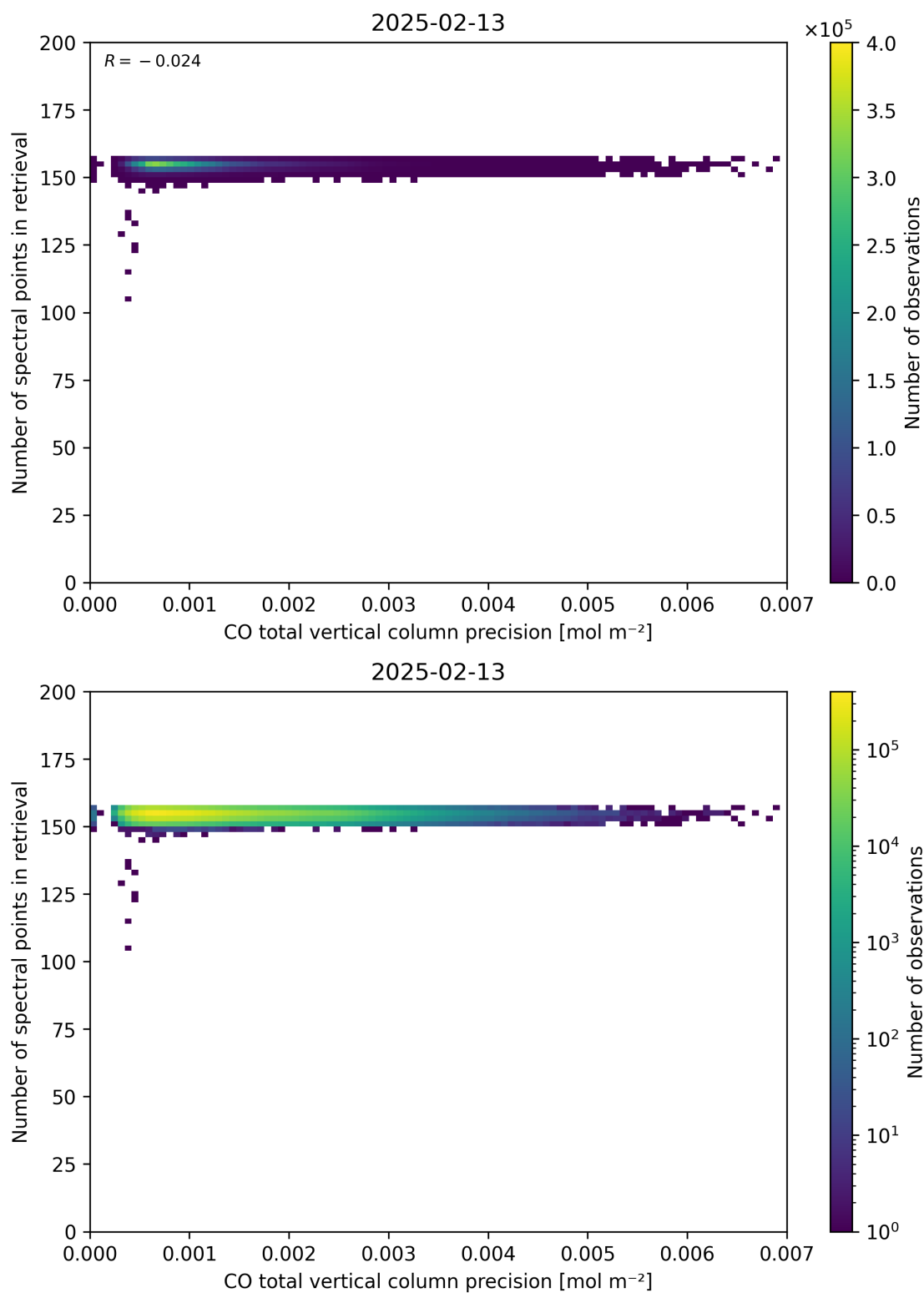
Figure 47: Scatter density plot of “CO total vertical column precision” against “Number of spectral points in retrieval” for 2025-02-13 to 2025-02-14.
