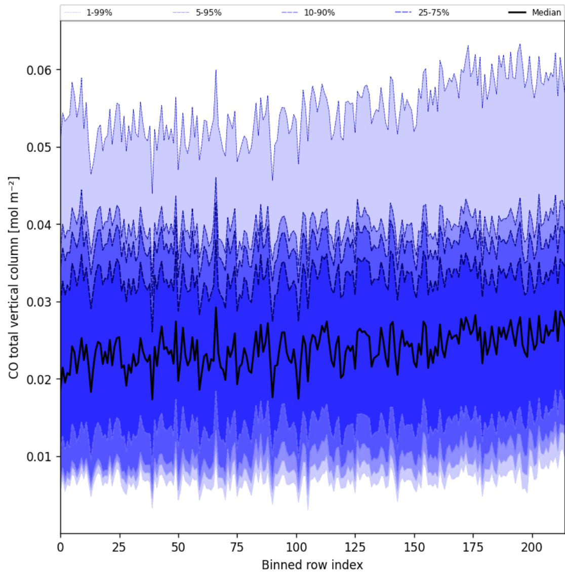
Figure 26: Along track statistics of “CO total vertical column” for 2025-02-13 to 2025-02-14
