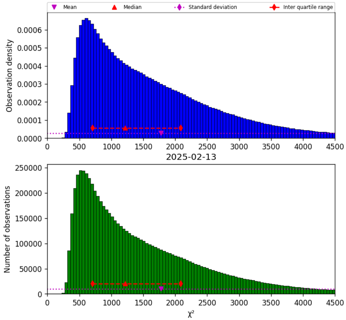
Figure 22: Histogram of “ \chi^2 ” for 2025-02-13 to 2025-02-14
