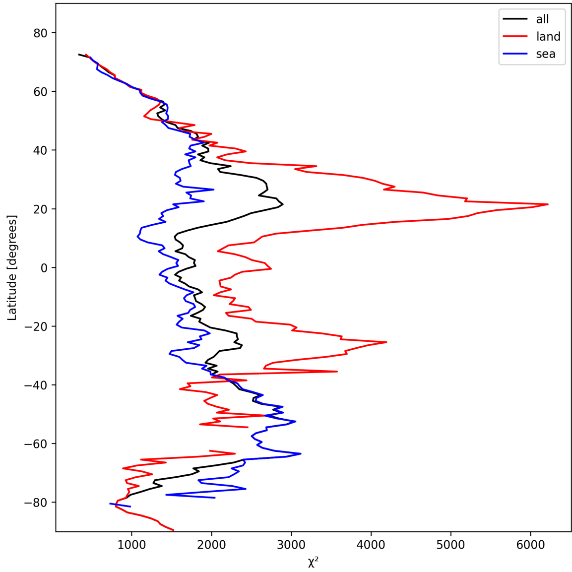
Figure 14: Zonal average of “ \chi^2 ” for 2025-02-13 to 2025-02-14.
