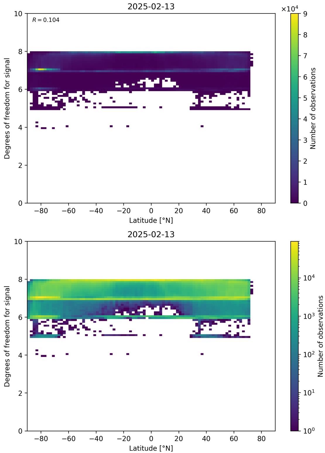
Figure 55: Scatter density plot of “Latitude” against “Degrees of freedom for signal” for 2025-02-13 to 2025-02-14.
