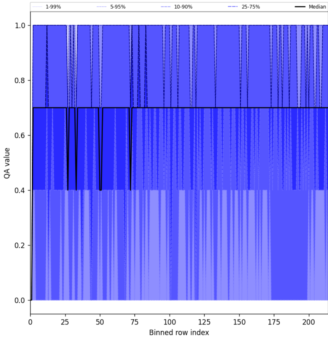
Figure 25: Along track statistics of “QA value” for 2025-02-13 to 2025-02-14
