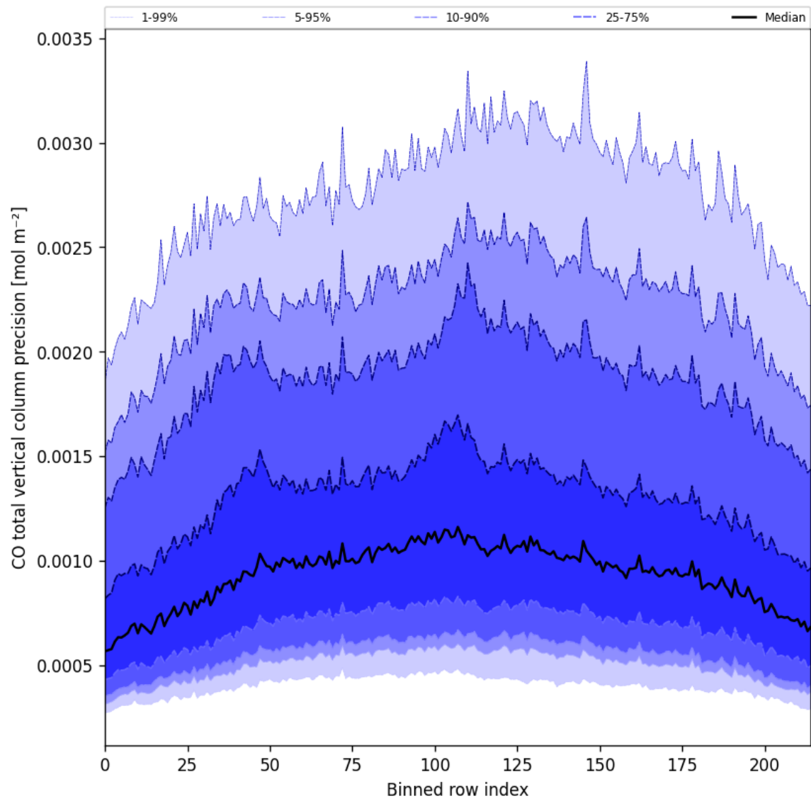
Figure 28: Along track statistics of “CO total vertical column precision” for 2025-02-13 to 2025-02-14
