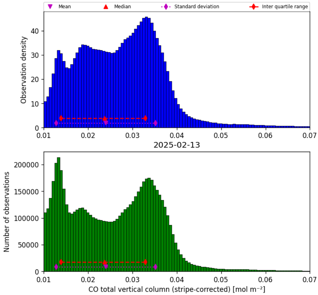
Figure 19: Histogram of “CO total vertical column (stripe-corrected)” for 2025-02-13 to 2025-02-14
