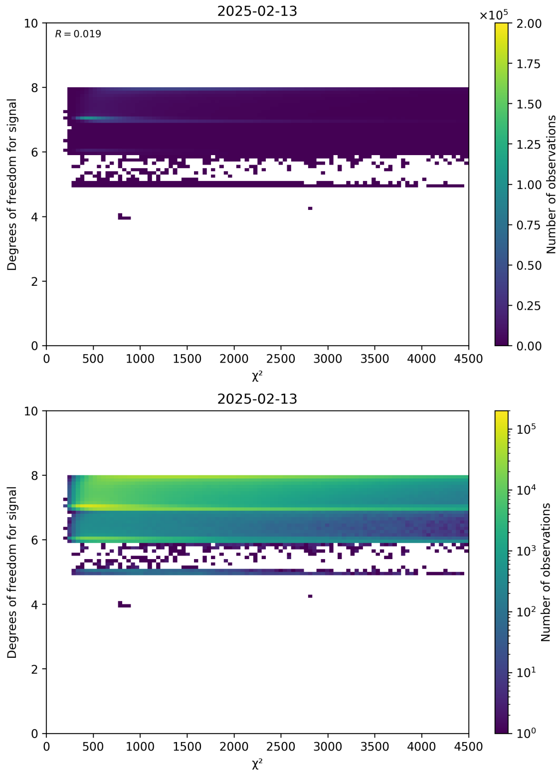
Figure 48: Scatter density plot of “ \chi^2 ” against “Degrees of freedom for signal” for 2025-02-13 to 2025-02-14.
