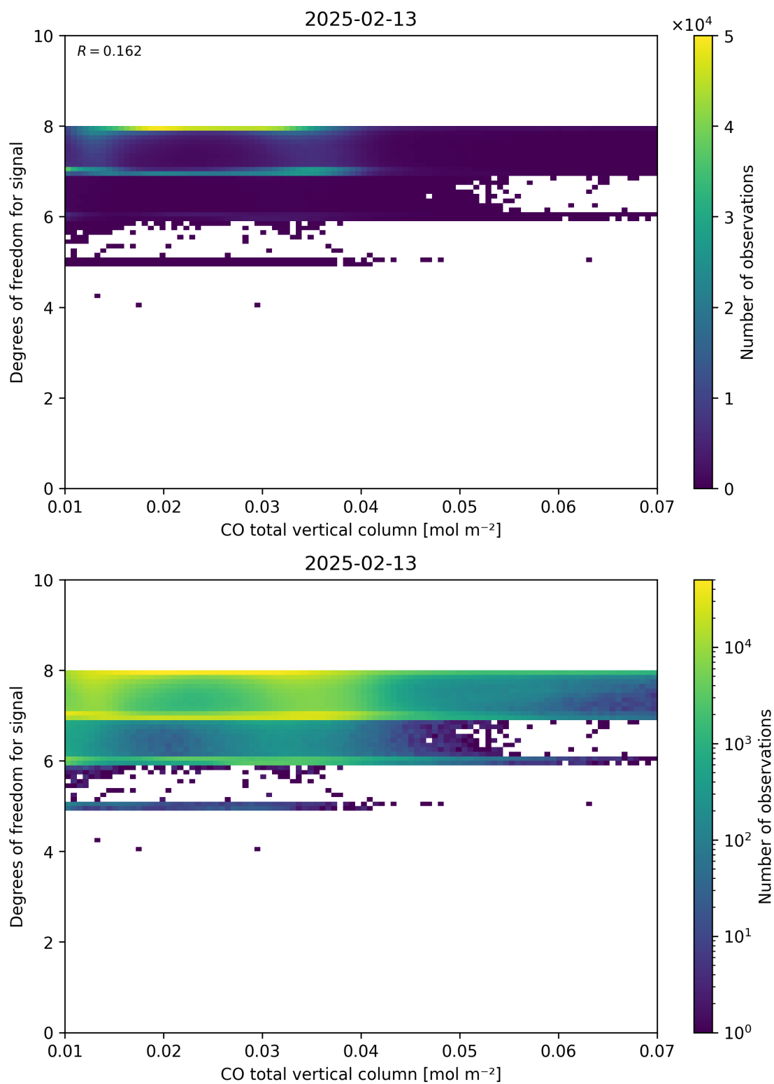
Figure 41: Scatter density plot of “CO total vertical column” against “Degrees of freedom for signal” for 2025-02-13 to 2025-02-14.
