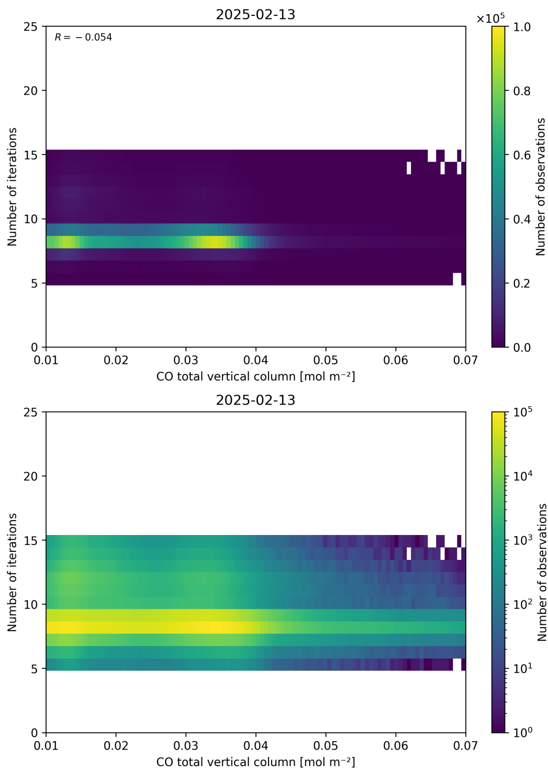
Figure 42: Scatter density plot of “CO total vertical column” against “Number of iterations” for 2025-02-13 to 2025-02-14.
