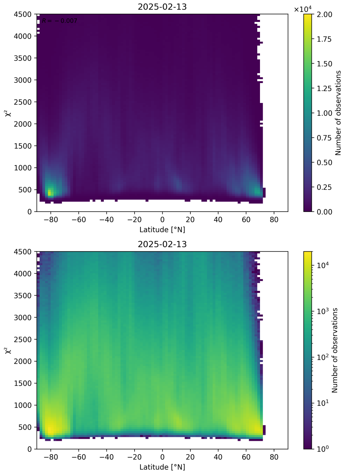
Figure 54: Scatter density plot of “Latitude” against “ \chi^2 ” for 2025-02-13 to 2025-02-14.
