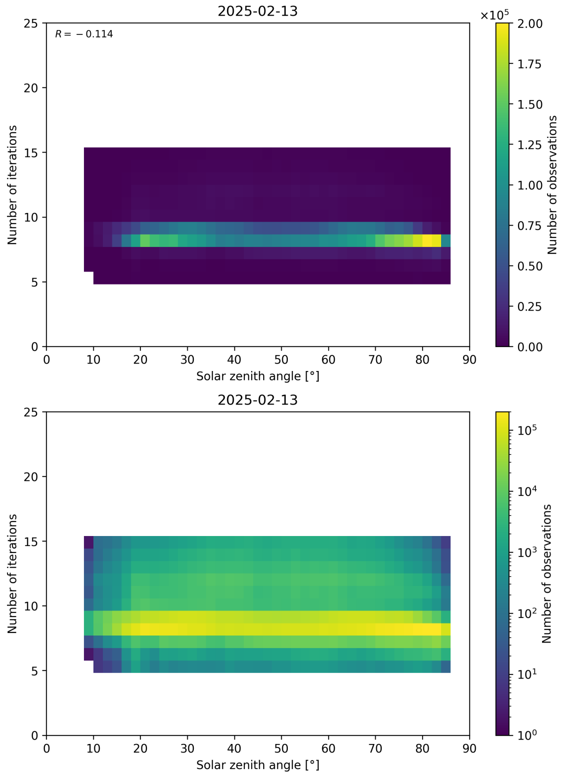
Figure 67: Scatter density plot of “Solar zenith angle” against “Number of iterations” for 2025-02-13 to 2025-02-14.
