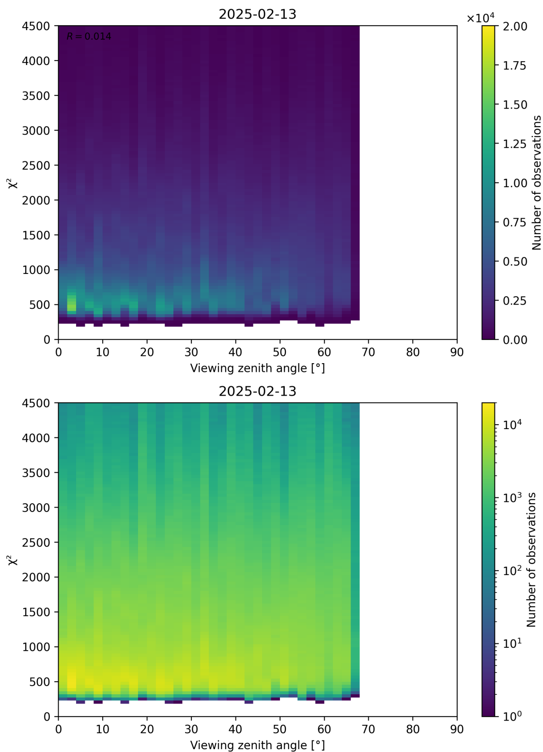
Figure 72: Scatter density plot of “Viewing zenith angle” against “ \chi^2 ” for 2025-02-13 to 2025-02-14.
