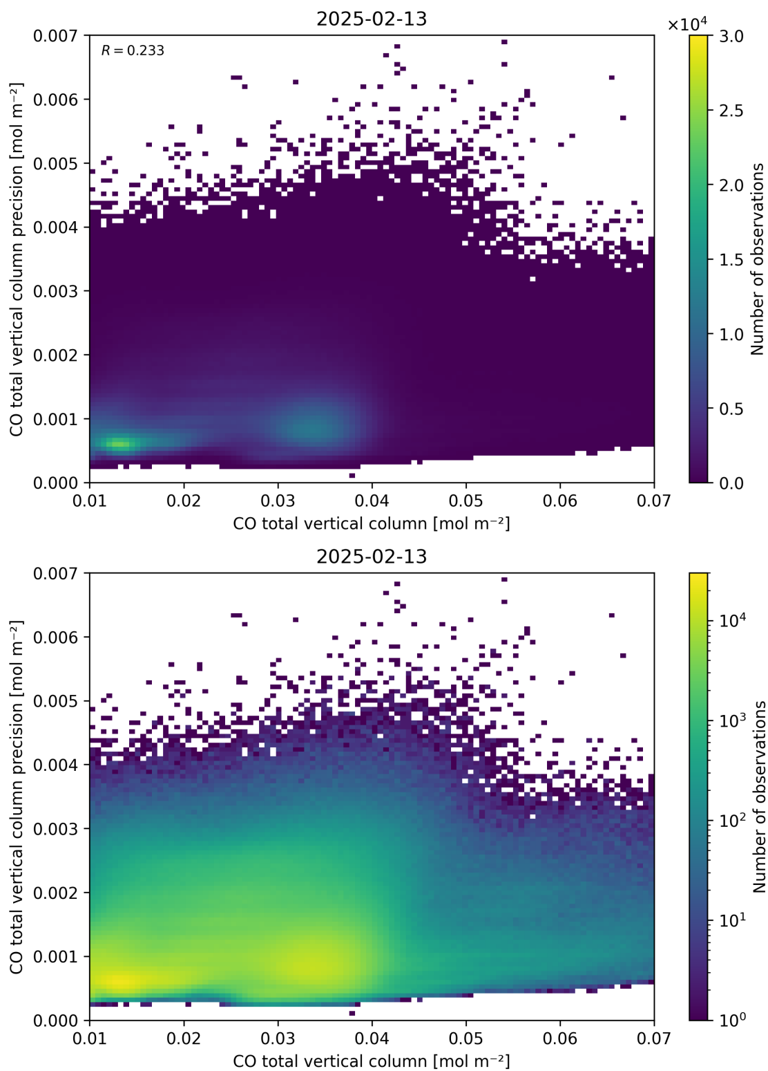
Figure 34: Scatter density plot of “CO total vertical column” against “CO total vertical column precision” for 2025-02-13 to 2025-02-14.
