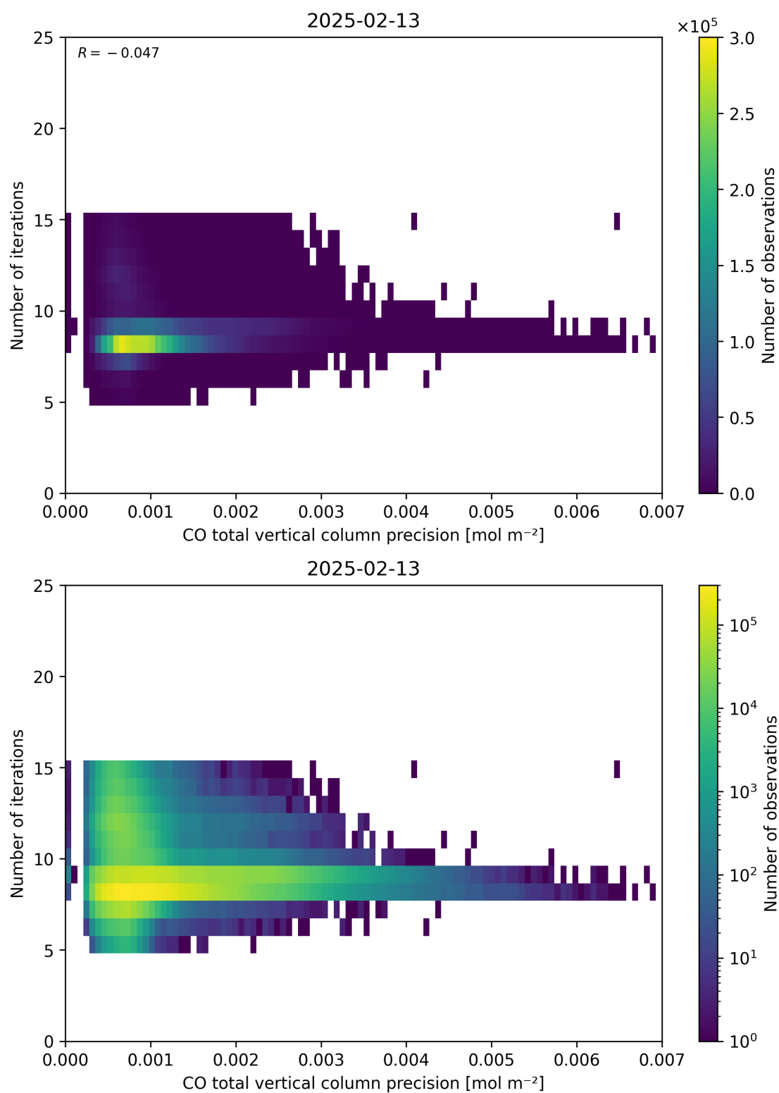
Figure 46: Scatter density plot of “CO total vertical column precision” against “Number of iterations” for 2025-02-13 to 2025-02-14.
