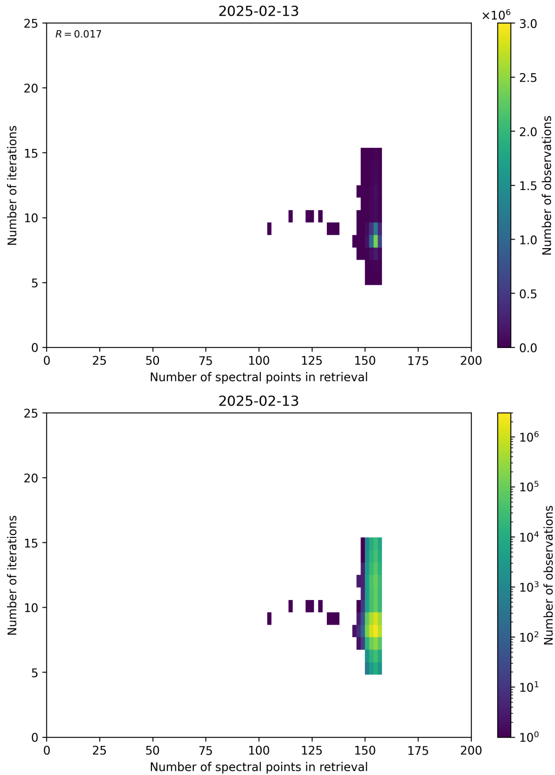
Figure 60: Scatter density plot of “Number of spectral points in retrieval” against “Number of iterations” for 2025-02-13 to 2025-02-14.
