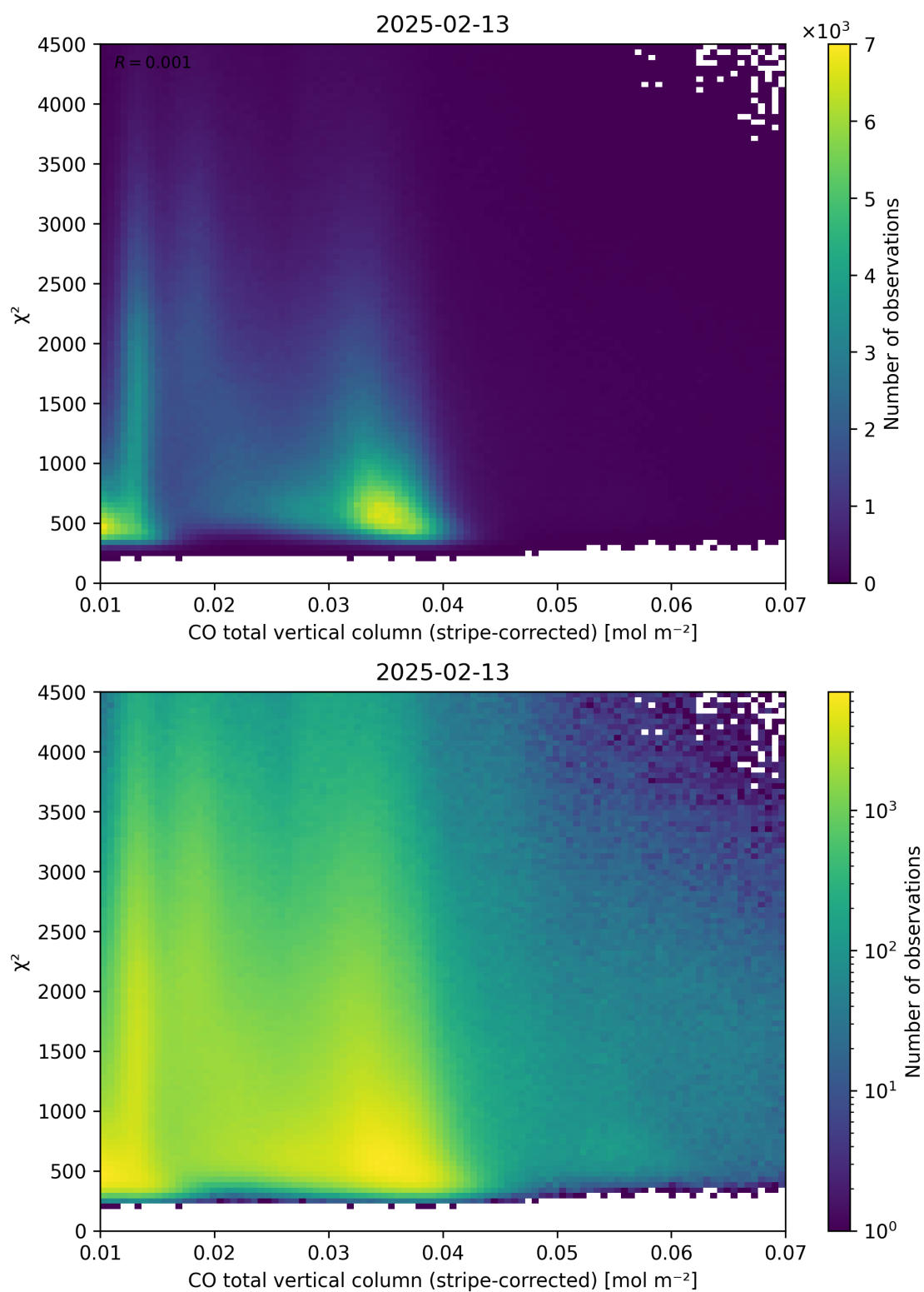
Figure 37: Scatter density plot of “CO total vertical column (stripe-corrected)” against “ \chi^2 ” for 2025-02-13 to 2025-02-14.
