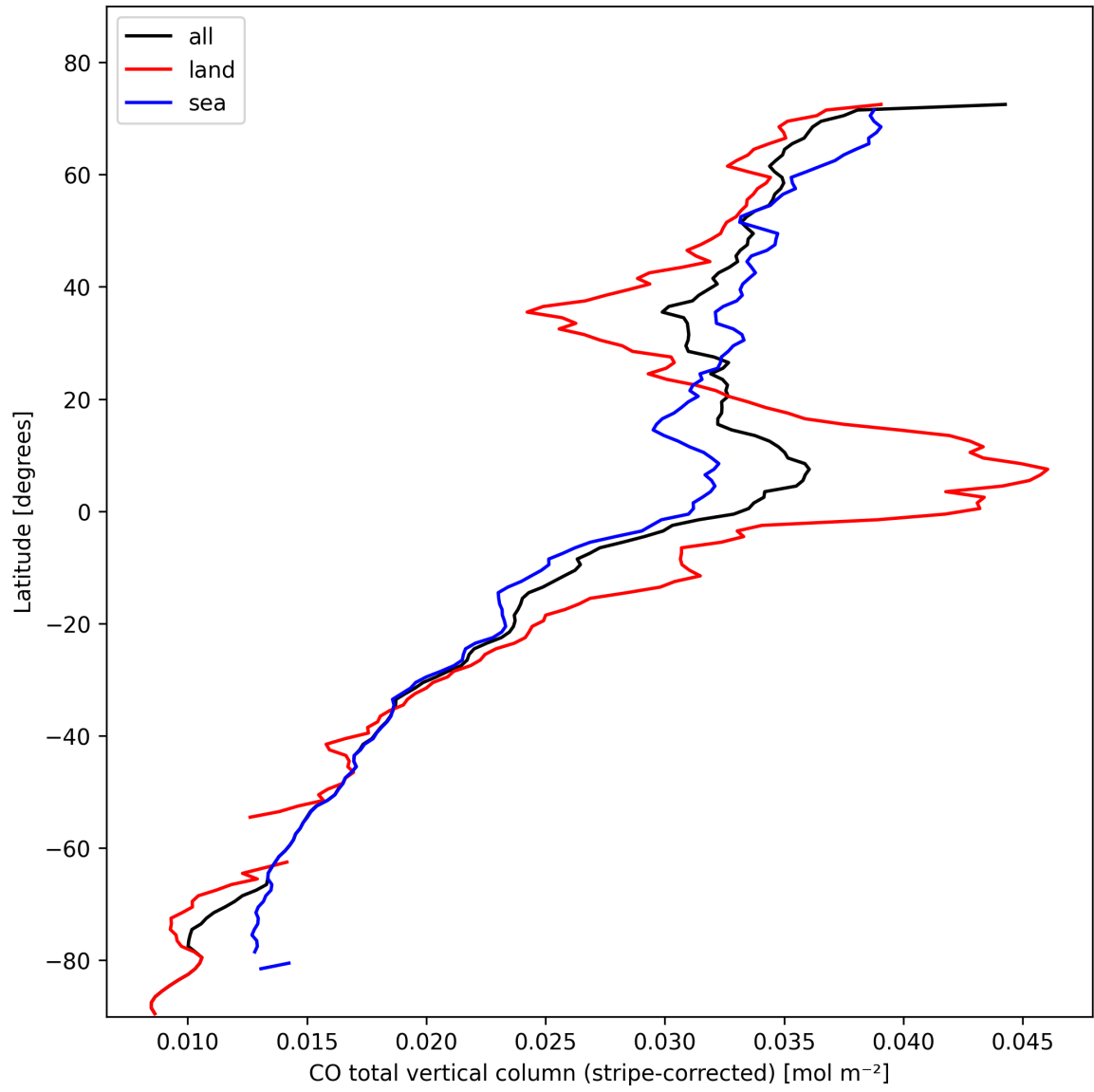
Figure 11: Zonal average of “CO total vertical column (stripe-corrected)” for 2025-02-13 to 2025-02-14.
