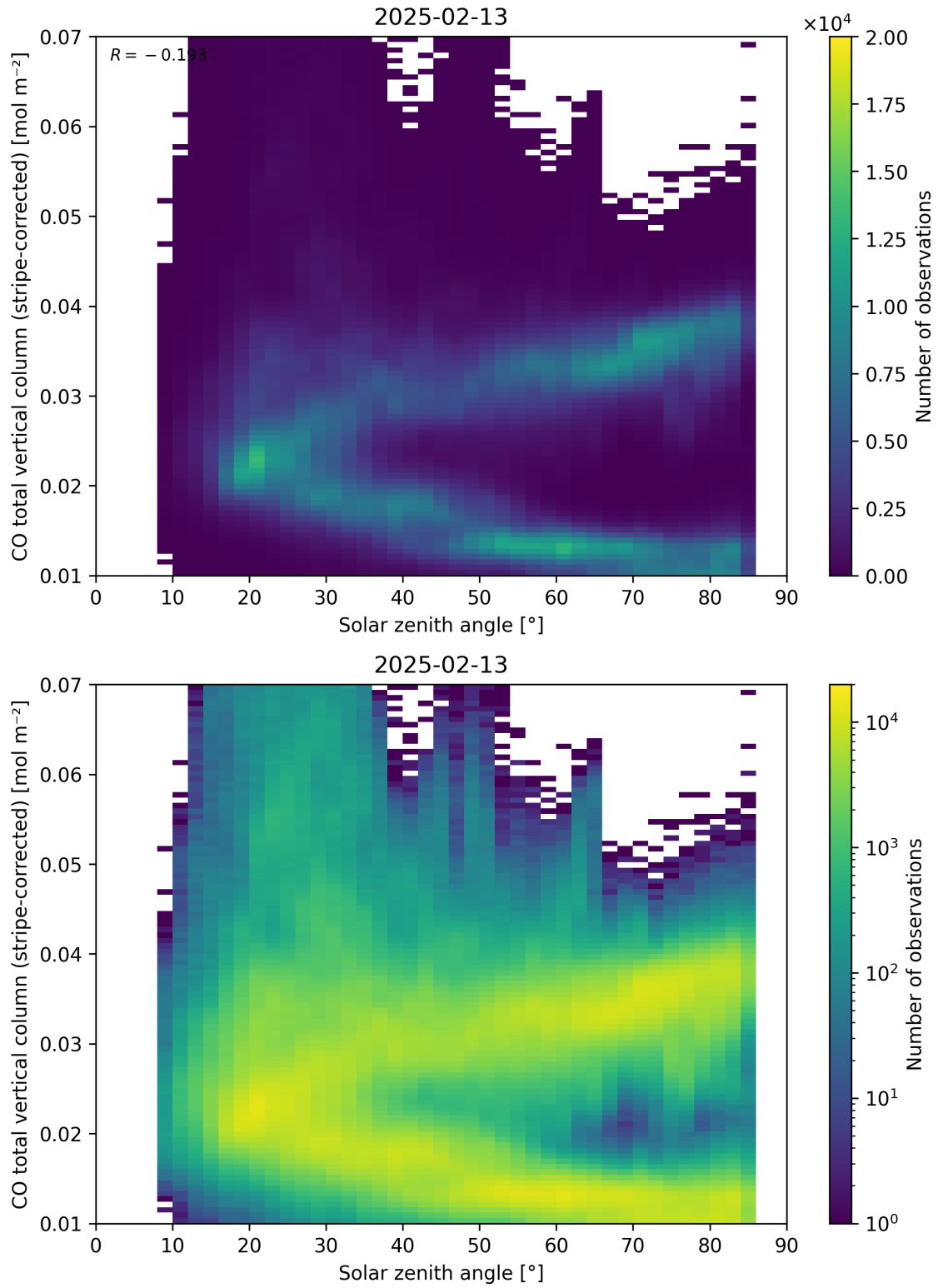
Figure 62: Scatter density plot of “Solar zenith angle” against “CO total vertical column (stripe-corrected)” for 2025-02-13 to 2025-02-14.
