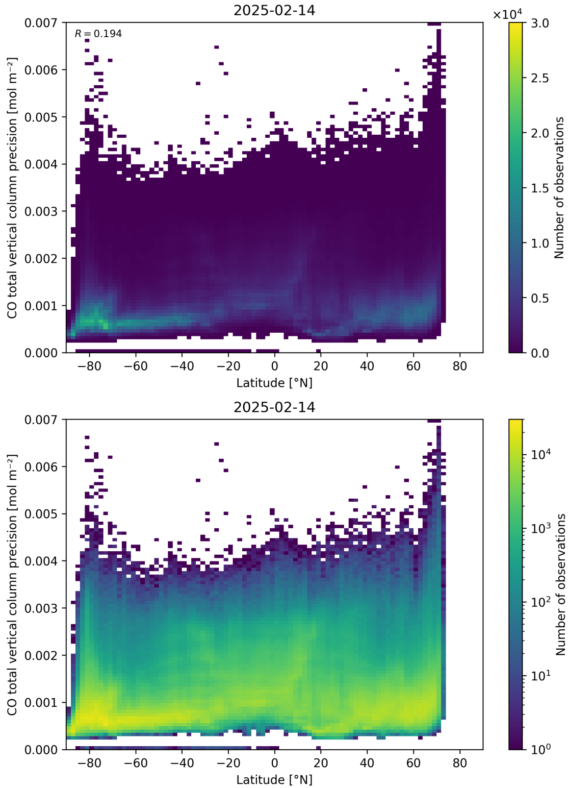
Figure 53: Scatter density plot of “Latitude” against “CO total vertical column precision” for 2025-02-13 to 2025-02-15.
