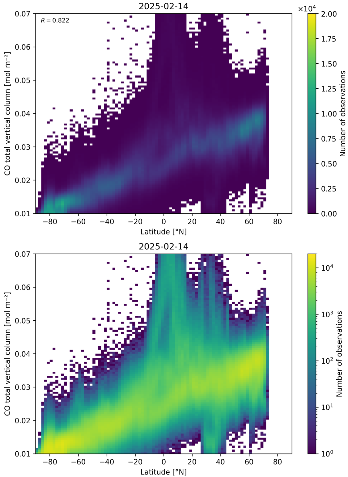
Figure 51: Scatter density plot of “Latitude” against “CO total vertical column” for 2025-02-13 to 2025-02-15.
