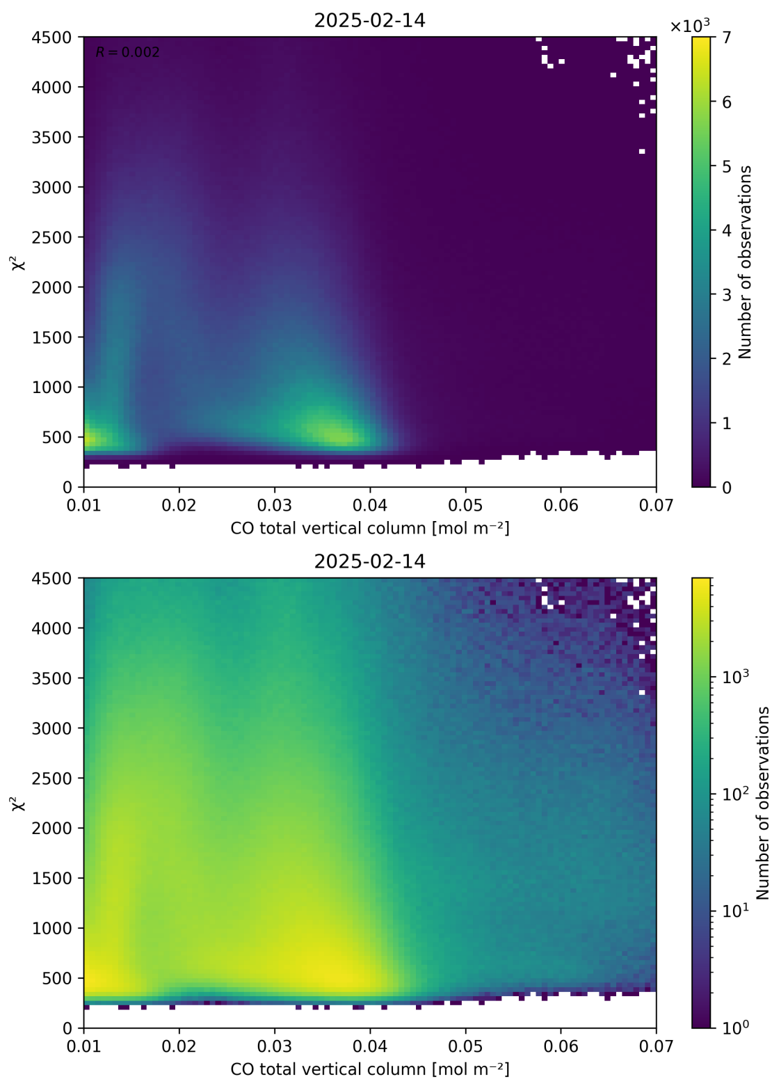
Figure 35: Scatter density plot of “CO total vertical column” against “ \chi^2 ” for 2025-02-13 to 2025-02-15.
