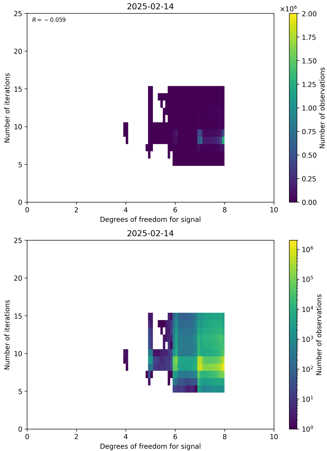
Figure 50: Scatter density plot of “Degrees of freedom for signal” against “Number of iterations” for 2025-02-13 to 2025-02-15.
