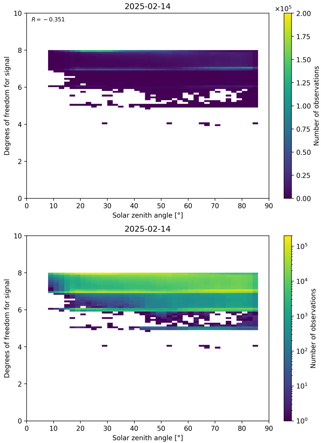
Figure 65: Scatter density plot of “Solar zenith angle” against “Degrees of freedom for signal” for 2025-02-13 to 2025-02-15.
