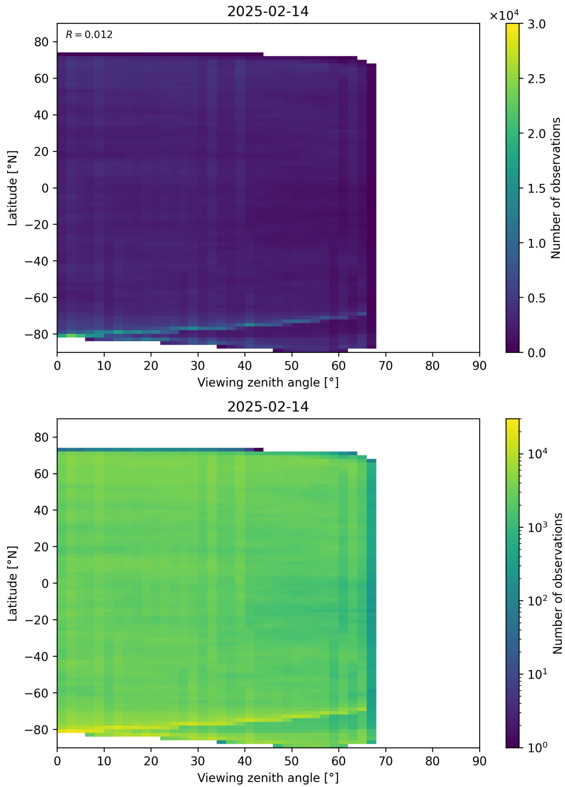
Figure 74: Scatter density plot of “Viewing zenith angle” against “Latitude” for 2025-02-13 to 2025-02-15.
