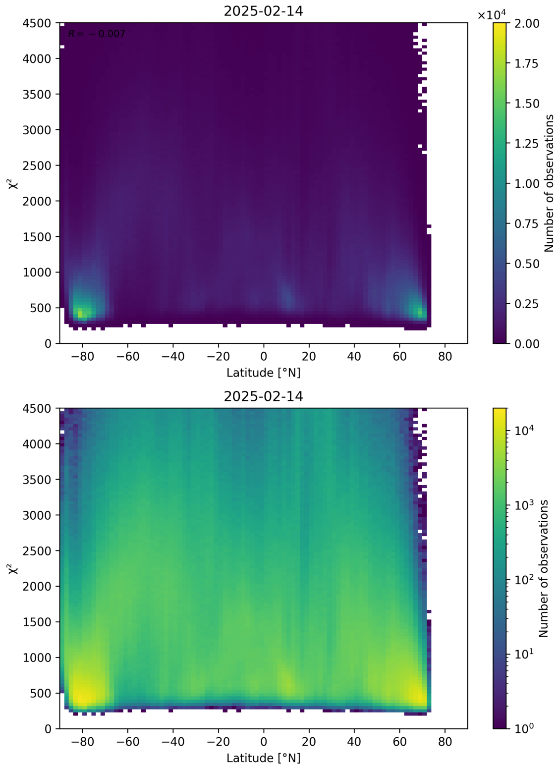
Figure 54: Scatter density plot of “Latitude” against “ \chi^2 ” for 2025-02-13 to 2025-02-15.
