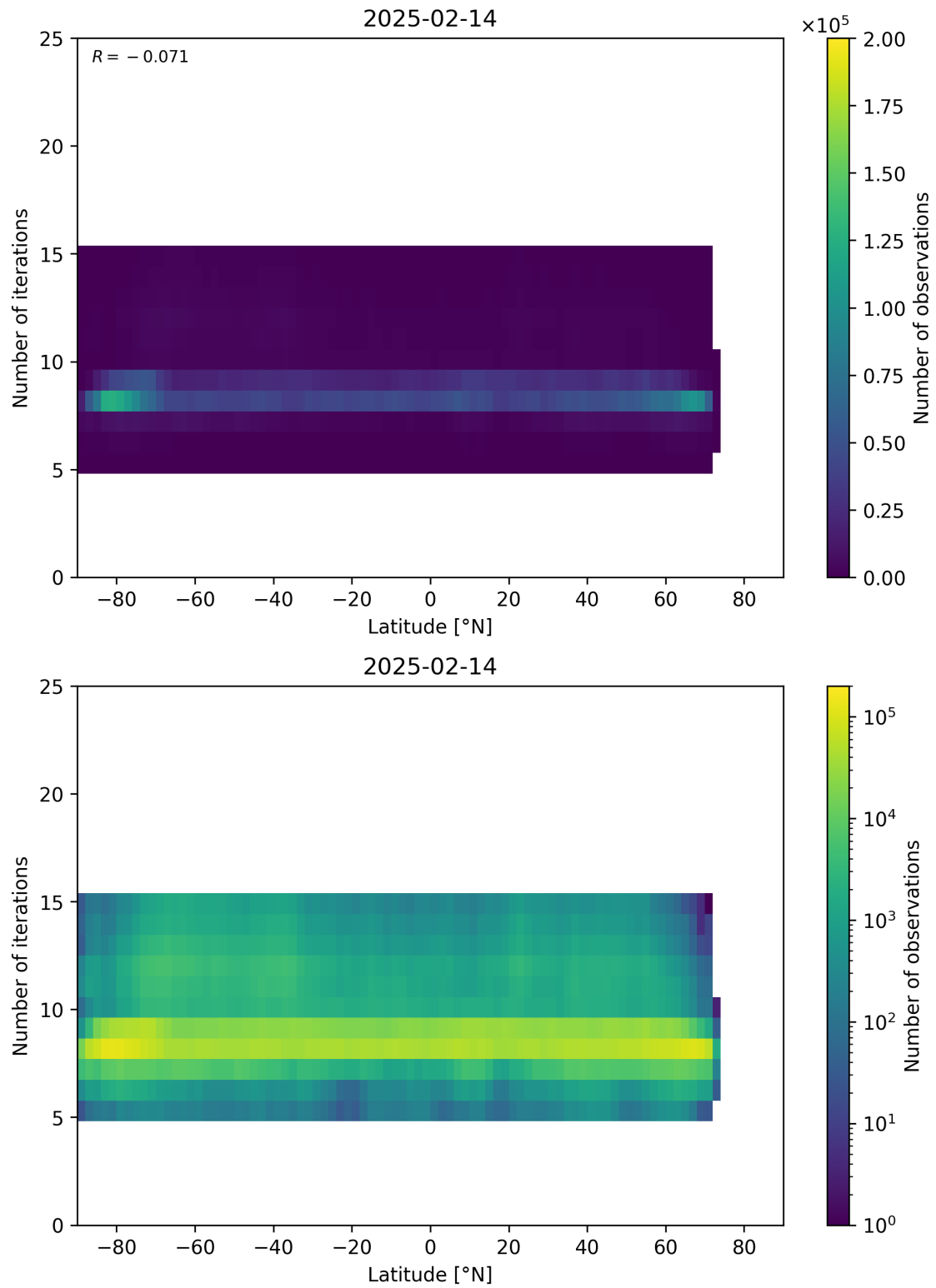
Figure 56: Scatter density plot of “Latitude” against “Number of iterations” for 2025-02-13 to 2025-02-15.
