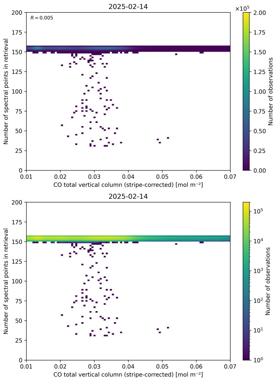
Figure 40: Scatter density plot of “CO total vertical column (stripe-corrected)” against “Number of spectral points in retrieval” for 2025-02-13 to 2025-02-15.
