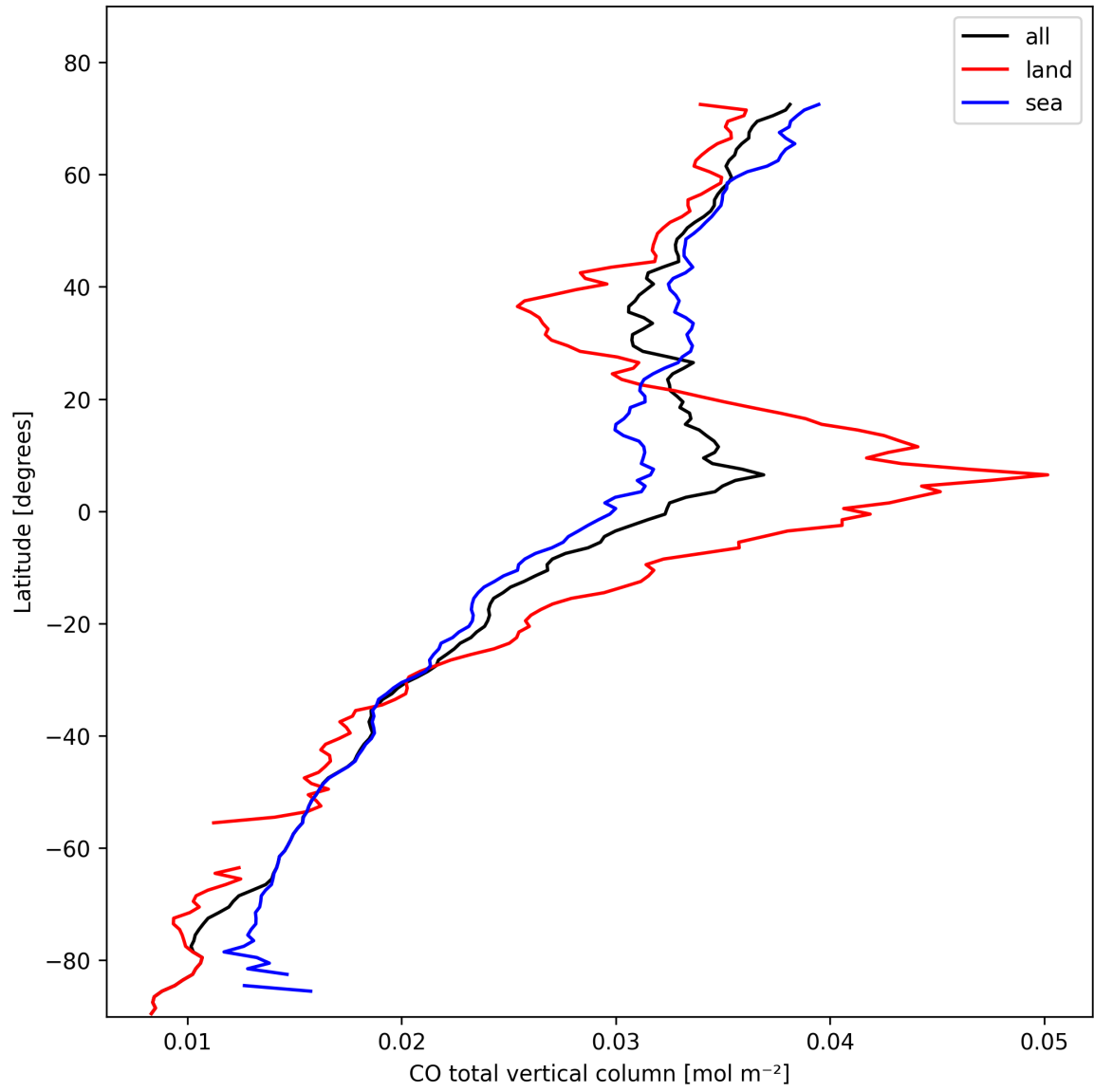
Figure 10: Zonal average of “CO total vertical column” for 2025-02-13 to 2025-02-15.
