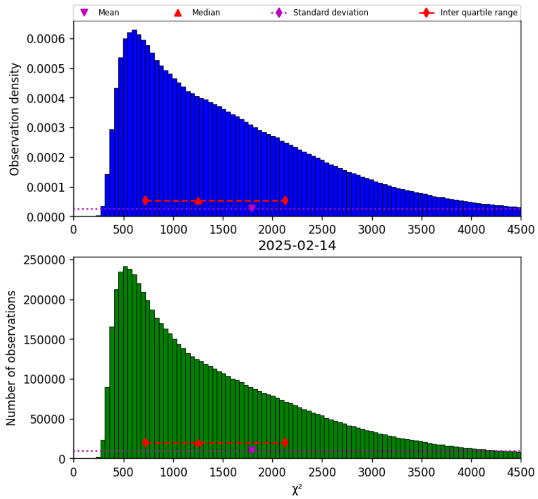
Figure 22: Histogram of “ \chi^2 ” for 2025-02-13 to 2025-02-15
