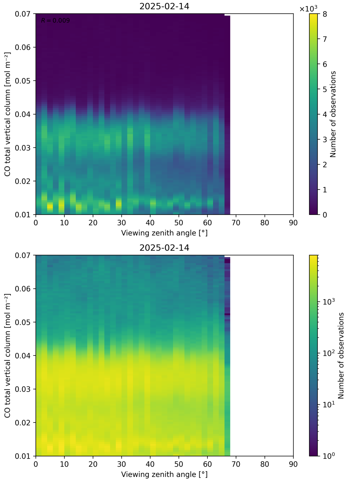
Figure 69: Scatter density plot of “Viewing zenith angle” against “CO total vertical column” for 2025-02-13 to 2025-02-15.
