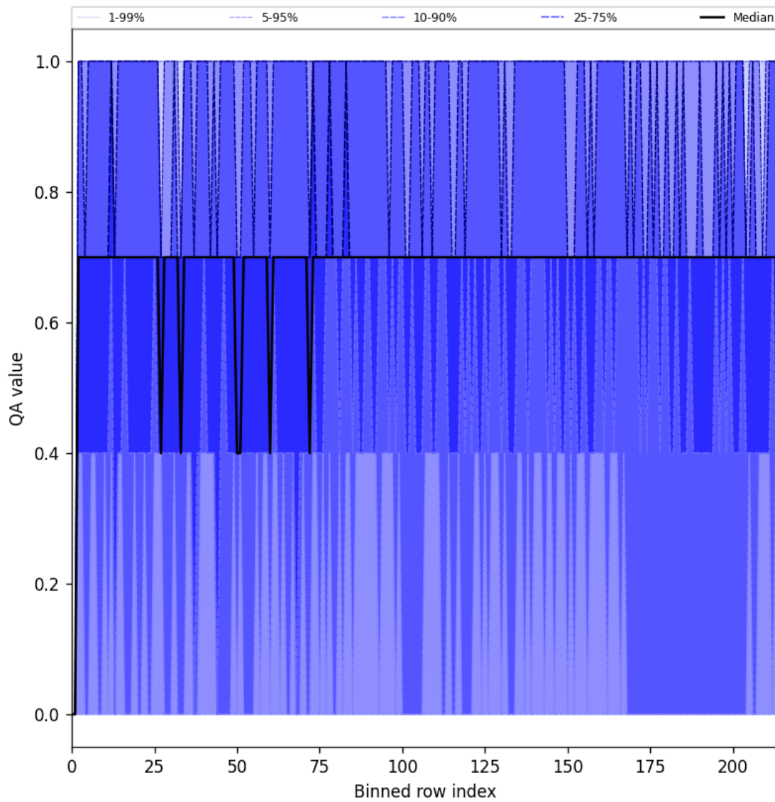
Figure 25: Along track statistics of “QA value” for 2025-02-13 to 2025-02-15
