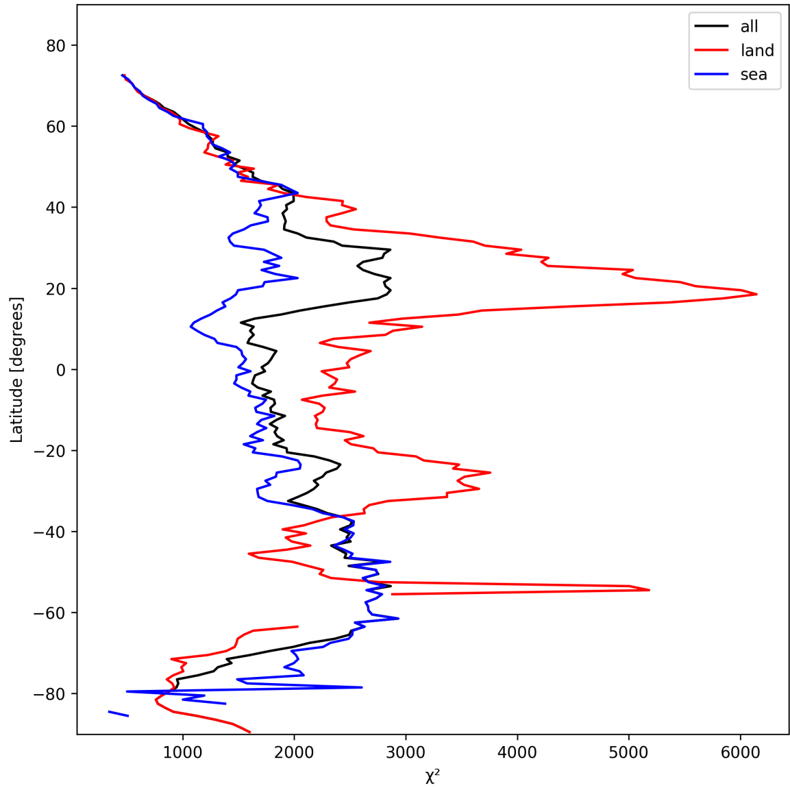
Figure 14: Zonal average of “ \chi^2 ” for 2025-02-13 to 2025-02-15.
