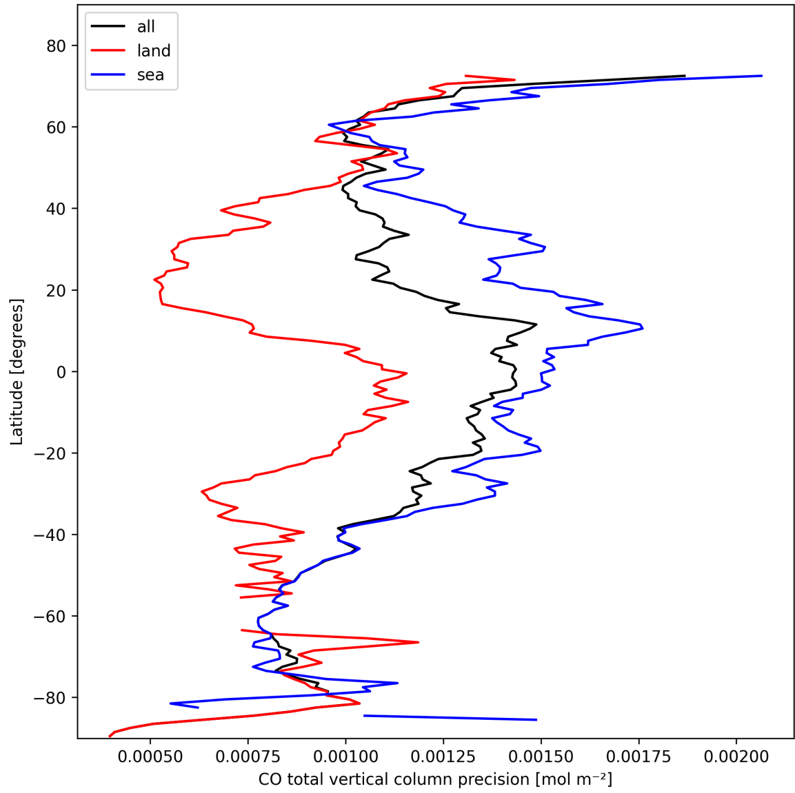
Figure 12: Zonal average of “CO total vertical column precision” for 2025-02-13 to 2025-02-15.
