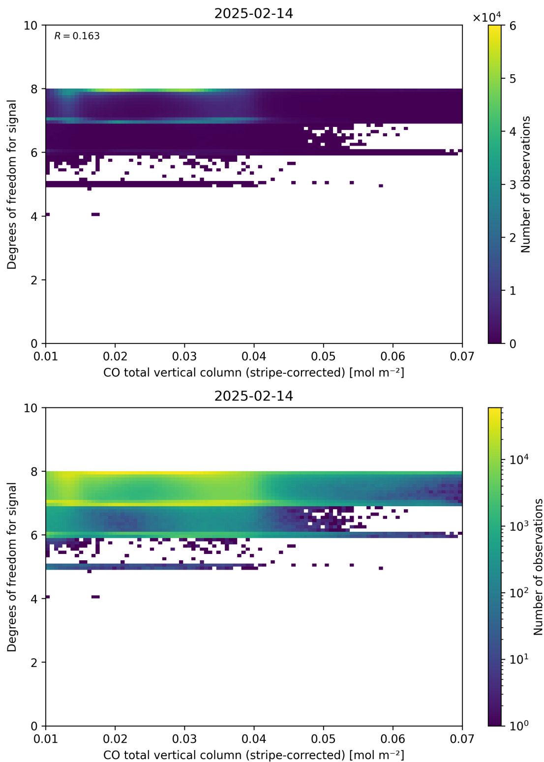
Figure 38: Scatter density plot of “CO total vertical column (stripe-corrected)” against “Degrees of freedom for signal” for 2025-02-13 to 2025-02-15.
