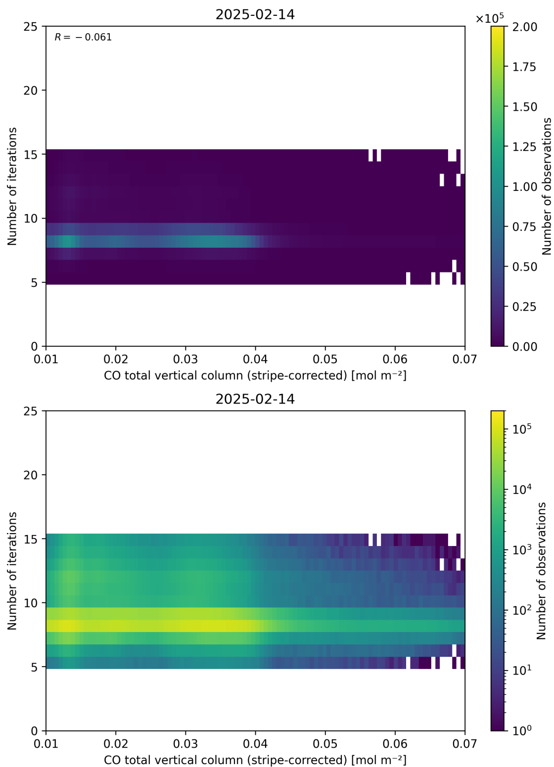
Figure 39: Scatter density plot of “CO total vertical column (stripe-corrected)” against “Number of iterations” for 2025-02-13 to 2025-02-15.
