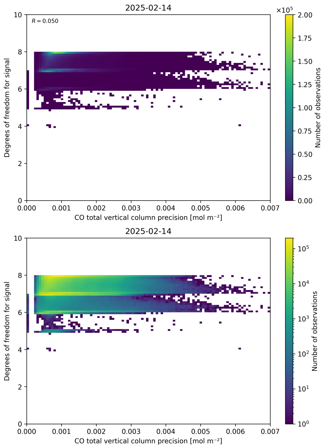
Figure 45: Scatter density plot of “CO total vertical column precision” against “Degrees of freedom for signal” for 2025-02-13 to 2025-02-15.
