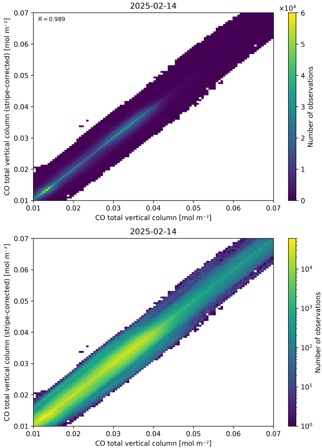
Figure 33: Scatter density plot of “CO total vertical column” against “CO total vertical column (stripe-corrected)” for 2025-02-13 to 2025-02-15.
