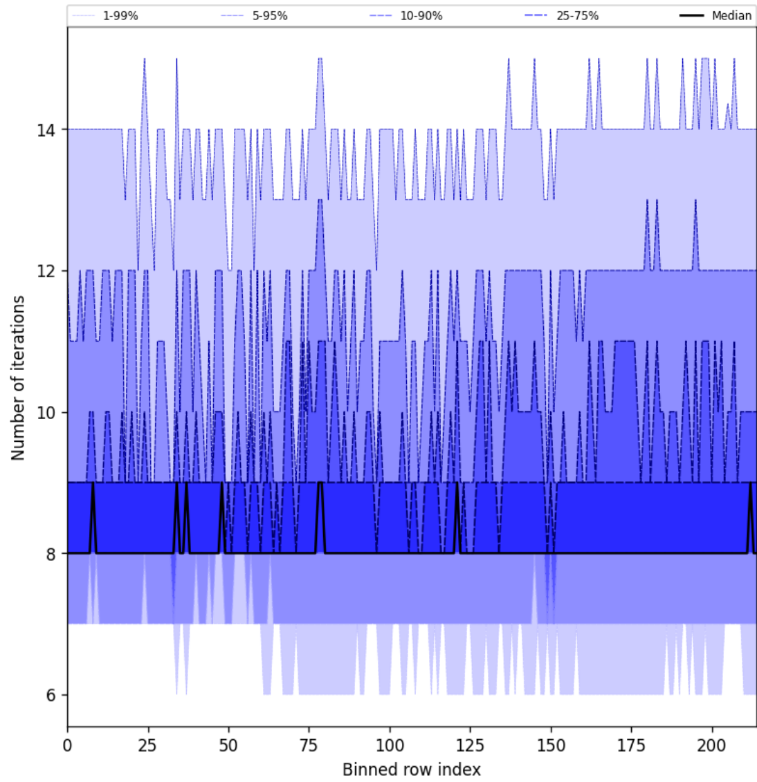
Figure 32: Along track statistics of “Number of iterations” for 2025-02-13 to 2025-02-15
