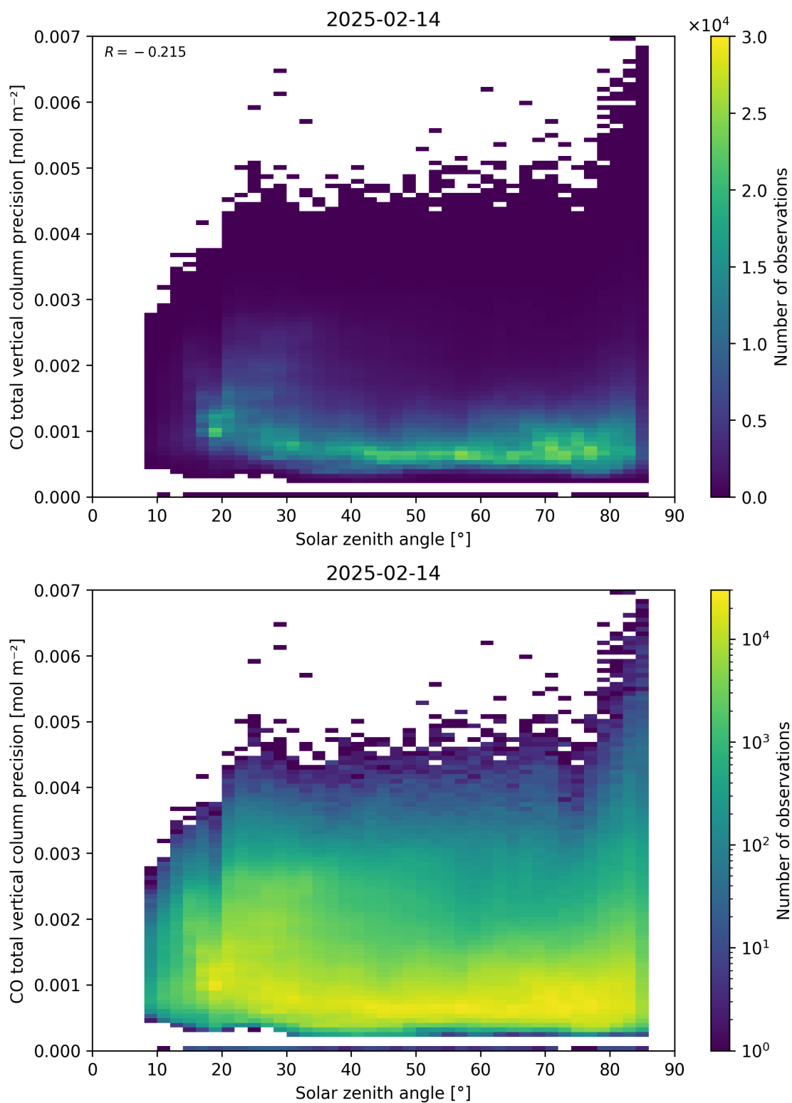
Figure 63: Scatter density plot of “Solar zenith angle” against “CO total vertical column precision” for 2025-02-13 to 2025-02-15.
