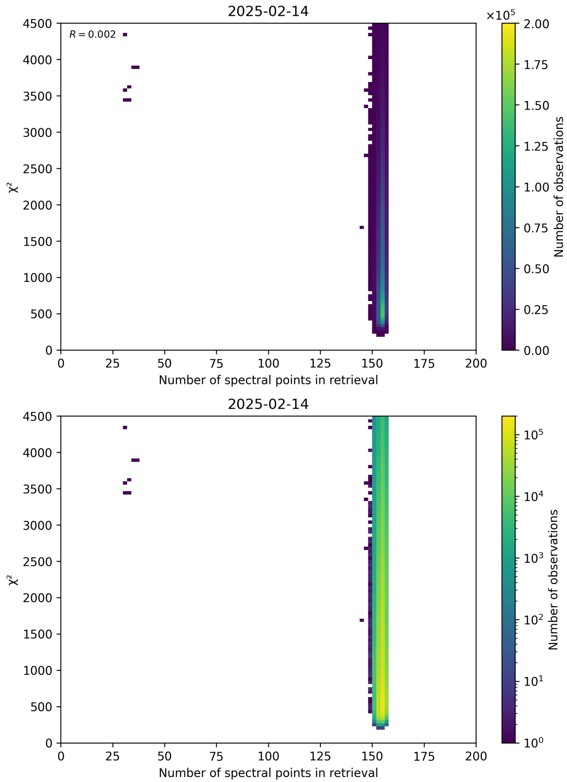
Figure 58: Scatter density plot of “Number of spectral points in retrieval” against “ \chi^2 ” for 2025-02-13 to 2025-02-15.
