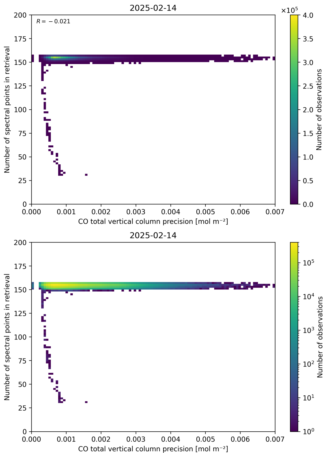
Figure 47: Scatter density plot of “CO total vertical column precision” against “Number of spectral points in retrieval” for 2025-02-13 to 2025-02-15.
