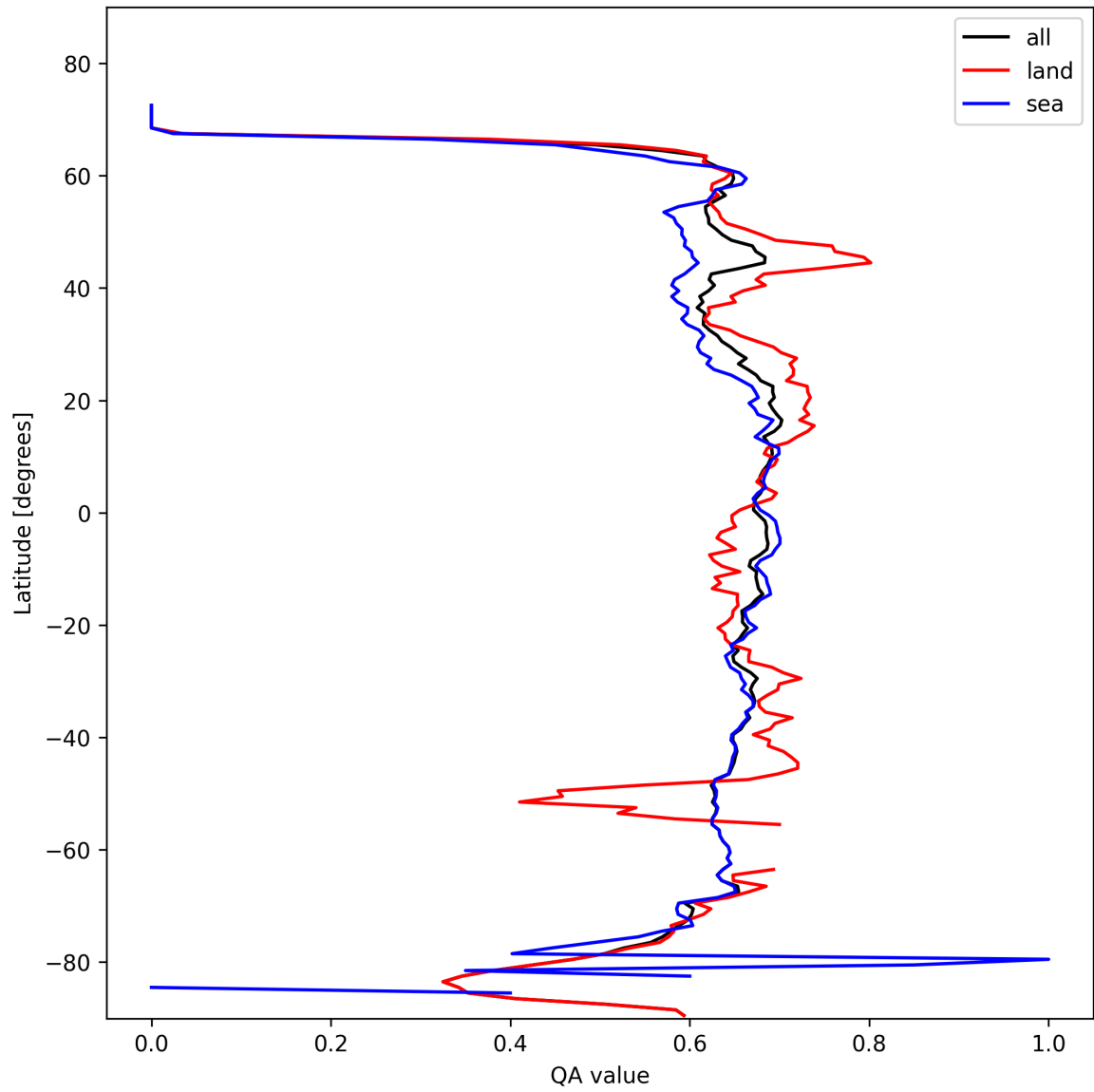
Figure 9: Zonal average of “QA value” for 2025-02-13 to 2025-02-15.
