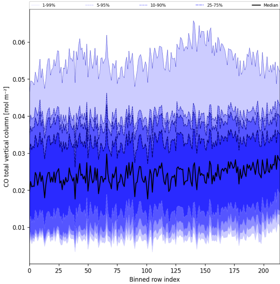
Figure 26: Along track statistics of “CO total vertical column” for 2025-02-13 to 2025-02-15
