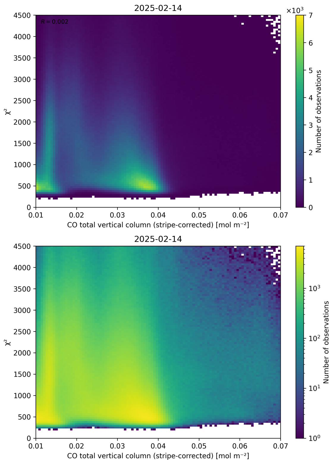
Figure 37: Scatter density plot of “CO total vertical column (stripe-corrected)” against “ \chi^2 ” for 2025-02-13 to 2025-02-15.
