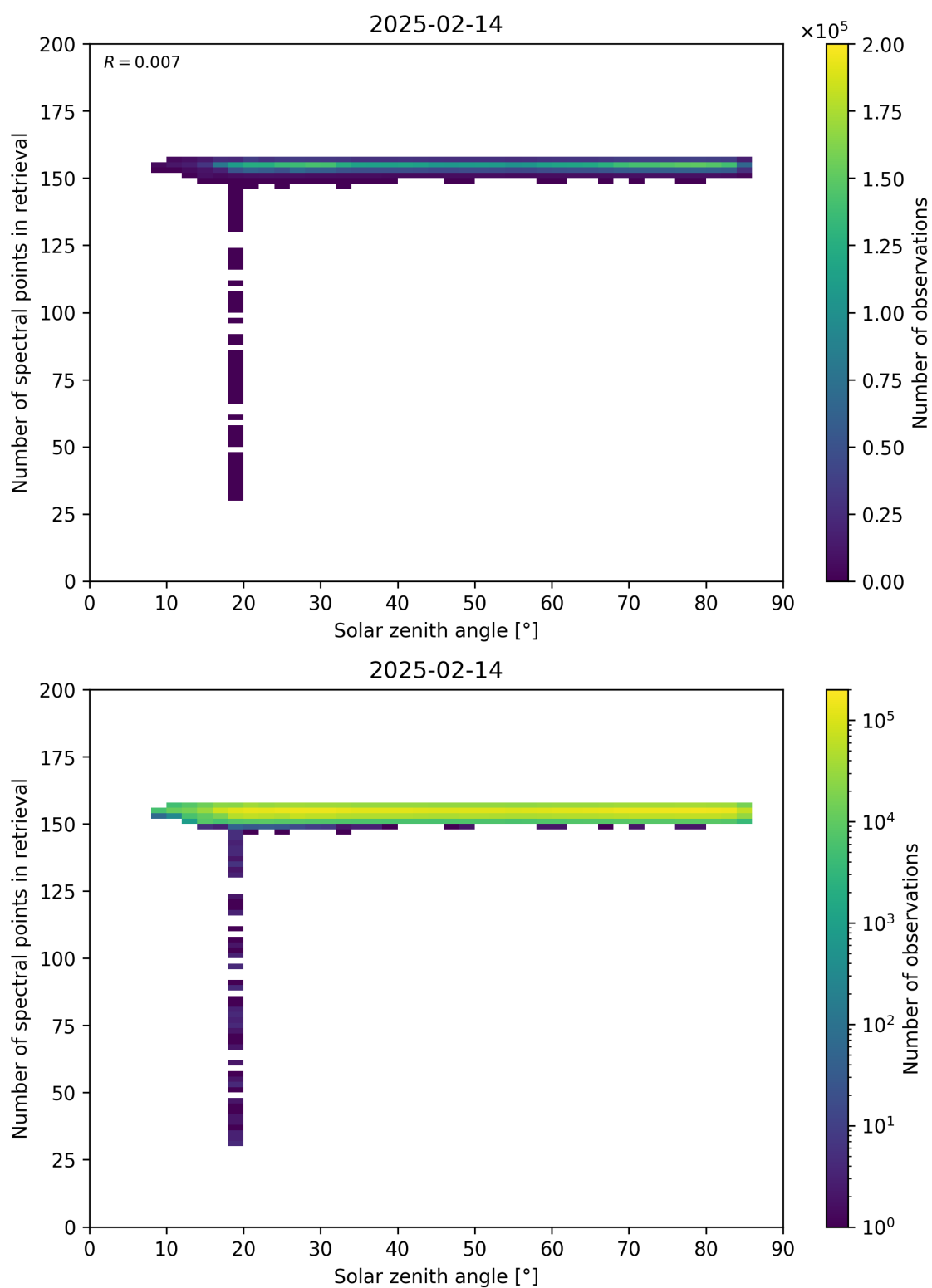
Figure 68: Scatter density plot of “Solar zenith angle” against “Number of spectral points in retrieval” for 2025-02-13 to 2025-02-15.
