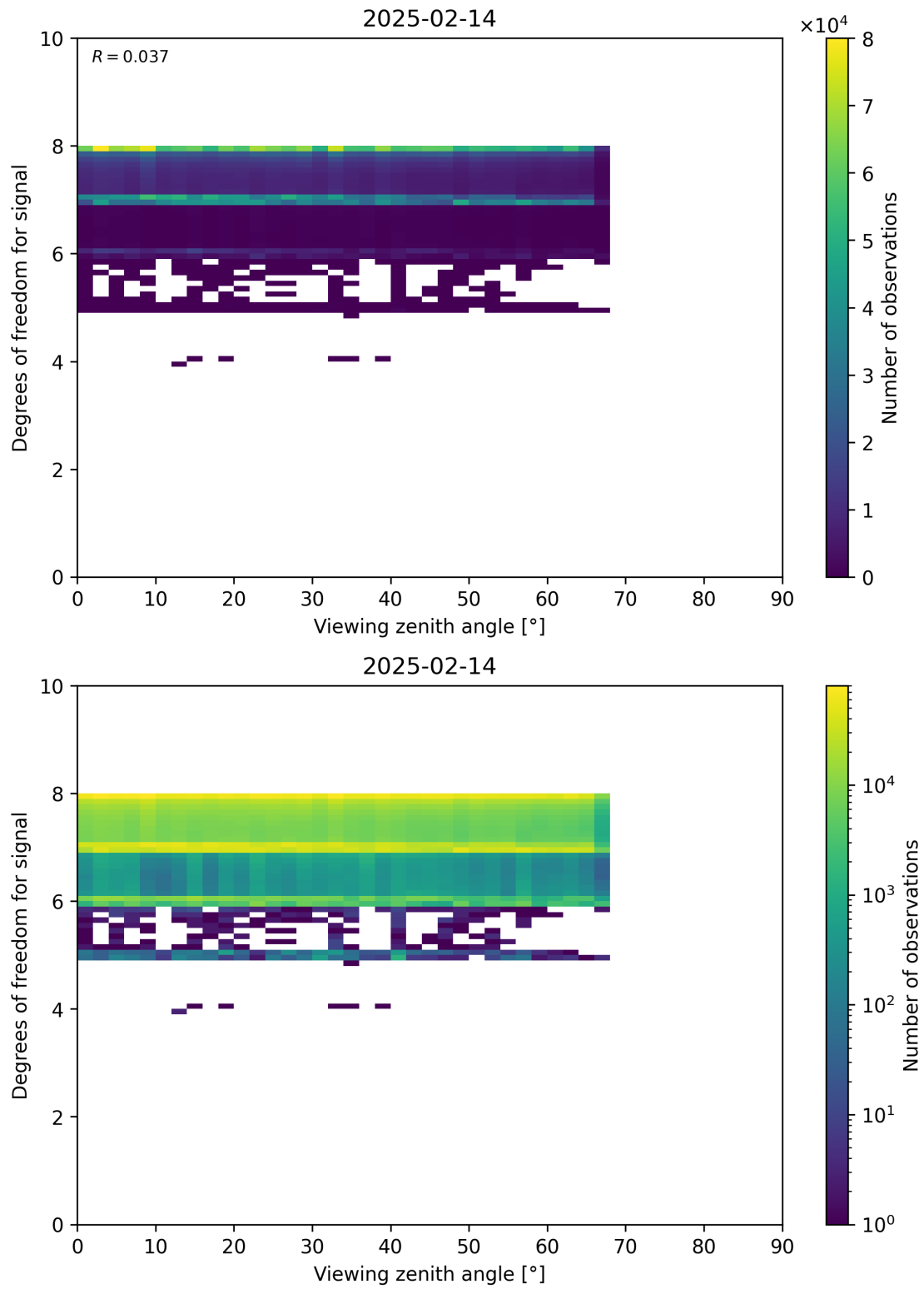
Figure 73: Scatter density plot of “Viewing zenith angle” against “Degrees of freedom for signal” for 2025-02-13 to 2025-02-15.
