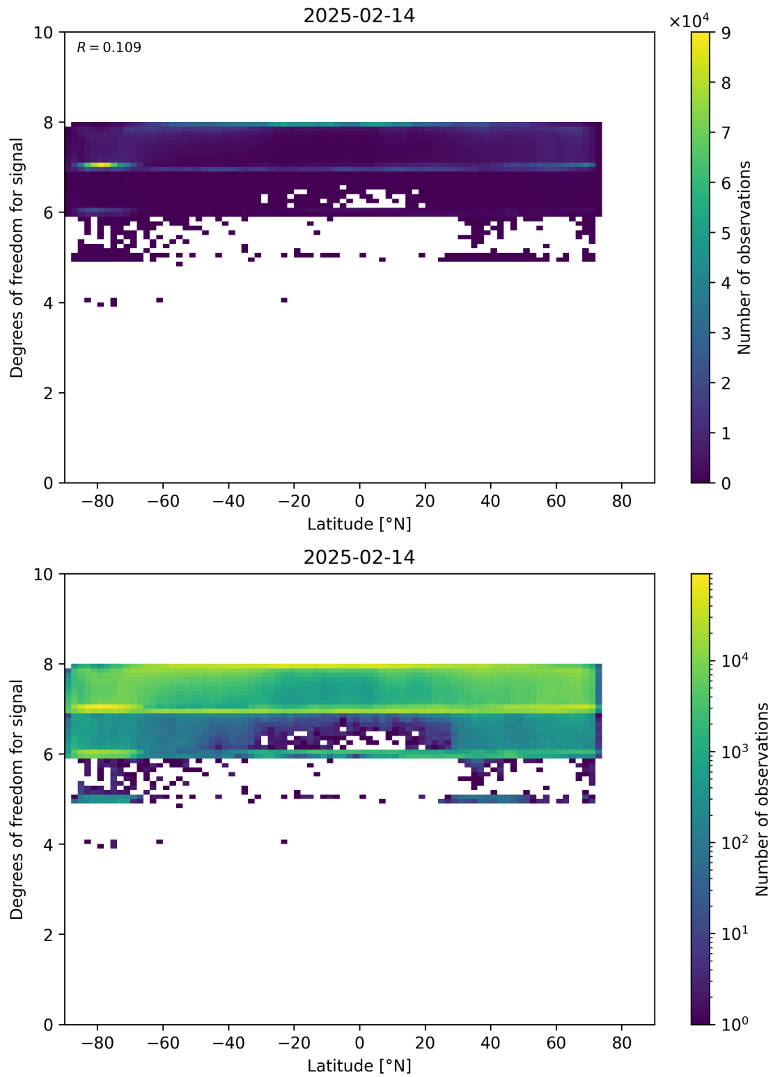
Figure 55: Scatter density plot of “Latitude” against “Degrees of freedom for signal” for 2025-02-13 to 2025-02-15.
