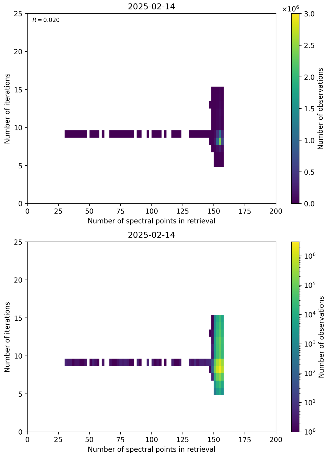
Figure 60: Scatter density plot of “Number of spectral points in retrieval” against “Number of iterations” for 2025-02-13 to 2025-02-15.
