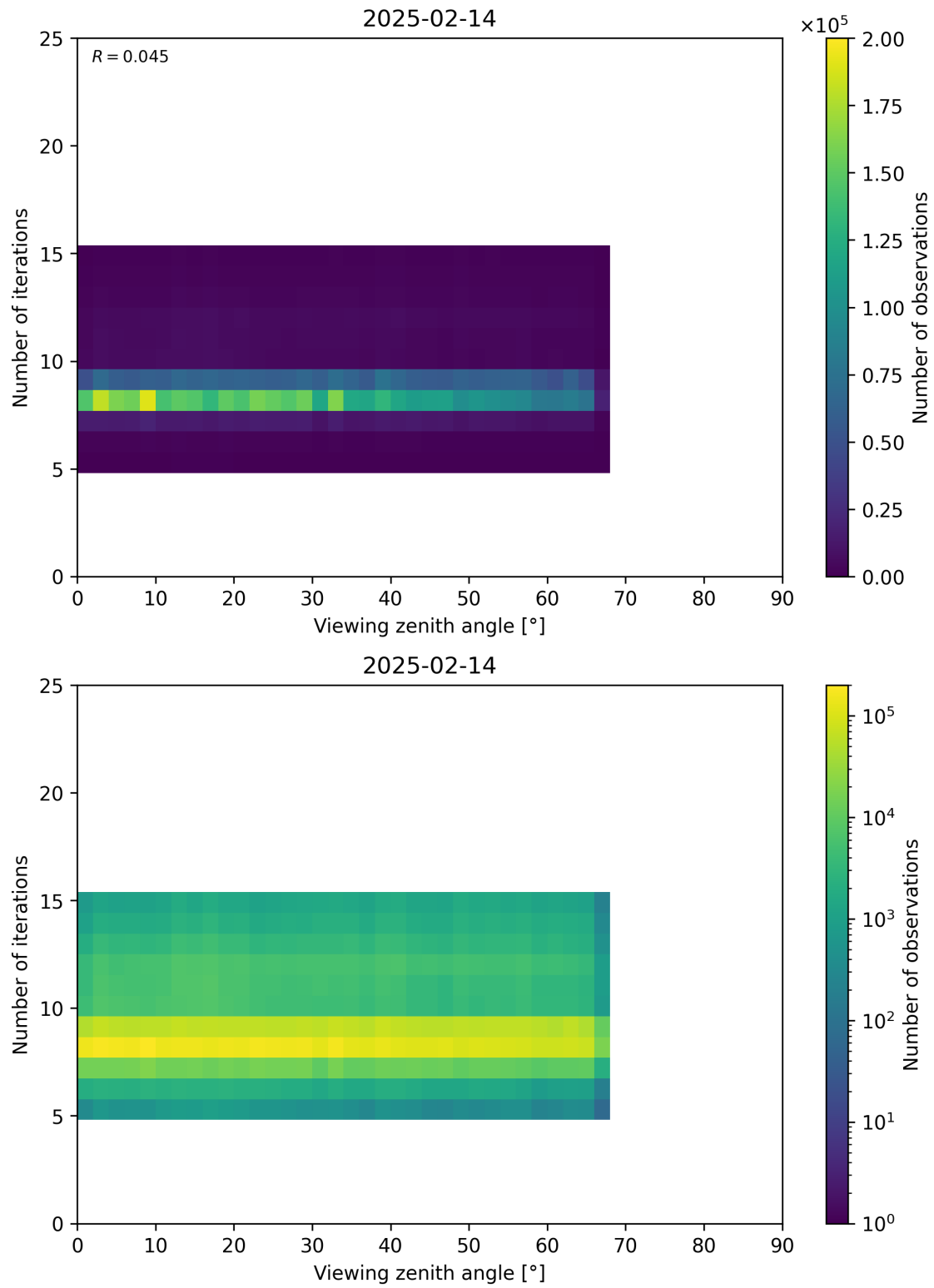
Figure 75: Scatter density plot of “Viewing zenith angle” against “Number of iterations” for 2025-02-13 to 2025-02-15.
