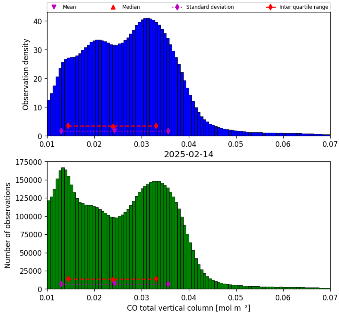
Figure 18: Histogram of “CO total vertical column” for 2025-02-13 to 2025-02-15
