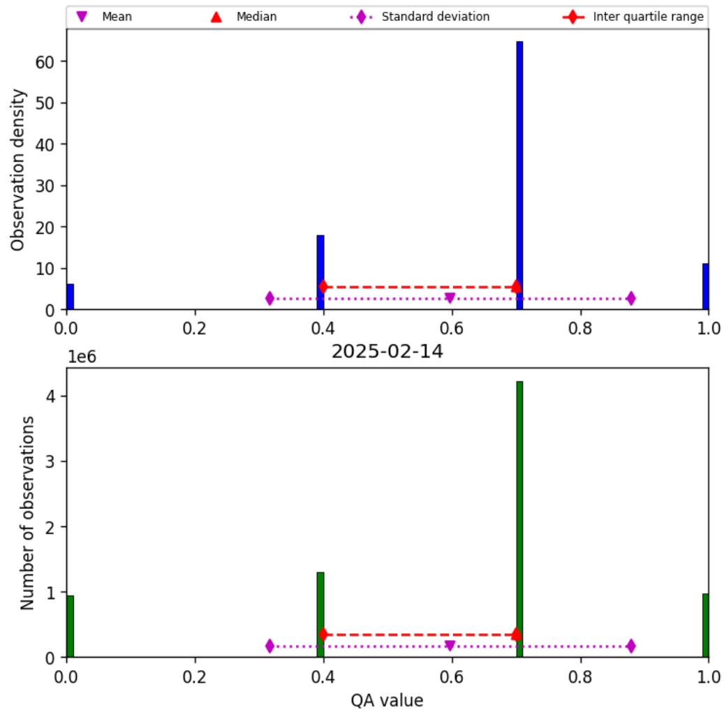
Figure 17: Histogram of “QA value” for 2025-02-13 to 2025-02-15
