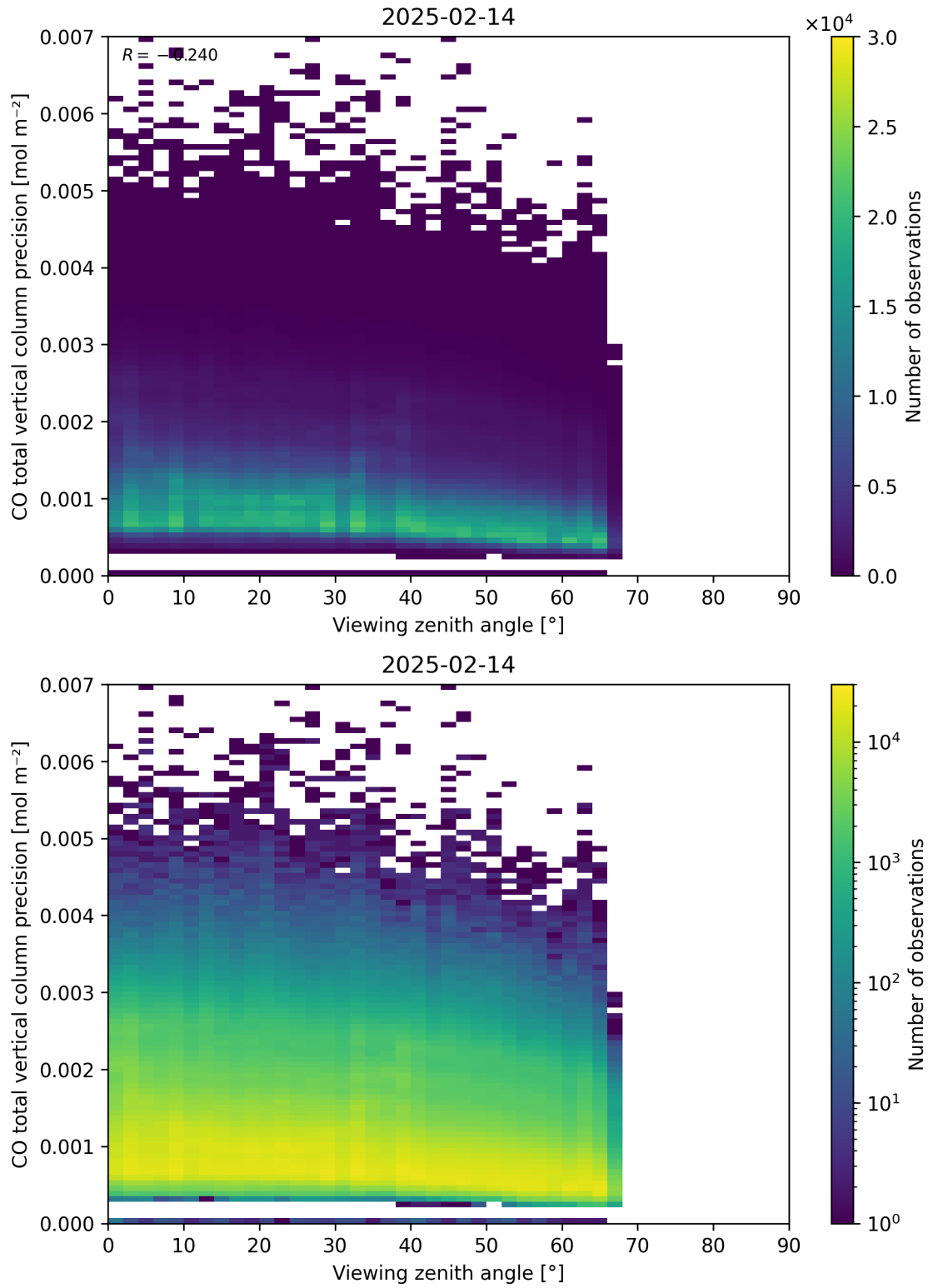
Figure 71: Scatter density plot of “Viewing zenith angle” against “CO total vertical column precision” for 2025-02-13 to 2025-02-15.
