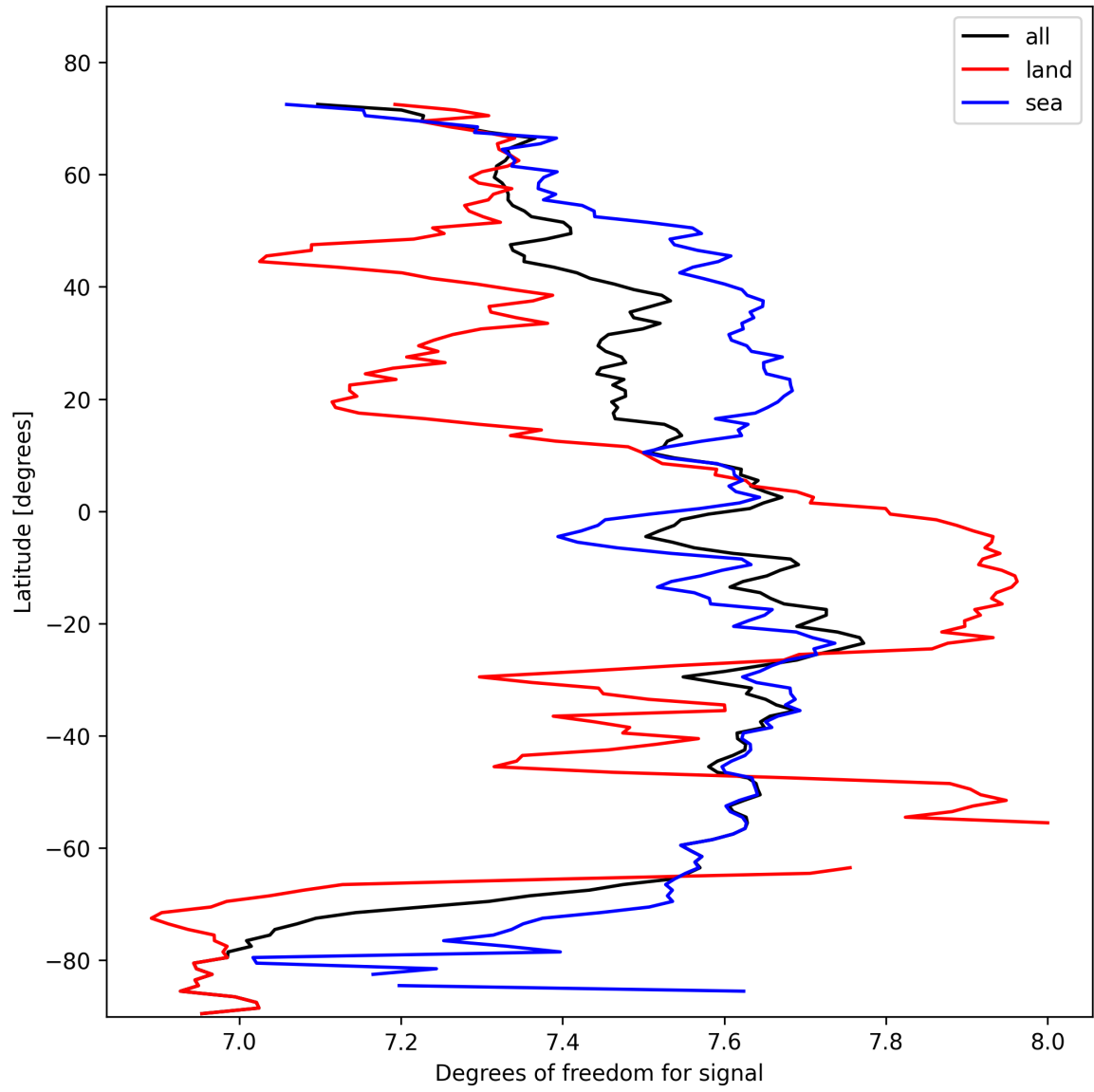
Figure 15: Zonal average of “Degrees of freedom for signal” for 2025-02-13 to 2025-02-15.
