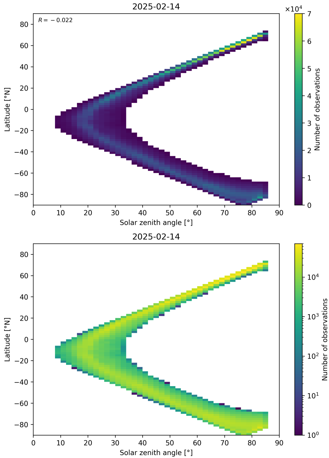
Figure 66: Scatter density plot of “Solar zenith angle” against “Latitude” for 2025-02-13 to 2025-02-15.
