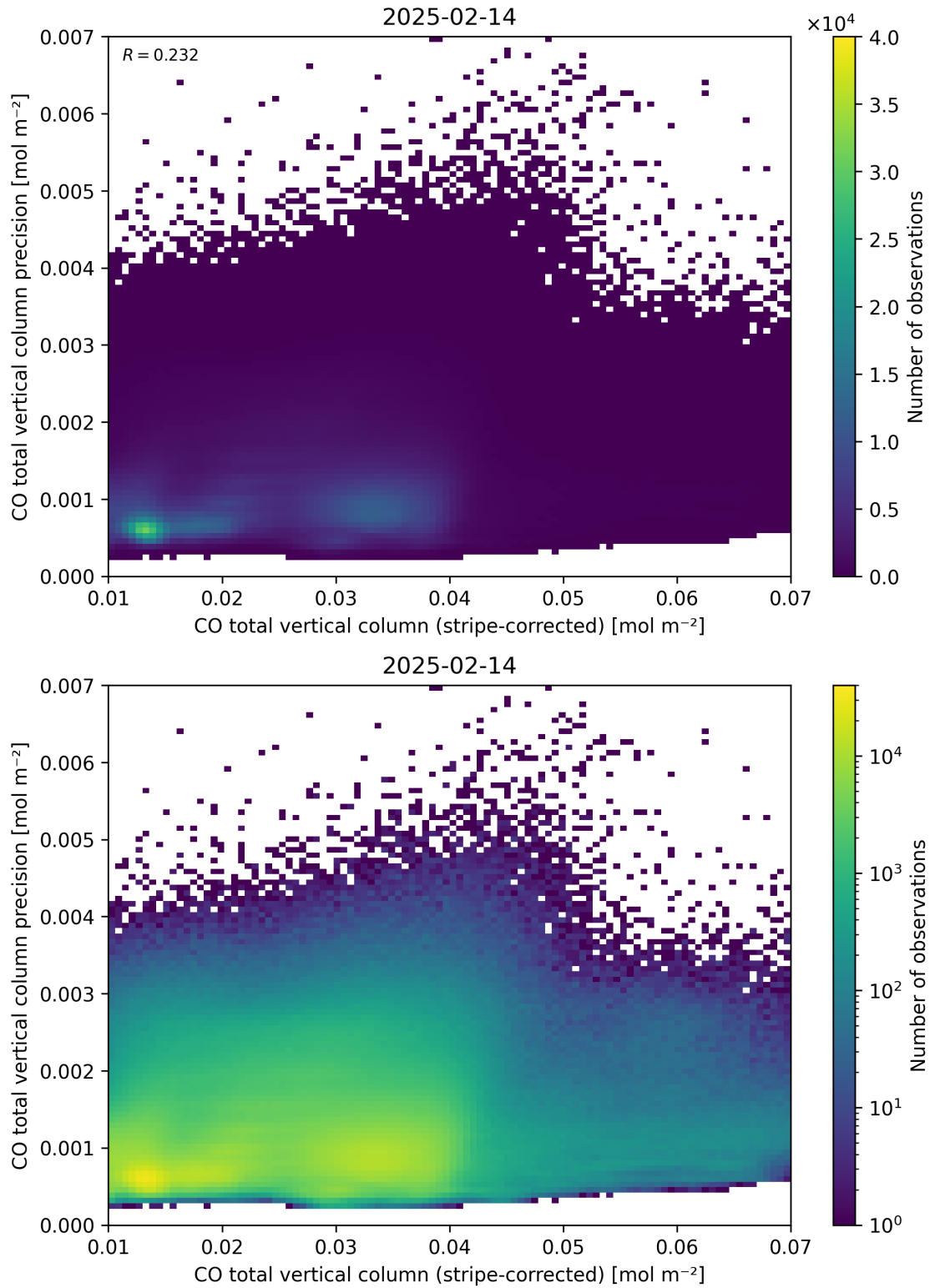
Figure 36: Scatter density plot of “CO total vertical column (stripe-corrected)” against “CO total vertical column precision” for 2025-02-13 to 2025-02-15.
