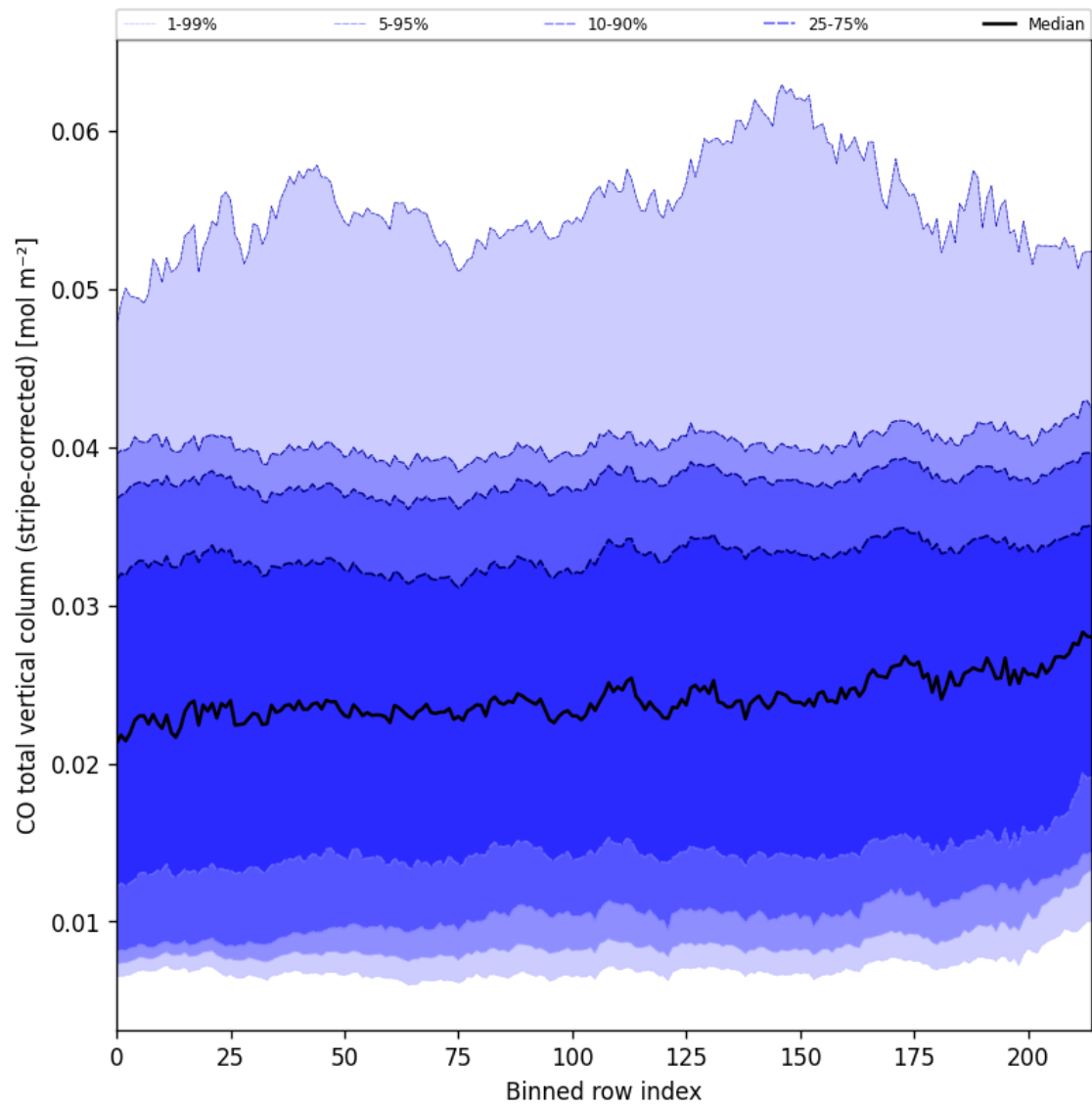
Figure 27: Along track statistics of “CO total vertical column (stripe-corrected)” for 2025-02-13 to 2025-02-15
