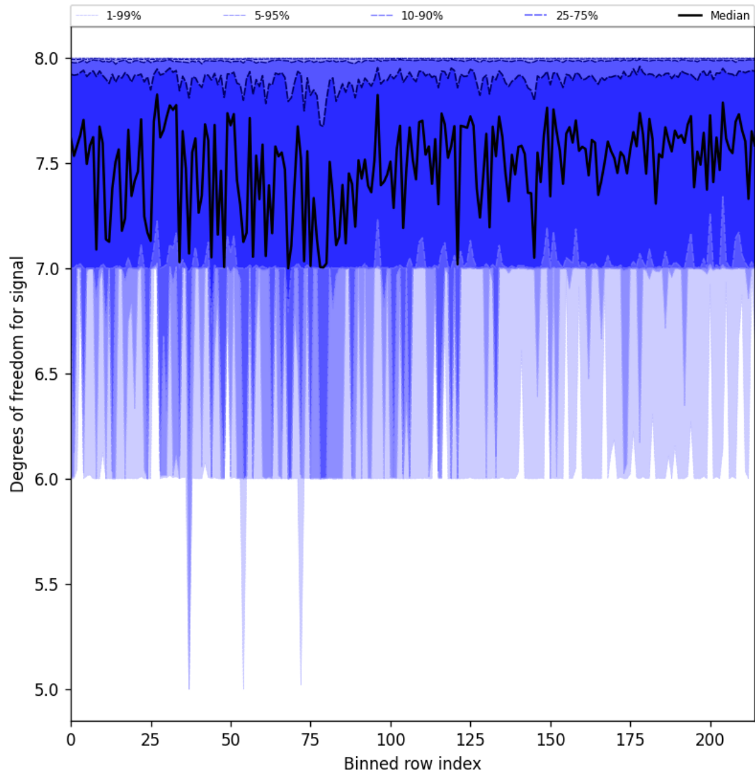
Figure 31: Along track statistics of “Degrees of freedom for signal” for 2025-02-13 to 2025-02-15
