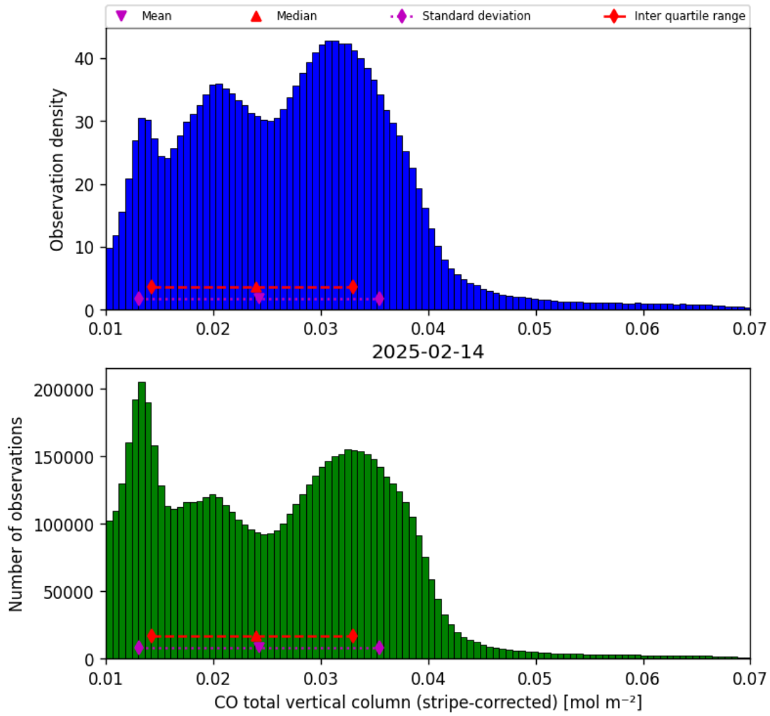
Figure 19: Histogram of “CO total vertical column (stripe-corrected)” for 2025-02-13 to 2025-02-15
