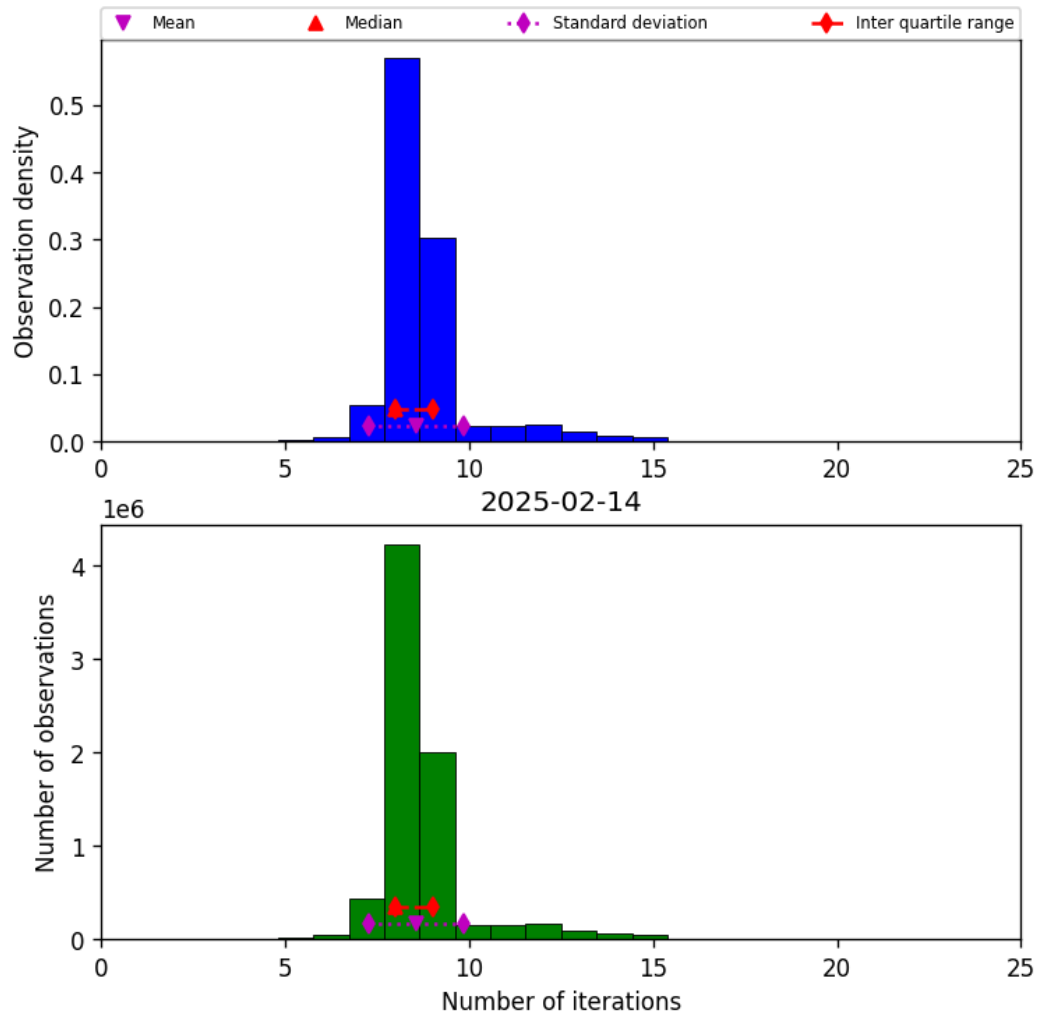
Figure 24: Histogram of “Number of iterations” for 2025-02-13 to 2025-02-15
