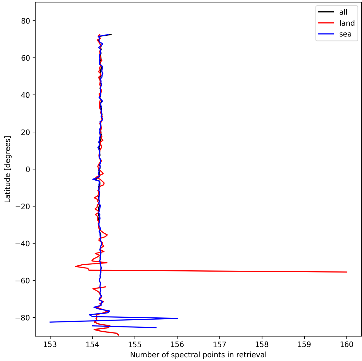
Figure 13: Zonal average of “Number of spectral points in retrieval” for 2025-02-13 to 2025-02-15.
