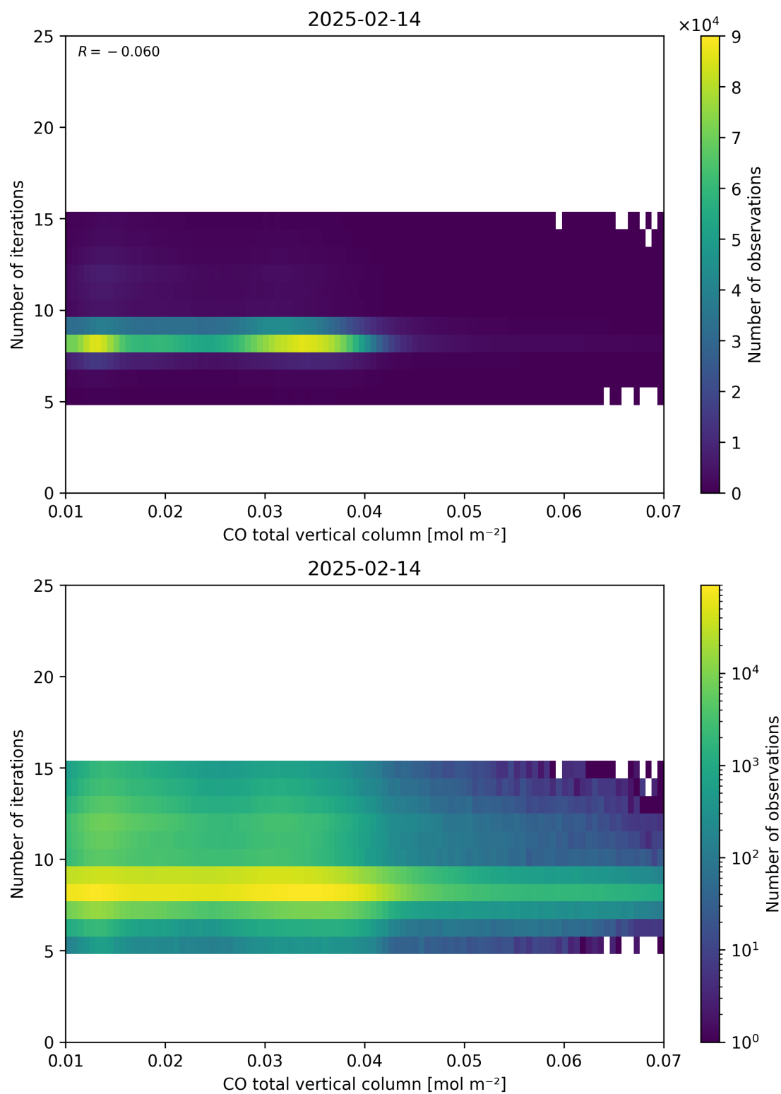
Figure 42: Scatter density plot of “CO total vertical column” against “Number of iterations” for 2025-02-13 to 2025-02-15.
