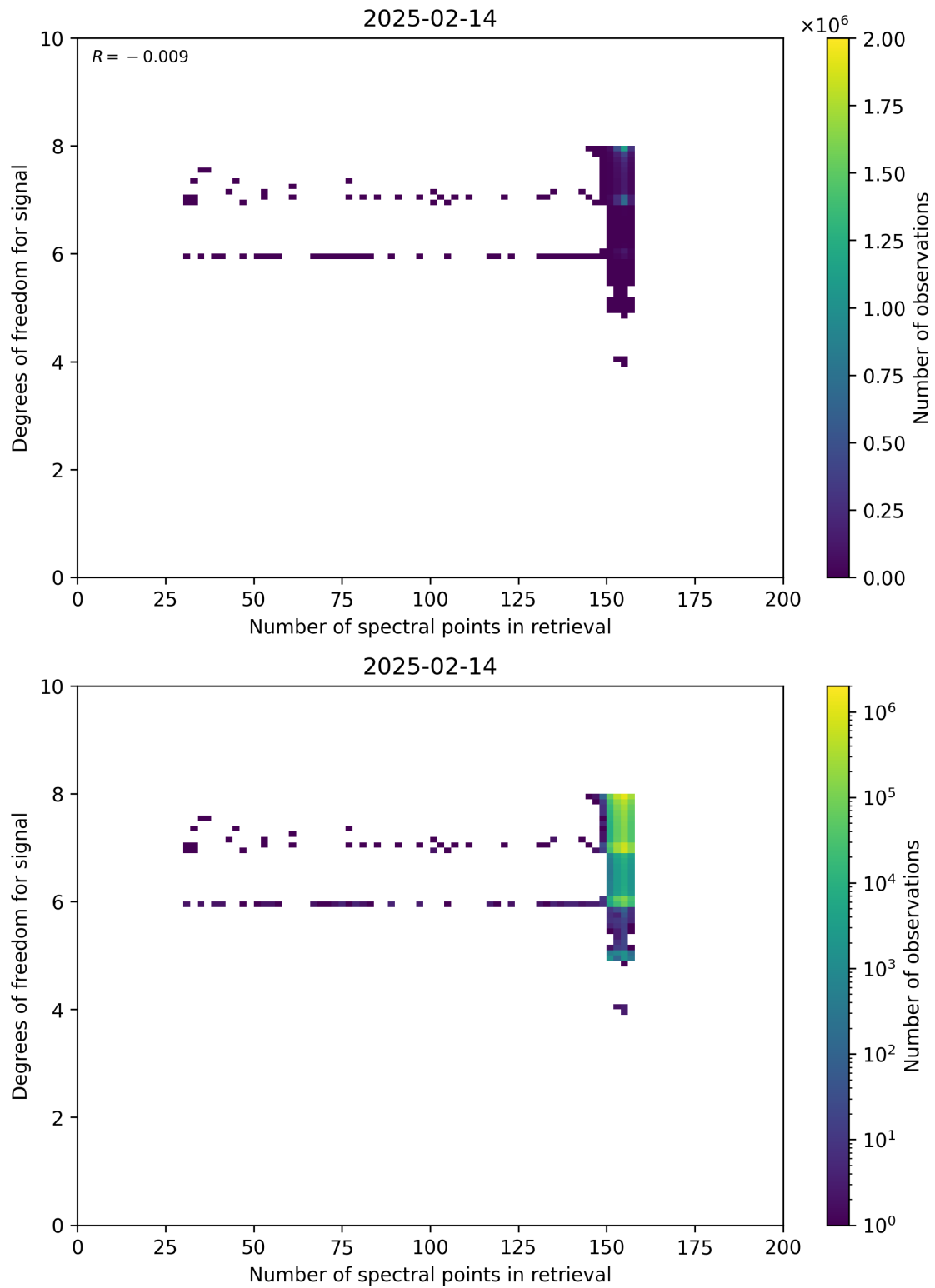
Figure 59: Scatter density plot of “Number of spectral points in retrieval” against “Degrees of freedom for signal” for 2025-02-13 to 2025-02-15.
