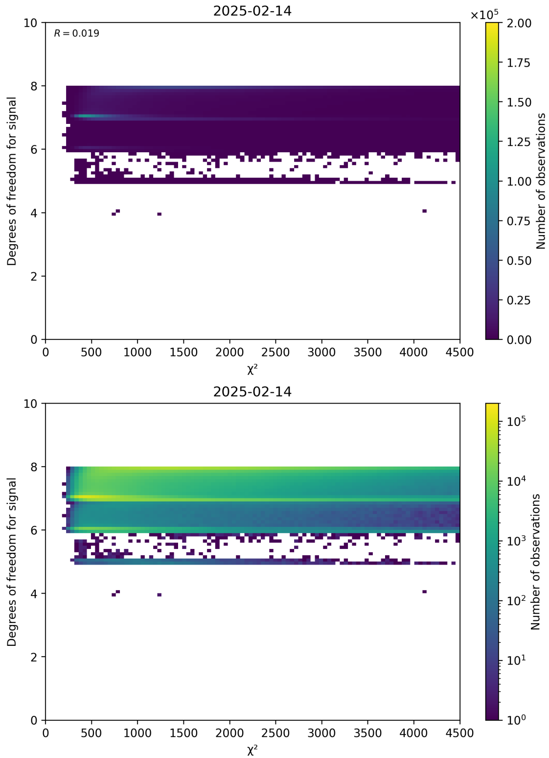
Figure 48: Scatter density plot of “ \chi^2 ” against “Degrees of freedom for signal” for 2025-02-13 to 2025-02-15.
