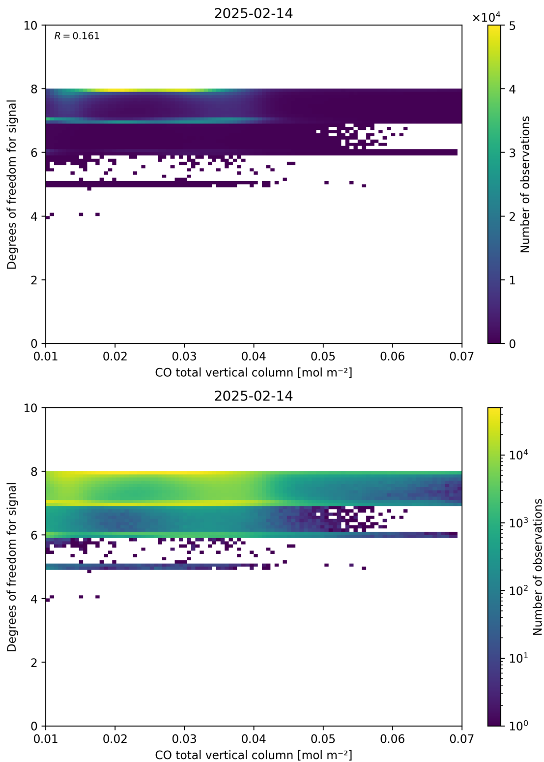
Figure 41: Scatter density plot of “CO total vertical column” against “Degrees of freedom for signal” for 2025-02-13 to 2025-02-15.
