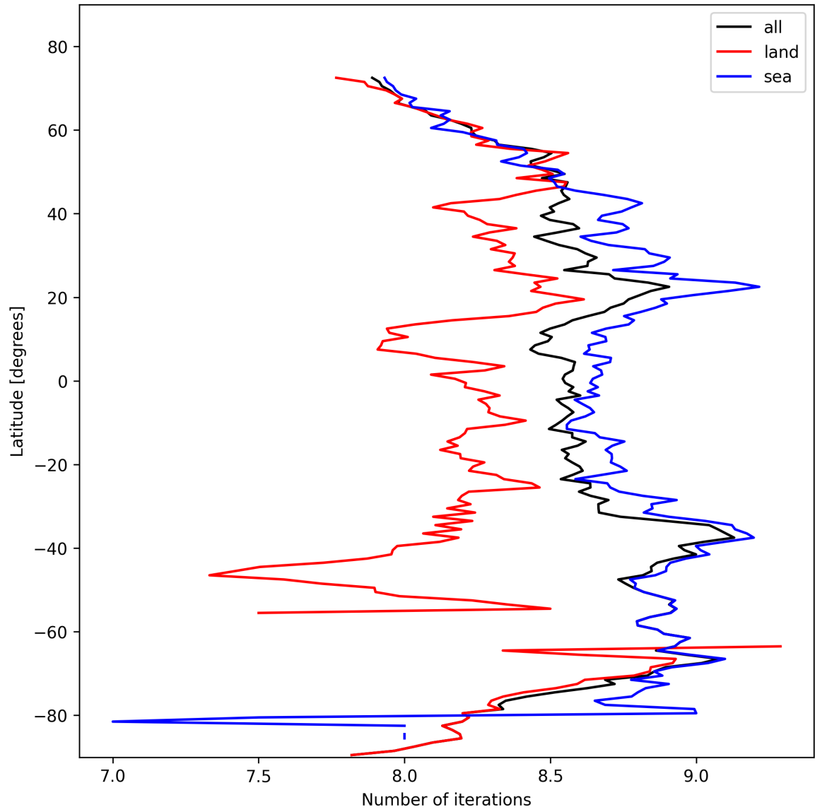
Figure 16: Zonal average of “Number of iterations” for 2025-02-13 to 2025-02-15.
