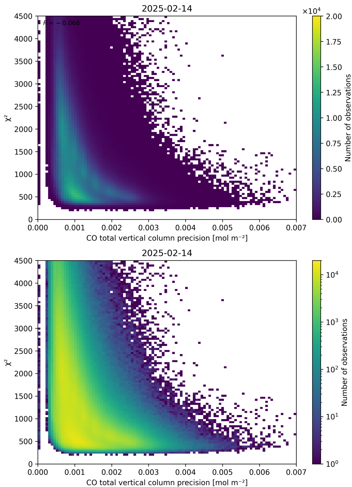
Figure 44: Scatter density plot of “CO total vertical column precision” against “ \chi^2 ” for 2025-02-13 to 2025-02-15.
