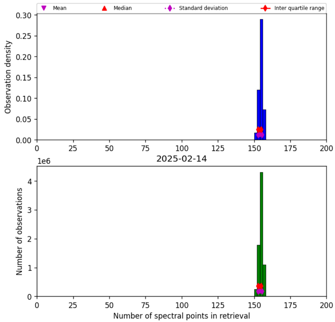
Figure 21: Histogram of “Number of spectral points in retrieval” for 2025-02-13 to 2025-02-15
