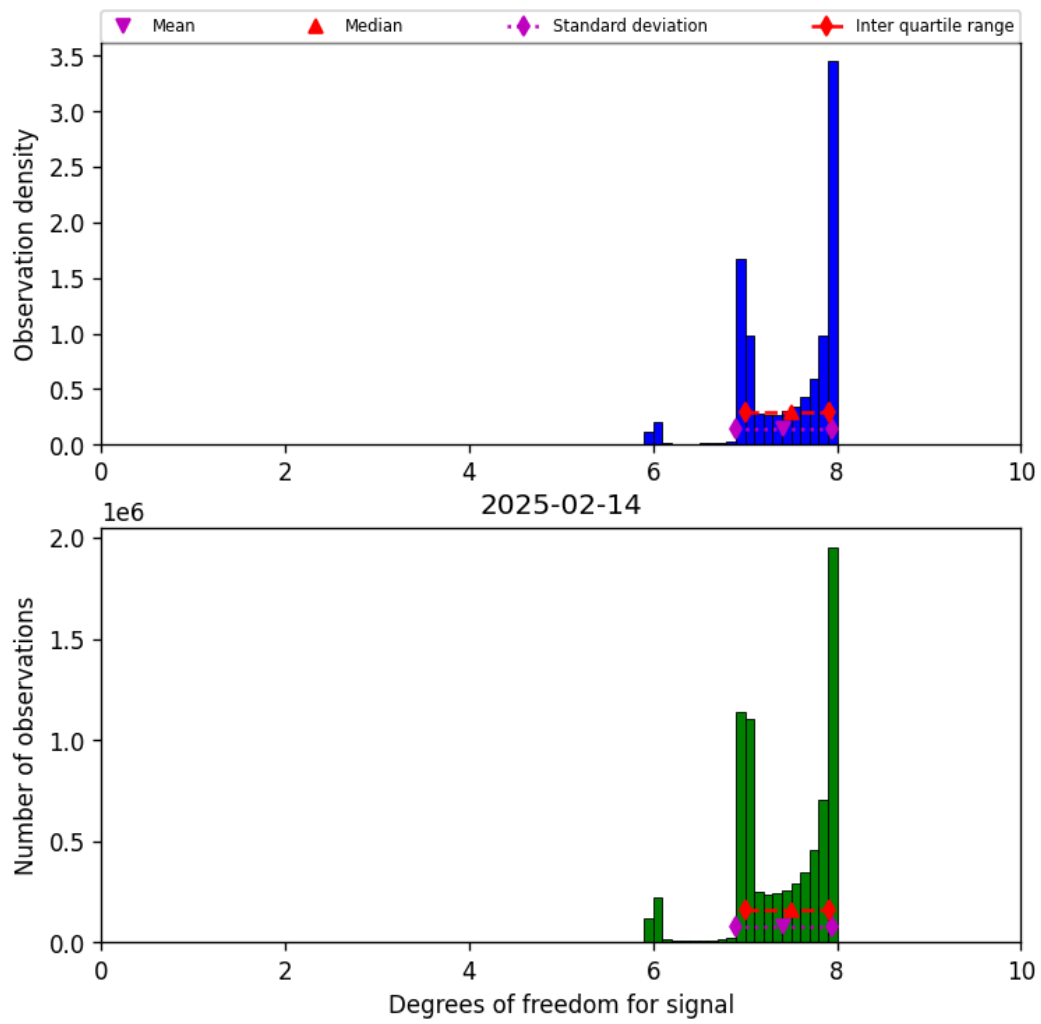
Figure 23: Histogram of “Degrees of freedom for signal” for 2025-02-13 to 2025-02-15
