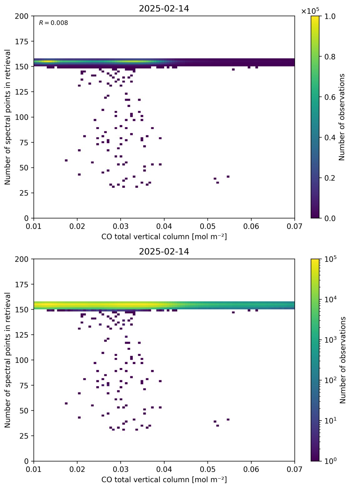
Figure 43: Scatter density plot of “CO total vertical column” against “Number of spectral points in retrieval” for 2025-02-13 to 2025-02-15.
