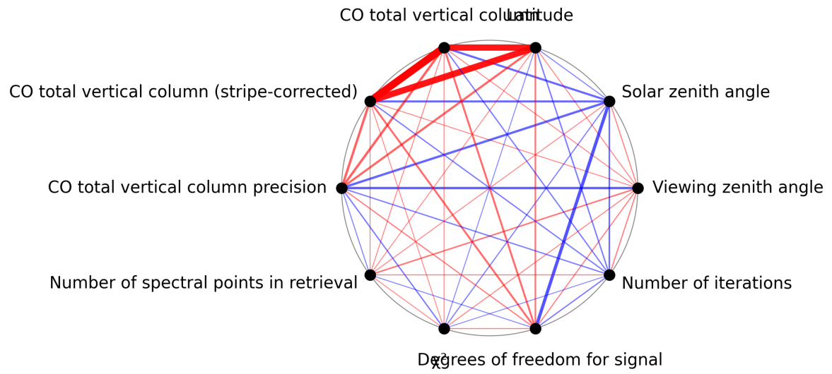
Figure 1: Map of correlation graph for 2025-02-13 to 2025-02-15.
