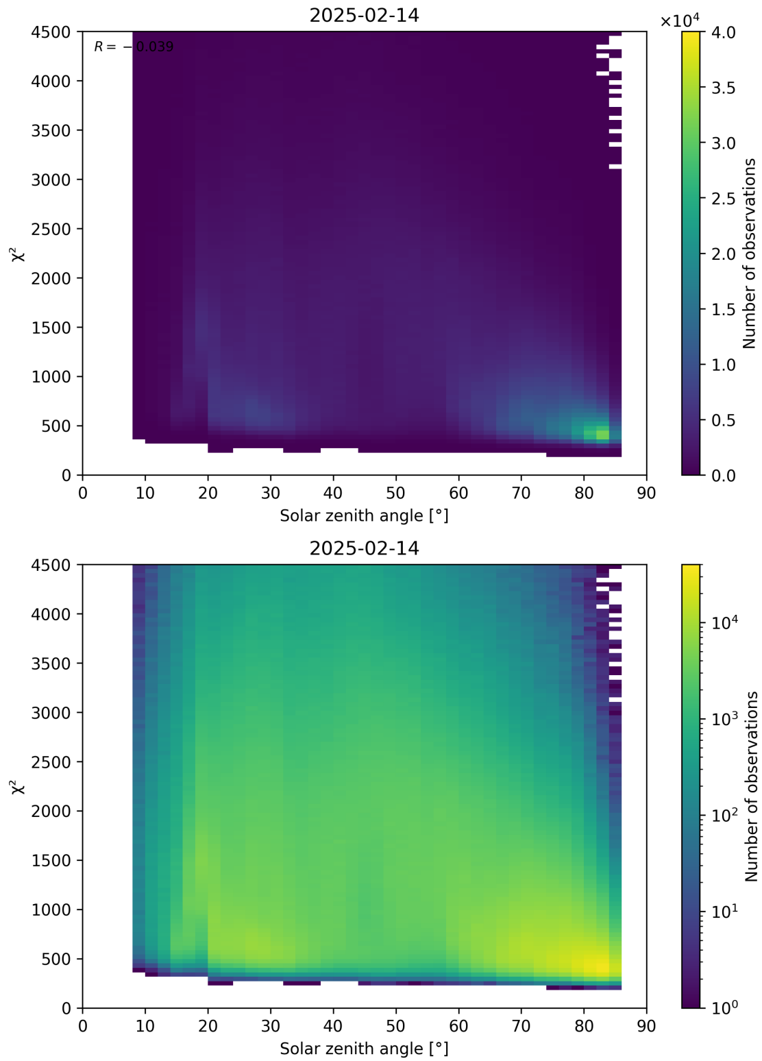
Figure 64: Scatter density plot of “Solar zenith angle” against “ \chi^2 ” for 2025-02-13 to 2025-02-15.
