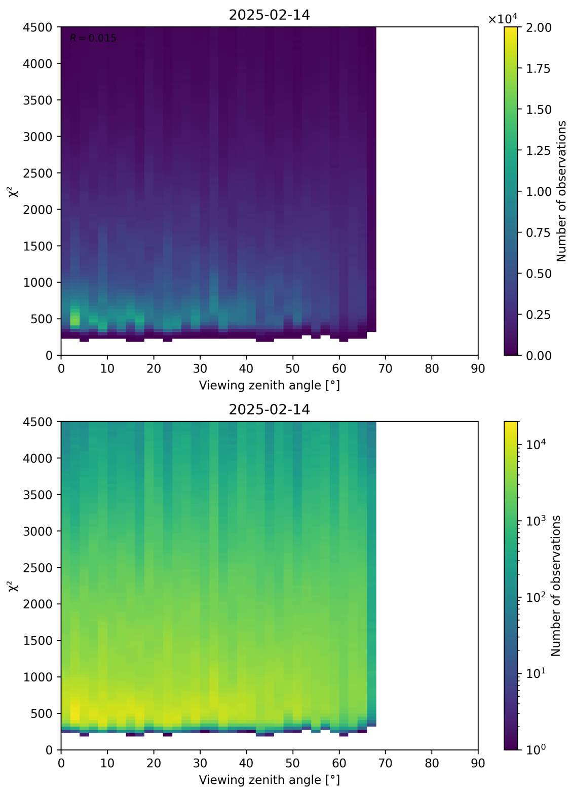
Figure 72: Scatter density plot of “Viewing zenith angle” against “ \chi^2 ” for 2025-02-13 to 2025-02-15.
