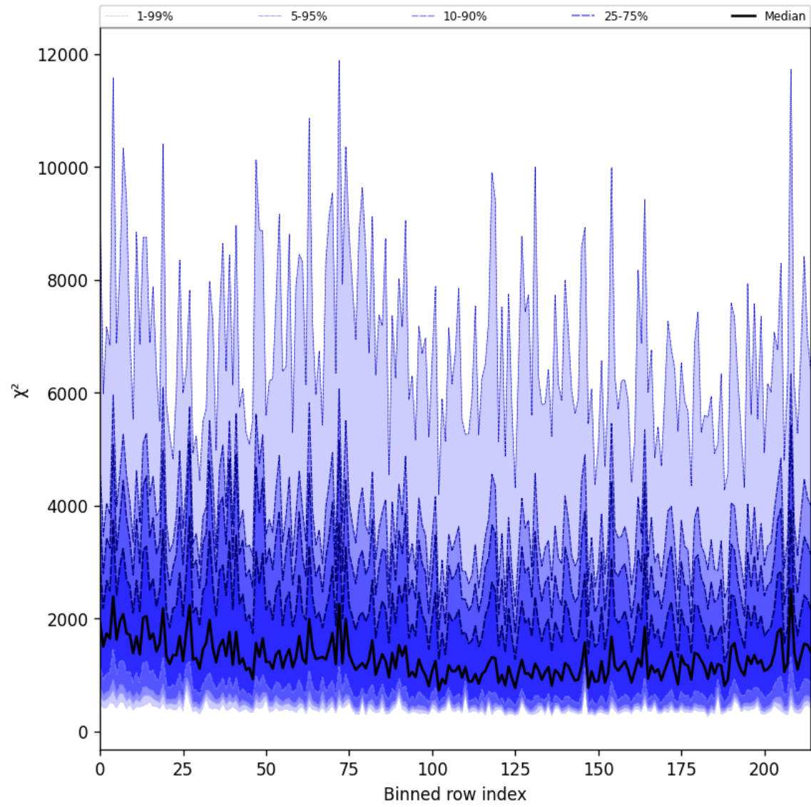
Figure 30: Along track statistics of “ \chi^2 ” for 2025-02-13 to 2025-02-15
