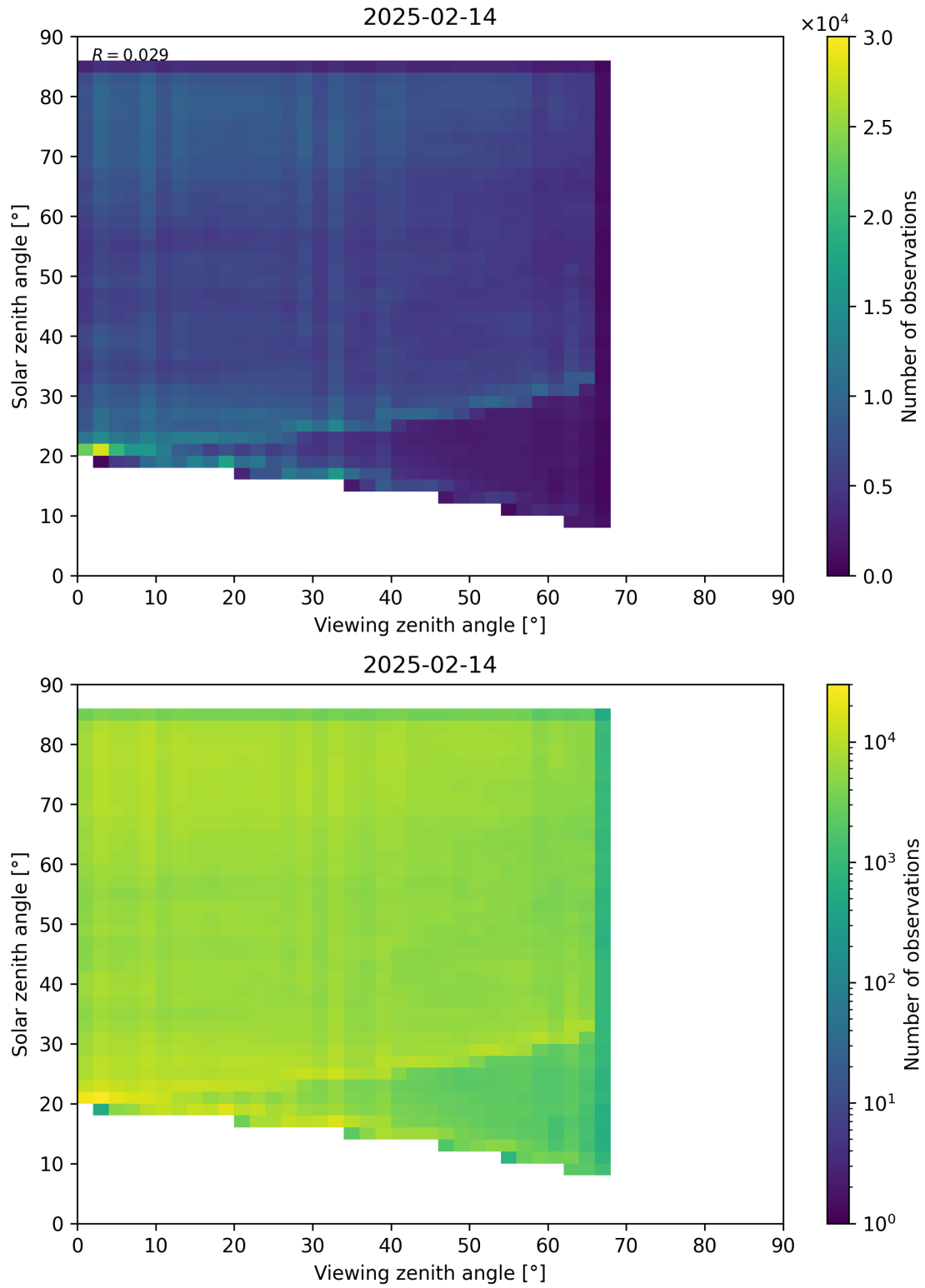
Figure 77: Scatter density plot of “Viewing zenith angle” against “Solar zenith angle” for 2025-02-13 to 2025-02-15.
