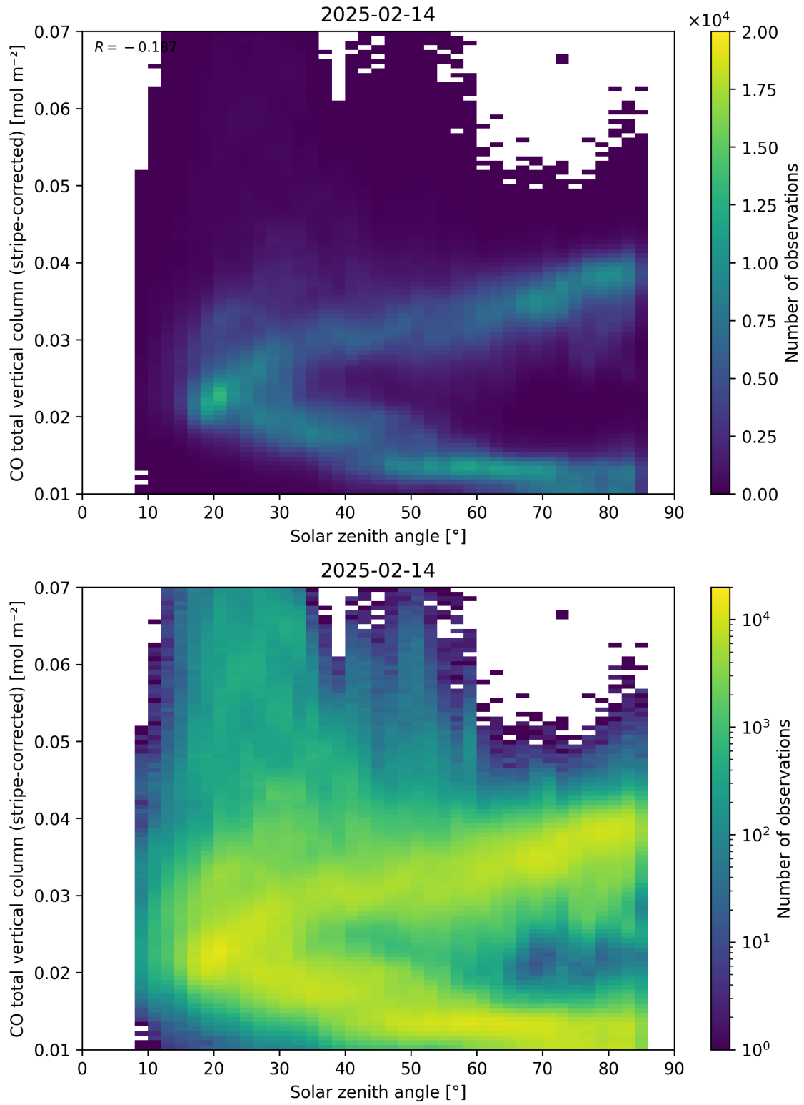
Figure 62: Scatter density plot of “Solar zenith angle” against “CO total vertical column (stripe-corrected)” for 2025-02-13 to 2025-02-15.
