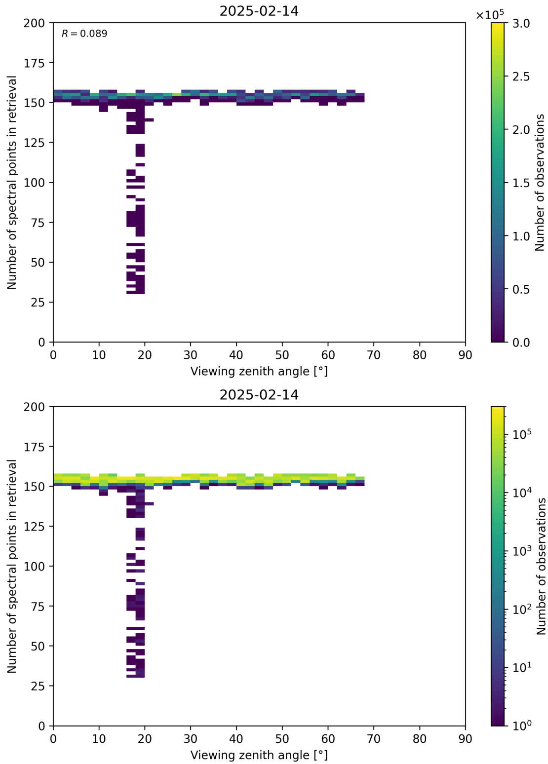
Figure 76: Scatter density plot of “Viewing zenith angle” against “Number of spectral points in retrieval” for 2025-02-13 to 2025-02-15.
