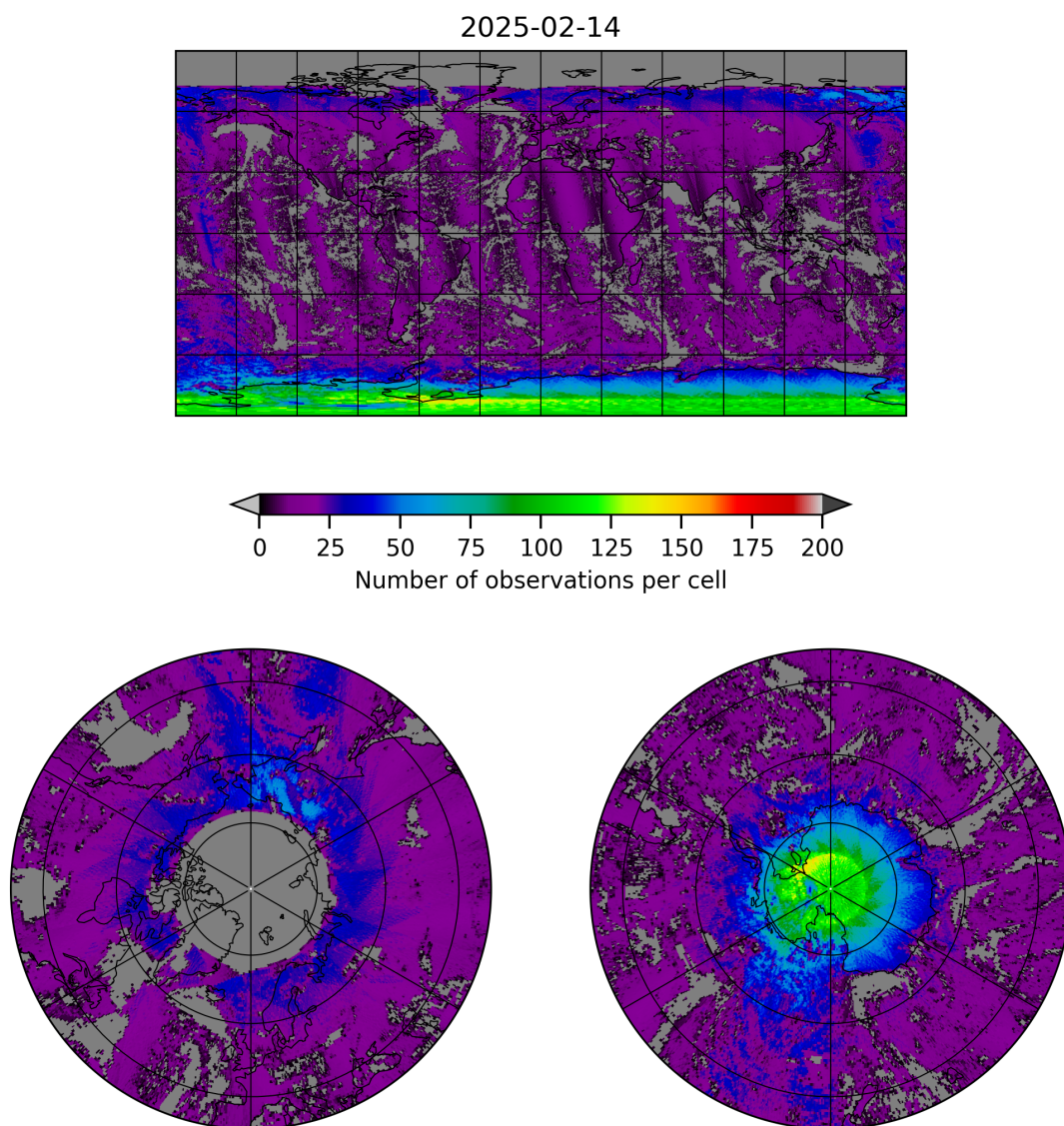
Figure 8: Map of the number of observations for 2025-02-13 to 2025-02-15
