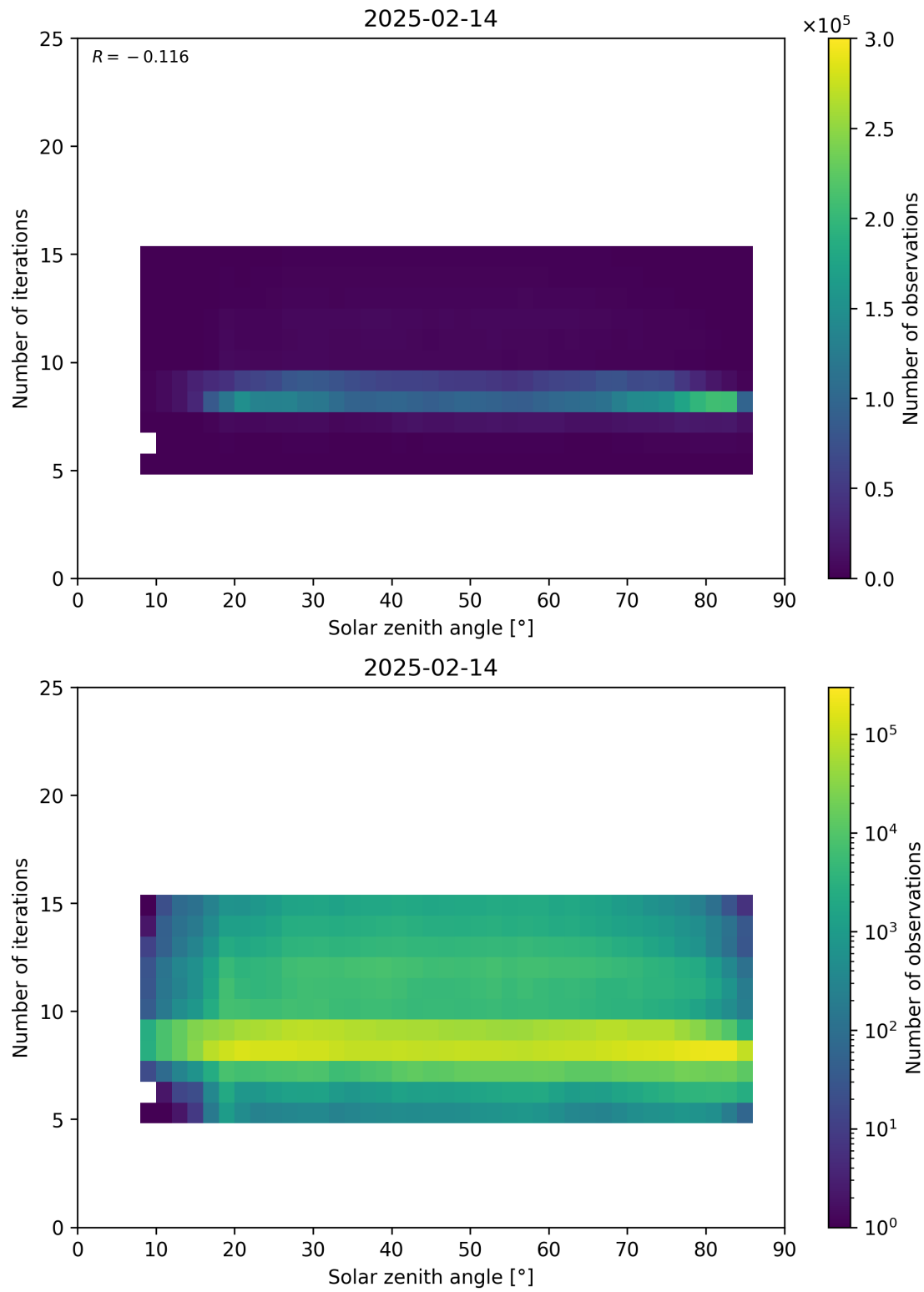
Figure 67: Scatter density plot of “Solar zenith angle” against “Number of iterations” for 2025-02-13 to 2025-02-15.
