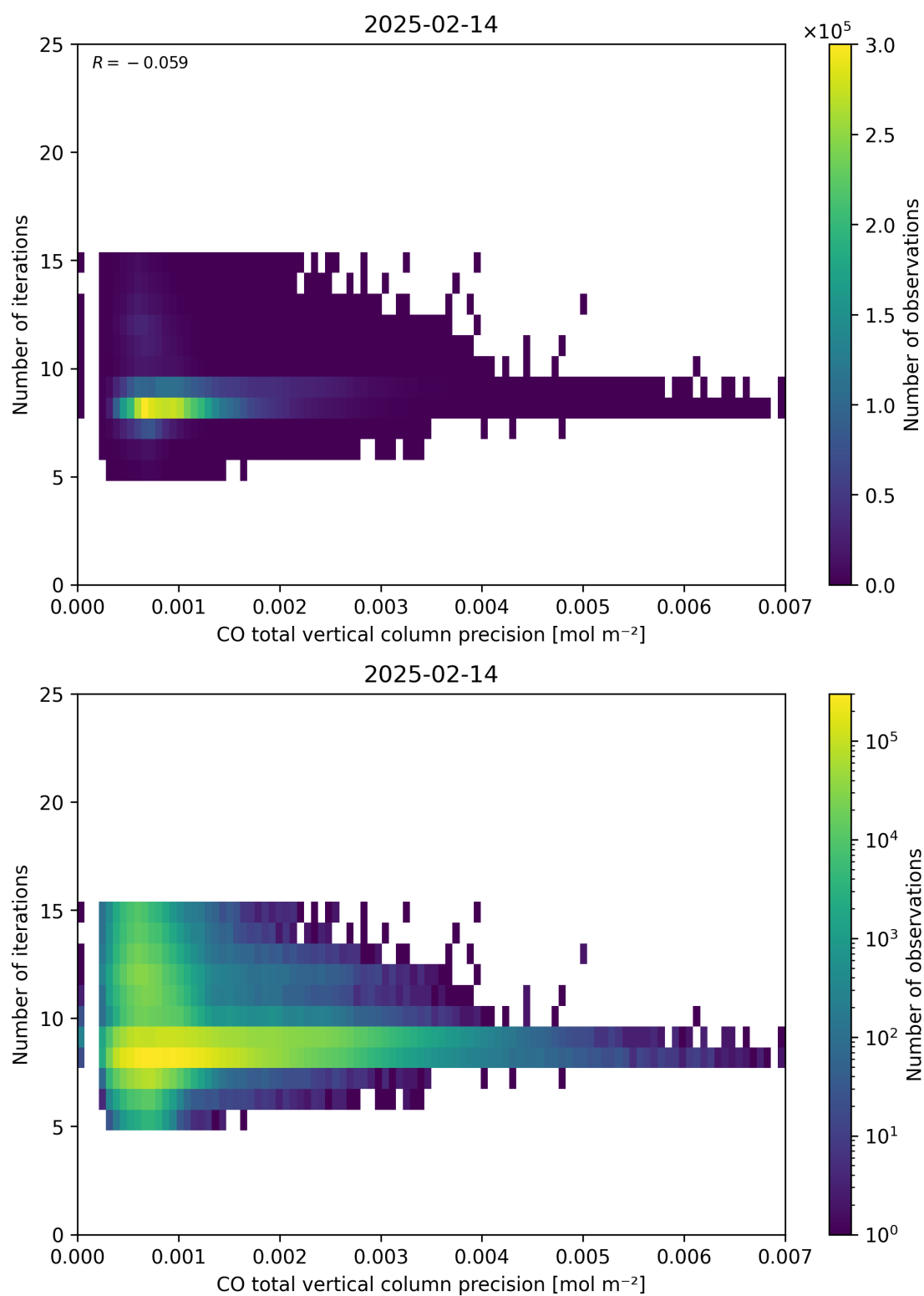
Figure 46: Scatter density plot of “CO total vertical column precision” against “Number of iterations” for 2025-02-13 to 2025-02-15.
