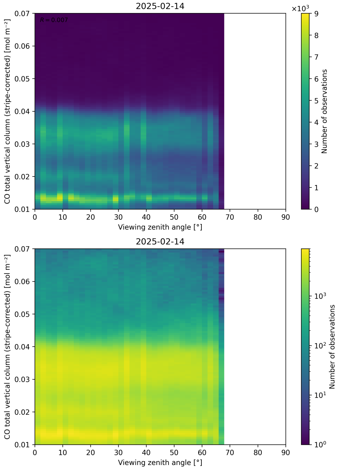
Figure 70: Scatter density plot of “Viewing zenith angle” against “CO total vertical column (stripe-corrected)” for 2025-02-13 to 2025-02-15.
