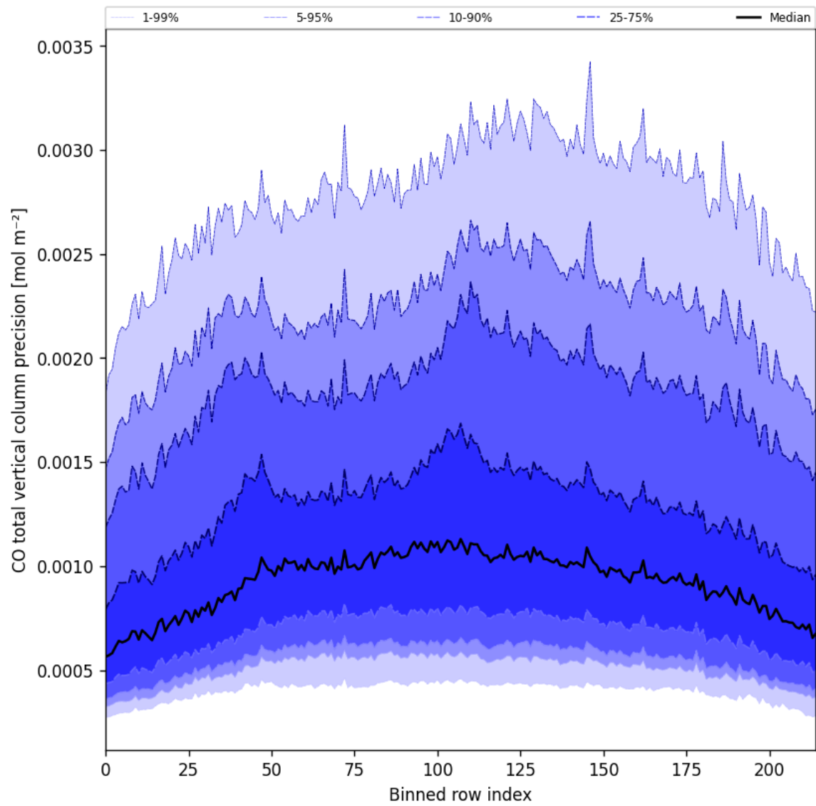
Figure 28: Along track statistics of “CO total vertical column precision” for 2025-02-13 to 2025-02-15
