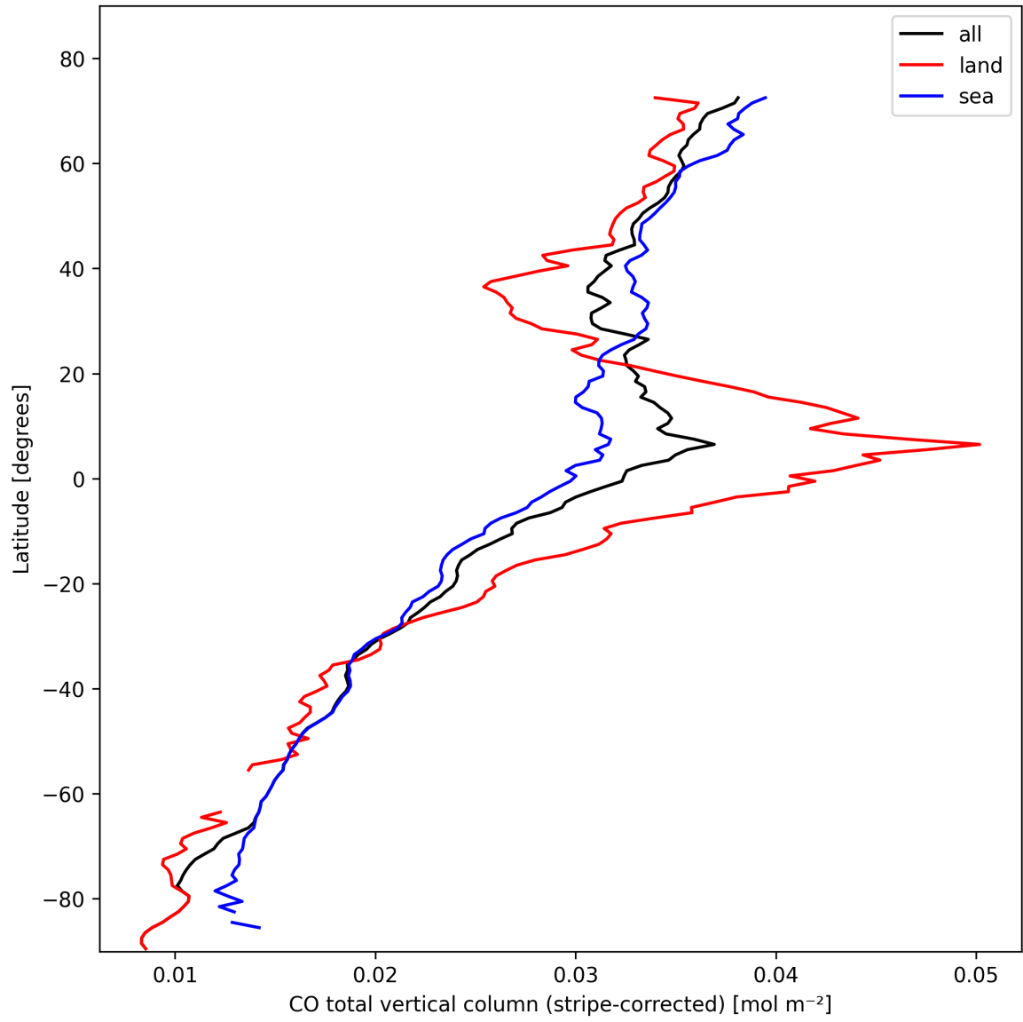
Figure 11: Zonal average of “CO total vertical column (stripe-corrected)” for 2025-02-13 to 2025-02-15.
