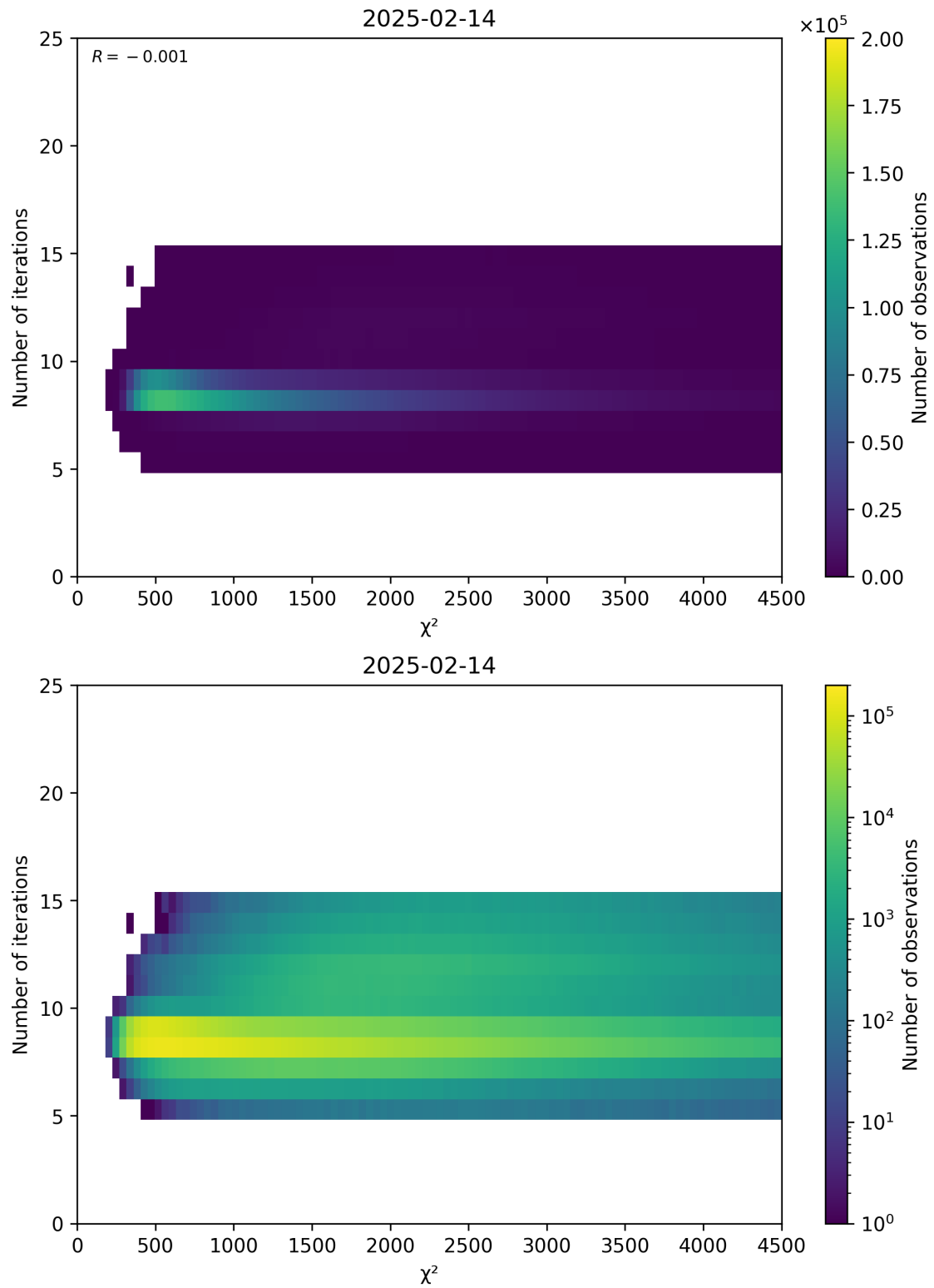
Figure 49: Scatter density plot of “ \chi^2 ” against “Number of iterations” for 2025-02-13 to 2025-02-15.
