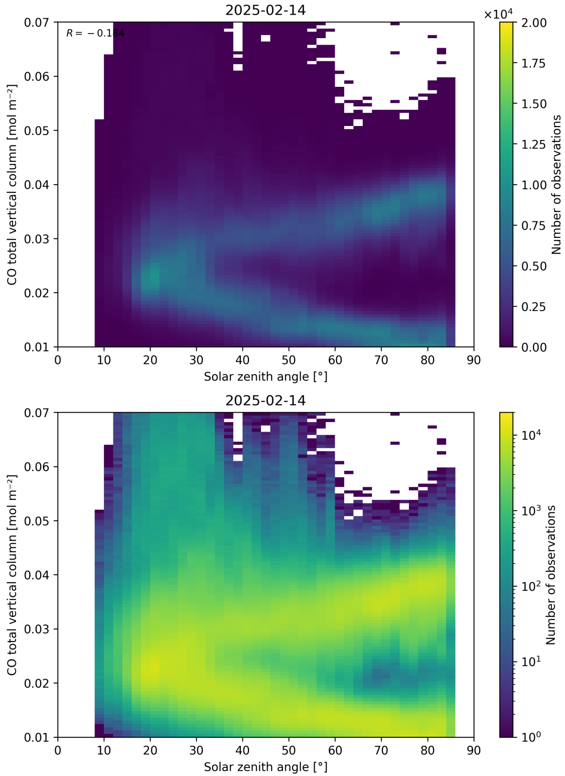
Figure 61: Scatter density plot of “Solar zenith angle” against “CO total vertical column” for 2025-02-13 to 2025-02-15.
