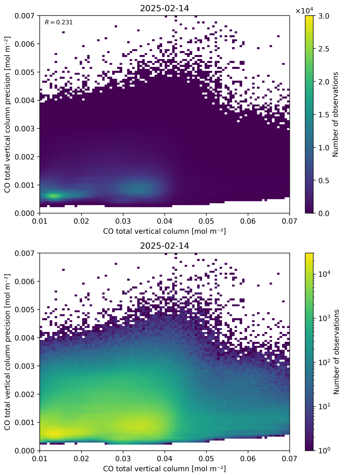
Figure 34: Scatter density plot of “CO total vertical column” against “CO total vertical column precision” for 2025-02-13 to 2025-02-15.
