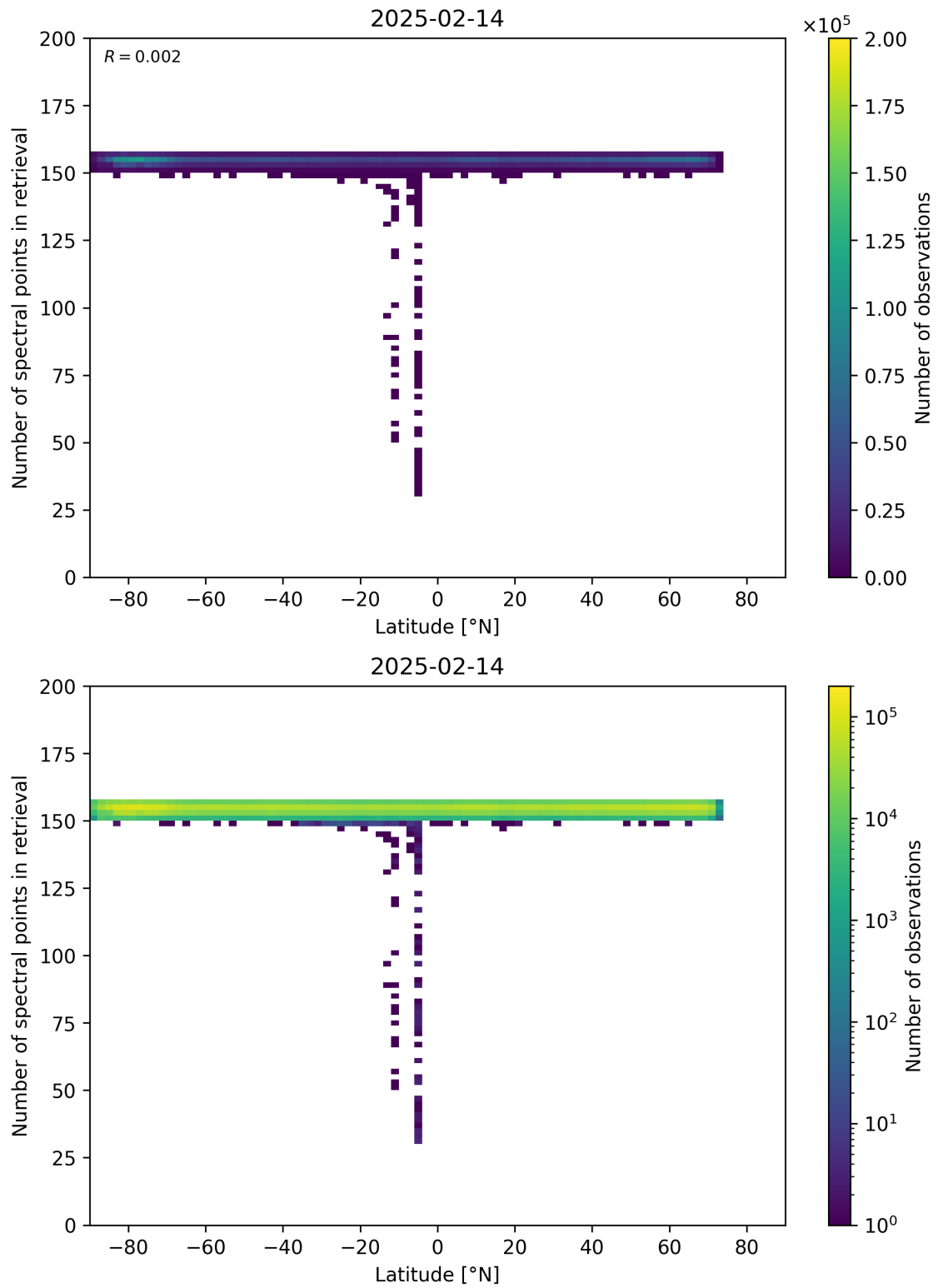
Figure 57: Scatter density plot of “Latitude” against “Number of spectral points in retrieval” for 2025-02-13 to 2025-02-15.
