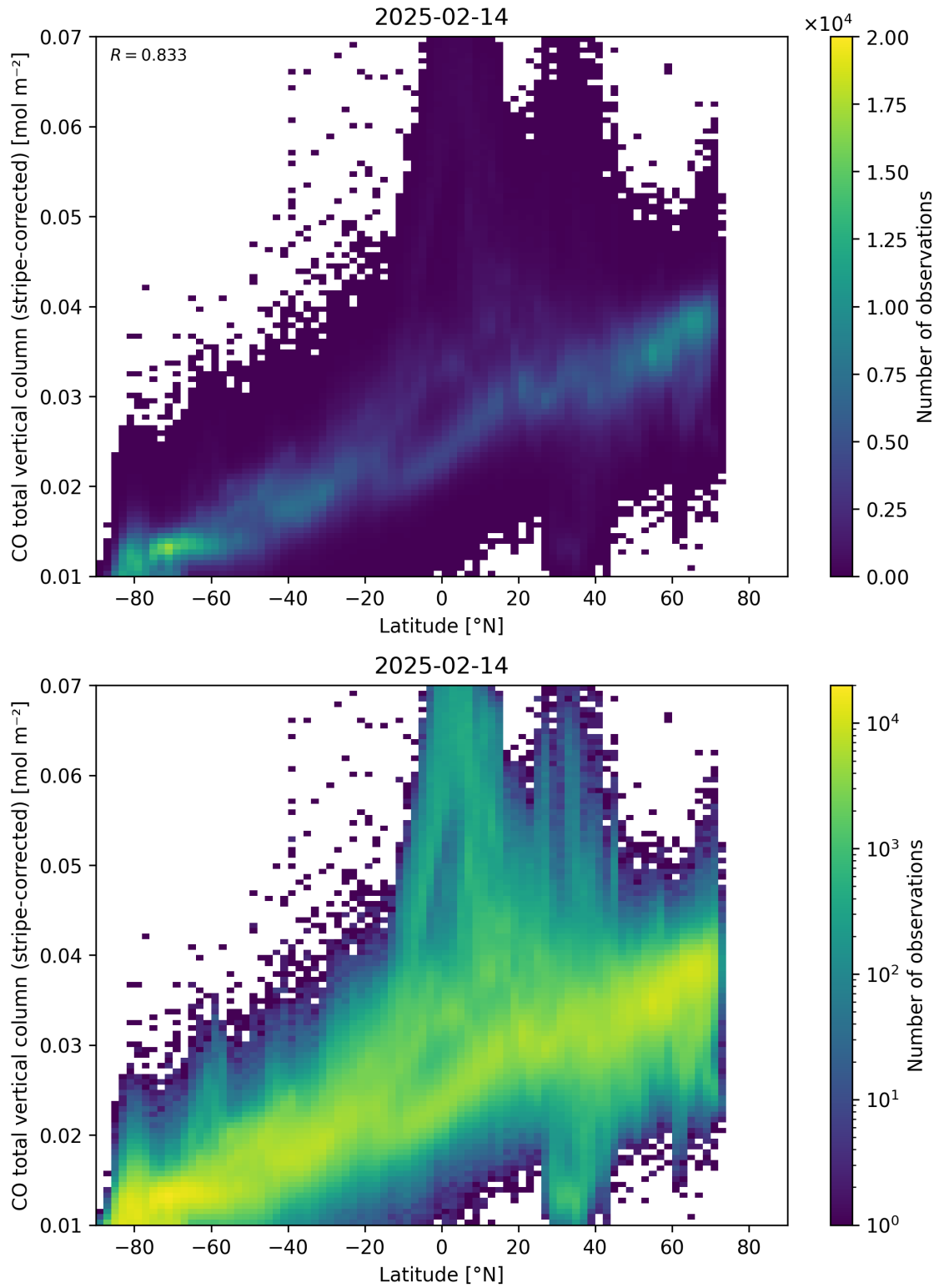
Figure 52: Scatter density plot of “Latitude” against “CO total vertical column (stripe-corrected)” for 2025-02-13 to 2025-02-15.
