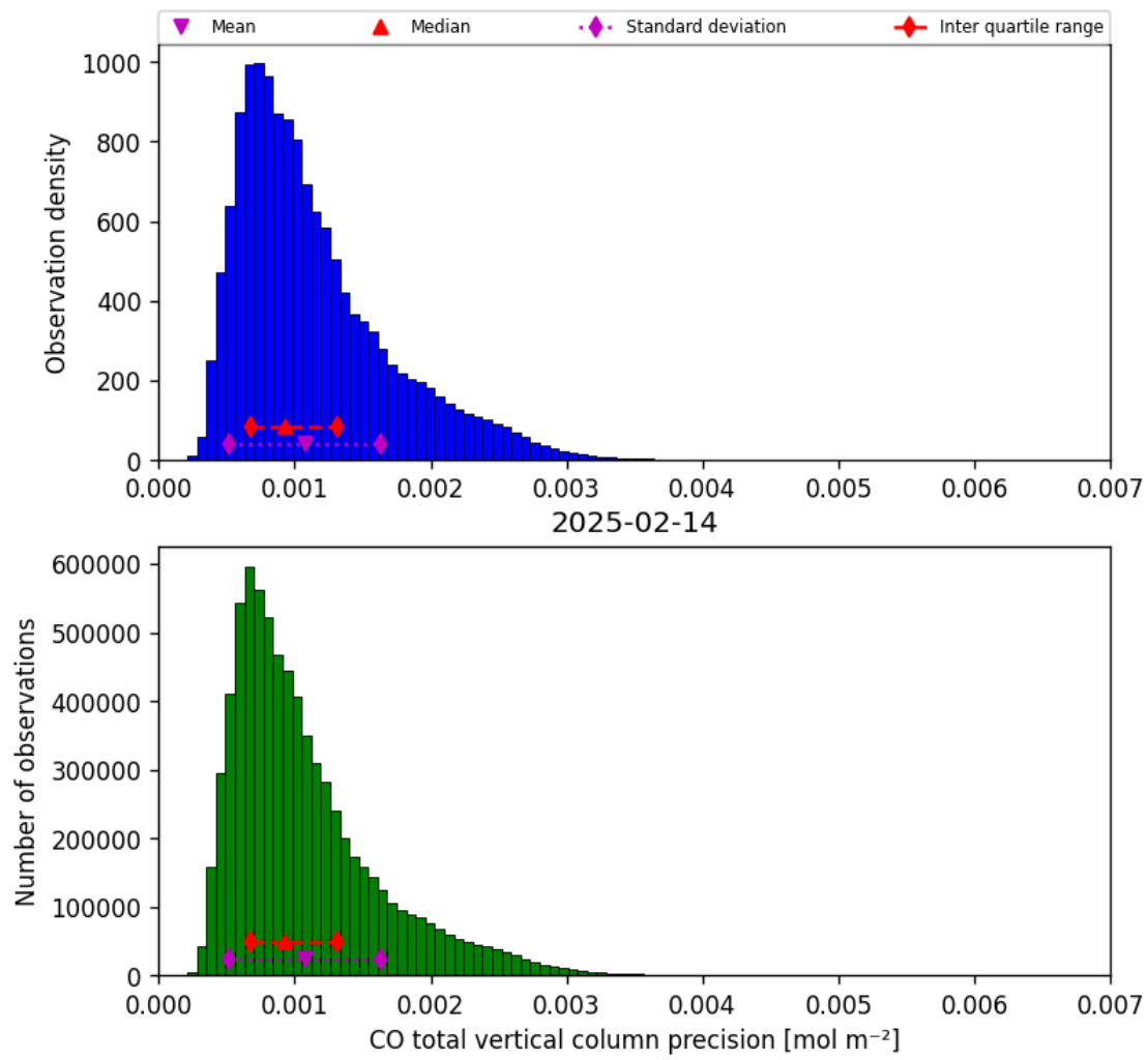
Figure 20: Histogram of “CO total vertical column precision” for 2025-02-13 to 2025-02-15
