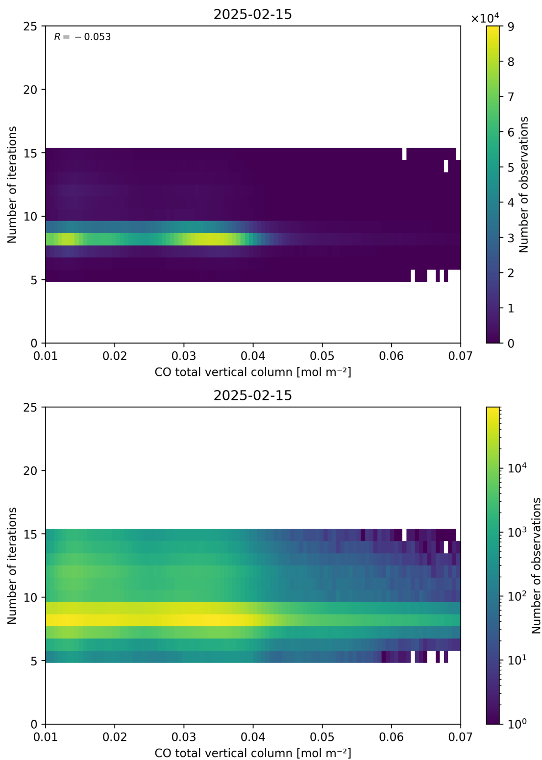
Figure 42: Scatter density plot of “CO total vertical column” against “Number of iterations” for 2025-02-14 to 2025-02-16.
