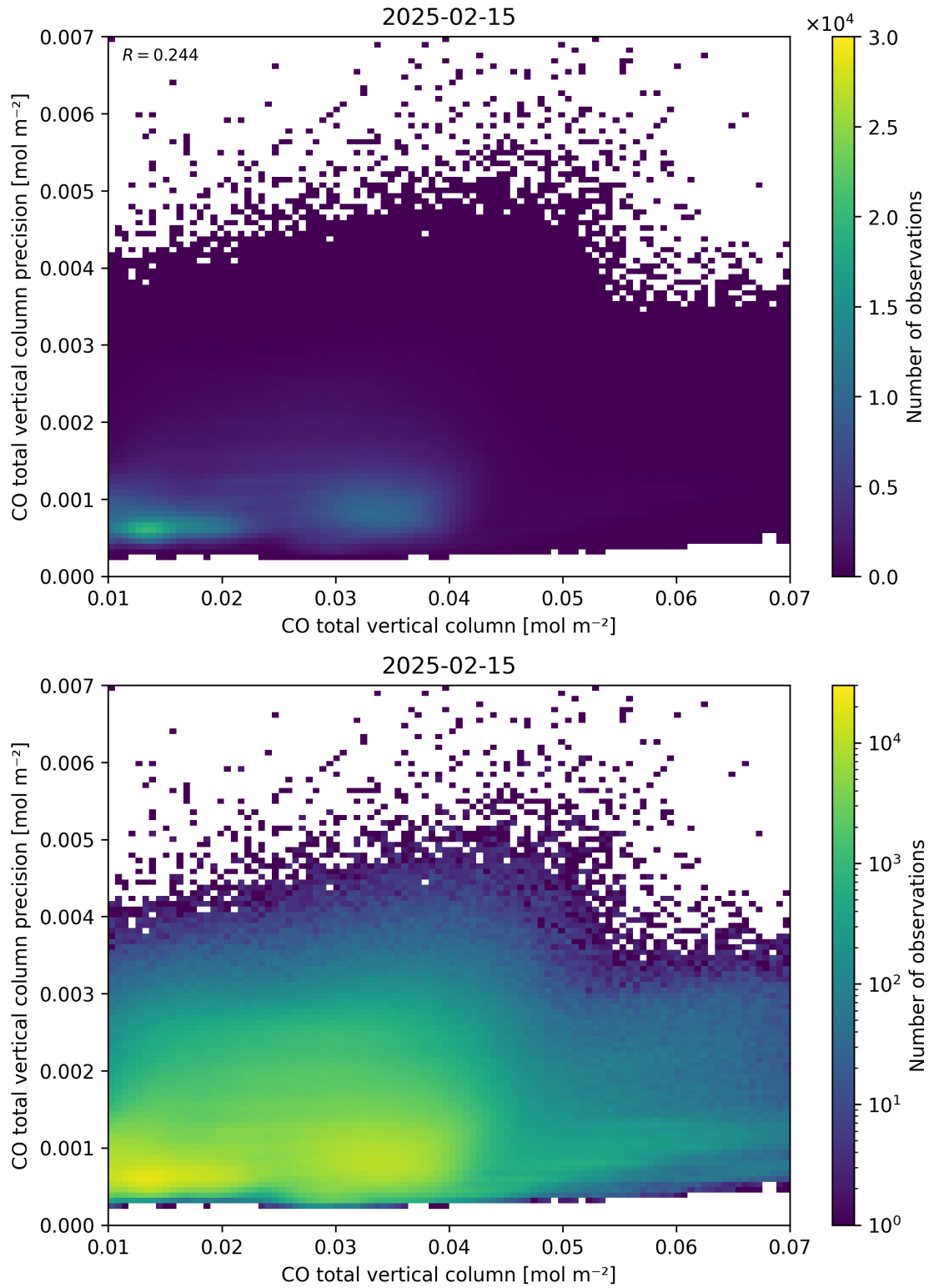
Figure 34: Scatter density plot of “CO total vertical column” against “CO total vertical column precision” for 2025-02-14 to 2025-02-16.
