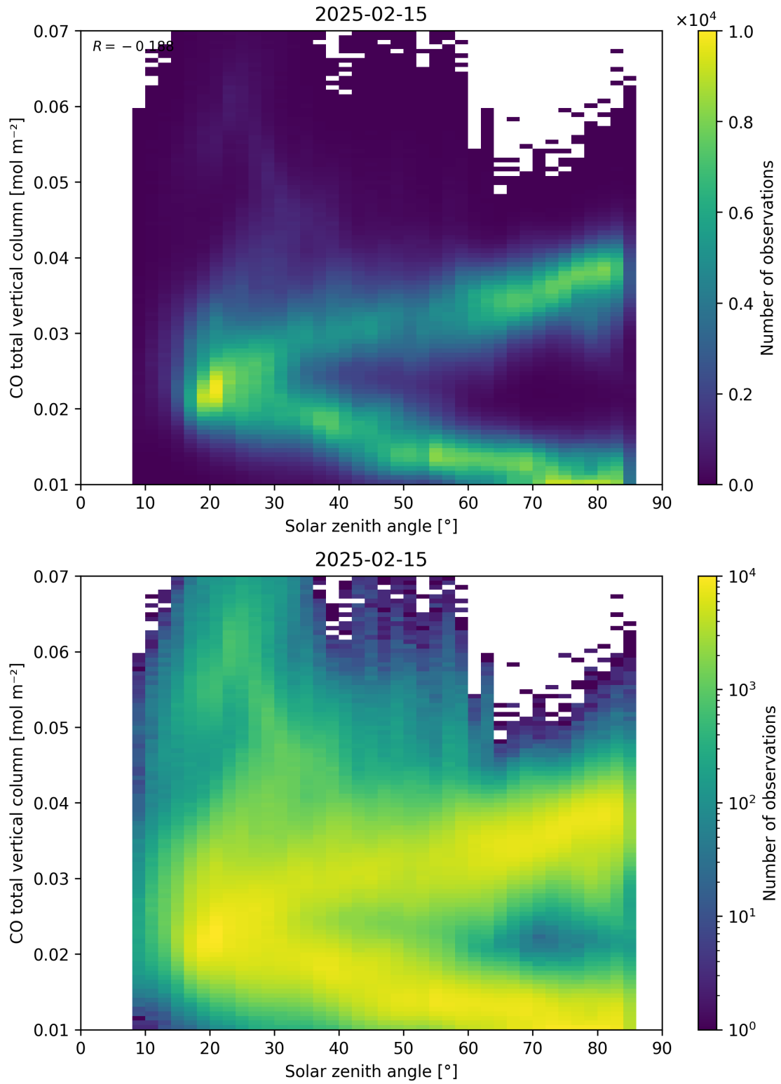
Figure 61: Scatter density plot of “Solar zenith angle” against “CO total vertical column” for 2025-02-14 to 2025-02-16.
