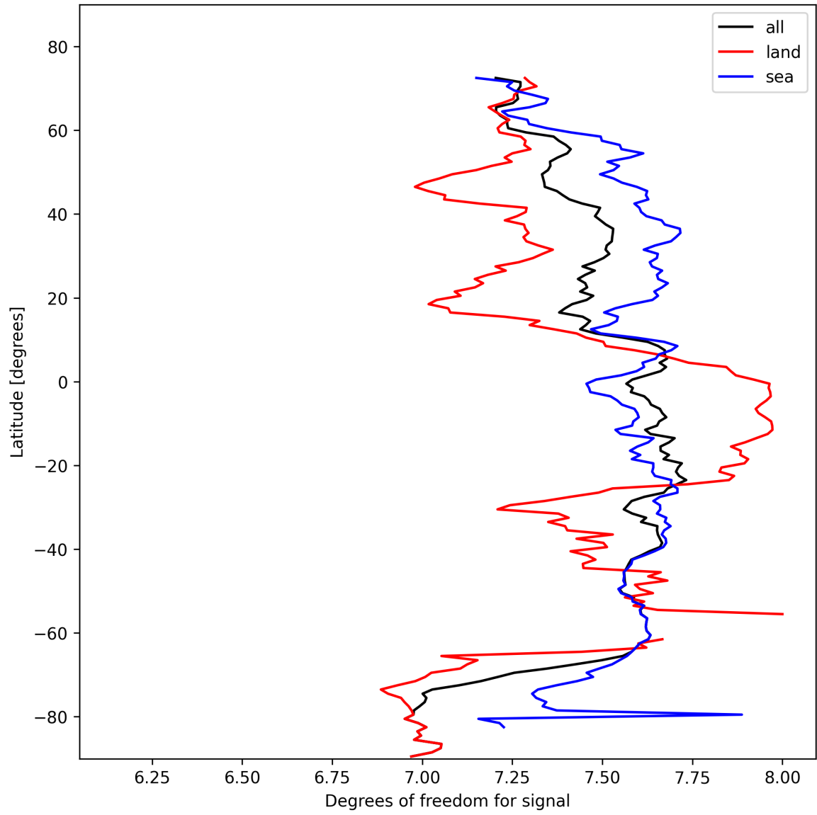
Figure 15: Zonal average of “Degrees of freedom for signal” for 2025-02-14 to 2025-02-16.
