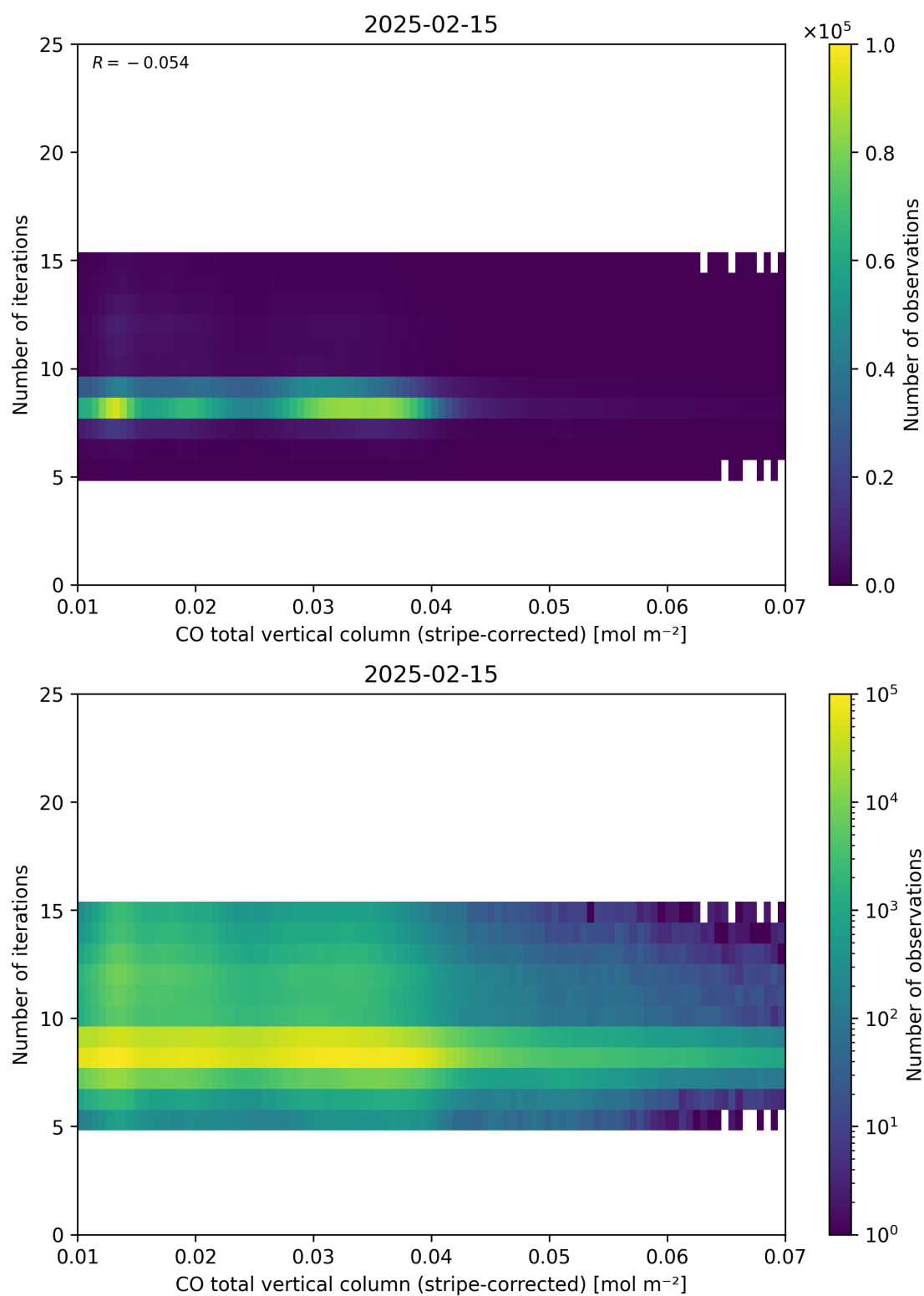
Figure 39: Scatter density plot of “CO total vertical column (stripe-corrected)” against “Number of iterations” for 2025-02-14 to 2025-02-16.
