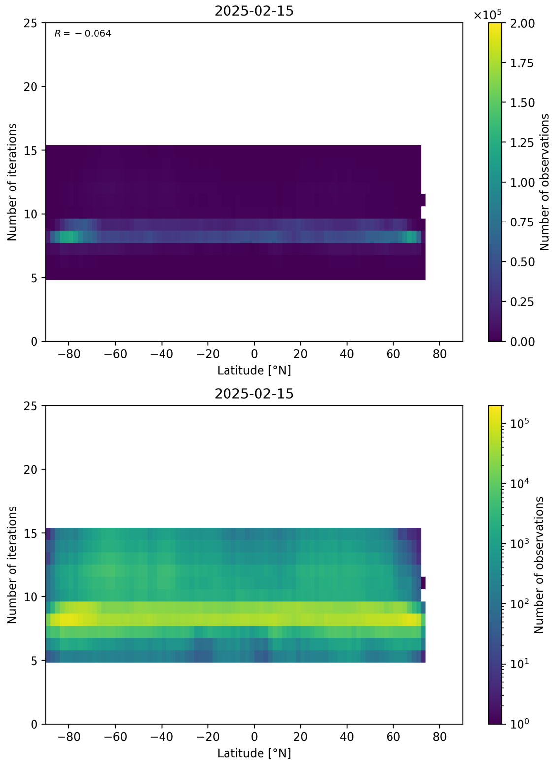
Figure 56: Scatter density plot of “Latitude” against “Number of iterations” for 2025-02-14 to 2025-02-16.
