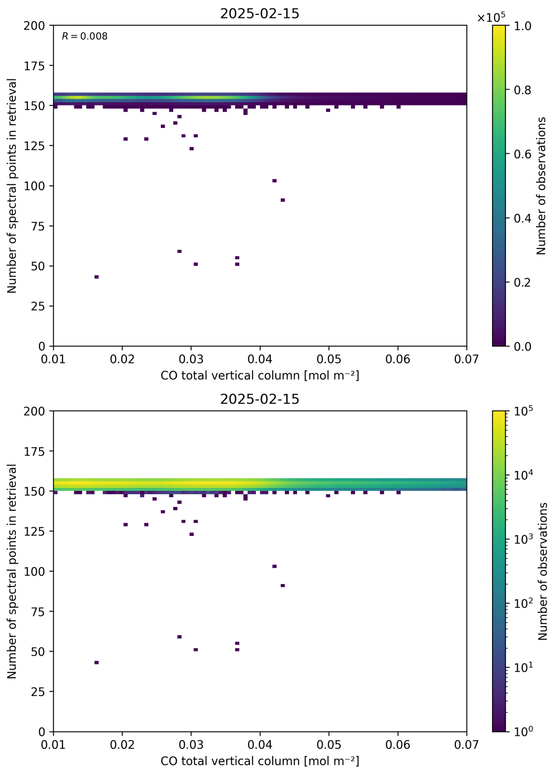
Figure 43: Scatter density plot of “CO total vertical column” against “Number of spectral points in retrieval” for 2025-02-14 to 2025-02-16.
