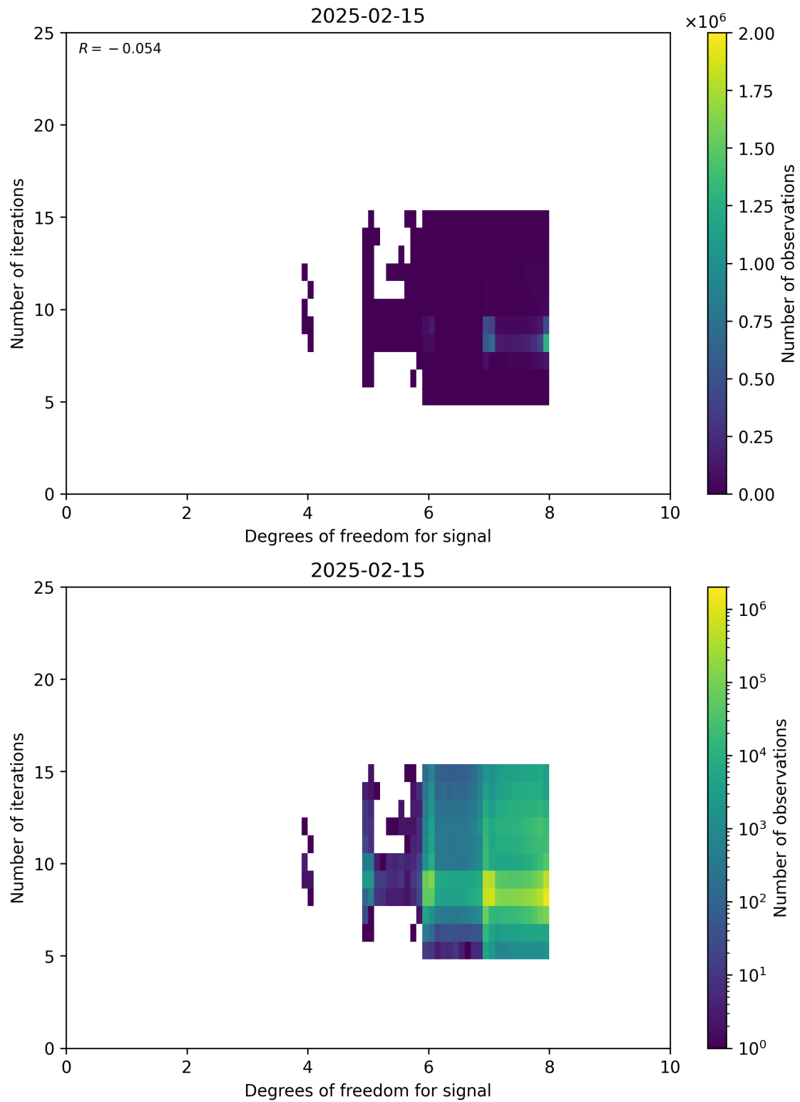
Figure 50: Scatter density plot of “Degrees of freedom for signal” against “Number of iterations” for 2025-02-14 to 2025-02-16.
