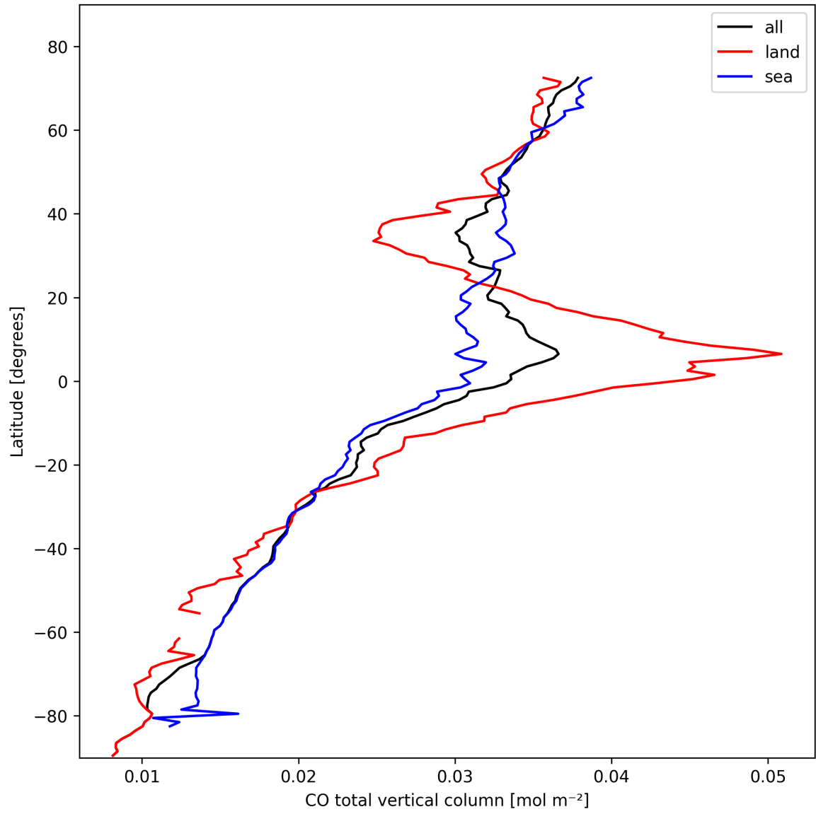
Figure 10: Zonal average of “CO total vertical column” for 2025-02-14 to 2025-02-16.
