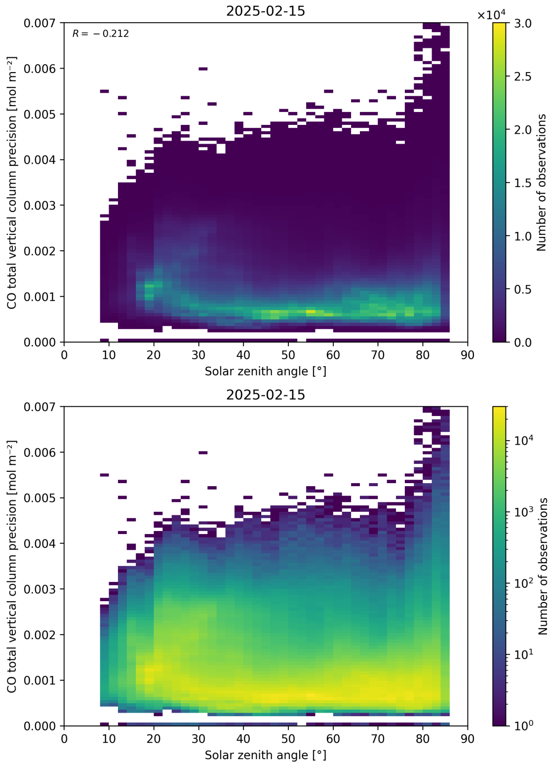
Figure 63: Scatter density plot of “Solar zenith angle” against “CO total vertical column precision” for 2025-02-14 to 2025-02-16.
