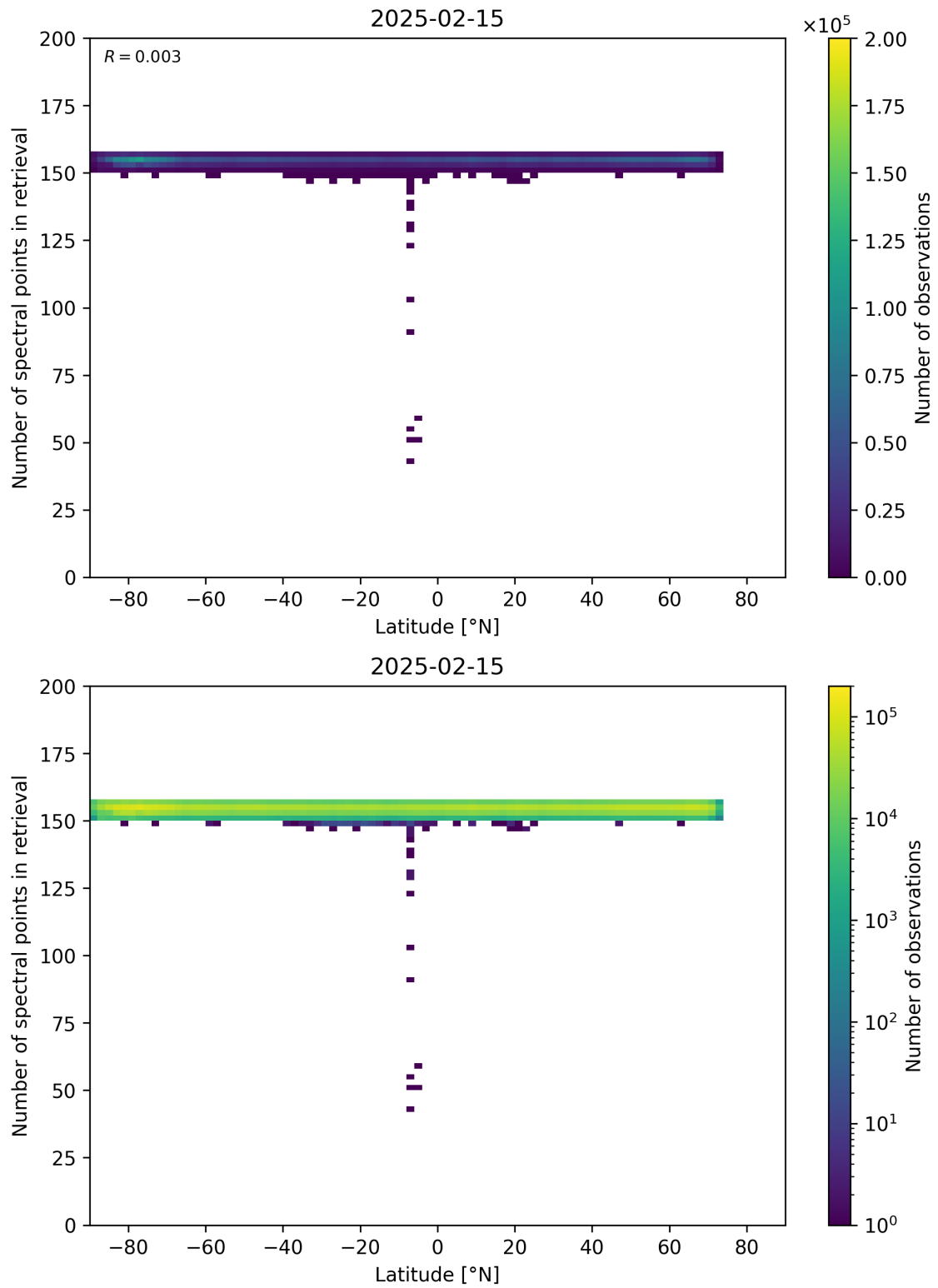
Figure 57: Scatter density plot of “Latitude” against “Number of spectral points in retrieval” for 2025-02-14 to 2025-02-16.
