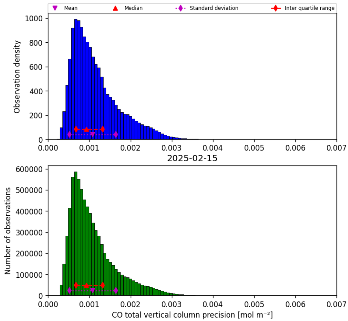
Figure 20: Histogram of “CO total vertical column precision” for 2025-02-14 to 2025-02-16
