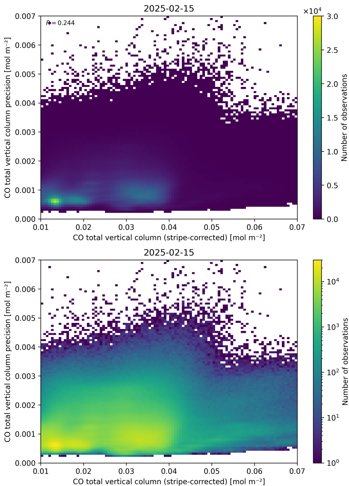
Figure 36: Scatter density plot of “CO total vertical column (stripe-corrected)” against “CO total vertical column precision” for 2025-02-14 to 2025-02-16.
