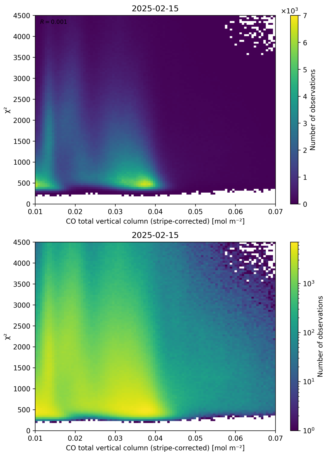
Figure 37: Scatter density plot of “CO total vertical column (stripe-corrected)” against “ \chi^2 ” for 2025-02-14 to 2025-02-16.
