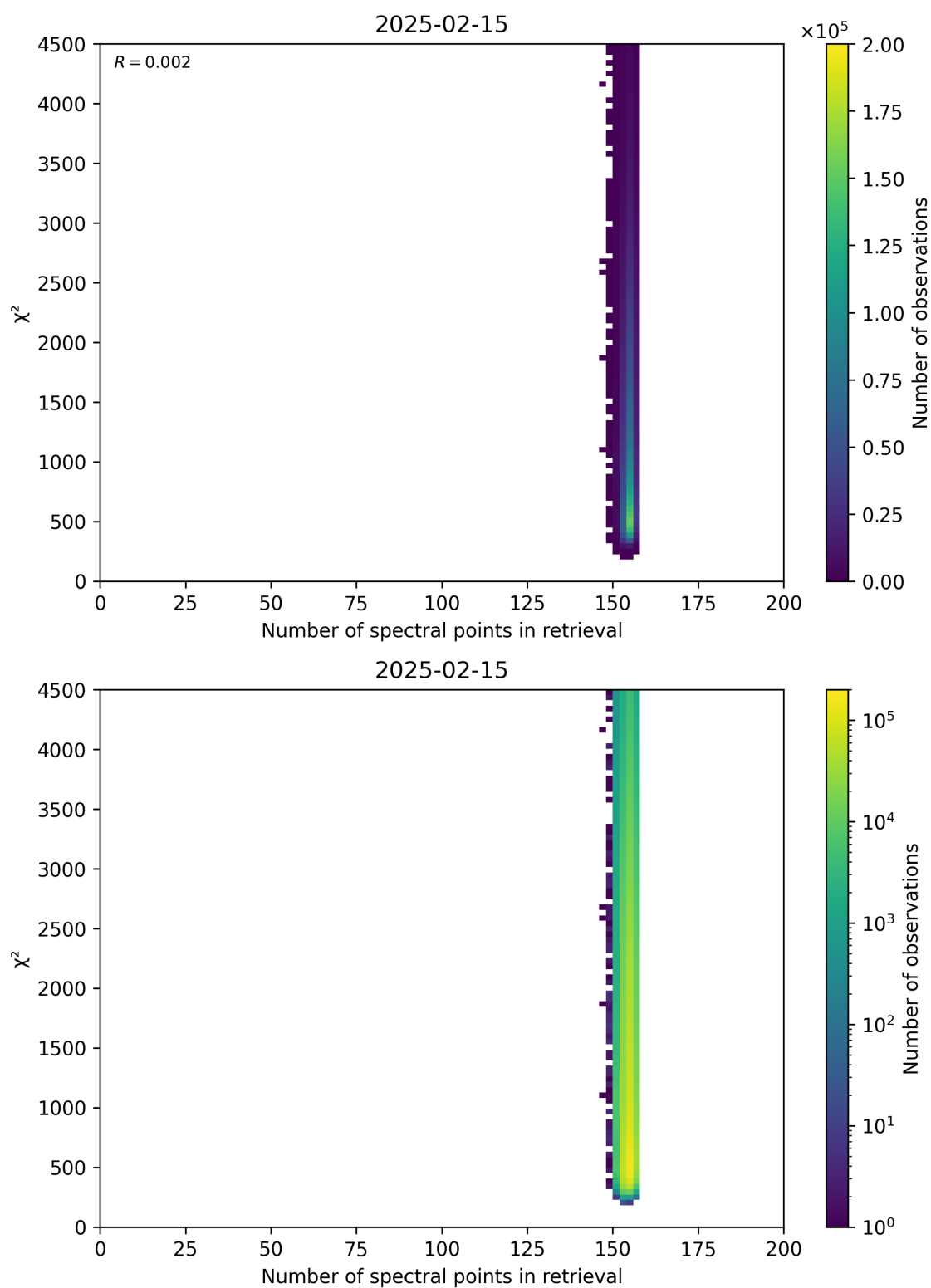
Figure 58: Scatter density plot of “Number of spectral points in retrieval” against “ \chi^2 ” for 2025-02-14 to 2025-02-16.
