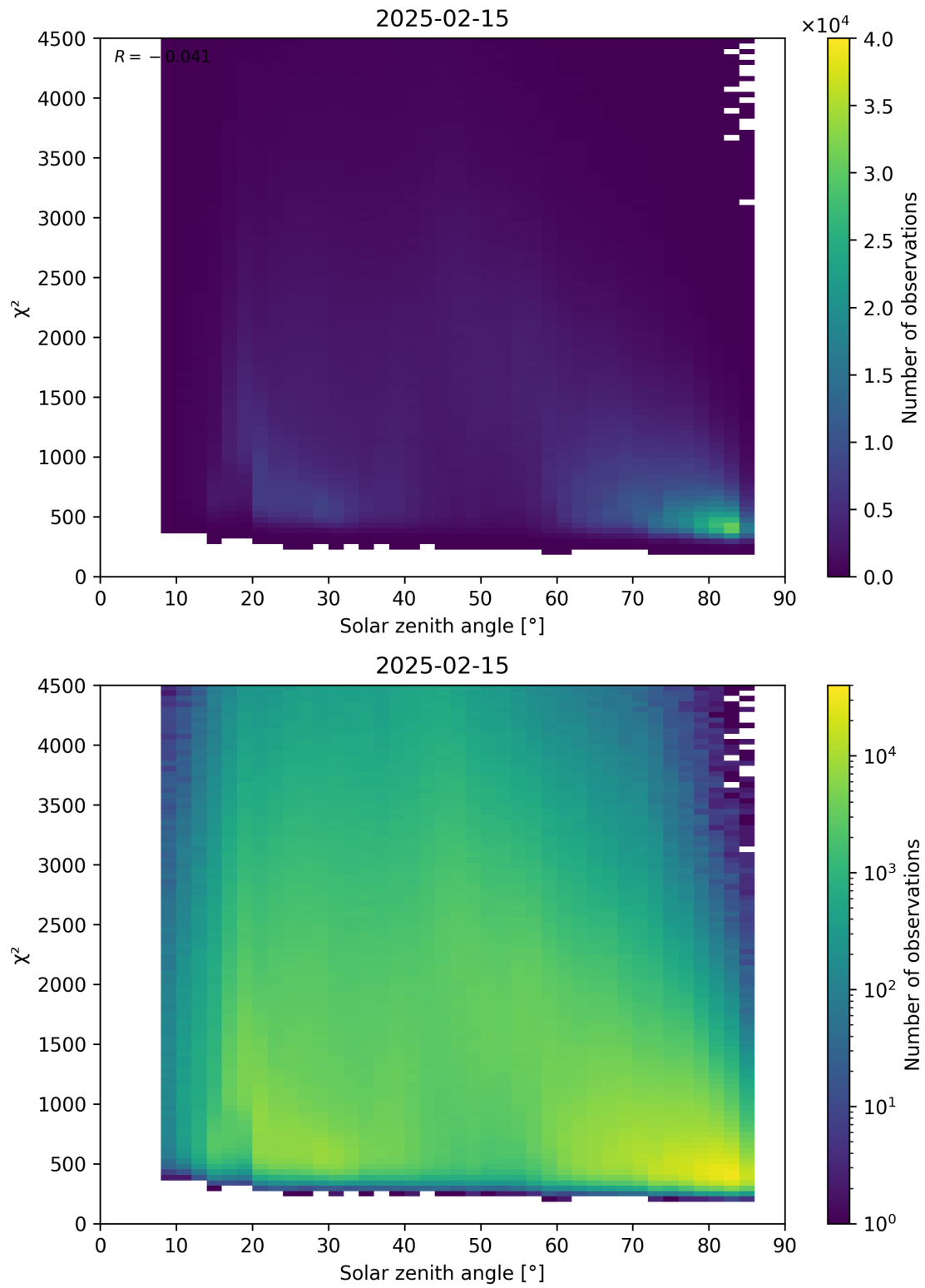
Figure 64: Scatter density plot of “Solar zenith angle” against “ \chi^2 ” for 2025-02-14 to 2025-02-16.
