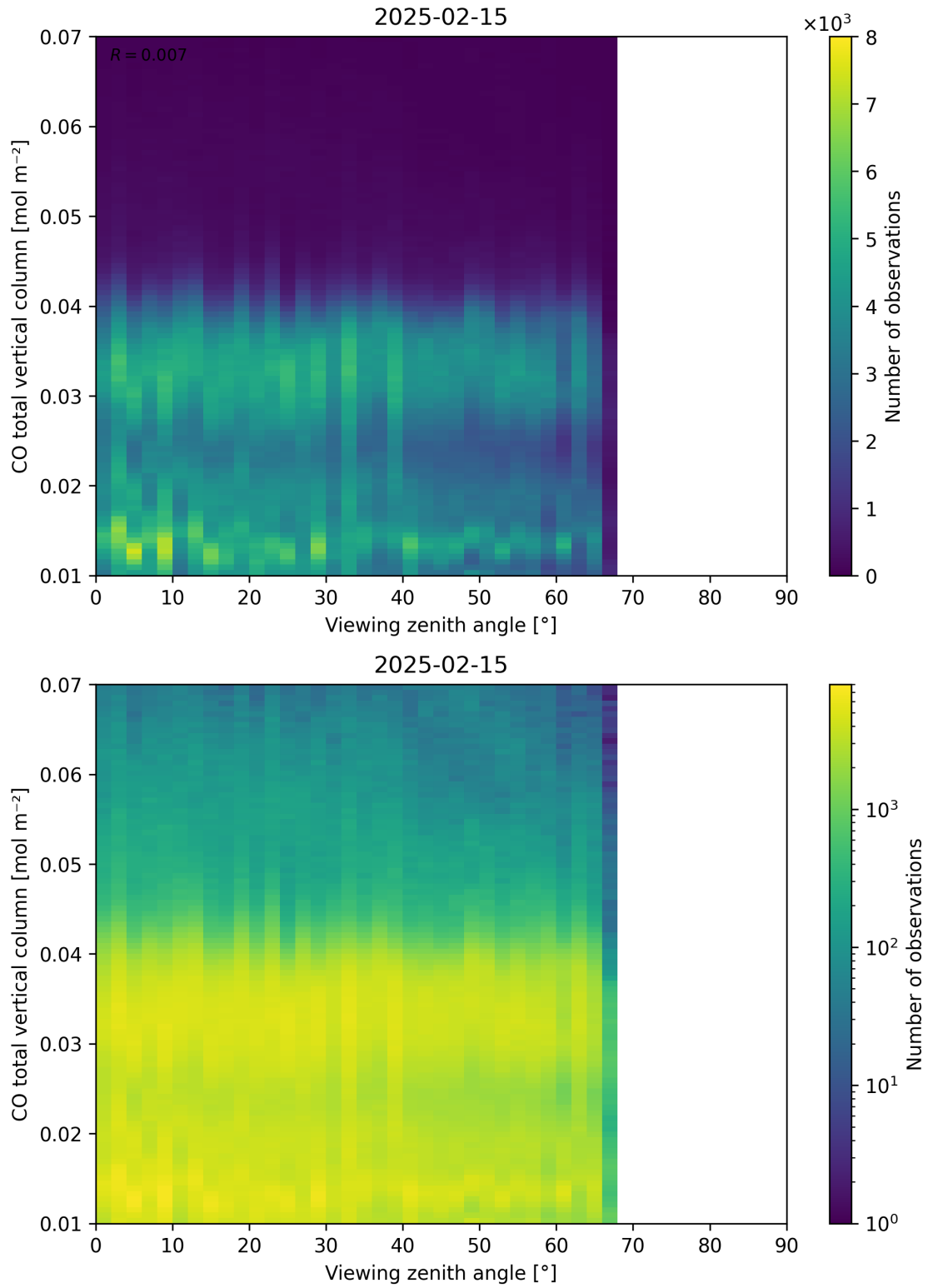
Figure 69: Scatter density plot of “Viewing zenith angle” against “CO total vertical column” for 2025-02-14 to 2025-02-16.
