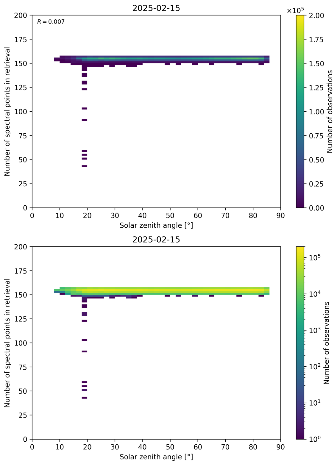
Figure 68: Scatter density plot of “Solar zenith angle” against “Number of spectral points in retrieval” for 2025-02-14 to 2025-02-16.
