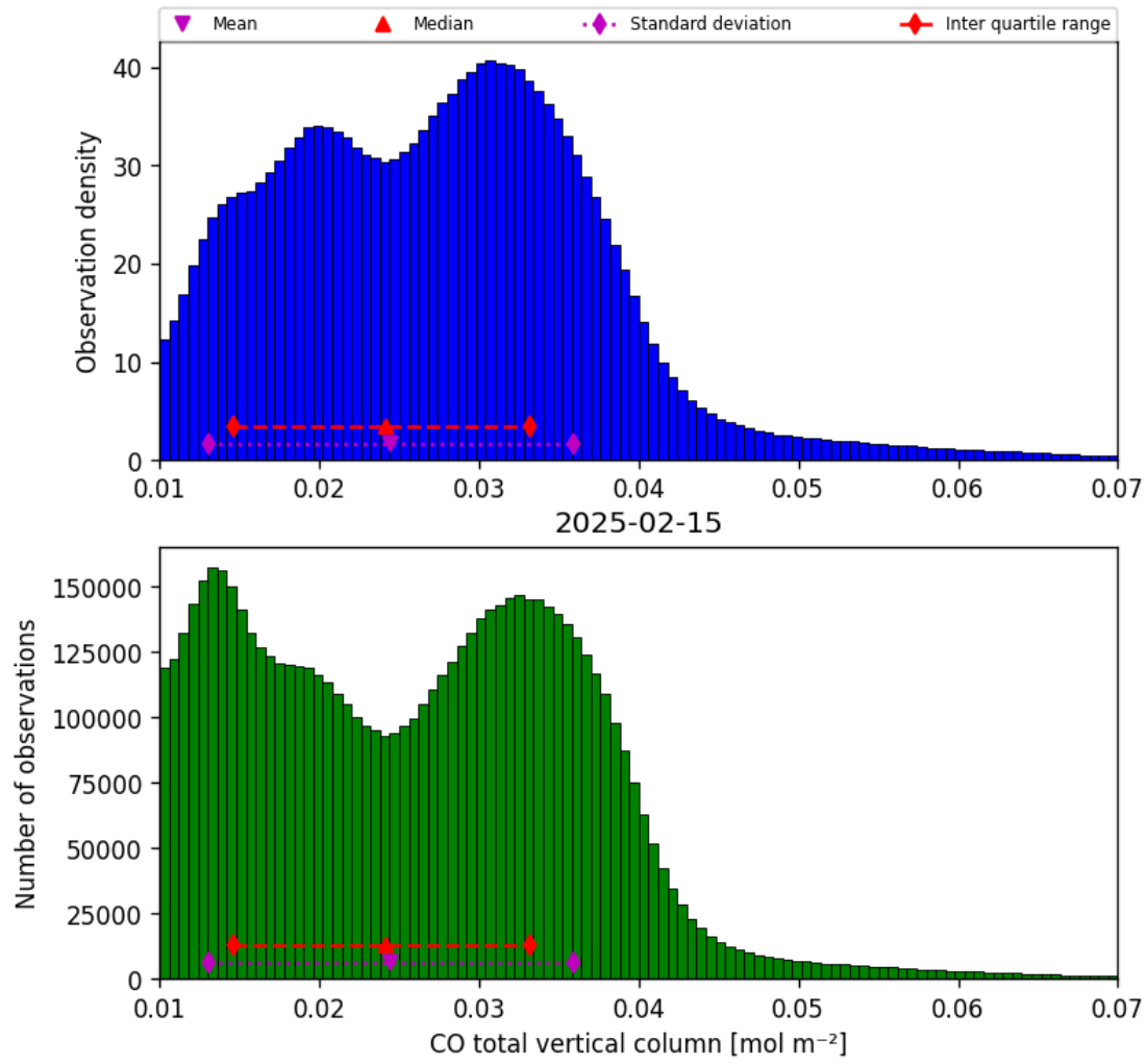
Figure 18: Histogram of “CO total vertical column” for 2025-02-14 to 2025-02-16
