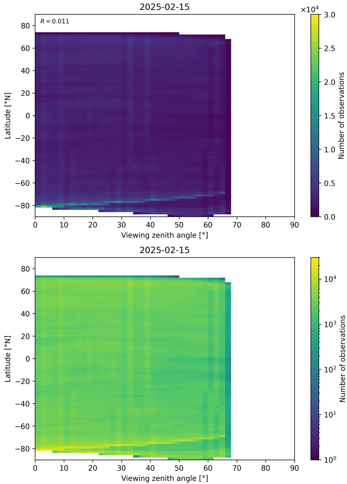
Figure 74: Scatter density plot of “Viewing zenith angle” against “Latitude” for 2025-02-14 to 2025-02-16.
