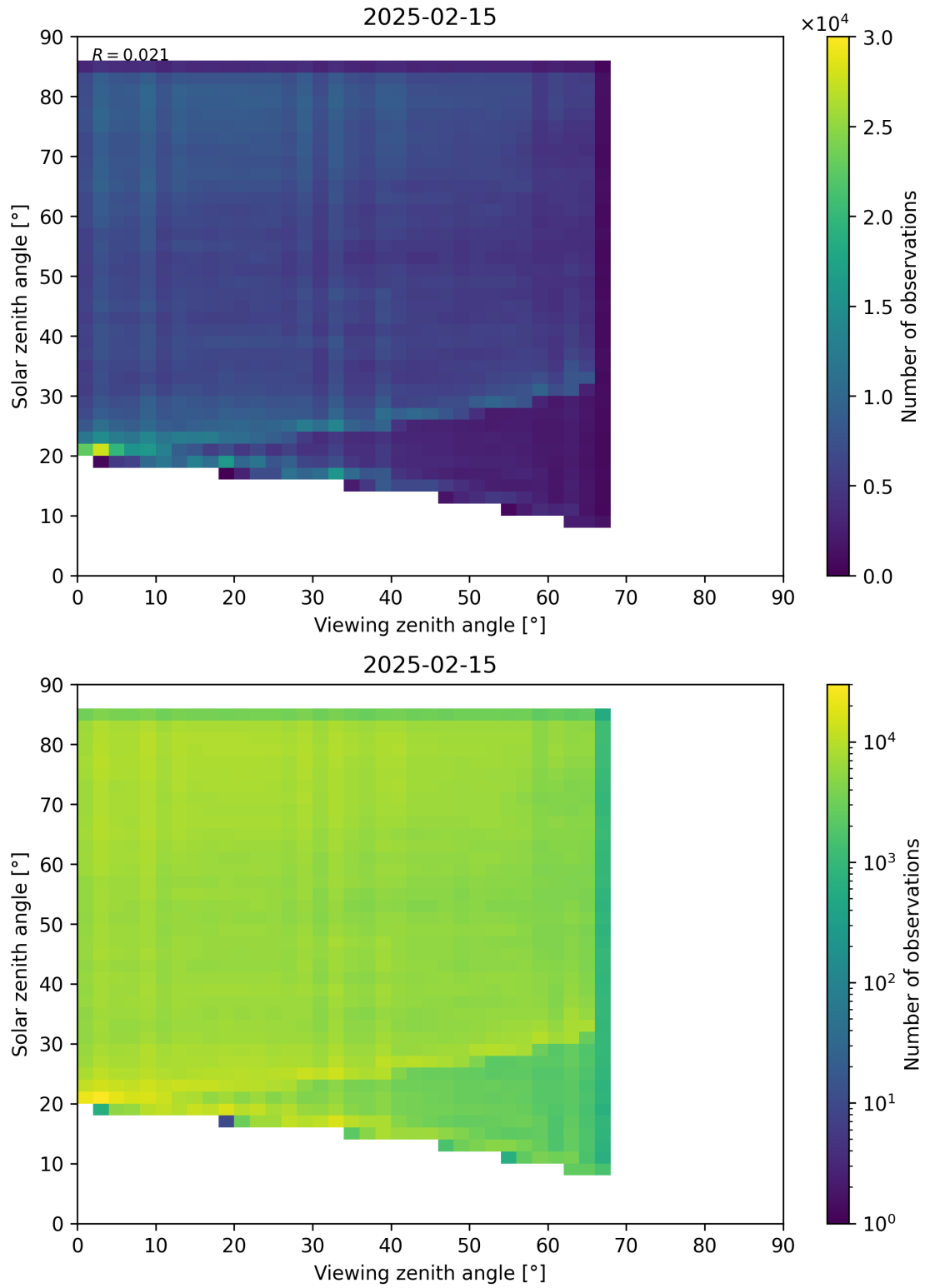
Figure 77: Scatter density plot of “Viewing zenith angle” against “Solar zenith angle” for 2025-02-14 to 2025-02-16.
