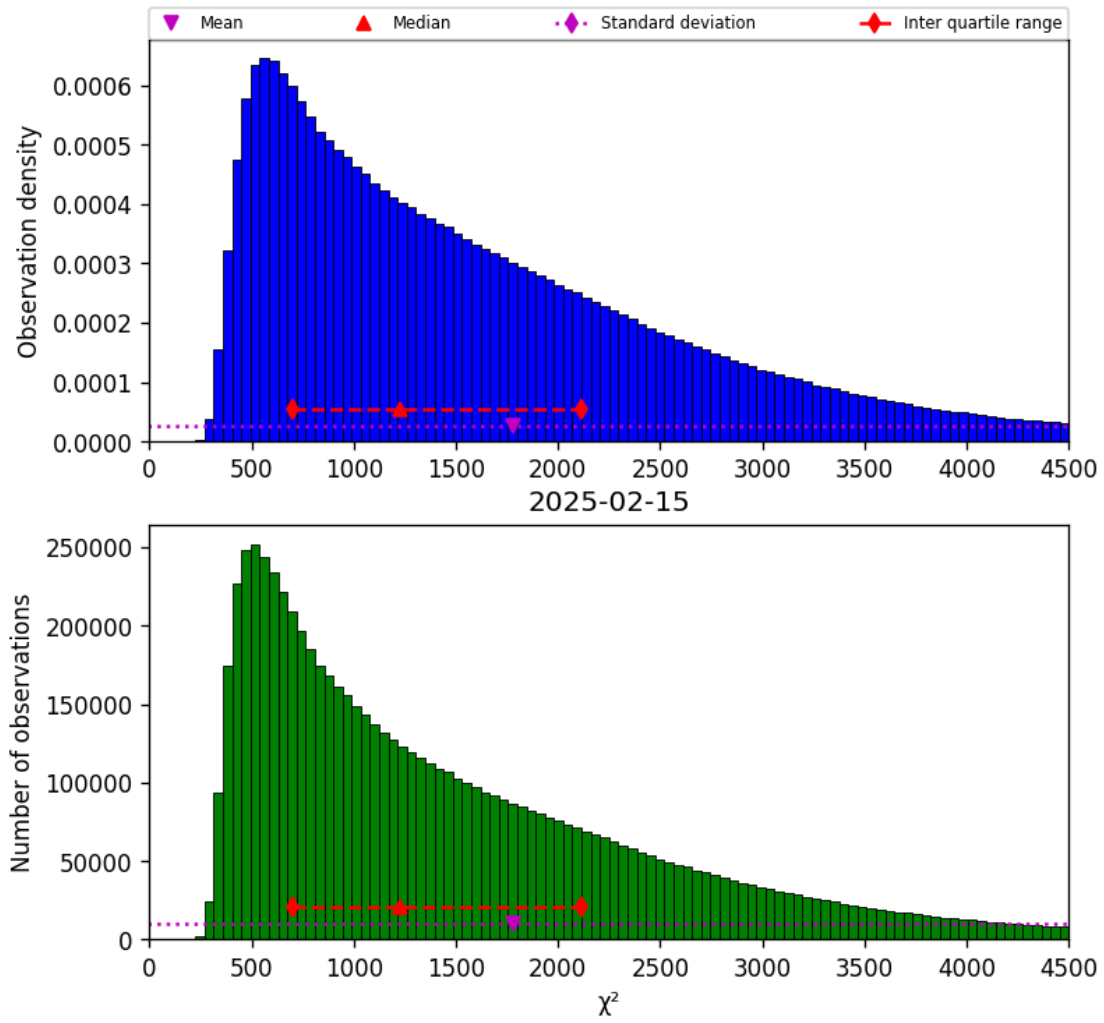
Figure 22: Histogram of “ \chi^2 ” for 2025-02-14 to 2025-02-16
