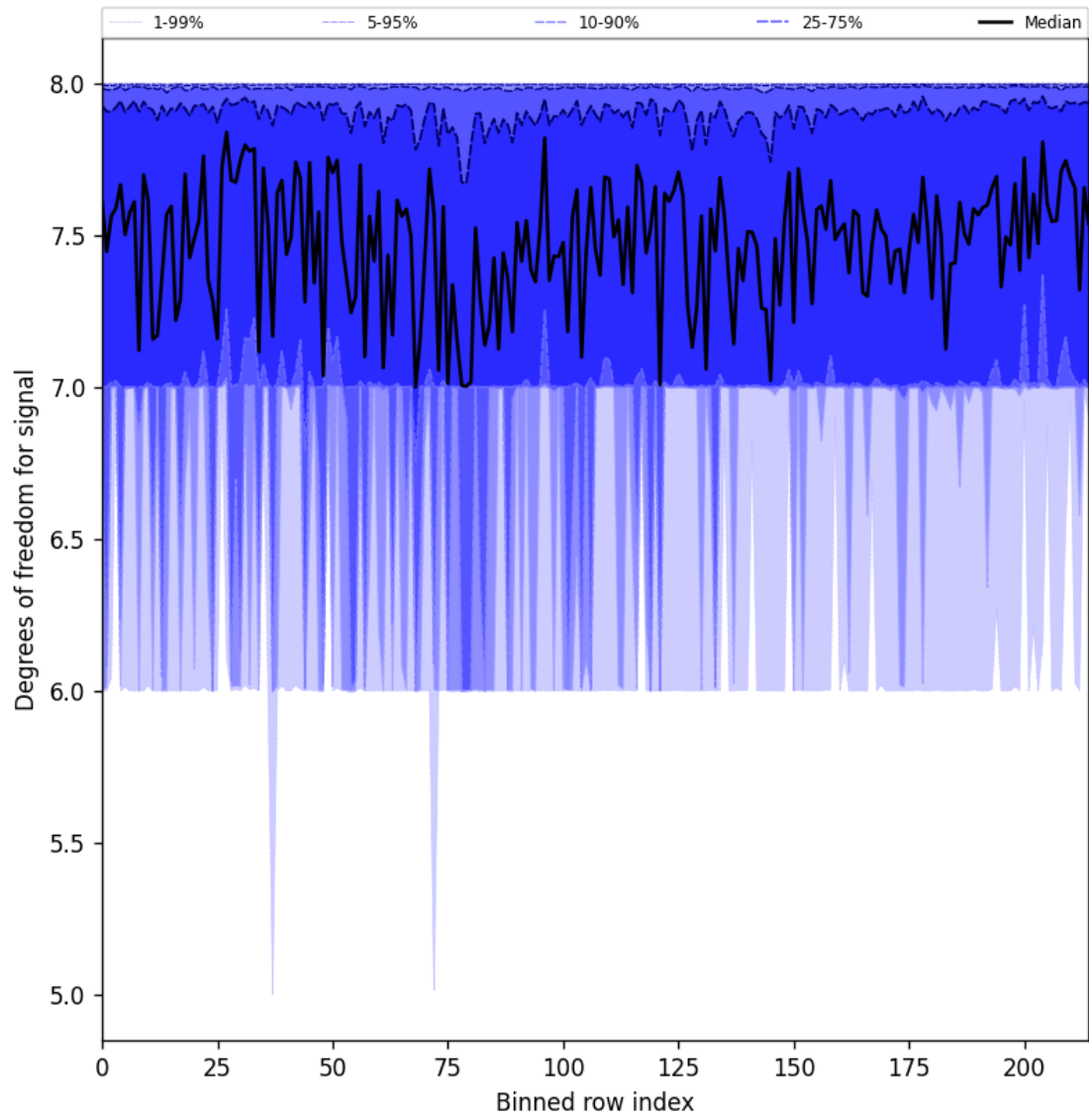
Figure 31: Along track statistics of “Degrees of freedom for signal” for 2025-02-14 to 2025-02-16
