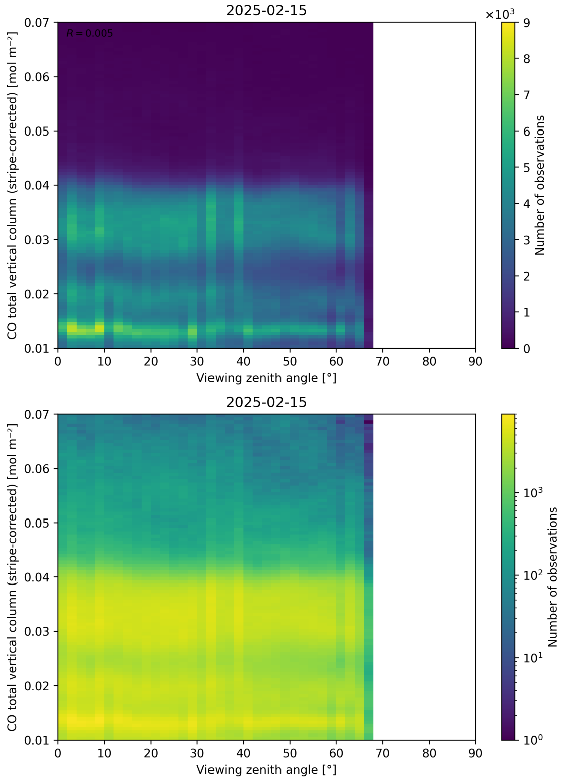
Figure 70: Scatter density plot of “Viewing zenith angle” against “CO total vertical column (stripe-corrected)” for 2025-02-14 to 2025-02-16.
