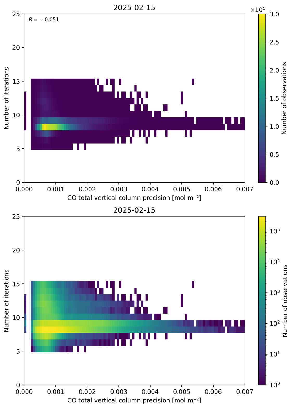
Figure 46: Scatter density plot of “CO total vertical column precision” against “Number of iterations” for 2025-02-14 to 2025-02-16.
