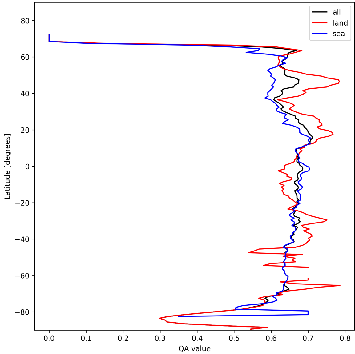
Figure 9: Zonal average of “QA value” for 2025-02-14 to 2025-02-16.
