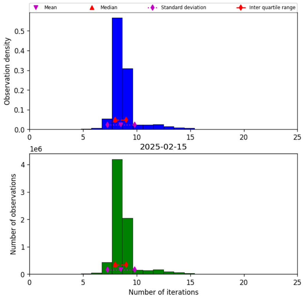
Figure 24: Histogram of “Number of iterations” for 2025-02-14 to 2025-02-16
