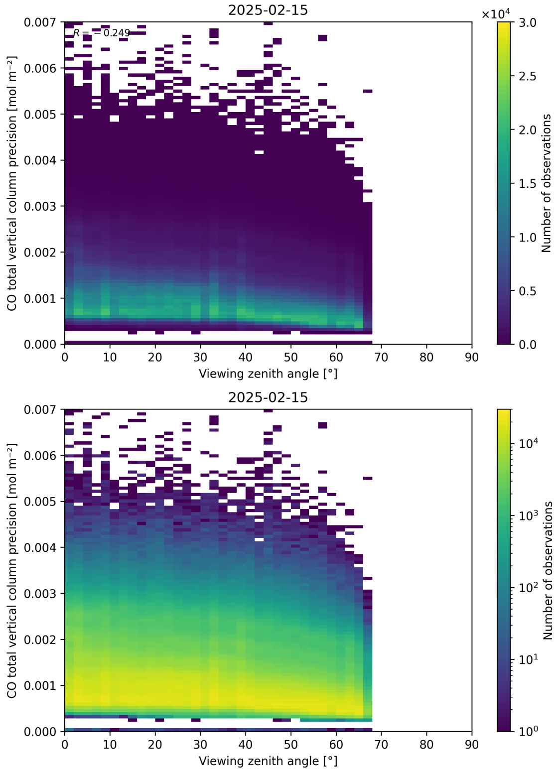
Figure 71: Scatter density plot of “Viewing zenith angle” against “CO total vertical column precision” for 2025-02-14 to 2025-02-16.
