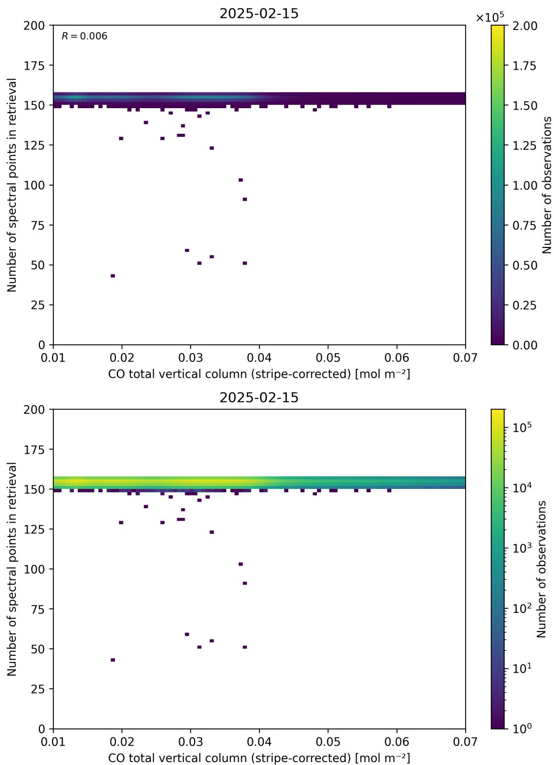
Figure 40: Scatter density plot of “CO total vertical column (stripe-corrected)” against “Number of spectral points in retrieval” for 2025-02-14 to 2025-02-16.
