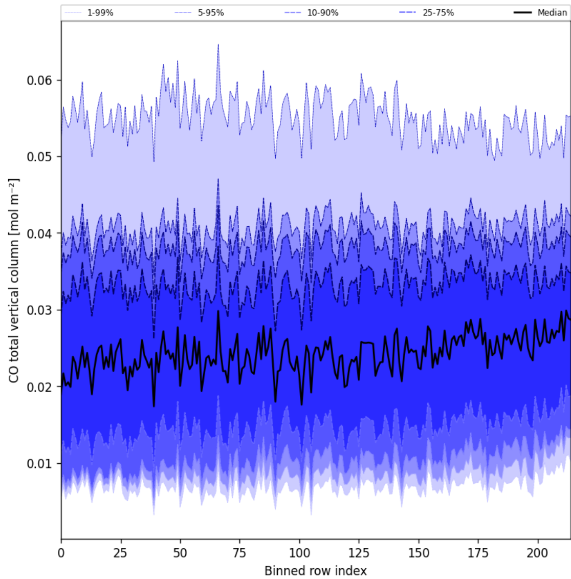
Figure 26: Along track statistics of “CO total vertical column” for 2025-02-14 to 2025-02-16
