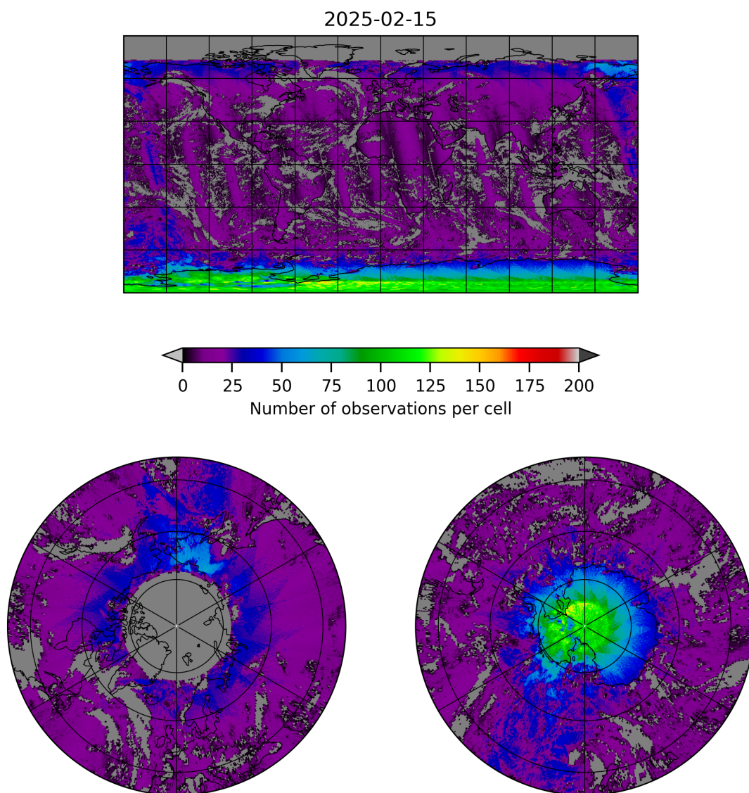
Figure 8: Map of the number of observations for 2025-02-14 to 2025-02-16
