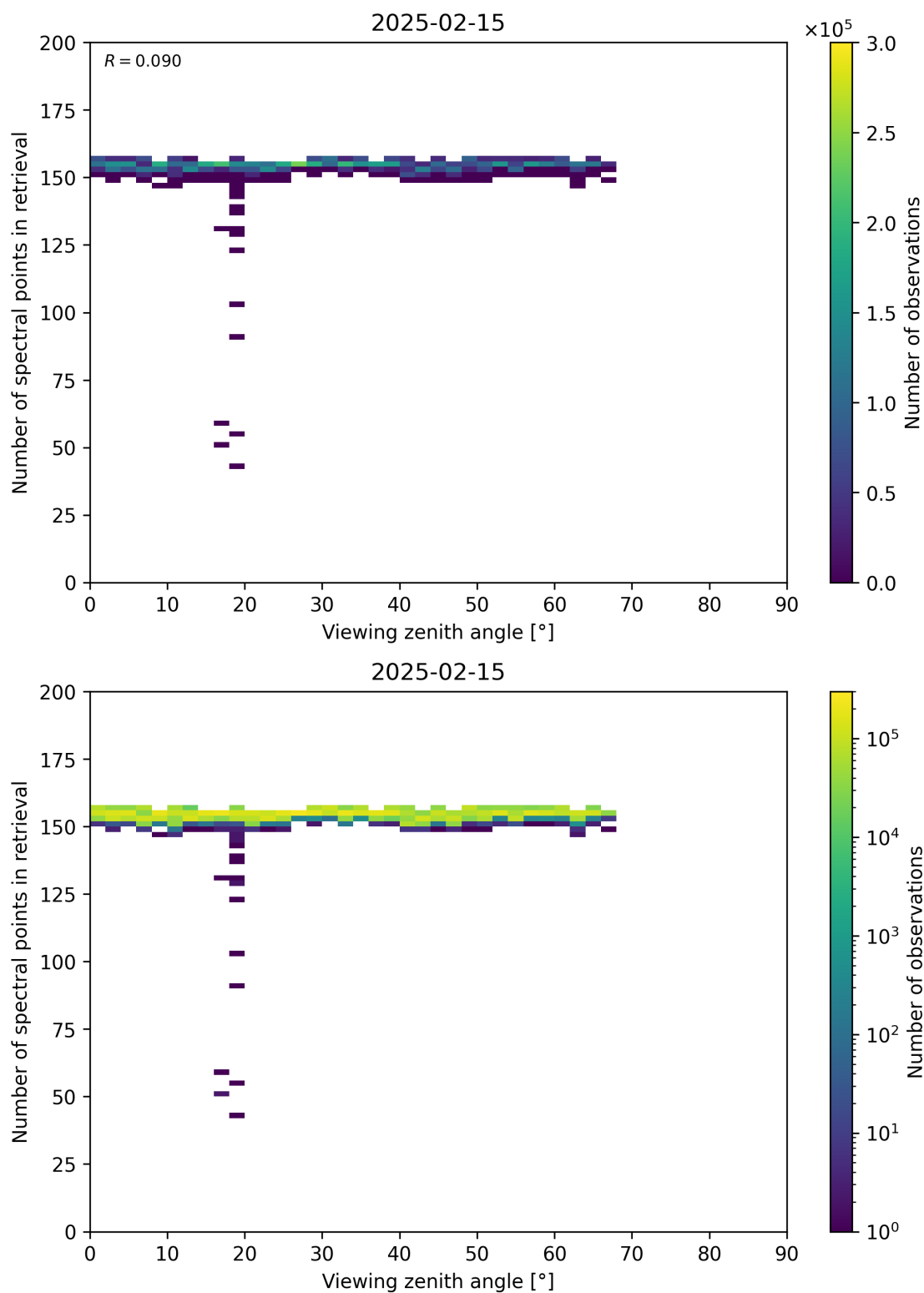
Figure 76: Scatter density plot of “Viewing zenith angle” against “Number of spectral points in retrieval” for 2025-02-14 to 2025-02-16.
