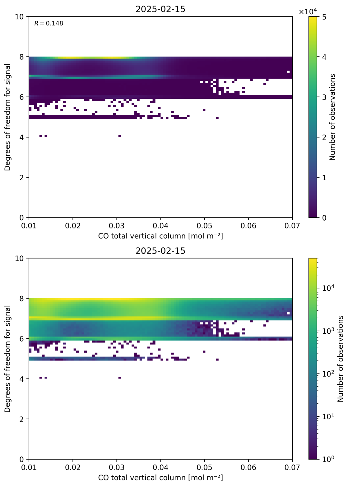
Figure 41: Scatter density plot of “CO total vertical column” against “Degrees of freedom for signal” for 2025-02-14 to 2025-02-16.
