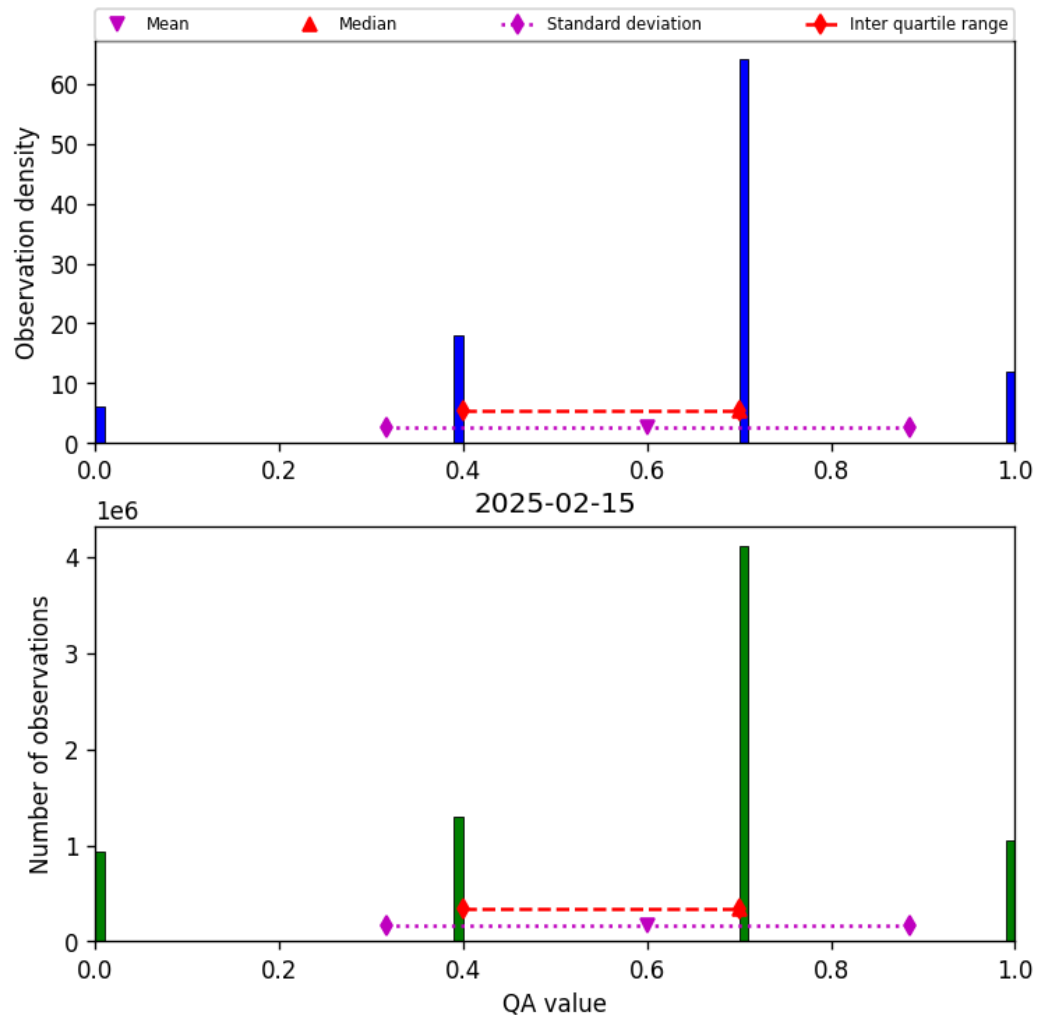
Figure 17: Histogram of “QA value” for 2025-02-14 to 2025-02-16
