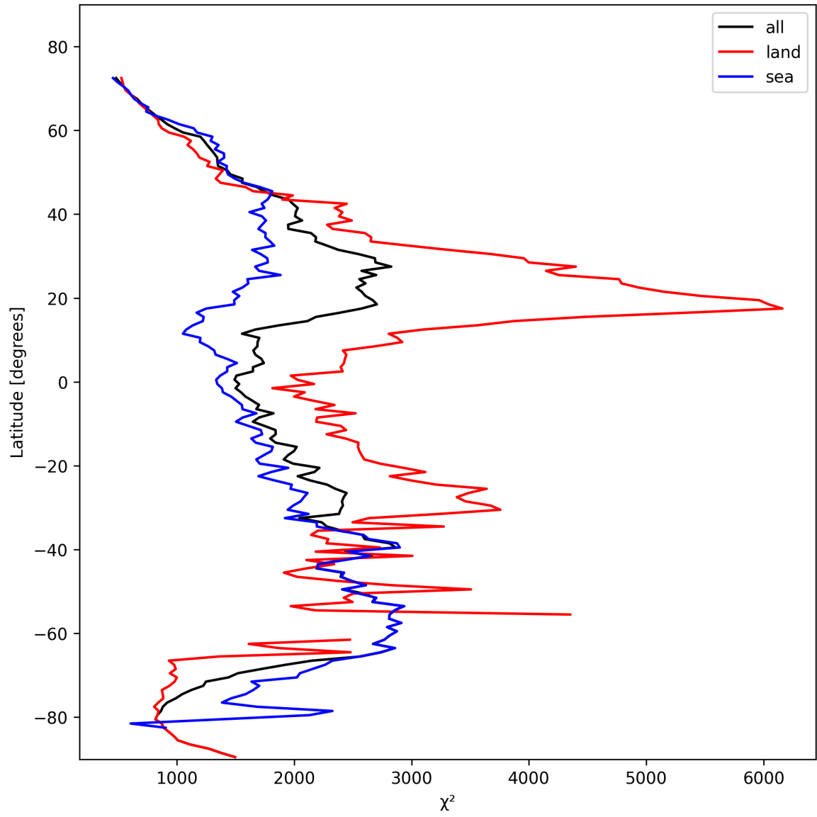
Figure 14: Zonal average of “ \chi^2 ” for 2025-02-14 to 2025-02-16.
