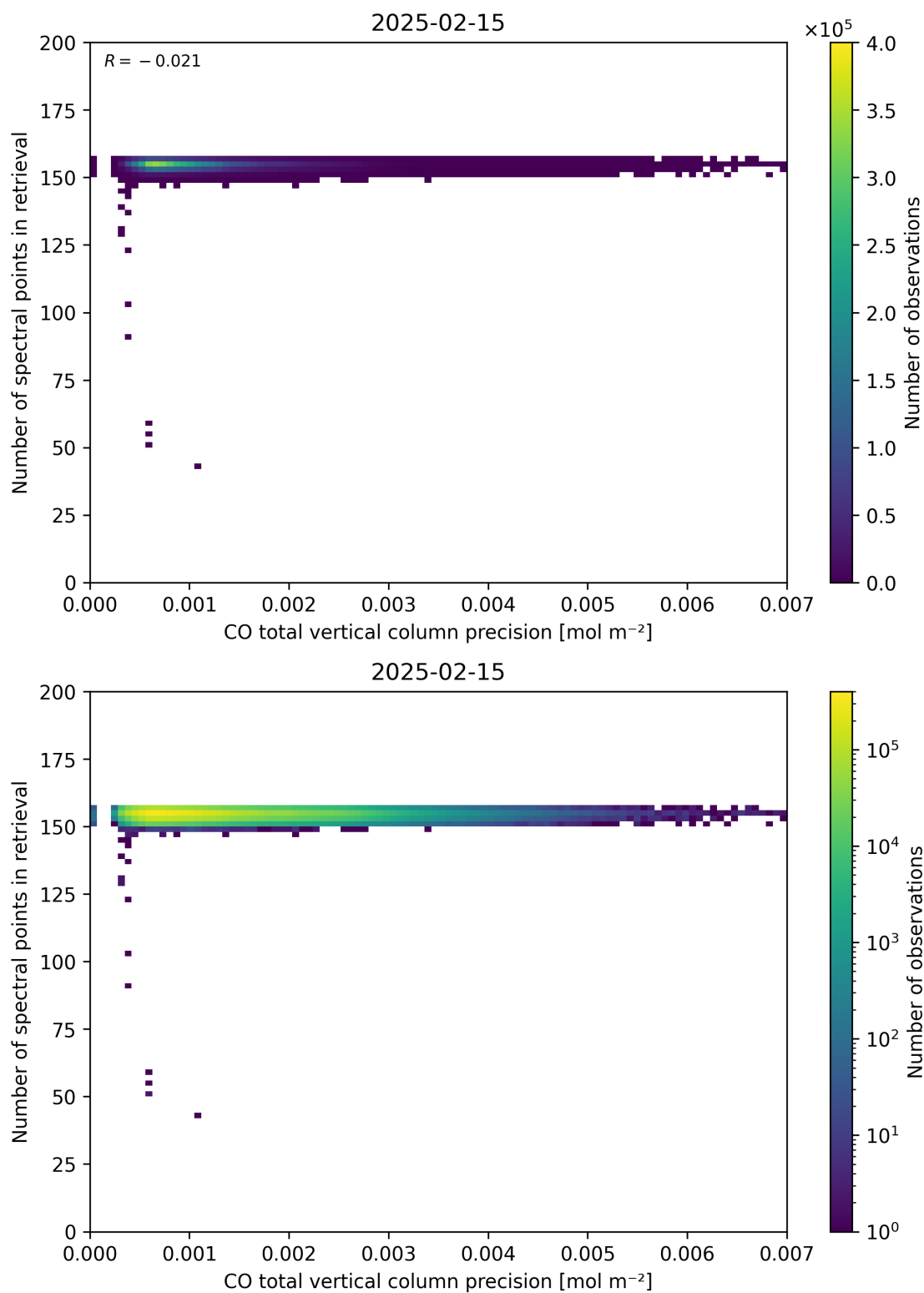
Figure 47: Scatter density plot of “CO total vertical column precision” against “Number of spectral points in retrieval” for 2025-02-14 to 2025-02-16.
