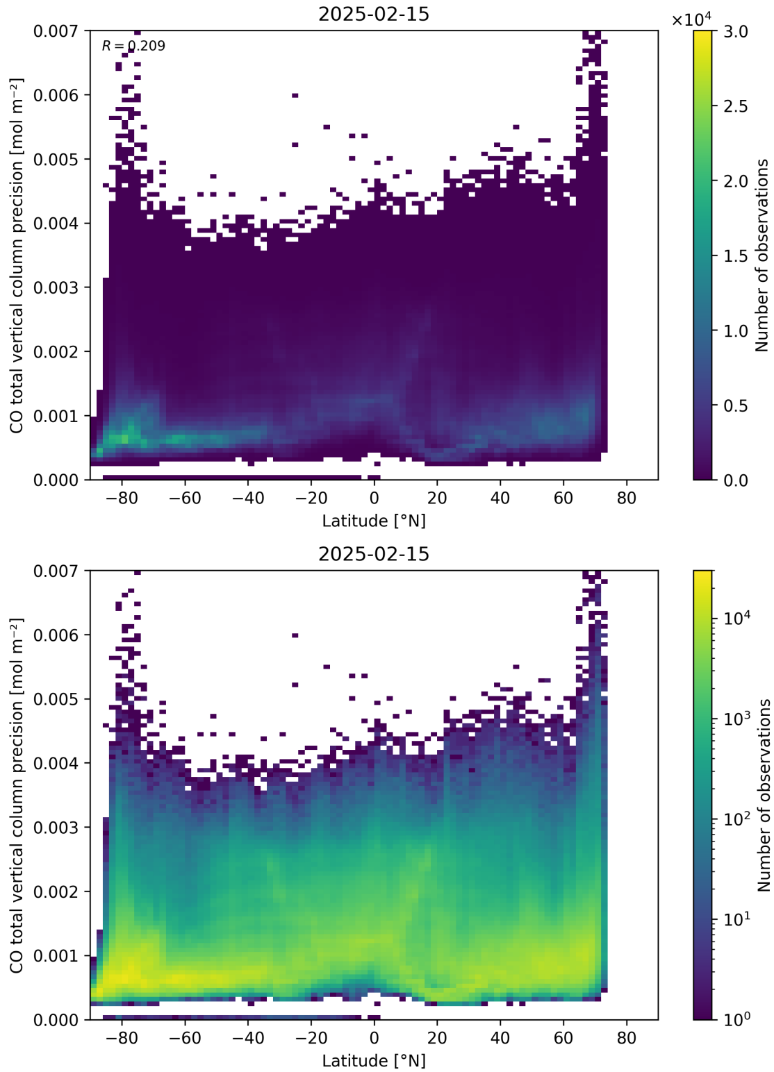
Figure 53: Scatter density plot of “Latitude” against “CO total vertical column precision” for 2025-02-14 to 2025-02-16.
