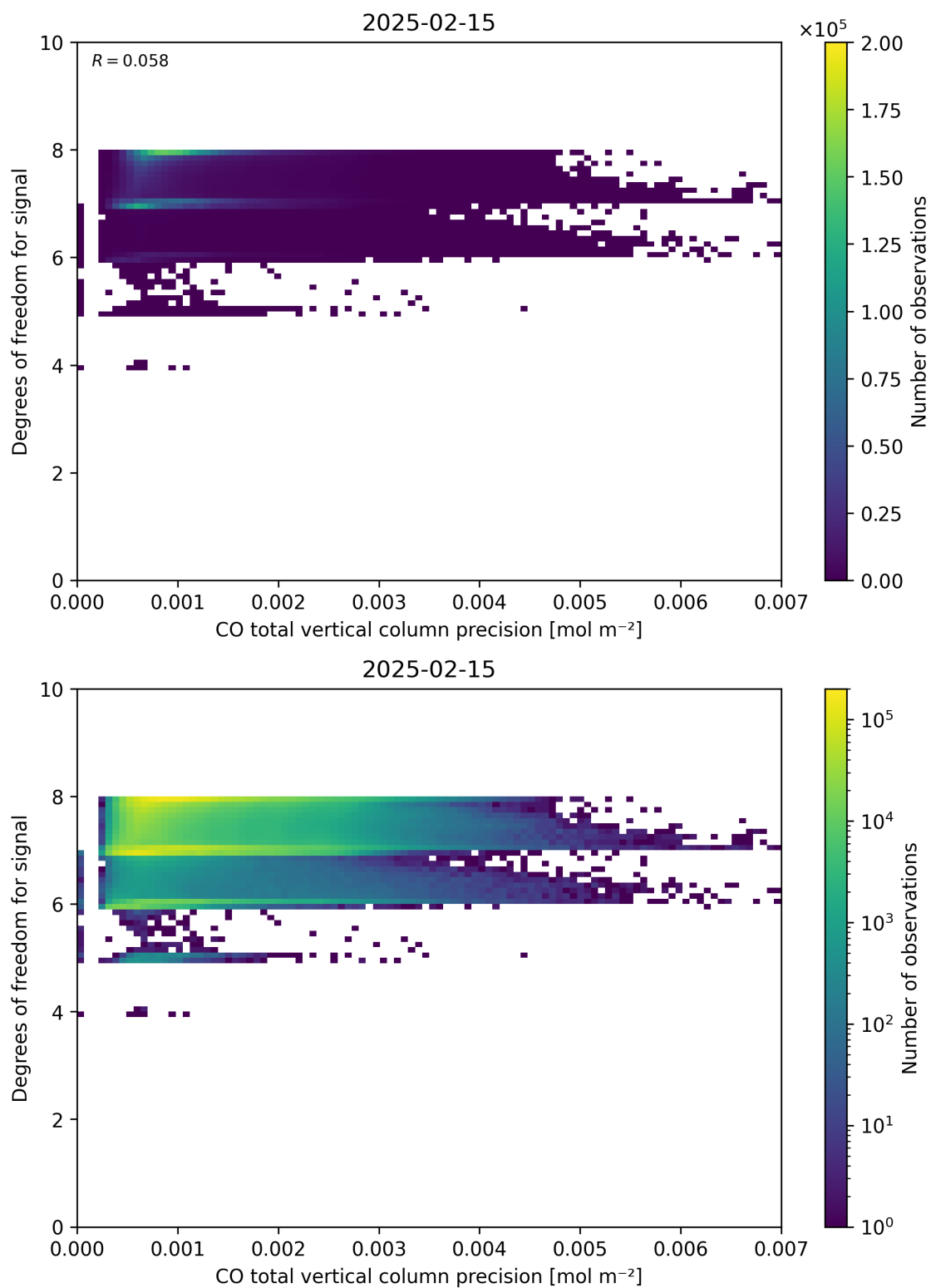
Figure 45: Scatter density plot of “CO total vertical column precision” against “Degrees of freedom for signal” for 2025-02-14 to 2025-02-16.
