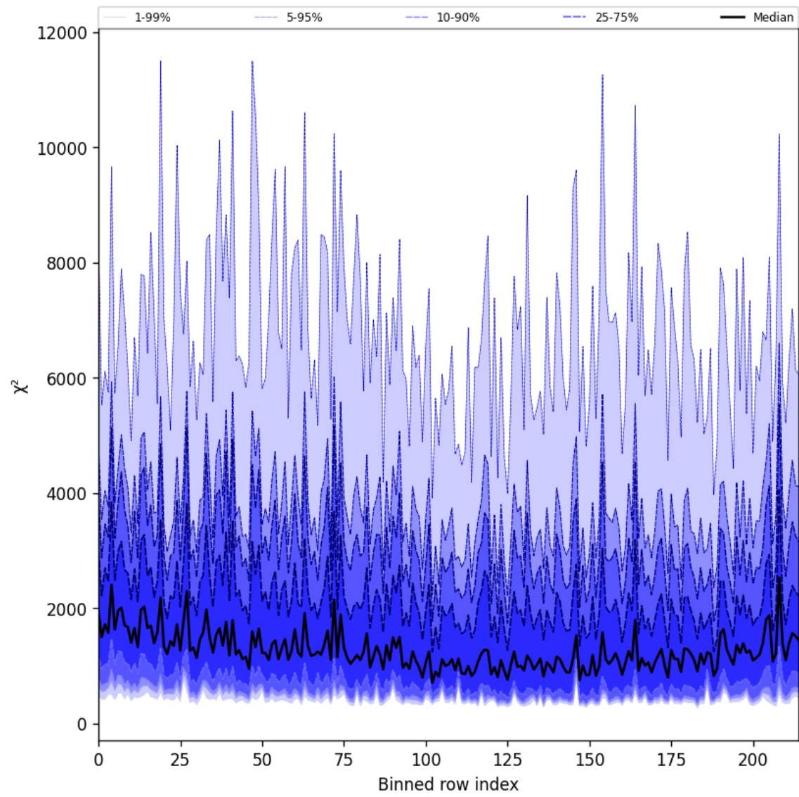
Figure 30: Along track statistics of “ \chi^2 ” for 2025-02-14 to 2025-02-16
