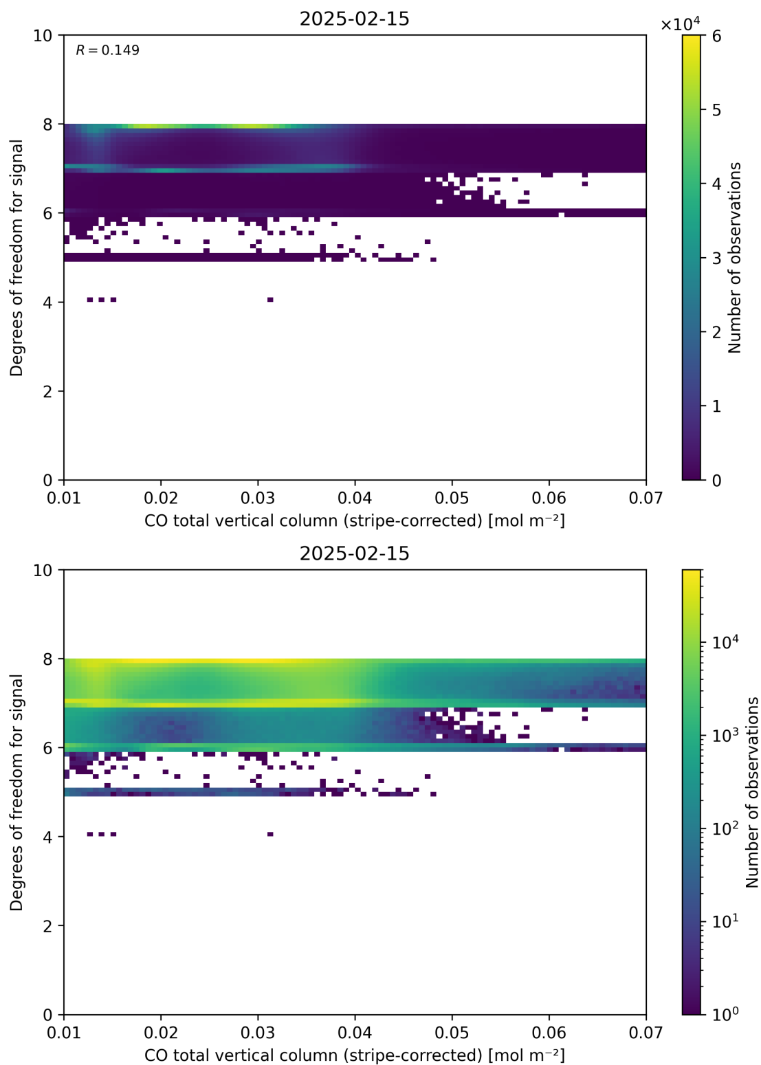
Figure 38: Scatter density plot of “CO total vertical column (stripe-corrected)” against “Degrees of freedom for signal” for 2025-02-14 to 2025-02-16.
