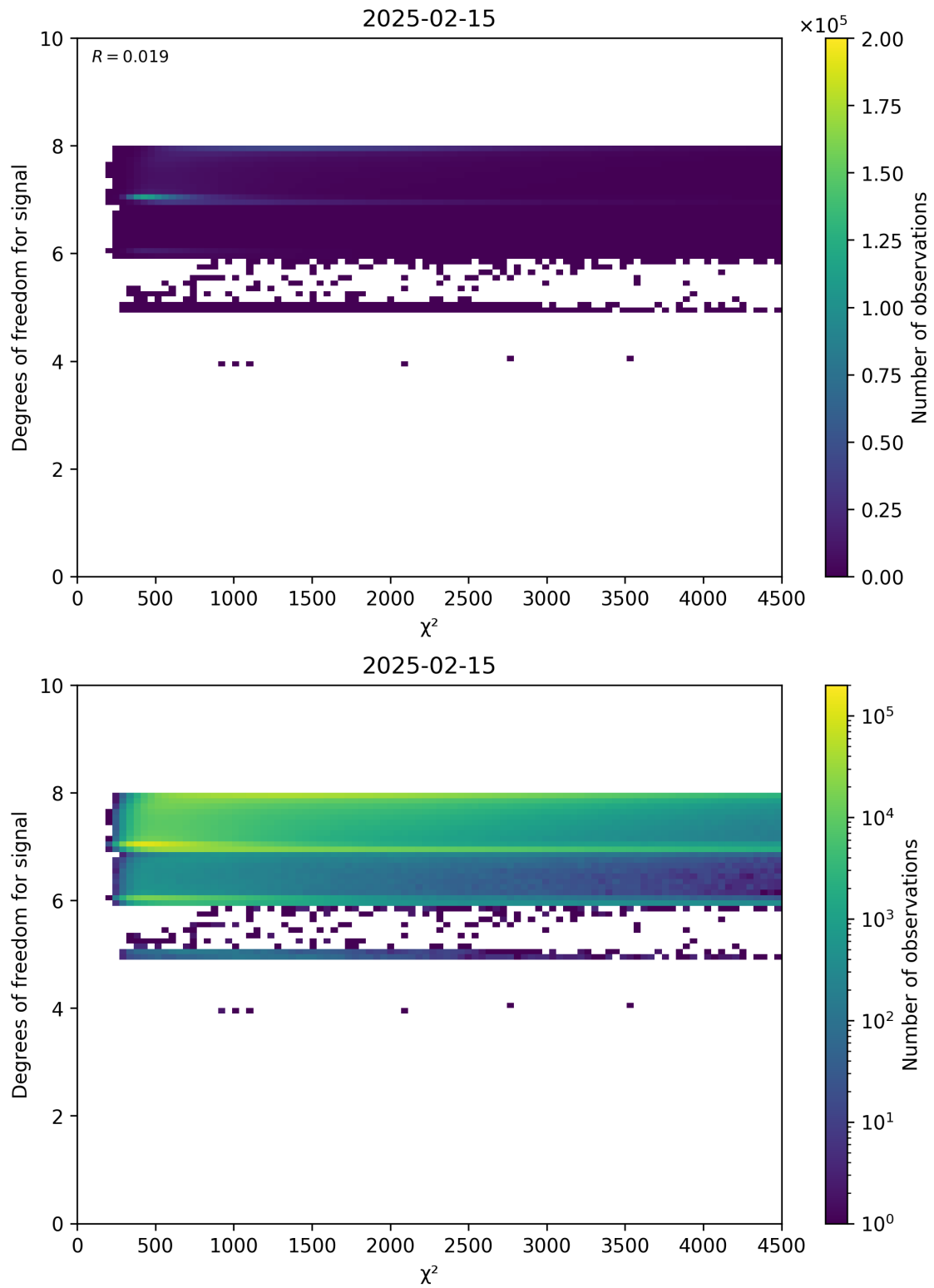
Figure 48: Scatter density plot of “ \chi^2 ” against “Degrees of freedom for signal” for 2025-02-14 to 2025-02-16.
