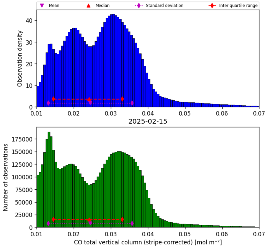
Figure 19: Histogram of “CO total vertical column (stripe-corrected)” for 2025-02-14 to 2025-02-16
