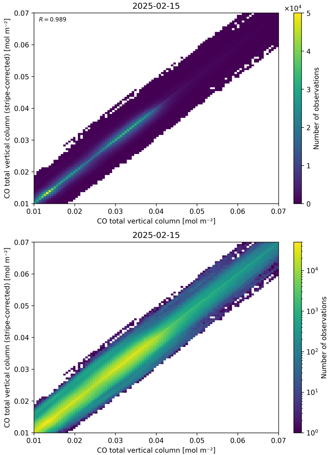
Figure 33: Scatter density plot of “CO total vertical column” against “CO total vertical column (stripe-corrected)” for 2025-02-14 to 2025-02-16.
