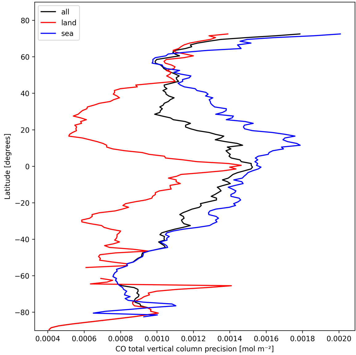
Figure 12: Zonal average of “CO total vertical column precision” for 2025-02-14 to 2025-02-16.
