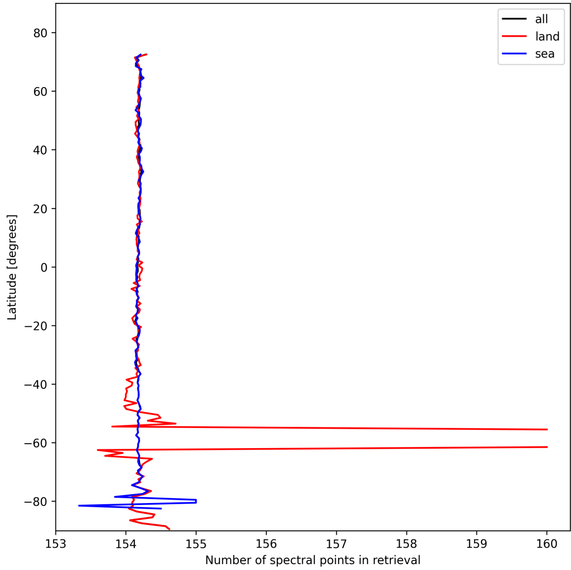
Figure 13: Zonal average of “Number of spectral points in retrieval” for 2025-02-14 to 2025-02-16.
