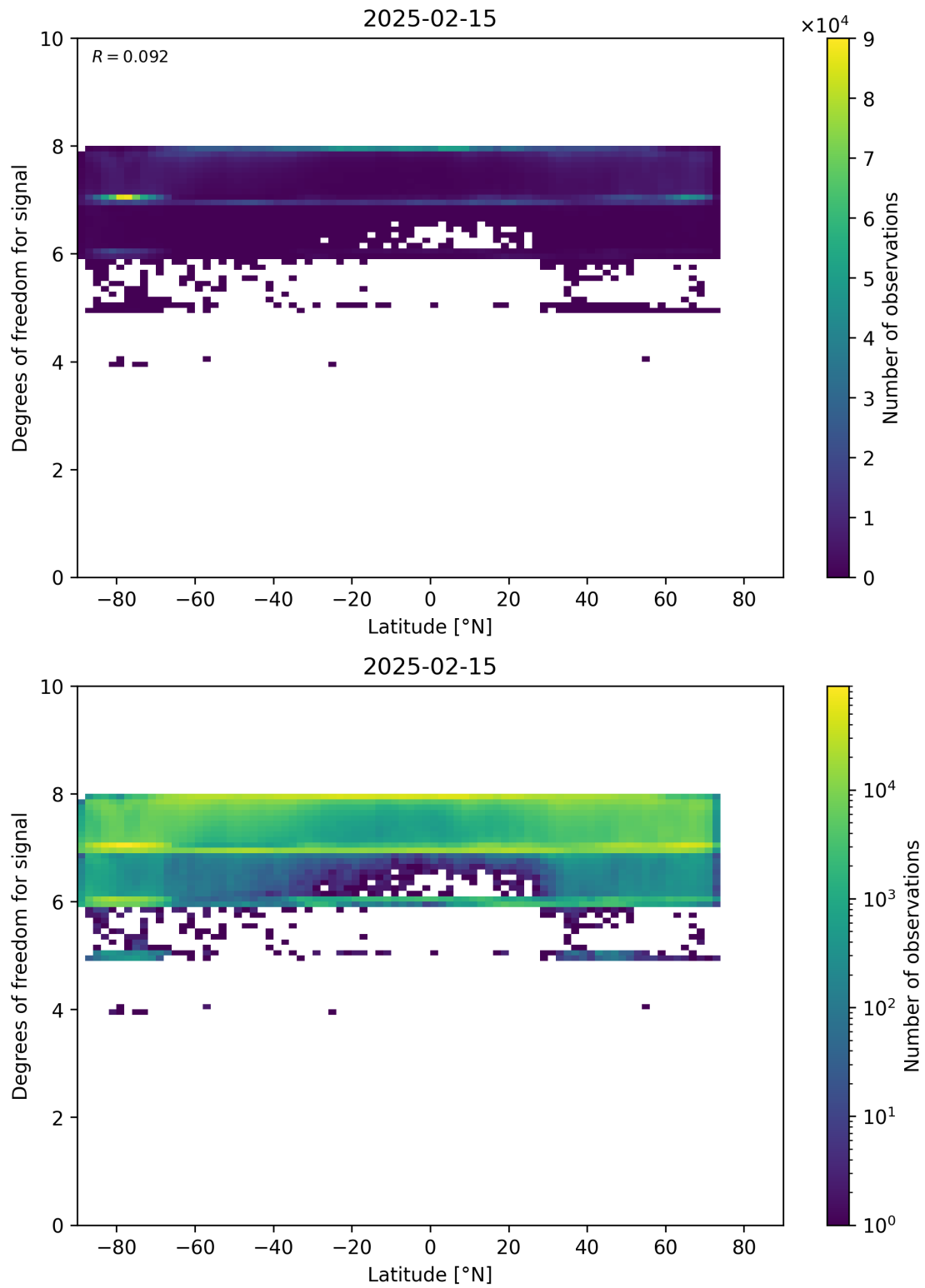
Figure 55: Scatter density plot of “Latitude” against “Degrees of freedom for signal” for 2025-02-14 to 2025-02-16.
