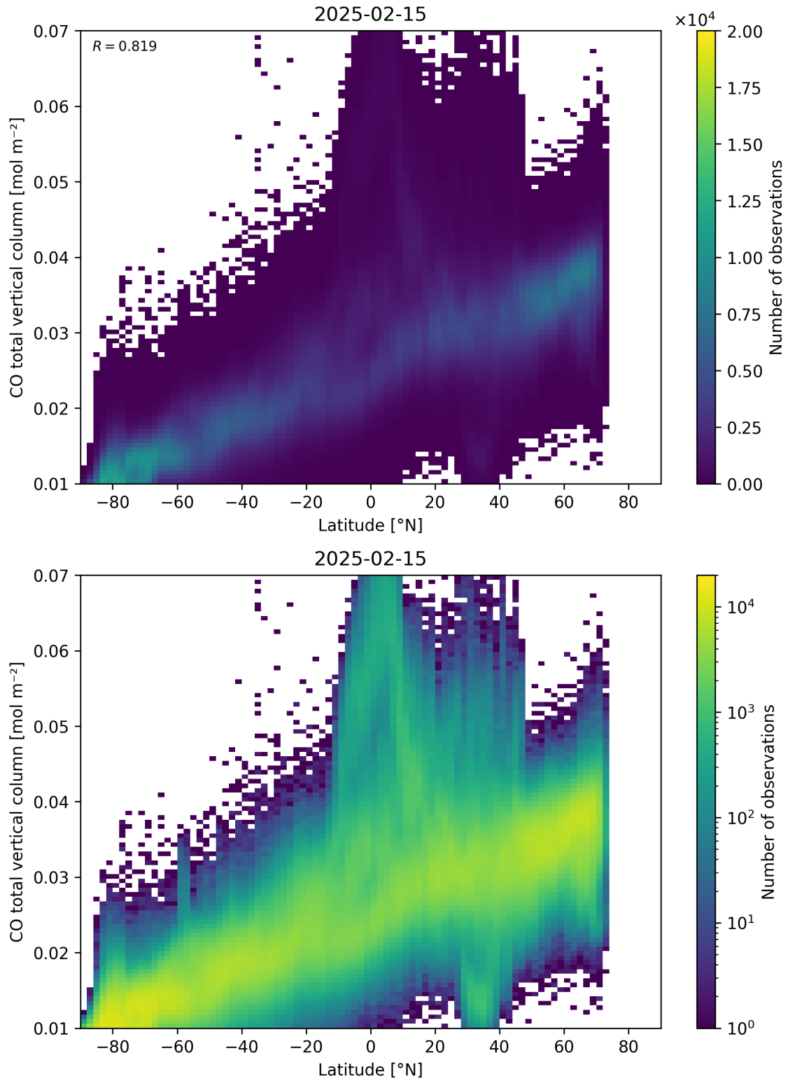
Figure 51: Scatter density plot of “Latitude” against “CO total vertical column” for 2025-02-14 to 2025-02-16.
