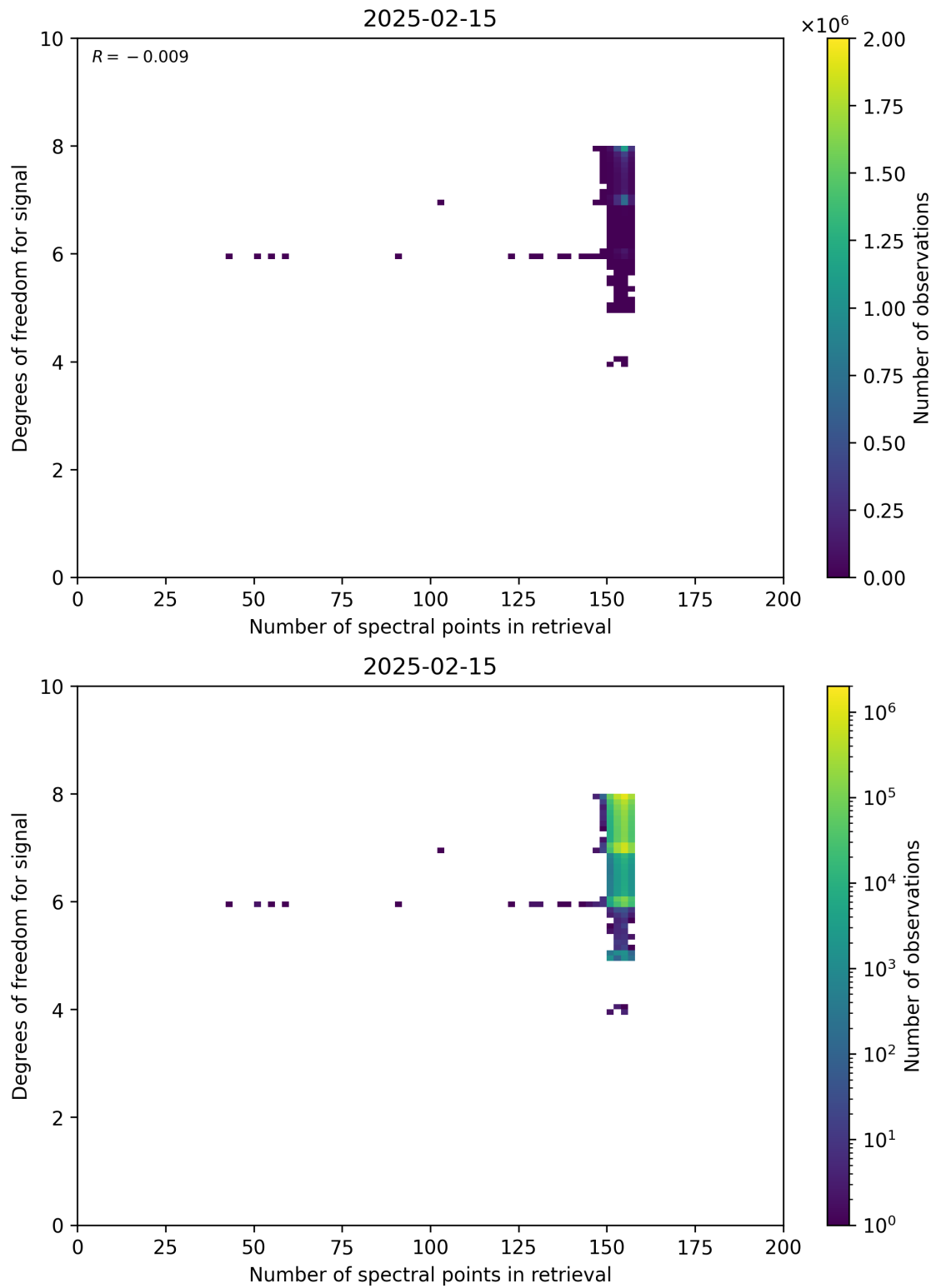
Figure 59: Scatter density plot of “Number of spectral points in retrieval” against “Degrees of freedom for signal” for 2025-02-14 to 2025-02-16.
