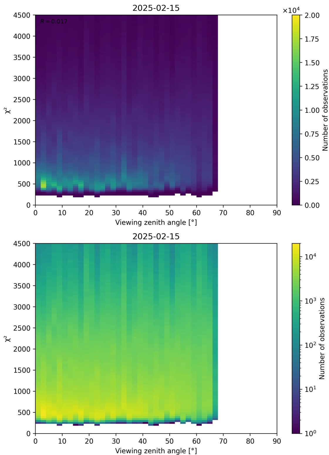
Figure 72: Scatter density plot of “Viewing zenith angle” against “ \chi^2 ” for 2025-02-14 to 2025-02-16.
