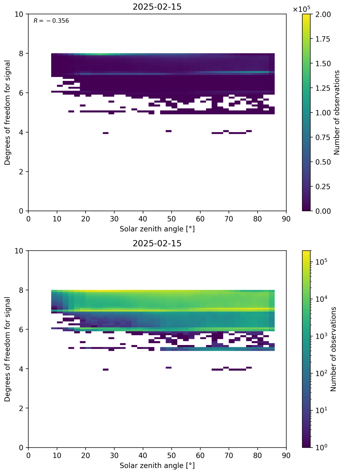
Figure 65: Scatter density plot of “Solar zenith angle” against “Degrees of freedom for signal” for 2025-02-14 to 2025-02-16.
