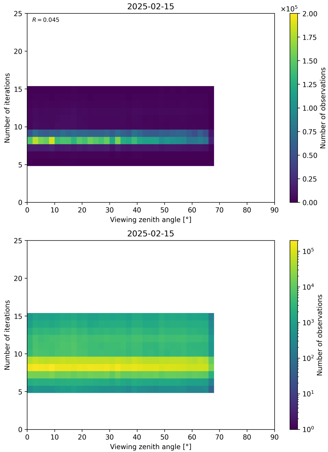
Figure 75: Scatter density plot of “Viewing zenith angle” against “Number of iterations” for 2025-02-14 to 2025-02-16.
