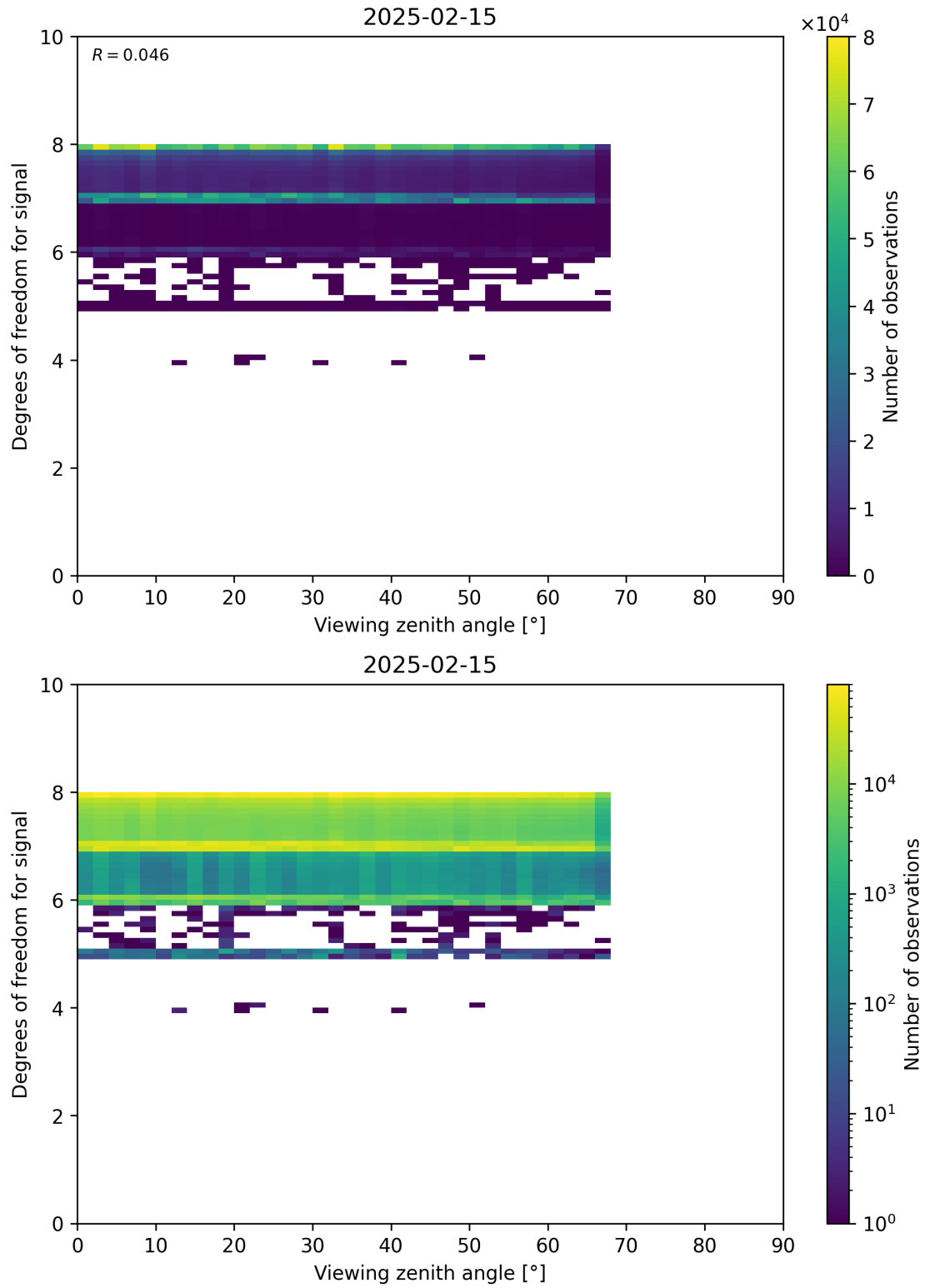
Figure 73: Scatter density plot of “Viewing zenith angle” against “Degrees of freedom for signal” for 2025-02-14 to 2025-02-16.
