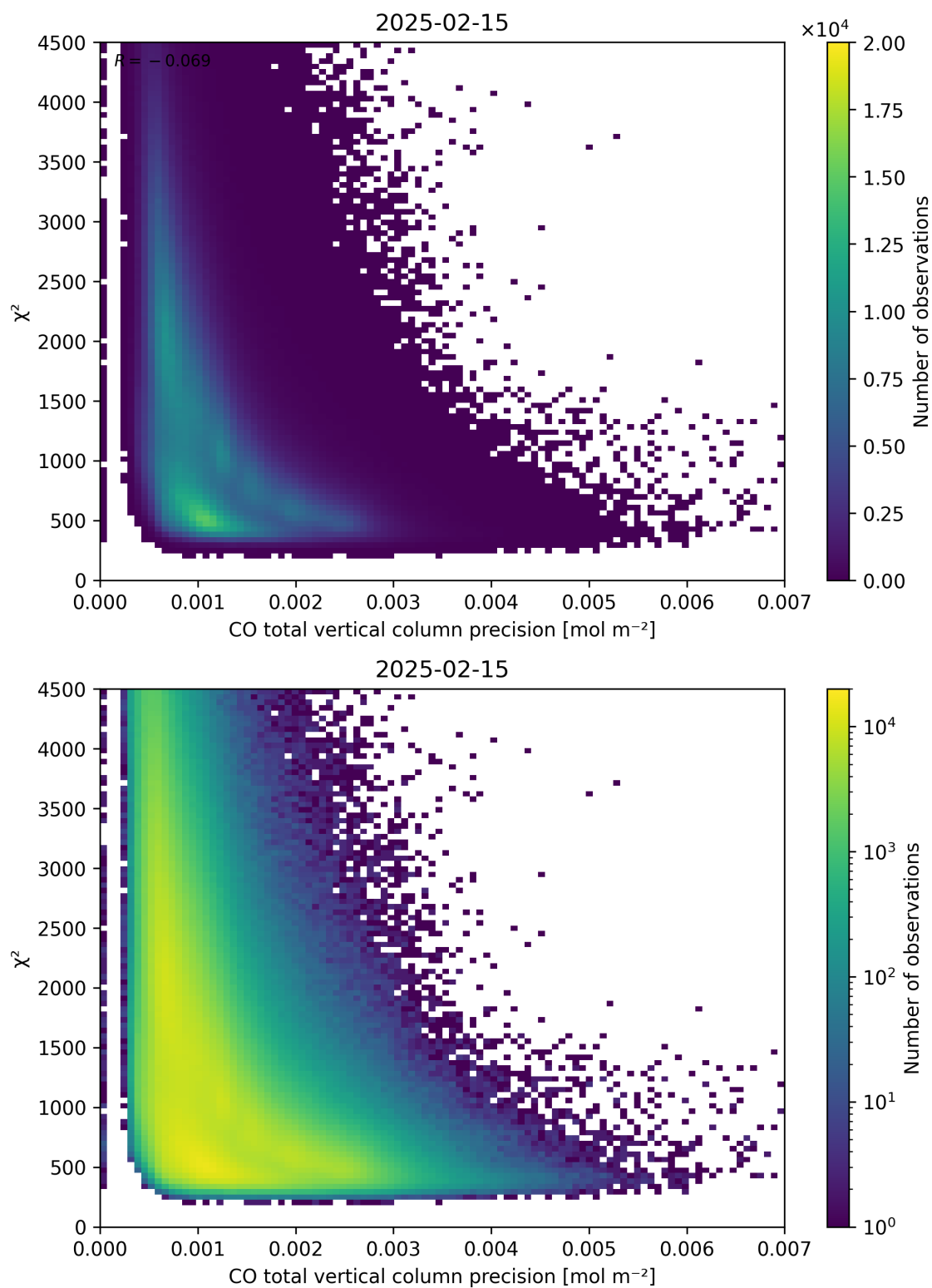
Figure 44: Scatter density plot of “CO total vertical column precision” against “ \chi^2 ” for 2025-02-14 to 2025-02-16.
