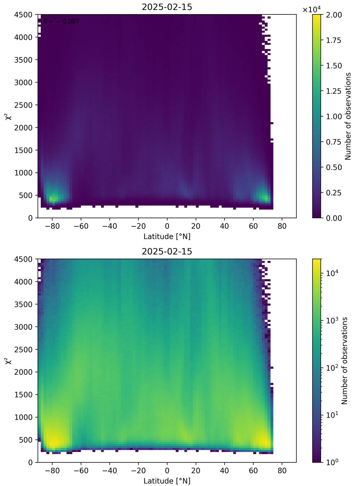
Figure 54: Scatter density plot of “Latitude” against “ \chi^2 ” for 2025-02-14 to 2025-02-16.
