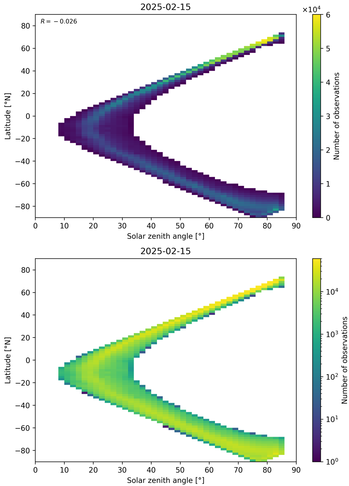
Figure 66: Scatter density plot of “Solar zenith angle” against “Latitude” for 2025-02-14 to 2025-02-16.
