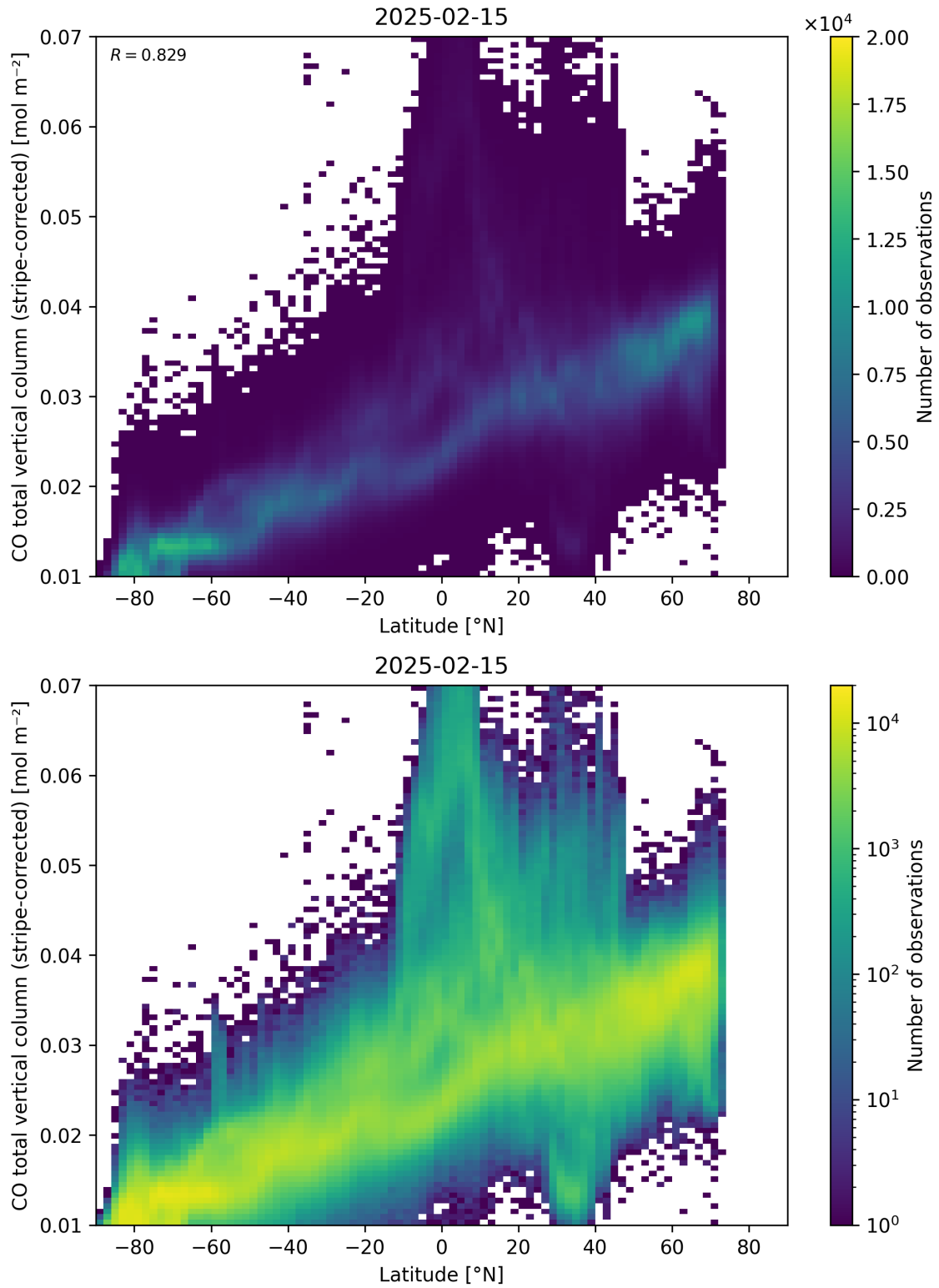
Figure 52: Scatter density plot of “Latitude” against “CO total vertical column (stripe-corrected)” for 2025-02-14 to 2025-02-16.
