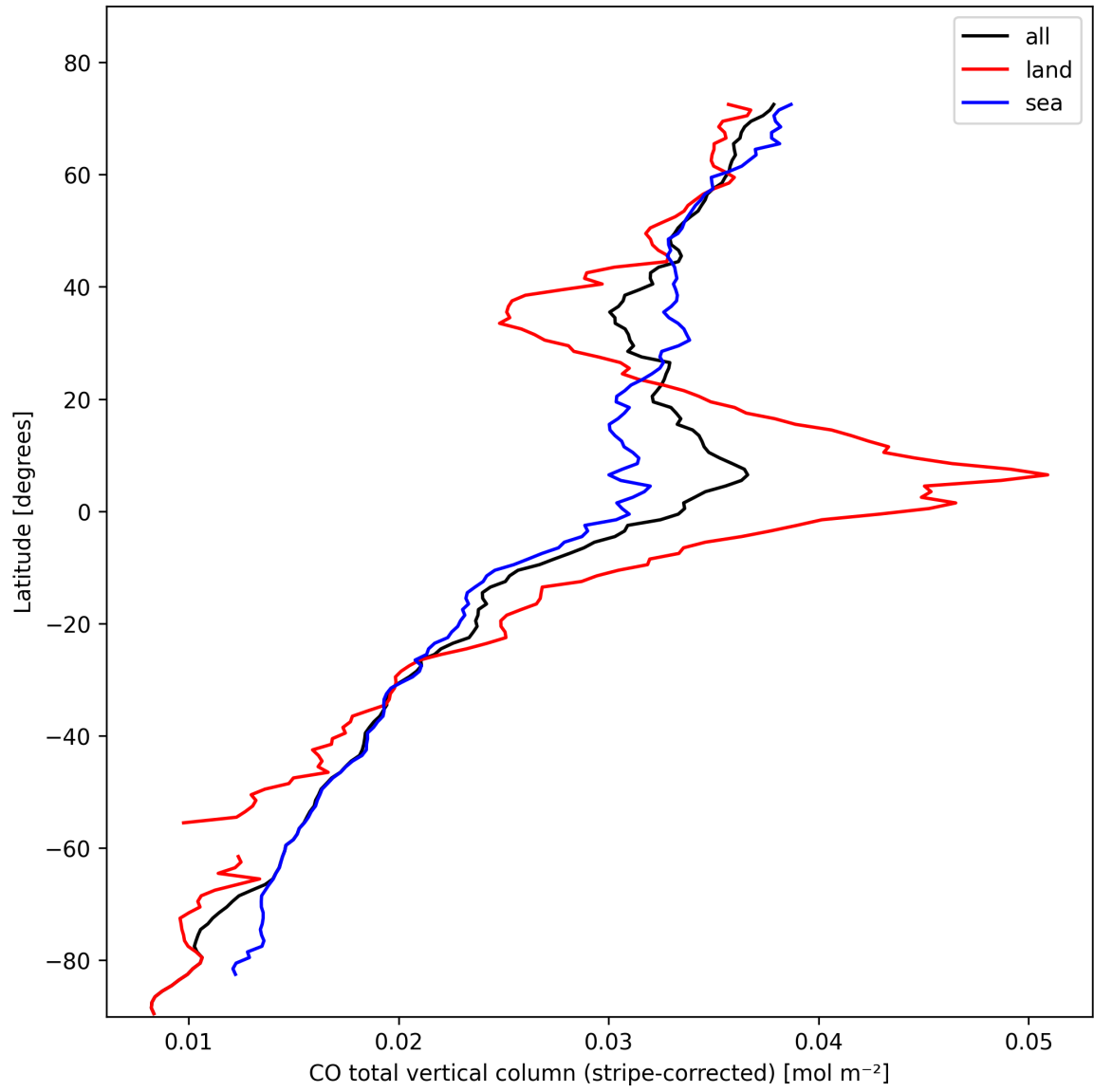
Figure 11: Zonal average of “CO total vertical column (stripe-corrected)” for 2025-02-14 to 2025-02-16.
