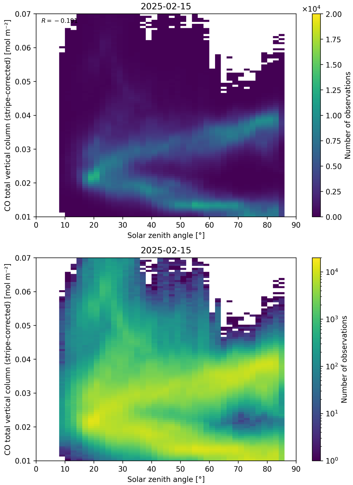
Figure 62: Scatter density plot of “Solar zenith angle” against “CO total vertical column (stripe-corrected)” for 2025-02-14 to 2025-02-16.
