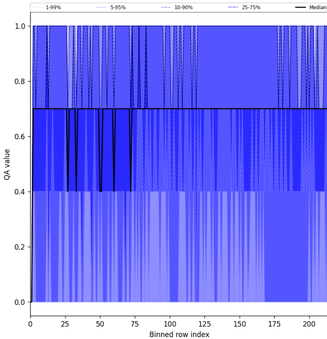
Figure 25: Along track statistics of “QA value” for 2025-02-14 to 2025-02-16
