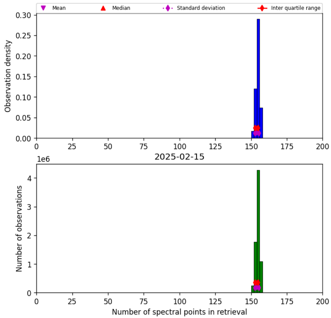
Figure 21: Histogram of “Number of spectral points in retrieval” for 2025-02-14 to 2025-02-16
