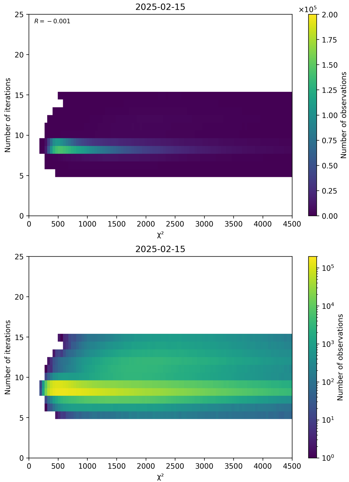
Figure 49: Scatter density plot of “ \chi^2 ” against “Number of iterations” for 2025-02-14 to 2025-02-16.
