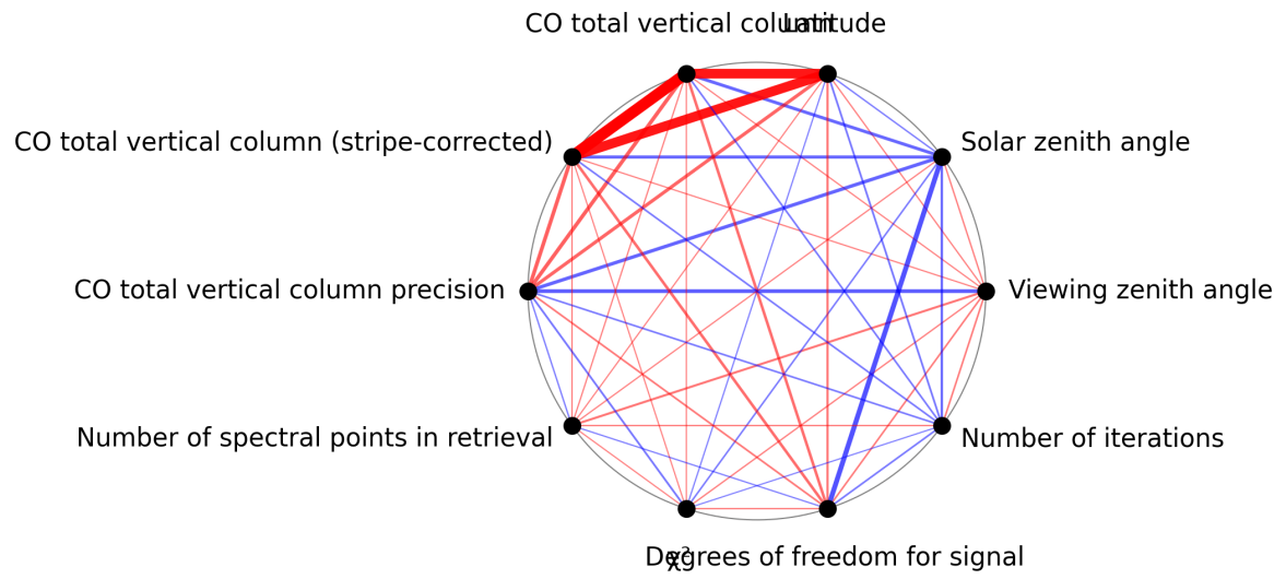
Figure 1: Map of correlation graph for 2025-02-14 to 2025-02-16.
