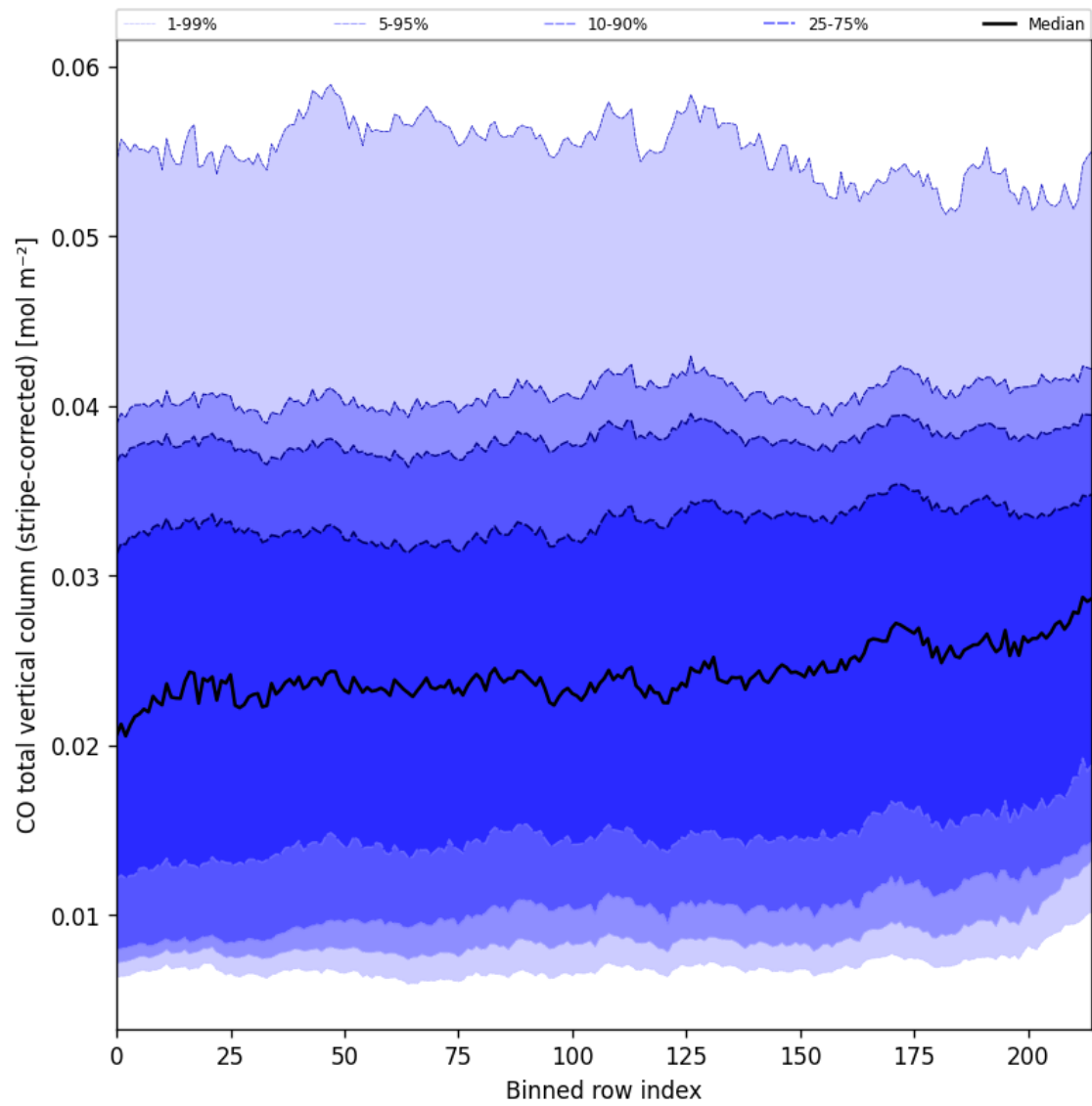
Figure 27: Along track statistics of “CO total vertical column (stripe-corrected)” for 2025-02-14 to 2025-02-16
