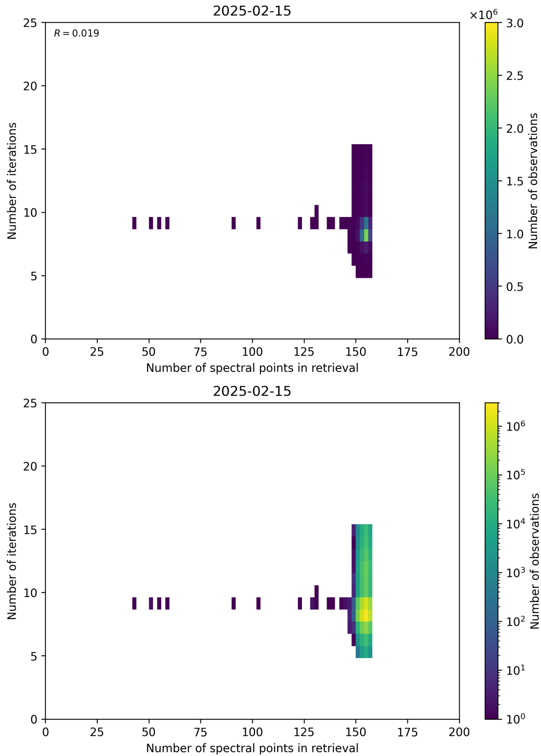
Figure 60: Scatter density plot of “Number of spectral points in retrieval” against “Number of iterations” for 2025-02-14 to 2025-02-16.
