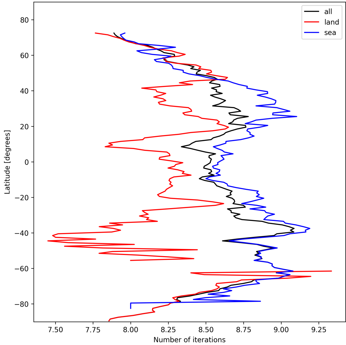
Figure 16: Zonal average of “Number of iterations” for 2025-02-14 to 2025-02-16.
