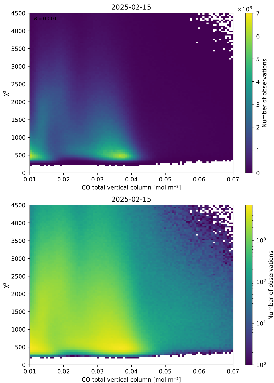
Figure 35: Scatter density plot of “CO total vertical column” against “ \chi^2 ” for 2025-02-14 to 2025-02-16.
