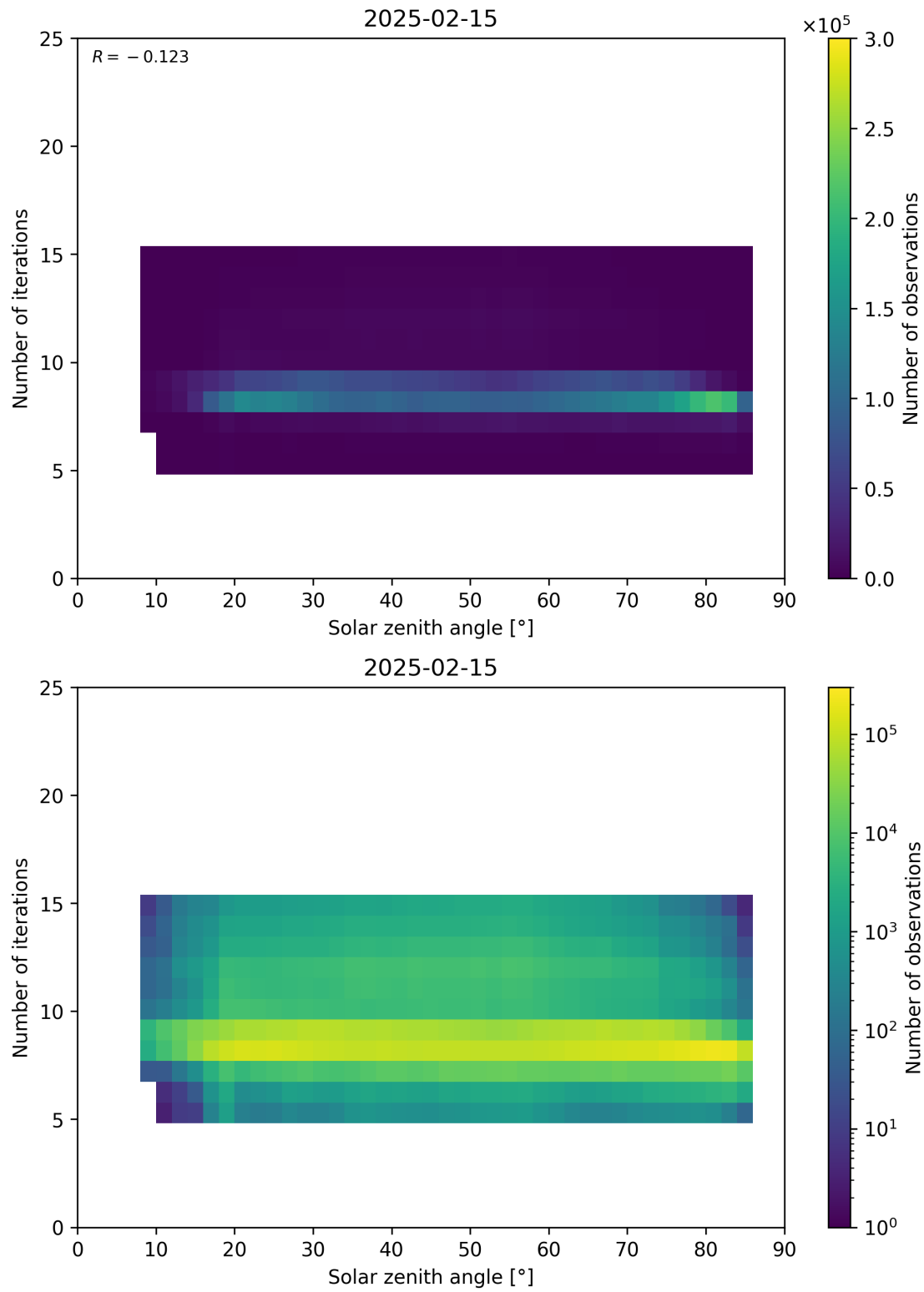
Figure 67: Scatter density plot of “Solar zenith angle” against “Number of iterations” for 2025-02-14 to 2025-02-16.
