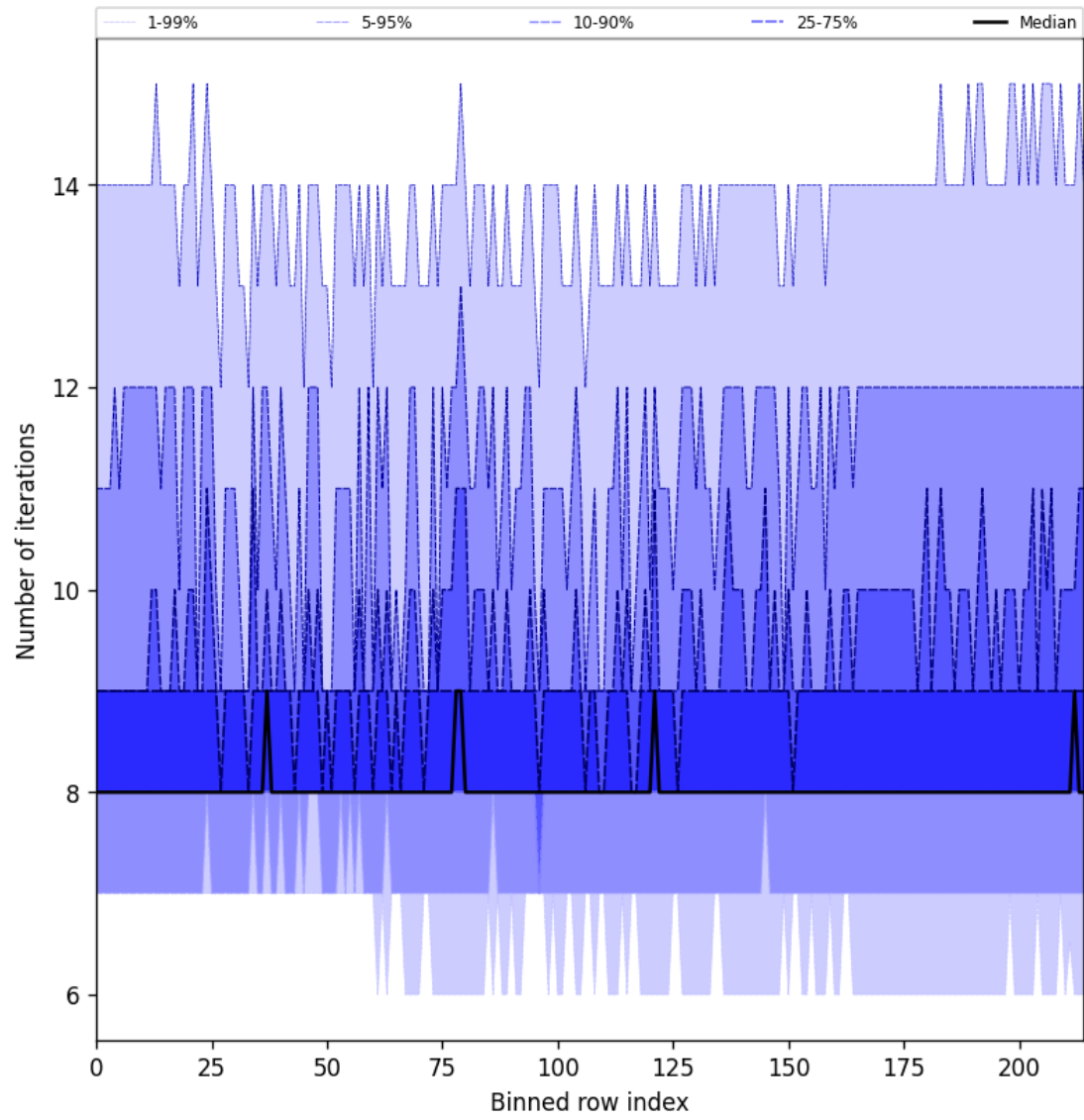
Figure 32: Along track statistics of “Number of iterations” for 2025-02-14 to 2025-02-16
