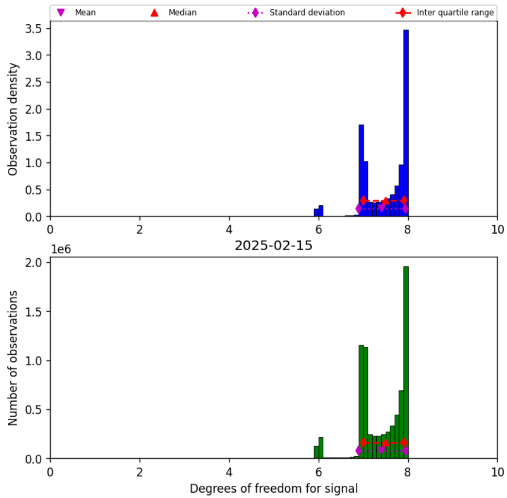
Figure 23: Histogram of “Degrees of freedom for signal” for 2025-02-14 to 2025-02-16
