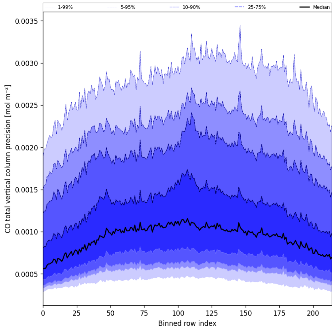
Figure 28: Along track statistics of “CO total vertical column precision” for 2025-02-14 to 2025-02-16
