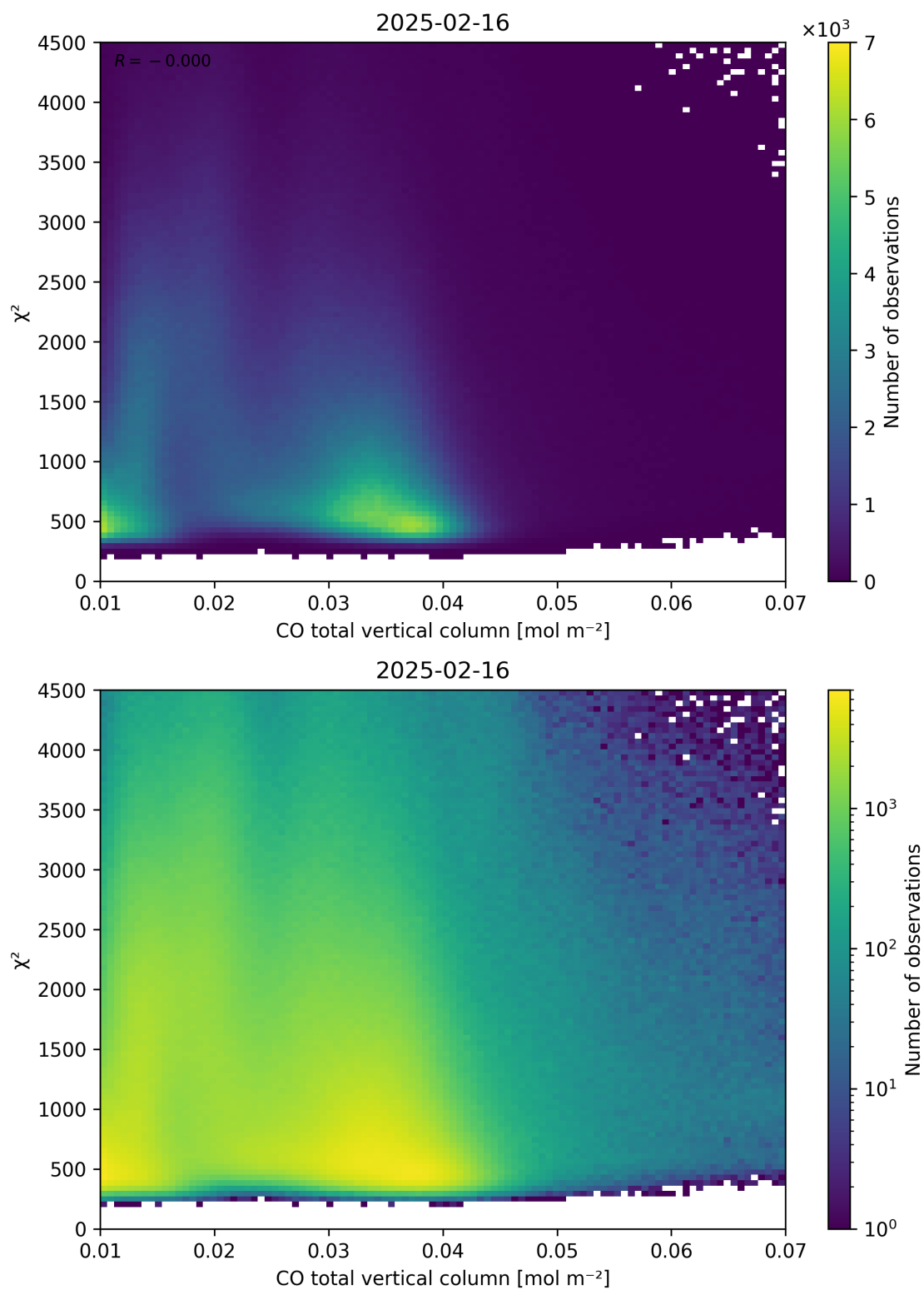
Figure 35: Scatter density plot of “CO total vertical column” against “ \chi^2 ” for 2025-02-15 to 2025-02-17.
