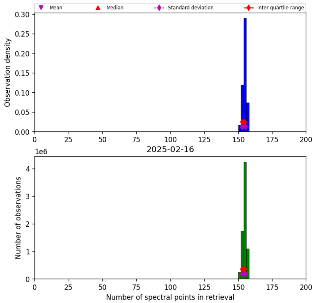
Figure 21: Histogram of “Number of spectral points in retrieval” for 2025-02-15 to 2025-02-17
