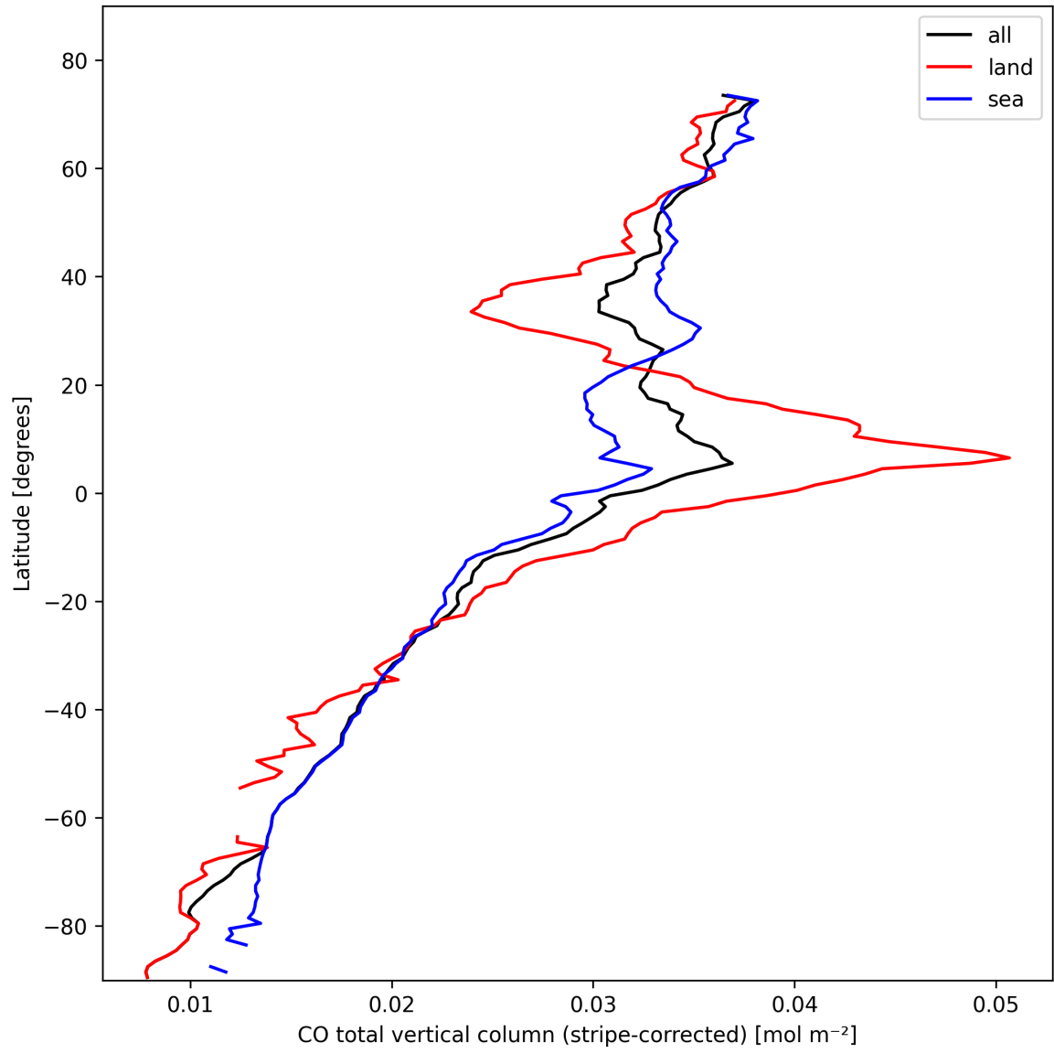
Figure 11: Zonal average of “CO total vertical column (stripe-corrected)” for 2025-02-15 to 2025-02-17.
