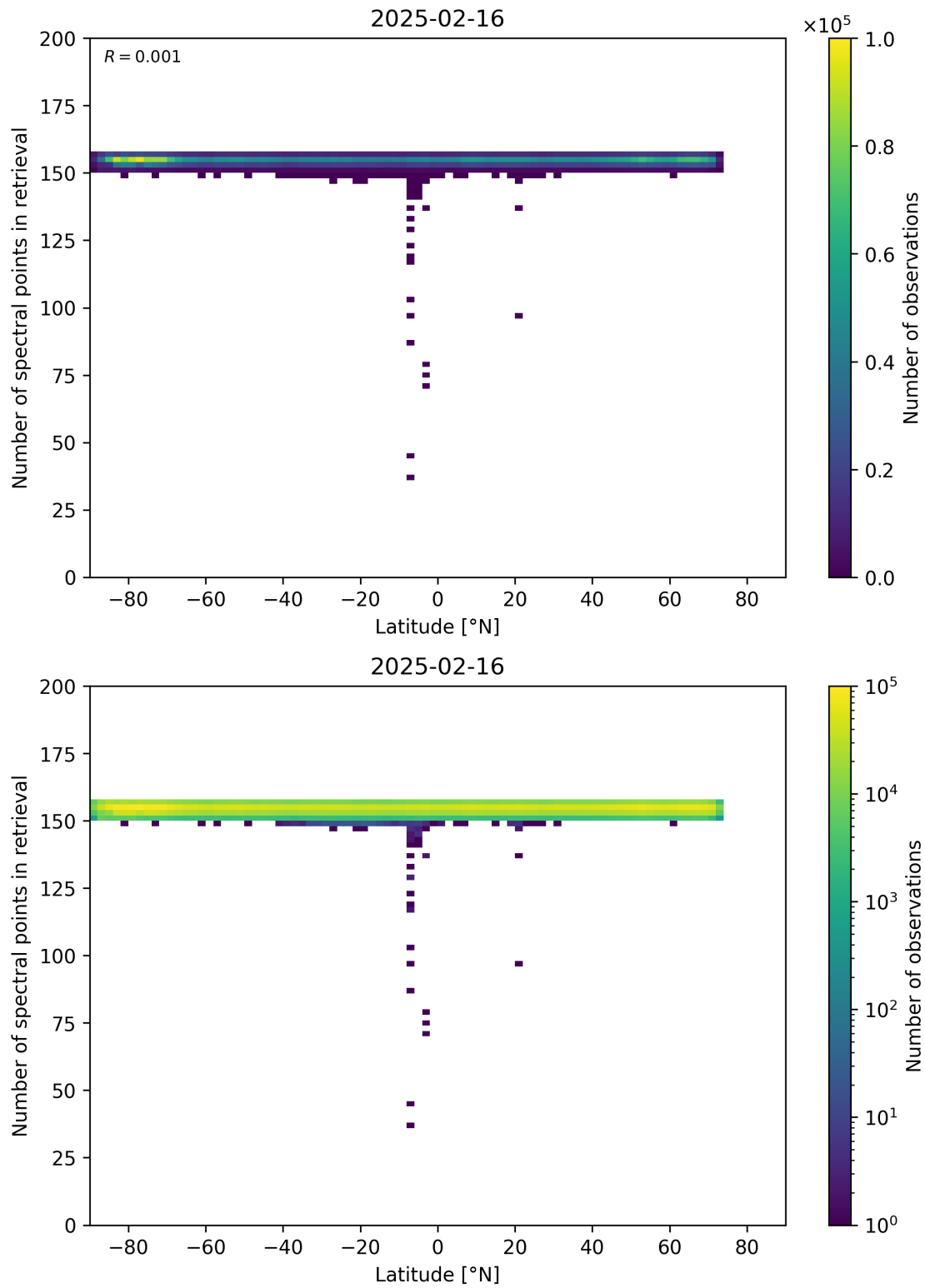
Figure 57: Scatter density plot of “Latitude” against “Number of spectral points in retrieval” for 2025-02-15 to 2025-02-17.
