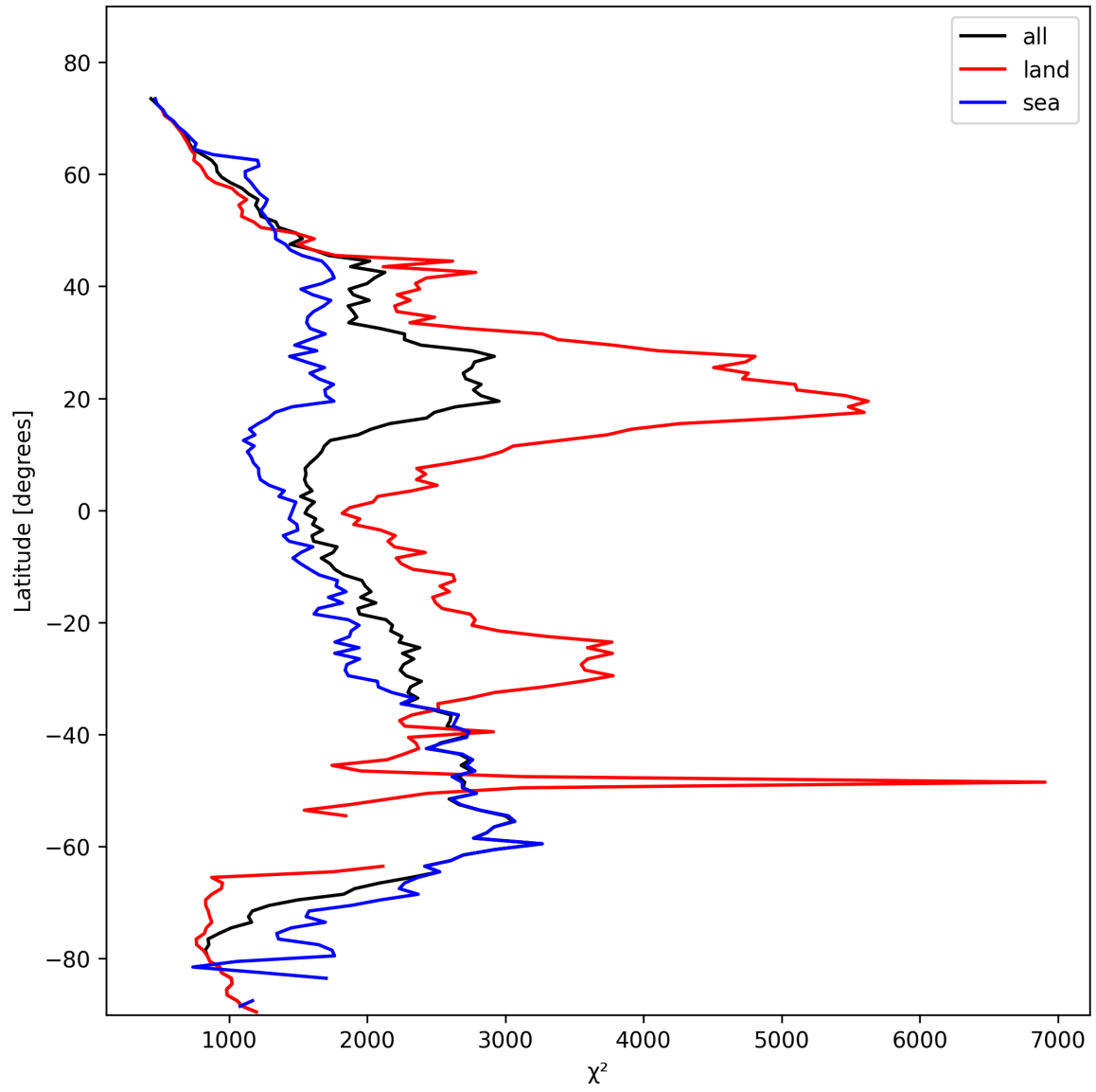
Figure 14: Zonal average of “ \chi^2 ” for 2025-02-15 to 2025-02-17.
