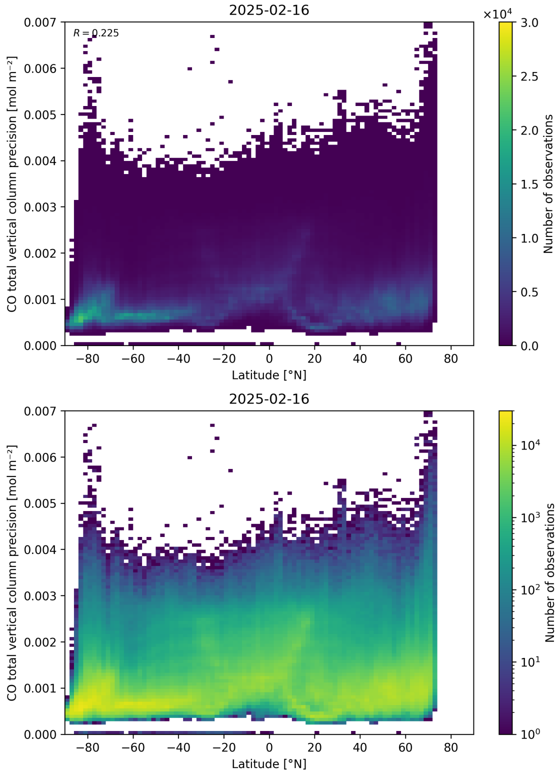
Figure 53: Scatter density plot of “Latitude” against “CO total vertical column precision” for 2025-02-15 to 2025-02-17.
