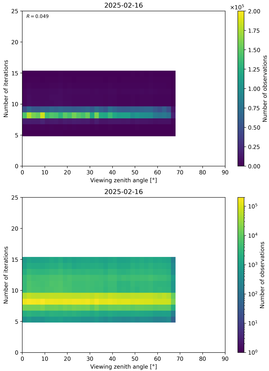
Figure 75: Scatter density plot of “Viewing zenith angle” against “Number of iterations” for 2025-02-15 to 2025-02-17.
