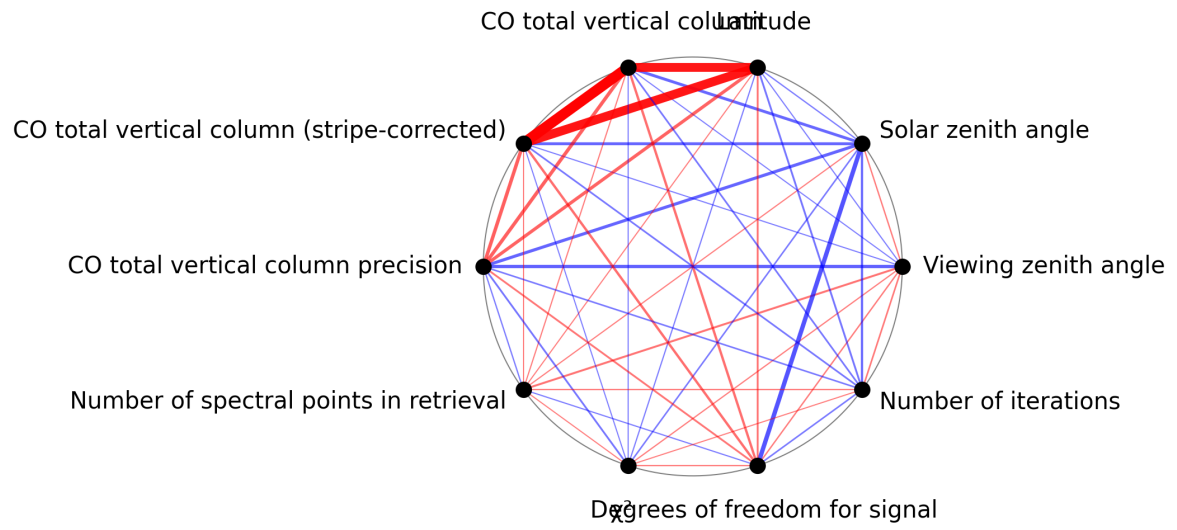
Figure 1: Map of correlation graph for 2025-02-15 to 2025-02-17.
