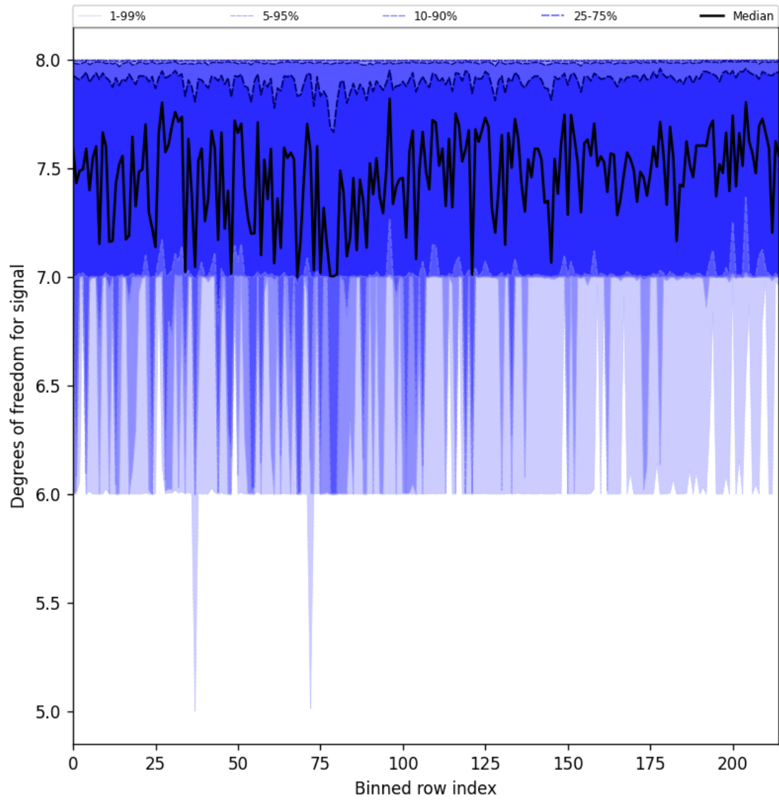
Figure 31: Along track statistics of “Degrees of freedom for signal” for 2025-02-15 to 2025-02-17
