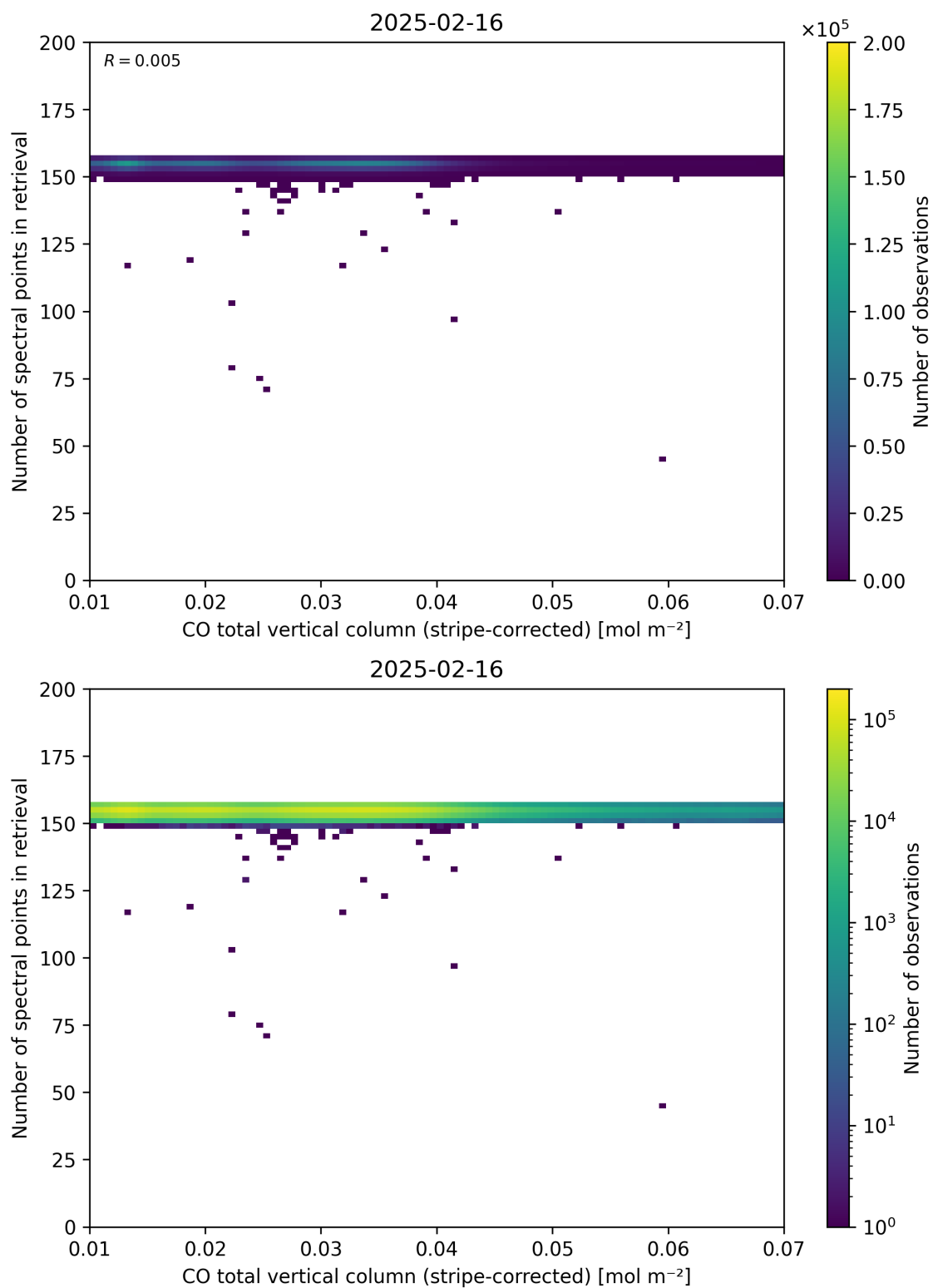
Figure 40: Scatter density plot of “CO total vertical column (stripe-corrected)” against “Number of spectral points in retrieval” for 2025-02-15 to 2025-02-17.
