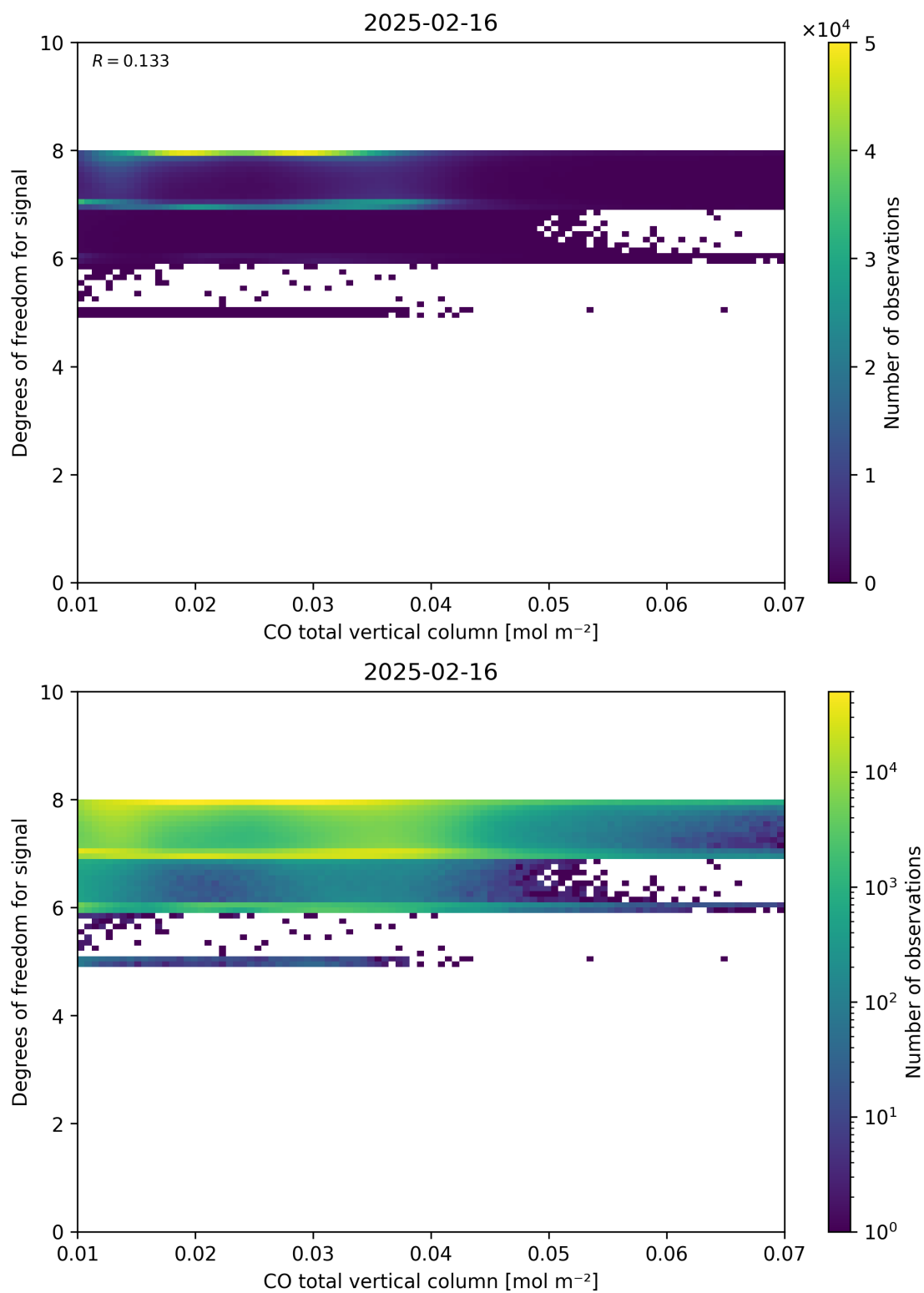
Figure 41: Scatter density plot of “CO total vertical column” against “Degrees of freedom for signal” for 2025-02-15 to 2025-02-17.
