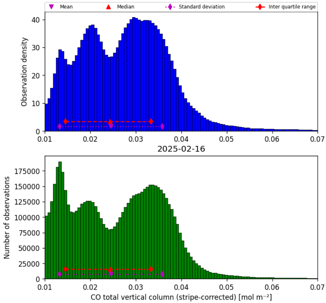
Figure 19: Histogram of “CO total vertical column (stripe-corrected)” for 2025-02-15 to 2025-02-17
