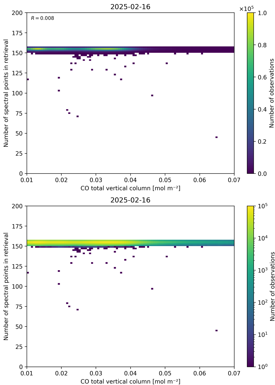
Figure 43: Scatter density plot of “CO total vertical column” against “Number of spectral points in retrieval” for 2025-02-15 to 2025-02-17.
