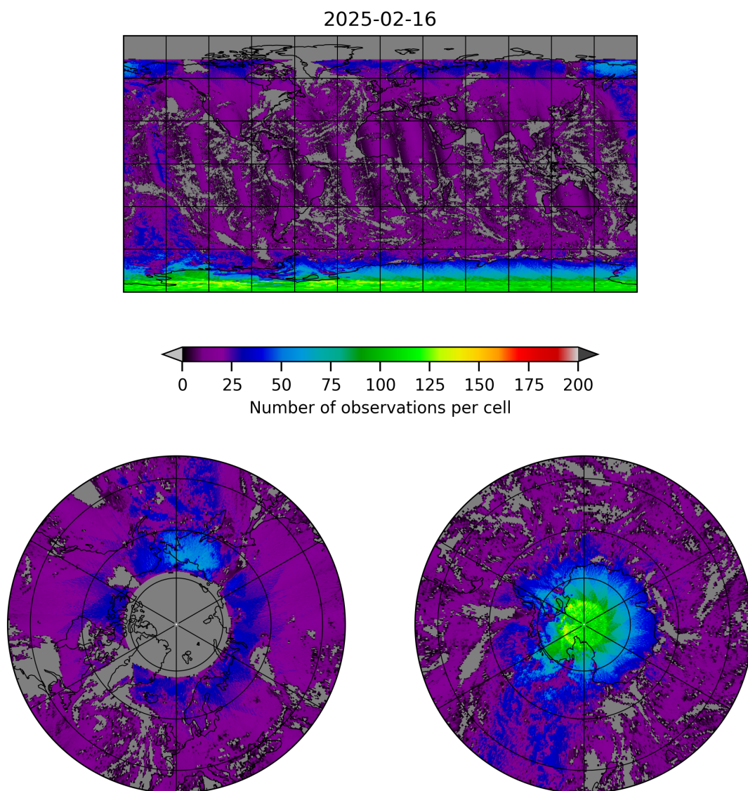
Figure 8: Map of the number of observations for 2025-02-15 to 2025-02-17
