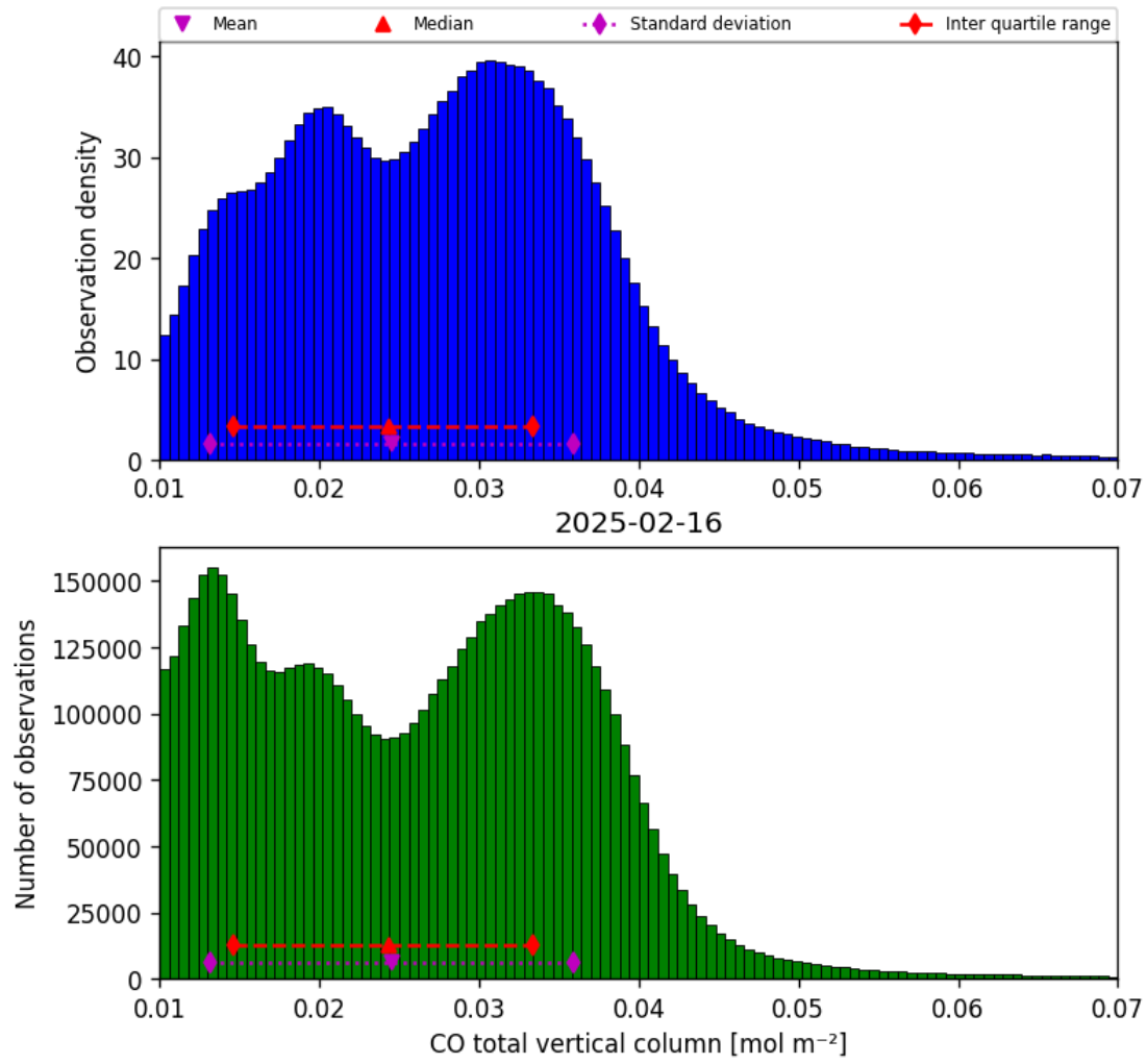
Figure 18: Histogram of “CO total vertical column” for 2025-02-15 to 2025-02-17
