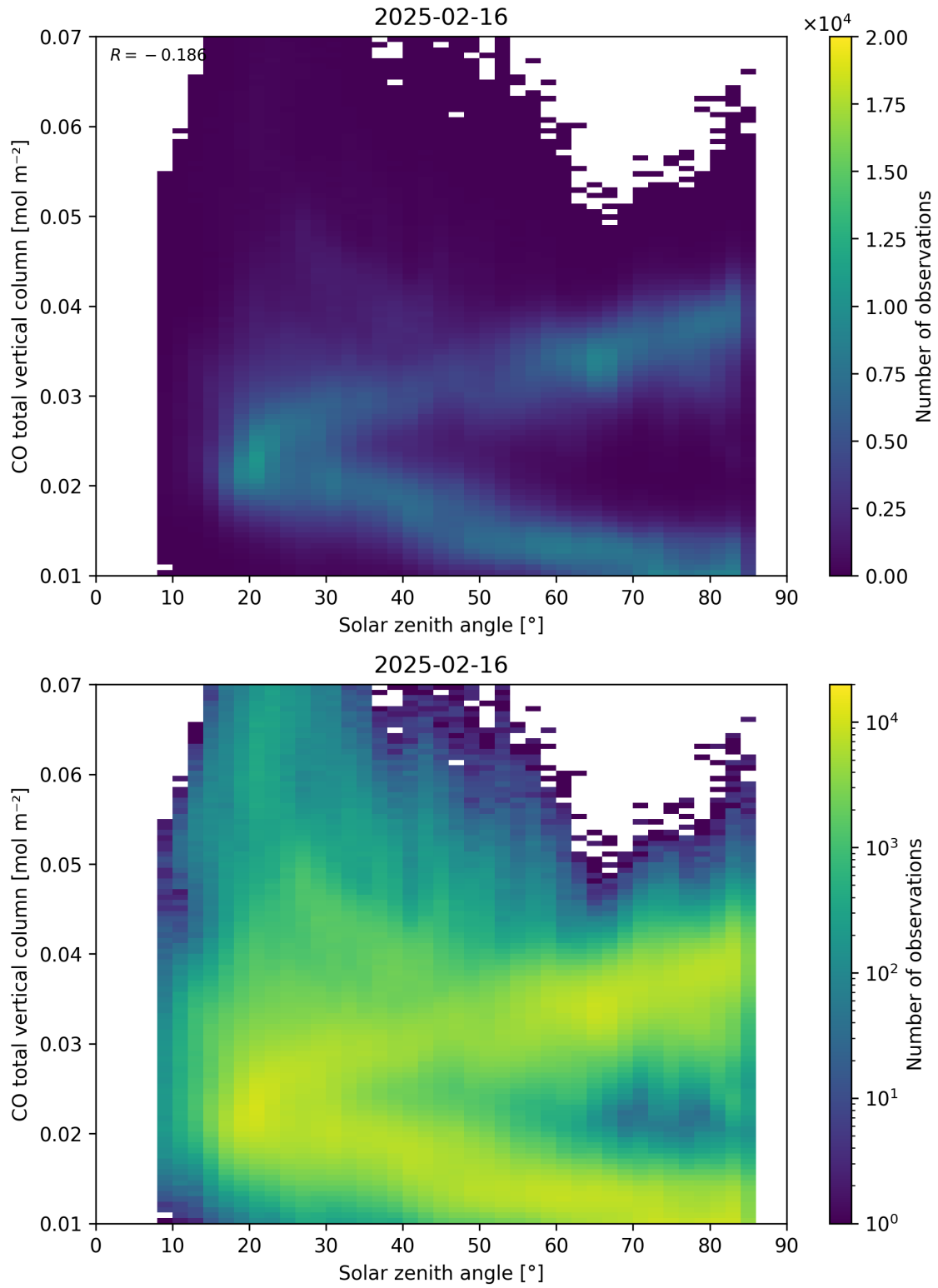
Figure 61: Scatter density plot of “Solar zenith angle” against “CO total vertical column” for 2025-02-15 to 2025-02-17.
