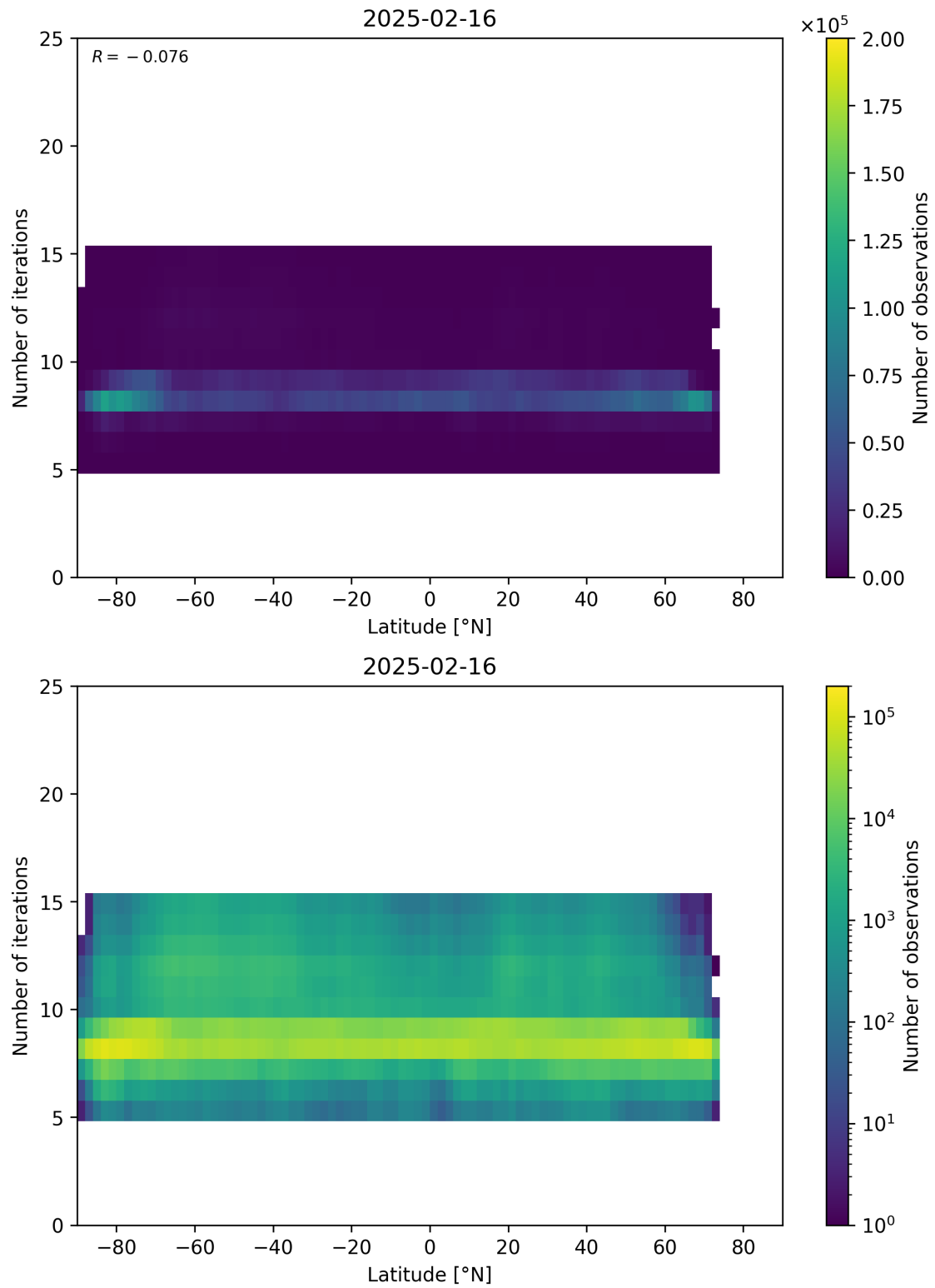
Figure 56: Scatter density plot of “Latitude” against “Number of iterations” for 2025-02-15 to 2025-02-17.
