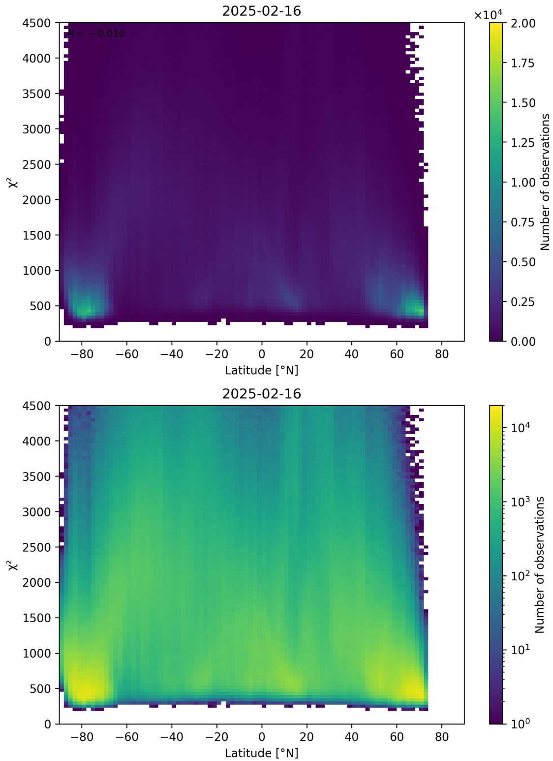
Figure 54: Scatter density plot of “Latitude” against “ \chi^2 ” for 2025-02-15 to 2025-02-17.
