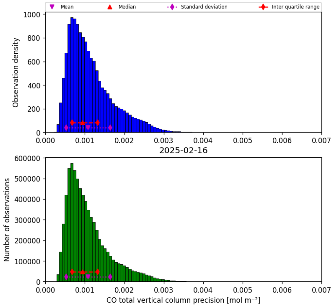
Figure 20: Histogram of “CO total vertical column precision” for 2025-02-15 to 2025-02-17
