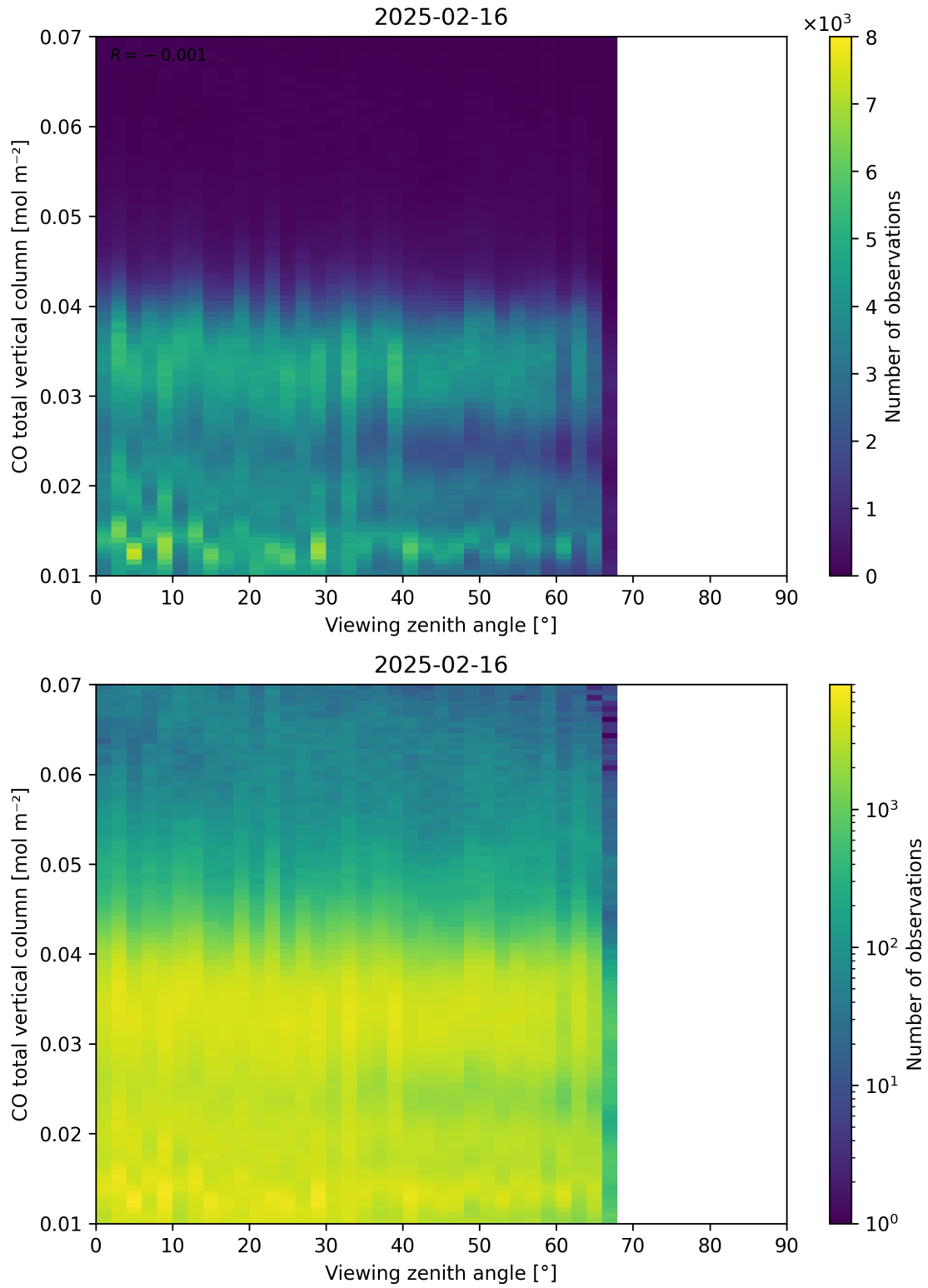
Figure 69: Scatter density plot of “Viewing zenith angle” against “CO total vertical column” for 2025-02-15 to 2025-02-17.
