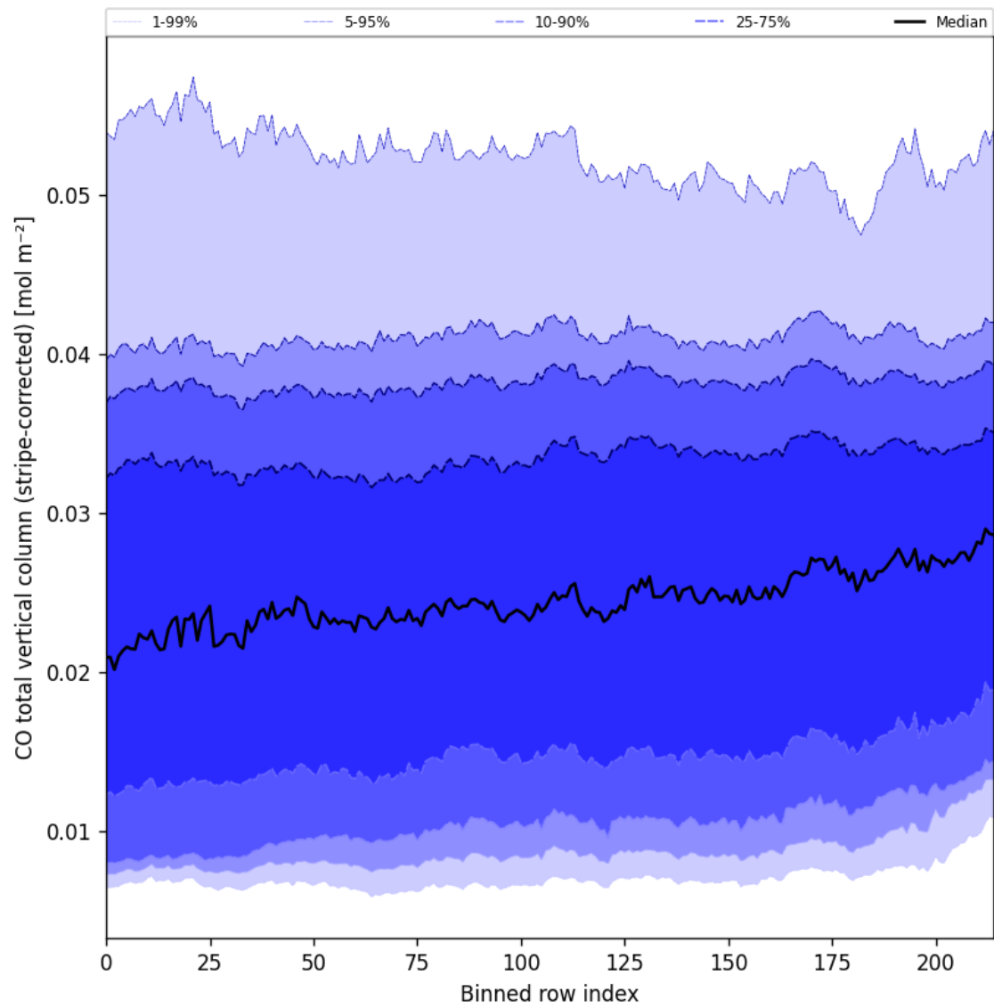
Figure 27: Along track statistics of “CO total vertical column (stripe-corrected)” for 2025-02-15 to 2025-02-17
