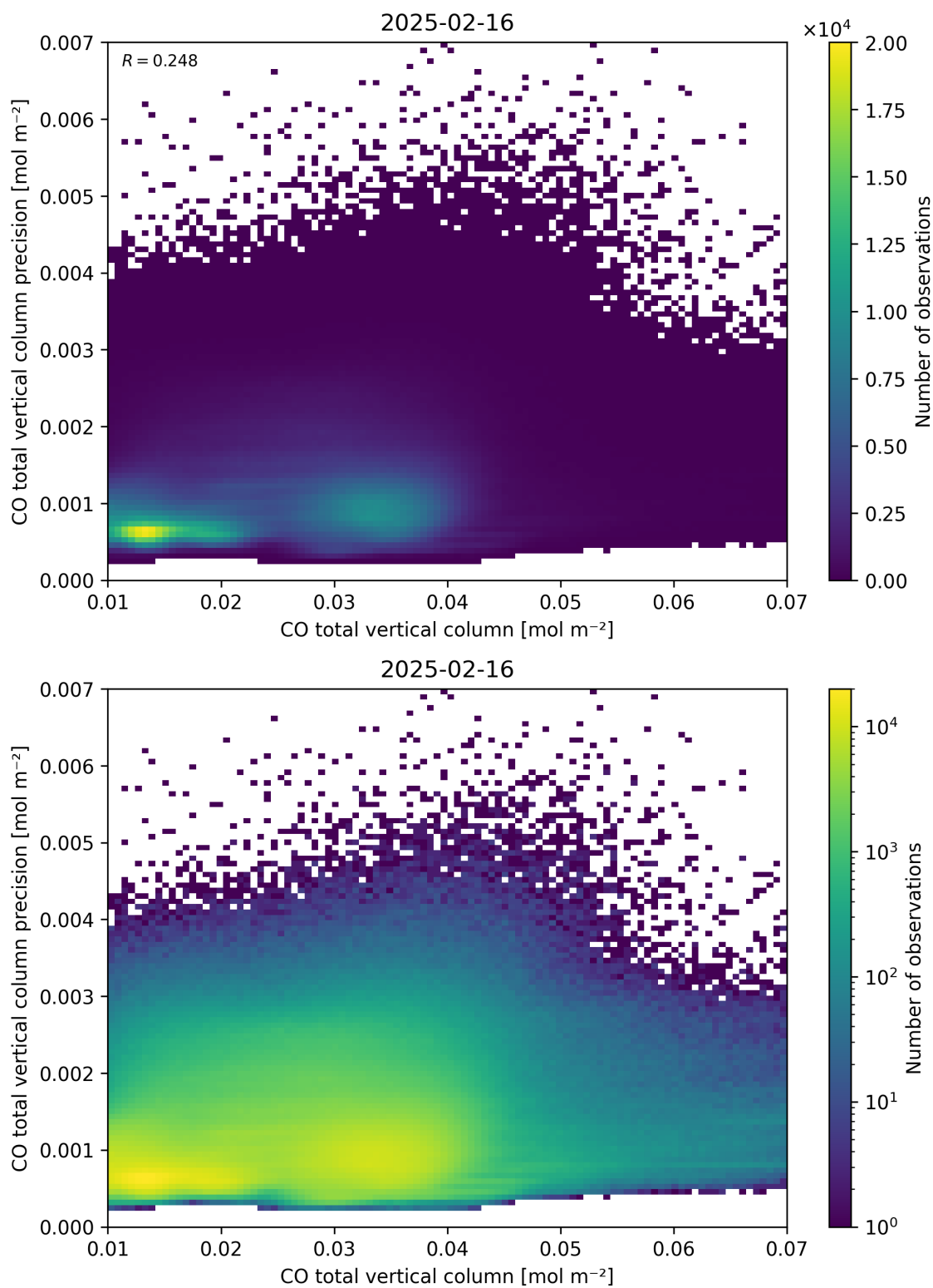
Figure 34: Scatter density plot of “CO total vertical column” against “CO total vertical column precision” for 2025-02-15 to 2025-02-17.
