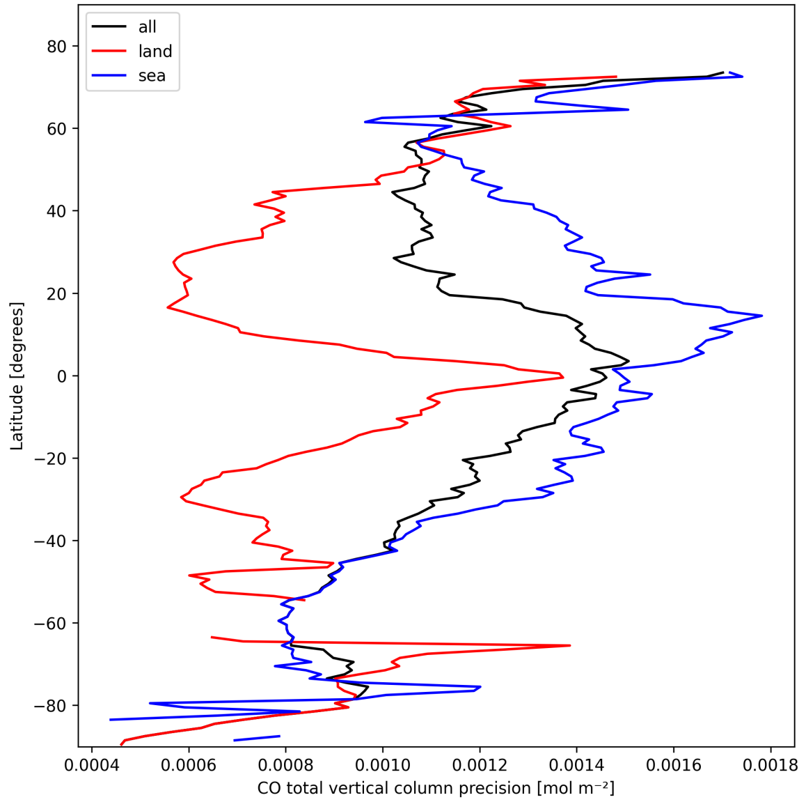
Figure 12: Zonal average of “CO total vertical column precision” for 2025-02-15 to 2025-02-17.
