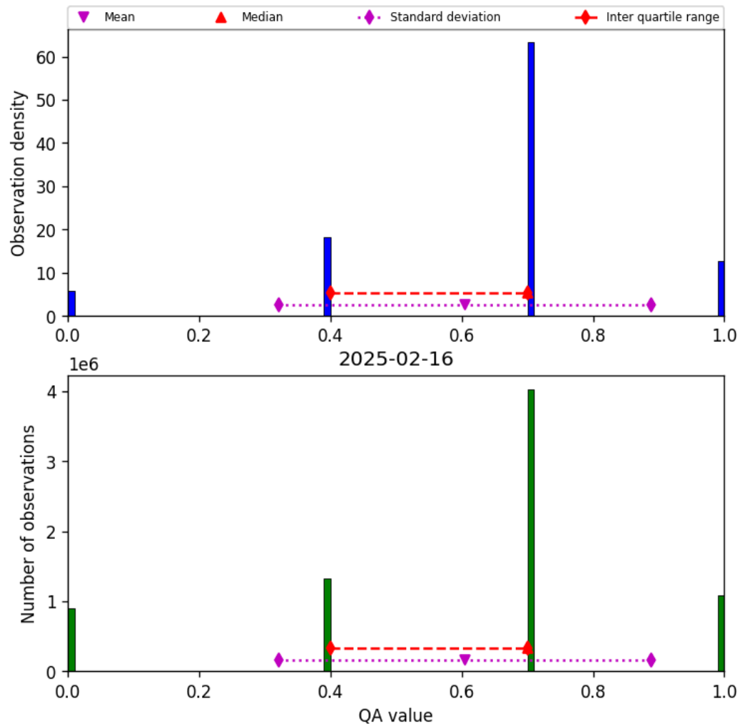
Figure 17: Histogram of “QA value” for 2025-02-15 to 2025-02-17
