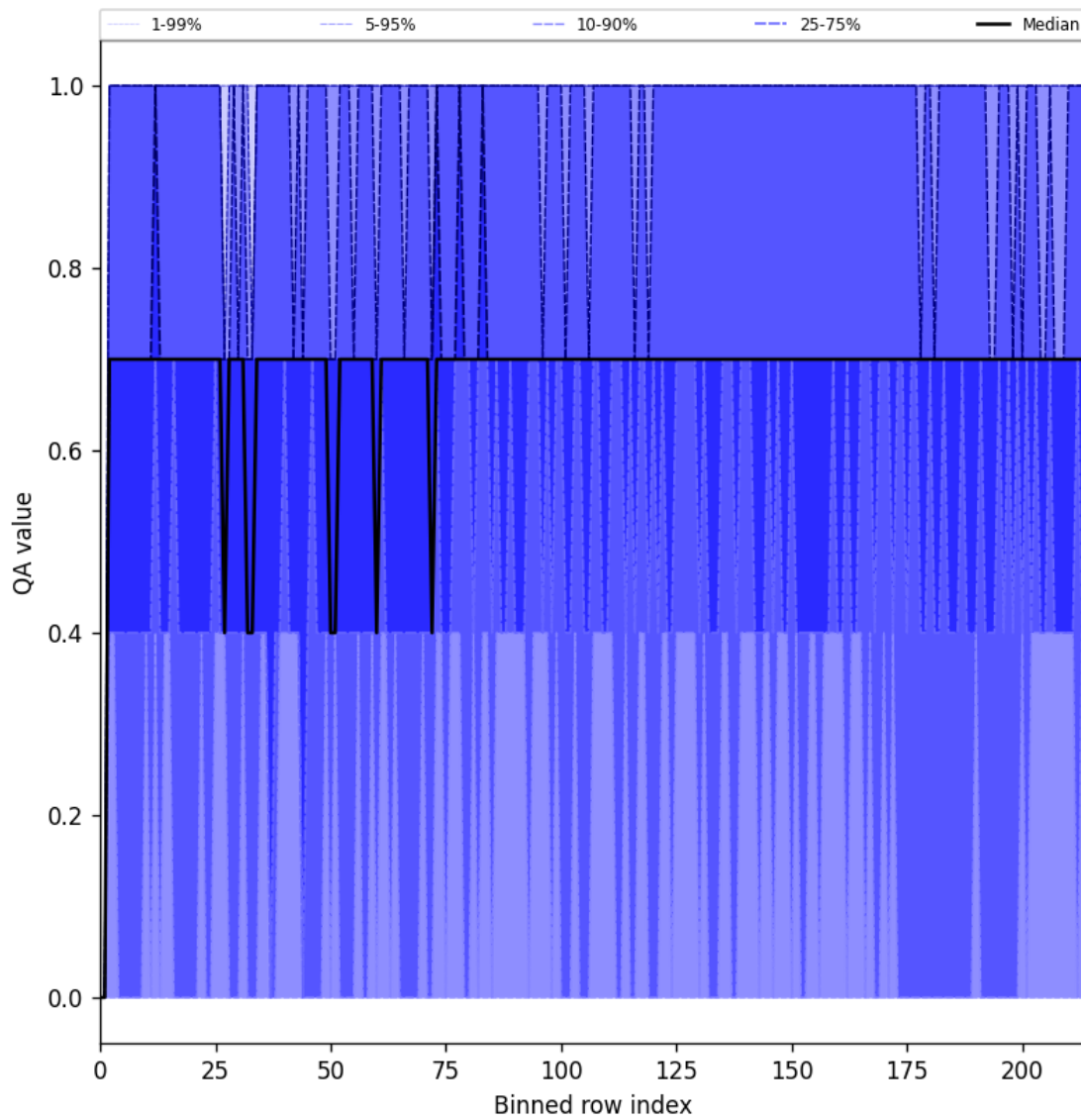
Figure 25: Along track statistics of “QA value” for 2025-02-15 to 2025-02-17
