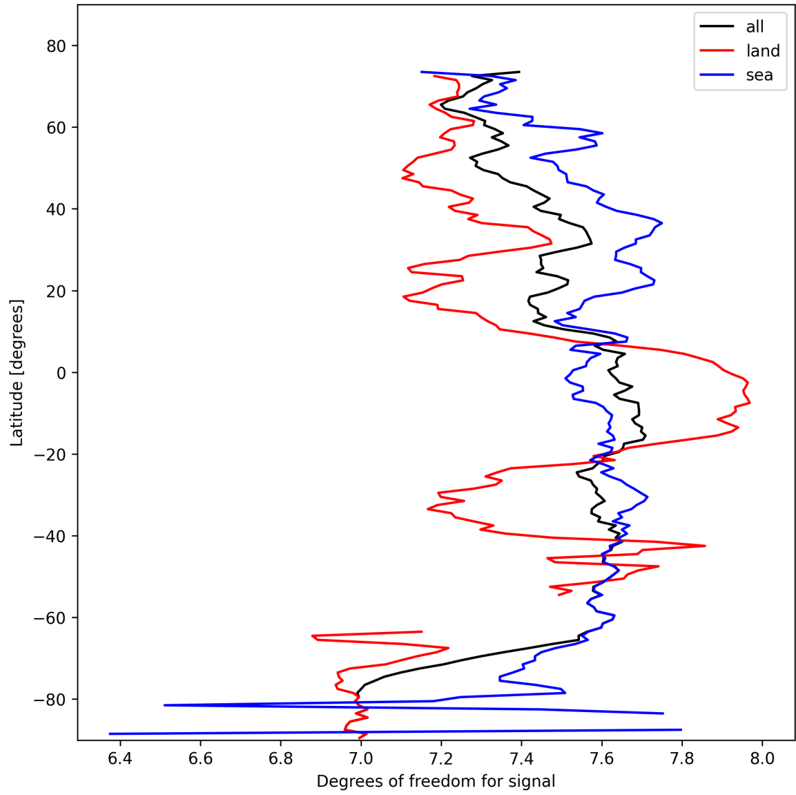
Figure 15: Zonal average of “Degrees of freedom for signal” for 2025-02-15 to 2025-02-17.
