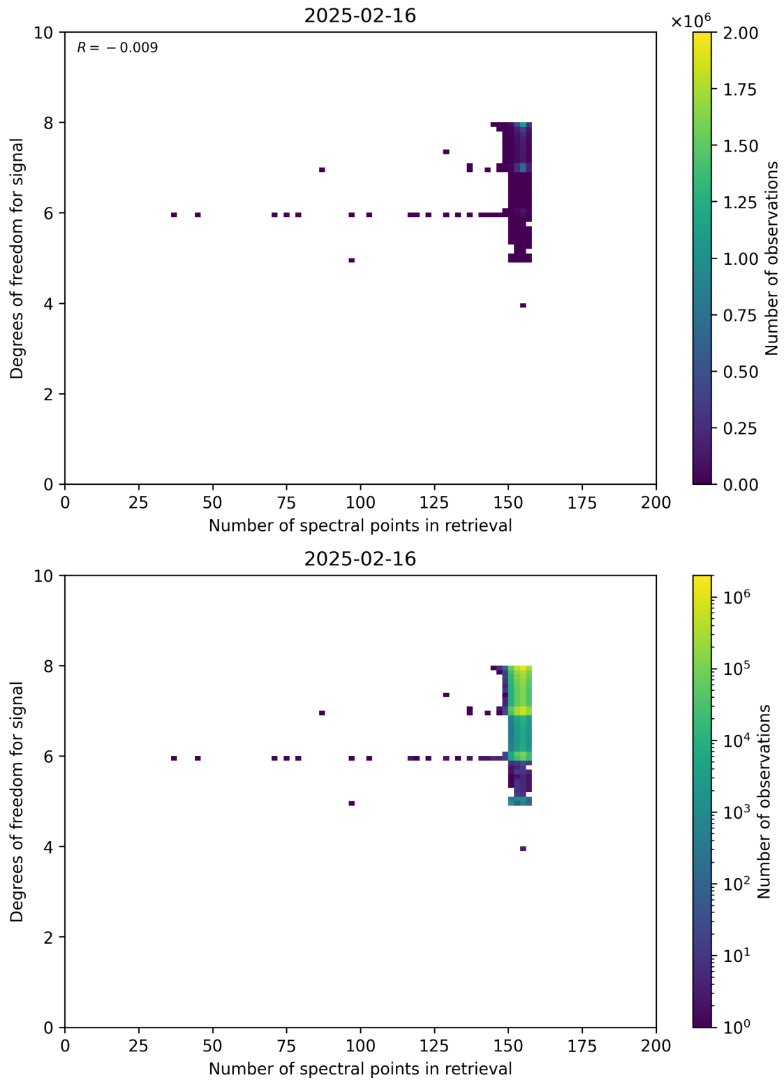
Figure 59: Scatter density plot of “Number of spectral points in retrieval” against “Degrees of freedom for signal” for 2025-02-15 to 2025-02-17.
