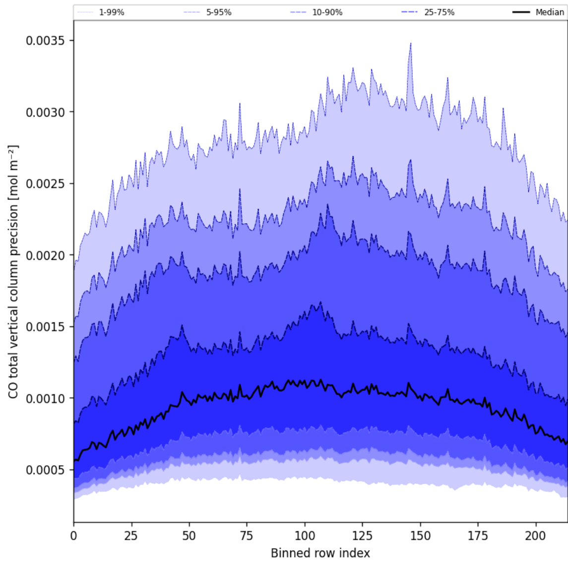
Figure 28: Along track statistics of “CO total vertical column precision” for 2025-02-15 to 2025-02-17
