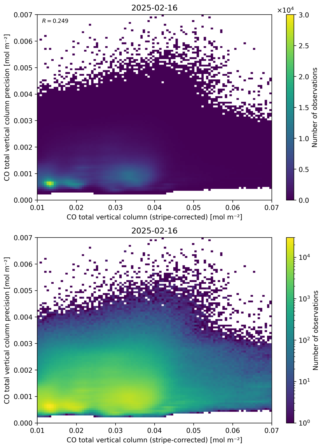
Figure 36: Scatter density plot of “CO total vertical column (stripe-corrected)” against “CO total vertical column precision” for 2025-02-15 to 2025-02-17.
