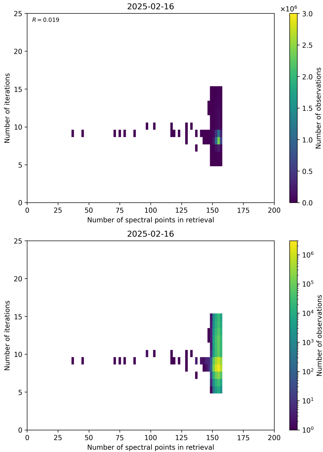
Figure 60: Scatter density plot of “Number of spectral points in retrieval” against “Number of iterations” for 2025-02-15 to 2025-02-17.
