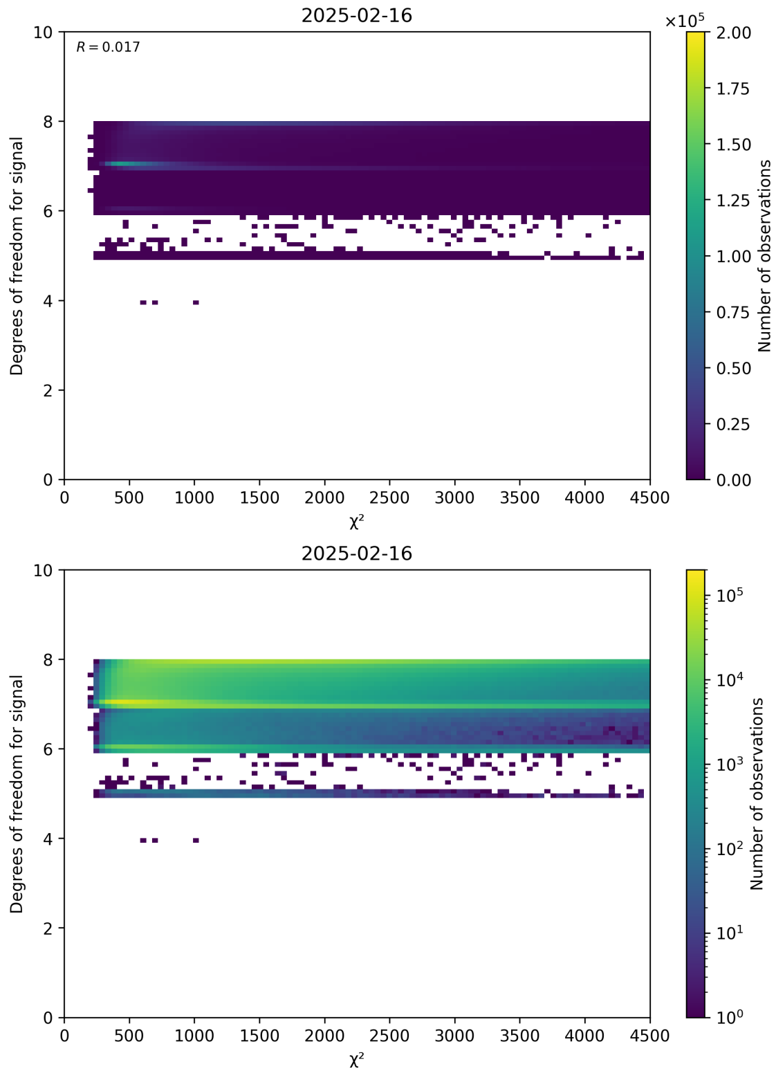
Figure 48: Scatter density plot of “ \chi^2 ” against “Degrees of freedom for signal” for 2025-02-15 to 2025-02-17.
