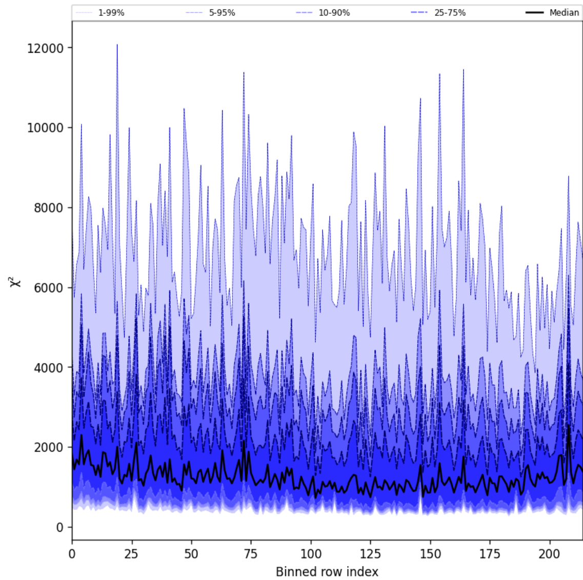
Figure 30: Along track statistics of “ \chi^2 ” for 2025-02-15 to 2025-02-17
