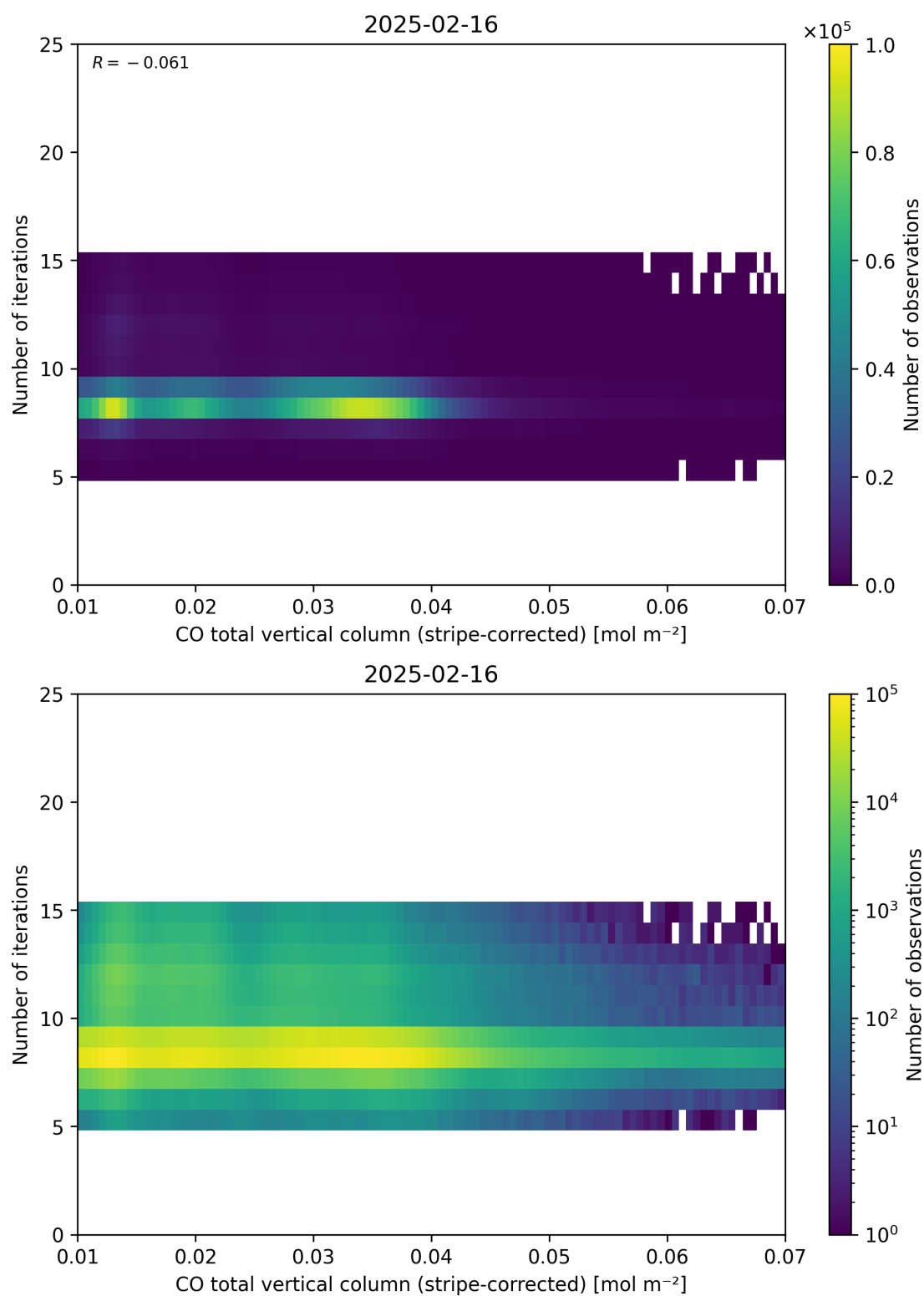
Figure 39: Scatter density plot of “CO total vertical column (stripe-corrected)” against “Number of iterations” for 2025-02-15 to 2025-02-17.
