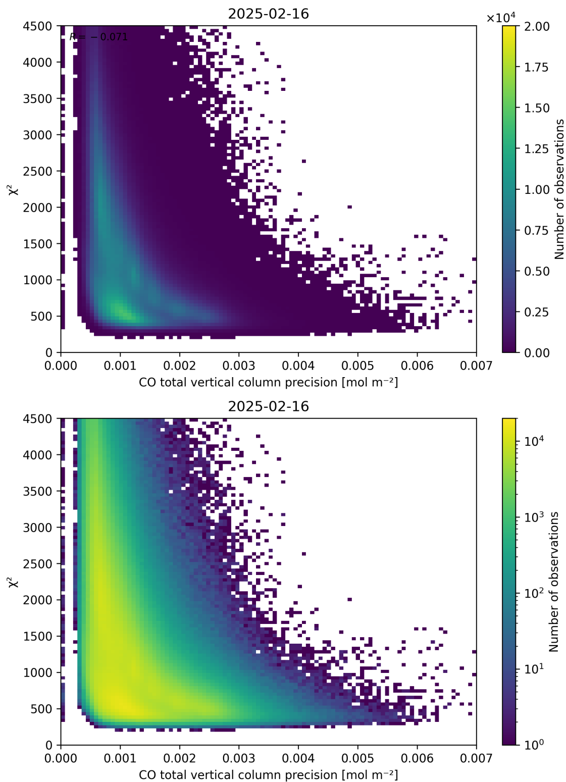
Figure 44: Scatter density plot of “CO total vertical column precision” against “ \chi^2 ” for 2025-02-15 to 2025-02-17.
