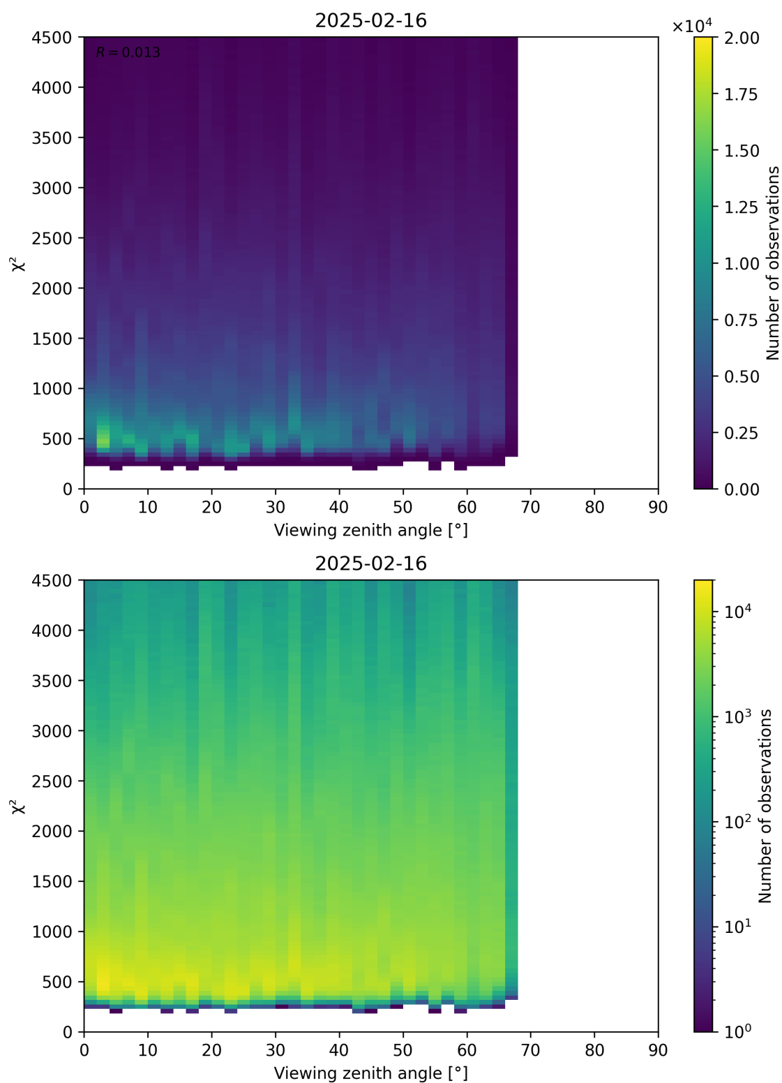
Figure 72: Scatter density plot of “Viewing zenith angle” against “ \chi^2 ” for 2025-02-15 to 2025-02-17.
