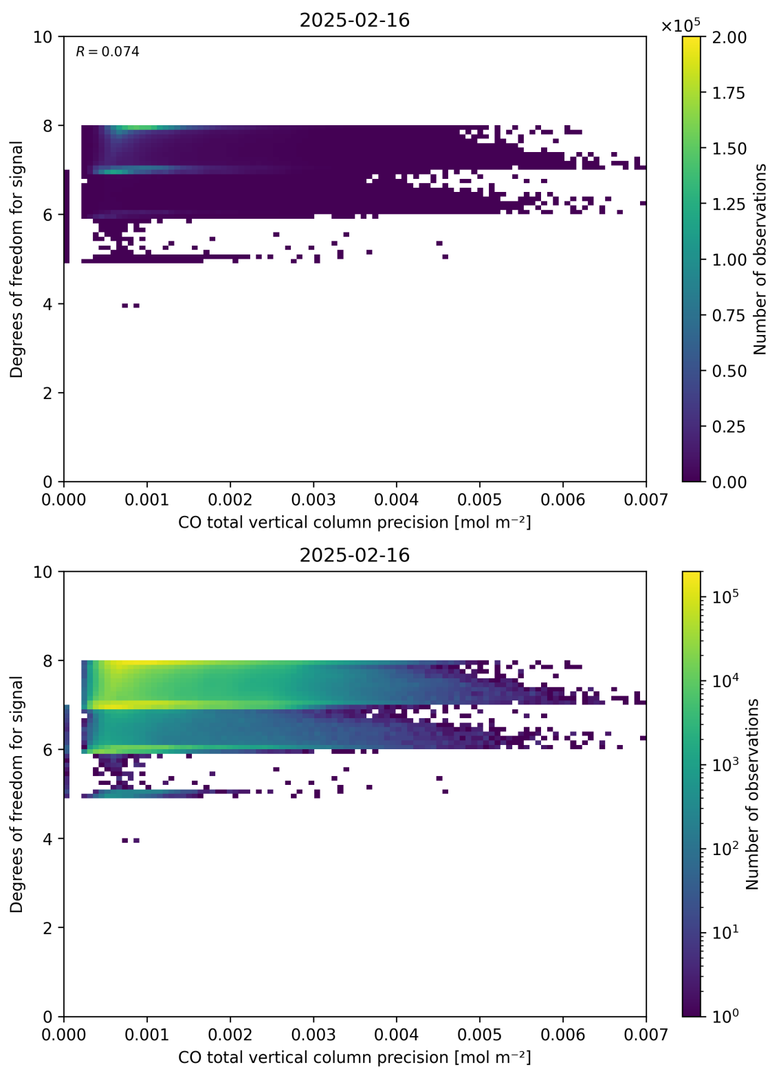
Figure 45: Scatter density plot of “CO total vertical column precision” against “Degrees of freedom for signal” for 2025-02-15 to 2025-02-17.
