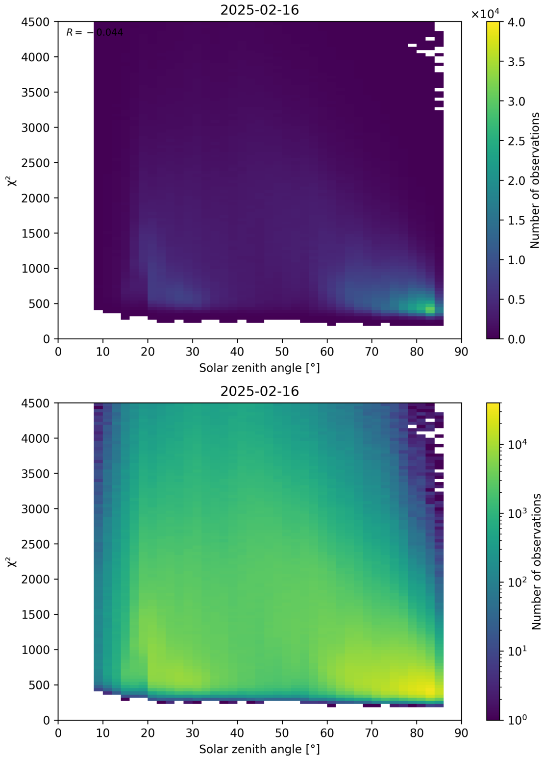
Figure 64: Scatter density plot of “Solar zenith angle” against “ \chi^2 ” for 2025-02-15 to 2025-02-17.
