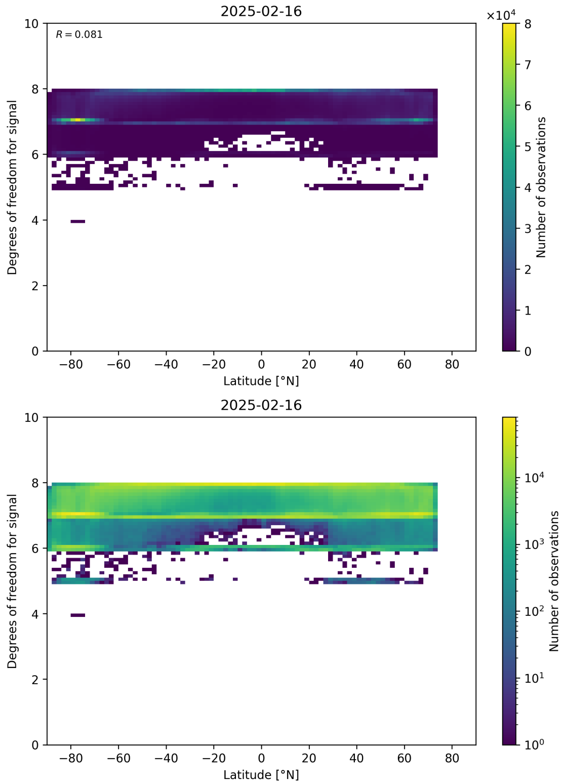
Figure 55: Scatter density plot of “Latitude” against “Degrees of freedom for signal” for 2025-02-15 to 2025-02-17.
