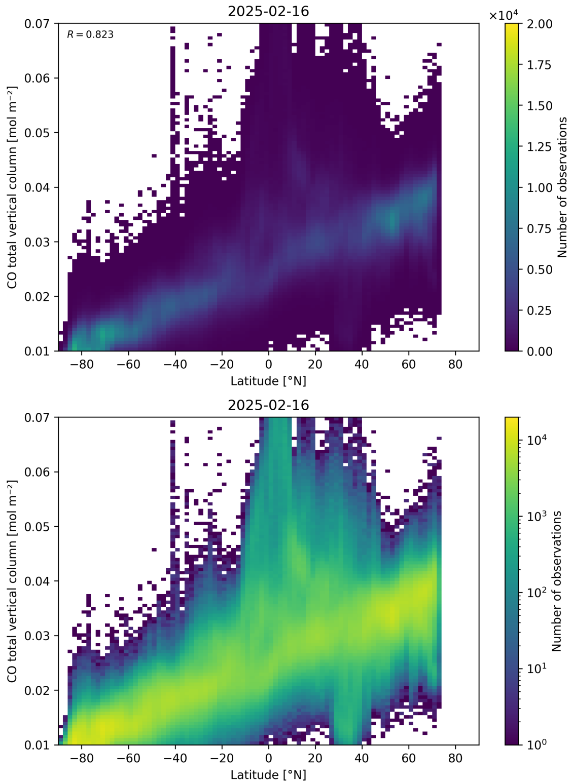
Figure 51: Scatter density plot of “Latitude” against “CO total vertical column” for 2025-02-15 to 2025-02-17.
