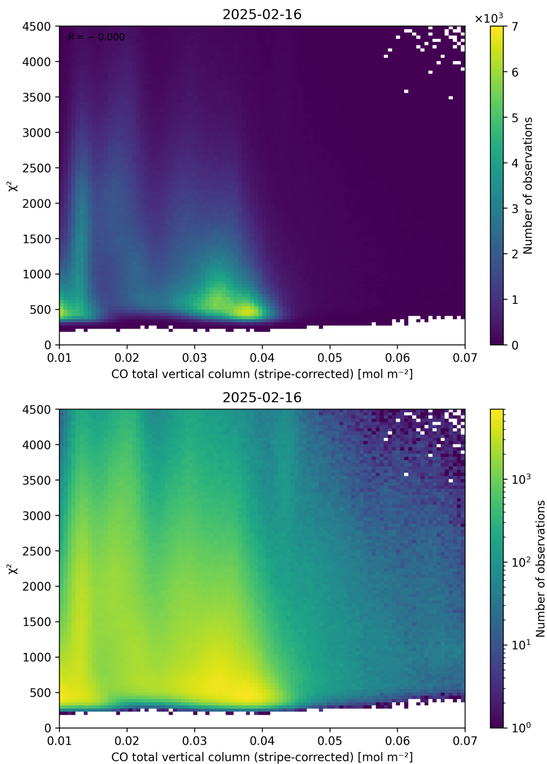
Figure 37: Scatter density plot of “CO total vertical column (stripe-corrected)” against “ \chi^2 ” for 2025-02-15 to 2025-02-17.
