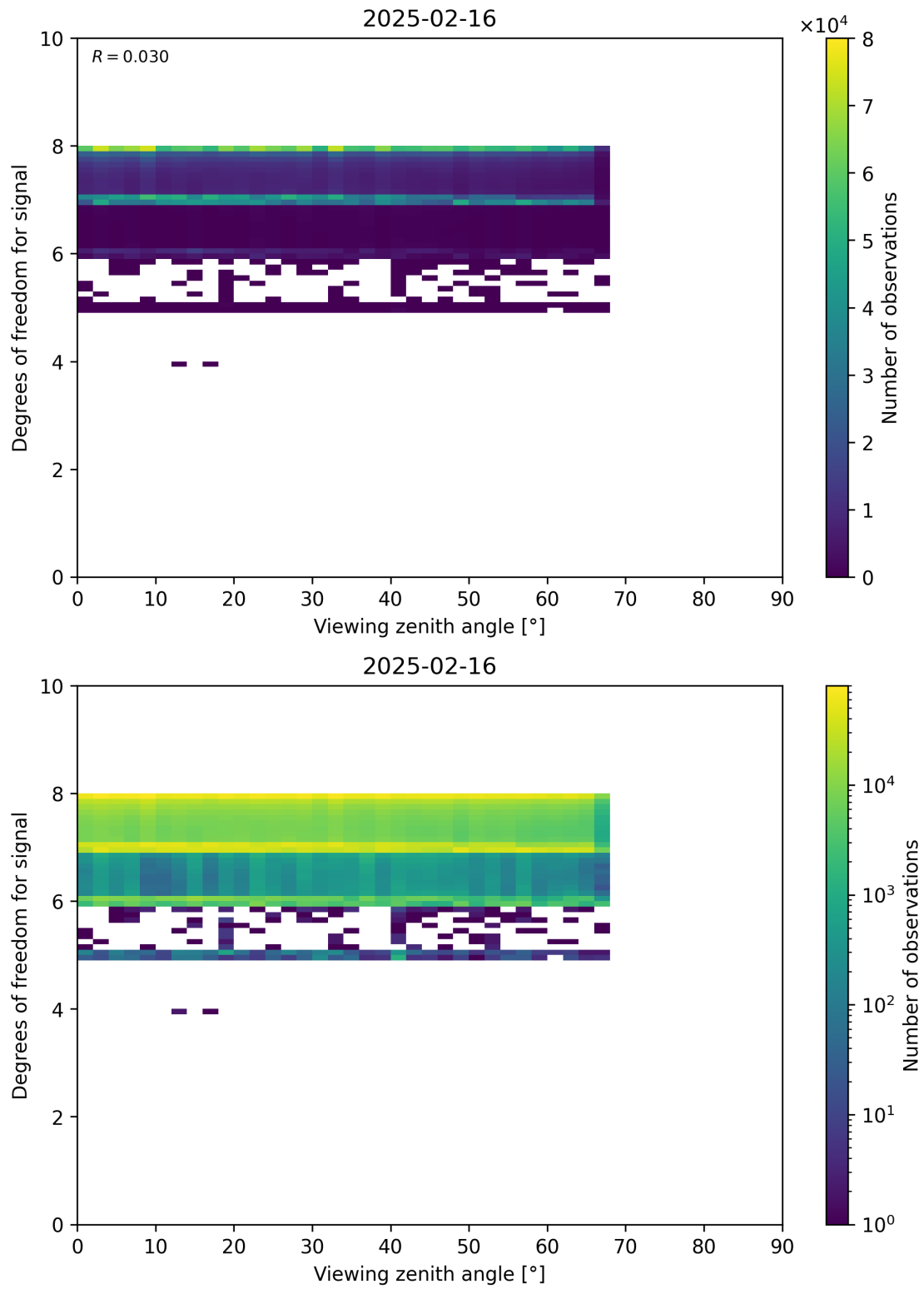
Figure 73: Scatter density plot of “Viewing zenith angle” against “Degrees of freedom for signal” for 2025-02-15 to 2025-02-17.
