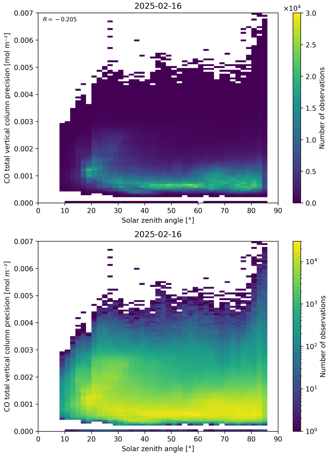
Figure 63: Scatter density plot of “Solar zenith angle” against “CO total vertical column precision” for 2025-02-15 to 2025-02-17.
