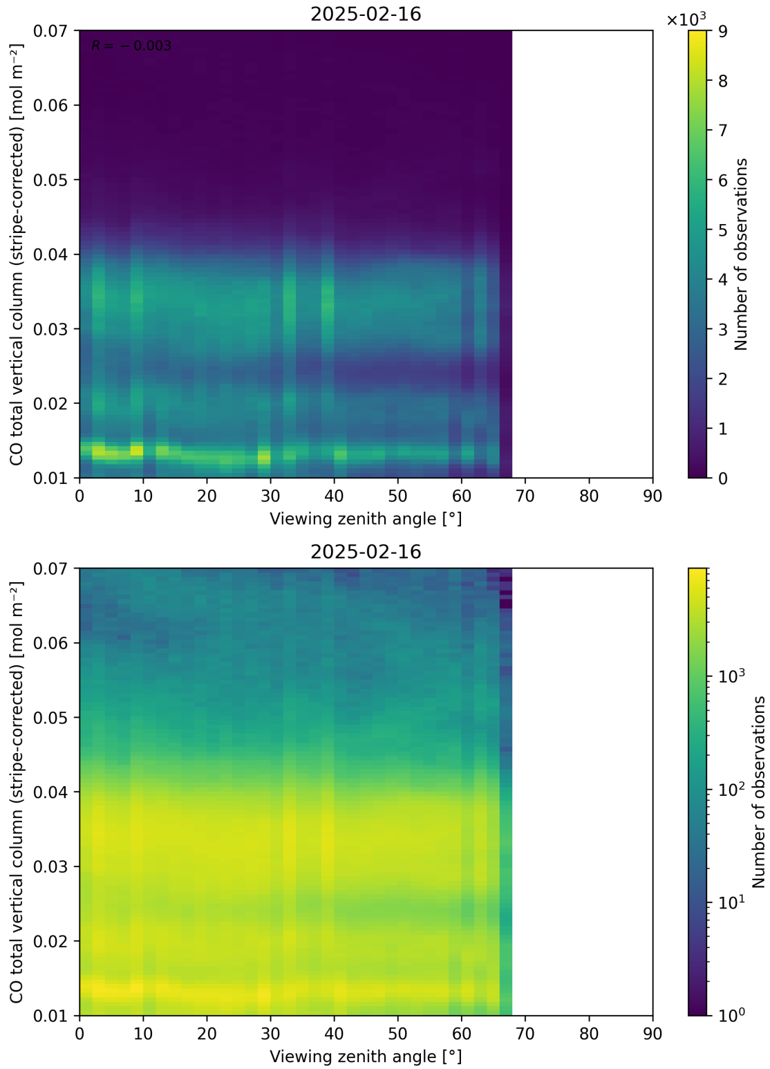
Figure 70: Scatter density plot of “Viewing zenith angle” against “CO total vertical column (stripe-corrected)” for 2025-02-15 to 2025-02-17.
