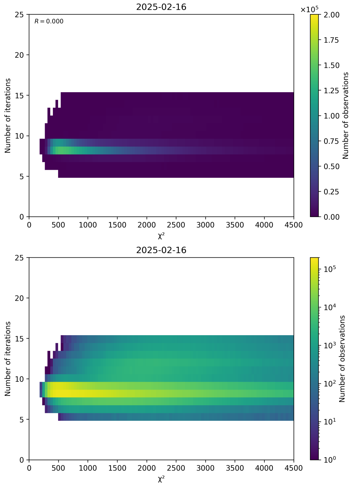
Figure 49: Scatter density plot of “ \chi^2 ” against “Number of iterations” for 2025-02-15 to 2025-02-17.
