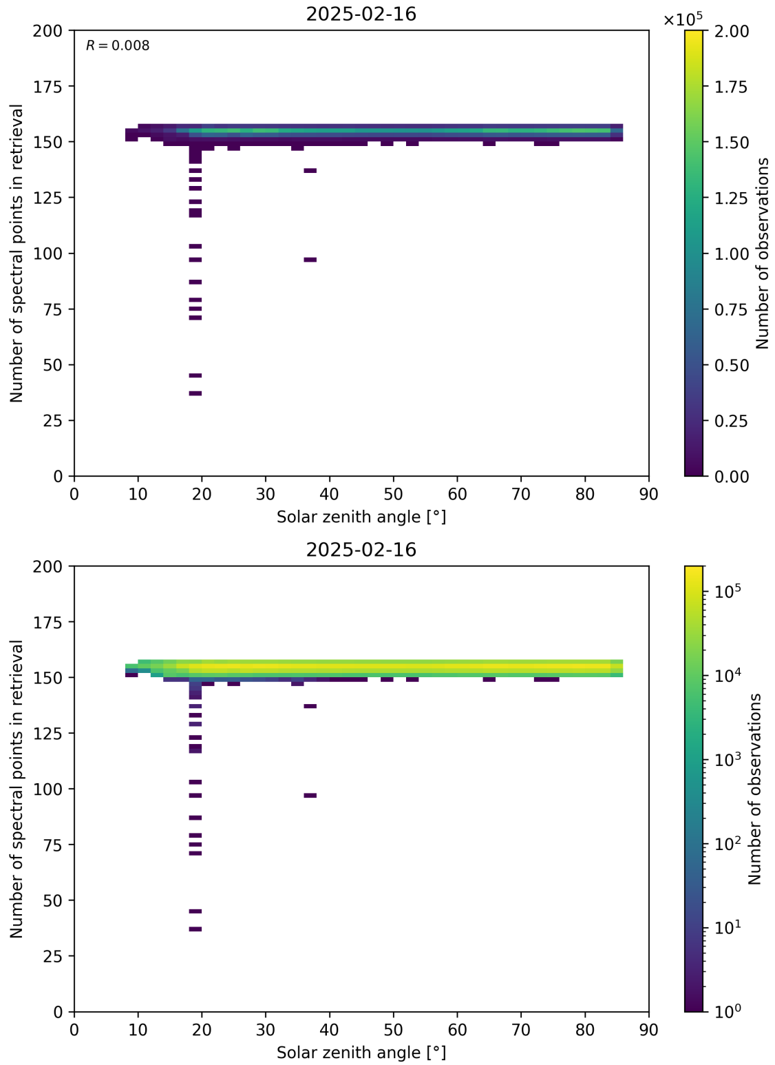
Figure 68: Scatter density plot of “Solar zenith angle” against “Number of spectral points in retrieval” for 2025-02-15 to 2025-02-17.
