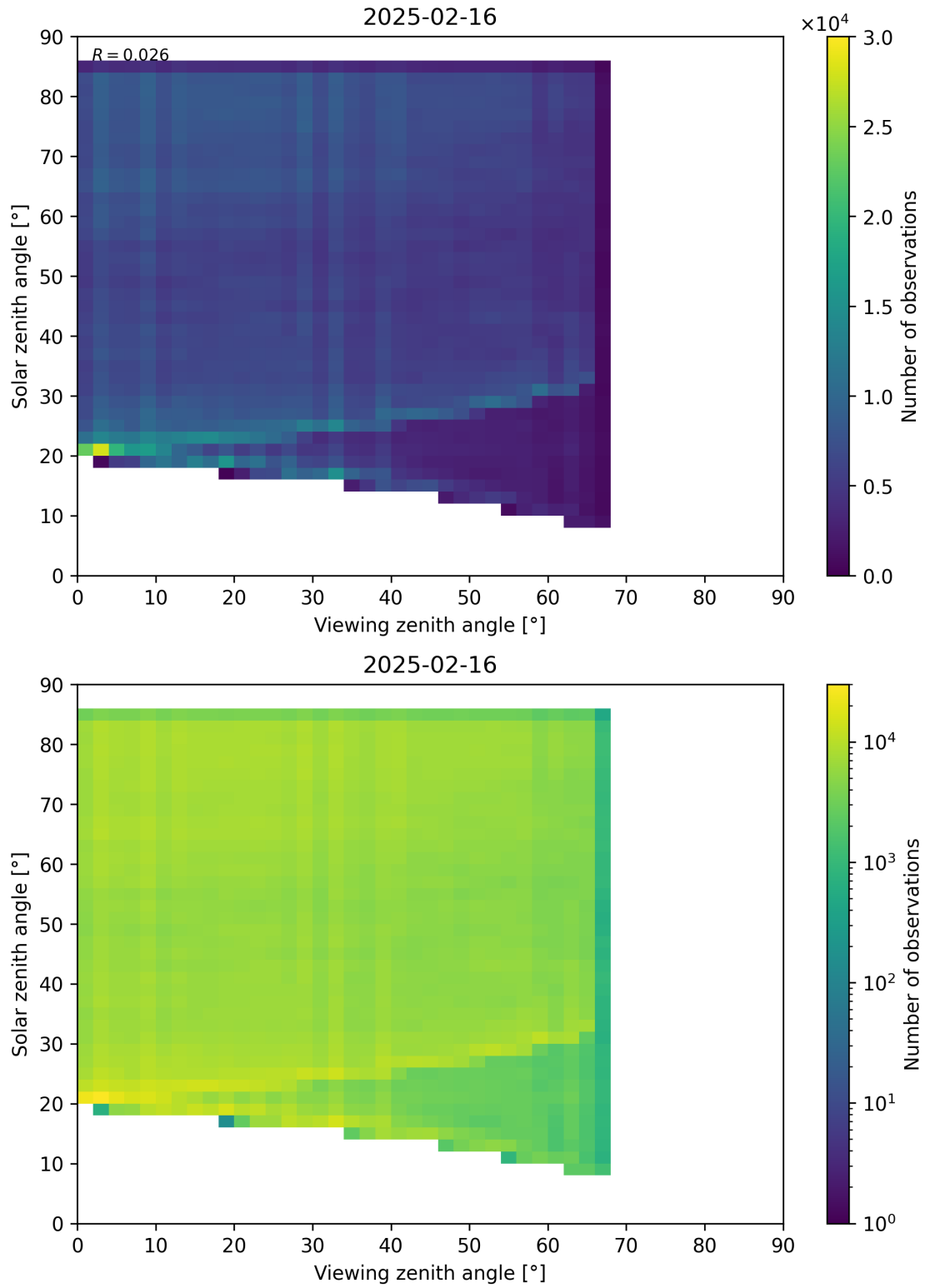
Figure 77: Scatter density plot of “Viewing zenith angle” against “Solar zenith angle” for 2025-02-15 to 2025-02-17.
