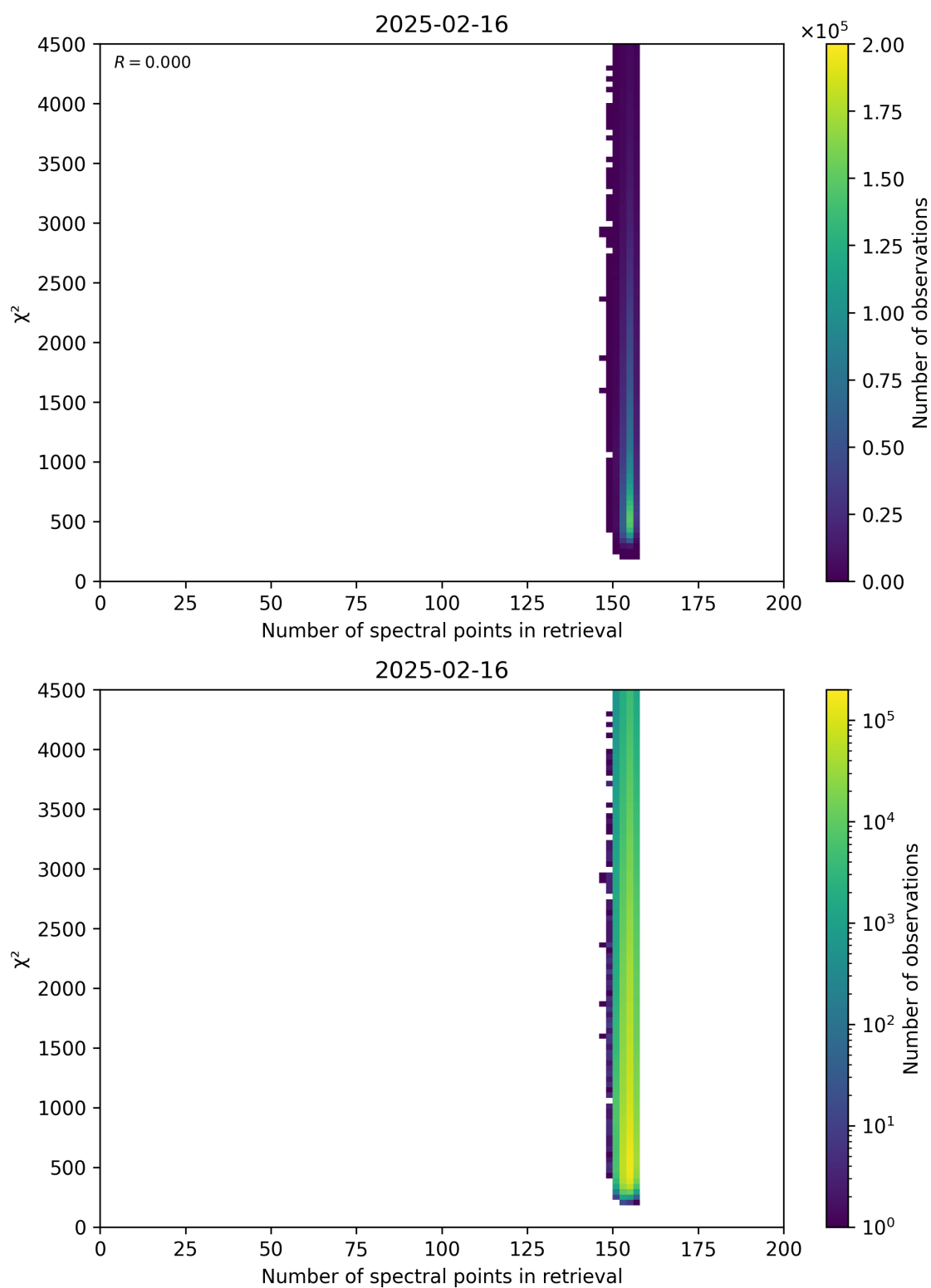
Figure 58: Scatter density plot of “Number of spectral points in retrieval” against “ \chi^2 ” for 2025-02-15 to 2025-02-17.
