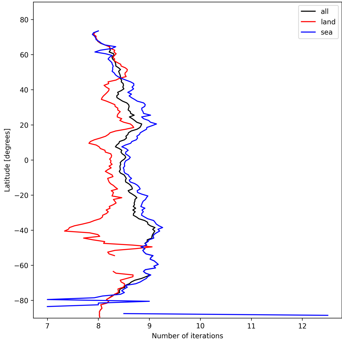
Figure 16: Zonal average of “Number of iterations” for 2025-02-15 to 2025-02-17.
