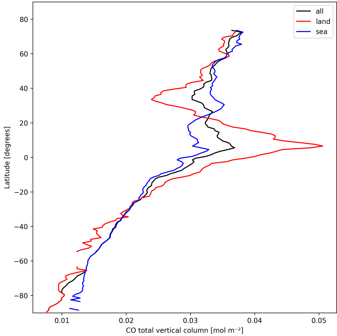
Figure 10: Zonal average of “CO total vertical column” for 2025-02-15 to 2025-02-17.
