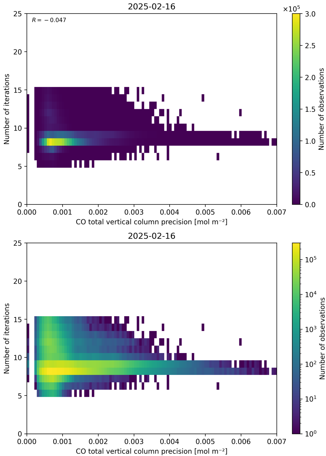
Figure 46: Scatter density plot of “CO total vertical column precision” against “Number of iterations” for 2025-02-15 to 2025-02-17.
