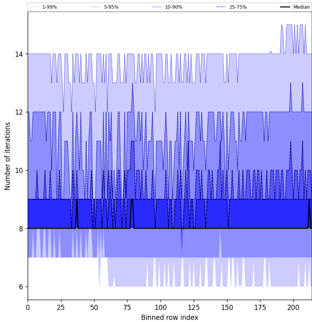
Figure 32: Along track statistics of “Number of iterations” for 2025-02-15 to 2025-02-17
