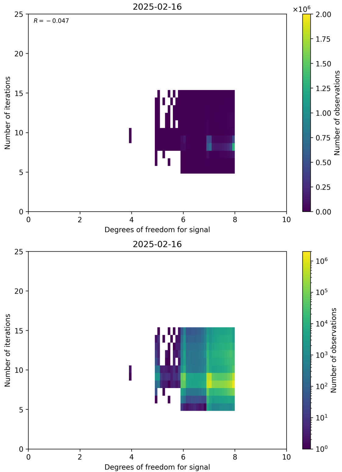
Figure 50: Scatter density plot of “Degrees of freedom for signal” against “Number of iterations” for 2025-02-15 to 2025-02-17.
