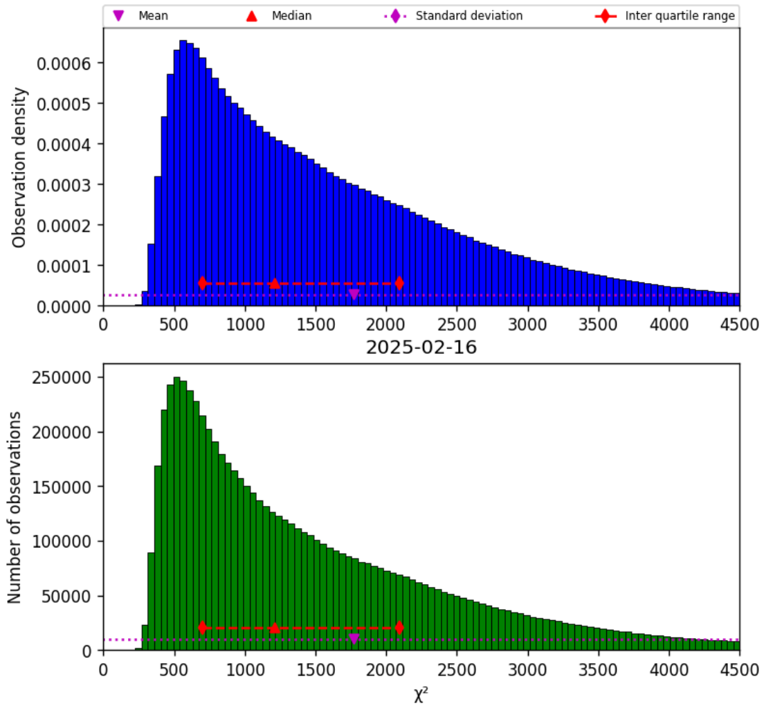
Figure 22: Histogram of “ \chi^2 ” for 2025-02-15 to 2025-02-17
