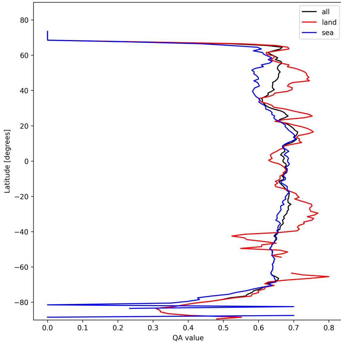
Figure 9: Zonal average of “QA value” for 2025-02-15 to 2025-02-17.
