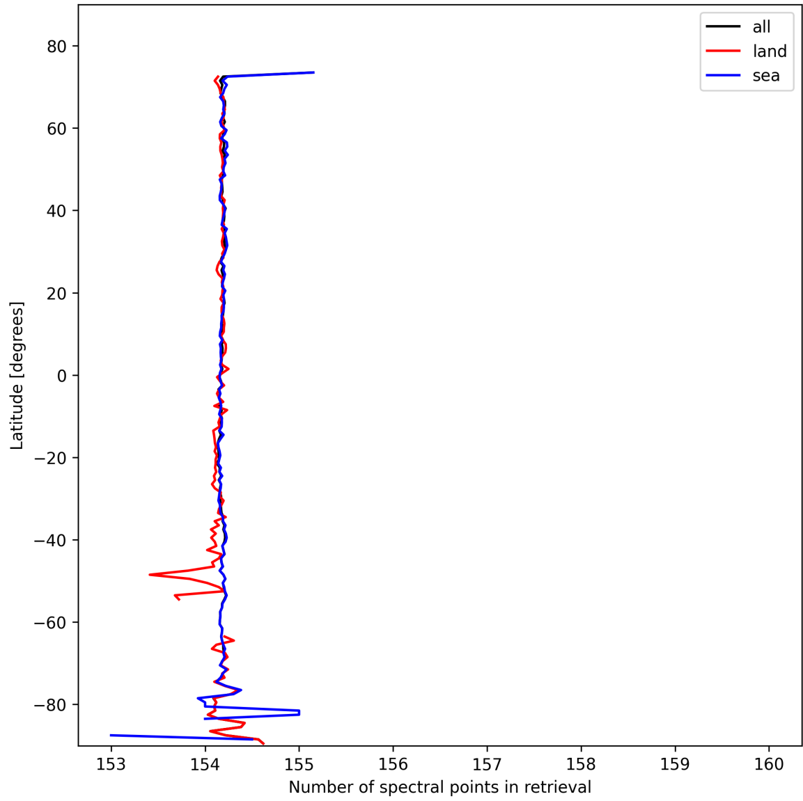
Figure 13: Zonal average of “Number of spectral points in retrieval” for 2025-02-15 to 2025-02-17.
