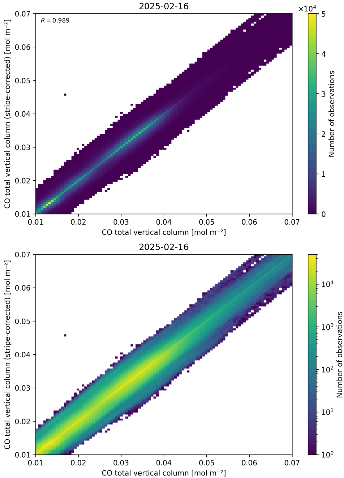
Figure 33: Scatter density plot of “CO total vertical column” against “CO total vertical column (stripe-corrected)” for 2025-02-15 to 2025-02-17.
