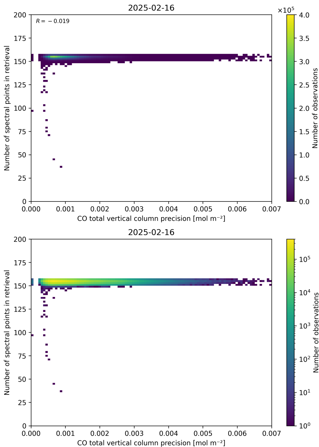
Figure 47: Scatter density plot of “CO total vertical column precision” against “Number of spectral points in retrieval” for 2025-02-15 to 2025-02-17.
