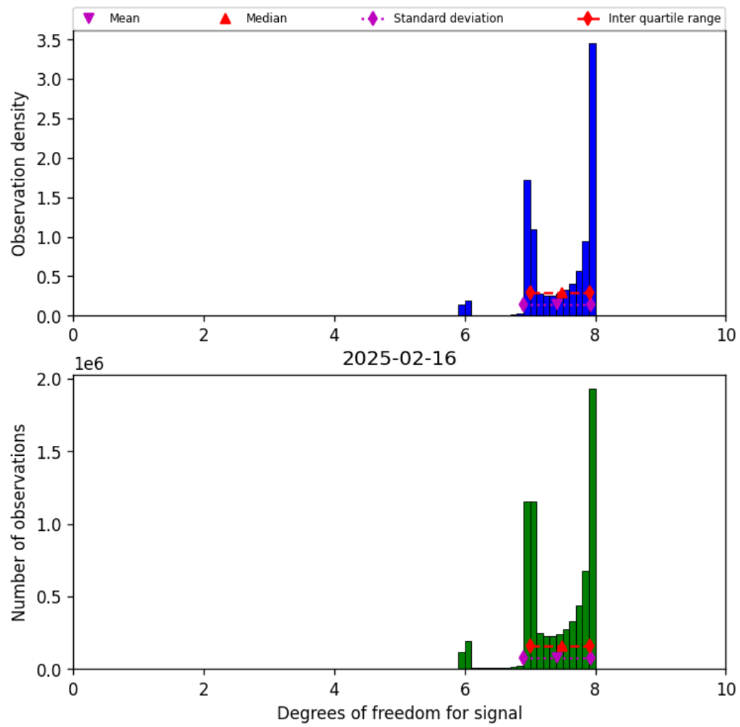
Figure 23: Histogram of “Degrees of freedom for signal” for 2025-02-15 to 2025-02-17
