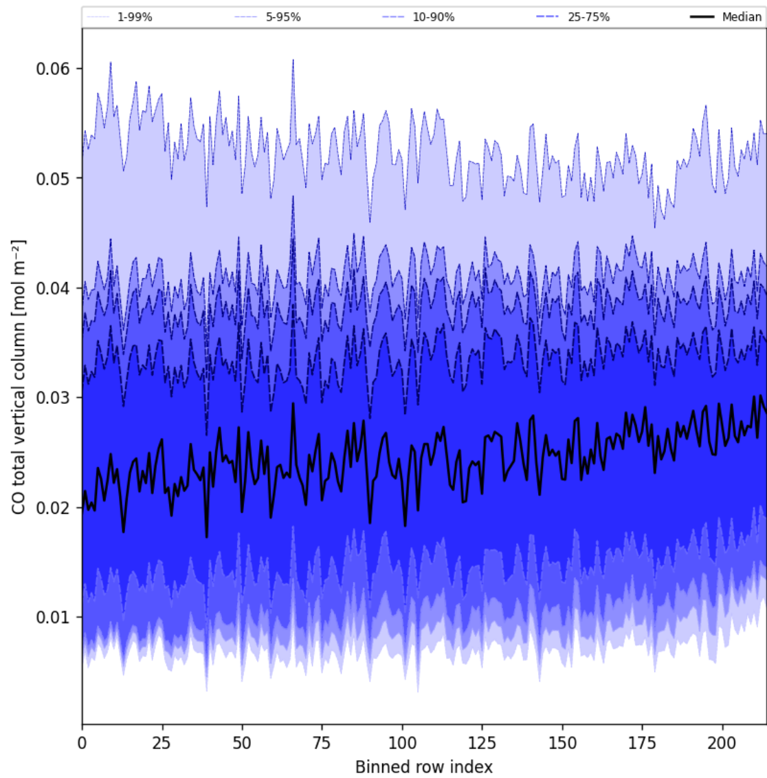
Figure 26: Along track statistics of “CO total vertical column” for 2025-02-15 to 2025-02-17
