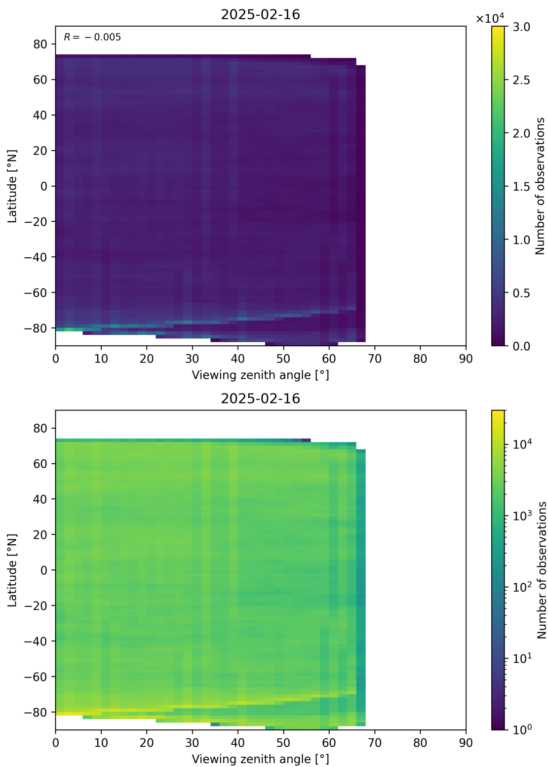
Figure 74: Scatter density plot of “Viewing zenith angle” against “Latitude” for 2025-02-15 to 2025-02-17.
