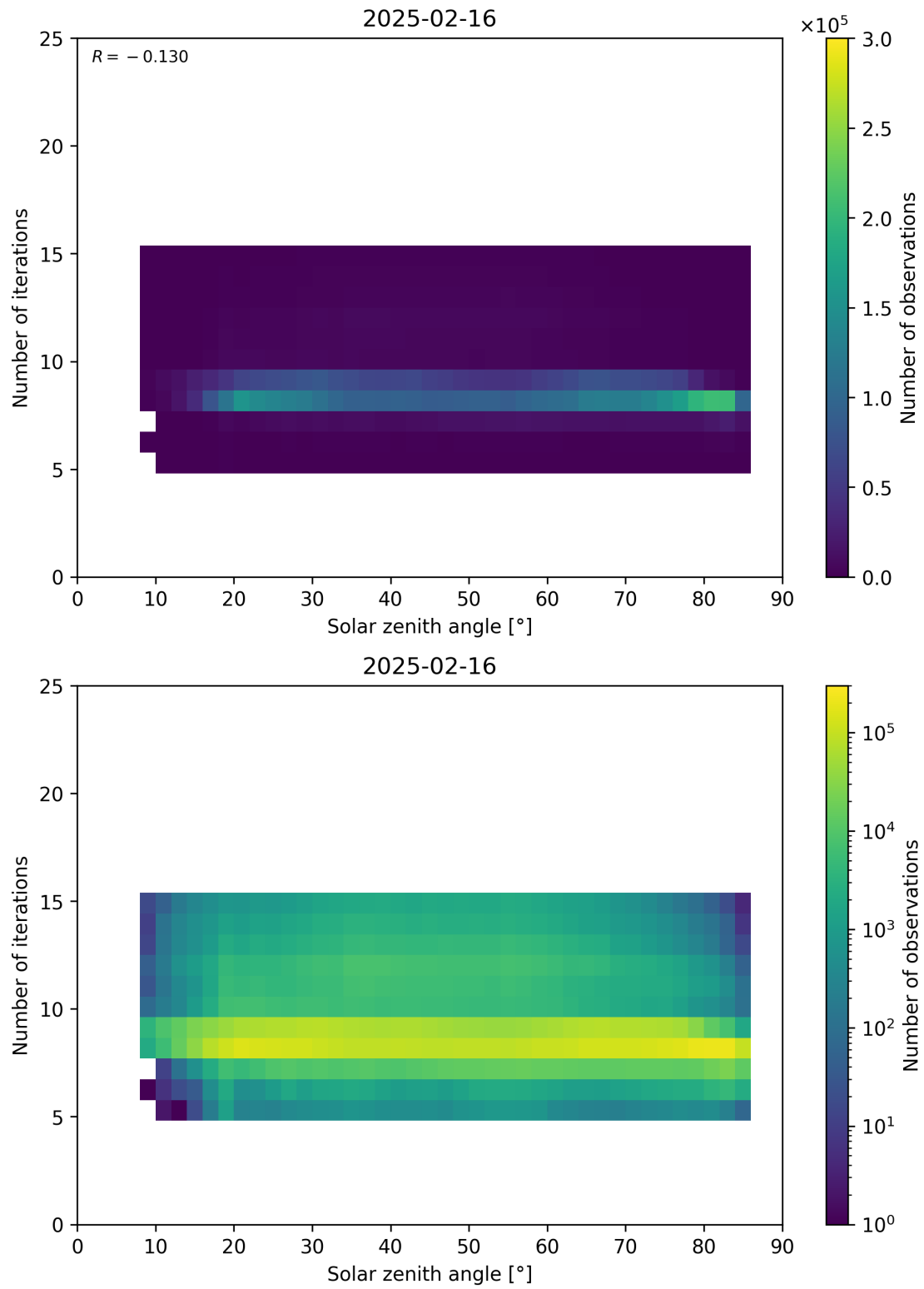
Figure 67: Scatter density plot of “Solar zenith angle” against “Number of iterations” for 2025-02-15 to 2025-02-17.
