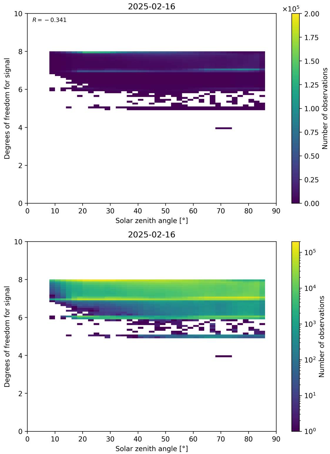
Figure 65: Scatter density plot of “Solar zenith angle” against “Degrees of freedom for signal” for 2025-02-15 to 2025-02-17.
