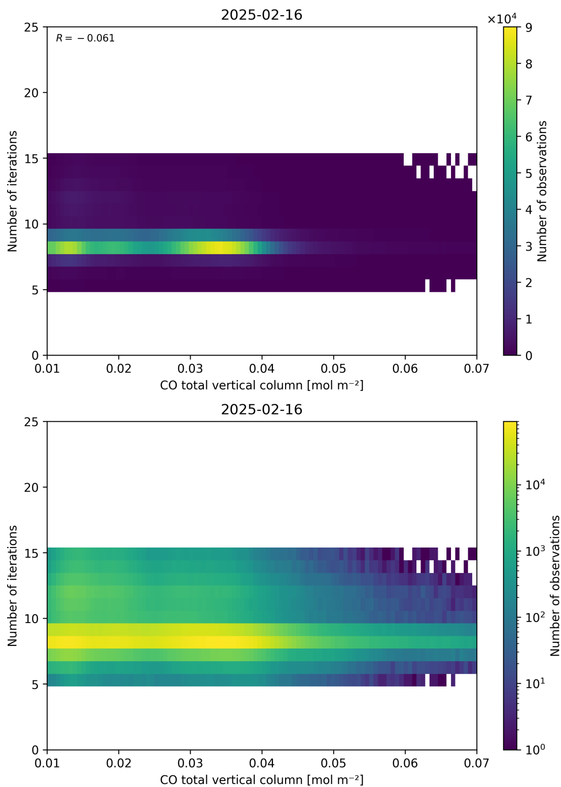
Figure 42: Scatter density plot of “CO total vertical column” against “Number of iterations” for 2025-02-15 to 2025-02-17.
