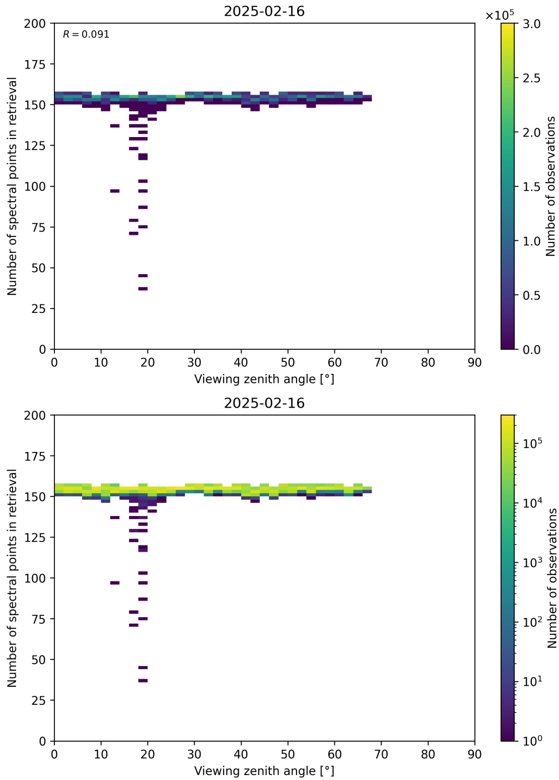
Figure 76: Scatter density plot of “Viewing zenith angle” against “Number of spectral points in retrieval” for 2025-02-15 to 2025-02-17.
