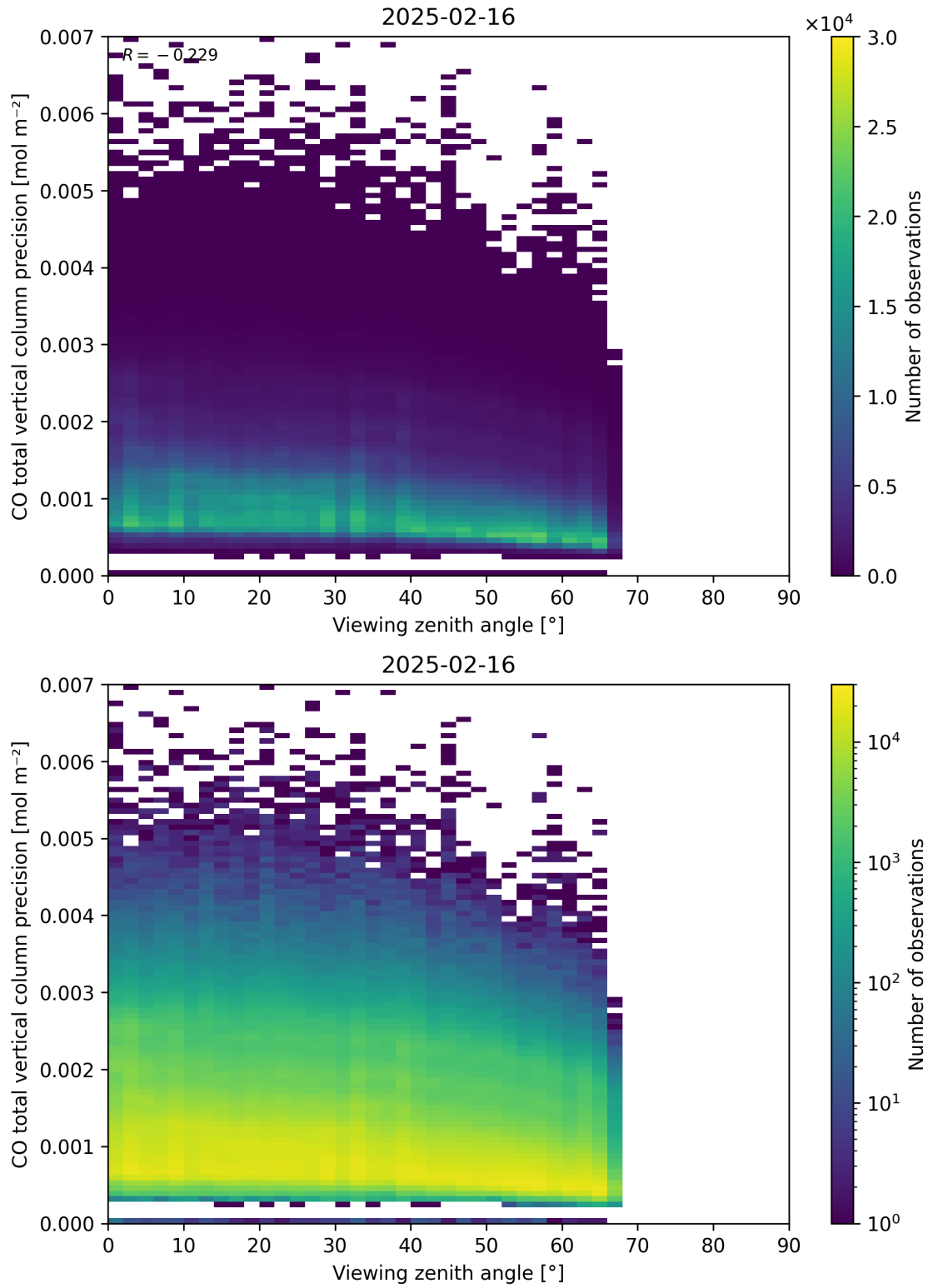
Figure 71: Scatter density plot of “Viewing zenith angle” against “CO total vertical column precision” for 2025-02-15 to 2025-02-17.
