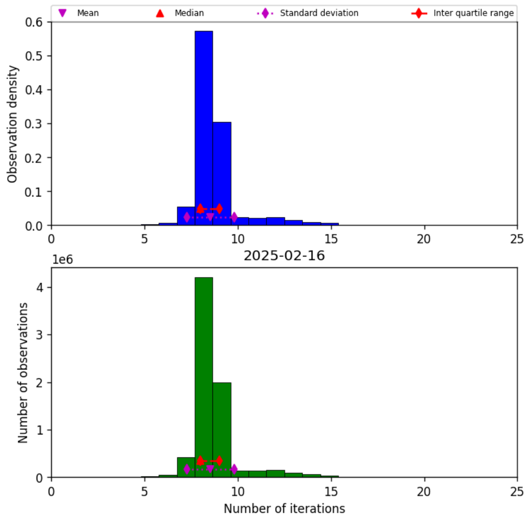
Figure 24: Histogram of “Number of iterations” for 2025-02-15 to 2025-02-17
