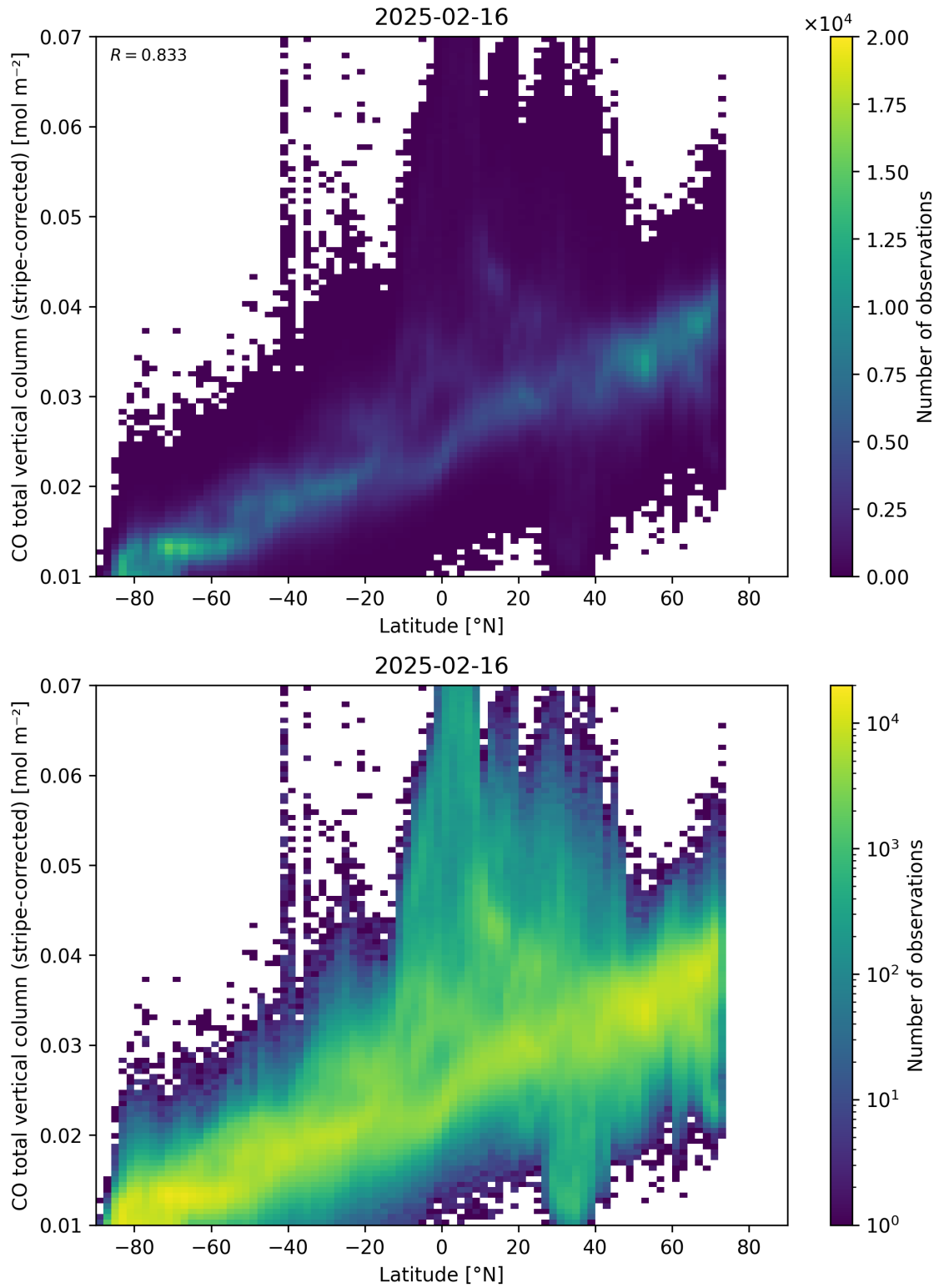
Figure 52: Scatter density plot of “Latitude” against “CO total vertical column (stripe-corrected)” for 2025-02-15 to 2025-02-17.
