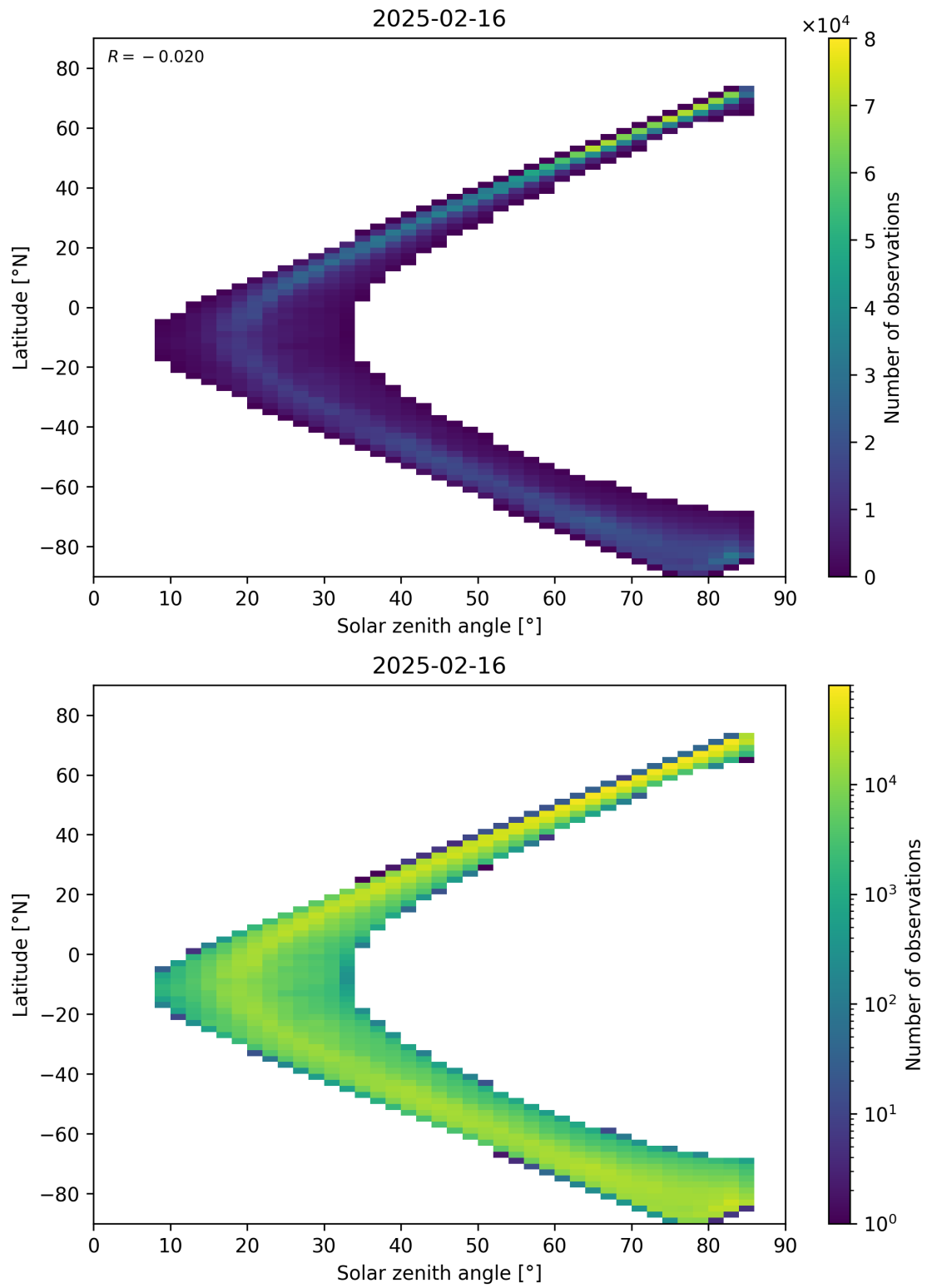
Figure 66: Scatter density plot of “Solar zenith angle” against “Latitude” for 2025-02-15 to 2025-02-17.
