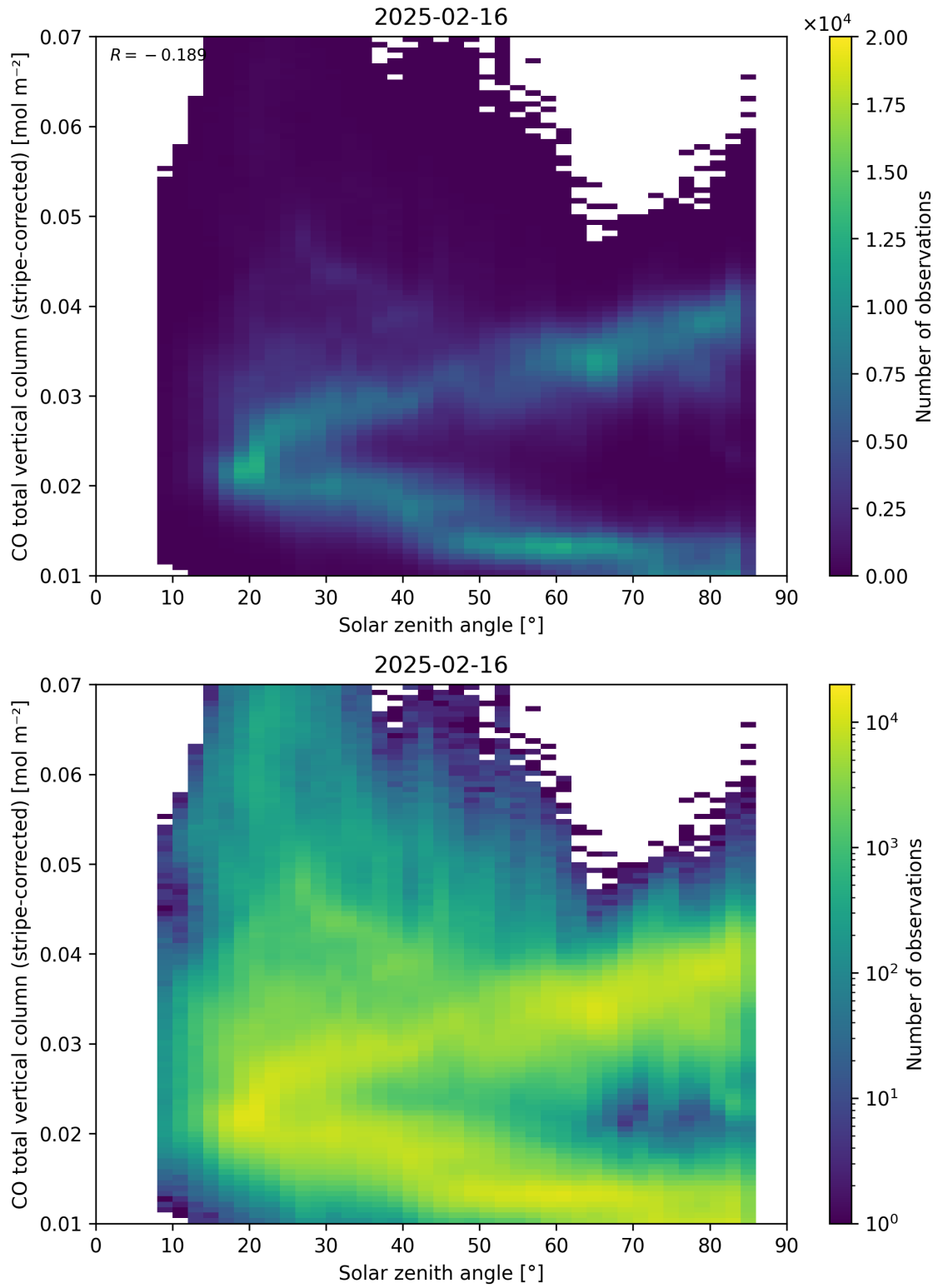
Figure 62: Scatter density plot of “Solar zenith angle” against “CO total vertical column (stripe-corrected)” for 2025-02-15 to 2025-02-17.
