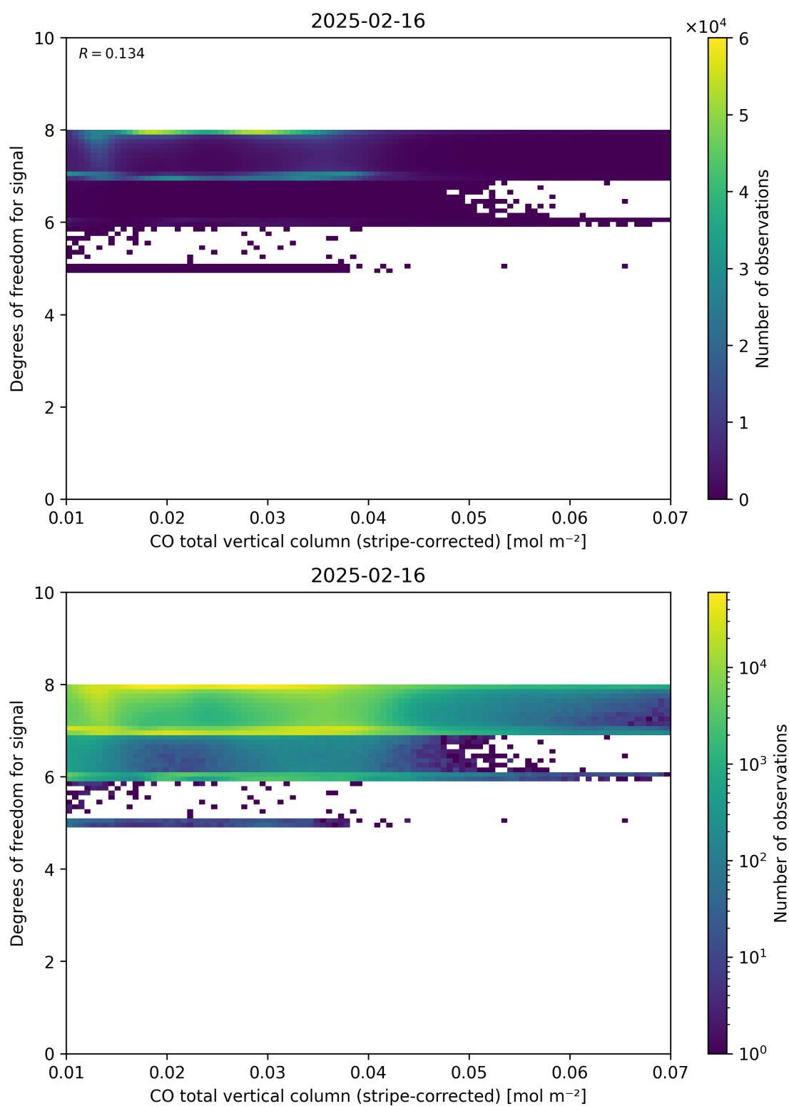
Figure 38: Scatter density plot of “CO total vertical column (stripe-corrected)” against “Degrees of freedom for signal” for 2025-02-15 to 2025-02-17.
