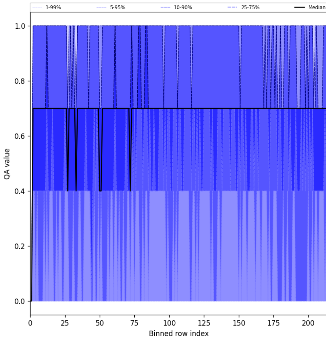
Figure 25: Along track statistics of “QA value” for 2025-02-16 to 2025-02-18
