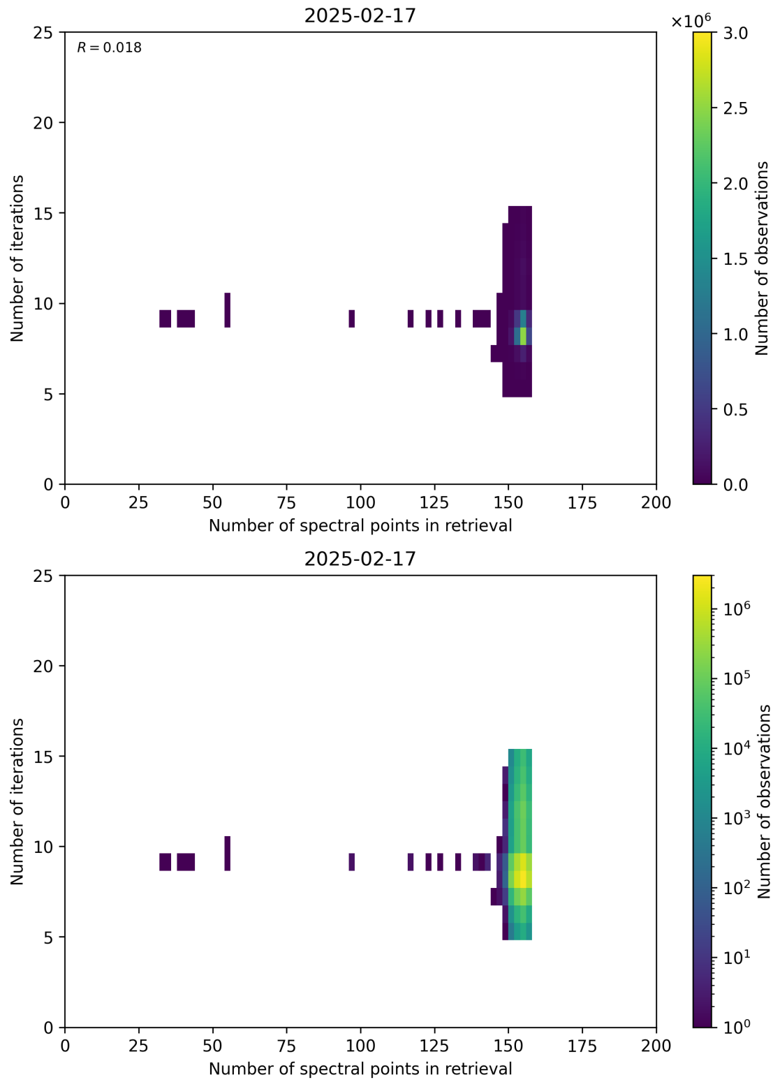
Figure 60: Scatter density plot of “Number of spectral points in retrieval” against “Number of iterations” for 2025-02-16 to 2025-02-18.
