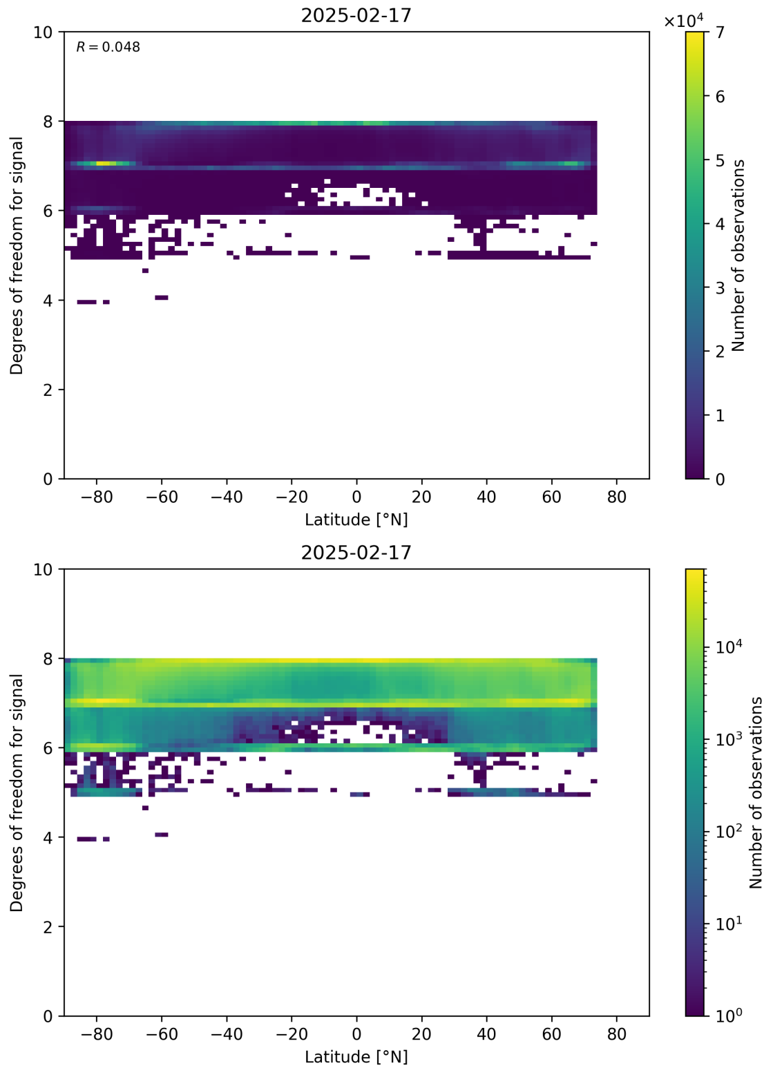
Figure 55: Scatter density plot of “Latitude” against “Degrees of freedom for signal” for 2025-02-16 to 2025-02-18.
