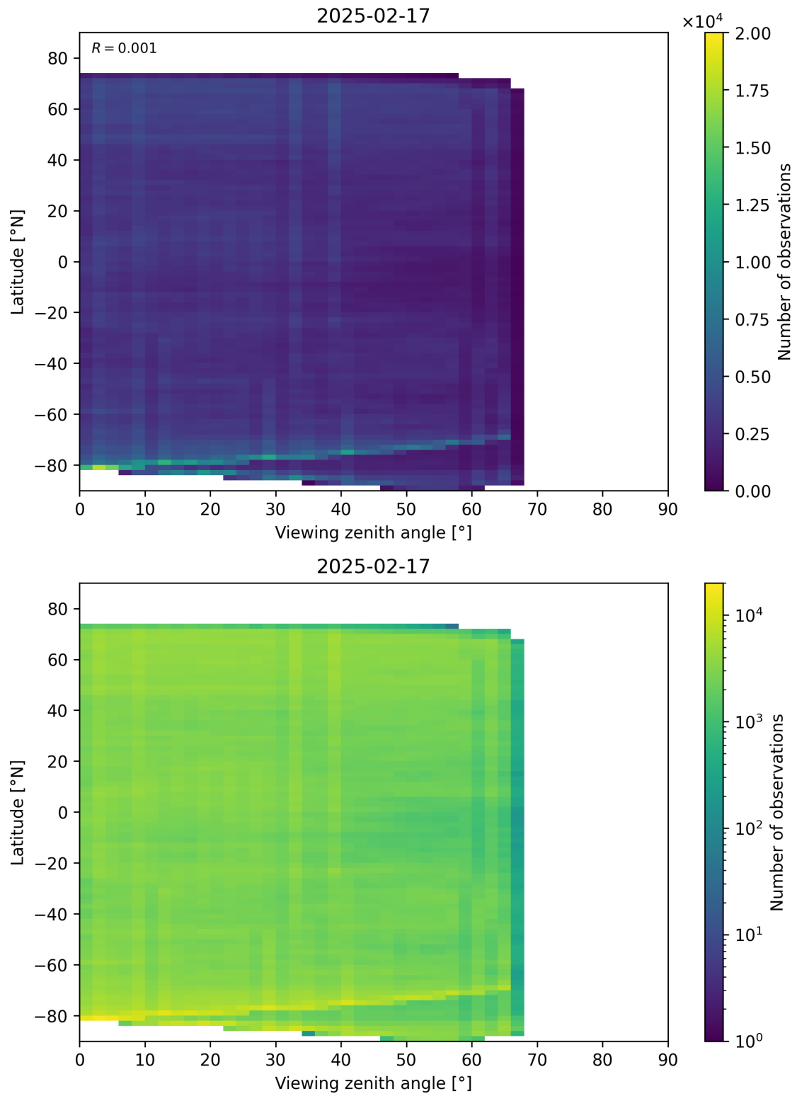
Figure 74: Scatter density plot of “Viewing zenith angle” against “Latitude” for 2025-02-16 to 2025-02-18.
