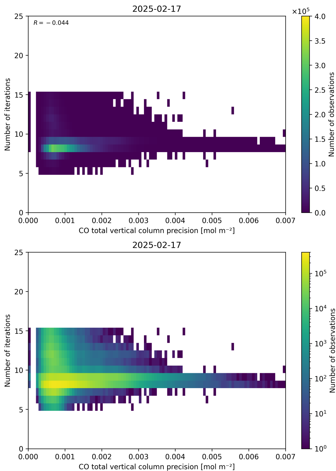
Figure 46: Scatter density plot of “CO total vertical column precision” against “Number of iterations” for 2025-02-16 to 2025-02-18.
