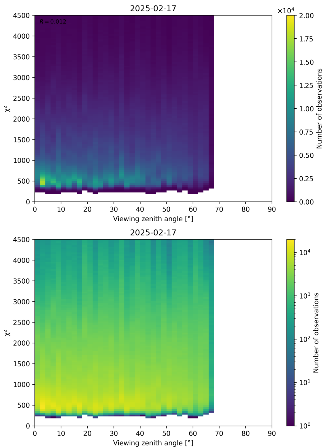
Figure 72: Scatter density plot of “Viewing zenith angle” against “ \chi^2 ” for 2025-02-16 to 2025-02-18.
