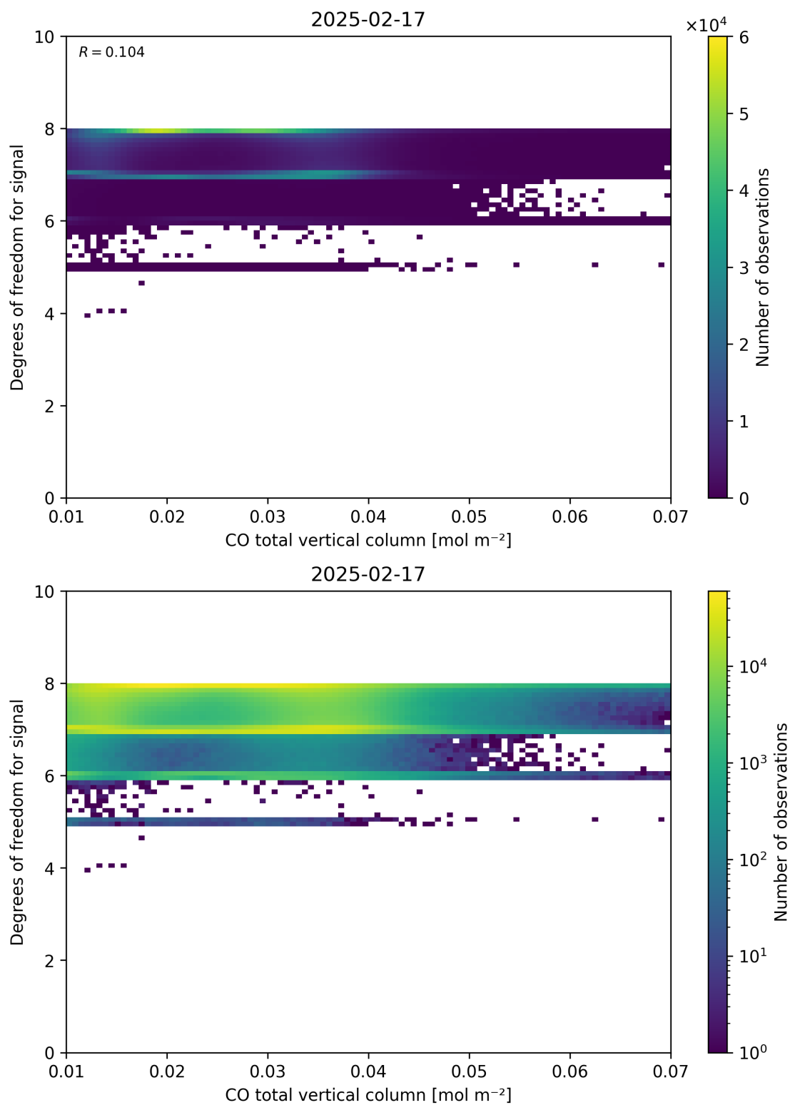
Figure 41: Scatter density plot of “CO total vertical column” against “Degrees of freedom for signal” for 2025-02-16 to 2025-02-18.
