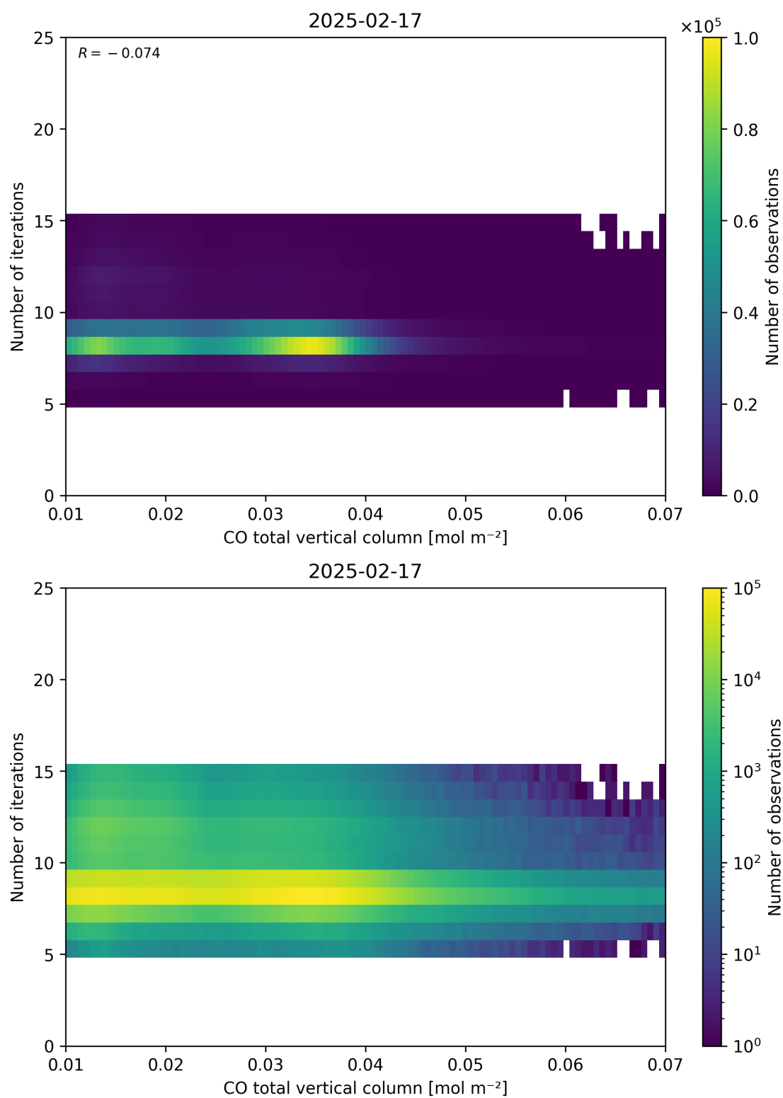
Figure 42: Scatter density plot of “CO total vertical column” against “Number of iterations” for 2025-02-16 to 2025-02-18.
