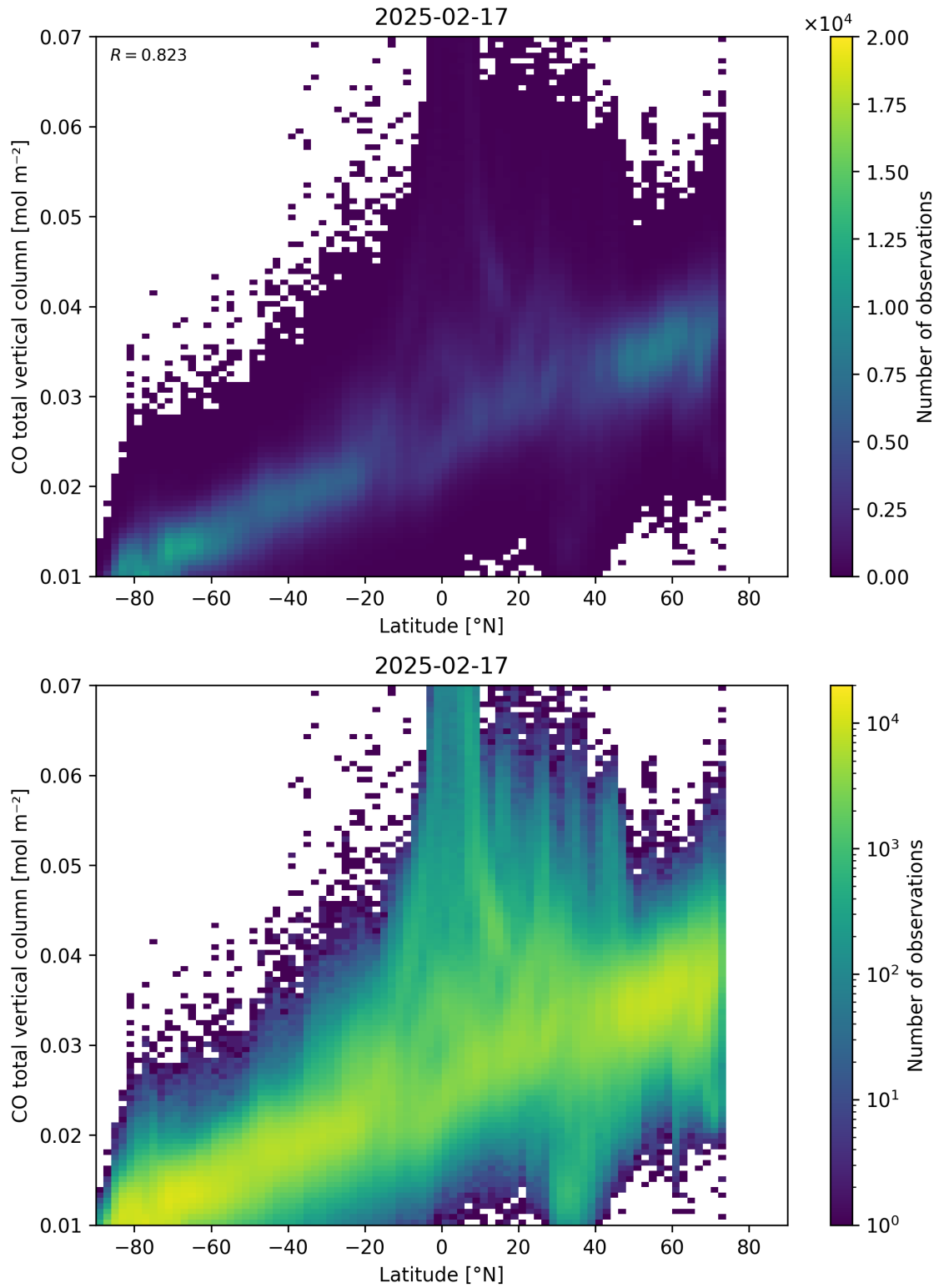
Figure 51: Scatter density plot of “Latitude” against “CO total vertical column” for 2025-02-16 to 2025-02-18.
