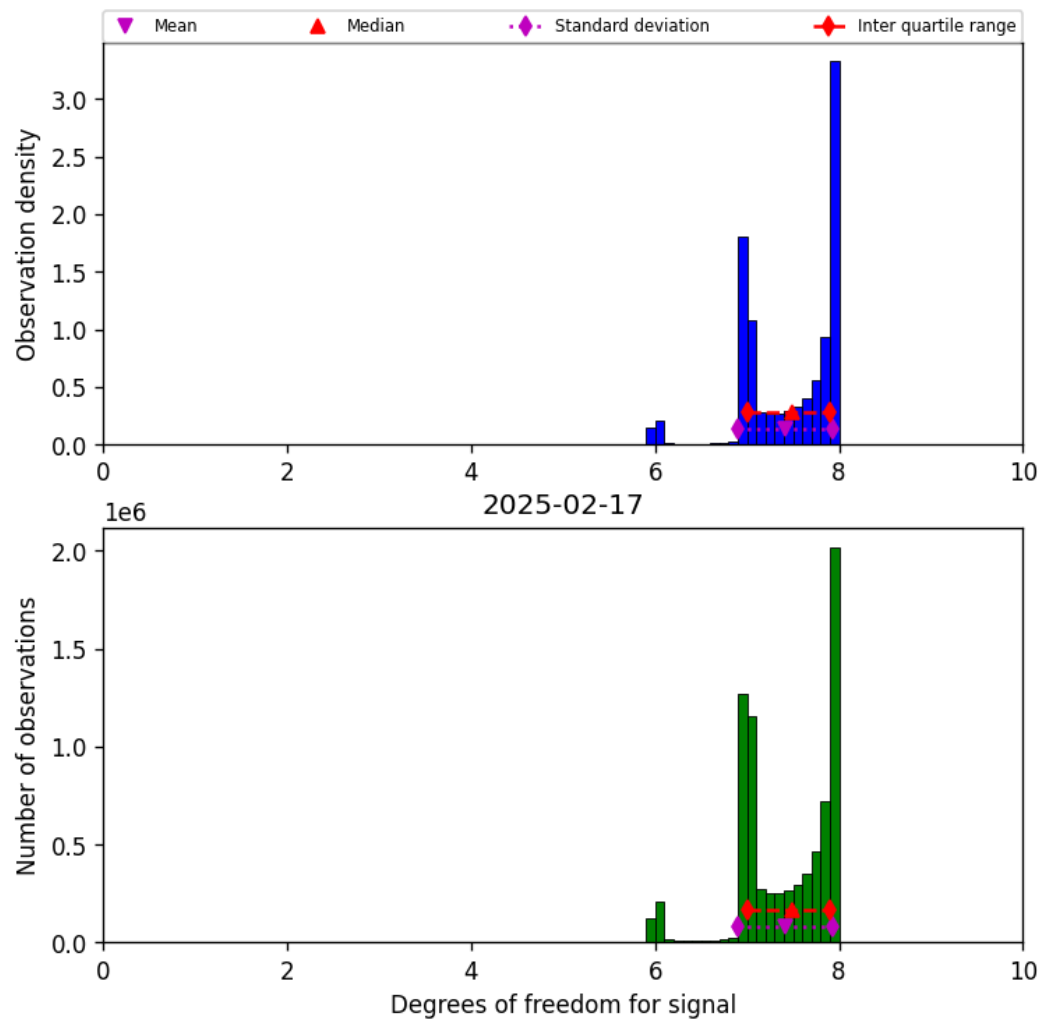
Figure 23: Histogram of “Degrees of freedom for signal” for 2025-02-16 to 2025-02-18
