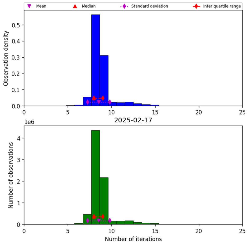
Figure 24: Histogram of “Number of iterations” for 2025-02-16 to 2025-02-18
