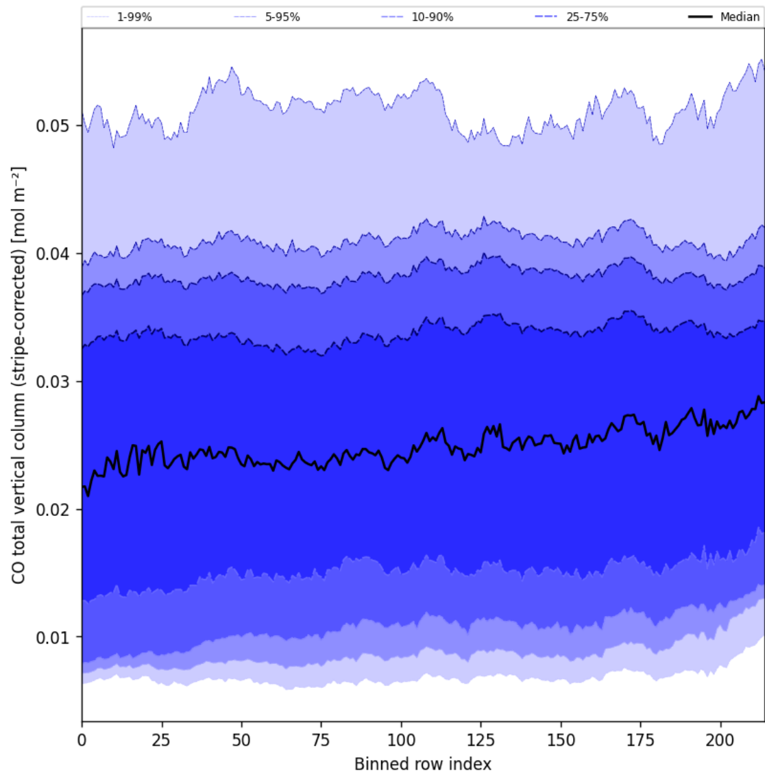
Figure 27: Along track statistics of “CO total vertical column (stripe-corrected)” for 2025-02-16 to 2025-02-18
