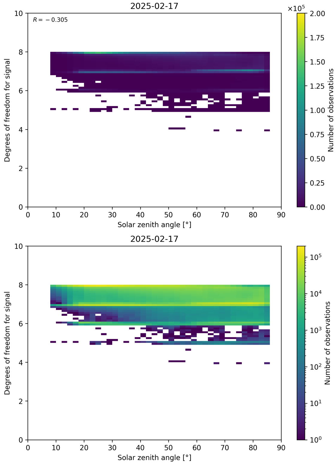
Figure 65: Scatter density plot of “Solar zenith angle” against “Degrees of freedom for signal” for 2025-02-16 to 2025-02-18.
