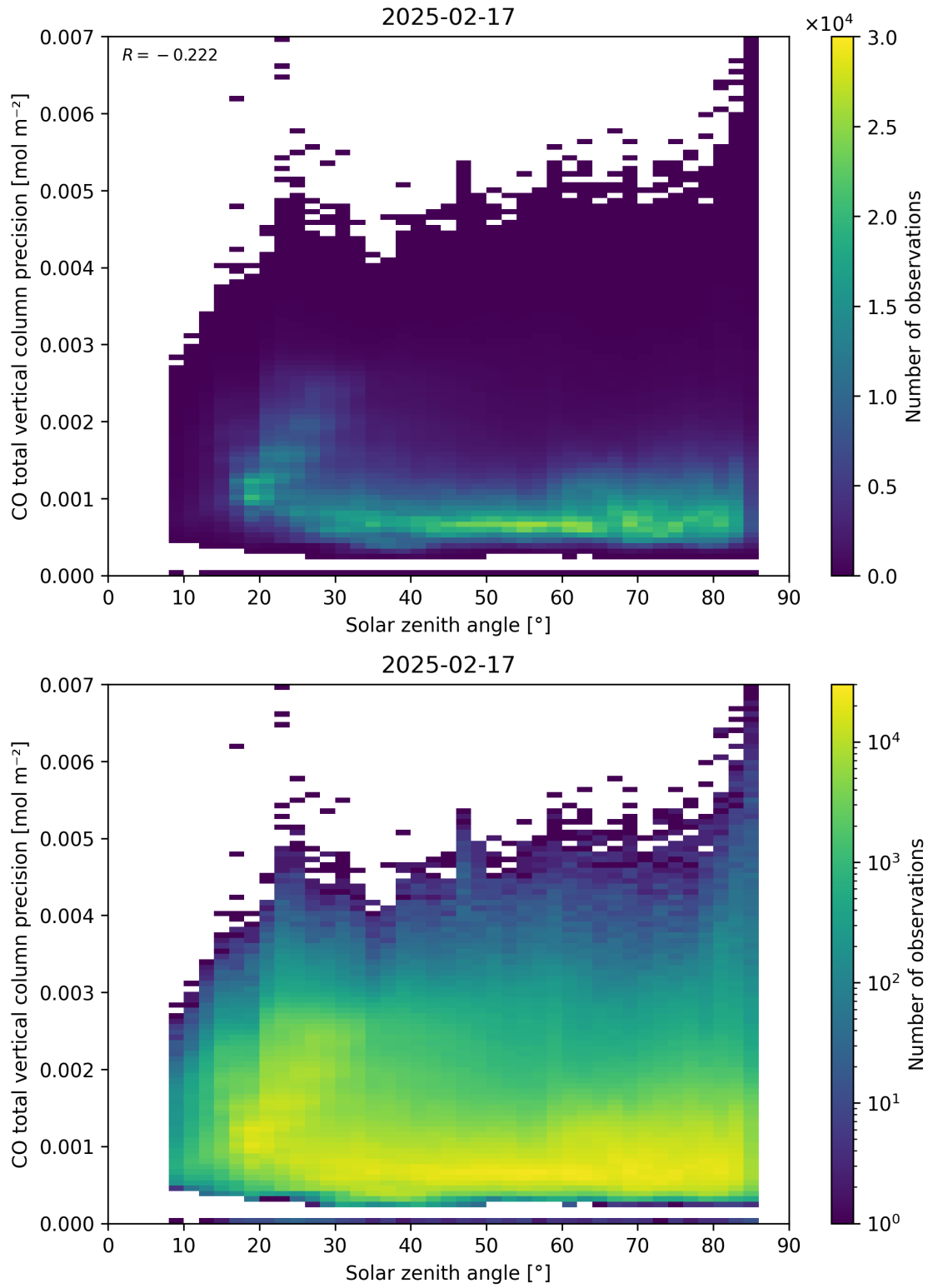
Figure 63: Scatter density plot of “Solar zenith angle” against “CO total vertical column precision” for 2025-02-16 to 2025-02-18.
