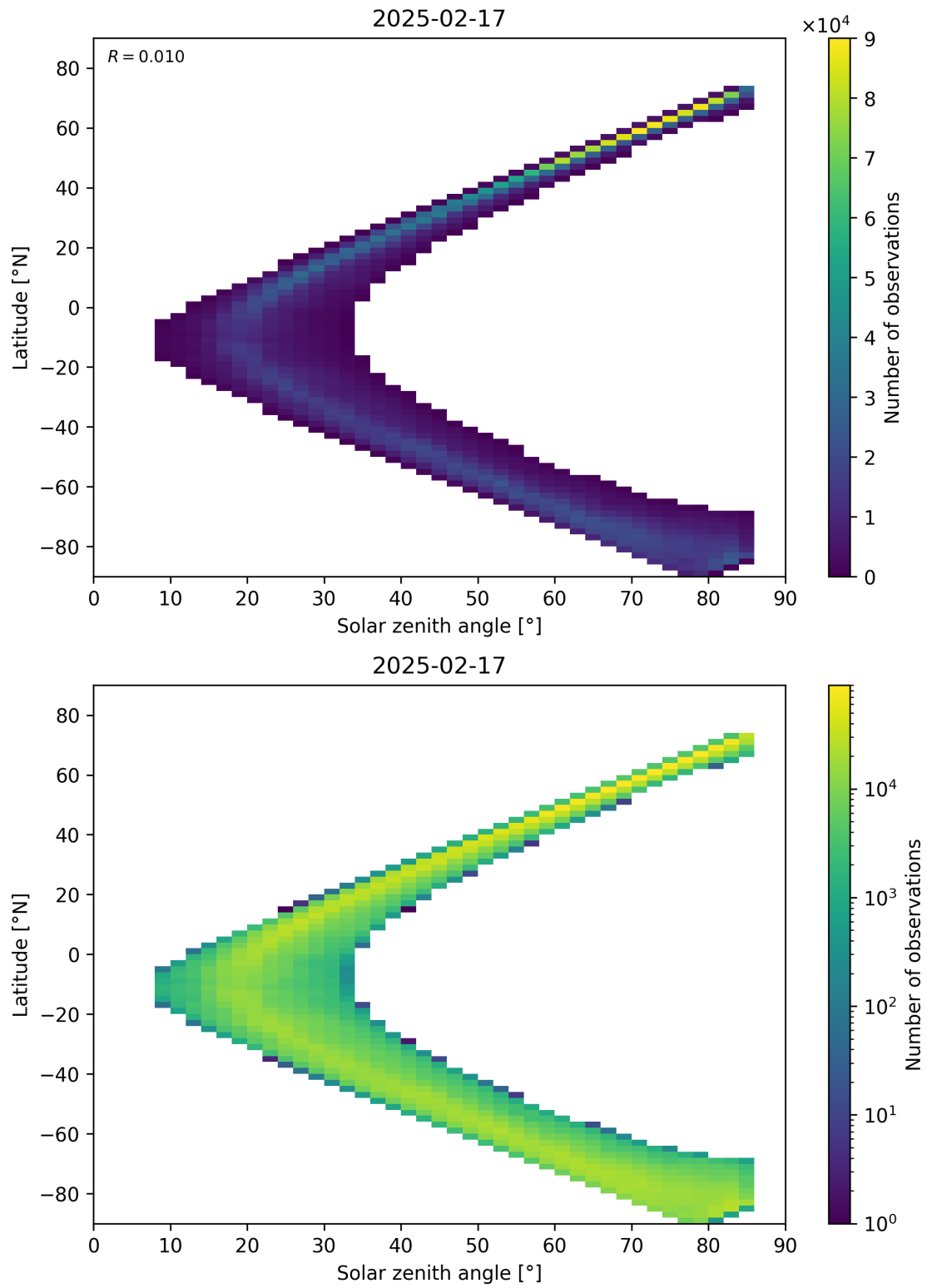
Figure 66: Scatter density plot of “Solar zenith angle” against “Latitude” for 2025-02-16 to 2025-02-18.
