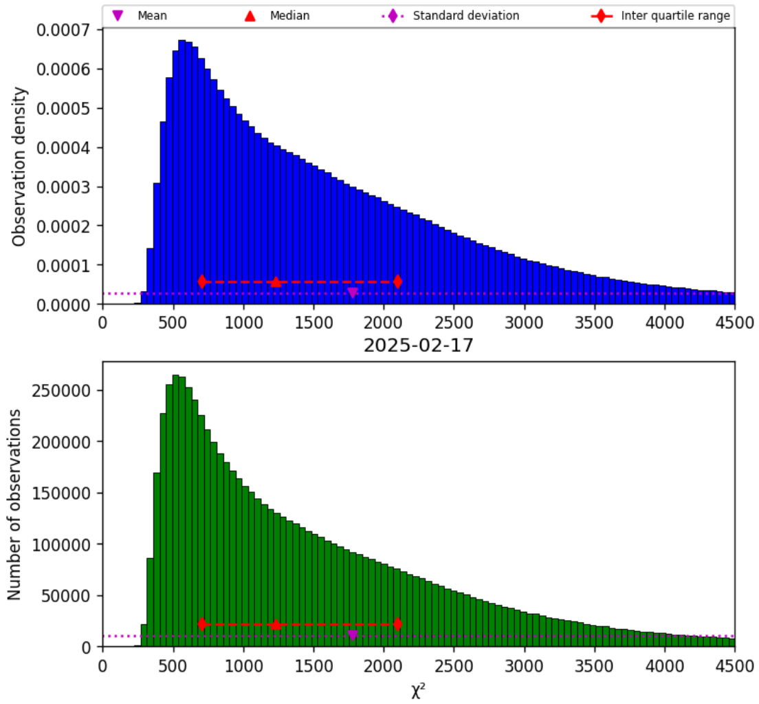
Figure 22: Histogram of “ \chi^2 ” for 2025-02-16 to 2025-02-18
