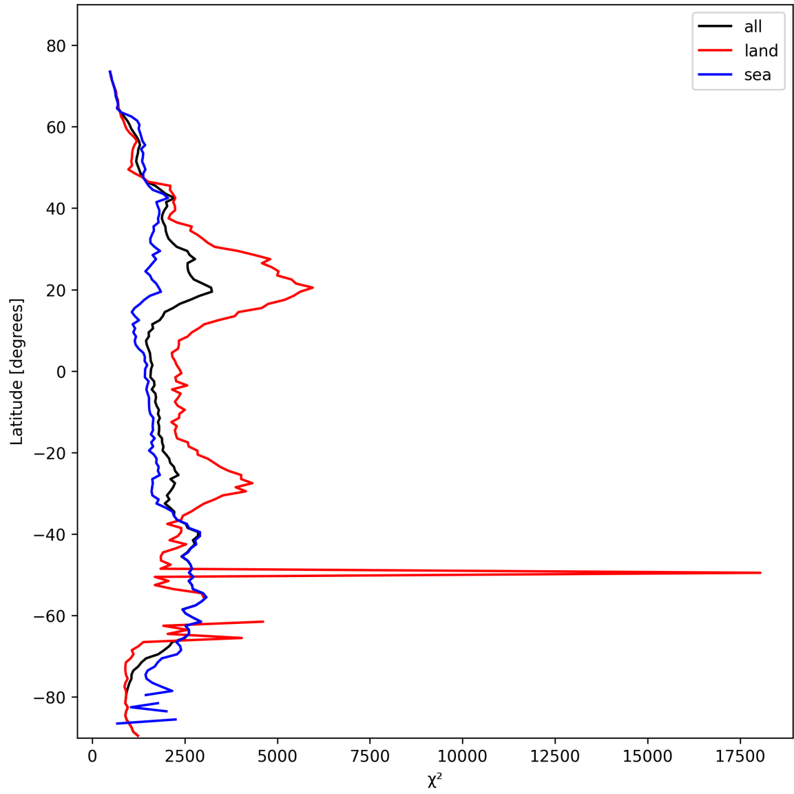
Figure 14: Zonal average of “ \chi^2 ” for 2025-02-16 to 2025-02-18.
