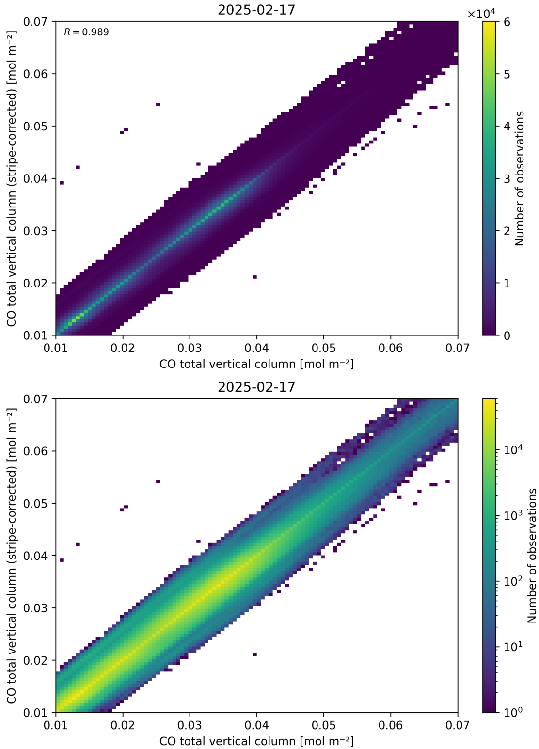
Figure 33: Scatter density plot of “CO total vertical column” against “CO total vertical column (stripe-corrected)” for 2025-02-16 to 2025-02-18.
