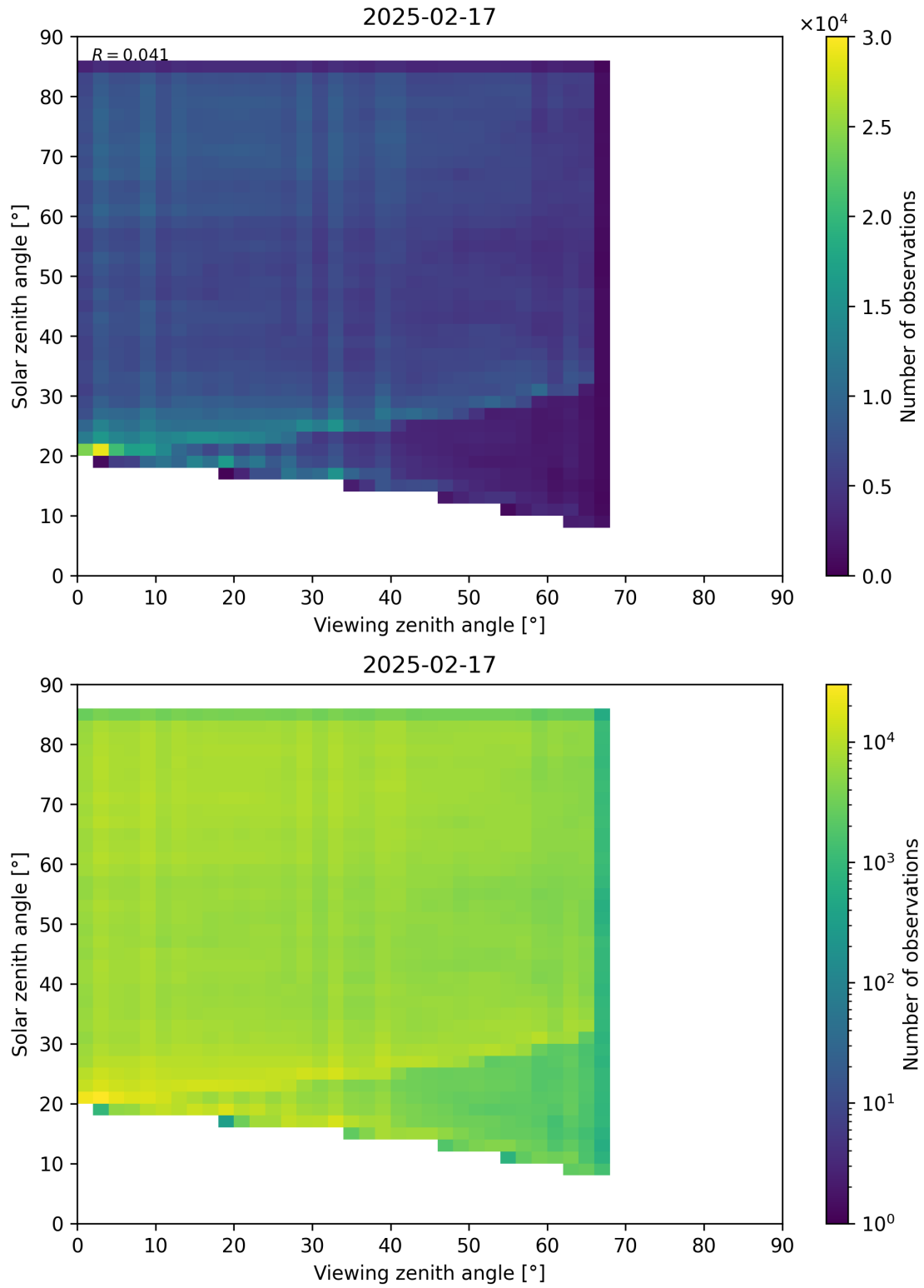
Figure 77: Scatter density plot of “Viewing zenith angle” against “Solar zenith angle” for 2025-02-16 to 2025-02-18.
