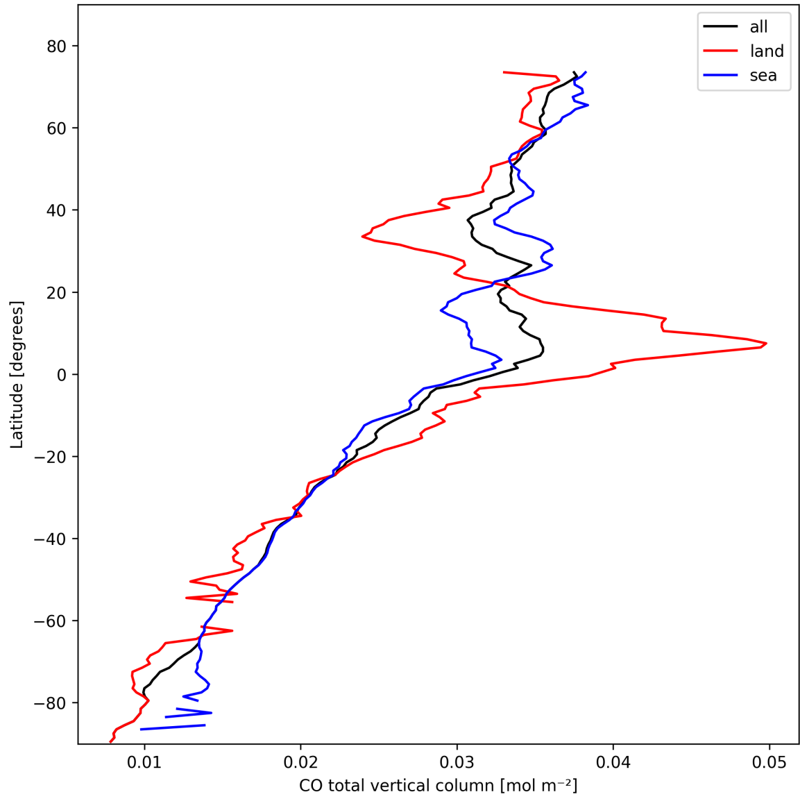
Figure 10: Zonal average of “CO total vertical column” for 2025-02-16 to 2025-02-18.
