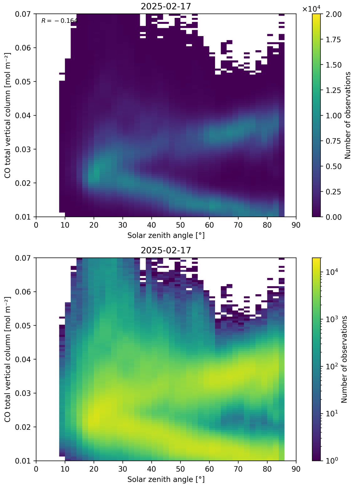
Figure 61: Scatter density plot of “Solar zenith angle” against “CO total vertical column” for 2025-02-16 to 2025-02-18.
