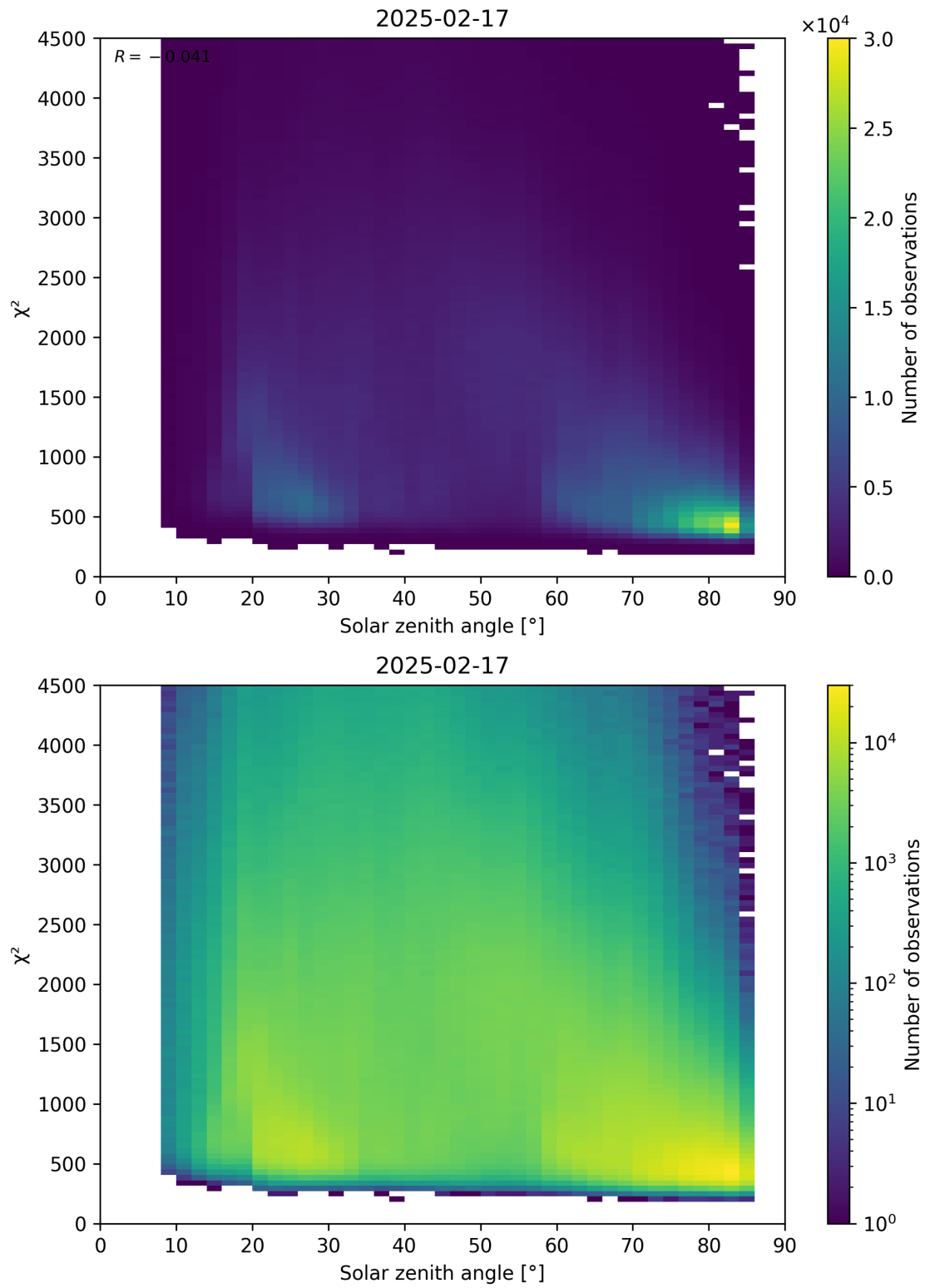
Figure 64: Scatter density plot of “Solar zenith angle” against “ \chi^2 ” for 2025-02-16 to 2025-02-18.
