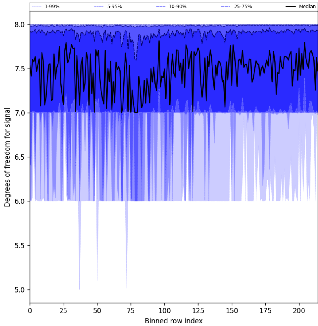
Figure 31: Along track statistics of “Degrees of freedom for signal” for 2025-02-16 to 2025-02-18
