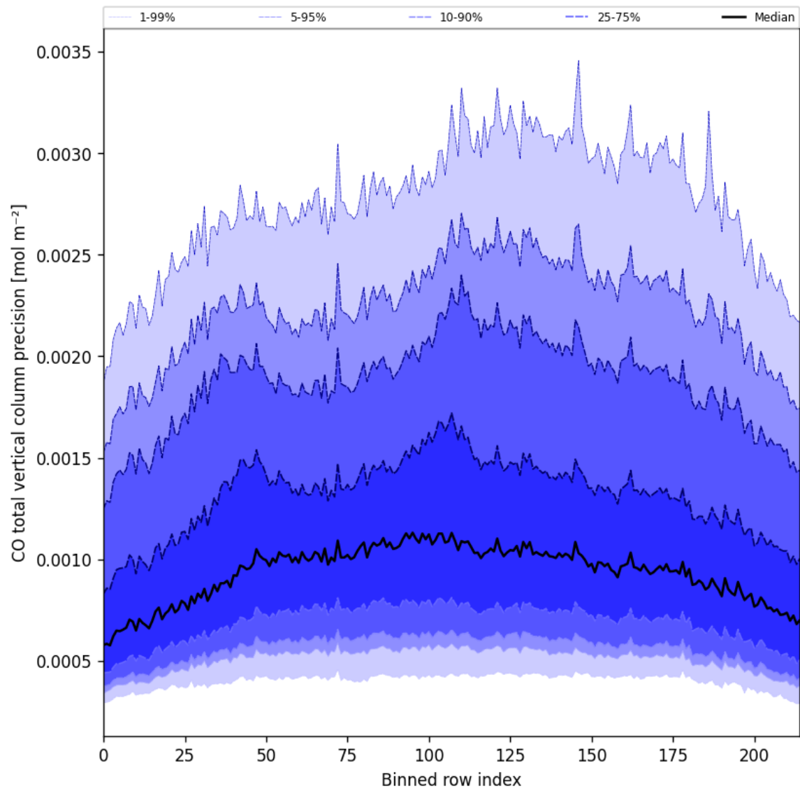
Figure 28: Along track statistics of “CO total vertical column precision” for 2025-02-16 to 2025-02-18
