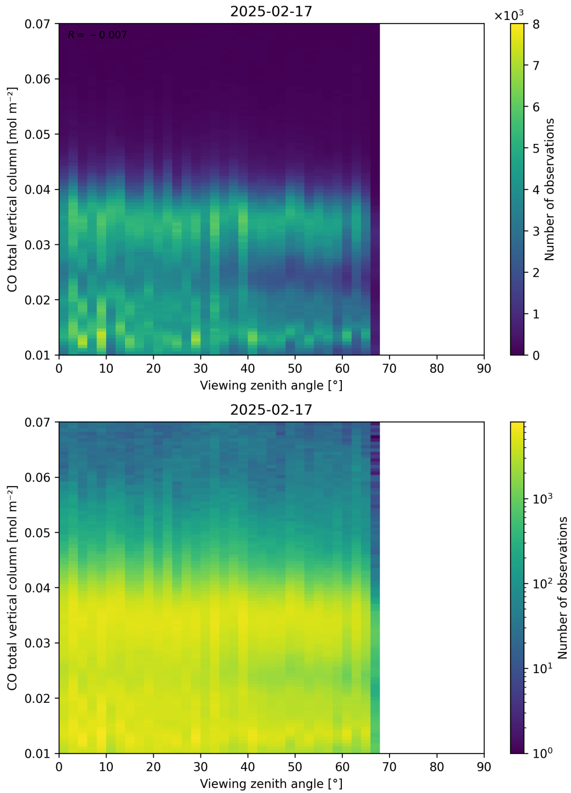
Figure 69: Scatter density plot of “Viewing zenith angle” against “CO total vertical column” for 2025-02-16 to 2025-02-18.
