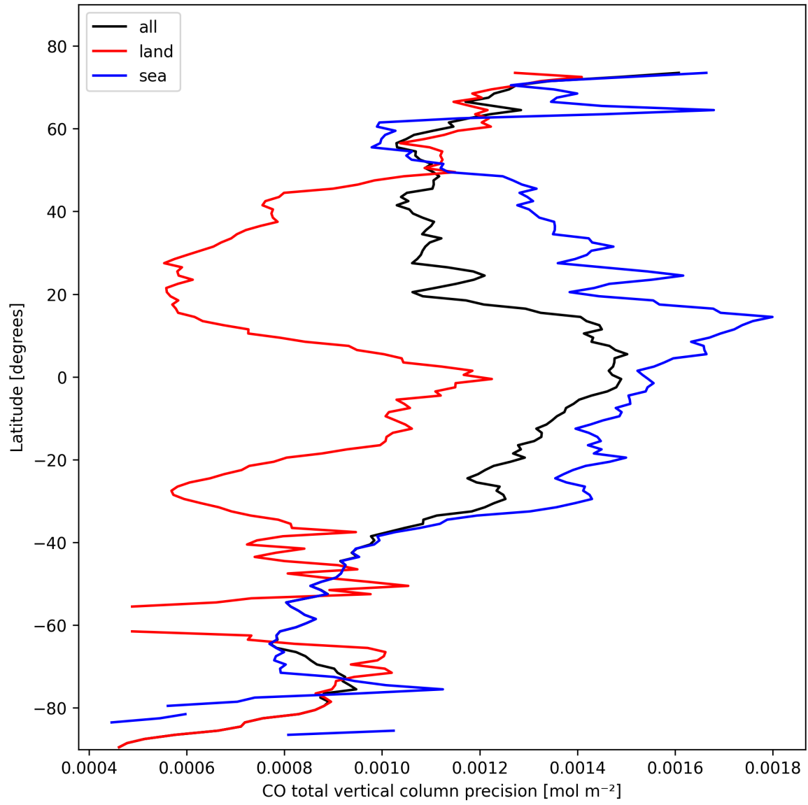
Figure 12: Zonal average of “CO total vertical column precision” for 2025-02-16 to 2025-02-18.
