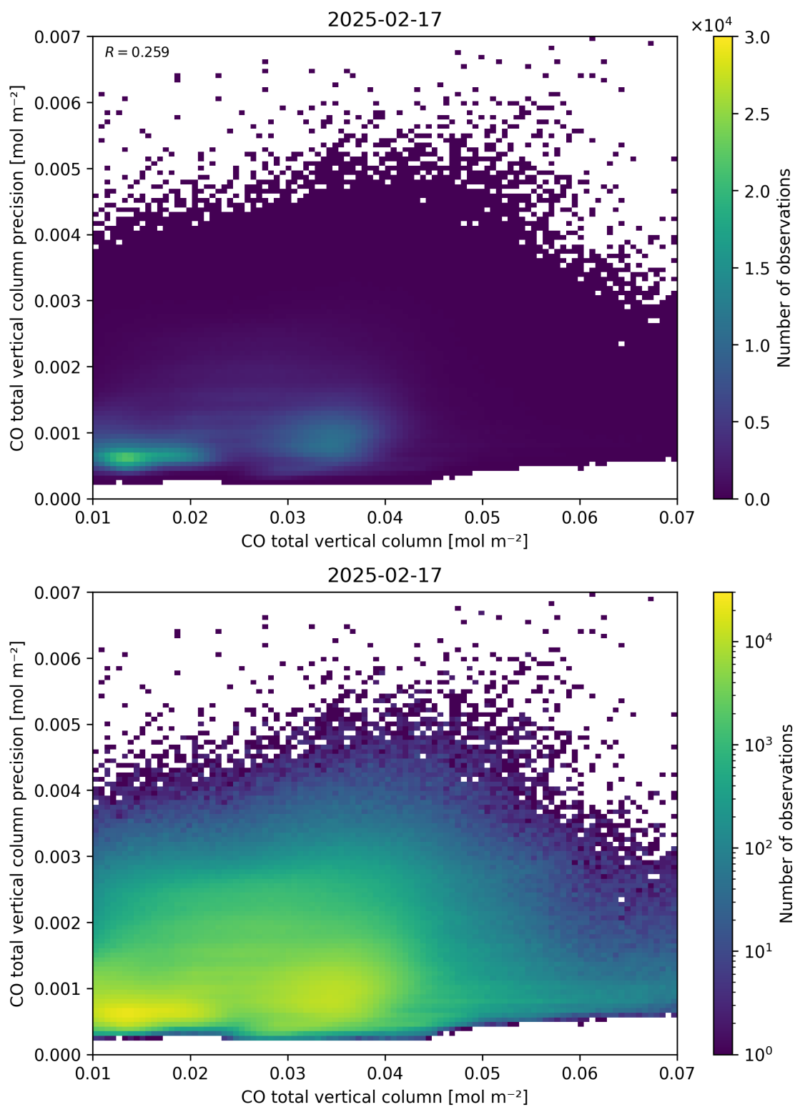
Figure 34: Scatter density plot of “CO total vertical column” against “CO total vertical column precision” for 2025-02-16 to 2025-02-18.
