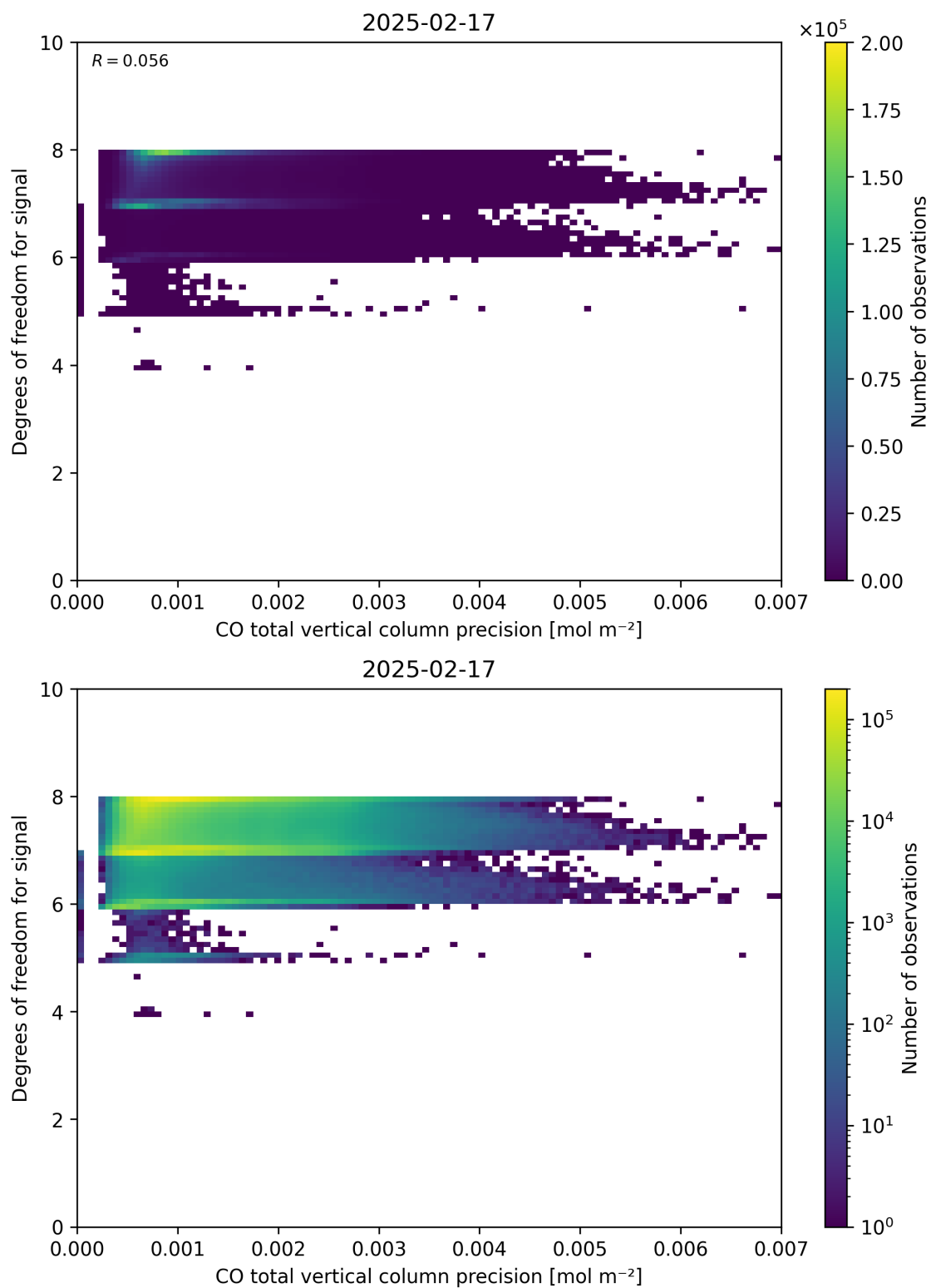
Figure 45: Scatter density plot of “CO total vertical column precision” against “Degrees of freedom for signal” for 2025-02-16 to 2025-02-18.
