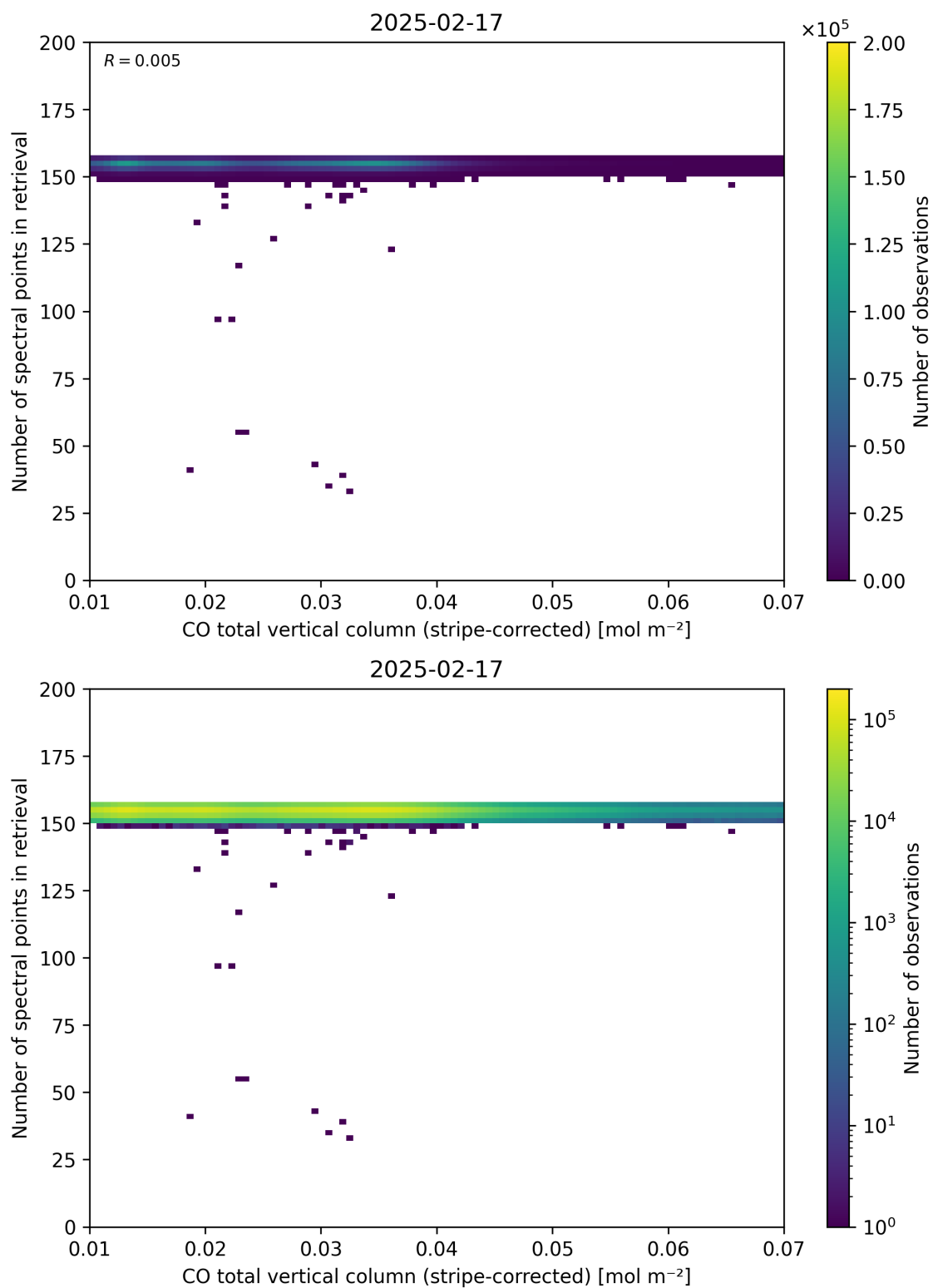
Figure 40: Scatter density plot of “CO total vertical column (stripe-corrected)” against “Number of spectral points in retrieval” for 2025-02-16 to 2025-02-18.
