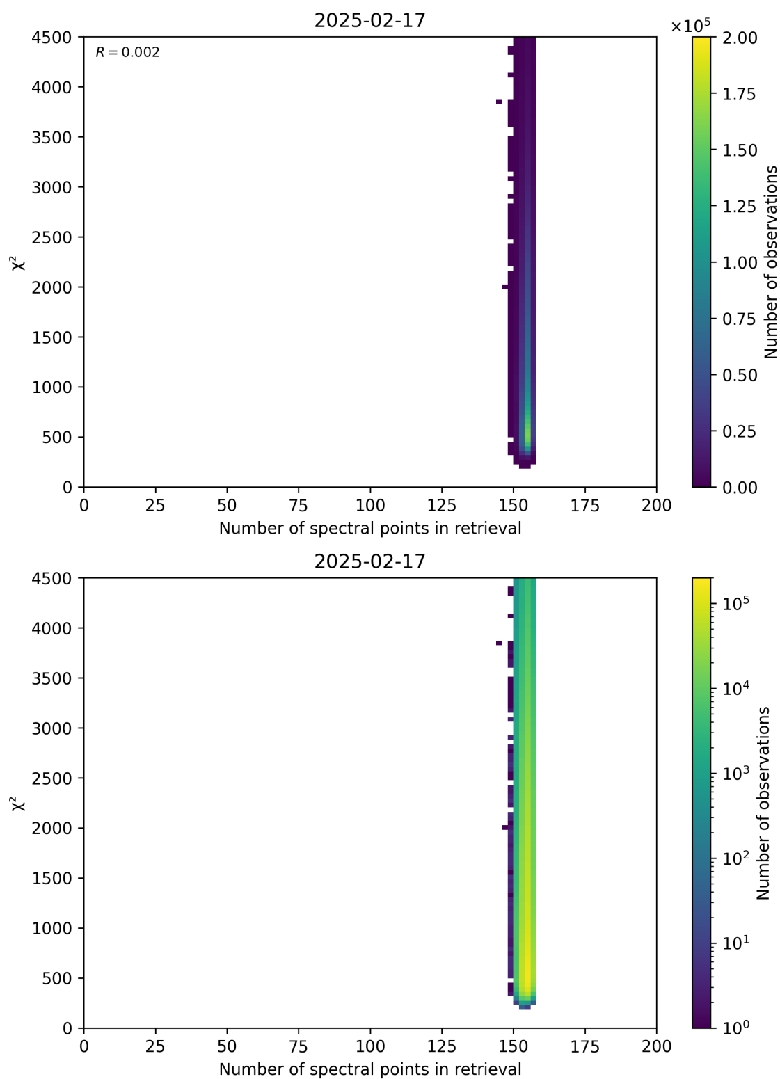
Figure 58: Scatter density plot of “Number of spectral points in retrieval” against “ \chi^2 ” for 2025-02-16 to 2025-02-18.
