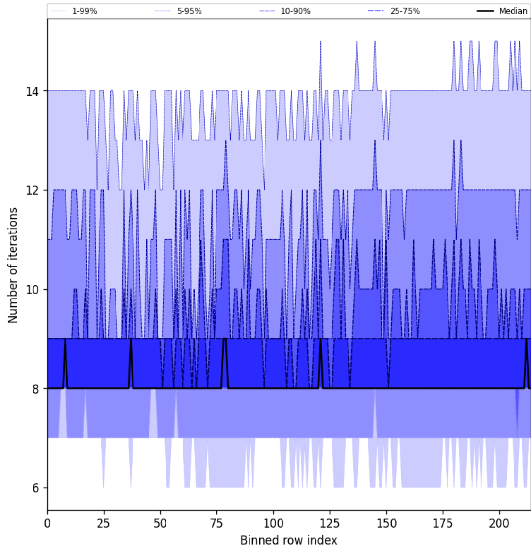
Figure 32: Along track statistics of “Number of iterations” for 2025-02-16 to 2025-02-18
