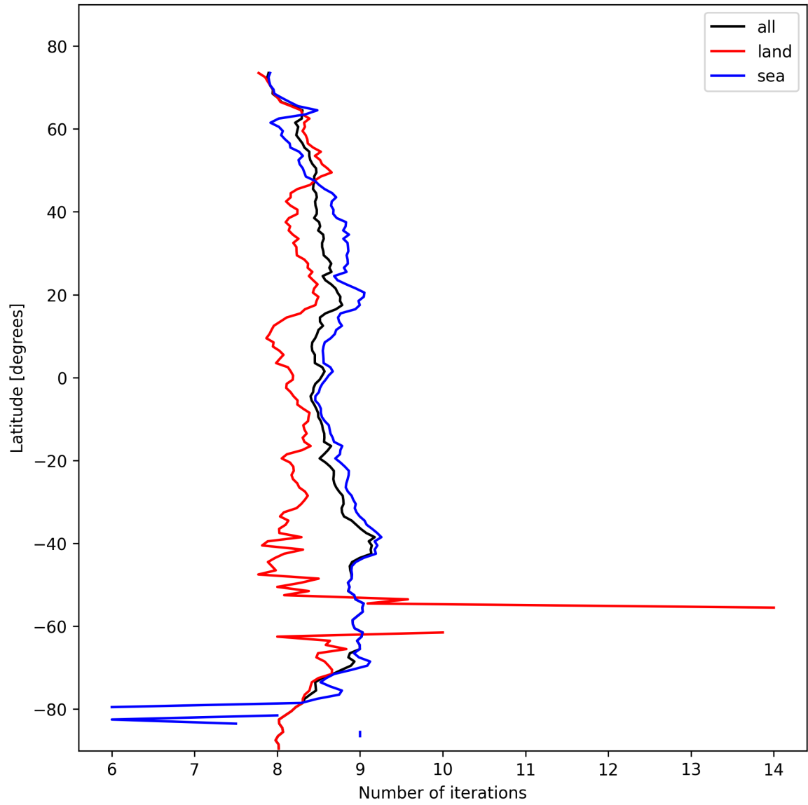
Figure 16: Zonal average of “Number of iterations” for 2025-02-16 to 2025-02-18.
