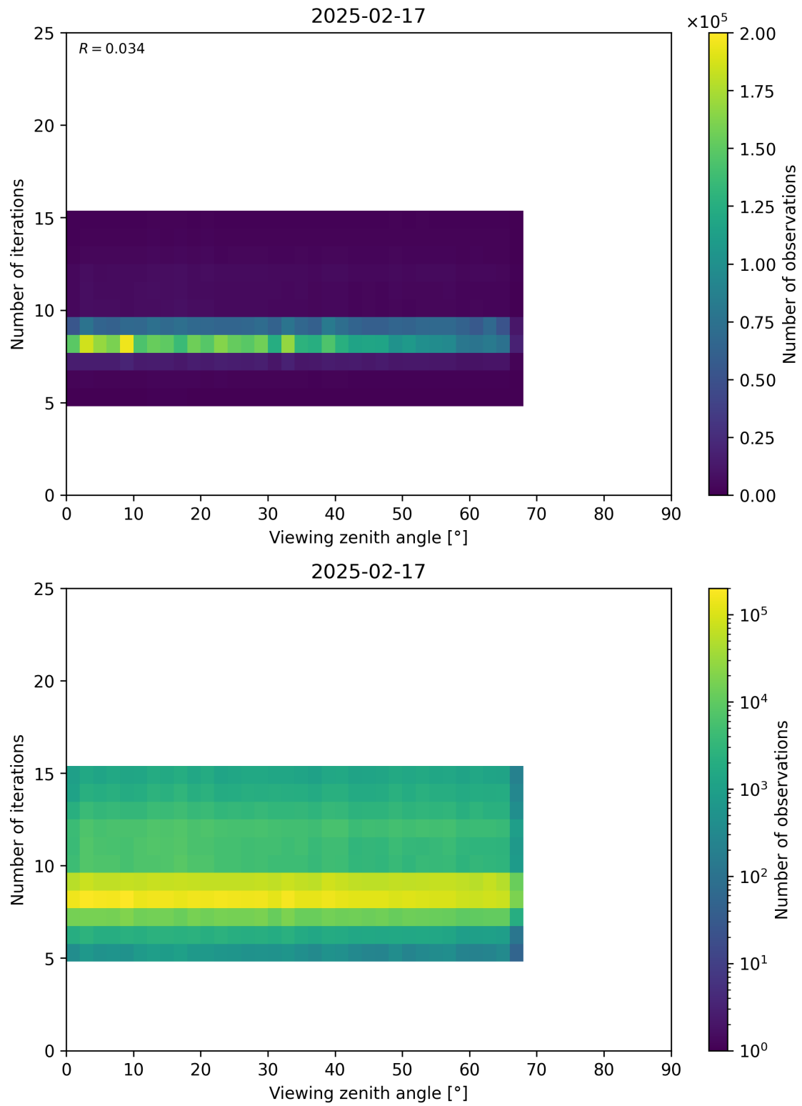
Figure 75: Scatter density plot of “Viewing zenith angle” against “Number of iterations” for 2025-02-16 to 2025-02-18.
