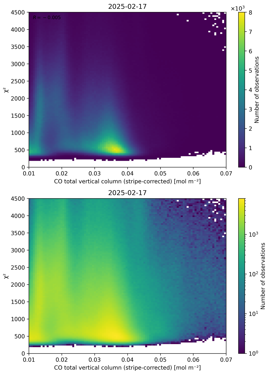
Figure 37: Scatter density plot of “CO total vertical column (stripe-corrected)” against “ \chi^2 ” for 2025-02-16 to 2025-02-18.
