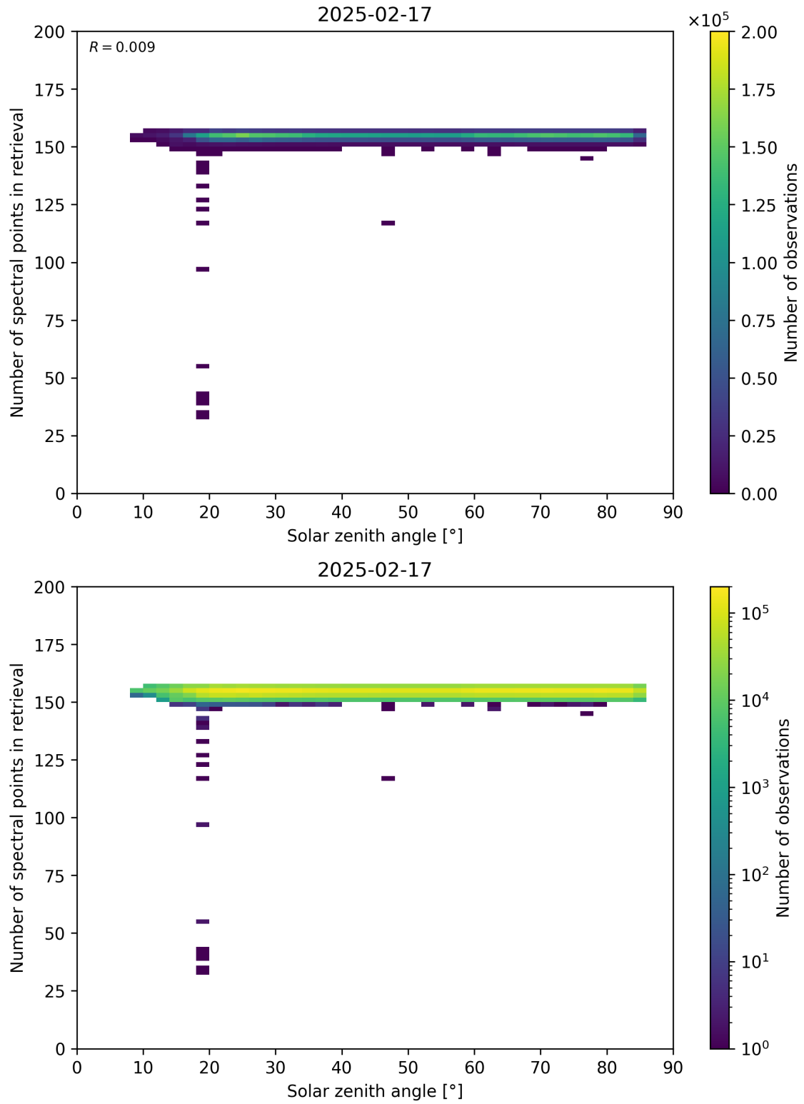
Figure 68: Scatter density plot of “Solar zenith angle” against “Number of spectral points in retrieval” for 2025-02-16 to 2025-02-18.
