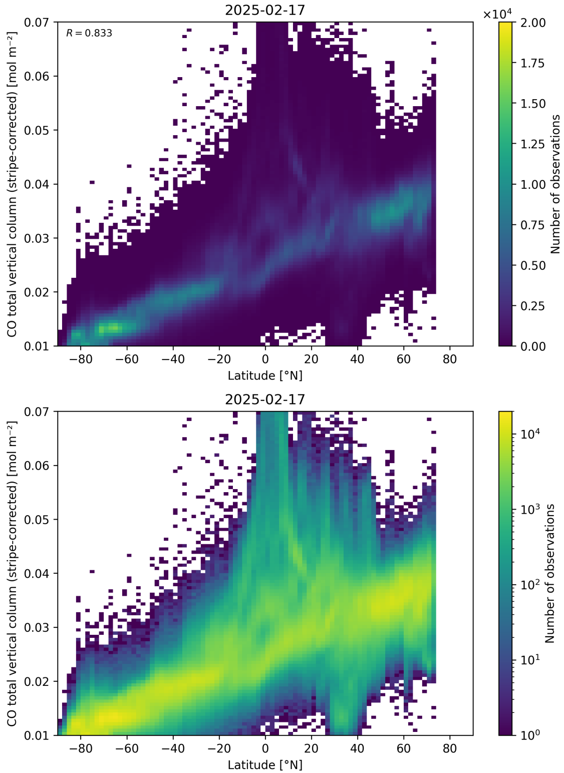
Figure 52: Scatter density plot of “Latitude” against “CO total vertical column (stripe-corrected)” for 2025-02-16 to 2025-02-18.
