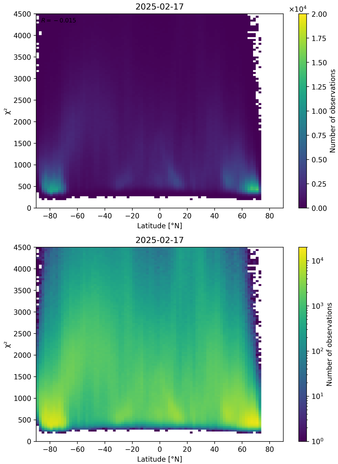
Figure 54: Scatter density plot of “Latitude” against “ \chi^2 ” for 2025-02-16 to 2025-02-18.
