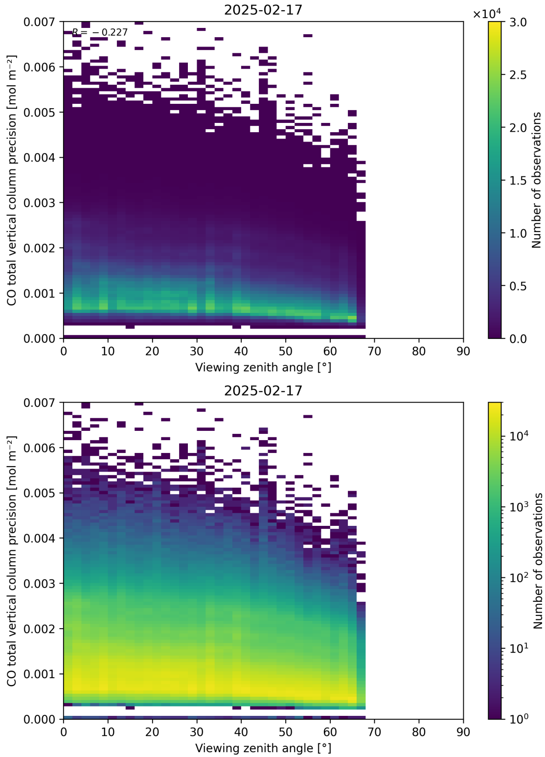
Figure 71: Scatter density plot of “Viewing zenith angle” against “CO total vertical column precision” for 2025-02-16 to 2025-02-18.
