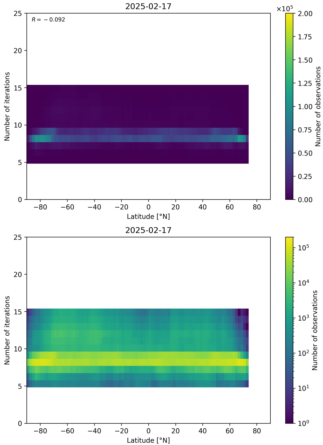
Figure 56: Scatter density plot of “Latitude” against “Number of iterations” for 2025-02-16 to 2025-02-18.
