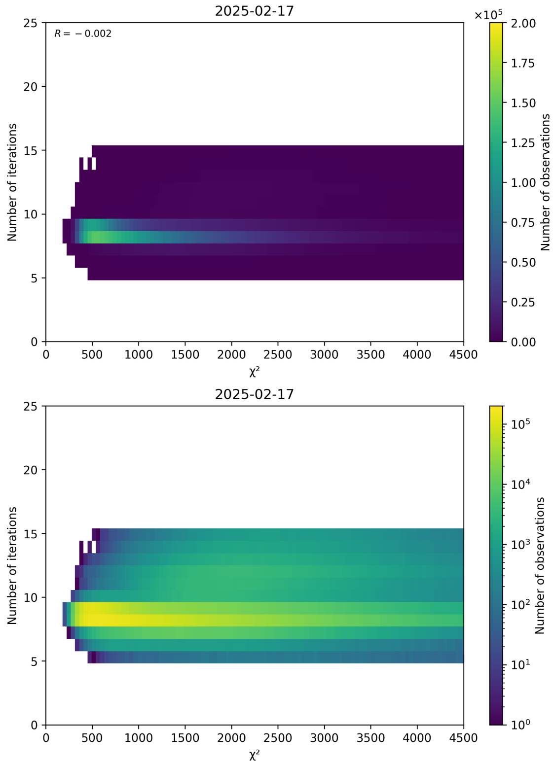
Figure 49: Scatter density plot of “ \chi^2 ” against “Number of iterations” for 2025-02-16 to 2025-02-18.
