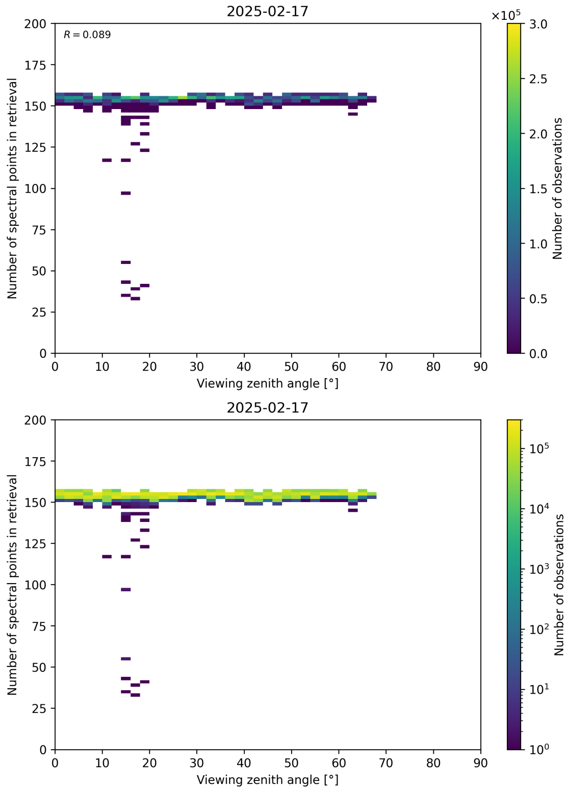
Figure 76: Scatter density plot of “Viewing zenith angle” against “Number of spectral points in retrieval” for 2025-02-16 to 2025-02-18.
