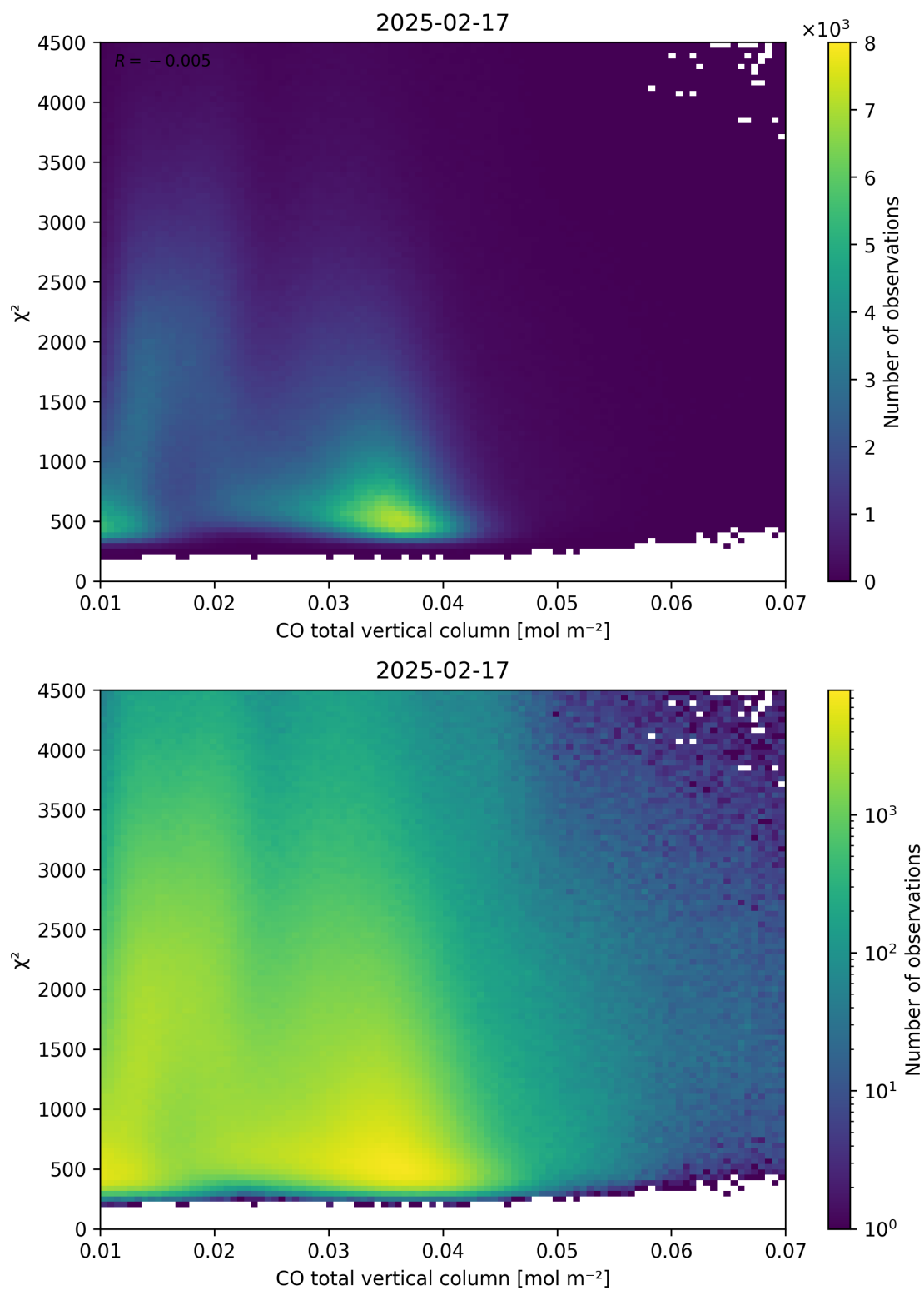
Figure 35: Scatter density plot of “CO total vertical column” against “ \chi^2 ” for 2025-02-16 to 2025-02-18.
