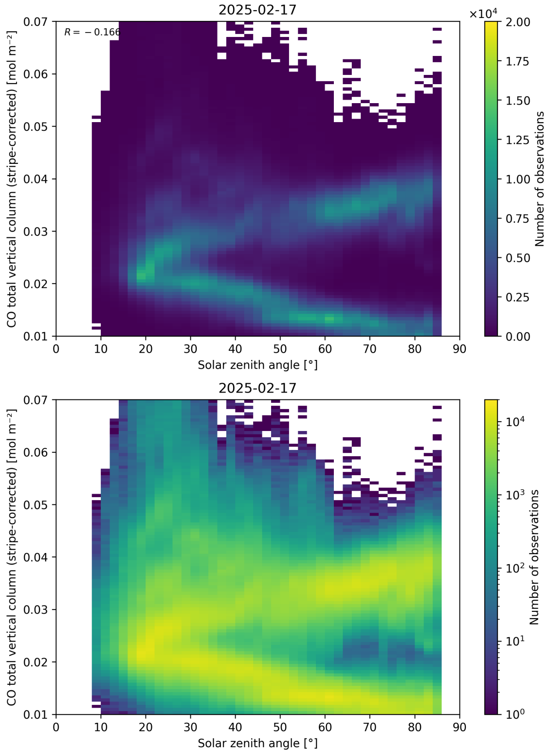
Figure 62: Scatter density plot of “Solar zenith angle” against “CO total vertical column (stripe-corrected)” for 2025-02-16 to 2025-02-18.
