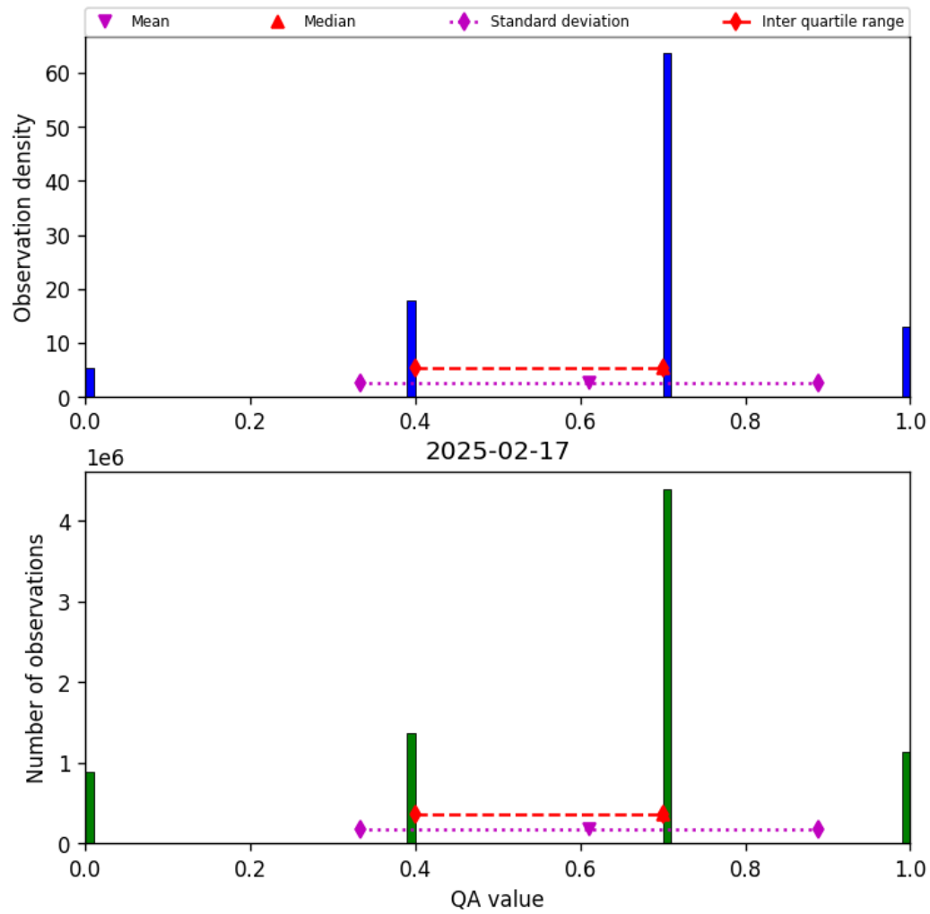
Figure 17: Histogram of “QA value” for 2025-02-16 to 2025-02-18
