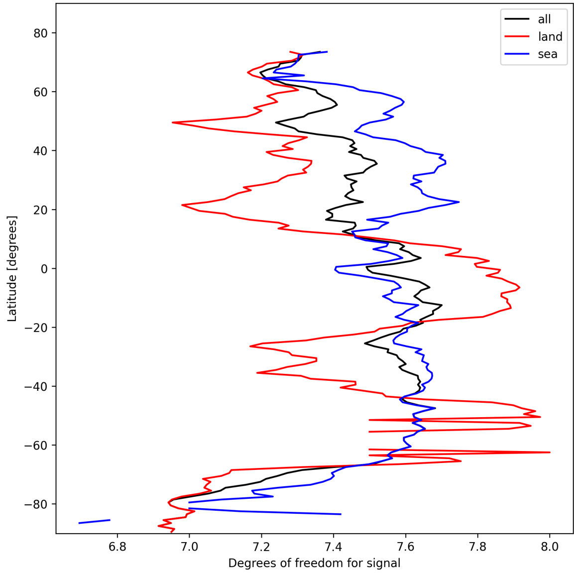
Figure 15: Zonal average of “Degrees of freedom for signal” for 2025-02-16 to 2025-02-18.
