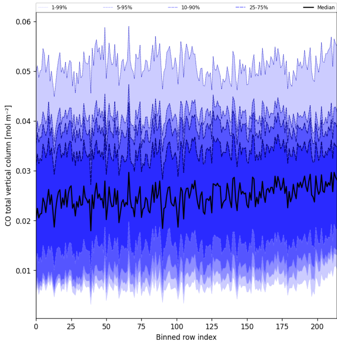
Figure 26: Along track statistics of “CO total vertical column” for 2025-02-16 to 2025-02-18
