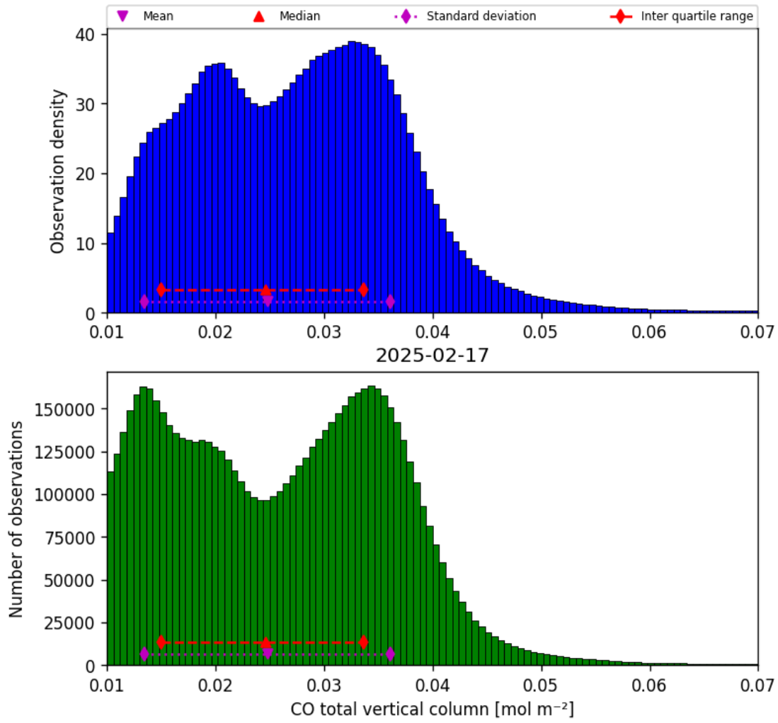
Figure 18: Histogram of “CO total vertical column” for 2025-02-16 to 2025-02-18
