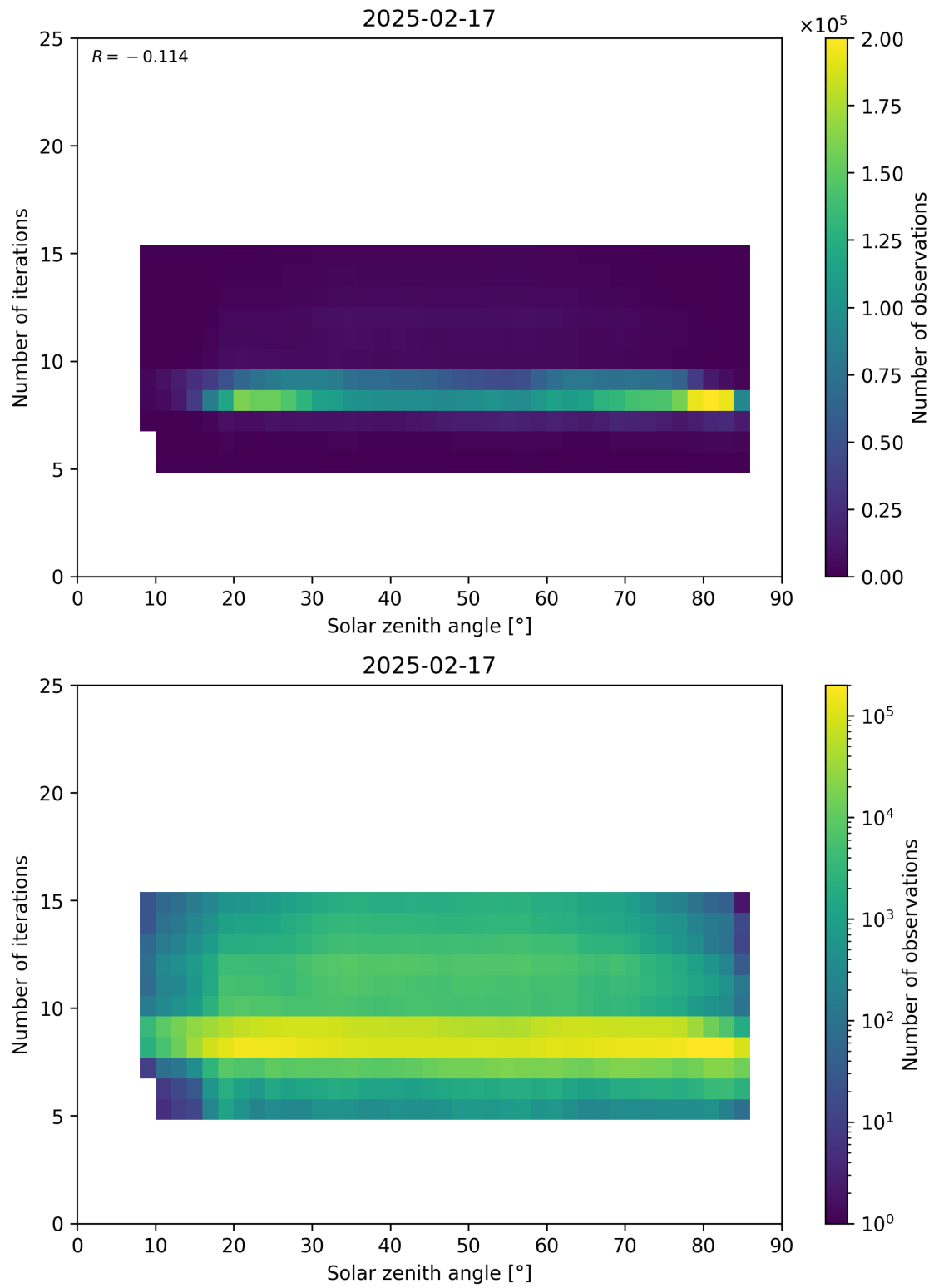
Figure 67: Scatter density plot of “Solar zenith angle” against “Number of iterations” for 2025-02-16 to 2025-02-18.
