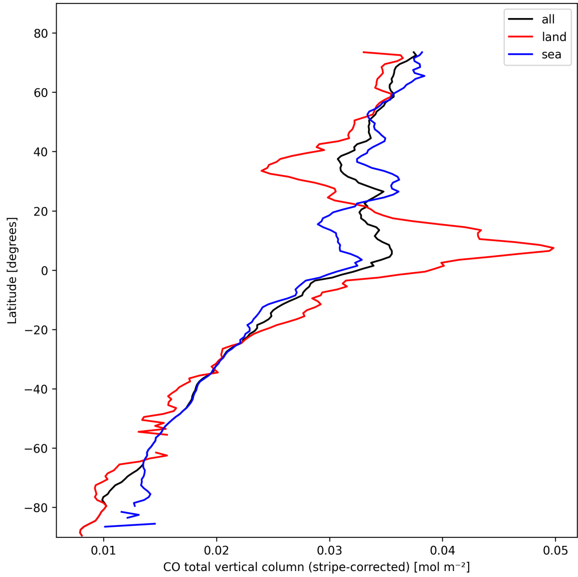
Figure 11: Zonal average of “CO total vertical column (stripe-corrected)” for 2025-02-16 to 2025-02-18.
