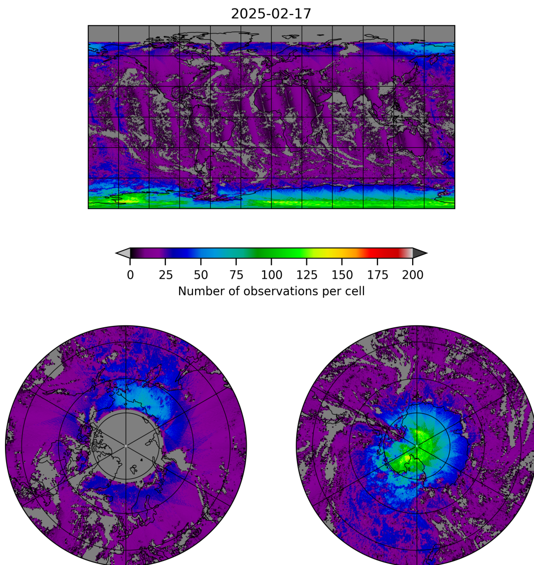
Figure 8: Map of the number of observations for 2025-02-16 to 2025-02-18
