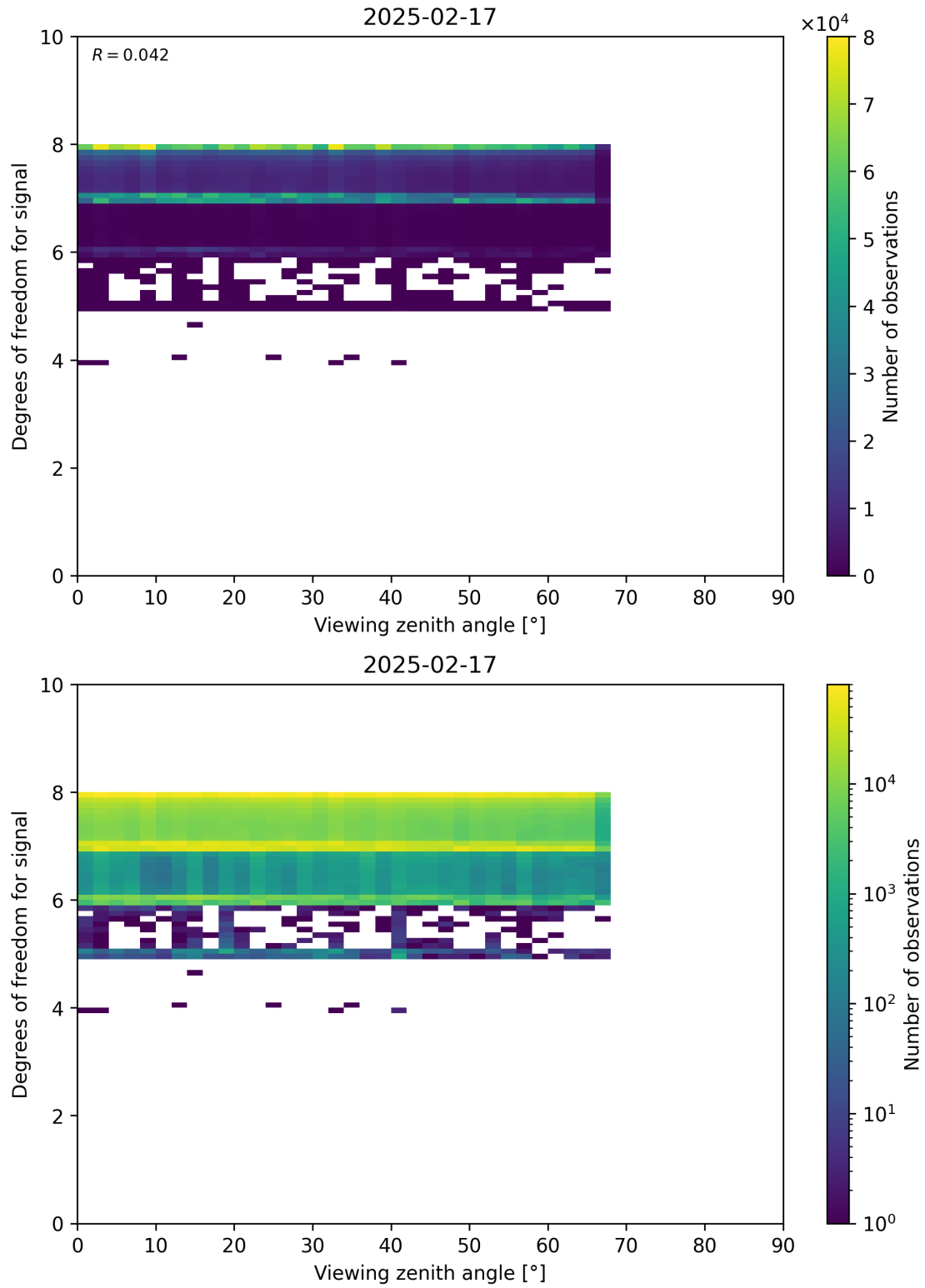
Figure 73: Scatter density plot of “Viewing zenith angle” against “Degrees of freedom for signal” for 2025-02-16 to 2025-02-18.
