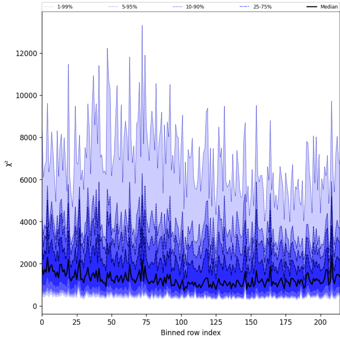
Figure 30: Along track statistics of “ \chi^2 ” for 2025-02-16 to 2025-02-18
