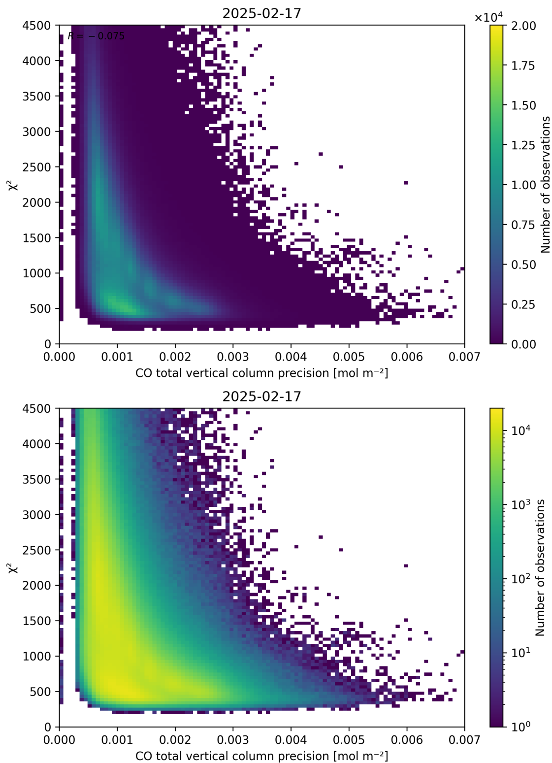
Figure 44: Scatter density plot of “CO total vertical column precision” against “ \chi^2 ” for 2025-02-16 to 2025-02-18.
