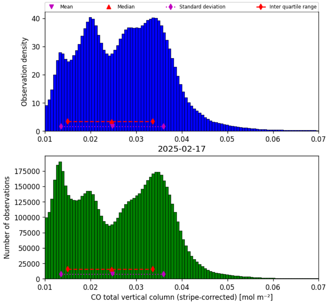
Figure 19: Histogram of “CO total vertical column (stripe-corrected)” for 2025-02-16 to 2025-02-18
