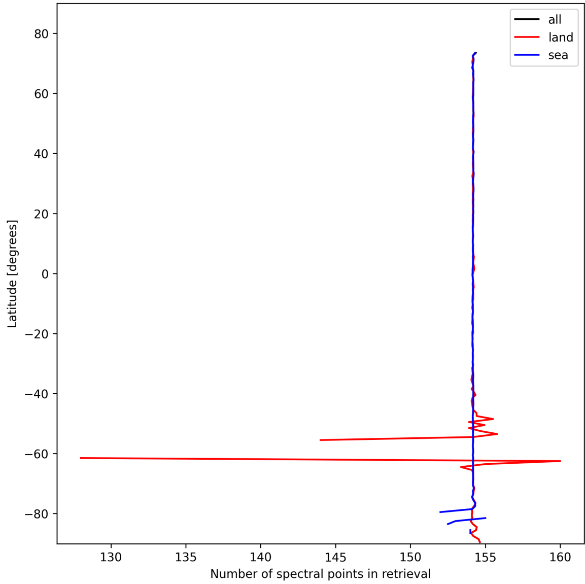
Figure 13: Zonal average of “Number of spectral points in retrieval” for 2025-02-16 to 2025-02-18.
