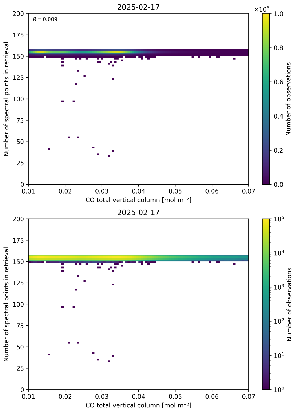
Figure 43: Scatter density plot of “CO total vertical column” against “Number of spectral points in retrieval” for 2025-02-16 to 2025-02-18.
