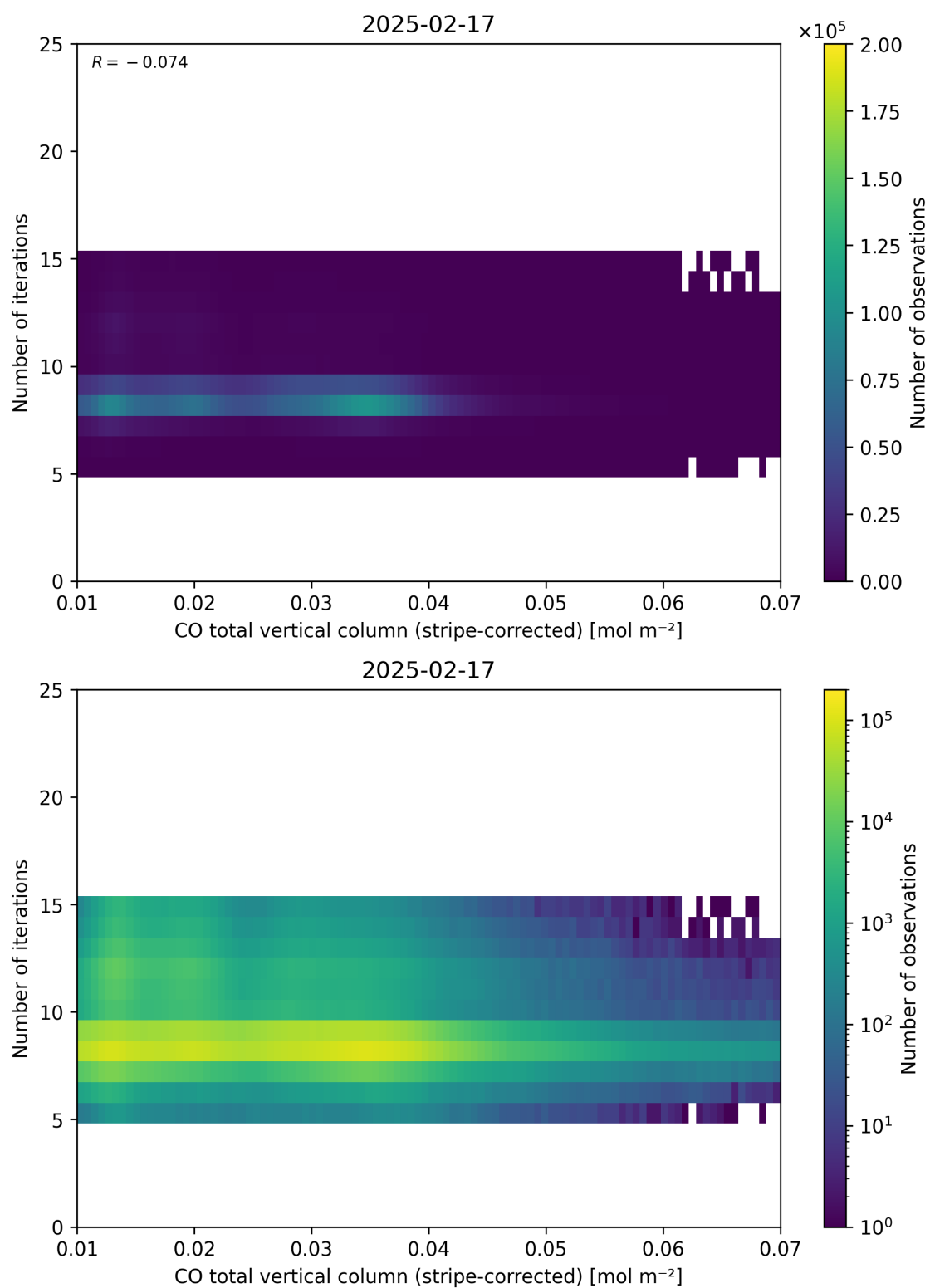
Figure 39: Scatter density plot of “CO total vertical column (stripe-corrected)” against “Number of iterations” for 2025-02-16 to 2025-02-18.
