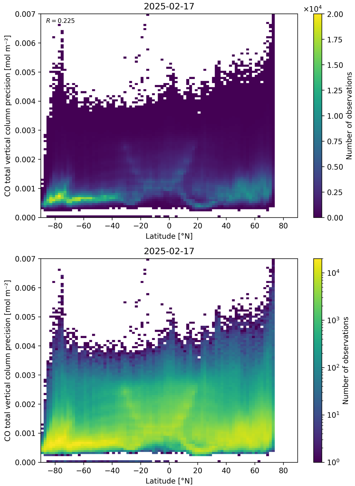
Figure 53: Scatter density plot of “Latitude” against “CO total vertical column precision” for 2025-02-16 to 2025-02-18.
