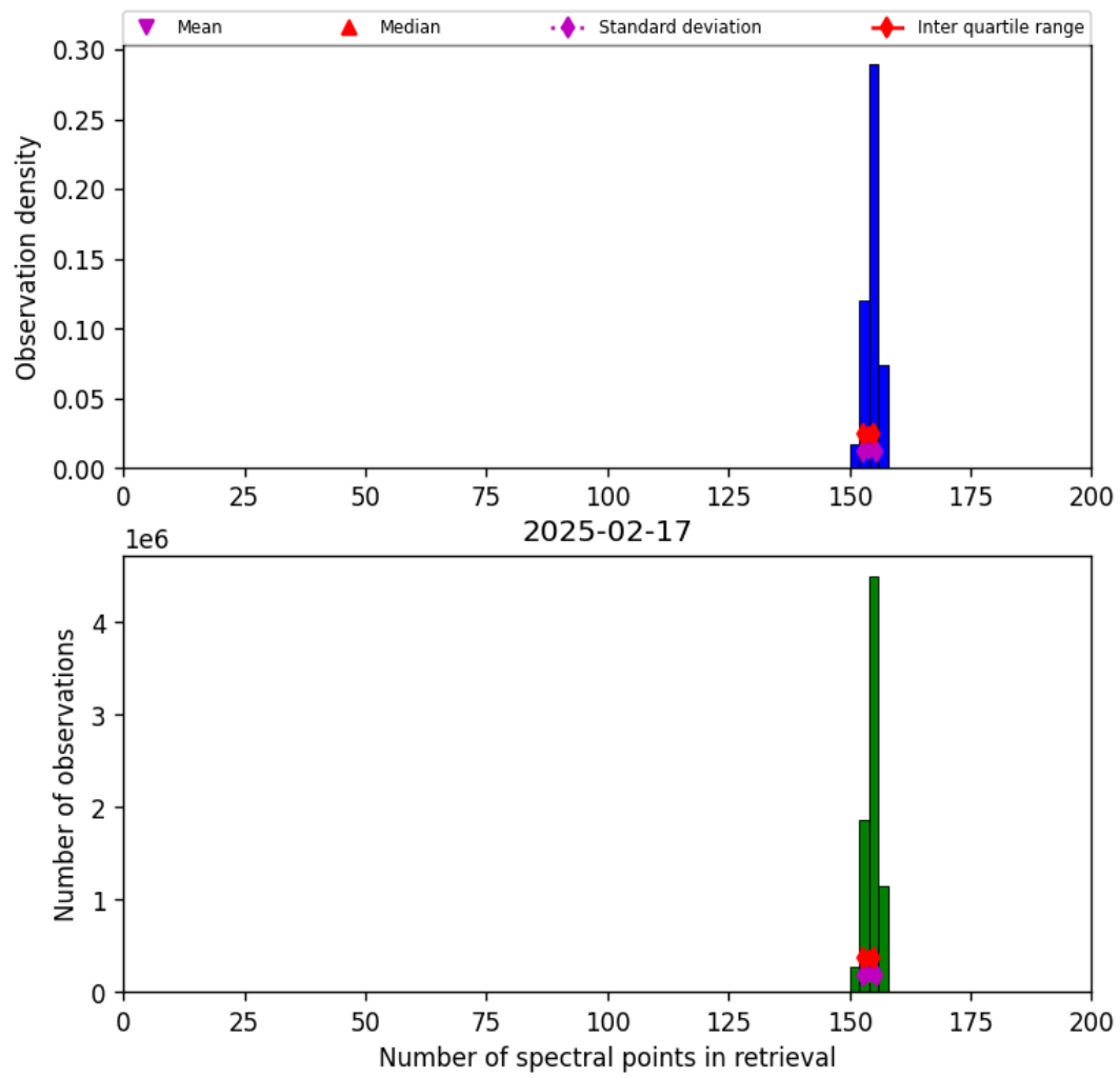
Figure 21: Histogram of “Number of spectral points in retrieval” for 2025-02-16 to 2025-02-18
