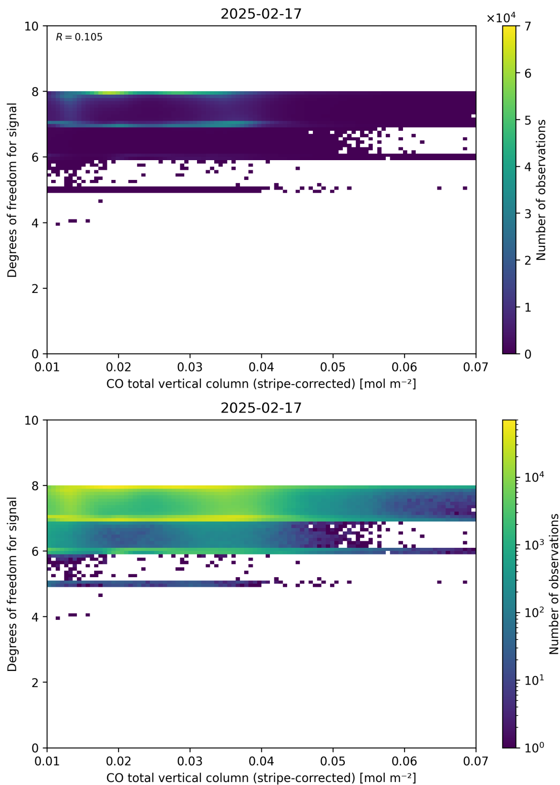
Figure 38: Scatter density plot of “CO total vertical column (stripe-corrected)” against “Degrees of freedom for signal” for 2025-02-16 to 2025-02-18.
