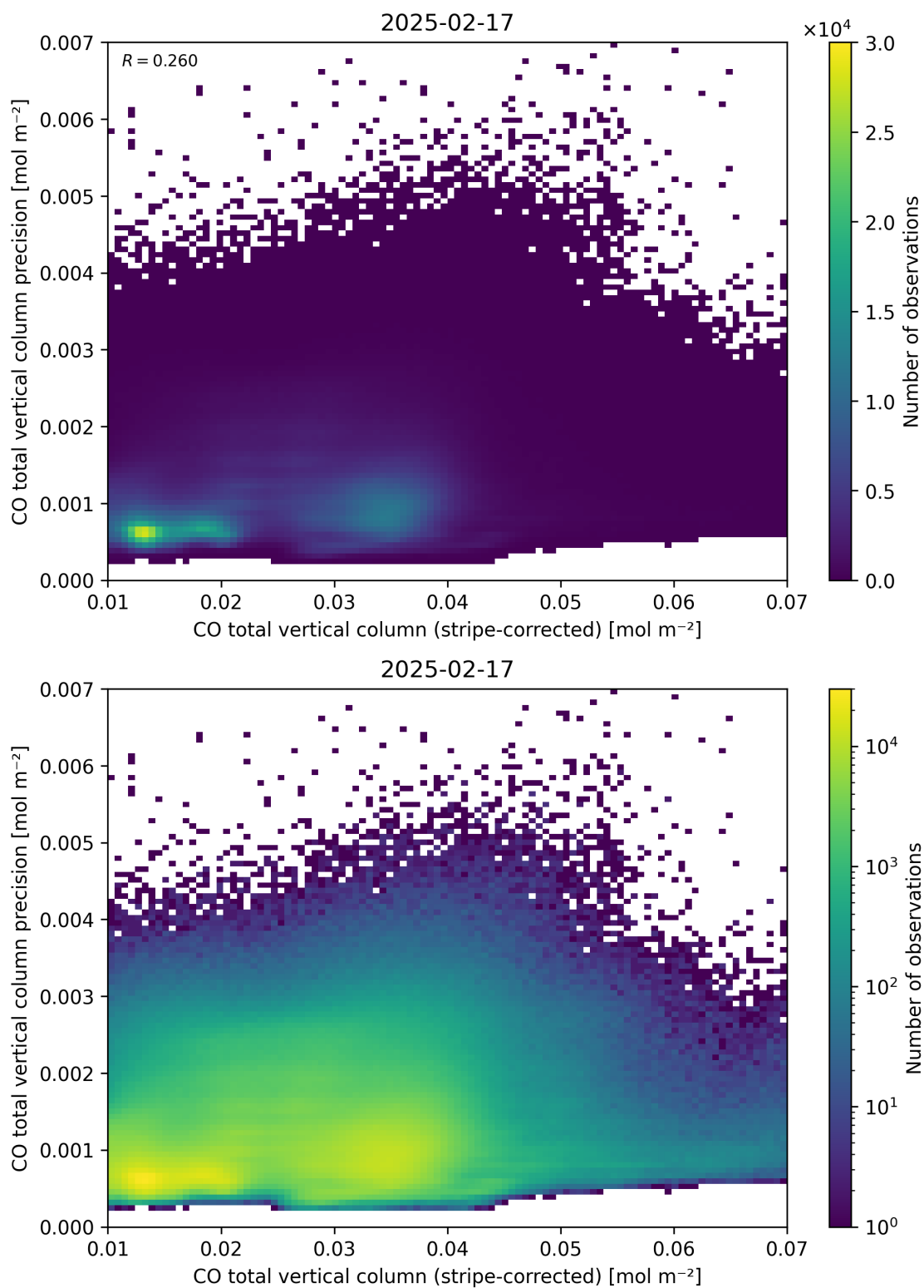
Figure 36: Scatter density plot of “CO total vertical column (stripe-corrected)” against “CO total vertical column precision” for 2025-02-16 to 2025-02-18.
