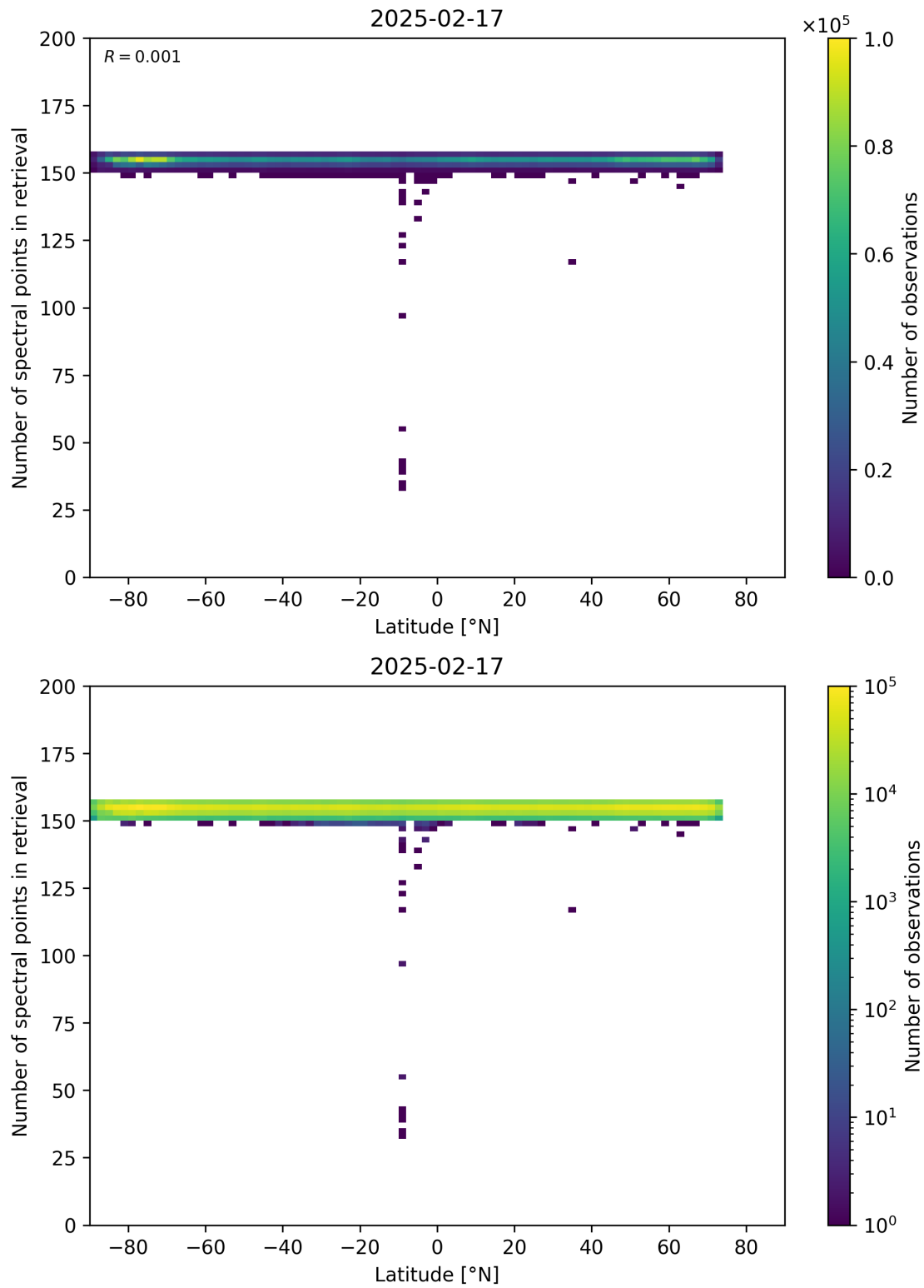
Figure 57: Scatter density plot of “Latitude” against “Number of spectral points in retrieval” for 2025-02-16 to 2025-02-18.
