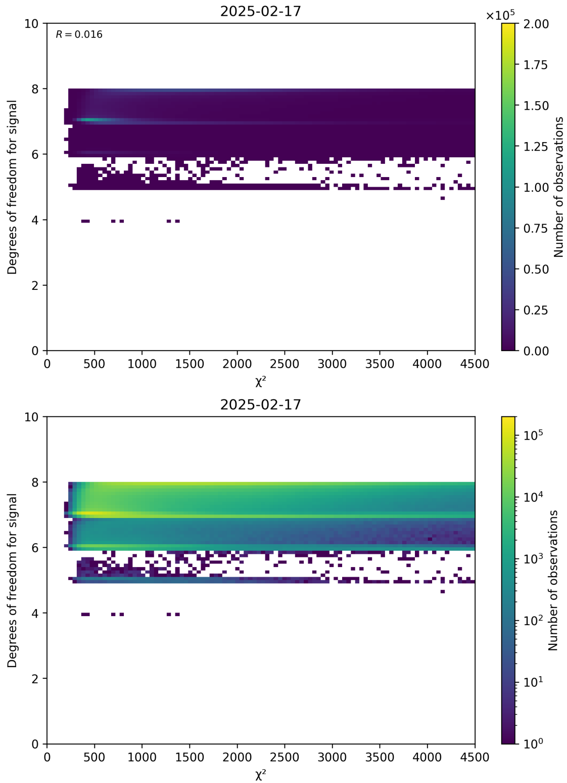
Figure 48: Scatter density plot of “ \chi^2 ” against “Degrees of freedom for signal” for 2025-02-16 to 2025-02-18.
