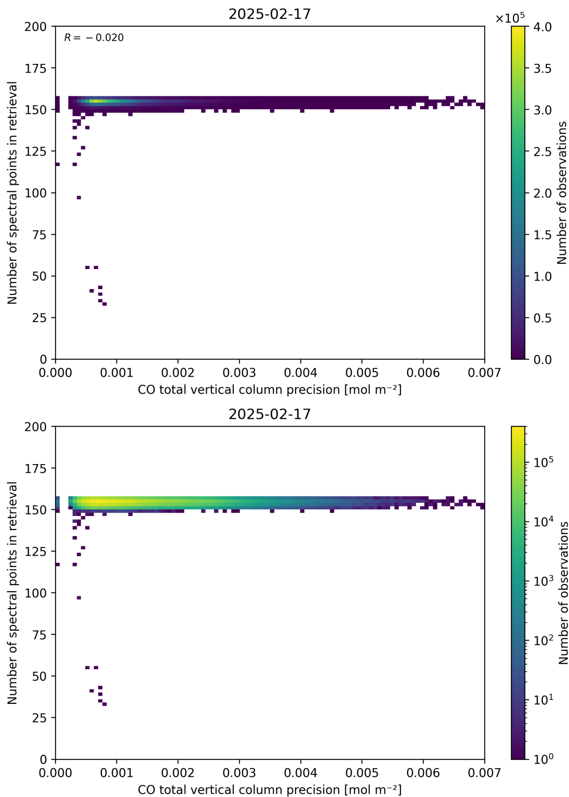
Figure 47: Scatter density plot of “CO total vertical column precision” against “Number of spectral points in retrieval” for 2025-02-16 to 2025-02-18.
