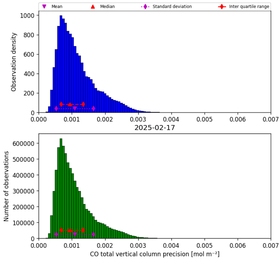
Figure 20: Histogram of “CO total vertical column precision” for 2025-02-16 to 2025-02-18
