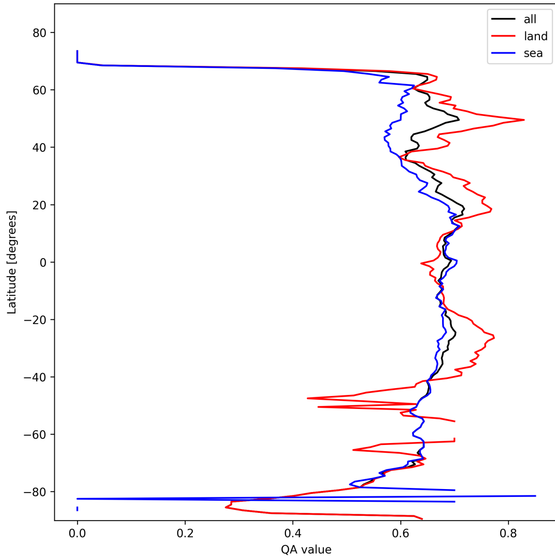
Figure 9: Zonal average of “QA value” for 2025-02-16 to 2025-02-18.
