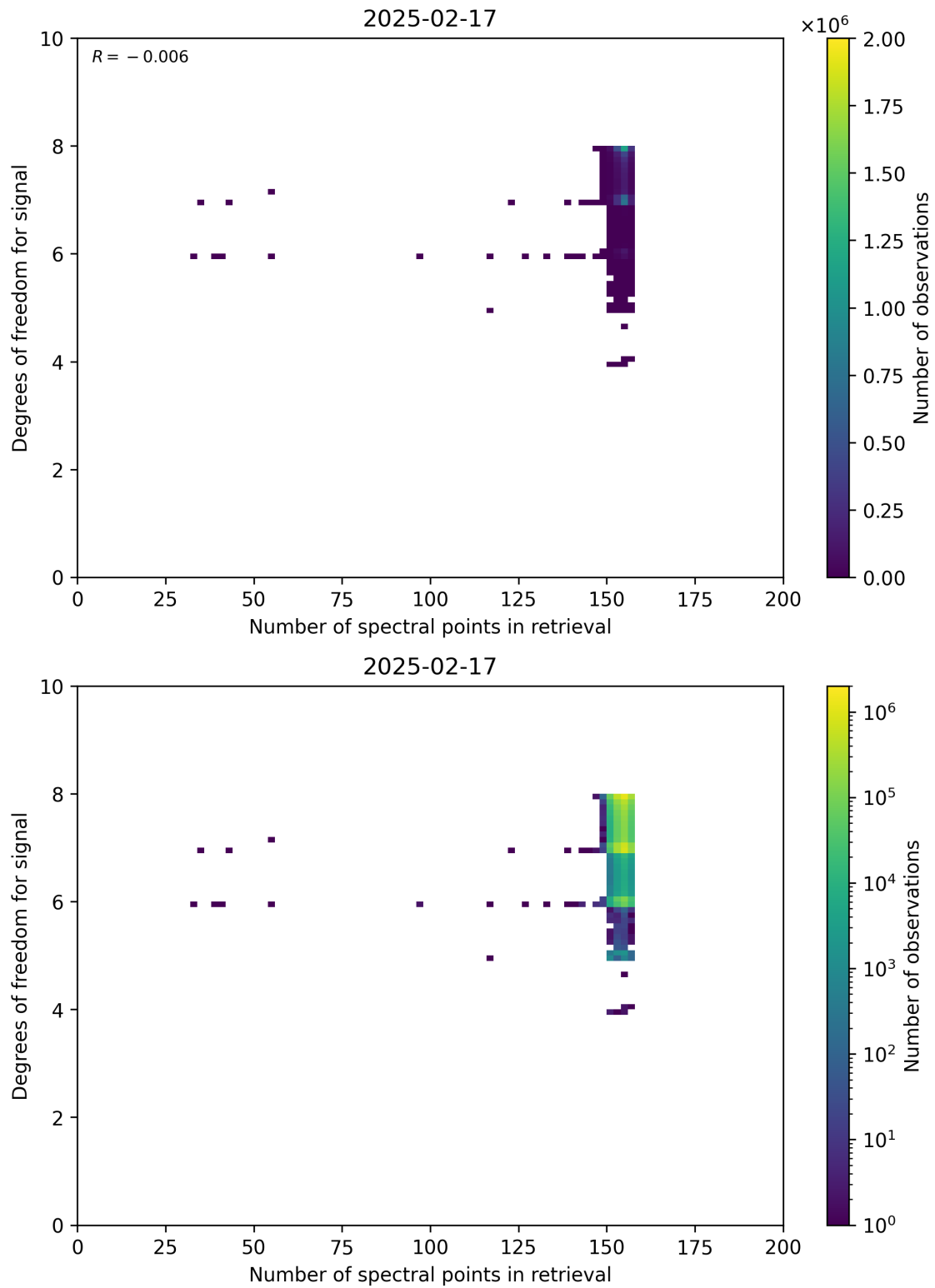
Figure 59: Scatter density plot of “Number of spectral points in retrieval” against “Degrees of freedom for signal” for 2025-02-16 to 2025-02-18.
