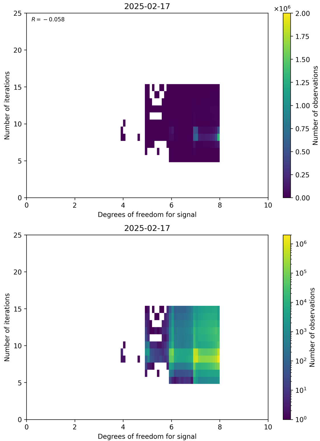
Figure 50: Scatter density plot of “Degrees of freedom for signal” against “Number of iterations” for 2025-02-16 to 2025-02-18.
