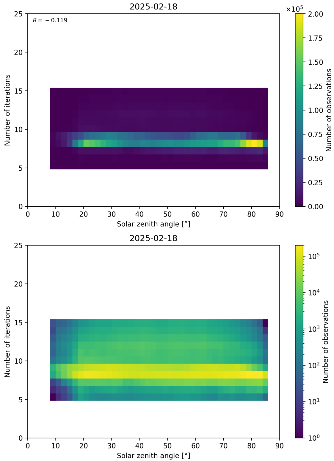
Figure 67: Scatter density plot of “Solar zenith angle” against “Number of iterations” for 2025-02-18 to 2025-02-19.
