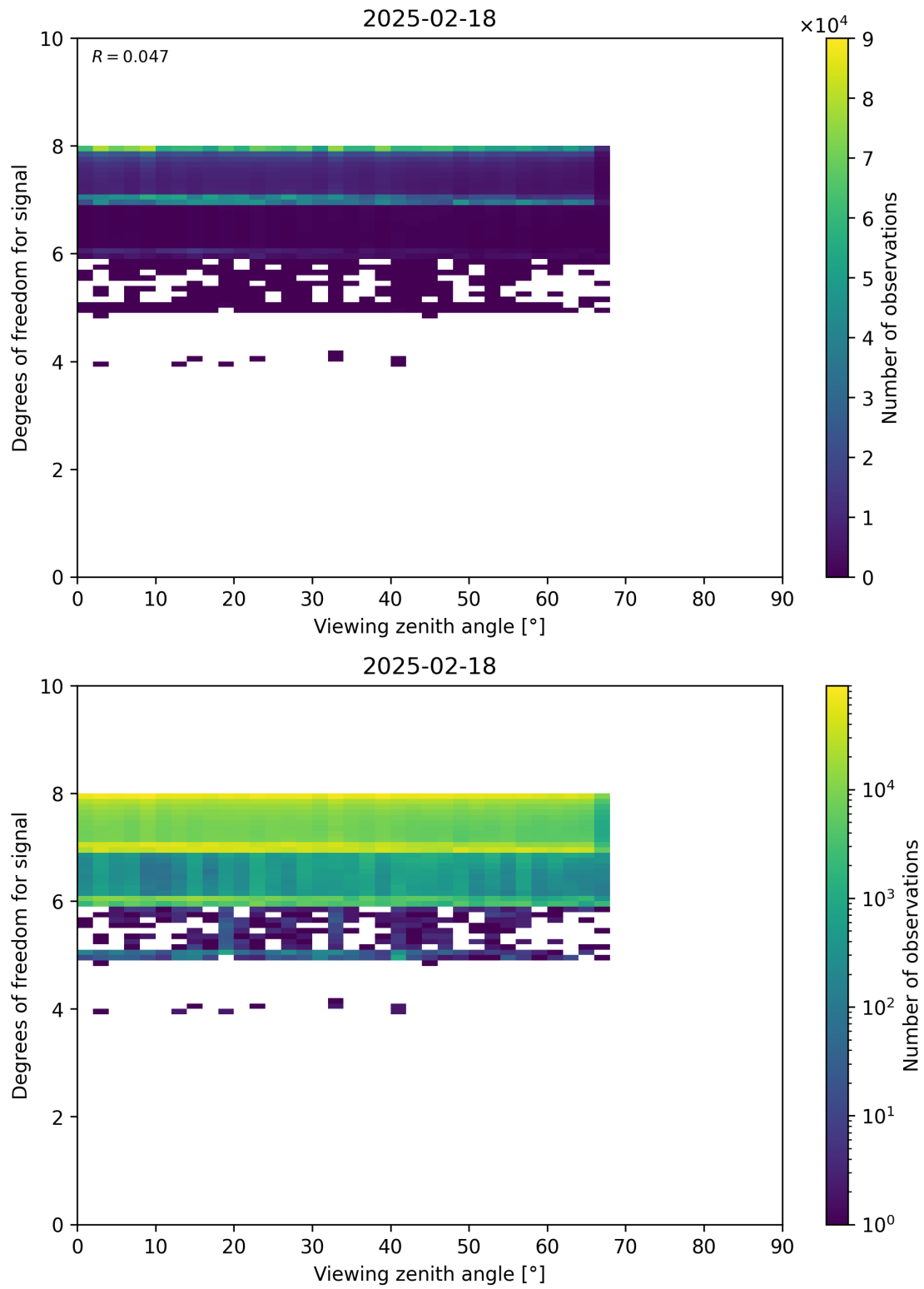
Figure 73: Scatter density plot of “Viewing zenith angle” against “Degrees of freedom for signal” for 2025-02-18 to 2025-02-19.
