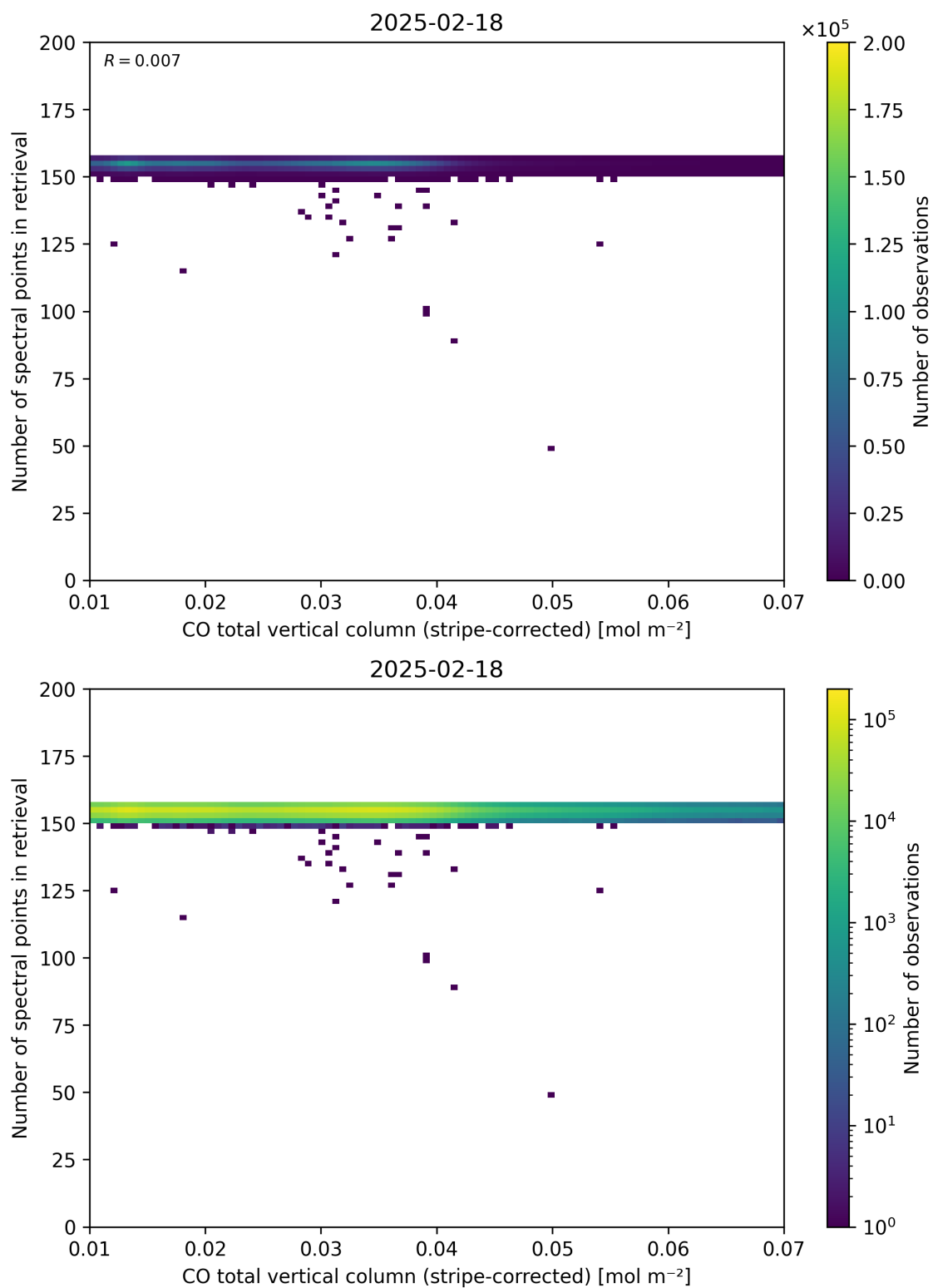
Figure 40: Scatter density plot of “CO total vertical column (stripe-corrected)” against “Number of spectral points in retrieval” for 2025-02-18 to 2025-02-19.
