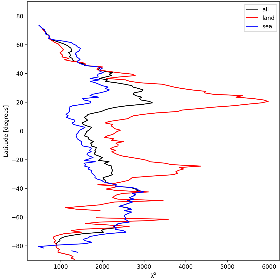
Figure 14: Zonal average of “ \chi^2 ” for 2025-02-18 to 2025-02-19.
