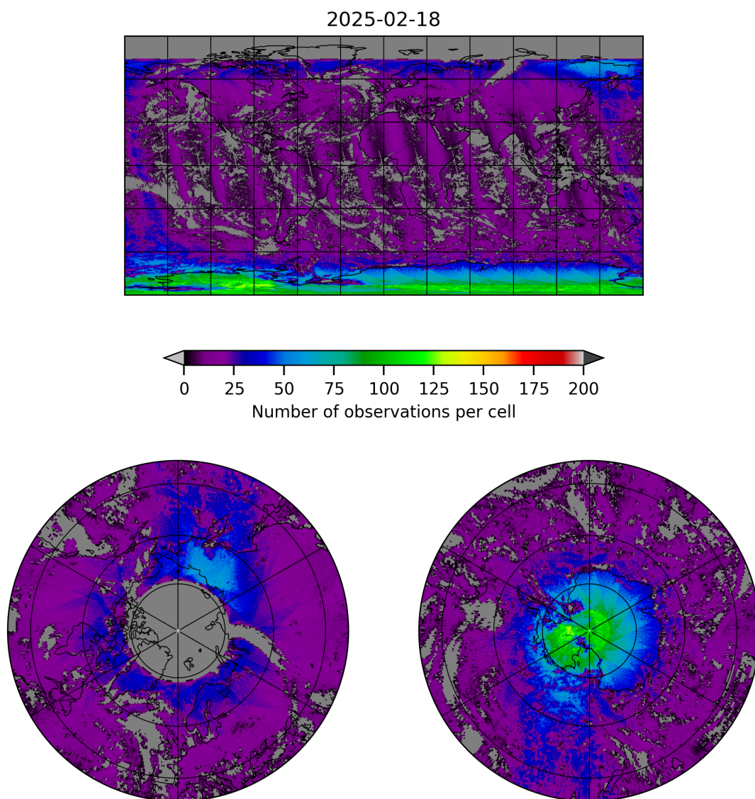
Figure 8: Map of the number of observations for 2025-02-18 to 2025-02-19
