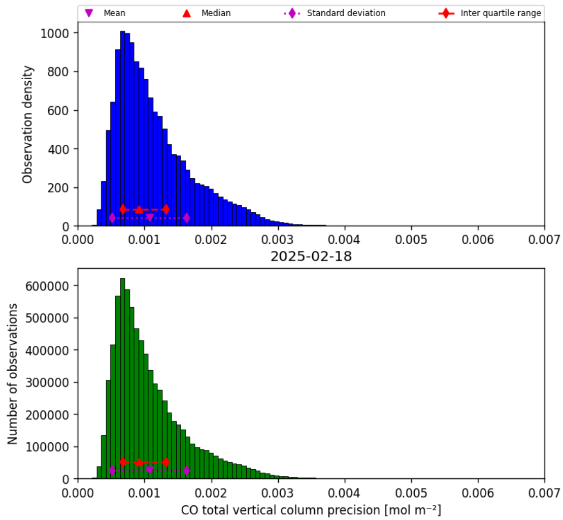
Figure 20: Histogram of “CO total vertical column precision” for 2025-02-18 to 2025-02-19
