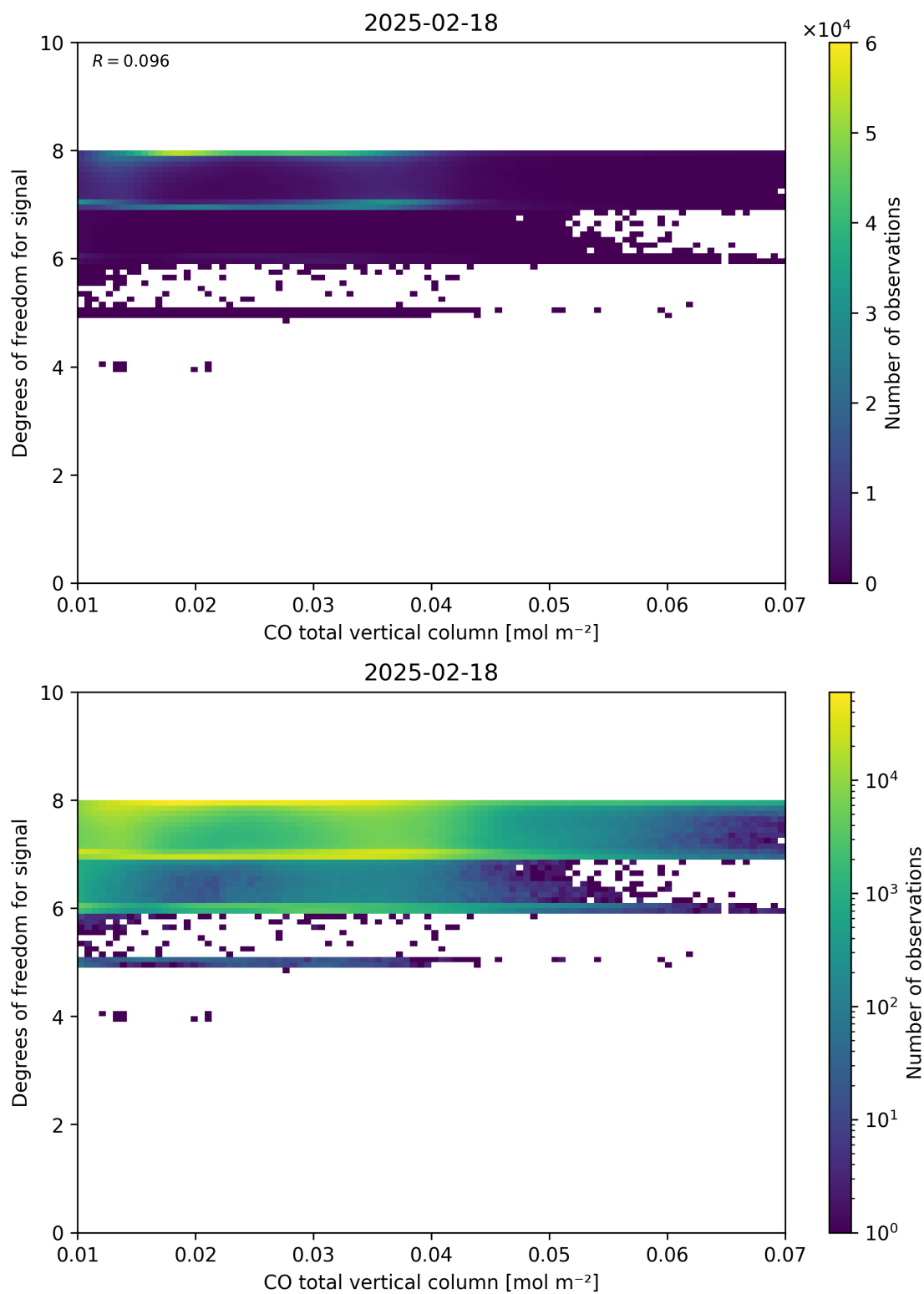
Figure 41: Scatter density plot of “CO total vertical column” against “Degrees of freedom for signal” for 2025-02-18 to 2025-02-19.
