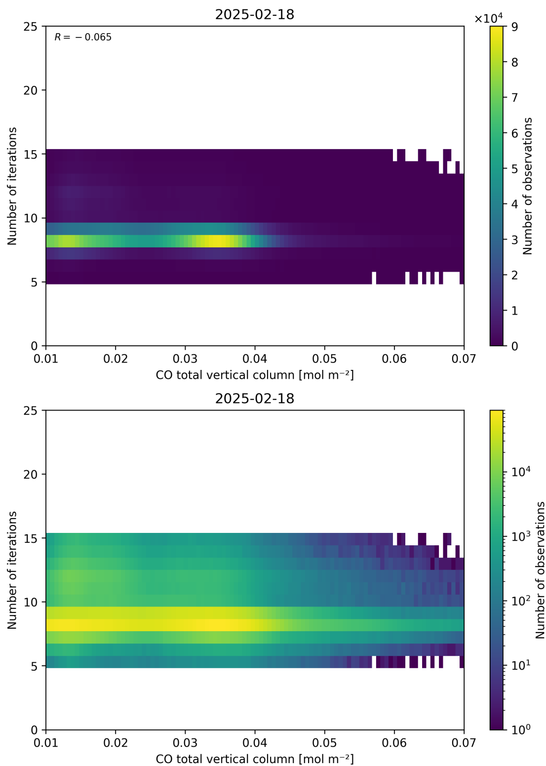
Figure 42: Scatter density plot of “CO total vertical column” against “Number of iterations” for 2025-02-18 to 2025-02-19.
