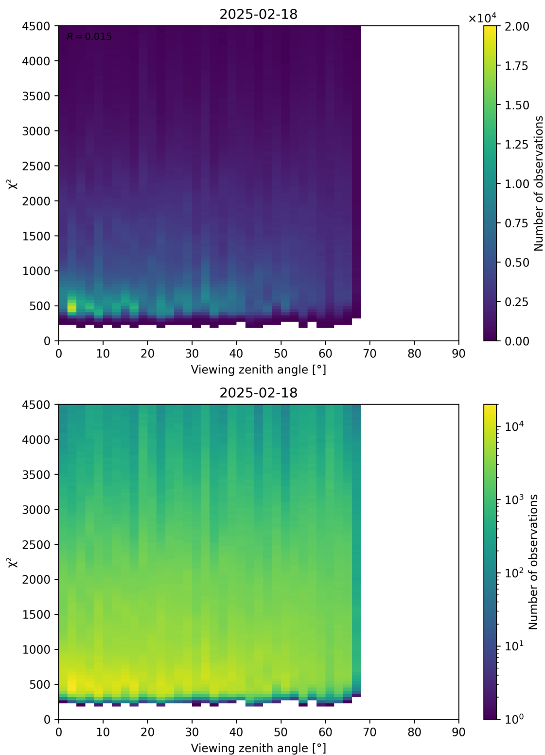
Figure 72: Scatter density plot of “Viewing zenith angle” against “ \chi^2 ” for 2025-02-18 to 2025-02-19.
