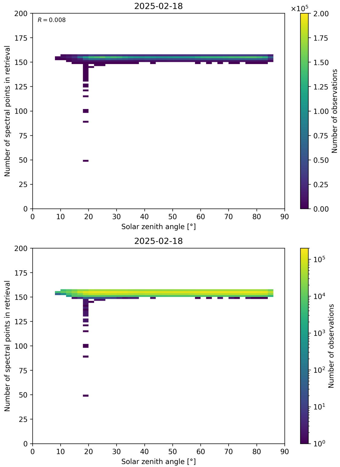
Figure 68: Scatter density plot of “Solar zenith angle” against “Number of spectral points in retrieval” for 2025-02-18 to 2025-02-19.
