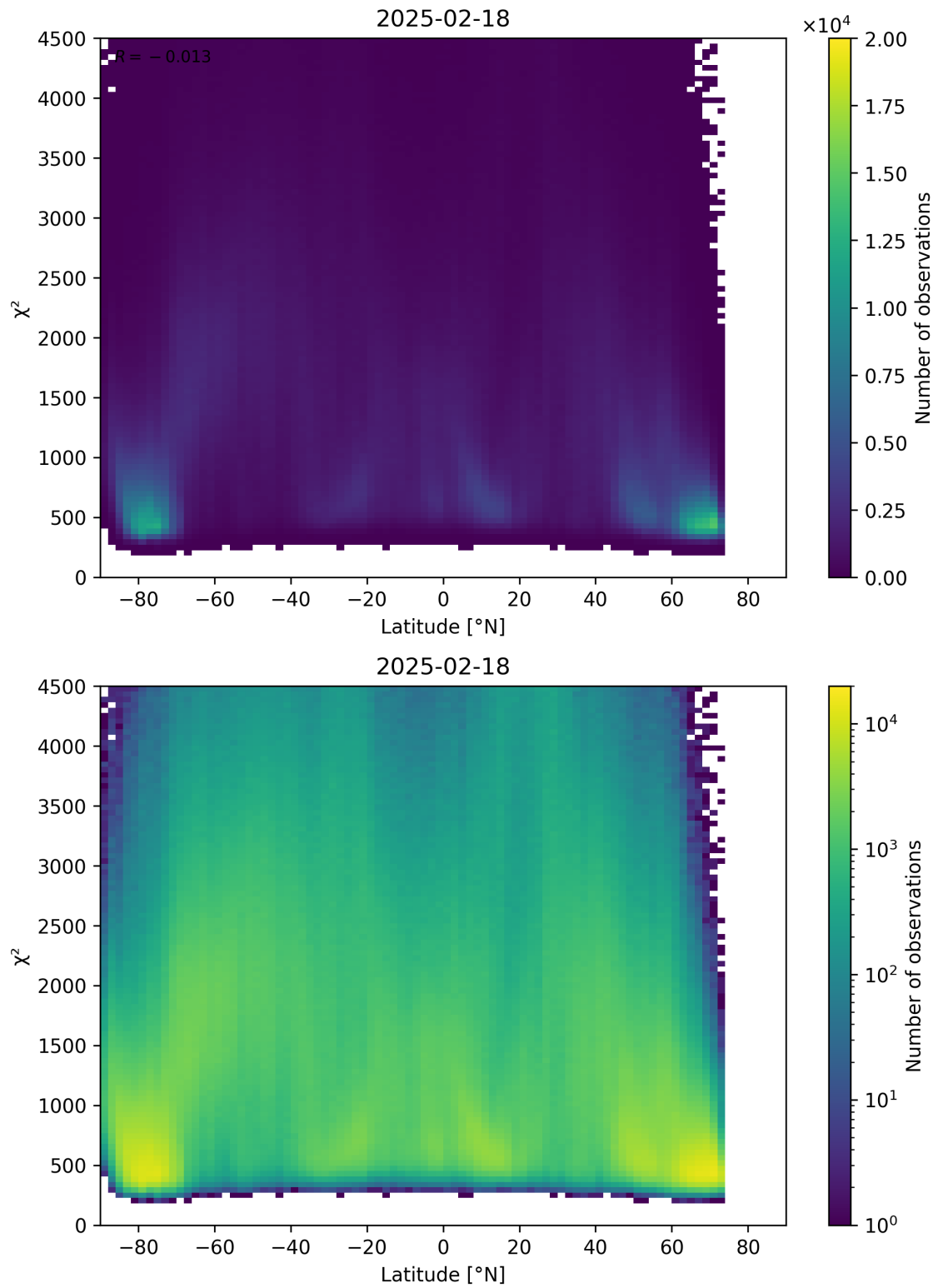
Figure 54: Scatter density plot of “Latitude” against “ \chi^2 ” for 2025-02-18 to 2025-02-19.
