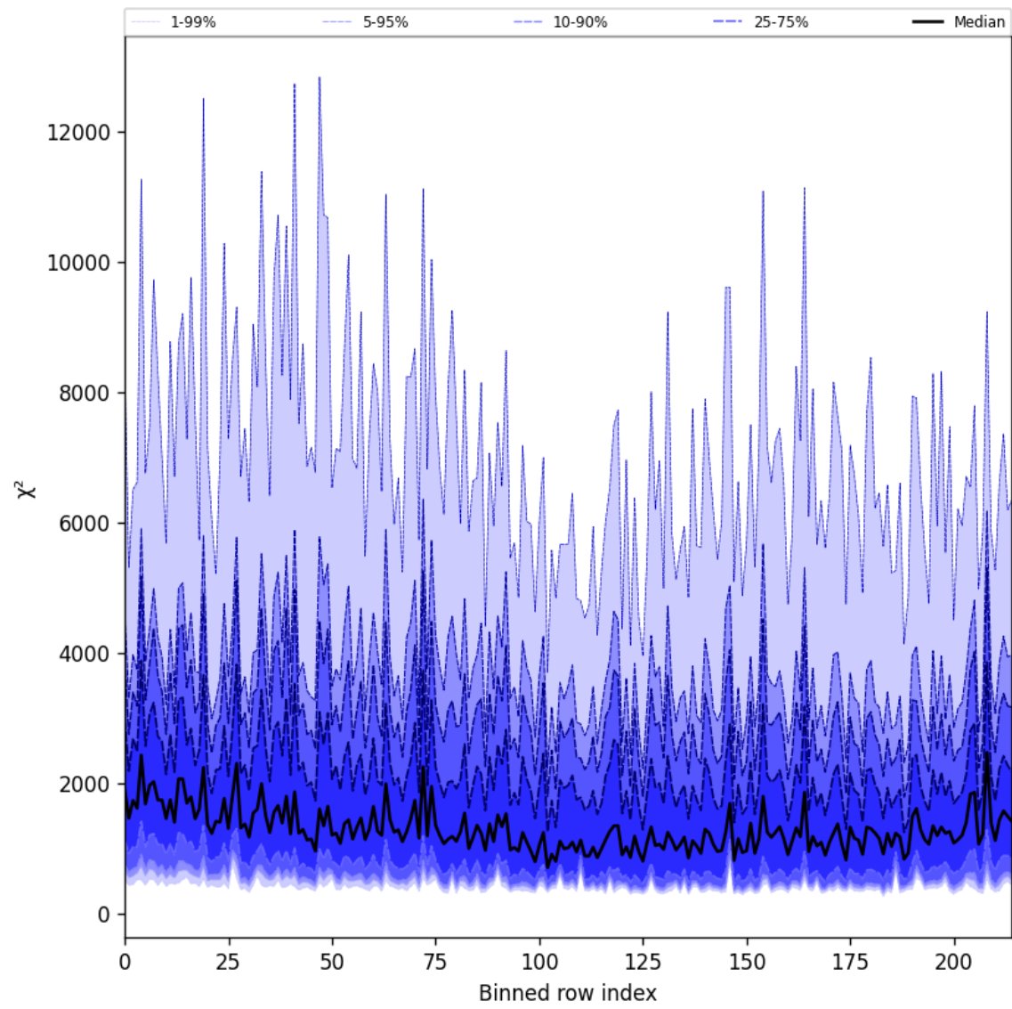
Figure 30: Along track statistics of “ \chi^2 ” for 2025-02-18 to 2025-02-19
