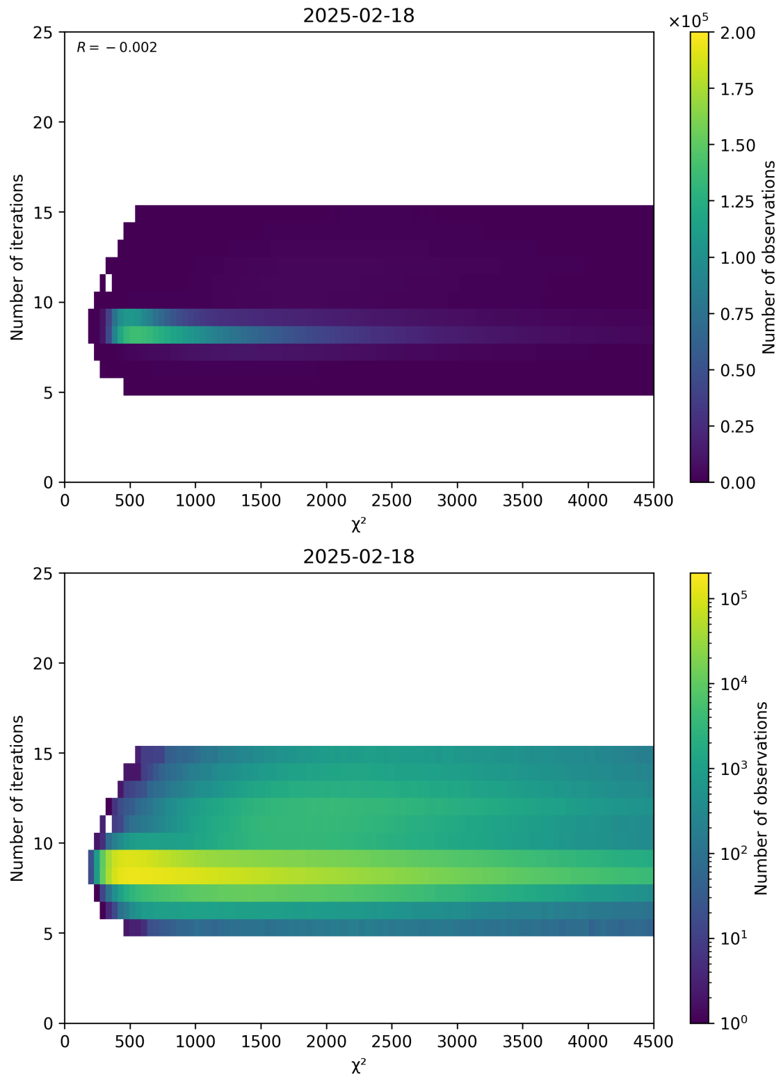
Figure 49: Scatter density plot of “ \chi^2 ” against “Number of iterations” for 2025-02-18 to 2025-02-19.
