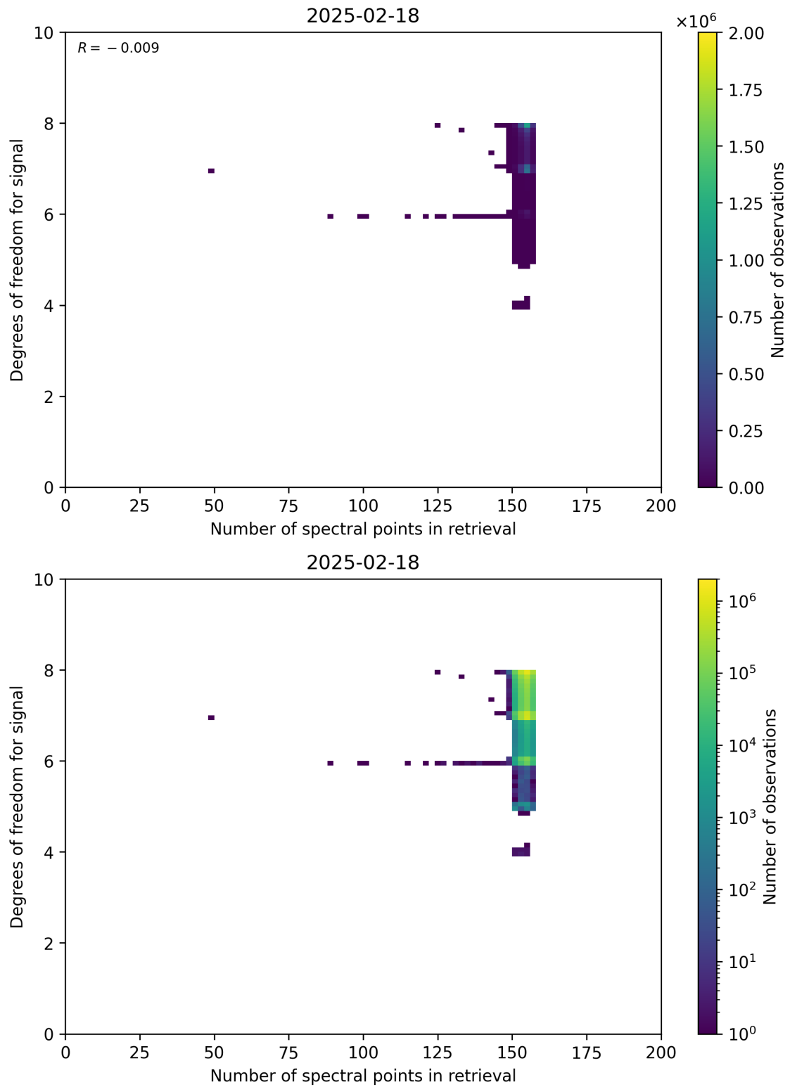
Figure 59: Scatter density plot of “Number of spectral points in retrieval” against “Degrees of freedom for signal” for 2025-02-18 to 2025-02-19.
