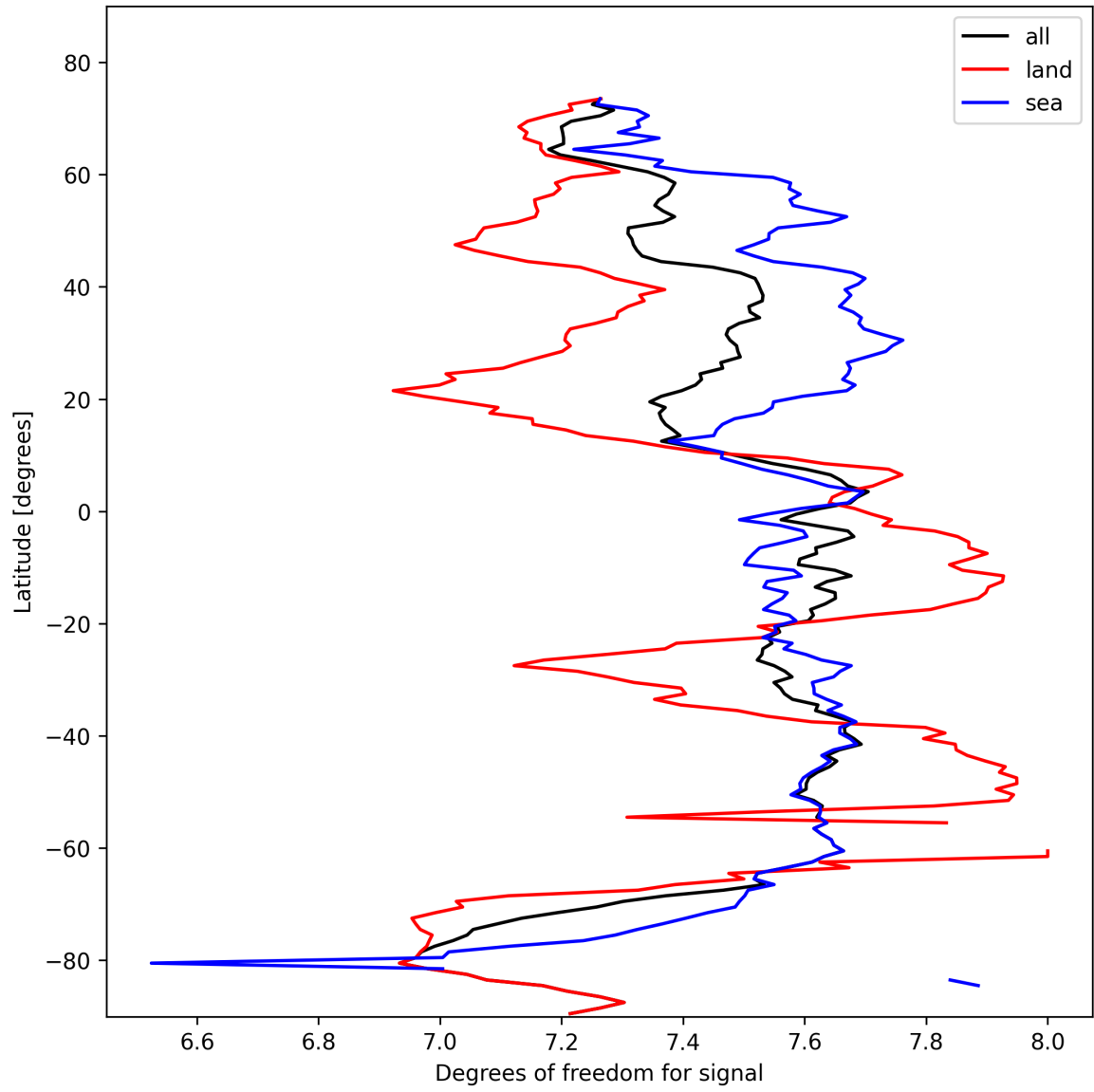
Figure 15: Zonal average of “Degrees of freedom for signal” for 2025-02-18 to 2025-02-19.
