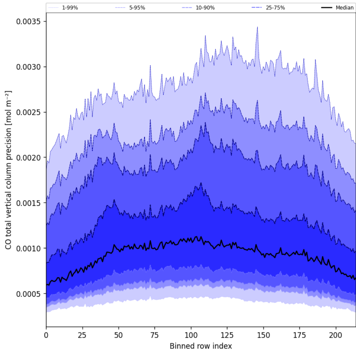
Figure 28: Along track statistics of “CO total vertical column precision” for 2025-02-18 to 2025-02-19
