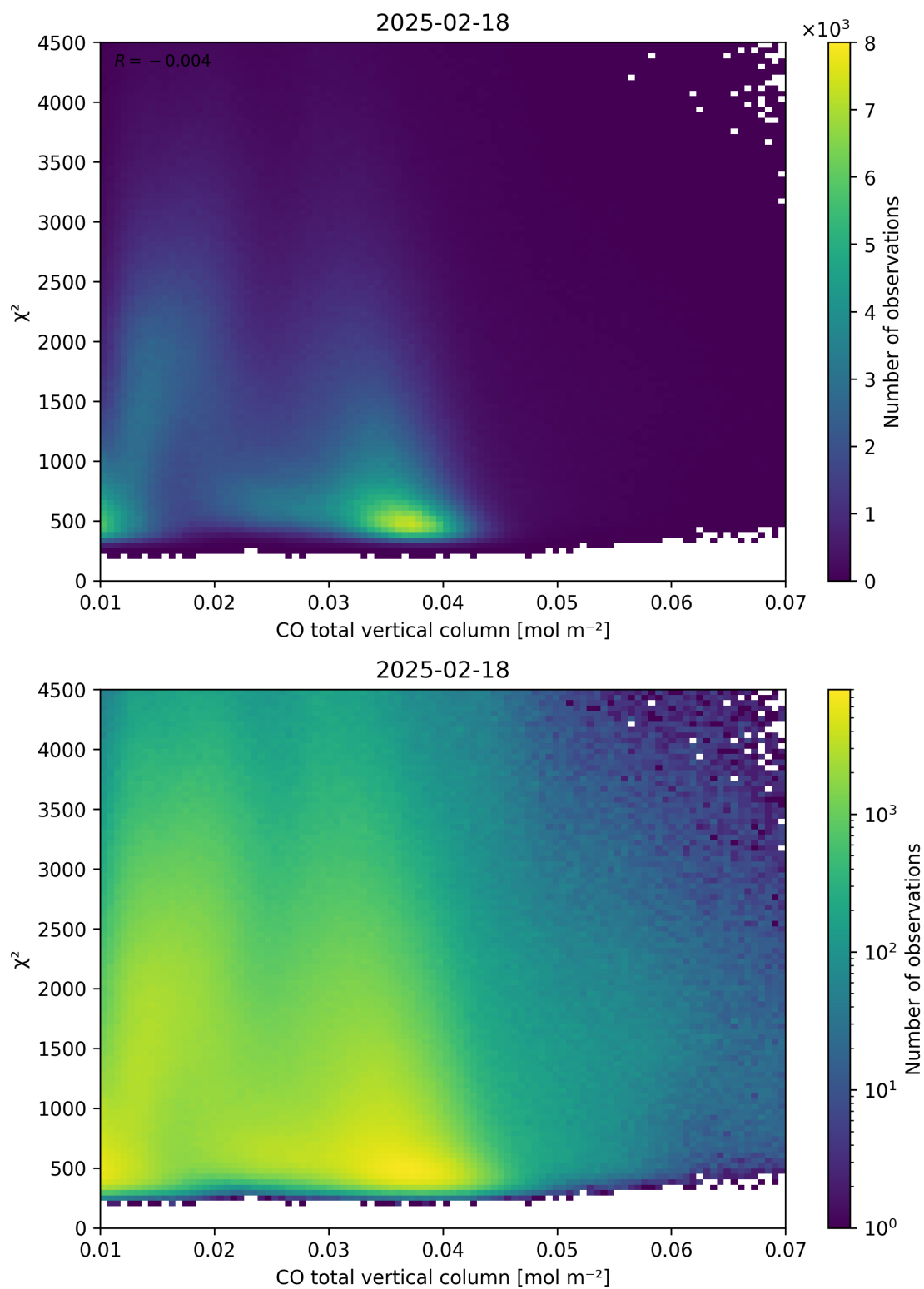
Figure 35: Scatter density plot of “CO total vertical column” against “ \chi^2 ” for 2025-02-18 to 2025-02-19.
