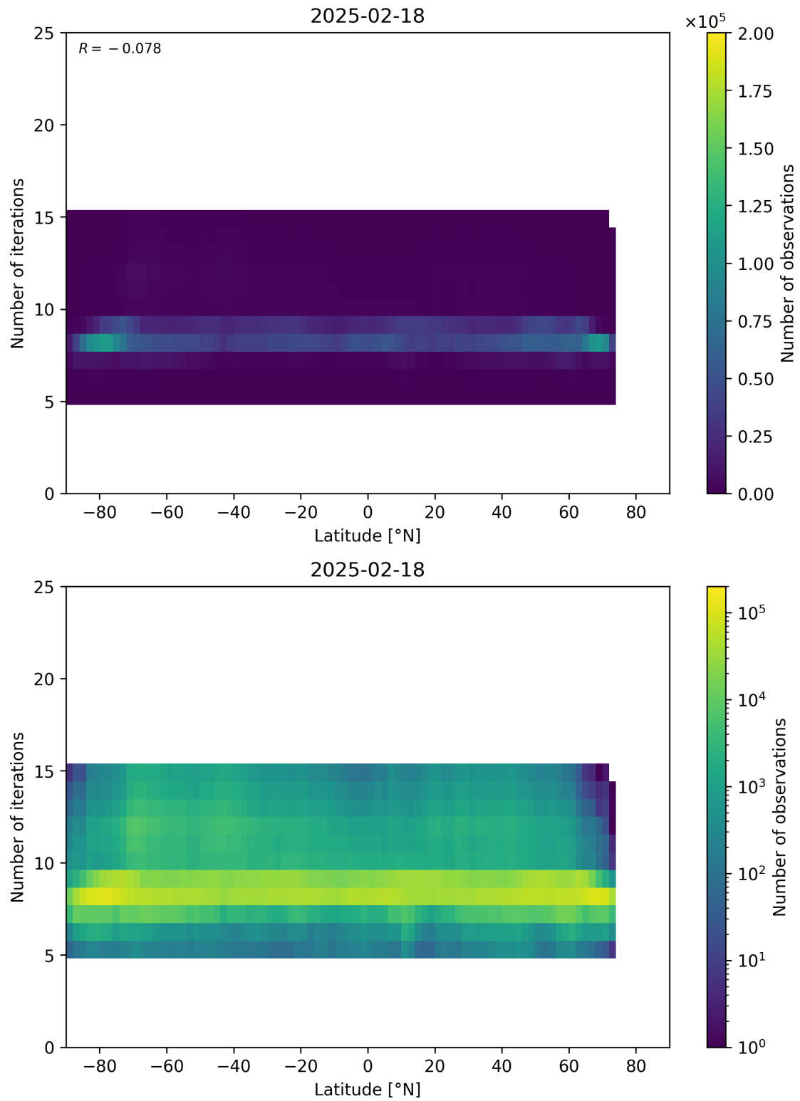
Figure 56: Scatter density plot of “Latitude” against “Number of iterations” for 2025-02-18 to 2025-02-19.
