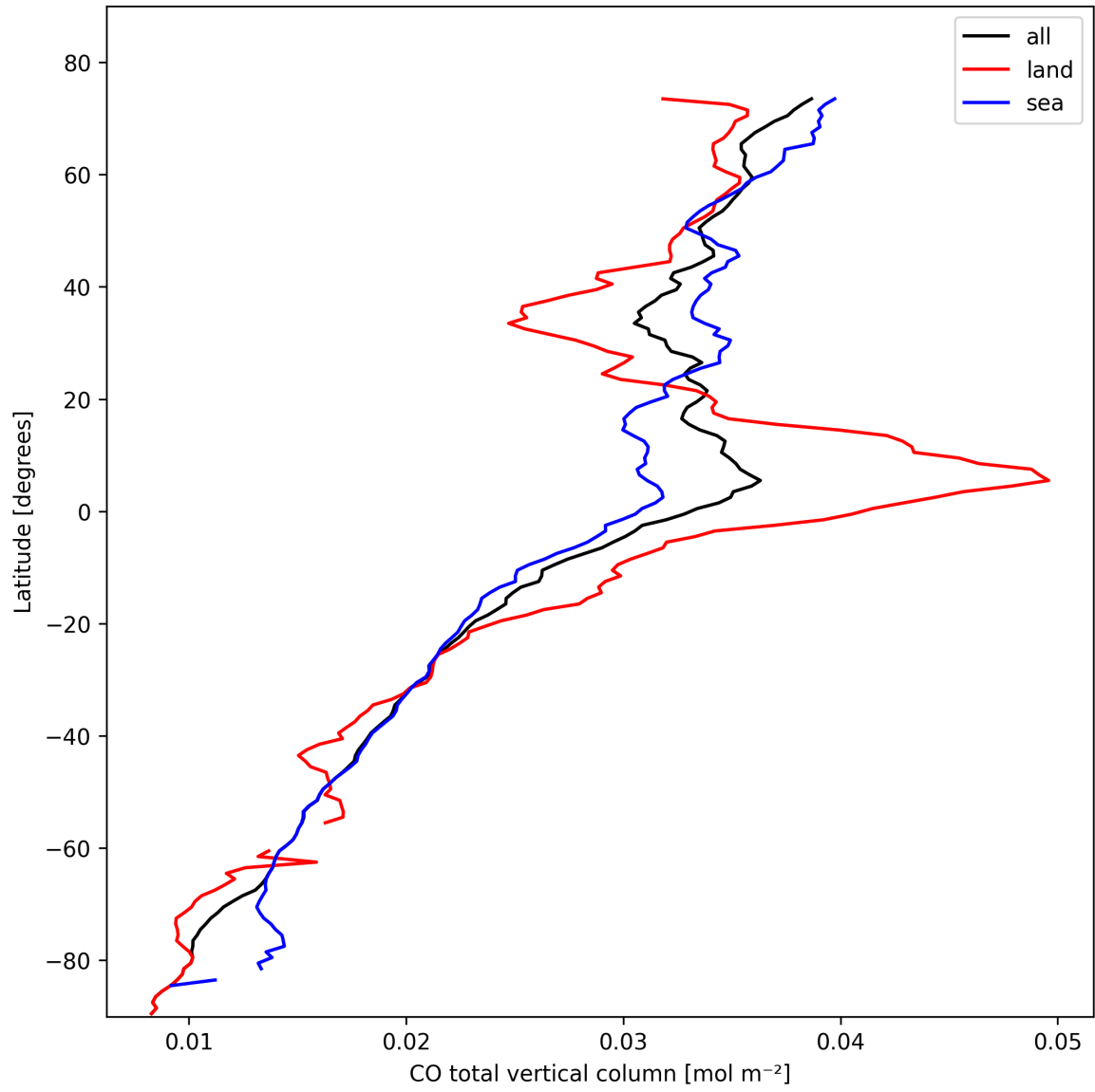
Figure 10: Zonal average of “CO total vertical column” for 2025-02-18 to 2025-02-19.
