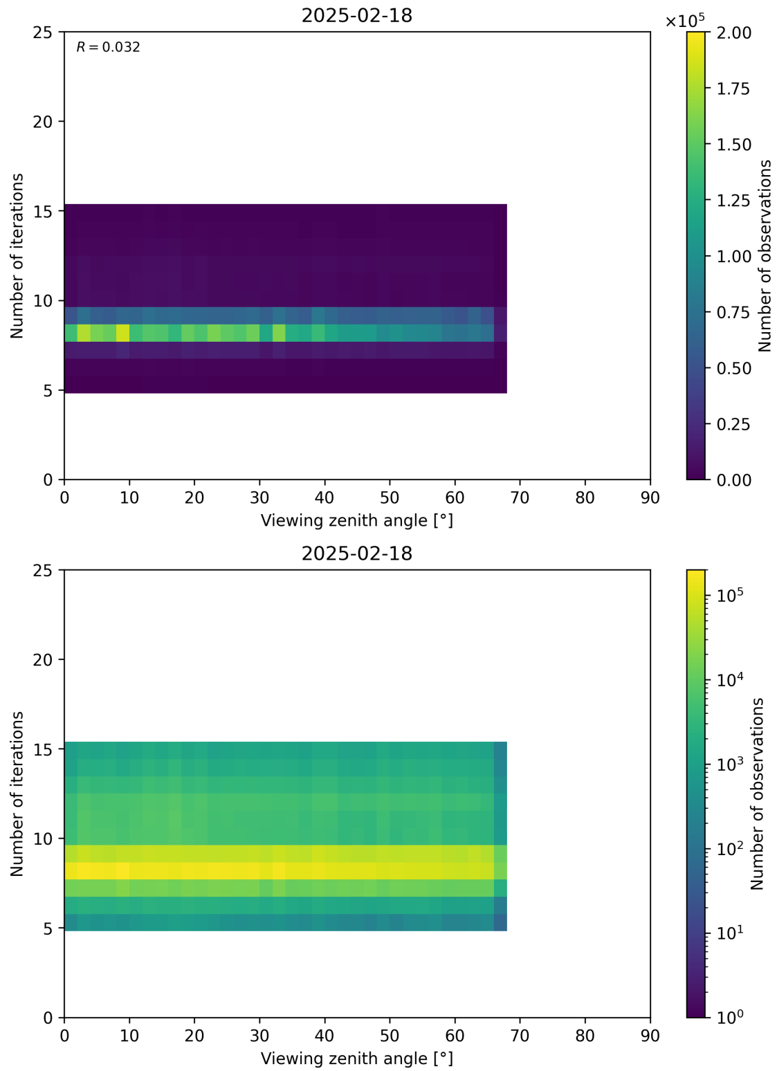
Figure 75: Scatter density plot of “Viewing zenith angle” against “Number of iterations” for 2025-02-18 to 2025-02-19.
