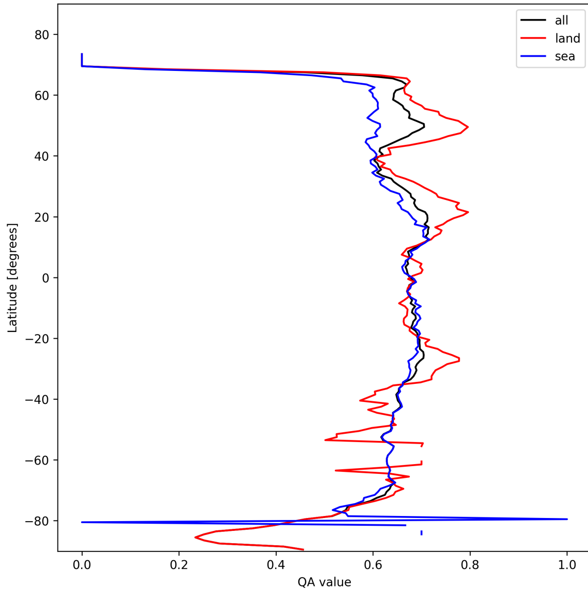
Figure 9: Zonal average of “QA value” for 2025-02-18 to 2025-02-19.
