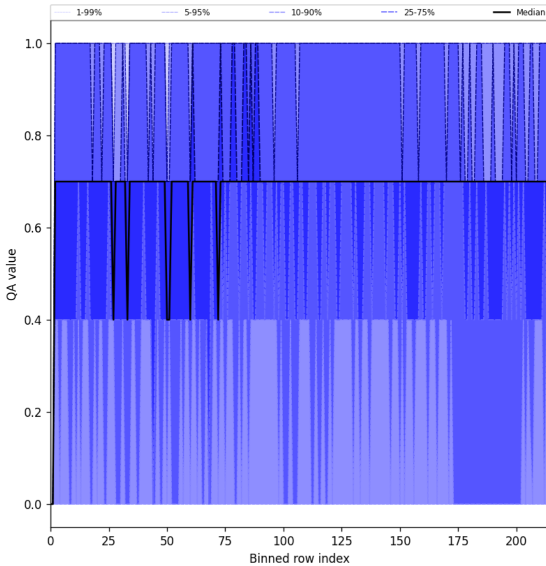
Figure 25: Along track statistics of “QA value” for 2025-02-18 to 2025-02-19
