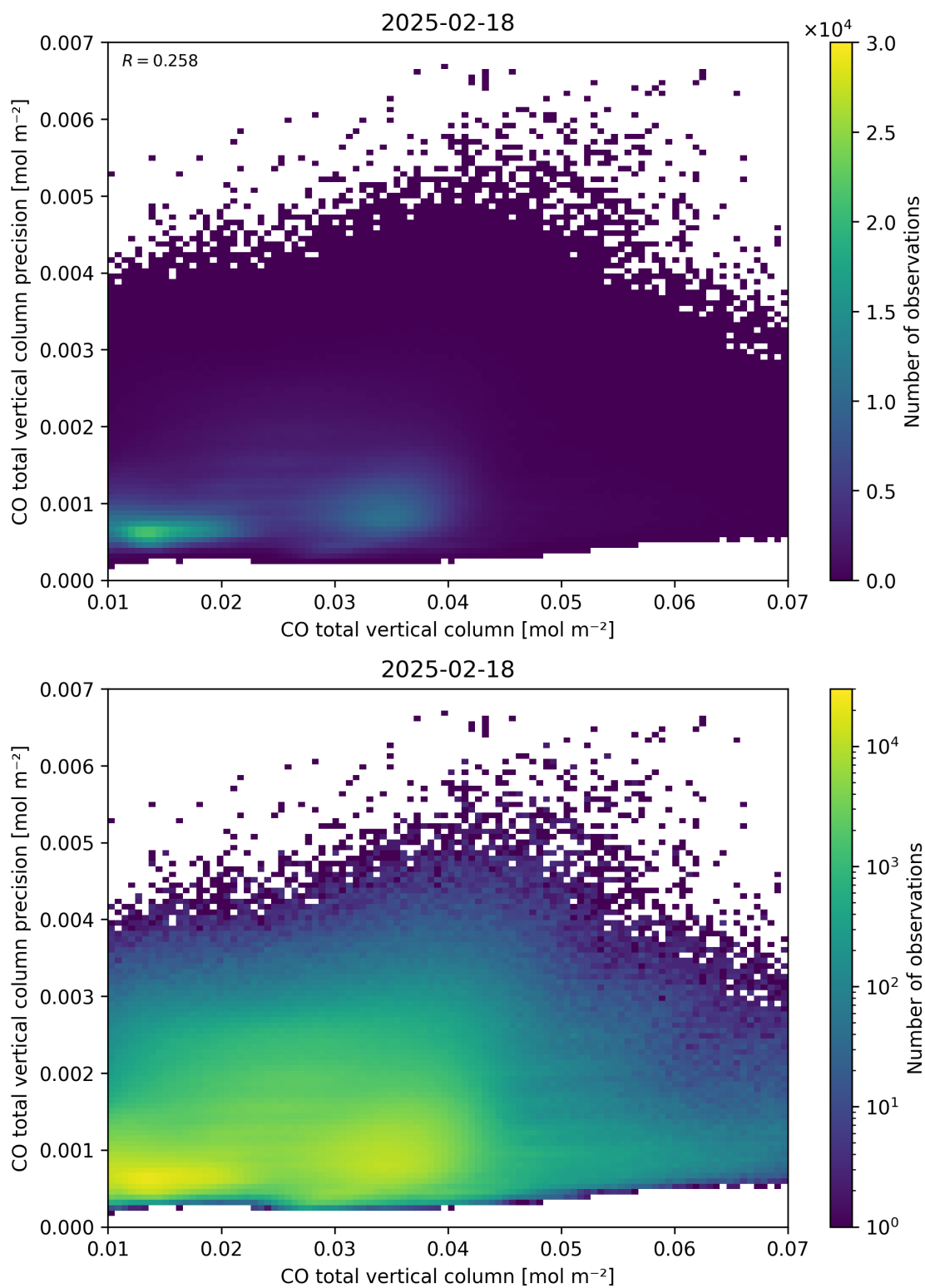
Figure 34: Scatter density plot of “CO total vertical column” against “CO total vertical column precision” for 2025-02-18 to 2025-02-19.
