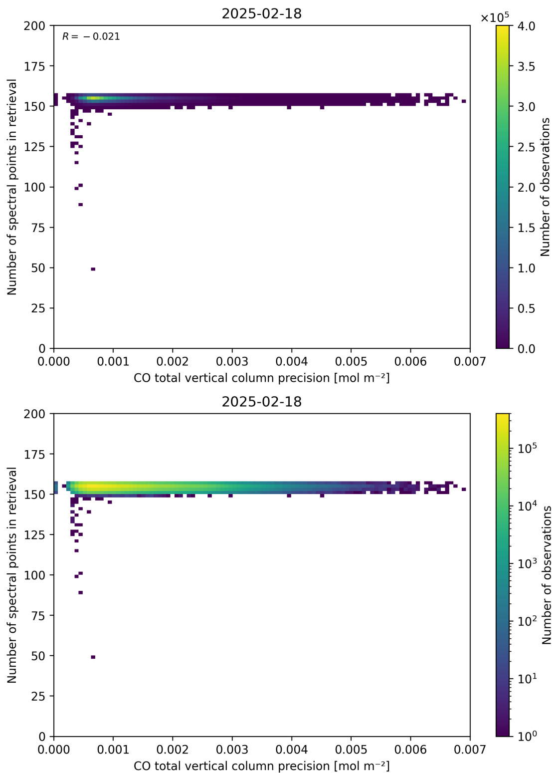
Figure 47: Scatter density plot of “CO total vertical column precision” against “Number of spectral points in retrieval” for 2025-02-18 to 2025-02-19.
