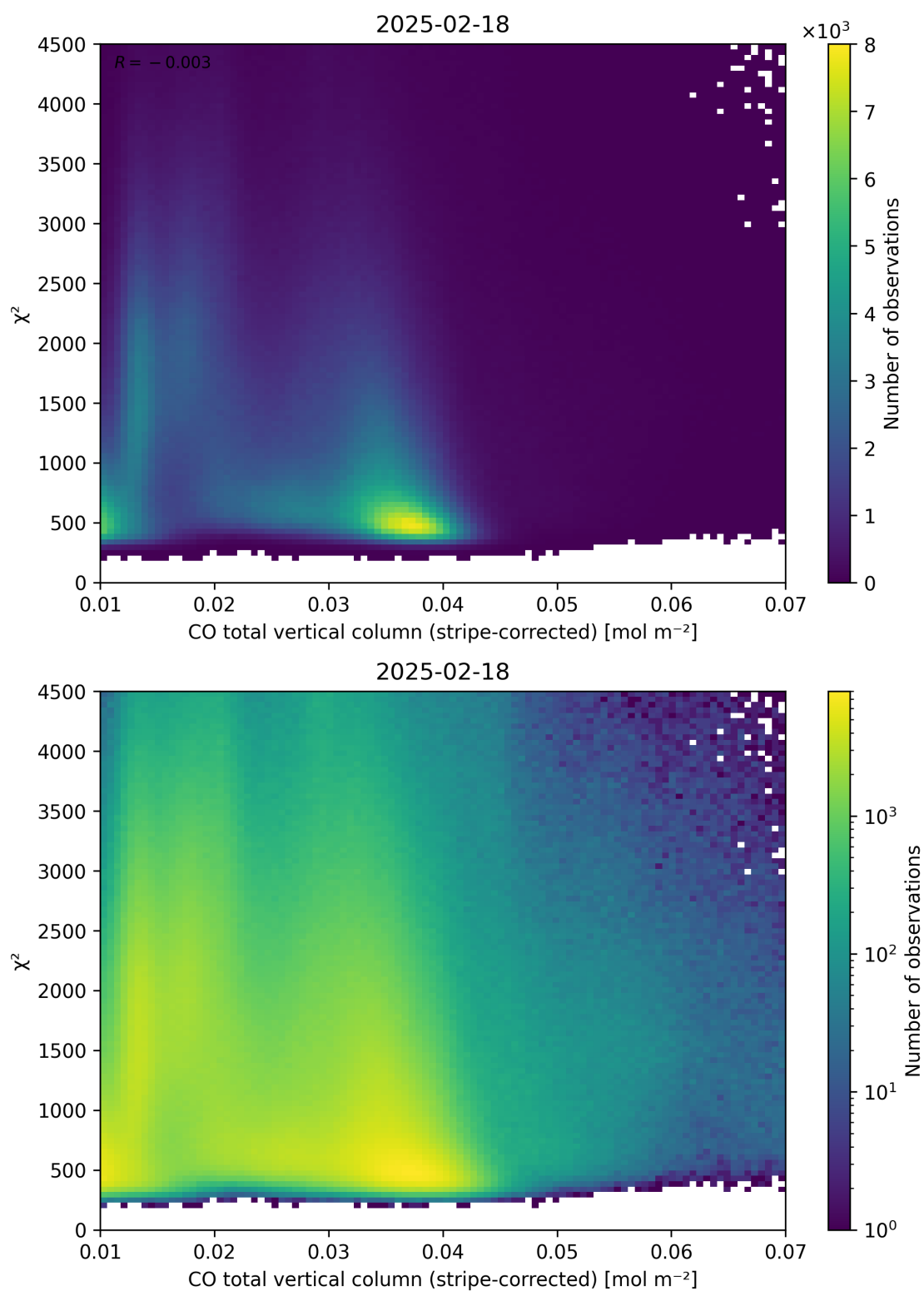
Figure 37: Scatter density plot of “CO total vertical column (stripe-corrected)” against “ \chi^2 ” for 2025-02-18 to 2025-02-19.
