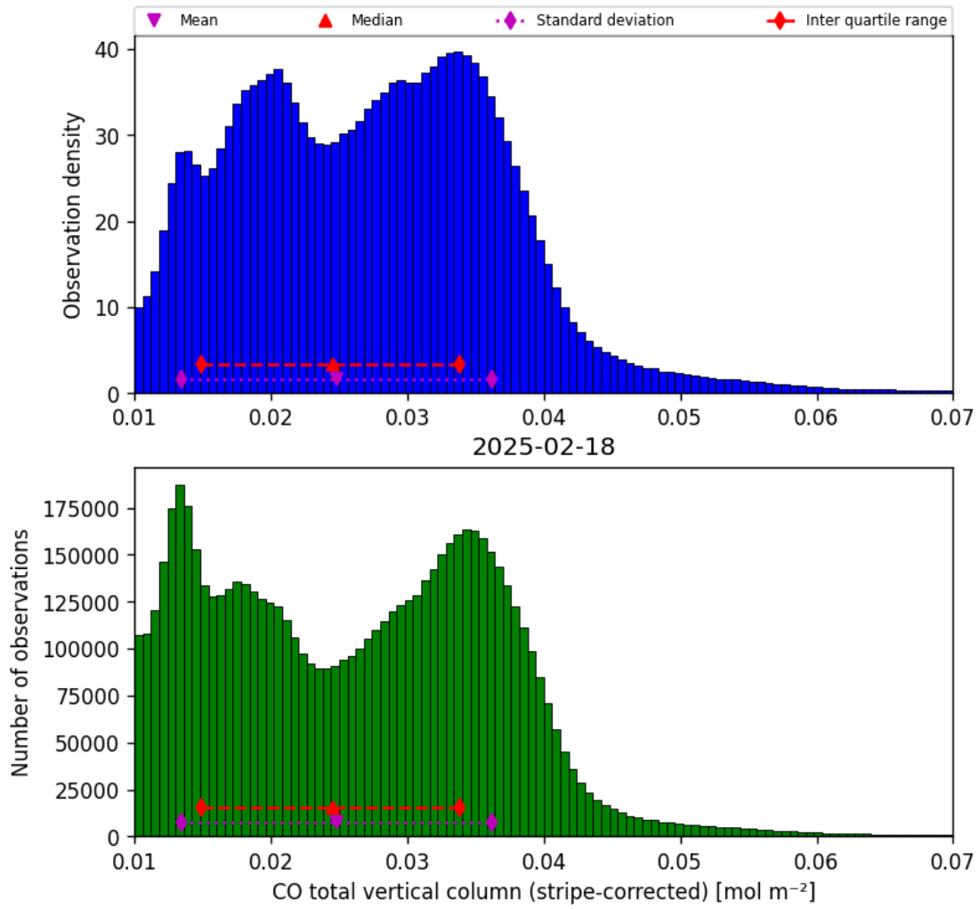
Figure 19: Histogram of “CO total vertical column (stripe-corrected)” for 2025-02-18 to 2025-02-19
