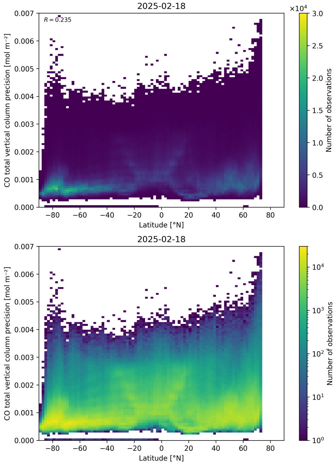
Figure 53: Scatter density plot of “Latitude” against “CO total vertical column precision” for 2025-02-18 to 2025-02-19.
