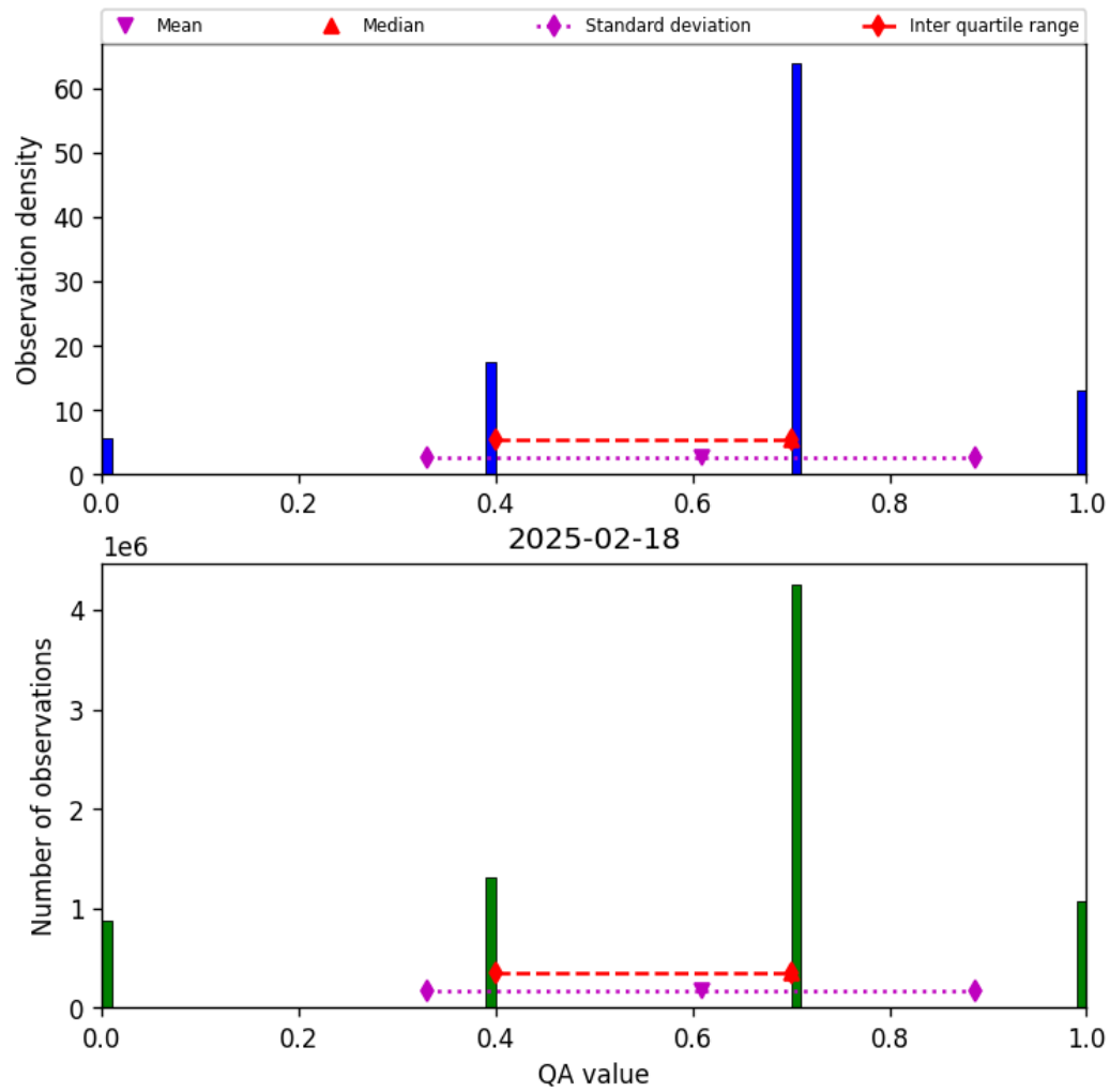
Figure 17: Histogram of “QA value” for 2025-02-18 to 2025-02-19
