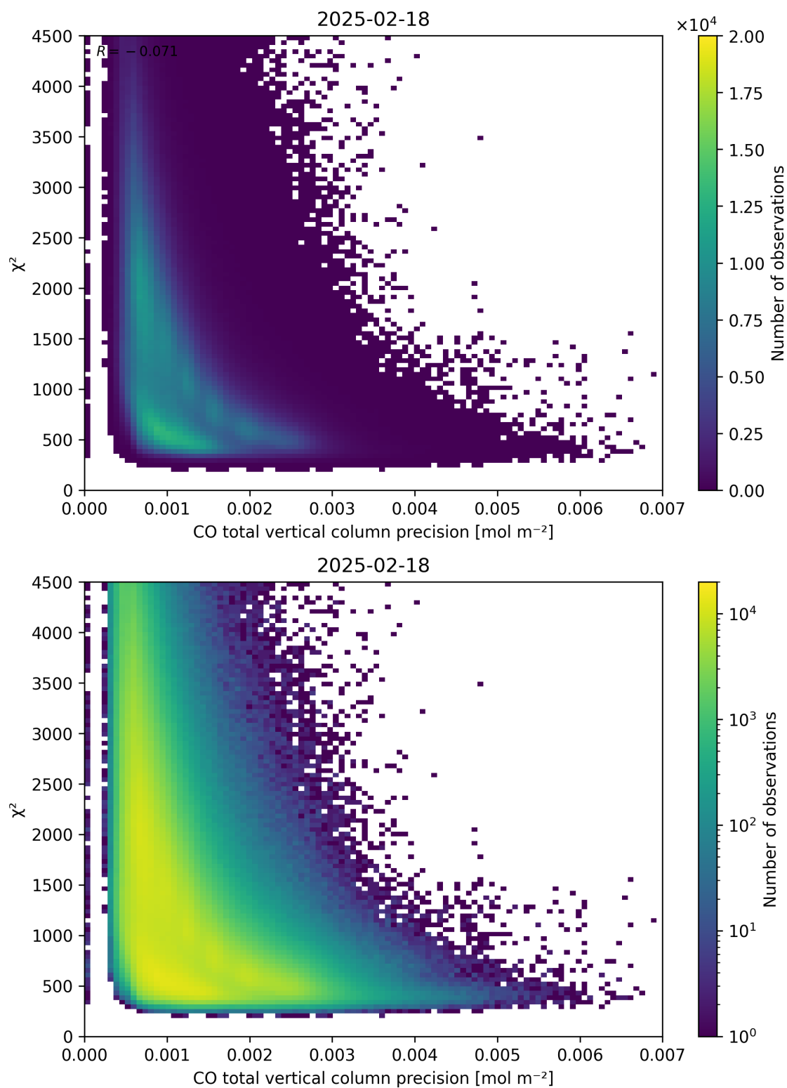
Figure 44: Scatter density plot of “CO total vertical column precision” against “ \chi^2 ” for 2025-02-18 to 2025-02-19.
