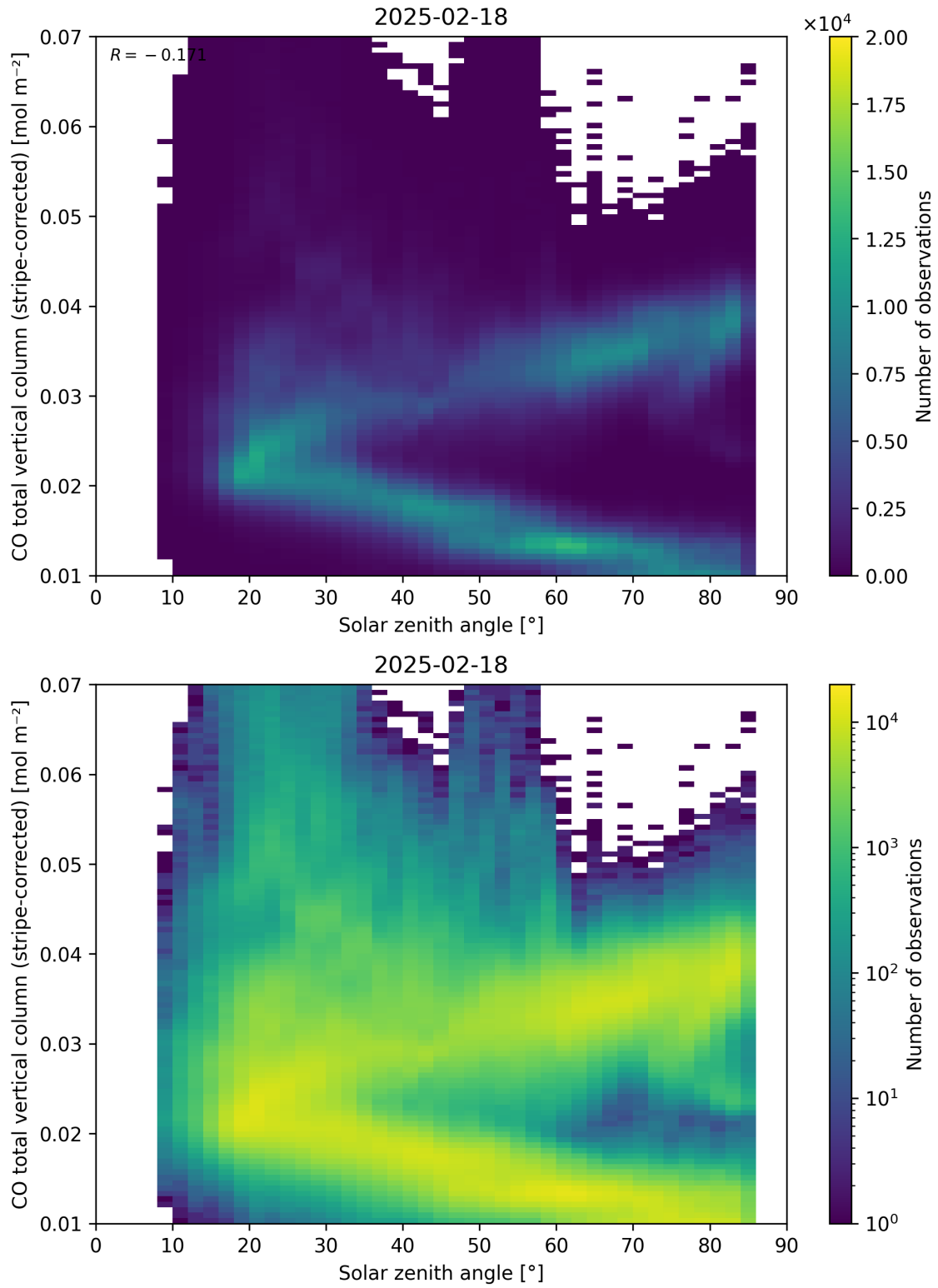
Figure 62: Scatter density plot of “Solar zenith angle” against “CO total vertical column (stripe-corrected)” for 2025-02-18 to 2025-02-19.
