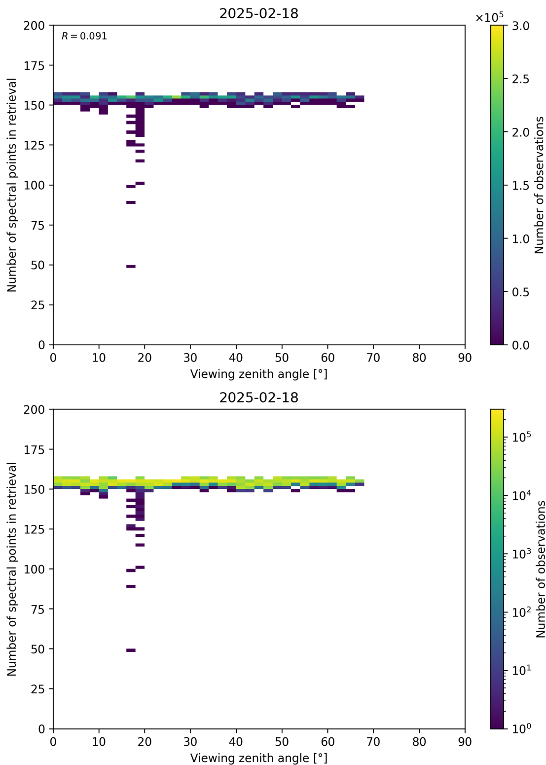
Figure 76: Scatter density plot of “Viewing zenith angle” against “Number of spectral points in retrieval” for 2025-02-18 to 2025-02-19.
