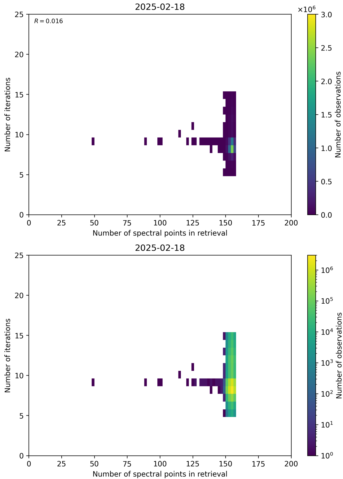
Figure 60: Scatter density plot of “Number of spectral points in retrieval” against “Number of iterations” for 2025-02-18 to 2025-02-19.
