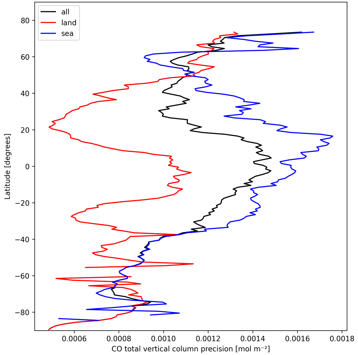
Figure 12: Zonal average of “CO total vertical column precision” for 2025-02-18 to 2025-02-19.
