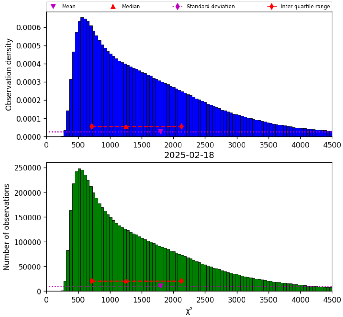
Figure 22: Histogram of “ \chi^2 ” for 2025-02-18 to 2025-02-19
