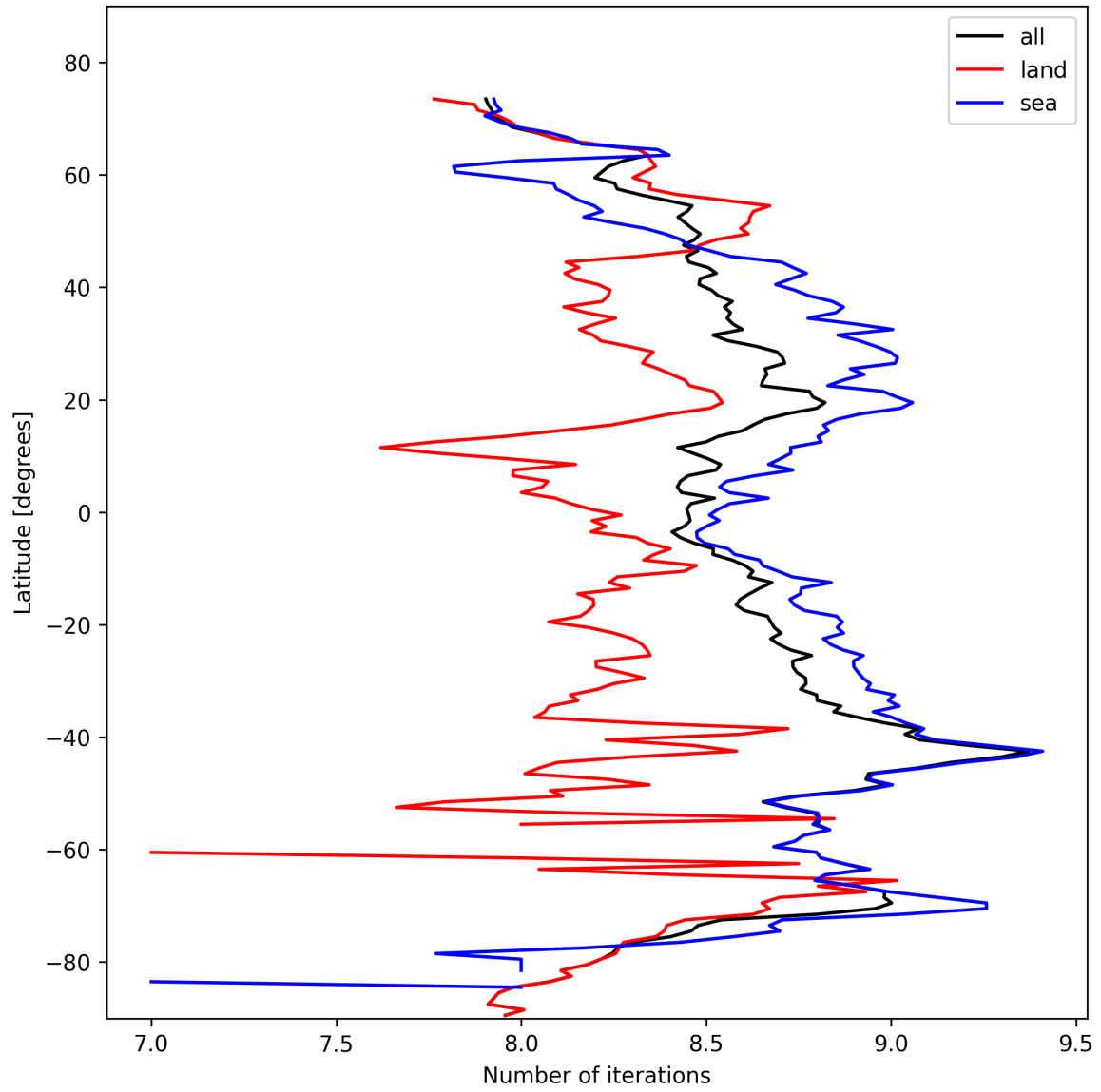
Figure 16: Zonal average of “Number of iterations” for 2025-02-18 to 2025-02-19.
