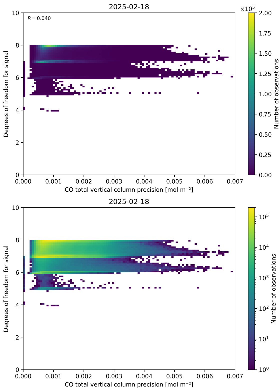
Figure 45: Scatter density plot of “CO total vertical column precision” against “Degrees of freedom for signal” for 2025-02-18 to 2025-02-19.
