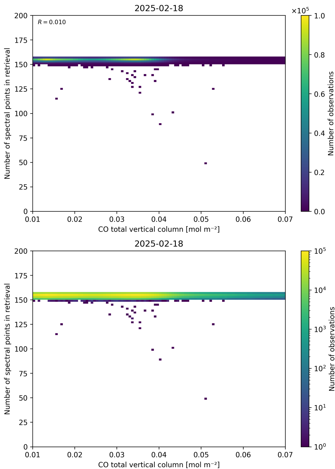
Figure 43: Scatter density plot of “CO total vertical column” against “Number of spectral points in retrieval” for 2025-02-18 to 2025-02-19.
