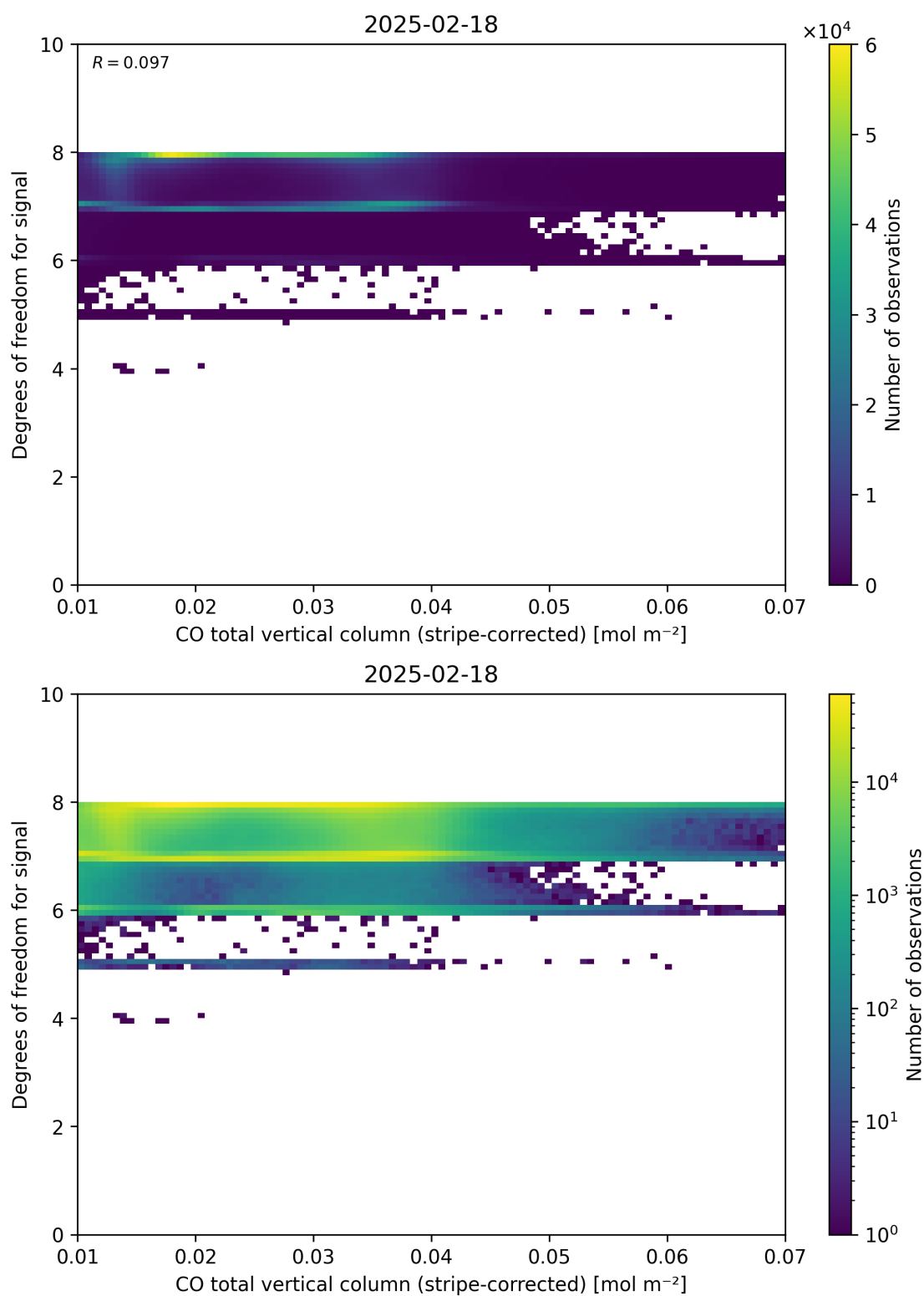
Figure 38: Scatter density plot of “CO total vertical column (stripe-corrected)” against “Degrees of freedom for signal” for 2025-02-18 to 2025-02-19.
