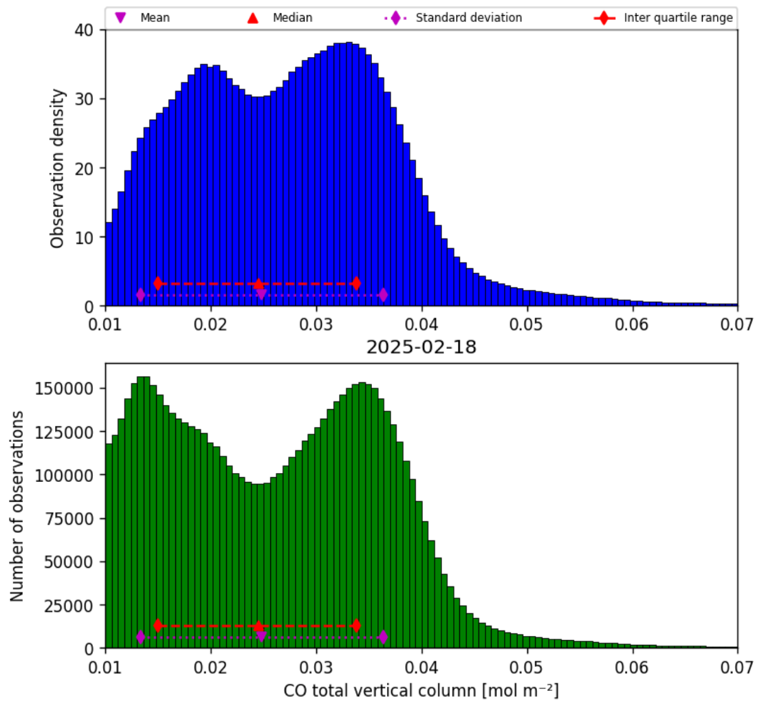
Figure 18: Histogram of “CO total vertical column” for 2025-02-18 to 2025-02-19
