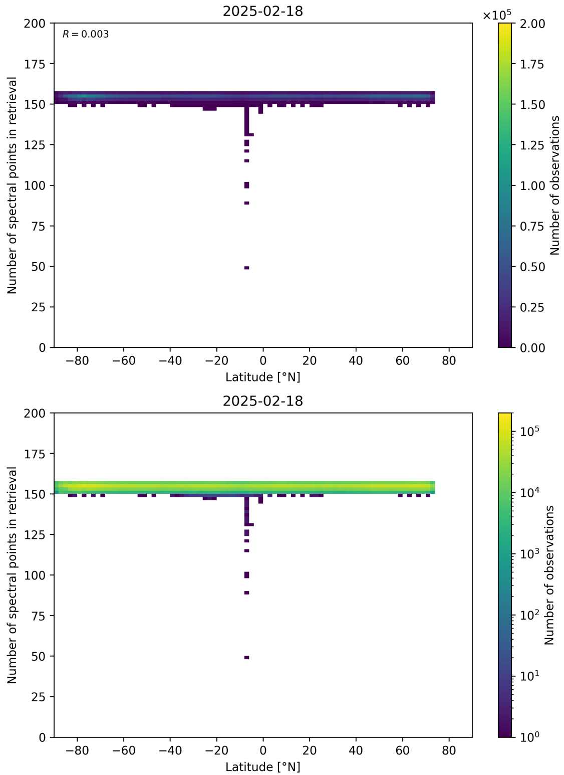
Figure 57: Scatter density plot of “Latitude” against “Number of spectral points in retrieval” for 2025-02-18 to 2025-02-19.
