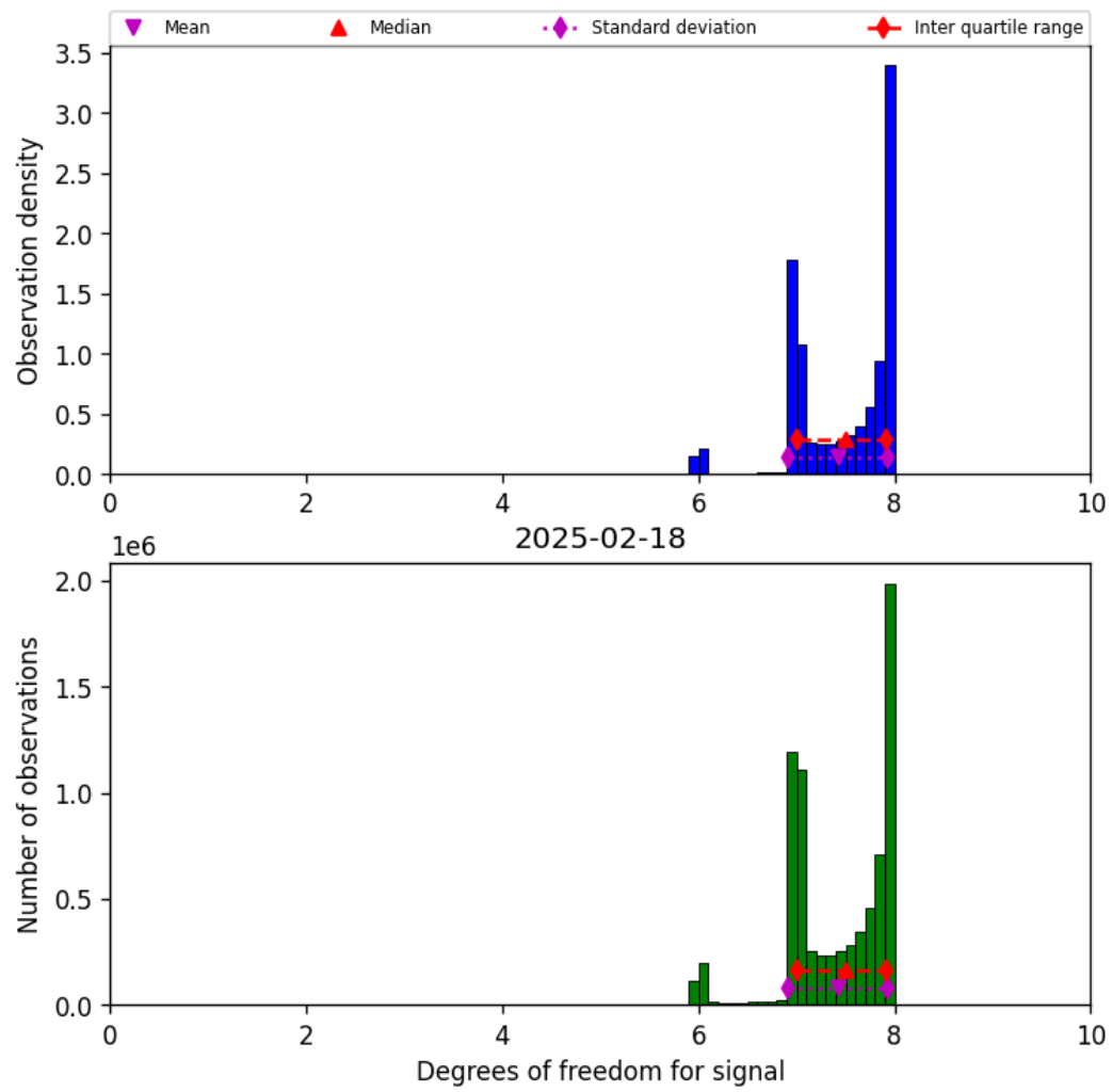
Figure 23: Histogram of “Degrees of freedom for signal” for 2025-02-18 to 2025-02-19
