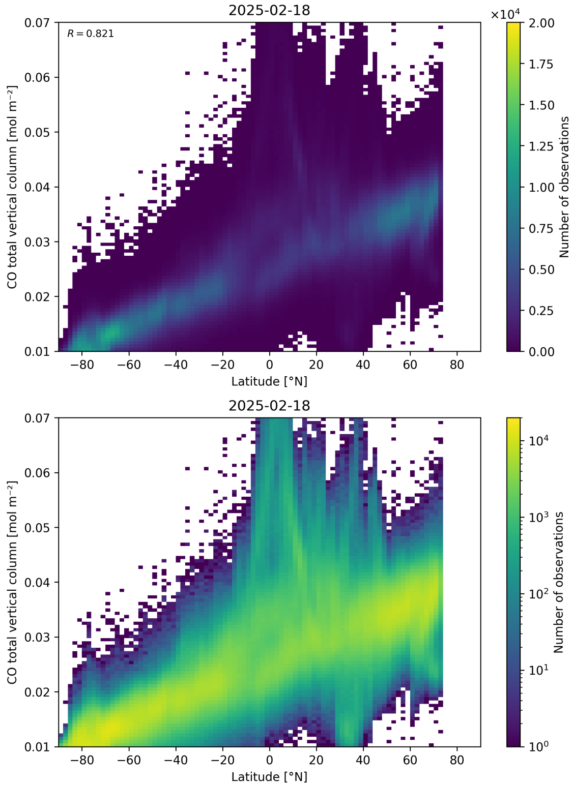
Figure 51: Scatter density plot of “Latitude” against “CO total vertical column” for 2025-02-18 to 2025-02-19.
