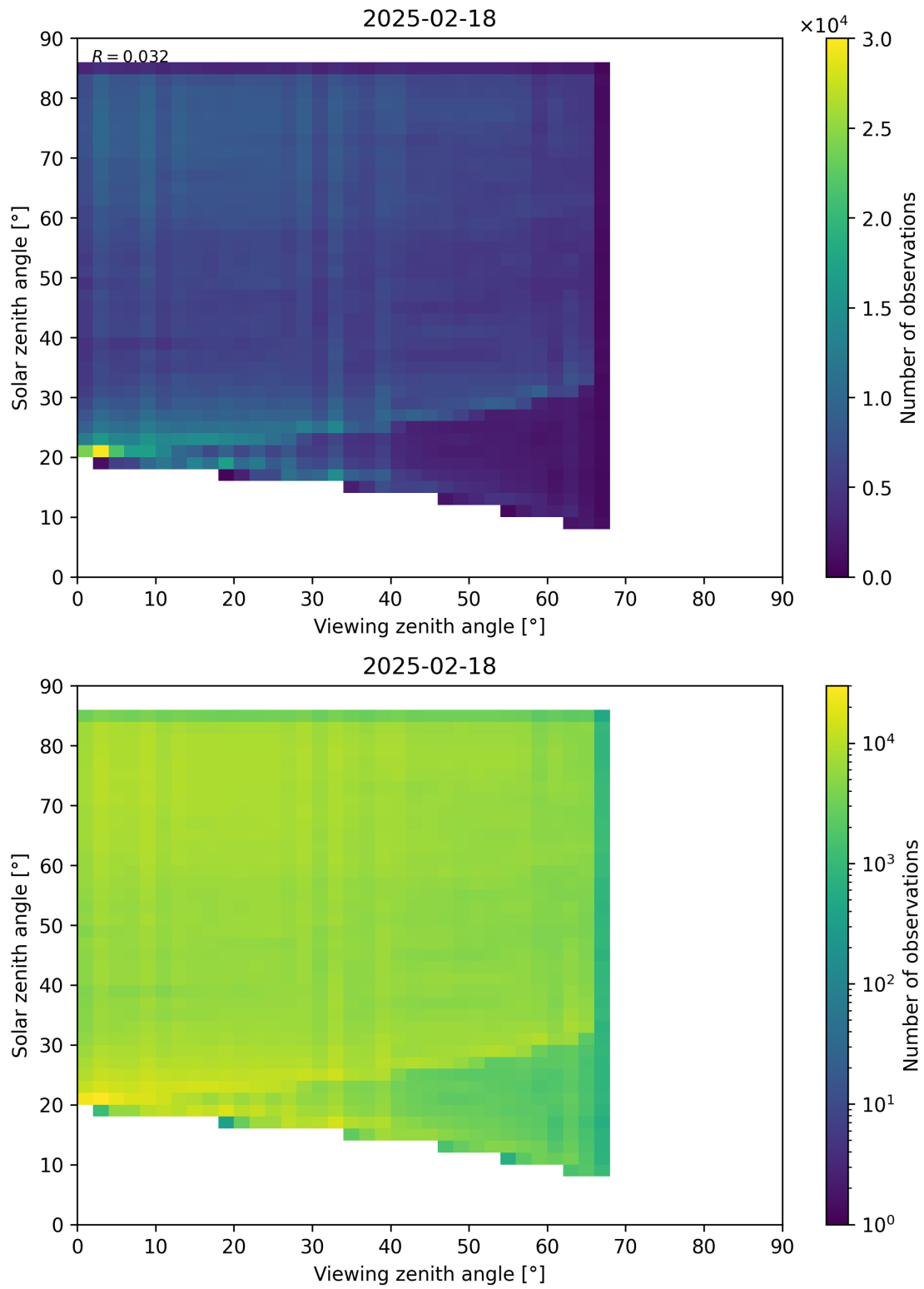
Figure 77: Scatter density plot of “Viewing zenith angle” against “Solar zenith angle” for 2025-02-18 to 2025-02-19.
