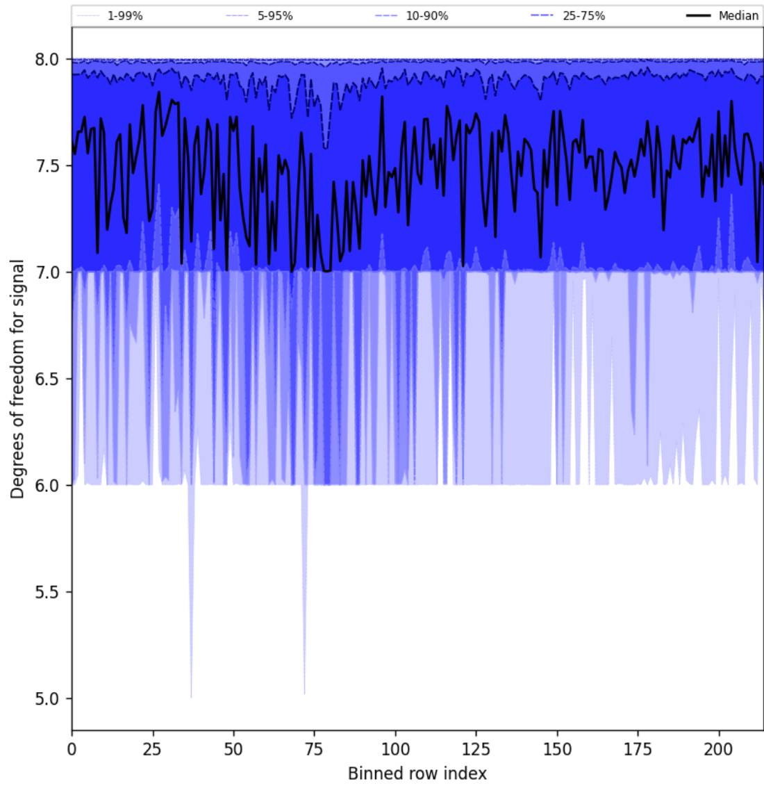
Figure 31: Along track statistics of “Degrees of freedom for signal” for 2025-02-18 to 2025-02-19
