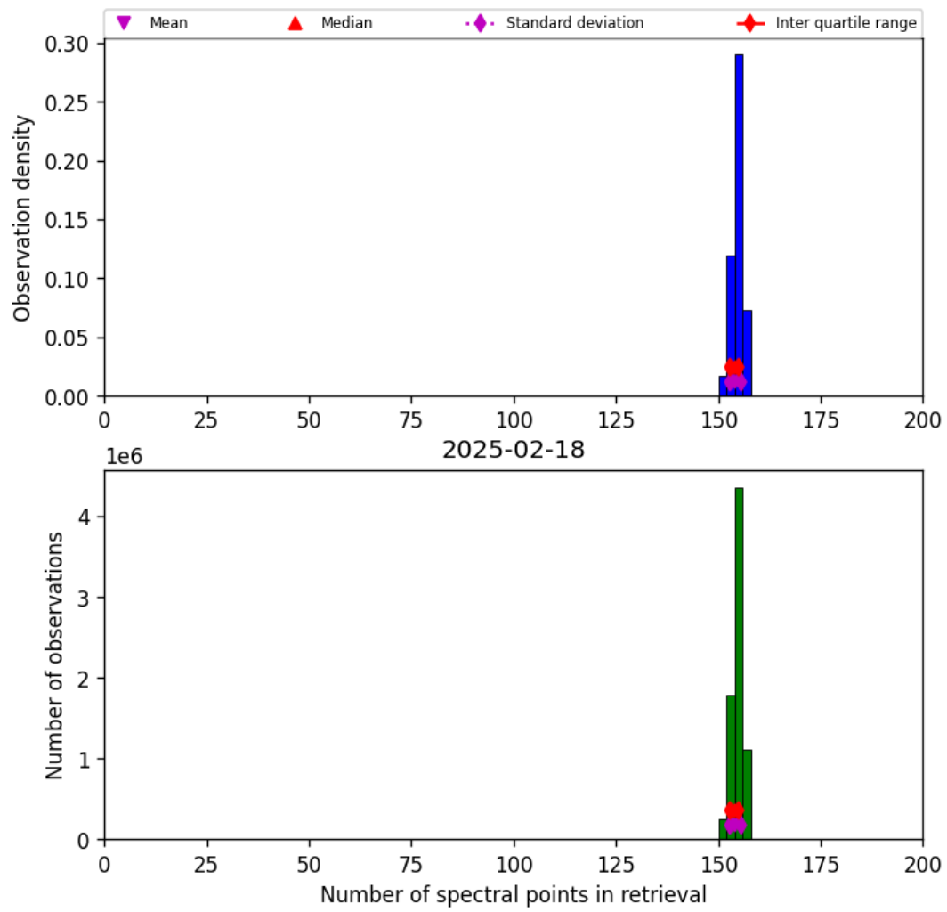
Figure 21: Histogram of “Number of spectral points in retrieval” for 2025-02-18 to 2025-02-19
