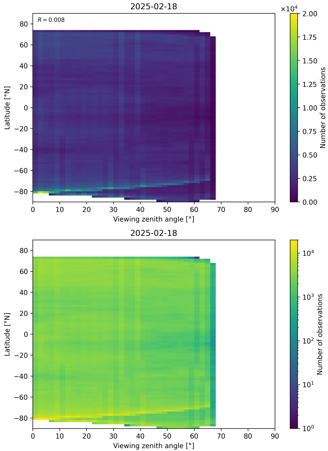
Figure 74: Scatter density plot of “Viewing zenith angle” against “Latitude” for 2025-02-18 to 2025-02-19.
