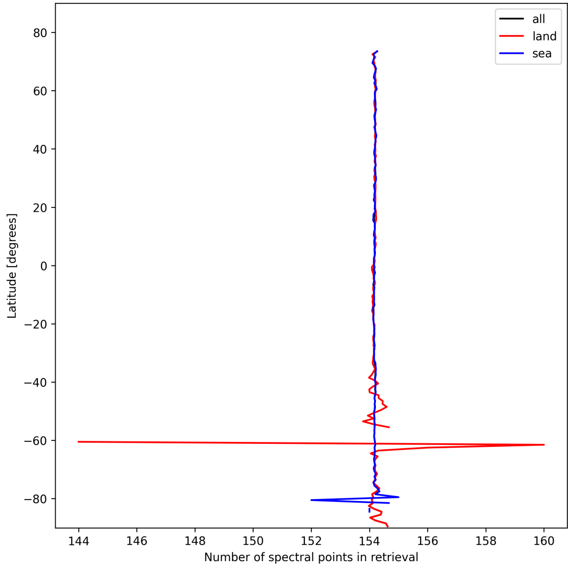
Figure 13: Zonal average of “Number of spectral points in retrieval” for 2025-02-18 to 2025-02-19.
