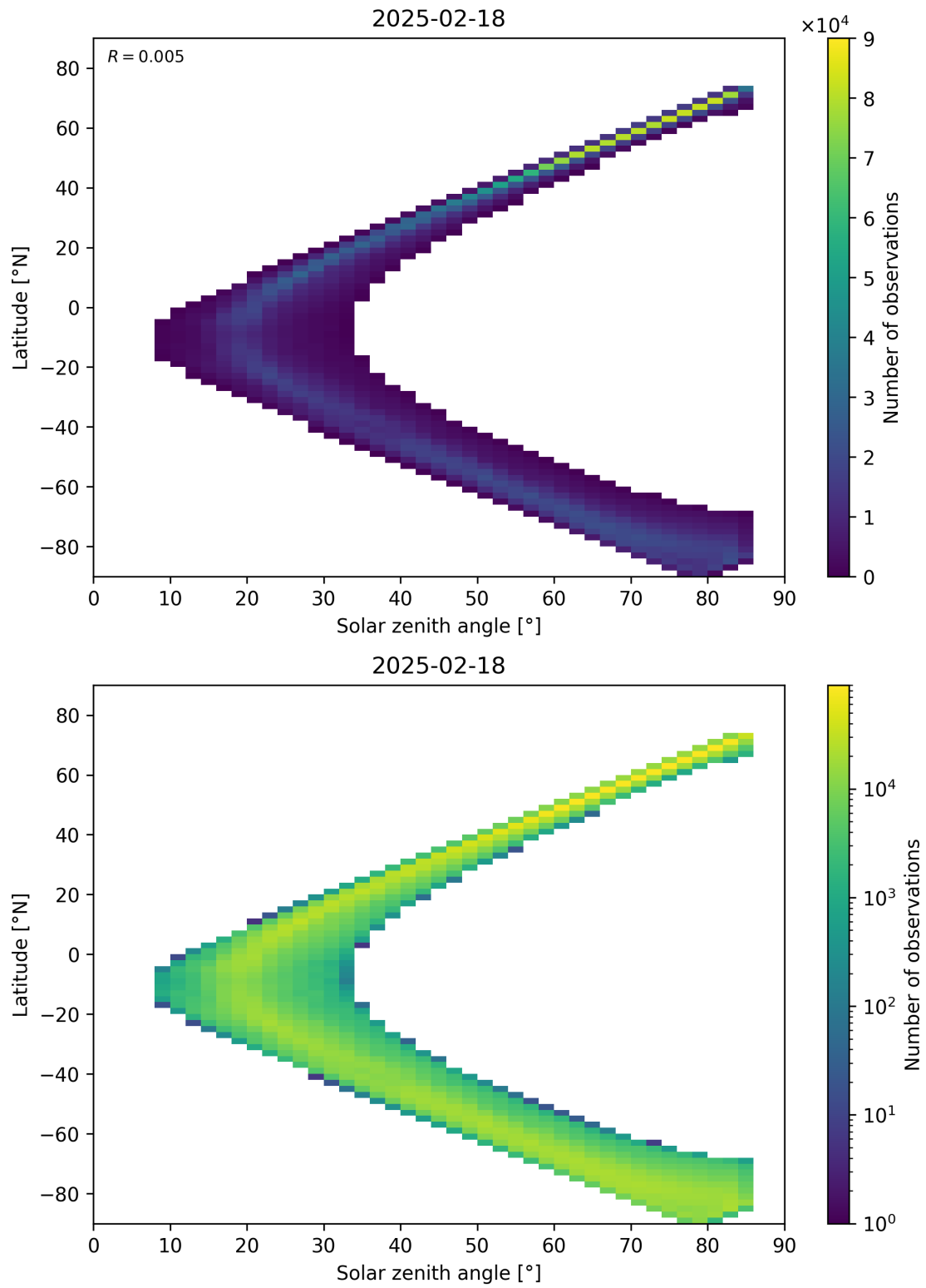
Figure 66: Scatter density plot of “Solar zenith angle” against “Latitude” for 2025-02-18 to 2025-02-19.
