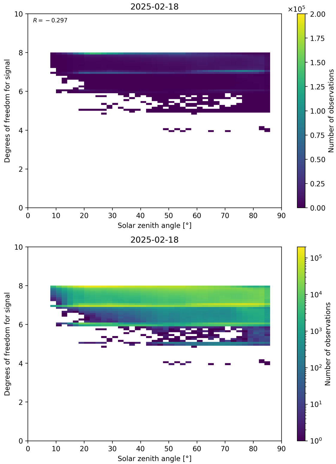
Figure 65: Scatter density plot of “Solar zenith angle” against “Degrees of freedom for signal” for 2025-02-18 to 2025-02-19.
