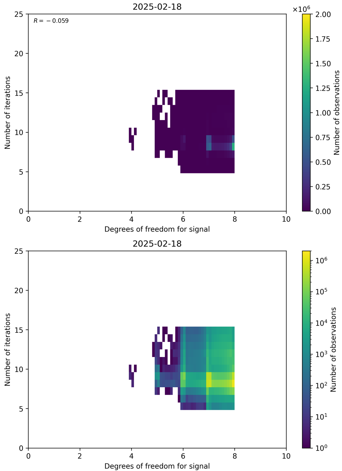
Figure 50: Scatter density plot of “Degrees of freedom for signal” against “Number of iterations” for 2025-02-18 to 2025-02-19.
