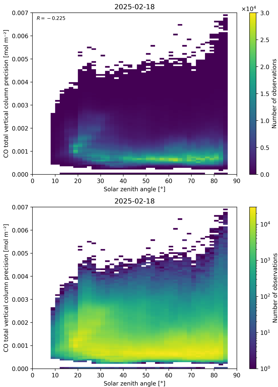
Figure 63: Scatter density plot of “Solar zenith angle” against “CO total vertical column precision” for 2025-02-18 to 2025-02-19.
