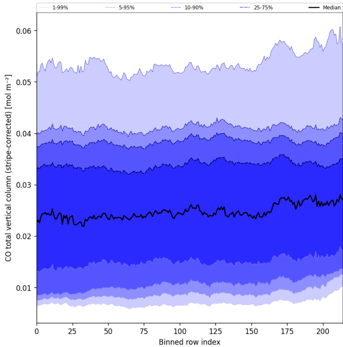
Figure 27: Along track statistics of “CO total vertical column (stripe-corrected)” for 2025-02-18 to 2025-02-19
