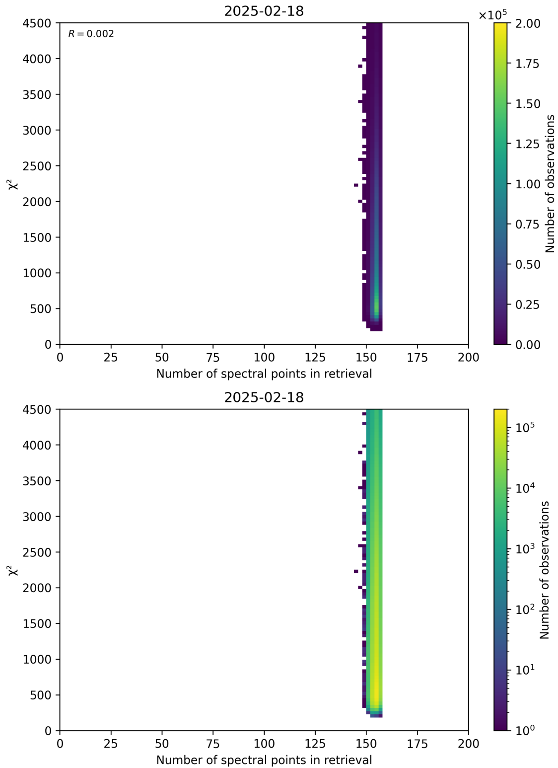
Figure 58: Scatter density plot of “Number of spectral points in retrieval” against “ \chi^2 ” for 2025-02-18 to 2025-02-19.
