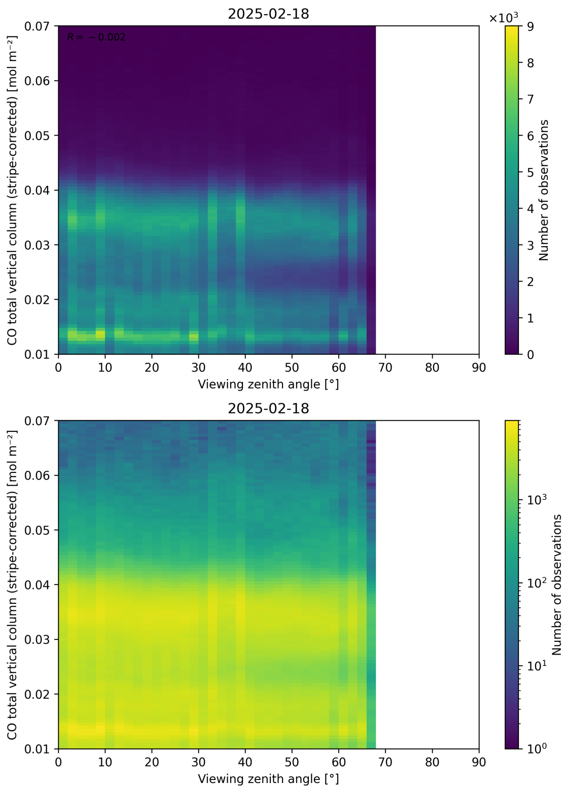
Figure 70: Scatter density plot of “Viewing zenith angle” against “CO total vertical column (stripe-corrected)” for 2025-02-18 to 2025-02-19.
