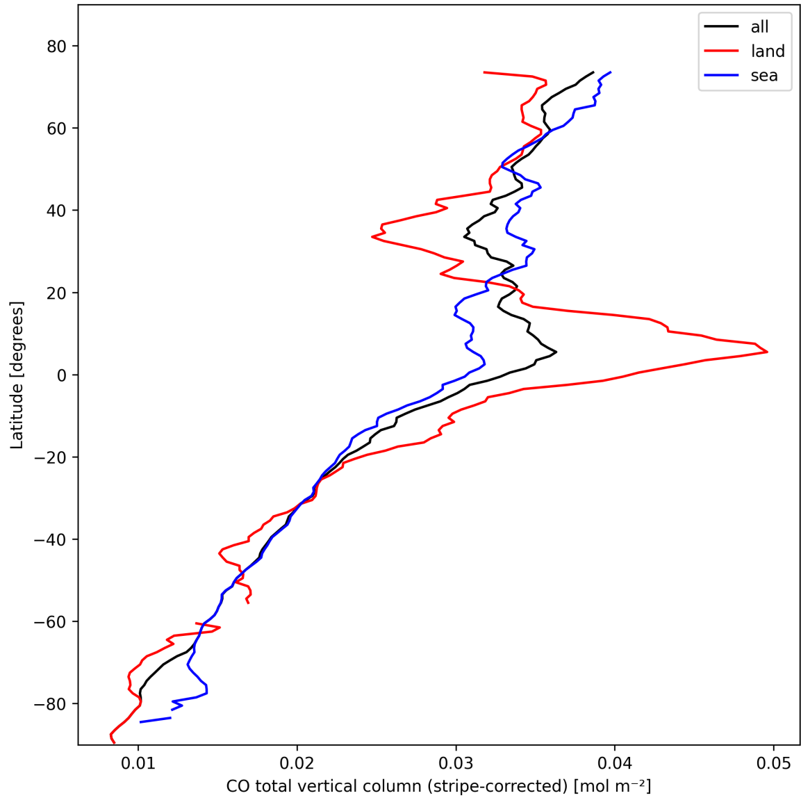
Figure 11: Zonal average of “CO total vertical column (stripe-corrected)” for 2025-02-18 to 2025-02-19.
