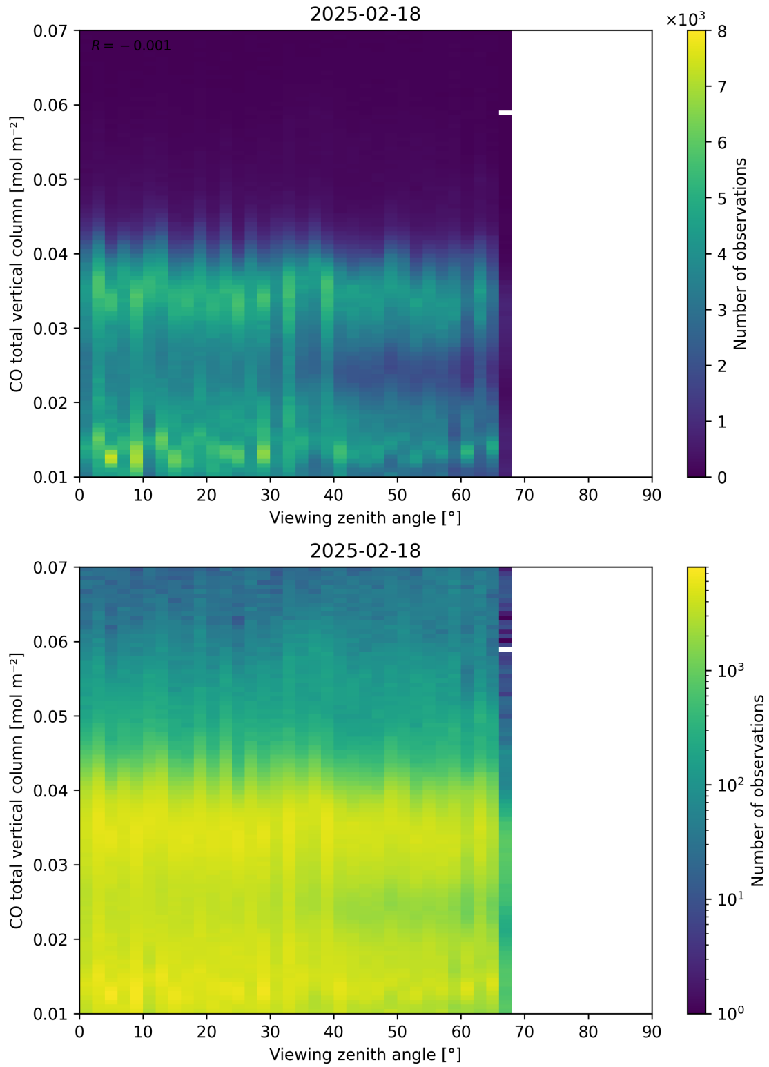
Figure 69: Scatter density plot of “Viewing zenith angle” against “CO total vertical column” for 2025-02-18 to 2025-02-19.
