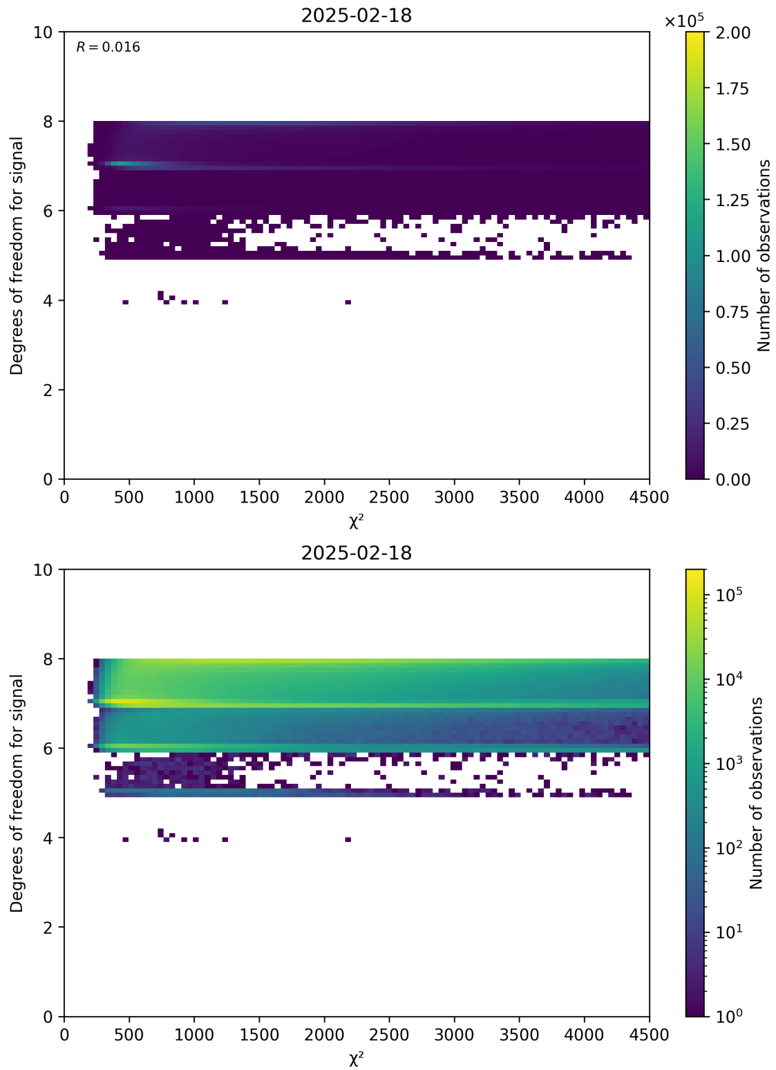
Figure 48: Scatter density plot of “ \chi^2 ” against “Degrees of freedom for signal” for 2025-02-18 to 2025-02-19.
