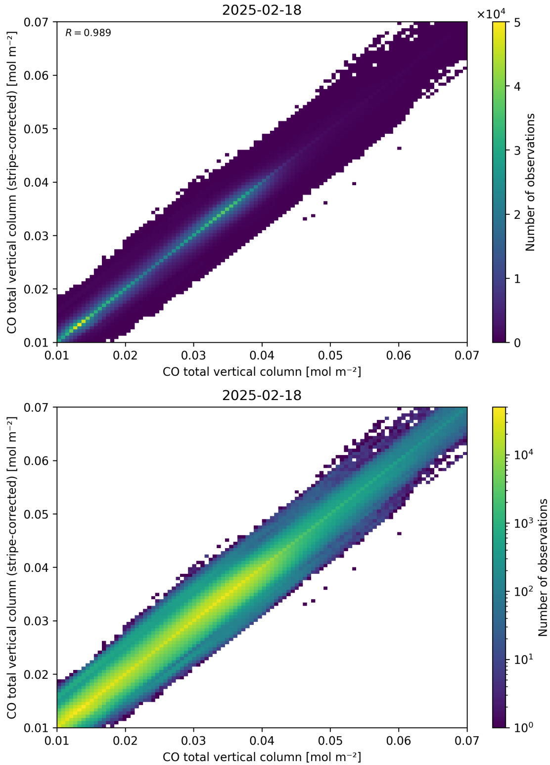
Figure 33: Scatter density plot of “CO total vertical column” against “CO total vertical column (stripe-corrected)” for 2025-02-18 to 2025-02-19.
