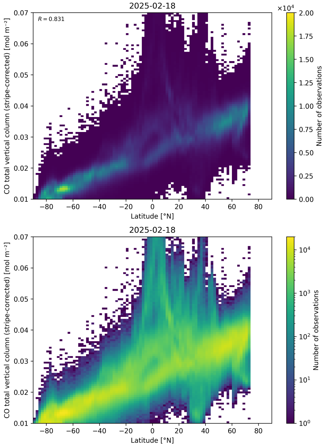
Figure 52: Scatter density plot of “Latitude” against “CO total vertical column (stripe-corrected)” for 2025-02-18 to 2025-02-19.
