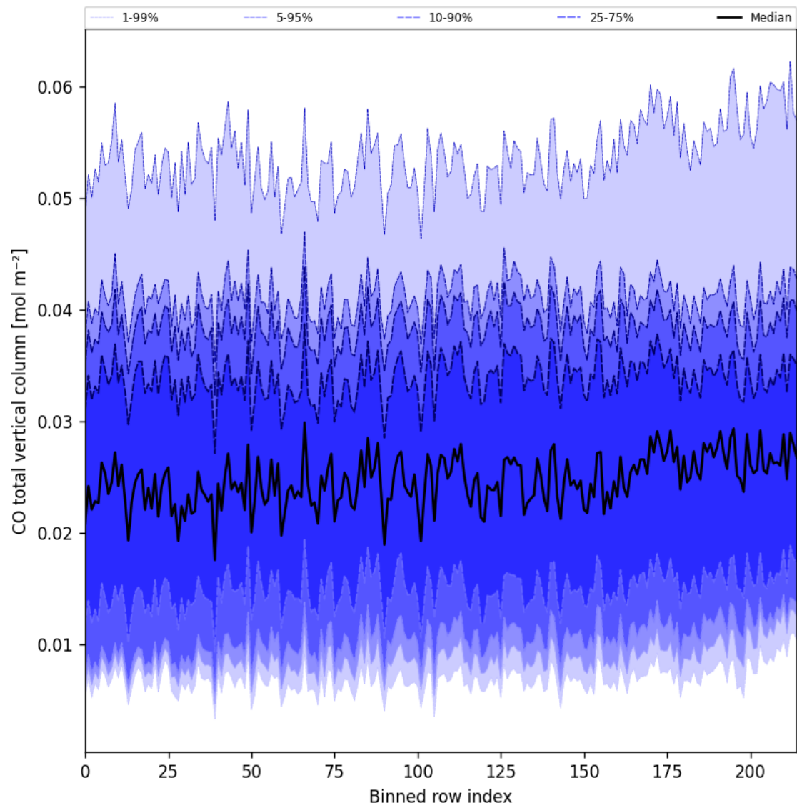
Figure 26: Along track statistics of “CO total vertical column” for 2025-02-18 to 2025-02-19
