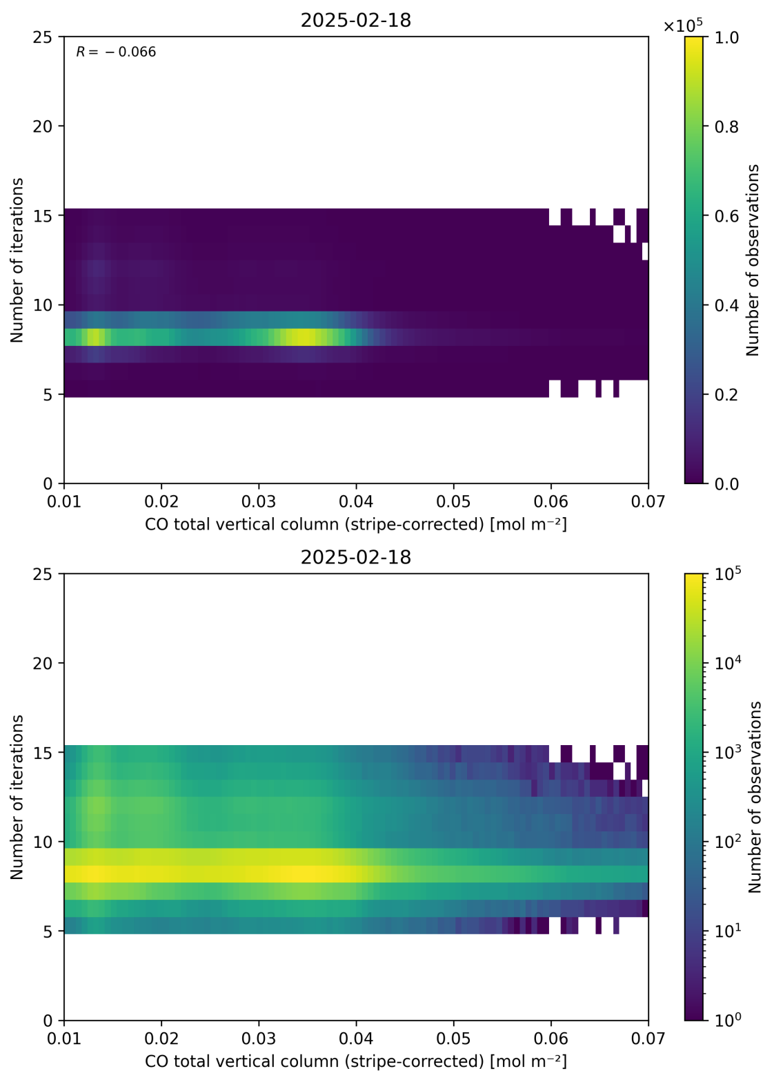
Figure 39: Scatter density plot of “CO total vertical column (stripe-corrected)” against “Number of iterations” for 2025-02-18 to 2025-02-19.
