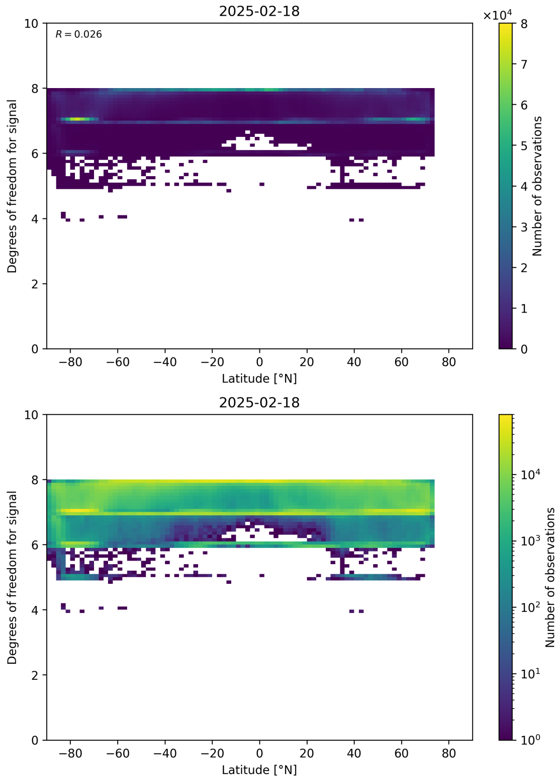
Figure 55: Scatter density plot of “Latitude” against “Degrees of freedom for signal” for 2025-02-18 to 2025-02-19.
