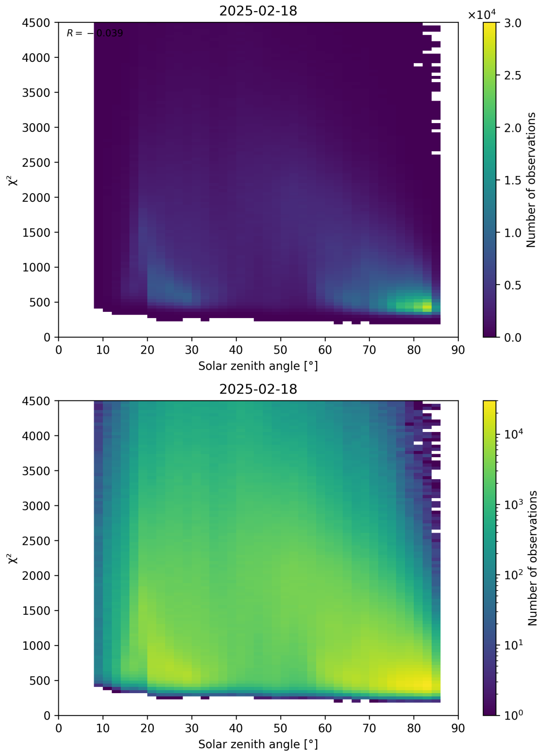
Figure 64: Scatter density plot of “Solar zenith angle” against “ \chi^2 ” for 2025-02-18 to 2025-02-19.
