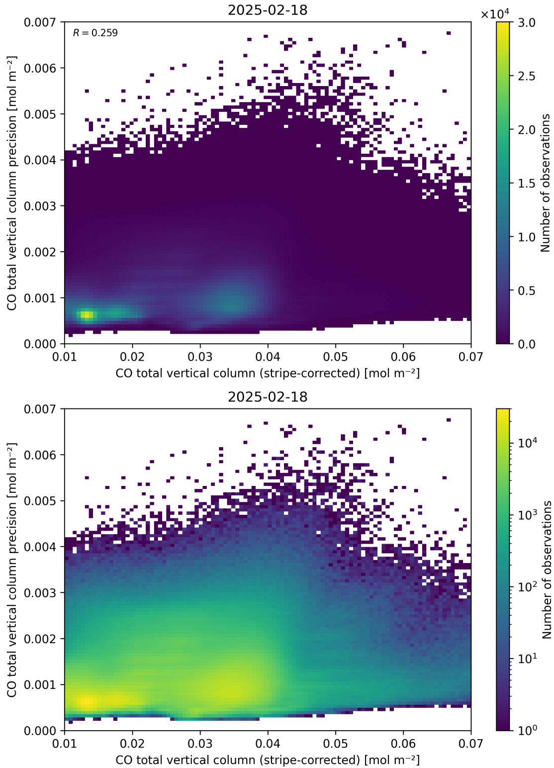
Figure 36: Scatter density plot of “CO total vertical column (stripe-corrected)” against “CO total vertical column precision” for 2025-02-18 to 2025-02-19.
