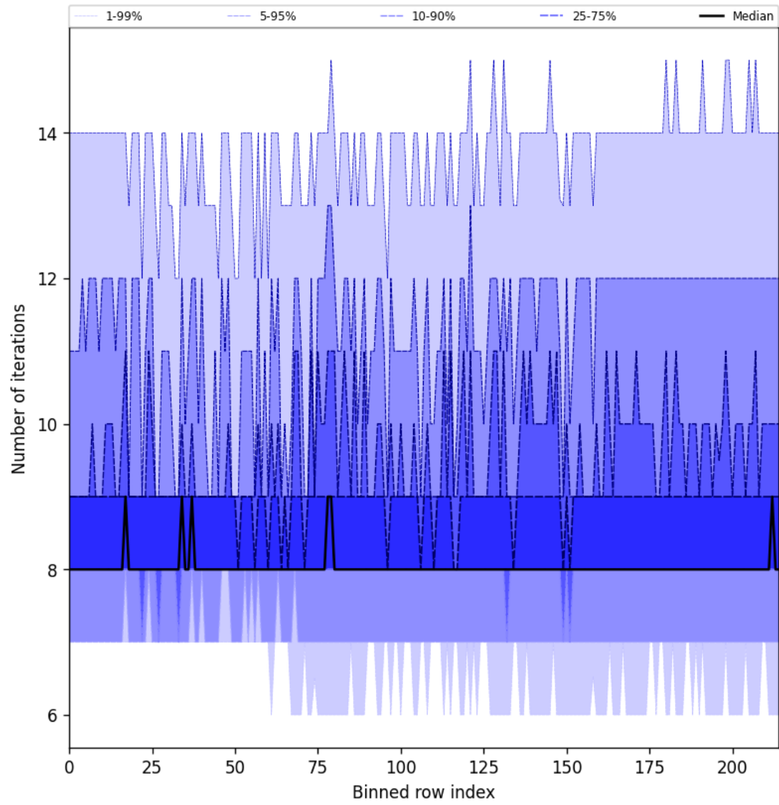
Figure 32: Along track statistics of “Number of iterations” for 2025-02-18 to 2025-02-19
