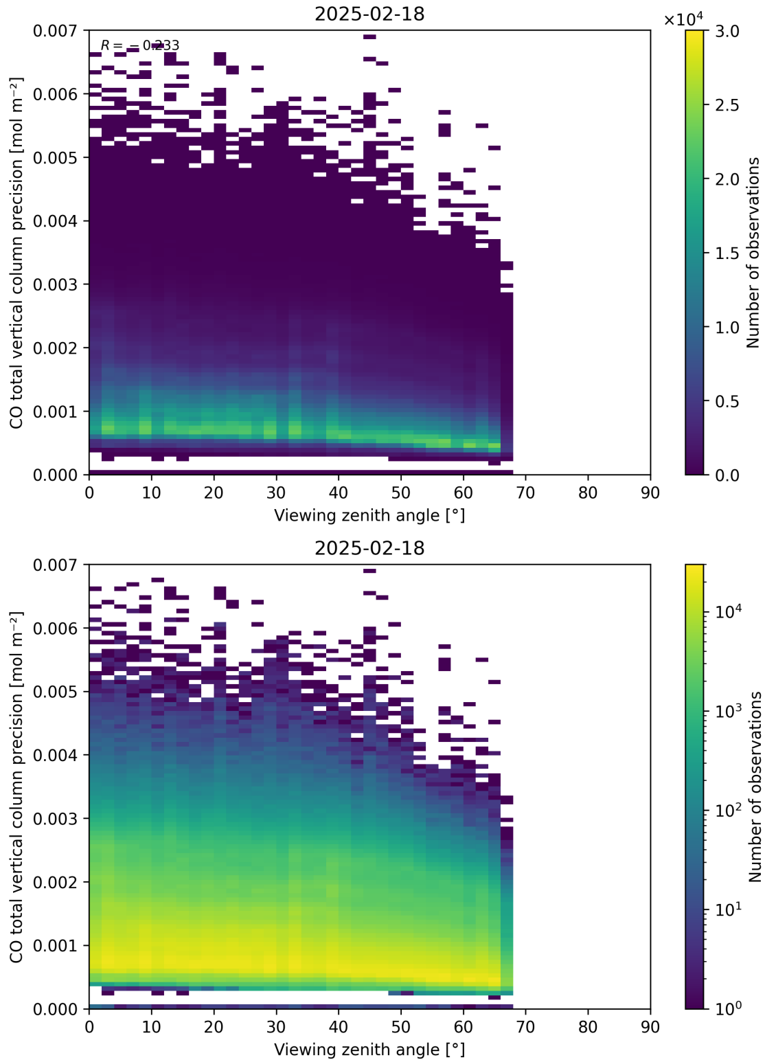
Figure 71: Scatter density plot of “Viewing zenith angle” against “CO total vertical column precision” for 2025-02-18 to 2025-02-19.
