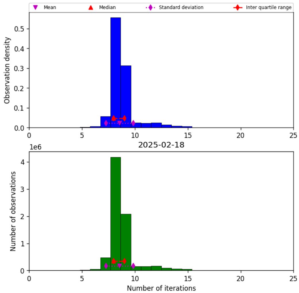
Figure 24: Histogram of “Number of iterations” for 2025-02-18 to 2025-02-19
