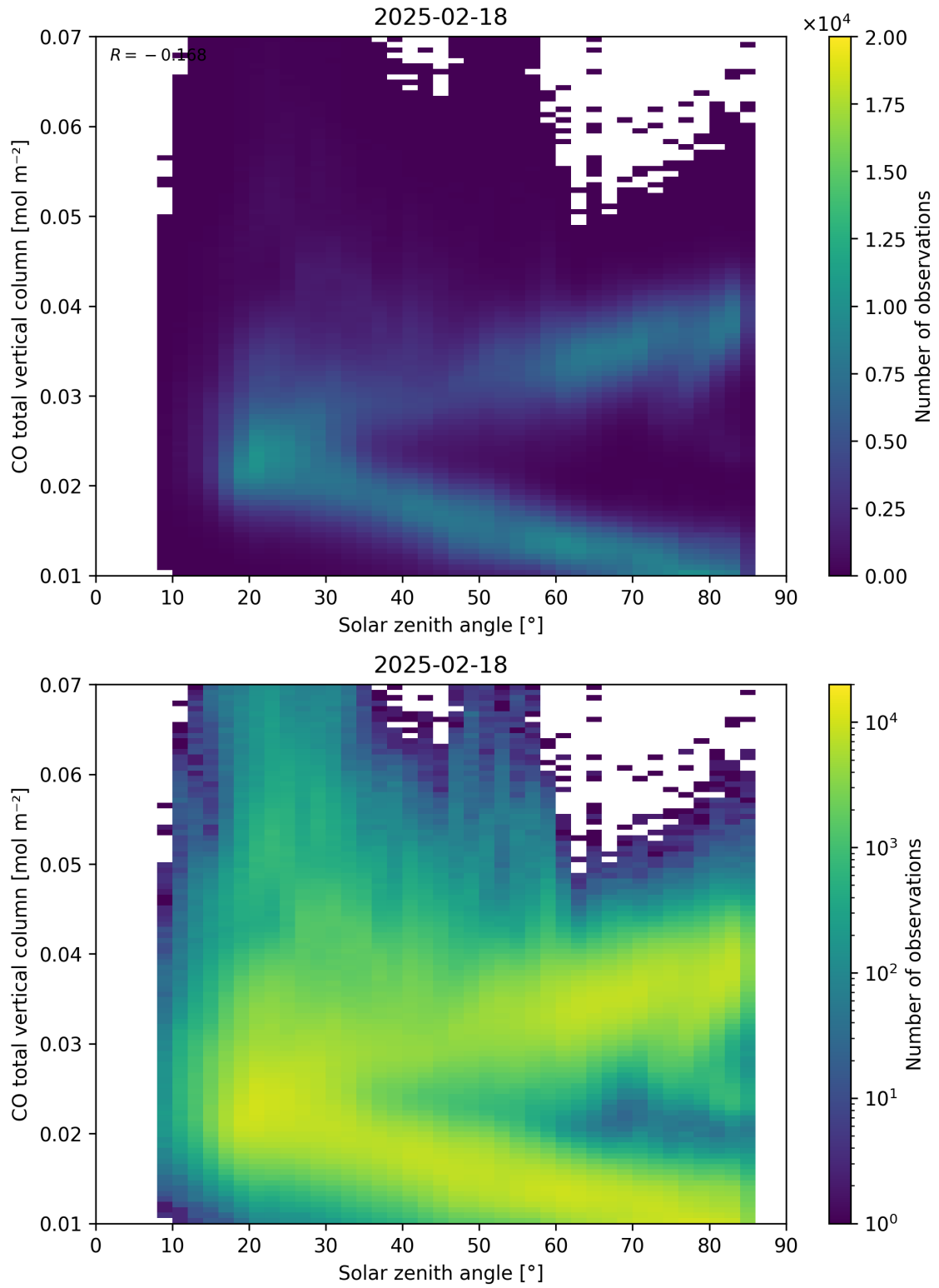
Figure 61: Scatter density plot of “Solar zenith angle” against “CO total vertical column” for 2025-02-18 to 2025-02-19.
