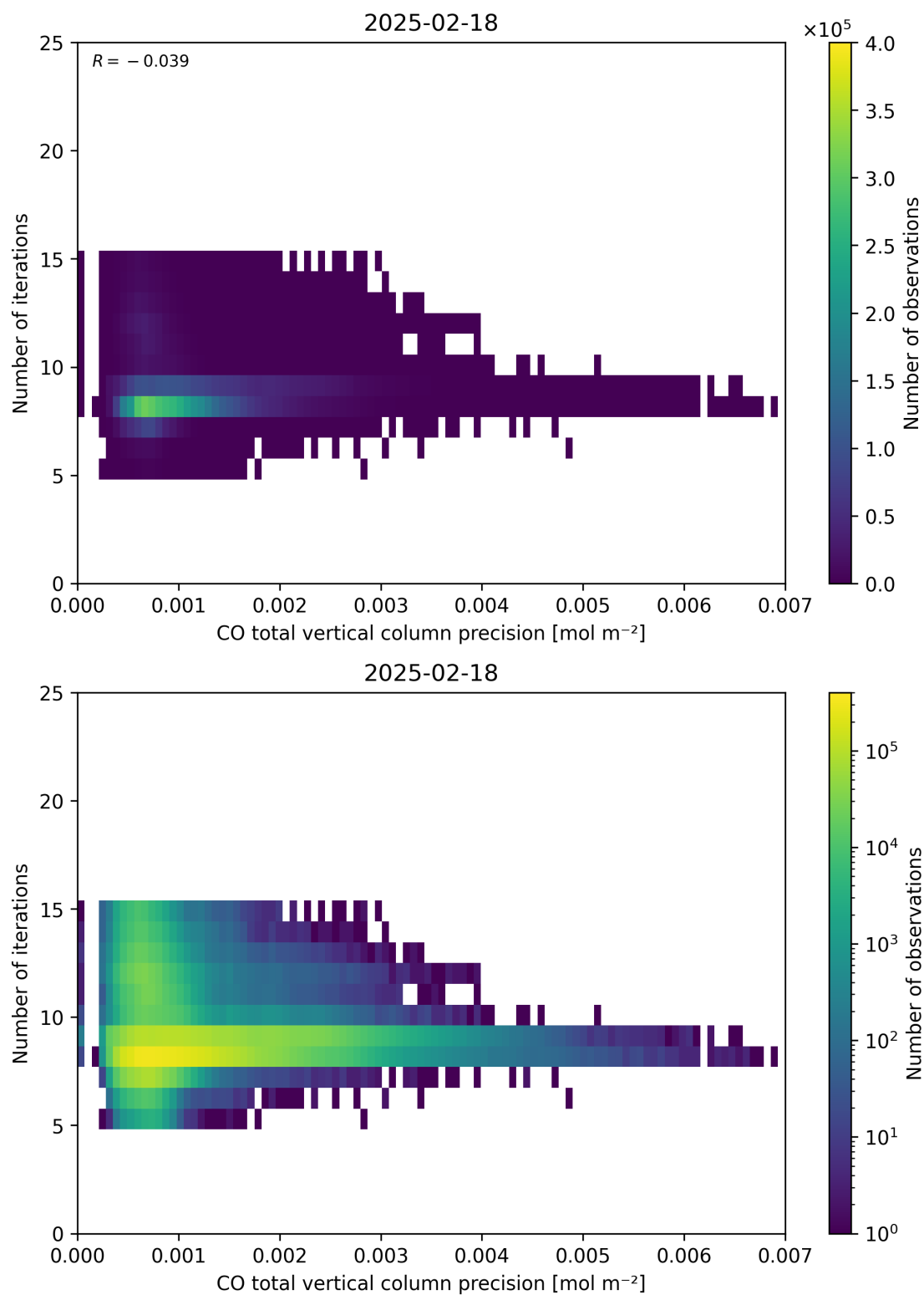
Figure 46: Scatter density plot of “CO total vertical column precision” against “Number of iterations” for 2025-02-18 to 2025-02-19.
