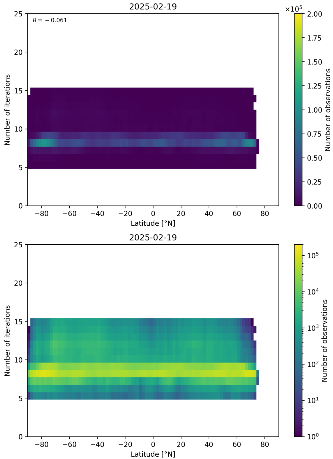
Figure 56: Scatter density plot of “Latitude” against “Number of iterations” for 2025-02-19 to 2025-02-20.
