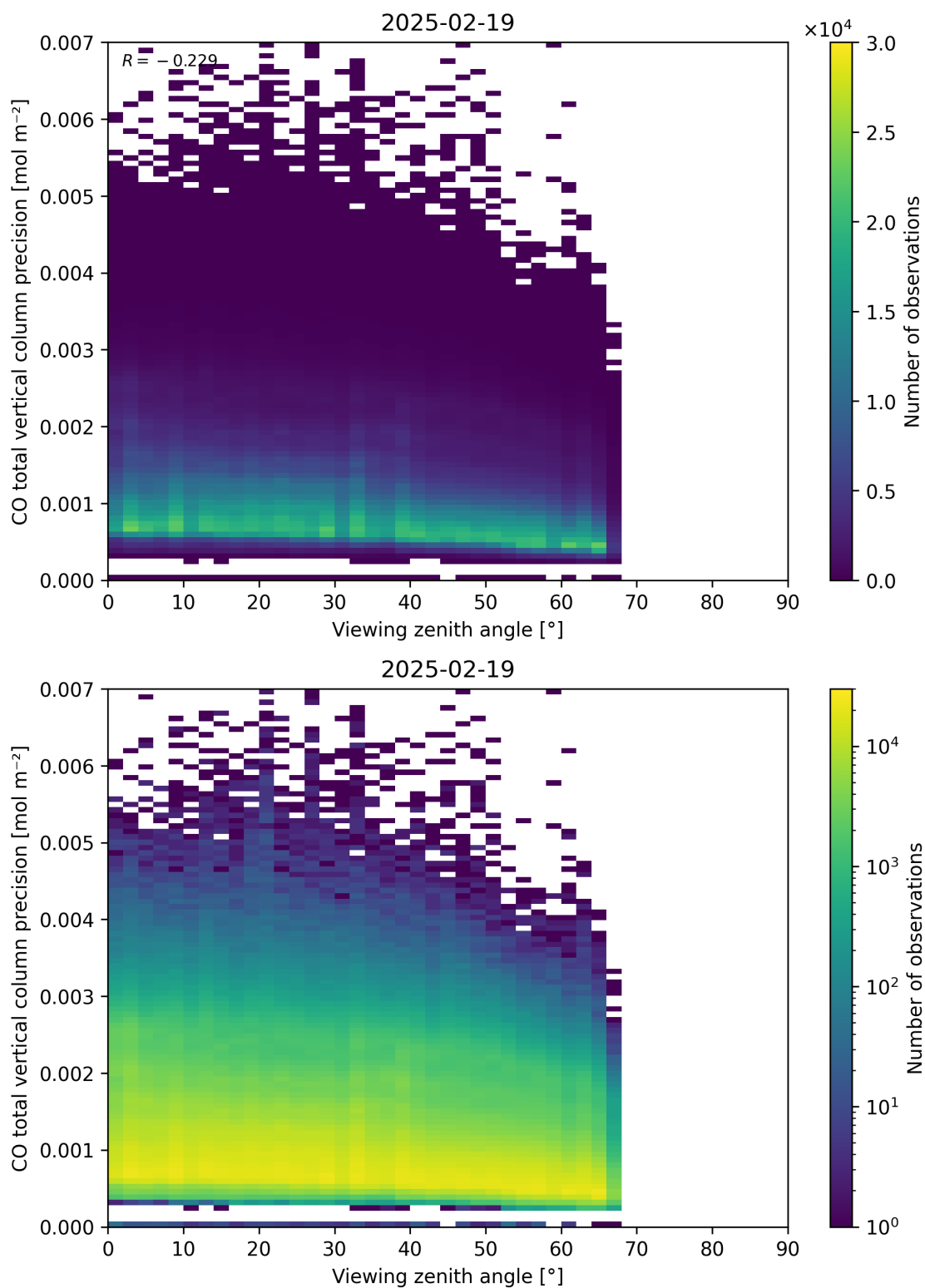
Figure 71: Scatter density plot of “Viewing zenith angle” against “CO total vertical column precision” for 2025-02-19 to 2025-02-20.
