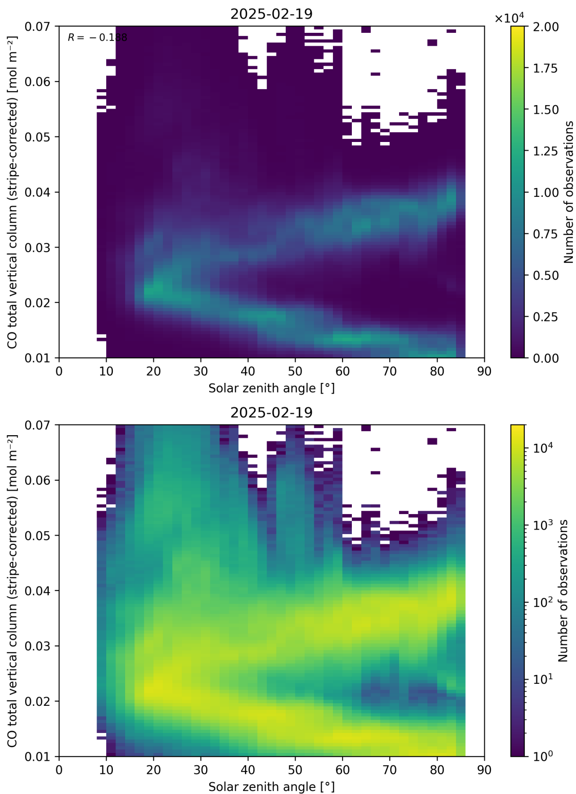
Figure 62: Scatter density plot of “Solar zenith angle” against “CO total vertical column (stripe-corrected)” for 2025-02-19 to 2025-02-20.
