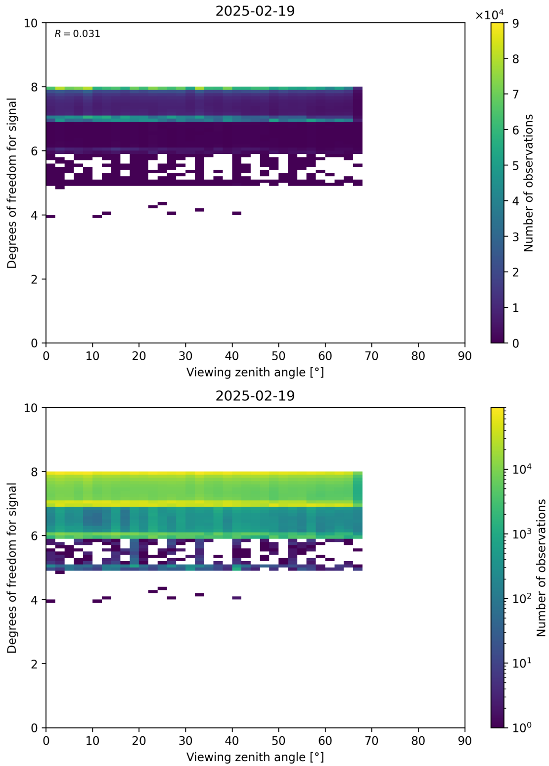
Figure 73: Scatter density plot of “Viewing zenith angle” against “Degrees of freedom for signal” for 2025-02-19 to 2025-02-20.
