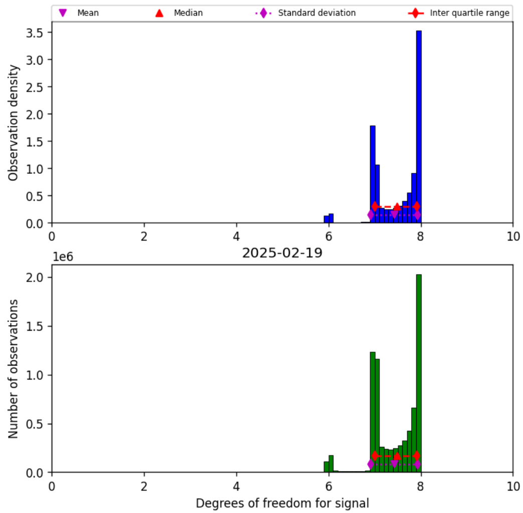
Figure 23: Histogram of “Degrees of freedom for signal” for 2025-02-19 to 2025-02-20
