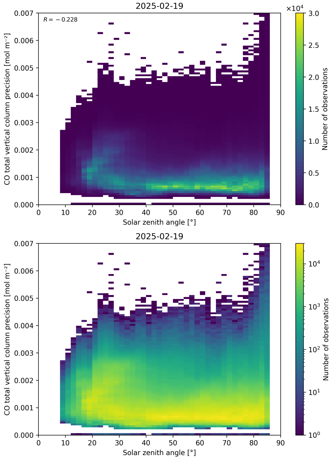
Figure 63: Scatter density plot of “Solar zenith angle” against “CO total vertical column precision” for 2025-02-19 to 2025-02-20.
