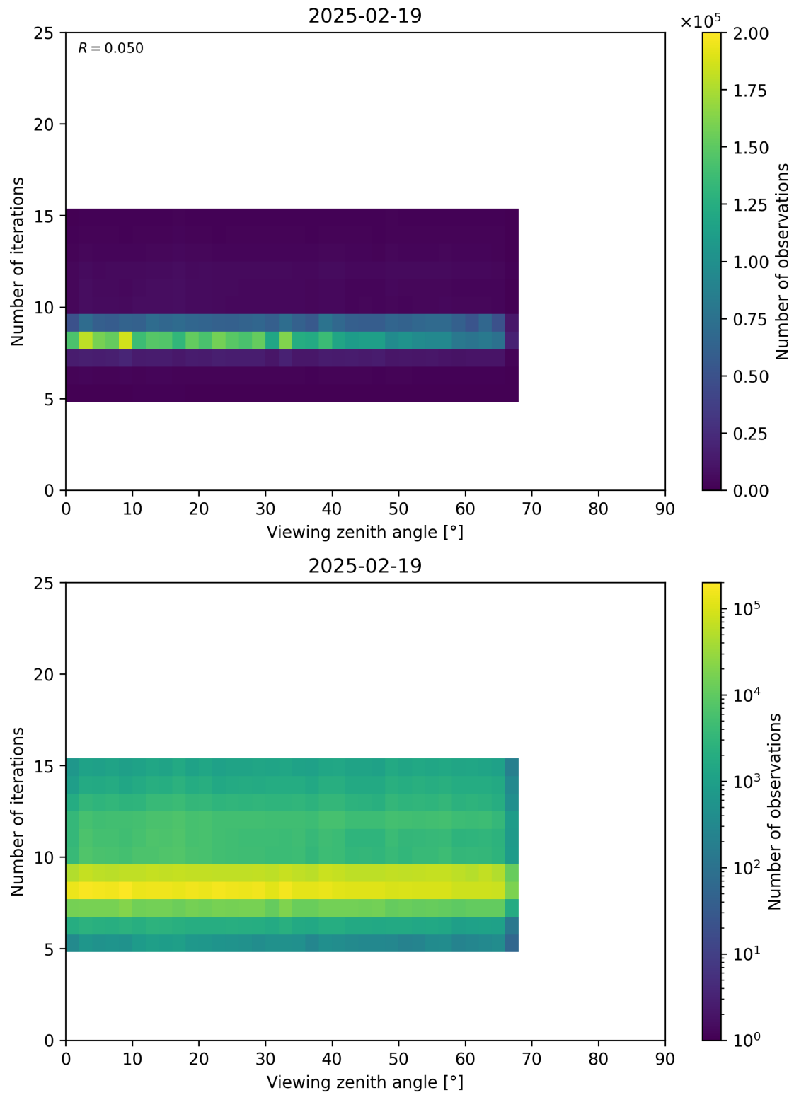
Figure 75: Scatter density plot of “Viewing zenith angle” against “Number of iterations” for 2025-02-19 to 2025-02-20.
