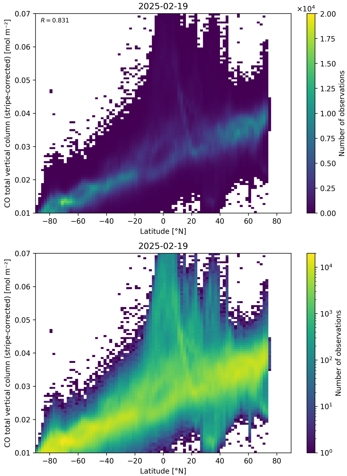
Figure 52: Scatter density plot of “Latitude” against “CO total vertical column (stripe-corrected)” for 2025-02-19 to 2025-02-20.
