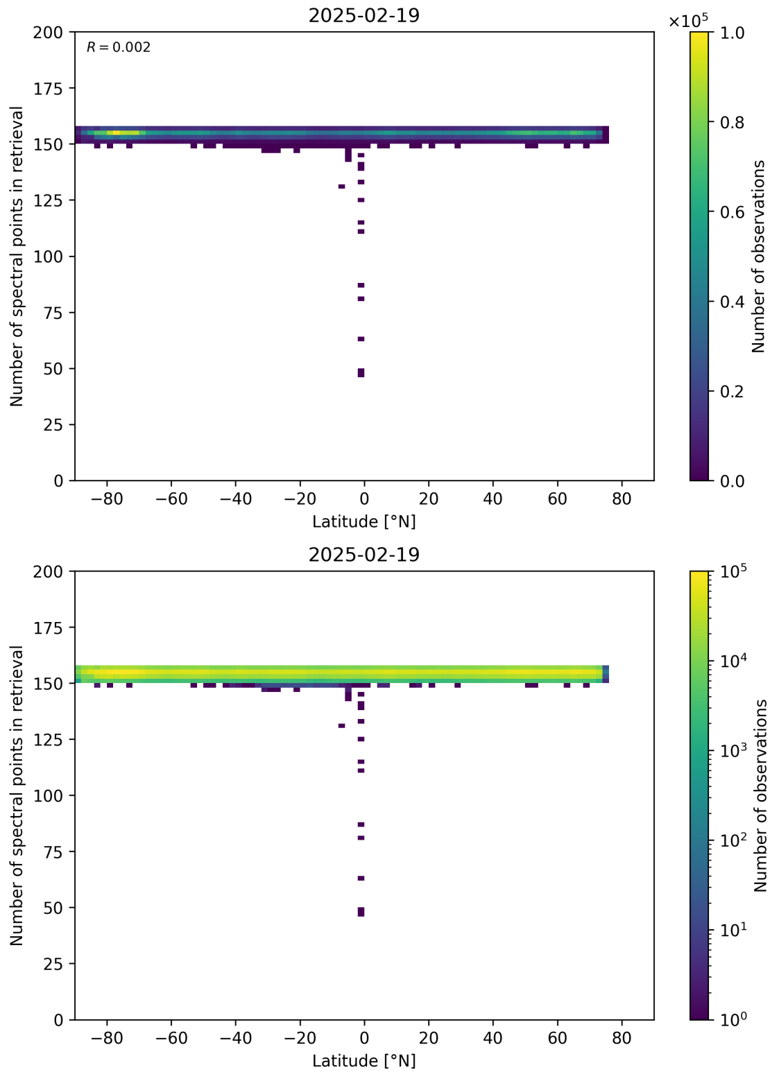
Figure 57: Scatter density plot of “Latitude” against “Number of spectral points in retrieval” for 2025-02-19 to 2025-02-20.
