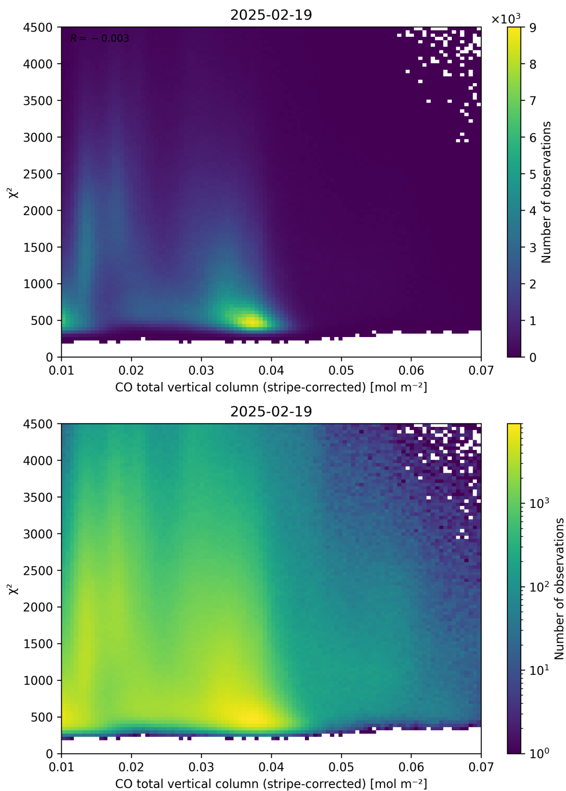
Figure 37: Scatter density plot of “CO total vertical column (stripe-corrected)” against “ \chi^2 ” for 2025-02-19 to 2025-02-20.
