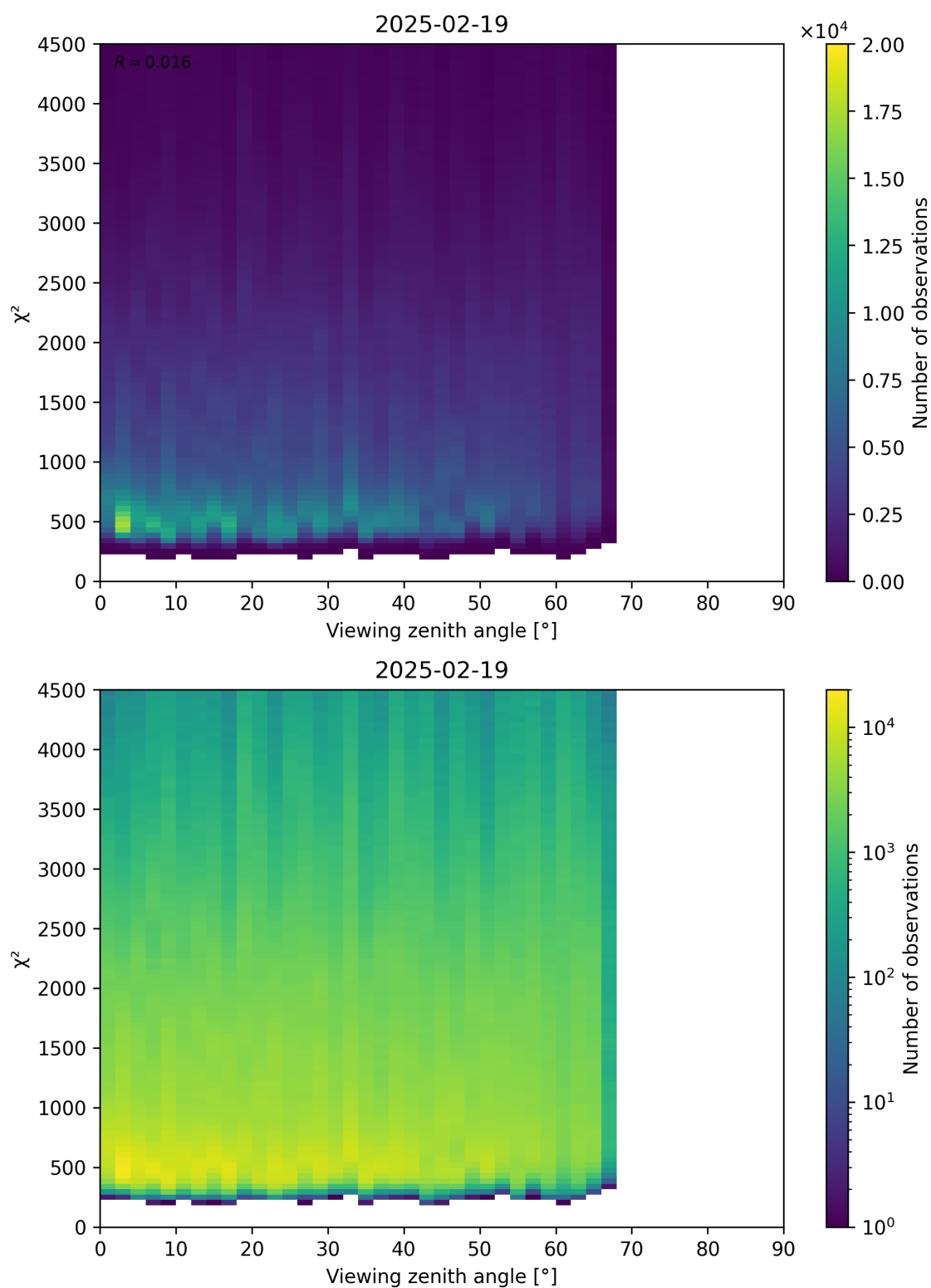
Figure 72: Scatter density plot of “Viewing zenith angle” against “ \chi^2 ” for 2025-02-19 to 2025-02-20.
