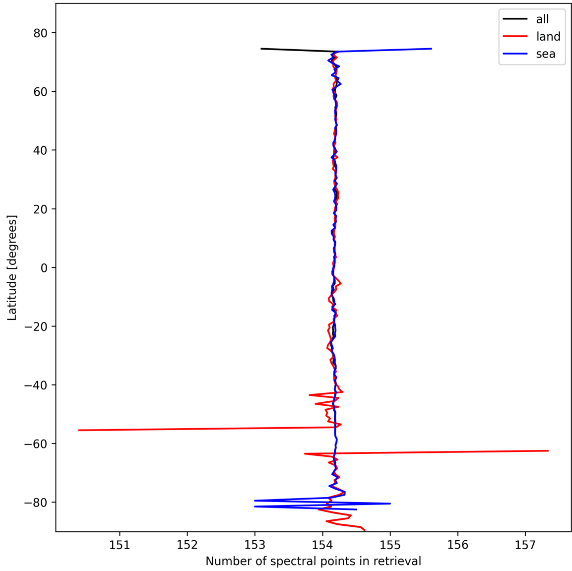
Figure 13: Zonal average of “Number of spectral points in retrieval” for 2025-02-19 to 2025-02-20.
