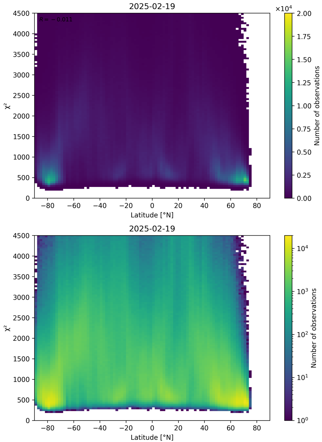
Figure 54: Scatter density plot of “Latitude” against “ \chi^2 ” for 2025-02-19 to 2025-02-20.
