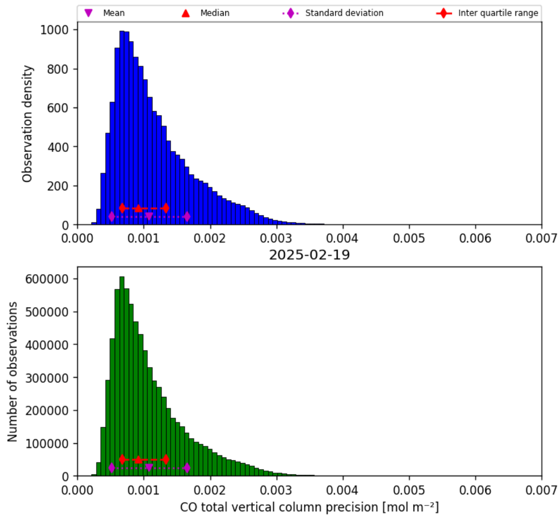
Figure 20: Histogram of “CO total vertical column precision” for 2025-02-19 to 2025-02-20
