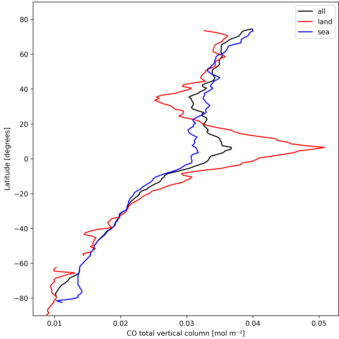
Figure 10: Zonal average of “CO total vertical column” for 2025-02-19 to 2025-02-20.
