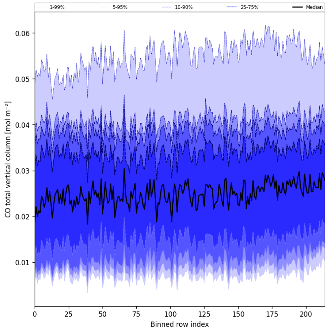
Figure 26: Along track statistics of “CO total vertical column” for 2025-02-19 to 2025-02-20
