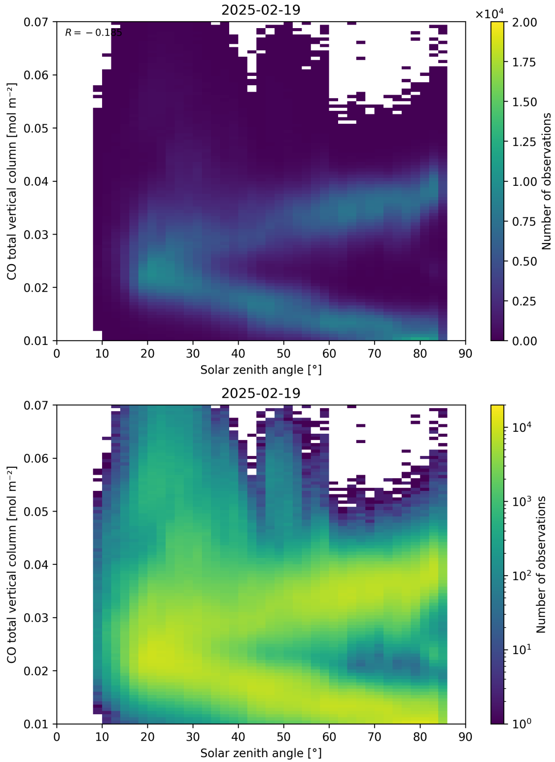
Figure 61: Scatter density plot of “Solar zenith angle” against “CO total vertical column” for 2025-02-19 to 2025-02-20.
