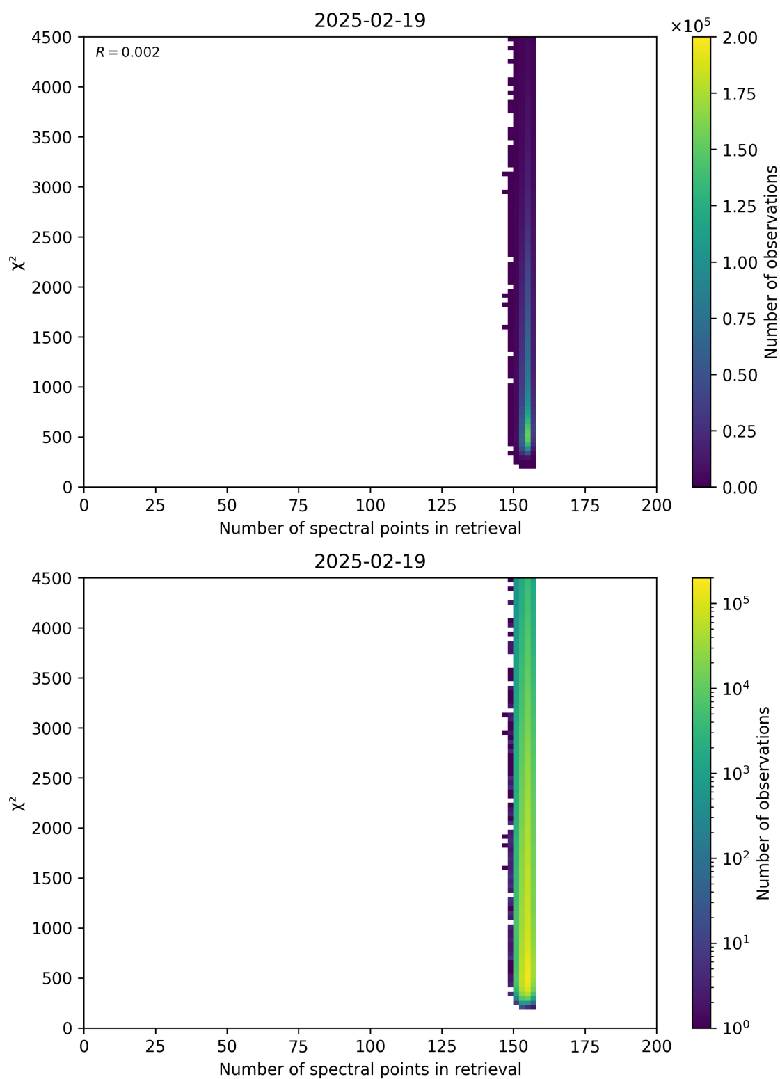
Figure 58: Scatter density plot of “Number of spectral points in retrieval” against “ \chi^2 ” for 2025-02-19 to 2025-02-20.
