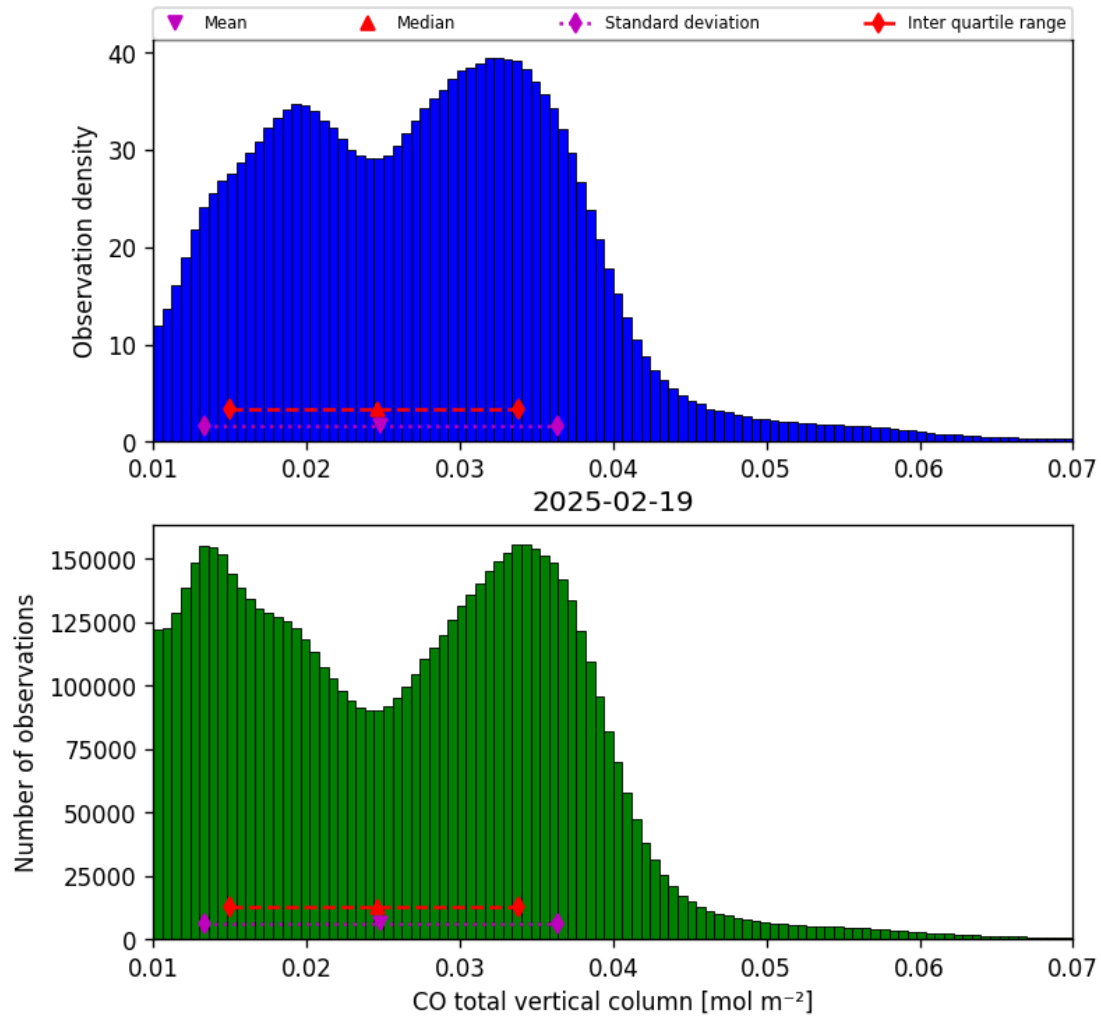
Figure 18: Histogram of “CO total vertical column” for 2025-02-19 to 2025-02-20
