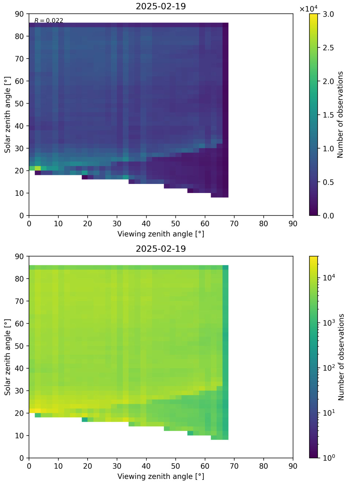
Figure 77: Scatter density plot of “Viewing zenith angle” against “Solar zenith angle” for 2025-02-19 to 2025-02-20.
