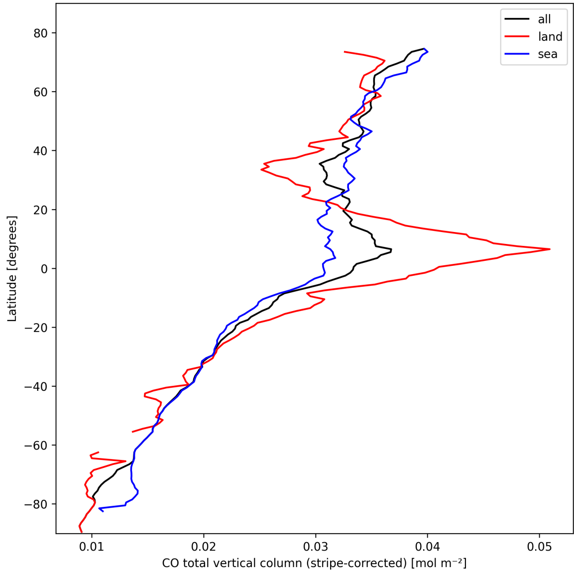
Figure 11: Zonal average of “CO total vertical column (stripe-corrected)” for 2025-02-19 to 2025-02-20.
