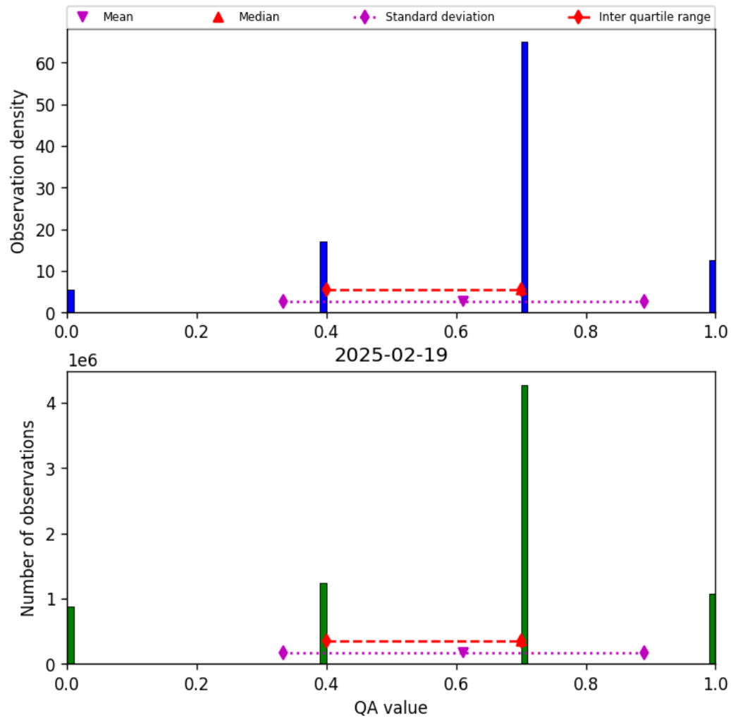
Figure 17: Histogram of “QA value” for 2025-02-19 to 2025-02-20
