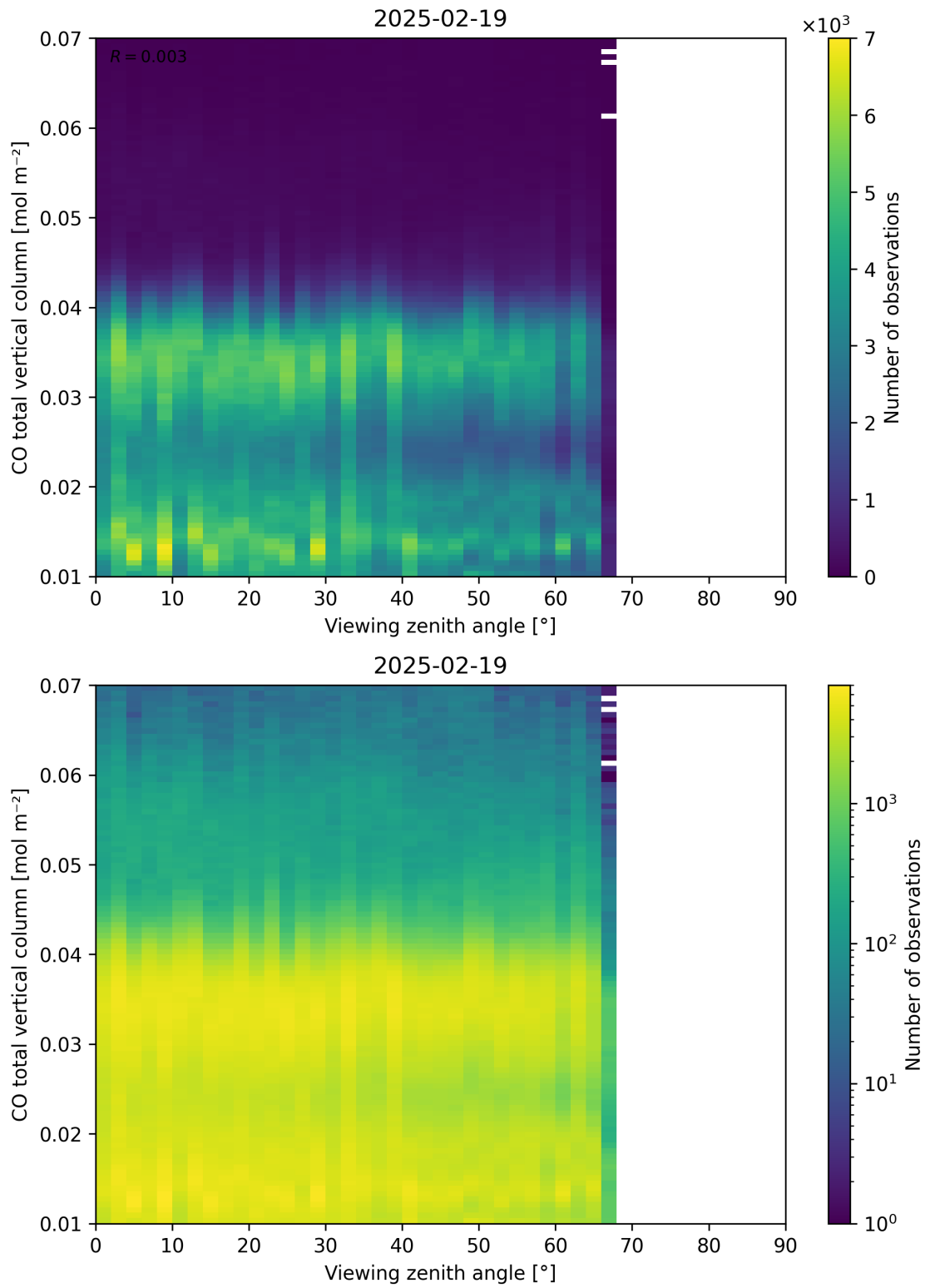
Figure 69: Scatter density plot of “Viewing zenith angle” against “CO total vertical column” for 2025-02-19 to 2025-02-20.
