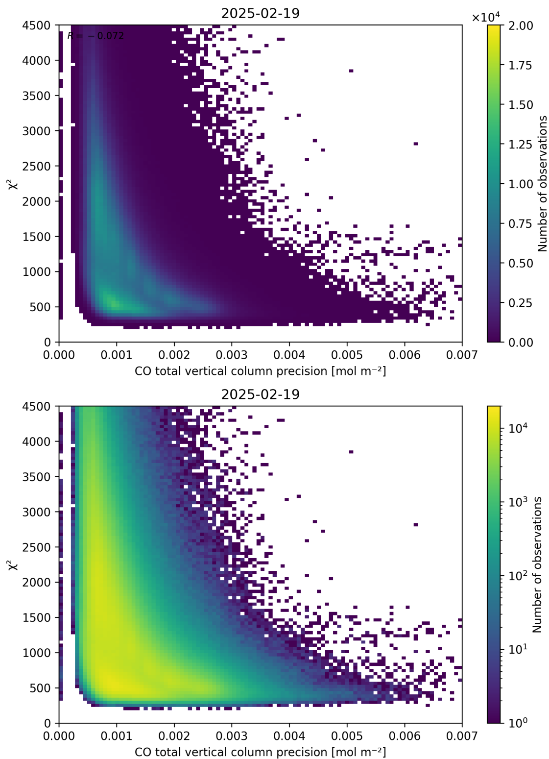
Figure 44: Scatter density plot of “CO total vertical column precision” against “ \chi^2 ” for 2025-02-19 to 2025-02-20.
