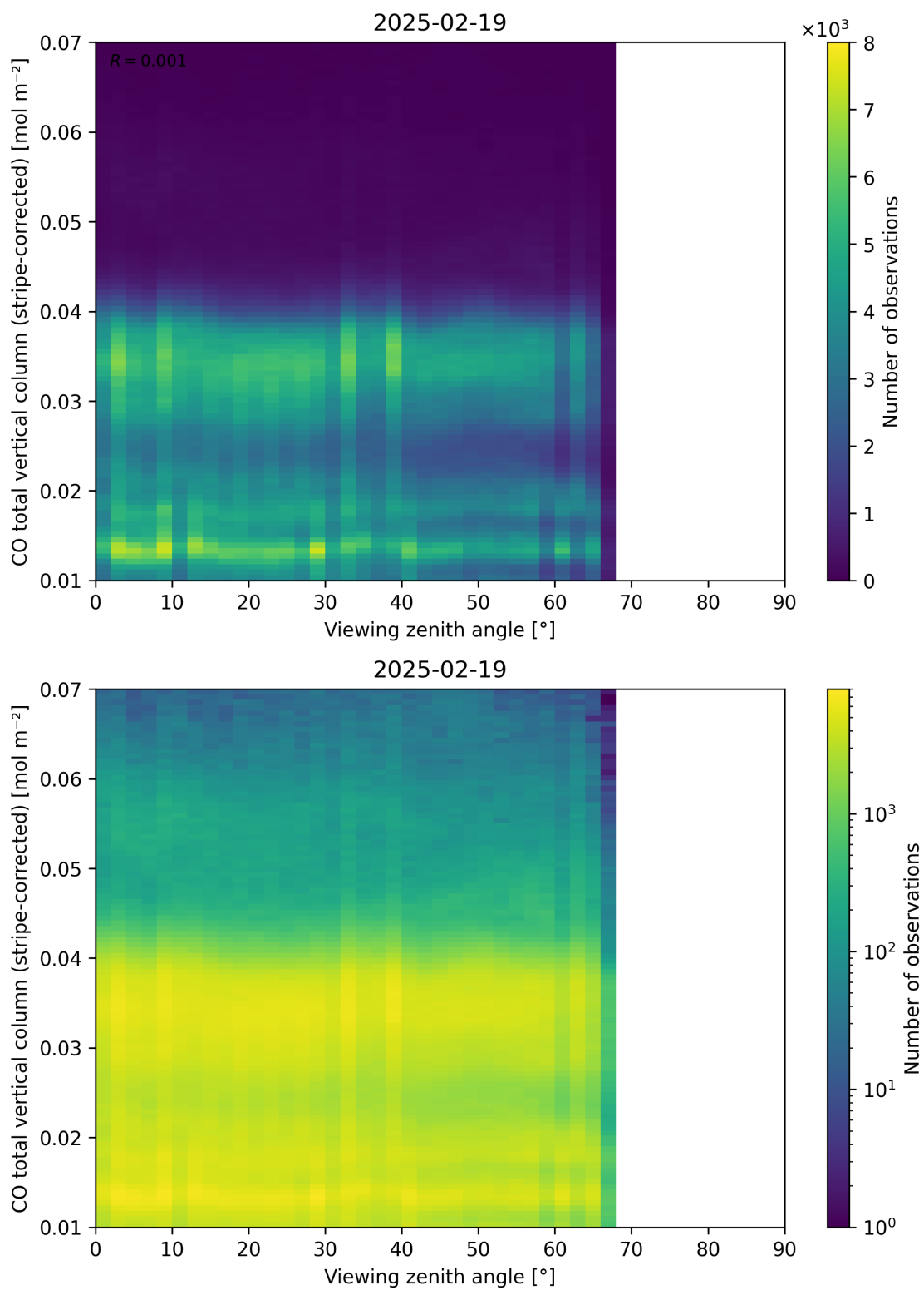
Figure 70: Scatter density plot of “Viewing zenith angle” against “CO total vertical column (stripe-corrected)” for 2025-02-19 to 2025-02-20.
