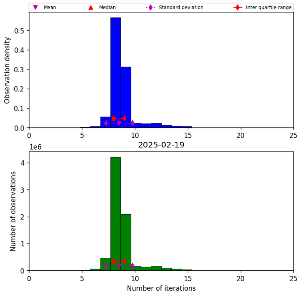
Figure 24: Histogram of “Number of iterations” for 2025-02-19 to 2025-02-20
