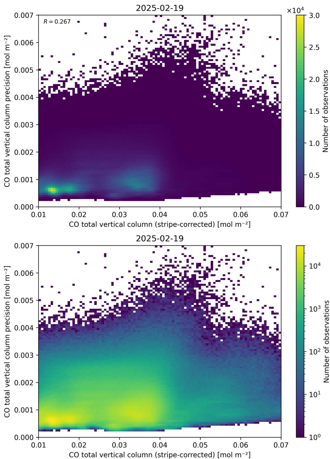
Figure 36: Scatter density plot of “CO total vertical column (stripe-corrected)” against “CO total vertical column precision” for 2025-02-19 to 2025-02-20.
