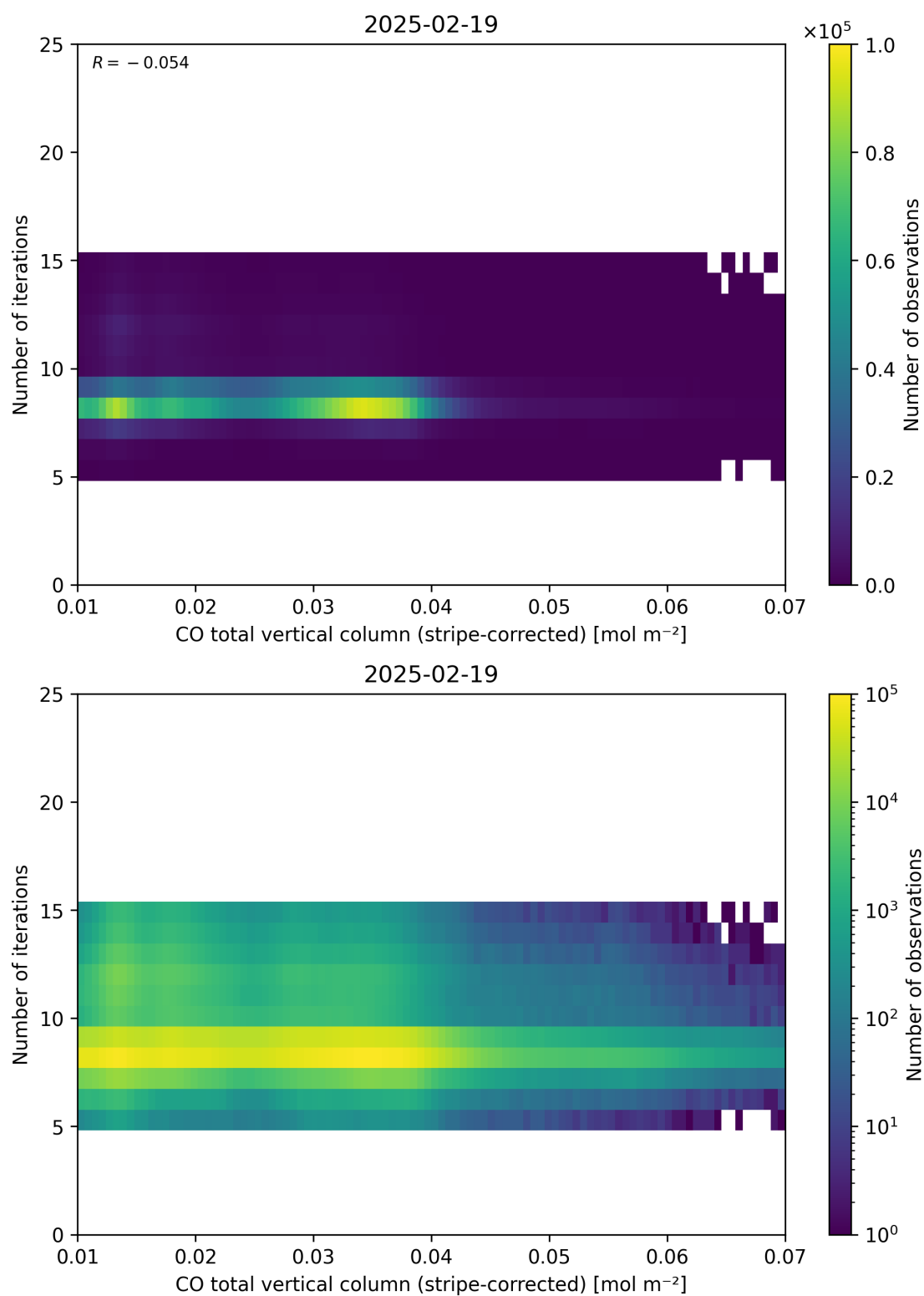
Figure 39: Scatter density plot of “CO total vertical column (stripe-corrected)” against “Number of iterations” for 2025-02-19 to 2025-02-20.
