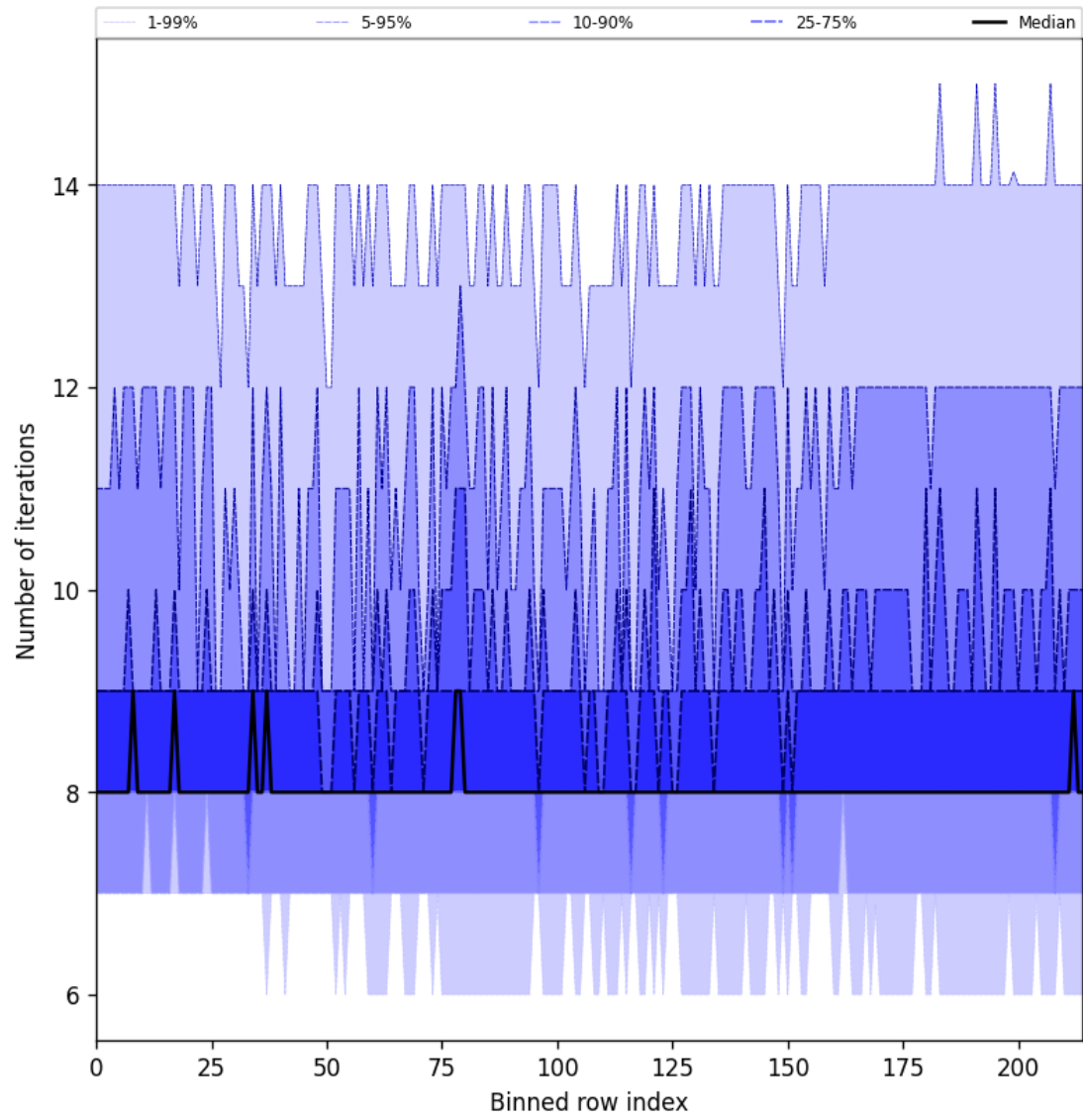
Figure 32: Along track statistics of “Number of iterations” for 2025-02-19 to 2025-02-20
