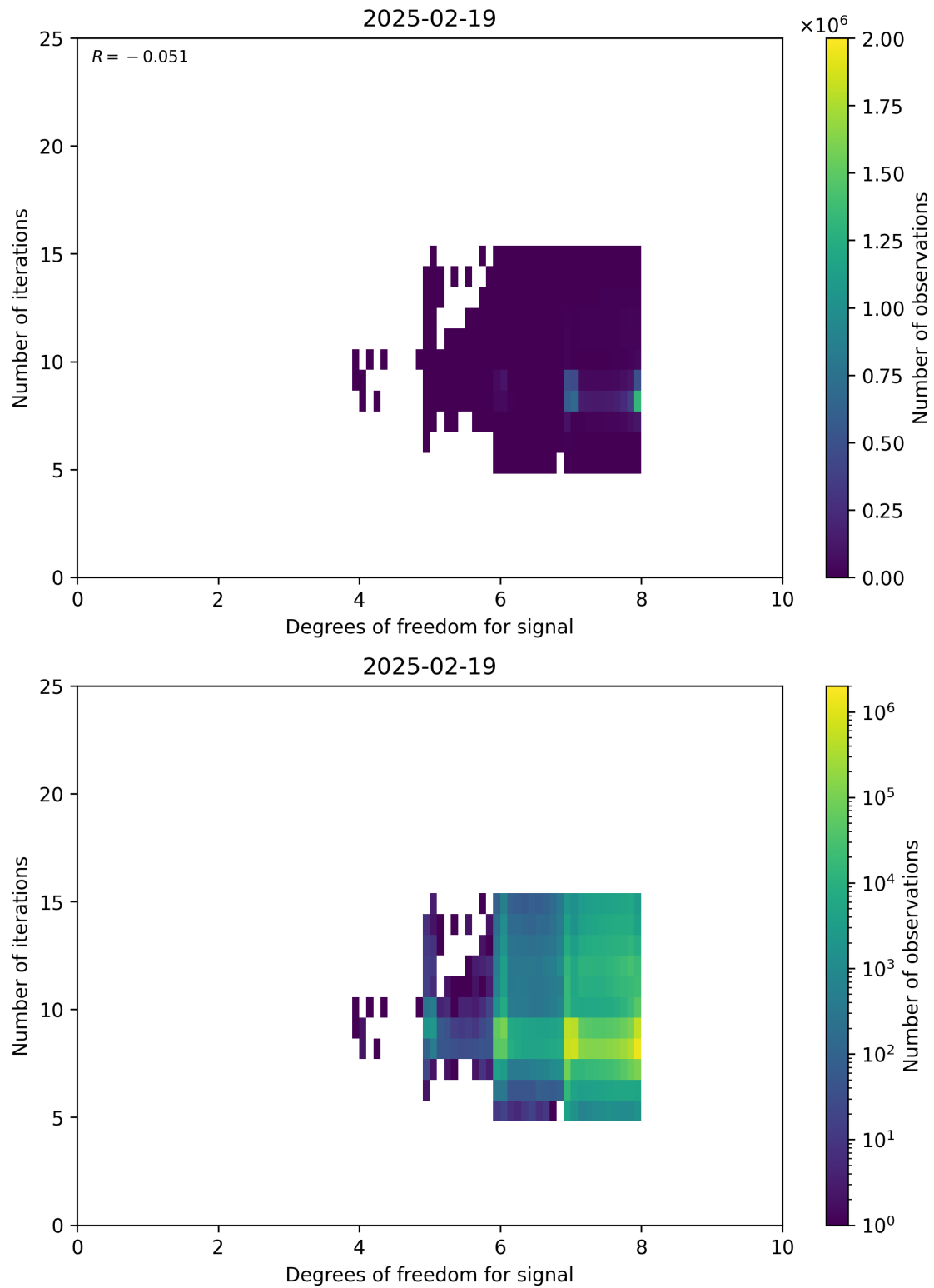
Figure 50: Scatter density plot of “Degrees of freedom for signal” against “Number of iterations” for 2025-02-19 to 2025-02-20.
