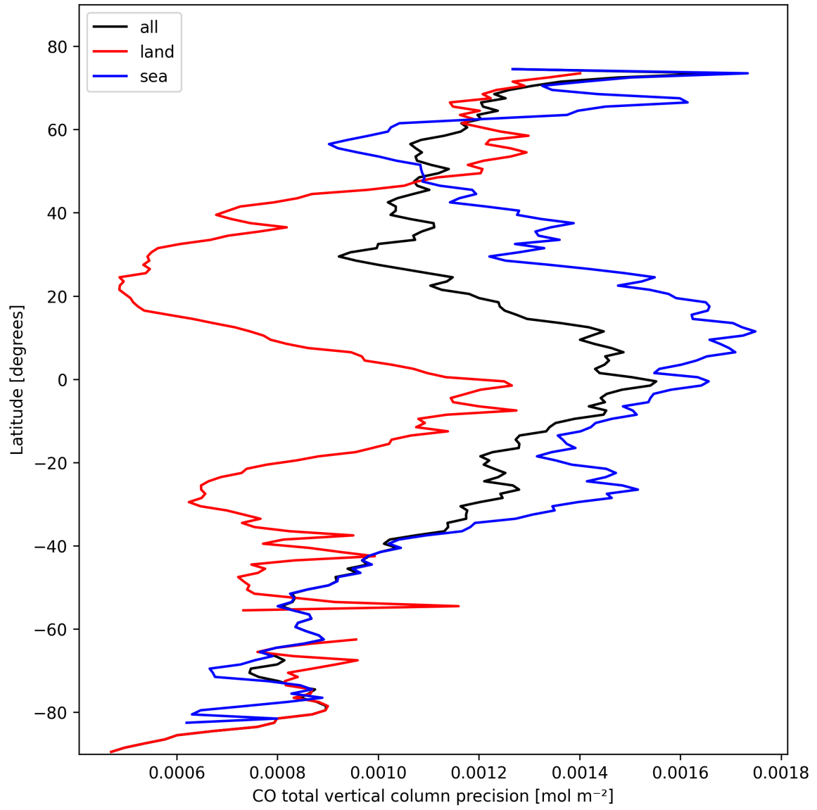
Figure 12: Zonal average of “CO total vertical column precision” for 2025-02-19 to 2025-02-20.
