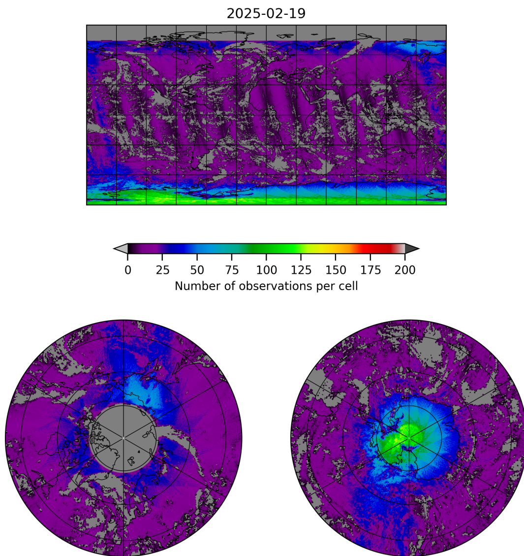
Figure 8: Map of the number of observations for 2025-02-19 to 2025-02-20
