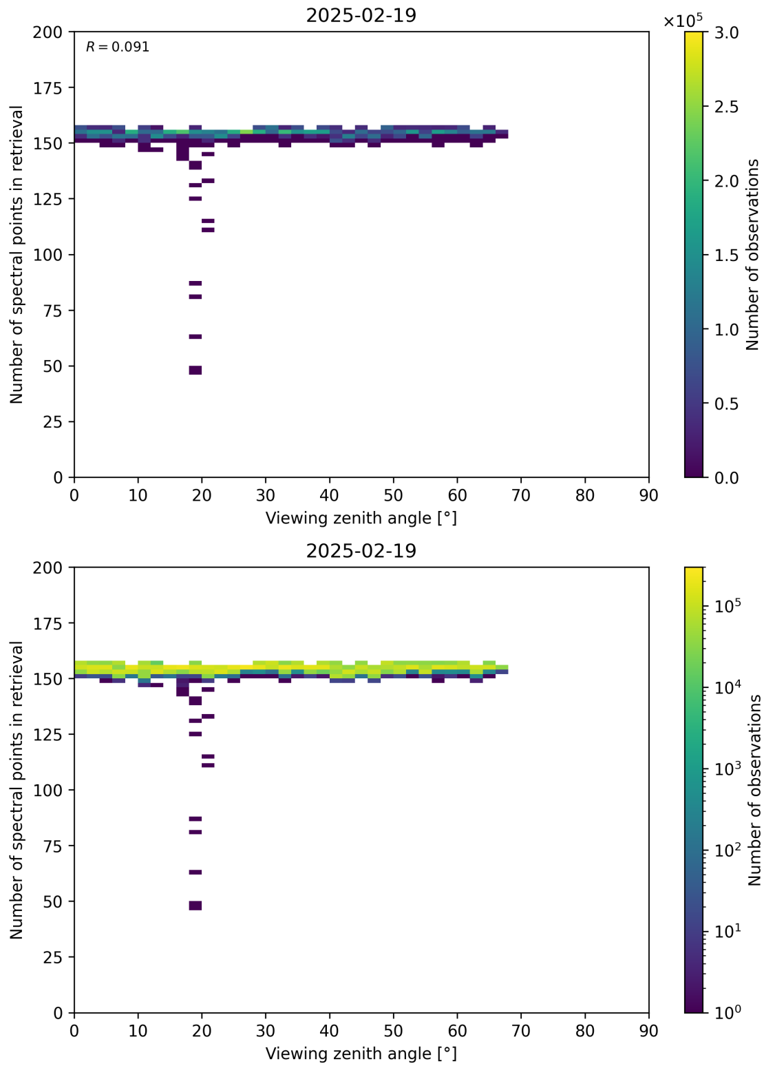
Figure 76: Scatter density plot of “Viewing zenith angle” against “Number of spectral points in retrieval” for 2025-02-19 to 2025-02-20.
