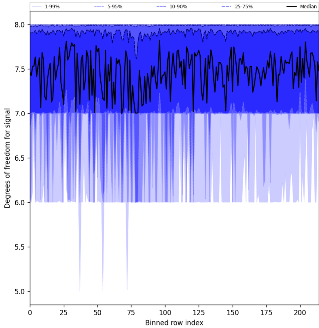
Figure 31: Along track statistics of “Degrees of freedom for signal” for 2025-02-19 to 2025-02-20
