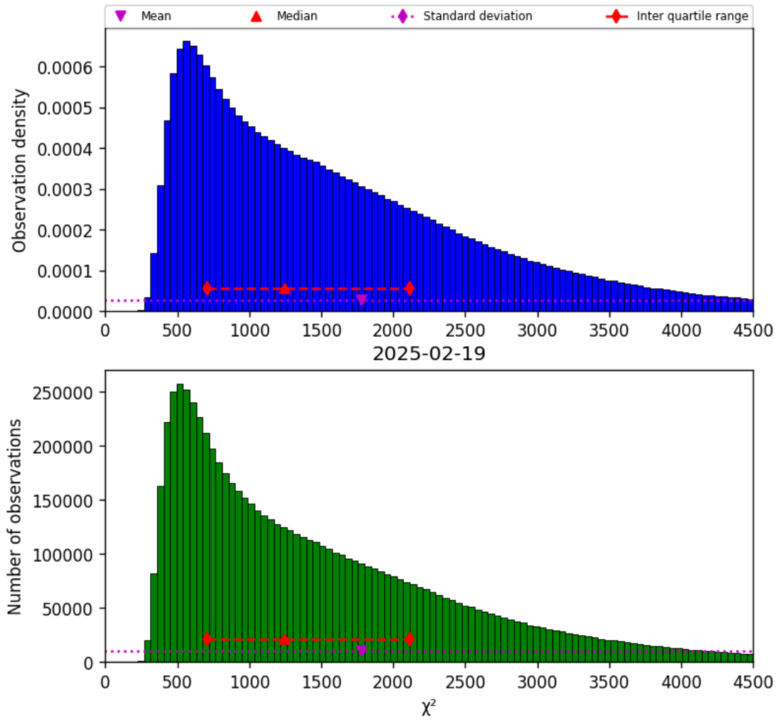
Figure 22: Histogram of “ \chi^2 ” for 2025-02-19 to 2025-02-20
