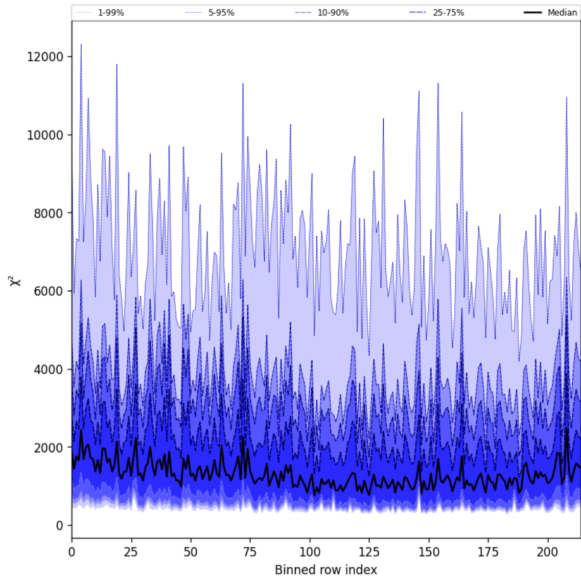
Figure 30: Along track statistics of “ \chi^2 ” for 2025-02-19 to 2025-02-20
