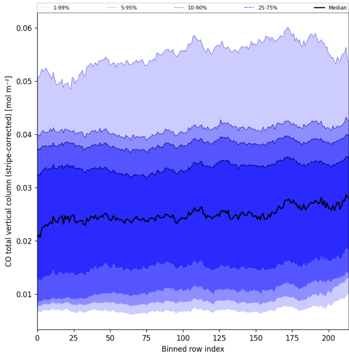
Figure 27: Along track statistics of “CO total vertical column (stripe-corrected)” for 2025-02-19 to 2025-02-20
