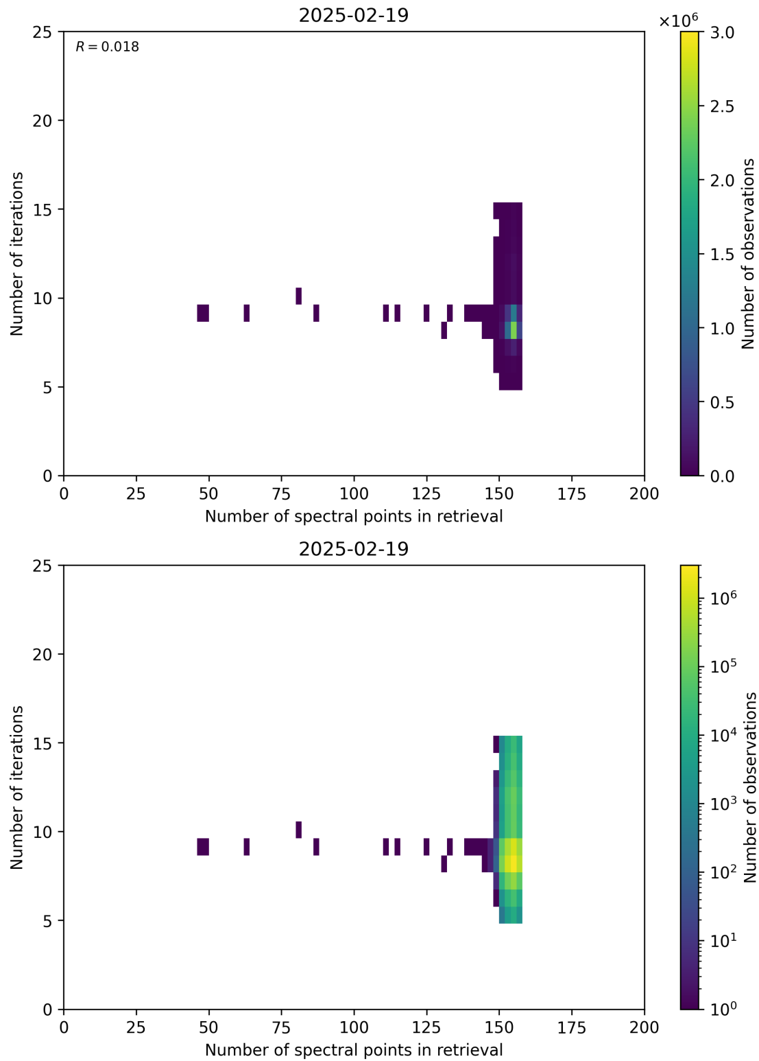
Figure 60: Scatter density plot of “Number of spectral points in retrieval” against “Number of iterations” for 2025-02-19 to 2025-02-20.
