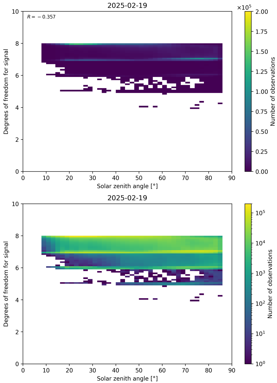
Figure 65: Scatter density plot of “Solar zenith angle” against “Degrees of freedom for signal” for 2025-02-19 to 2025-02-20.
