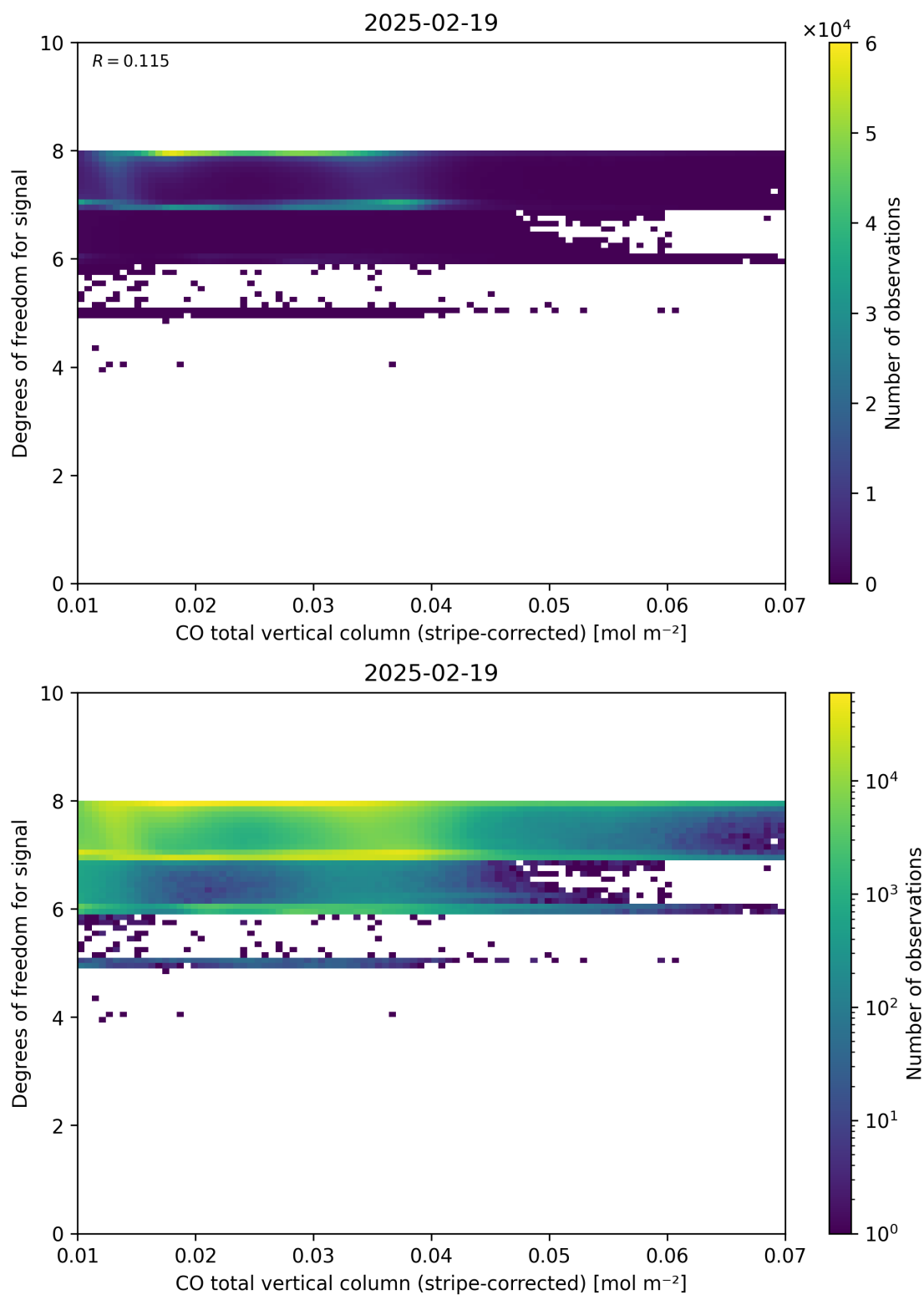
Figure 38: Scatter density plot of “CO total vertical column (stripe-corrected)” against “Degrees of freedom for signal” for 2025-02-19 to 2025-02-20.
