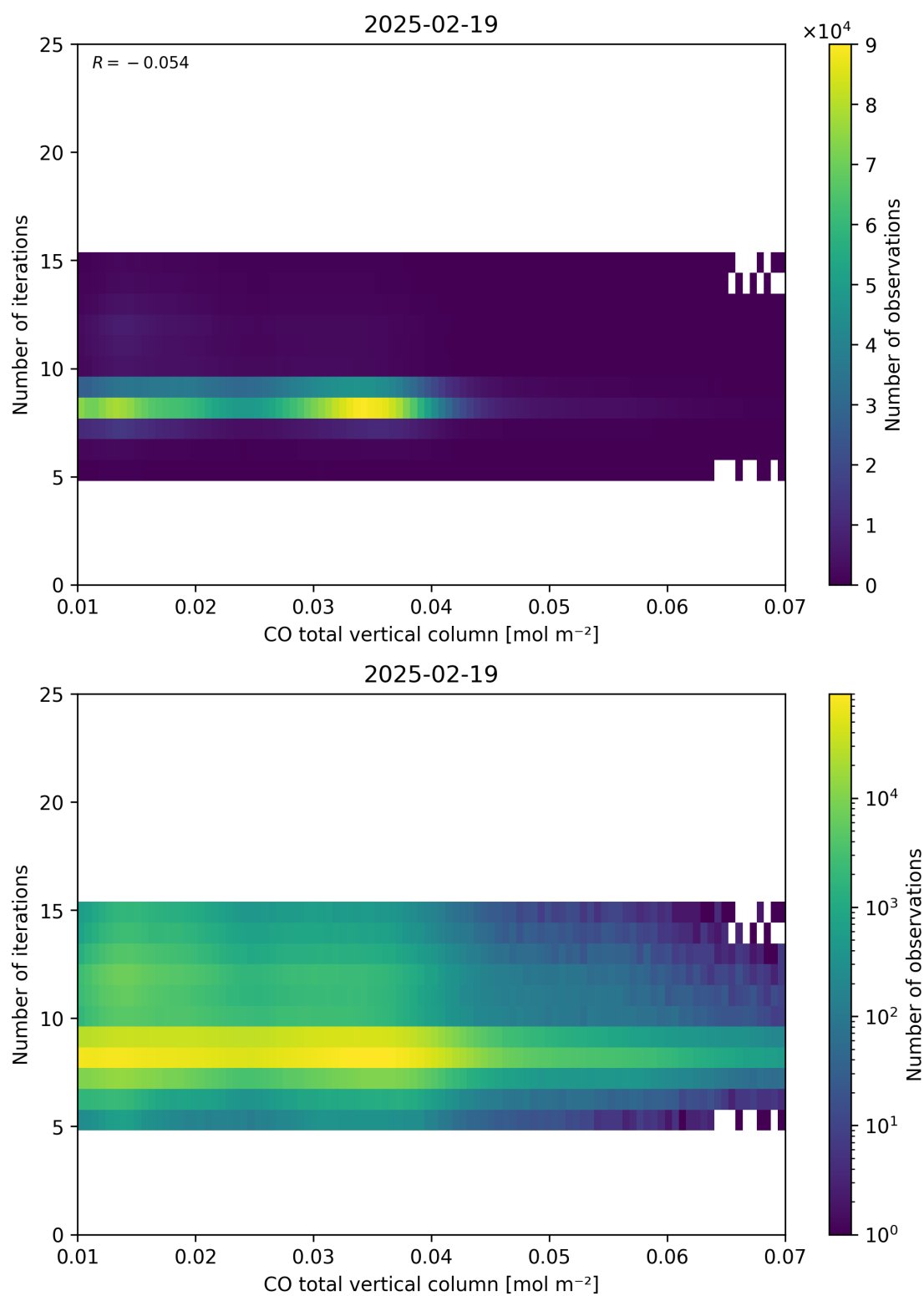
Figure 42: Scatter density plot of “CO total vertical column” against “Number of iterations” for 2025-02-19 to 2025-02-20.
