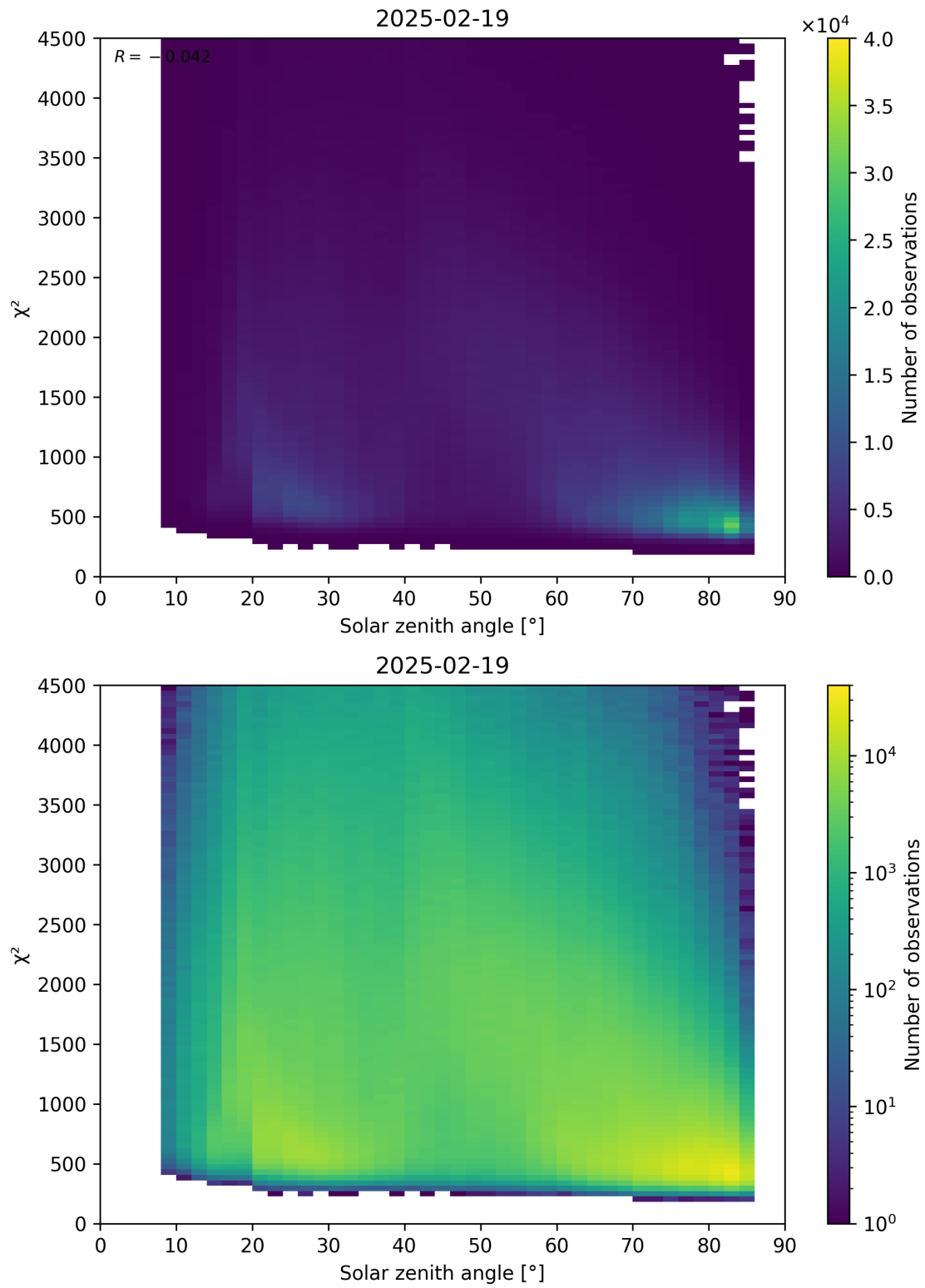
Figure 64: Scatter density plot of “Solar zenith angle” against “ \chi^2 ” for 2025-02-19 to 2025-02-20.
