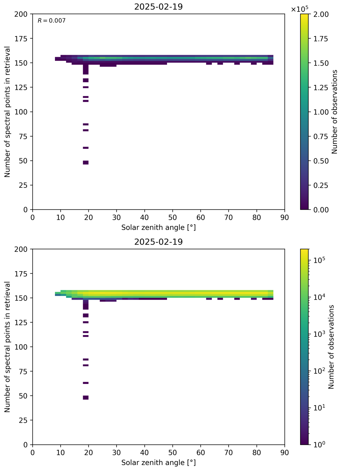
Figure 68: Scatter density plot of “Solar zenith angle” against “Number of spectral points in retrieval” for 2025-02-19 to 2025-02-20.
