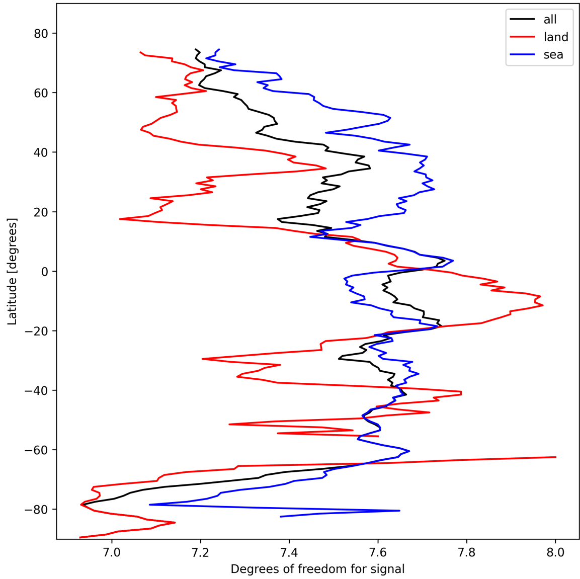
Figure 15: Zonal average of “Degrees of freedom for signal” for 2025-02-19 to 2025-02-20.
