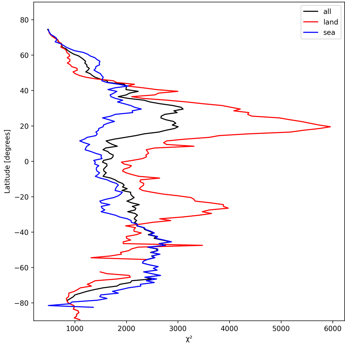
Figure 14: Zonal average of “ \chi^2 ” for 2025-02-19 to 2025-02-20.
