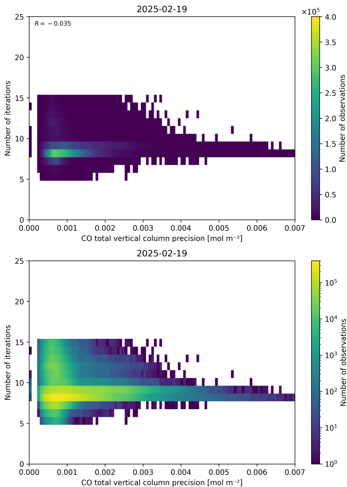
Figure 46: Scatter density plot of “CO total vertical column precision” against “Number of iterations” for 2025-02-19 to 2025-02-20.
