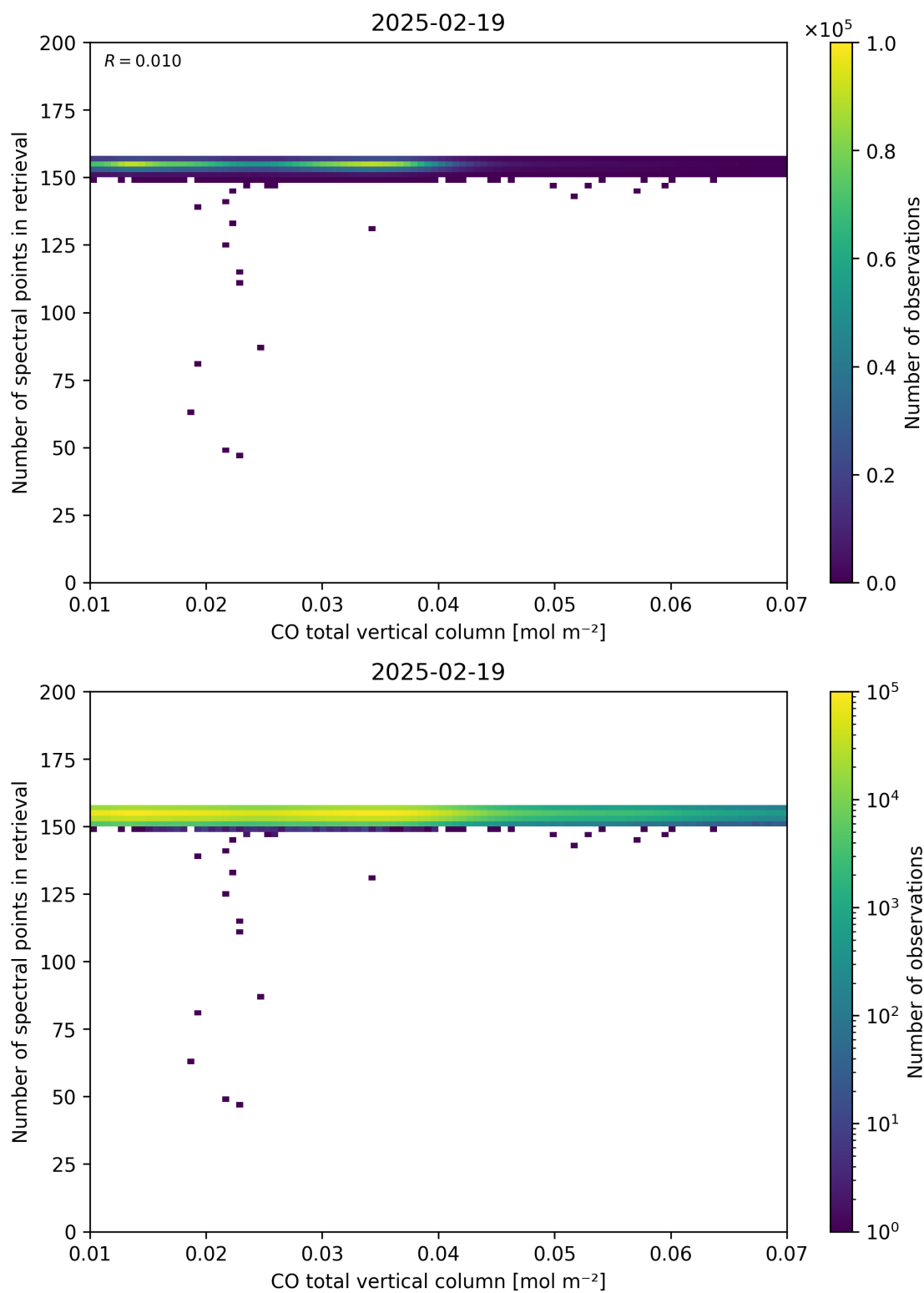
Figure 43: Scatter density plot of “CO total vertical column” against “Number of spectral points in retrieval” for 2025-02-19 to 2025-02-20.
