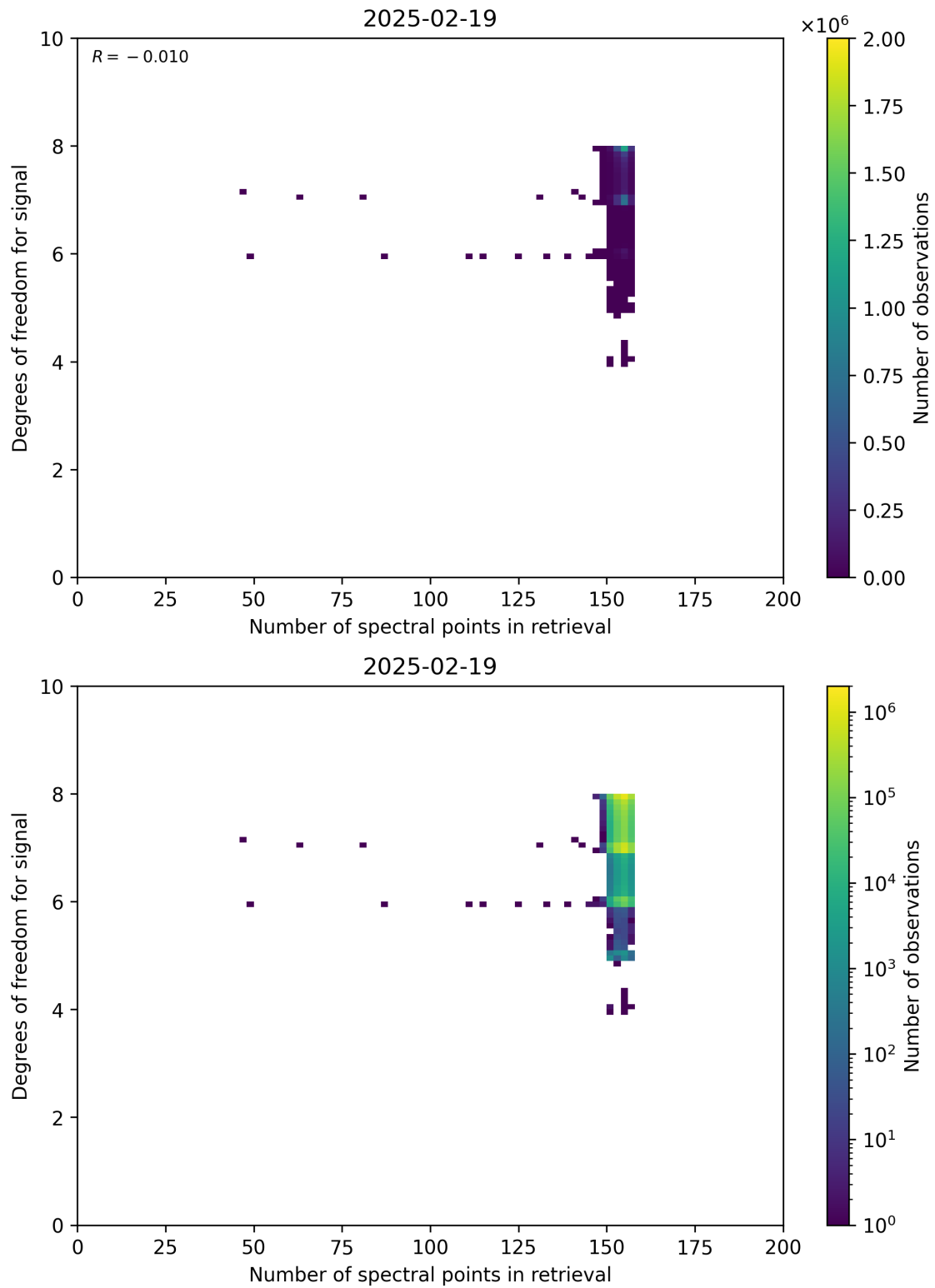
Figure 59: Scatter density plot of “Number of spectral points in retrieval” against “Degrees of freedom for signal” for 2025-02-19 to 2025-02-20.
