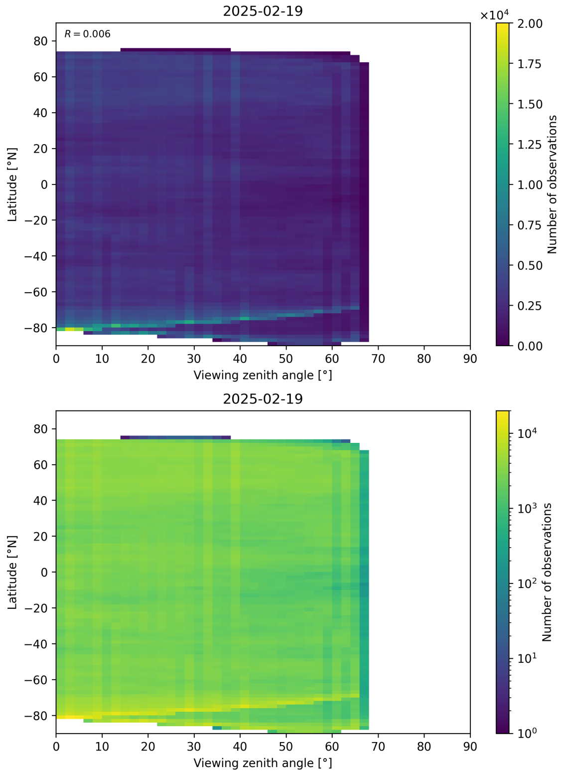
Figure 74: Scatter density plot of “Viewing zenith angle” against “Latitude” for 2025-02-19 to 2025-02-20.
