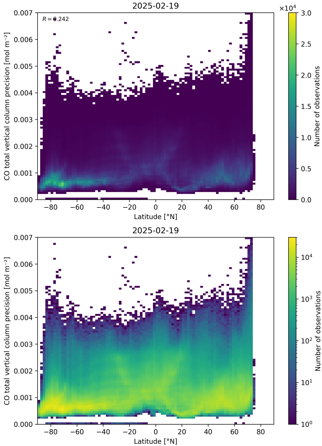
Figure 53: Scatter density plot of “Latitude” against “CO total vertical column precision” for 2025-02-19 to 2025-02-20.
