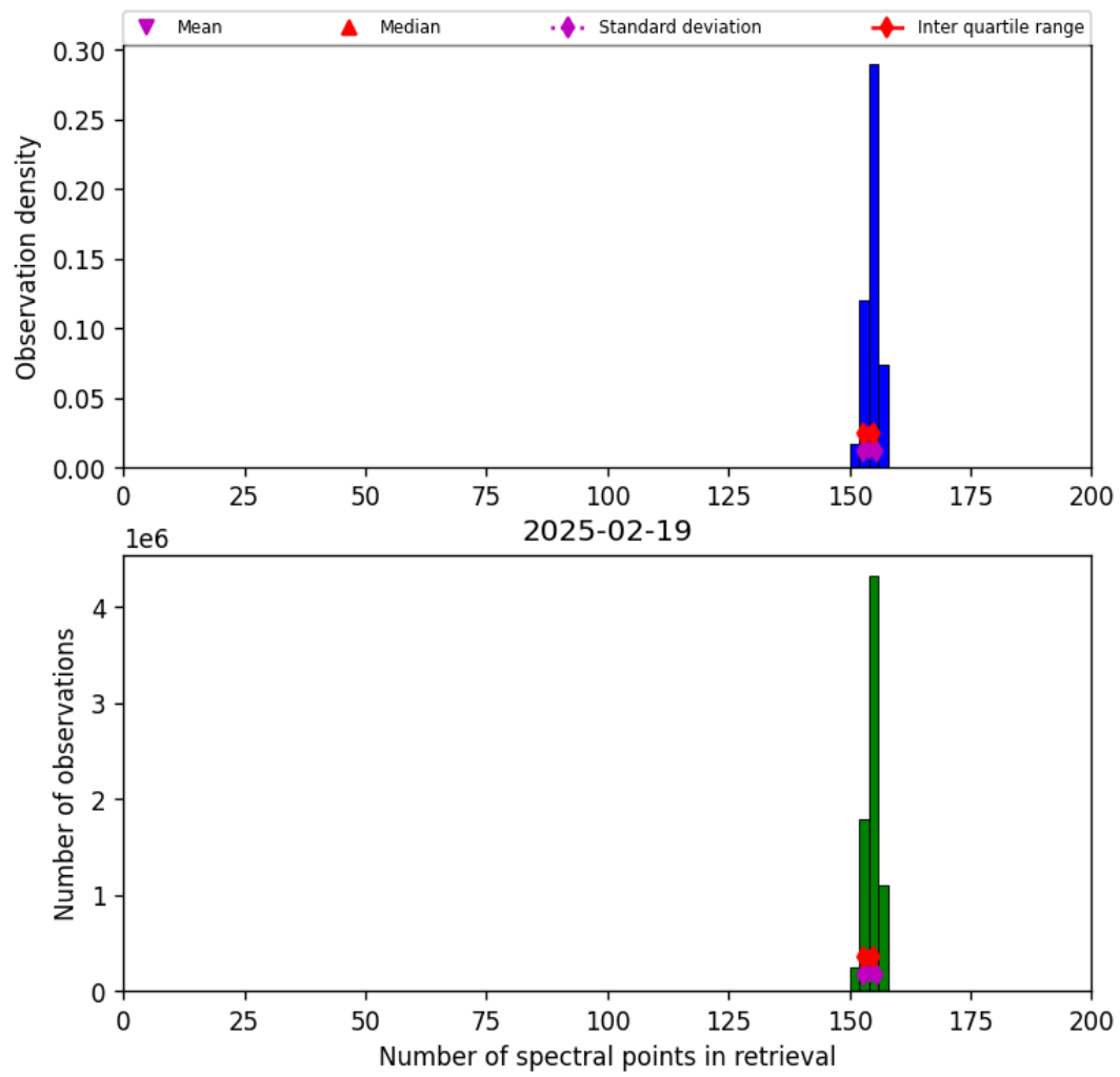
Figure 21: Histogram of “Number of spectral points in retrieval” for 2025-02-19 to 2025-02-20
