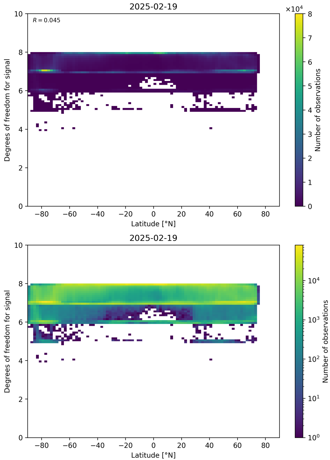
Figure 55: Scatter density plot of “Latitude” against “Degrees of freedom for signal” for 2025-02-19 to 2025-02-20.
