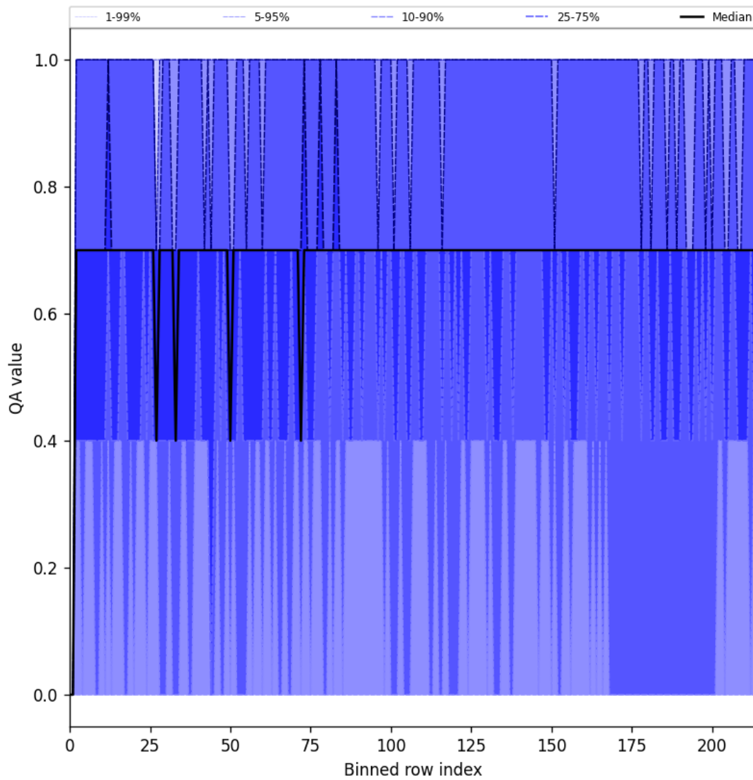
Figure 25: Along track statistics of “QA value” for 2025-02-19 to 2025-02-20
