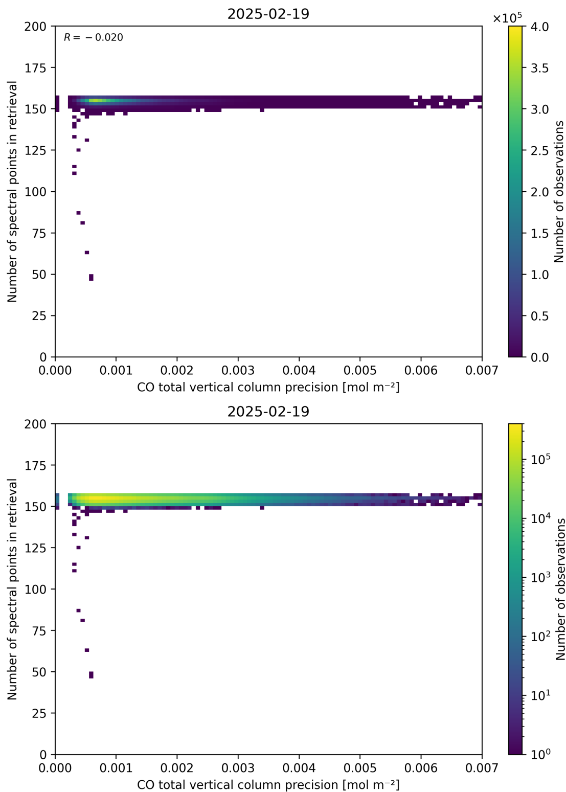
Figure 47: Scatter density plot of “CO total vertical column precision” against “Number of spectral points in retrieval” for 2025-02-19 to 2025-02-20.
