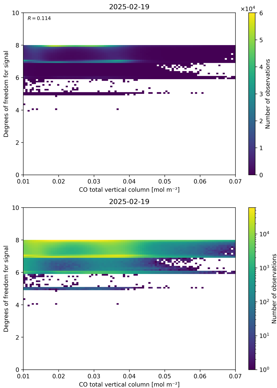
Figure 41: Scatter density plot of “CO total vertical column” against “Degrees of freedom for signal” for 2025-02-19 to 2025-02-20.
