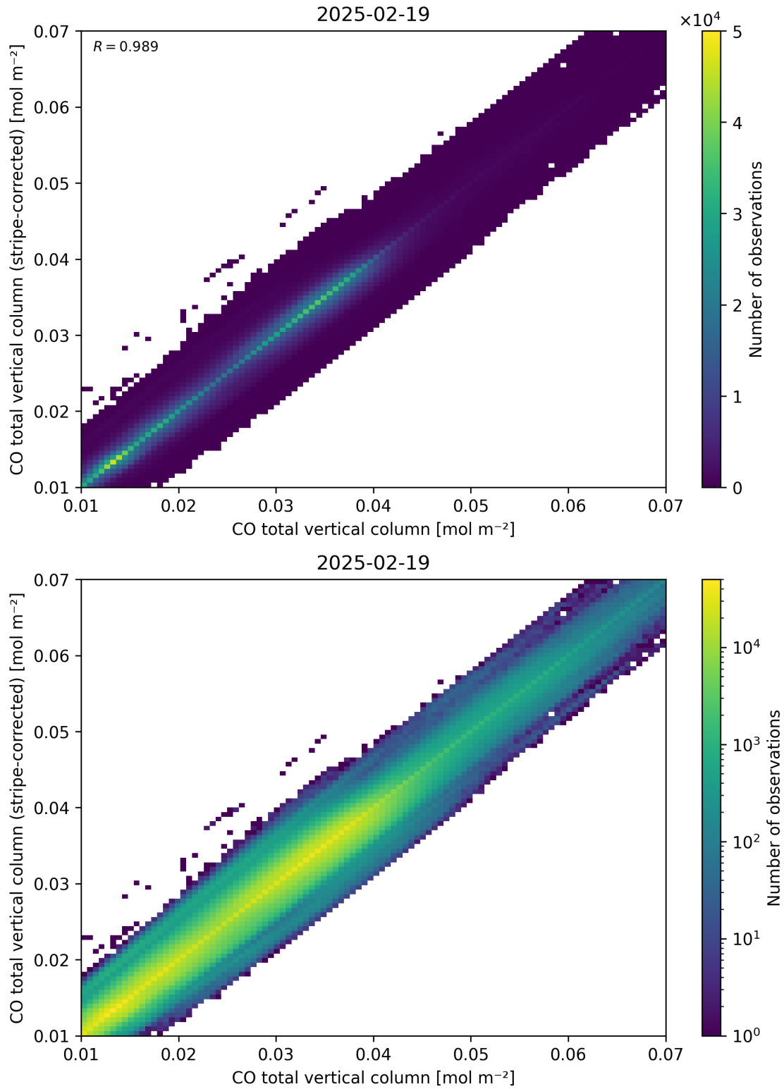
Figure 33: Scatter density plot of “CO total vertical column” against “CO total vertical column (stripe-corrected)” for 2025-02-19 to 2025-02-20.
