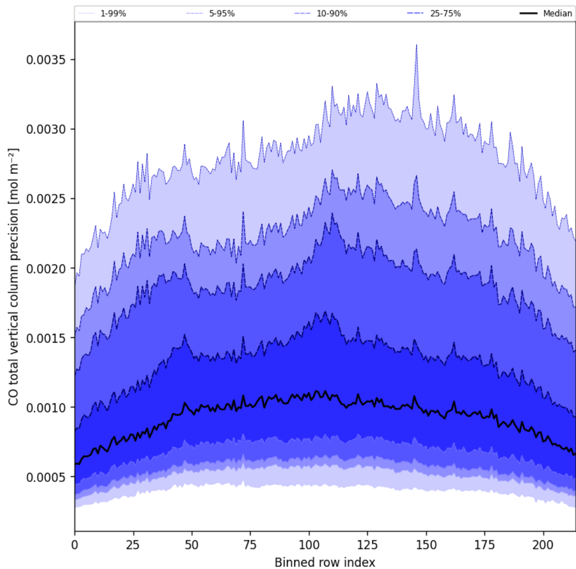
Figure 28: Along track statistics of “CO total vertical column precision” for 2025-02-19 to 2025-02-20
