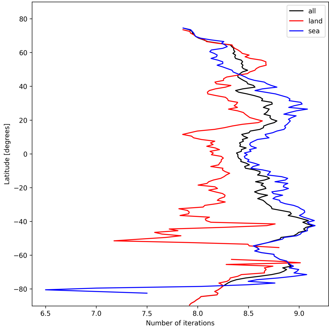
Figure 16: Zonal average of “Number of iterations” for 2025-02-19 to 2025-02-20.
