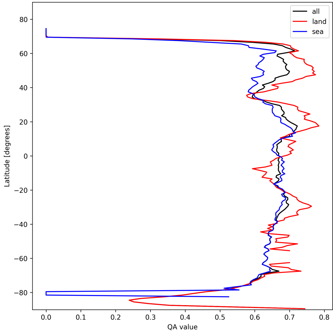
Figure 9: Zonal average of “QA value” for 2025-02-19 to 2025-02-20.
