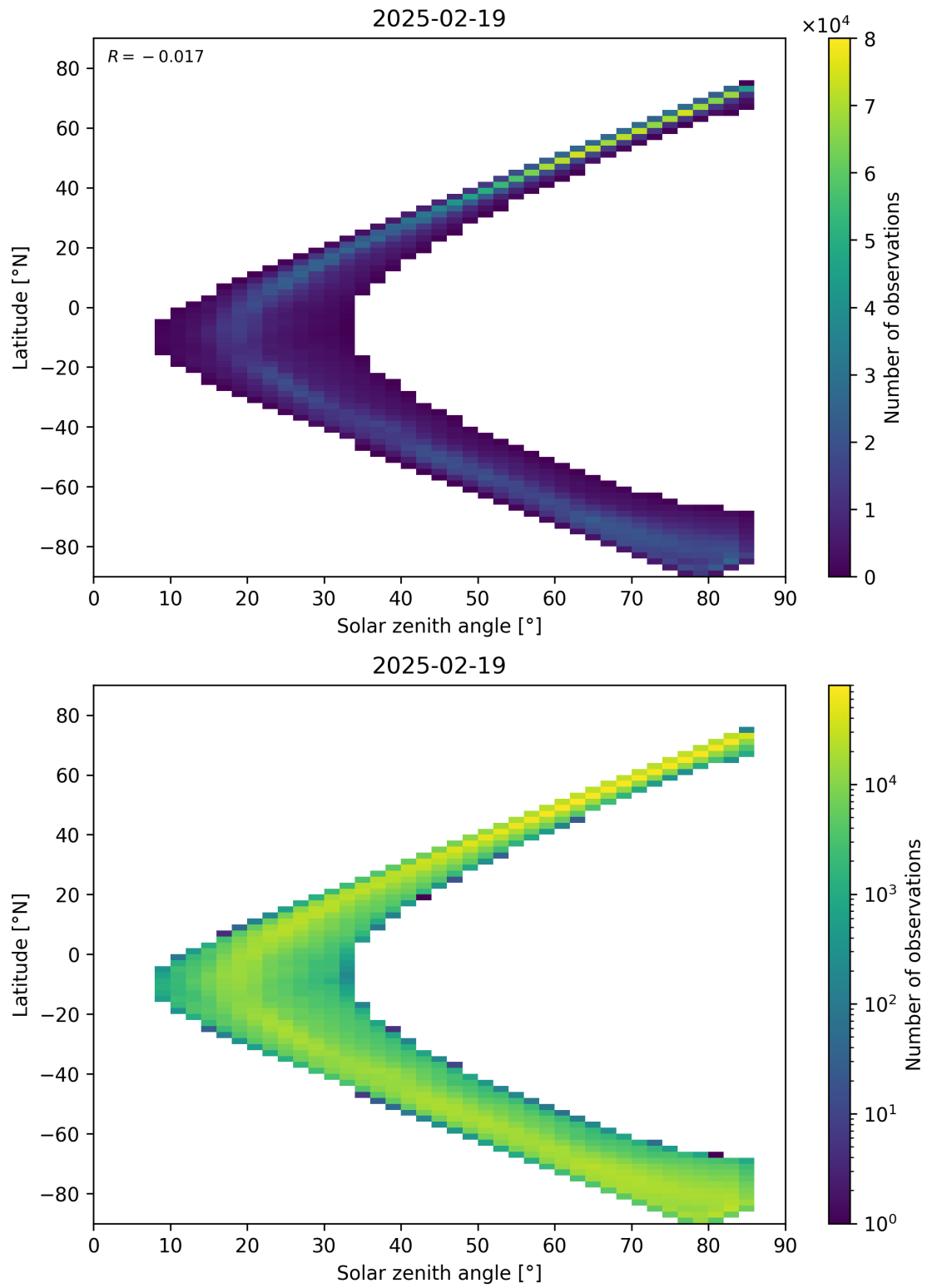
Figure 66: Scatter density plot of “Solar zenith angle” against “Latitude” for 2025-02-19 to 2025-02-20.
