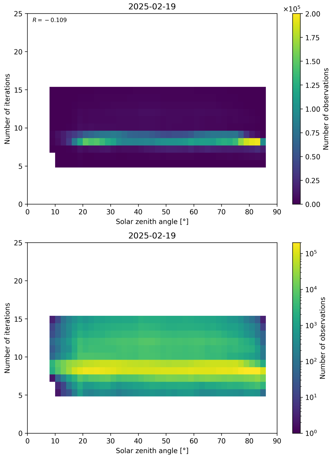
Figure 67: Scatter density plot of “Solar zenith angle” against “Number of iterations” for 2025-02-19 to 2025-02-20.
