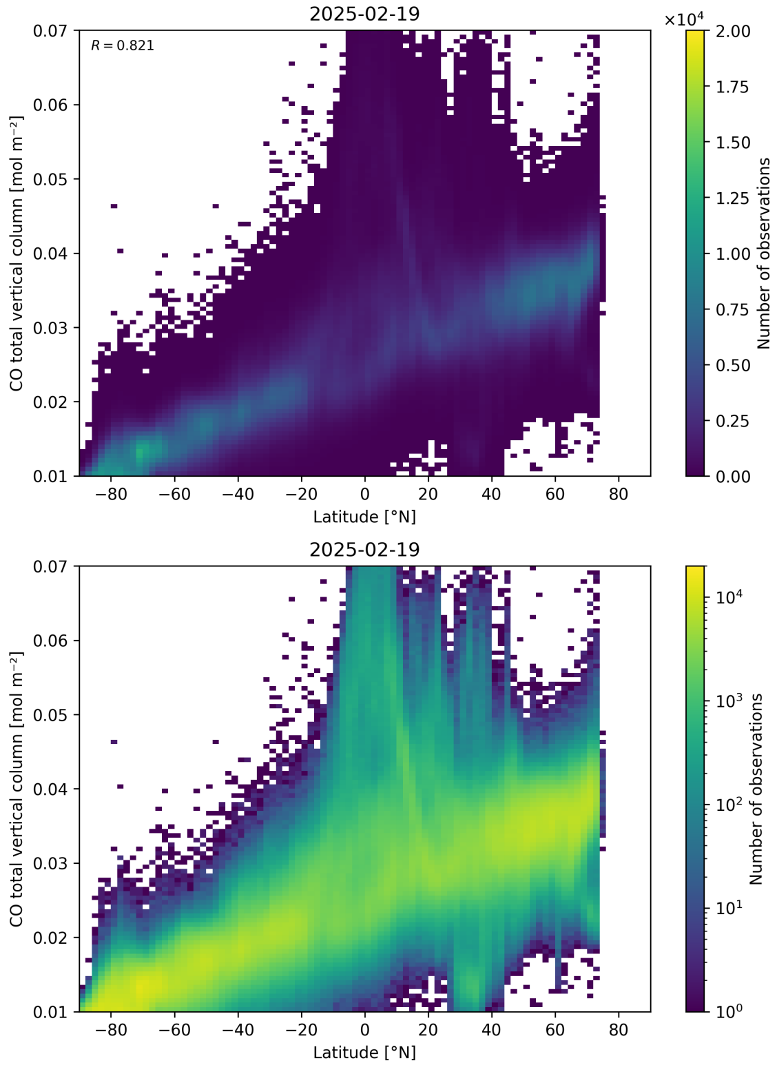
Figure 51: Scatter density plot of “Latitude” against “CO total vertical column” for 2025-02-19 to 2025-02-20.
