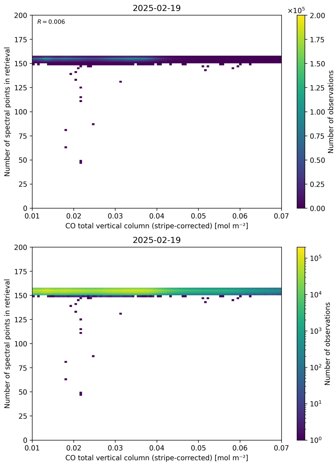
Figure 40: Scatter density plot of “CO total vertical column (stripe-corrected)” against “Number of spectral points in retrieval” for 2025-02-19 to 2025-02-20.
