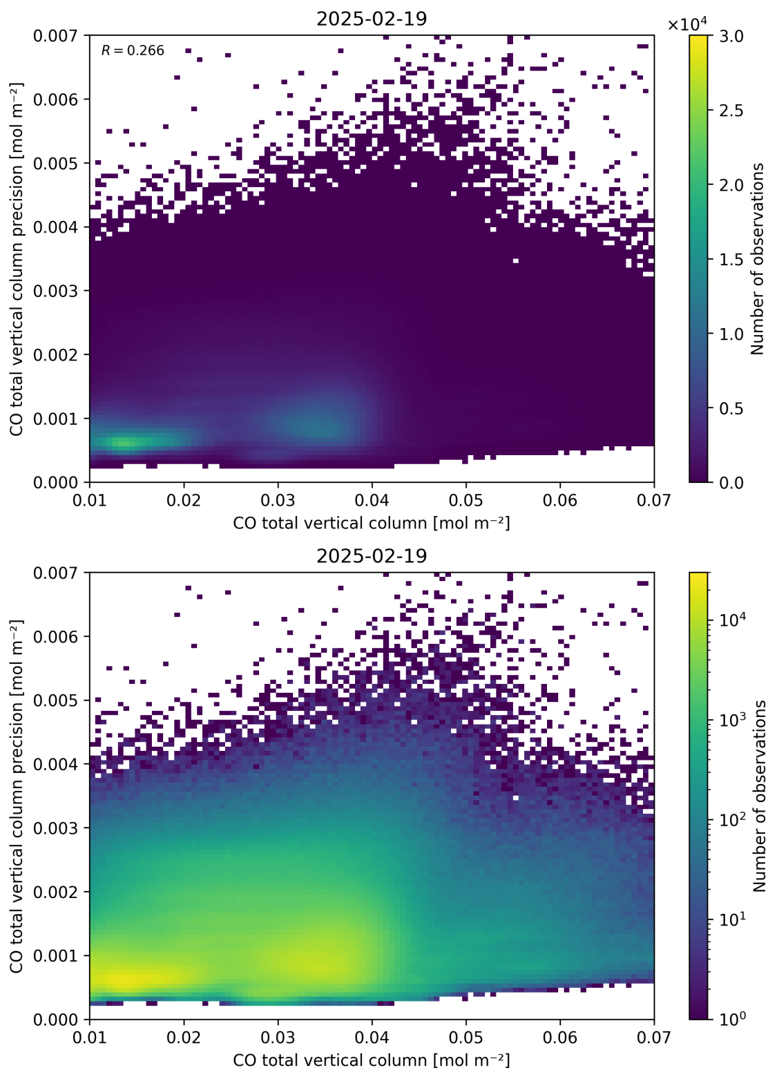
Figure 34: Scatter density plot of “CO total vertical column” against “CO total vertical column precision” for 2025-02-19 to 2025-02-20.
