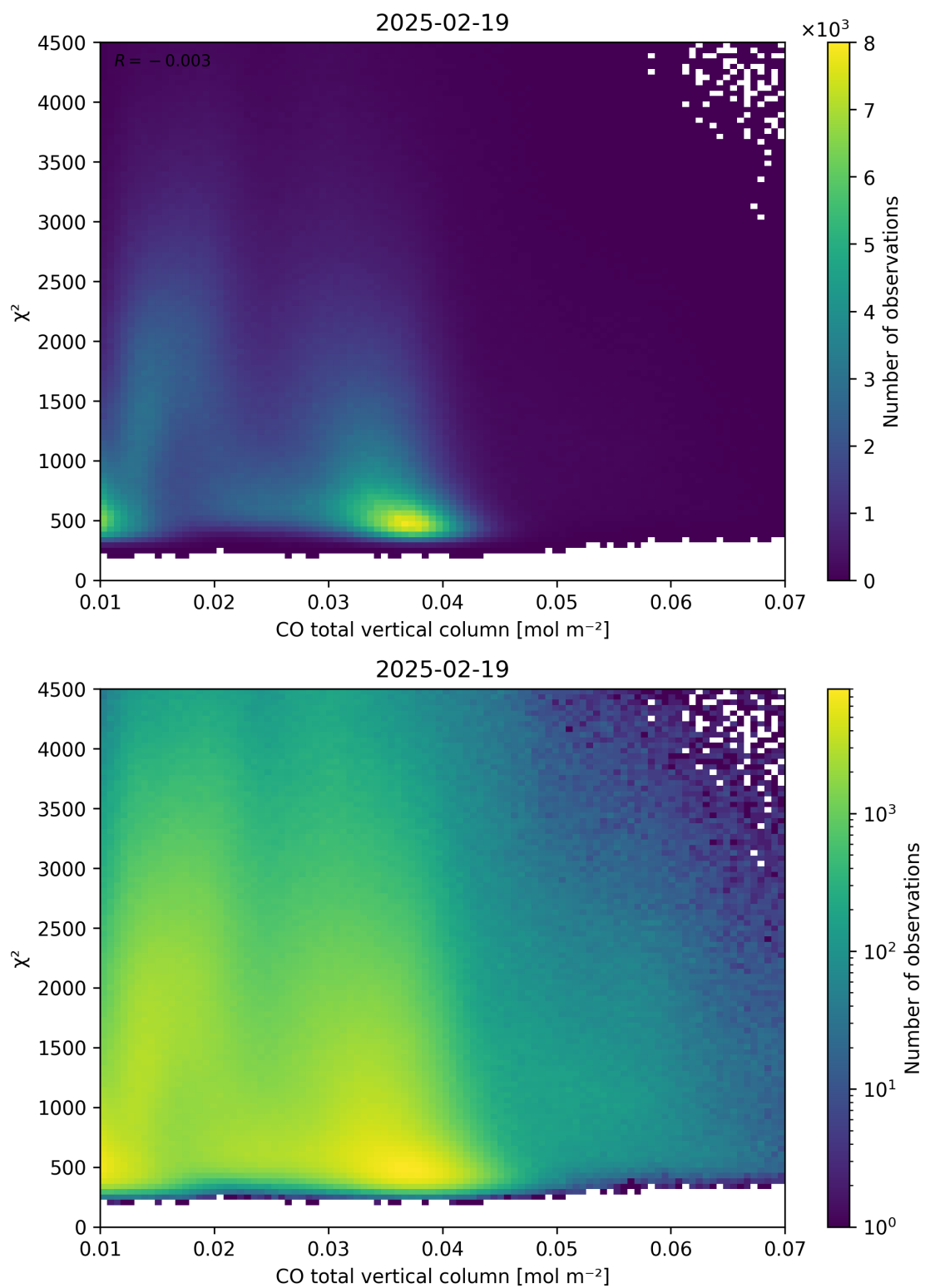
Figure 35: Scatter density plot of “CO total vertical column” against “ \chi^2 ” for 2025-02-19 to 2025-02-20.
