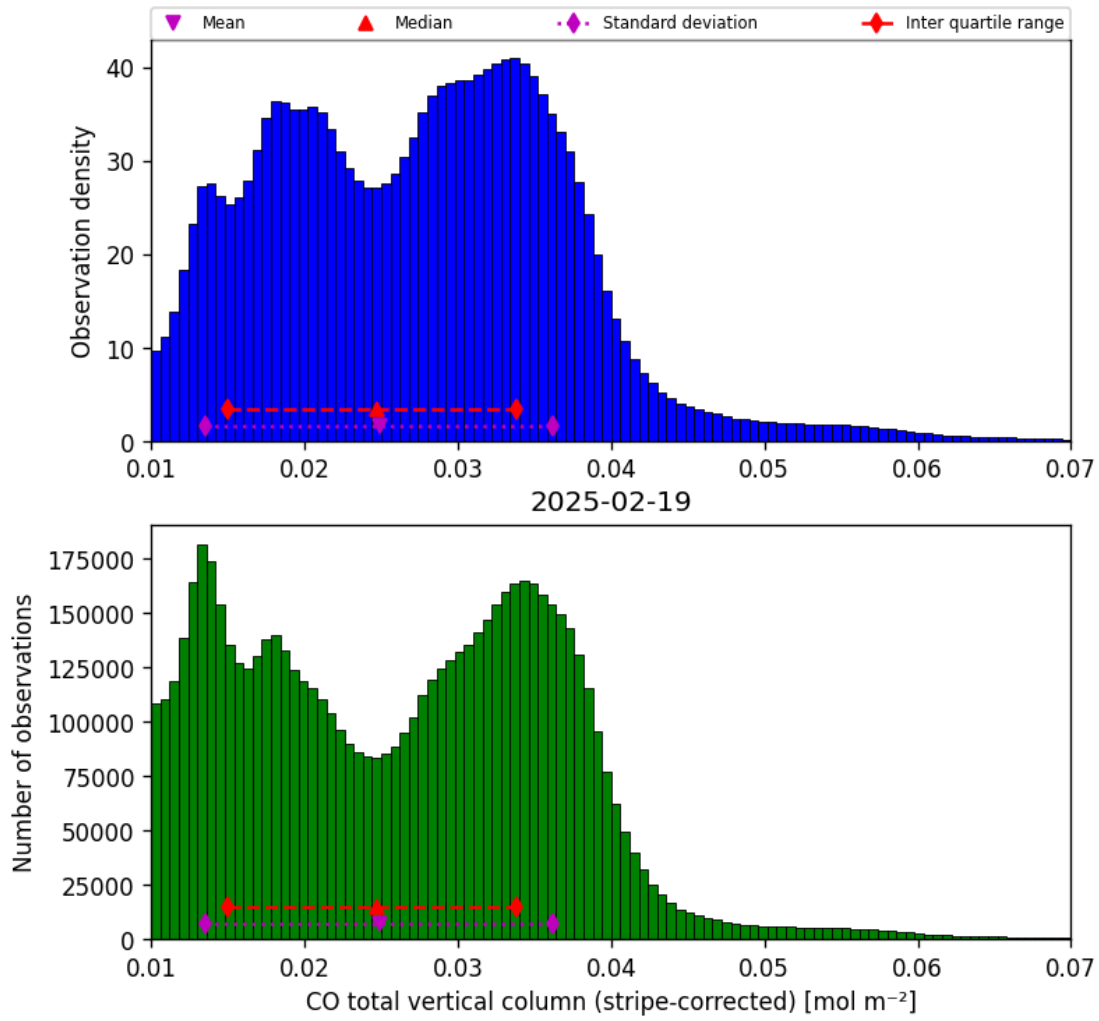
Figure 19: Histogram of “CO total vertical column (stripe-corrected)” for 2025-02-19 to 2025-02-20
