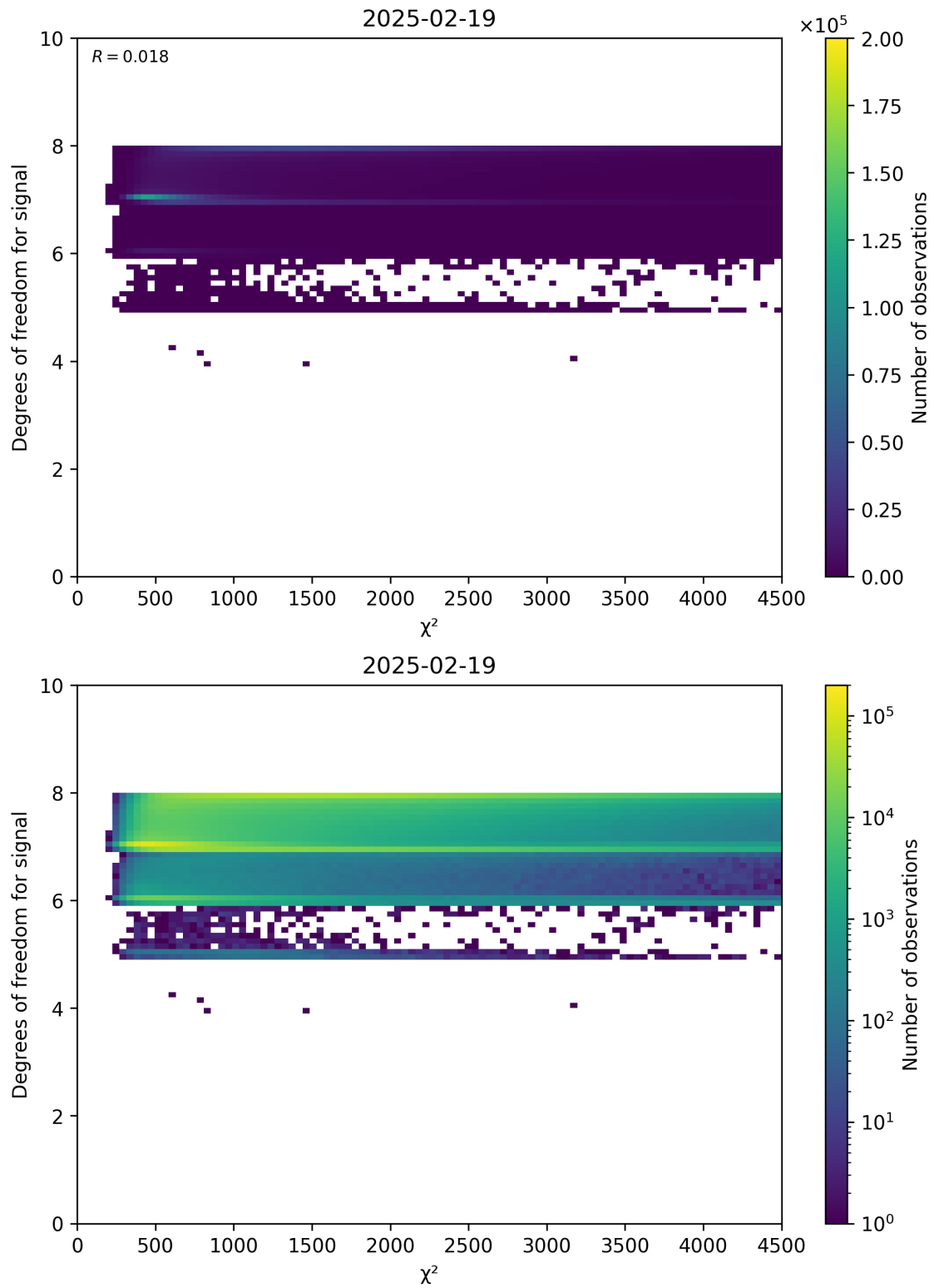
Figure 48: Scatter density plot of “ \chi^2 ” against “Degrees of freedom for signal” for 2025-02-19 to 2025-02-20.
