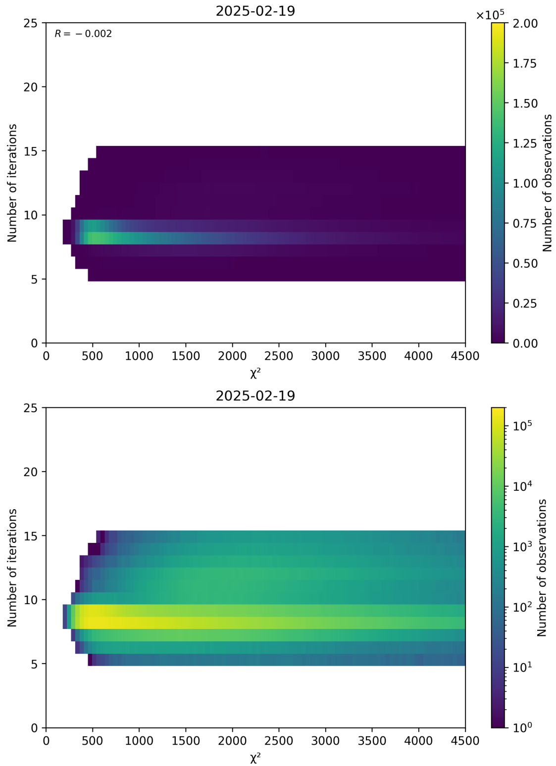
Figure 49: Scatter density plot of “ \chi^2 ” against “Number of iterations” for 2025-02-19 to 2025-02-20.
