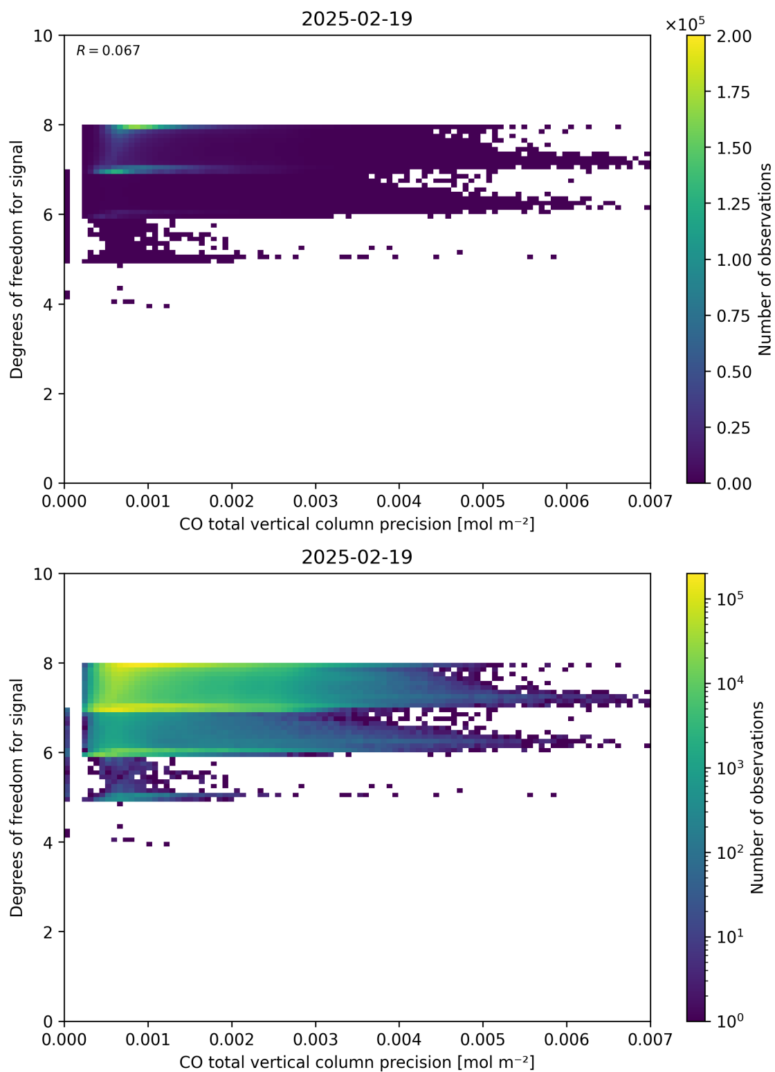
Figure 45: Scatter density plot of “CO total vertical column precision” against “Degrees of freedom for signal” for 2025-02-19 to 2025-02-20.
