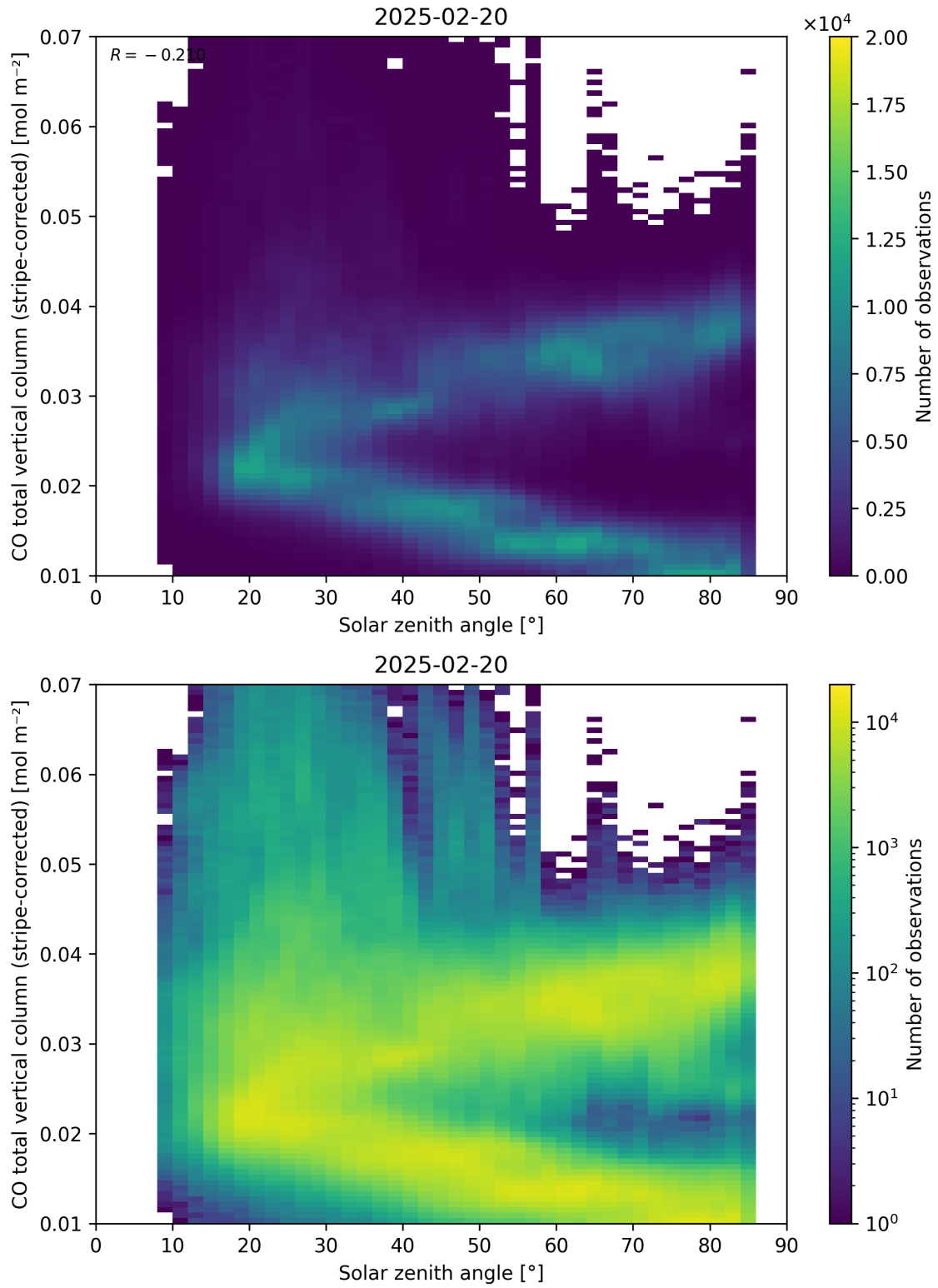
Figure 62: Scatter density plot of “Solar zenith angle” against “CO total vertical column (stripe-corrected)” for 2025-02-19 to 2025-02-21.
