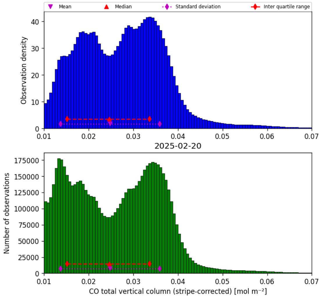
Figure 19: Histogram of “CO total vertical column (stripe-corrected)” for 2025-02-19 to 2025-02-21
