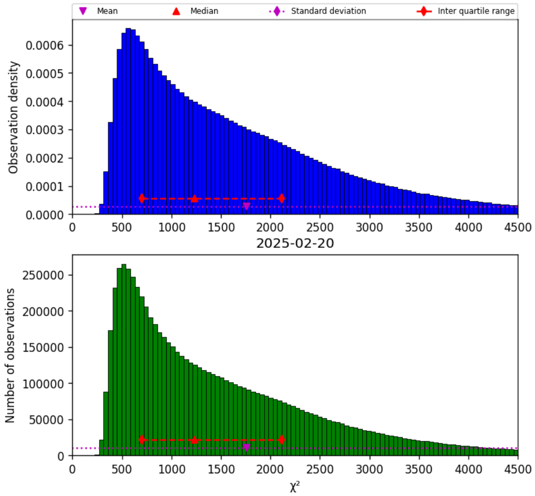
Figure 22: Histogram of “ \chi^2 ” for 2025-02-19 to 2025-02-21
