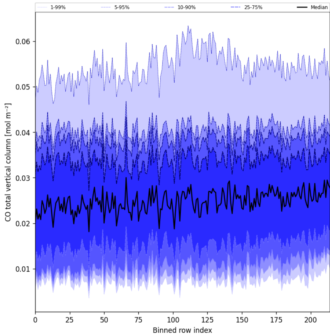
Figure 26: Along track statistics of “CO total vertical column” for 2025-02-19 to 2025-02-21
