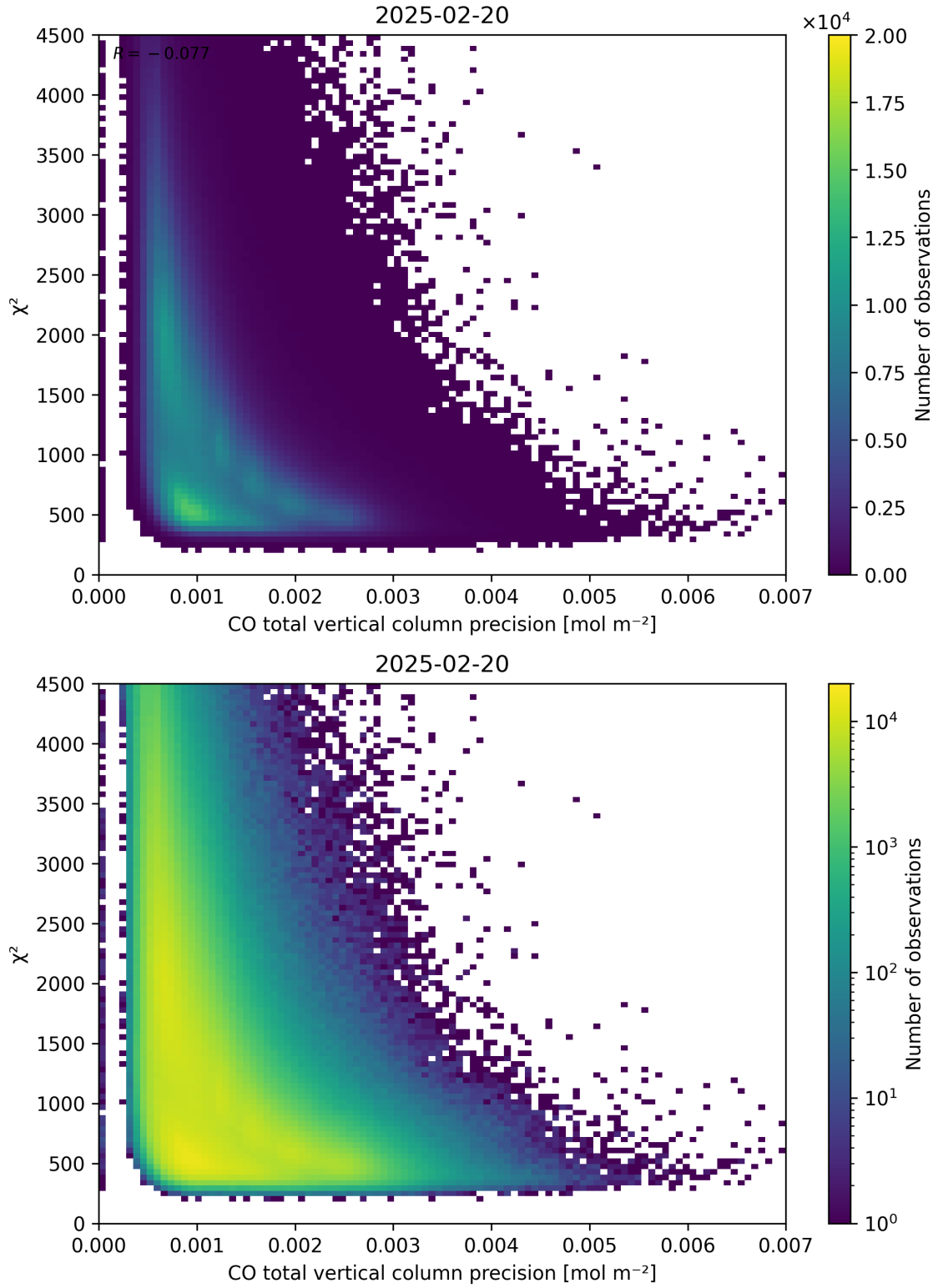
Figure 44: Scatter density plot of “CO total vertical column precision” against “ \chi^2 ” for 2025-02-19 to 2025-02-21.
