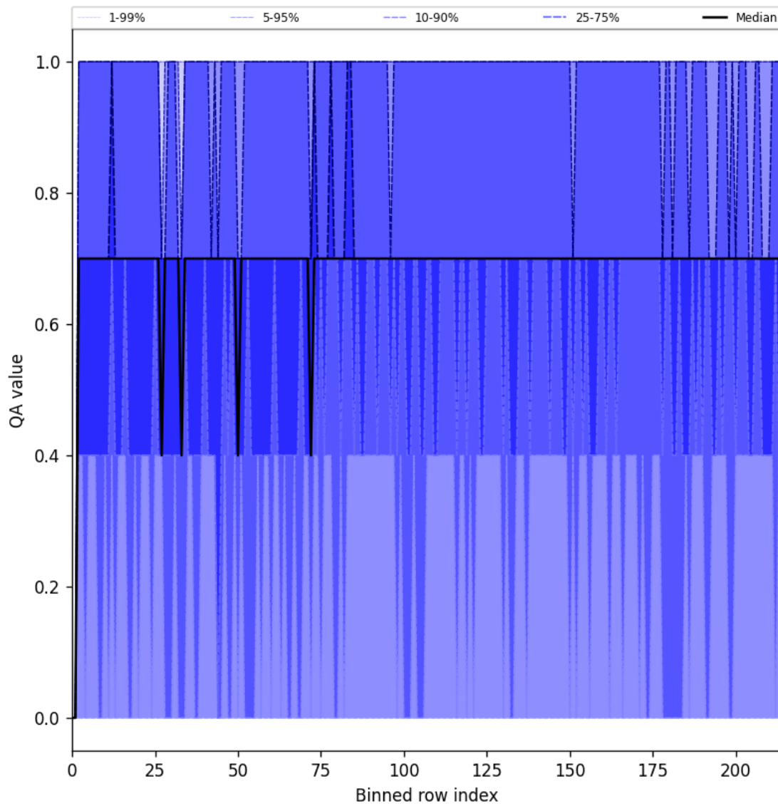
Figure 25: Along track statistics of “QA value” for 2025-02-19 to 2025-02-21
