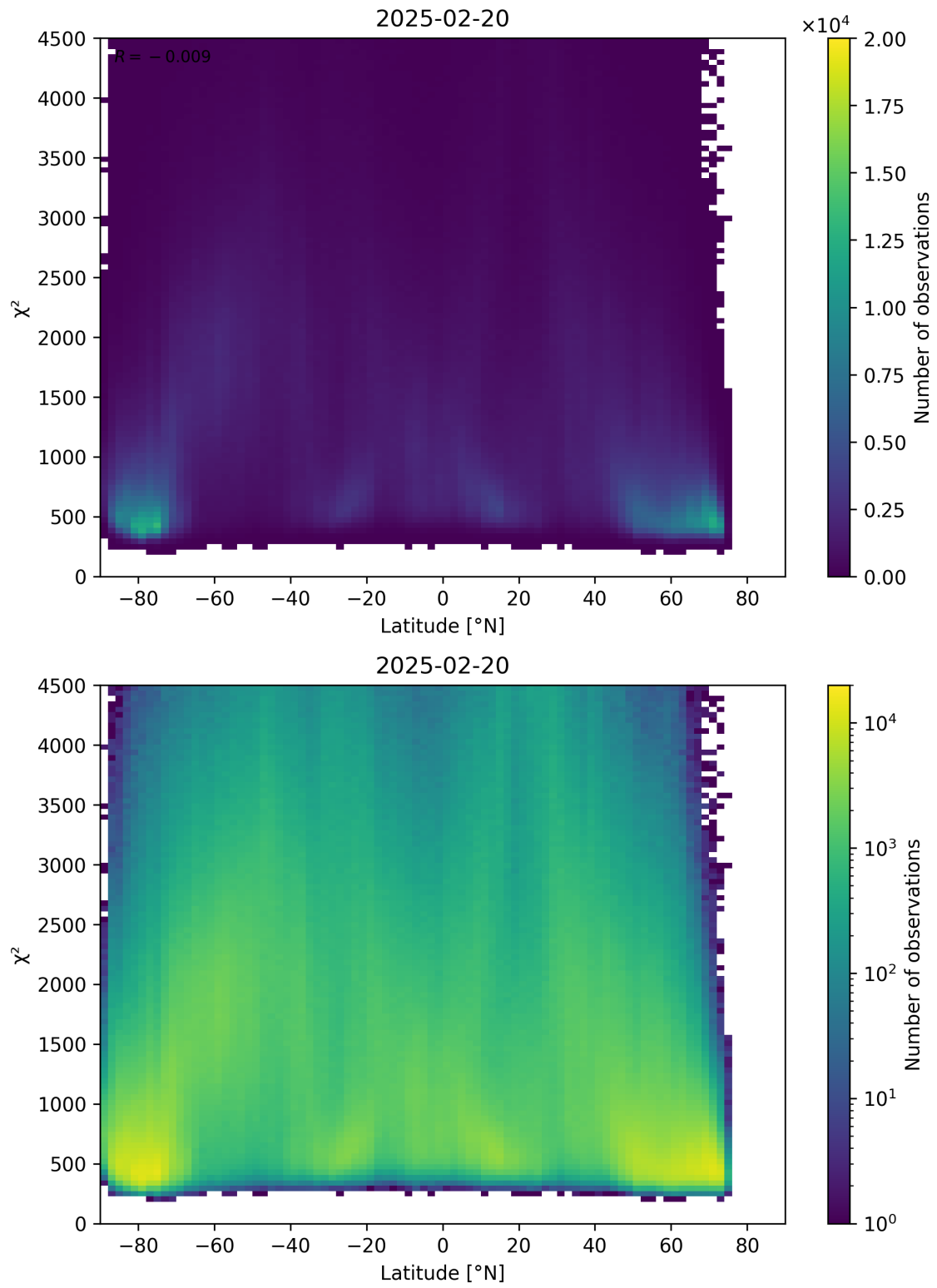
Figure 54: Scatter density plot of “Latitude” against “ \chi^2 ” for 2025-02-19 to 2025-02-21.
