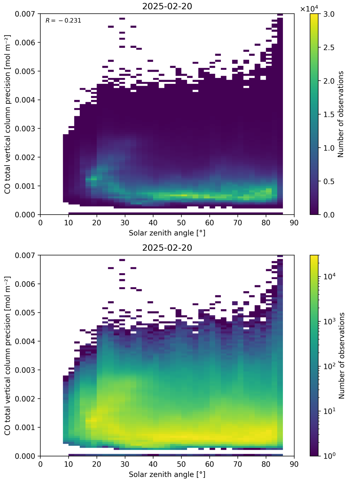
Figure 63: Scatter density plot of “Solar zenith angle” against “CO total vertical column precision” for 2025-02-19 to 2025-02-21.
