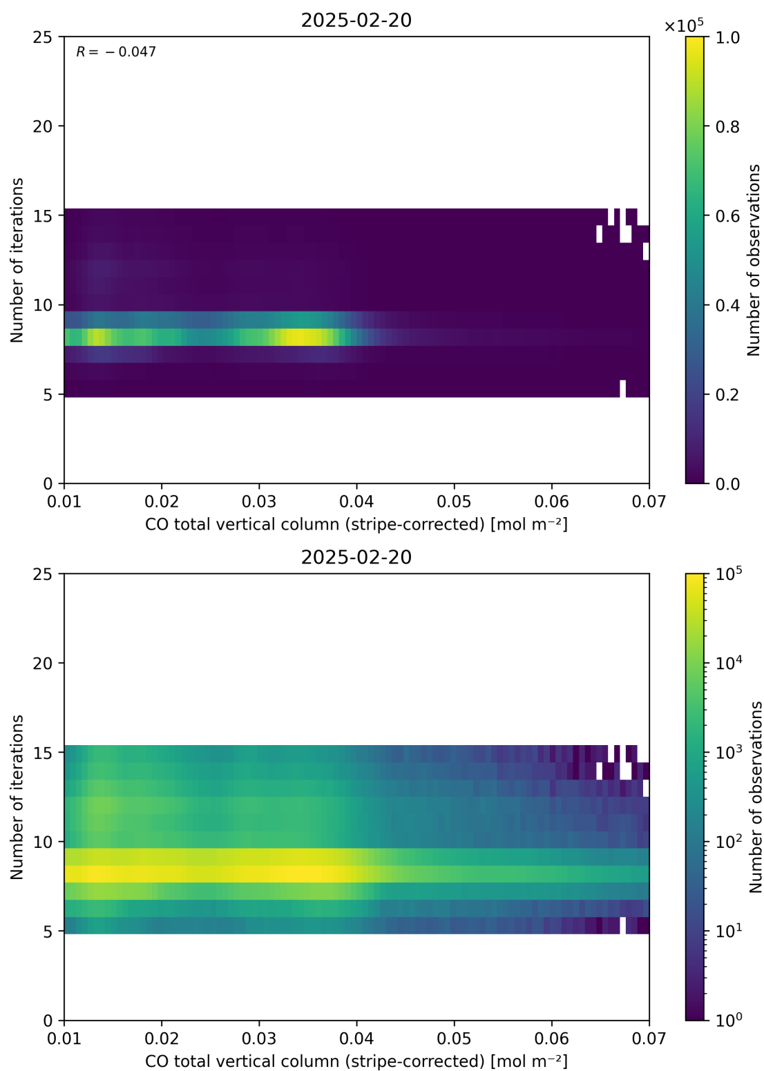
Figure 39: Scatter density plot of “CO total vertical column (stripe-corrected)” against “Number of iterations” for 2025-02-19 to 2025-02-21.
