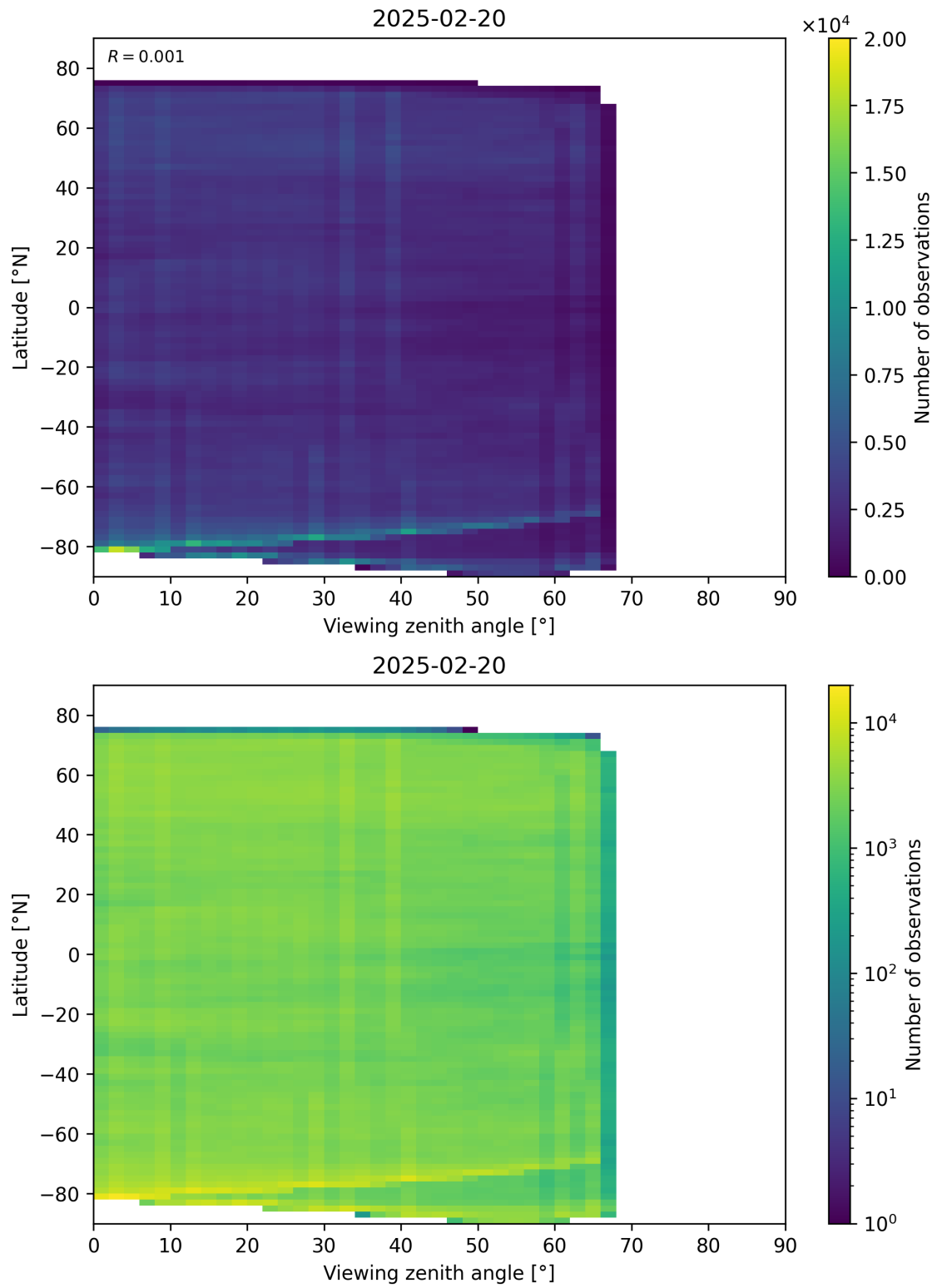
Figure 74: Scatter density plot of “Viewing zenith angle” against “Latitude” for 2025-02-19 to 2025-02-21.
