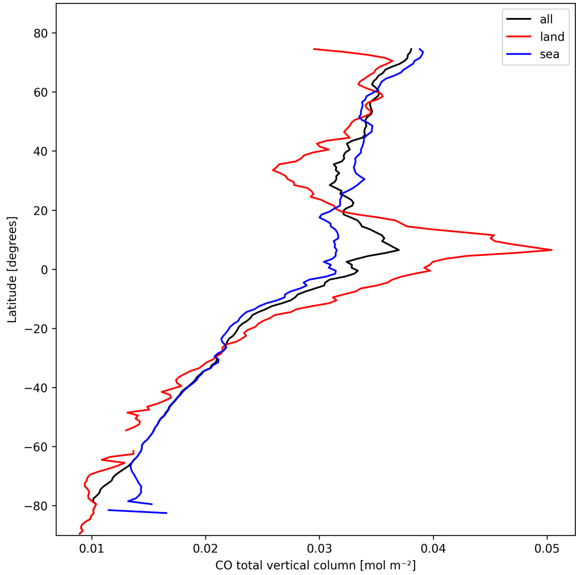
Figure 10: Zonal average of “CO total vertical column” for 2025-02-19 to 2025-02-21.
