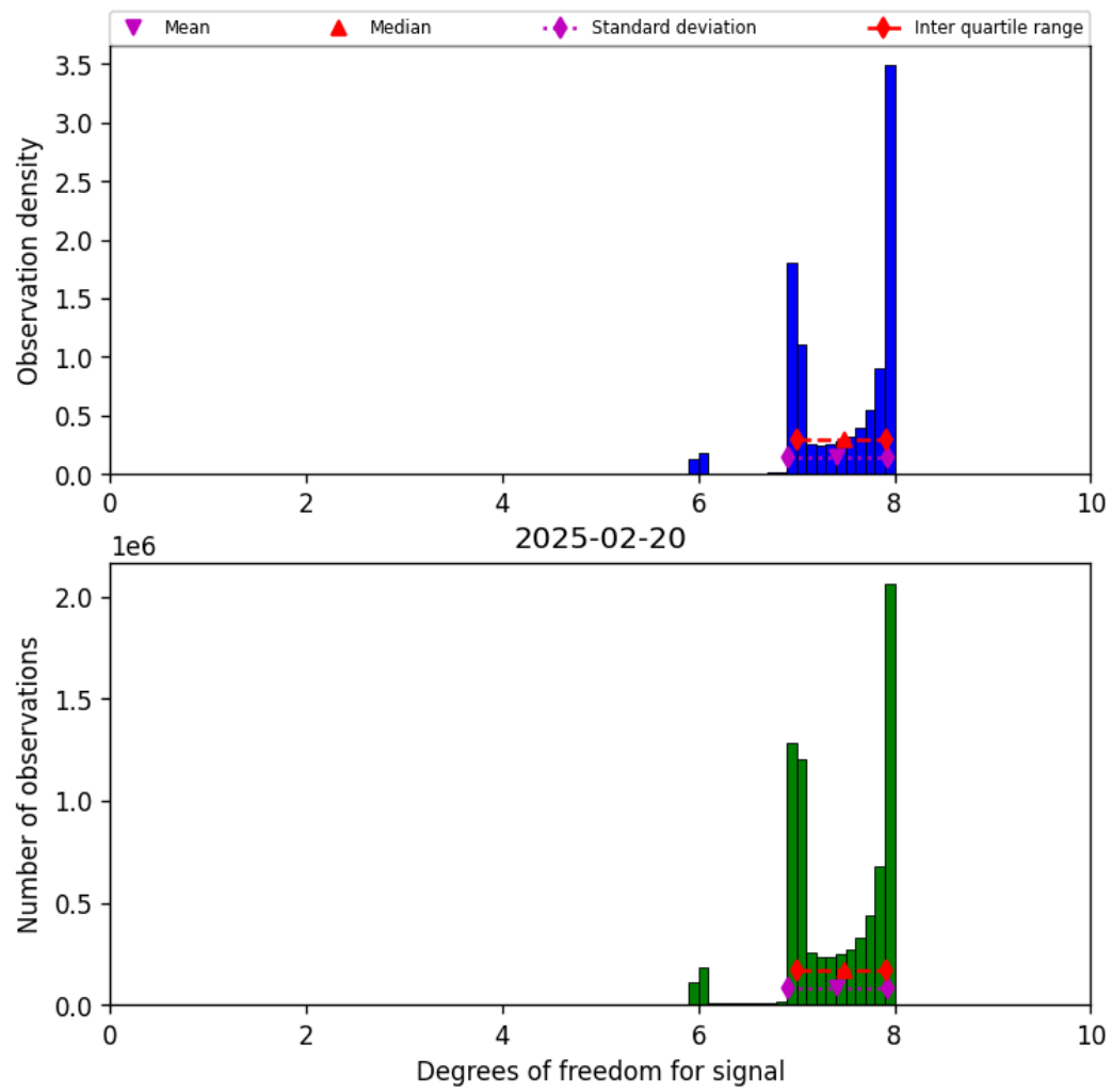
Figure 23: Histogram of “Degrees of freedom for signal” for 2025-02-19 to 2025-02-21
