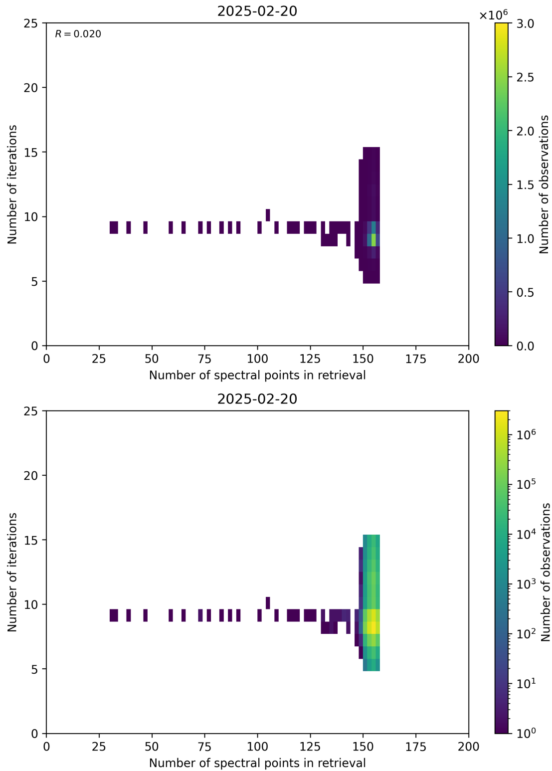
Figure 60: Scatter density plot of “Number of spectral points in retrieval” against “Number of iterations” for 2025-02-19 to 2025-02-21.
