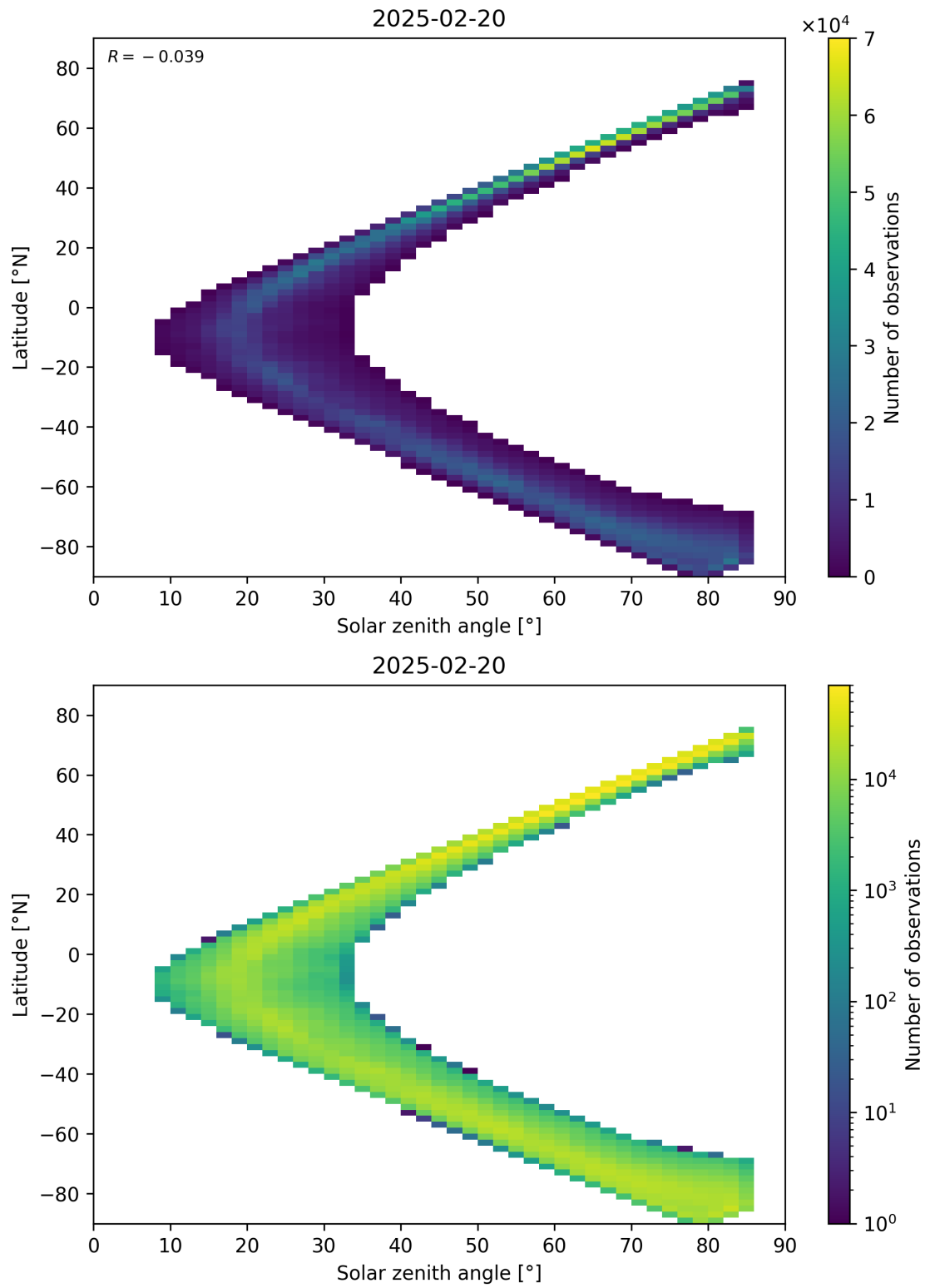
Figure 66: Scatter density plot of “Solar zenith angle” against “Latitude” for 2025-02-19 to 2025-02-21.
