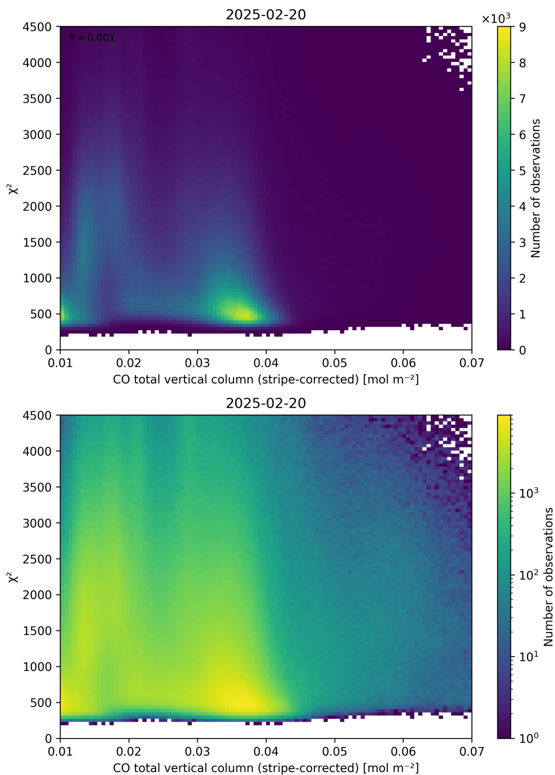
Figure 37: Scatter density plot of “CO total vertical column (stripe-corrected)” against “ \chi^2 ” for 2025-02-19 to 2025-02-21.
