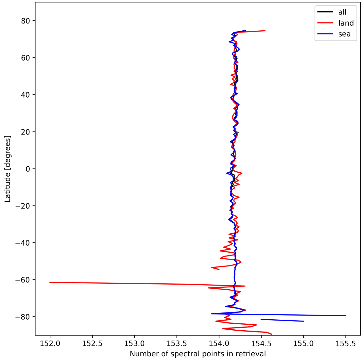
Figure 13: Zonal average of “Number of spectral points in retrieval” for 2025-02-19 to 2025-02-21.
