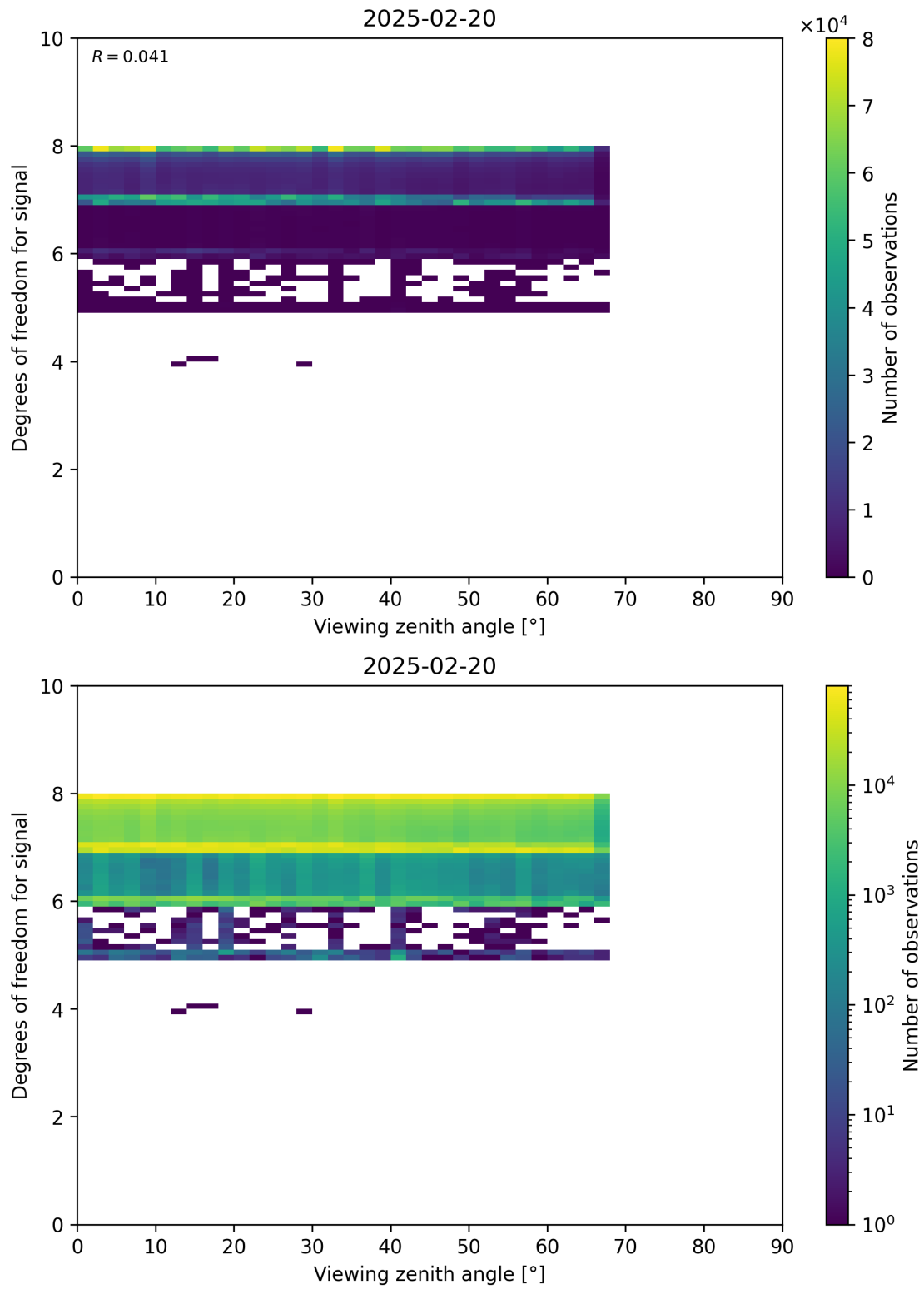
Figure 73: Scatter density plot of “Viewing zenith angle” against “Degrees of freedom for signal” for 2025-02-19 to 2025-02-21.
