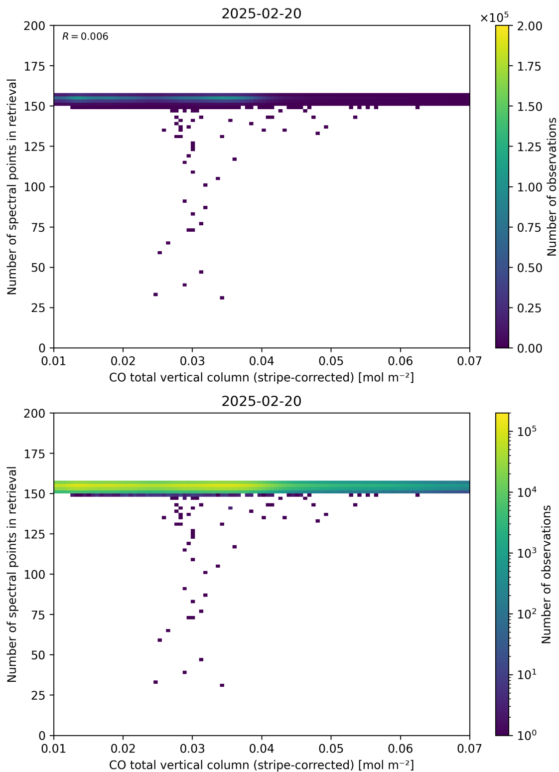
Figure 40: Scatter density plot of “CO total vertical column (stripe-corrected)” against “Number of spectral points in retrieval” for 2025-02-19 to 2025-02-21.
