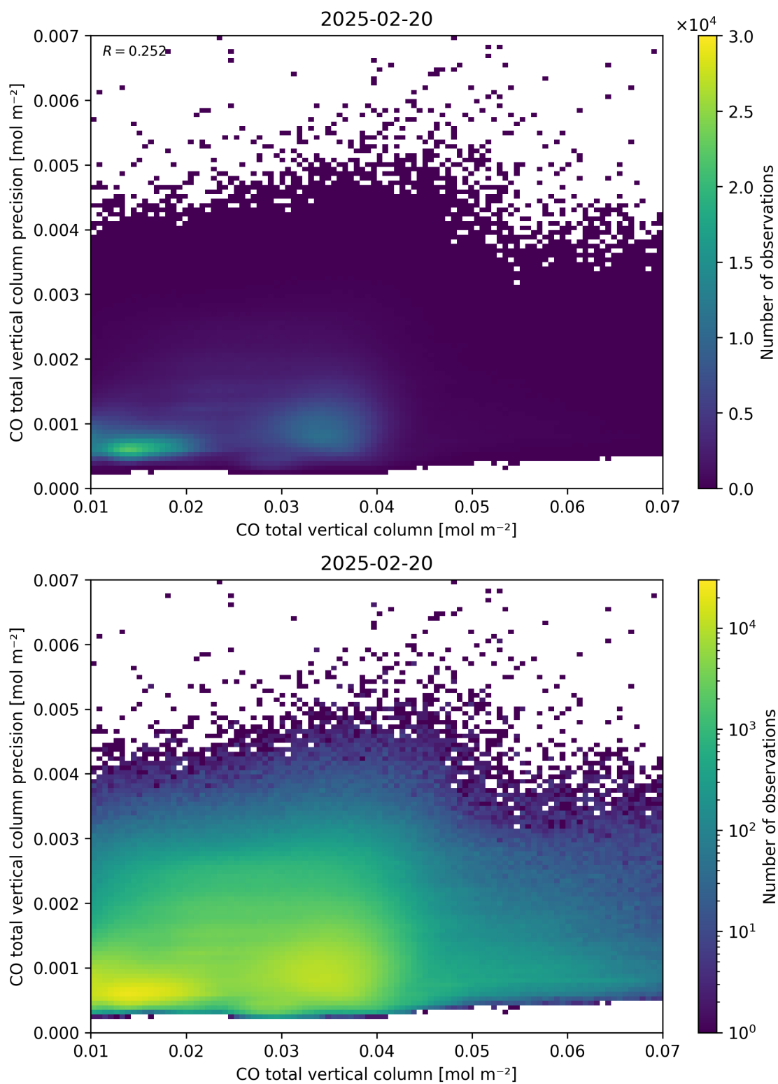
Figure 34: Scatter density plot of “CO total vertical column” against “CO total vertical column precision” for 2025-02-19 to 2025-02-21.
