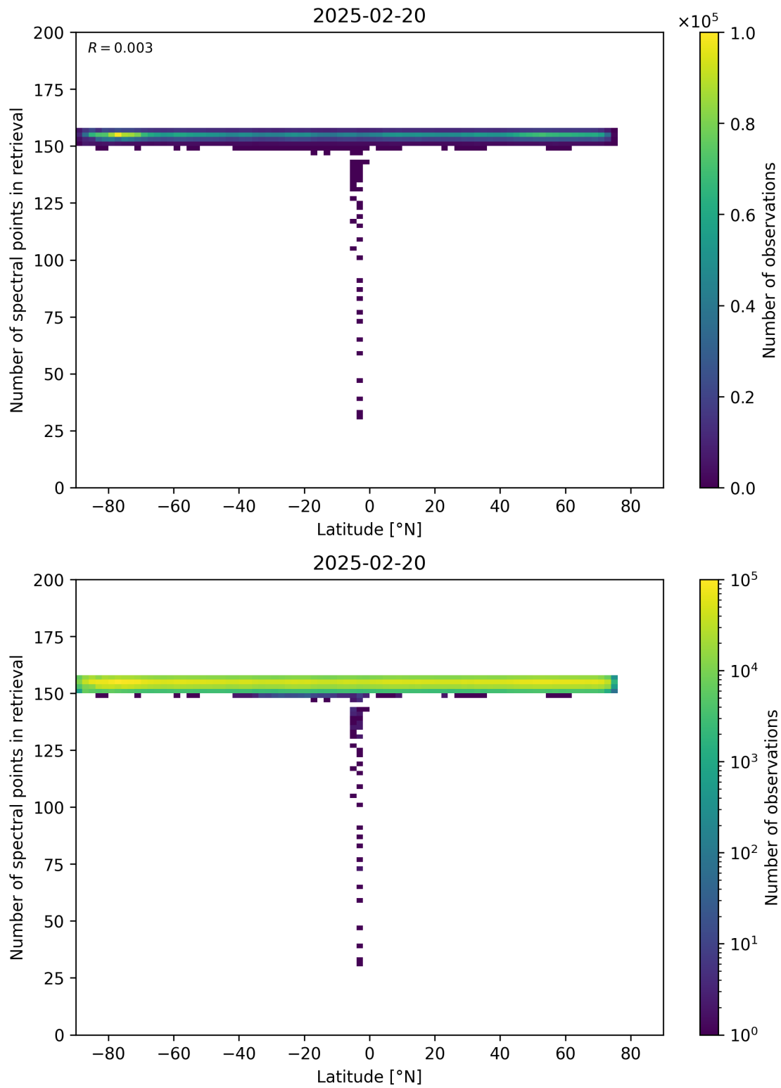
Figure 57: Scatter density plot of “Latitude” against “Number of spectral points in retrieval” for 2025-02-19 to 2025-02-21.
