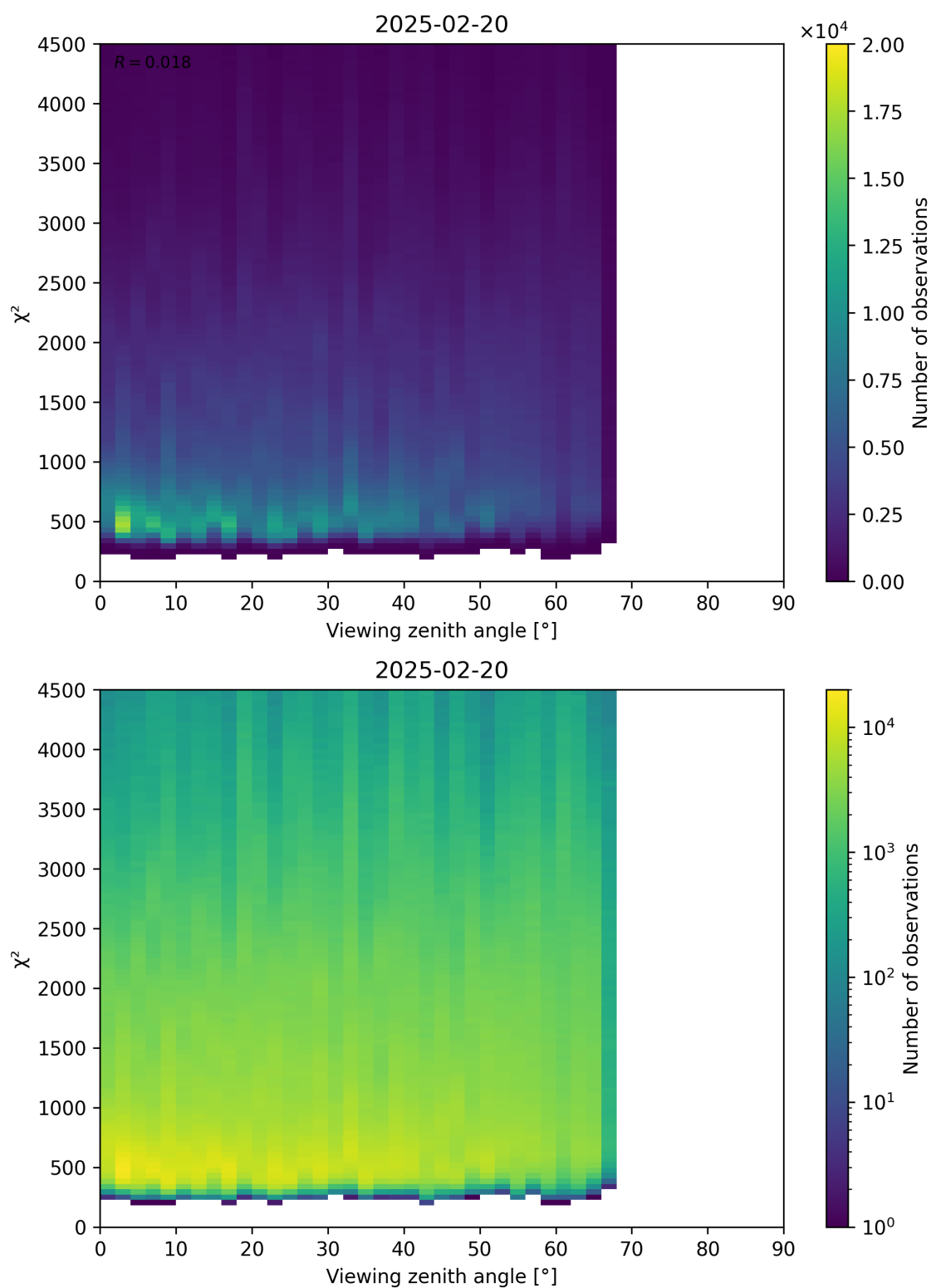
Figure 72: Scatter density plot of “Viewing zenith angle” against “ \chi^2 ” for 2025-02-19 to 2025-02-21.
