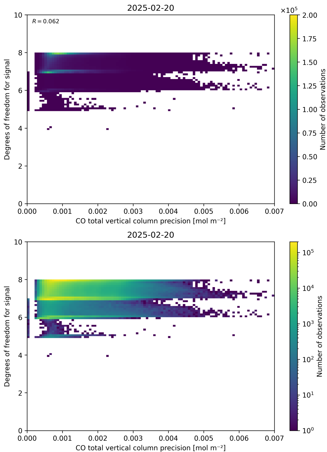
Figure 45: Scatter density plot of “CO total vertical column precision” against “Degrees of freedom for signal” for 2025-02-19 to 2025-02-21.
