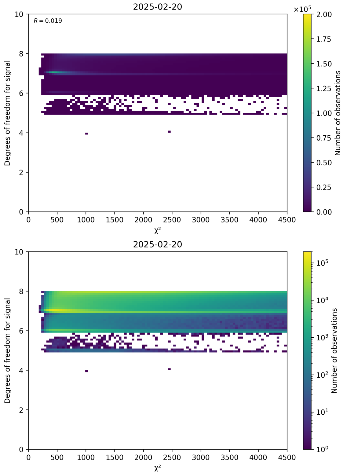
Figure 48: Scatter density plot of “ \chi^2 ” against “Degrees of freedom for signal” for 2025-02-19 to 2025-02-21.
