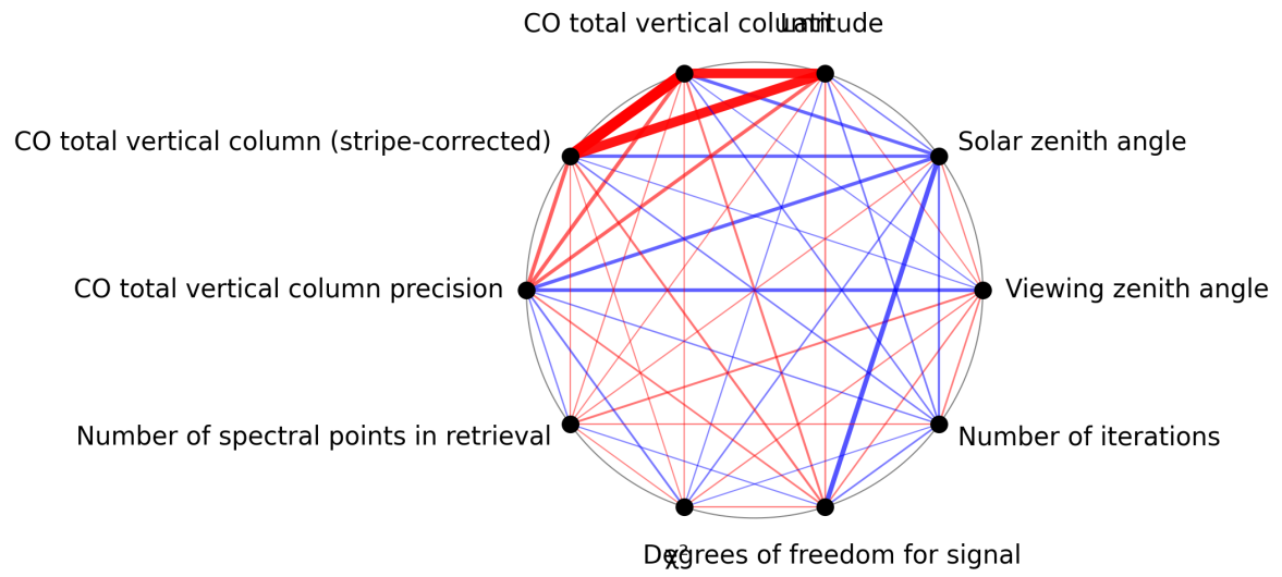
Figure 1: Map of correlation graph for 2025-02-19 to 2025-02-21.
