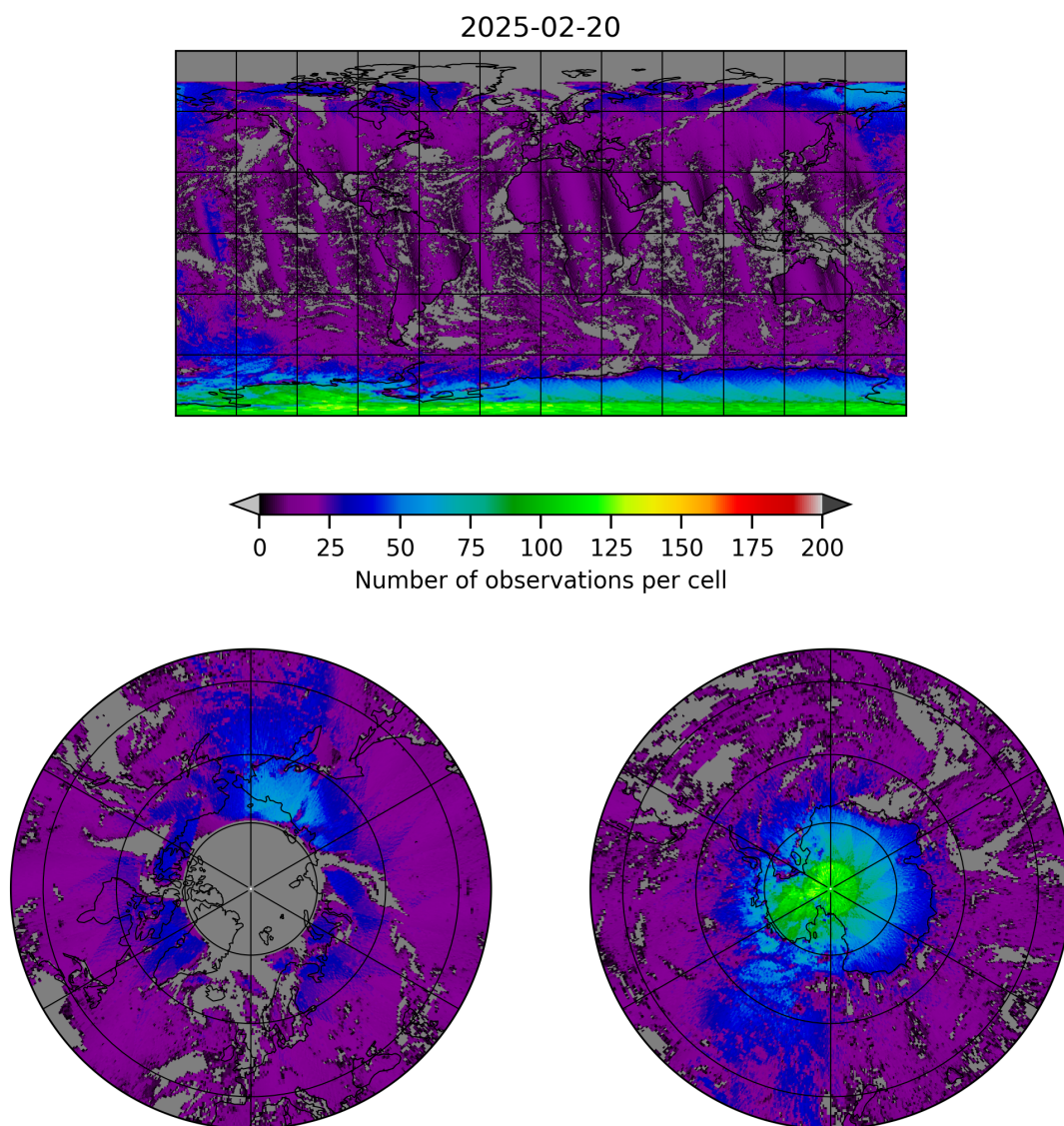
Figure 8: Map of the number of observations for 2025-02-19 to 2025-02-21
