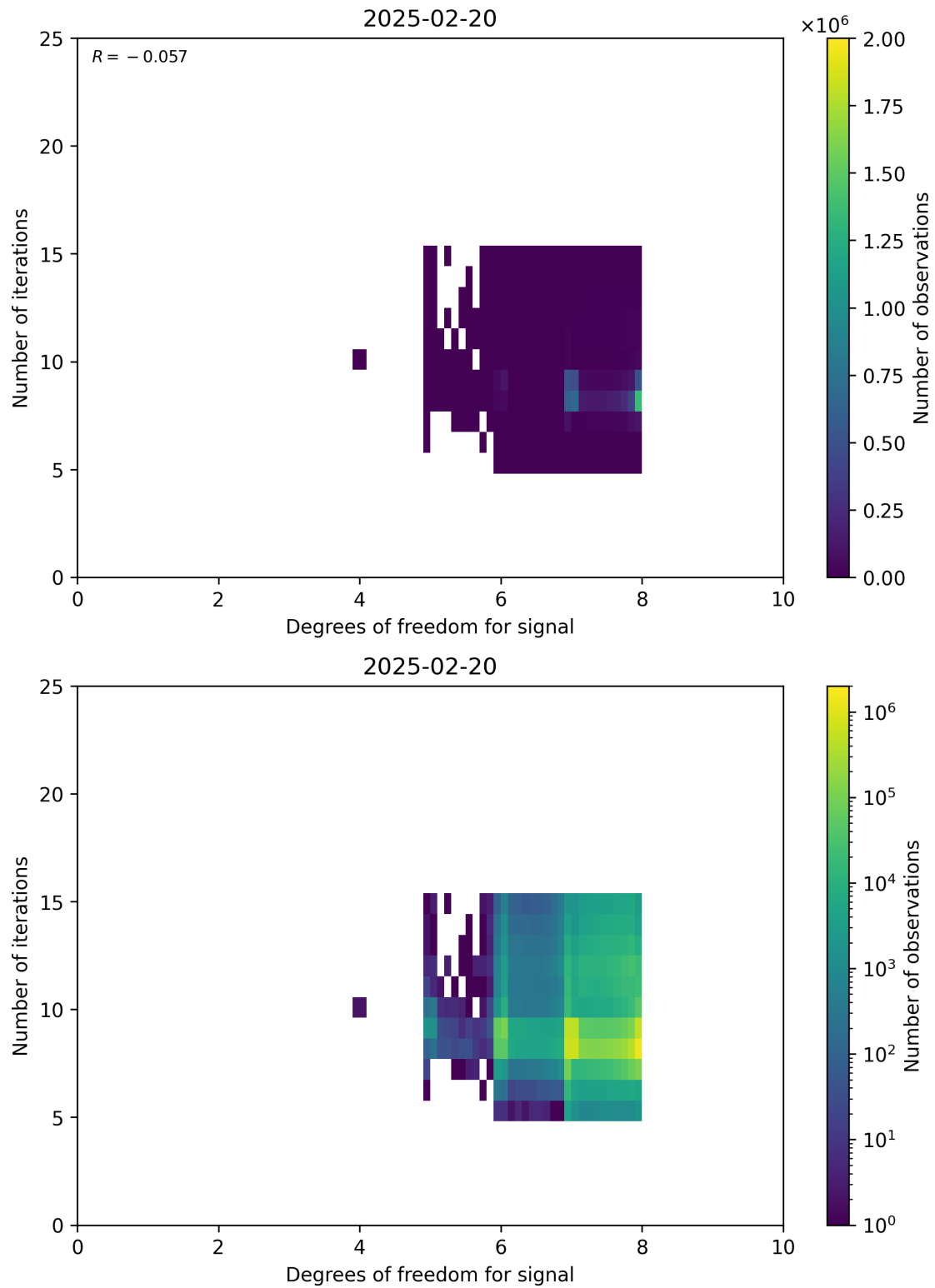
Figure 50: Scatter density plot of “Degrees of freedom for signal” against “Number of iterations” for 2025-02-19 to 2025-02-21.
