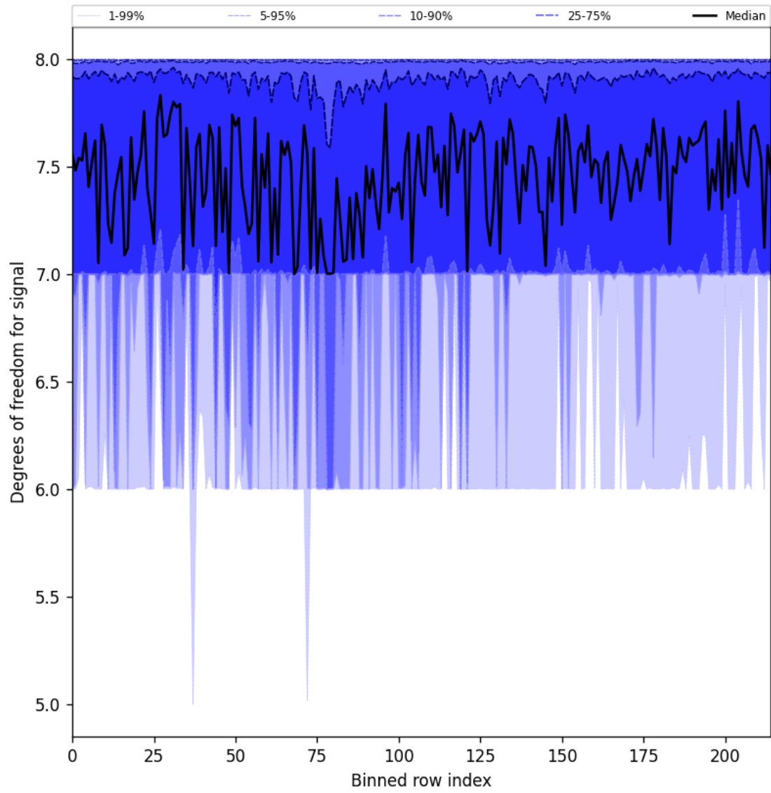
Figure 31: Along track statistics of “Degrees of freedom for signal” for 2025-02-19 to 2025-02-21
