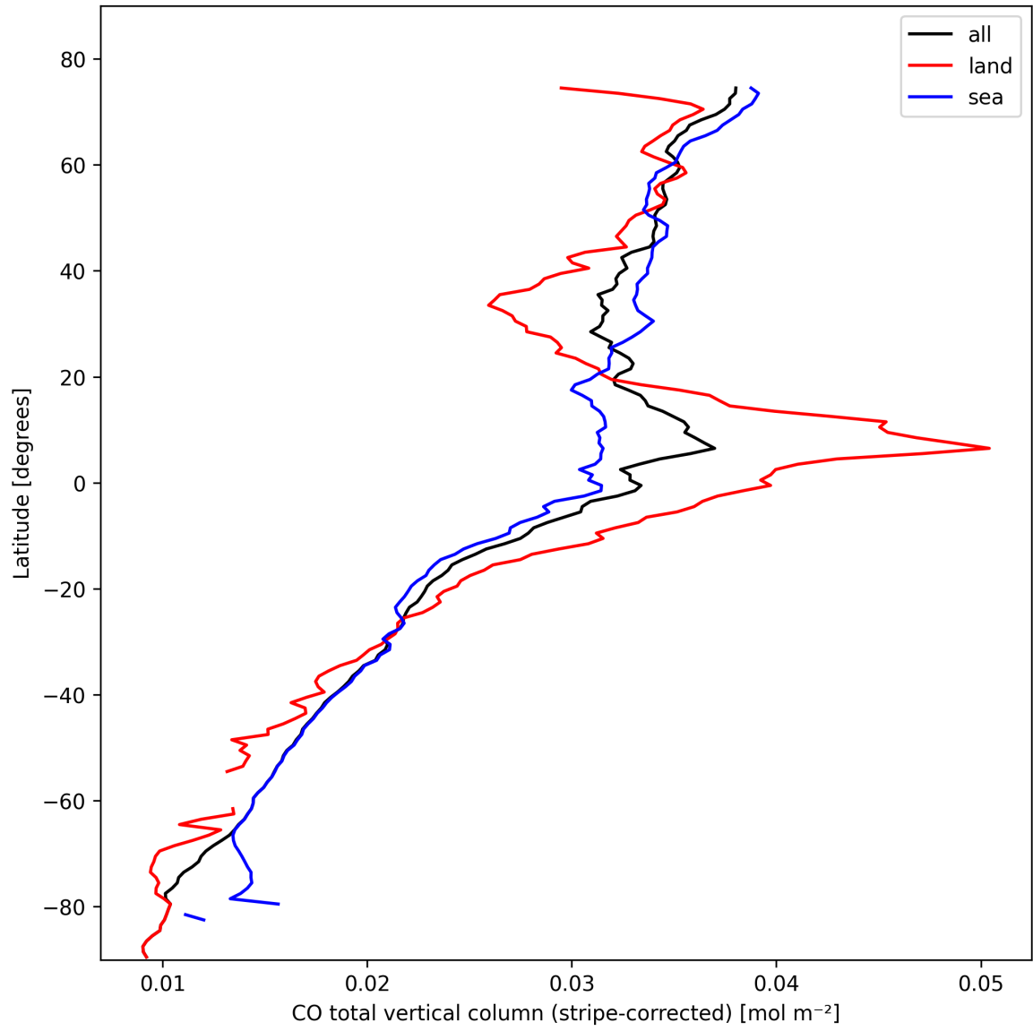
Figure 11: Zonal average of “CO total vertical column (stripe-corrected)” for 2025-02-19 to 2025-02-21.
