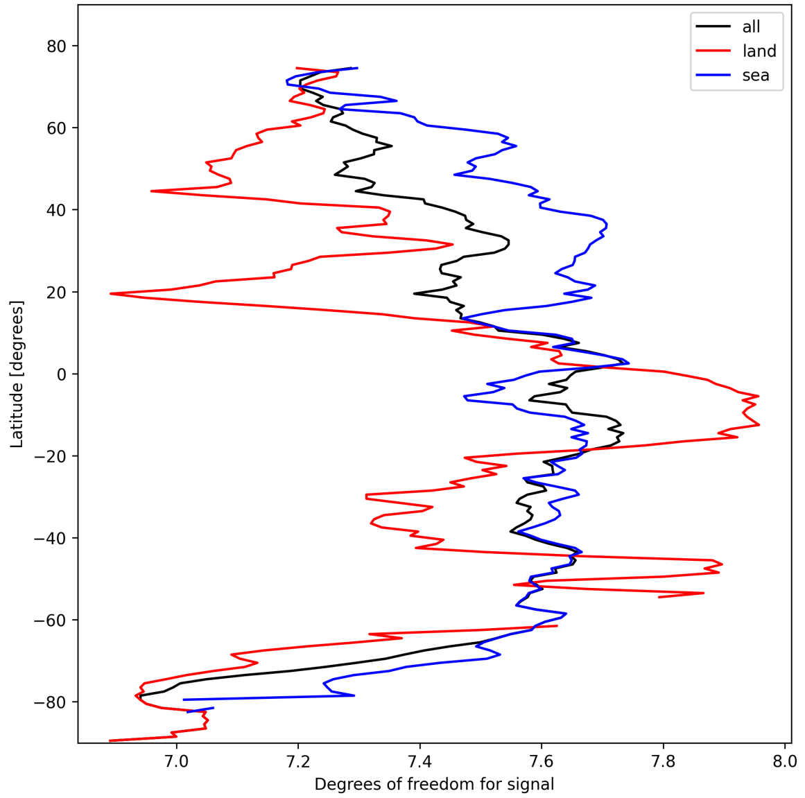
Figure 15: Zonal average of “Degrees of freedom for signal” for 2025-02-19 to 2025-02-21.
