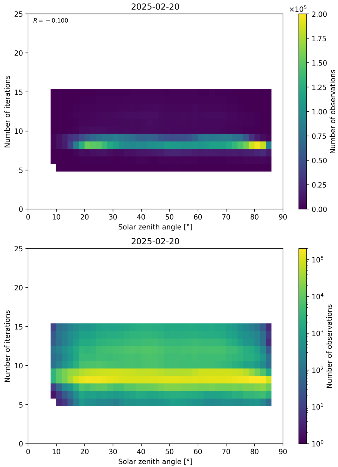
Figure 67: Scatter density plot of “Solar zenith angle” against “Number of iterations” for 2025-02-19 to 2025-02-21.
