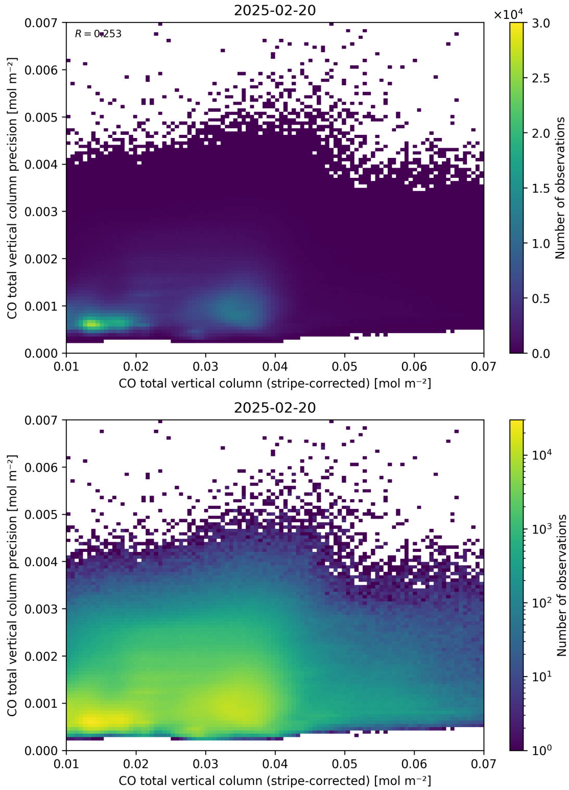
Figure 36: Scatter density plot of “CO total vertical column (stripe-corrected)” against “CO total vertical column precision” for 2025-02-19 to 2025-02-21.
