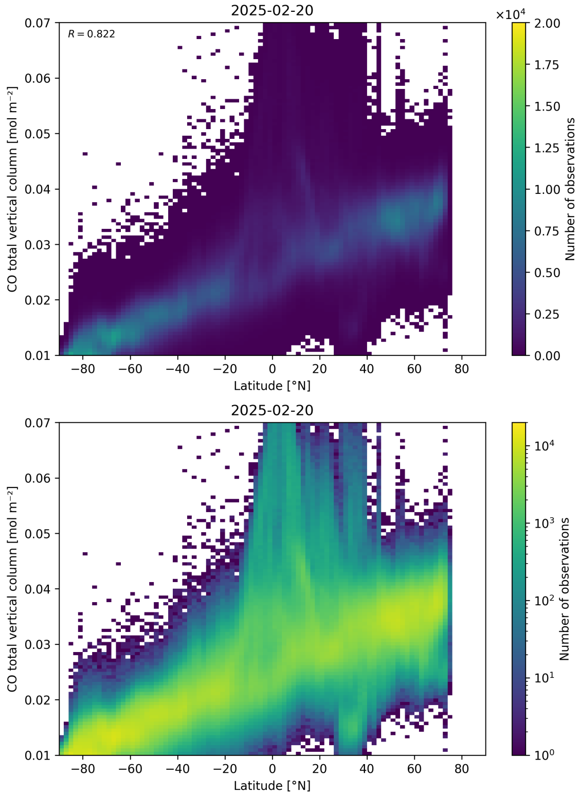
Figure 51: Scatter density plot of “Latitude” against “CO total vertical column” for 2025-02-19 to 2025-02-21.
