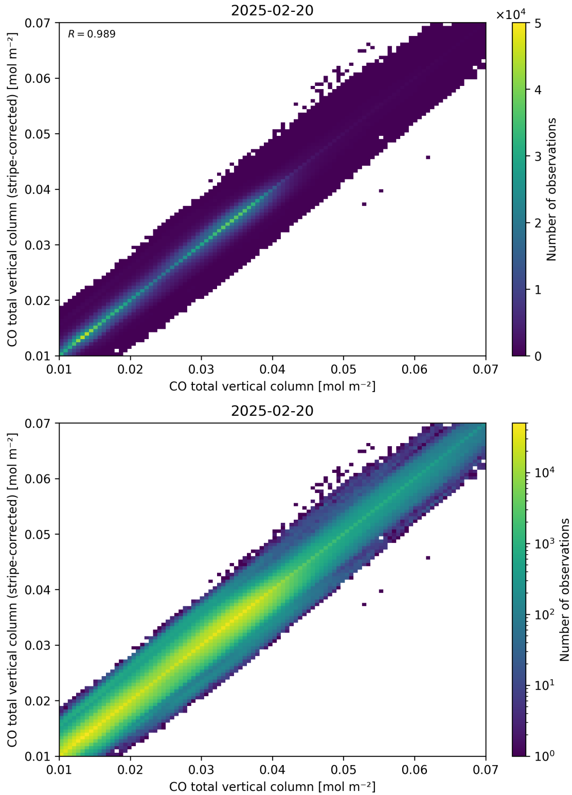
Figure 33: Scatter density plot of “CO total vertical column” against “CO total vertical column (stripe-corrected)” for 2025-02-19 to 2025-02-21.
