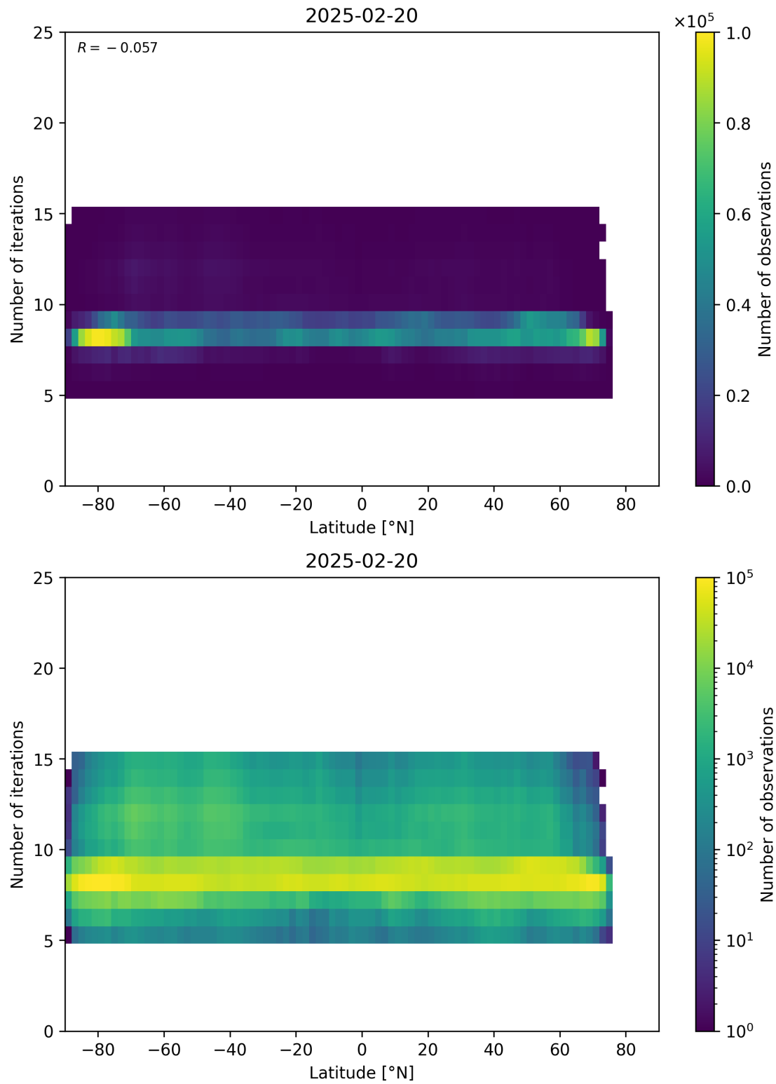
Figure 56: Scatter density plot of “Latitude” against “Number of iterations” for 2025-02-19 to 2025-02-21.
