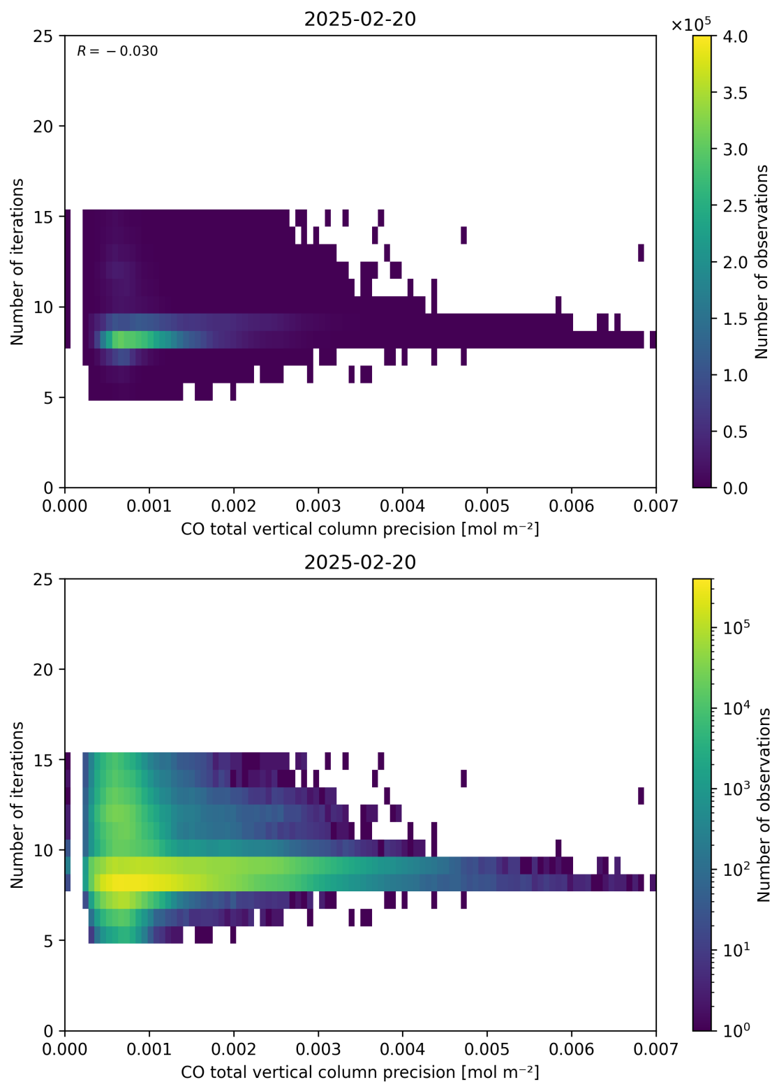
Figure 46: Scatter density plot of “CO total vertical column precision” against “Number of iterations” for 2025-02-19 to 2025-02-21.
