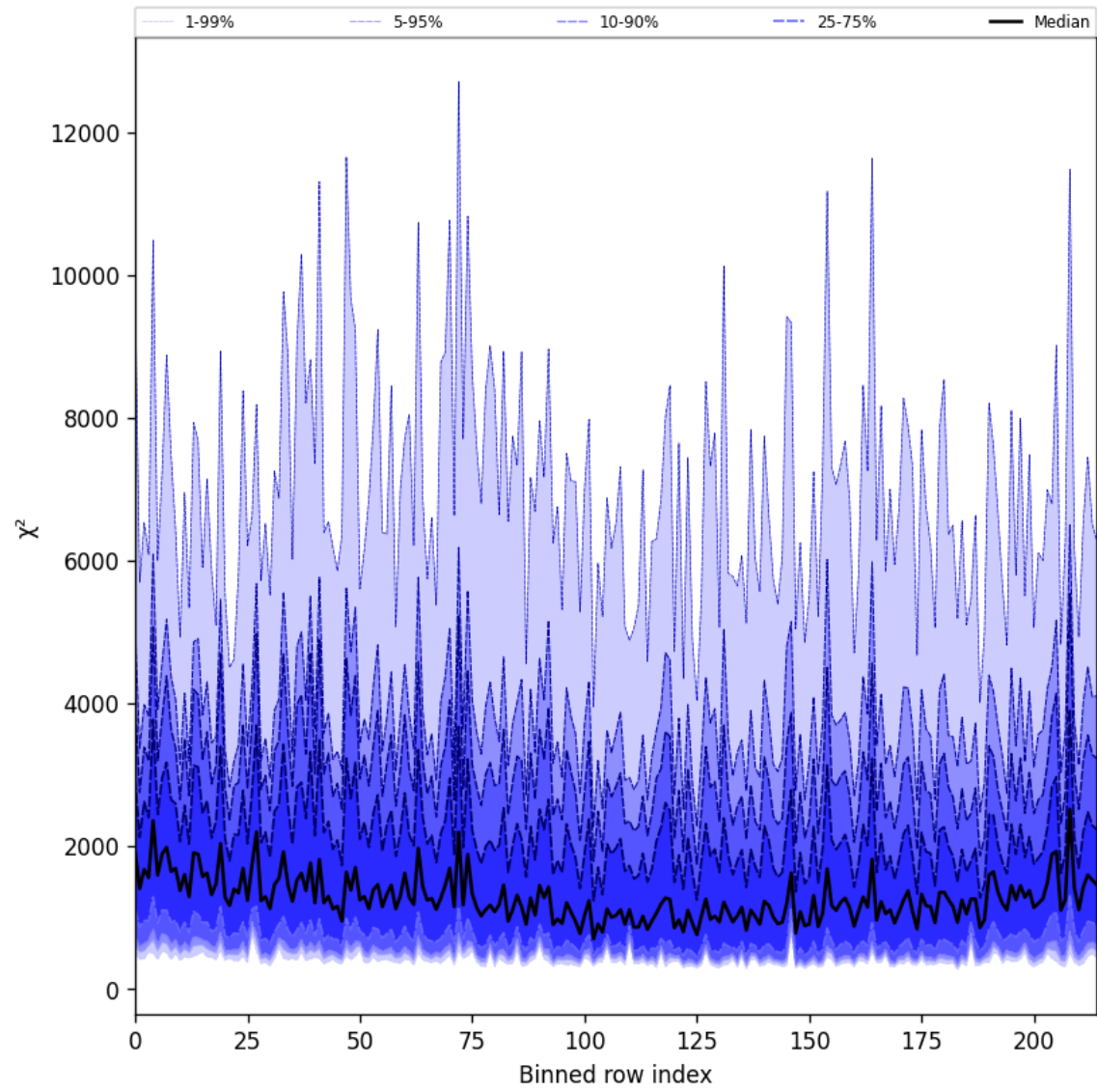
Figure 30: Along track statistics of “ \chi^2 ” for 2025-02-19 to 2025-02-21
