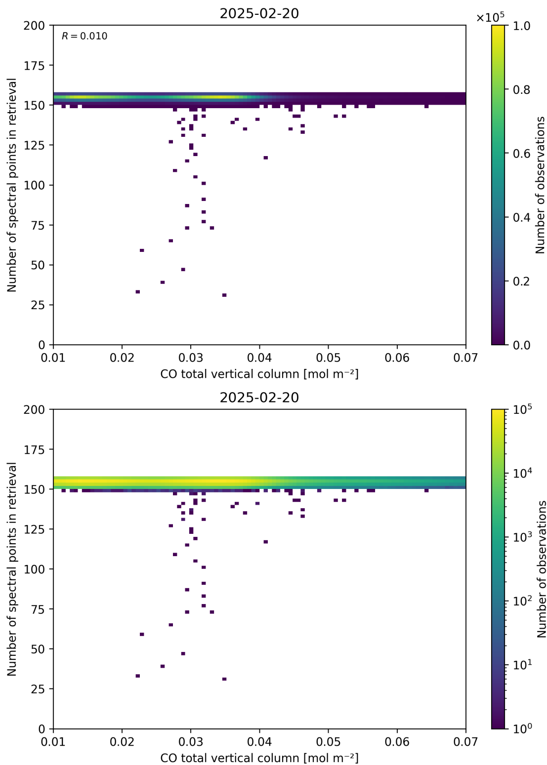
Figure 43: Scatter density plot of “CO total vertical column” against “Number of spectral points in retrieval” for 2025-02-19 to 2025-02-21.
