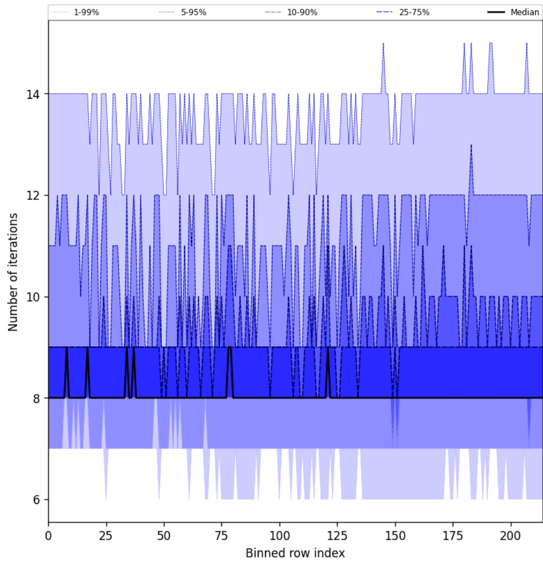
Figure 32: Along track statistics of “Number of iterations” for 2025-02-19 to 2025-02-21
