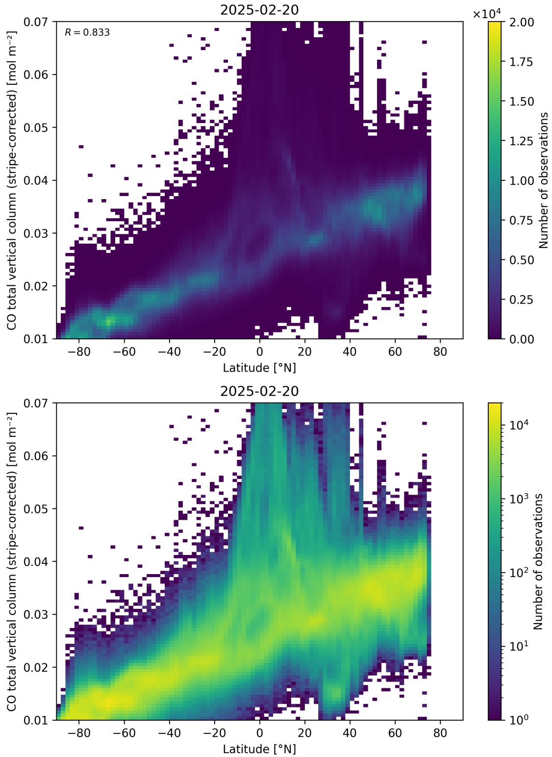
Figure 52: Scatter density plot of “Latitude” against “CO total vertical column (stripe-corrected)” for 2025-02-19 to 2025-02-21.
