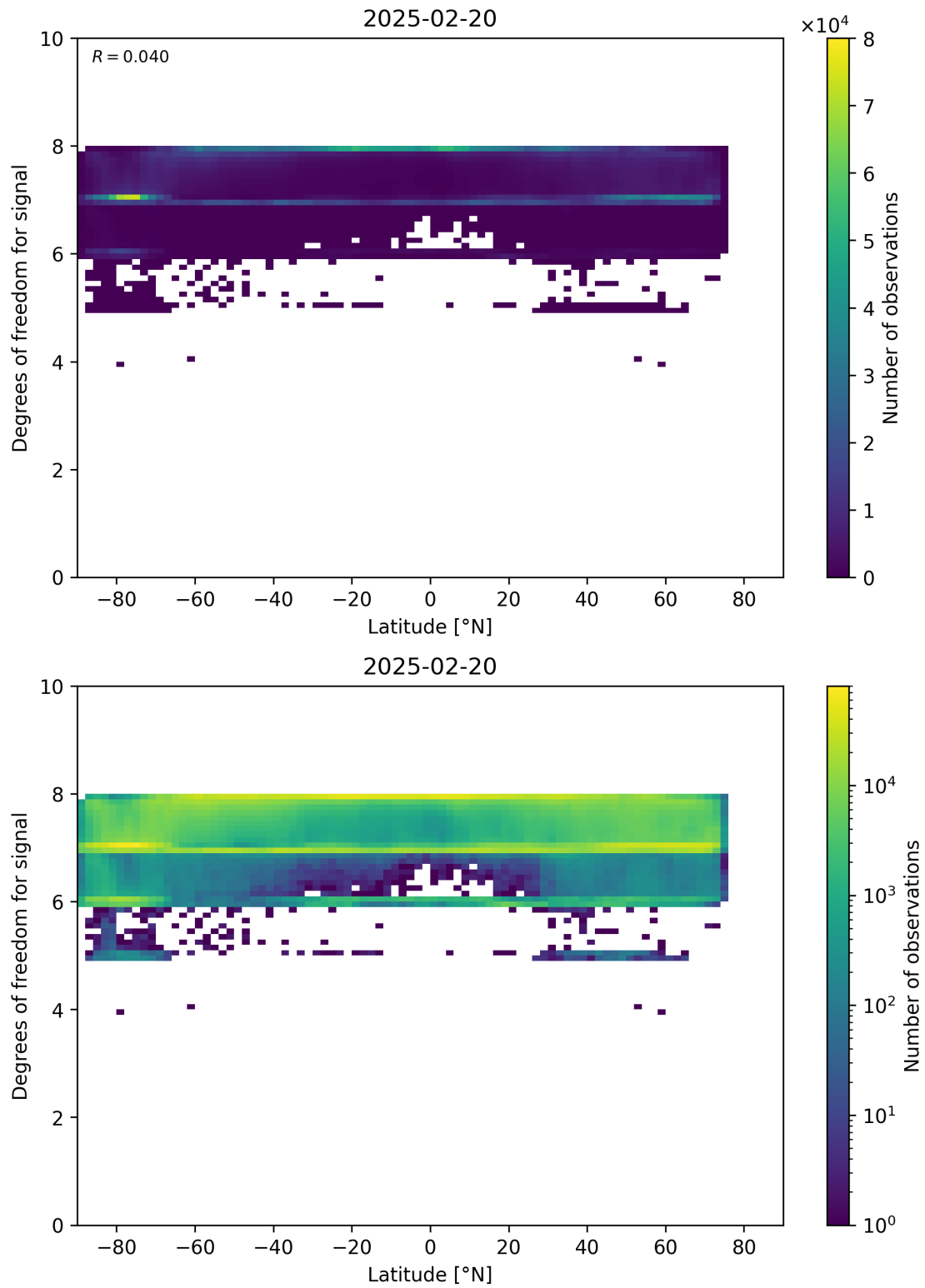
Figure 55: Scatter density plot of “Latitude” against “Degrees of freedom for signal” for 2025-02-19 to 2025-02-21.
