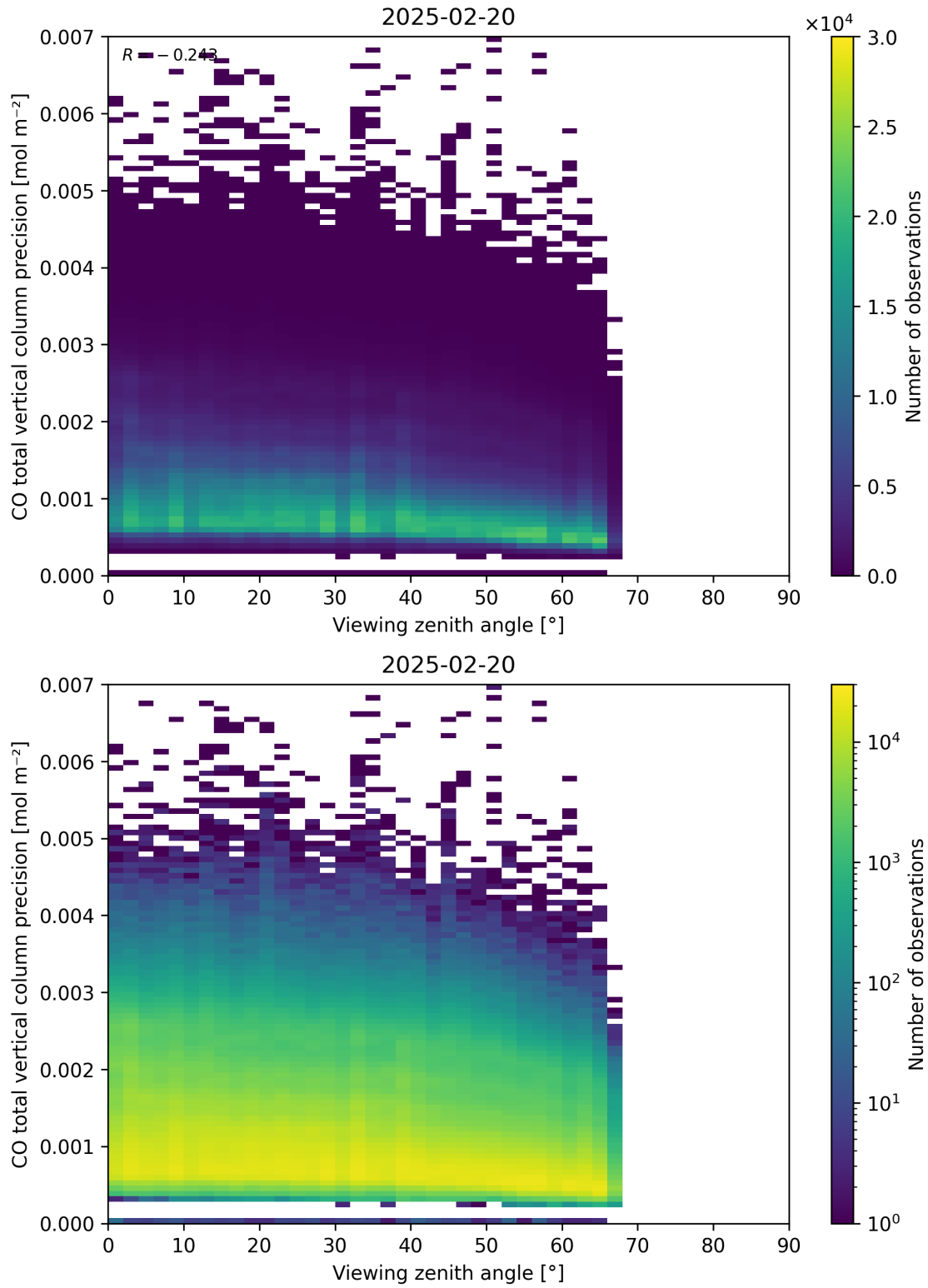
Figure 71: Scatter density plot of “Viewing zenith angle” against “CO total vertical column precision” for 2025-02-19 to 2025-02-21.
