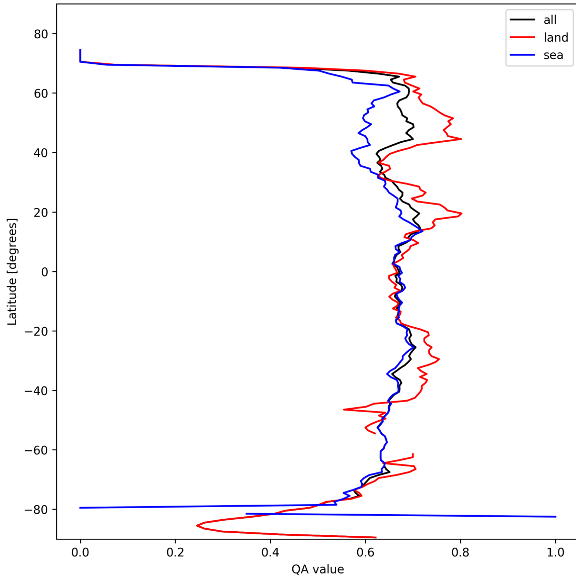
Figure 9: Zonal average of “QA value” for 2025-02-19 to 2025-02-21.
