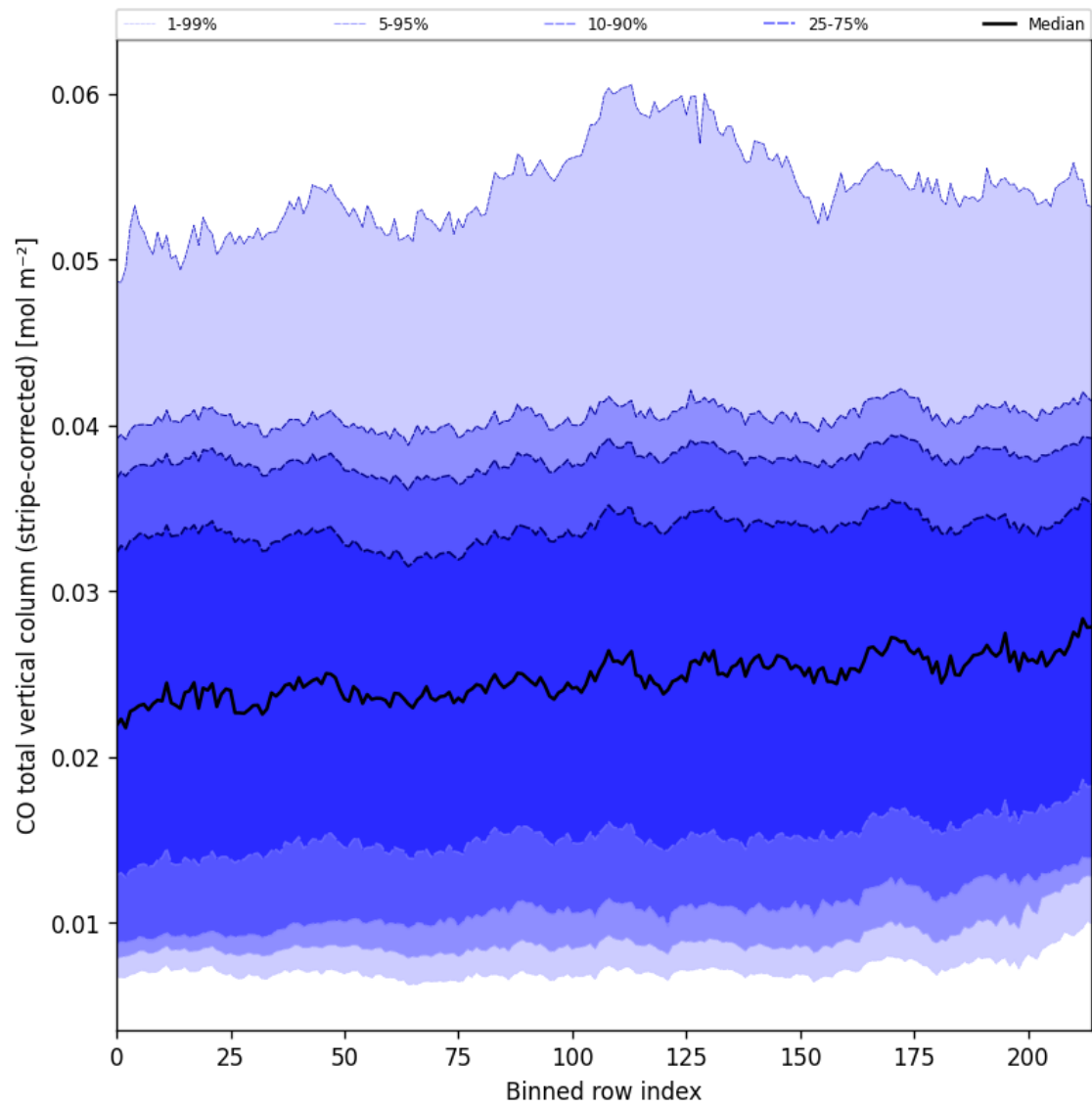
Figure 27: Along track statistics of “CO total vertical column (stripe-corrected)” for 2025-02-19 to 2025-02-21
