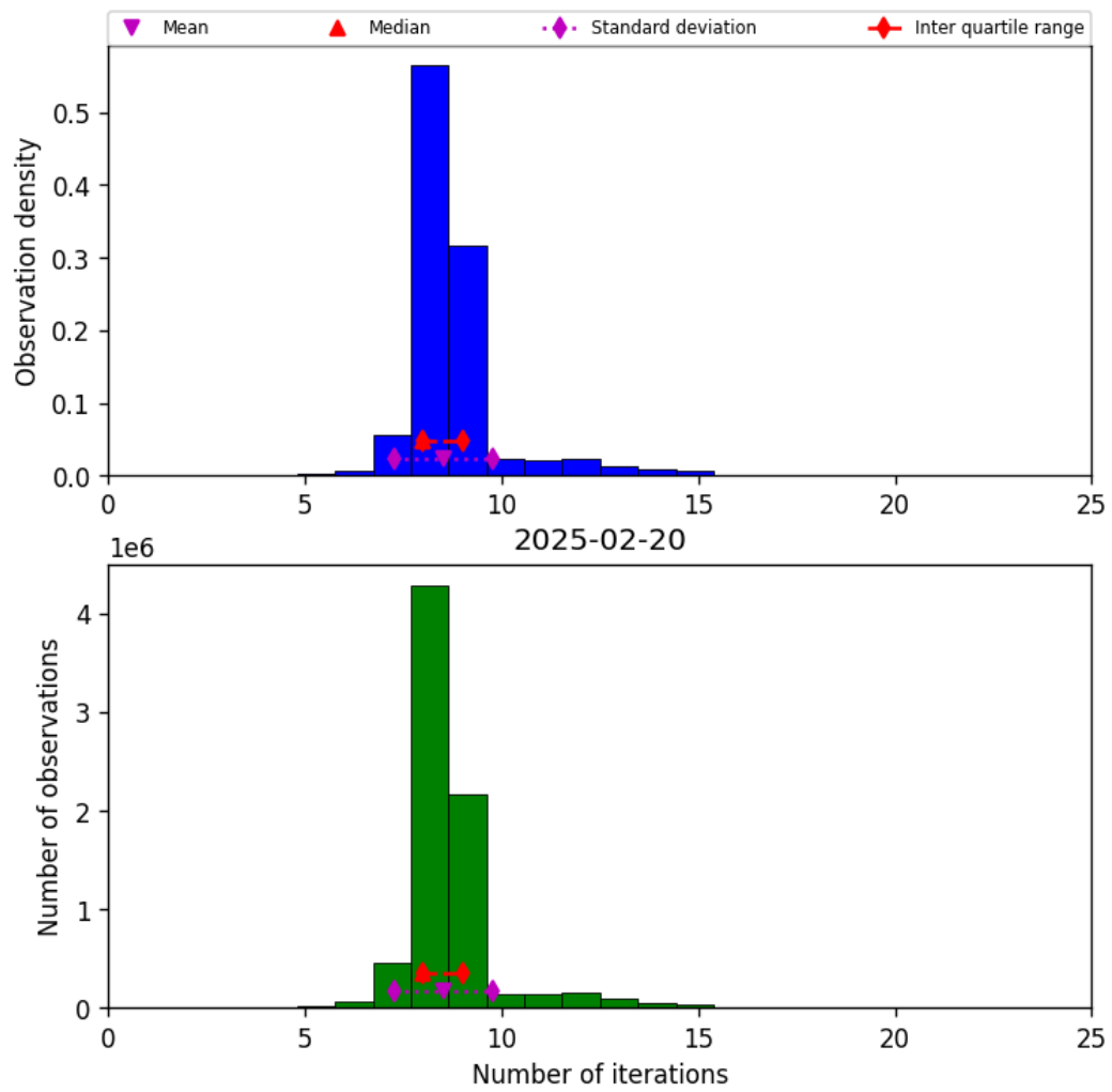
Figure 24: Histogram of “Number of iterations” for 2025-02-19 to 2025-02-21
