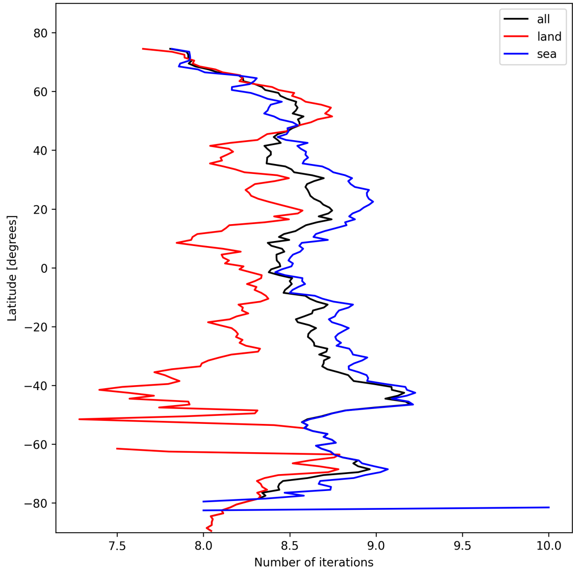
Figure 16: Zonal average of “Number of iterations” for 2025-02-19 to 2025-02-21.
