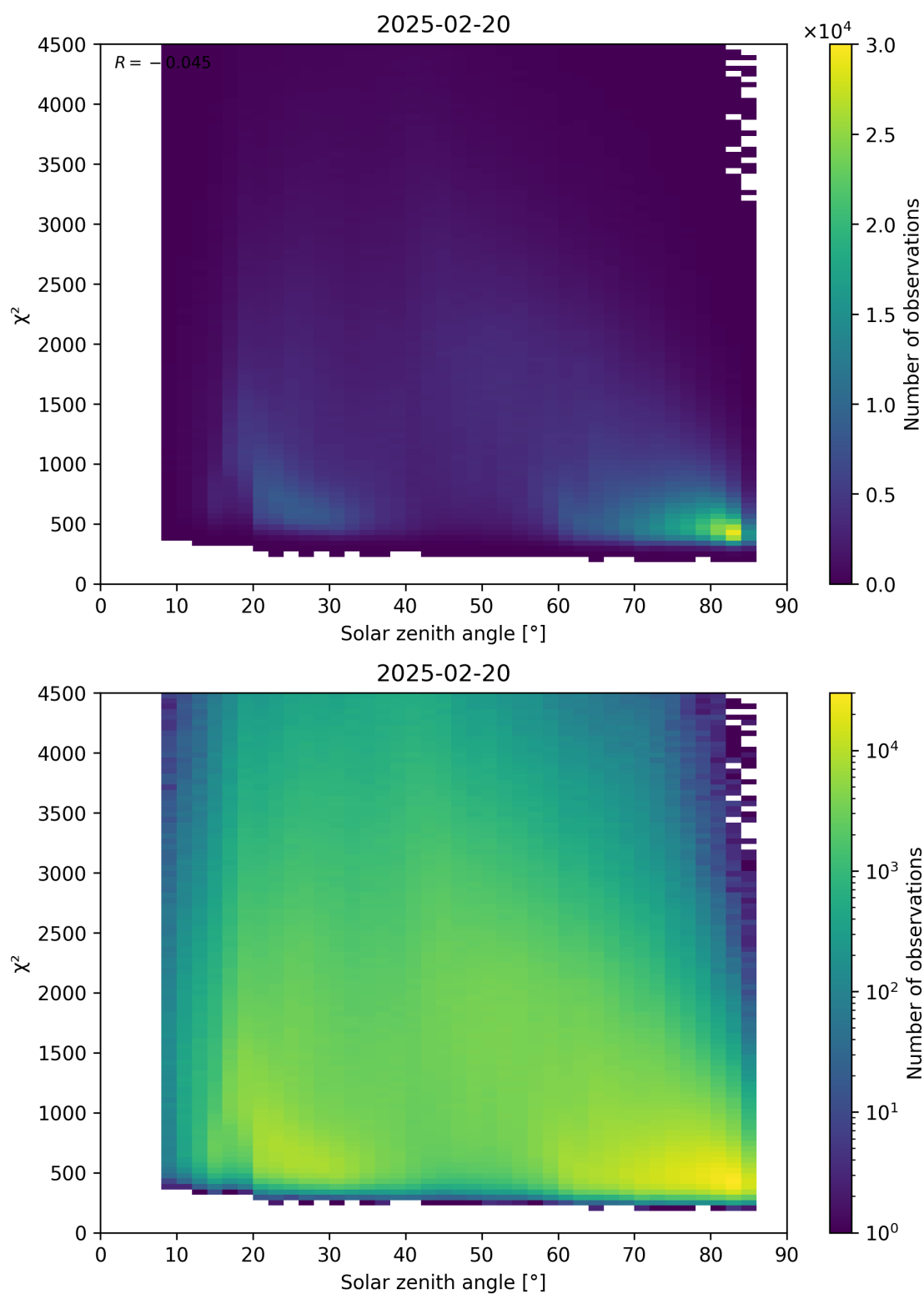
Figure 64: Scatter density plot of “Solar zenith angle” against “ \chi^2 ” for 2025-02-19 to 2025-02-21.
