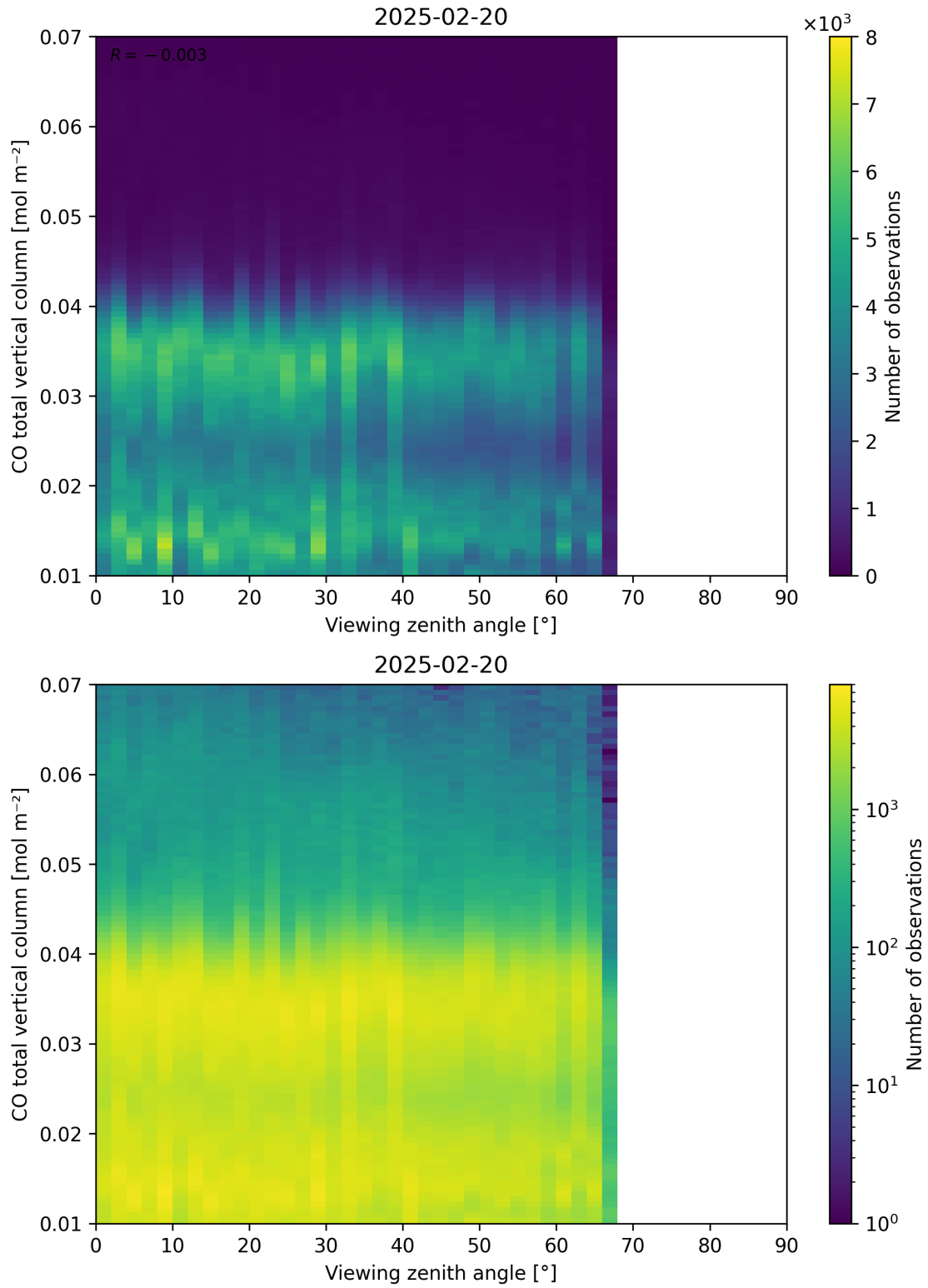
Figure 69: Scatter density plot of “Viewing zenith angle” against “CO total vertical column” for 2025-02-19 to 2025-02-21.
