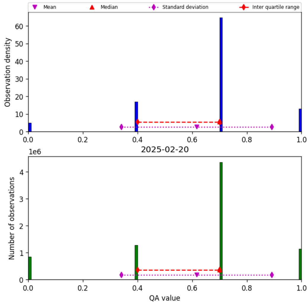
Figure 17: Histogram of “QA value” for 2025-02-19 to 2025-02-21
