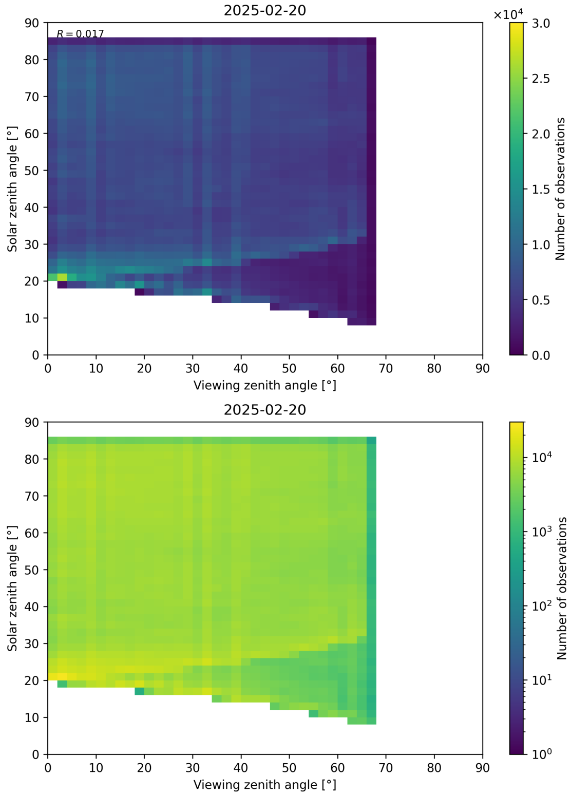
Figure 77: Scatter density plot of “Viewing zenith angle” against “Solar zenith angle” for 2025-02-19 to 2025-02-21.
