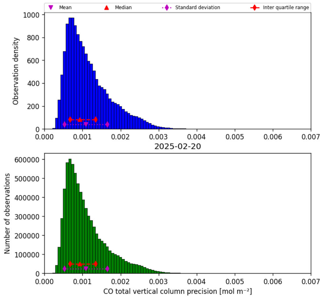
Figure 20: Histogram of “CO total vertical column precision” for 2025-02-19 to 2025-02-21
