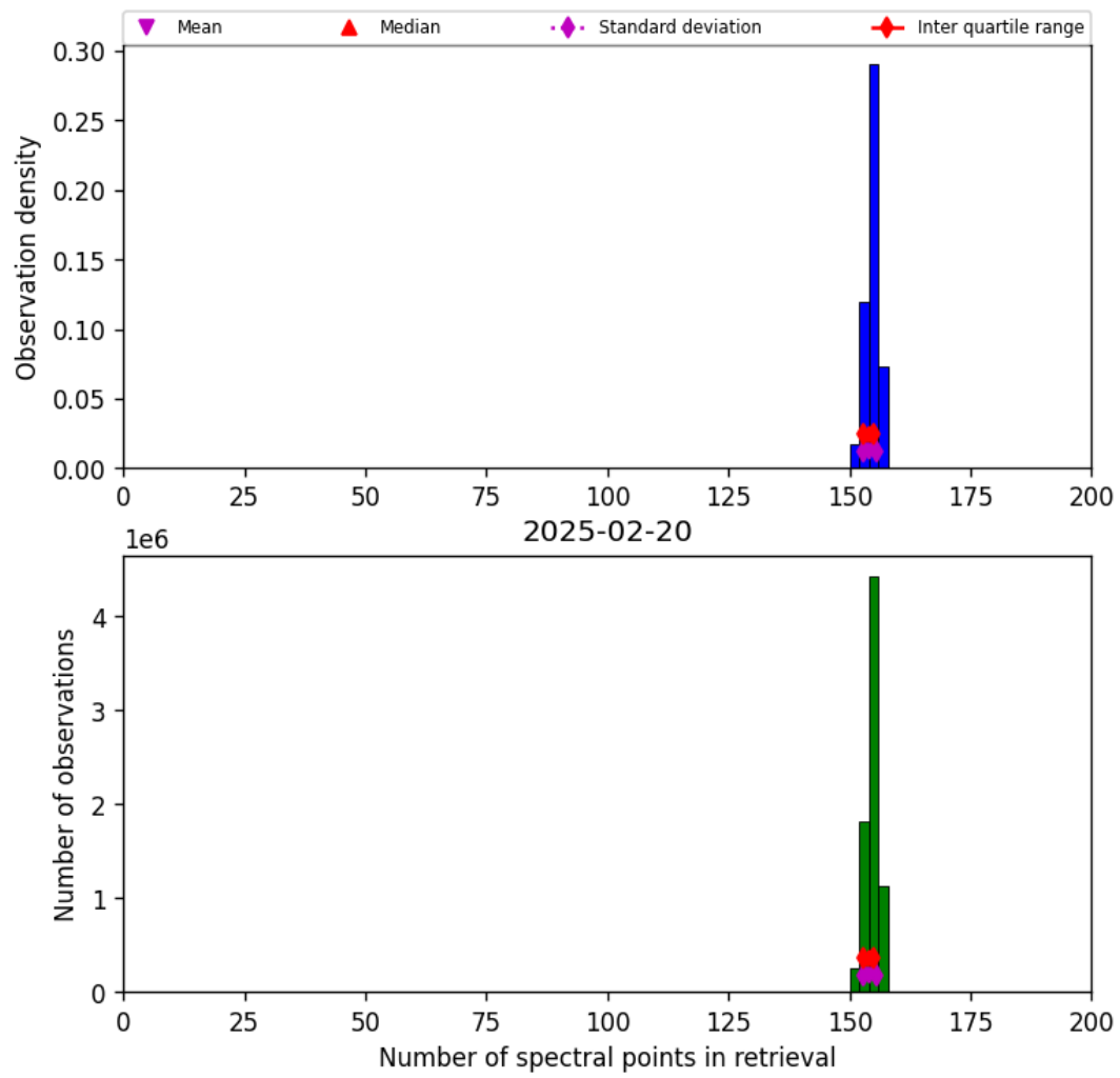
Figure 21: Histogram of “Number of spectral points in retrieval” for 2025-02-19 to 2025-02-21
