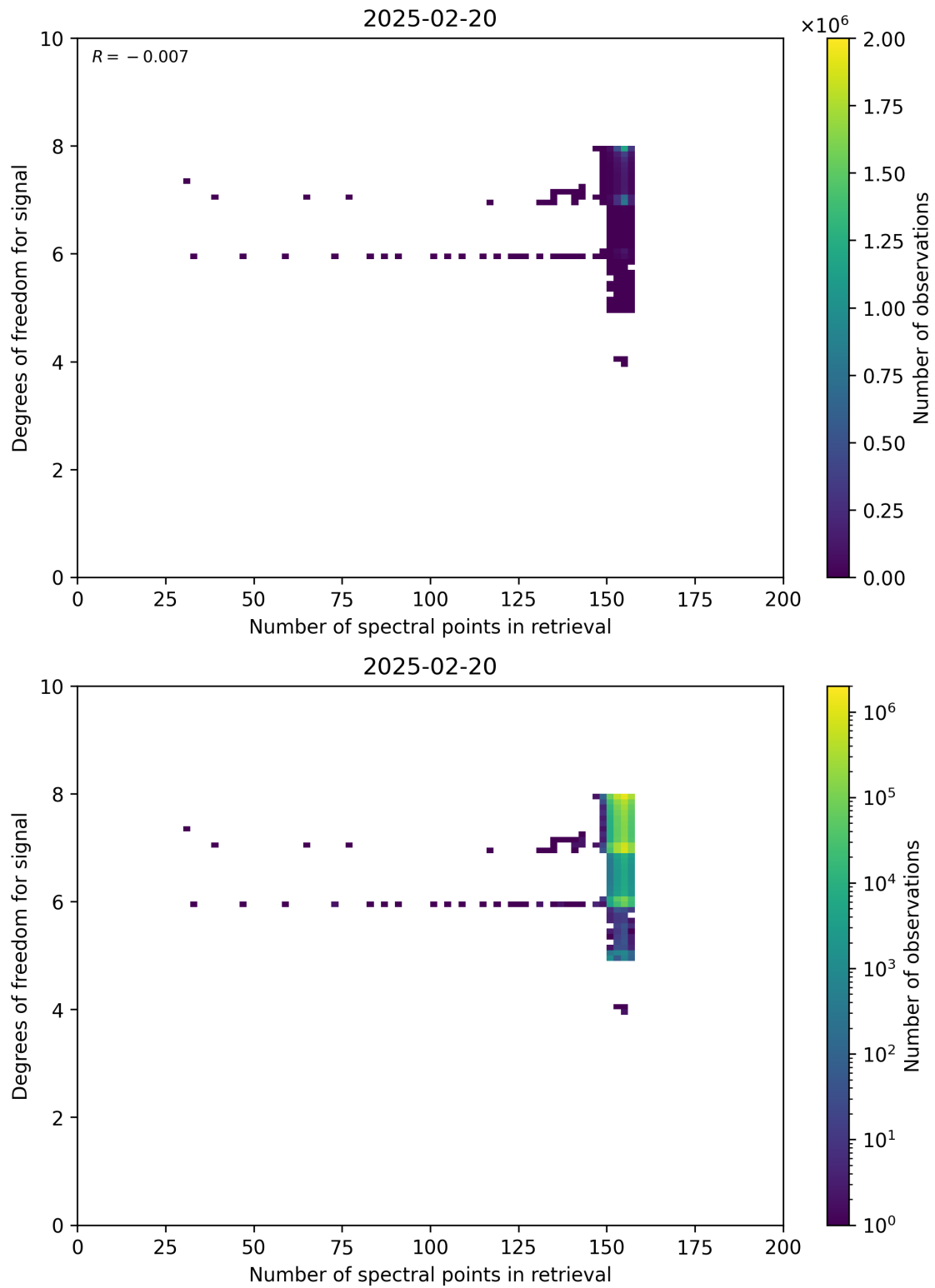
Figure 59: Scatter density plot of “Number of spectral points in retrieval” against “Degrees of freedom for signal” for 2025-02-19 to 2025-02-21.
