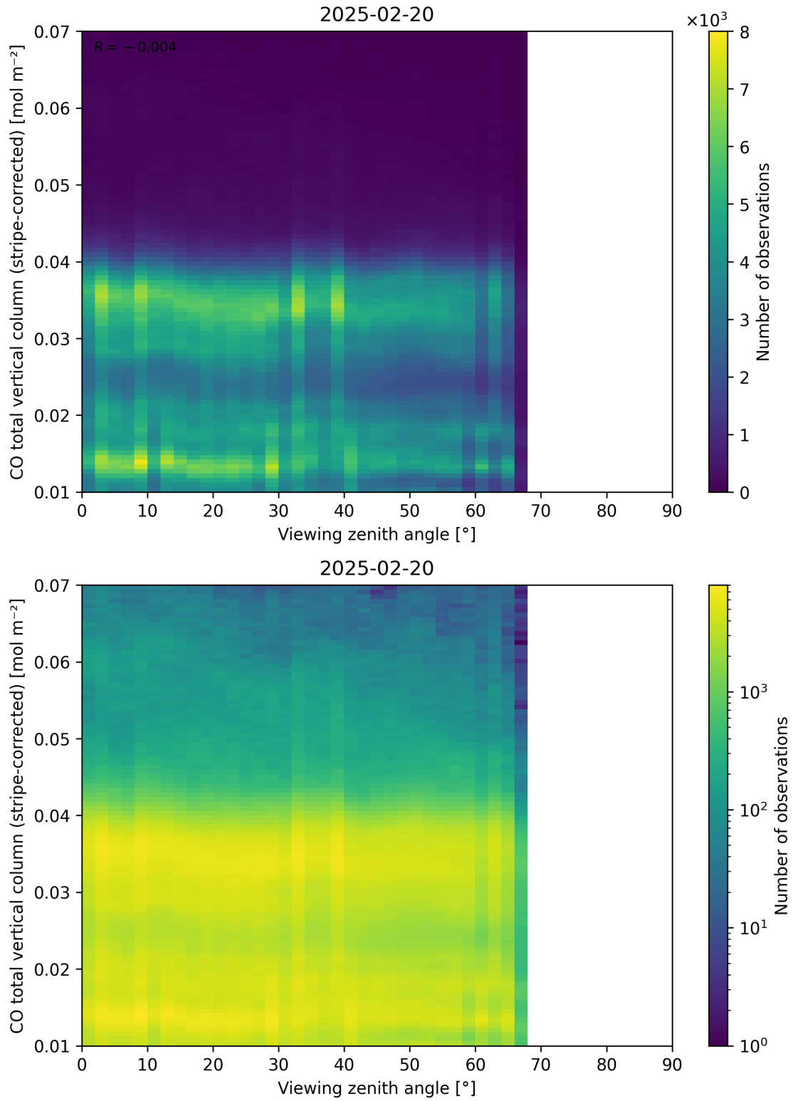
Figure 70: Scatter density plot of “Viewing zenith angle” against “CO total vertical column (stripe-corrected)” for 2025-02-19 to 2025-02-21.
