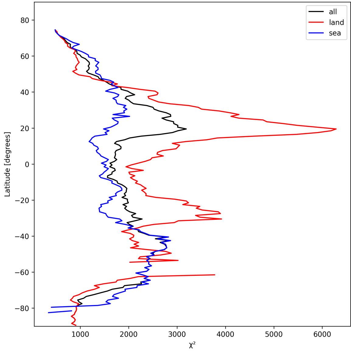
Figure 14: Zonal average of “ \chi^2 ” for 2025-02-19 to 2025-02-21.
