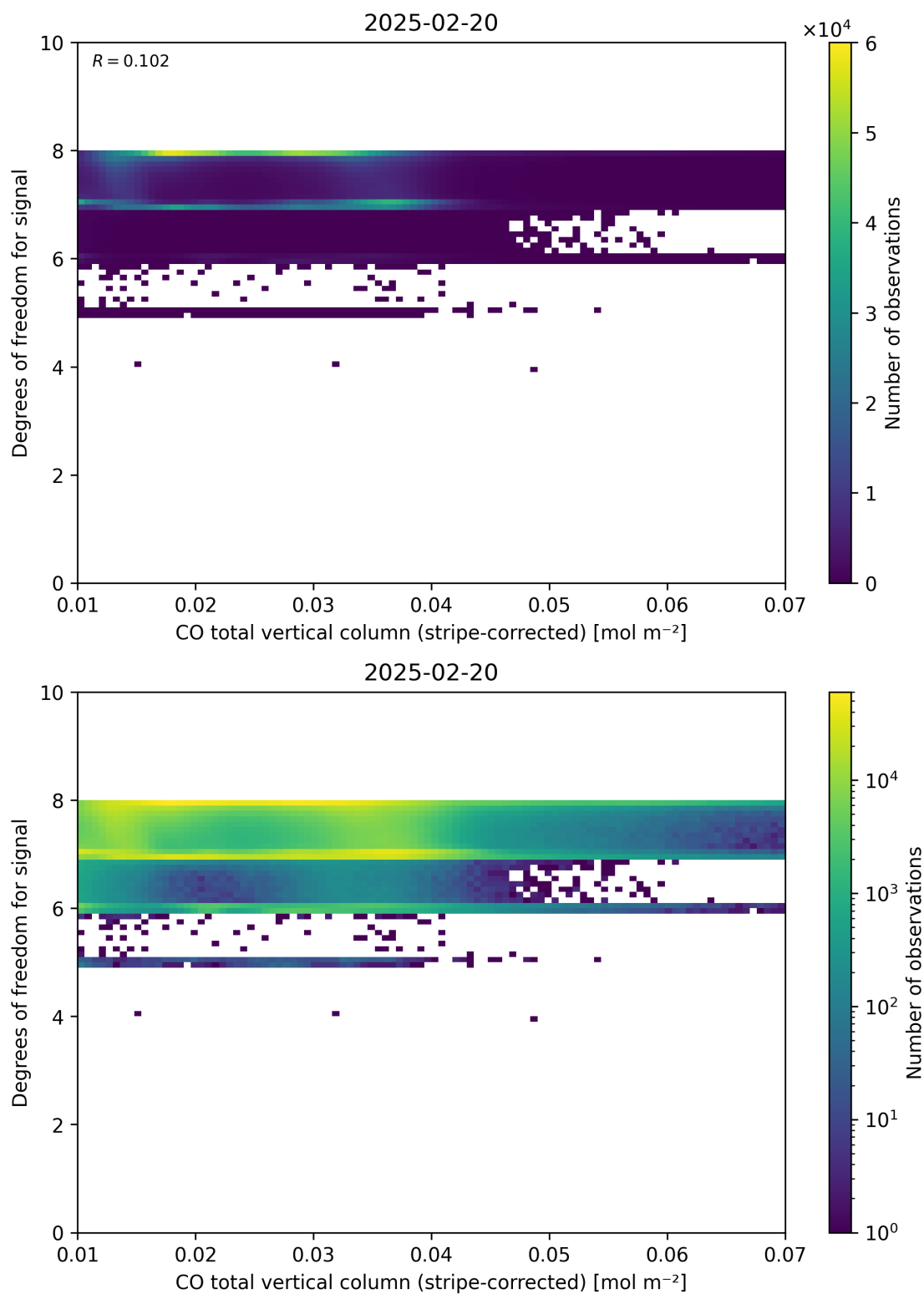
Figure 38: Scatter density plot of “CO total vertical column (stripe-corrected)” against “Degrees of freedom for signal” for 2025-02-19 to 2025-02-21.
