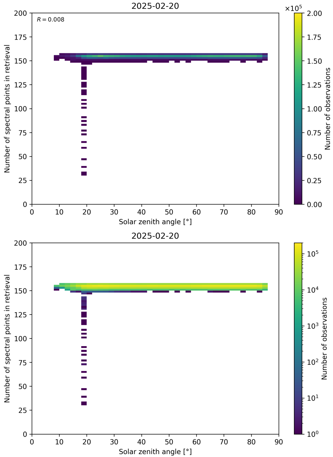
Figure 68: Scatter density plot of “Solar zenith angle” against “Number of spectral points in retrieval” for 2025-02-19 to 2025-02-21.
