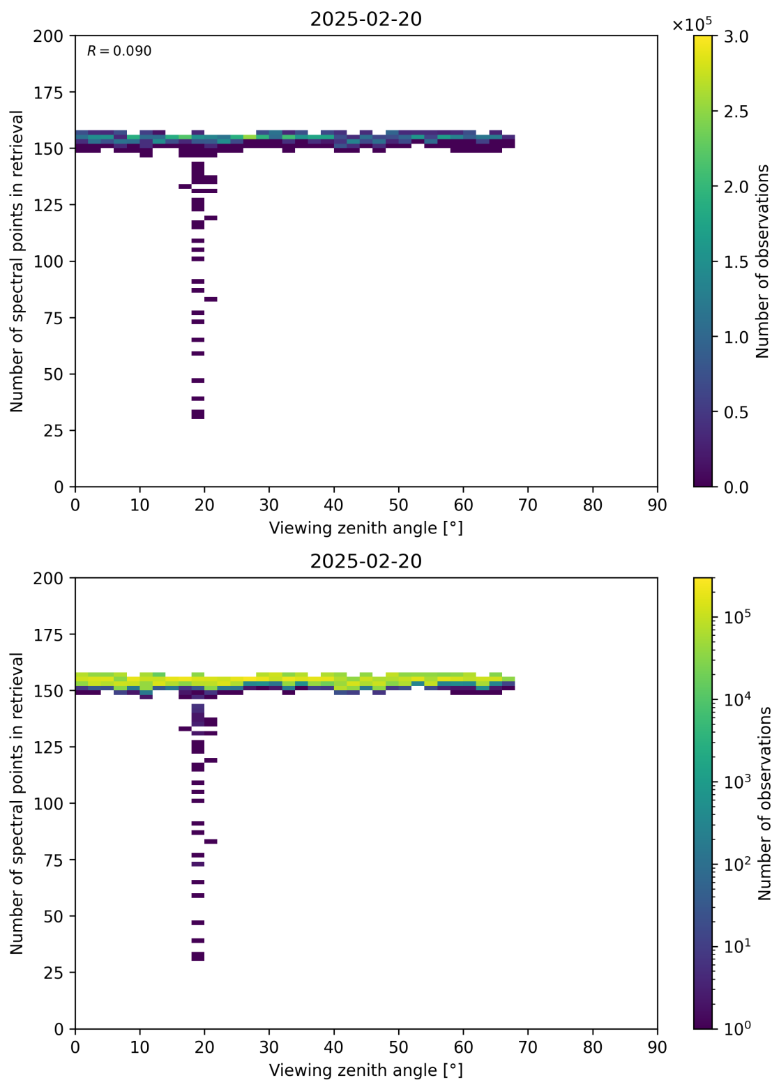
Figure 76: Scatter density plot of “Viewing zenith angle” against “Number of spectral points in retrieval” for 2025-02-19 to 2025-02-21.
