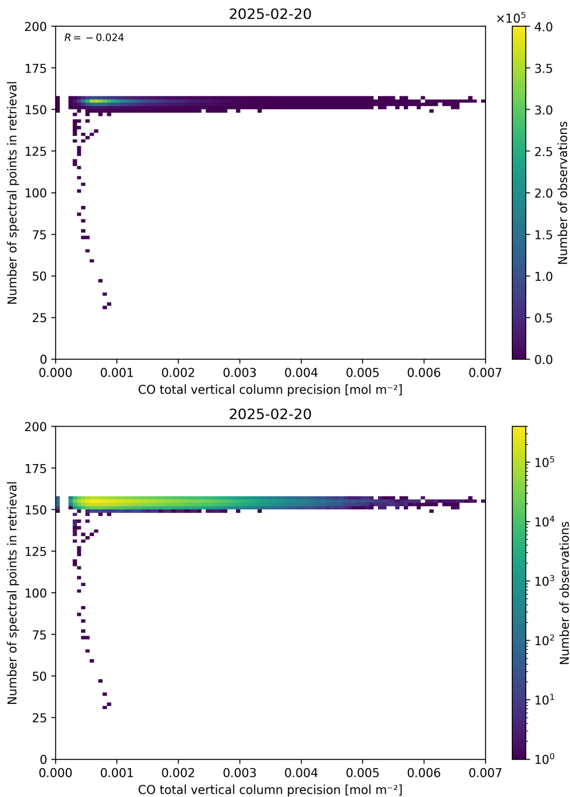
Figure 47: Scatter density plot of “CO total vertical column precision” against “Number of spectral points in retrieval” for 2025-02-19 to 2025-02-21.
