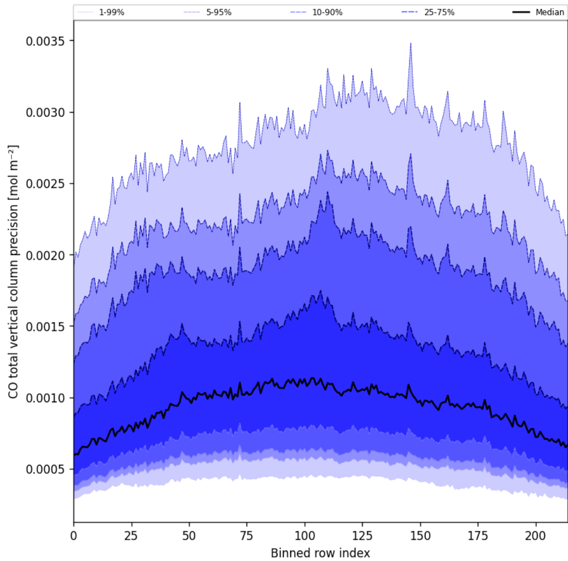
Figure 28: Along track statistics of “CO total vertical column precision” for 2025-02-19 to 2025-02-21
