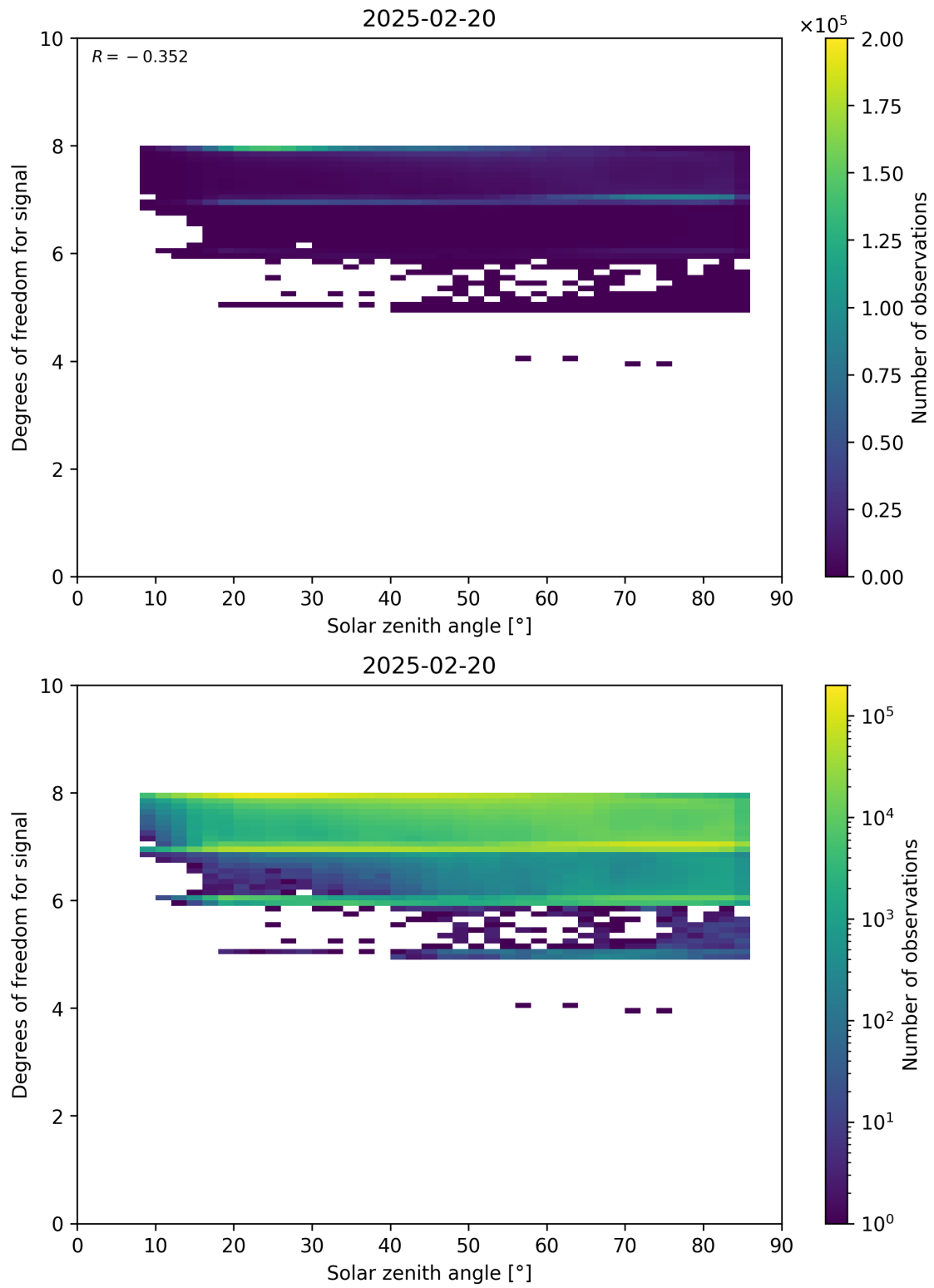
Figure 65: Scatter density plot of “Solar zenith angle” against “Degrees of freedom for signal” for 2025-02-19 to 2025-02-21.
