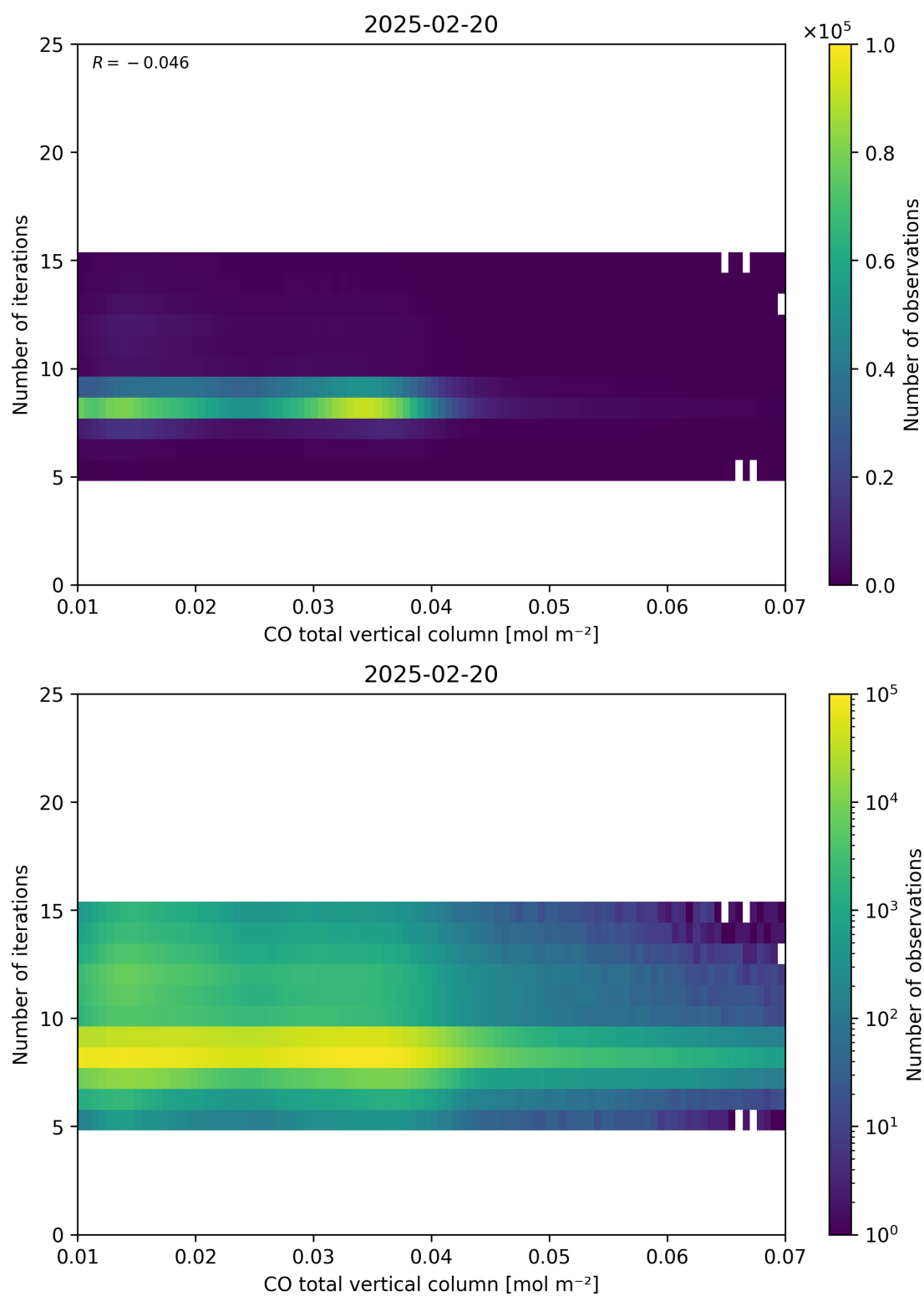
Figure 42: Scatter density plot of “CO total vertical column” against “Number of iterations” for 2025-02-19 to 2025-02-21.
