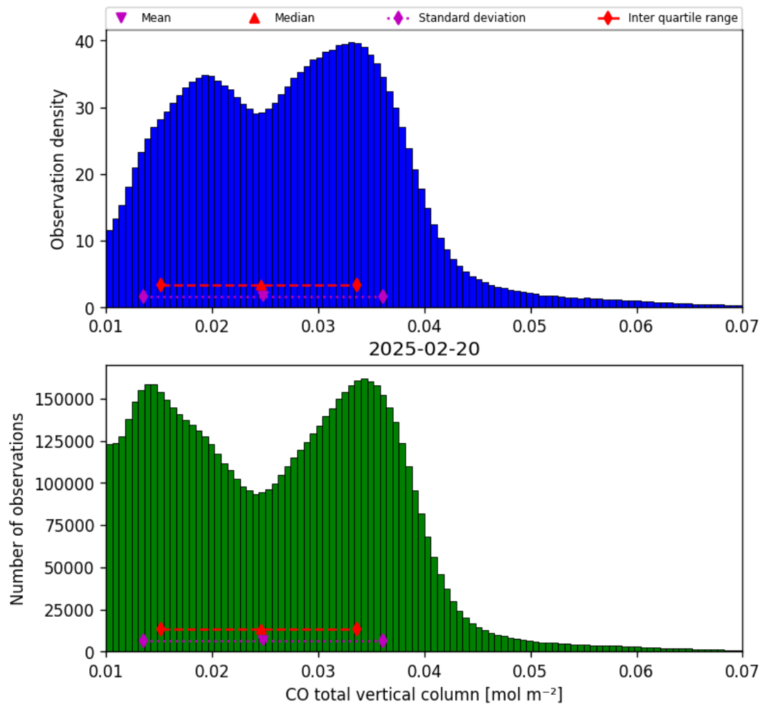
Figure 18: Histogram of “CO total vertical column” for 2025-02-19 to 2025-02-21
