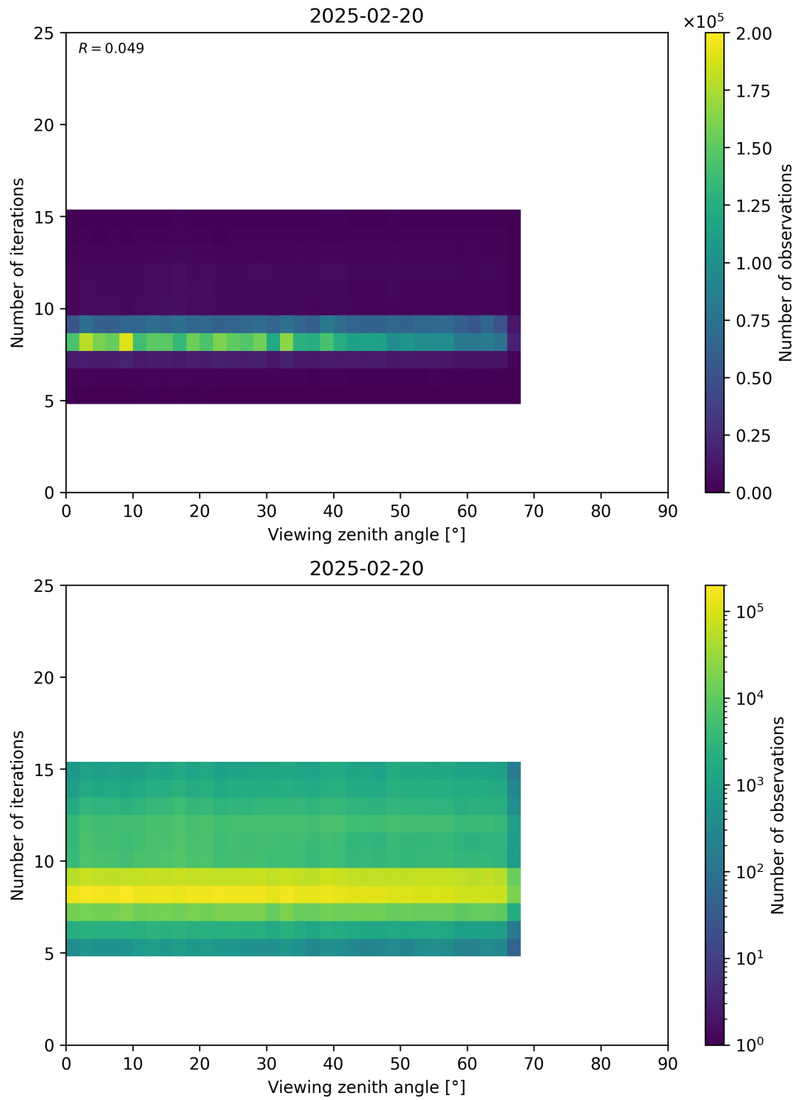
Figure 75: Scatter density plot of “Viewing zenith angle” against “Number of iterations” for 2025-02-19 to 2025-02-21.
