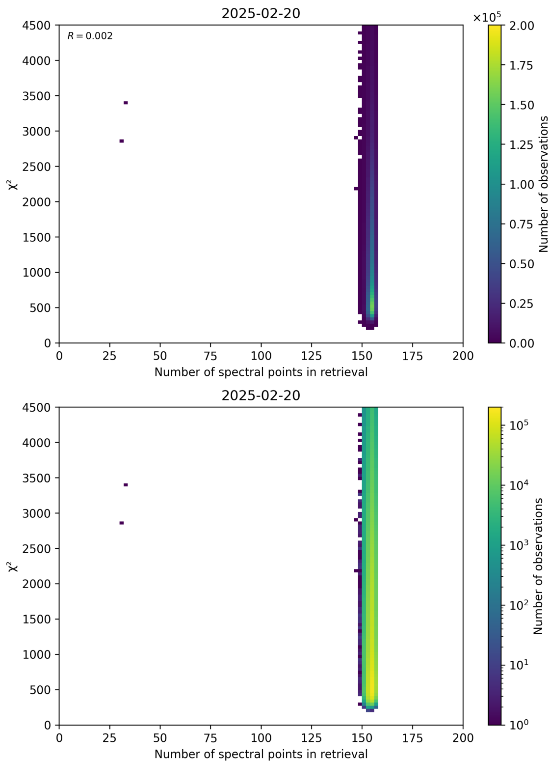
Figure 58: Scatter density plot of “Number of spectral points in retrieval” against “ \chi^2 ” for 2025-02-19 to 2025-02-21.
