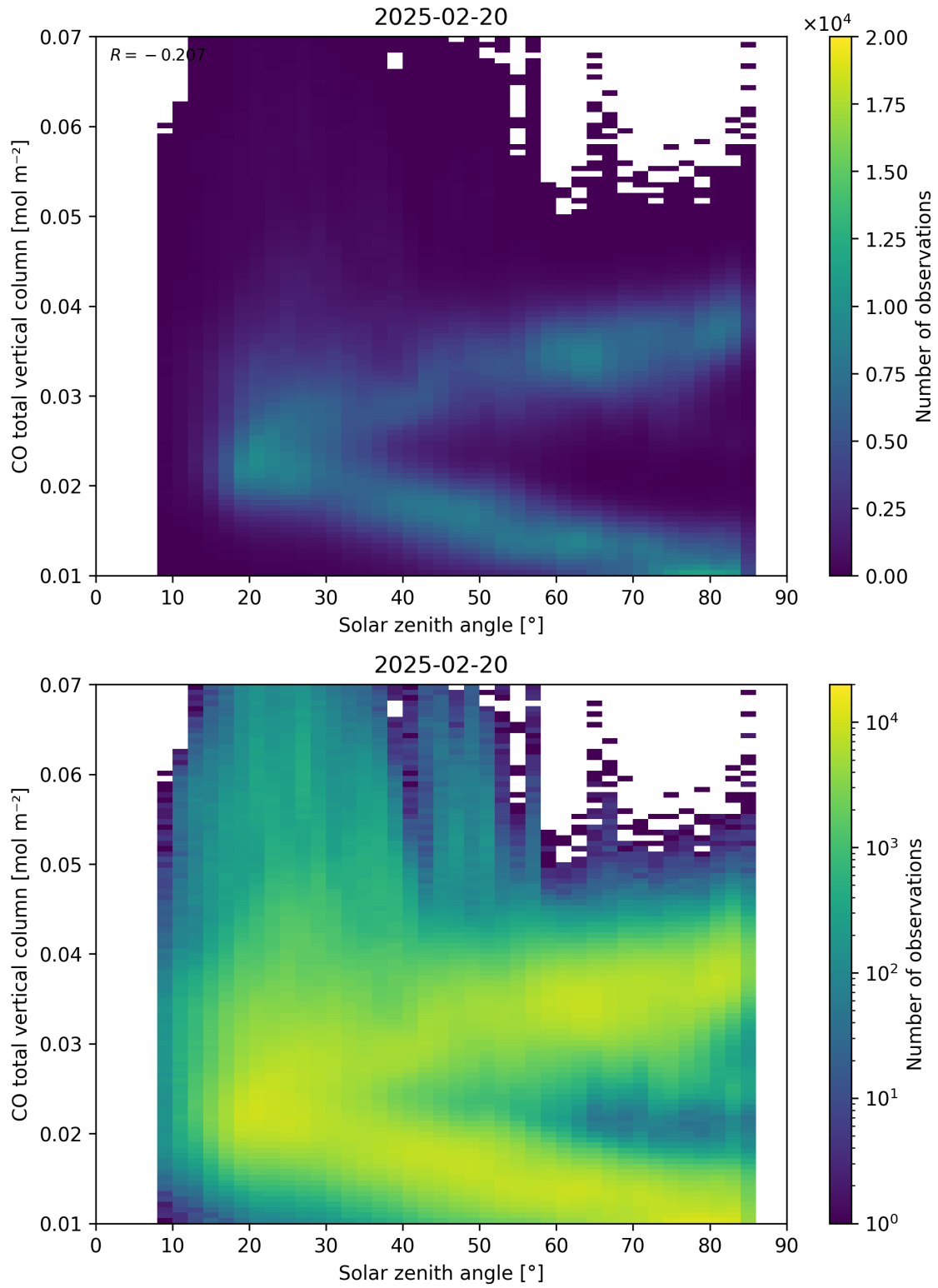
Figure 61: Scatter density plot of “Solar zenith angle” against “CO total vertical column” for 2025-02-19 to 2025-02-21.
