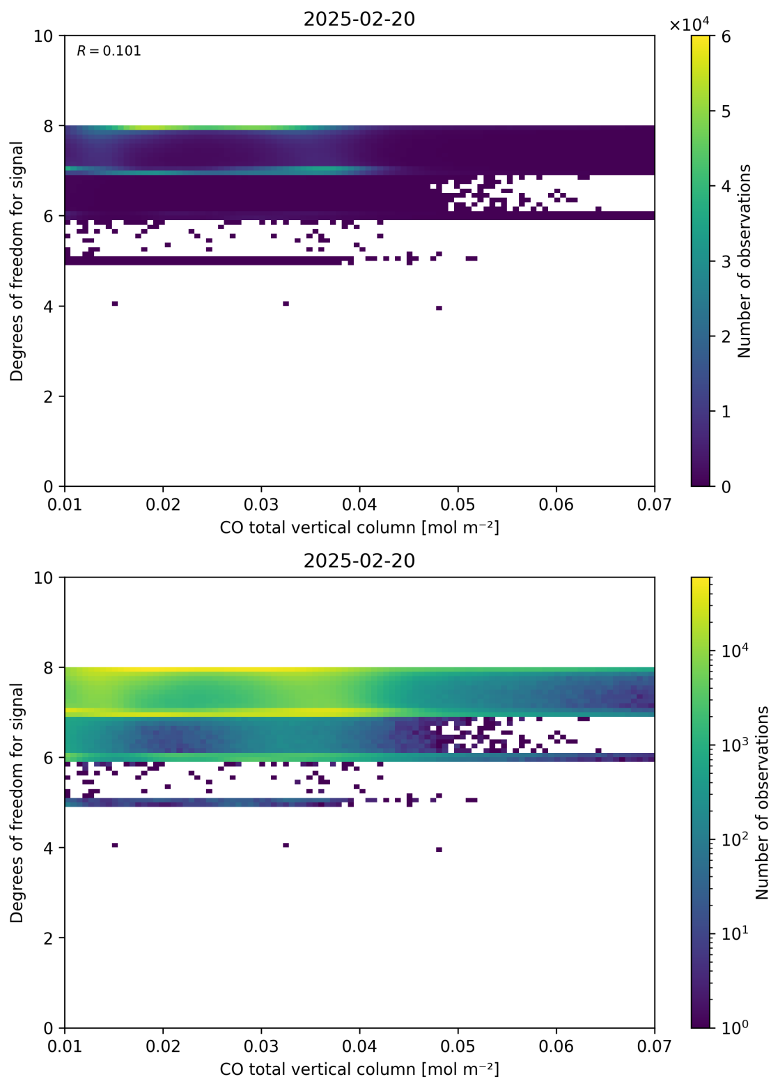
Figure 41: Scatter density plot of “CO total vertical column” against “Degrees of freedom for signal” for 2025-02-19 to 2025-02-21.
