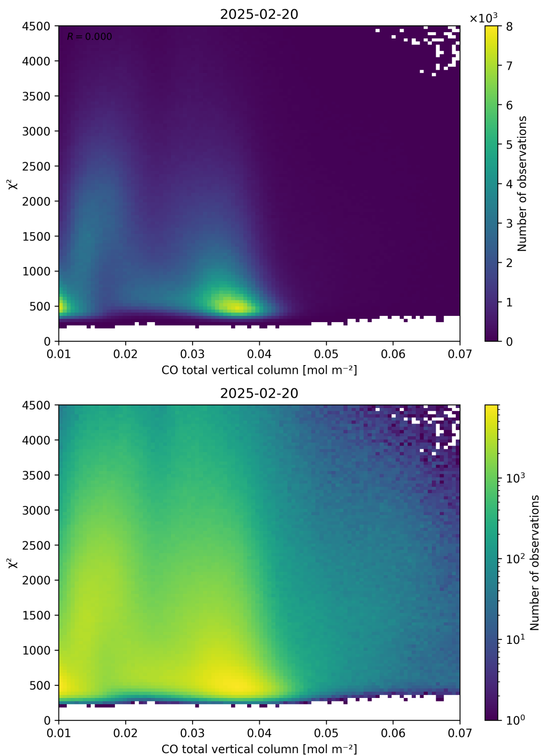
Figure 35: Scatter density plot of “CO total vertical column” against “ \chi^2 ” for 2025-02-19 to 2025-02-21.
