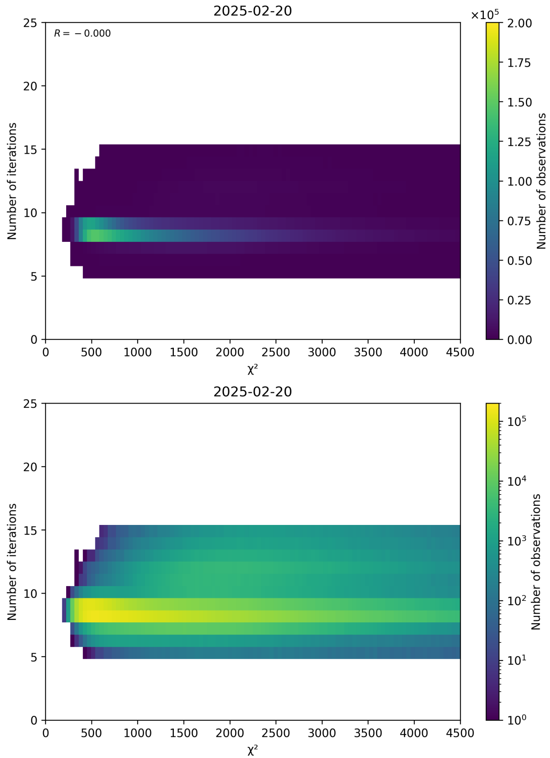
Figure 49: Scatter density plot of “ \chi^2 ” against “Number of iterations” for 2025-02-19 to 2025-02-21.
