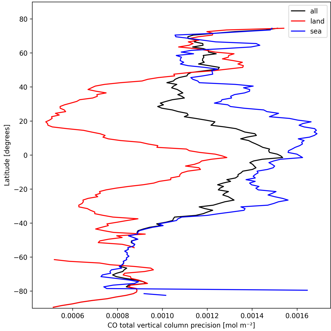
Figure 12: Zonal average of “CO total vertical column precision” for 2025-02-19 to 2025-02-21.
