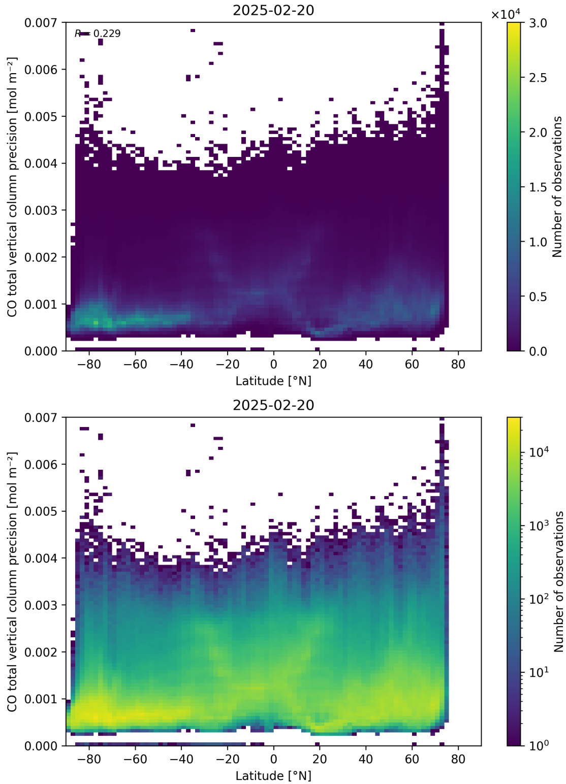
Figure 53: Scatter density plot of “Latitude” against “CO total vertical column precision” for 2025-02-19 to 2025-02-21.
