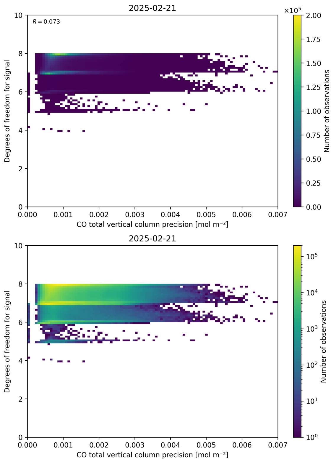
Figure 45: Scatter density plot of “CO total vertical column precision” against “Degrees of freedom for signal” for 2025-02-20 to 2025-02-22.
