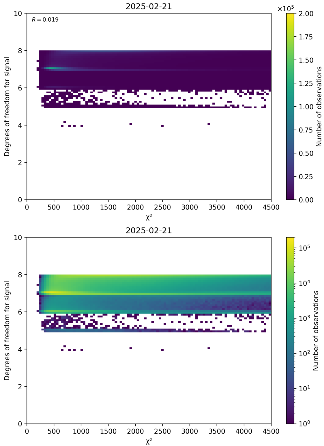
Figure 48: Scatter density plot of “ \chi^2 ” against “Degrees of freedom for signal” for 2025-02-20 to 2025-02-22.
