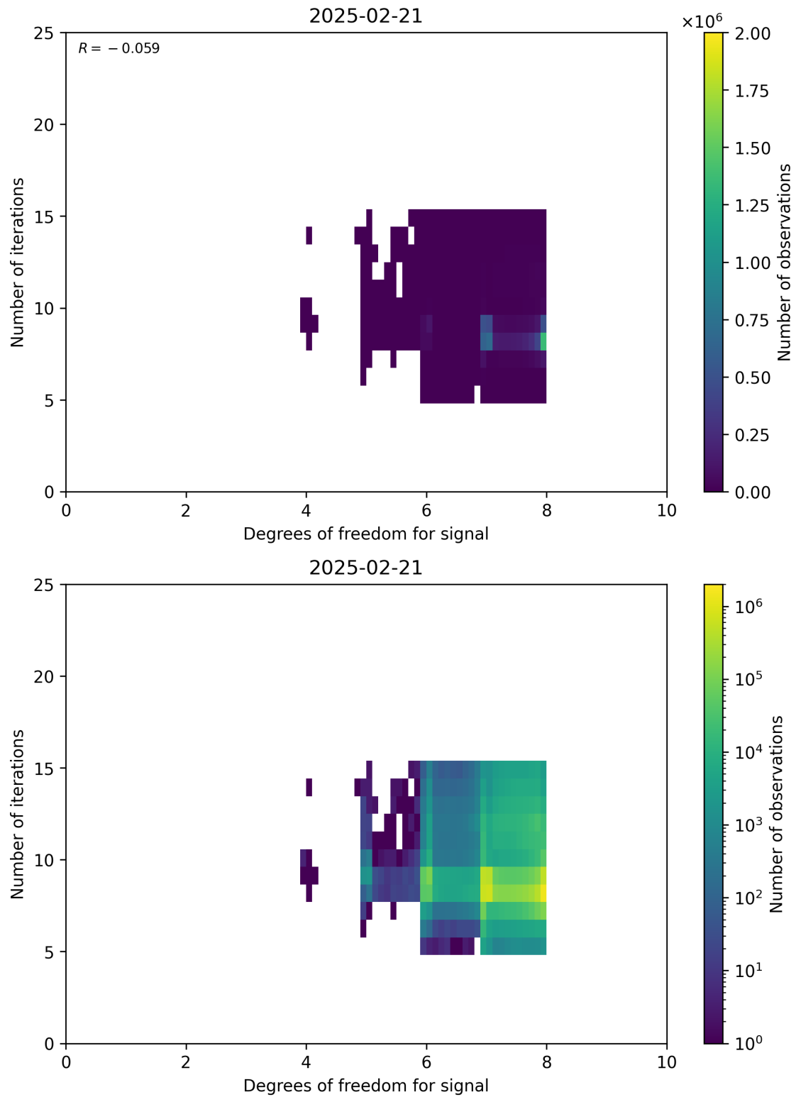
Figure 50: Scatter density plot of “Degrees of freedom for signal” against “Number of iterations” for 2025-02-20 to 2025-02-22.
