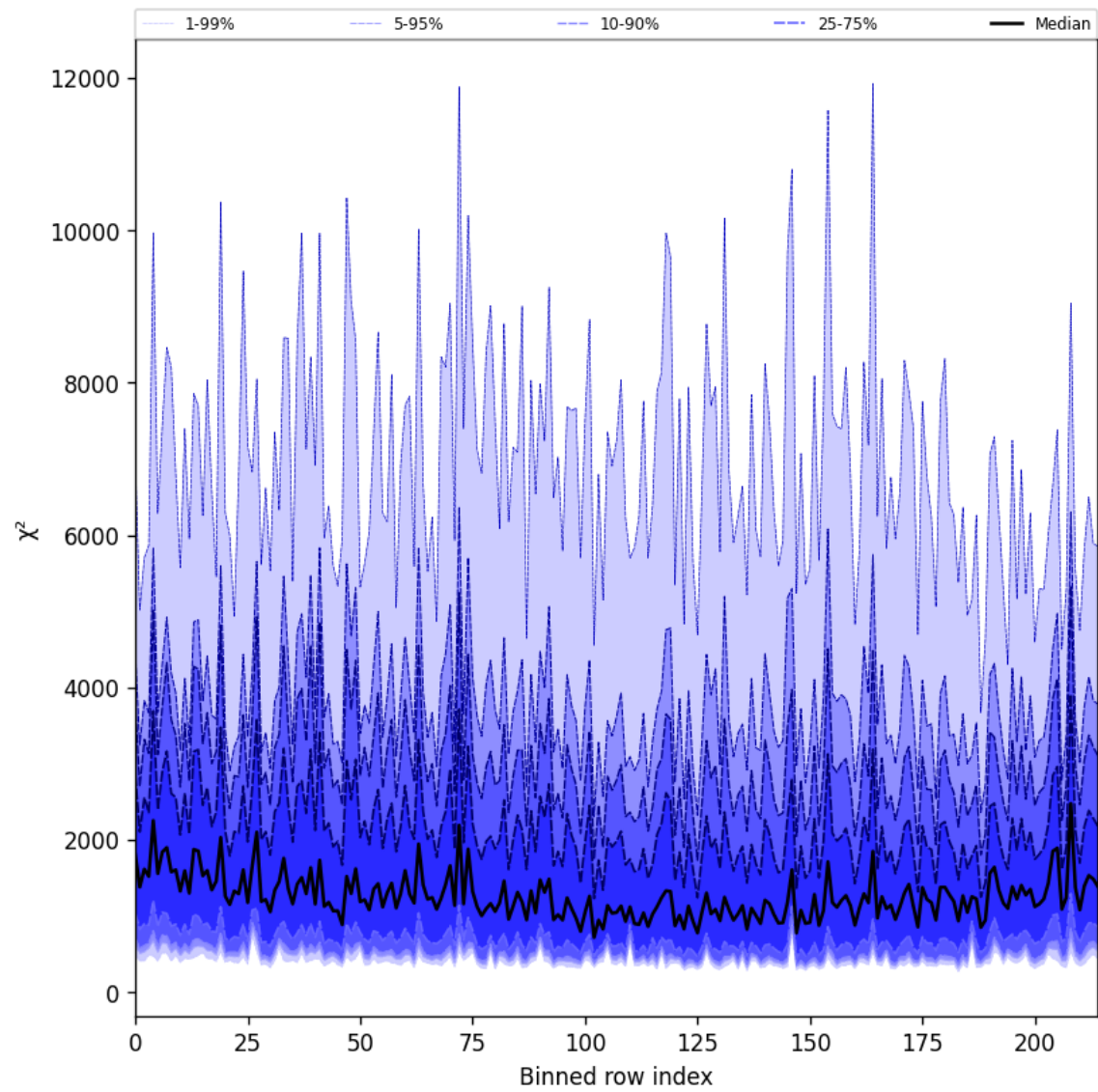
Figure 30: Along track statistics of “ \chi^2 ” for 2025-02-20 to 2025-02-22
