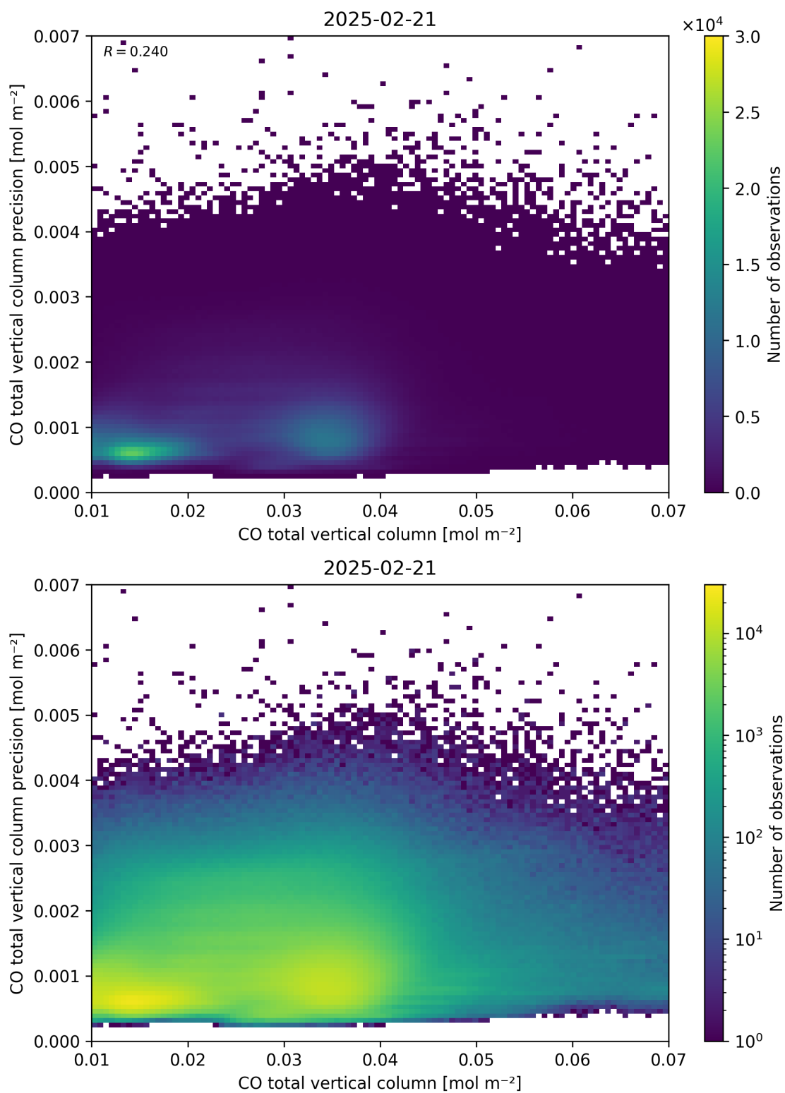
Figure 34: Scatter density plot of “CO total vertical column” against “CO total vertical column precision” for 2025-02-20 to 2025-02-22.
