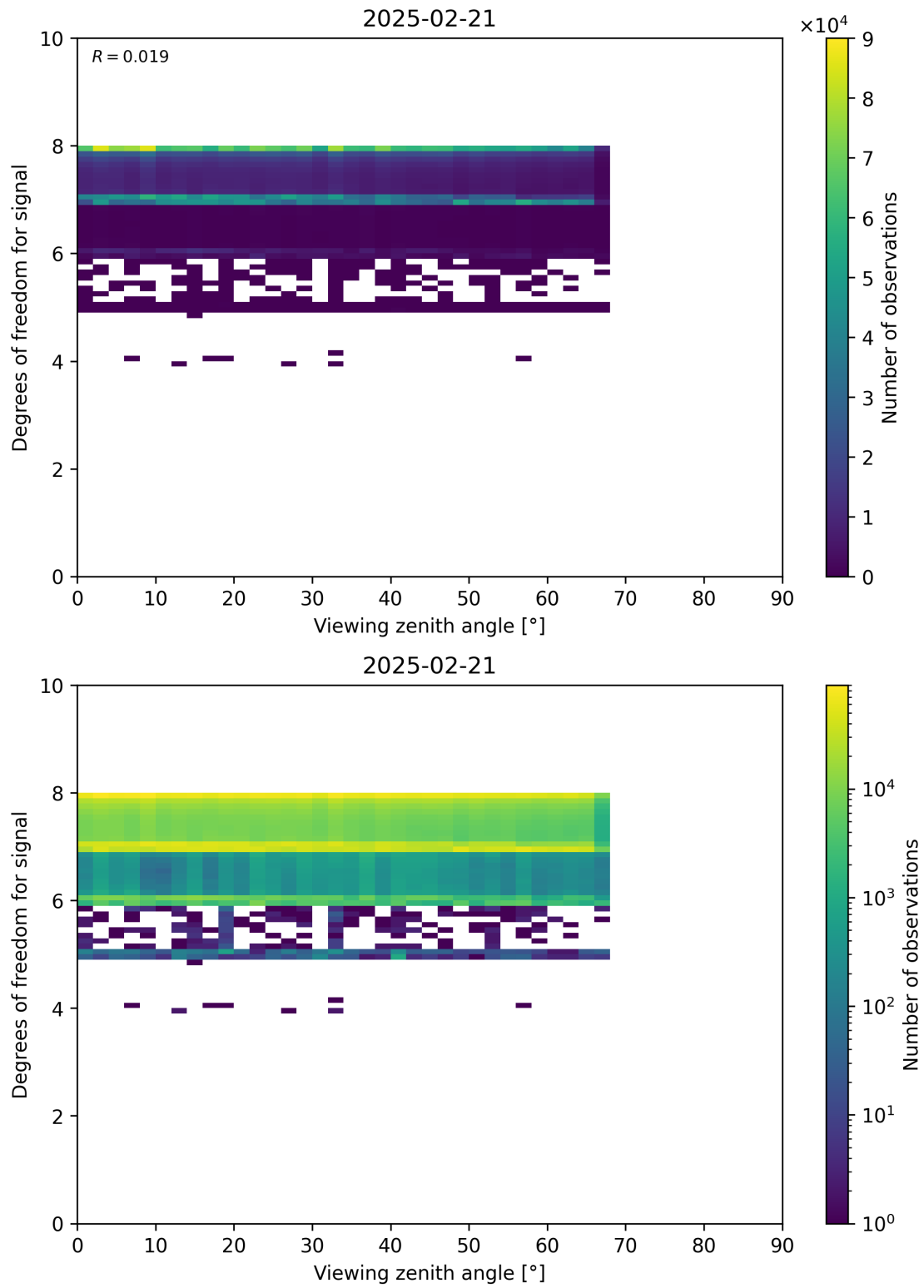
Figure 73: Scatter density plot of “Viewing zenith angle” against “Degrees of freedom for signal” for 2025-02-20 to 2025-02-22.
