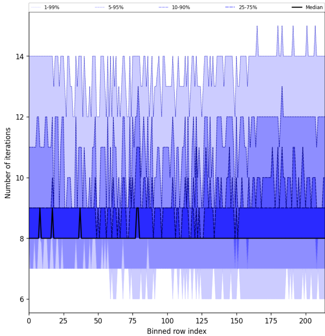
Figure 32: Along track statistics of “Number of iterations” for 2025-02-20 to 2025-02-22
