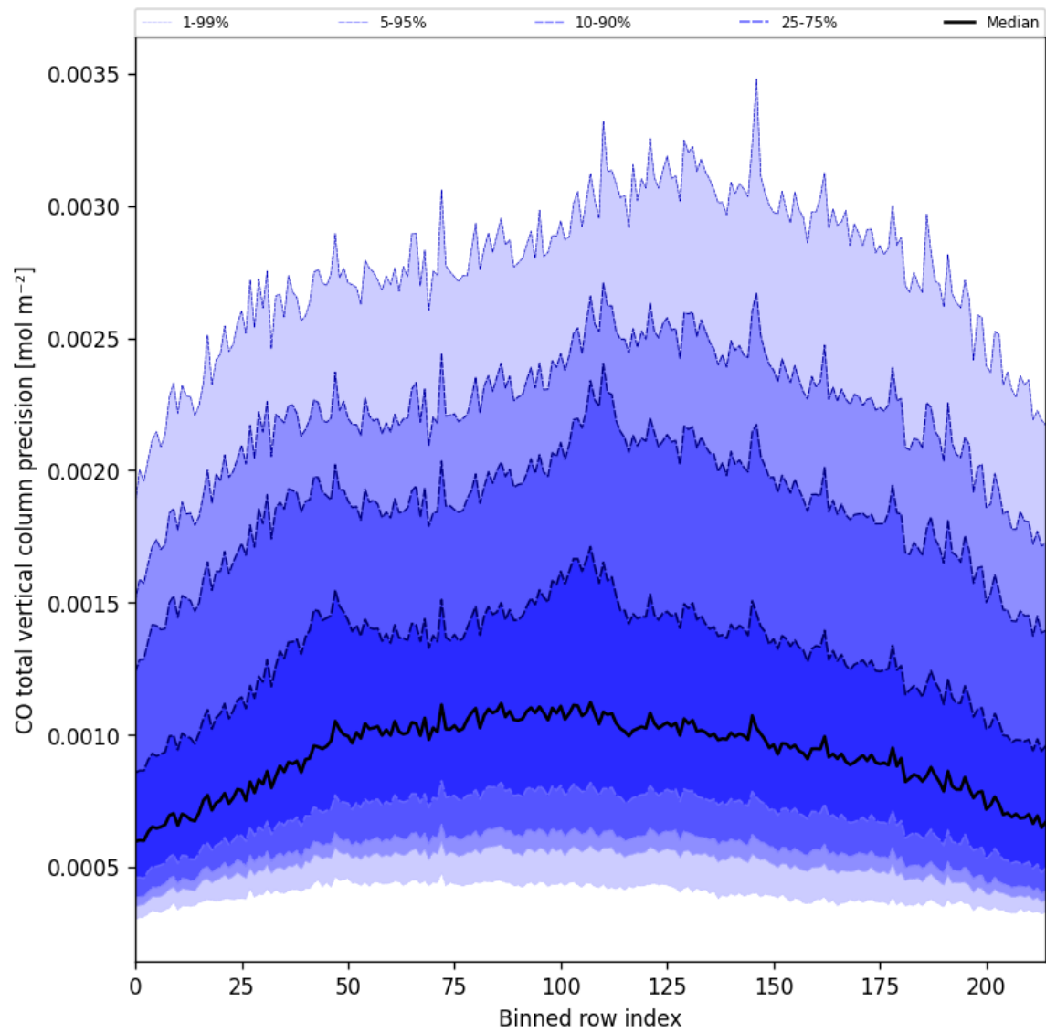
Figure 28: Along track statistics of “CO total vertical column precision” for 2025-02-20 to 2025-02-22
