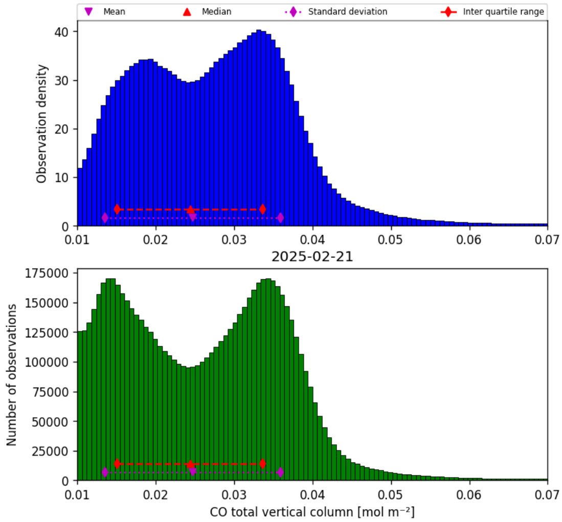
Figure 18: Histogram of “CO total vertical column” for 2025-02-20 to 2025-02-22
