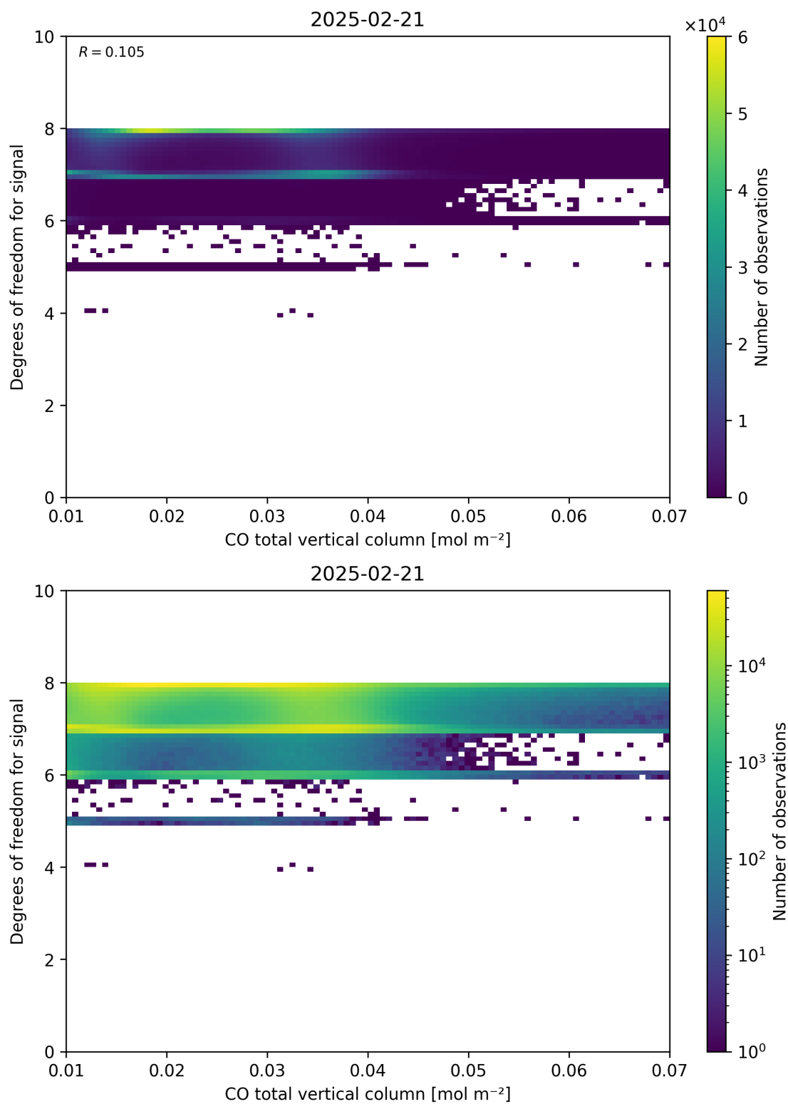
Figure 41: Scatter density plot of “CO total vertical column” against “Degrees of freedom for signal” for 2025-02-20 to 2025-02-22.
