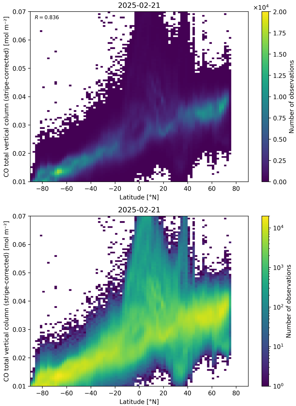
Figure 52: Scatter density plot of “Latitude” against “CO total vertical column (stripe-corrected)” for 2025-02-20 to 2025-02-22.
