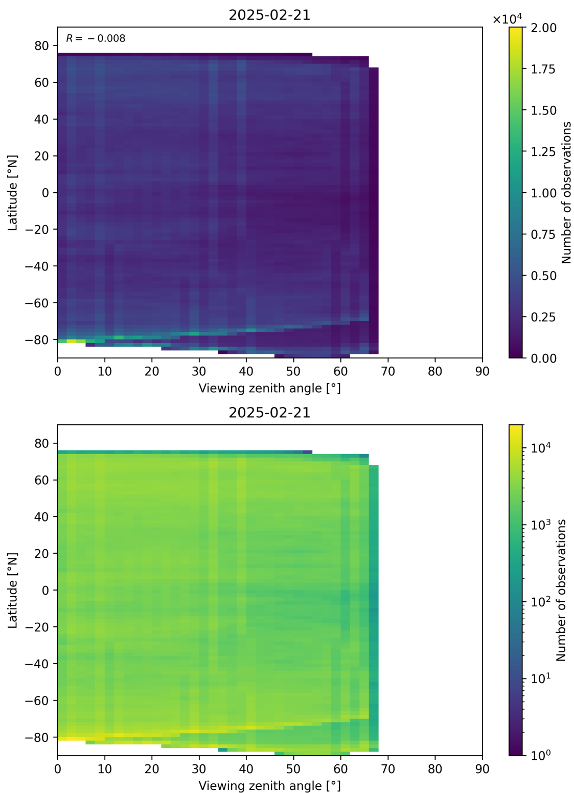
Figure 74: Scatter density plot of “Viewing zenith angle” against “Latitude” for 2025-02-20 to 2025-02-22.
