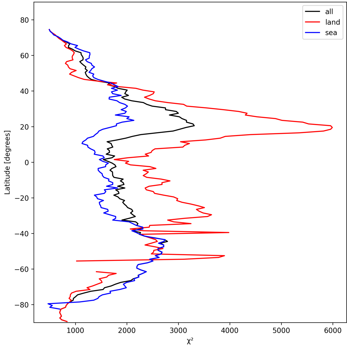
Figure 14: Zonal average of “ \chi^2 ” for 2025-02-20 to 2025-02-22.
