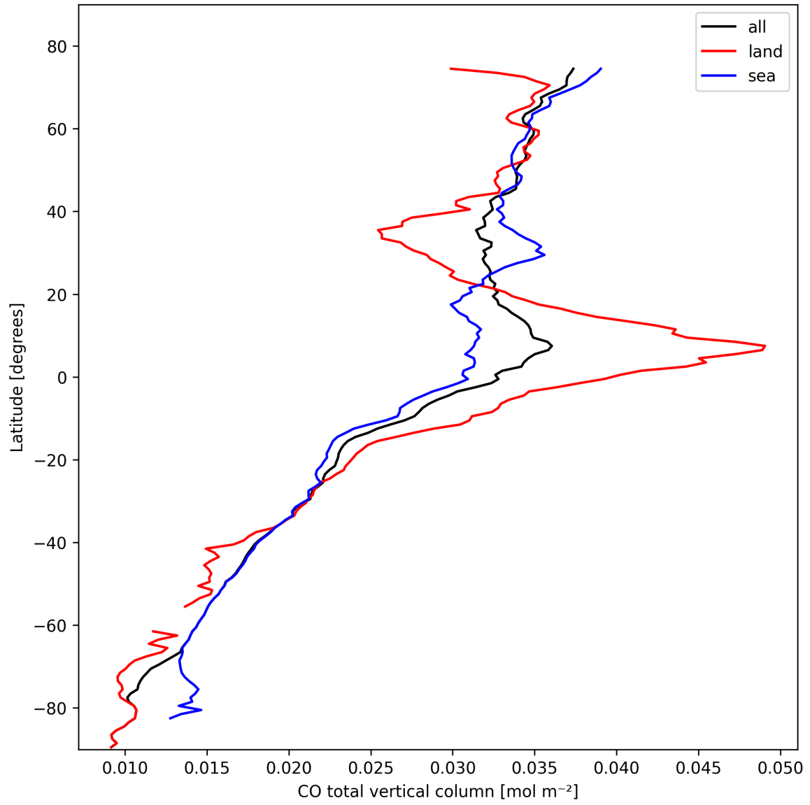
Figure 10: Zonal average of “CO total vertical column” for 2025-02-20 to 2025-02-22.
