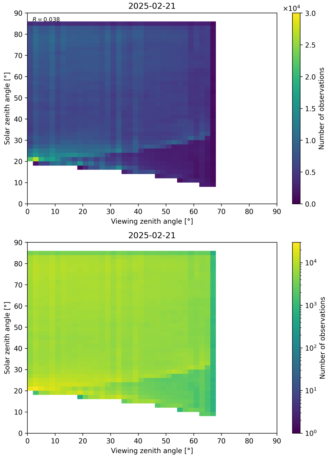
Figure 77: Scatter density plot of “Viewing zenith angle” against “Solar zenith angle” for 2025-02-20 to 2025-02-22.
