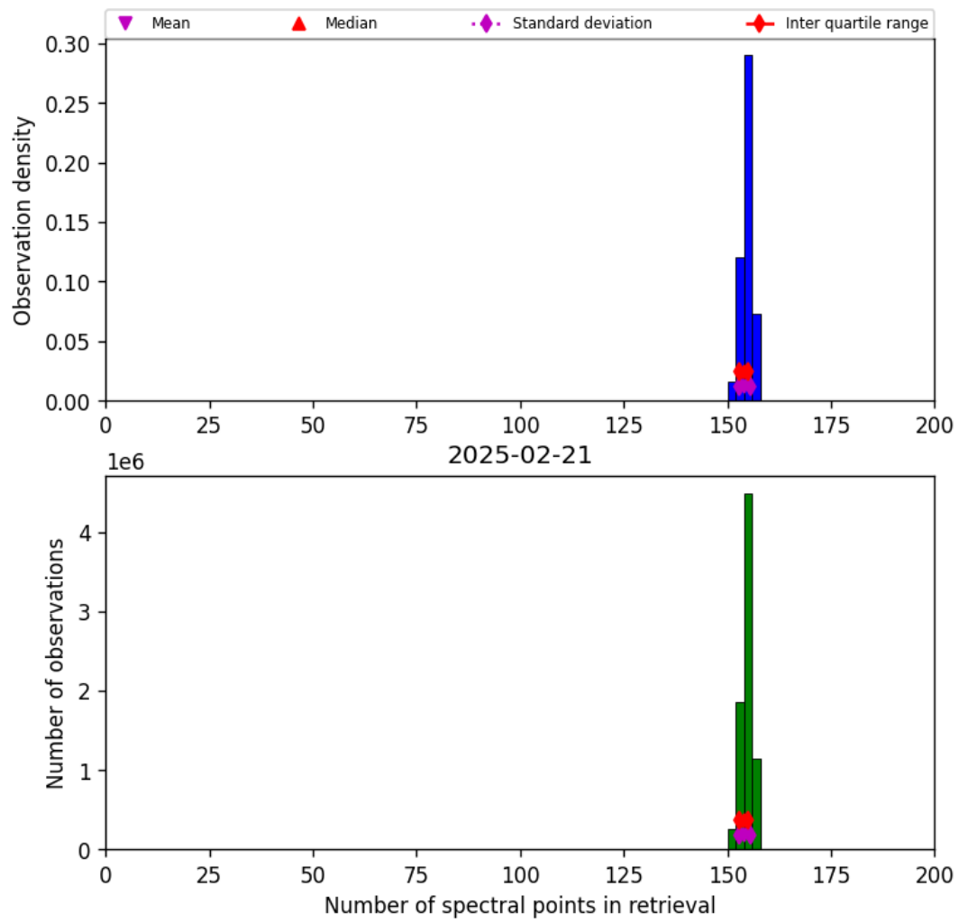
Figure 21: Histogram of “Number of spectral points in retrieval” for 2025-02-20 to 2025-02-22
