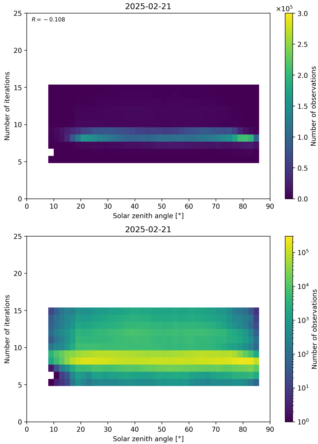
Figure 67: Scatter density plot of “Solar zenith angle” against “Number of iterations” for 2025-02-20 to 2025-02-22.
