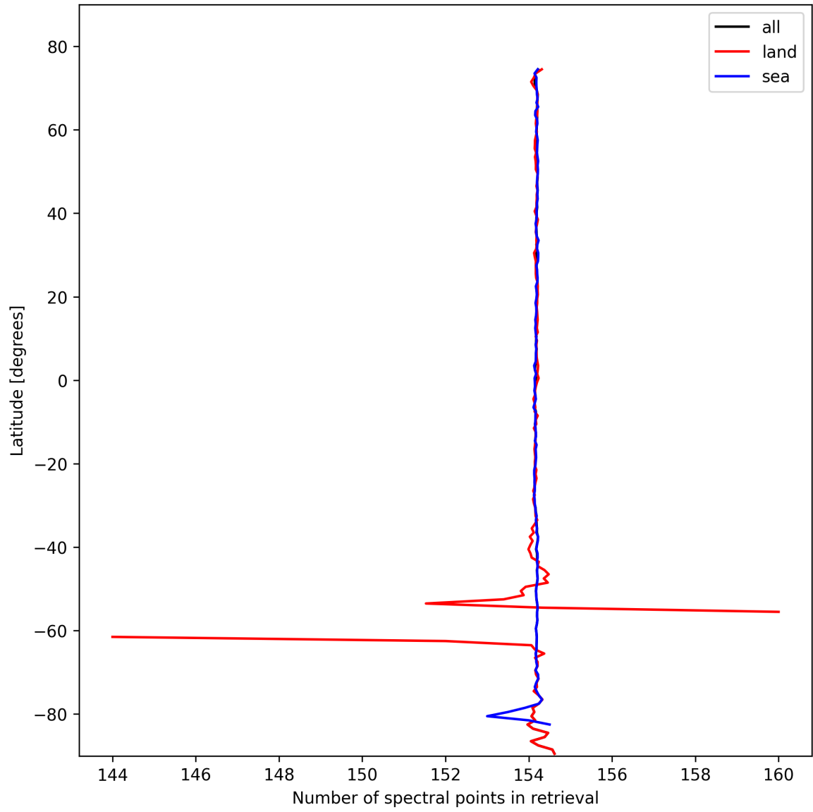
Figure 13: Zonal average of “Number of spectral points in retrieval” for 2025-02-20 to 2025-02-22.
