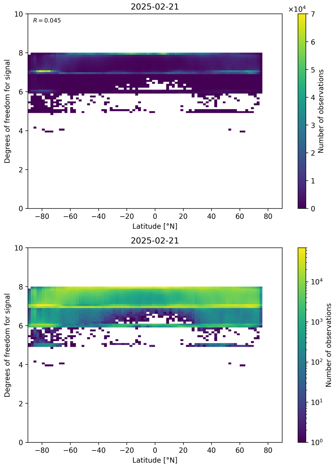
Figure 55: Scatter density plot of “Latitude” against “Degrees of freedom for signal” for 2025-02-20 to 2025-02-22.
