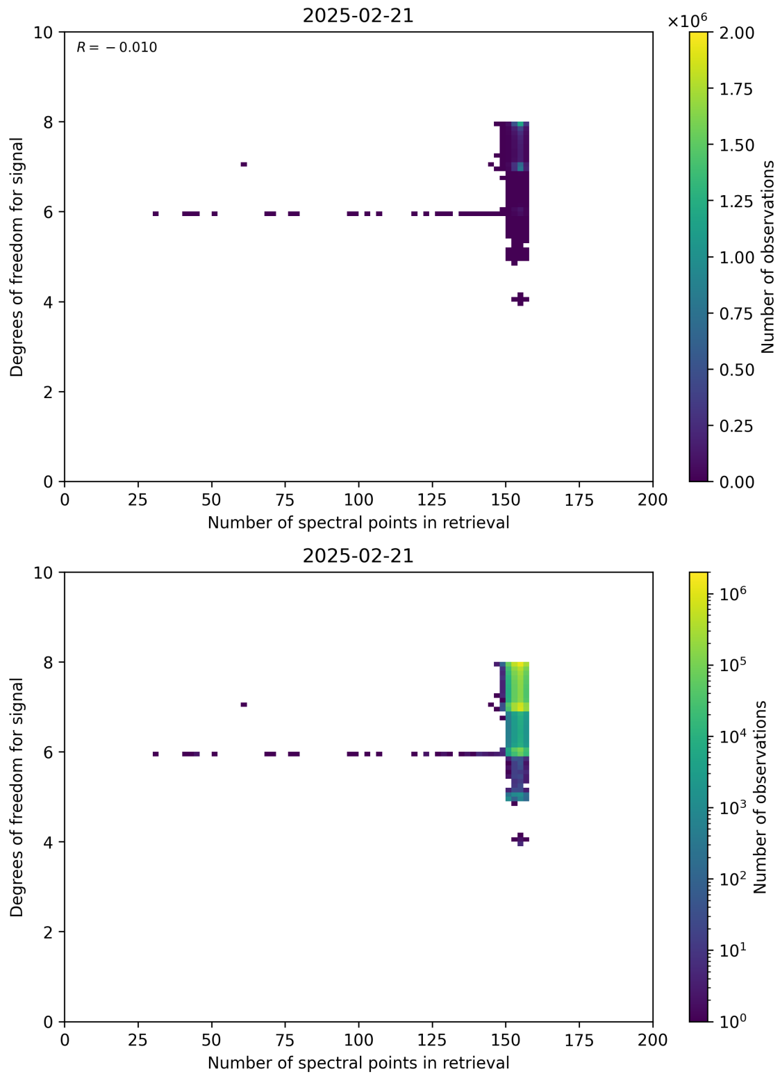
Figure 59: Scatter density plot of “Number of spectral points in retrieval” against “Degrees of freedom for signal” for 2025-02-20 to 2025-02-22.
