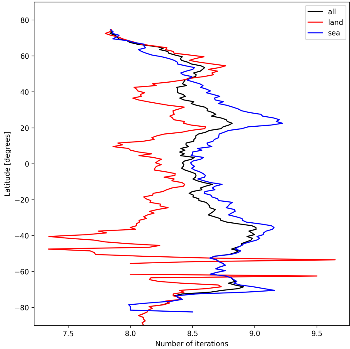
Figure 16: Zonal average of “Number of iterations” for 2025-02-20 to 2025-02-22.
