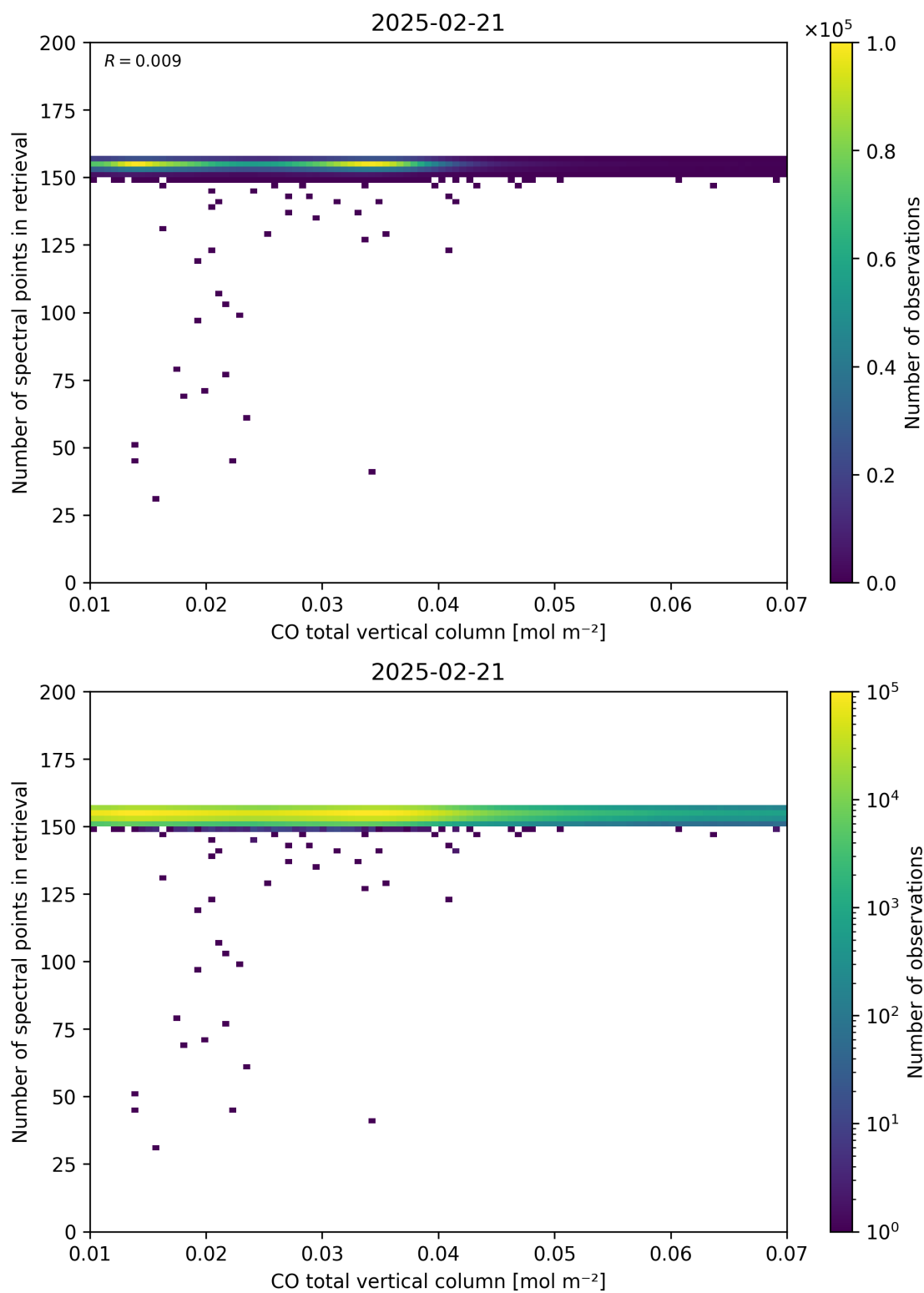
Figure 43: Scatter density plot of “CO total vertical column” against “Number of spectral points in retrieval” for 2025-02-20 to 2025-02-22.
