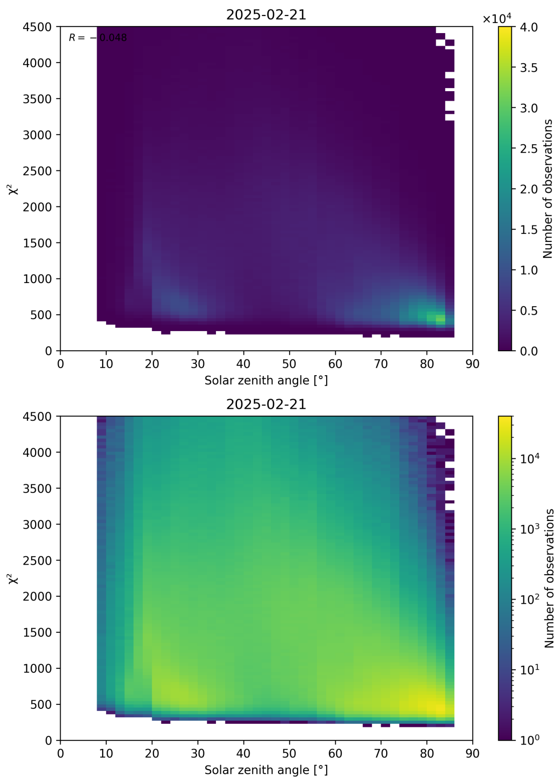
Figure 64: Scatter density plot of “Solar zenith angle” against “ \chi^2 ” for 2025-02-20 to 2025-02-22.
