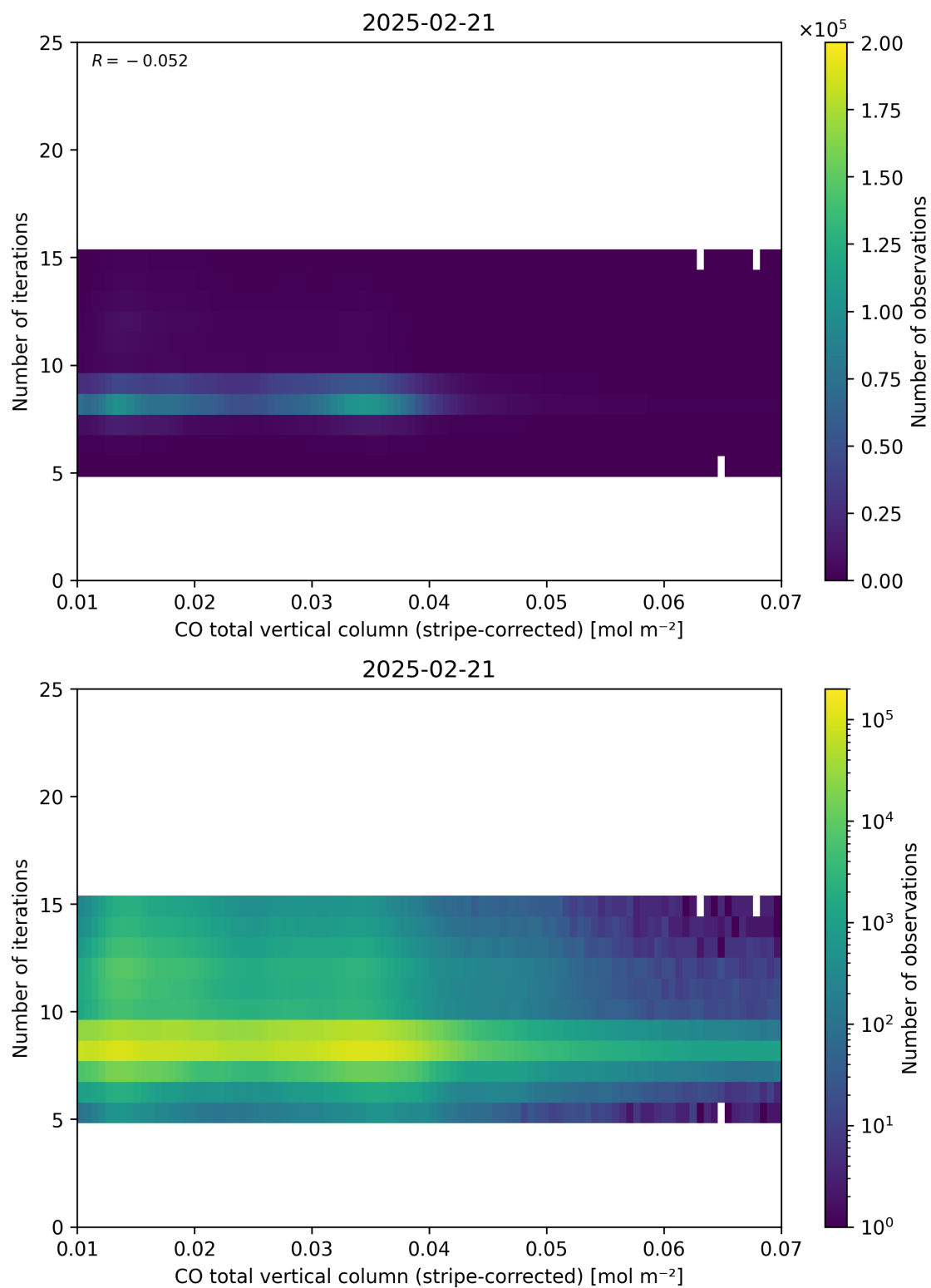
Figure 39: Scatter density plot of “CO total vertical column (stripe-corrected)” against “Number of iterations” for 2025-02-20 to 2025-02-22.
