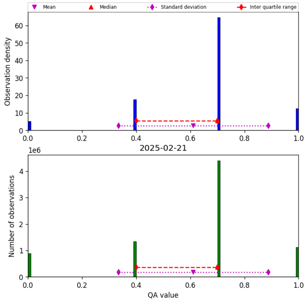
Figure 17: Histogram of “QA value” for 2025-02-20 to 2025-02-22
