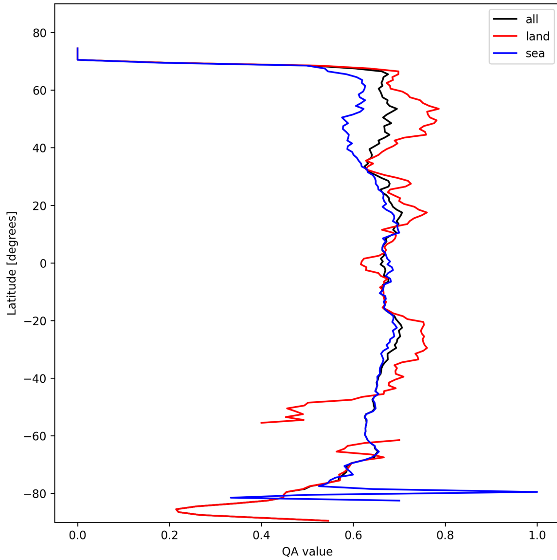
Figure 9: Zonal average of “QA value” for 2025-02-20 to 2025-02-22.
