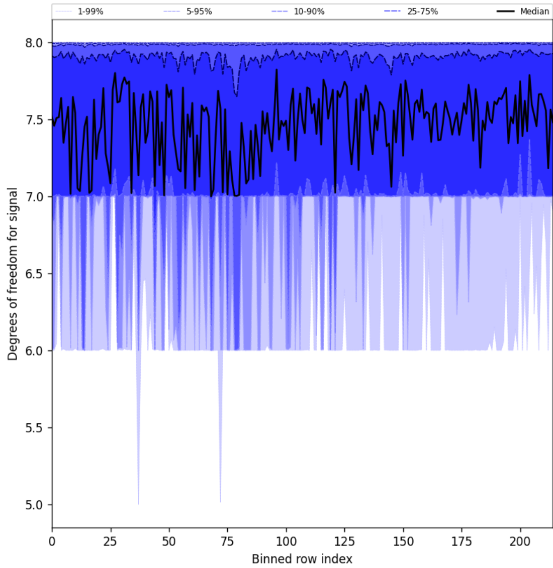
Figure 31: Along track statistics of “Degrees of freedom for signal” for 2025-02-20 to 2025-02-22
