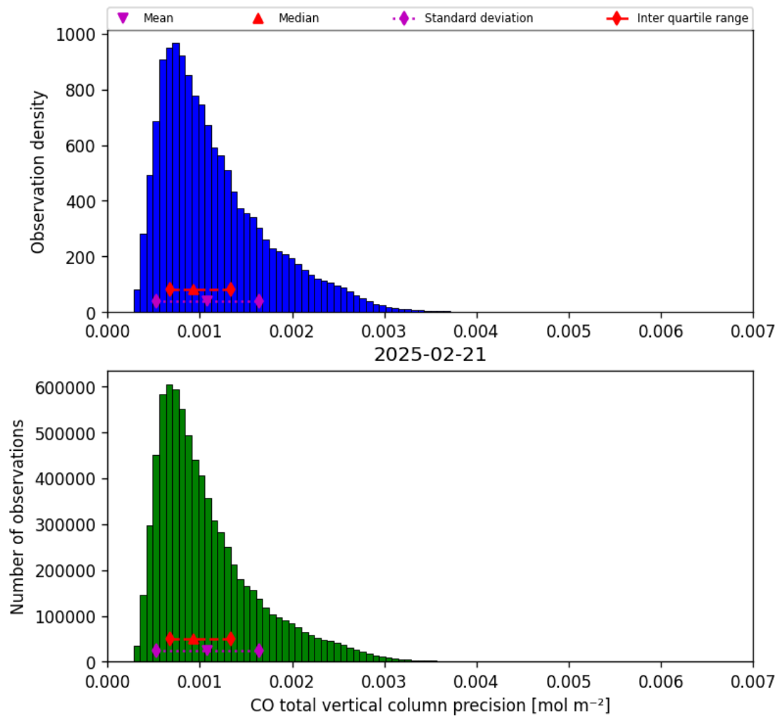
Figure 20: Histogram of “CO total vertical column precision” for 2025-02-20 to 2025-02-22
