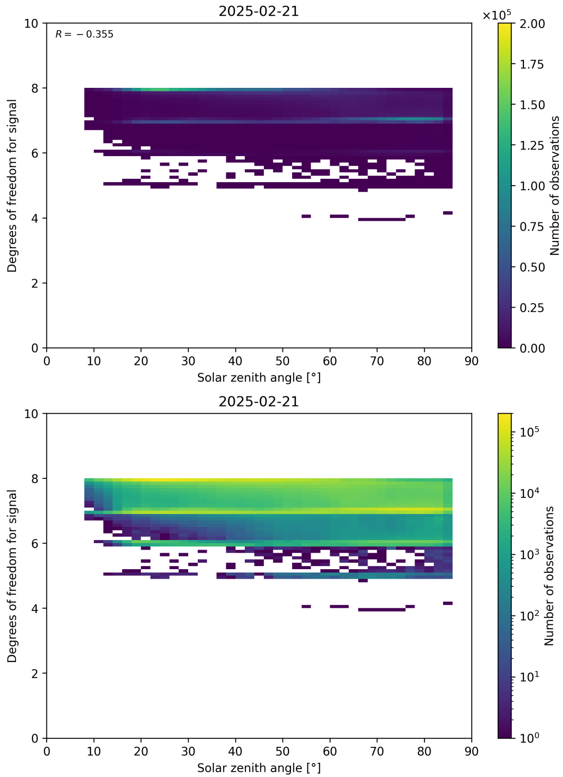
Figure 65: Scatter density plot of “Solar zenith angle” against “Degrees of freedom for signal” for 2025-02-20 to 2025-02-22.
