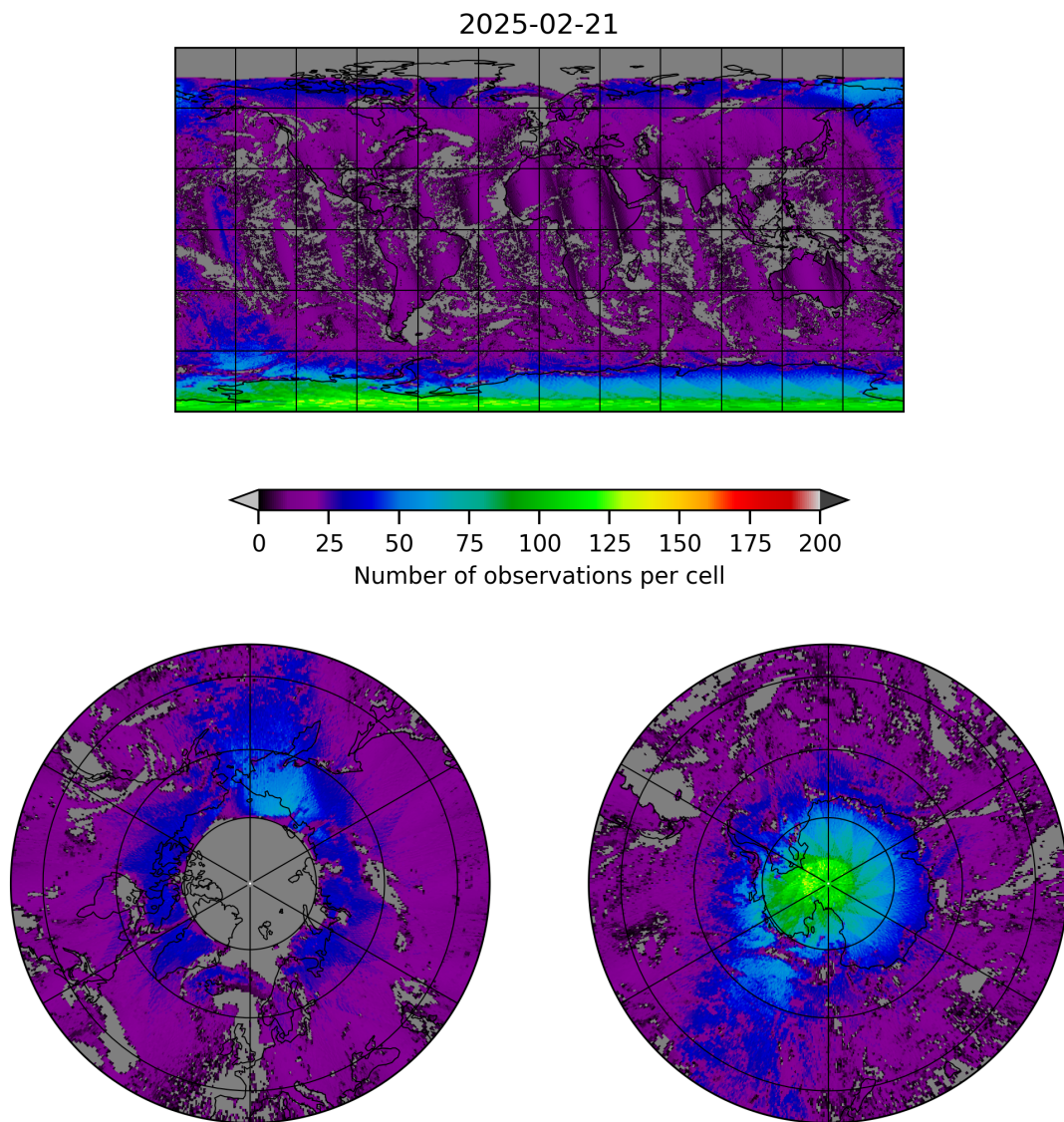
Figure 8: Map of the number of observations for 2025-02-20 to 2025-02-22
