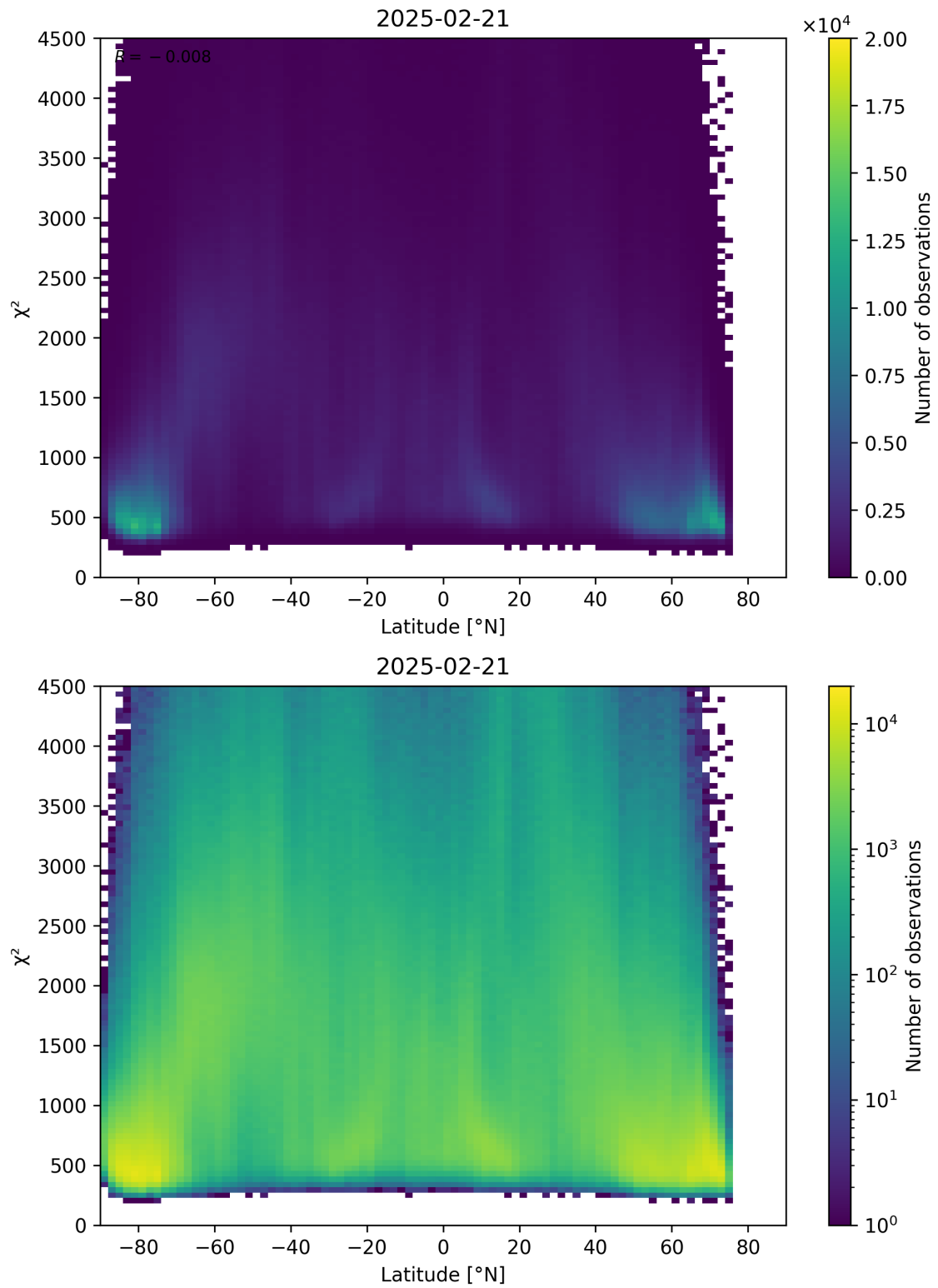
Figure 54: Scatter density plot of “Latitude” against “ \chi^2 ” for 2025-02-20 to 2025-02-22.
