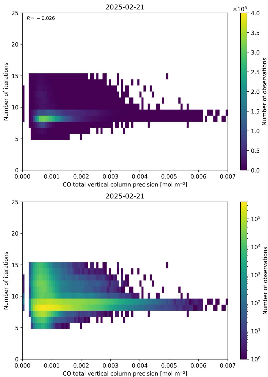
Figure 46: Scatter density plot of “CO total vertical column precision” against “Number of iterations” for 2025-02-20 to 2025-02-22.
