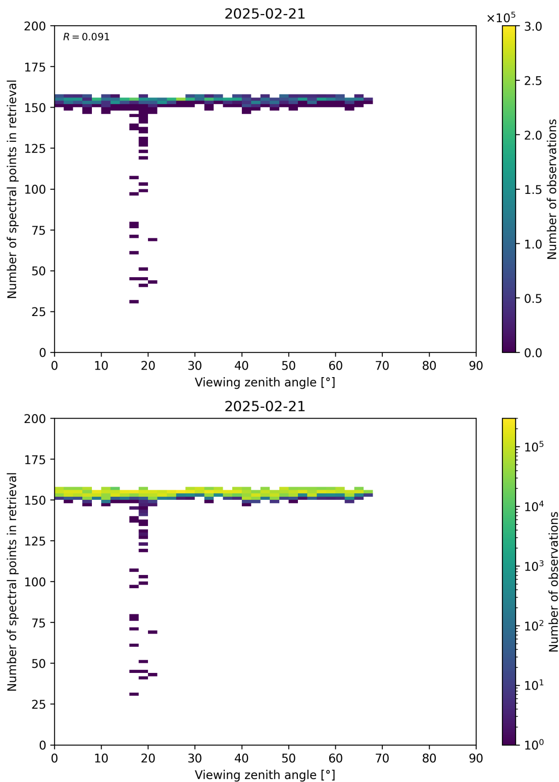
Figure 76: Scatter density plot of “Viewing zenith angle” against “Number of spectral points in retrieval” for 2025-02-20 to 2025-02-22.
