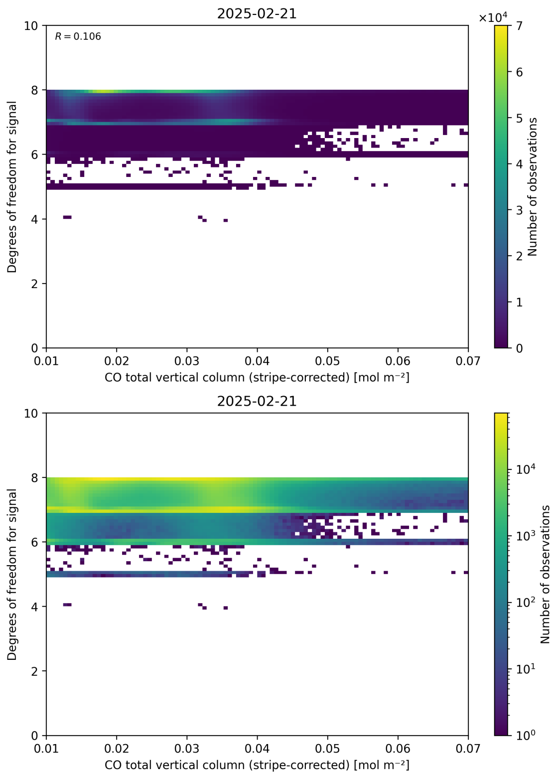
Figure 38: Scatter density plot of “CO total vertical column (stripe-corrected)” against “Degrees of freedom for signal” for 2025-02-20 to 2025-02-22.
