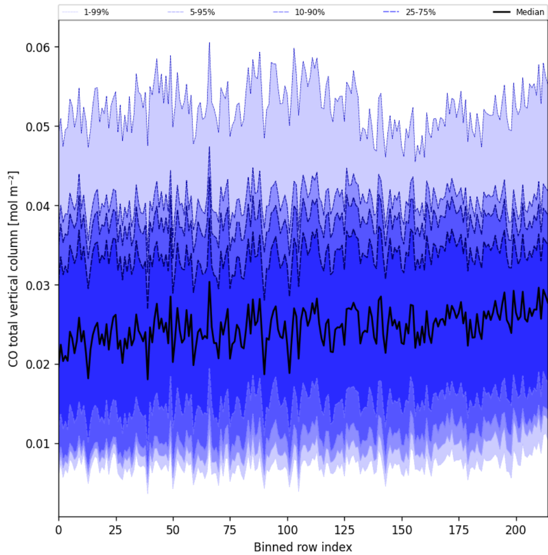
Figure 26: Along track statistics of “CO total vertical column” for 2025-02-20 to 2025-02-22
