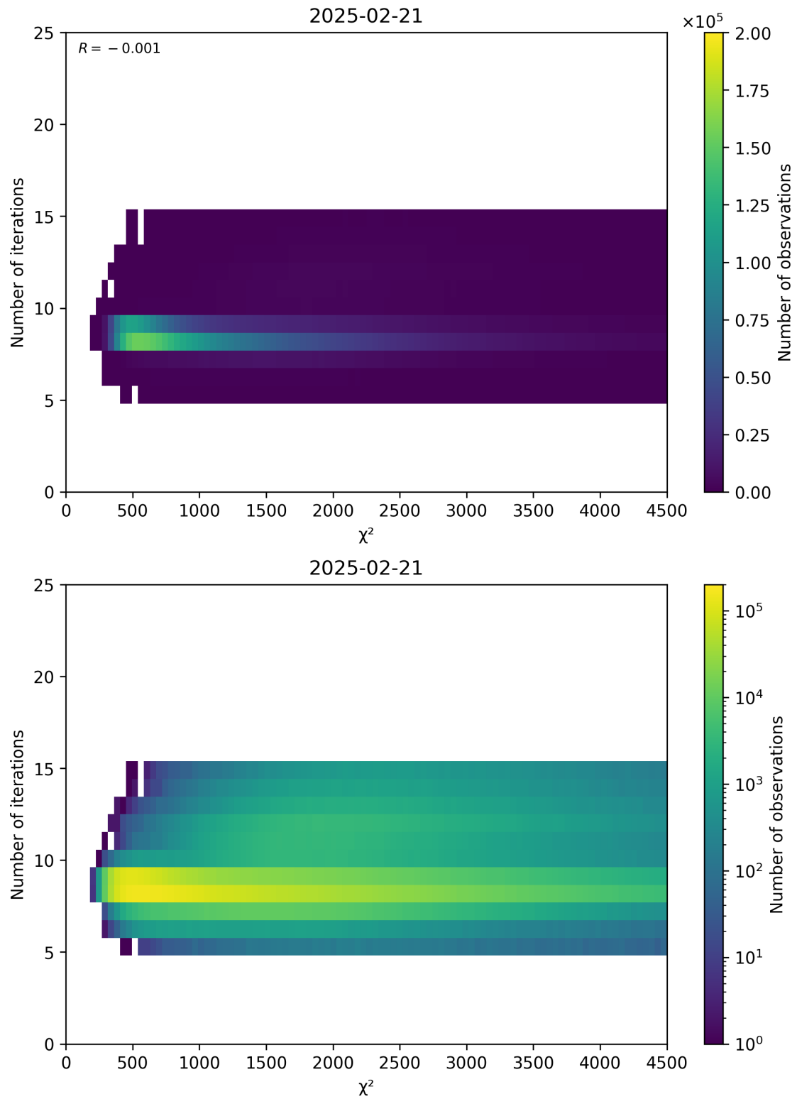
Figure 49: Scatter density plot of “ \chi^2 ” against “Number of iterations” for 2025-02-20 to 2025-02-22.
