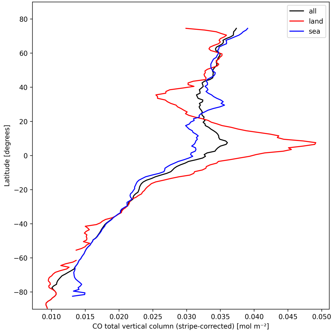
Figure 11: Zonal average of “CO total vertical column (stripe-corrected)” for 2025-02-20 to 2025-02-22.
