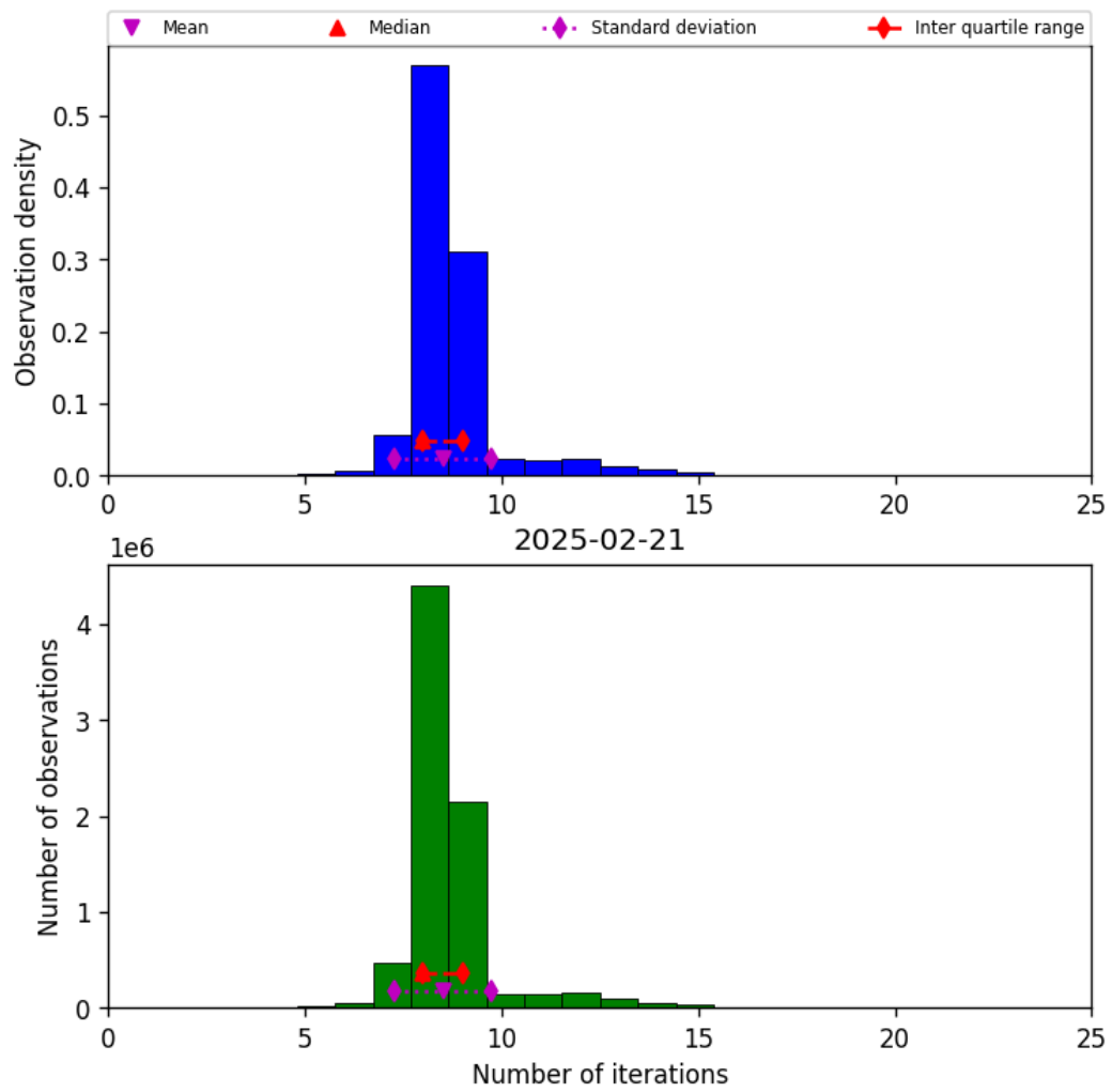
Figure 24: Histogram of “Number of iterations” for 2025-02-20 to 2025-02-22
