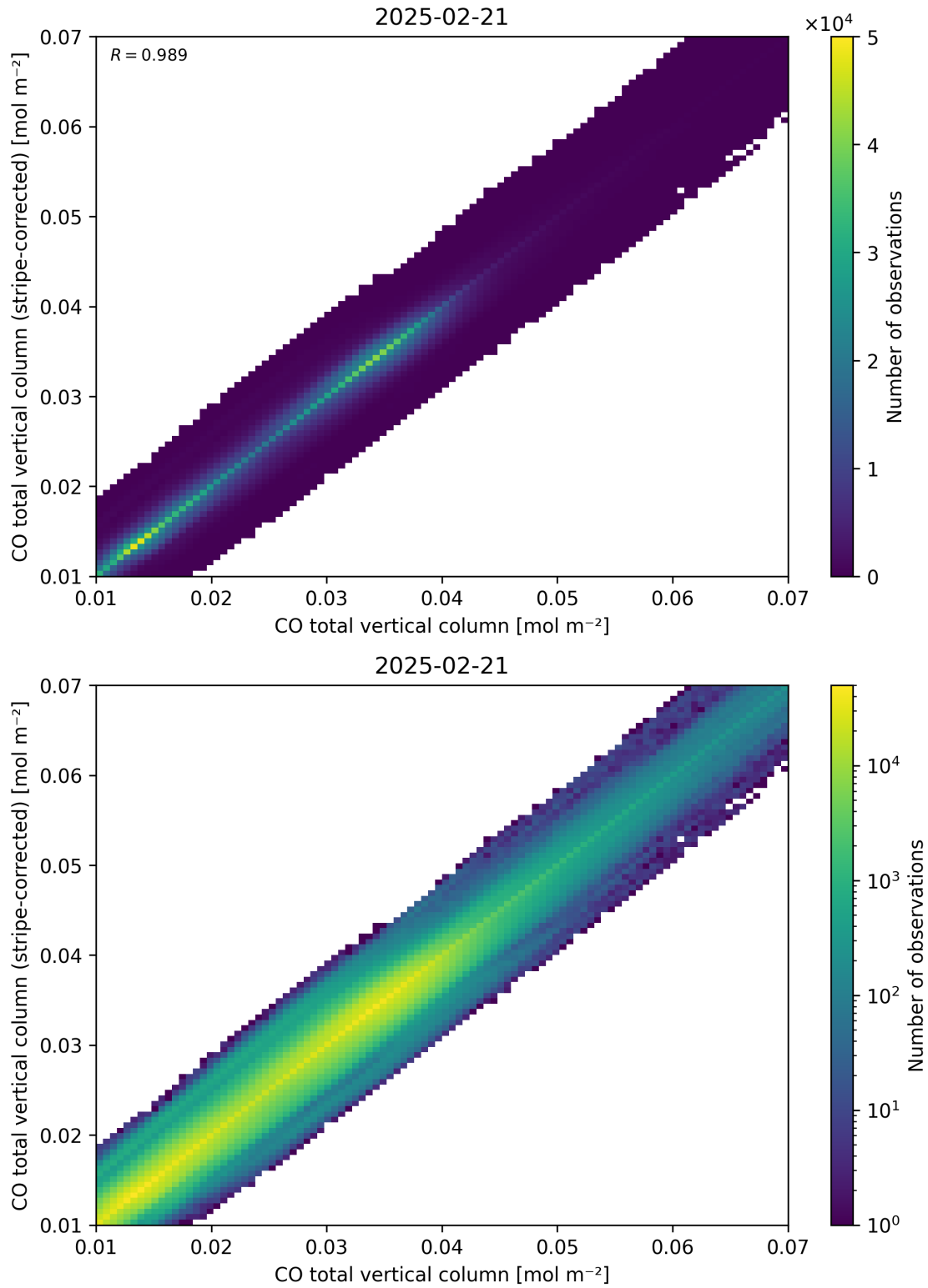
Figure 33: Scatter density plot of “CO total vertical column” against “CO total vertical column (stripe-corrected)” for 2025-02-20 to 2025-02-22.
