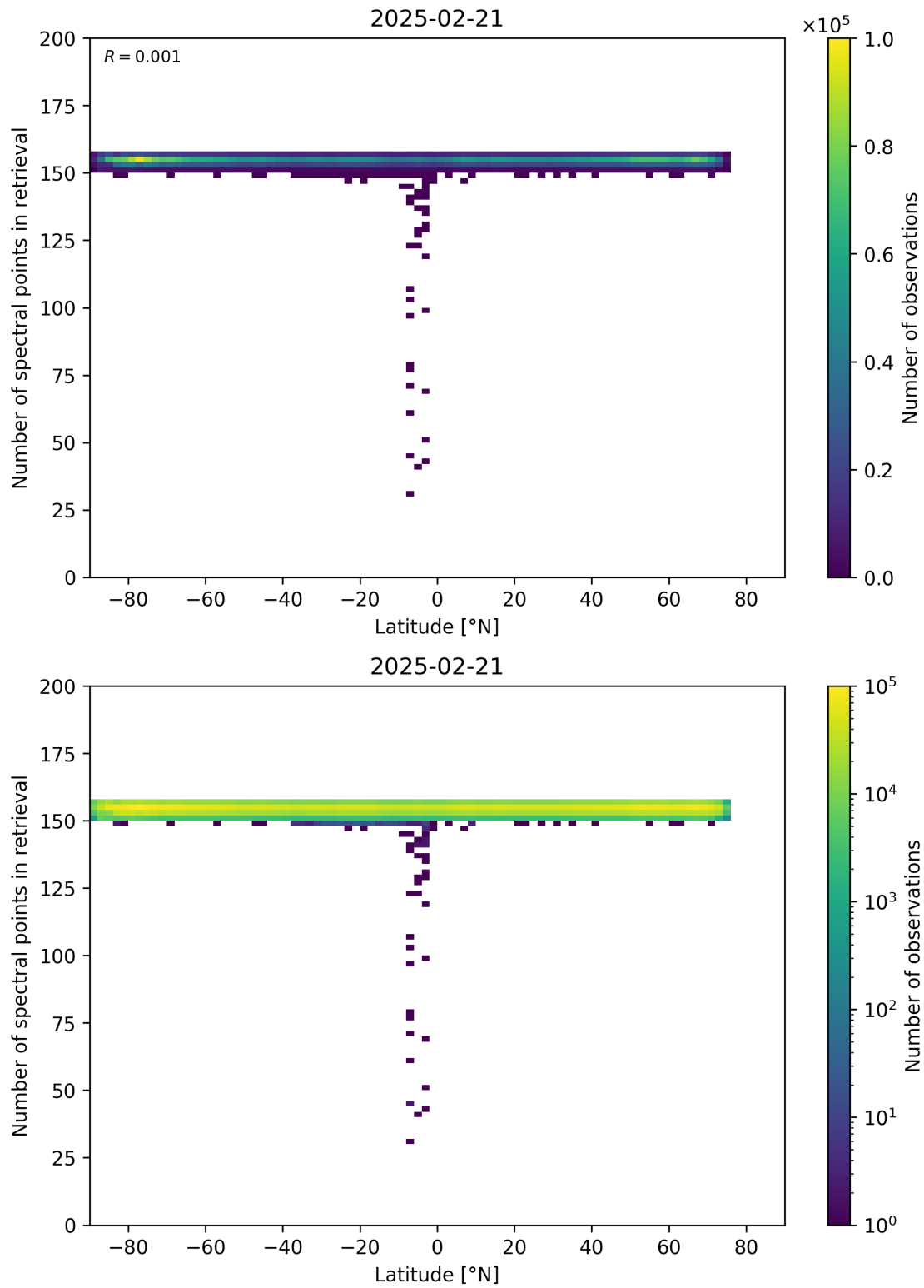
Figure 57: Scatter density plot of “Latitude” against “Number of spectral points in retrieval” for 2025-02-20 to 2025-02-22.
