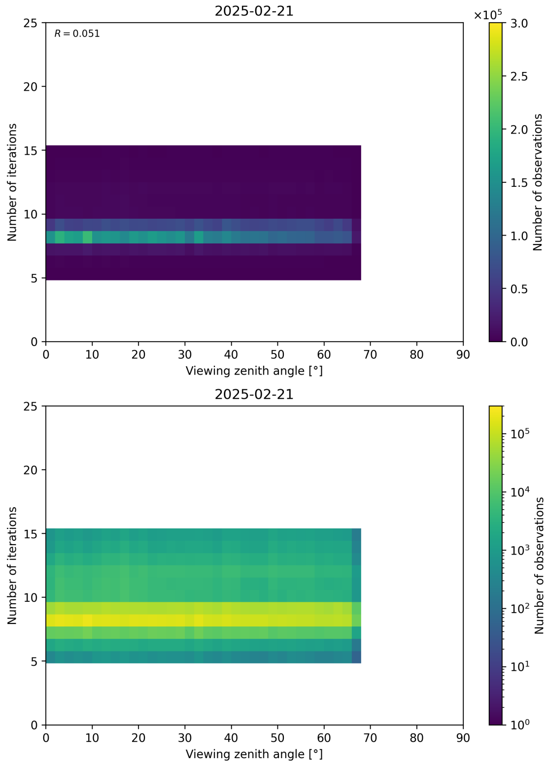
Figure 75: Scatter density plot of “Viewing zenith angle” against “Number of iterations” for 2025-02-20 to 2025-02-22.
