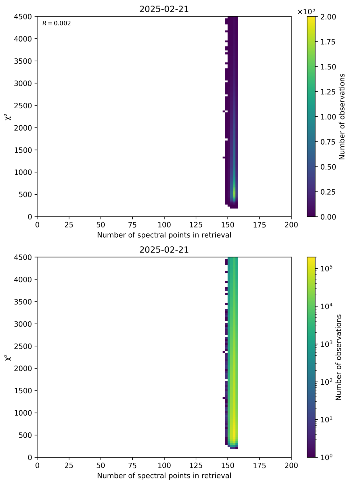
Figure 58: Scatter density plot of “Number of spectral points in retrieval” against “ \chi^2 ” for 2025-02-20 to 2025-02-22.
