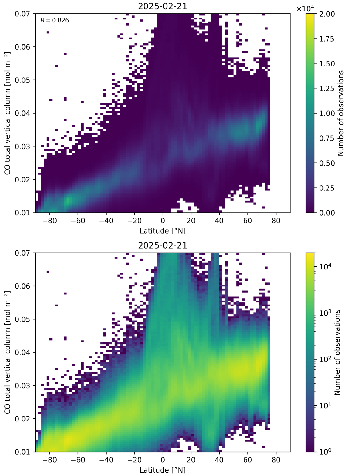
Figure 51: Scatter density plot of “Latitude” against “CO total vertical column” for 2025-02-20 to 2025-02-22.
