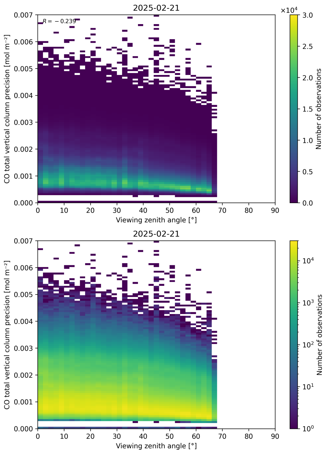
Figure 71: Scatter density plot of “Viewing zenith angle” against “CO total vertical column precision” for 2025-02-20 to 2025-02-22.
