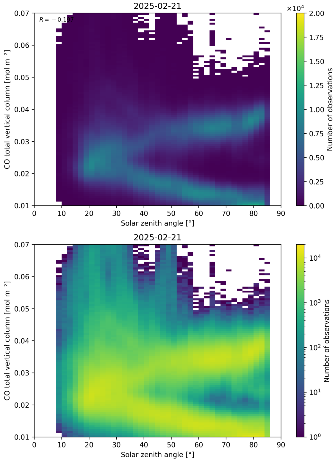
Figure 61: Scatter density plot of “Solar zenith angle” against “CO total vertical column” for 2025-02-20 to 2025-02-22.
