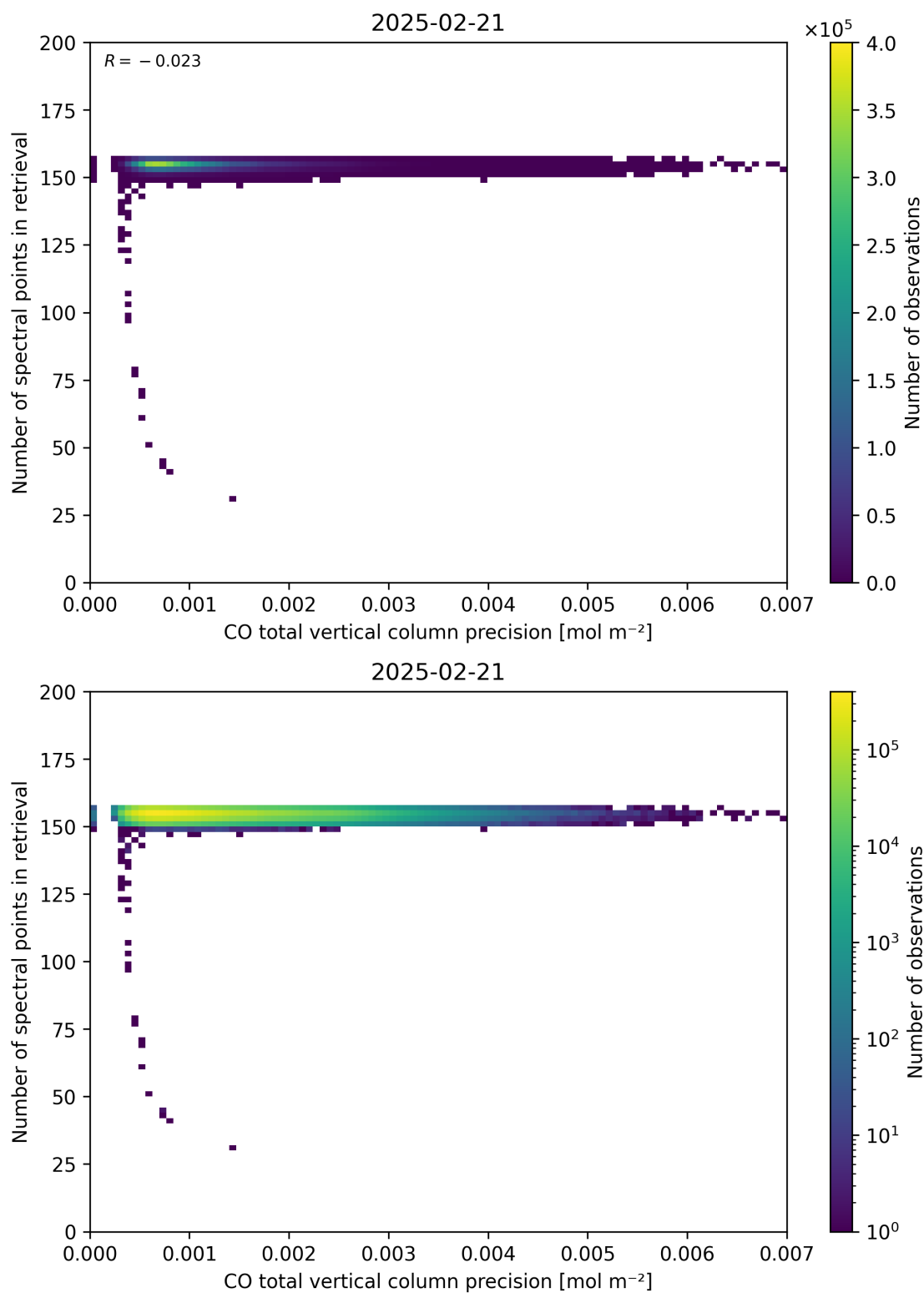
Figure 47: Scatter density plot of “CO total vertical column precision” against “Number of spectral points in retrieval” for 2025-02-20 to 2025-02-22.
