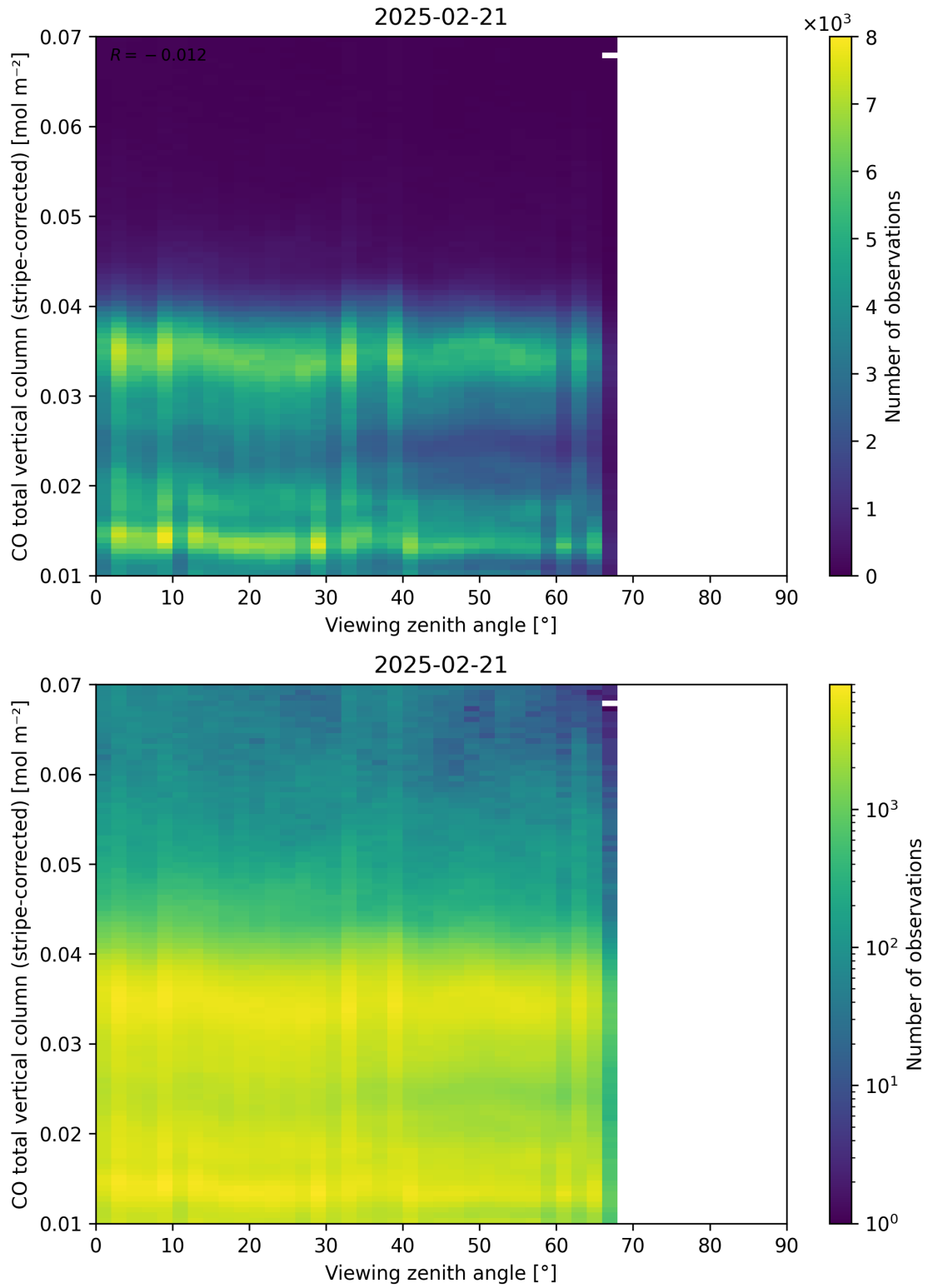
Figure 70: Scatter density plot of “Viewing zenith angle” against “CO total vertical column (stripe-corrected)” for 2025-02-20 to 2025-02-22.
