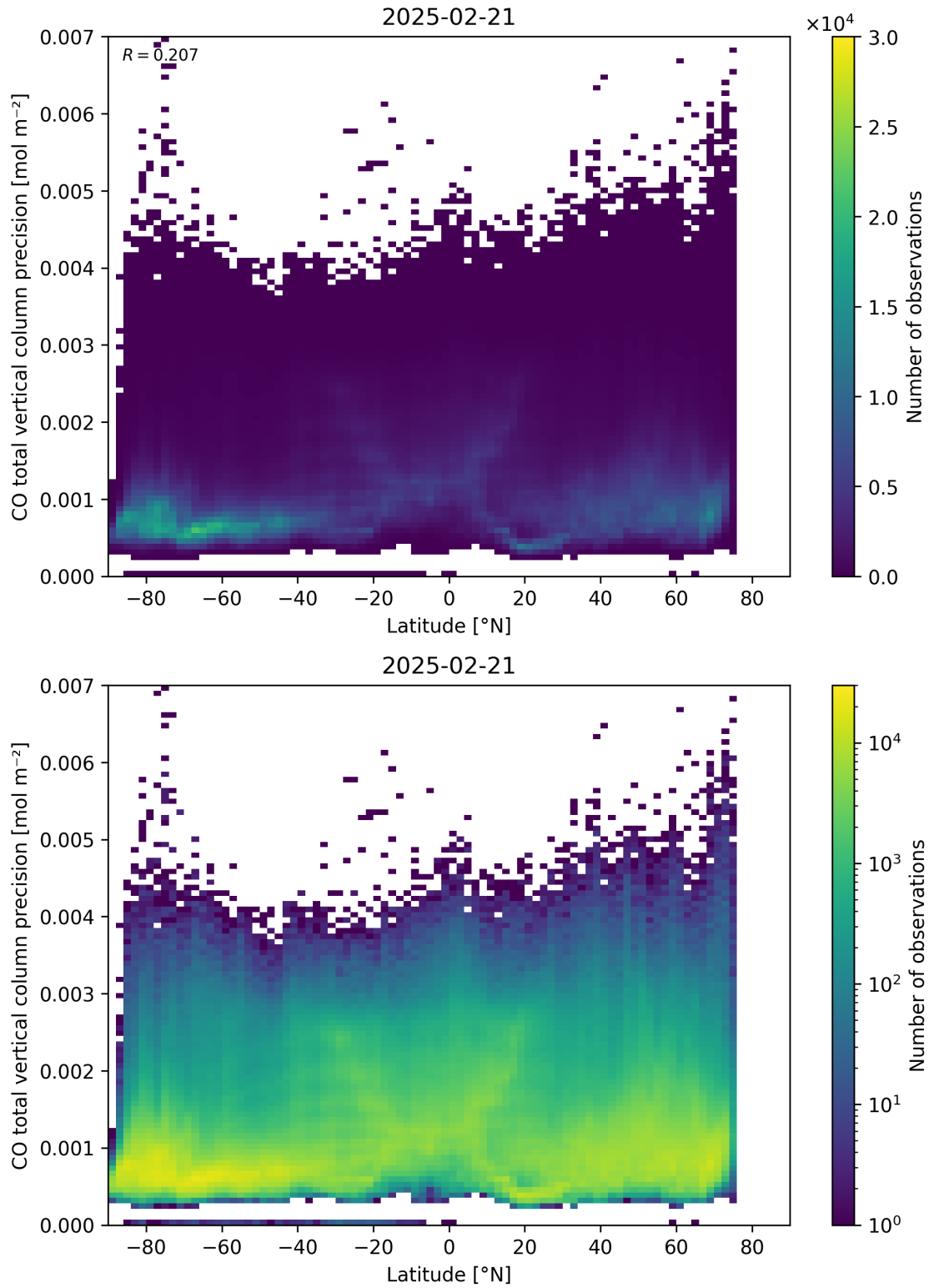
Figure 53: Scatter density plot of “Latitude” against “CO total vertical column precision” for 2025-02-20 to 2025-02-22.
