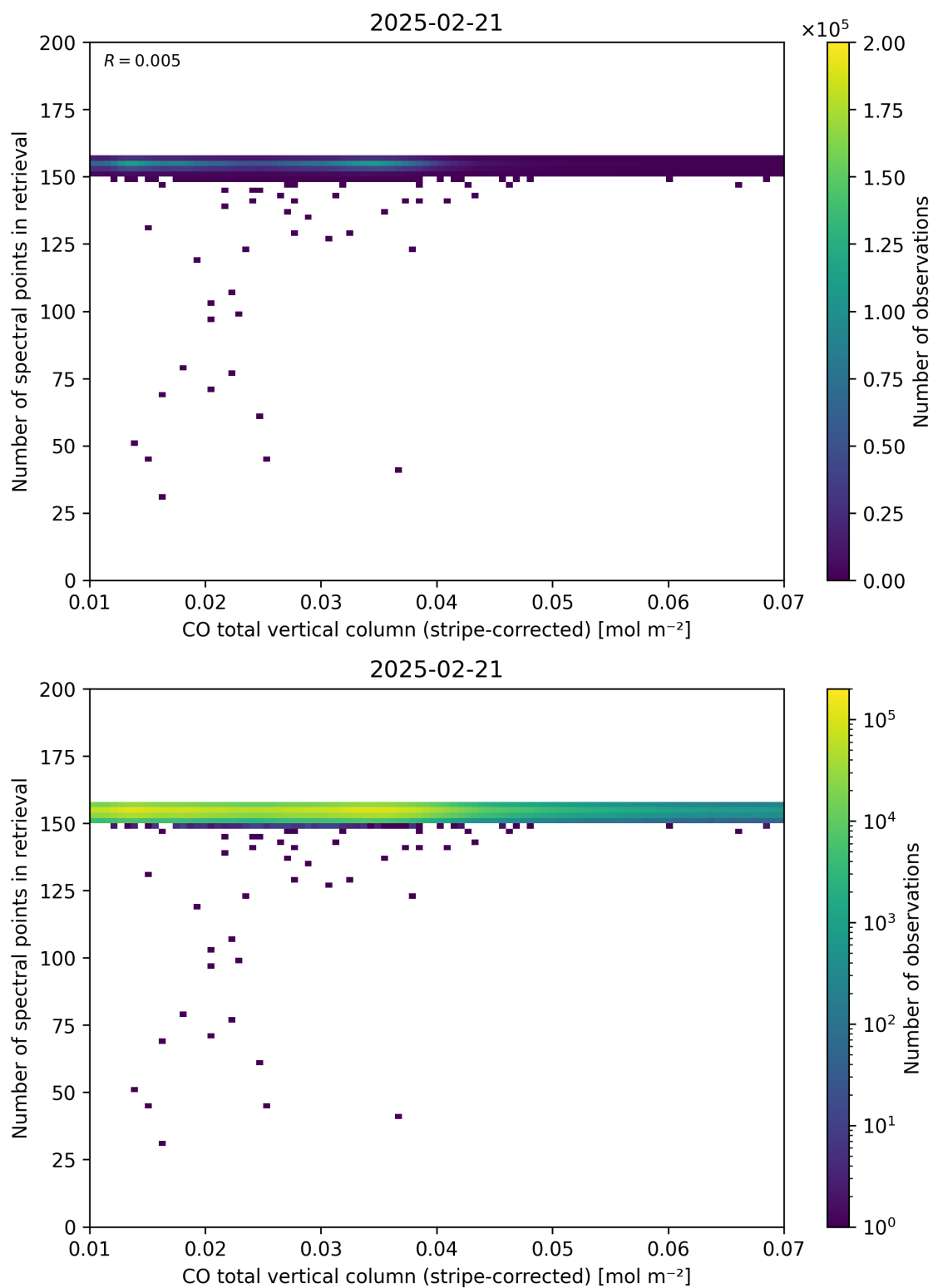
Figure 40: Scatter density plot of “CO total vertical column (stripe-corrected)” against “Number of spectral points in retrieval” for 2025-02-20 to 2025-02-22.
