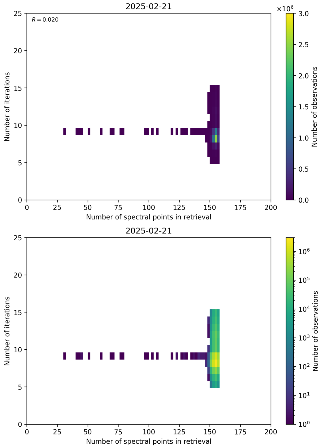
Figure 60: Scatter density plot of “Number of spectral points in retrieval” against “Number of iterations” for 2025-02-20 to 2025-02-22.
