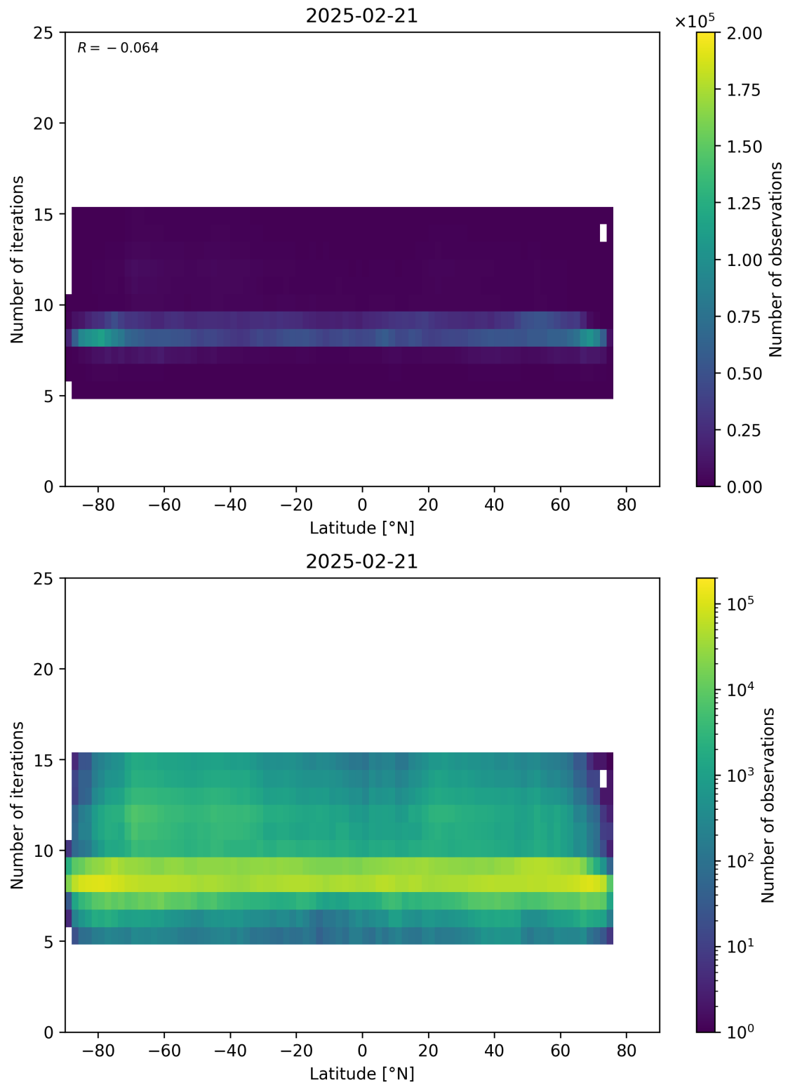
Figure 56: Scatter density plot of “Latitude” against “Number of iterations” for 2025-02-20 to 2025-02-22.
