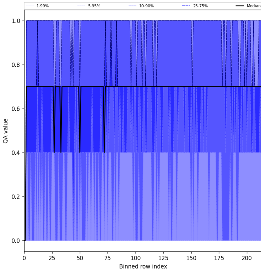
Figure 25: Along track statistics of “QA value” for 2025-02-20 to 2025-02-22
