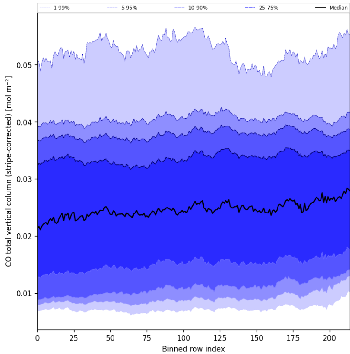
Figure 27: Along track statistics of “CO total vertical column (stripe-corrected)” for 2025-02-20 to 2025-02-22
