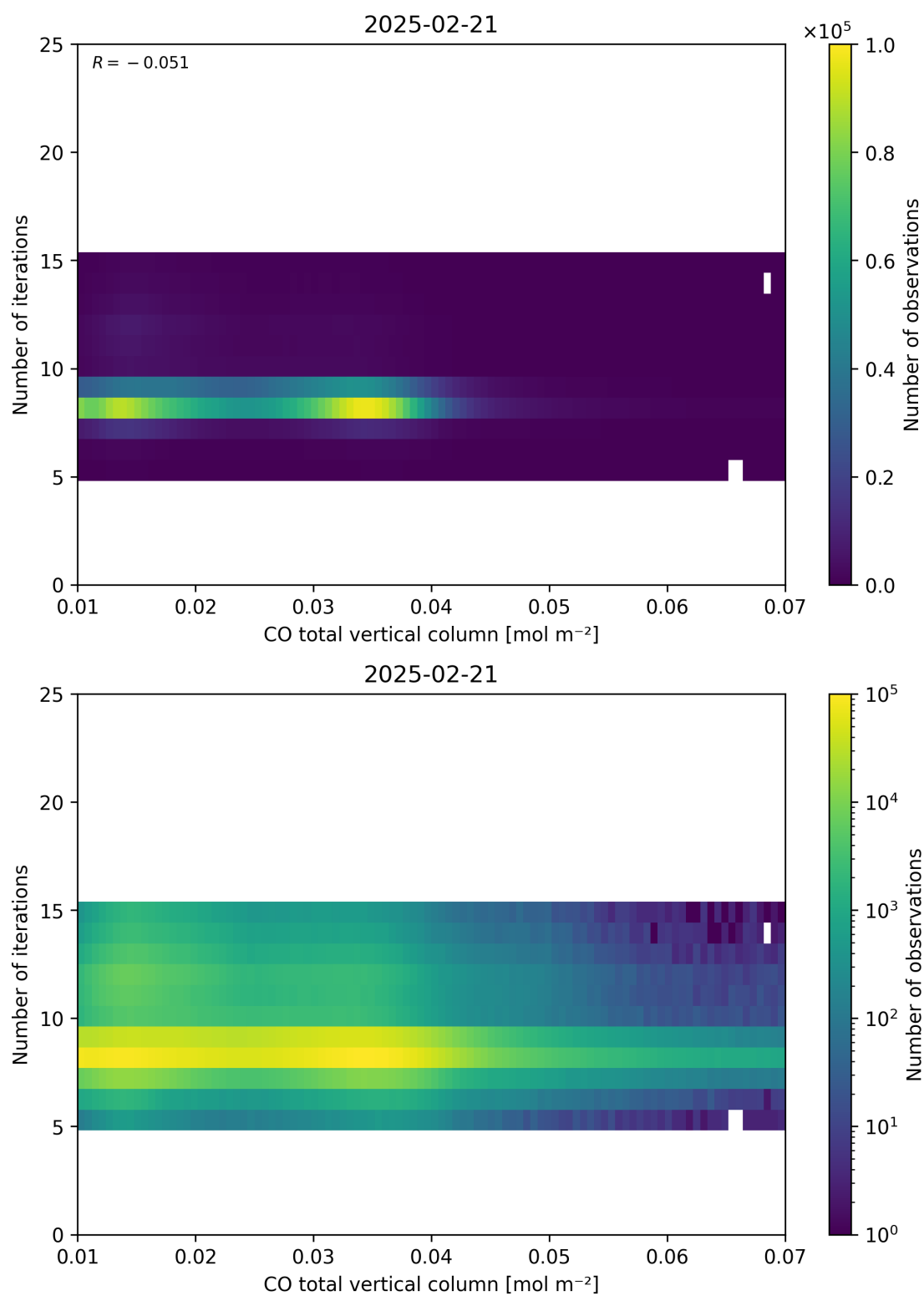
Figure 42: Scatter density plot of “CO total vertical column” against “Number of iterations” for 2025-02-20 to 2025-02-22.
