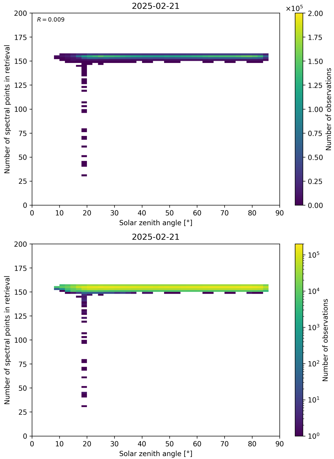
Figure 68: Scatter density plot of “Solar zenith angle” against “Number of spectral points in retrieval” for 2025-02-20 to 2025-02-22.
