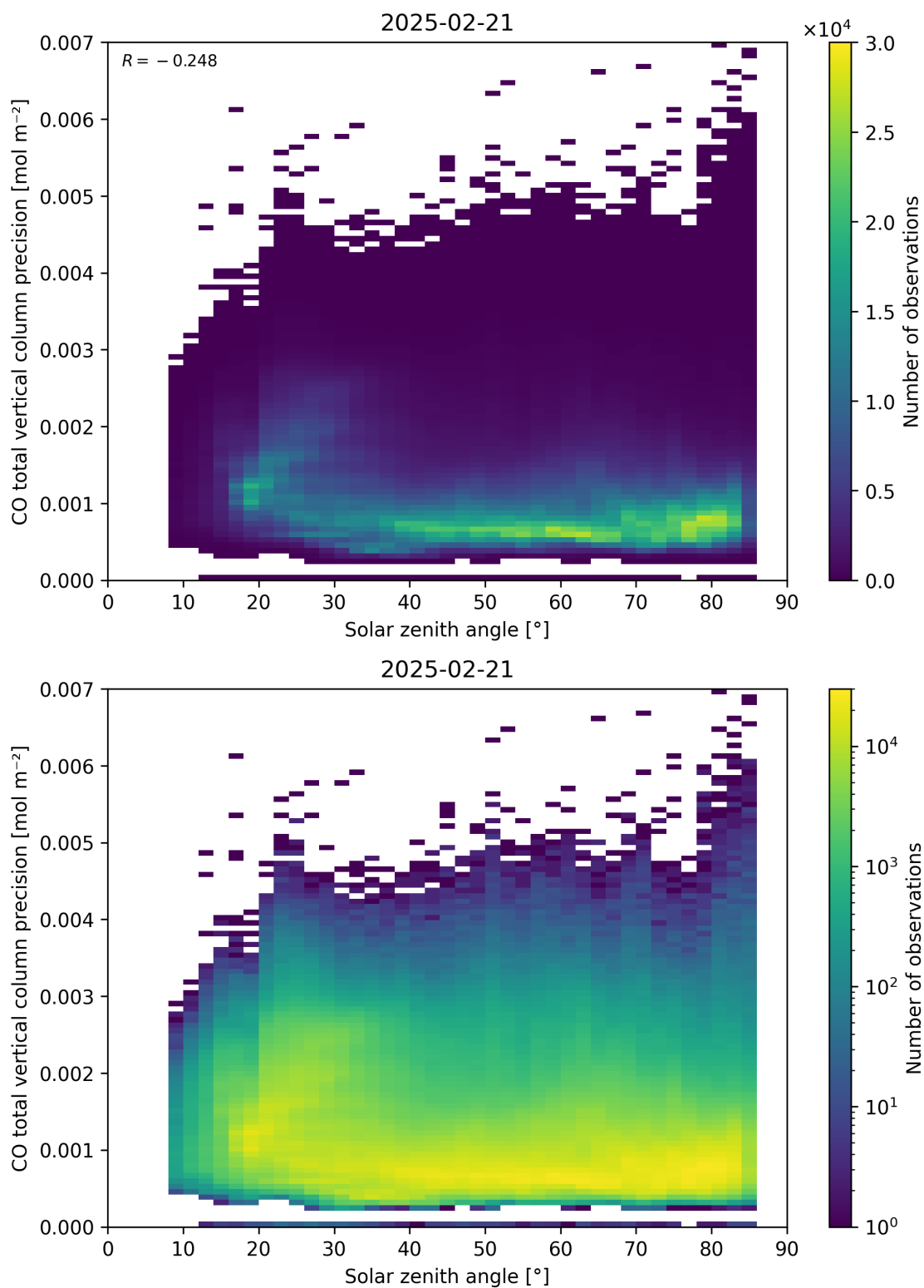
Figure 63: Scatter density plot of “Solar zenith angle” against “CO total vertical column precision” for 2025-02-20 to 2025-02-22.
