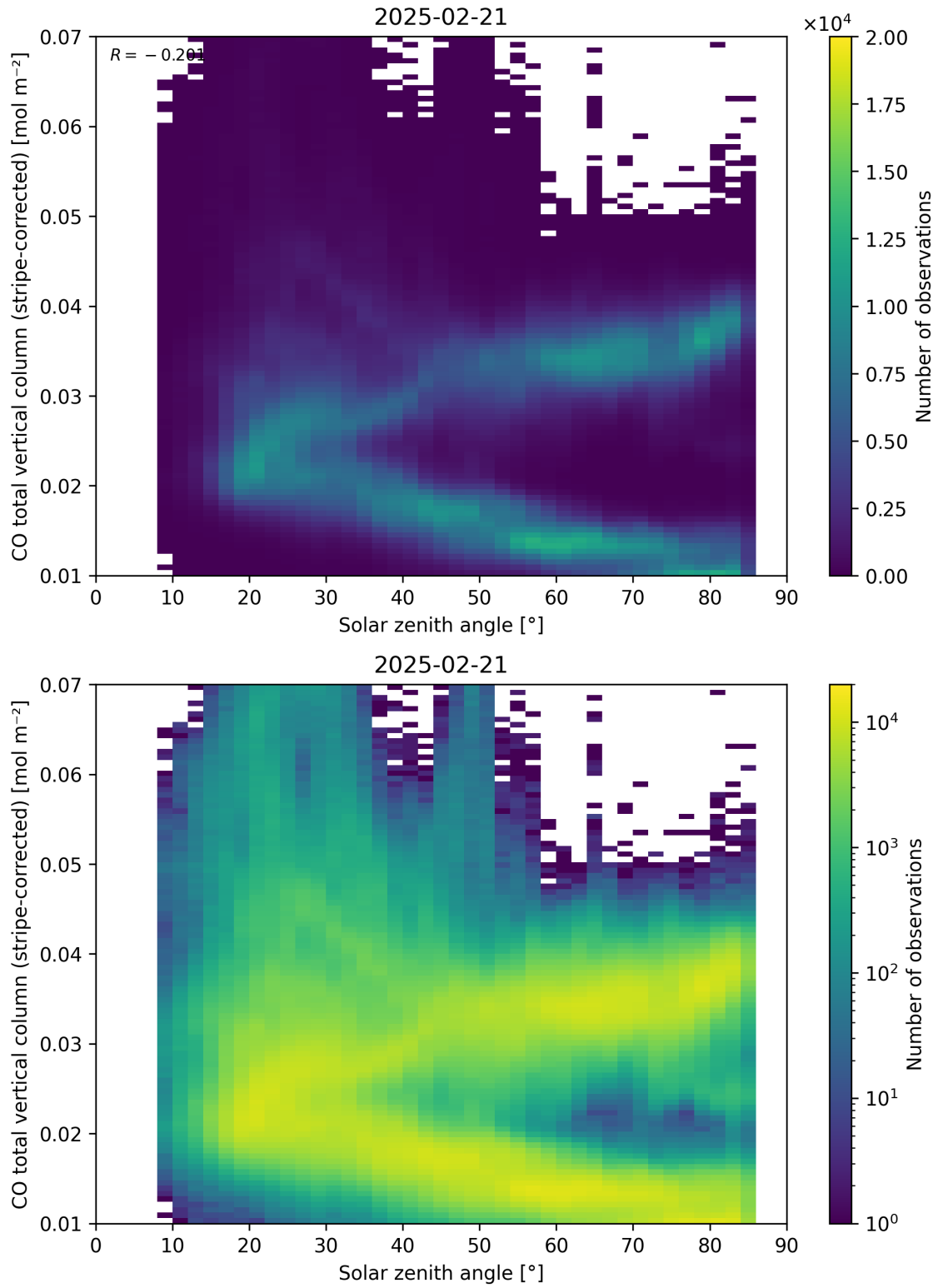
Figure 62: Scatter density plot of “Solar zenith angle” against “CO total vertical column (stripe-corrected)” for 2025-02-20 to 2025-02-22.
