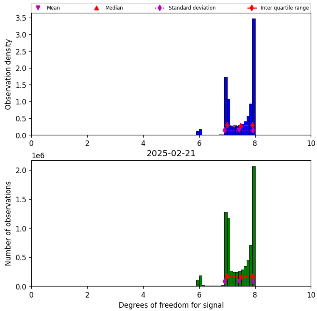
Figure 23: Histogram of “Degrees of freedom for signal” for 2025-02-20 to 2025-02-22
