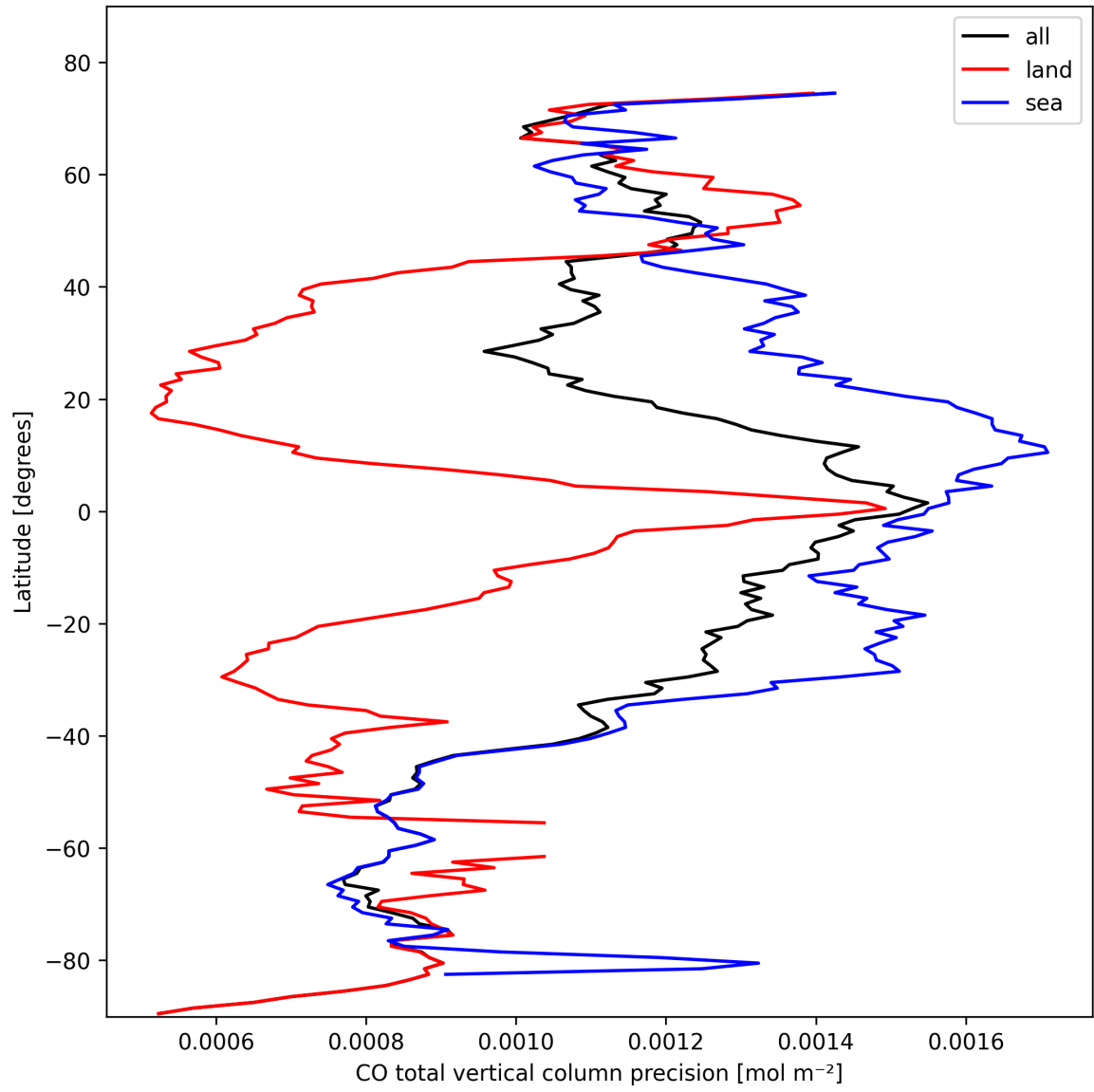
Figure 12: Zonal average of "CO total vertical column precision" for 2025-02-20 to 2025-02-22.
