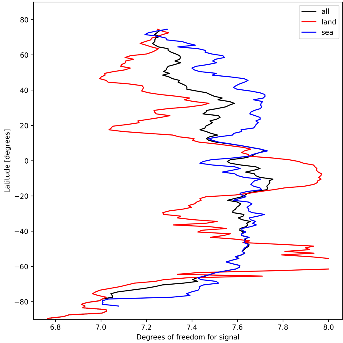
Figure 15: Zonal average of “Degrees of freedom for signal” for 2025-02-20 to 2025-02-22.
