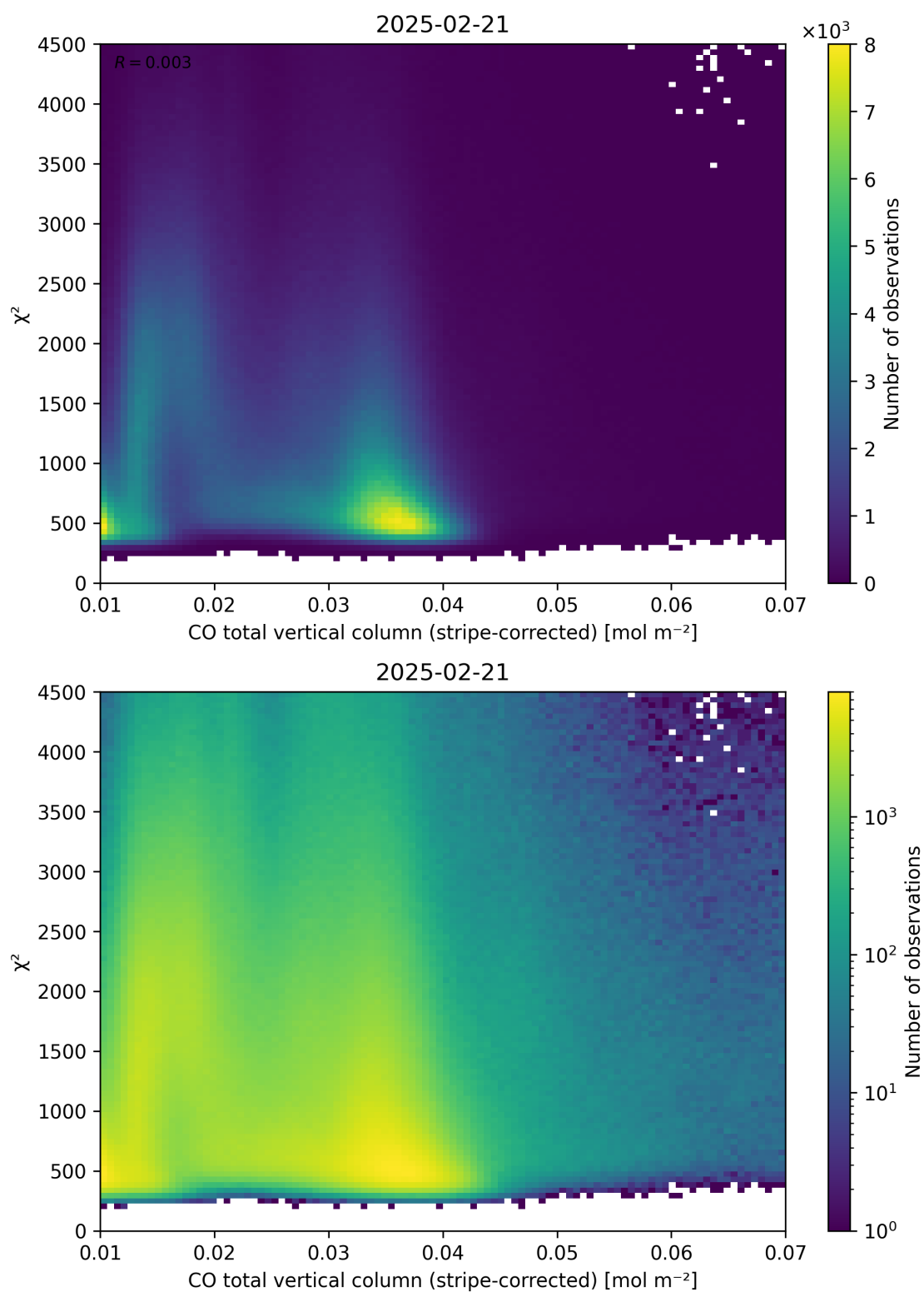
Figure 37: Scatter density plot of “CO total vertical column (stripe-corrected)” against “ \chi^2 ” for 2025-02-20 to 2025-02-22.
