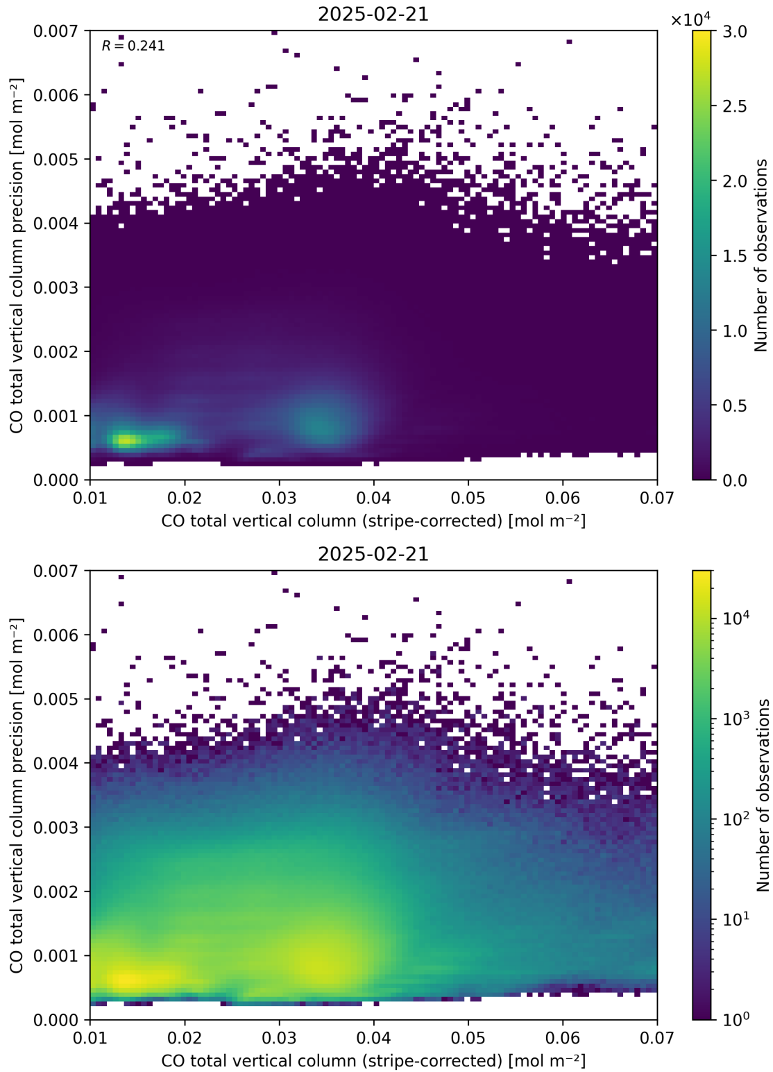
Figure 36: Scatter density plot of “CO total vertical column (stripe-corrected)” against “CO total vertical column precision” for 2025-02-20 to 2025-02-22.
