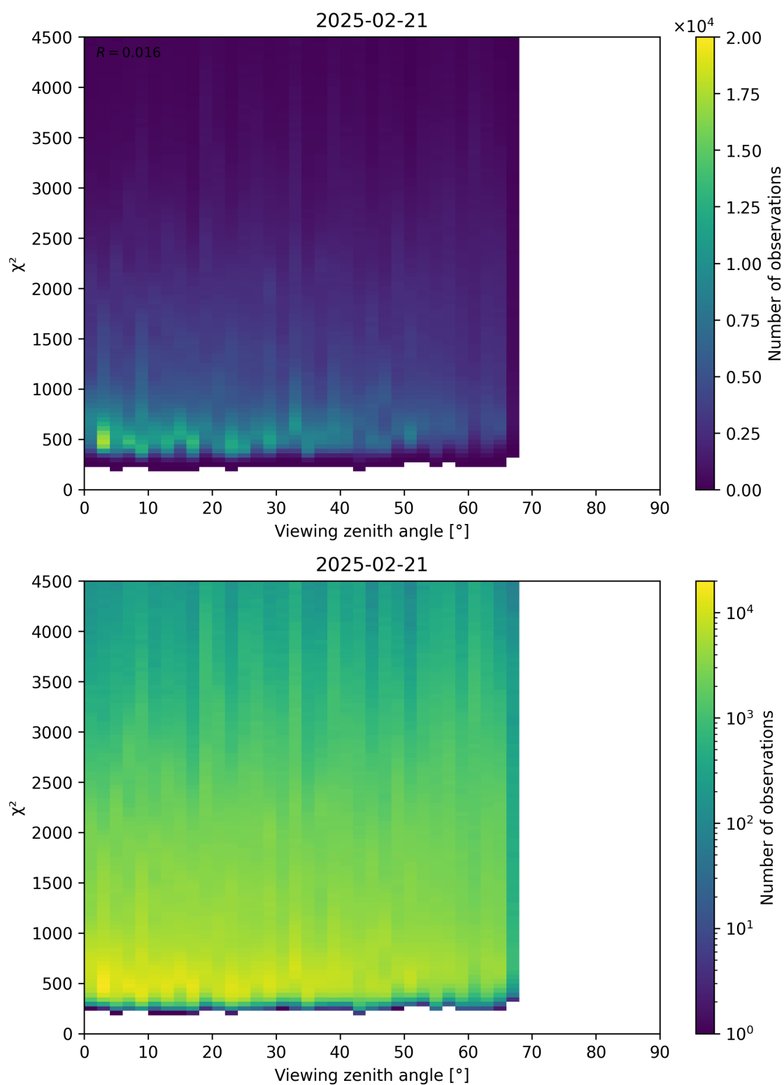
Figure 72: Scatter density plot of “Viewing zenith angle” against “ \chi^2 ” for 2025-02-20 to 2025-02-22.
