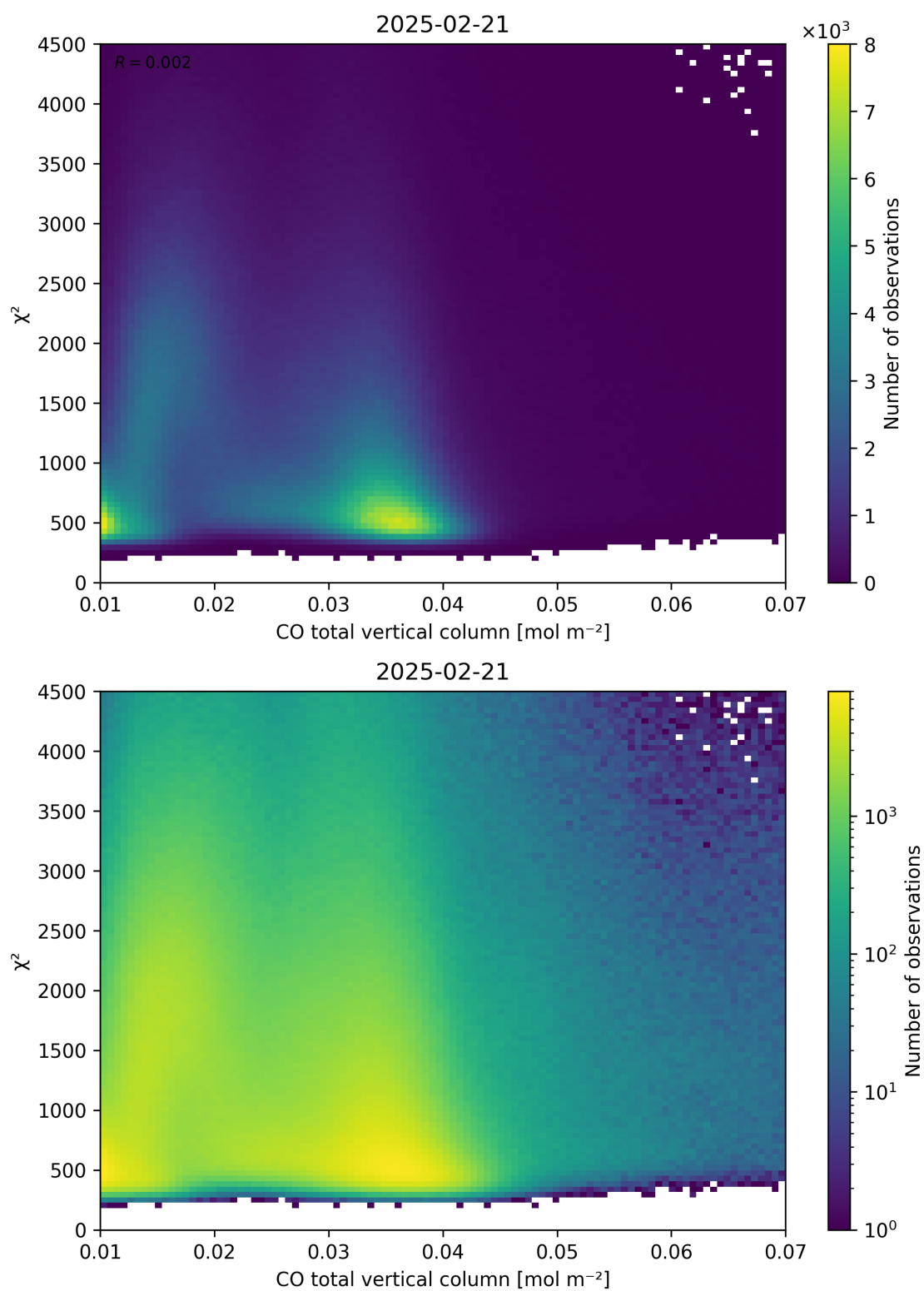
Figure 35: Scatter density plot of “CO total vertical column” against “ \chi^2 ” for 2025-02-20 to 2025-02-22.
