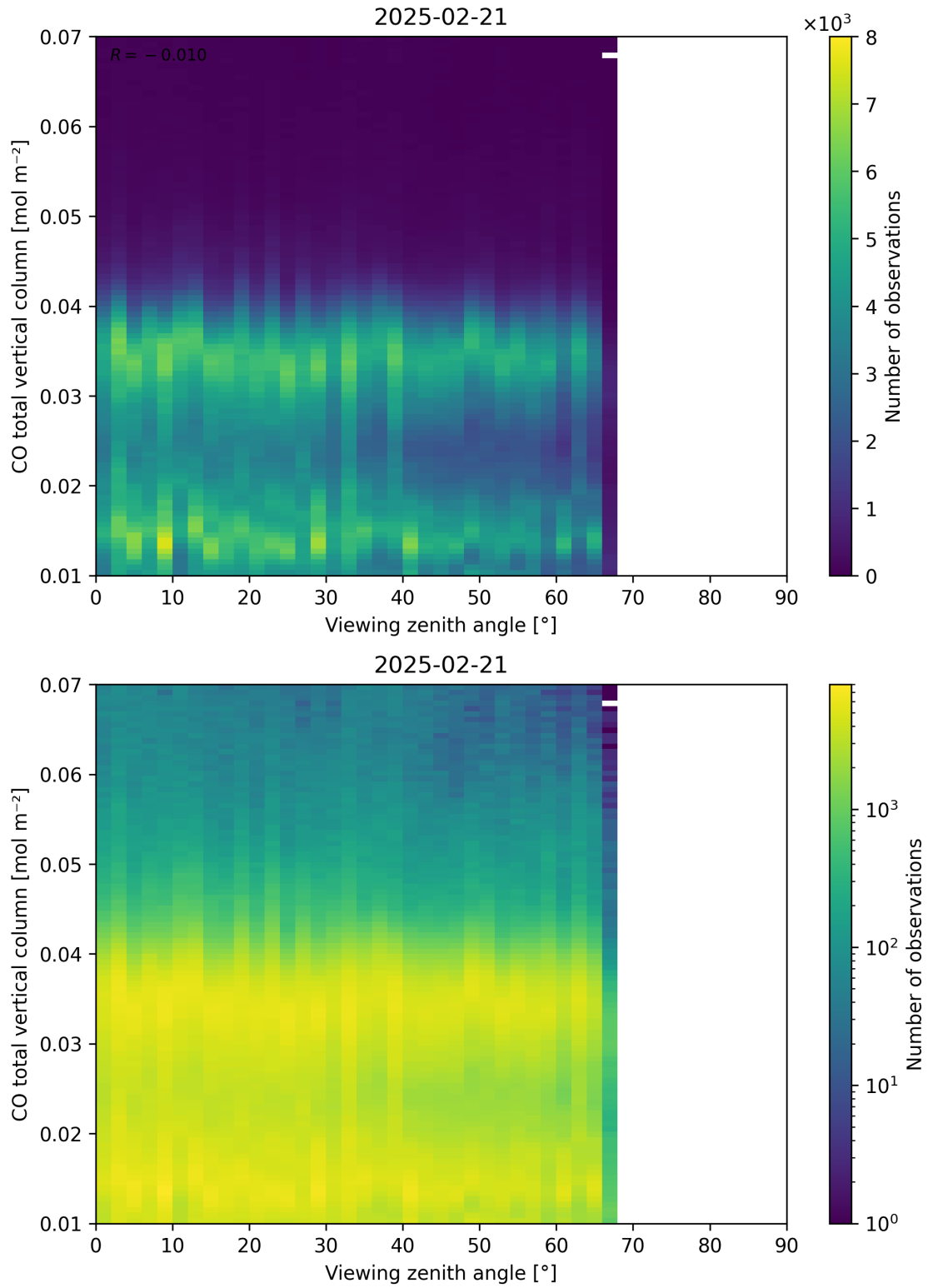
Figure 69: Scatter density plot of “Viewing zenith angle” against “CO total vertical column” for 2025-02-20 to 2025-02-22.
