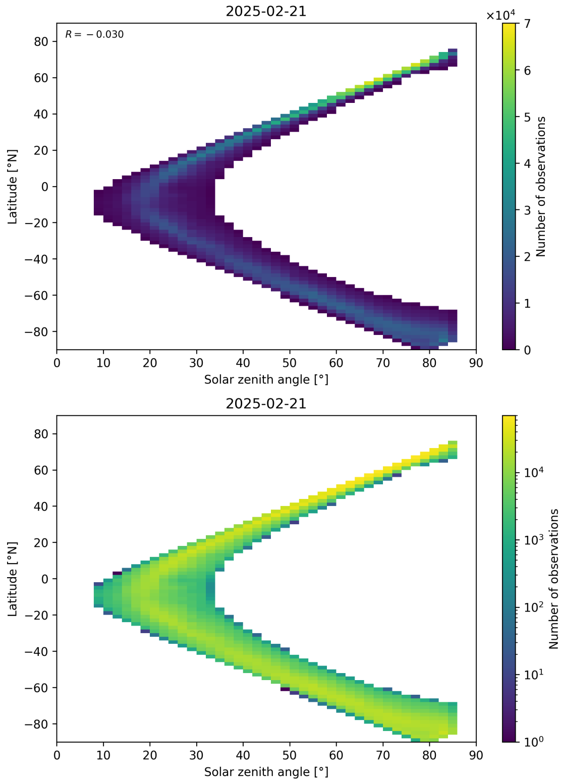
Figure 66: Scatter density plot of “Solar zenith angle” against “Latitude” for 2025-02-20 to 2025-02-22.
