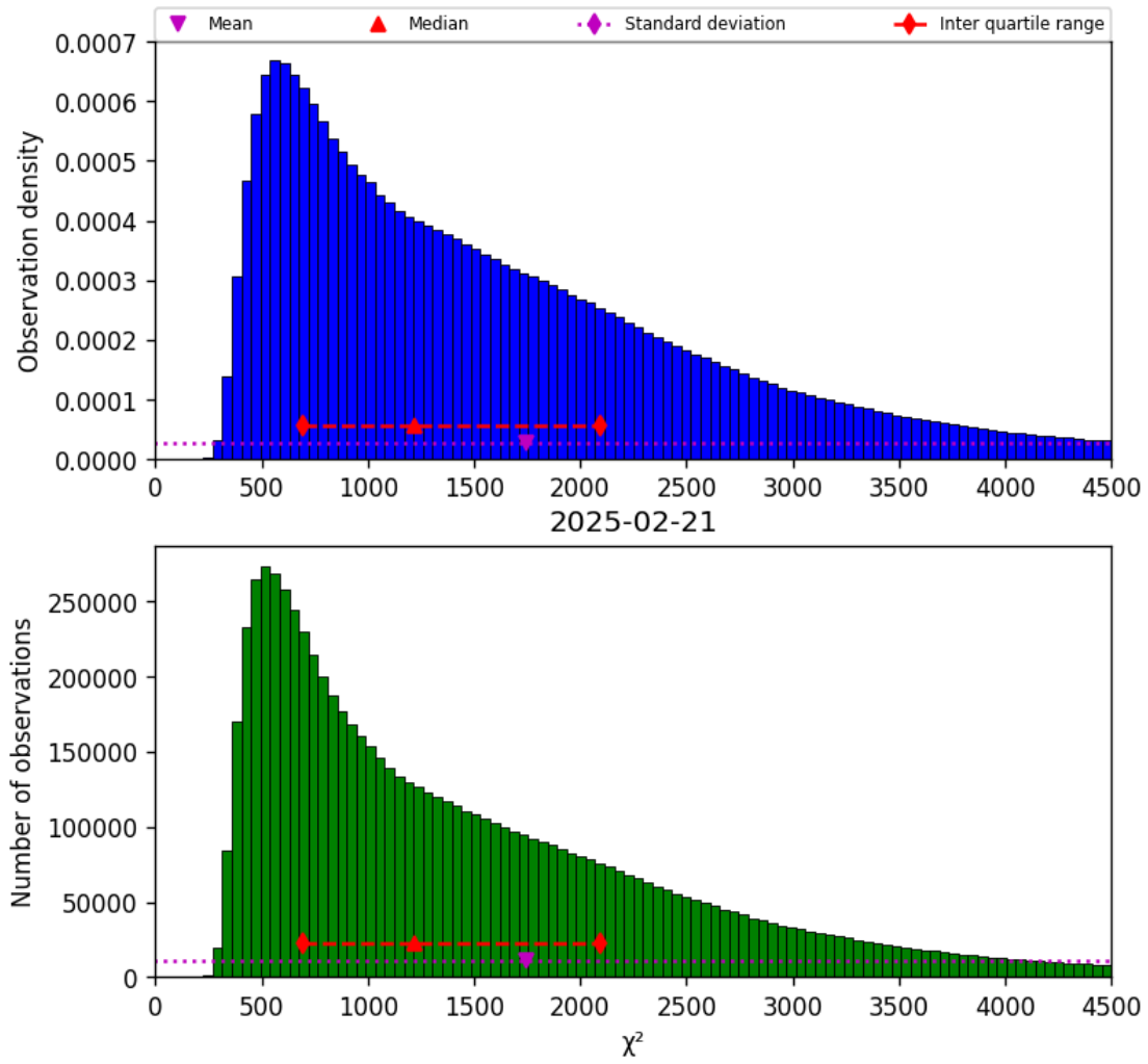
Figure 22: Histogram of “ \chi^2 ” for 2025-02-20 to 2025-02-22
