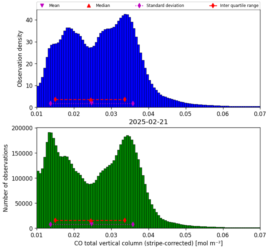
Figure 19: Histogram of “CO total vertical column (stripe-corrected)” for 2025-02-20 to 2025-02-22
