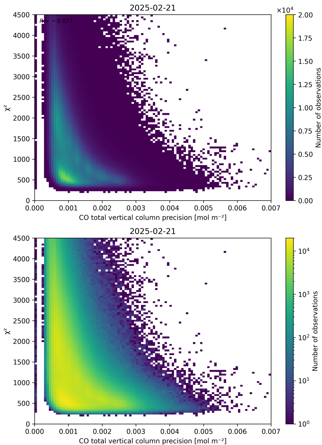
Figure 44: Scatter density plot of “CO total vertical column precision” against “ \chi^2 ” for 2025-02-20 to 2025-02-22.
