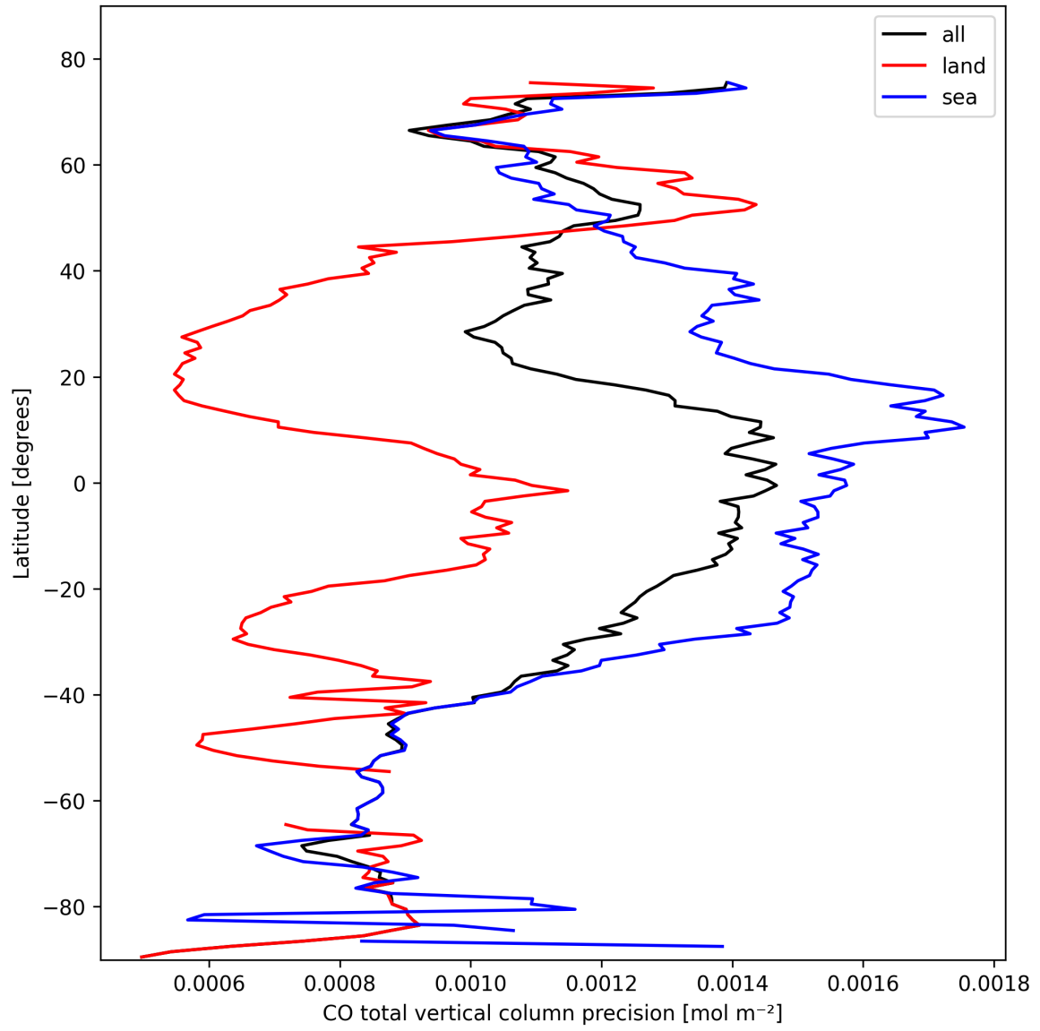
Figure 12: Zonal average of "CO total vertical column precision" for 2025-02-21 to 2025-02-23.
