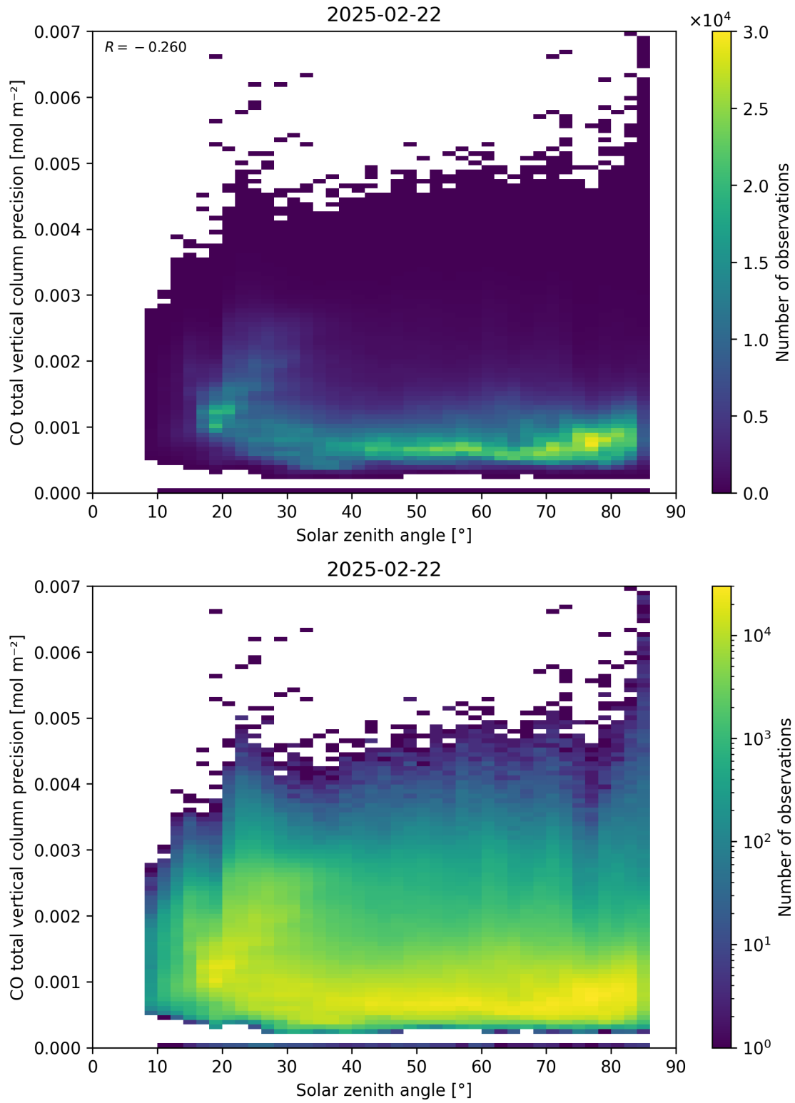
Figure 63: Scatter density plot of “Solar zenith angle” against “CO total vertical column precision” for 2025-02-21 to 2025-02-23.
