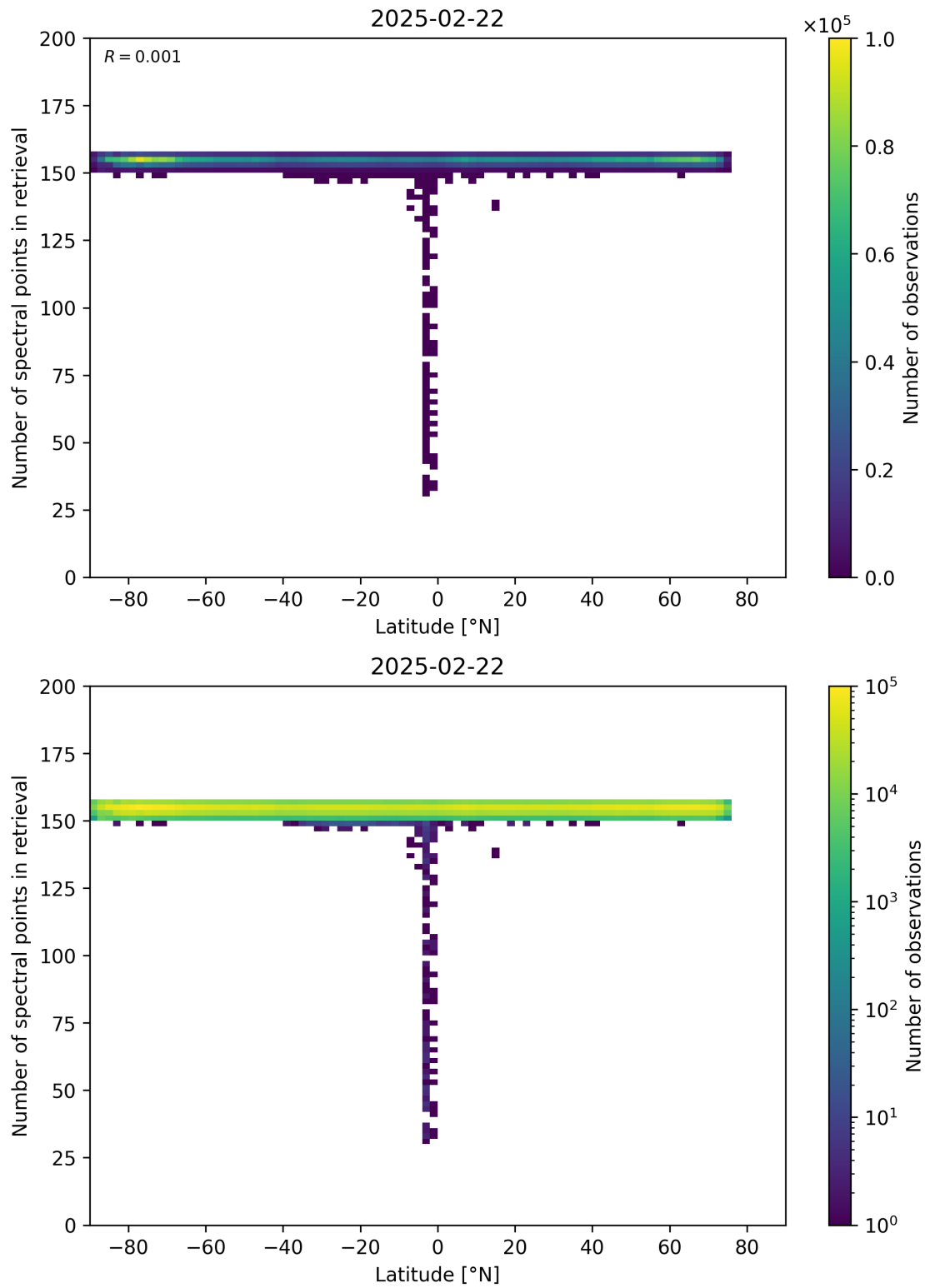
Figure 57: Scatter density plot of “Latitude” against “Number of spectral points in retrieval” for 2025-02-21 to 2025-02-23.
