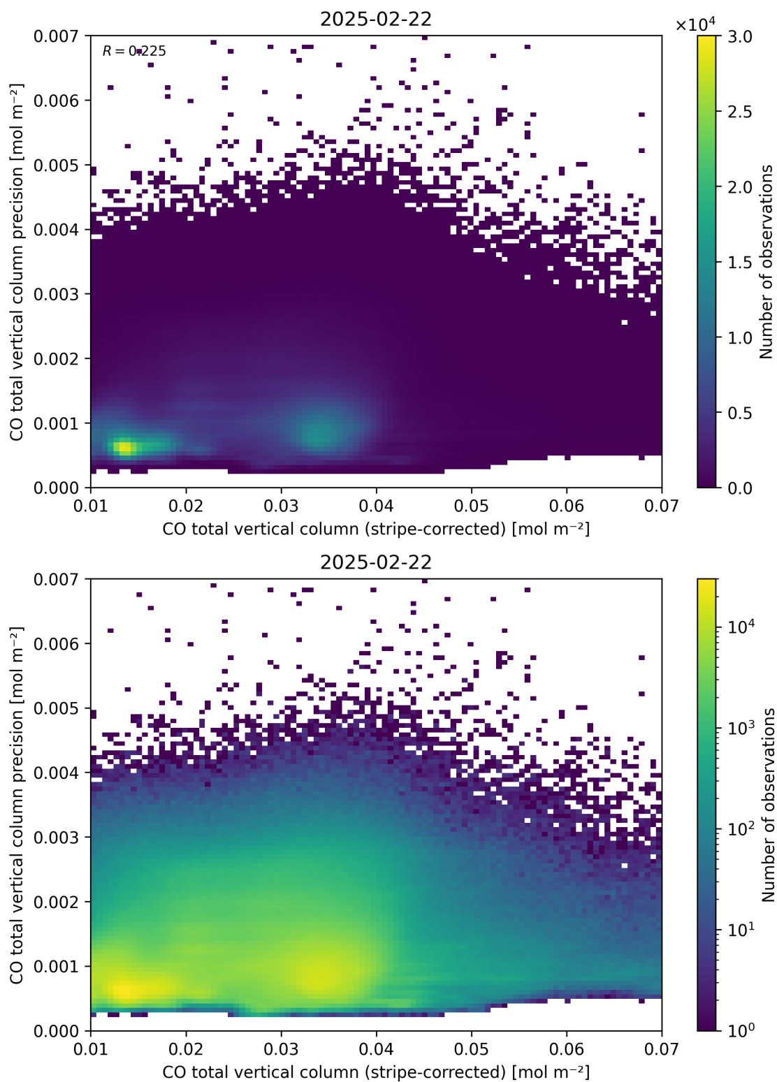
Figure 36: Scatter density plot of “CO total vertical column (stripe-corrected)” against “CO total vertical column precision” for 2025-02-21 to 2025-02-23.
