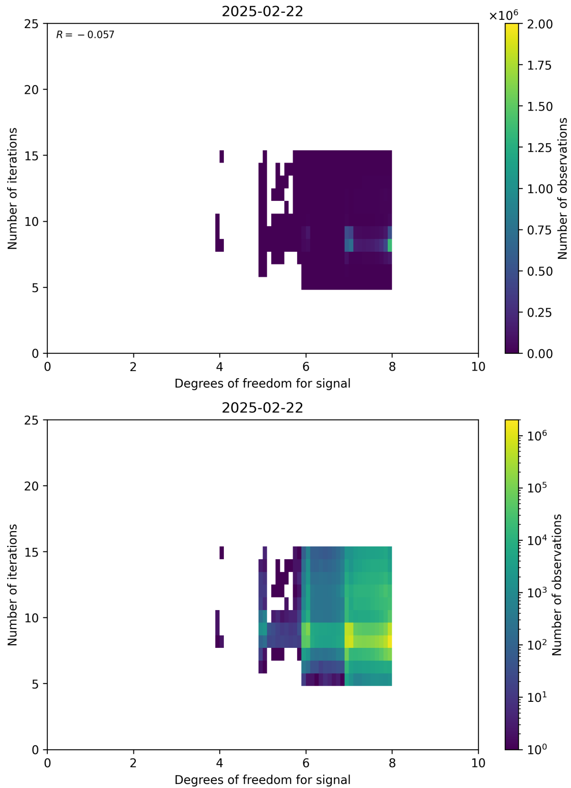
Figure 50: Scatter density plot of “Degrees of freedom for signal” against “Number of iterations” for 2025-02-21 to 2025-02-23.
