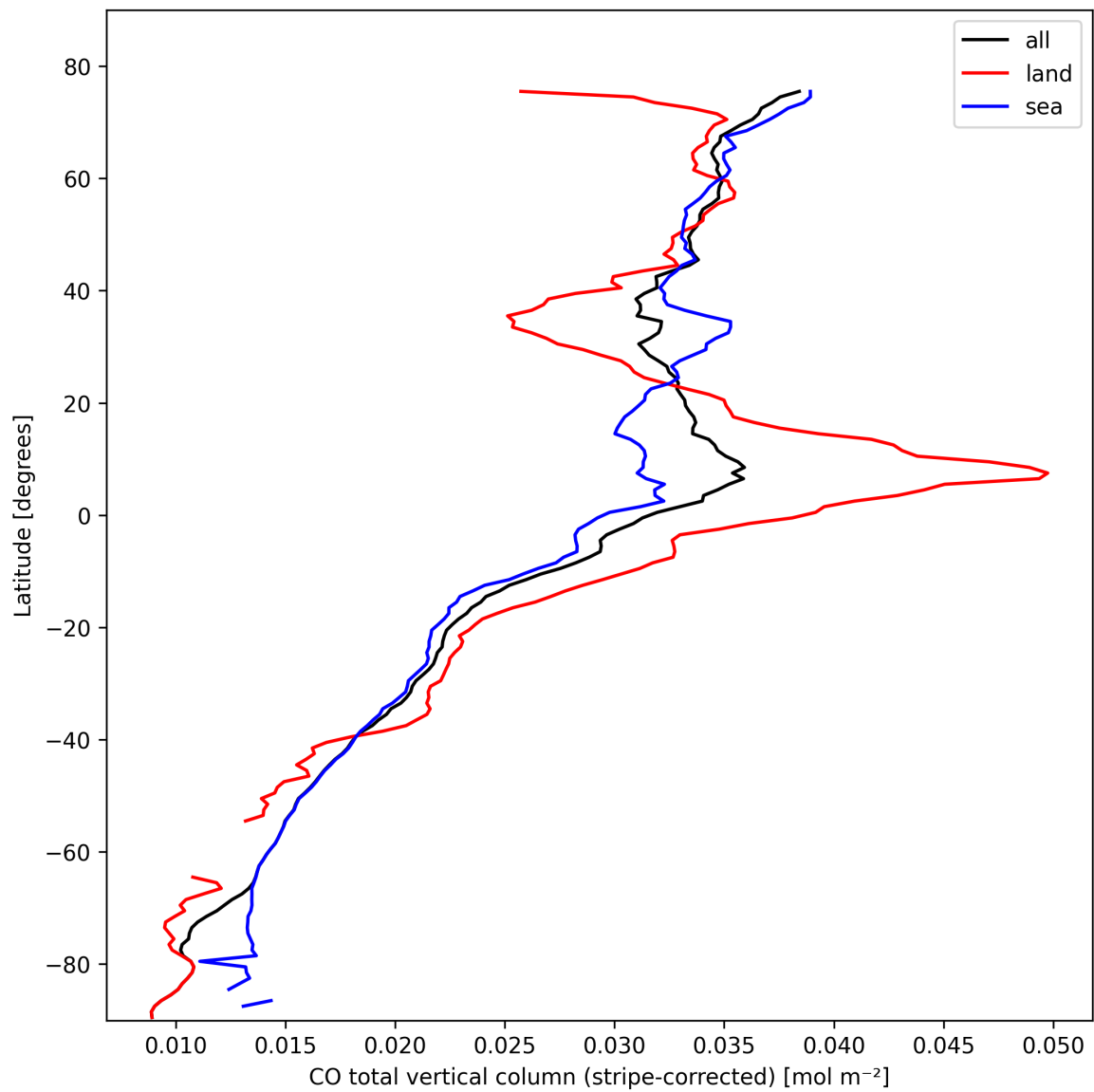
Figure 11: Zonal average of “CO total vertical column (stripe-corrected)” for 2025-02-21 to 2025-02-23.
