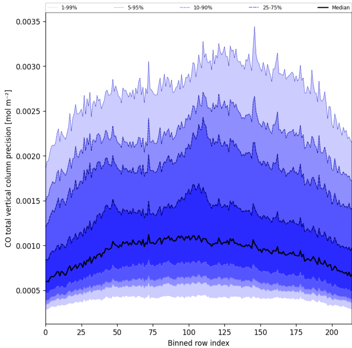
Figure 28: Along track statistics of “CO total vertical column precision” for 2025-02-21 to 2025-02-23
