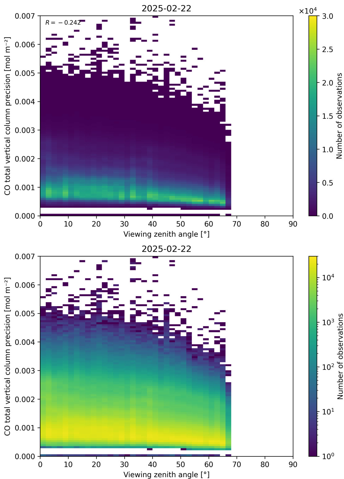
Figure 71: Scatter density plot of “Viewing zenith angle” against “CO total vertical column precision” for 2025-02-21 to 2025-02-23.
