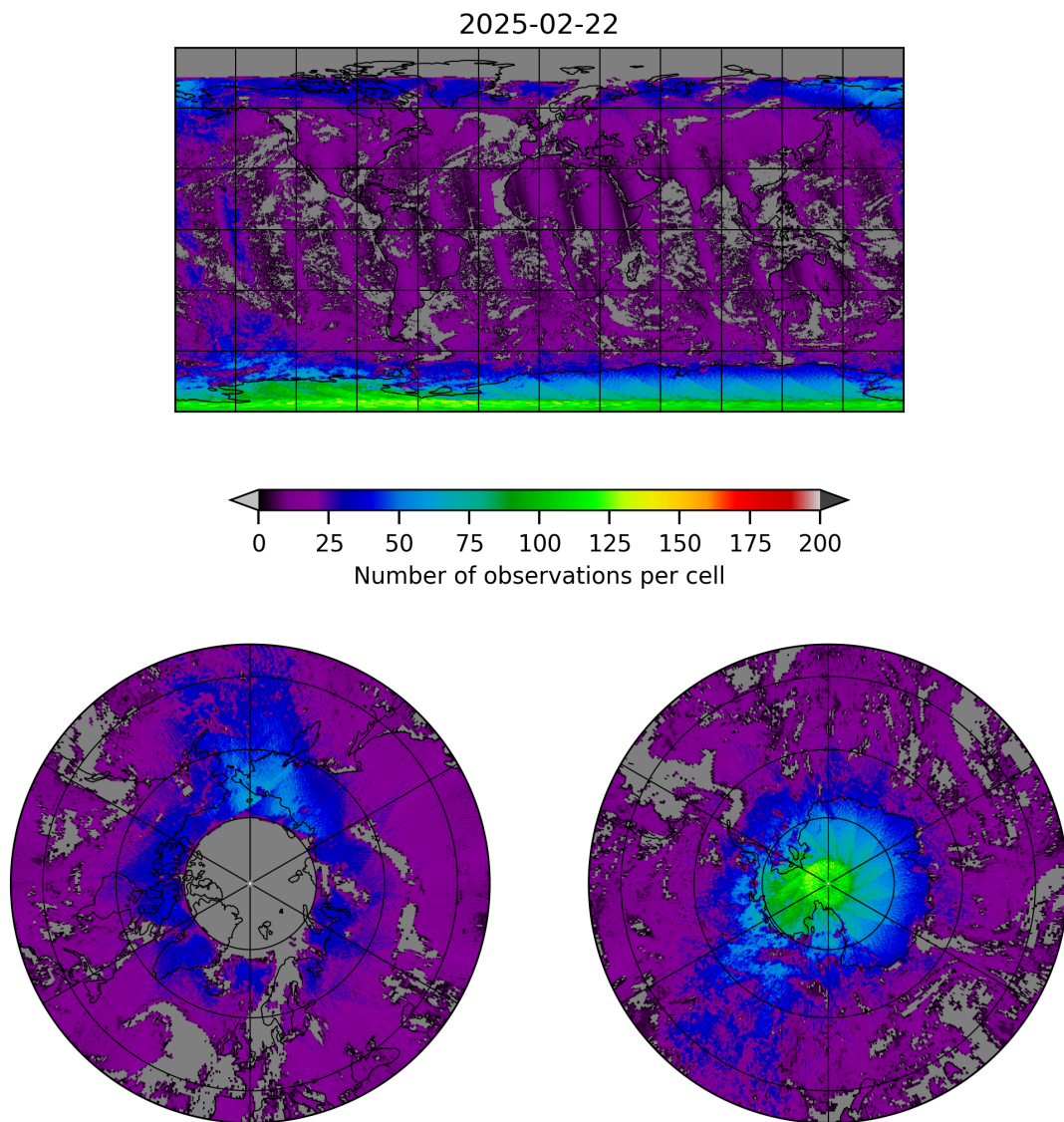
Figure 8: Map of the number of observations for 2025-02-21 to 2025-02-23
