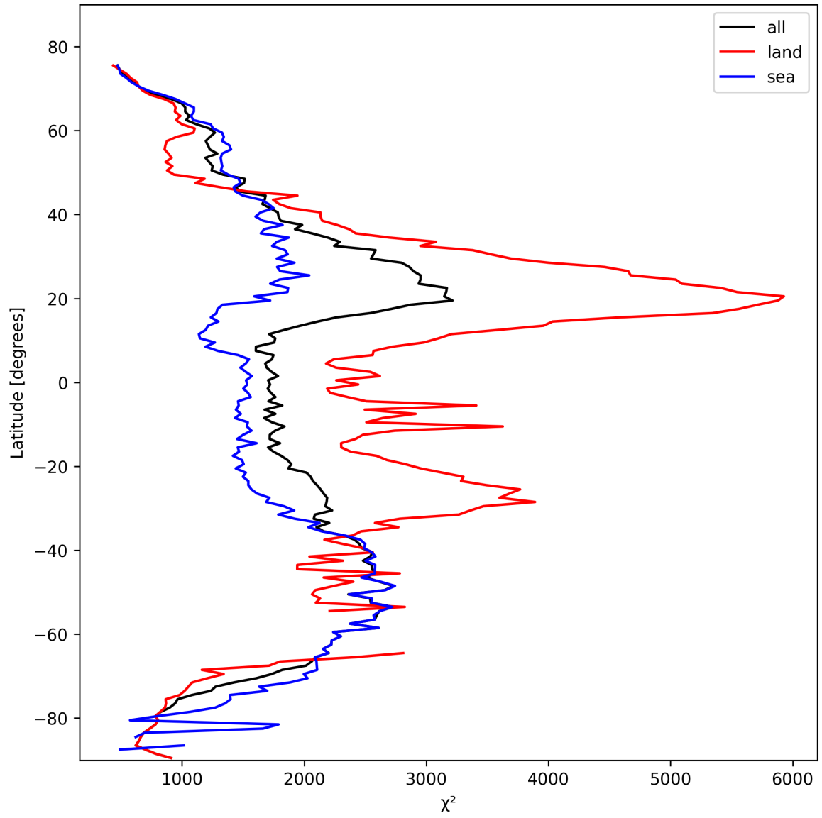
Figure 14: Zonal average of “ \chi^2 ” for 2025-02-21 to 2025-02-23.
