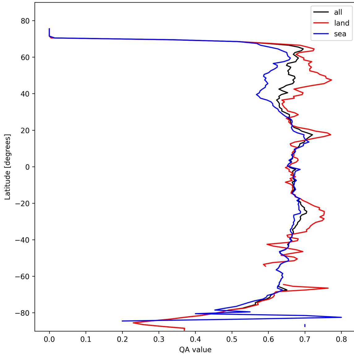
Figure 9: Zonal average of “QA value” for 2025-02-21 to 2025-02-23.
