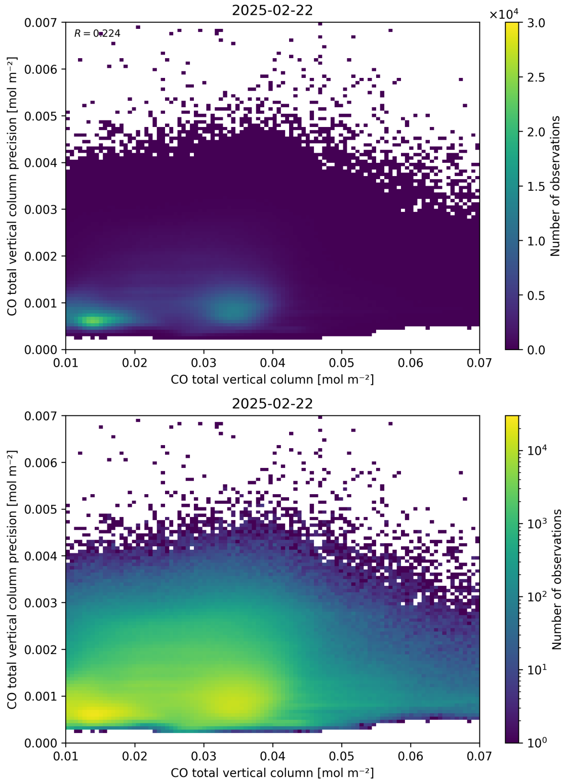
Figure 34: Scatter density plot of “CO total vertical column” against “CO total vertical column precision” for 2025-02-21 to 2025-02-23.
