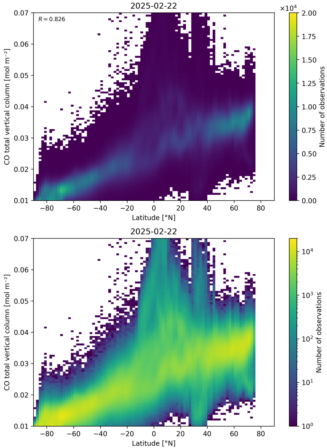
Figure 51: Scatter density plot of “Latitude” against “CO total vertical column” for 2025-02-21 to 2025-02-23.
