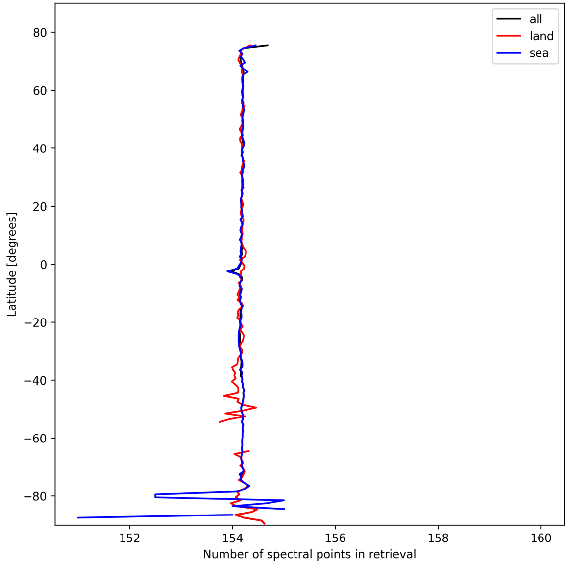
Figure 13: Zonal average of “Number of spectral points in retrieval” for 2025-02-21 to 2025-02-23.
