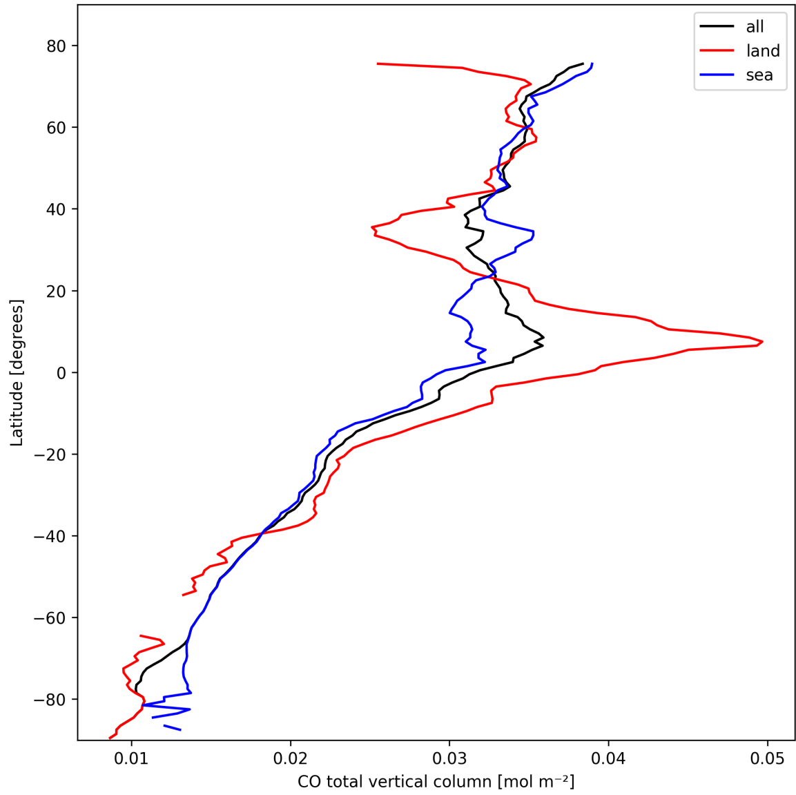
Figure 10: Zonal average of “CO total vertical column” for 2025-02-21 to 2025-02-23.
