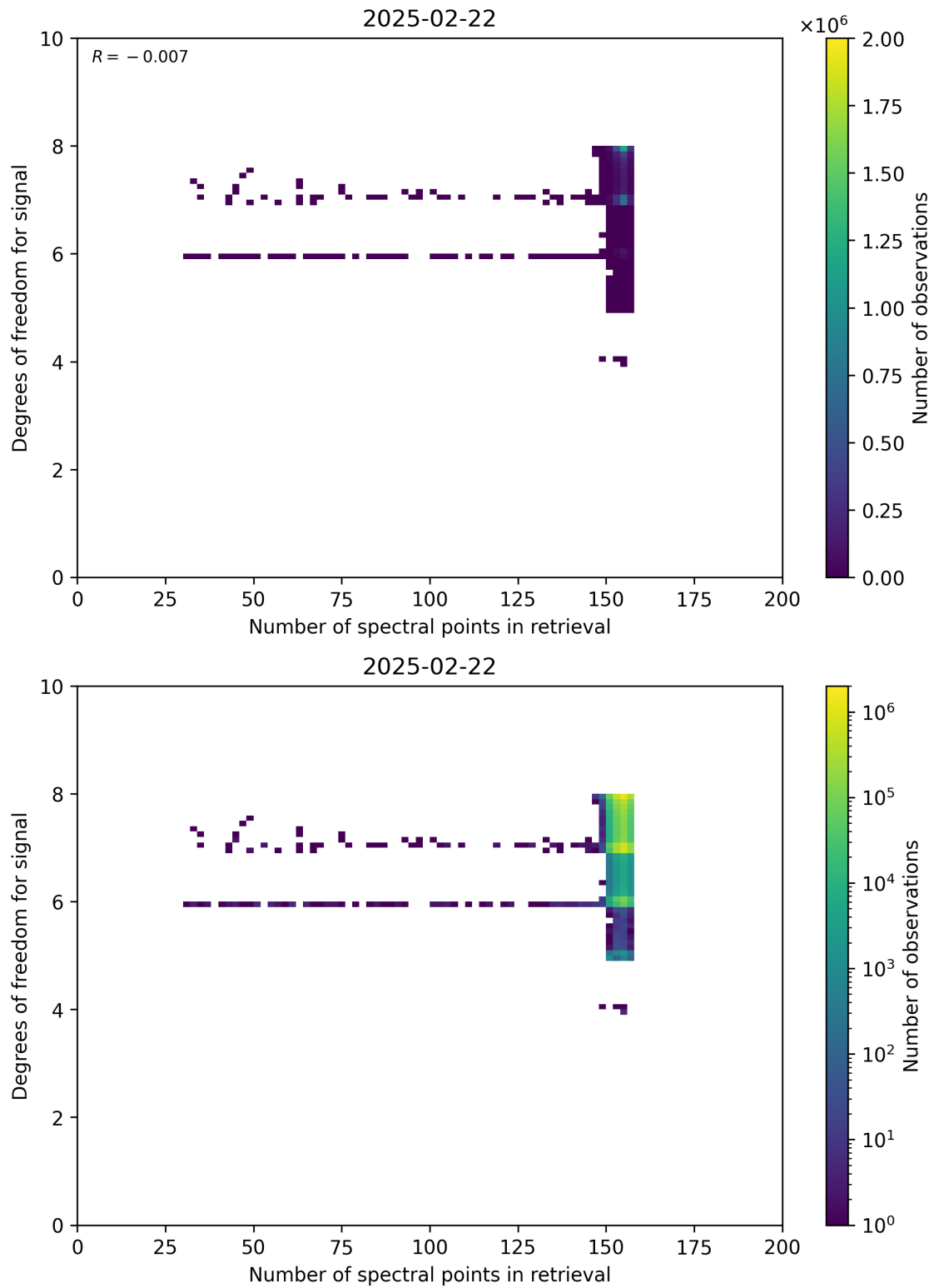
Figure 59: Scatter density plot of “Number of spectral points in retrieval” against “Degrees of freedom for signal” for 2025-02-21 to 2025-02-23.
