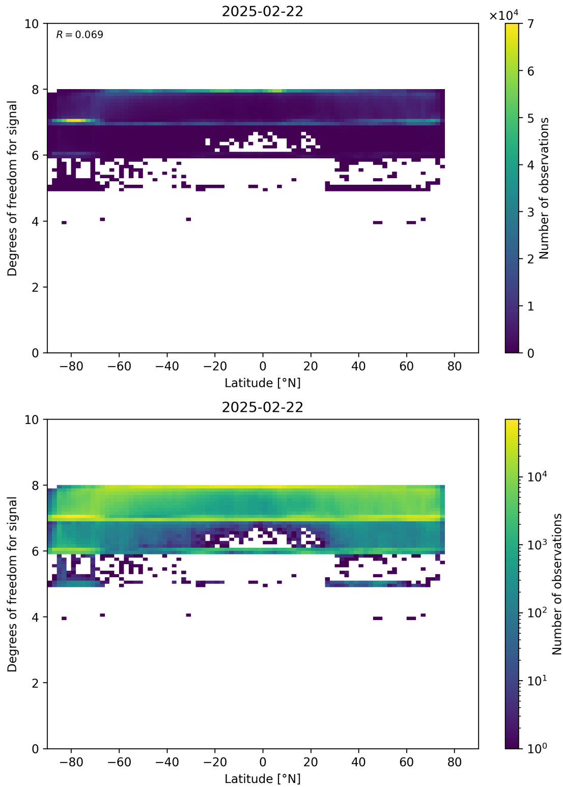
Figure 55: Scatter density plot of “Latitude” against “Degrees of freedom for signal” for 2025-02-21 to 2025-02-23.
