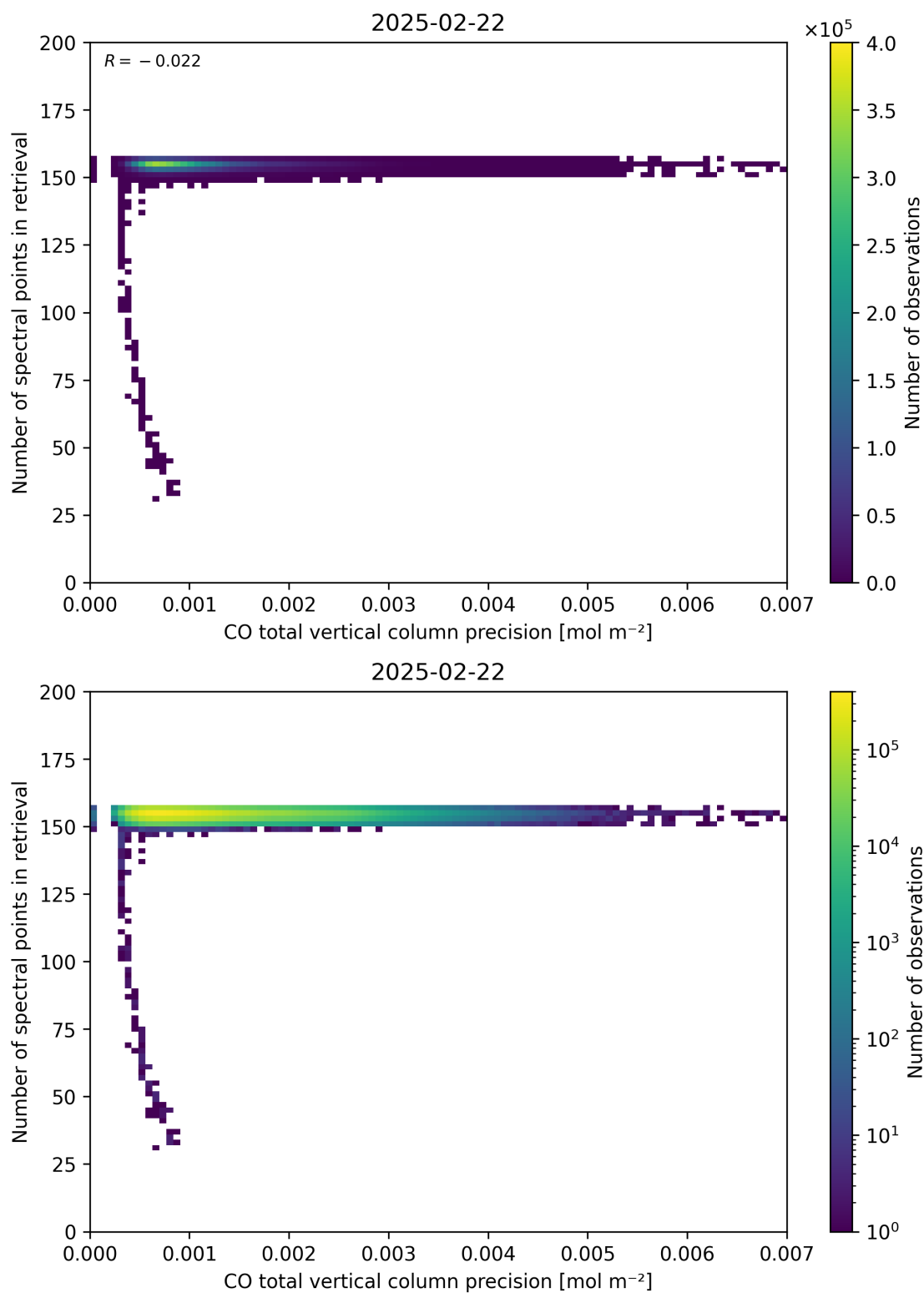
Figure 47: Scatter density plot of “CO total vertical column precision” against “Number of spectral points in retrieval” for 2025-02-21 to 2025-02-23.
