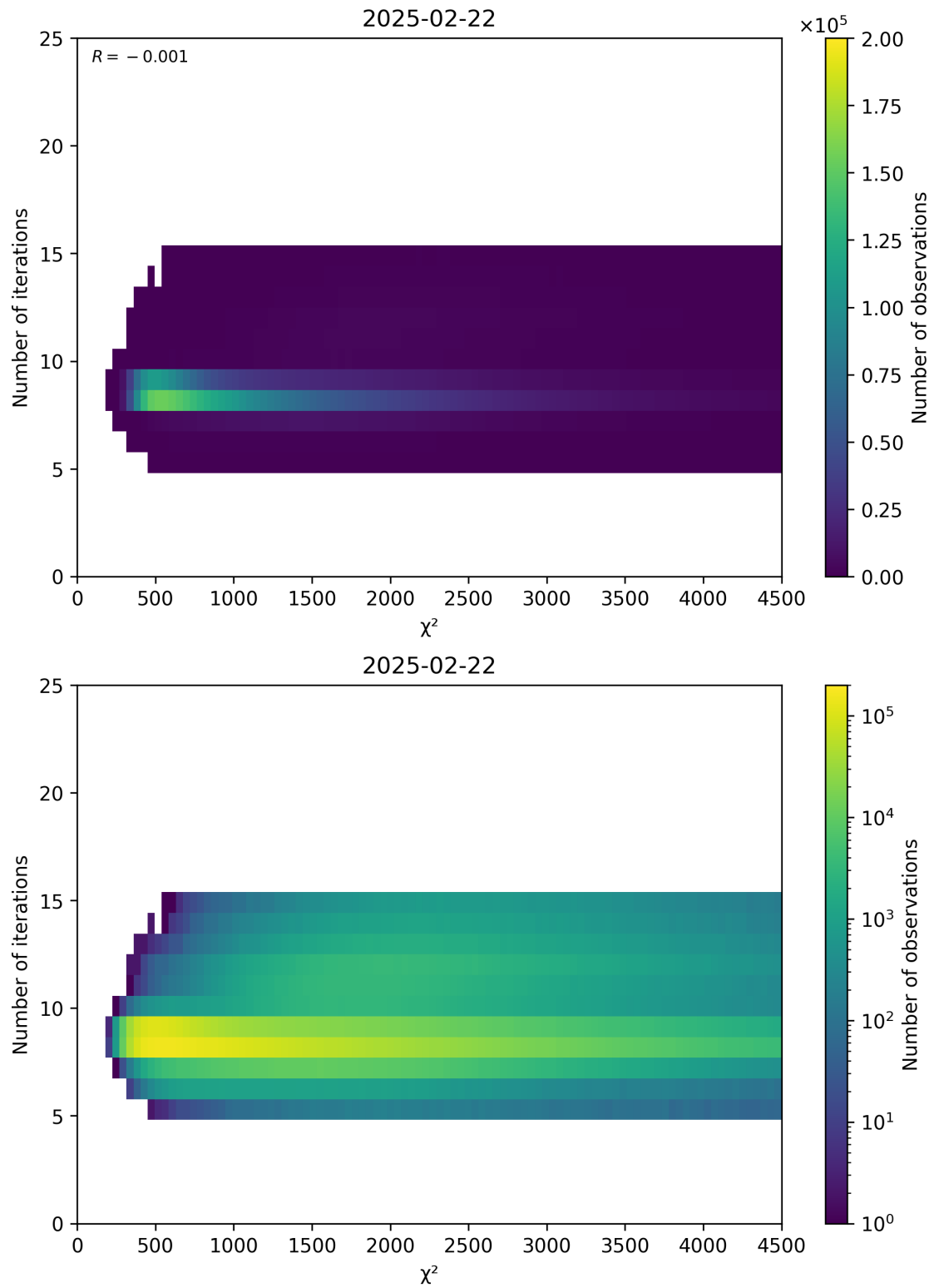
Figure 49: Scatter density plot of “ \chi^2 ” against “Number of iterations” for 2025-02-21 to 2025-02-23.
