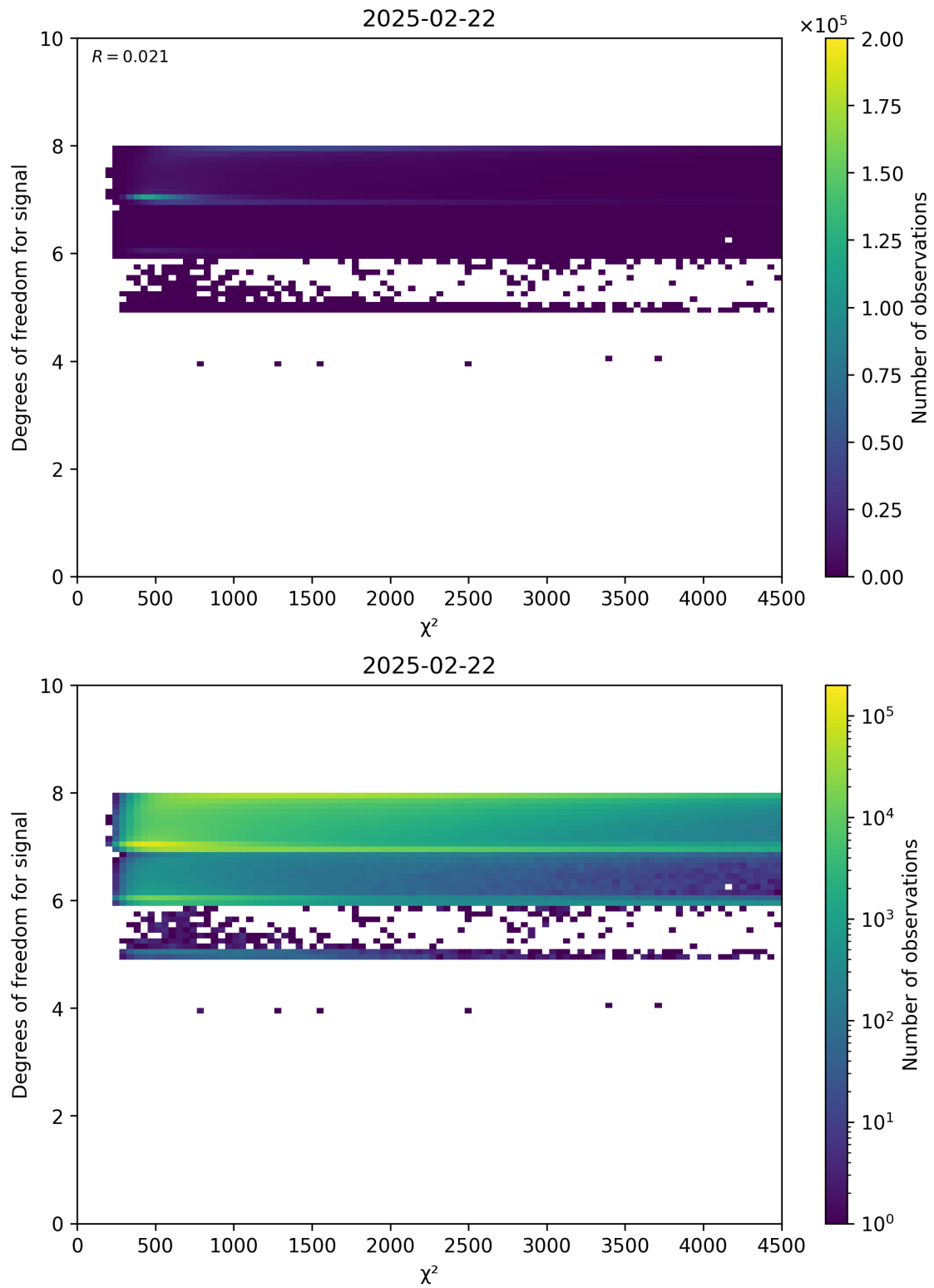
Figure 48: Scatter density plot of “ \chi^2 ” against “Degrees of freedom for signal” for 2025-02-21 to 2025-02-23.
