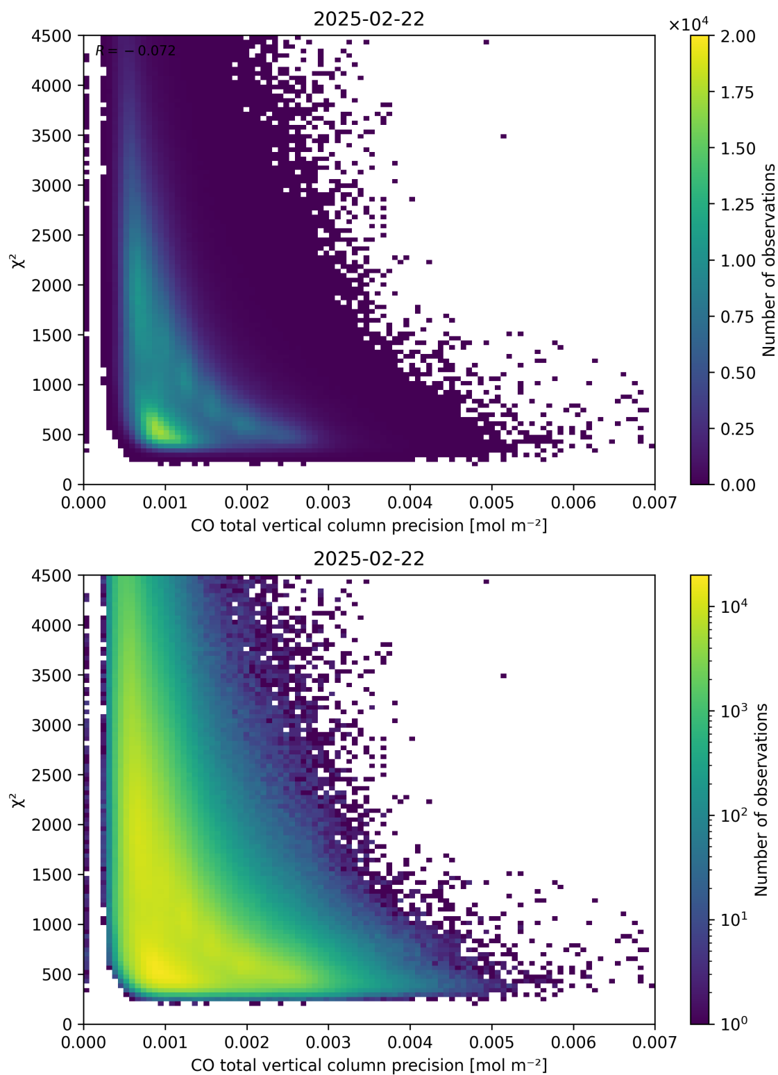
Figure 44: Scatter density plot of “CO total vertical column precision” against “ \chi^2 ” for 2025-02-21 to 2025-02-23.
