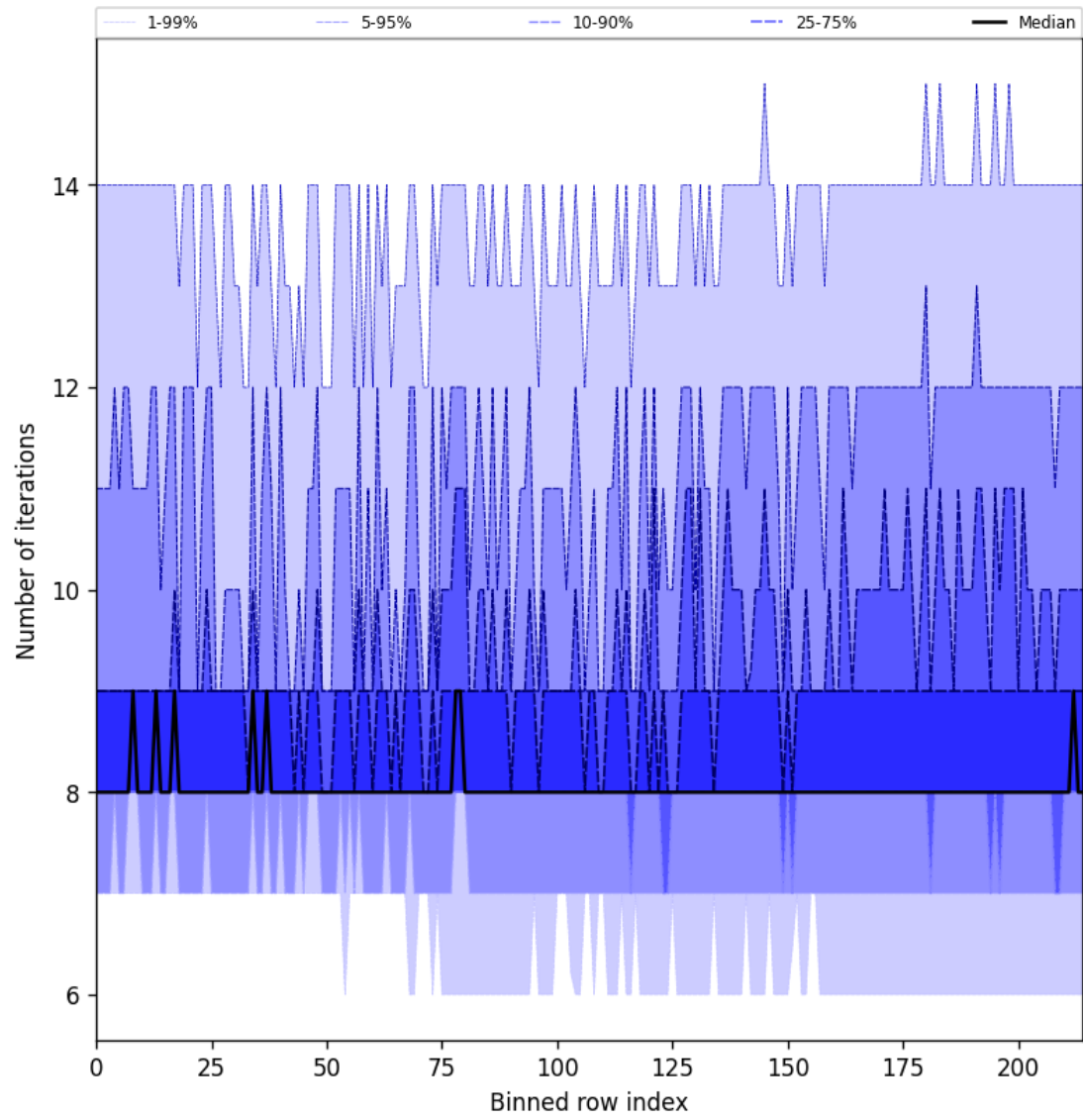
Figure 32: Along track statistics of “Number of iterations” for 2025-02-21 to 2025-02-23
