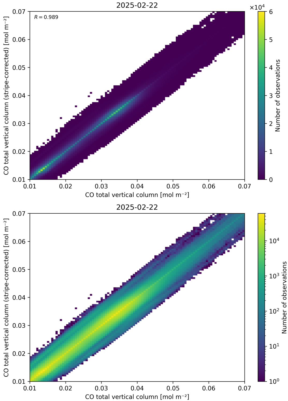
Figure 33: Scatter density plot of “CO total vertical column” against “CO total vertical column (stripe-corrected)” for 2025-02-21 to 2025-02-23.
