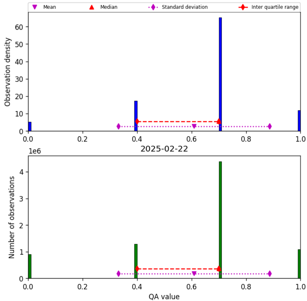
Figure 17: Histogram of “QA value” for 2025-02-21 to 2025-02-23
