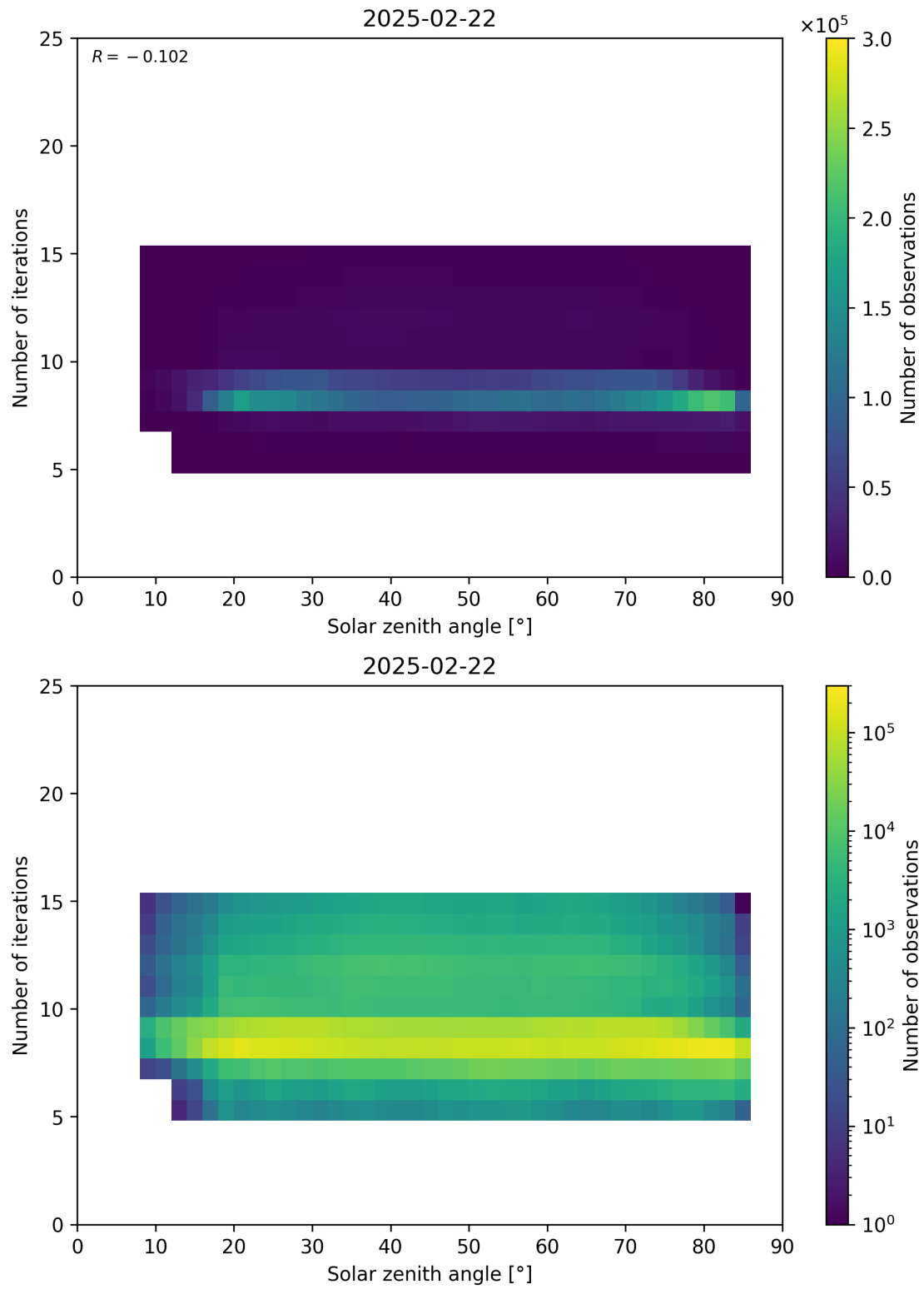
Figure 67: Scatter density plot of “Solar zenith angle” against “Number of iterations” for 2025-02-21 to 2025-02-23.
