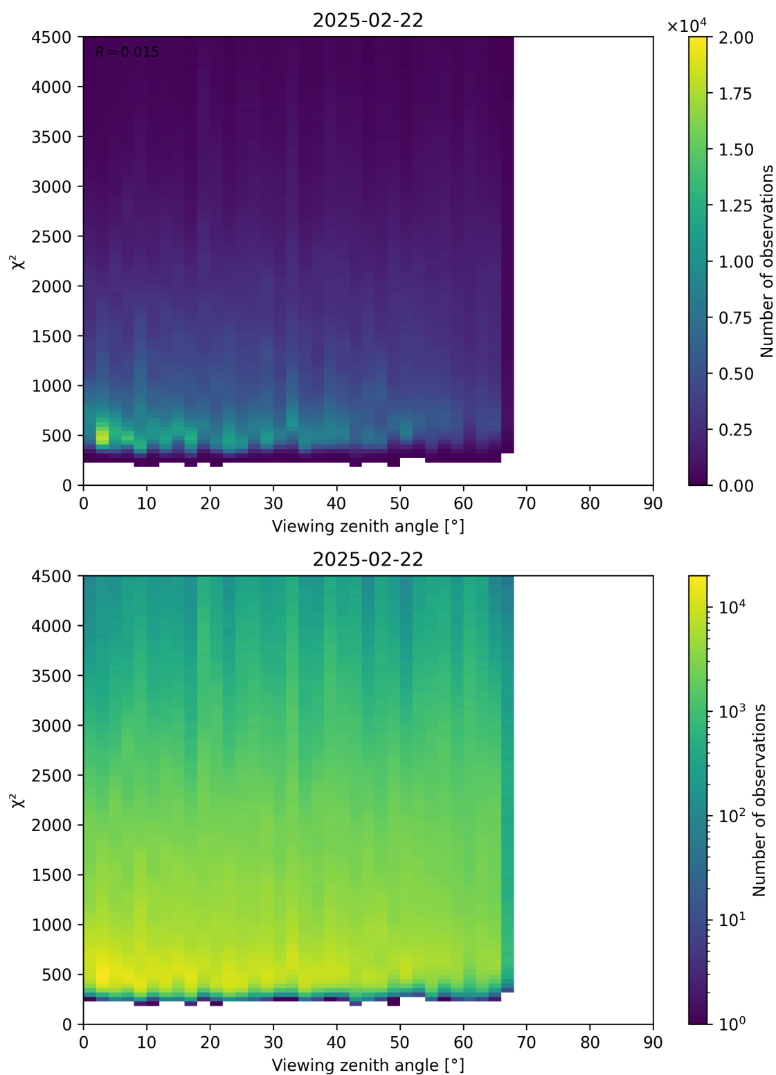
Figure 72: Scatter density plot of “Viewing zenith angle” against “ \chi^2 ” for 2025-02-21 to 2025-02-23.
