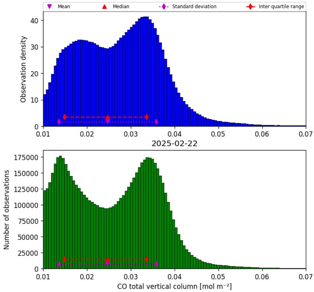
Figure 18: Histogram of “CO total vertical column” for 2025-02-21 to 2025-02-23
