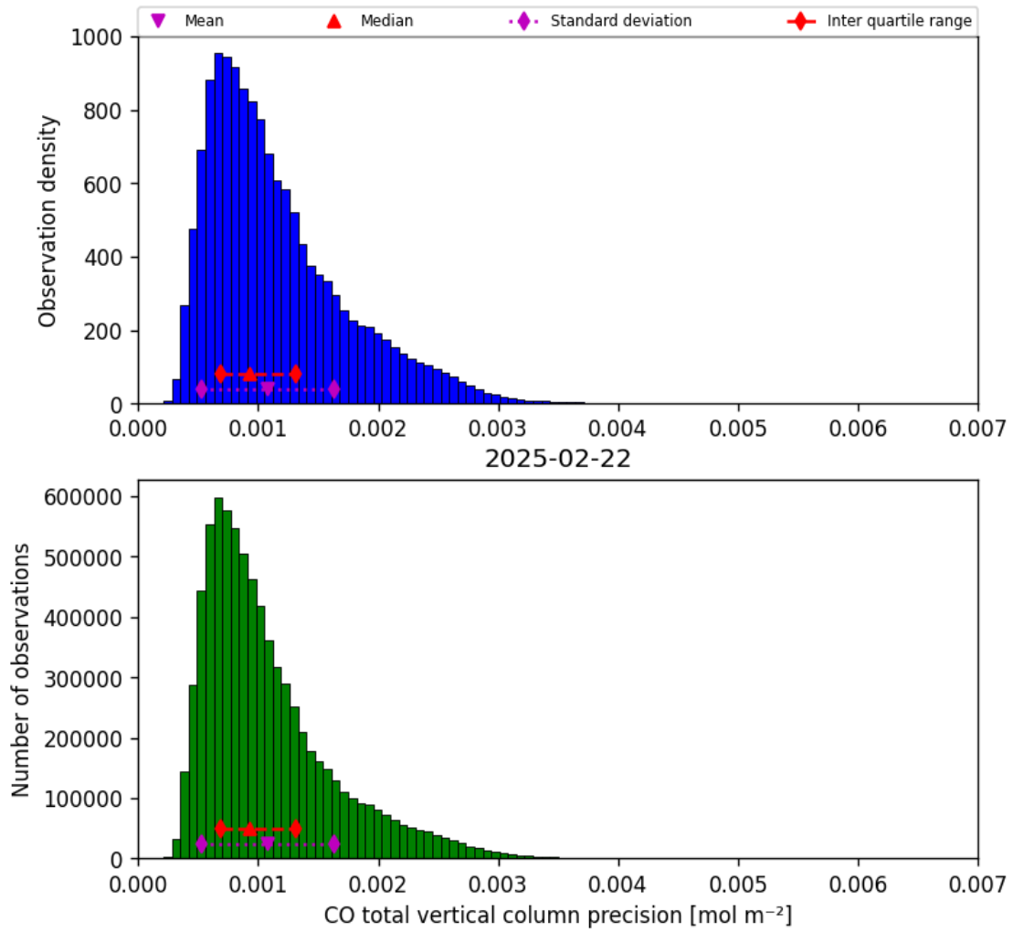
Figure 20: Histogram of “CO total vertical column precision” for 2025-02-21 to 2025-02-23
