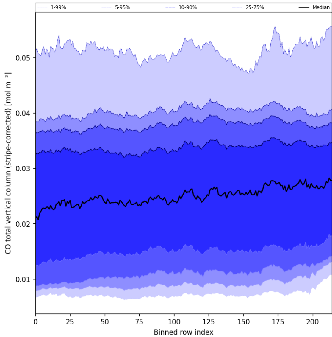
Figure 27: Along track statistics of “CO total vertical column (stripe-corrected)” for 2025-02-21 to 2025-02-23
