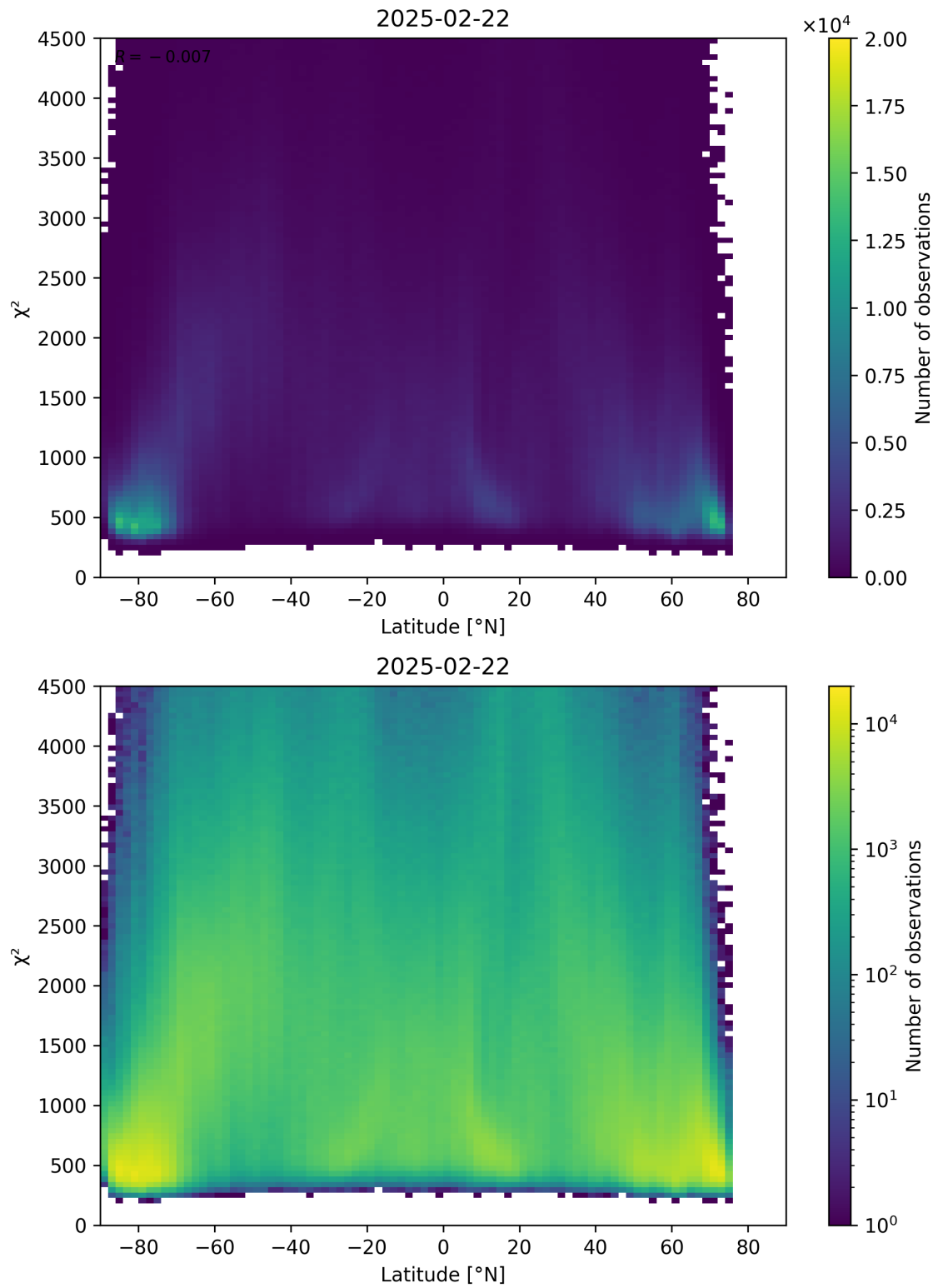
Figure 54: Scatter density plot of “Latitude” against “ \chi^2 ” for 2025-02-21 to 2025-02-23.
