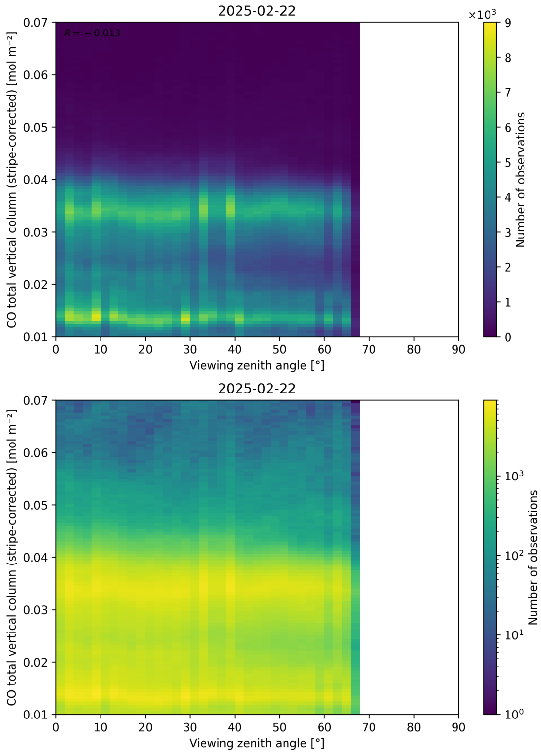
Figure 70: Scatter density plot of “Viewing zenith angle” against “CO total vertical column (stripe-corrected)” for 2025-02-21 to 2025-02-23.
