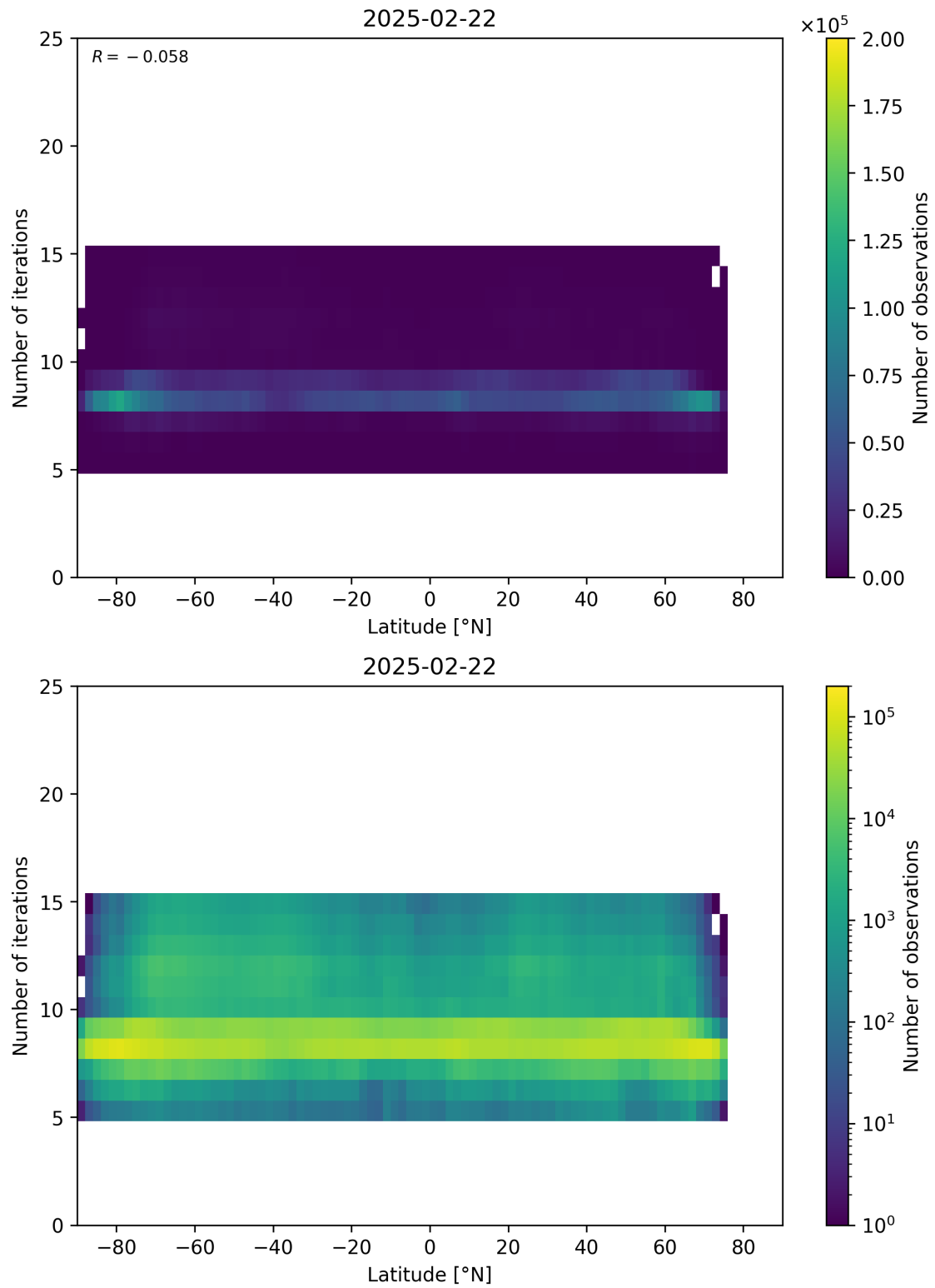
Figure 56: Scatter density plot of “Latitude” against “Number of iterations” for 2025-02-21 to 2025-02-23.
