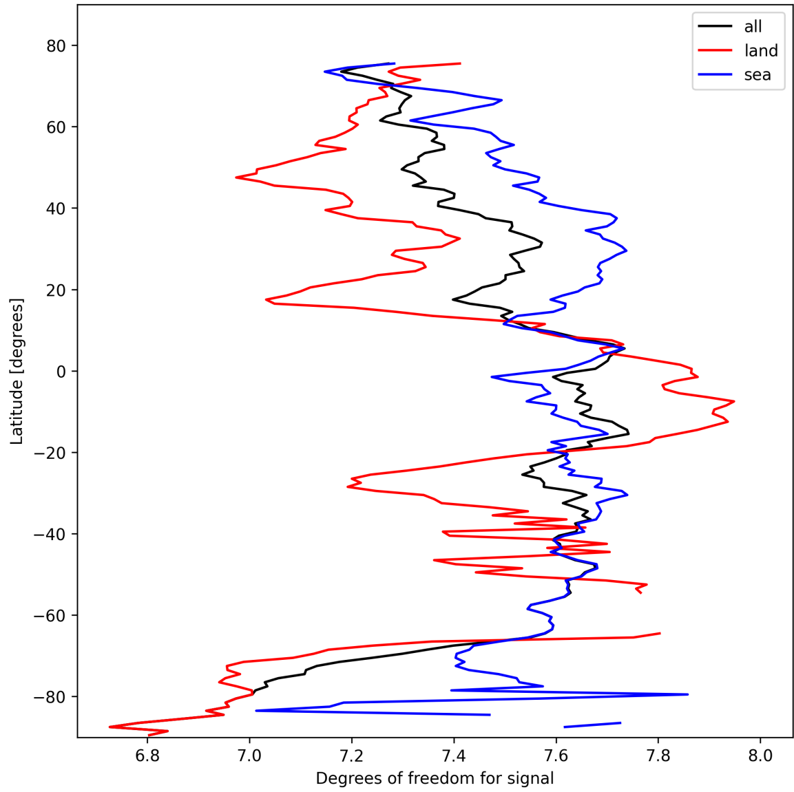
Figure 15: Zonal average of “Degrees of freedom for signal” for 2025-02-21 to 2025-02-23.
