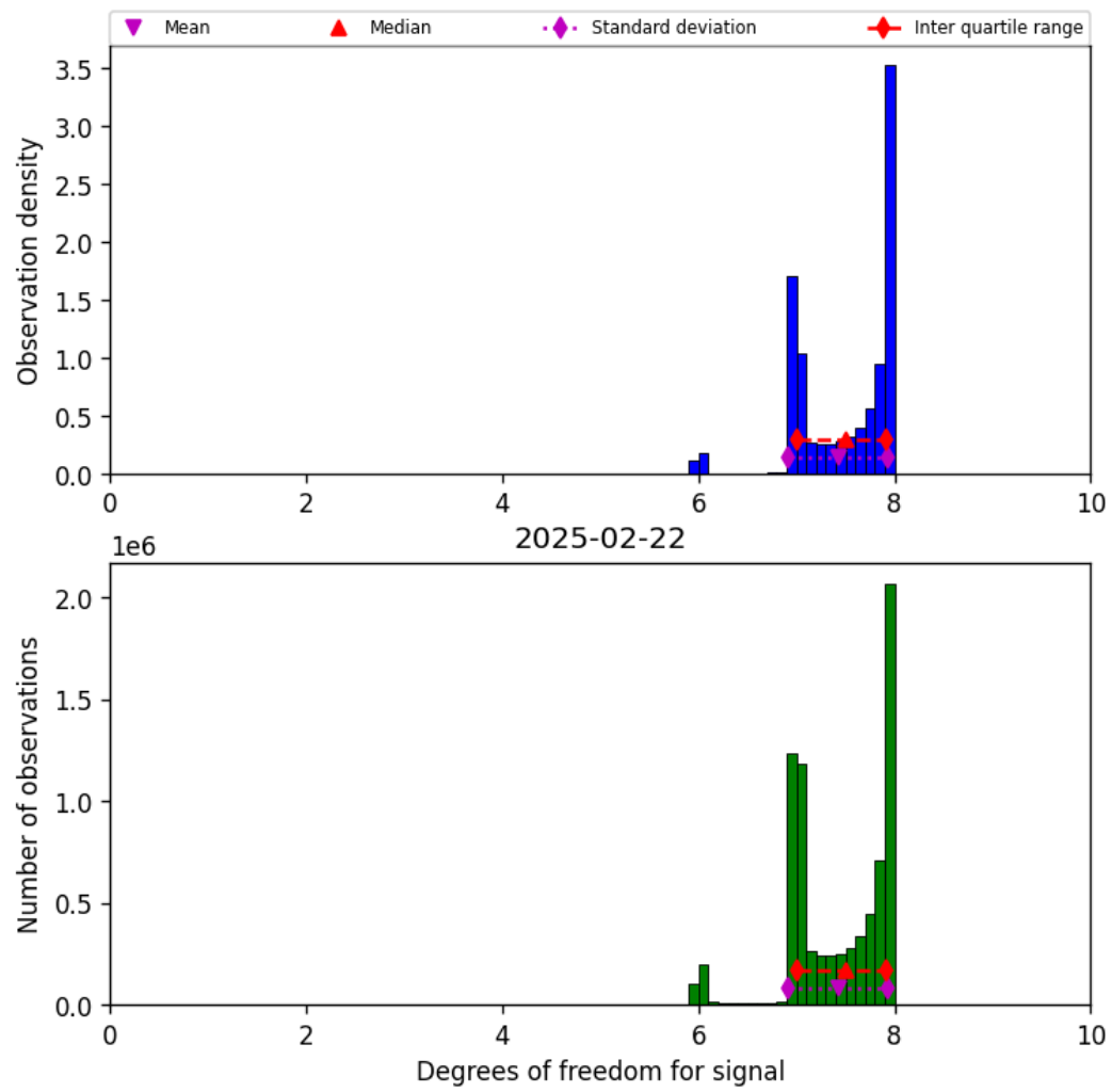
Figure 23: Histogram of “Degrees of freedom for signal” for 2025-02-21 to 2025-02-23
