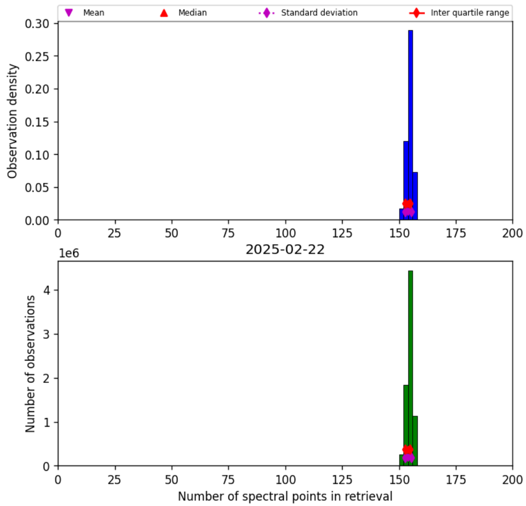
Figure 21: Histogram of “Number of spectral points in retrieval” for 2025-02-21 to 2025-02-23
