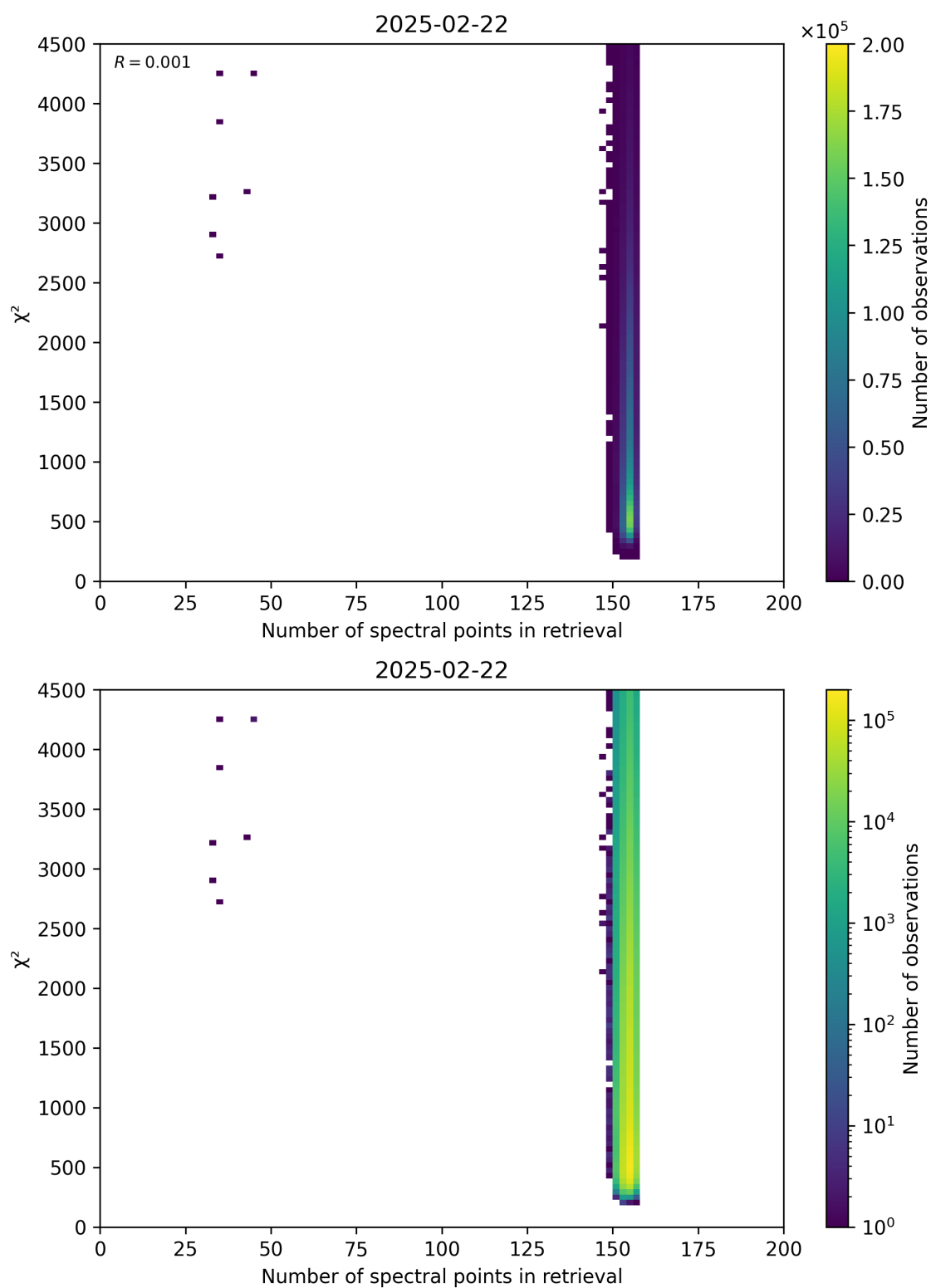
Figure 58: Scatter density plot of “Number of spectral points in retrieval” against “ \chi^2 ” for 2025-02-21 to 2025-02-23.
