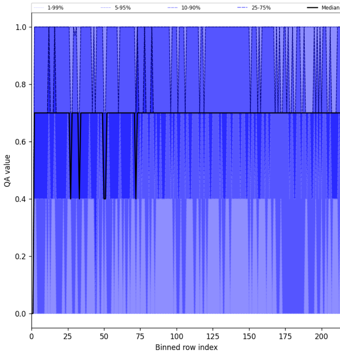
Figure 25: Along track statistics of “QA value” for 2025-02-21 to 2025-02-23
