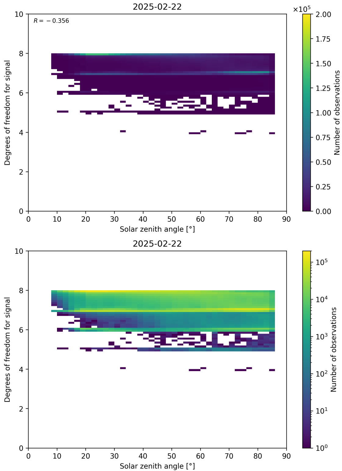
Figure 65: Scatter density plot of “Solar zenith angle” against “Degrees of freedom for signal” for 2025-02-21 to 2025-02-23.
