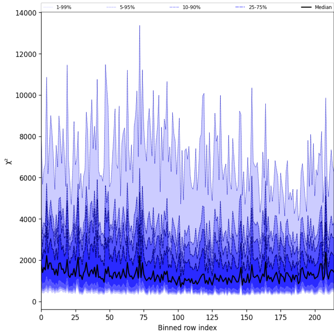
Figure 30: Along track statistics of “ \chi^2 ” for 2025-02-21 to 2025-02-23
