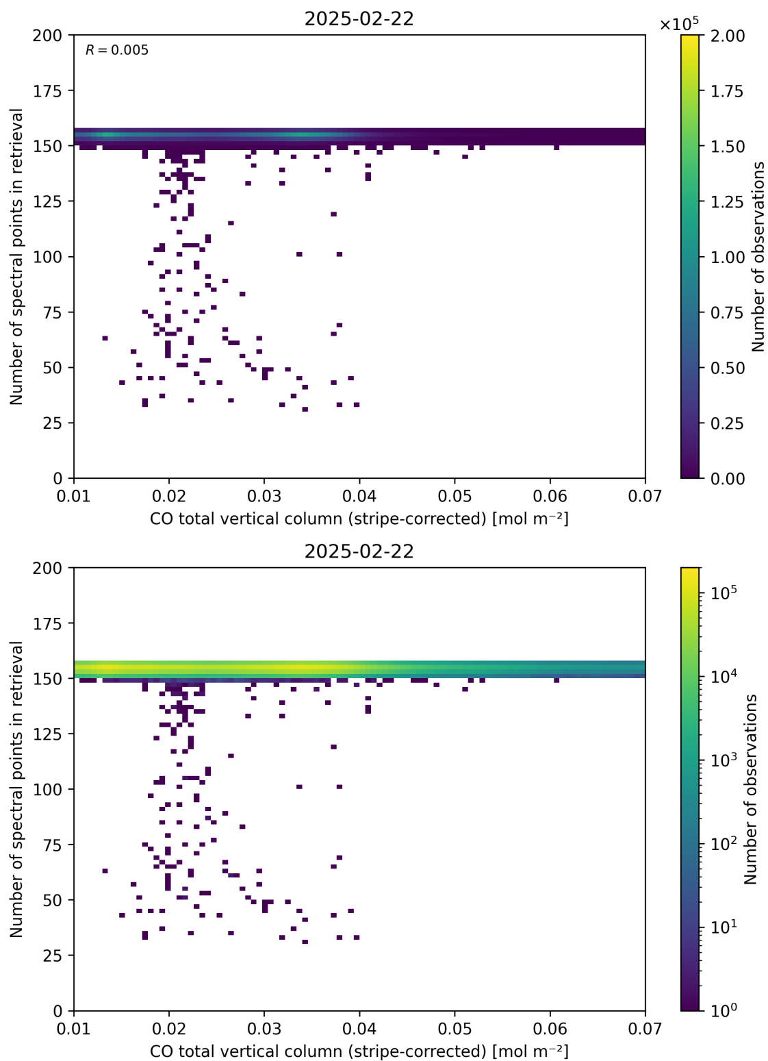
Figure 40: Scatter density plot of “CO total vertical column (stripe-corrected)” against “Number of spectral points in retrieval” for 2025-02-21 to 2025-02-23.
