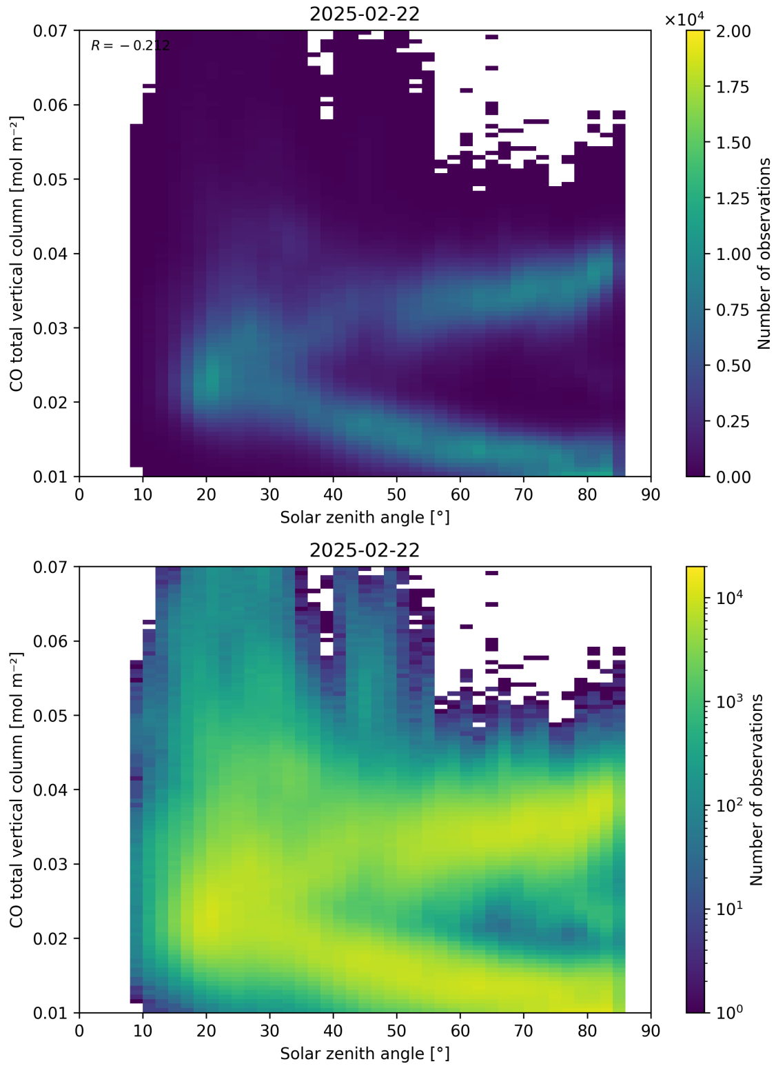
Figure 61: Scatter density plot of “Solar zenith angle” against “CO total vertical column” for 2025-02-21 to 2025-02-23.
