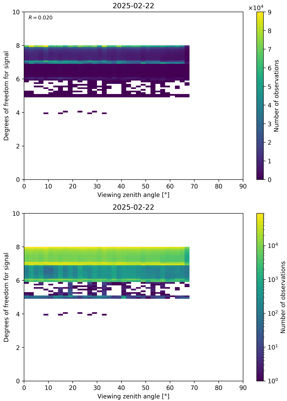
Figure 73: Scatter density plot of “Viewing zenith angle” against “Degrees of freedom for signal” for 2025-02-21 to 2025-02-23.
