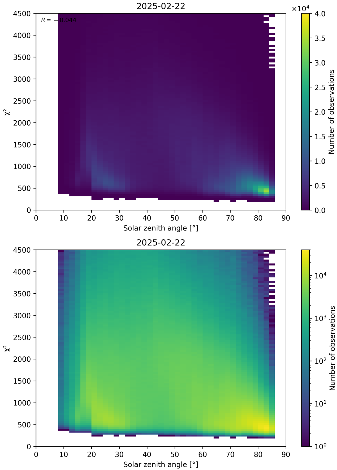
Figure 64: Scatter density plot of “Solar zenith angle” against “ \chi^2 ” for 2025-02-21 to 2025-02-23.
