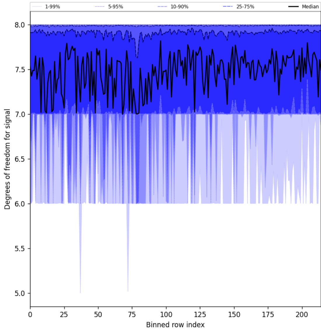
Figure 31: Along track statistics of “Degrees of freedom for signal” for 2025-02-21 to 2025-02-23
