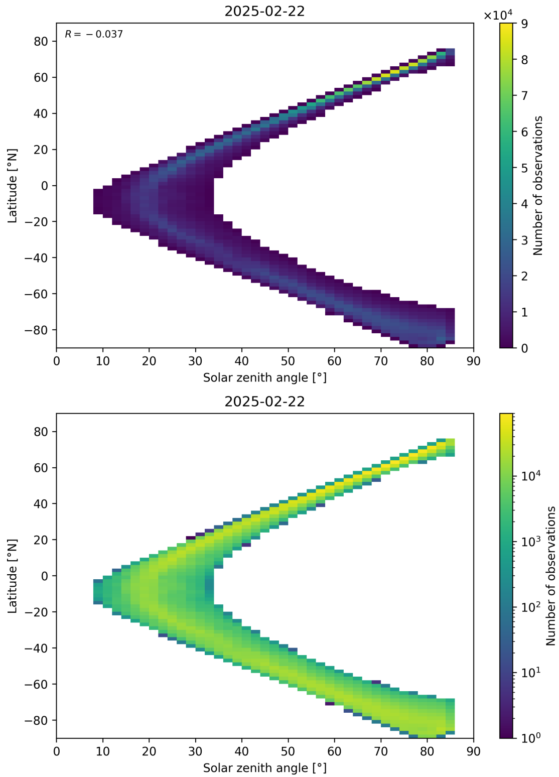
Figure 66: Scatter density plot of “Solar zenith angle” against “Latitude” for 2025-02-21 to 2025-02-23.
