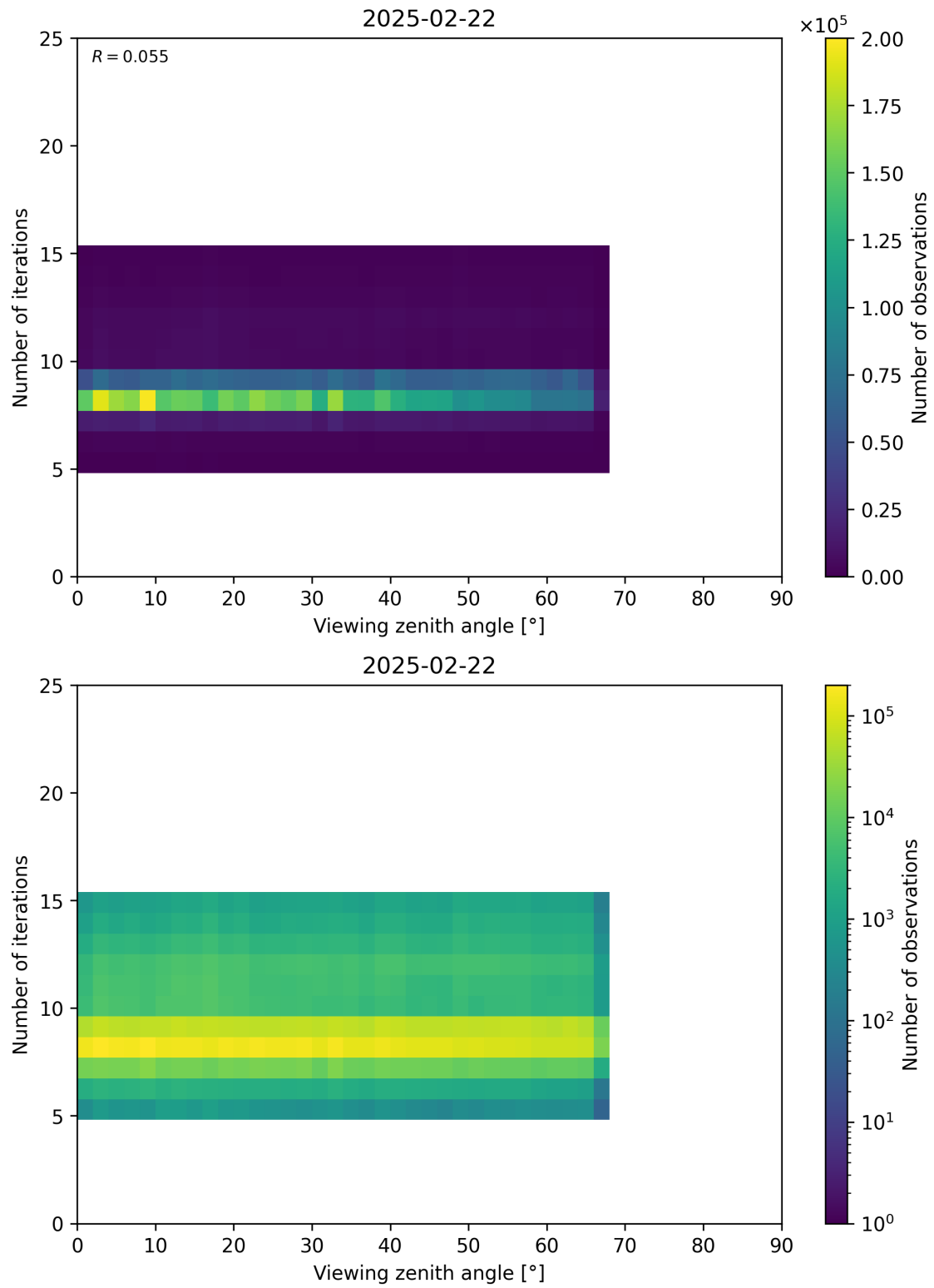
Figure 75: Scatter density plot of “Viewing zenith angle” against “Number of iterations” for 2025-02-21 to 2025-02-23.
