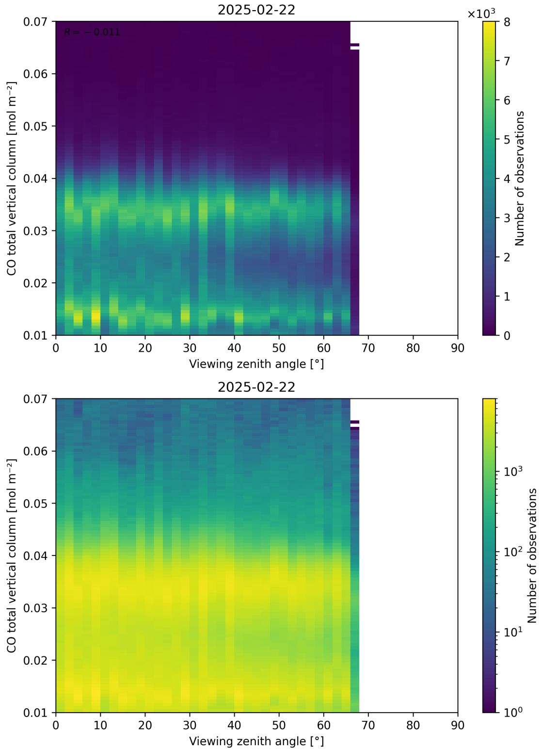
Figure 69: Scatter density plot of “Viewing zenith angle” against “CO total vertical column” for 2025-02-21 to 2025-02-23.
