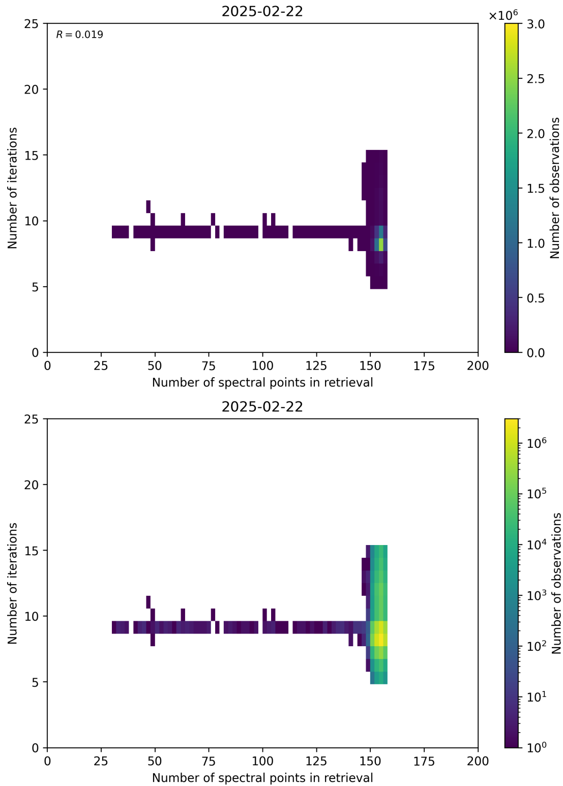
Figure 60: Scatter density plot of “Number of spectral points in retrieval” against “Number of iterations” for 2025-02-21 to 2025-02-23.
