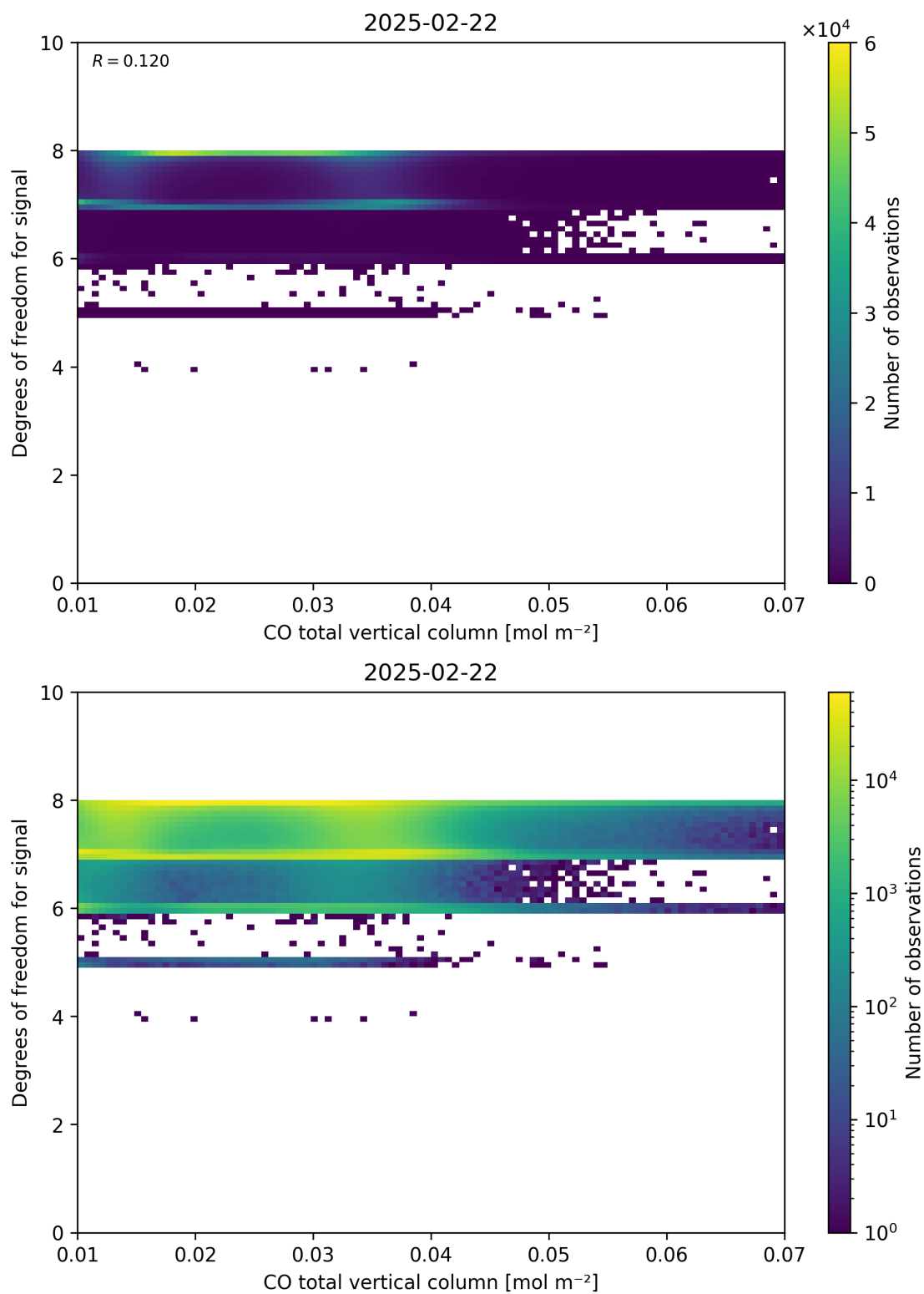
Figure 41: Scatter density plot of “CO total vertical column” against “Degrees of freedom for signal” for 2025-02-21 to 2025-02-23.
