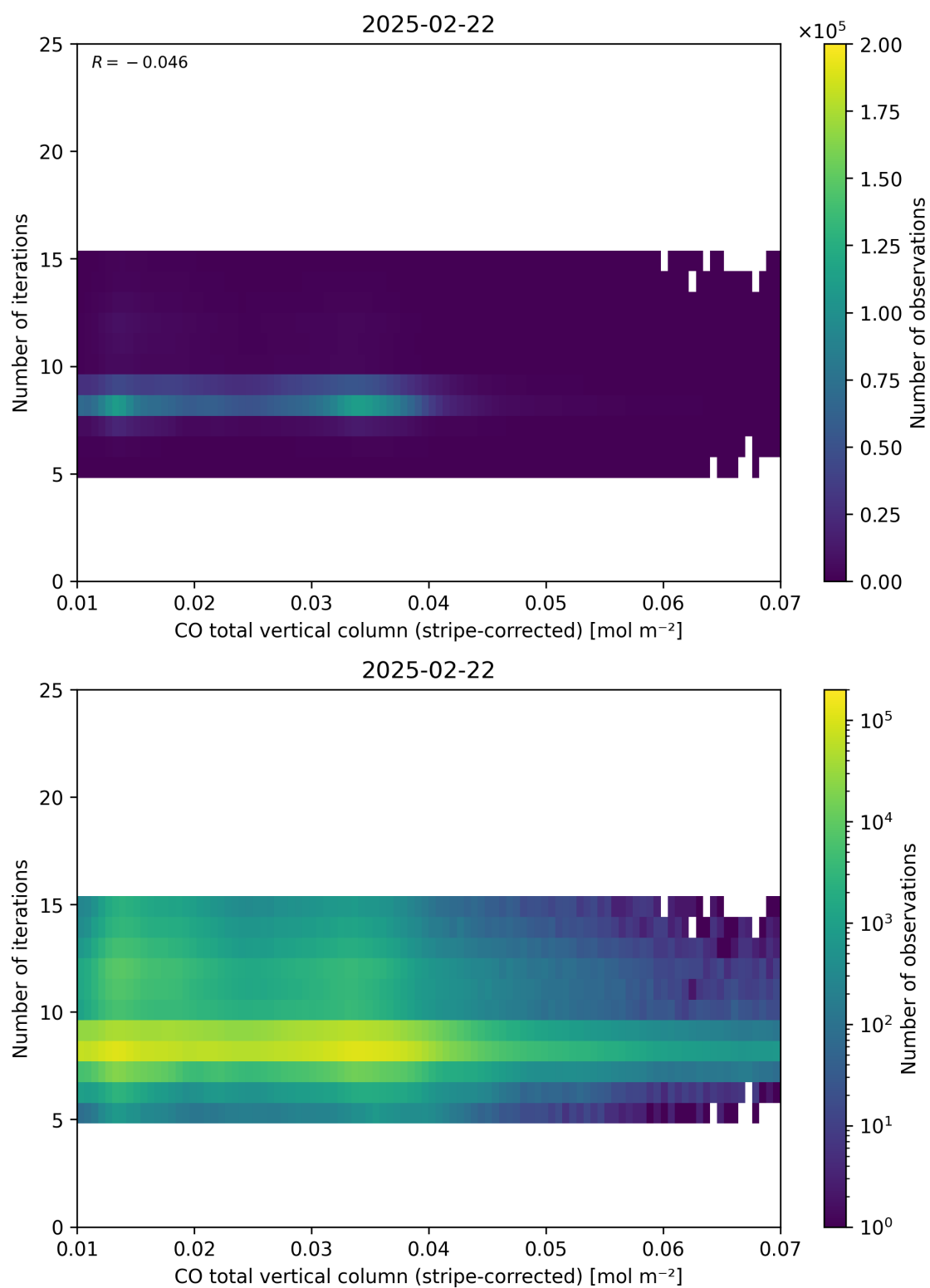
Figure 39: Scatter density plot of “CO total vertical column (stripe-corrected)” against “Number of iterations” for 2025-02-21 to 2025-02-23.
