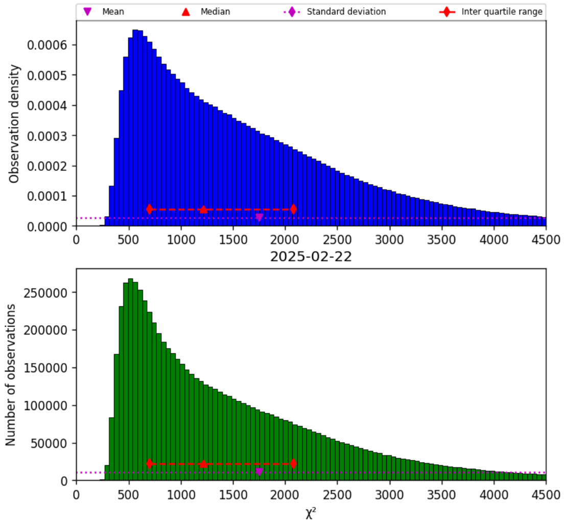
Figure 22: Histogram of “ \chi^2 ” for 2025-02-21 to 2025-02-23
