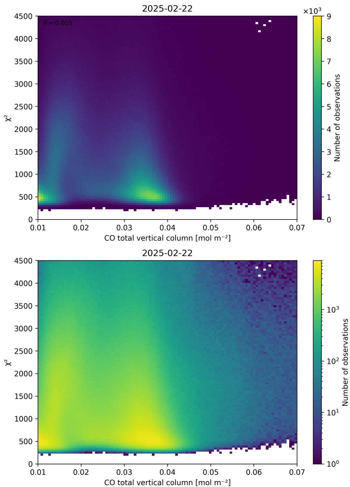
Figure 35: Scatter density plot of “CO total vertical column” against “ \chi^2 ” for 2025-02-21 to 2025-02-23.
