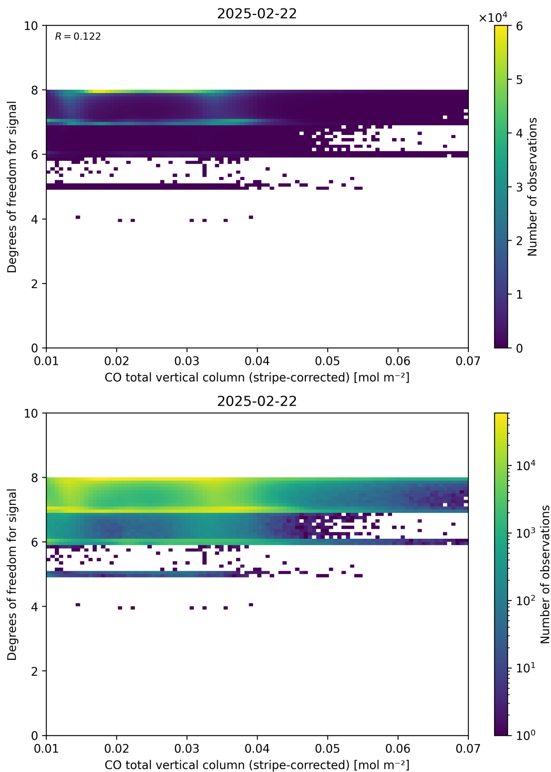
Figure 38: Scatter density plot of “CO total vertical column (stripe-corrected)” against “Degrees of freedom for signal” for 2025-02-21 to 2025-02-23.
