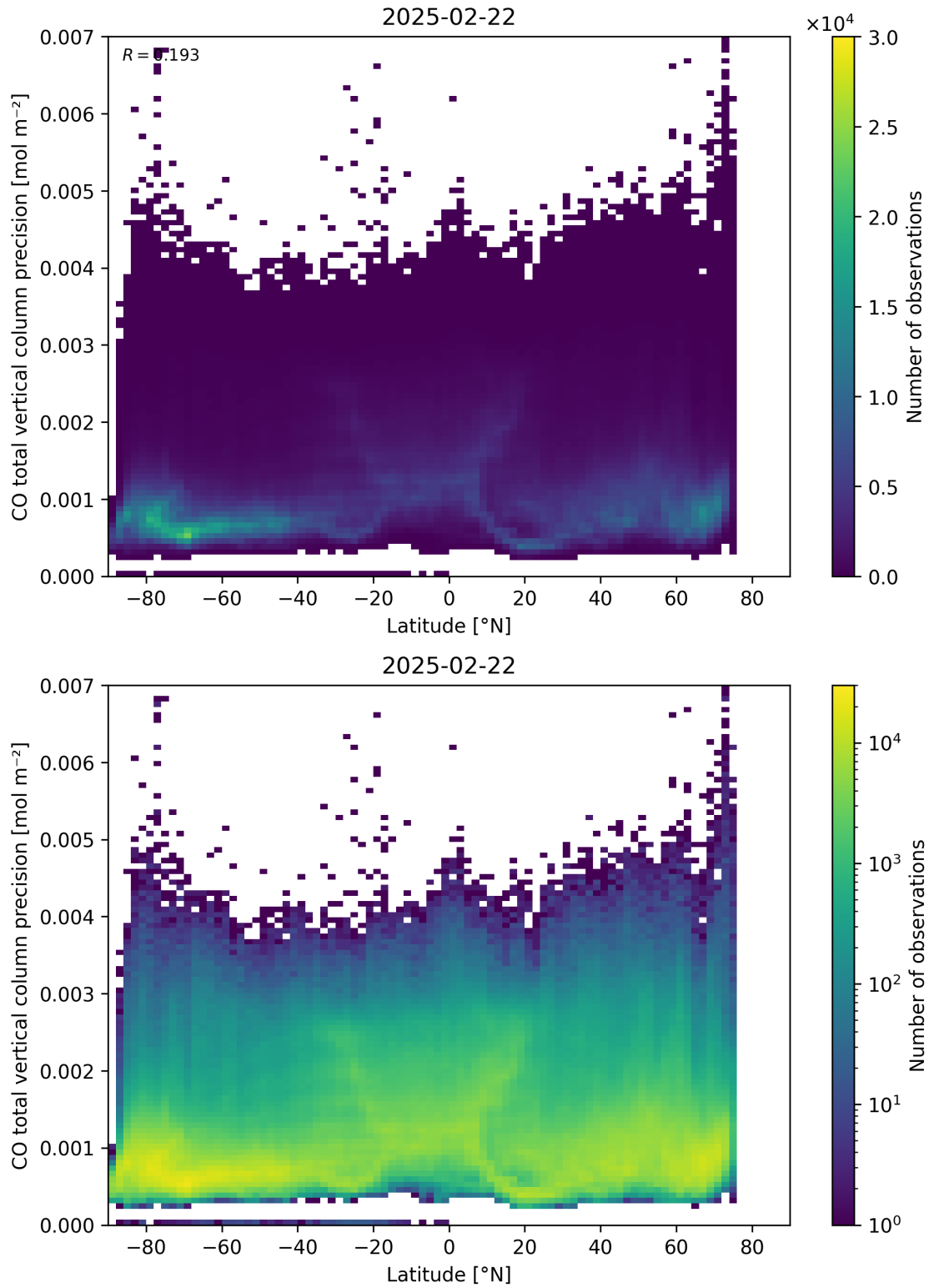
Figure 53: Scatter density plot of “Latitude” against “CO total vertical column precision” for 2025-02-21 to 2025-02-23.
