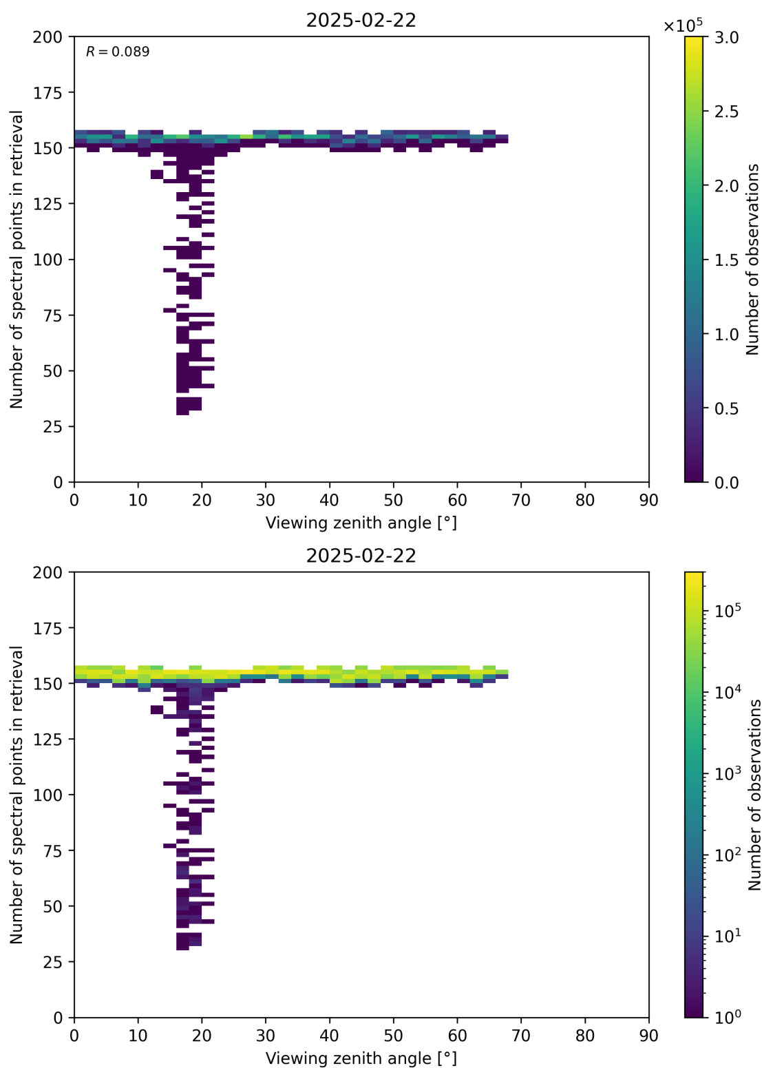
Figure 76: Scatter density plot of “Viewing zenith angle” against “Number of spectral points in retrieval” for 2025-02-21 to 2025-02-23.
