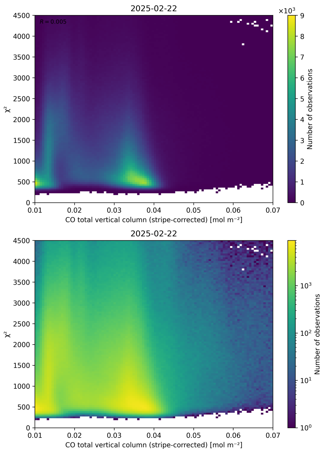
Figure 37: Scatter density plot of “CO total vertical column (stripe-corrected)” against “ \chi^2 ” for 2025-02-21 to 2025-02-23.
