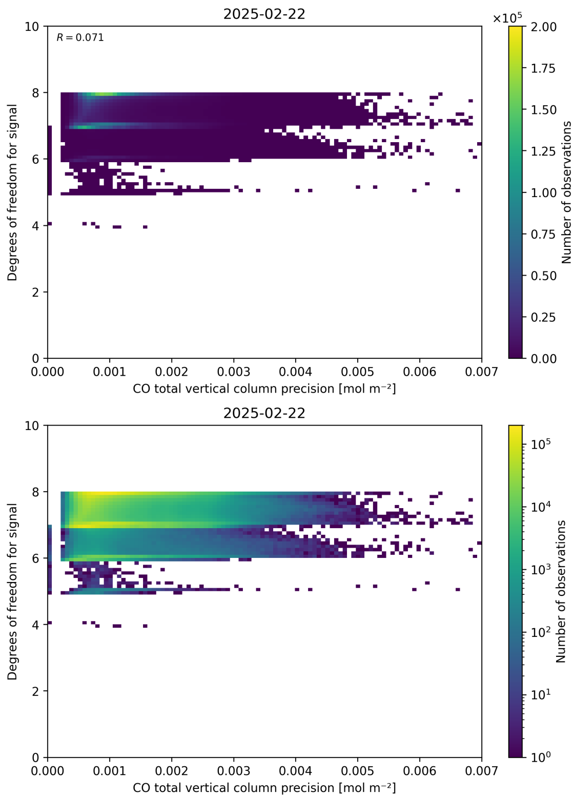
Figure 45: Scatter density plot of “CO total vertical column precision” against “Degrees of freedom for signal” for 2025-02-21 to 2025-02-23.
