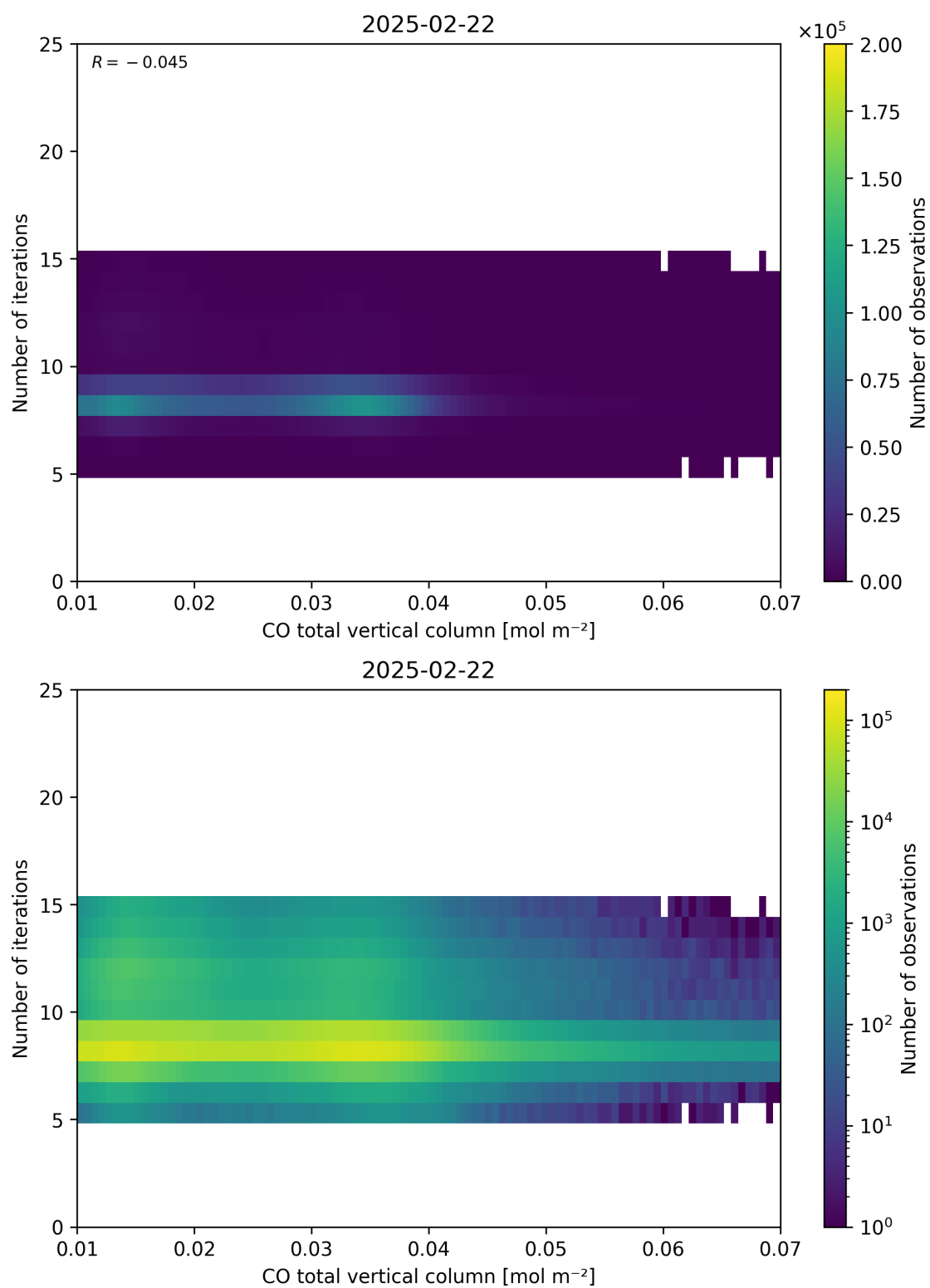
Figure 42: Scatter density plot of “CO total vertical column” against “Number of iterations” for 2025-02-21 to 2025-02-23.
