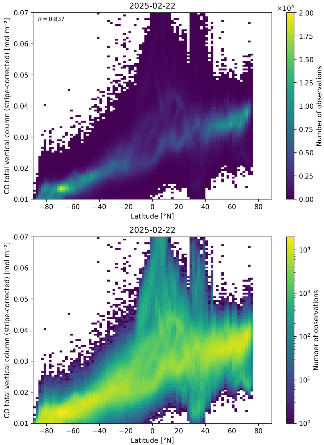
Figure 52: Scatter density plot of “Latitude” against “CO total vertical column (stripe-corrected)” for 2025-02-21 to 2025-02-23.
