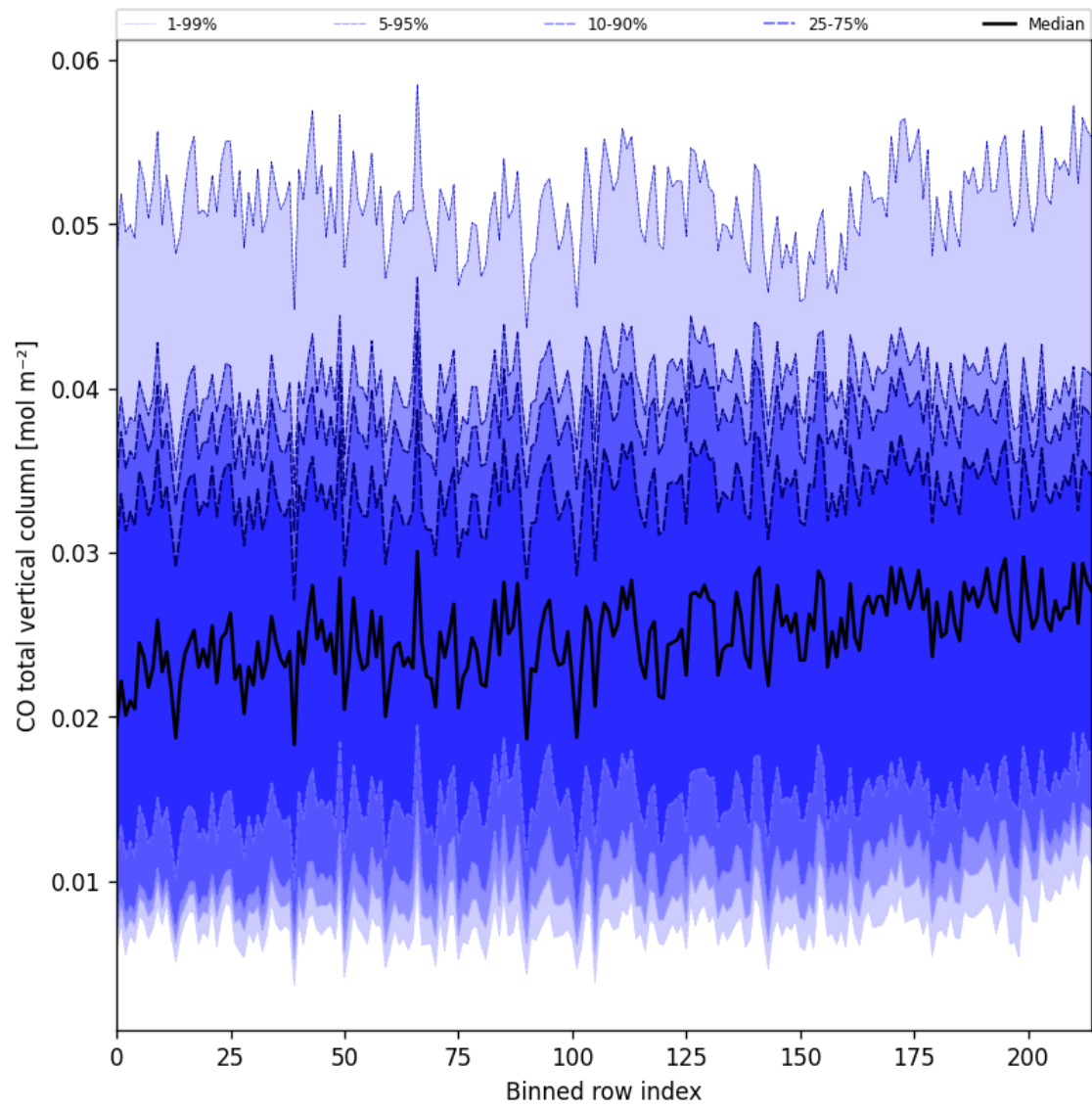
Figure 26: Along track statistics of “CO total vertical column” for 2025-02-21 to 2025-02-23
