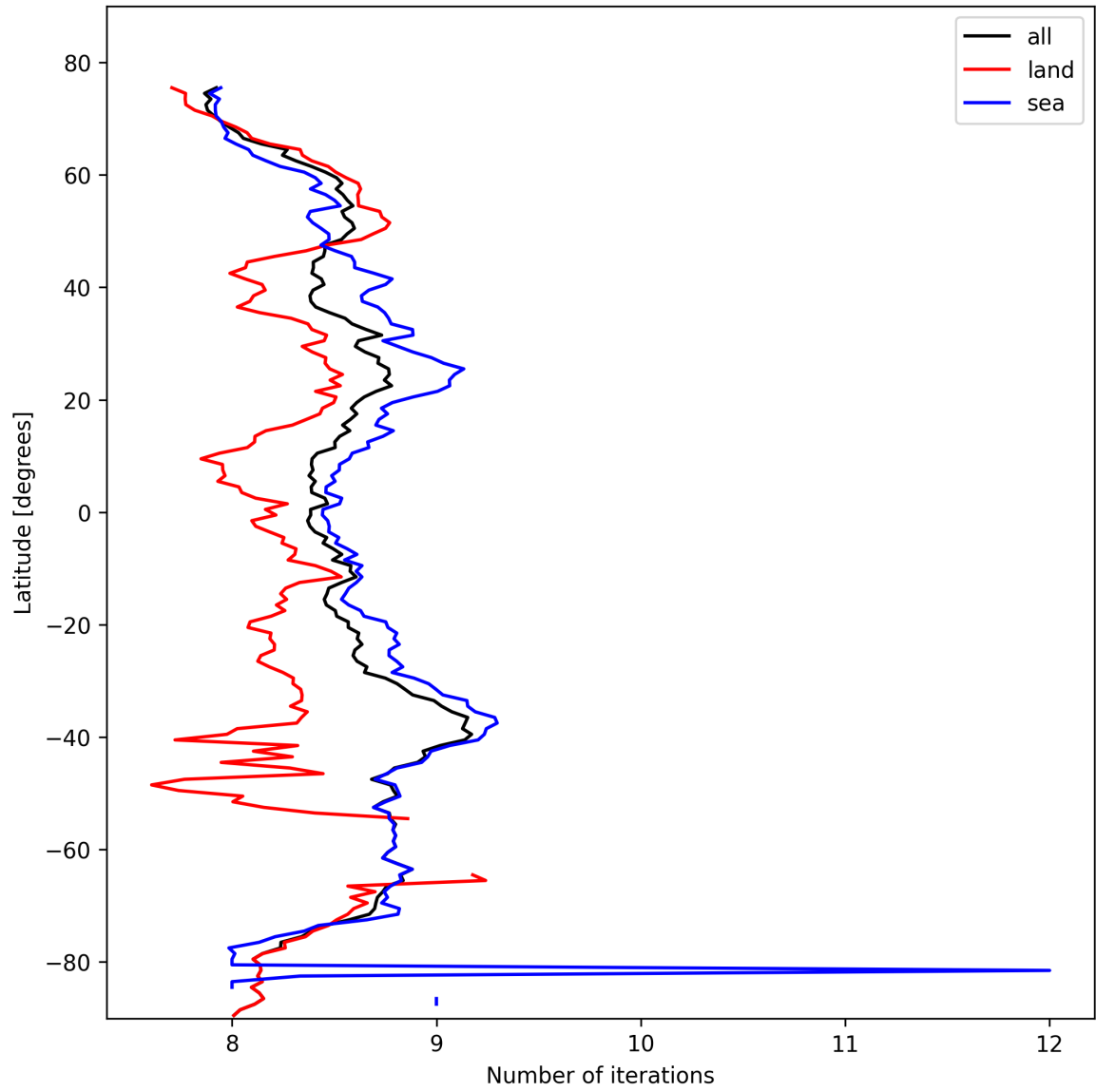
Figure 16: Zonal average of “Number of iterations” for 2025-02-21 to 2025-02-23.
