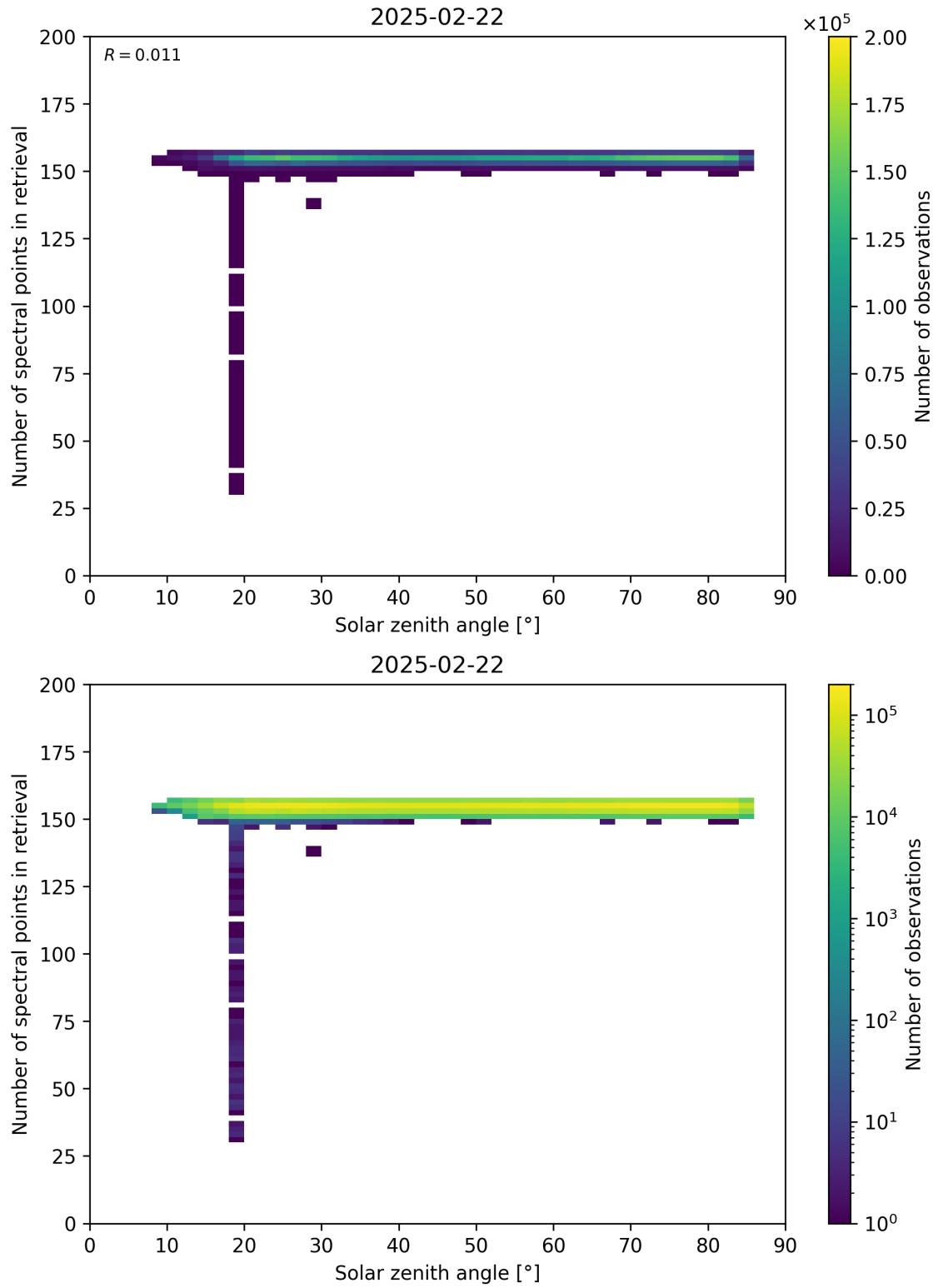
Figure 68: Scatter density plot of “Solar zenith angle” against “Number of spectral points in retrieval” for 2025-02-21 to 2025-02-23.
