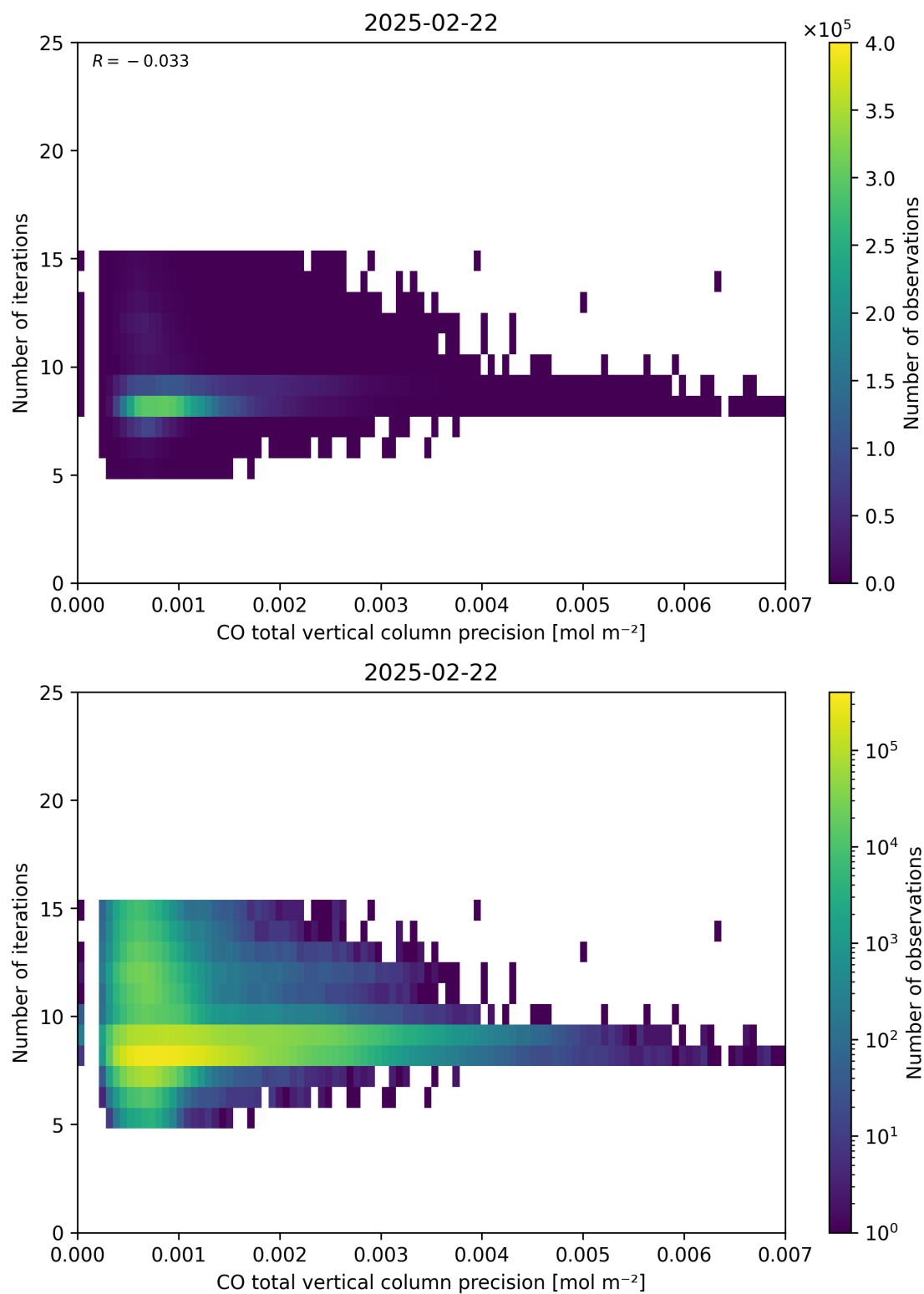
Figure 46: Scatter density plot of “CO total vertical column precision” against “Number of iterations” for 2025-02-21 to 2025-02-23.
