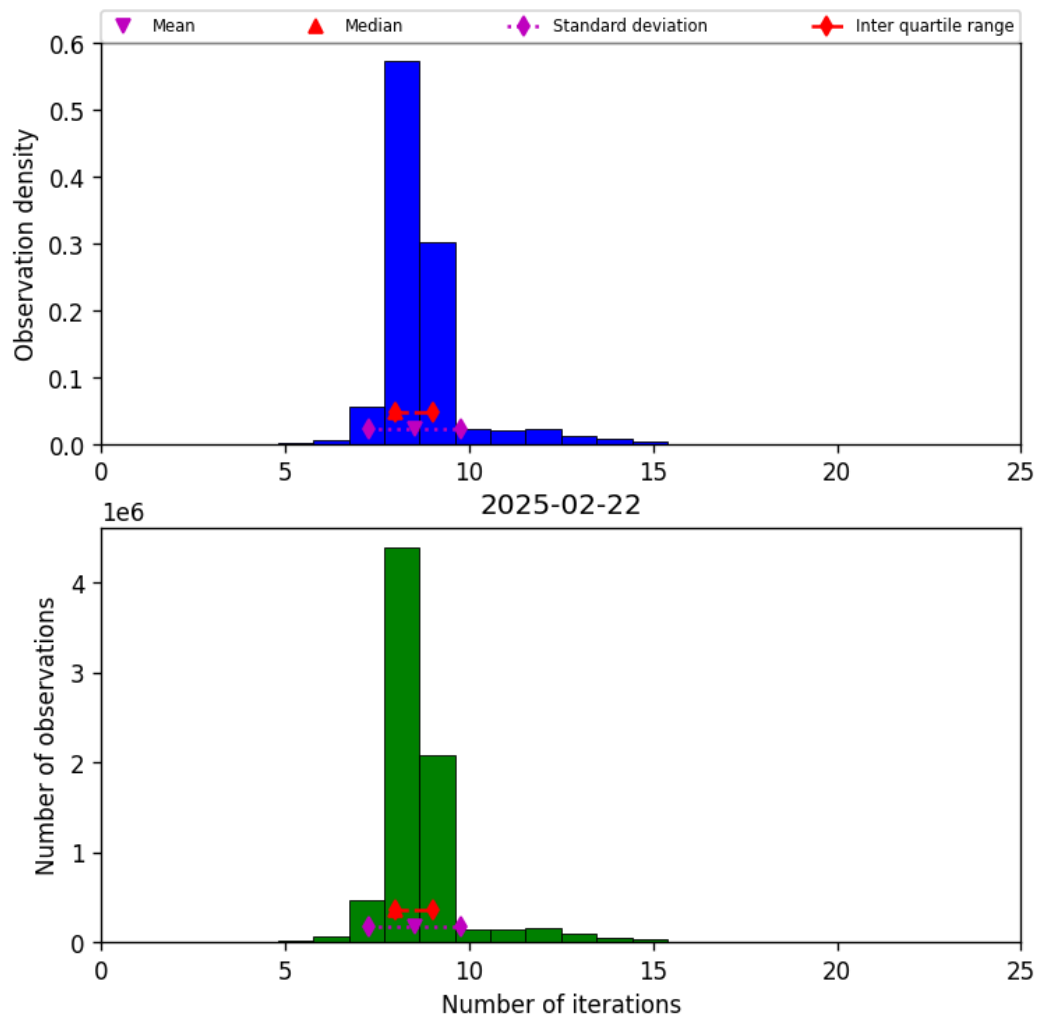
Figure 24: Histogram of “Number of iterations” for 2025-02-21 to 2025-02-23
