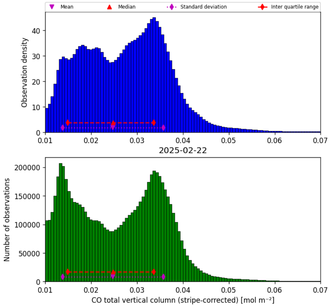
Figure 19: Histogram of “CO total vertical column (stripe-corrected)” for 2025-02-21 to 2025-02-23
