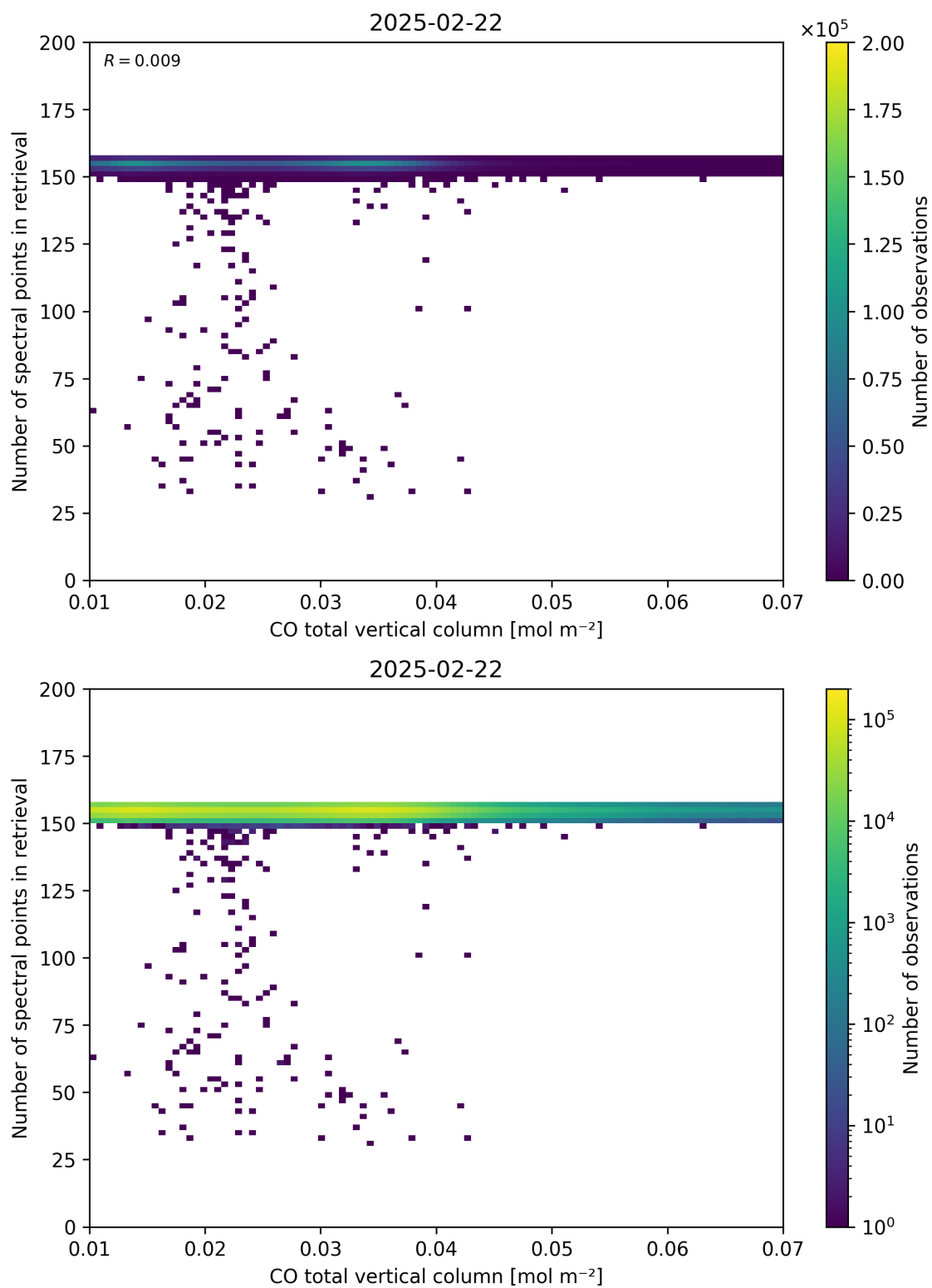
Figure 43: Scatter density plot of “CO total vertical column” against “Number of spectral points in retrieval” for 2025-02-21 to 2025-02-23.
