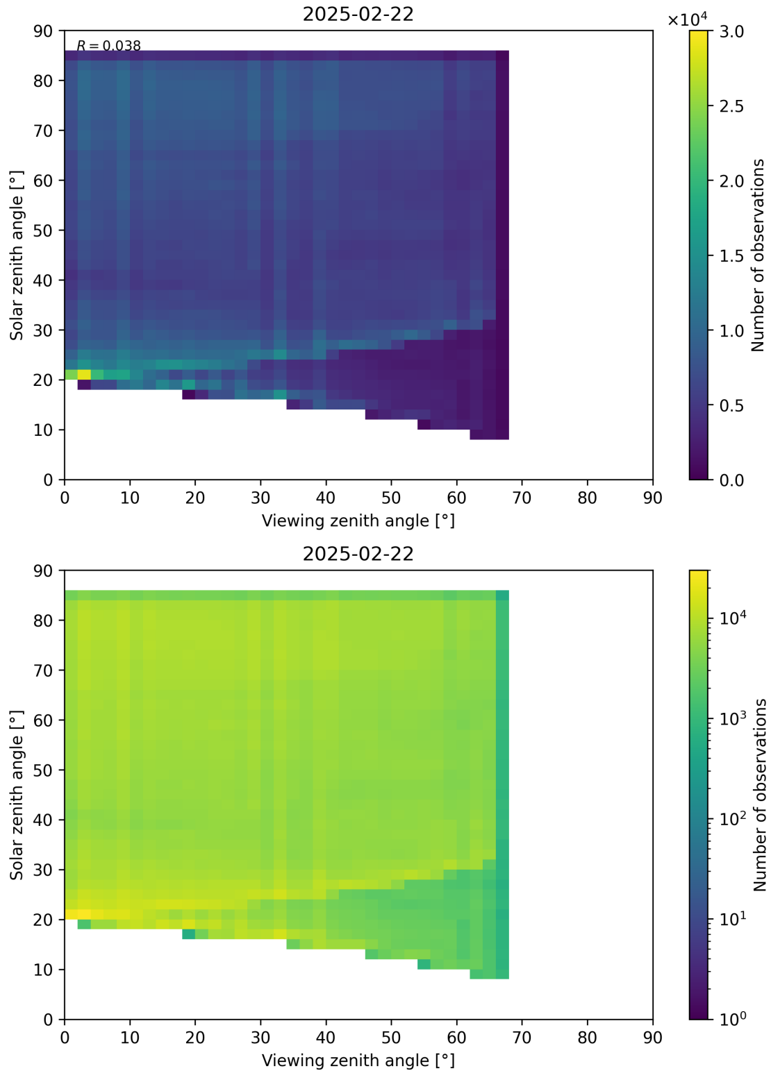
Figure 77: Scatter density plot of “Viewing zenith angle” against “Solar zenith angle” for 2025-02-21 to 2025-02-23.
