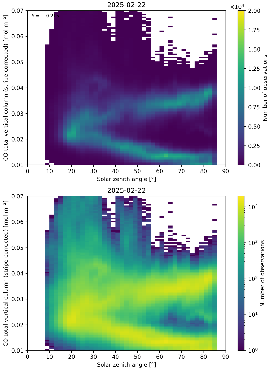
Figure 62: Scatter density plot of “Solar zenith angle” against “CO total vertical column (stripe-corrected)” for 2025-02-21 to 2025-02-23.
