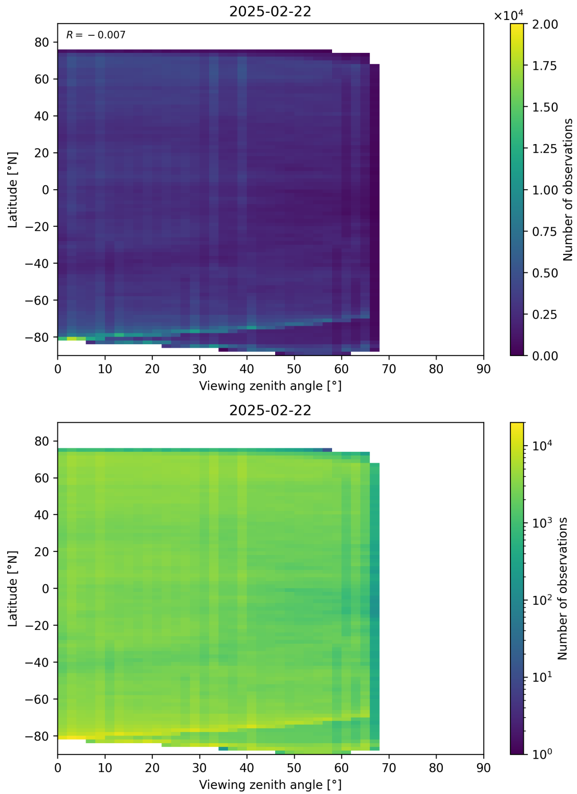
Figure 74: Scatter density plot of “Viewing zenith angle” against “Latitude” for 2025-02-21 to 2025-02-23.
