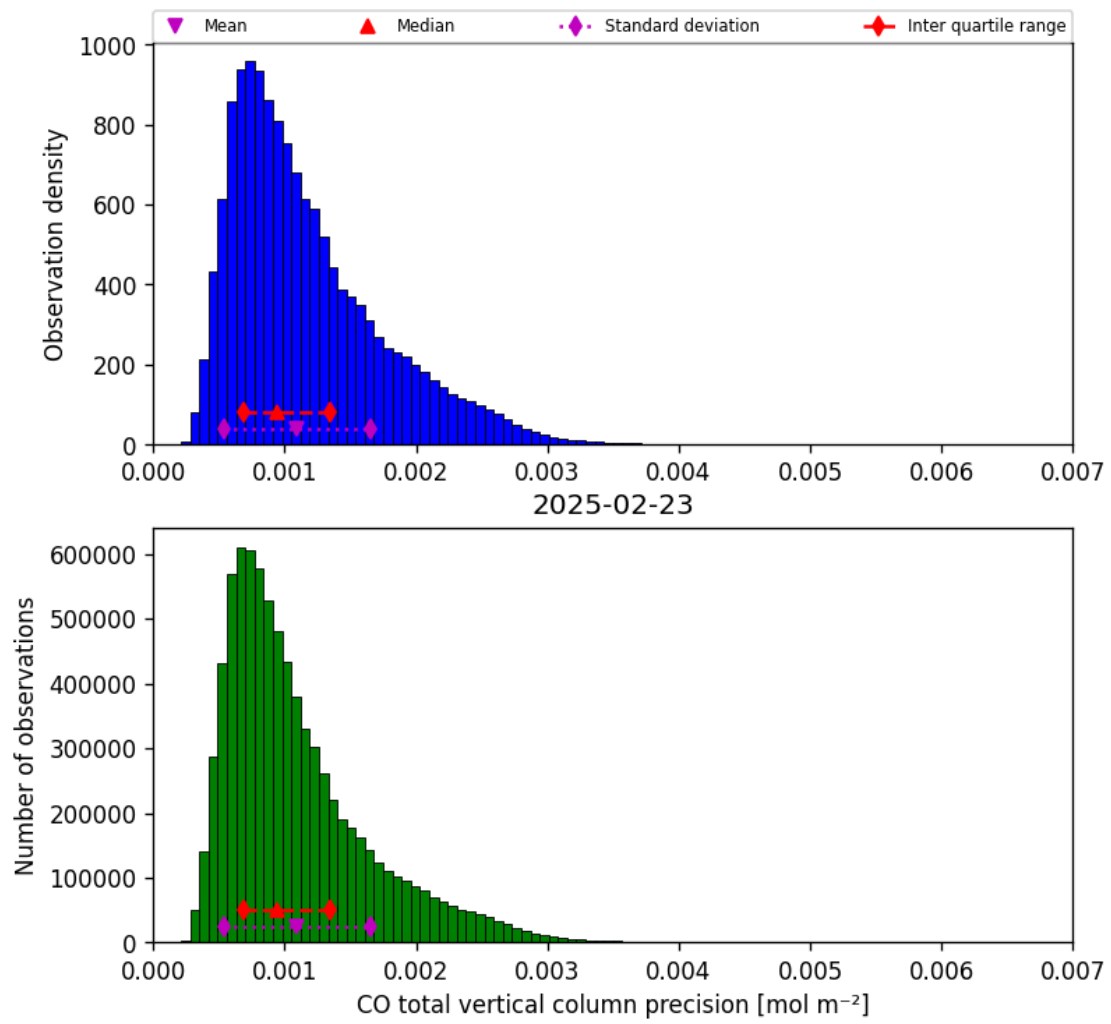
Figure 20: Histogram of “CO total vertical column precision” for 2025-02-22 to 2025-02-24
