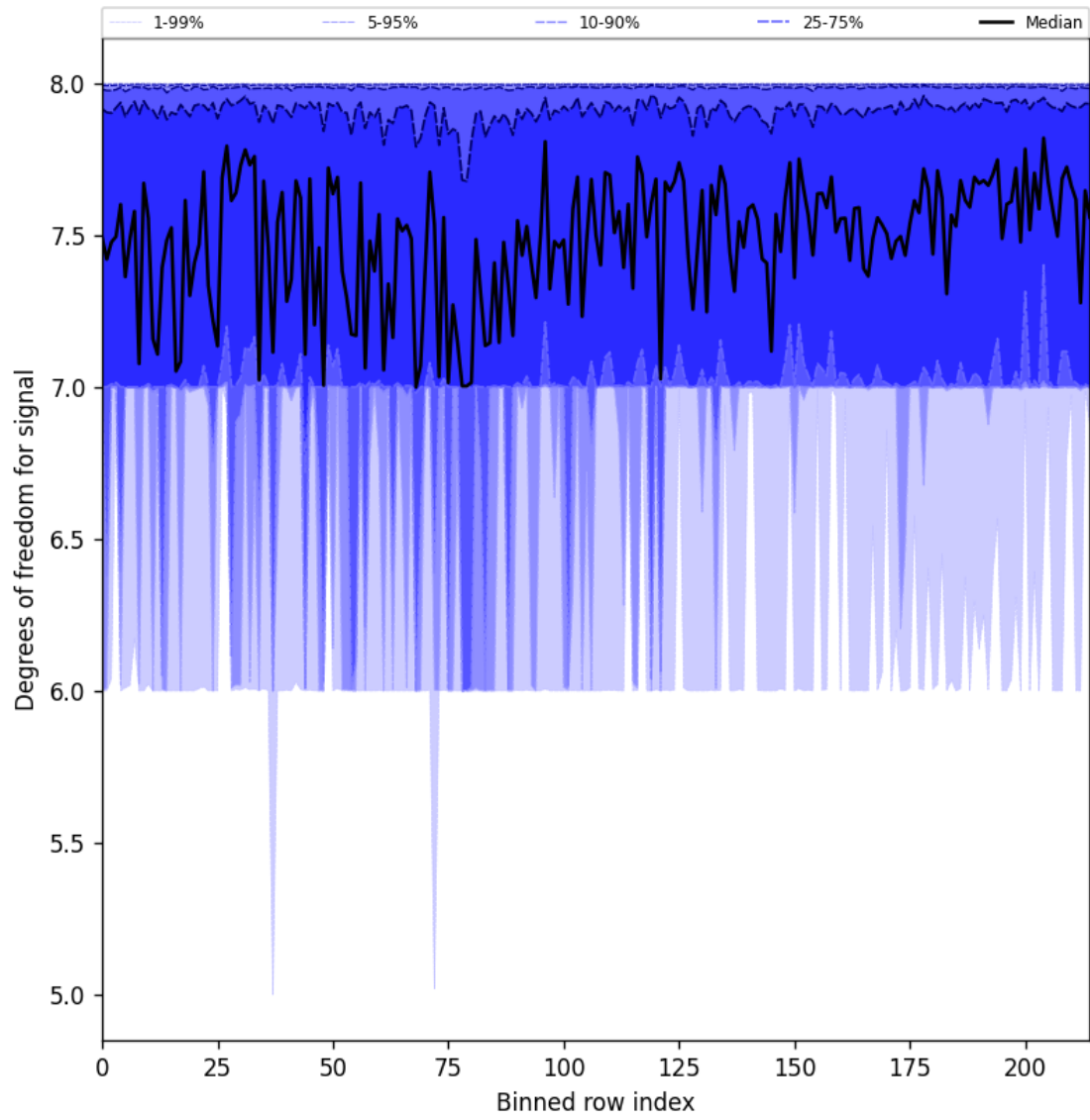
Figure 31: Along track statistics of “Degrees of freedom for signal” for 2025-02-22 to 2025-02-24
