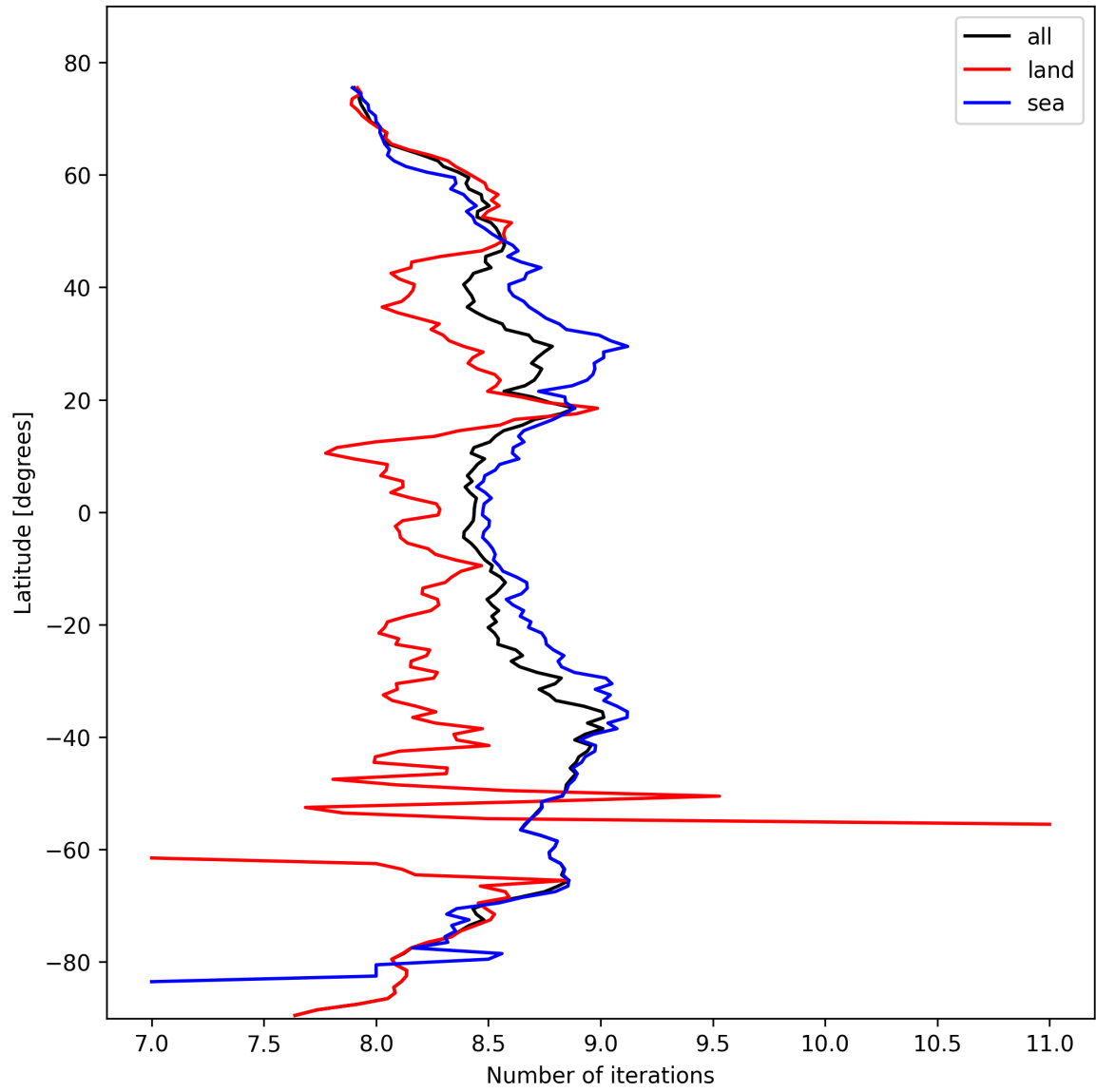
Figure 16: Zonal average of “Number of iterations” for 2025-02-22 to 2025-02-24.
