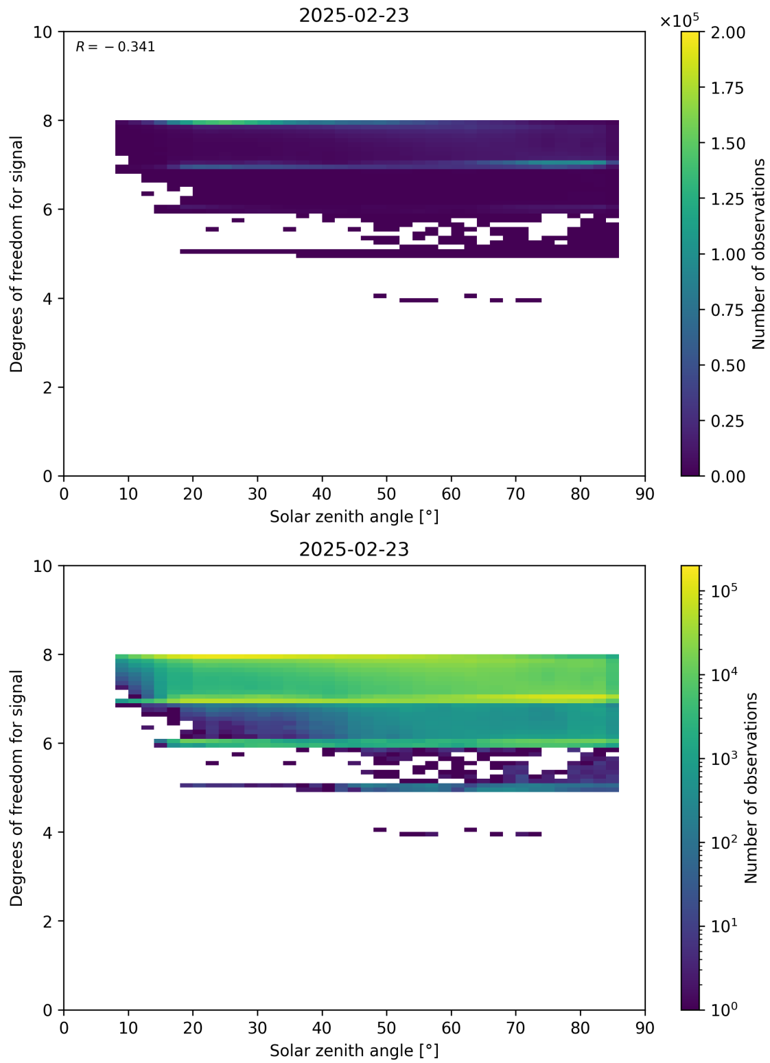
Figure 65: Scatter density plot of “Solar zenith angle” against “Degrees of freedom for signal” for 2025-02-22 to 2025-02-24.
