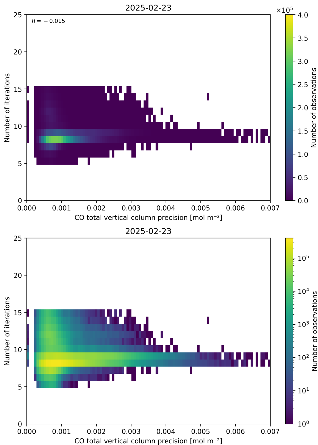
Figure 46: Scatter density plot of “CO total vertical column precision” against “Number of iterations” for 2025-02-22 to 2025-02-24.
