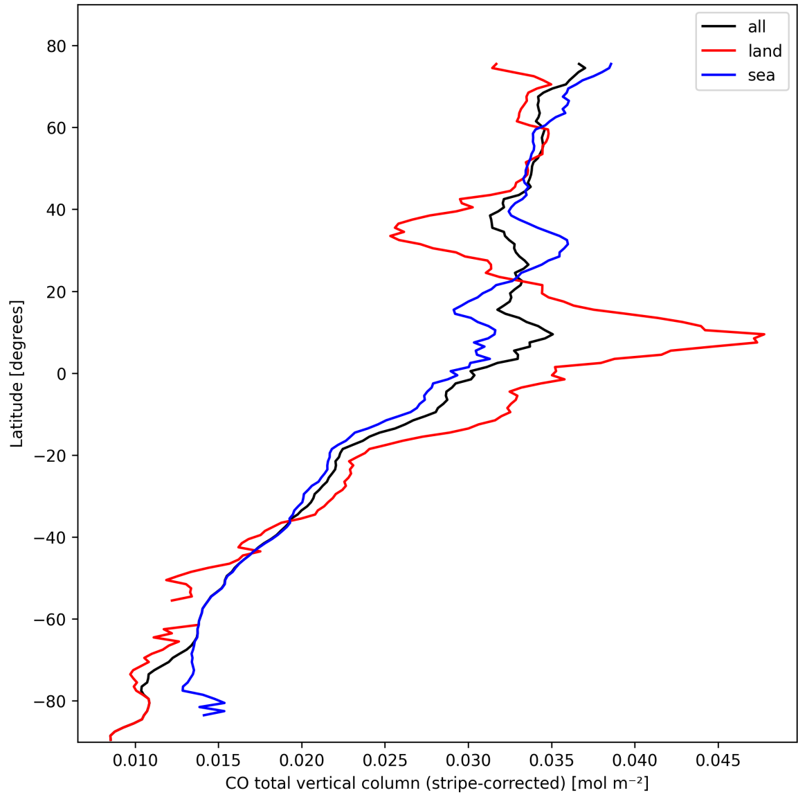
Figure 11: Zonal average of “CO total vertical column (stripe-corrected)” for 2025-02-22 to 2025-02-24.
