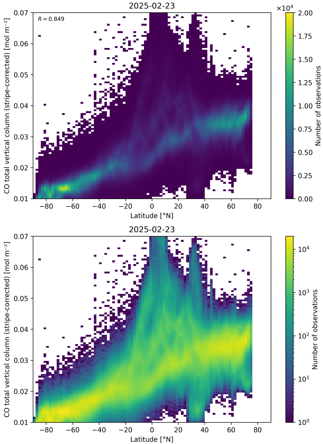
Figure 52: Scatter density plot of “Latitude” against “CO total vertical column (stripe-corrected)” for 2025-02-22 to 2025-02-24.
