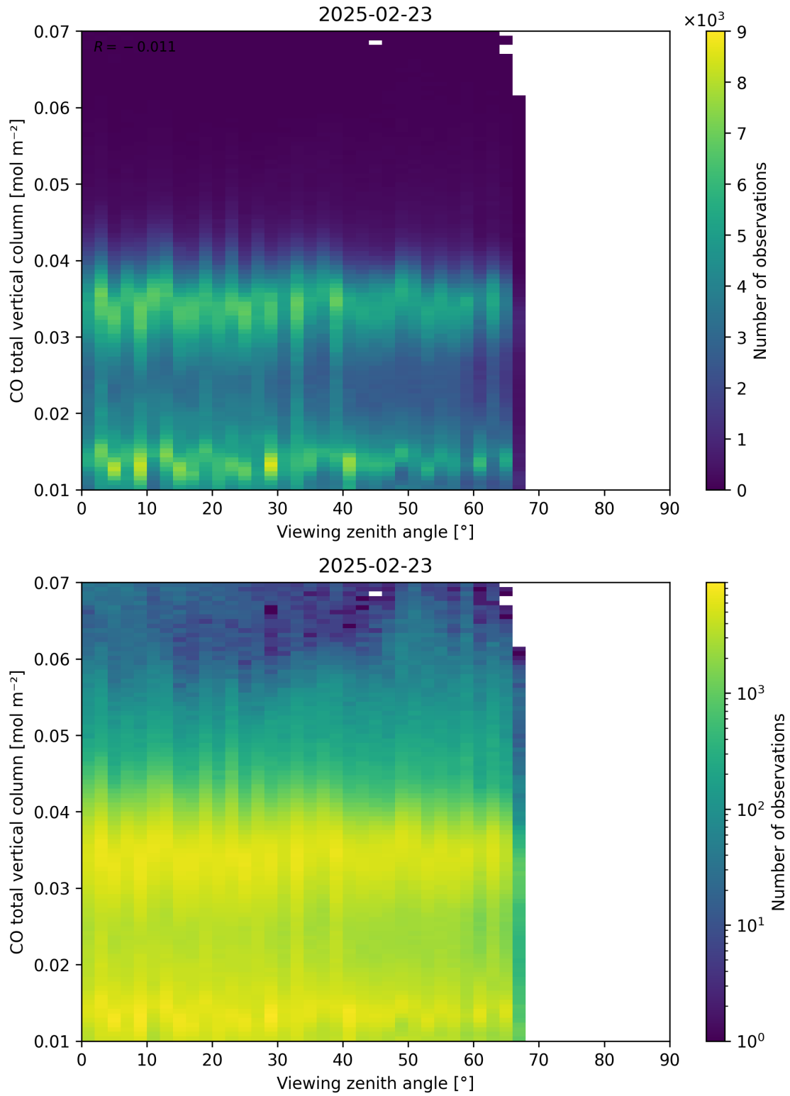
Figure 69: Scatter density plot of “Viewing zenith angle” against “CO total vertical column” for 2025-02-22 to 2025-02-24.
