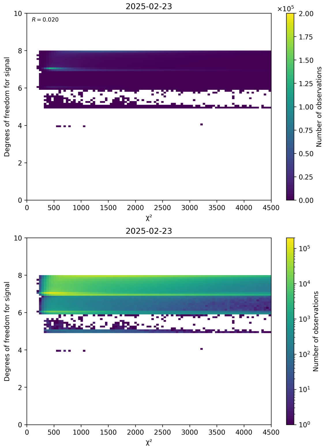
Figure 48: Scatter density plot of “ \chi^2 ” against “Degrees of freedom for signal” for 2025-02-22 to 2025-02-24.
