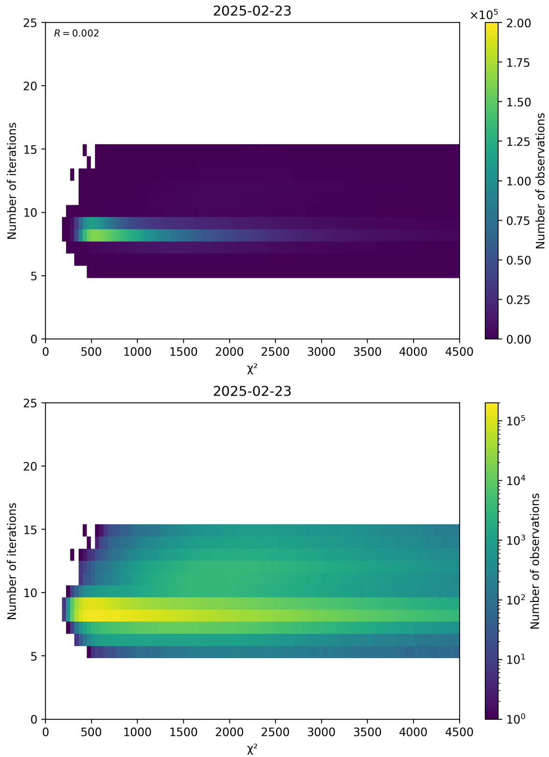
Figure 49: Scatter density plot of “ \chi^2 ” against “Number of iterations” for 2025-02-22 to 2025-02-24.
