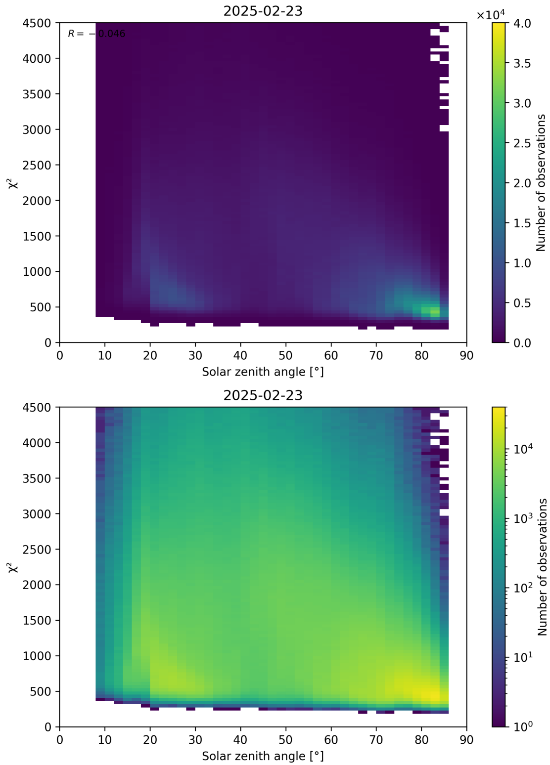
Figure 64: Scatter density plot of “Solar zenith angle” against “ \chi^2 ” for 2025-02-22 to 2025-02-24.
