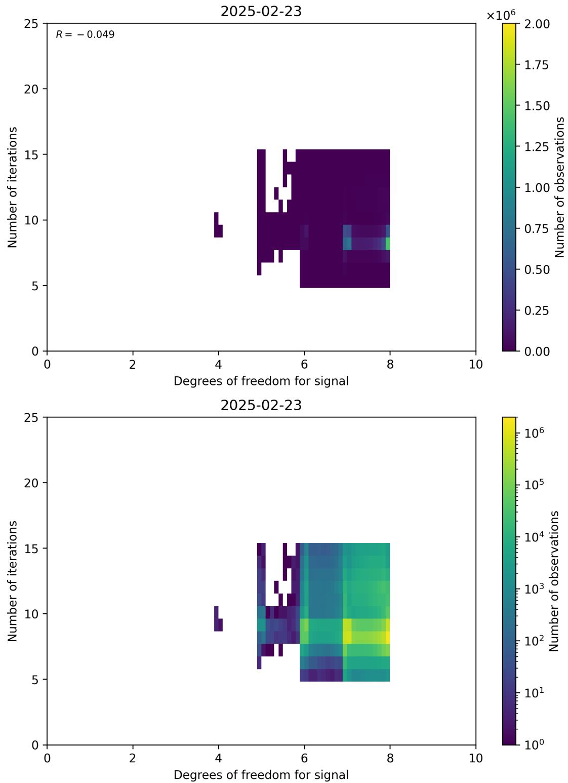
Figure 50: Scatter density plot of “Degrees of freedom for signal” against “Number of iterations” for 2025-02-22 to 2025-02-24.
