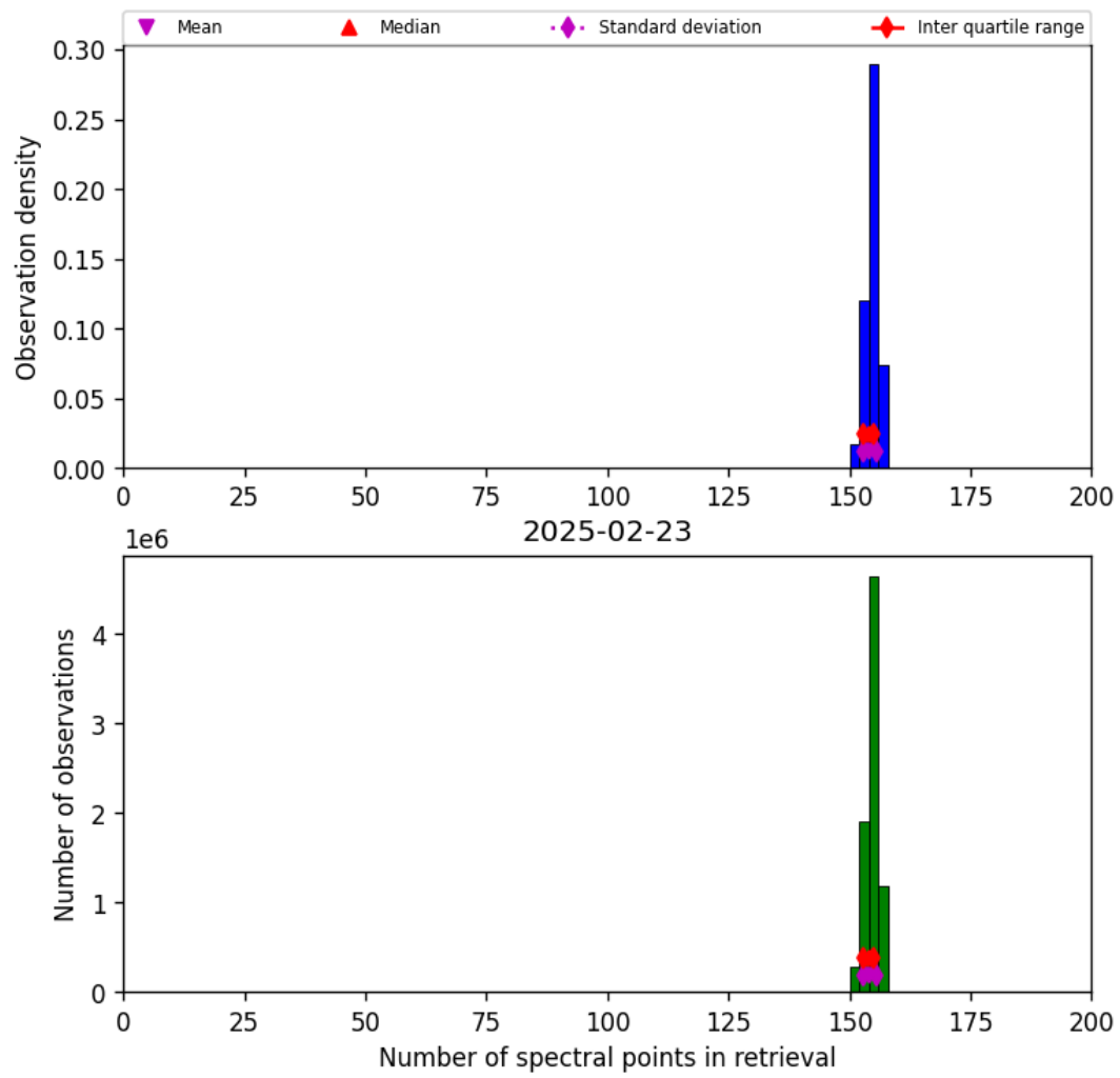
Figure 21: Histogram of “Number of spectral points in retrieval” for 2025-02-22 to 2025-02-24
