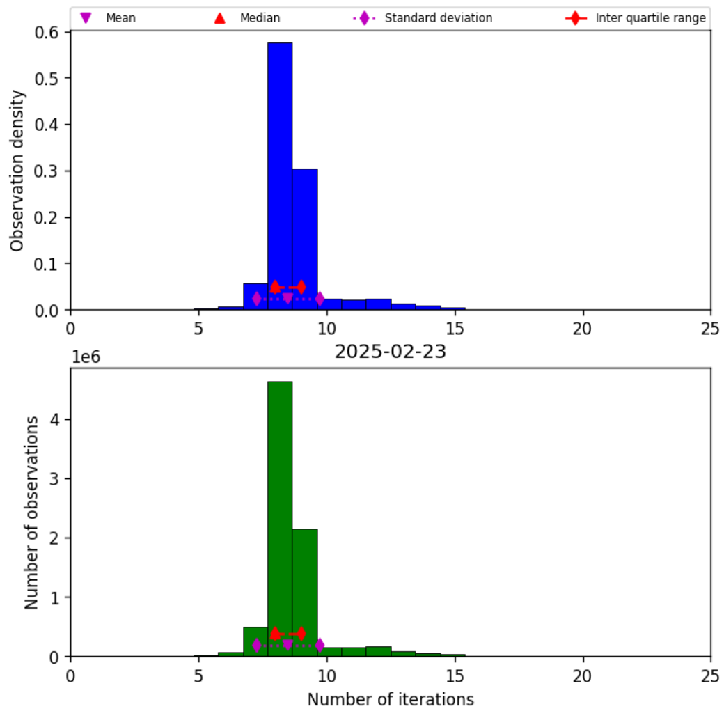
Figure 24: Histogram of “Number of iterations” for 2025-02-22 to 2025-02-24
