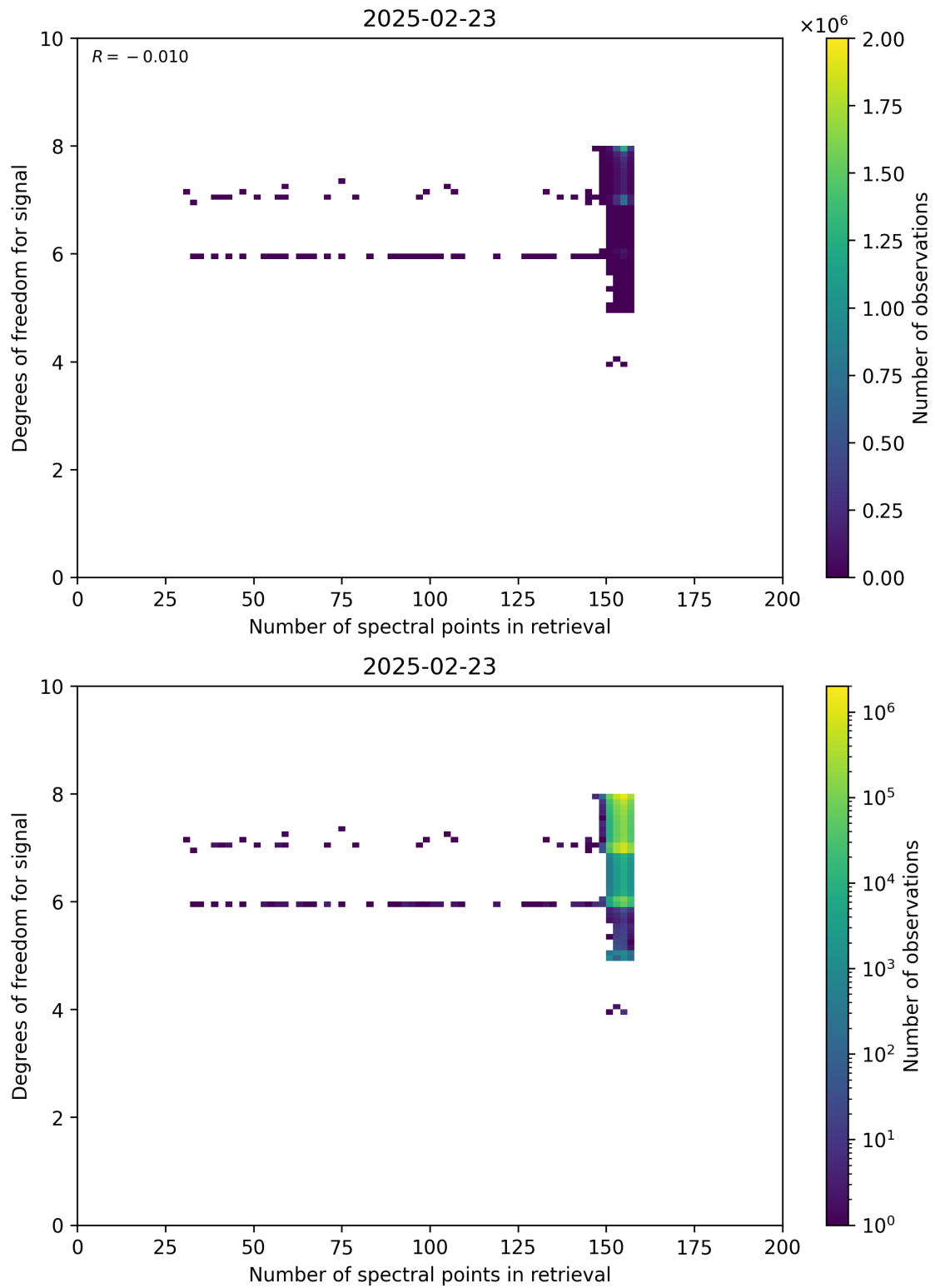
Figure 59: Scatter density plot of “Number of spectral points in retrieval” against “Degrees of freedom for signal” for 2025-02-22 to 2025-02-24.
