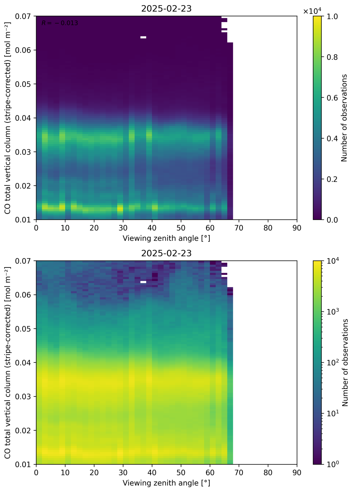
Figure 70: Scatter density plot of “Viewing zenith angle” against “CO total vertical column (stripe-corrected)” for 2025-02-22 to 2025-02-24.
