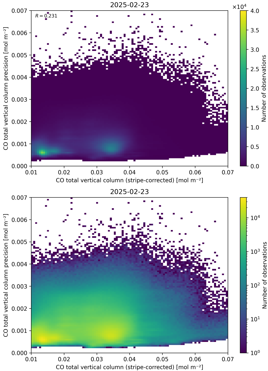
Figure 36: Scatter density plot of “CO total vertical column (stripe-corrected)” against “CO total vertical column precision” for 2025-02-22 to 2025-02-24.
