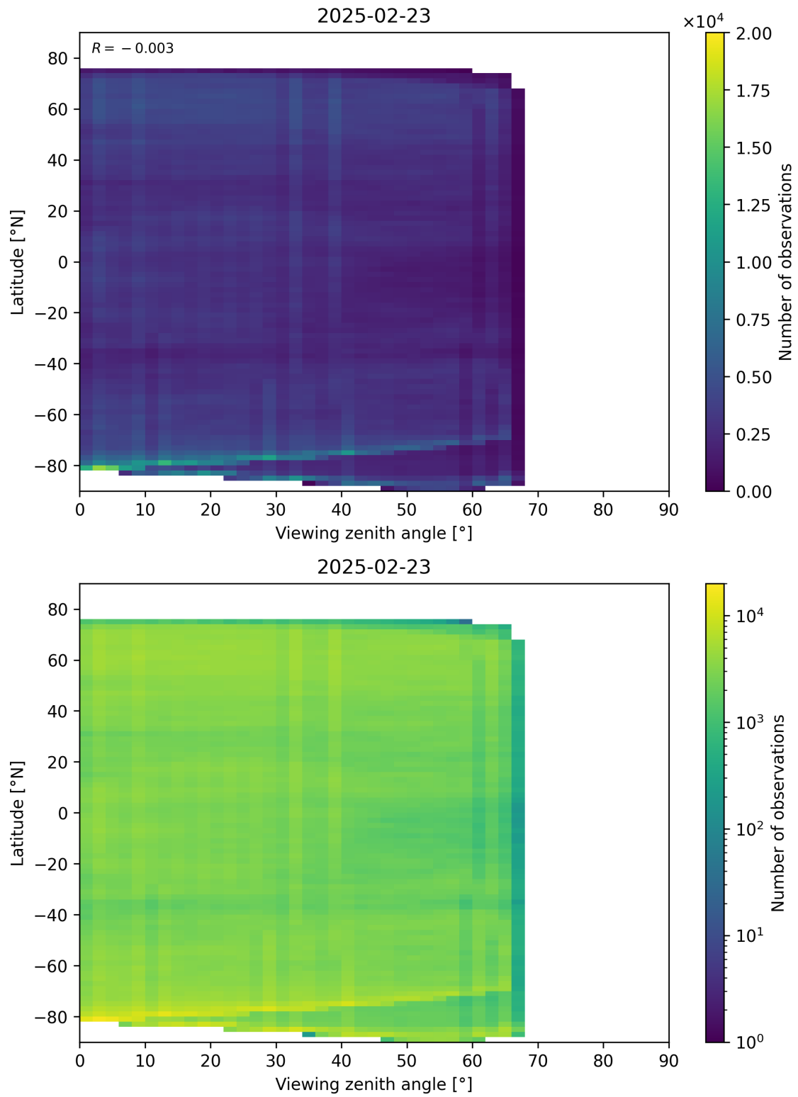
Figure 74: Scatter density plot of “Viewing zenith angle” against “Latitude” for 2025-02-22 to 2025-02-24.
