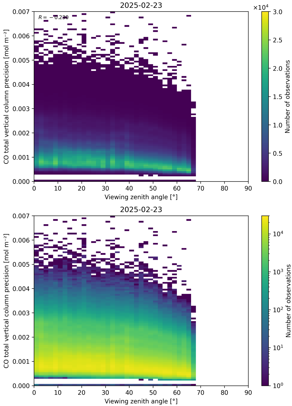
Figure 71: Scatter density plot of “Viewing zenith angle” against “CO total vertical column precision” for 2025-02-22 to 2025-02-24.
