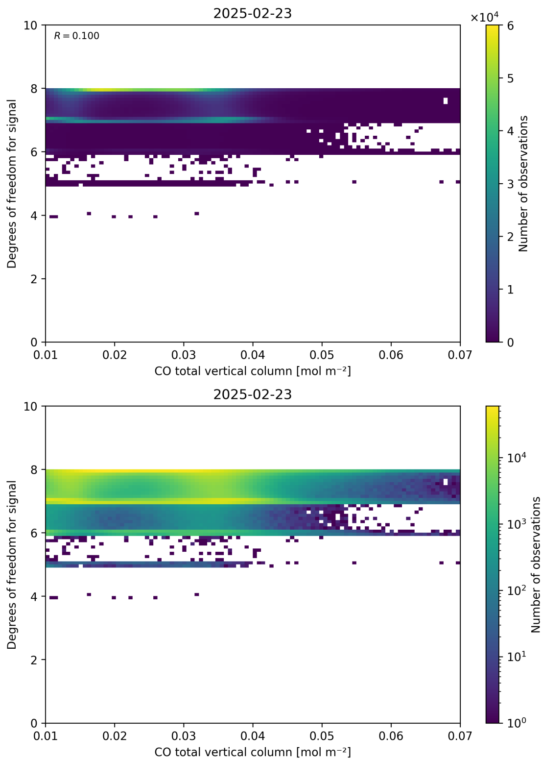
Figure 41: Scatter density plot of “CO total vertical column” against “Degrees of freedom for signal” for 2025-02-22 to 2025-02-24.
