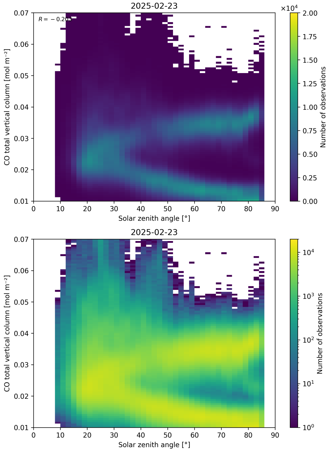
Figure 61: Scatter density plot of “Solar zenith angle” against “CO total vertical column” for 2025-02-22 to 2025-02-24.
