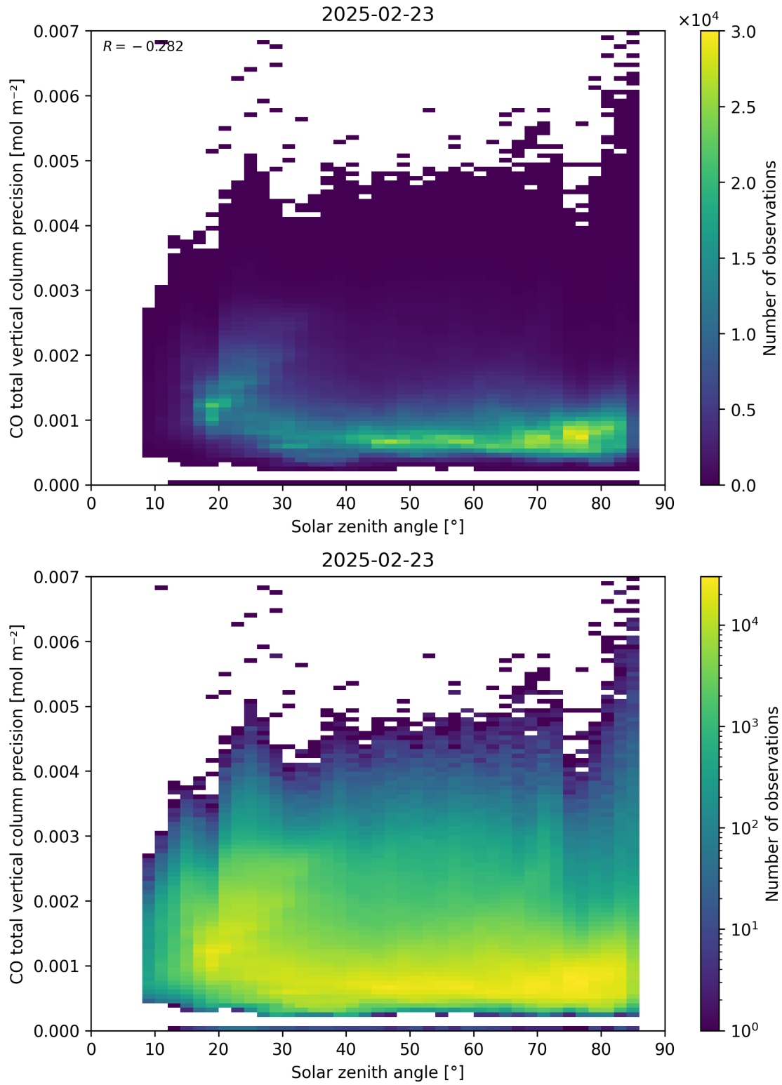
Figure 63: Scatter density plot of “Solar zenith angle” against “CO total vertical column precision” for 2025-02-22 to 2025-02-24.
