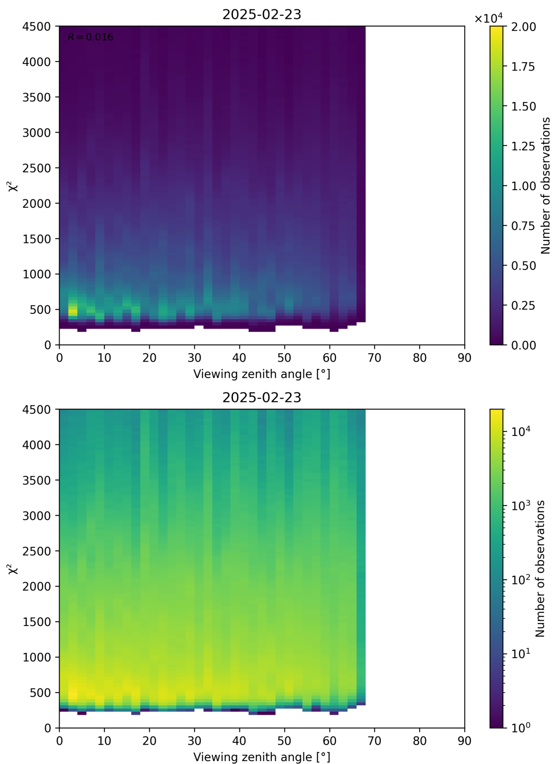
Figure 72: Scatter density plot of “Viewing zenith angle” against “ \chi^2 ” for 2025-02-22 to 2025-02-24.
