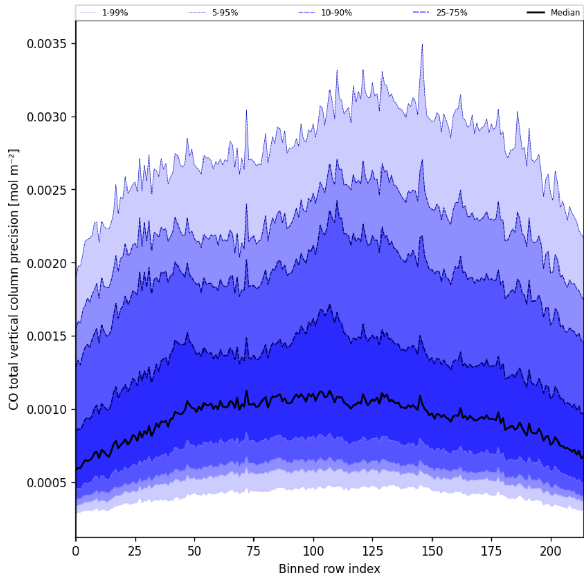
Figure 28: Along track statistics of “CO total vertical column precision” for 2025-02-22 to 2025-02-24
