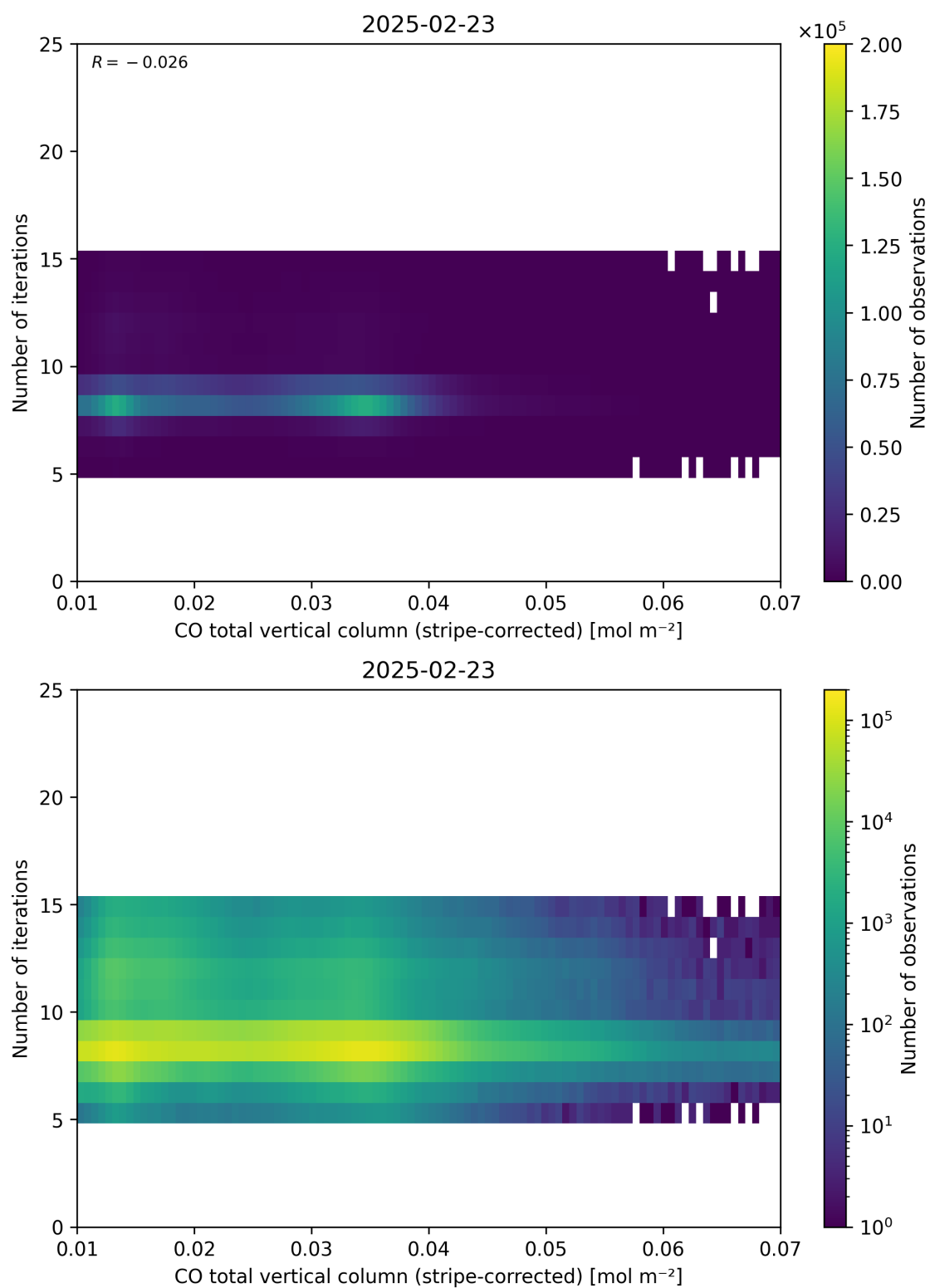
Figure 39: Scatter density plot of “CO total vertical column (stripe-corrected)” against “Number of iterations” for 2025-02-22 to 2025-02-24.
