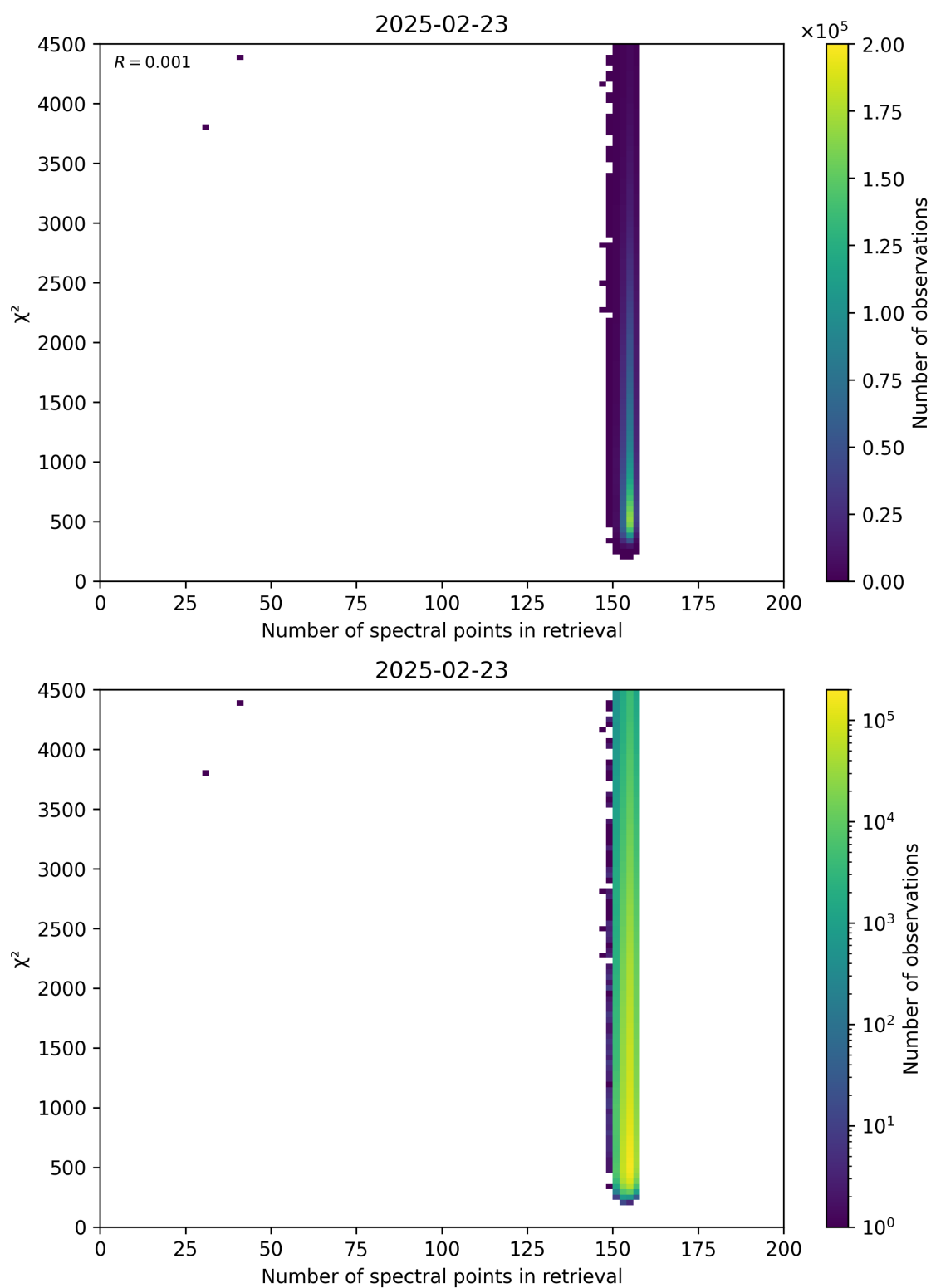
Figure 58: Scatter density plot of “Number of spectral points in retrieval” against “ \chi^2 ” for 2025-02-22 to 2025-02-24.
