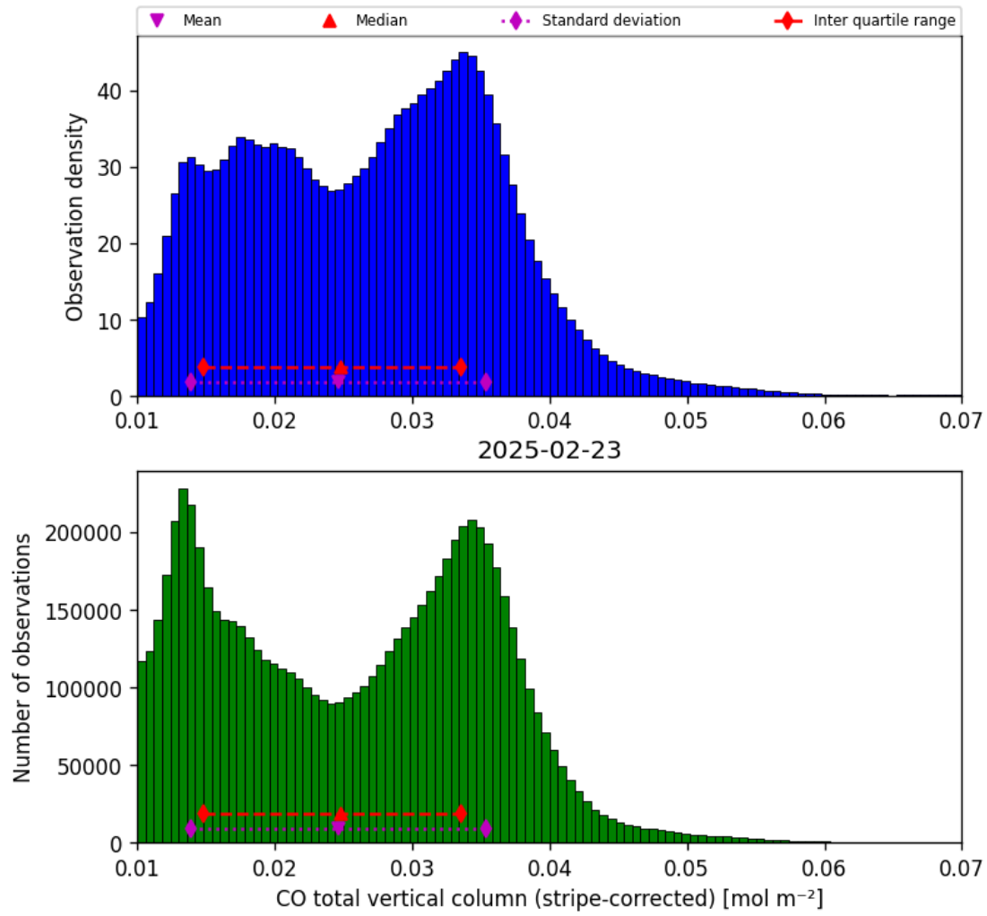
Figure 19: Histogram of “CO total vertical column (stripe-corrected)” for 2025-02-22 to 2025-02-24
