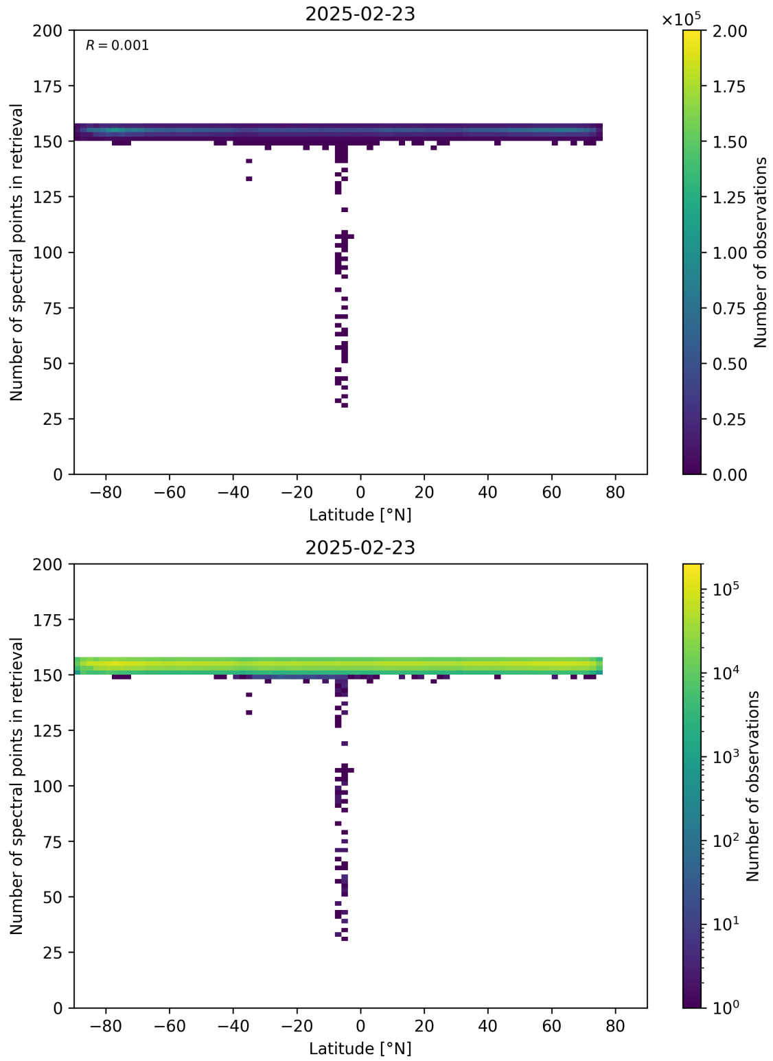
Figure 57: Scatter density plot of “Latitude” against “Number of spectral points in retrieval” for 2025-02-22 to 2025-02-24.
