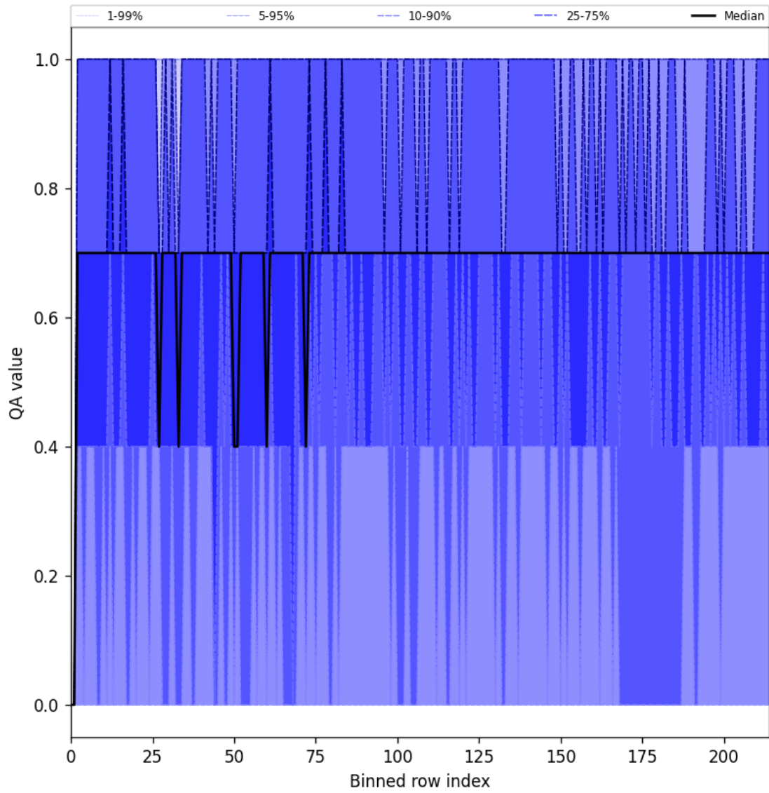
Figure 25: Along track statistics of “QA value” for 2025-02-22 to 2025-02-24
