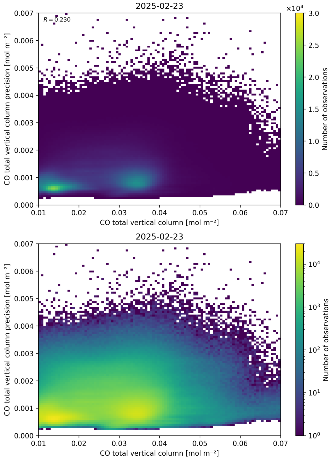
Figure 34: Scatter density plot of “CO total vertical column” against “CO total vertical column precision” for 2025-02-22 to 2025-02-24.
