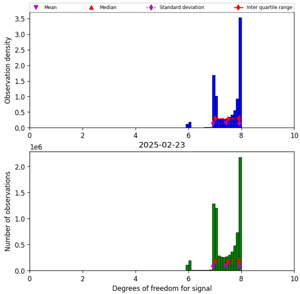
Figure 23: Histogram of “Degrees of freedom for signal” for 2025-02-22 to 2025-02-24
