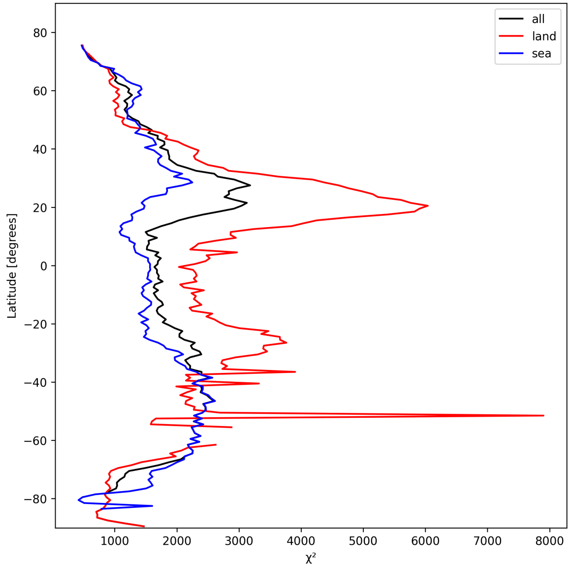
Figure 14: Zonal average of “ \chi^2 ” for 2025-02-22 to 2025-02-24.
