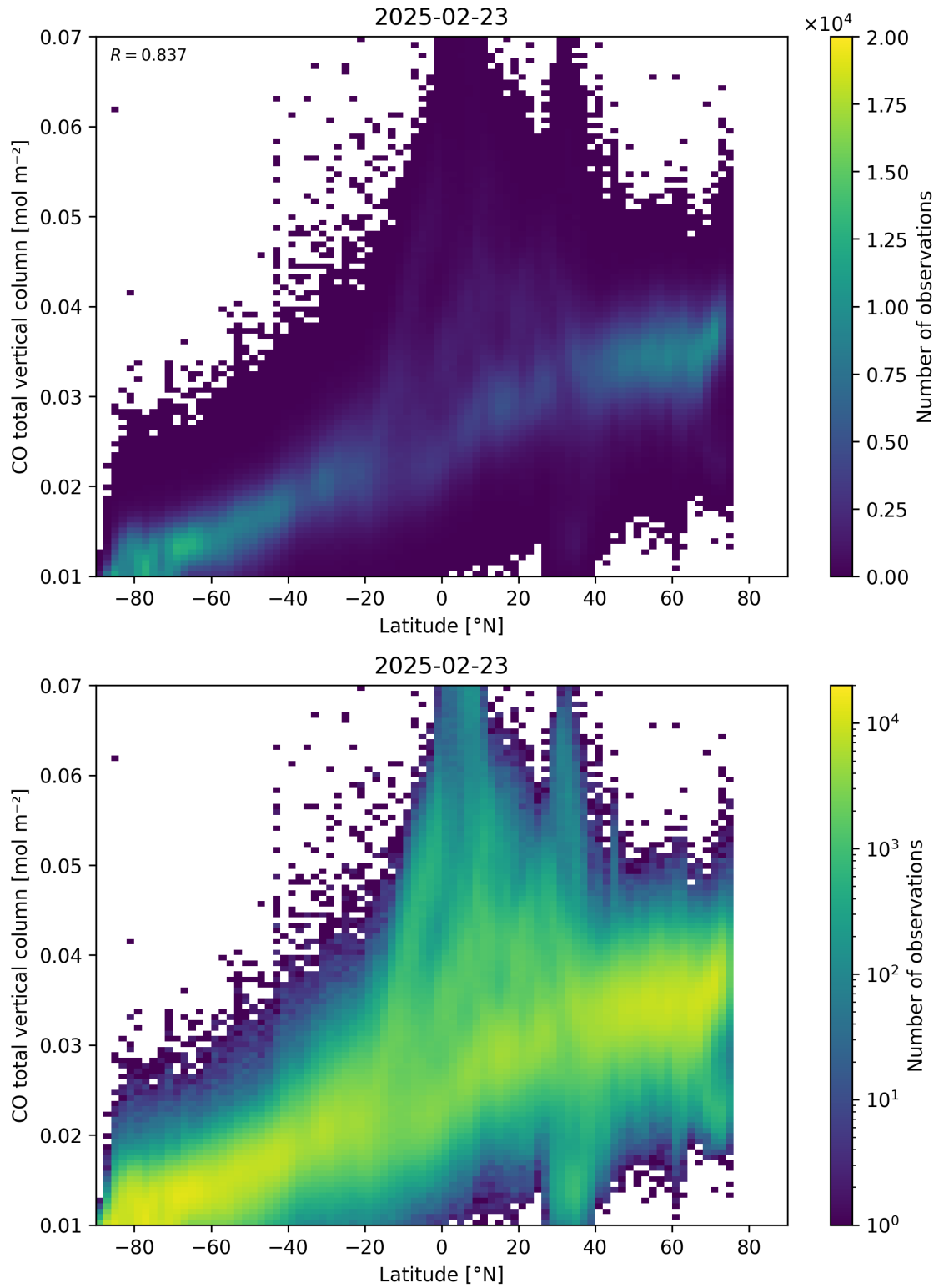
Figure 51: Scatter density plot of “Latitude” against “CO total vertical column” for 2025-02-22 to 2025-02-24.
