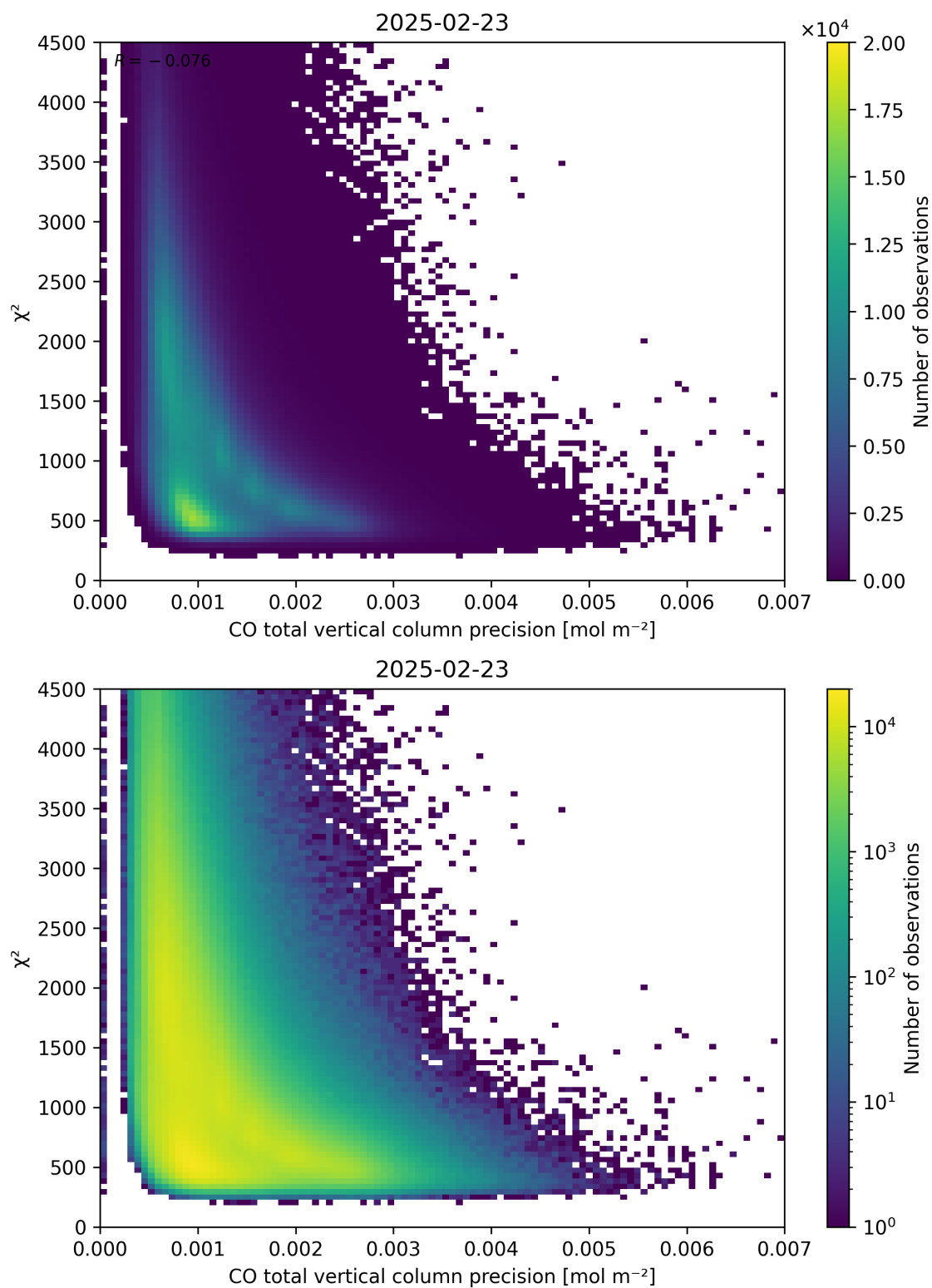
Figure 44: Scatter density plot of “CO total vertical column precision” against “ \chi^2 ” for 2025-02-22 to 2025-02-24.
