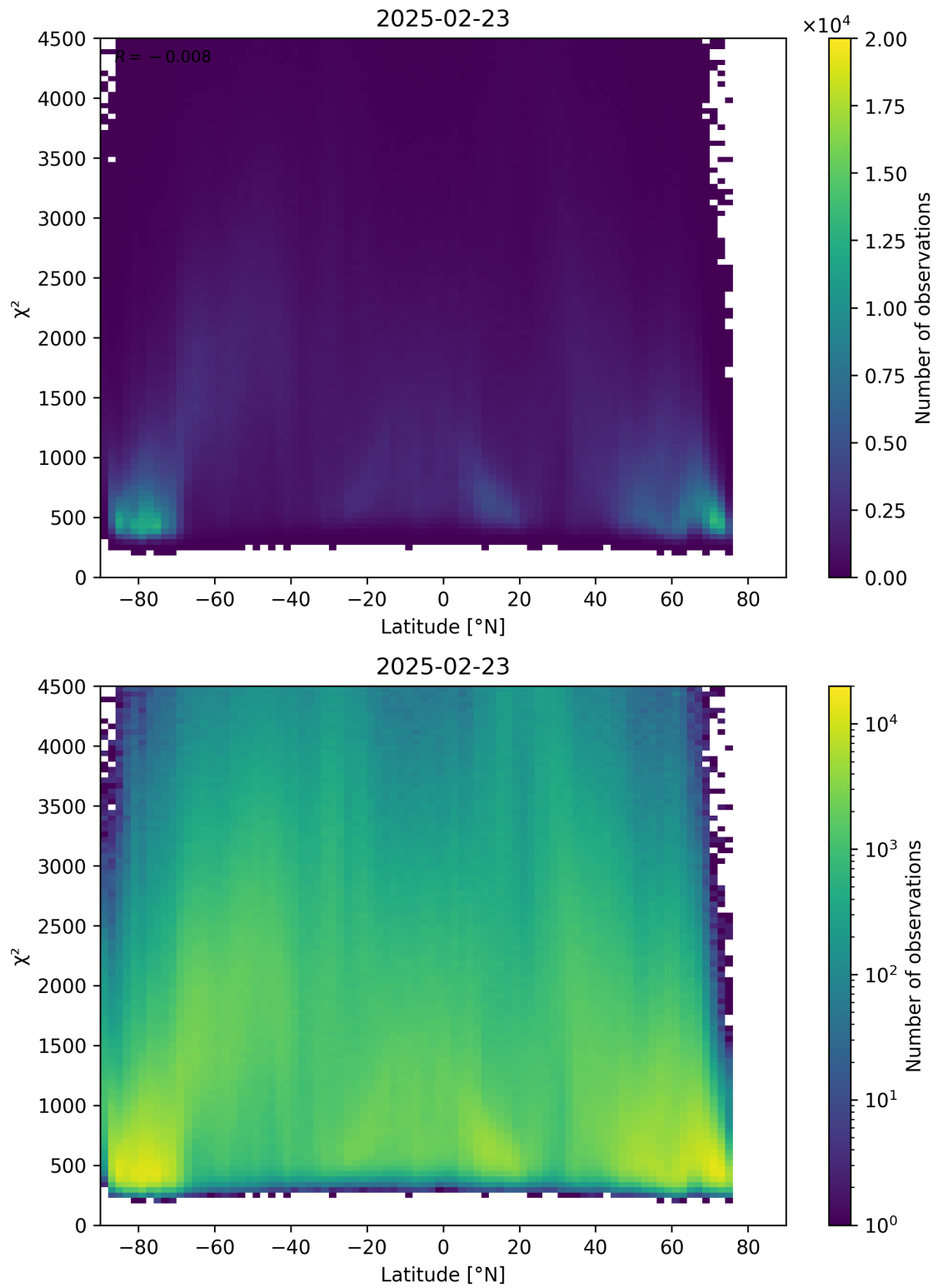
Figure 54: Scatter density plot of “Latitude” against “ \chi^2 ” for 2025-02-22 to 2025-02-24.
