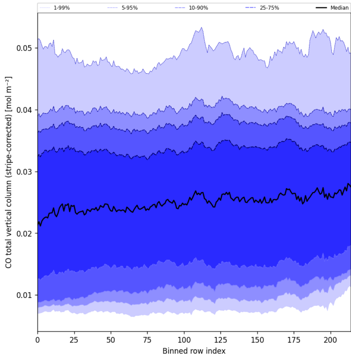
Figure 27: Along track statistics of “CO total vertical column (stripe-corrected)” for 2025-02-22 to 2025-02-24
