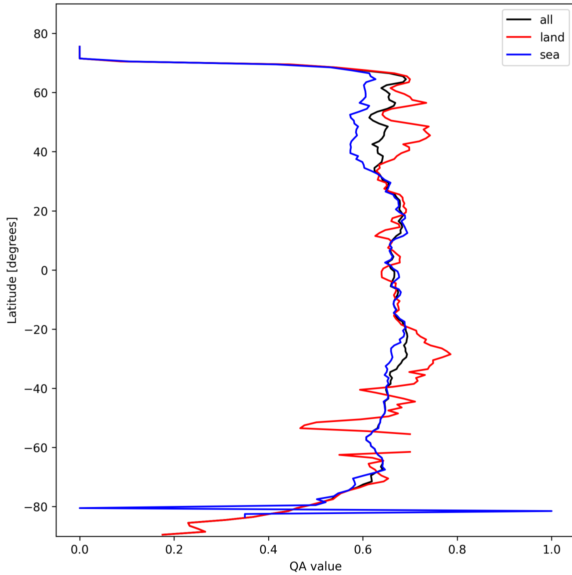
Figure 9: Zonal average of “QA value” for 2025-02-22 to 2025-02-24.
