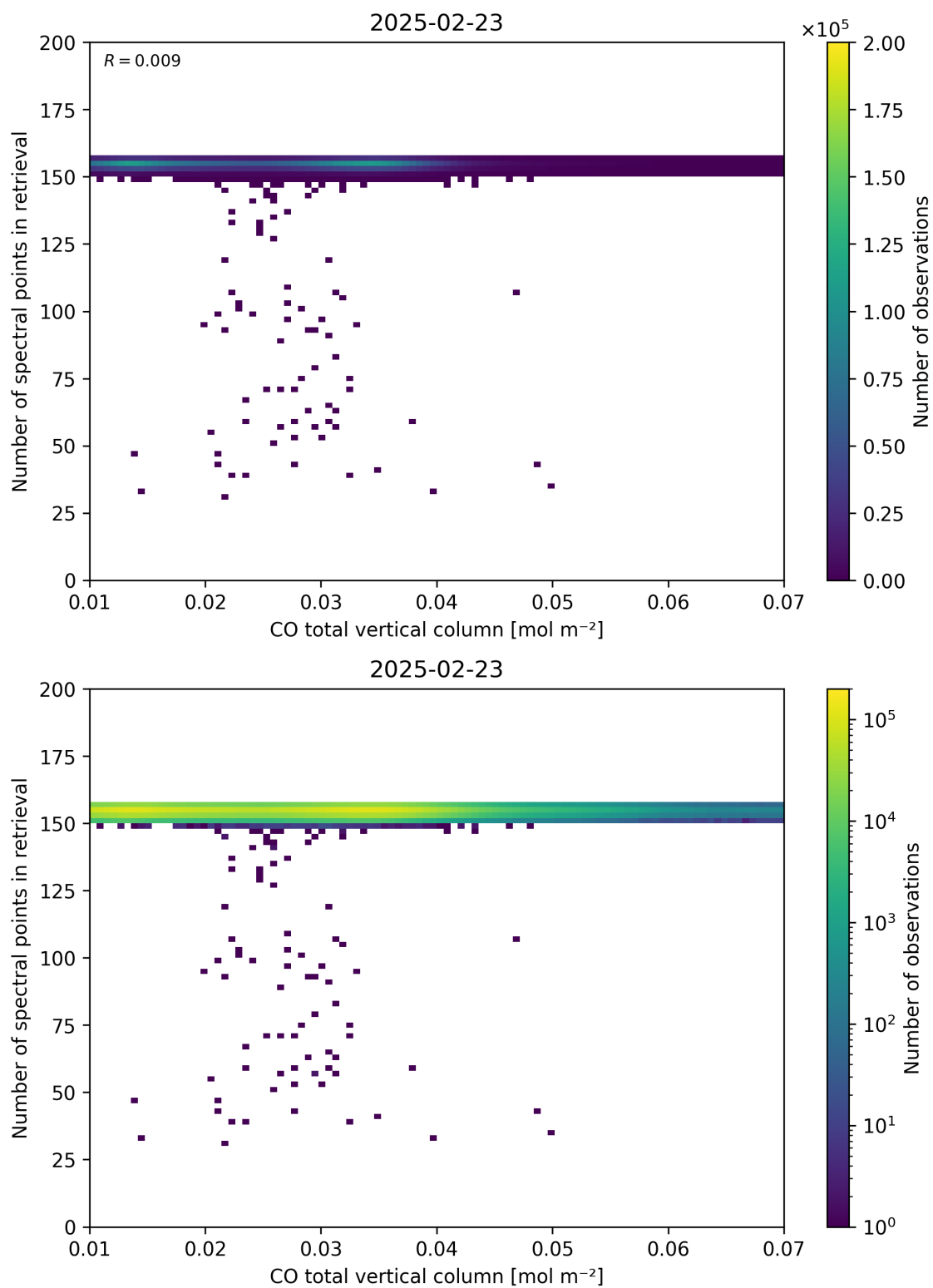
Figure 43: Scatter density plot of “CO total vertical column” against “Number of spectral points in retrieval” for 2025-02-22 to 2025-02-24.
