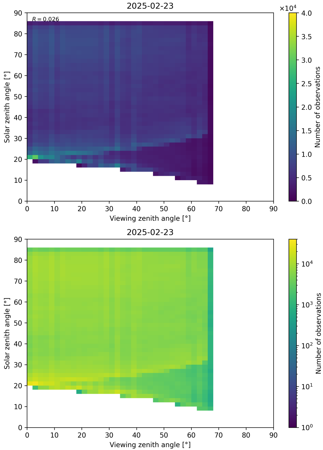
Figure 77: Scatter density plot of “Viewing zenith angle” against “Solar zenith angle” for 2025-02-22 to 2025-02-24.
