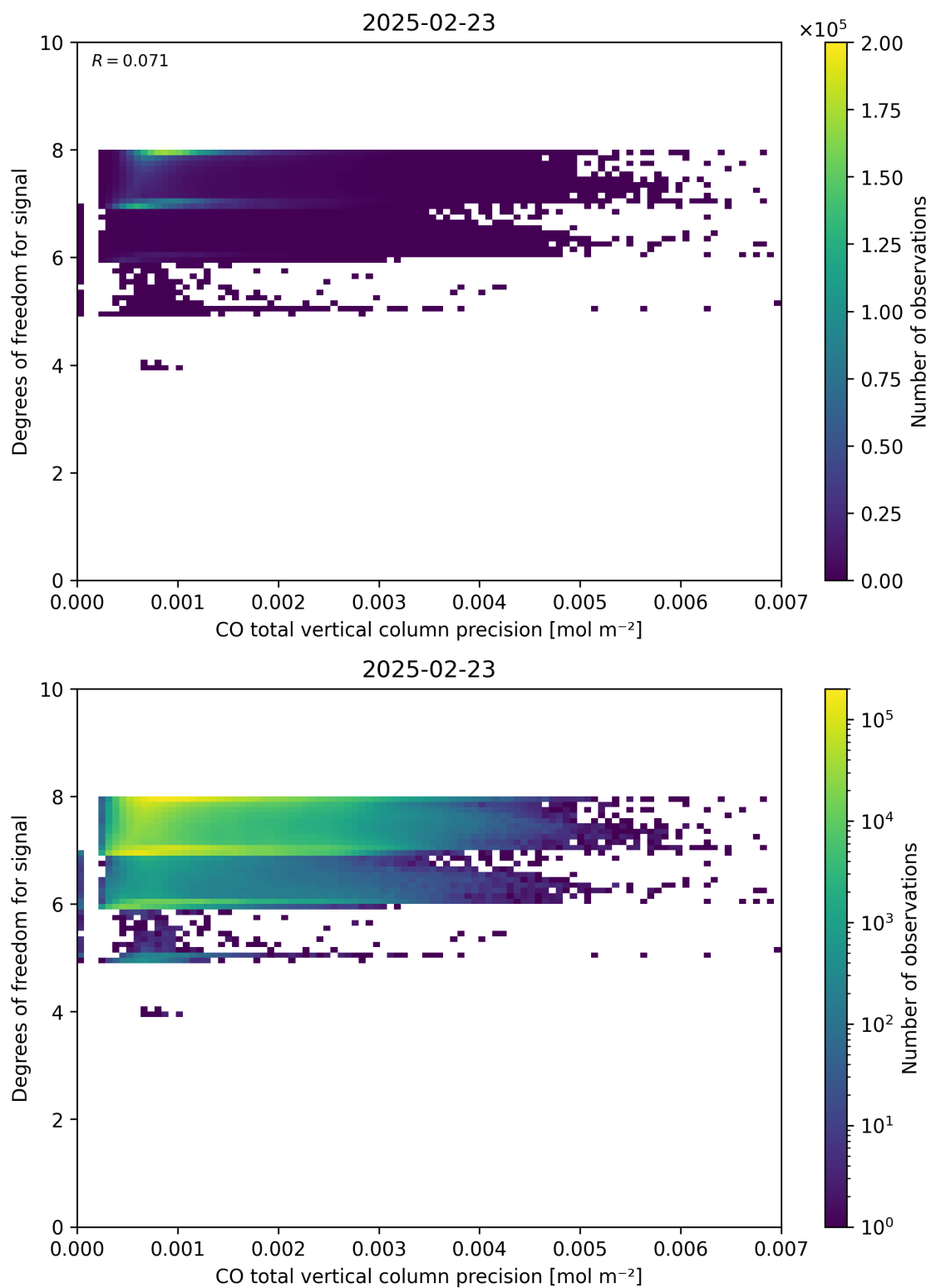
Figure 45: Scatter density plot of “CO total vertical column precision” against “Degrees of freedom for signal” for 2025-02-22 to 2025-02-24.
