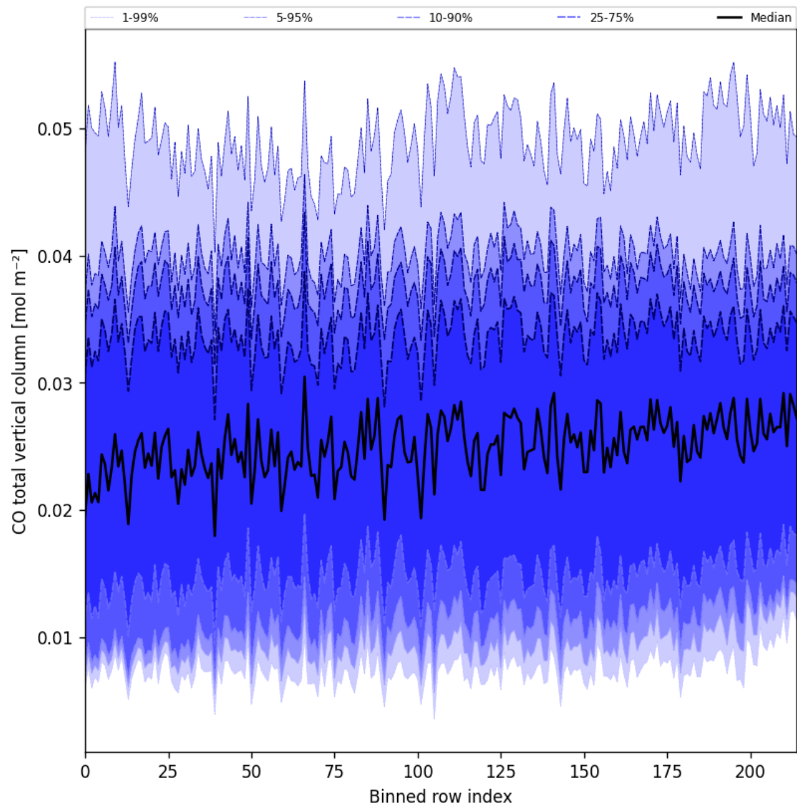
Figure 26: Along track statistics of “CO total vertical column” for 2025-02-22 to 2025-02-24
