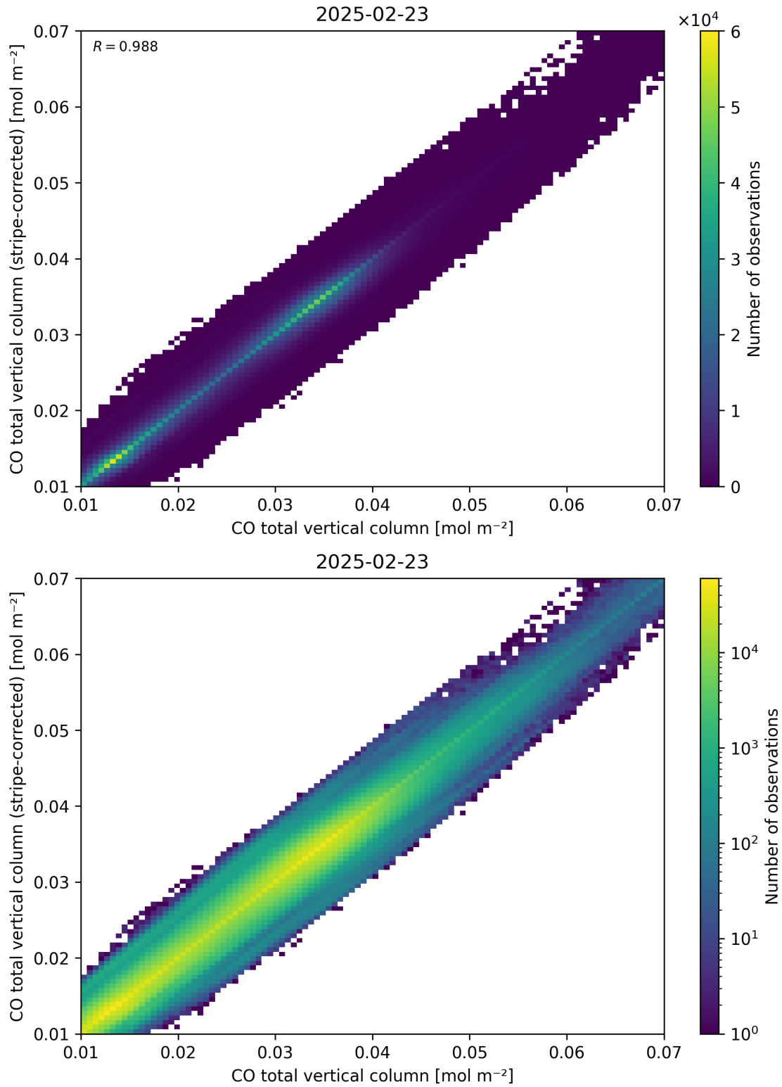
Figure 33: Scatter density plot of “CO total vertical column” against “CO total vertical column (stripe-corrected)” for 2025-02-22 to 2025-02-24.
