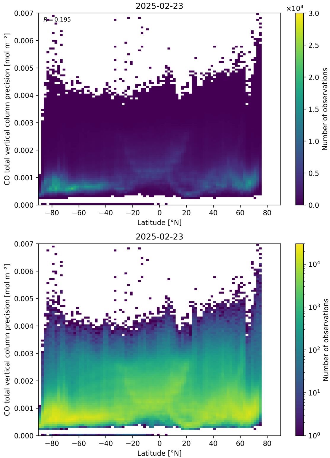
Figure 53: Scatter density plot of “Latitude” against “CO total vertical column precision” for 2025-02-22 to 2025-02-24.
