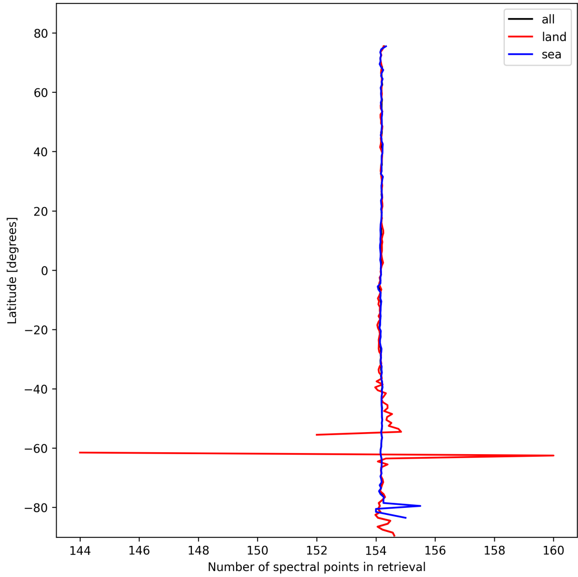
Figure 13: Zonal average of “Number of spectral points in retrieval” for 2025-02-22 to 2025-02-24.
