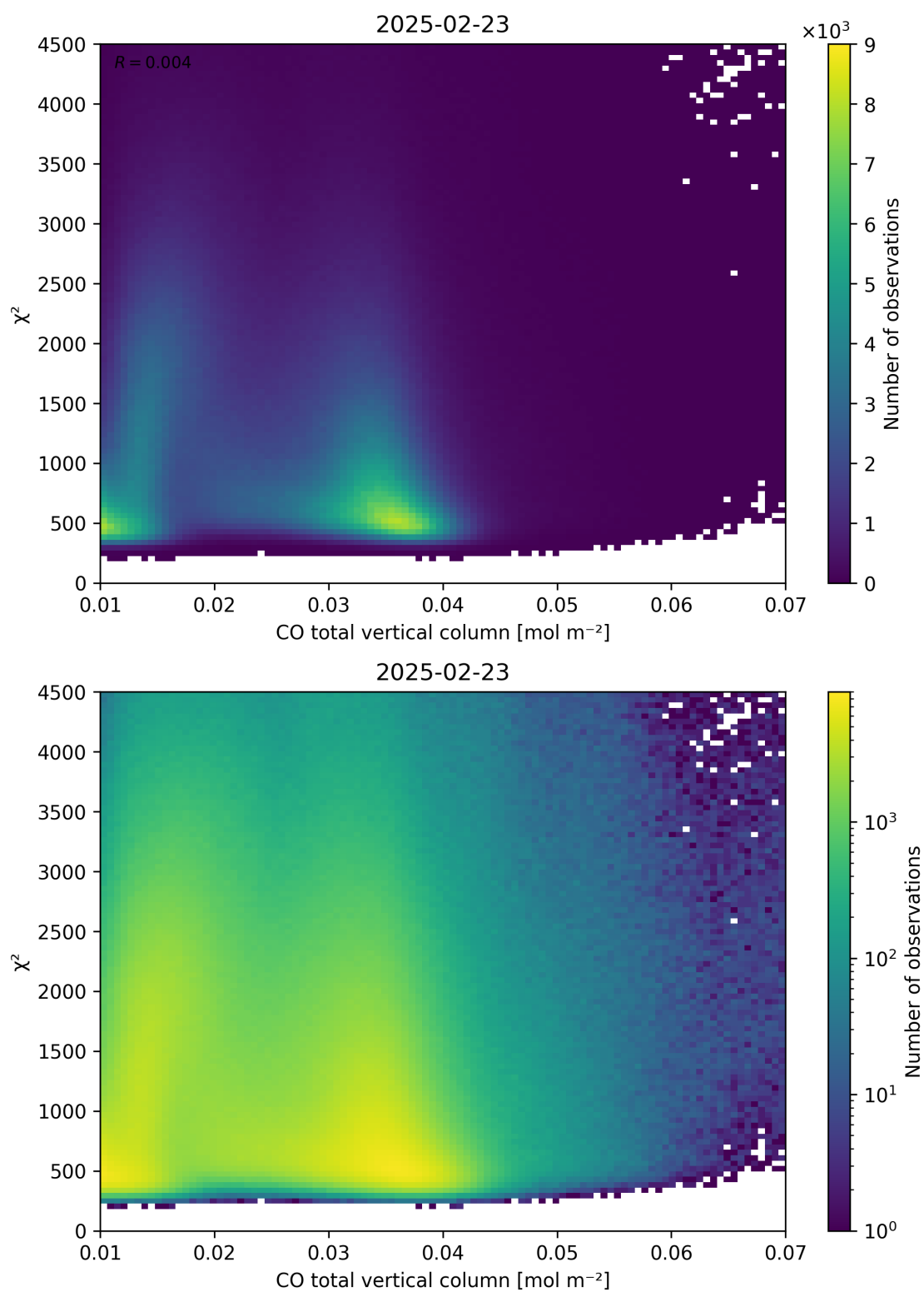
Figure 35: Scatter density plot of “CO total vertical column” against “ \chi^2 ” for 2025-02-22 to 2025-02-24.
