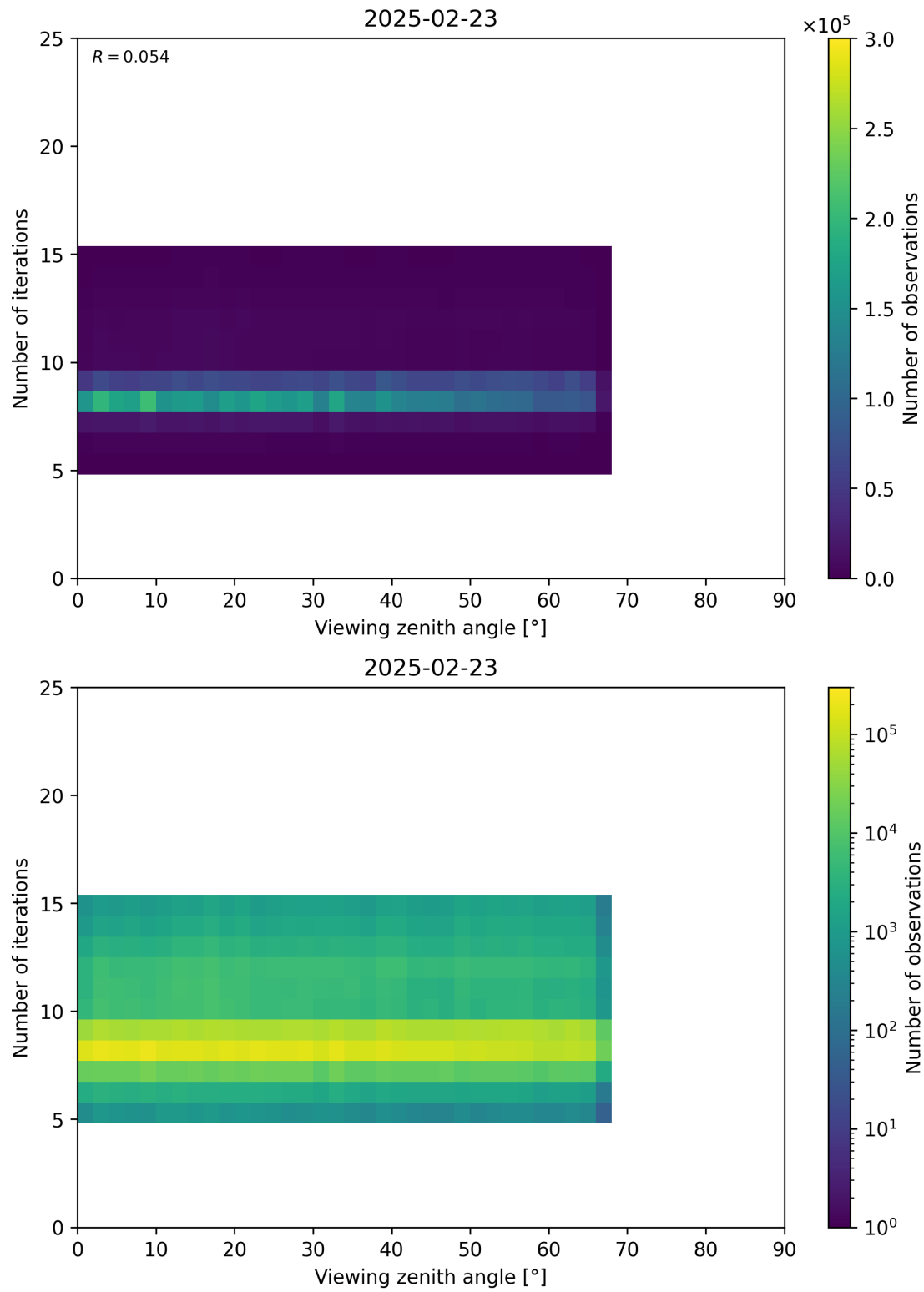
Figure 75: Scatter density plot of “Viewing zenith angle” against “Number of iterations” for 2025-02-22 to 2025-02-24.
