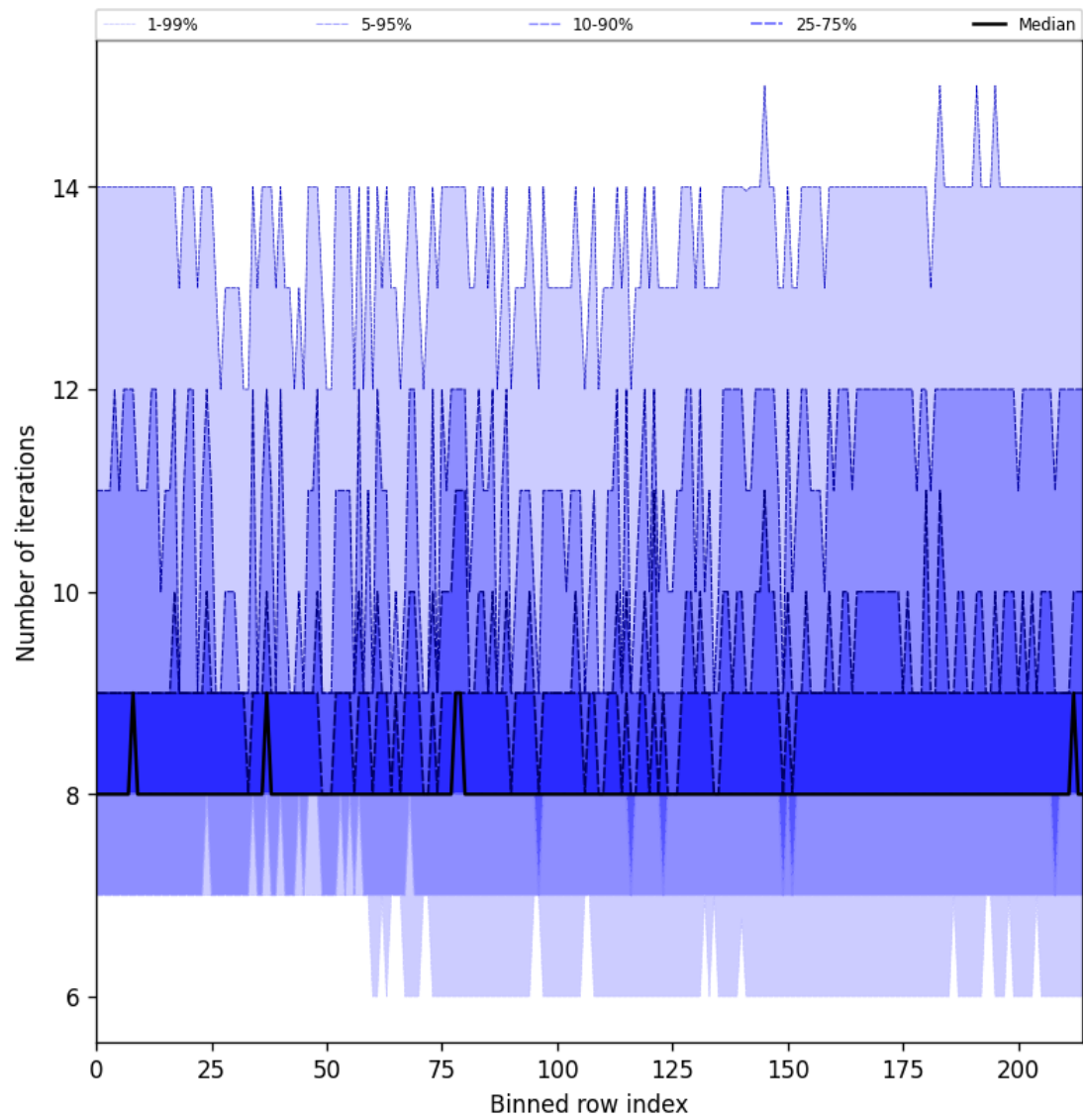
Figure 32: Along track statistics of “Number of iterations” for 2025-02-22 to 2025-02-24
