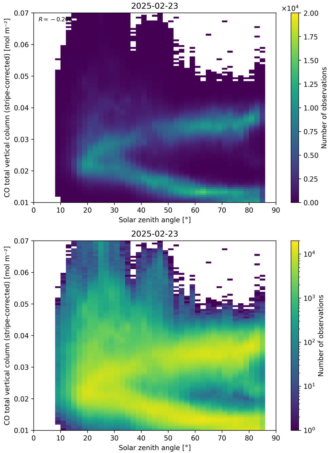
Figure 62: Scatter density plot of “Solar zenith angle” against “CO total vertical column (stripe-corrected)” for 2025-02-22 to 2025-02-24.
