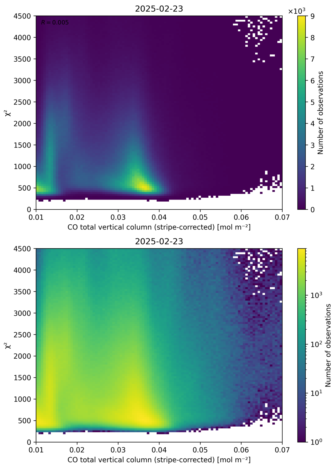
Figure 37: Scatter density plot of “CO total vertical column (stripe-corrected)” against “ \chi^2 ” for 2025-02-22 to 2025-02-24.
