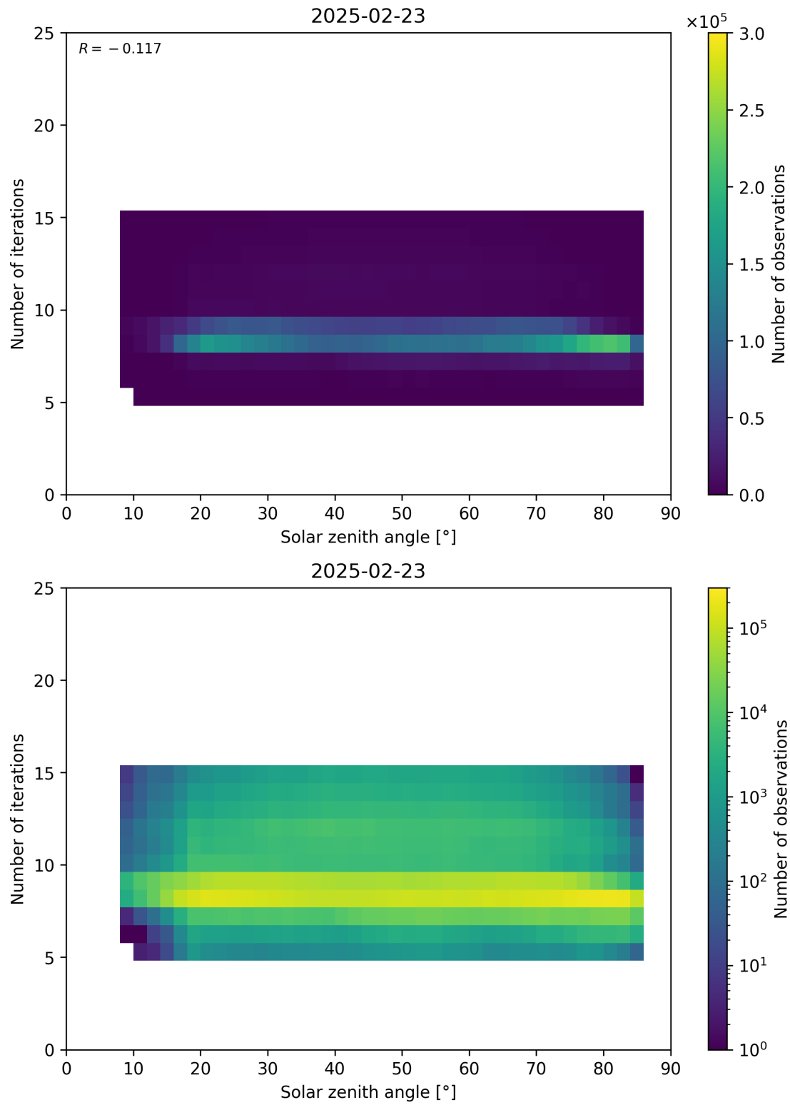
Figure 67: Scatter density plot of “Solar zenith angle” against “Number of iterations” for 2025-02-22 to 2025-02-24.
