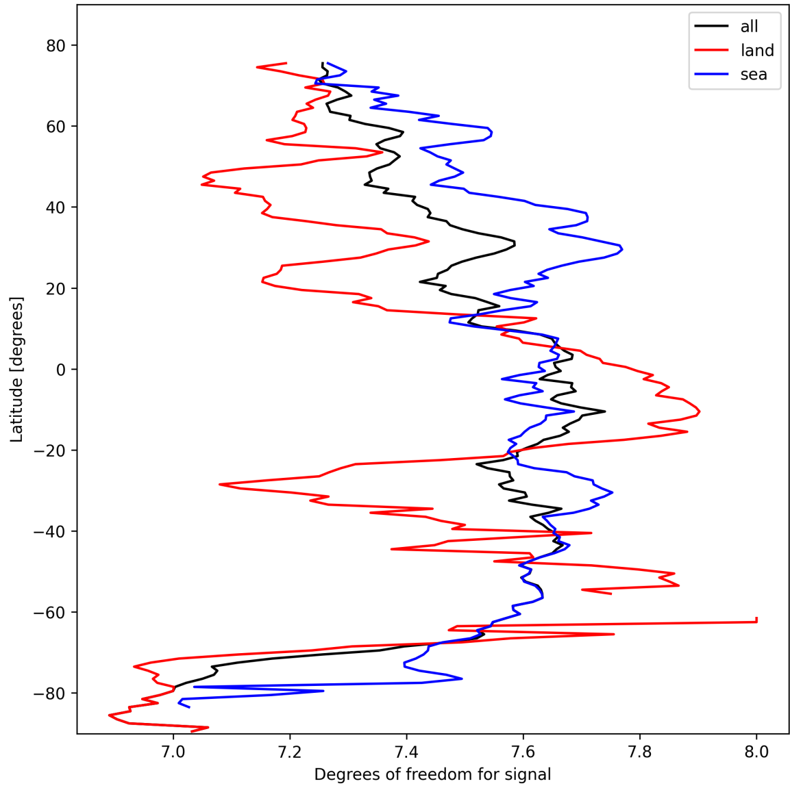
Figure 15: Zonal average of “Degrees of freedom for signal” for 2025-02-22 to 2025-02-24.
