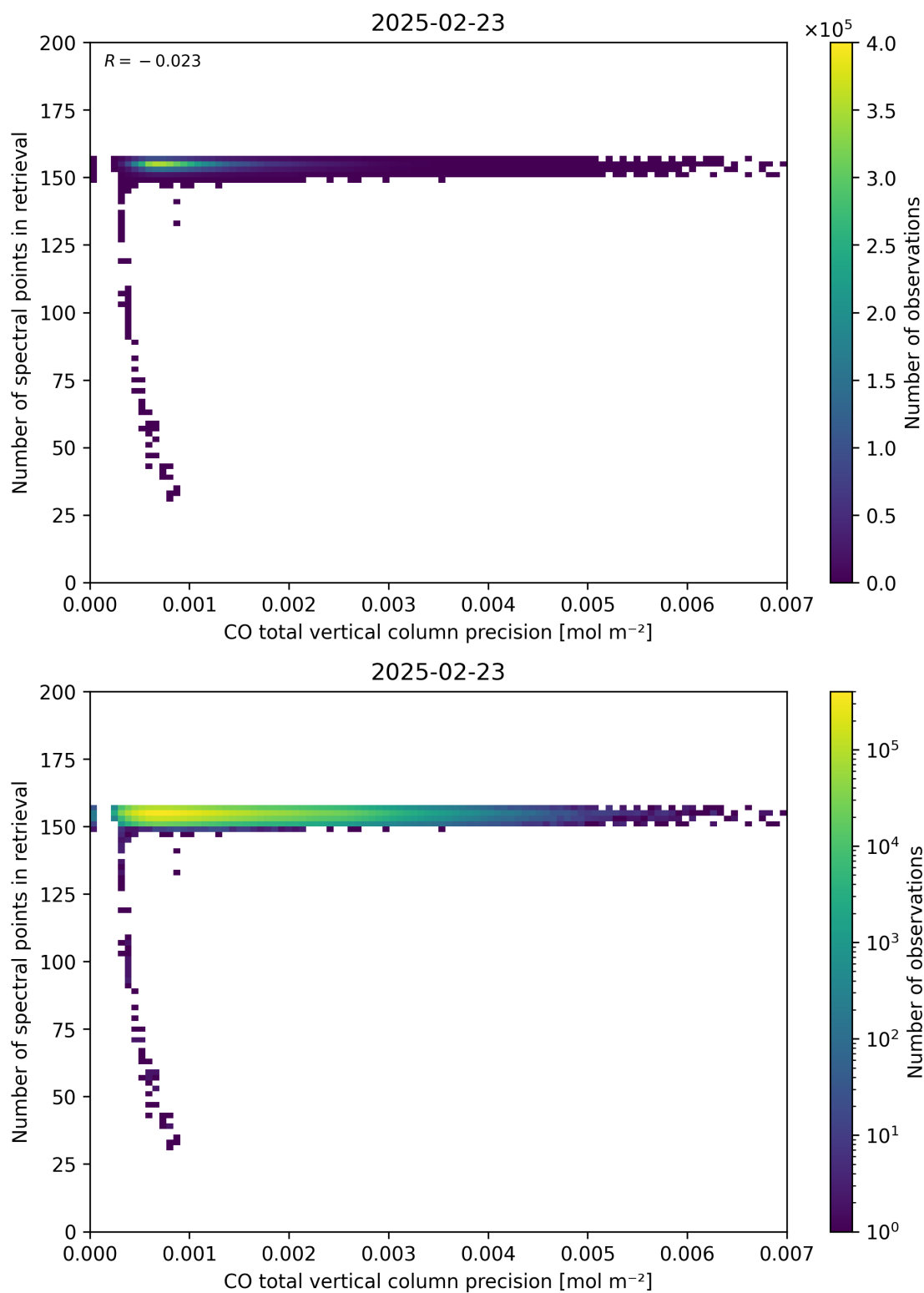
Figure 47: Scatter density plot of “CO total vertical column precision” against “Number of spectral points in retrieval” for 2025-02-22 to 2025-02-24.
