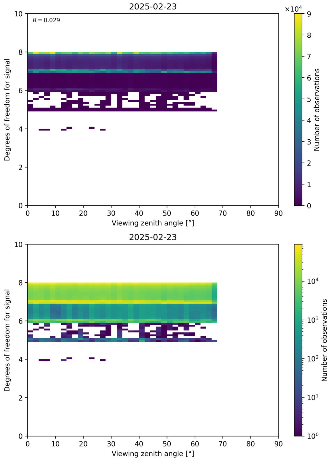
Figure 73: Scatter density plot of “Viewing zenith angle” against “Degrees of freedom for signal” for 2025-02-22 to 2025-02-24.
