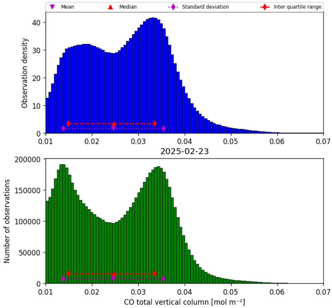
Figure 18: Histogram of “CO total vertical column” for 2025-02-22 to 2025-02-24
