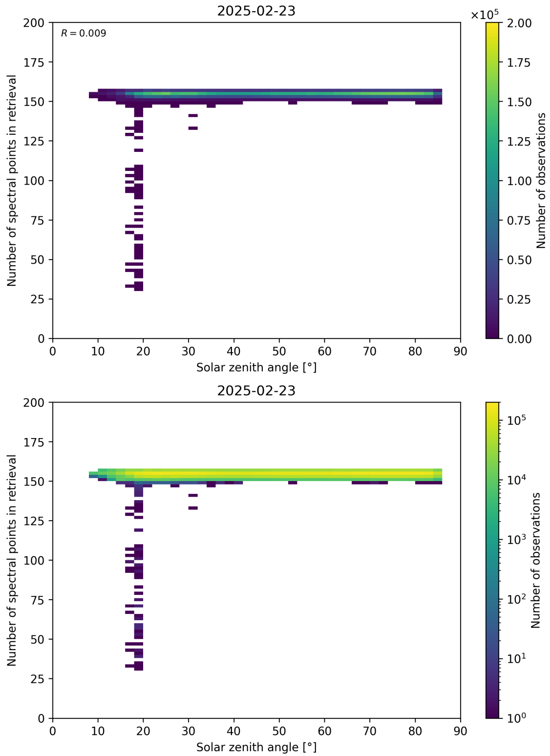
Figure 68: Scatter density plot of “Solar zenith angle” against “Number of spectral points in retrieval” for 2025-02-22 to 2025-02-24.
