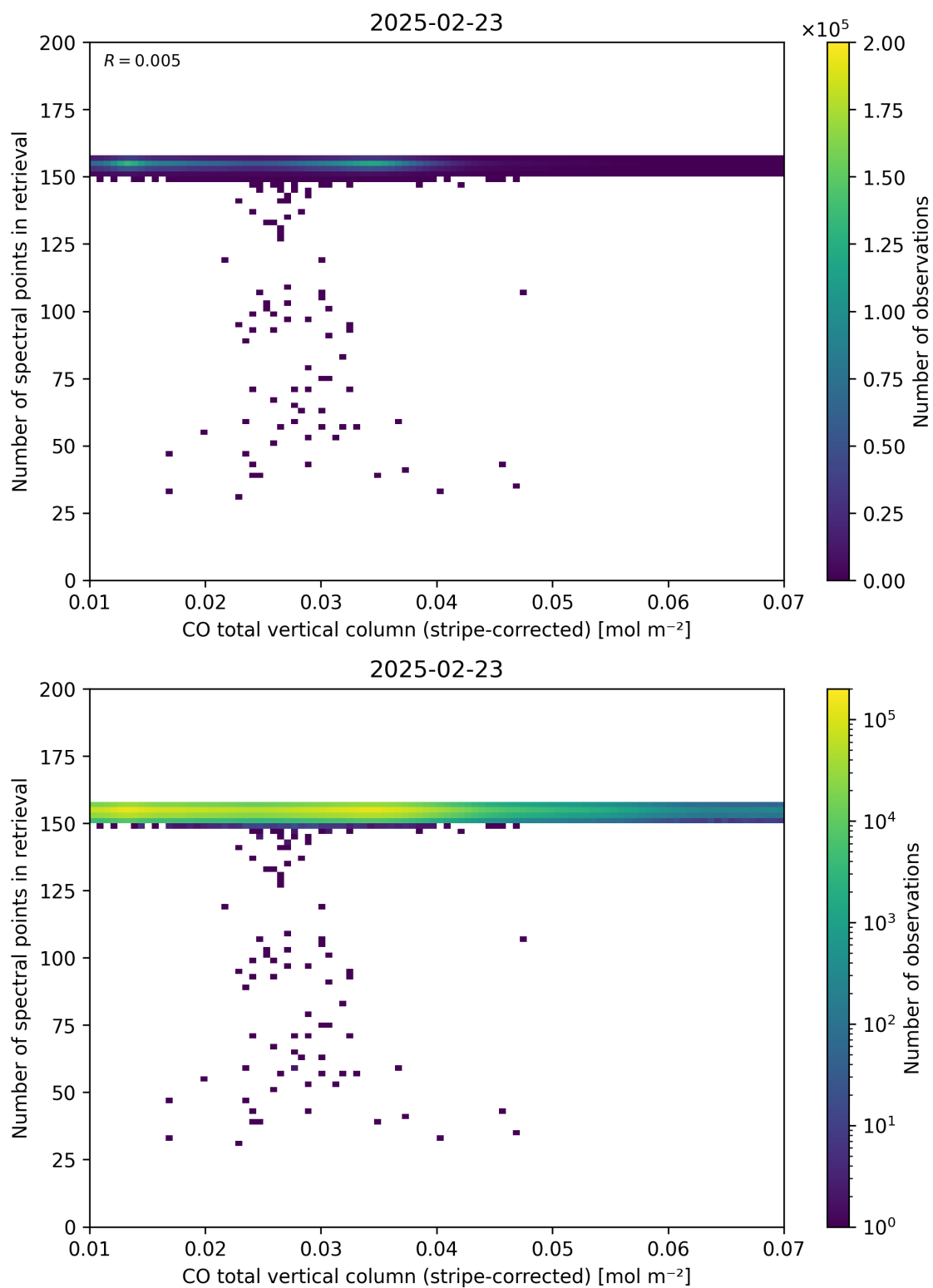
Figure 40: Scatter density plot of “CO total vertical column (stripe-corrected)” against “Number of spectral points in retrieval” for 2025-02-22 to 2025-02-24.
