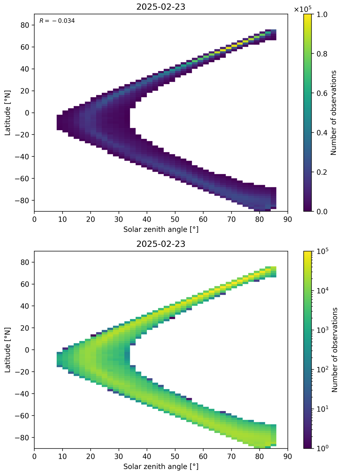
Figure 66: Scatter density plot of “Solar zenith angle” against “Latitude” for 2025-02-22 to 2025-02-24.
