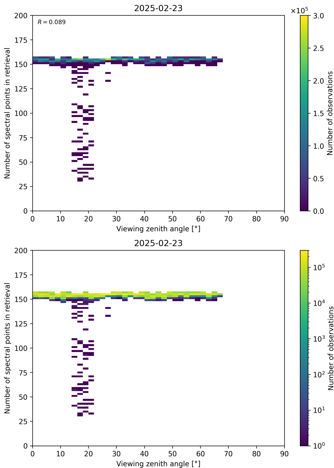
Figure 76: Scatter density plot of “Viewing zenith angle” against “Number of spectral points in retrieval” for 2025-02-22 to 2025-02-24.
