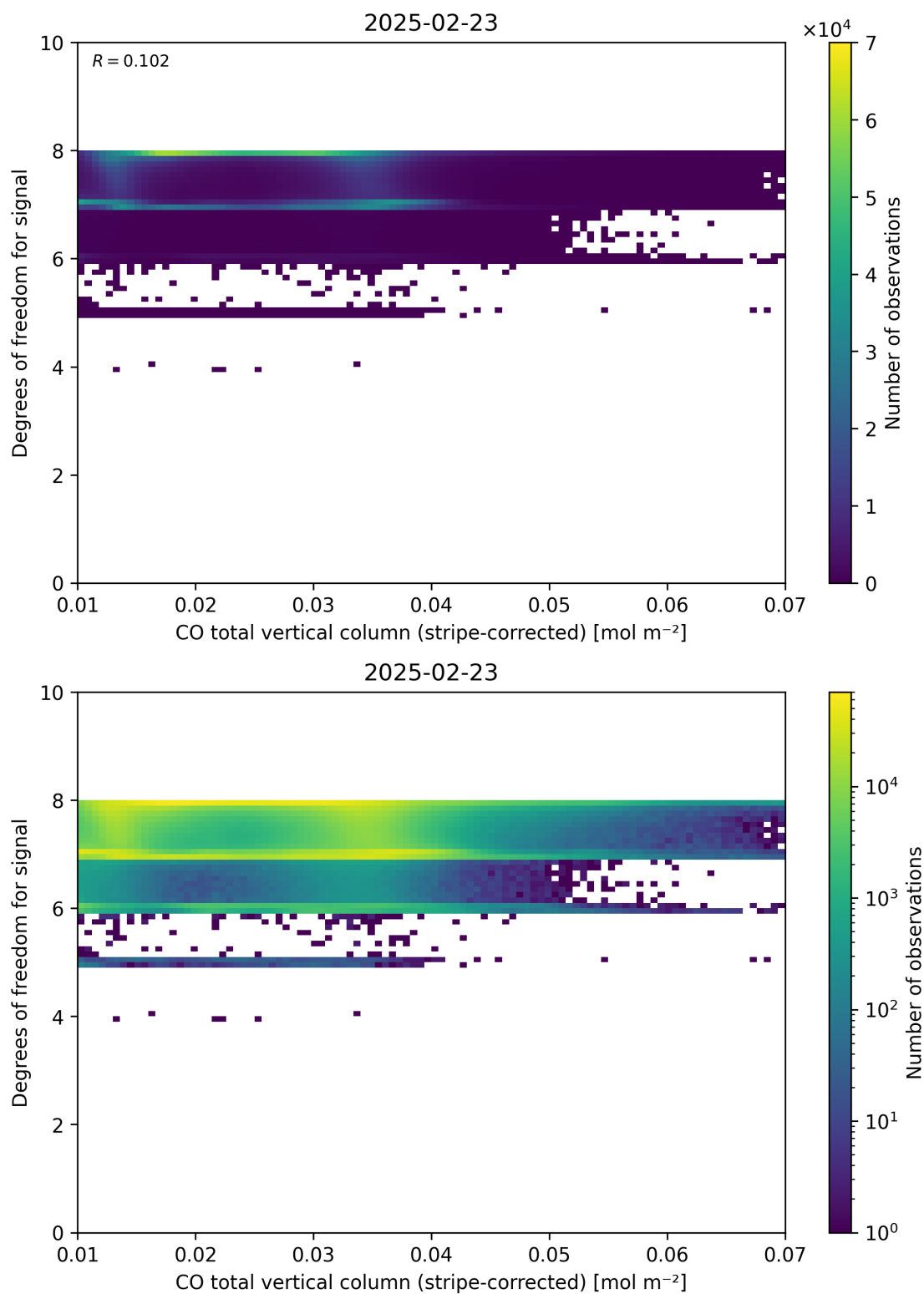
Figure 38: Scatter density plot of “CO total vertical column (stripe-corrected)” against “Degrees of freedom for signal” for 2025-02-22 to 2025-02-24.
