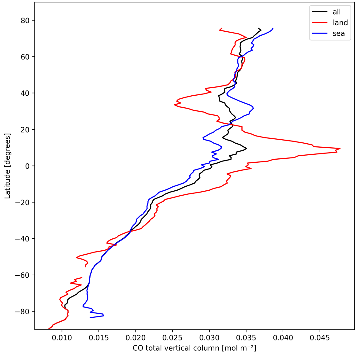
Figure 10: Zonal average of “CO total vertical column” for 2025-02-22 to 2025-02-24.
