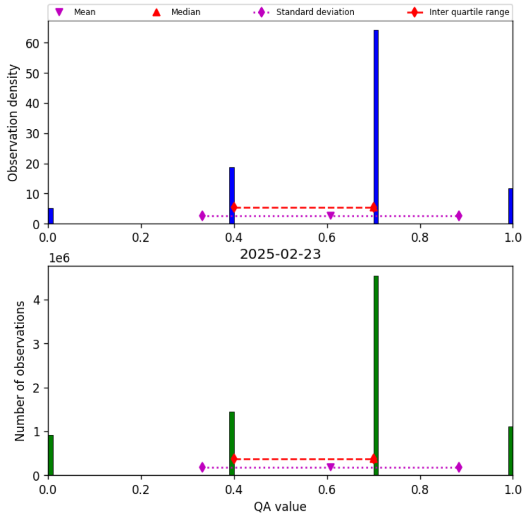
Figure 17: Histogram of “QA value” for 2025-02-22 to 2025-02-24
