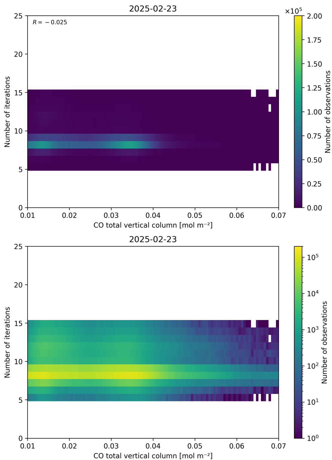
Figure 42: Scatter density plot of “CO total vertical column” against “Number of iterations” for 2025-02-22 to 2025-02-24.
