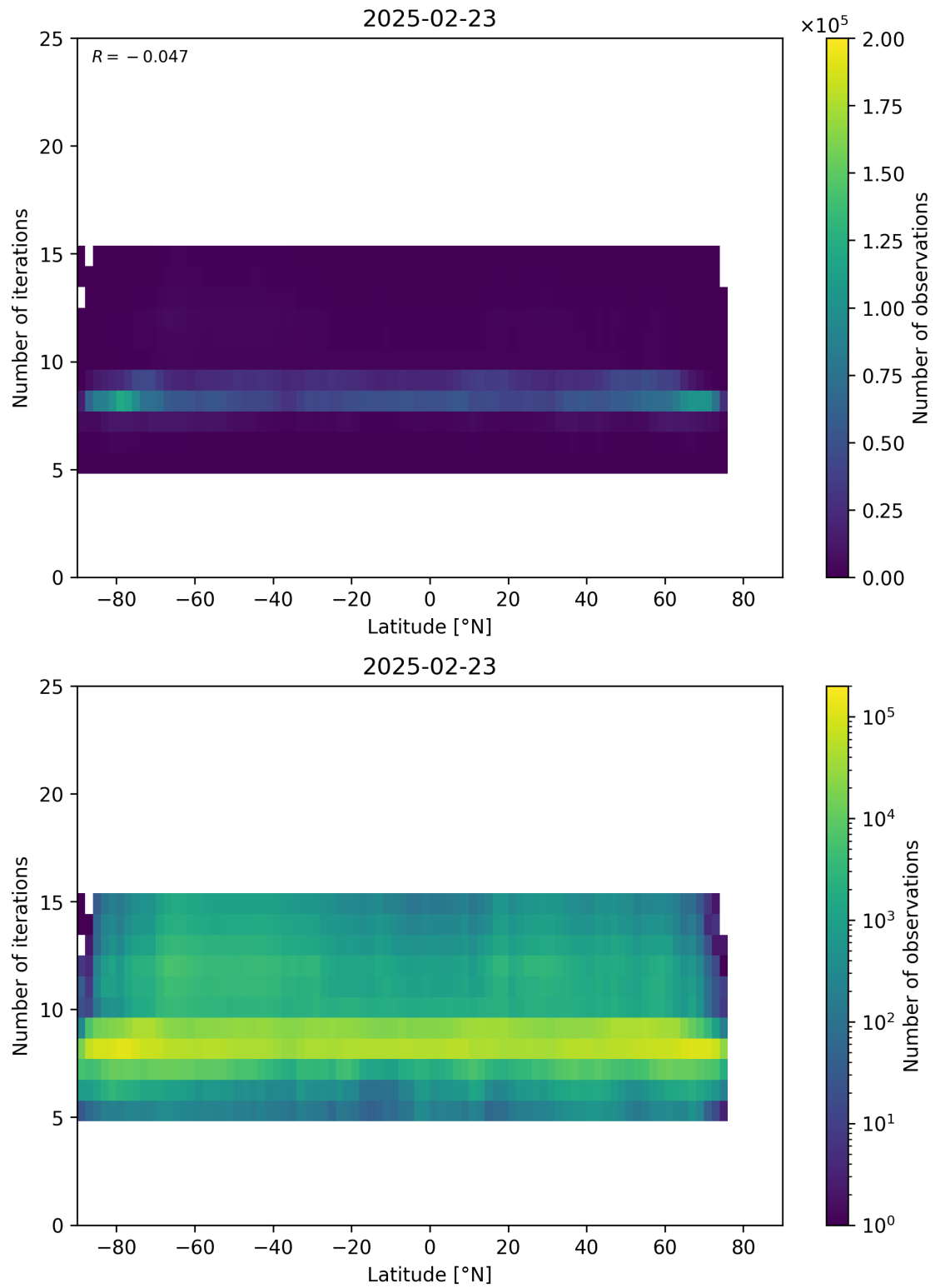
Figure 56: Scatter density plot of “Latitude” against “Number of iterations” for 2025-02-22 to 2025-02-24.
