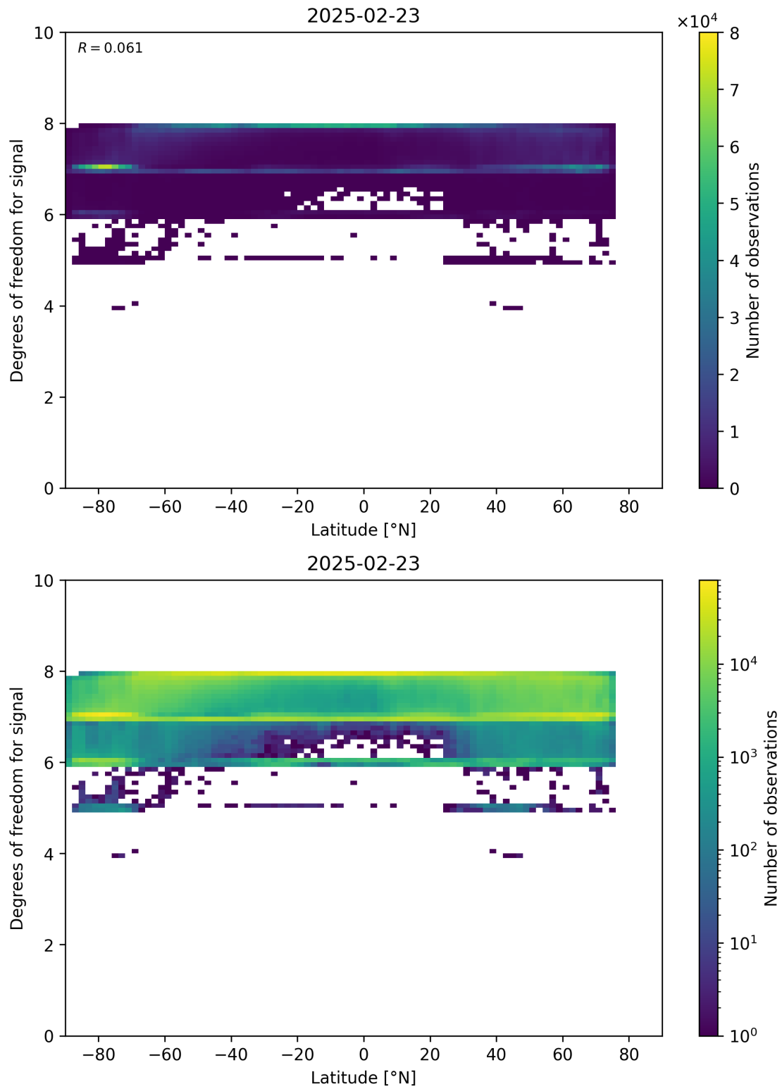
Figure 55: Scatter density plot of “Latitude” against “Degrees of freedom for signal” for 2025-02-22 to 2025-02-24.
