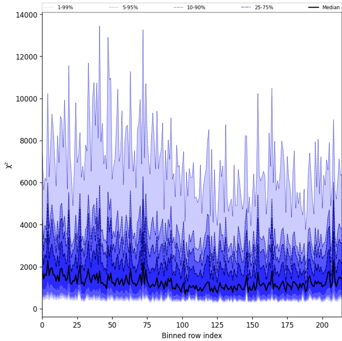
Figure 30: Along track statistics of “ \chi^2 ” for 2025-02-22 to 2025-02-24
