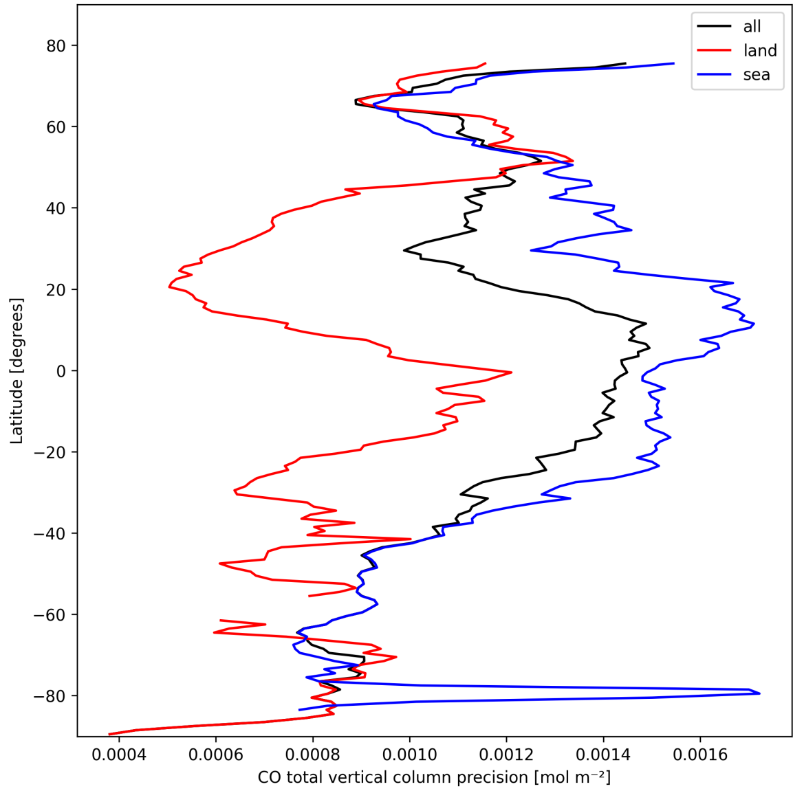
Figure 12: Zonal average of “CO total vertical column precision” for 2025-02-22 to 2025-02-24.
