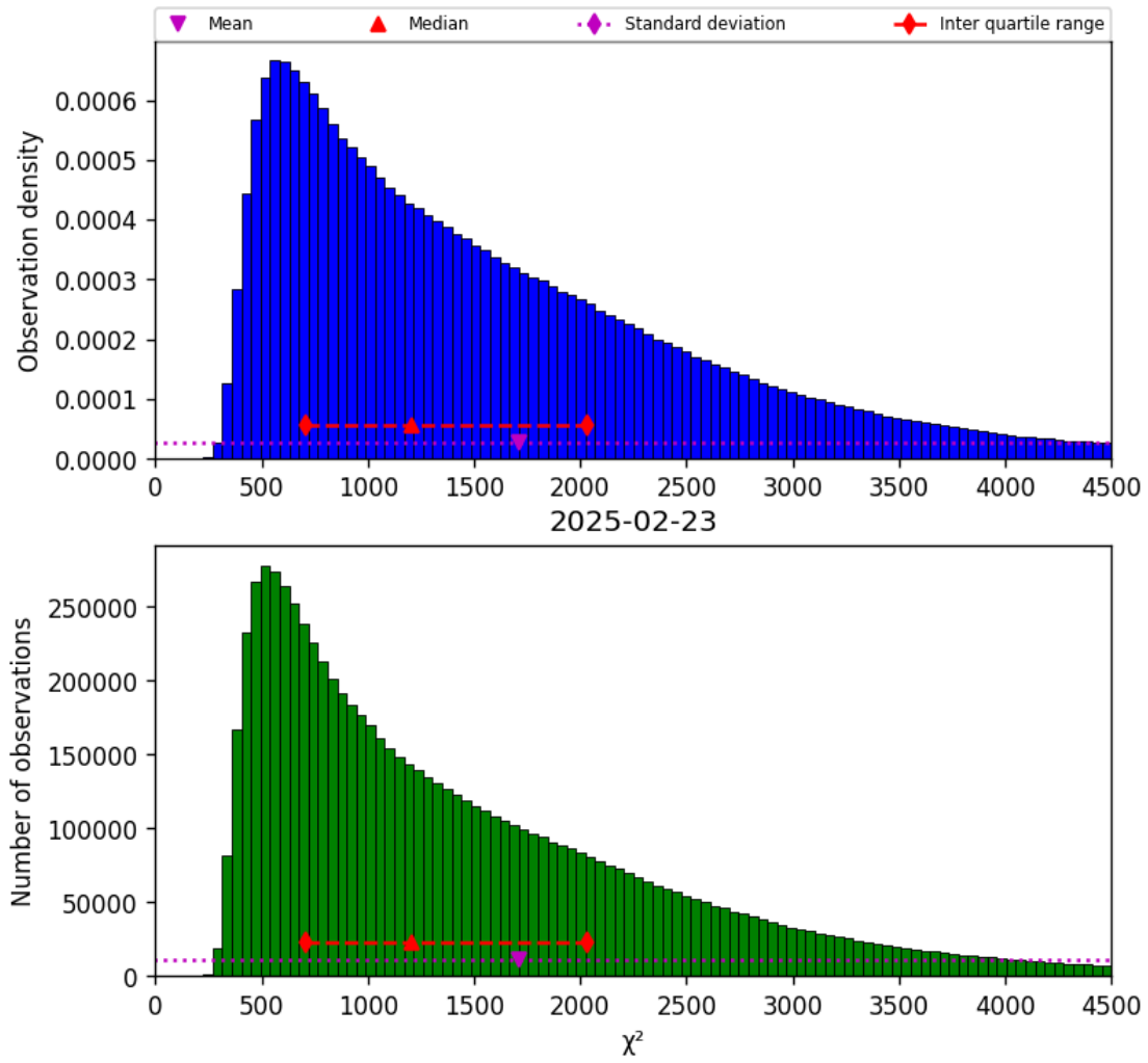
Figure 22: Histogram of “ \chi^2 ” for 2025-02-22 to 2025-02-24
