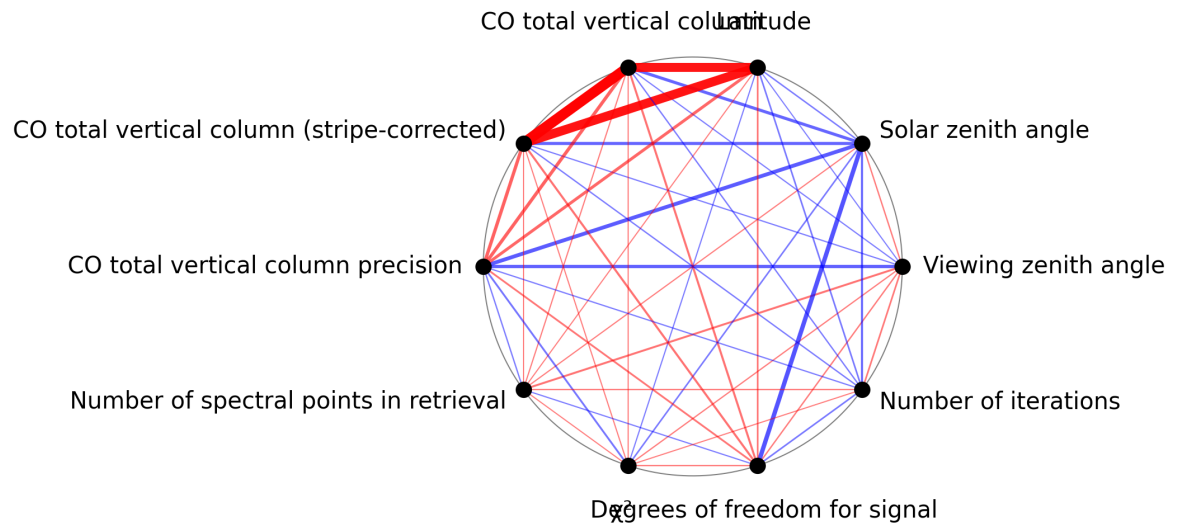
Figure 1: Map of correlation graph for 2025-02-22 to 2025-02-24.
