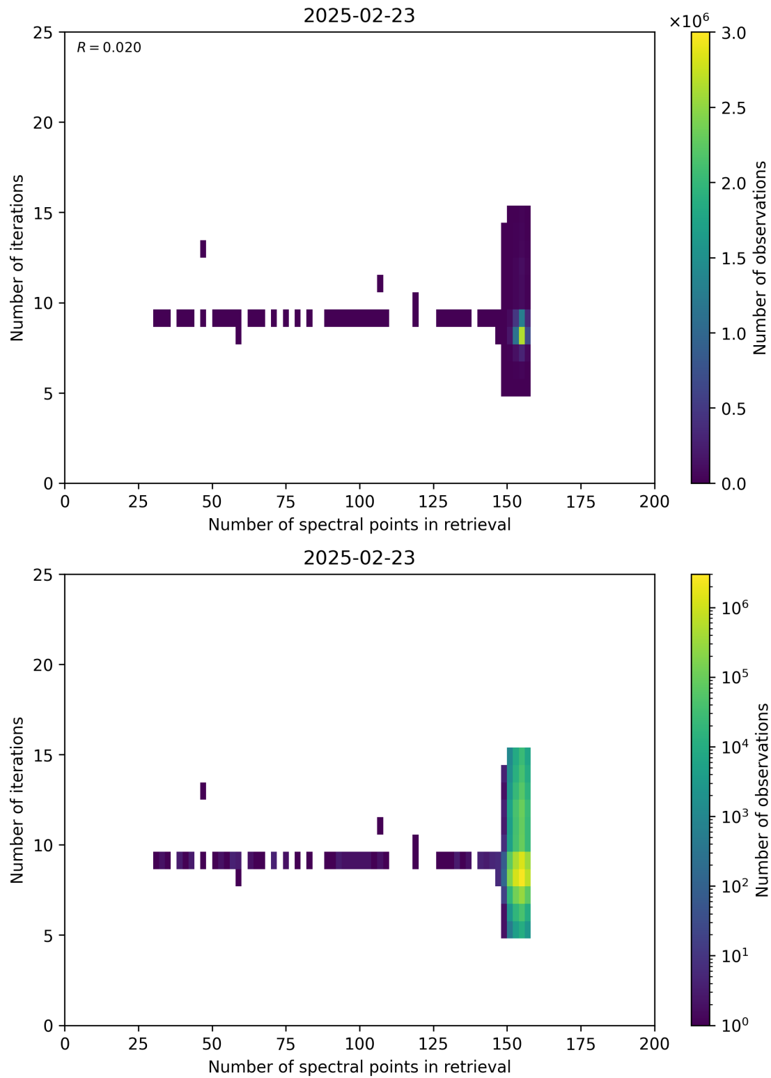
Figure 60: Scatter density plot of “Number of spectral points in retrieval” against “Number of iterations” for 2025-02-22 to 2025-02-24.
