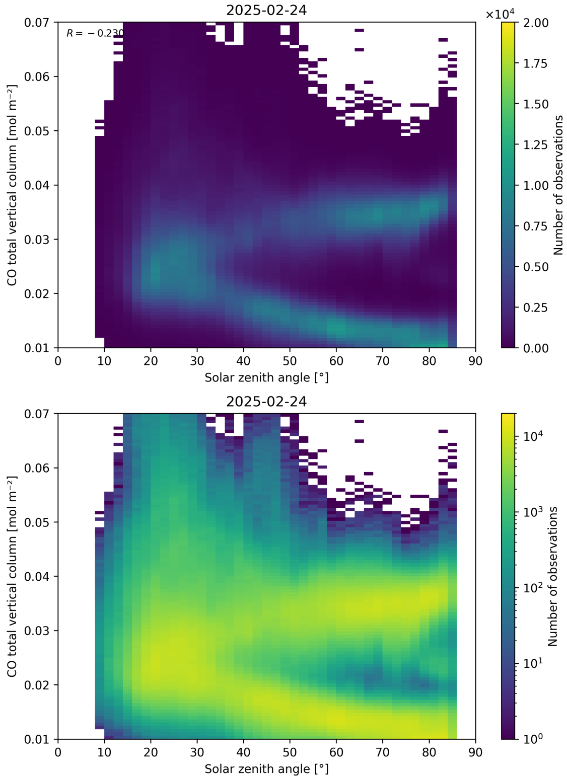
Figure 61: Scatter density plot of “Solar zenith angle” against “CO total vertical column” for 2025-02-24 to 2025-02-25.
