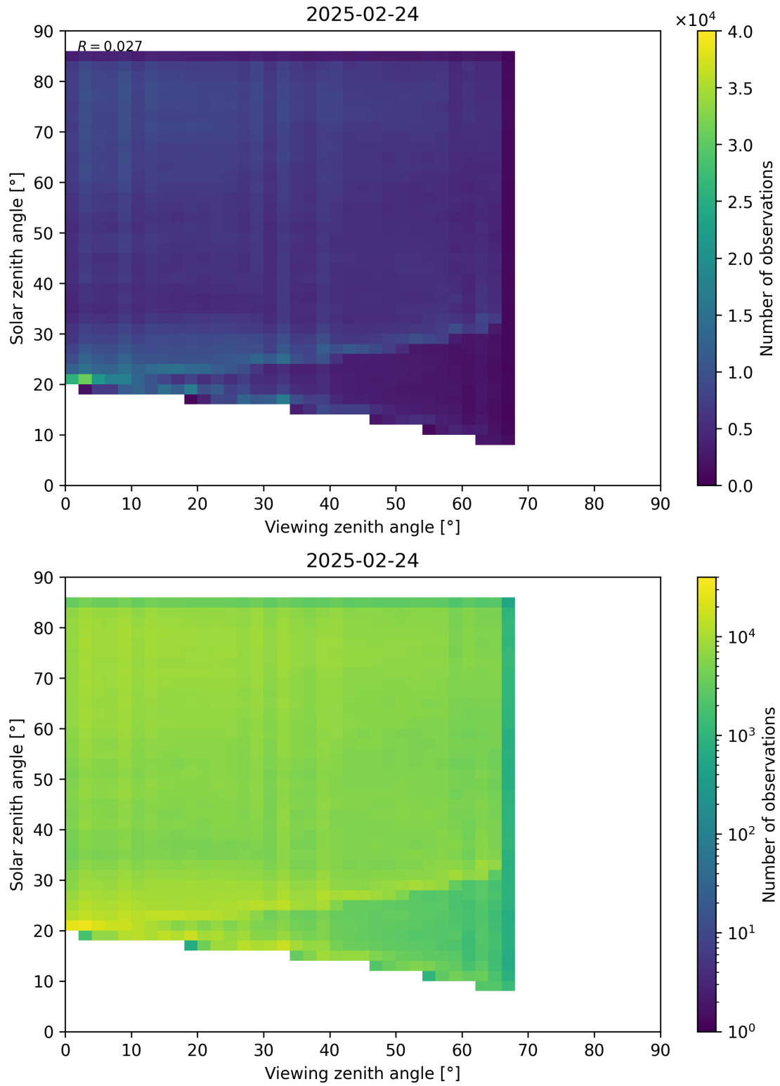
Figure 77: Scatter density plot of “Viewing zenith angle” against “Solar zenith angle” for 2025-02-24 to 2025-02-25.
