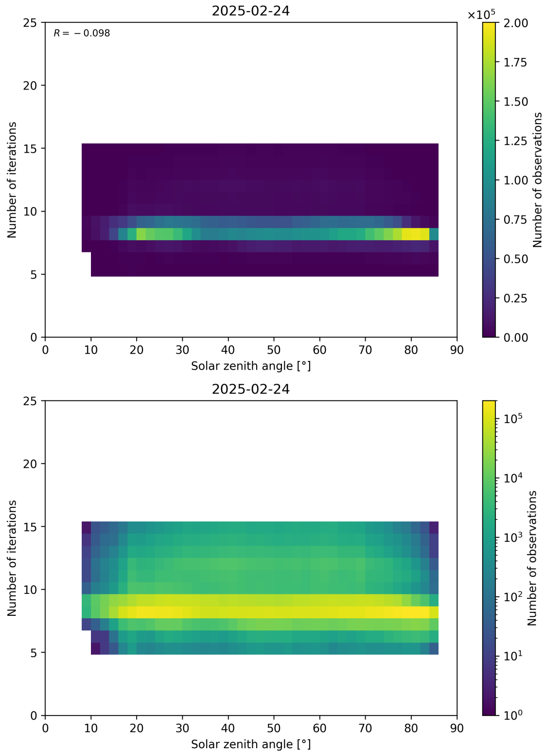
Figure 67: Scatter density plot of “Solar zenith angle” against “Number of iterations” for 2025-02-24 to 2025-02-25.
