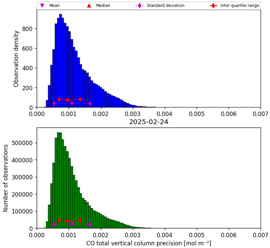
Figure 20: Histogram of “CO total vertical column precision” for 2025-02-24 to 2025-02-25
