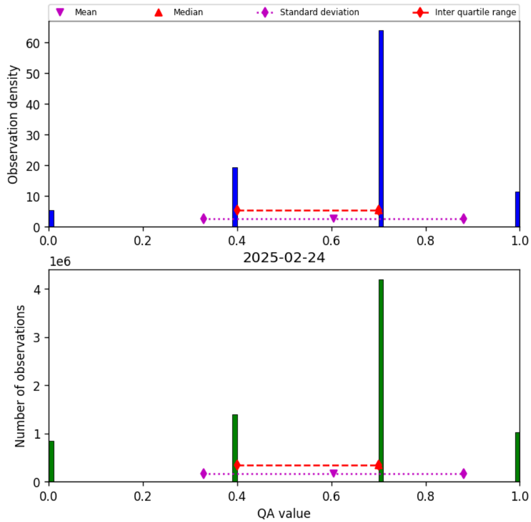
Figure 17: Histogram of “QA value” for 2025-02-24 to 2025-02-25
