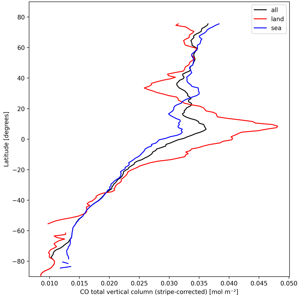
Figure 11: Zonal average of “CO total vertical column (stripe-corrected)” for 2025-02-24 to 2025-02-25.
