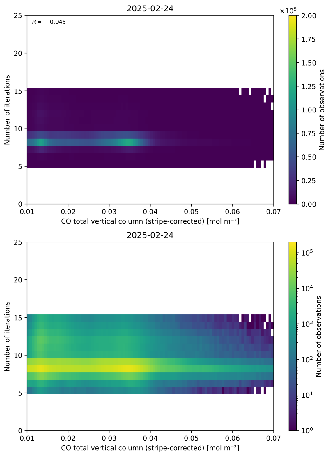
Figure 39: Scatter density plot of “CO total vertical column (stripe-corrected)” against “Number of iterations” for 2025-02-24 to 2025-02-25.
