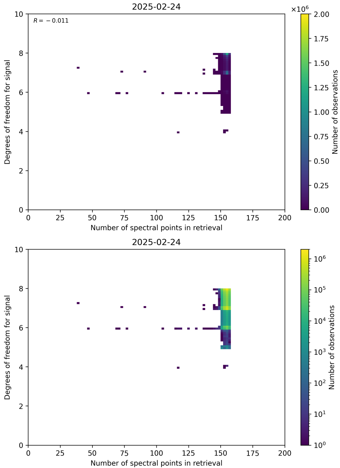
Figure 59: Scatter density plot of “Number of spectral points in retrieval” against “Degrees of freedom for signal” for 2025-02-24 to 2025-02-25.
