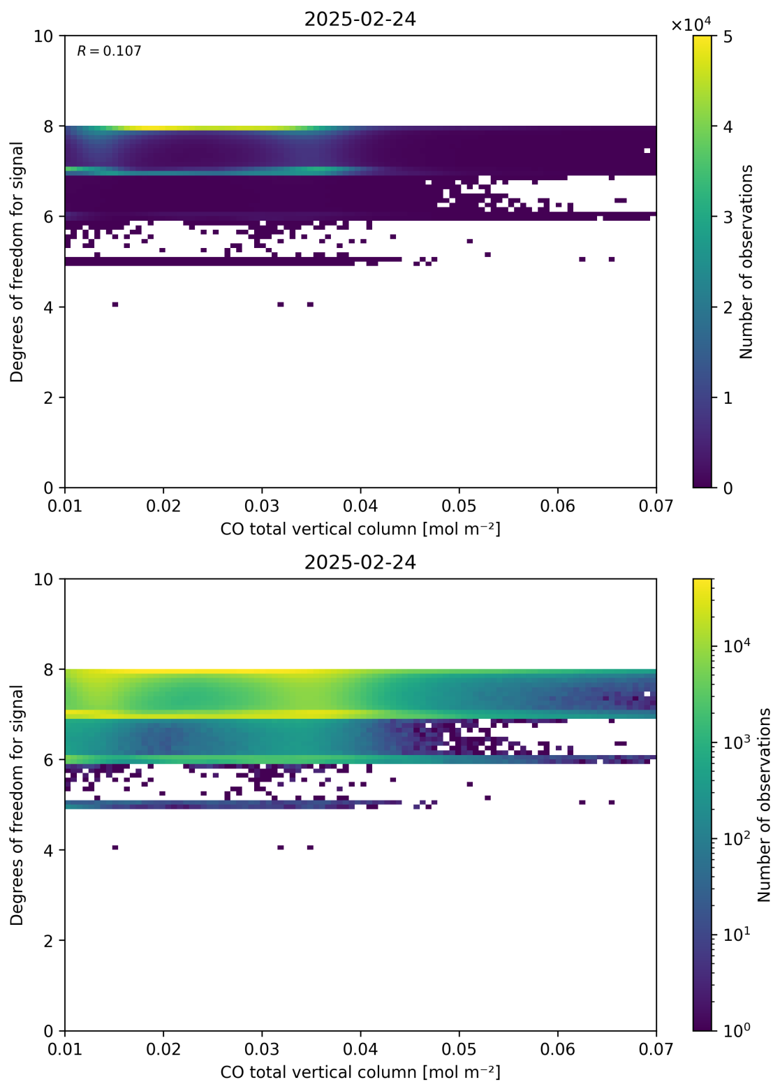
Figure 41: Scatter density plot of “CO total vertical column” against “Degrees of freedom for signal” for 2025-02-24 to 2025-02-25.
