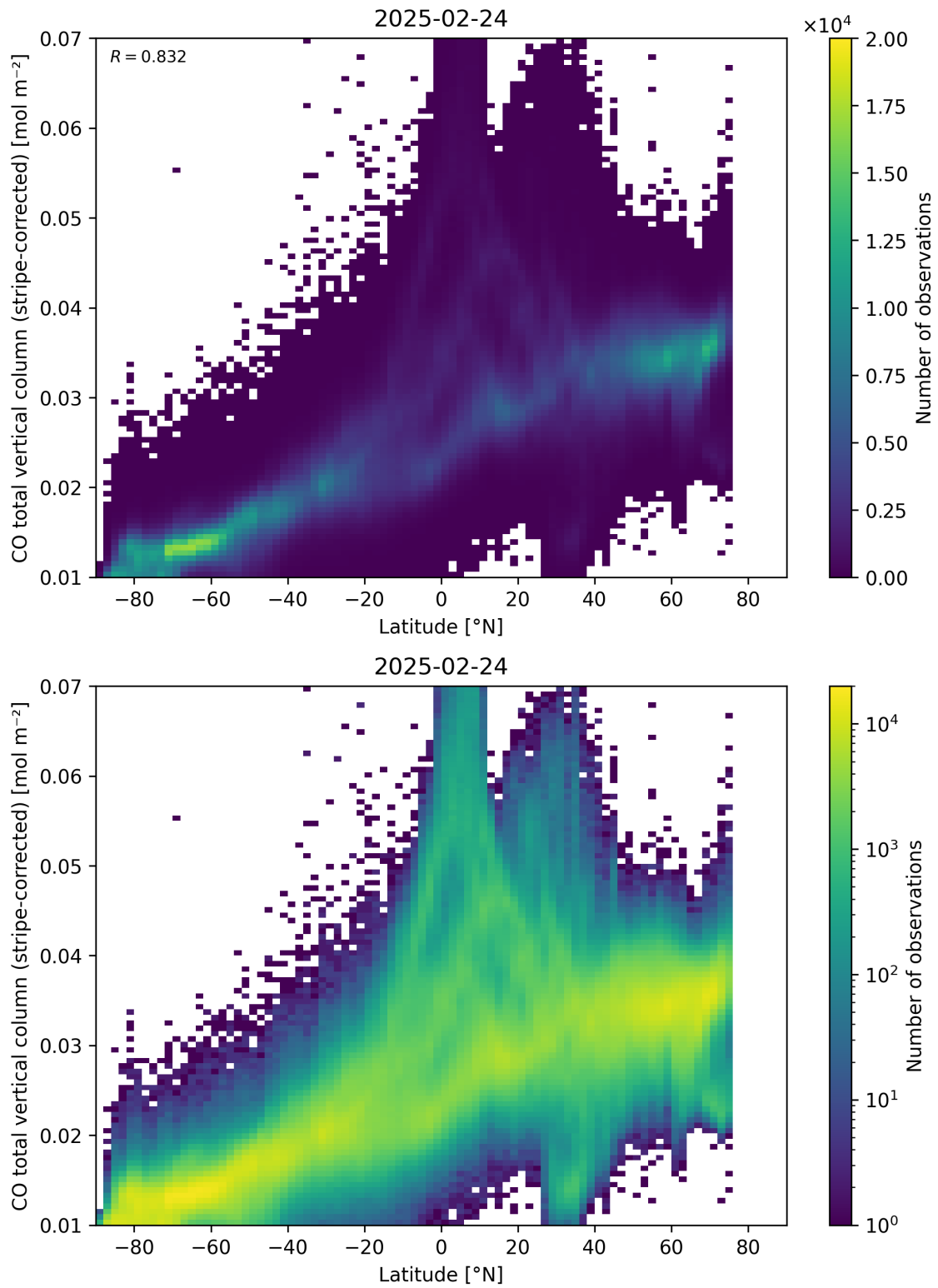
Figure 52: Scatter density plot of “Latitude” against “CO total vertical column (stripe-corrected)” for 2025-02-24 to 2025-02-25.
