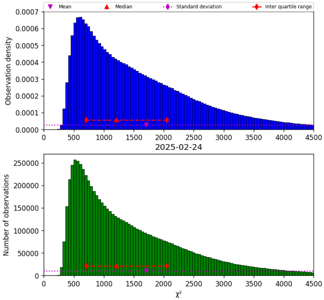
Figure 22: Histogram of “ \chi^2 ” for 2025-02-24 to 2025-02-25
