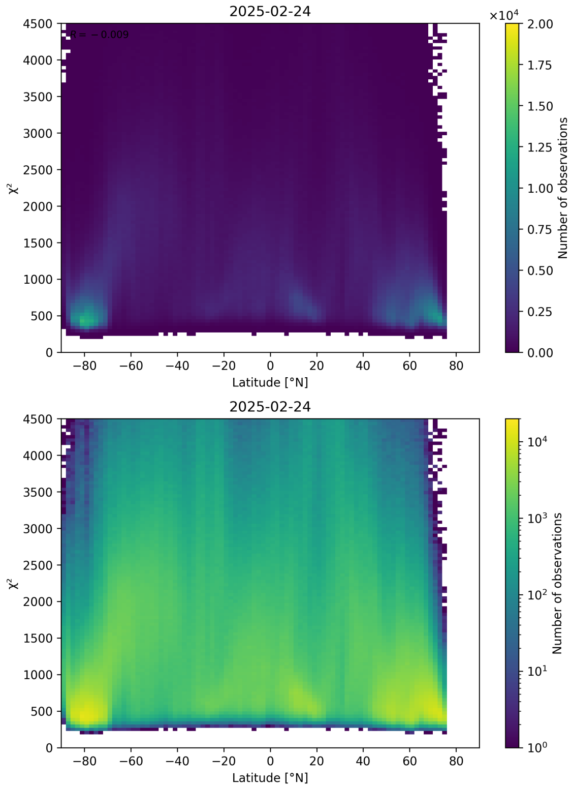
Figure 54: Scatter density plot of “Latitude” against “ \chi^2 ” for 2025-02-24 to 2025-02-25.
