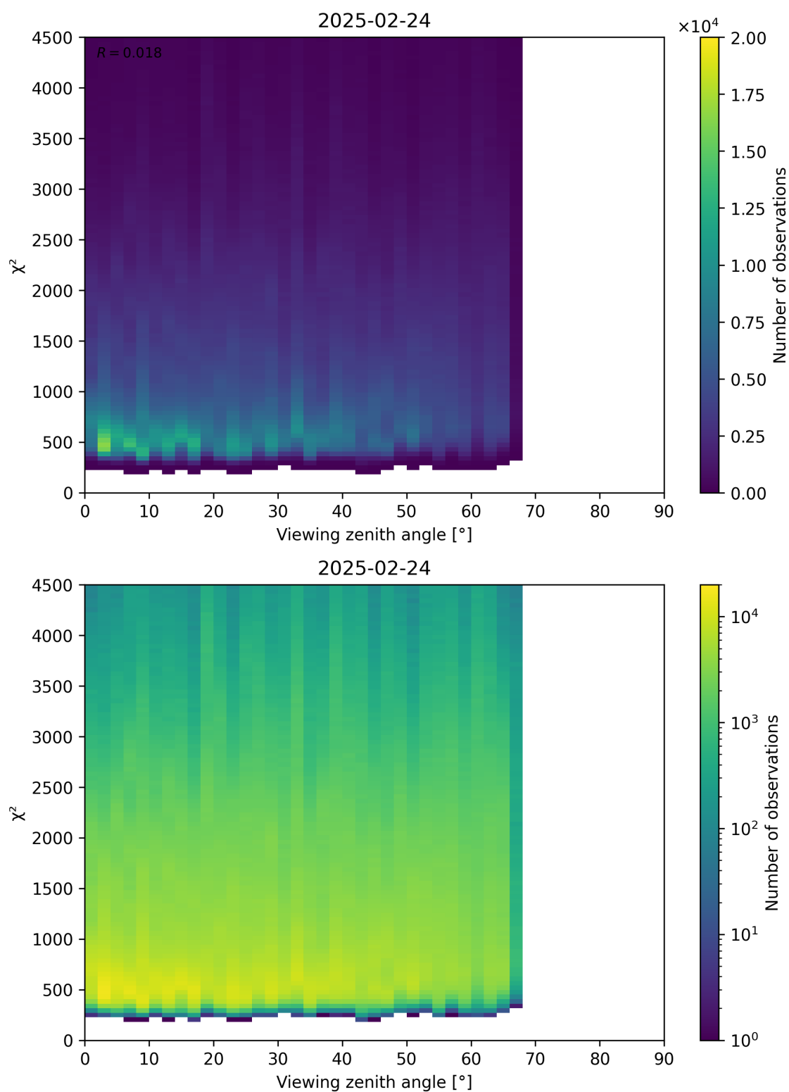
Figure 72: Scatter density plot of “Viewing zenith angle” against “ \chi^2 ” for 2025-02-24 to 2025-02-25.
