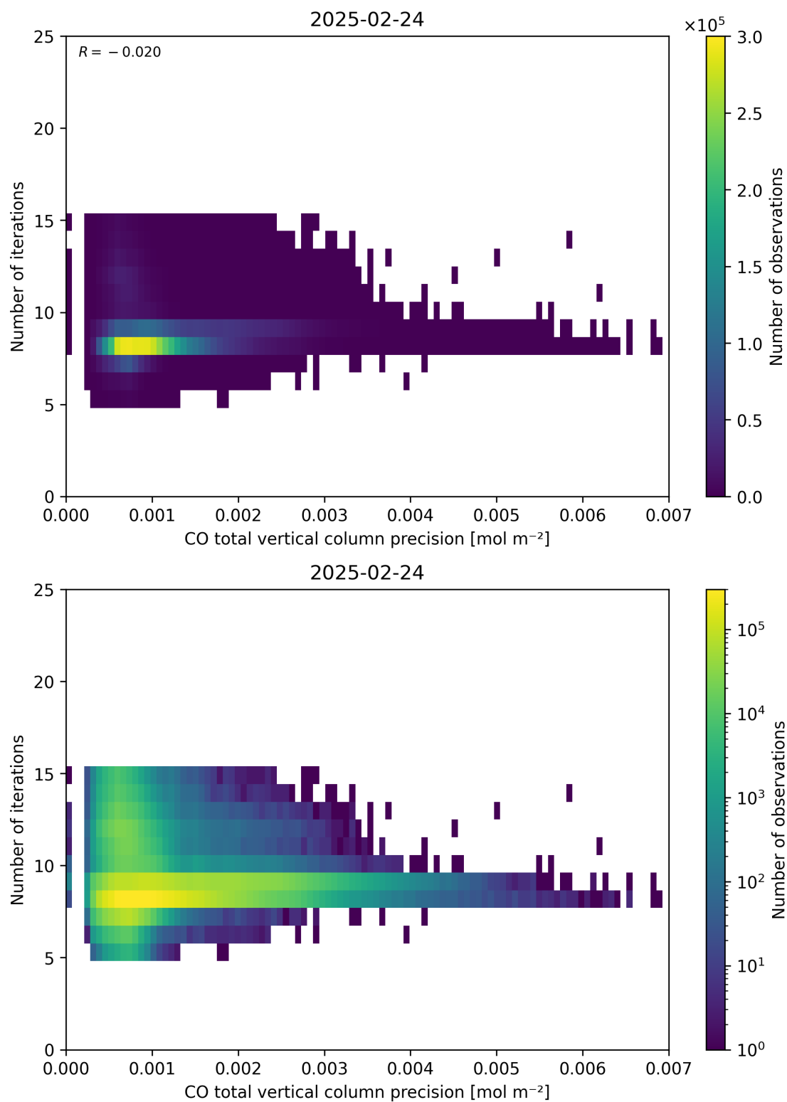
Figure 46: Scatter density plot of “CO total vertical column precision” against “Number of iterations” for 2025-02-24 to 2025-02-25.
