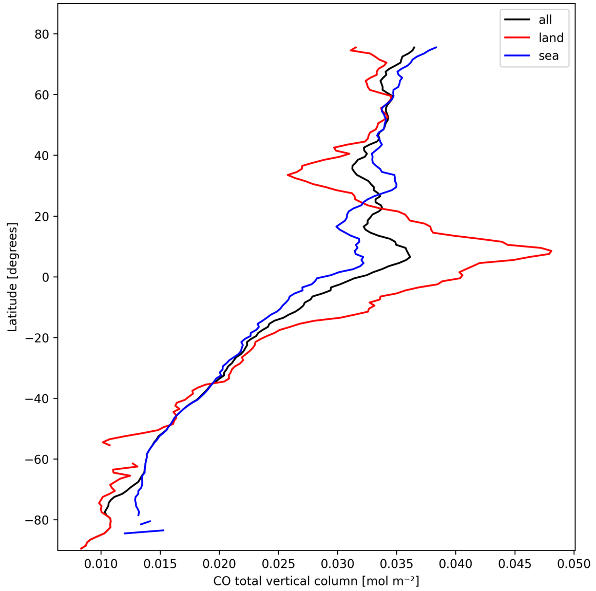
Figure 10: Zonal average of “CO total vertical column” for 2025-02-24 to 2025-02-25.
