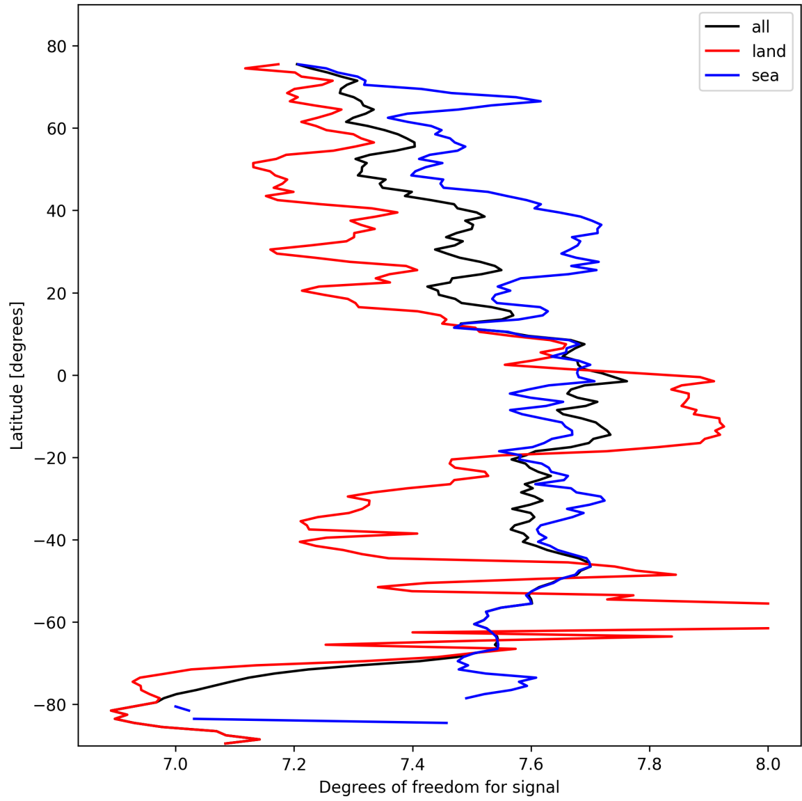
Figure 15: Zonal average of “Degrees of freedom for signal” for 2025-02-24 to 2025-02-25.
