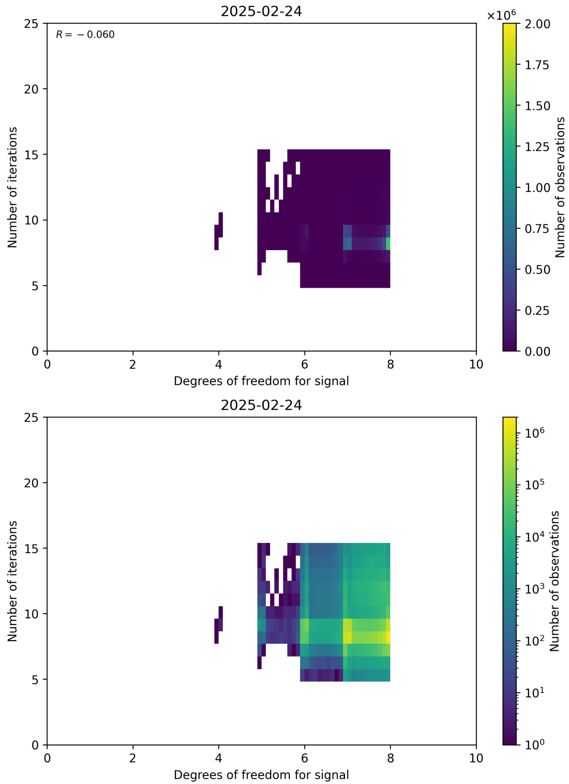
Figure 50: Scatter density plot of “Degrees of freedom for signal” against “Number of iterations” for 2025-02-24 to 2025-02-25.
