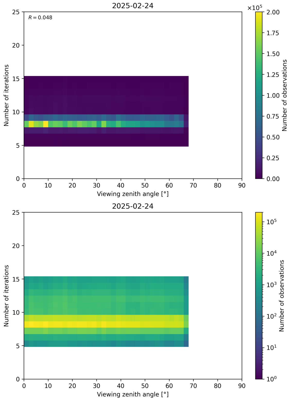
Figure 75: Scatter density plot of “Viewing zenith angle” against “Number of iterations” for 2025-02-24 to 2025-02-25.
