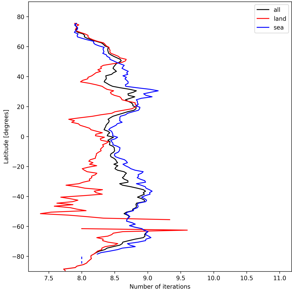
Figure 16: Zonal average of “Number of iterations” for 2025-02-24 to 2025-02-25.
