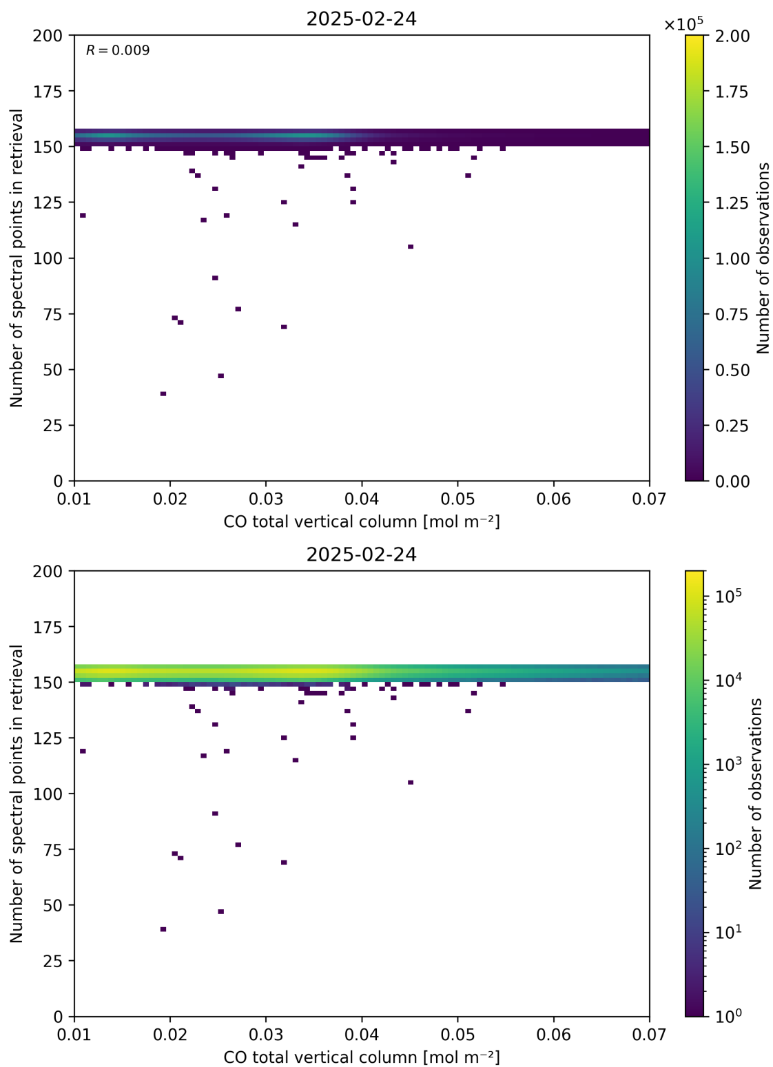
Figure 43: Scatter density plot of “CO total vertical column” against “Number of spectral points in retrieval” for 2025-02-24 to 2025-02-25.
