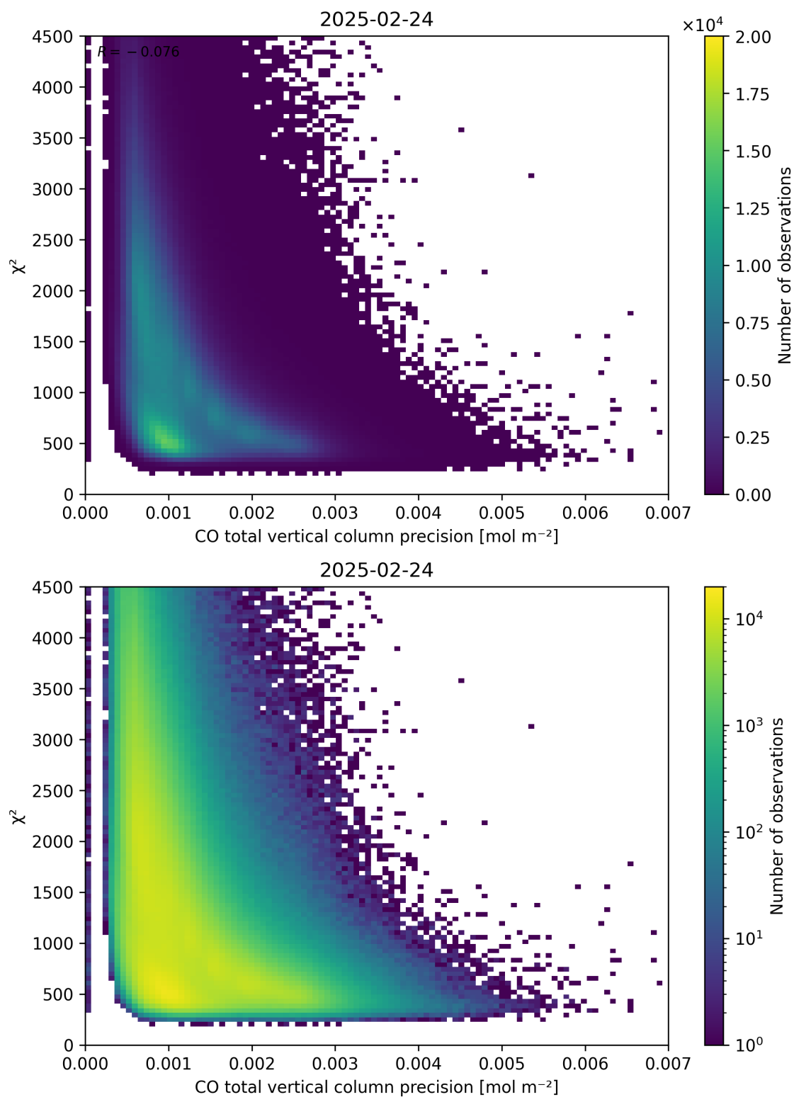
Figure 44: Scatter density plot of “CO total vertical column precision” against “ \chi^2 ” for 2025-02-24 to 2025-02-25.
