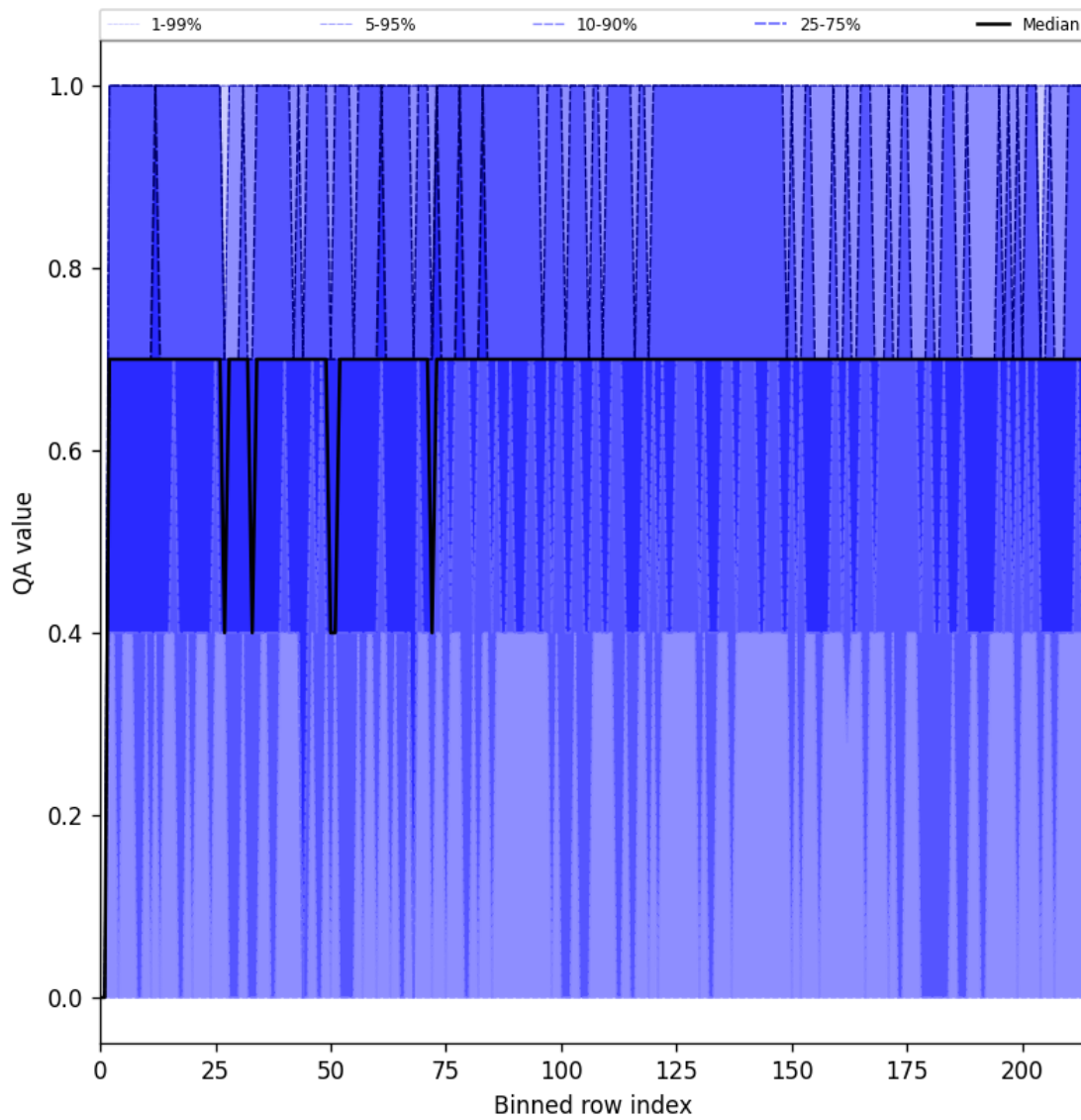
Figure 25: Along track statistics of “QA value” for 2025-02-24 to 2025-02-25
