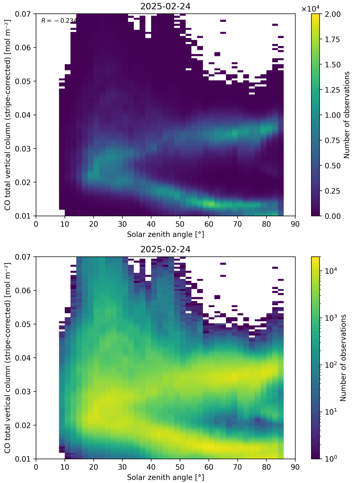
Figure 62: Scatter density plot of “Solar zenith angle” against “CO total vertical column (stripe-corrected)” for 2025-02-24 to 2025-02-25.
