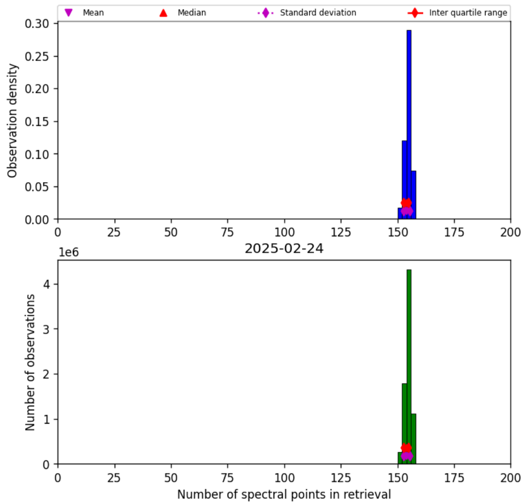
Figure 21: Histogram of “Number of spectral points in retrieval” for 2025-02-24 to 2025-02-25
