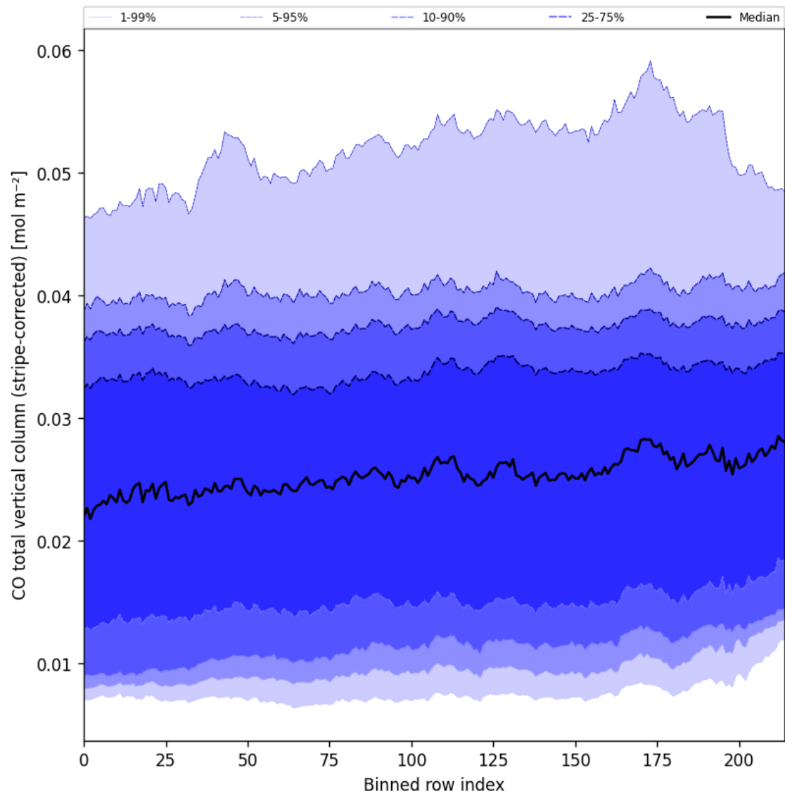
Figure 27: Along track statistics of “CO total vertical column (stripe-corrected)” for 2025-02-24 to 2025-02-25
