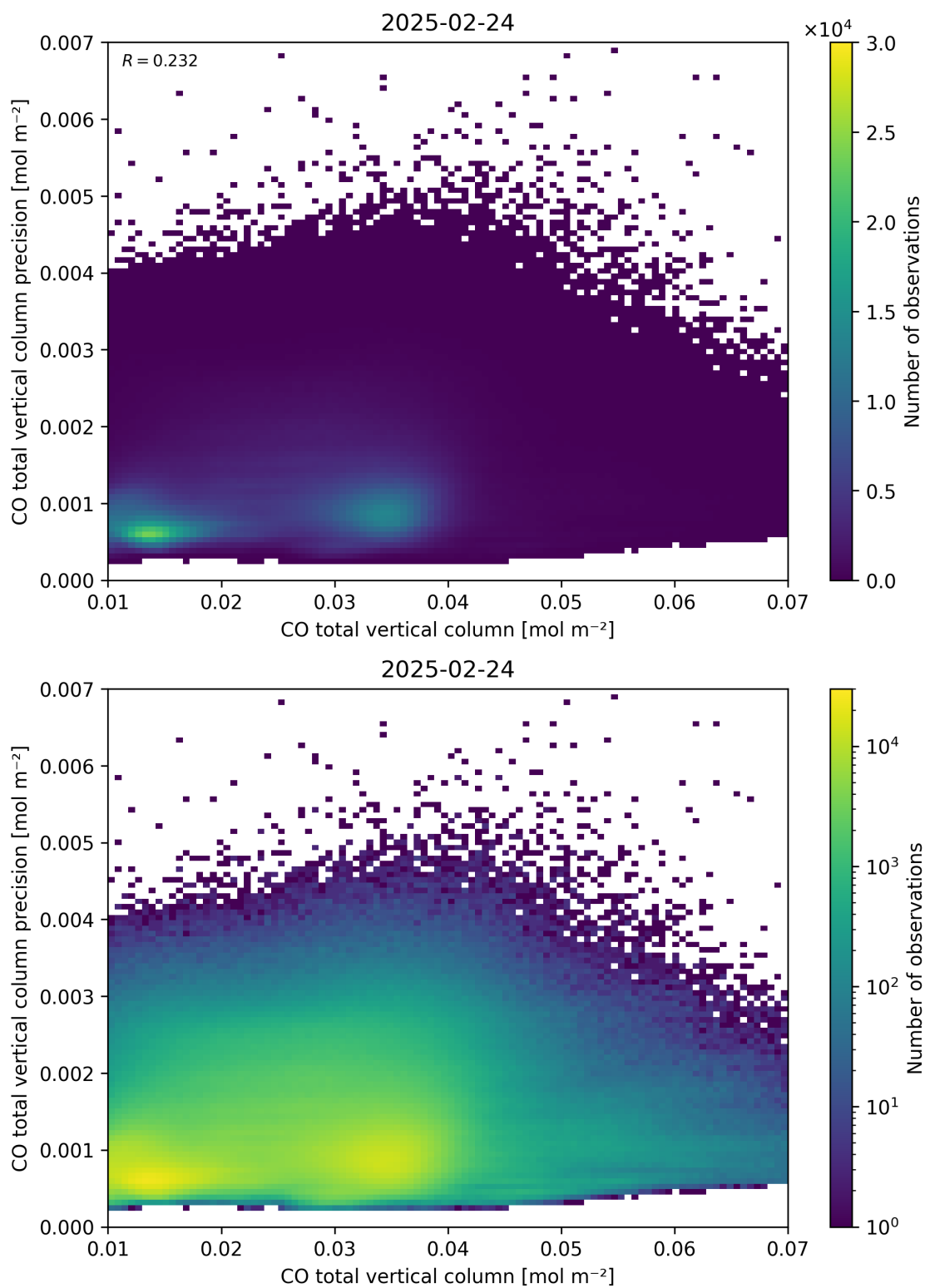
Figure 34: Scatter density plot of “CO total vertical column” against “CO total vertical column precision” for 2025-02-24 to 2025-02-25.
