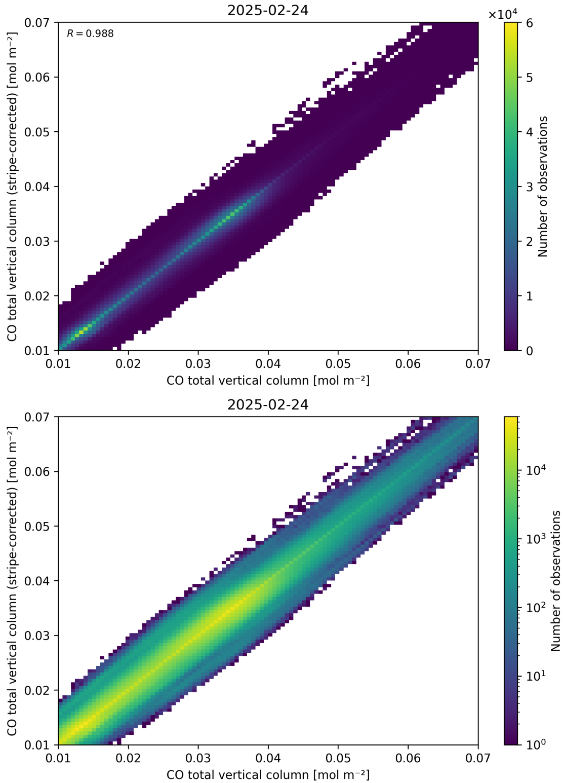
Figure 33: Scatter density plot of “CO total vertical column” against “CO total vertical column (stripe-corrected)” for 2025-02-24 to 2025-02-25.
