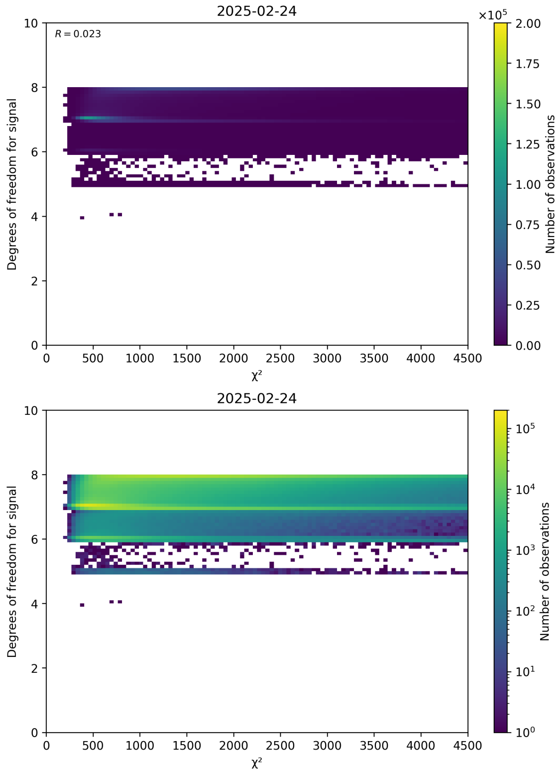
Figure 48: Scatter density plot of “ \chi^2 ” against “Degrees of freedom for signal” for 2025-02-24 to 2025-02-25.
