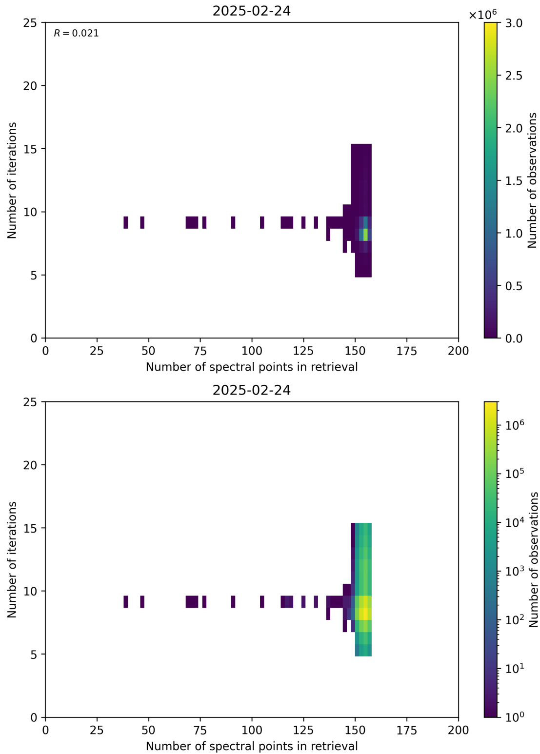
Figure 60: Scatter density plot of “Number of spectral points in retrieval” against “Number of iterations” for 2025-02-24 to 2025-02-25.
