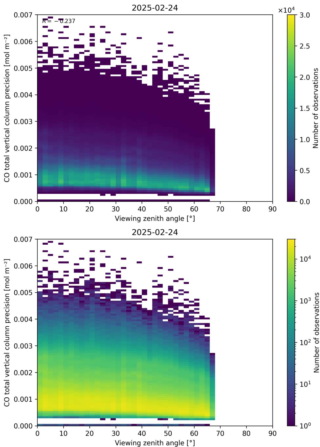
Figure 71: Scatter density plot of “Viewing zenith angle” against “CO total vertical column precision” for 2025-02-24 to 2025-02-25.
