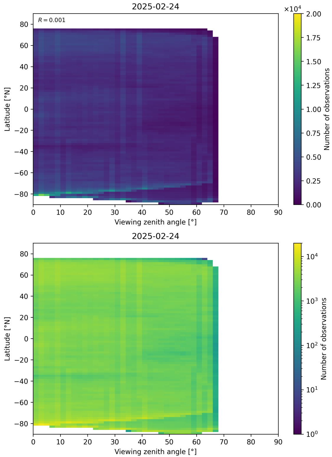
Figure 74: Scatter density plot of “Viewing zenith angle” against “Latitude” for 2025-02-24 to 2025-02-25.
