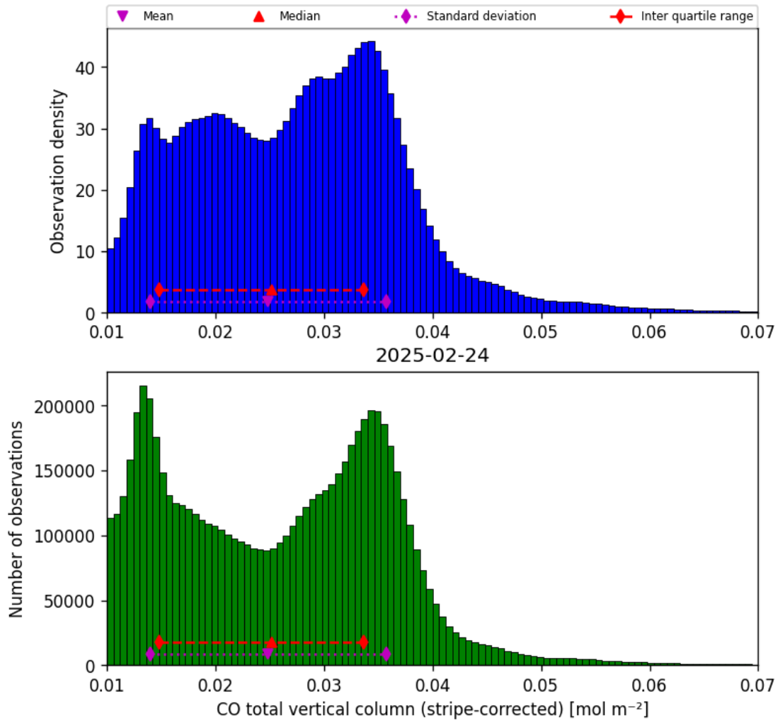
Figure 19: Histogram of “CO total vertical column (stripe-corrected)” for 2025-02-24 to 2025-02-25
