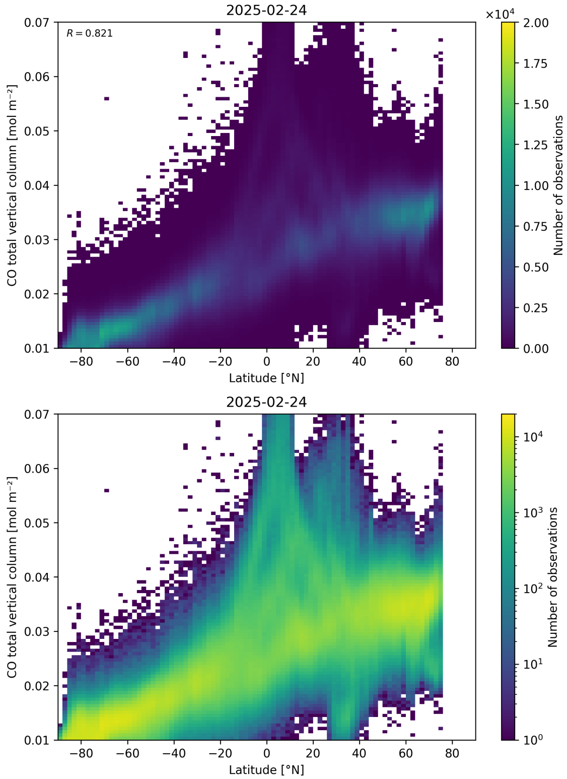
Figure 51: Scatter density plot of “Latitude” against “CO total vertical column” for 2025-02-24 to 2025-02-25.
