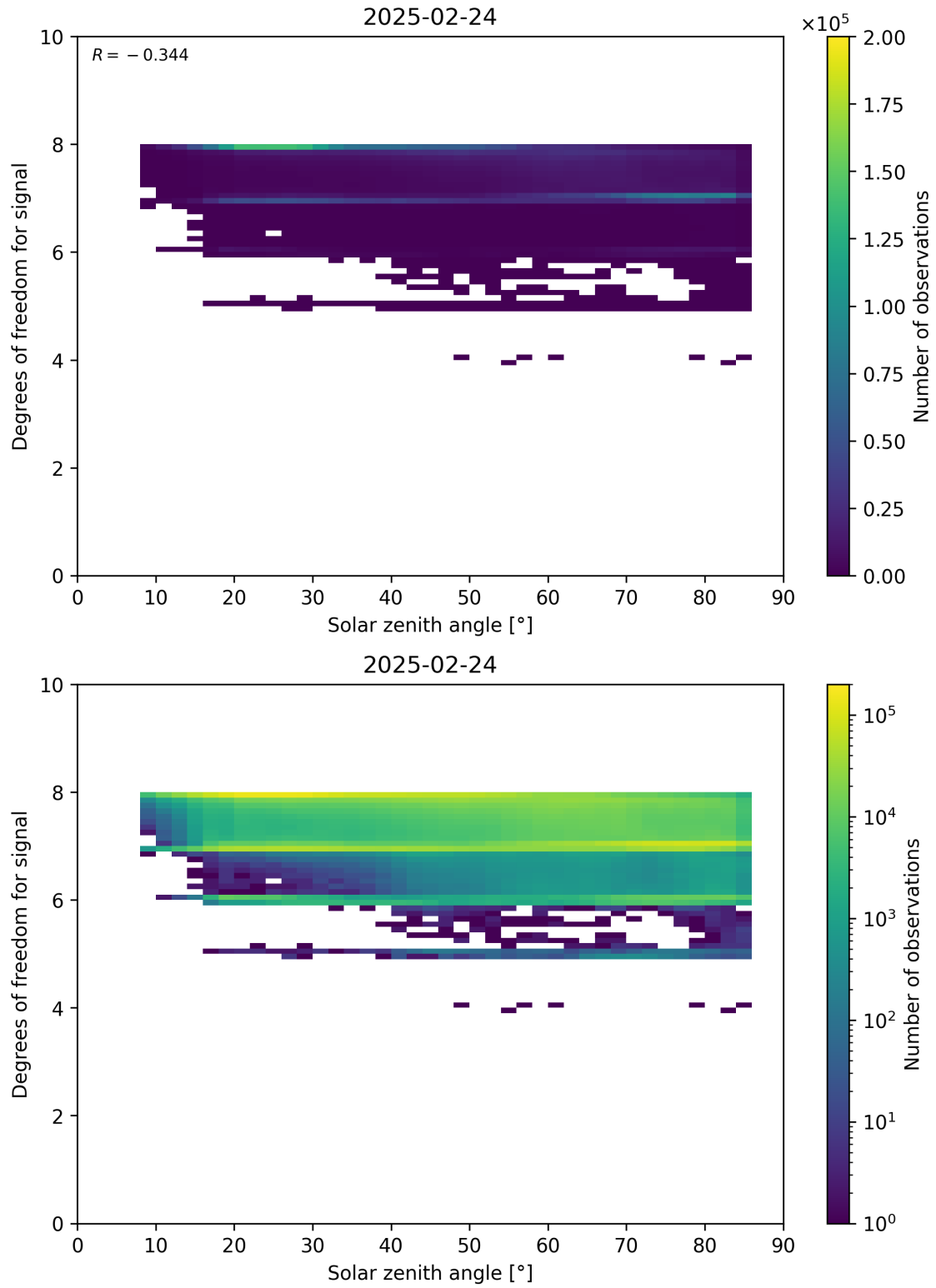
Figure 65: Scatter density plot of “Solar zenith angle” against “Degrees of freedom for signal” for 2025-02-24 to 2025-02-25.
