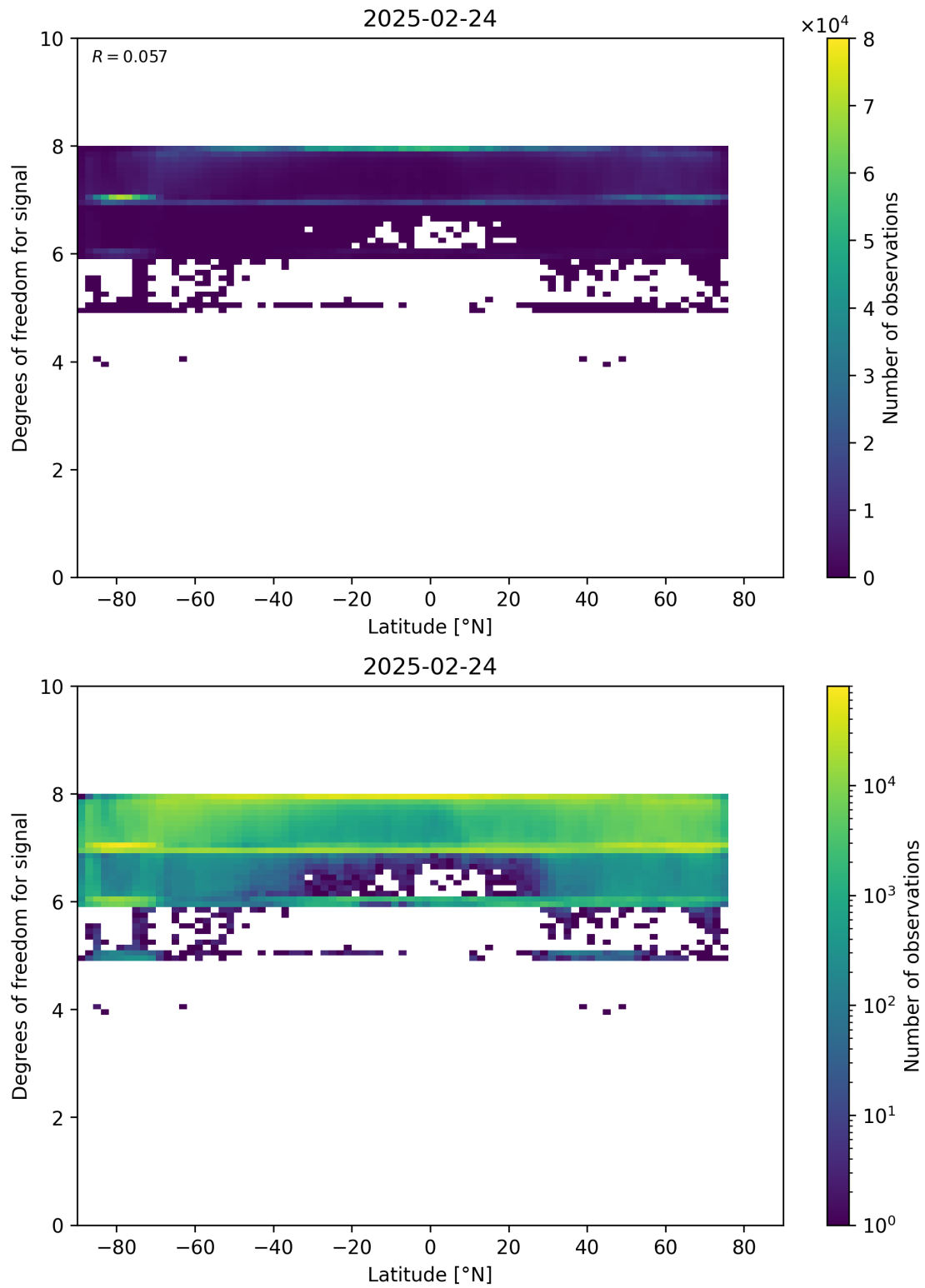
Figure 55: Scatter density plot of “Latitude” against “Degrees of freedom for signal” for 2025-02-24 to 2025-02-25.
