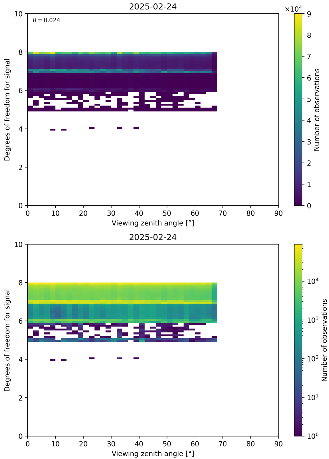
Figure 73: Scatter density plot of “Viewing zenith angle” against “Degrees of freedom for signal” for 2025-02-24 to 2025-02-25.
