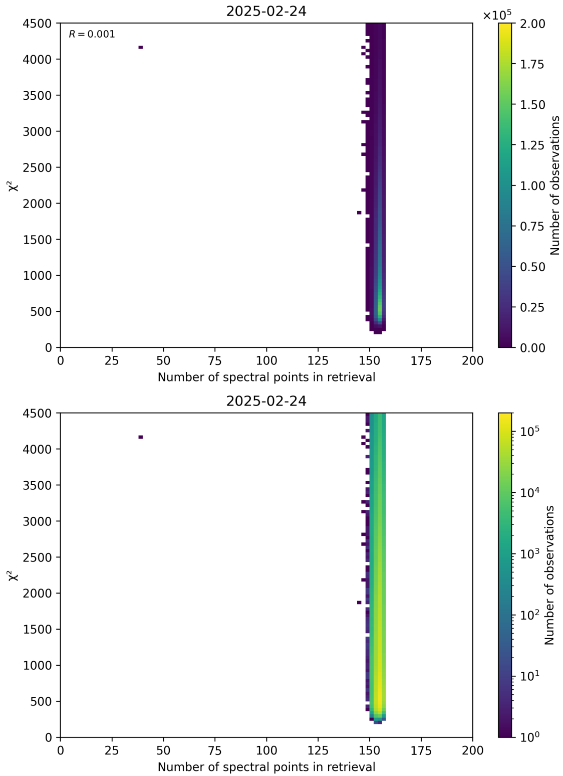
Figure 58: Scatter density plot of “Number of spectral points in retrieval” against “ \chi^2 ” for 2025-02-24 to 2025-02-25.
