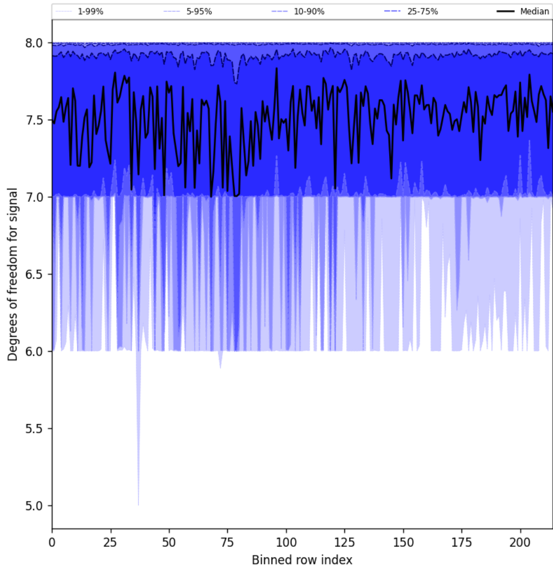
Figure 31: Along track statistics of “Degrees of freedom for signal” for 2025-02-24 to 2025-02-25
