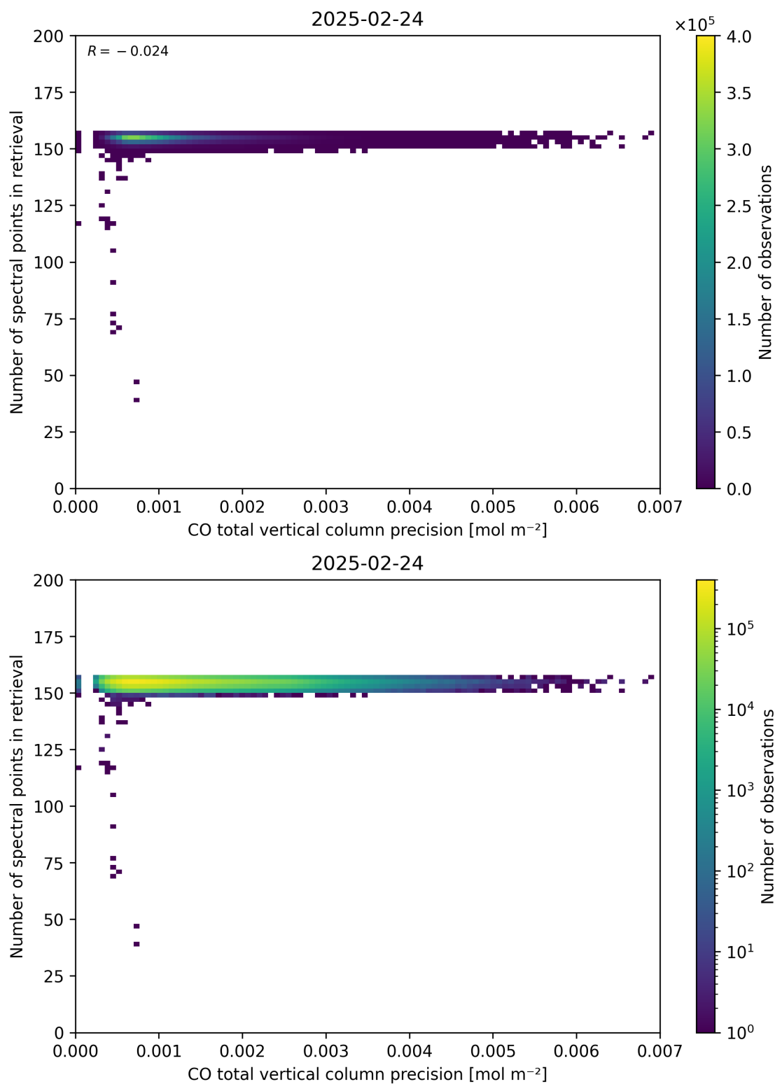
Figure 47: Scatter density plot of “CO total vertical column precision” against “Number of spectral points in retrieval” for 2025-02-24 to 2025-02-25.
