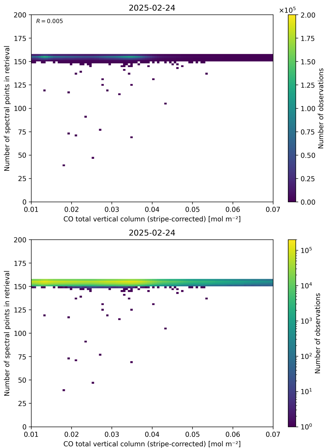
Figure 40: Scatter density plot of “CO total vertical column (stripe-corrected)” against “Number of spectral points in retrieval” for 2025-02-24 to 2025-02-25.
