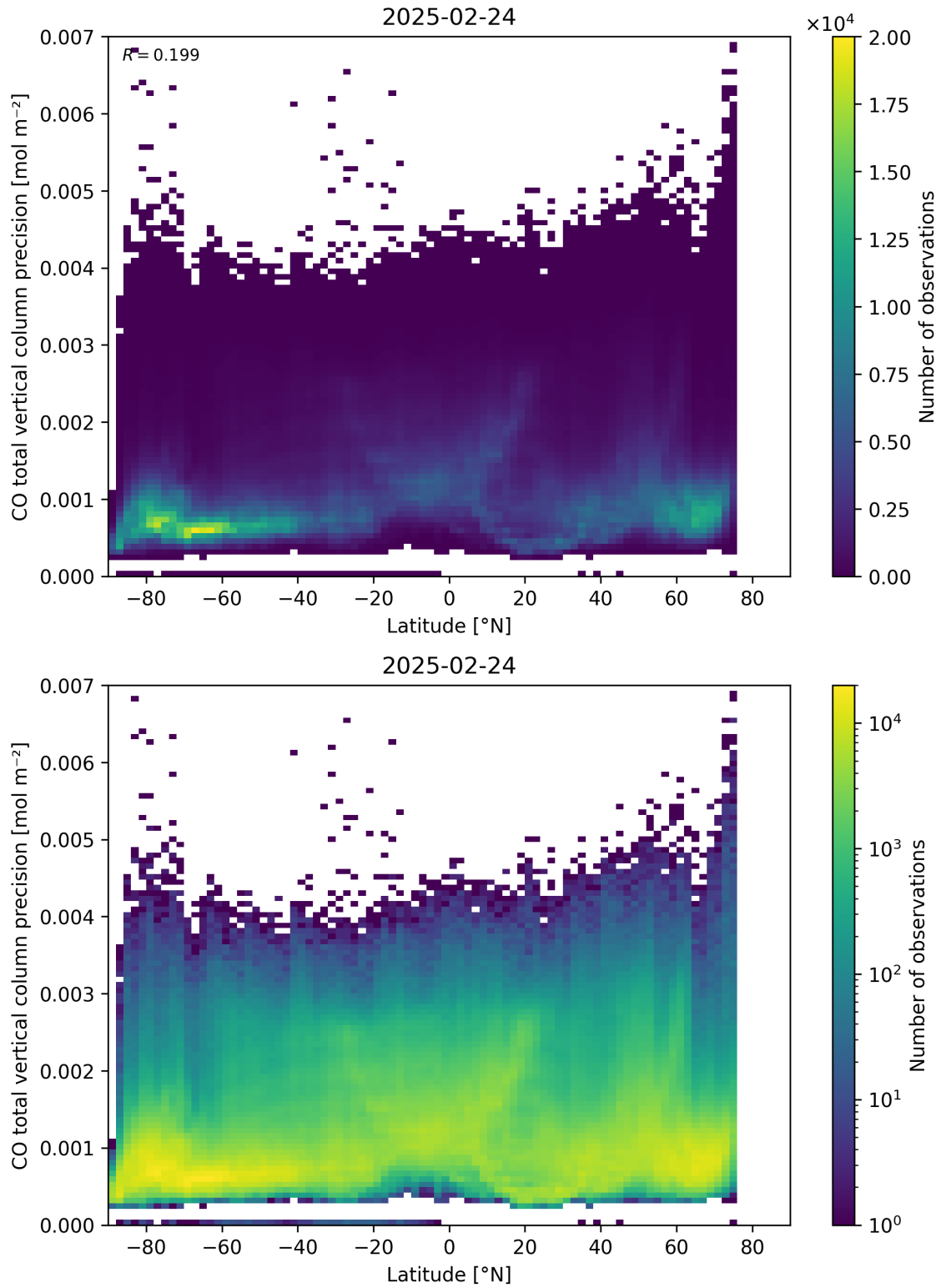
Figure 53: Scatter density plot of “Latitude” against “CO total vertical column precision” for 2025-02-24 to 2025-02-25.
