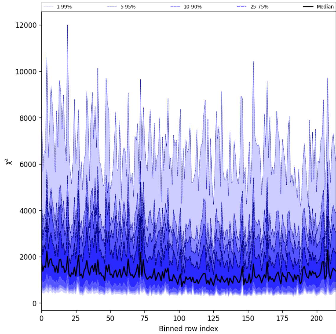
Figure 30: Along track statistics of “ \chi^2 ” for 2025-02-24 to 2025-02-25
