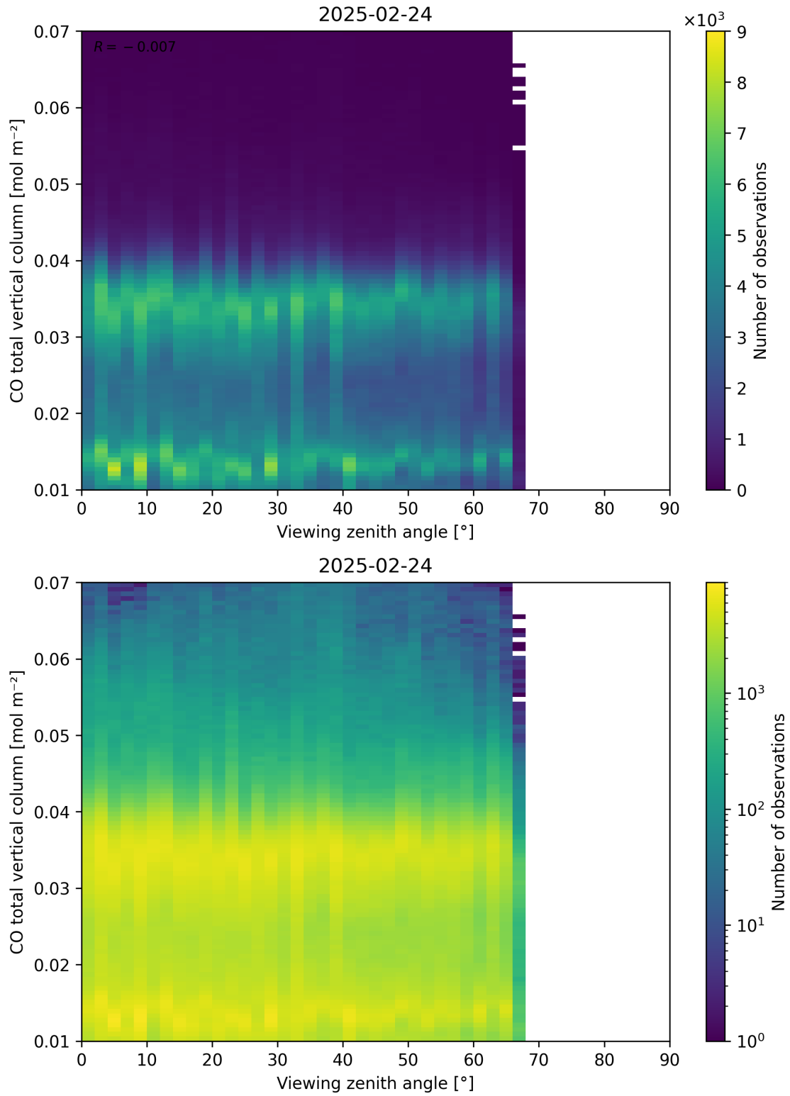
Figure 69: Scatter density plot of “Viewing zenith angle” against “CO total vertical column” for 2025-02-24 to 2025-02-25.
