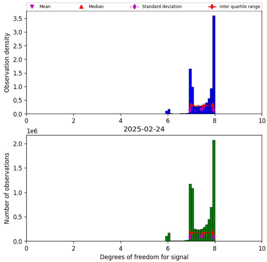
Figure 23: Histogram of “Degrees of freedom for signal” for 2025-02-24 to 2025-02-25
