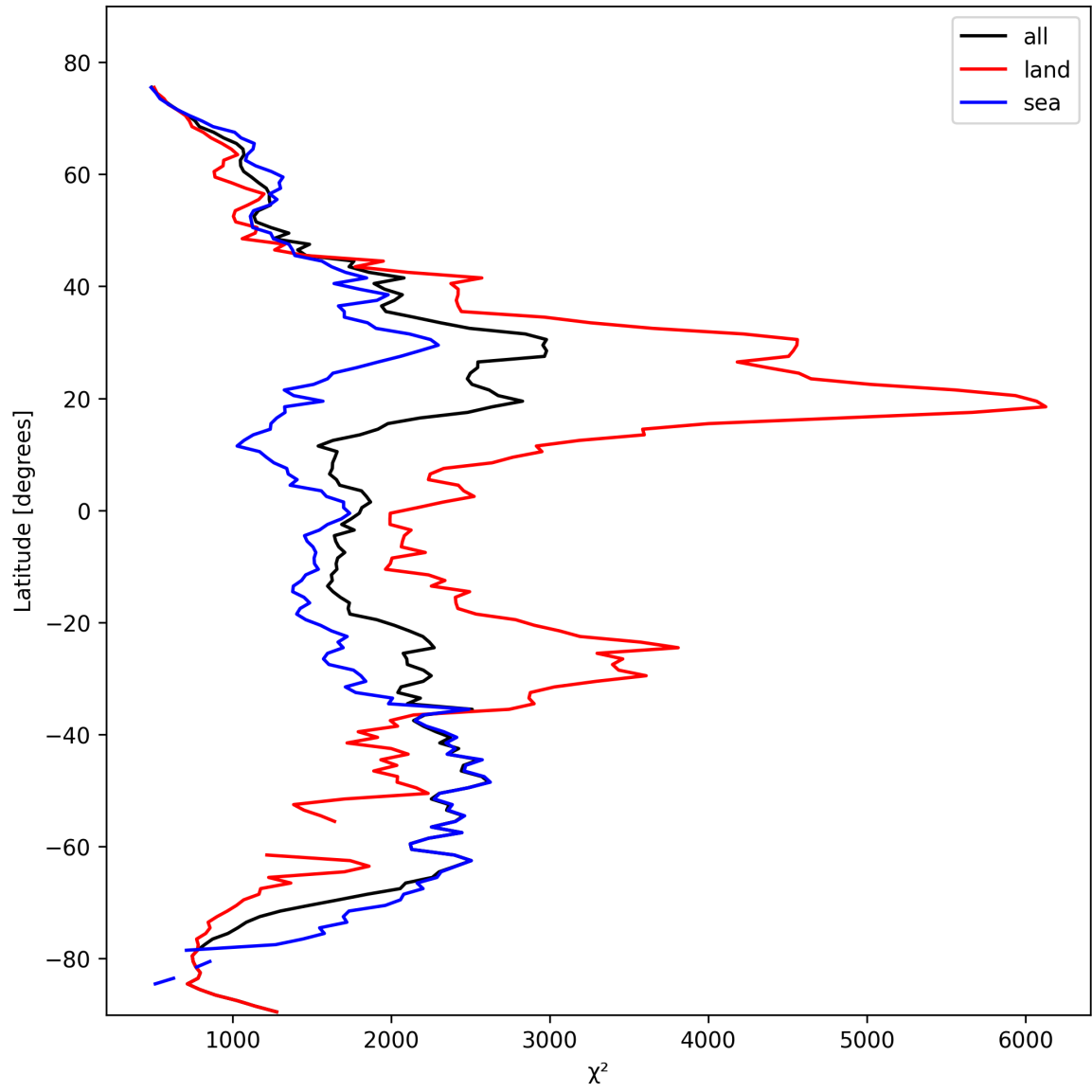
Figure 14: Zonal average of “ \chi^2 ” for 2025-02-24 to 2025-02-25.
