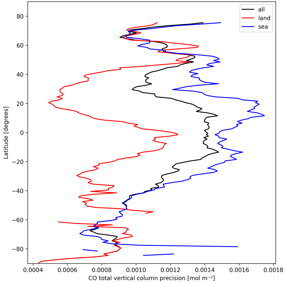
Figure 12: Zonal average of "CO total vertical column precision" for 2025-02-24 to 2025-02-25.
