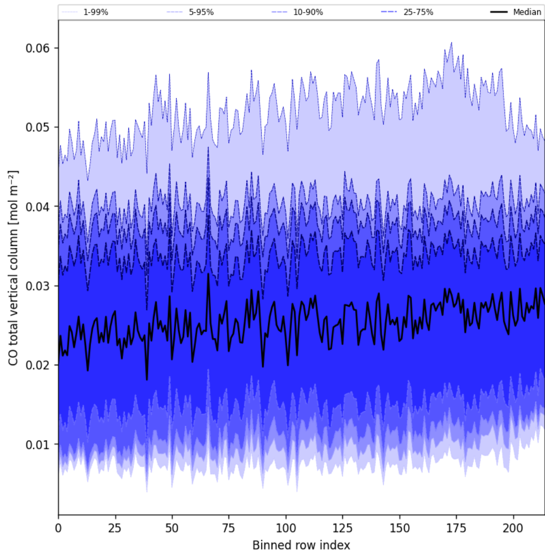
Figure 26: Along track statistics of “CO total vertical column” for 2025-02-24 to 2025-02-25
