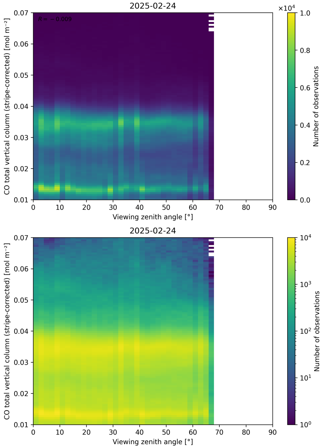
Figure 70: Scatter density plot of “Viewing zenith angle” against “CO total vertical column (stripe-corrected)” for 2025-02-24 to 2025-02-25.
