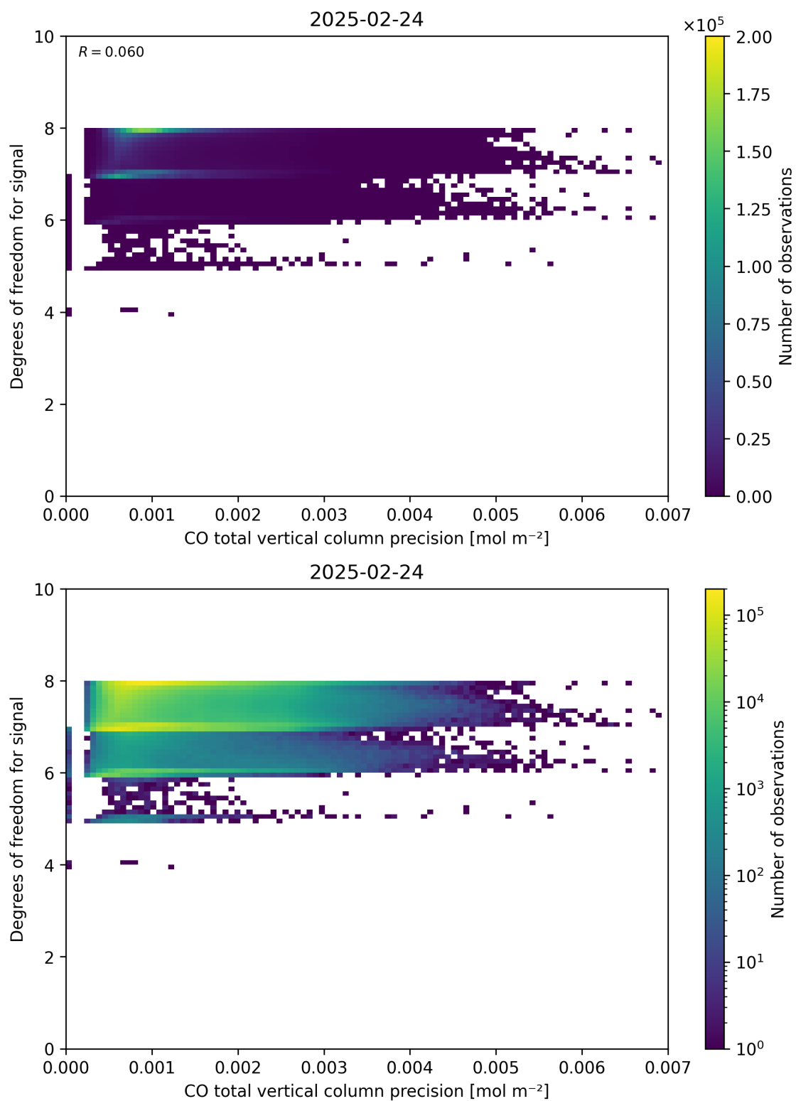
Figure 45: Scatter density plot of “CO total vertical column precision” against “Degrees of freedom for signal” for 2025-02-24 to 2025-02-25.
