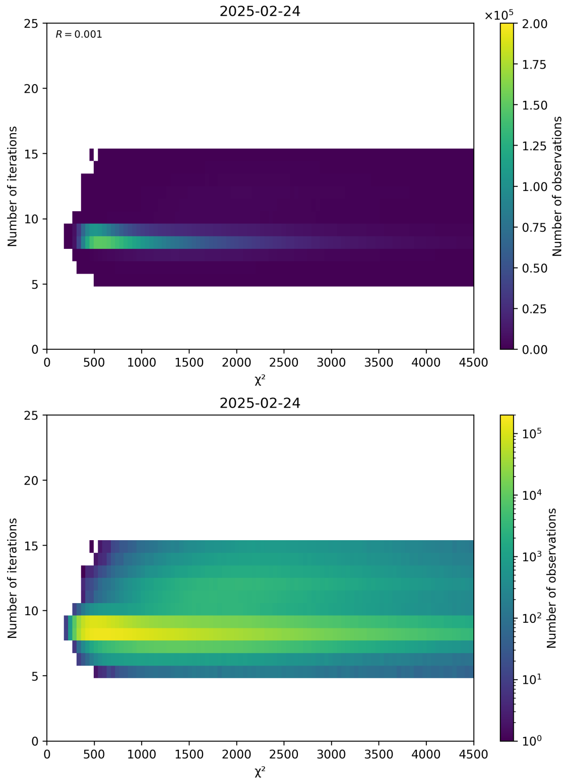
Figure 49: Scatter density plot of “ \chi^2 ” against “Number of iterations” for 2025-02-24 to 2025-02-25.
