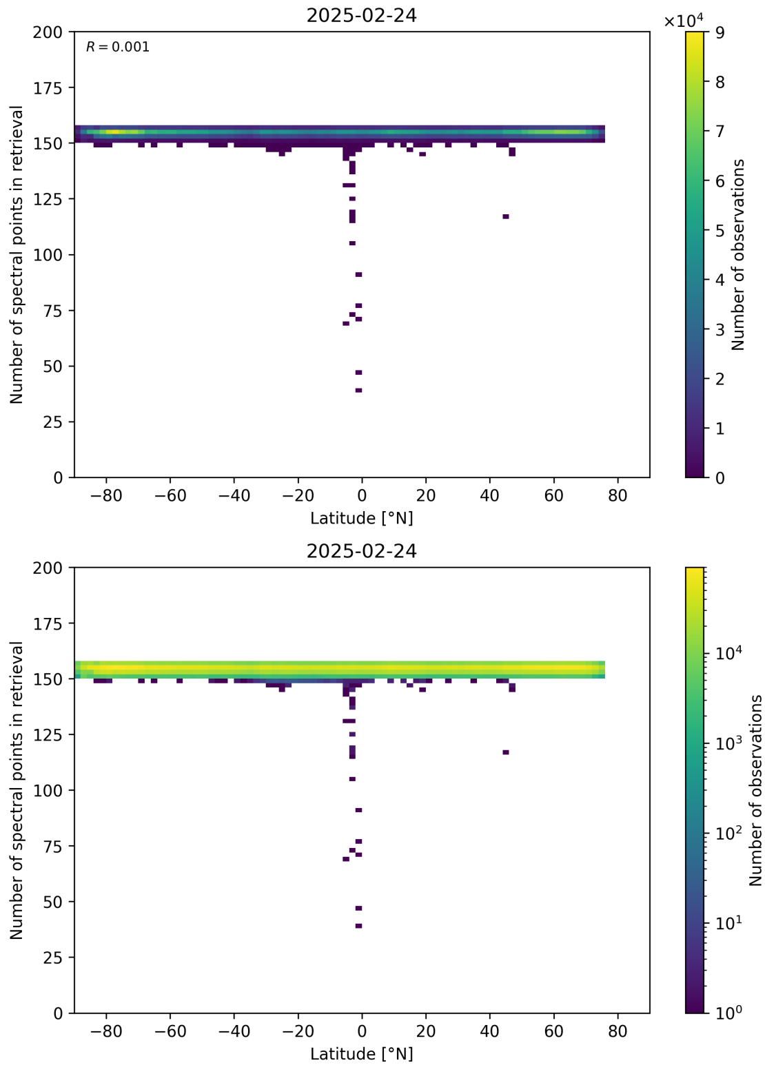
Figure 57: Scatter density plot of “Latitude” against “Number of spectral points in retrieval” for 2025-02-24 to 2025-02-25.
