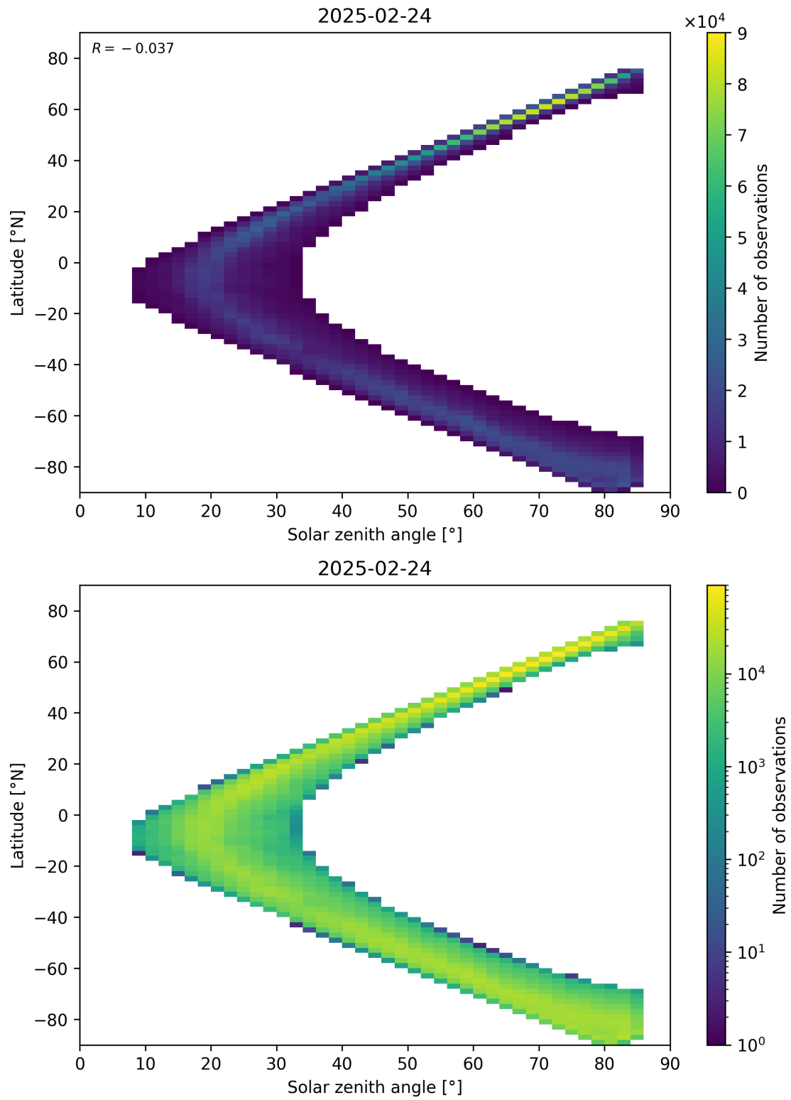
Figure 66: Scatter density plot of “Solar zenith angle” against “Latitude” for 2025-02-24 to 2025-02-25.
