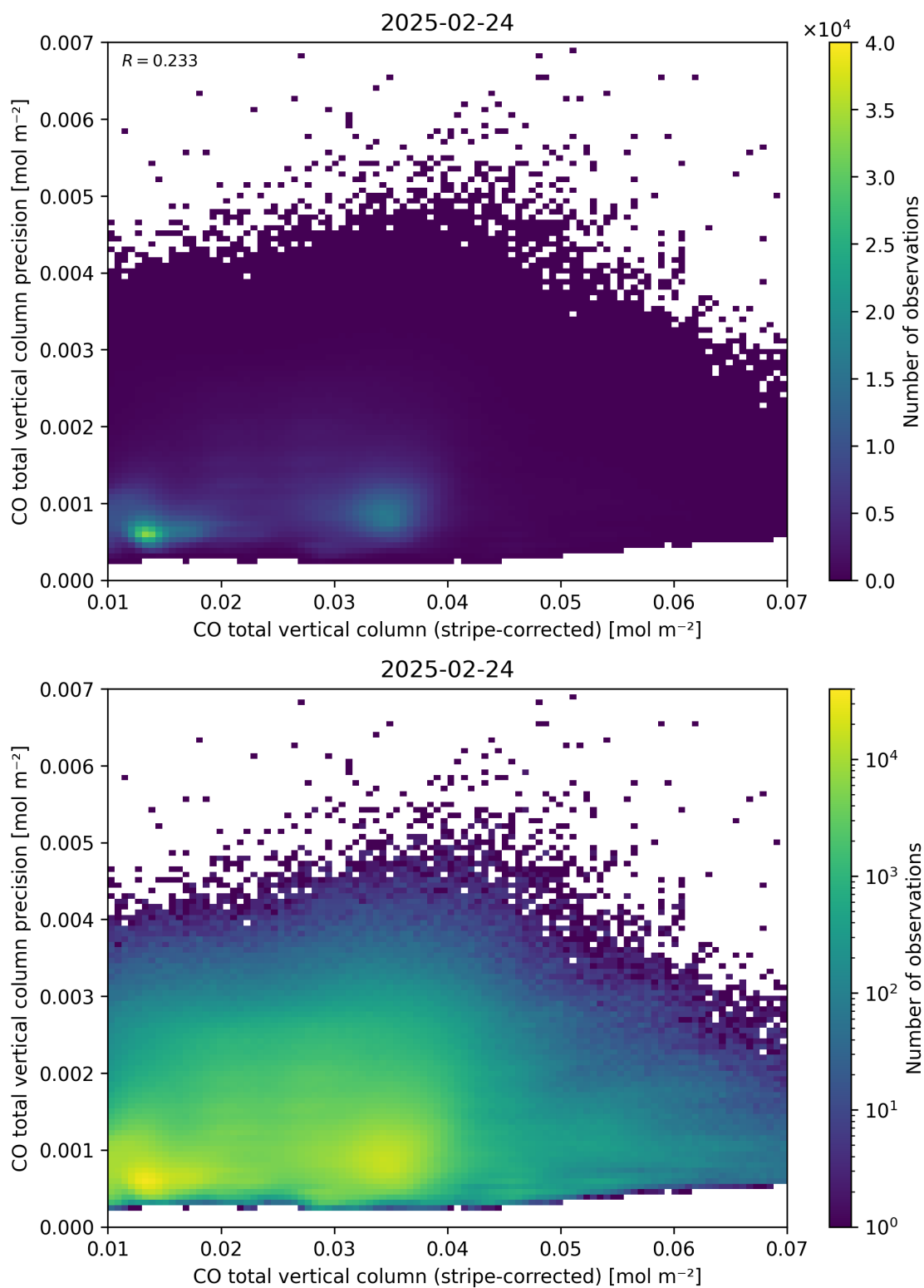
Figure 36: Scatter density plot of “CO total vertical column (stripe-corrected)” against “CO total vertical column precision” for 2025-02-24 to 2025-02-25.
