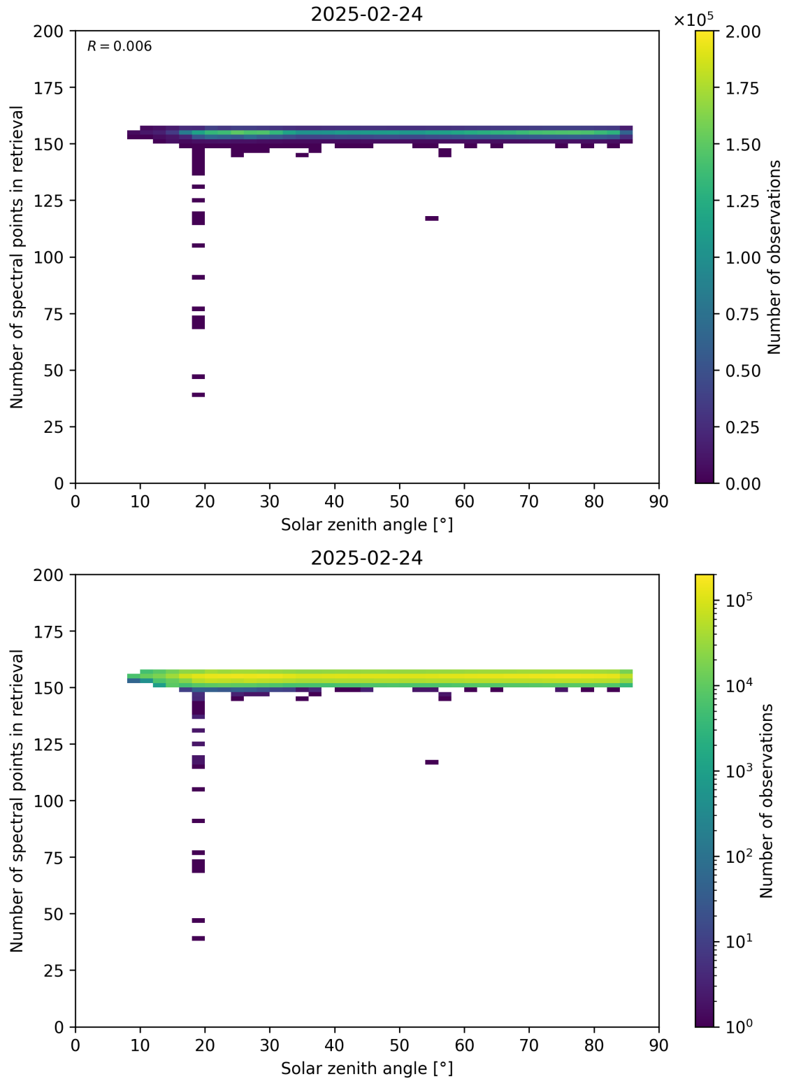
Figure 68: Scatter density plot of “Solar zenith angle” against “Number of spectral points in retrieval” for 2025-02-24 to 2025-02-25.
