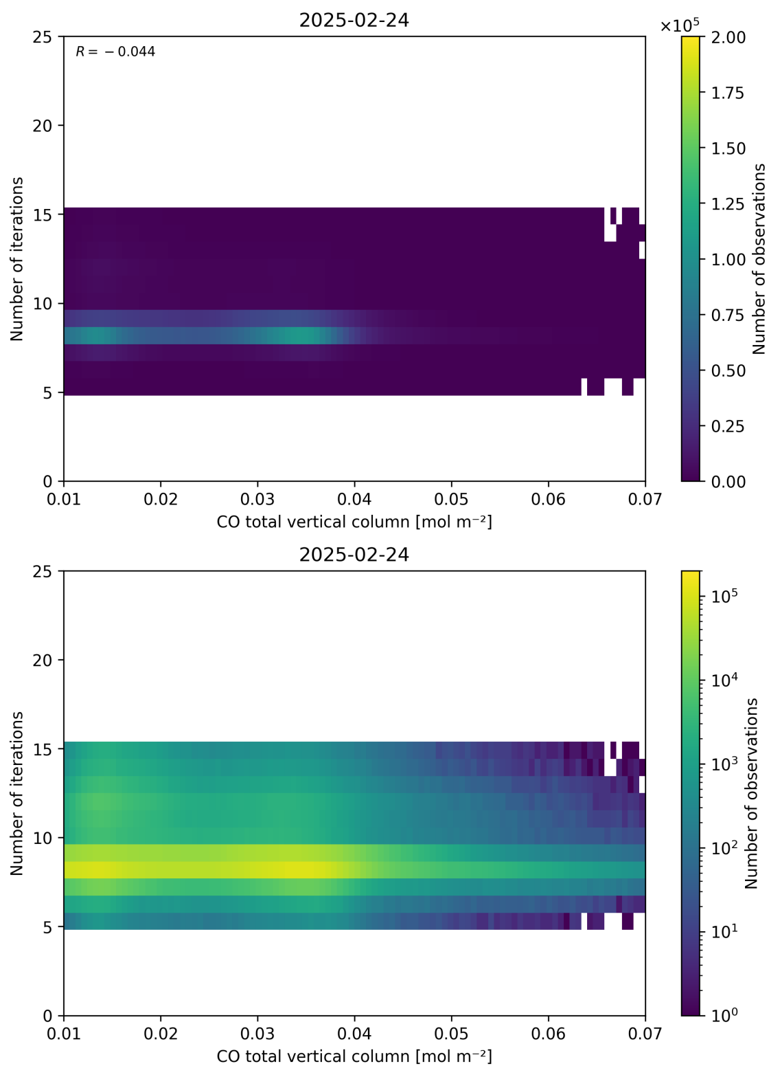
Figure 42: Scatter density plot of “CO total vertical column” against “Number of iterations” for 2025-02-24 to 2025-02-25.
