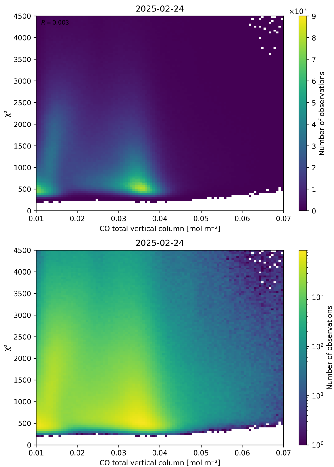
Figure 35: Scatter density plot of “CO total vertical column” against “ \chi^2 ” for 2025-02-24 to 2025-02-25.
