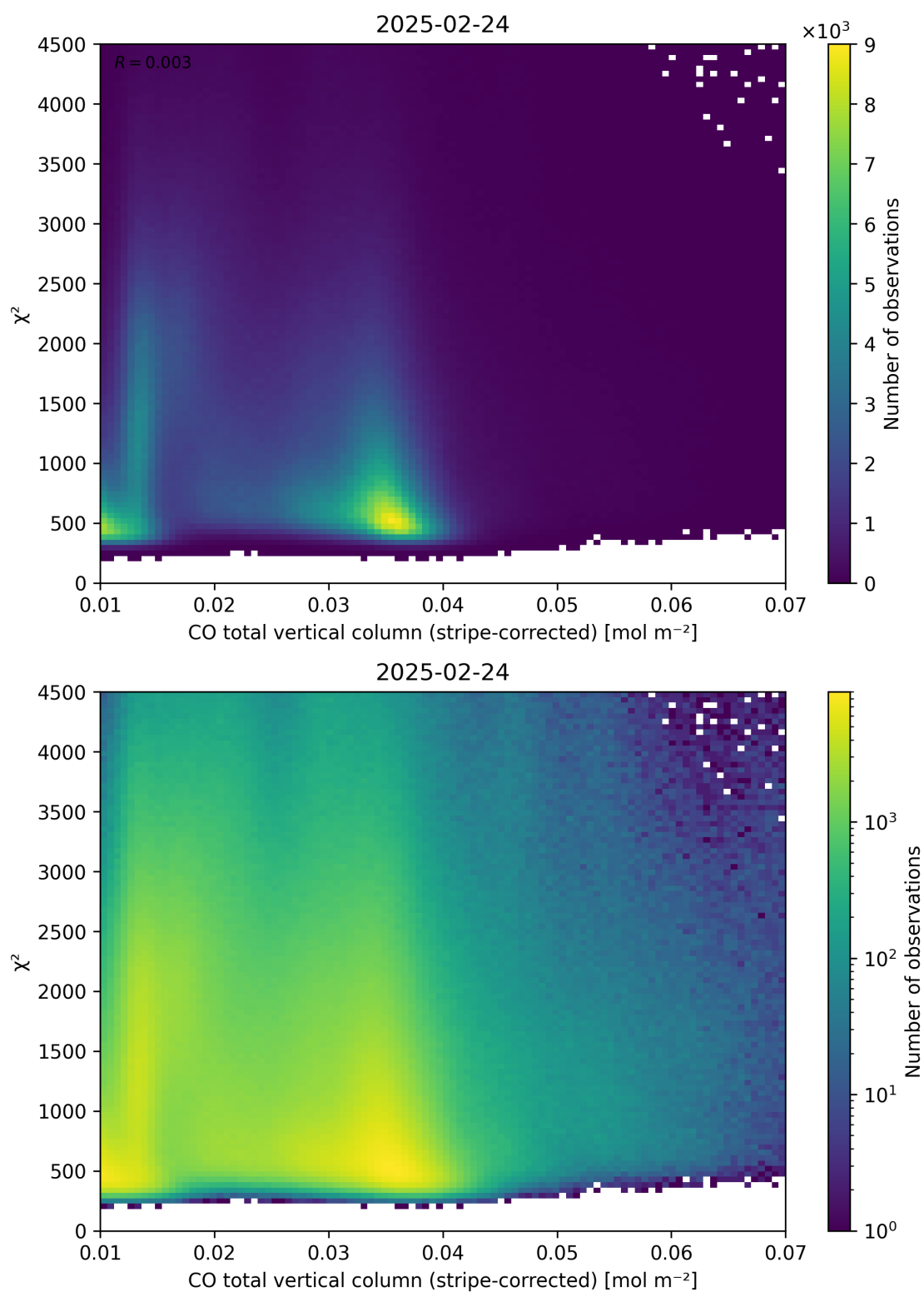
Figure 37: Scatter density plot of “CO total vertical column (stripe-corrected)” against “ \chi^2 ” for 2025-02-24 to 2025-02-25.
