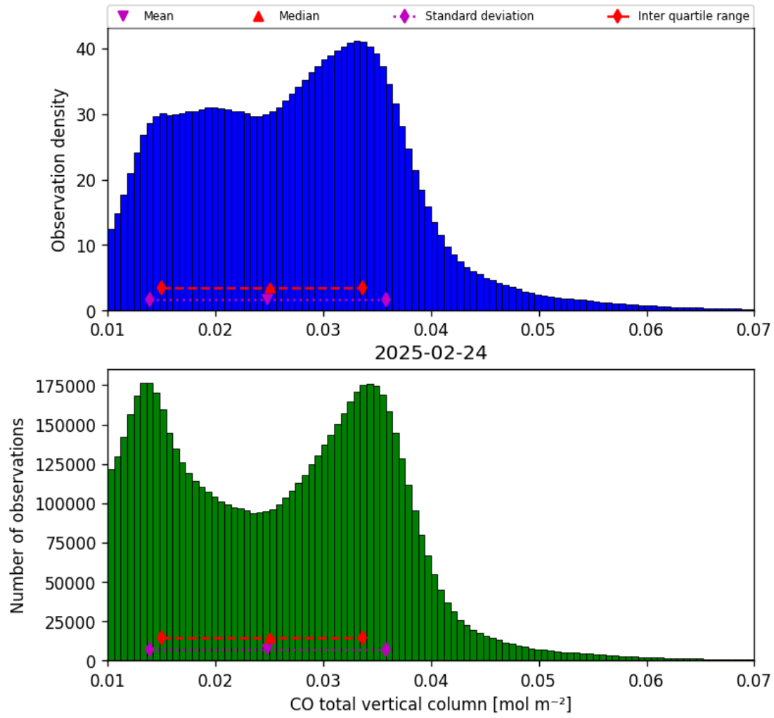
Figure 18: Histogram of “CO total vertical column” for 2025-02-24 to 2025-02-25
