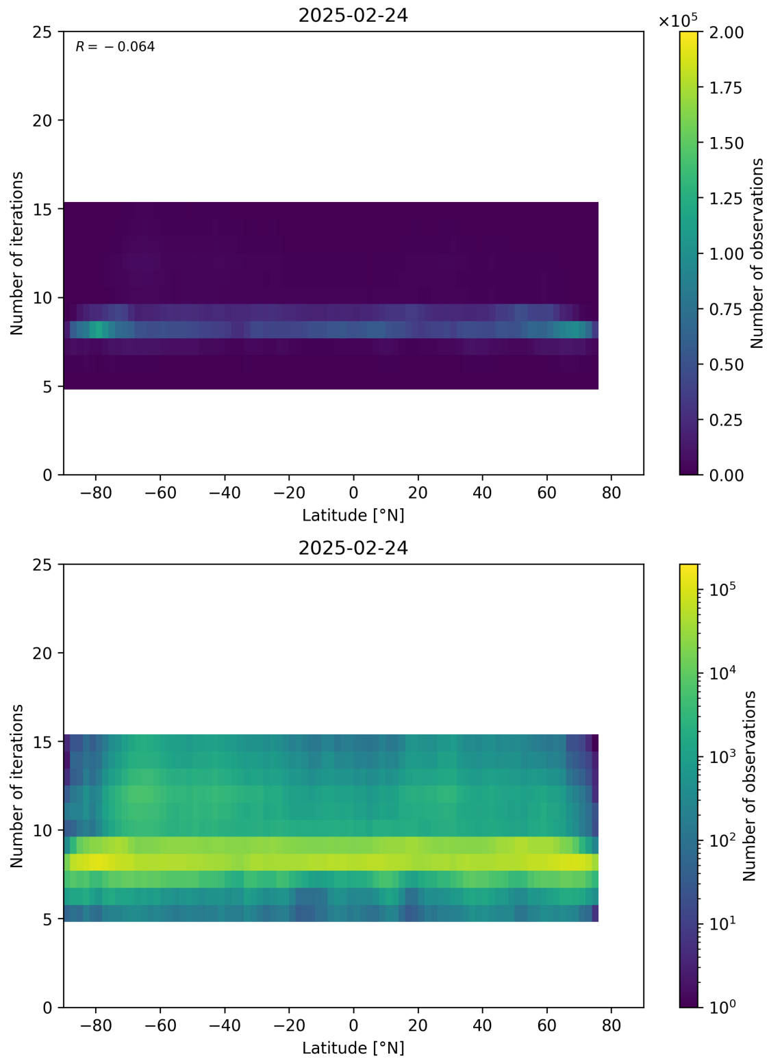
Figure 56: Scatter density plot of “Latitude” against “Number of iterations” for 2025-02-24 to 2025-02-25.
