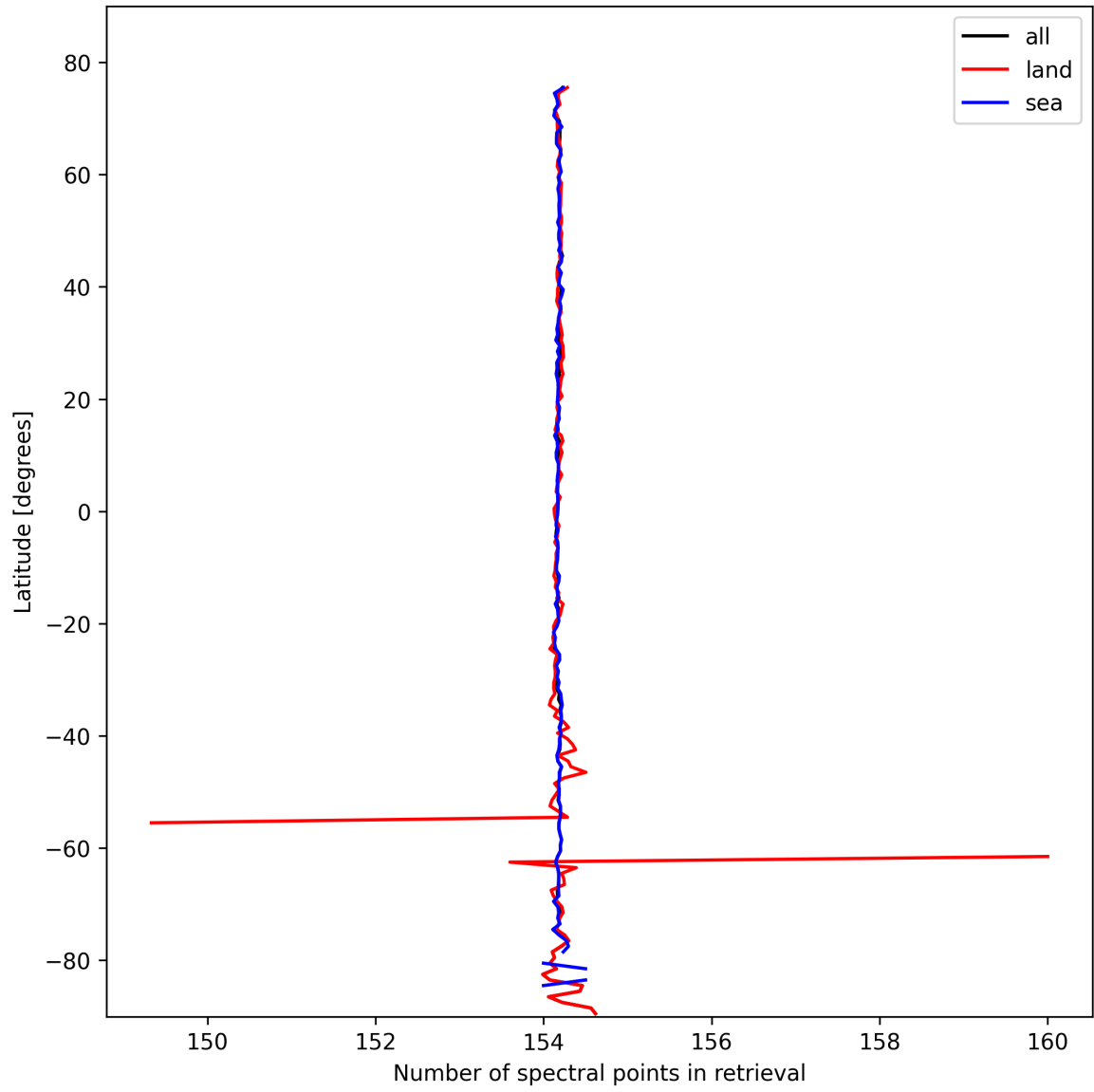
Figure 13: Zonal average of “Number of spectral points in retrieval” for 2025-02-24 to 2025-02-25.
