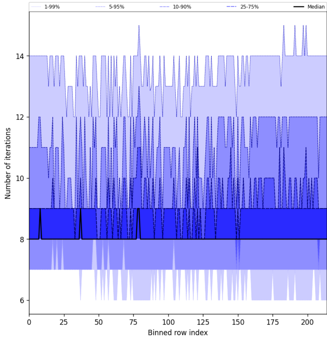
Figure 32: Along track statistics of “Number of iterations” for 2025-02-24 to 2025-02-25
