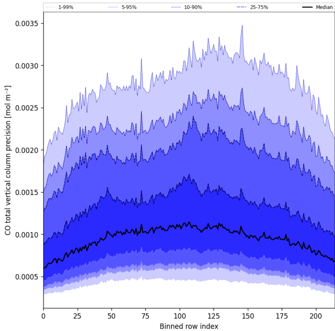
Figure 28: Along track statistics of “CO total vertical column precision” for 2025-02-24 to 2025-02-25
