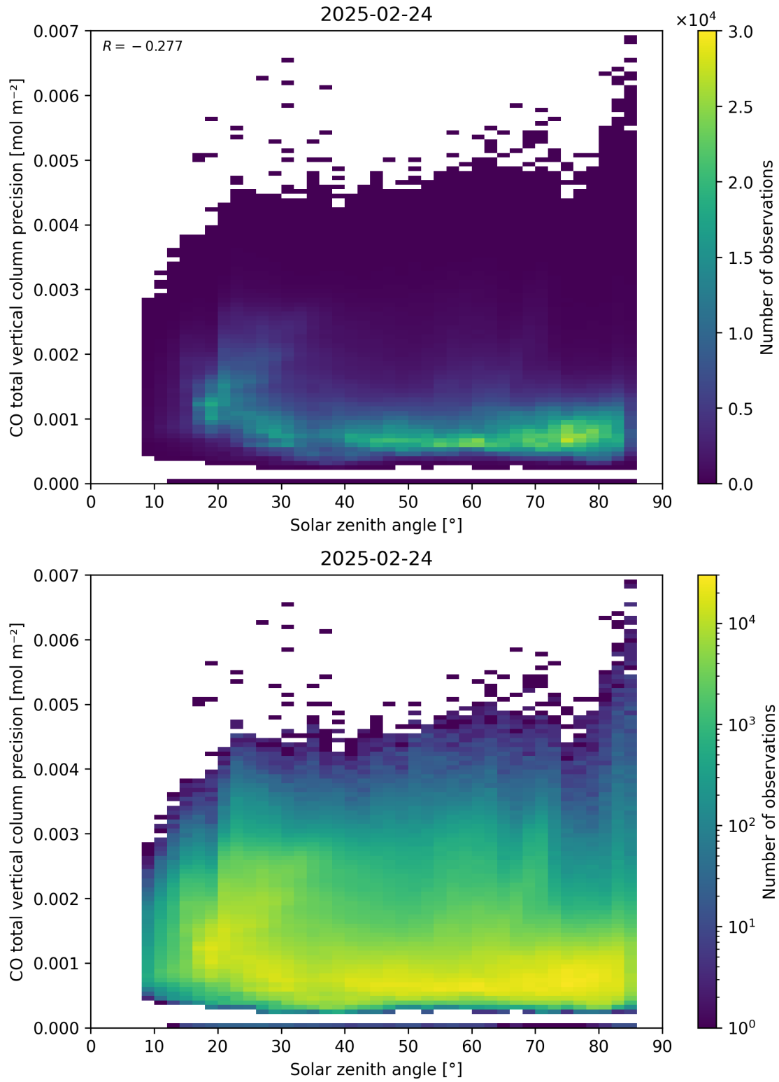
Figure 63: Scatter density plot of “Solar zenith angle” against “CO total vertical column precision” for 2025-02-24 to 2025-02-25.
