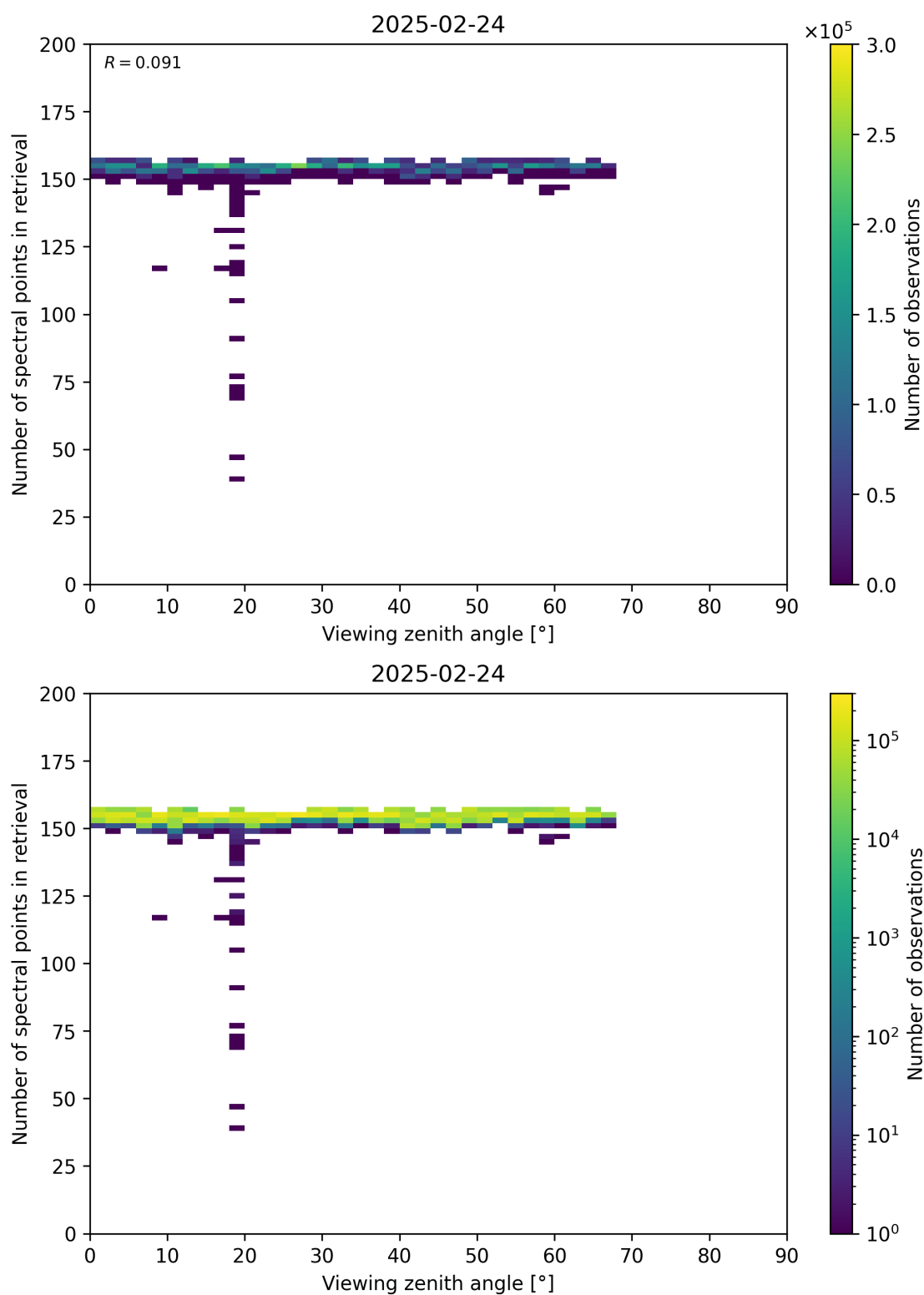
Figure 76: Scatter density plot of “Viewing zenith angle” against “Number of spectral points in retrieval” for 2025-02-24 to 2025-02-25.
