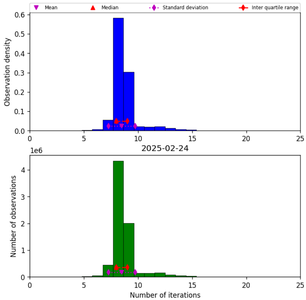
Figure 24: Histogram of “Number of iterations” for 2025-02-24 to 2025-02-25
