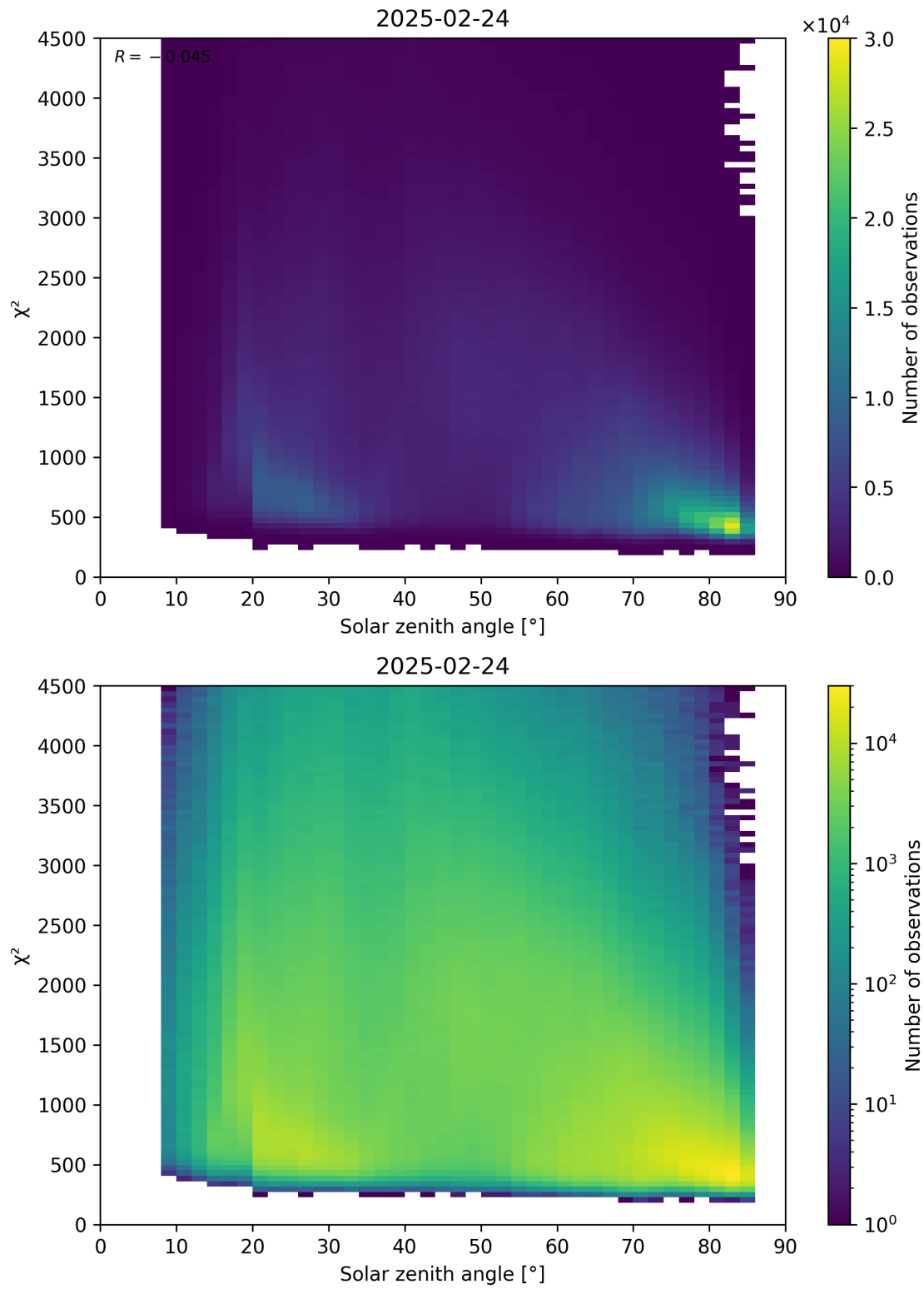
Figure 64: Scatter density plot of “Solar zenith angle” against “ \chi^2 ” for 2025-02-24 to 2025-02-25.
