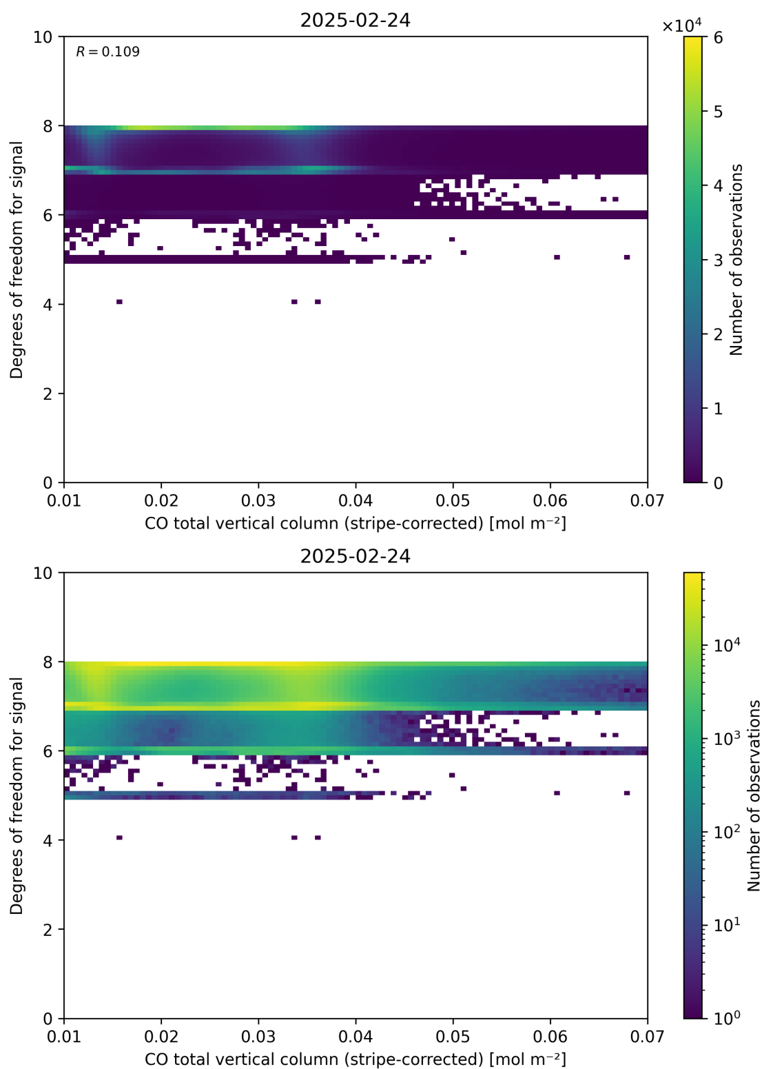
Figure 38: Scatter density plot of “CO total vertical column (stripe-corrected)” against “Degrees of freedom for signal” for 2025-02-24 to 2025-02-25.
