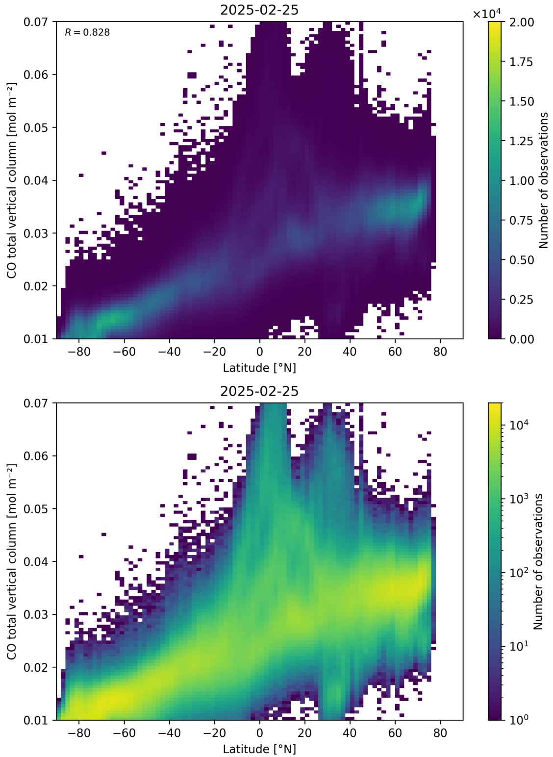
Figure 51: Scatter density plot of “Latitude” against “CO total vertical column” for 2025-02-24 to 2025-02-26.
