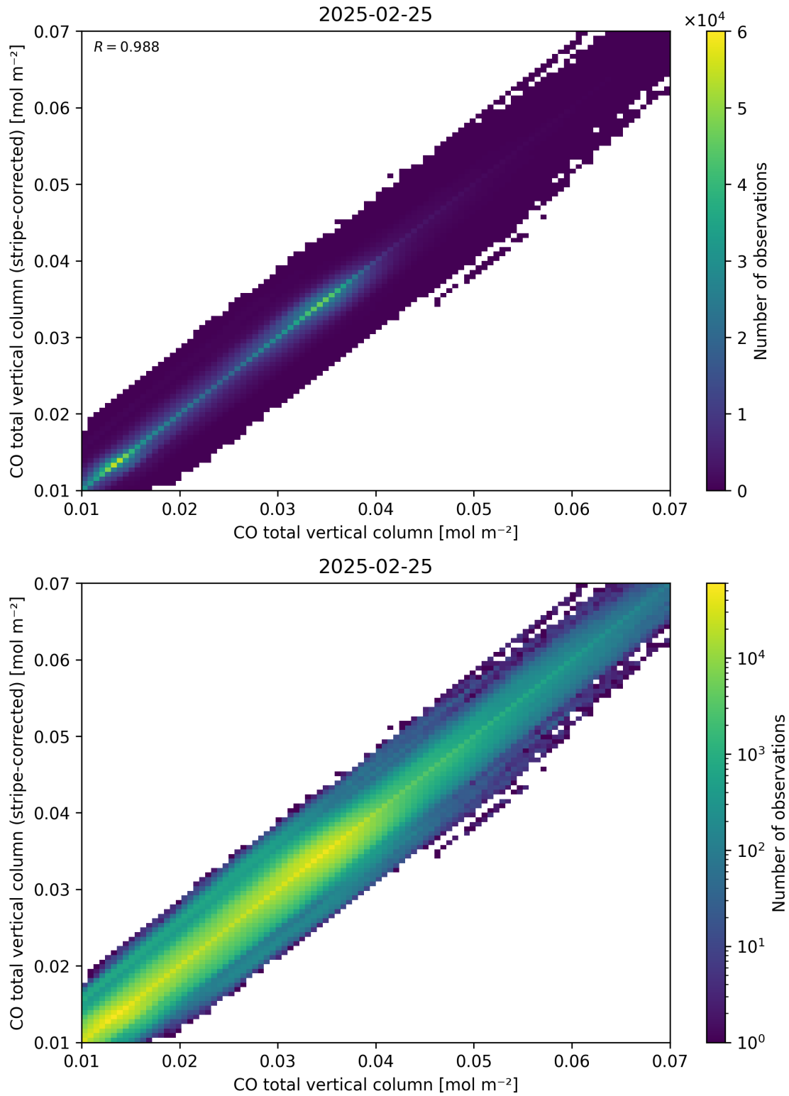
Figure 33: Scatter density plot of “CO total vertical column” against “CO total vertical column (stripe-corrected)” for 2025-02-24 to 2025-02-26.
