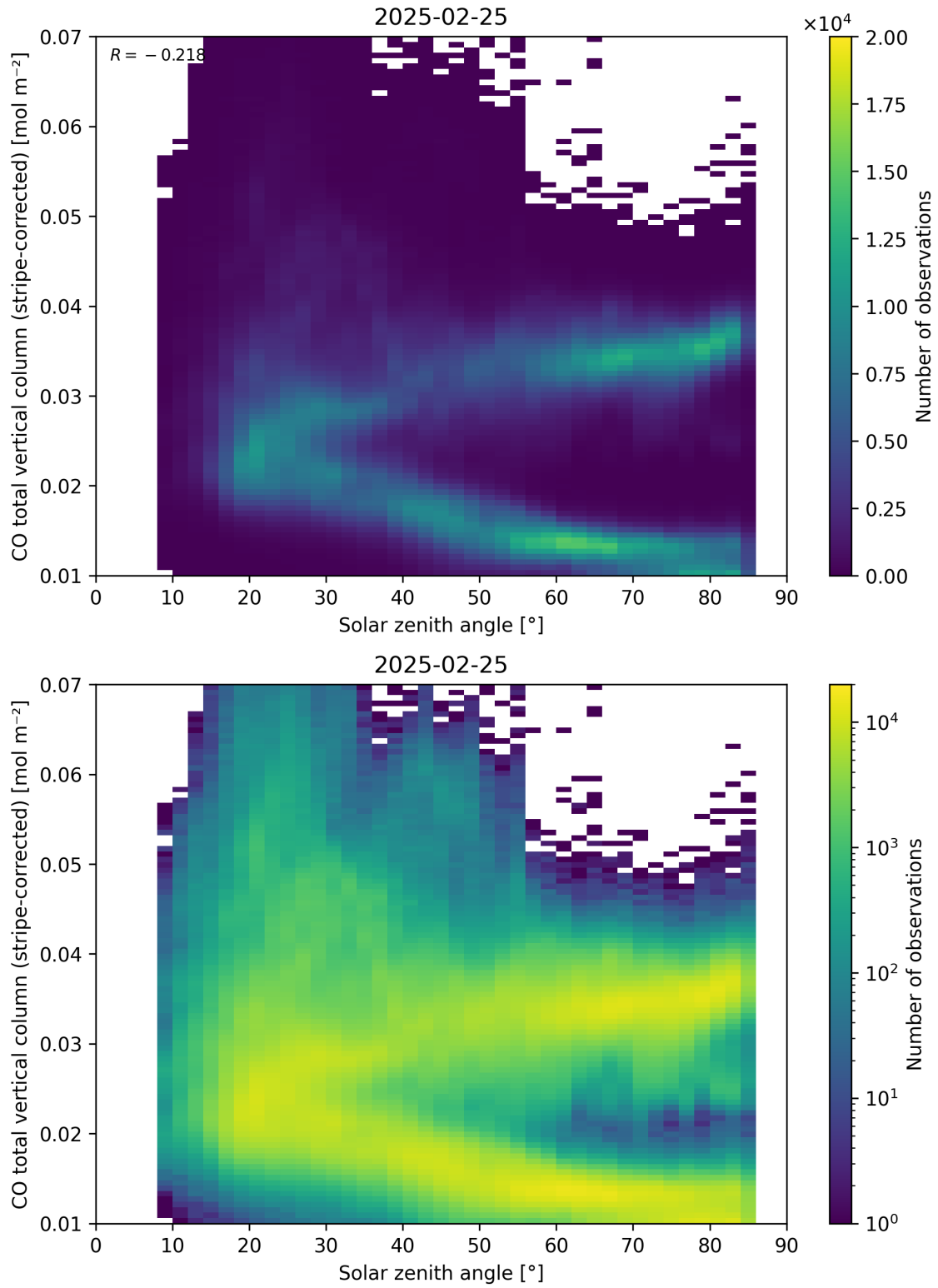
Figure 62: Scatter density plot of “Solar zenith angle” against “CO total vertical column (stripe-corrected)” for 2025-02-24 to 2025-02-26.
