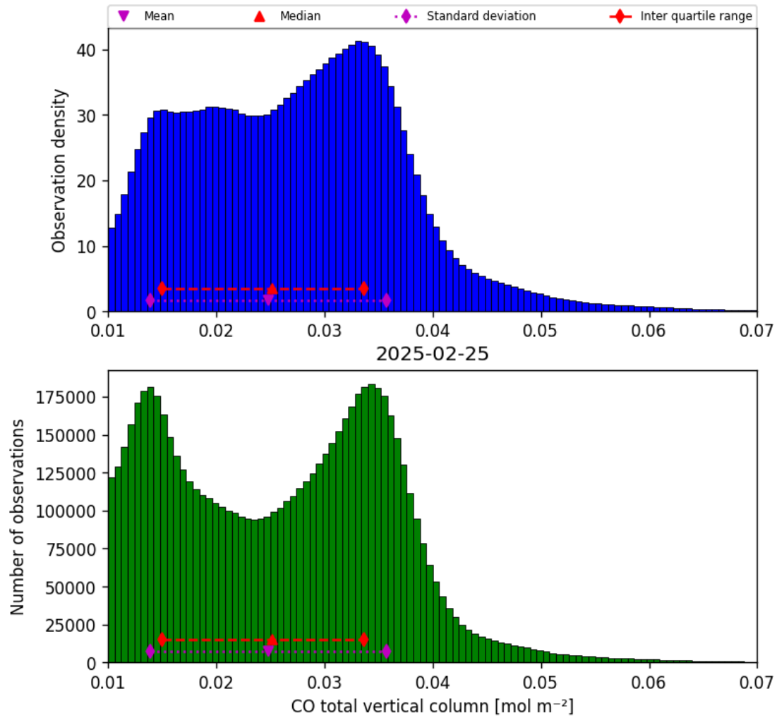
Figure 18: Histogram of “CO total vertical column” for 2025-02-24 to 2025-02-26
