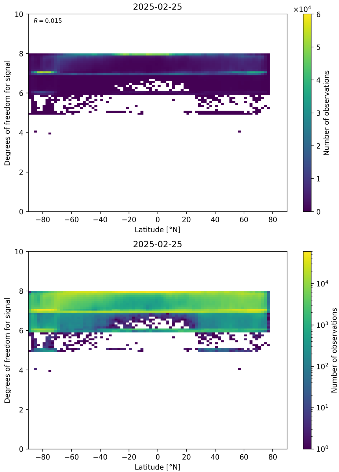
Figure 55: Scatter density plot of “Latitude” against “Degrees of freedom for signal” for 2025-02-24 to 2025-02-26.
