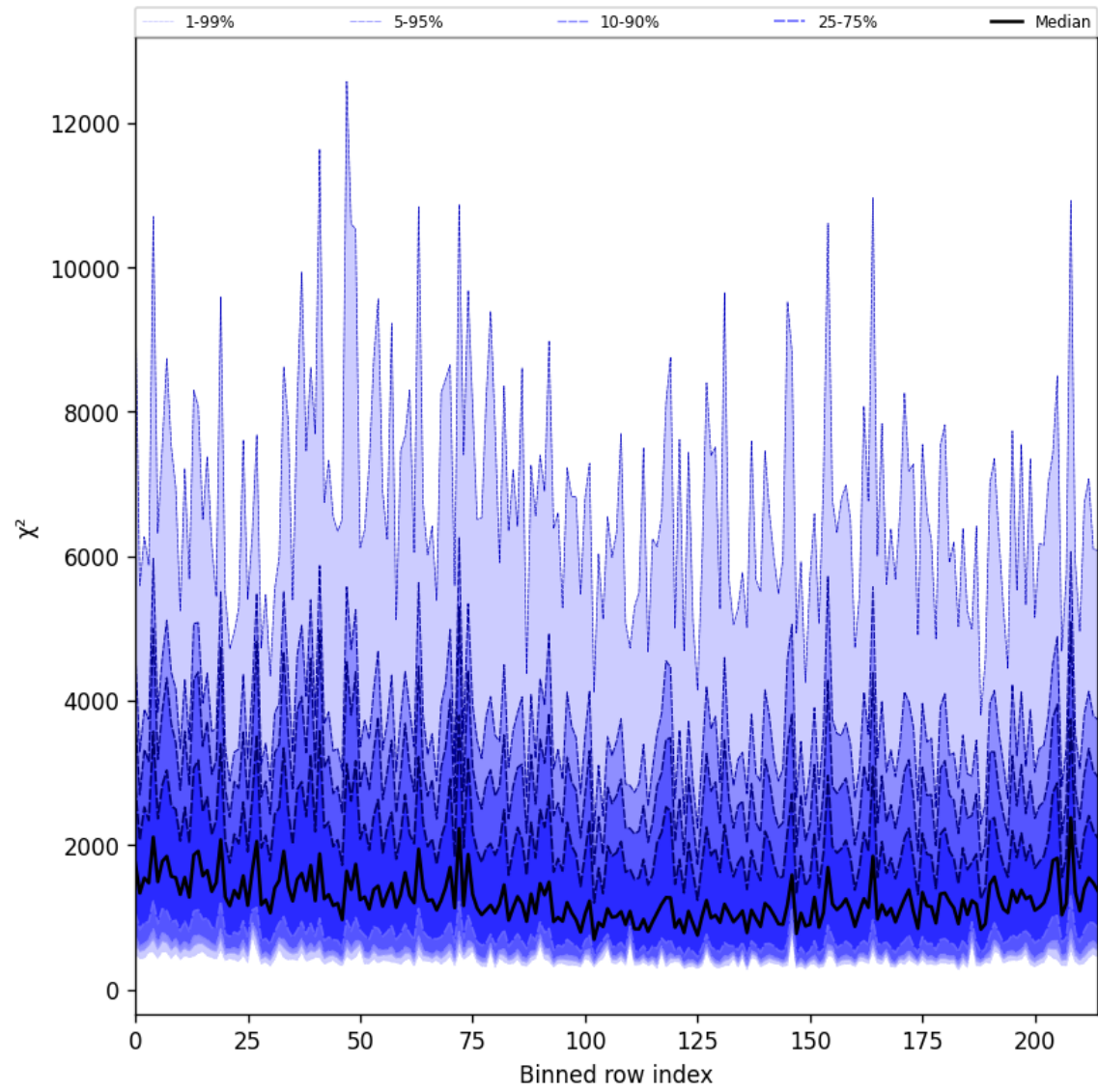
Figure 30: Along track statistics of “ \chi^2 ” for 2025-02-24 to 2025-02-26
