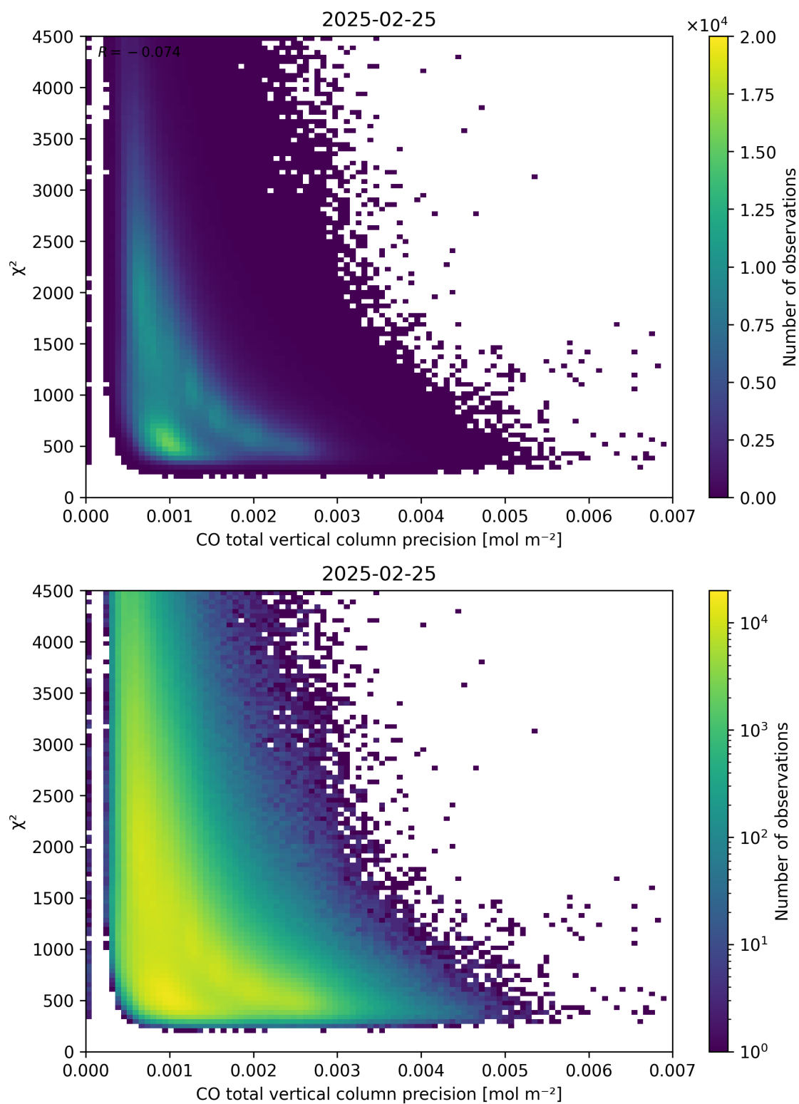
Figure 44: Scatter density plot of “CO total vertical column precision” against “ \chi^2 ” for 2025-02-24 to 2025-02-26.
