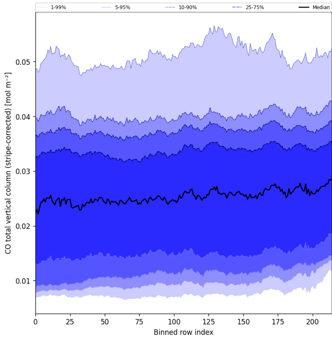
Figure 27: Along track statistics of “CO total vertical column (stripe-corrected)” for 2025-02-24 to 2025-02-26
