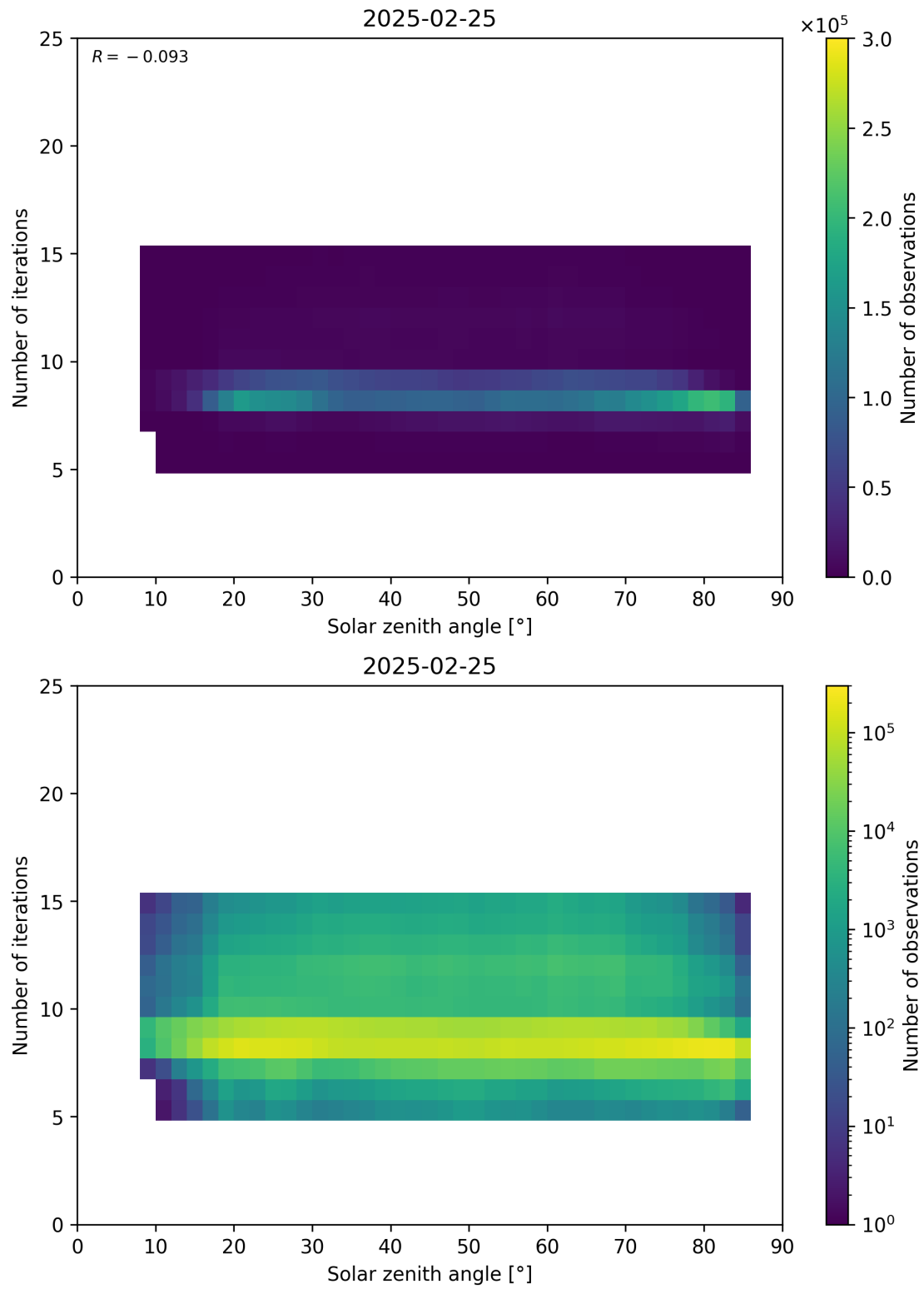
Figure 67: Scatter density plot of “Solar zenith angle” against “Number of iterations” for 2025-02-24 to 2025-02-26.
