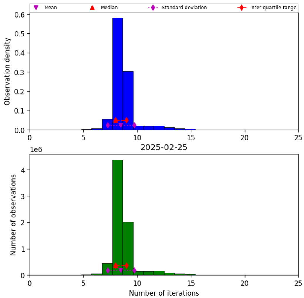
Figure 24: Histogram of “Number of iterations” for 2025-02-24 to 2025-02-26
