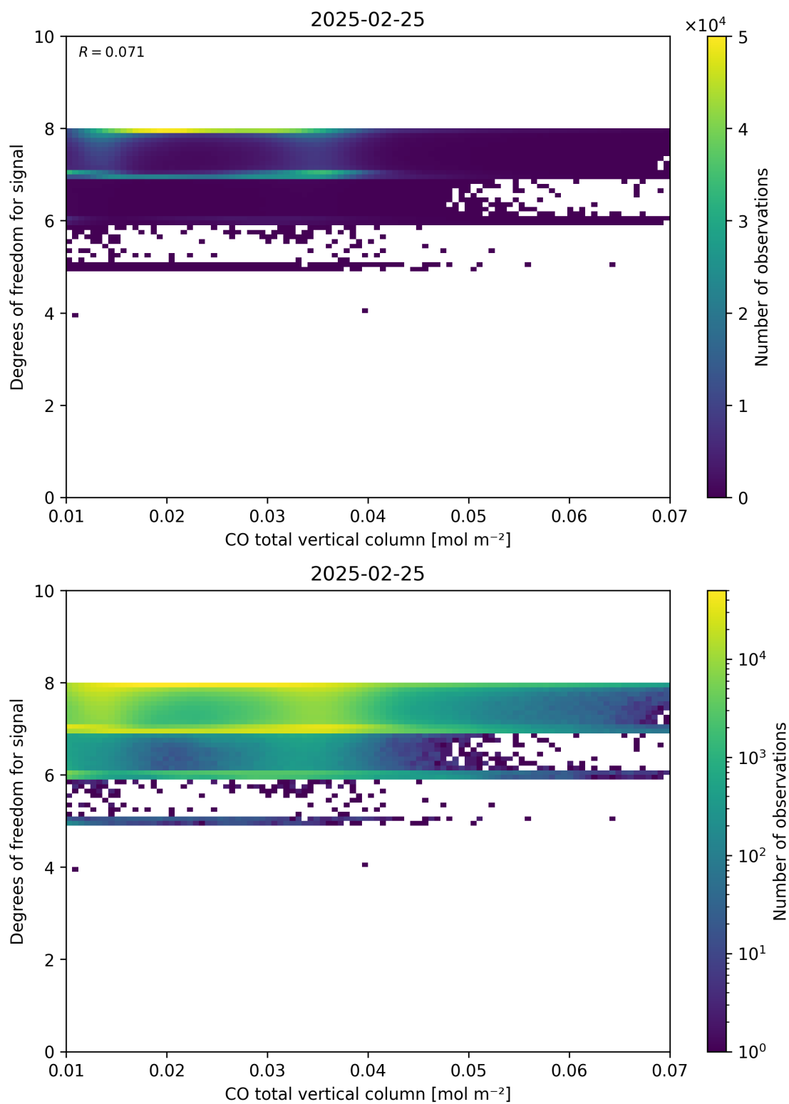
Figure 41: Scatter density plot of “CO total vertical column” against “Degrees of freedom for signal” for 2025-02-24 to 2025-02-26.
