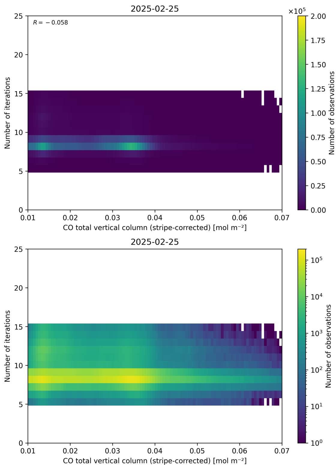
Figure 39: Scatter density plot of “CO total vertical column (stripe-corrected)” against “Number of iterations” for 2025-02-24 to 2025-02-26.
