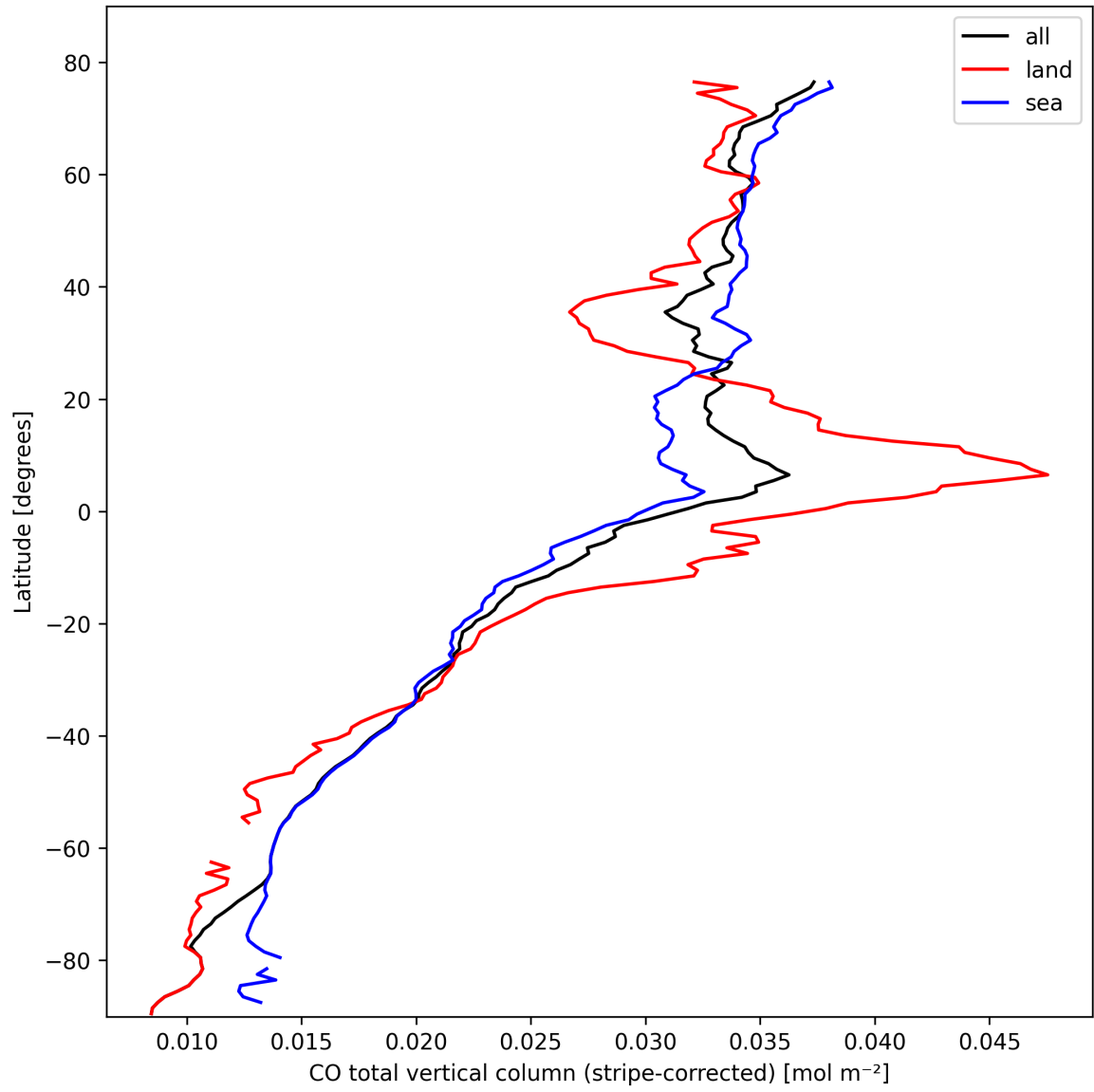
Figure 11: Zonal average of “CO total vertical column (stripe-corrected)” for 2025-02-24 to 2025-02-26.
