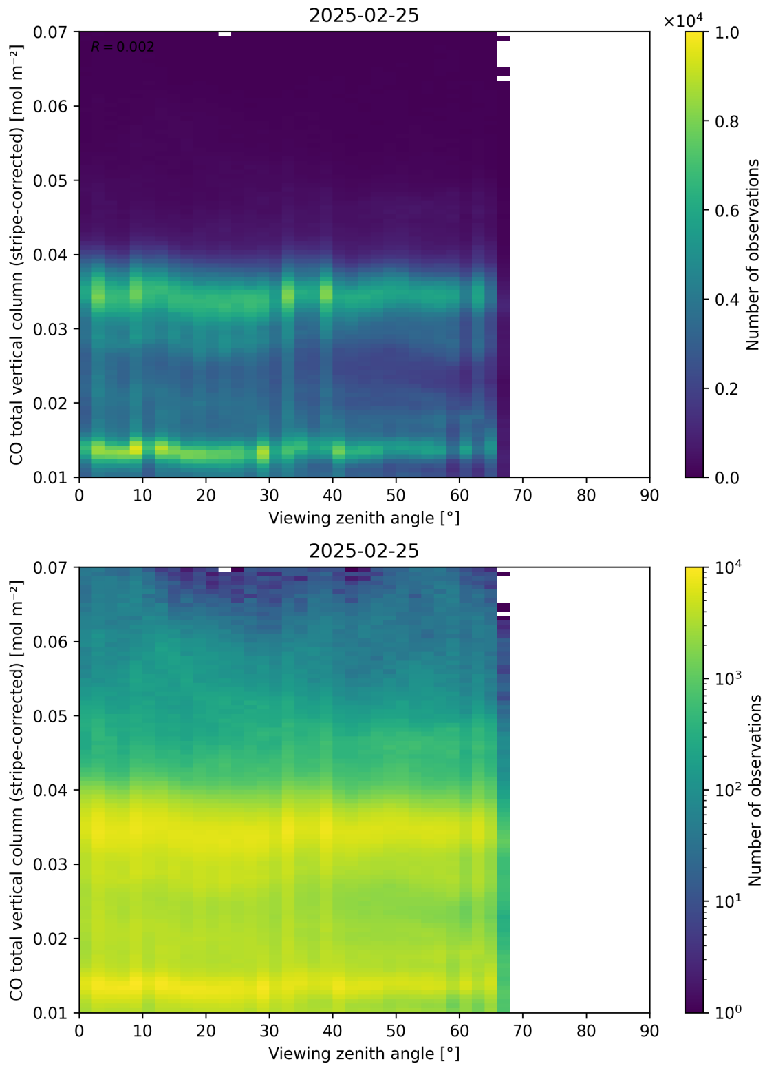
Figure 70: Scatter density plot of “Viewing zenith angle” against “CO total vertical column (stripe-corrected)” for 2025-02-24 to 2025-02-26.
