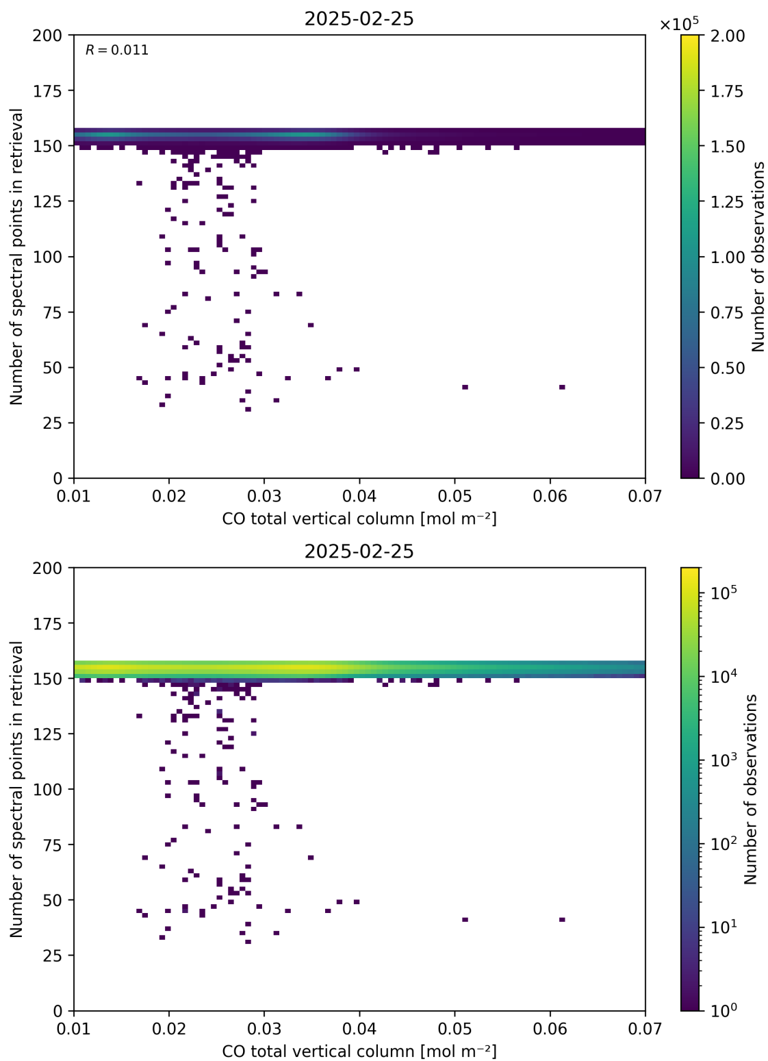
Figure 43: Scatter density plot of “CO total vertical column” against “Number of spectral points in retrieval” for 2025-02-24 to 2025-02-26.
