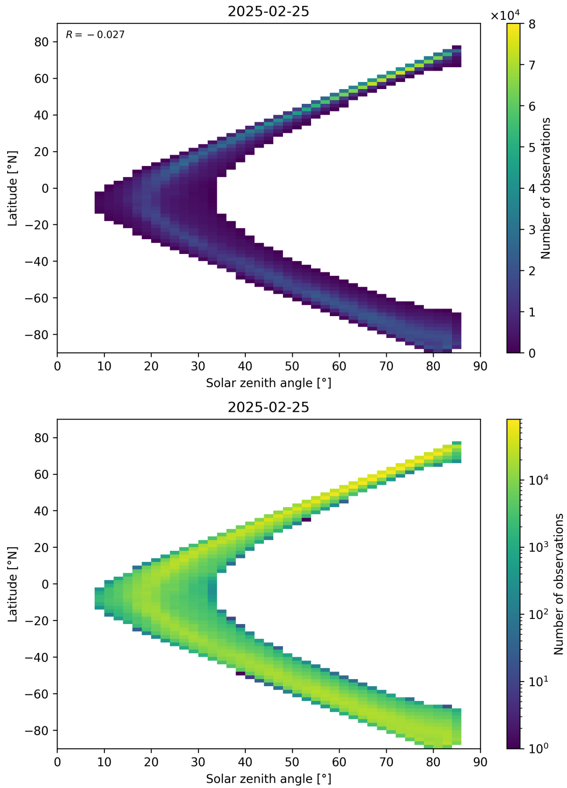
Figure 66: Scatter density plot of “Solar zenith angle” against “Latitude” for 2025-02-24 to 2025-02-26.
