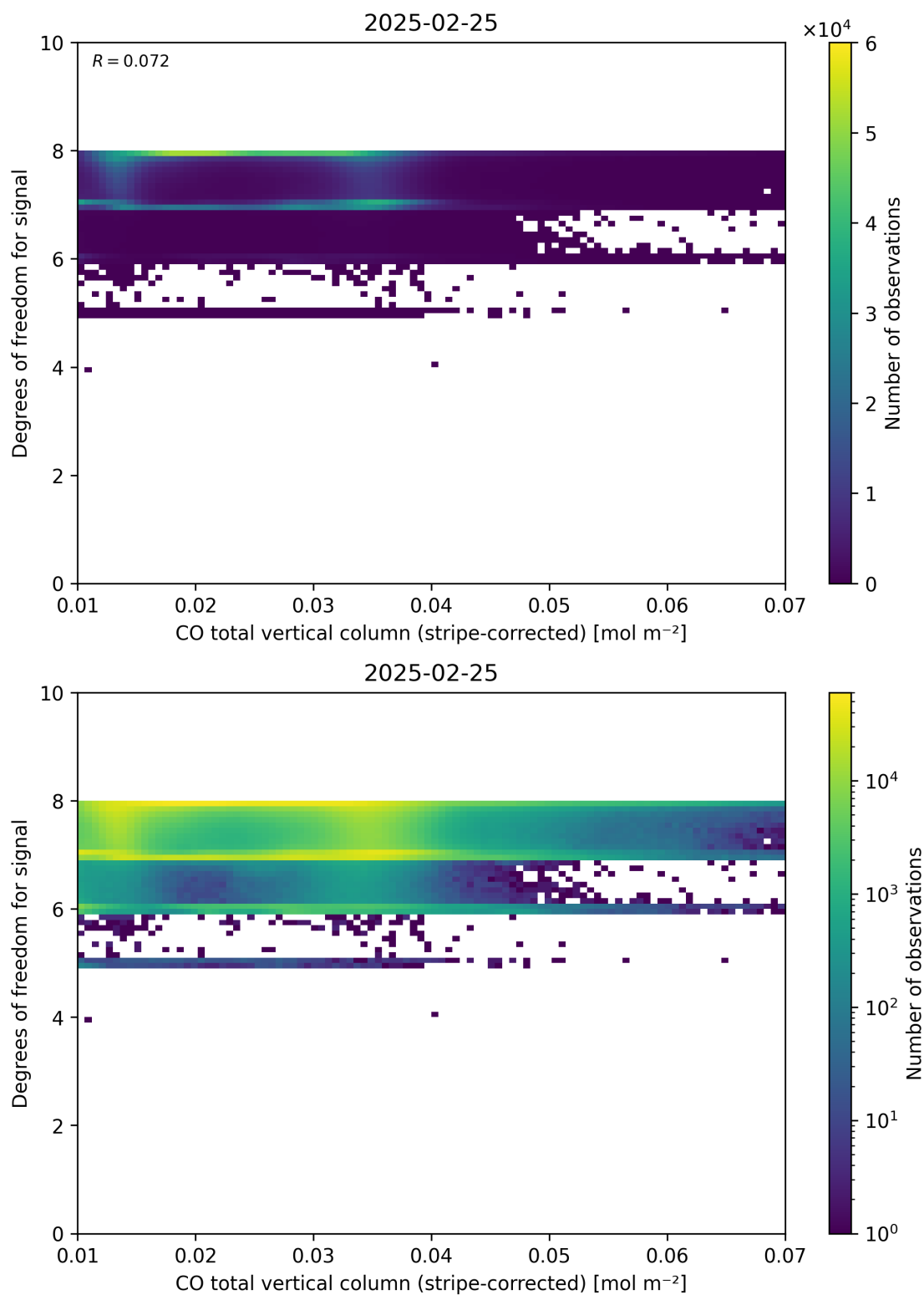
Figure 38: Scatter density plot of “CO total vertical column (stripe-corrected)” against “Degrees of freedom for signal” for 2025-02-24 to 2025-02-26.
