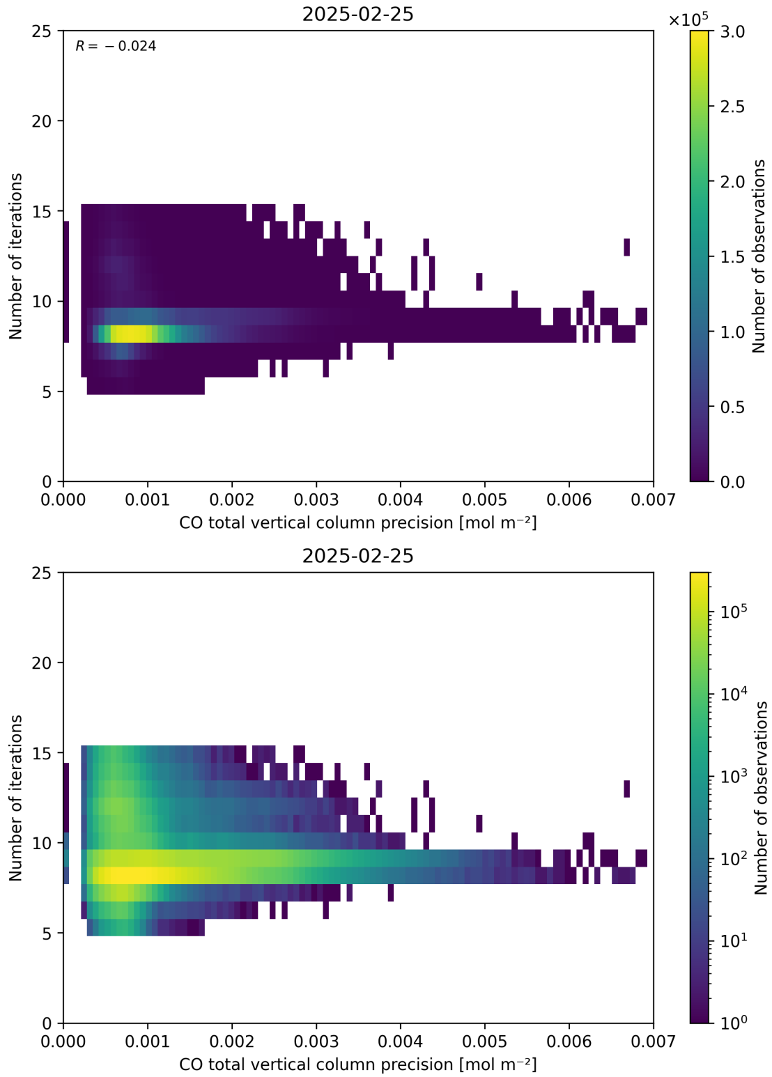
Figure 46: Scatter density plot of “CO total vertical column precision” against “Number of iterations” for 2025-02-24 to 2025-02-26.
