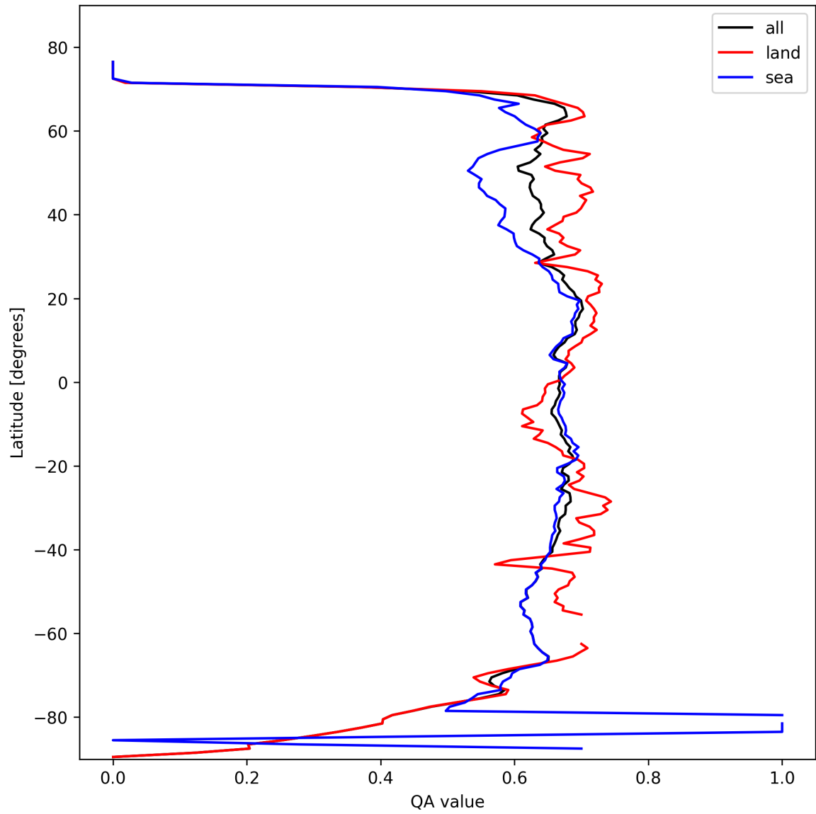
Figure 9: Zonal average of “QA value” for 2025-02-24 to 2025-02-26.
