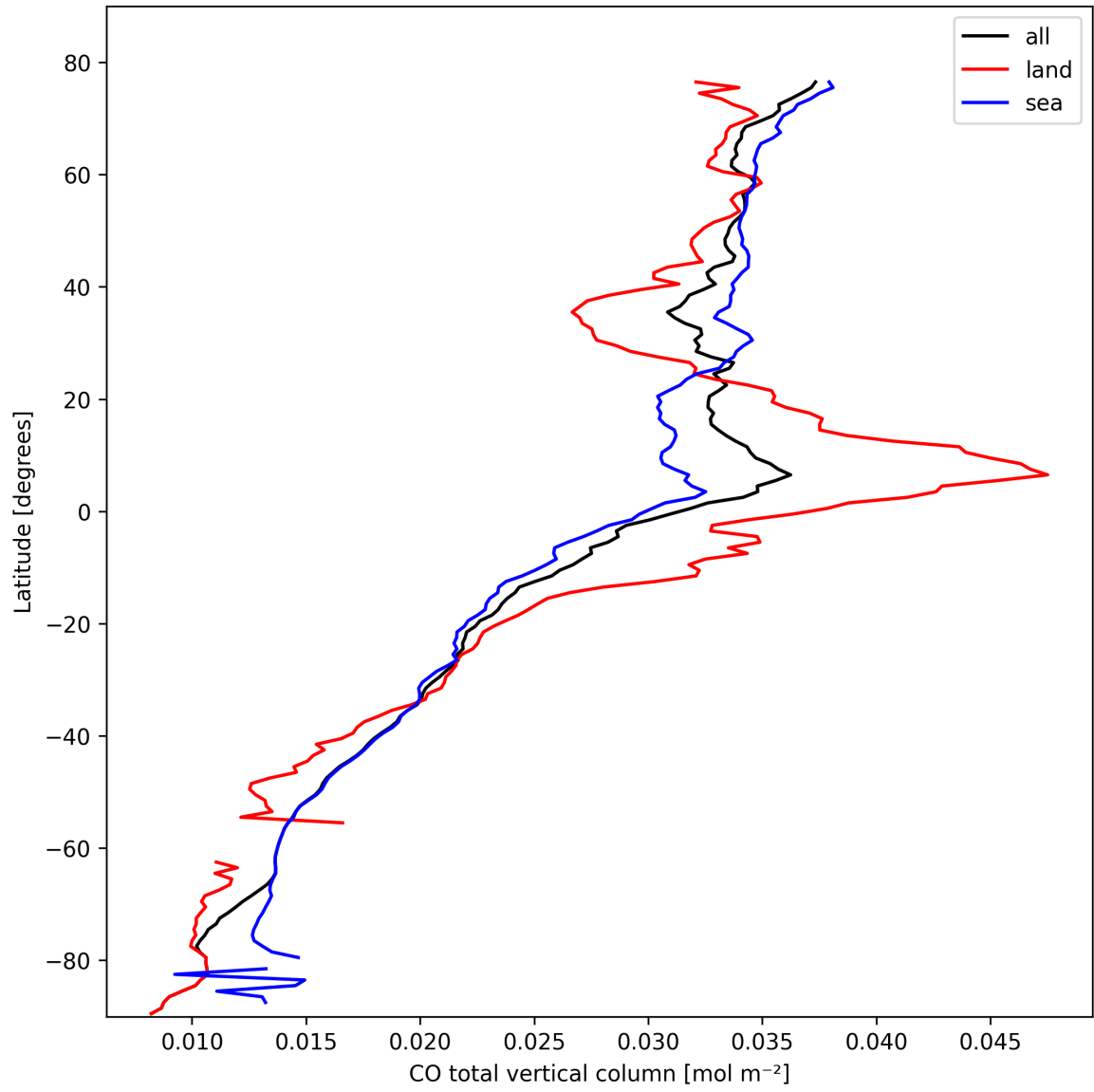
Figure 10: Zonal average of “CO total vertical column” for 2025-02-24 to 2025-02-26.
