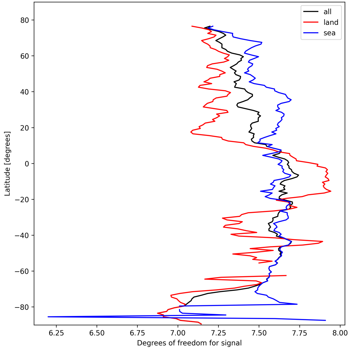
Figure 15: Zonal average of “Degrees of freedom for signal” for 2025-02-24 to 2025-02-26.
