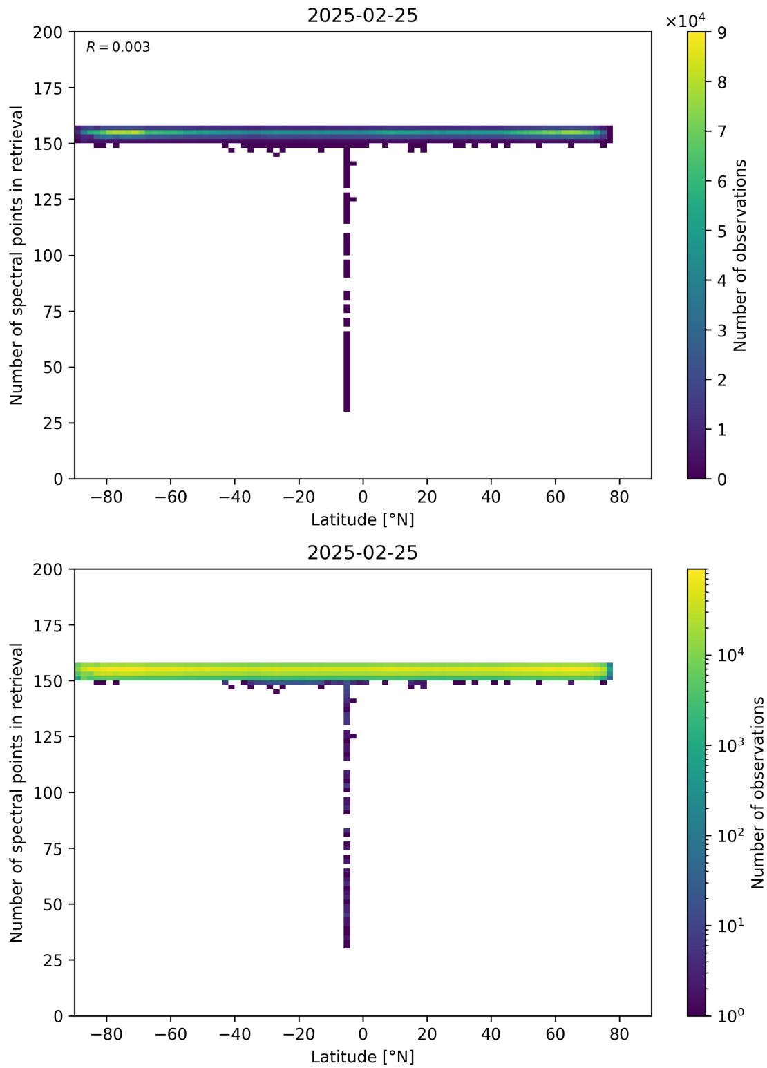
Figure 57: Scatter density plot of “Latitude” against “Number of spectral points in retrieval” for 2025-02-24 to 2025-02-26.
