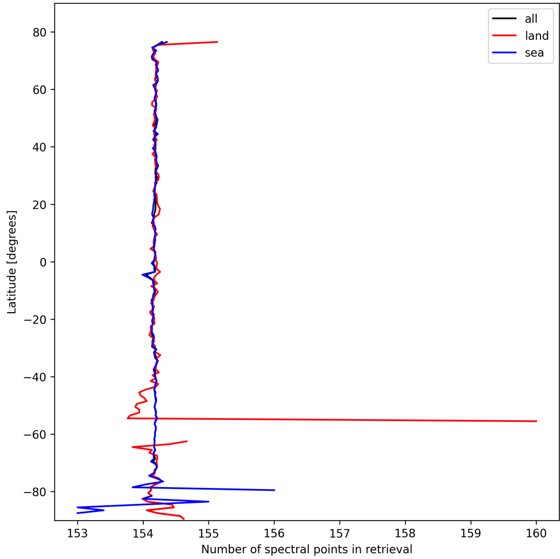
Figure 13: Zonal average of “Number of spectral points in retrieval” for 2025-02-24 to 2025-02-26.
