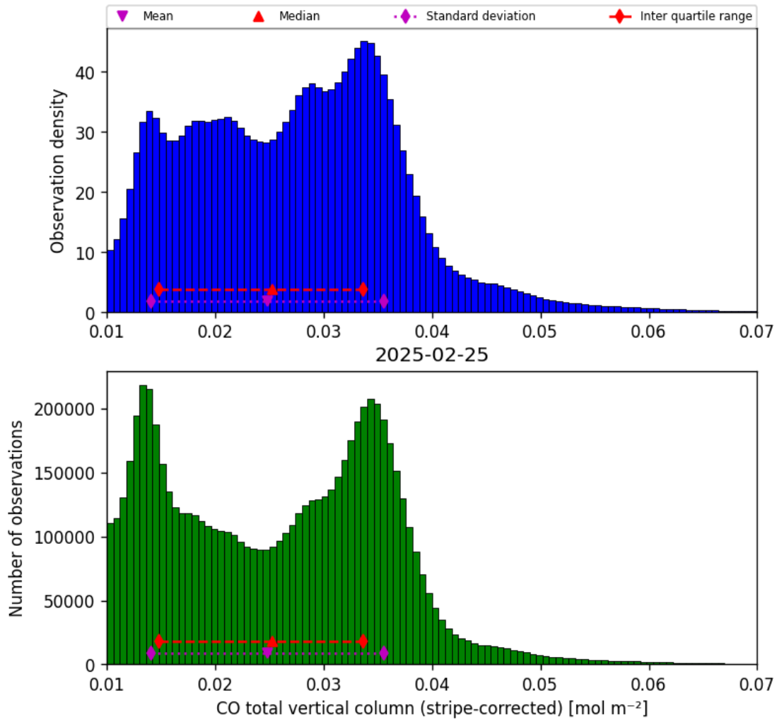
Figure 19: Histogram of “CO total vertical column (stripe-corrected)” for 2025-02-24 to 2025-02-26
