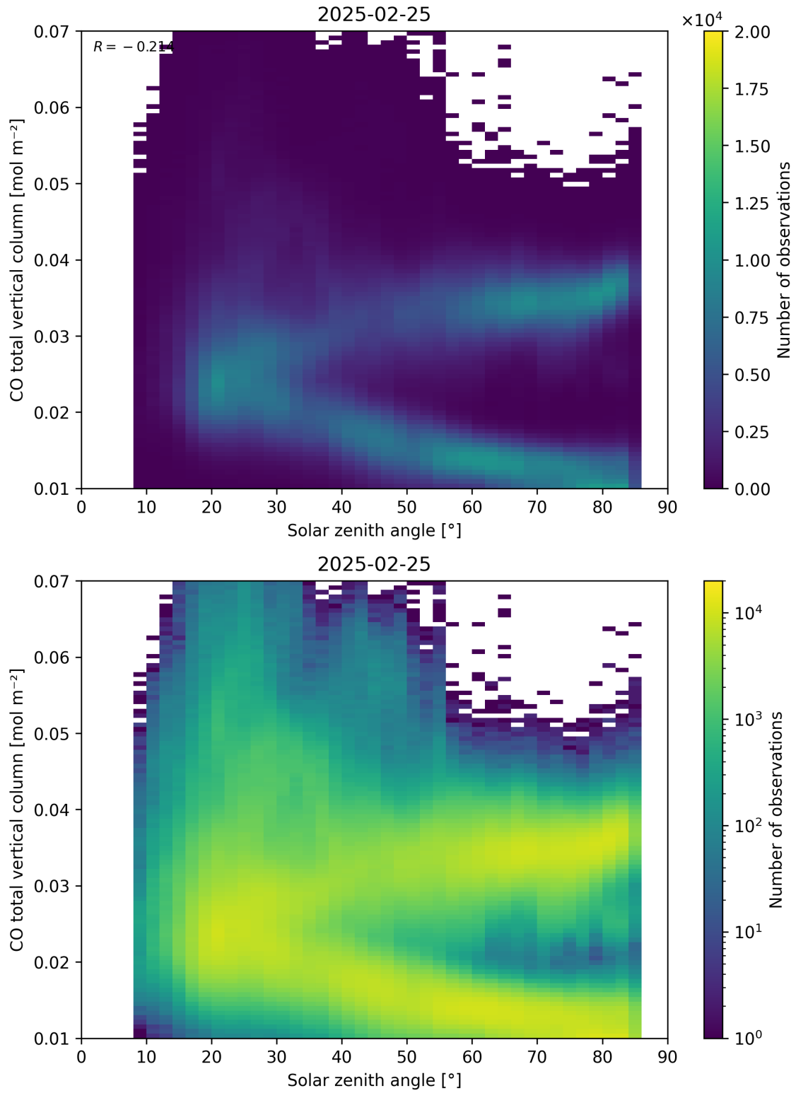
Figure 61: Scatter density plot of “Solar zenith angle” against “CO total vertical column” for 2025-02-24 to 2025-02-26.
