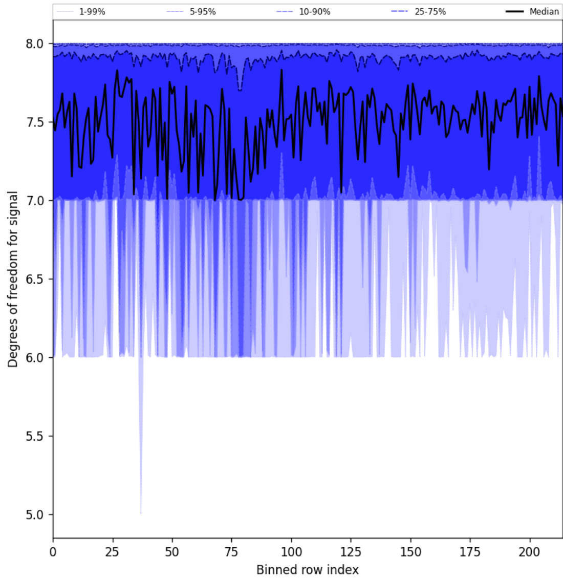
Figure 31: Along track statistics of “Degrees of freedom for signal” for 2025-02-24 to 2025-02-26
