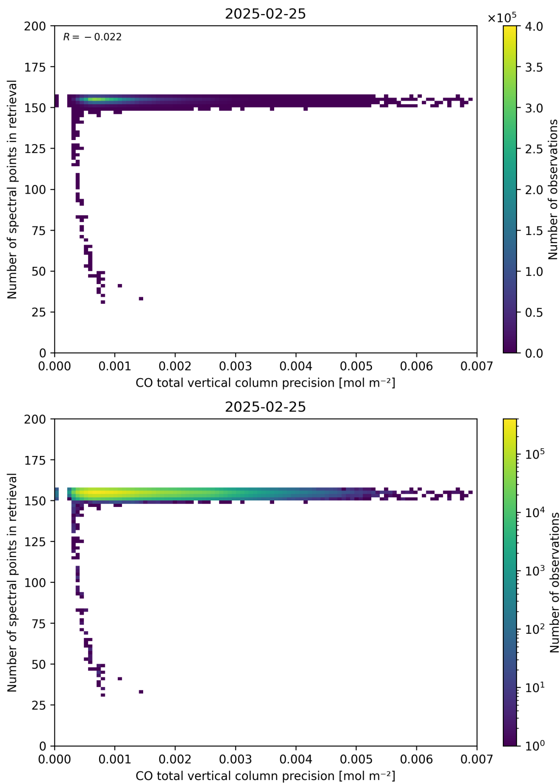
Figure 47: Scatter density plot of “CO total vertical column precision” against “Number of spectral points in retrieval” for 2025-02-24 to 2025-02-26.
