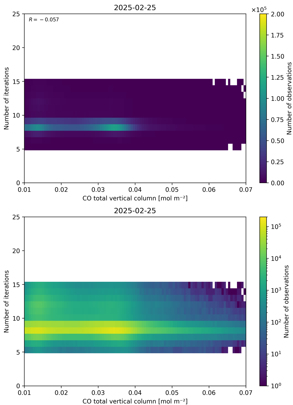
Figure 42: Scatter density plot of “CO total vertical column” against “Number of iterations” for 2025-02-24 to 2025-02-26.
