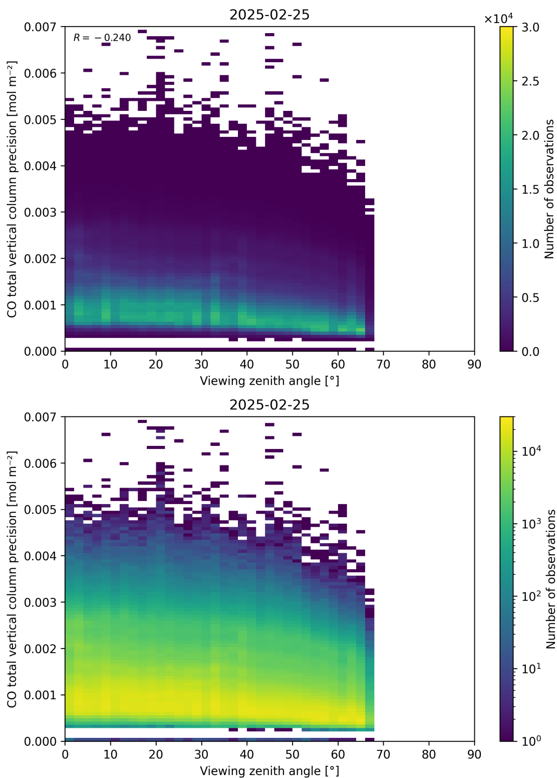
Figure 71: Scatter density plot of “Viewing zenith angle” against “CO total vertical column precision” for 2025-02-24 to 2025-02-26.
