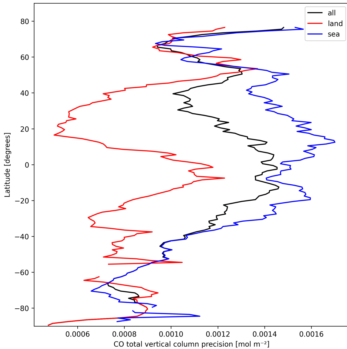
Figure 12: Zonal average of “CO total vertical column precision” for 2025-02-24 to 2025-02-26.
