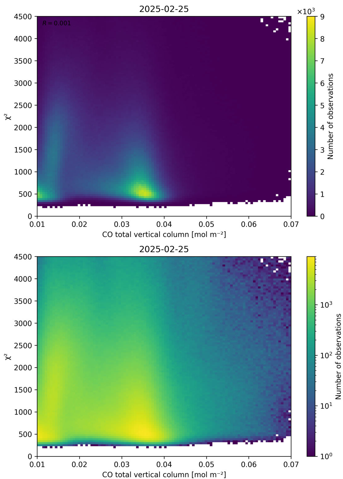
Figure 35: Scatter density plot of “CO total vertical column” against “ \chi^2 ” for 2025-02-24 to 2025-02-26.
