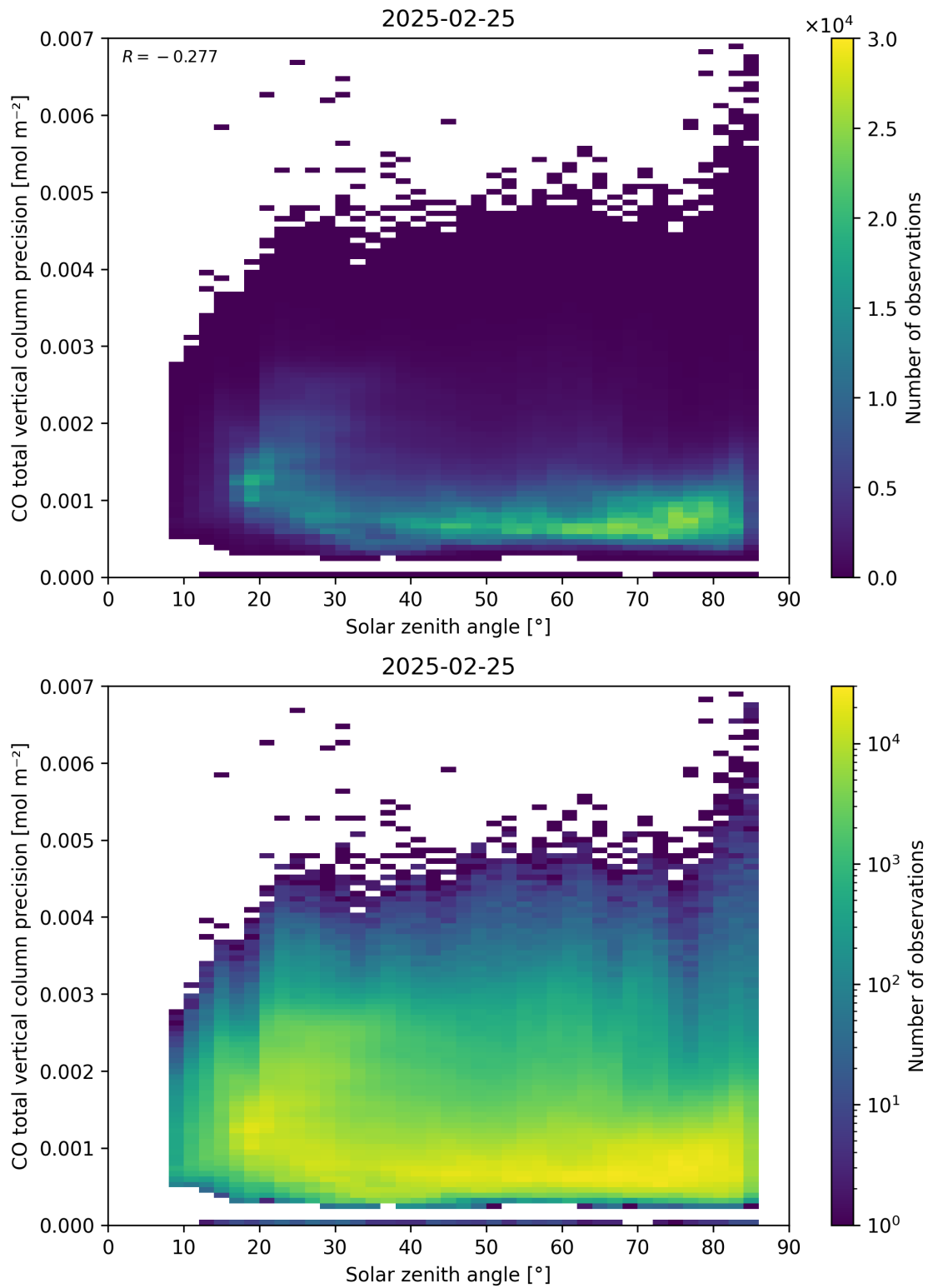
Figure 63: Scatter density plot of “Solar zenith angle” against “CO total vertical column precision” for 2025-02-24 to 2025-02-26.
