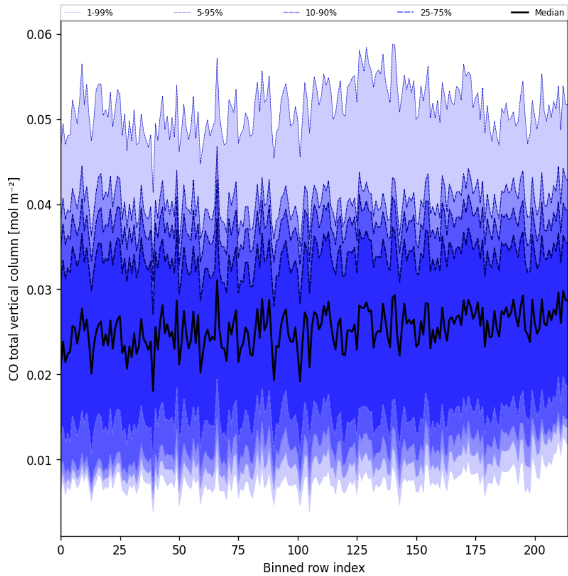
Figure 26: Along track statistics of “CO total vertical column” for 2025-02-24 to 2025-02-26
