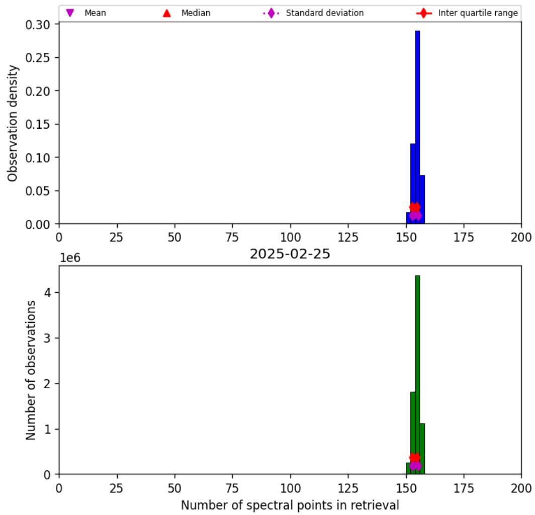
Figure 21: Histogram of “Number of spectral points in retrieval” for 2025-02-24 to 2025-02-26
