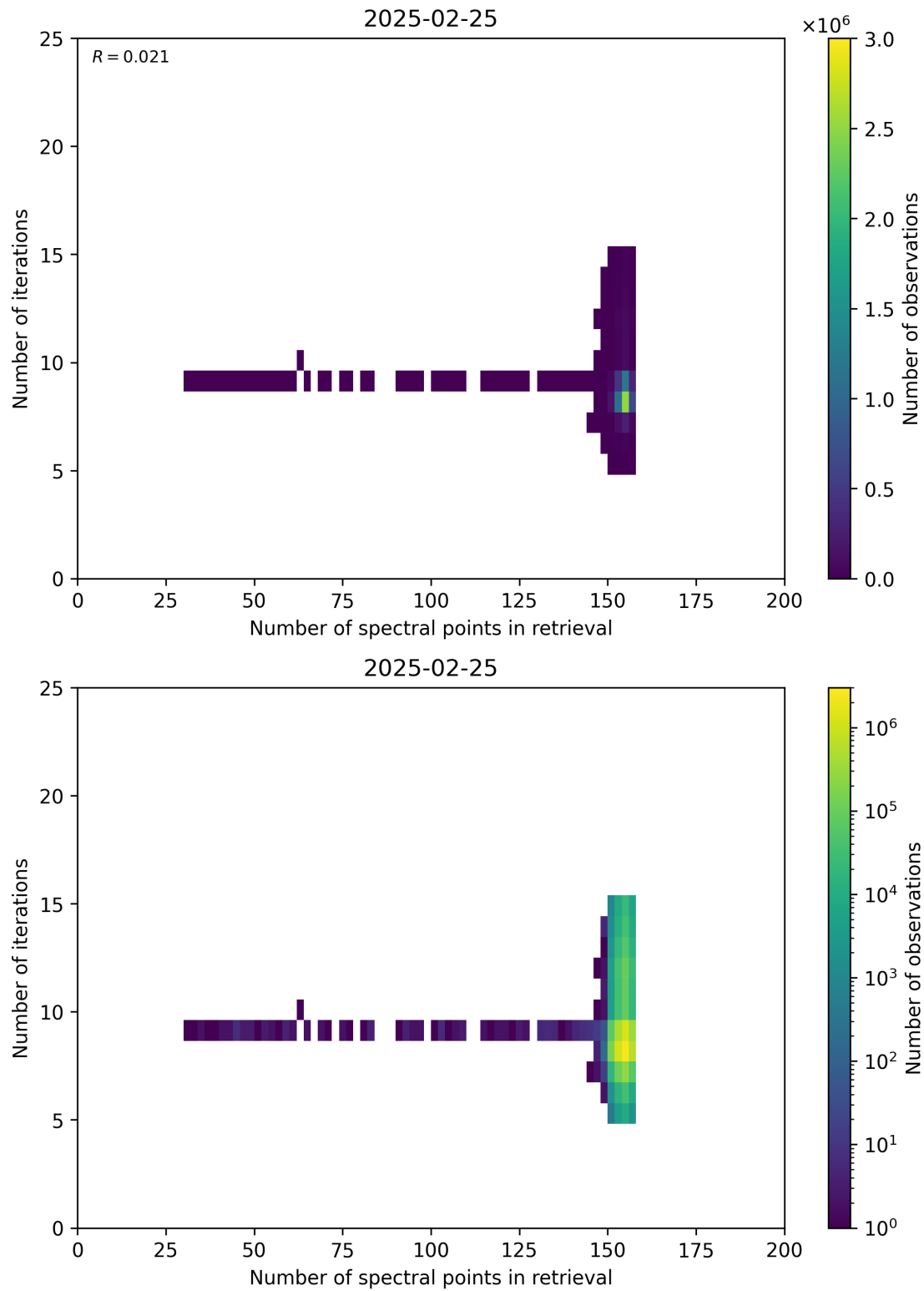
Figure 60: Scatter density plot of “Number of spectral points in retrieval” against “Number of iterations” for 2025-02-24 to 2025-02-26.
