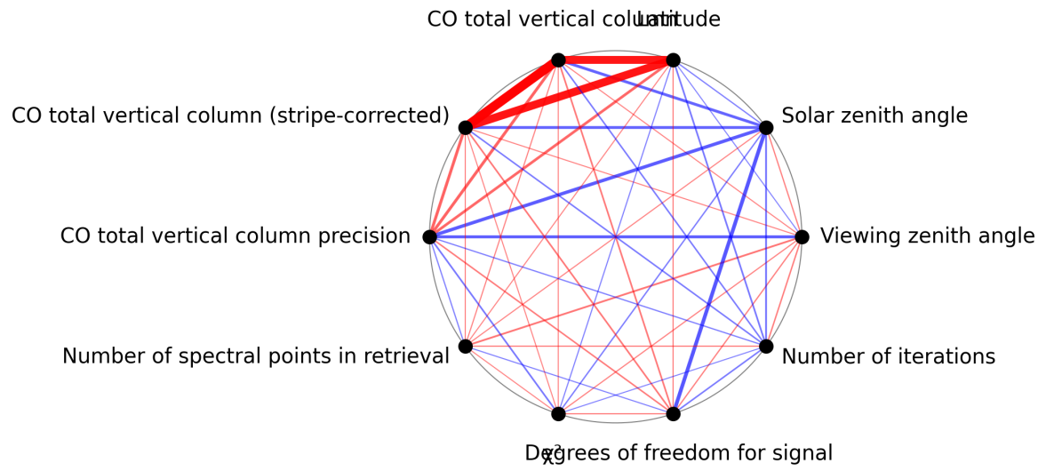
Figure 1: Map of correlation graph for 2025-02-24 to 2025-02-26.
