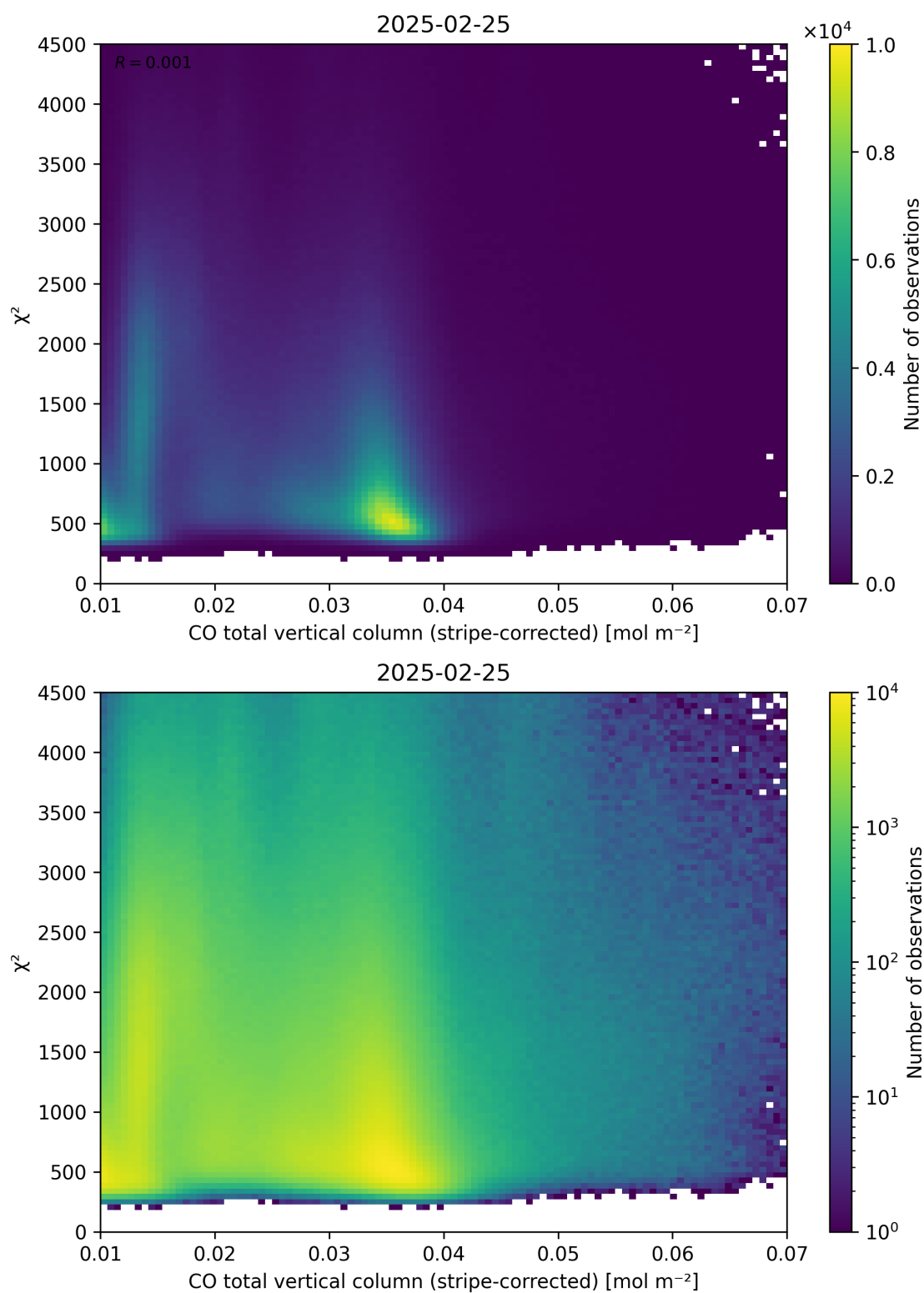
Figure 37: Scatter density plot of “CO total vertical column (stripe-corrected)” against “ \chi^2 ” for 2025-02-24 to 2025-02-26.
