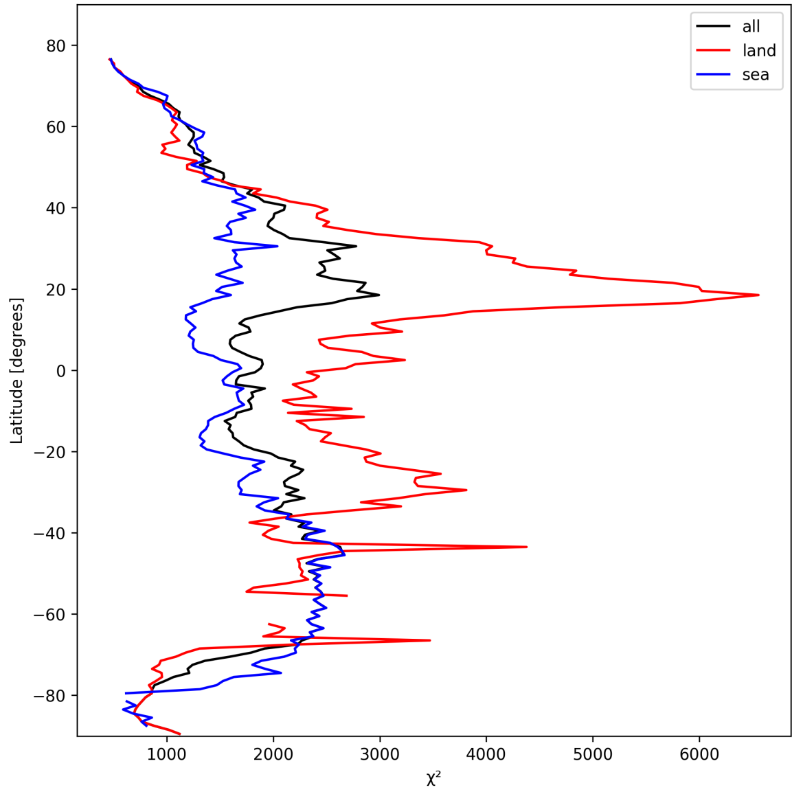
Figure 14: Zonal average of “ \chi^2 ” for 2025-02-24 to 2025-02-26.
