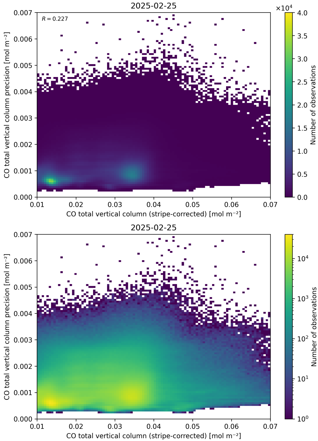
Figure 36: Scatter density plot of “CO total vertical column (stripe-corrected)” against “CO total vertical column precision” for 2025-02-24 to 2025-02-26.
