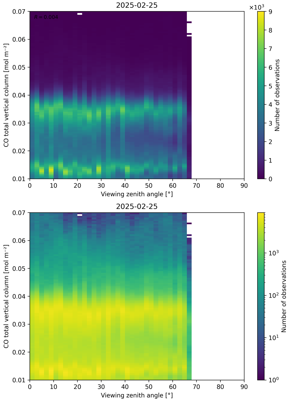
Figure 69: Scatter density plot of “Viewing zenith angle” against “CO total vertical column” for 2025-02-24 to 2025-02-26.
