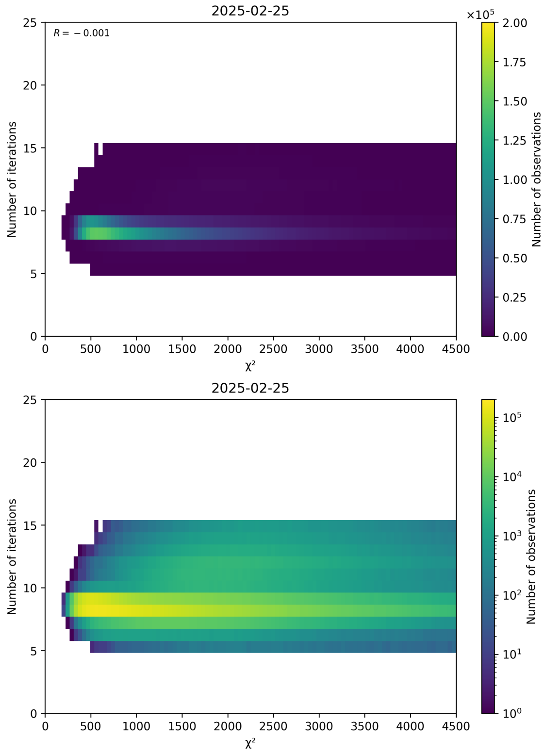
Figure 49: Scatter density plot of “ \chi^2 ” against “Number of iterations” for 2025-02-24 to 2025-02-26.
