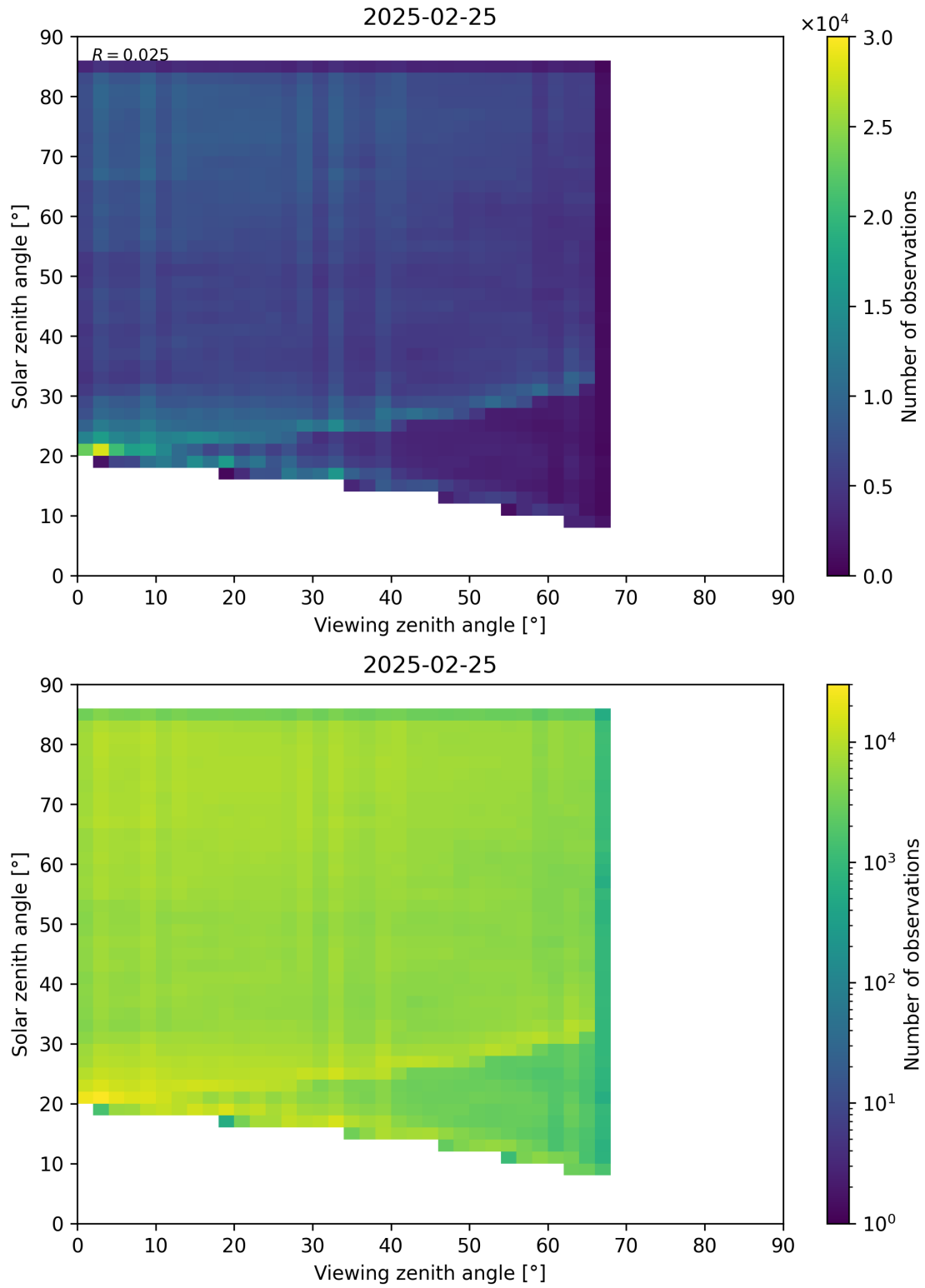
Figure 77: Scatter density plot of “Viewing zenith angle” against “Solar zenith angle” for 2025-02-24 to 2025-02-26.
