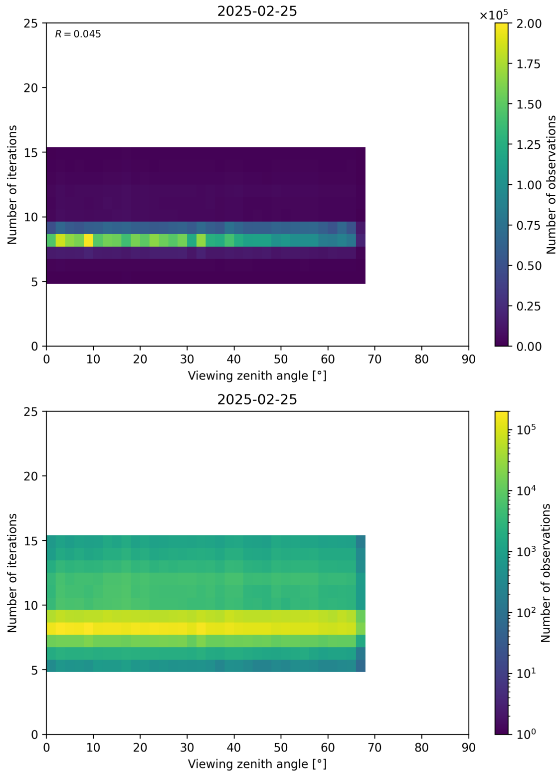
Figure 75: Scatter density plot of “Viewing zenith angle” against “Number of iterations” for 2025-02-24 to 2025-02-26.
