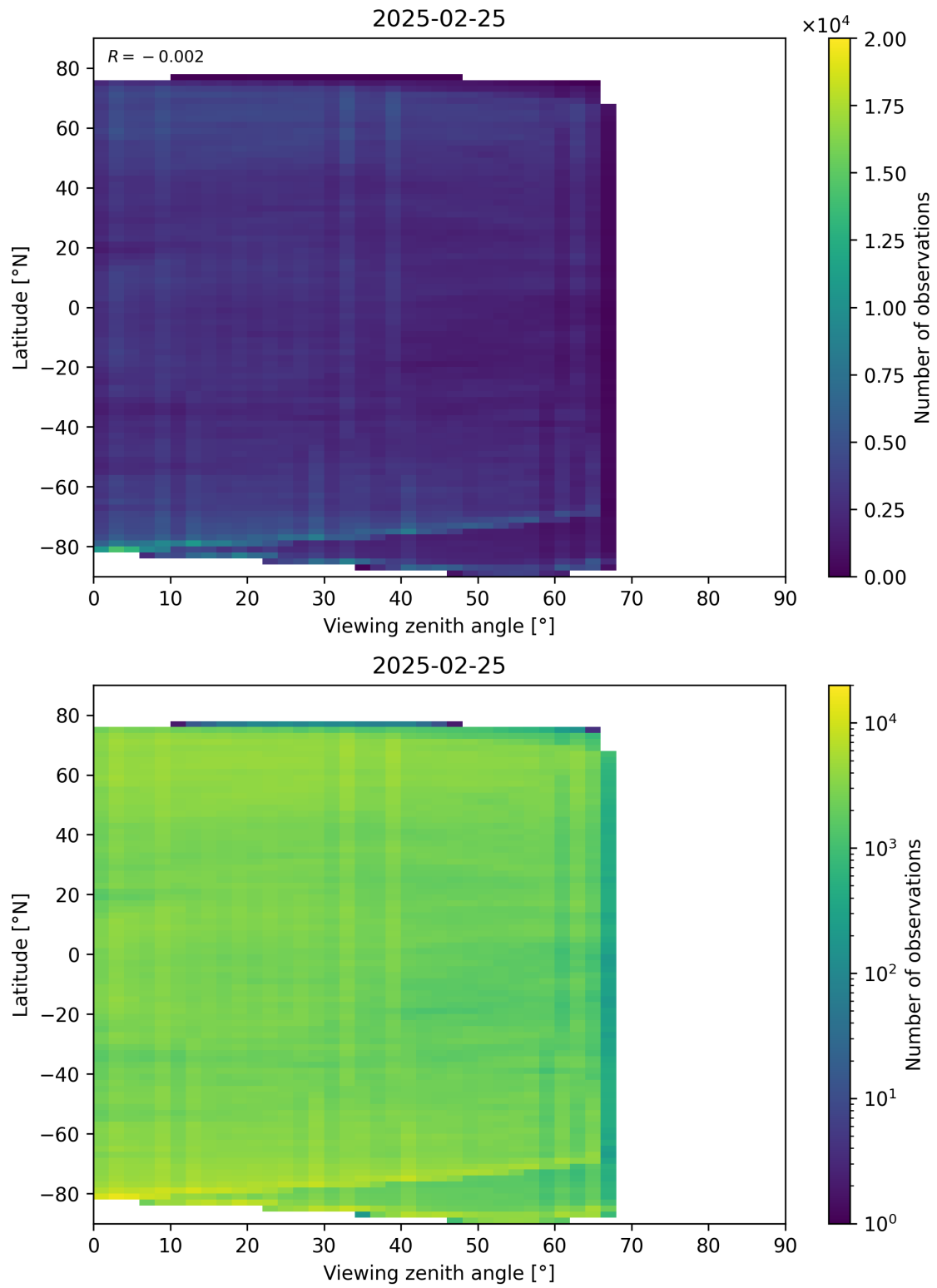
Figure 74: Scatter density plot of “Viewing zenith angle” against “Latitude” for 2025-02-24 to 2025-02-26.
