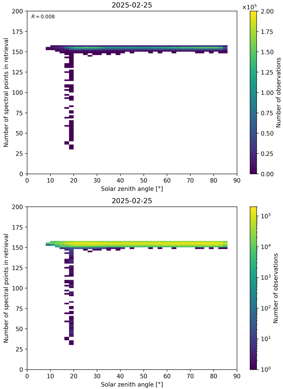
Figure 68: Scatter density plot of “Solar zenith angle” against “Number of spectral points in retrieval” for 2025-02-24 to 2025-02-26.
