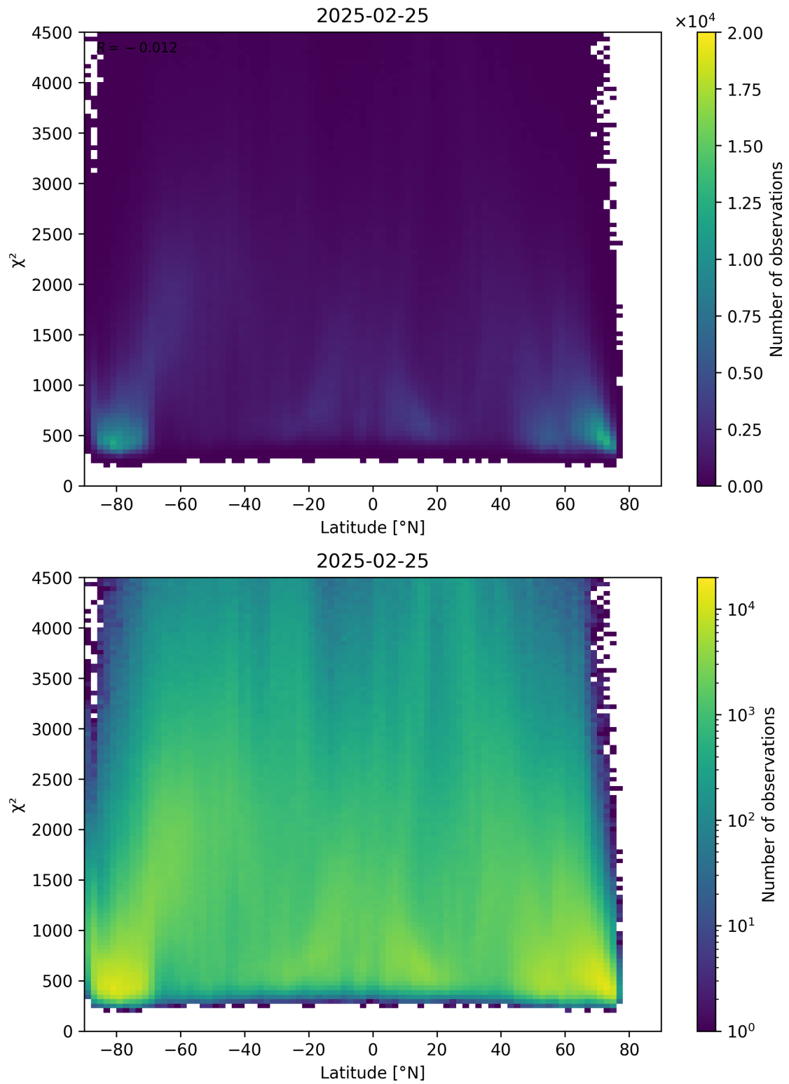
Figure 54: Scatter density plot of “Latitude” against “ \chi^2 ” for 2025-02-24 to 2025-02-26.
