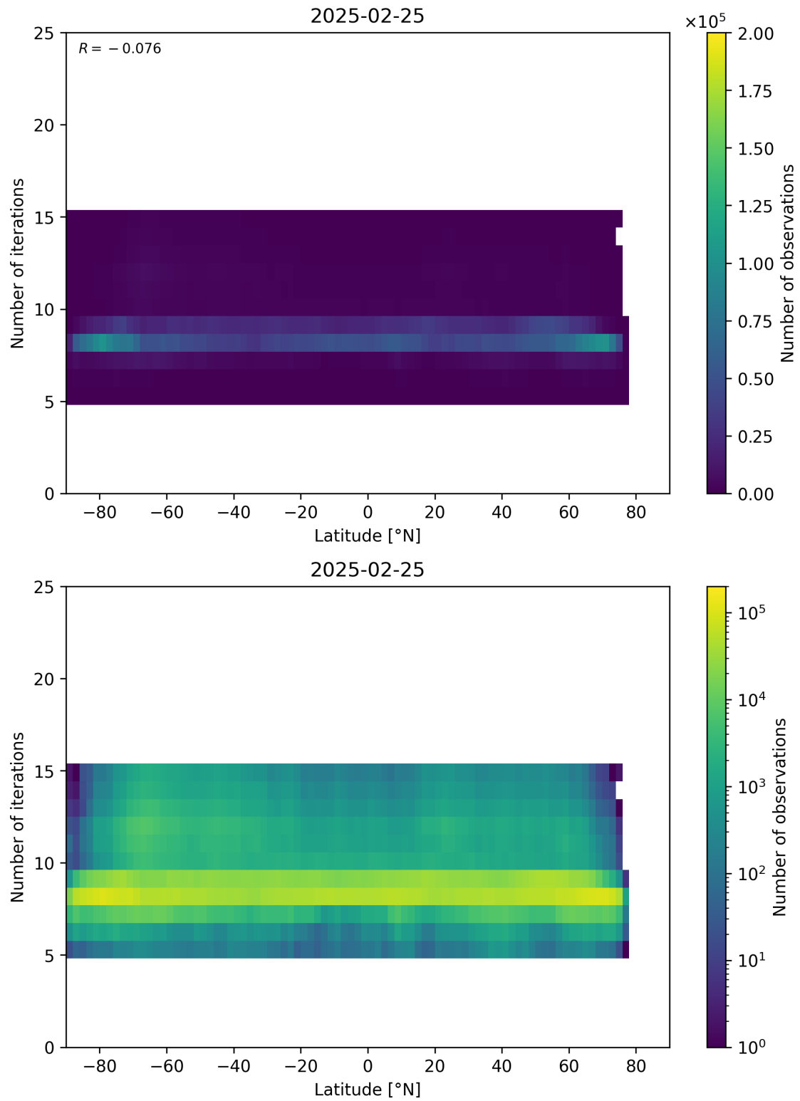
Figure 56: Scatter density plot of “Latitude” against “Number of iterations” for 2025-02-24 to 2025-02-26.
