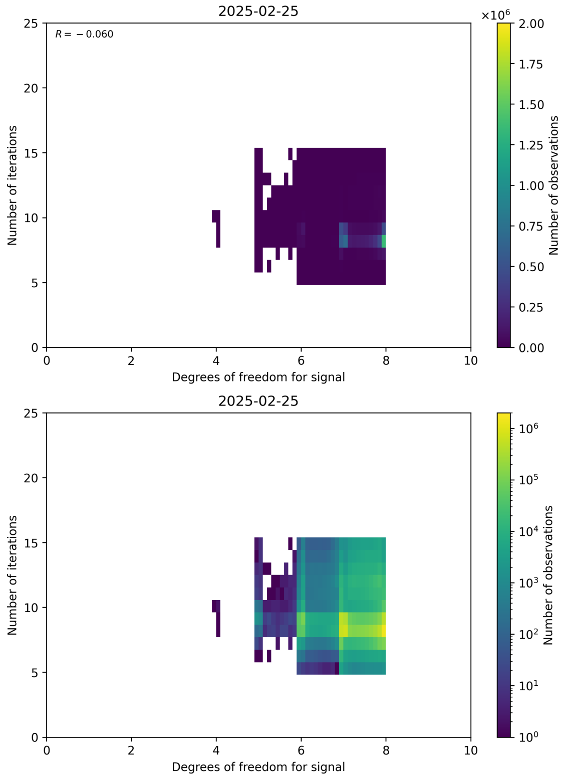
Figure 50: Scatter density plot of “Degrees of freedom for signal” against “Number of iterations” for 2025-02-24 to 2025-02-26.
