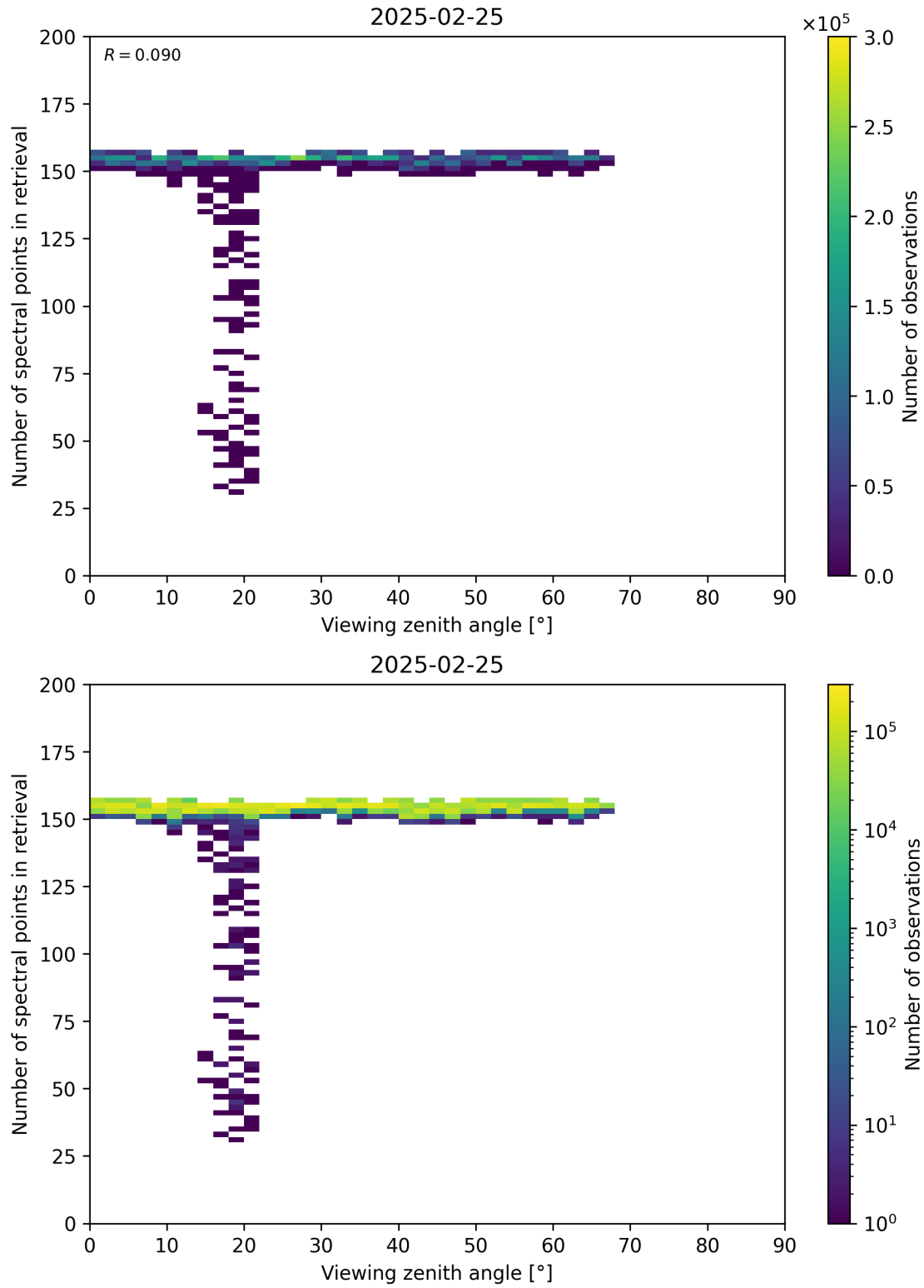
Figure 76: Scatter density plot of “Viewing zenith angle” against “Number of spectral points in retrieval” for 2025-02-24 to 2025-02-26.
