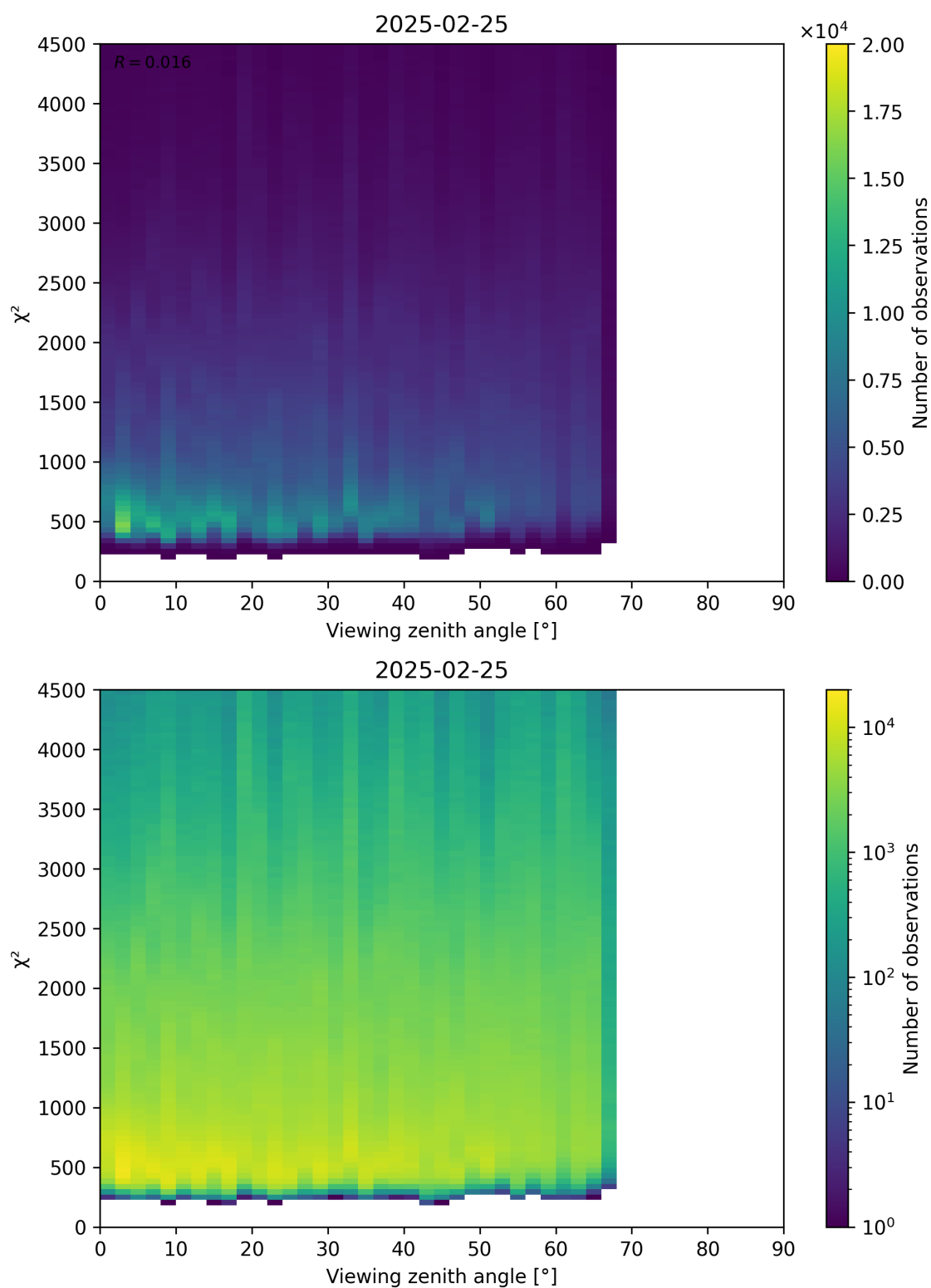
Figure 72: Scatter density plot of “Viewing zenith angle” against “ \chi^2 ” for 2025-02-24 to 2025-02-26.
