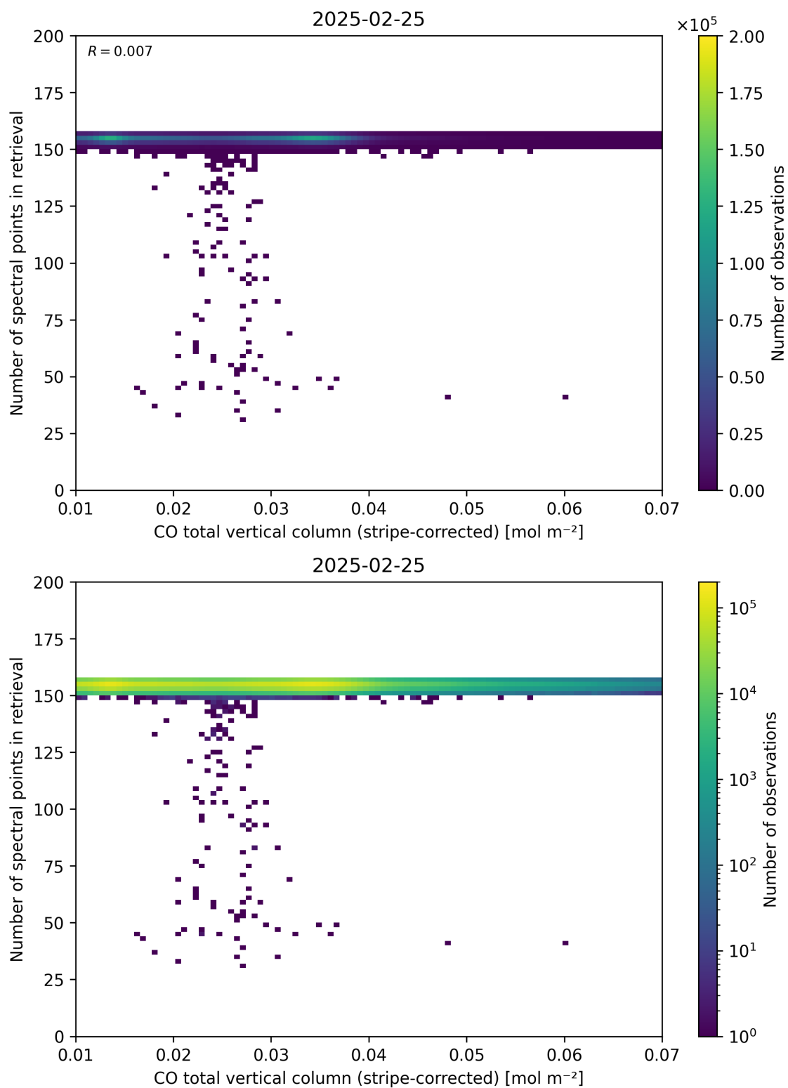
Figure 40: Scatter density plot of “CO total vertical column (stripe-corrected)” against “Number of spectral points in retrieval” for 2025-02-24 to 2025-02-26.
