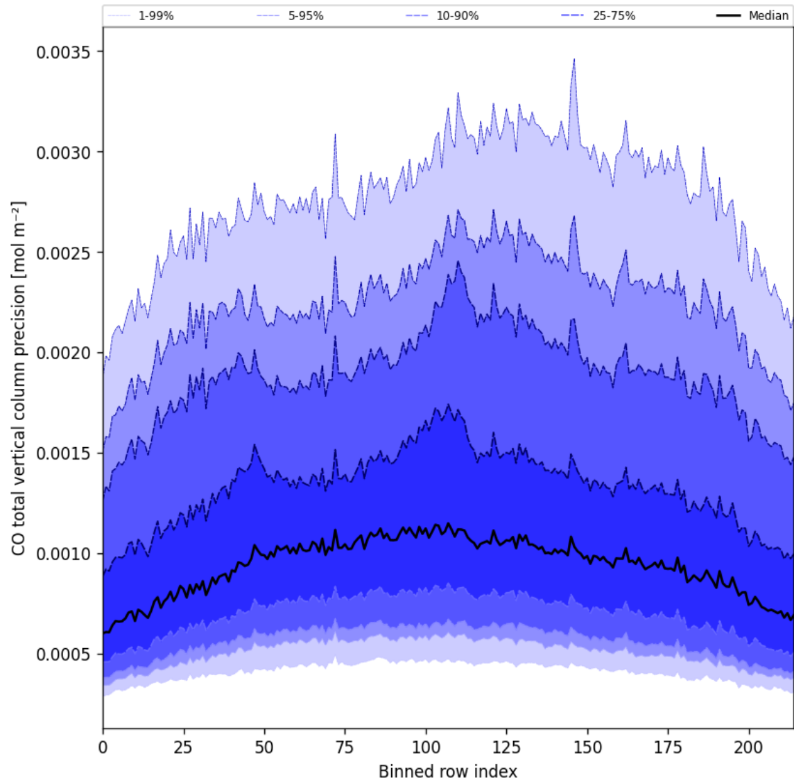
Figure 28: Along track statistics of “CO total vertical column precision” for 2025-02-24 to 2025-02-26
