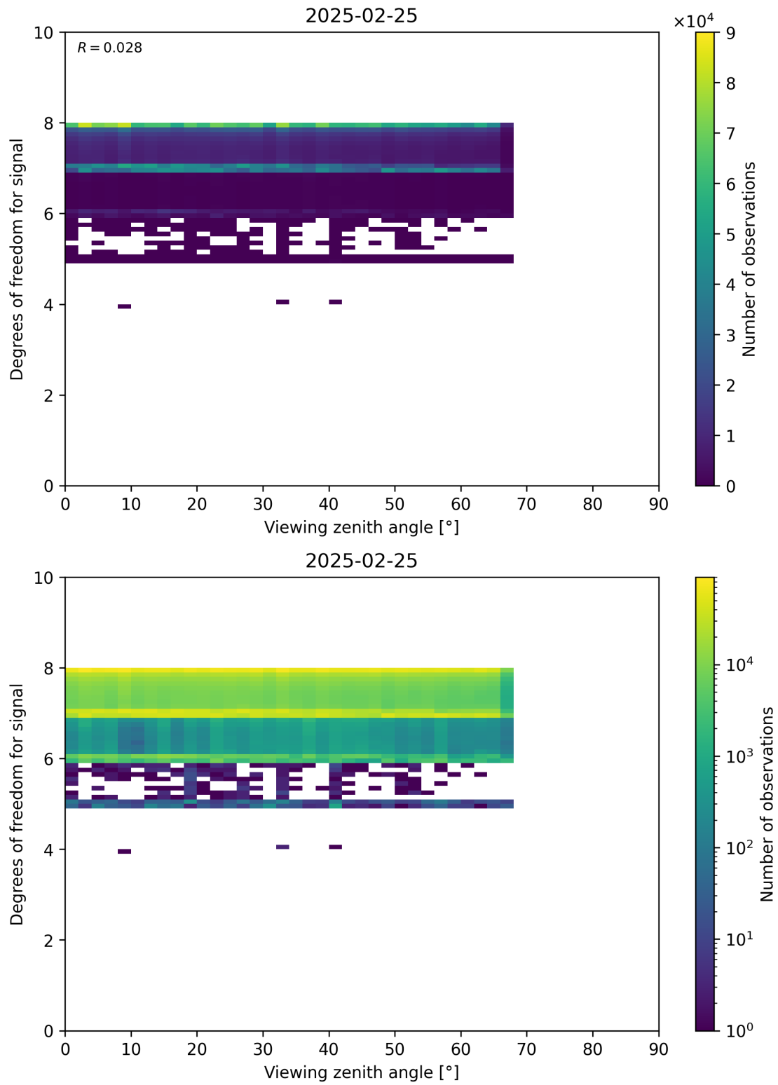
Figure 73: Scatter density plot of “Viewing zenith angle” against “Degrees of freedom for signal” for 2025-02-24 to 2025-02-26.
