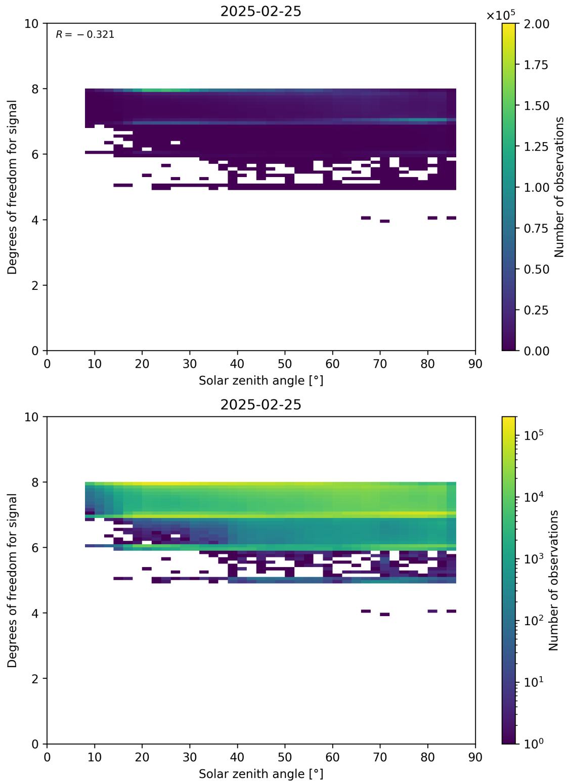
Figure 65: Scatter density plot of “Solar zenith angle” against “Degrees of freedom for signal” for 2025-02-24 to 2025-02-26.
