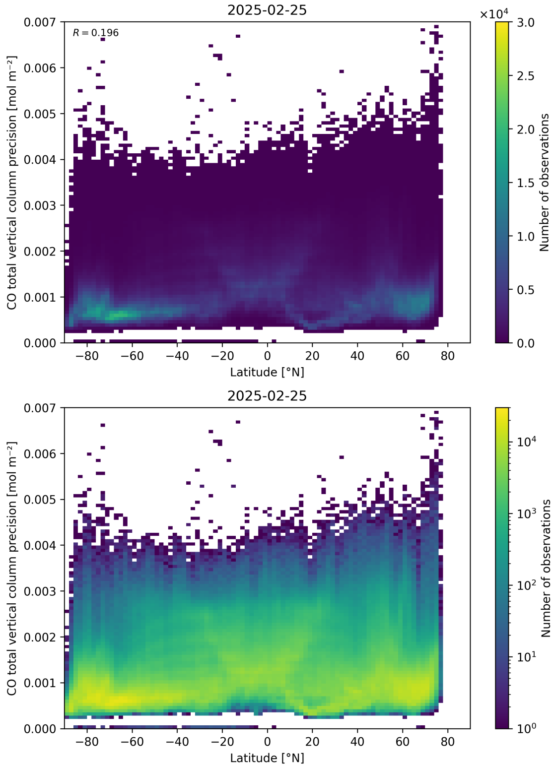
Figure 53: Scatter density plot of “Latitude” against “CO total vertical column precision” for 2025-02-24 to 2025-02-26.
