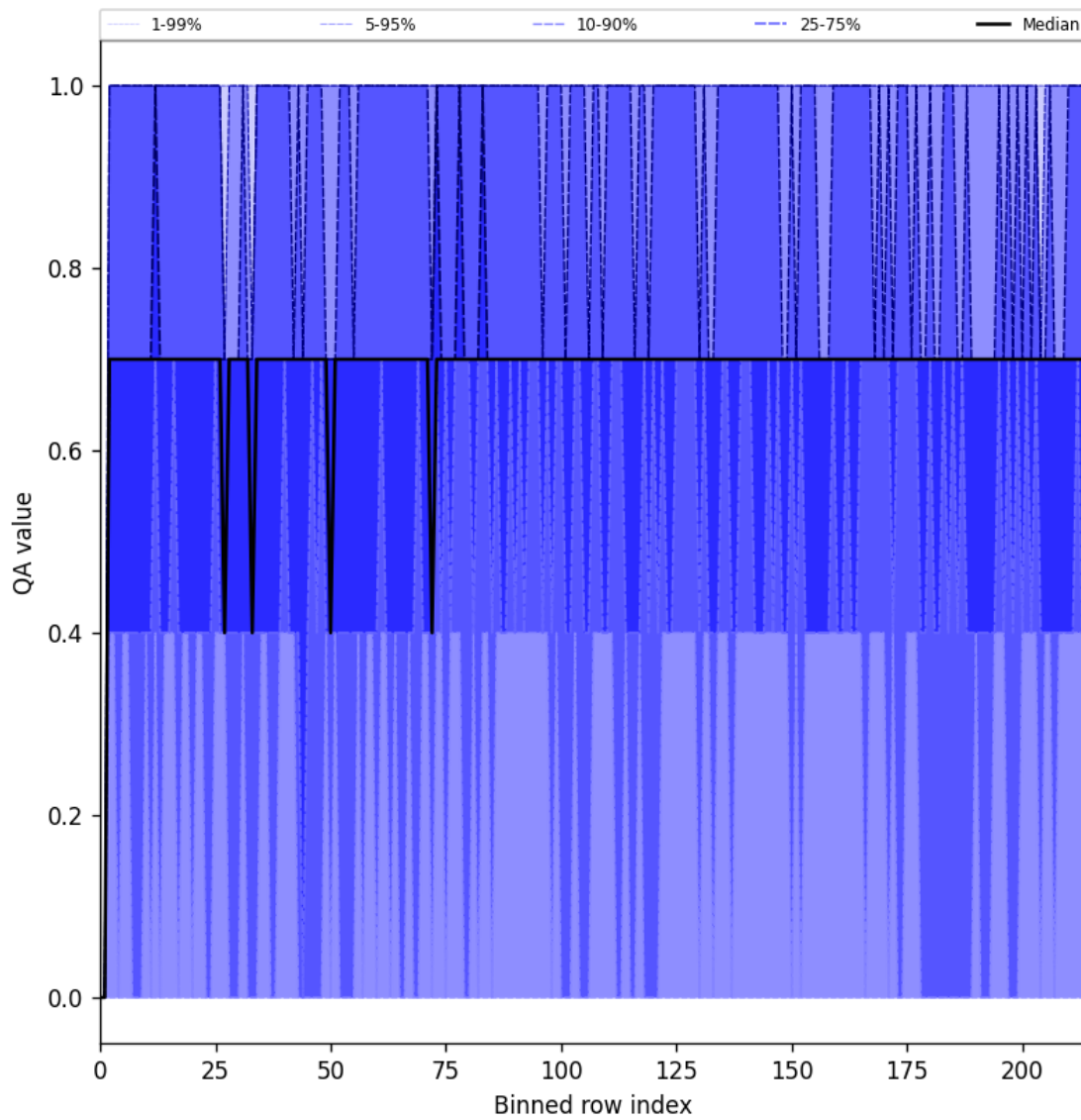
Figure 25: Along track statistics of “QA value” for 2025-02-24 to 2025-02-26
