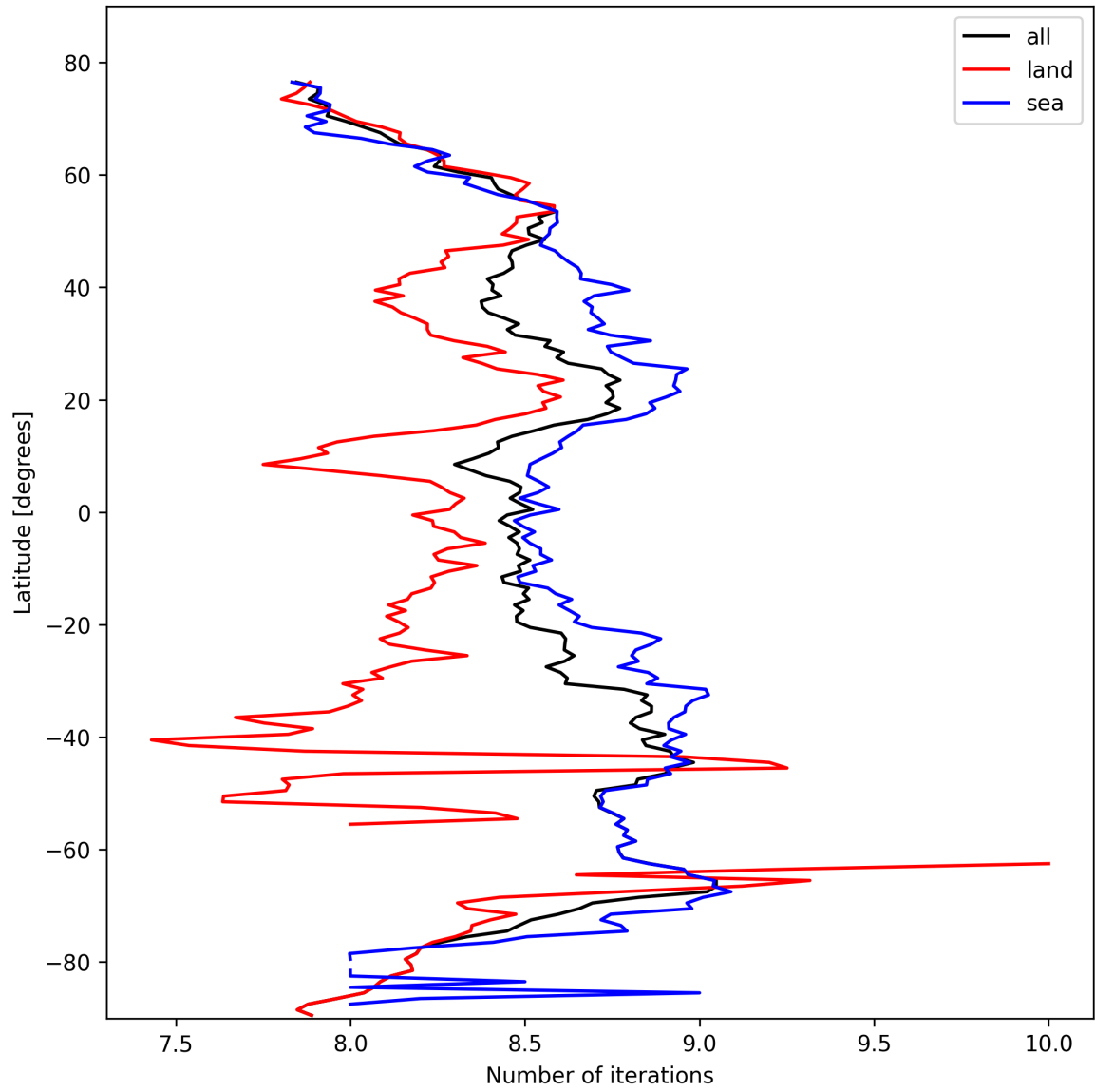
Figure 16: Zonal average of “Number of iterations” for 2025-02-24 to 2025-02-26.
