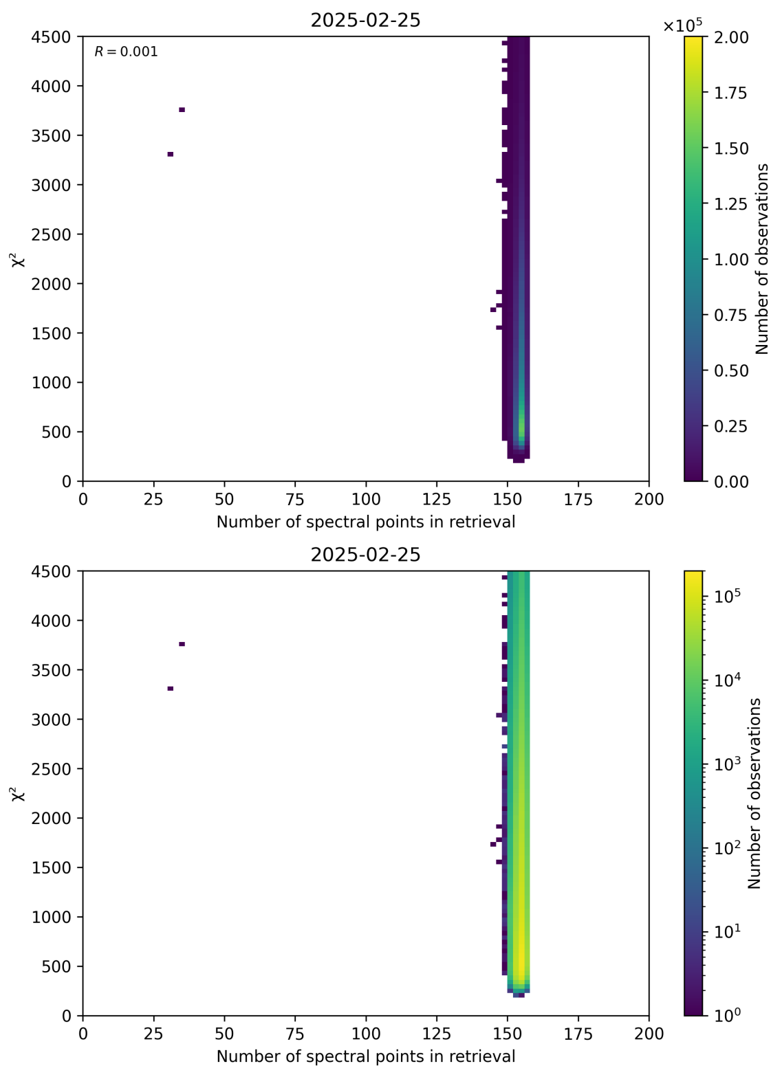
Figure 58: Scatter density plot of “Number of spectral points in retrieval” against “ \chi^2 ” for 2025-02-24 to 2025-02-26.
