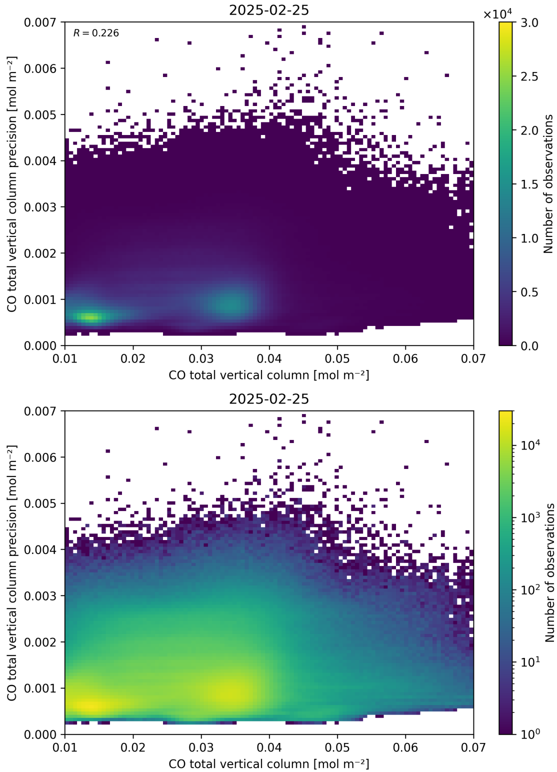
Figure 34: Scatter density plot of “CO total vertical column” against “CO total vertical column precision” for 2025-02-24 to 2025-02-26.
