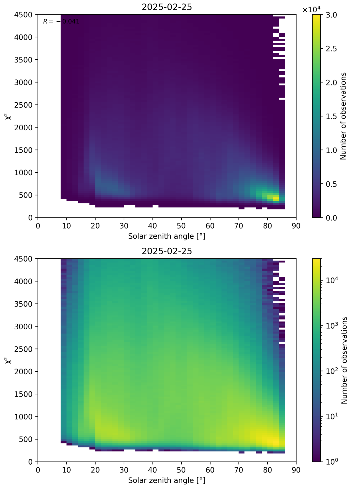
Figure 64: Scatter density plot of “Solar zenith angle” against “ \chi^2 ” for 2025-02-24 to 2025-02-26.
