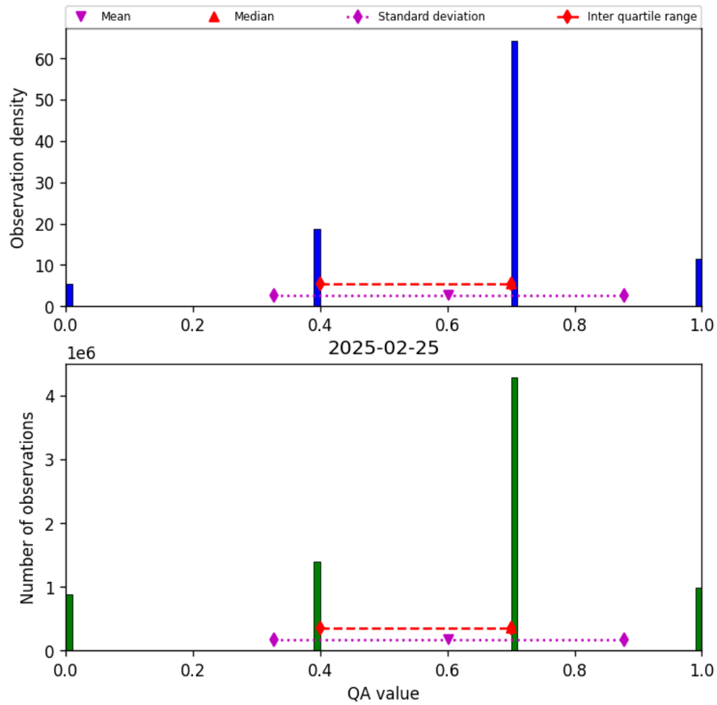
Figure 17: Histogram of “QA value” for 2025-02-24 to 2025-02-26
