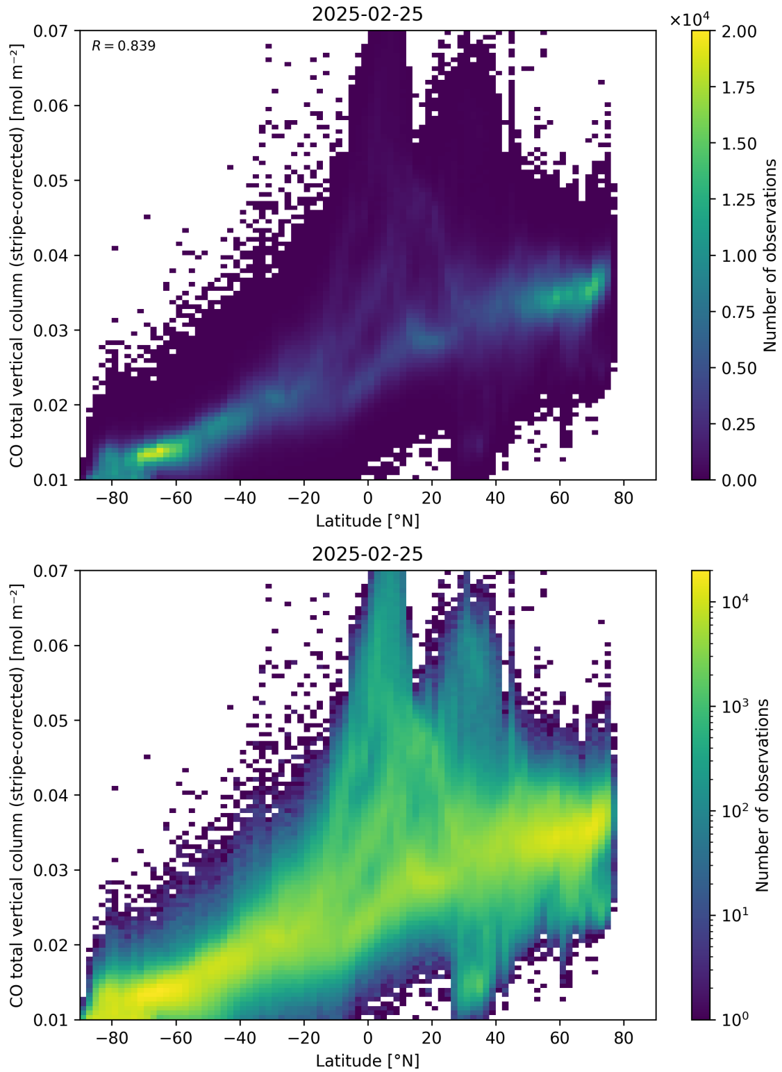
Figure 52: Scatter density plot of “Latitude” against “CO total vertical column (stripe-corrected)” for 2025-02-24 to 2025-02-26.
