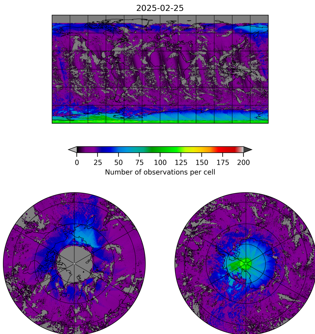
Figure 8: Map of the number of observations for 2025-02-24 to 2025-02-26
