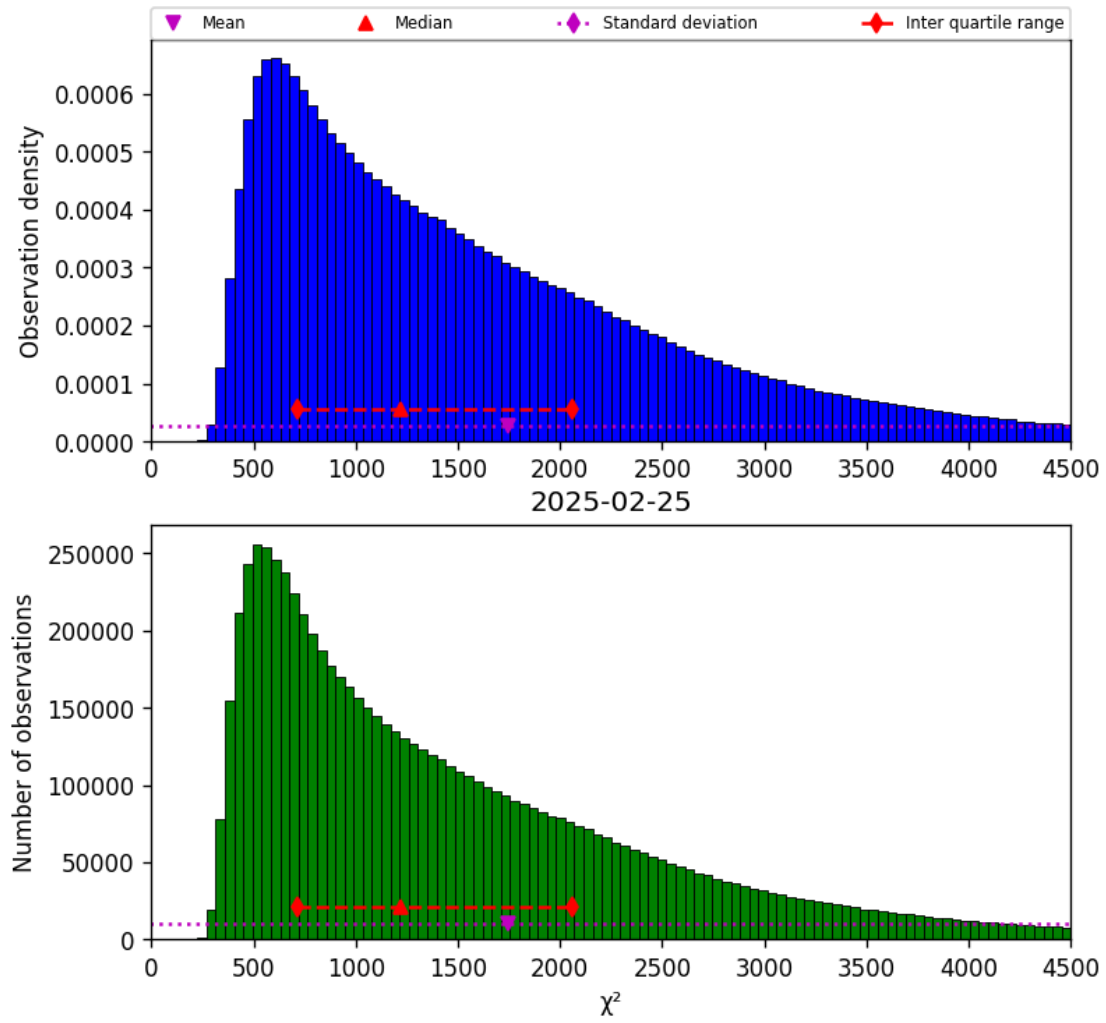
Figure 22: Histogram of “ \chi^2 ” for 2025-02-24 to 2025-02-26
