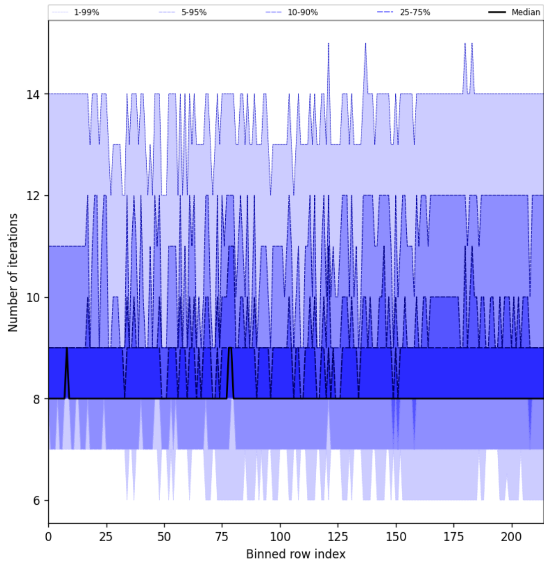
Figure 32: Along track statistics of “Number of iterations” for 2025-02-24 to 2025-02-26
