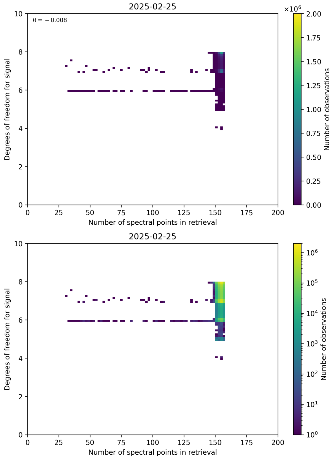
Figure 59: Scatter density plot of “Number of spectral points in retrieval” against “Degrees of freedom for signal” for 2025-02-24 to 2025-02-26.
