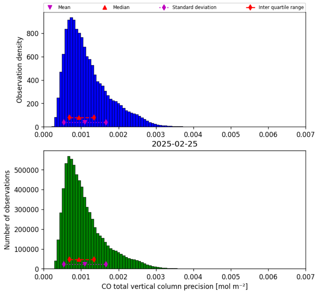
Figure 20: Histogram of “CO total vertical column precision” for 2025-02-24 to 2025-02-26
