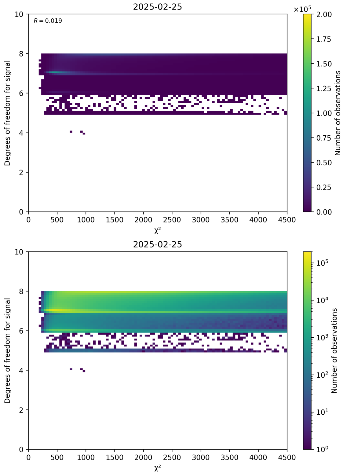
Figure 48: Scatter density plot of “ \chi^2 ” against “Degrees of freedom for signal” for 2025-02-24 to 2025-02-26.
