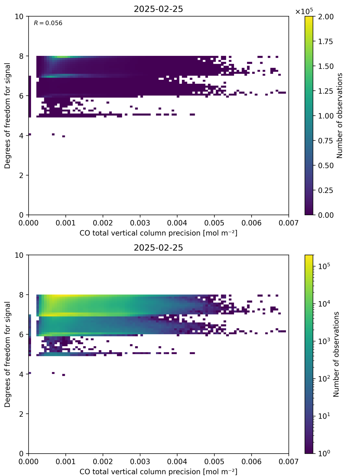
Figure 45: Scatter density plot of “CO total vertical column precision” against “Degrees of freedom for signal” for 2025-02-24 to 2025-02-26.
