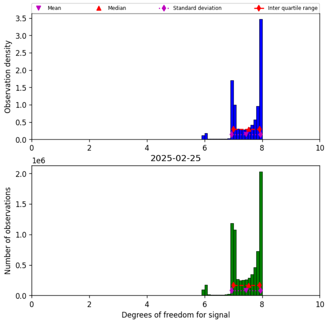
Figure 23: Histogram of “Degrees of freedom for signal” for 2025-02-24 to 2025-02-26
