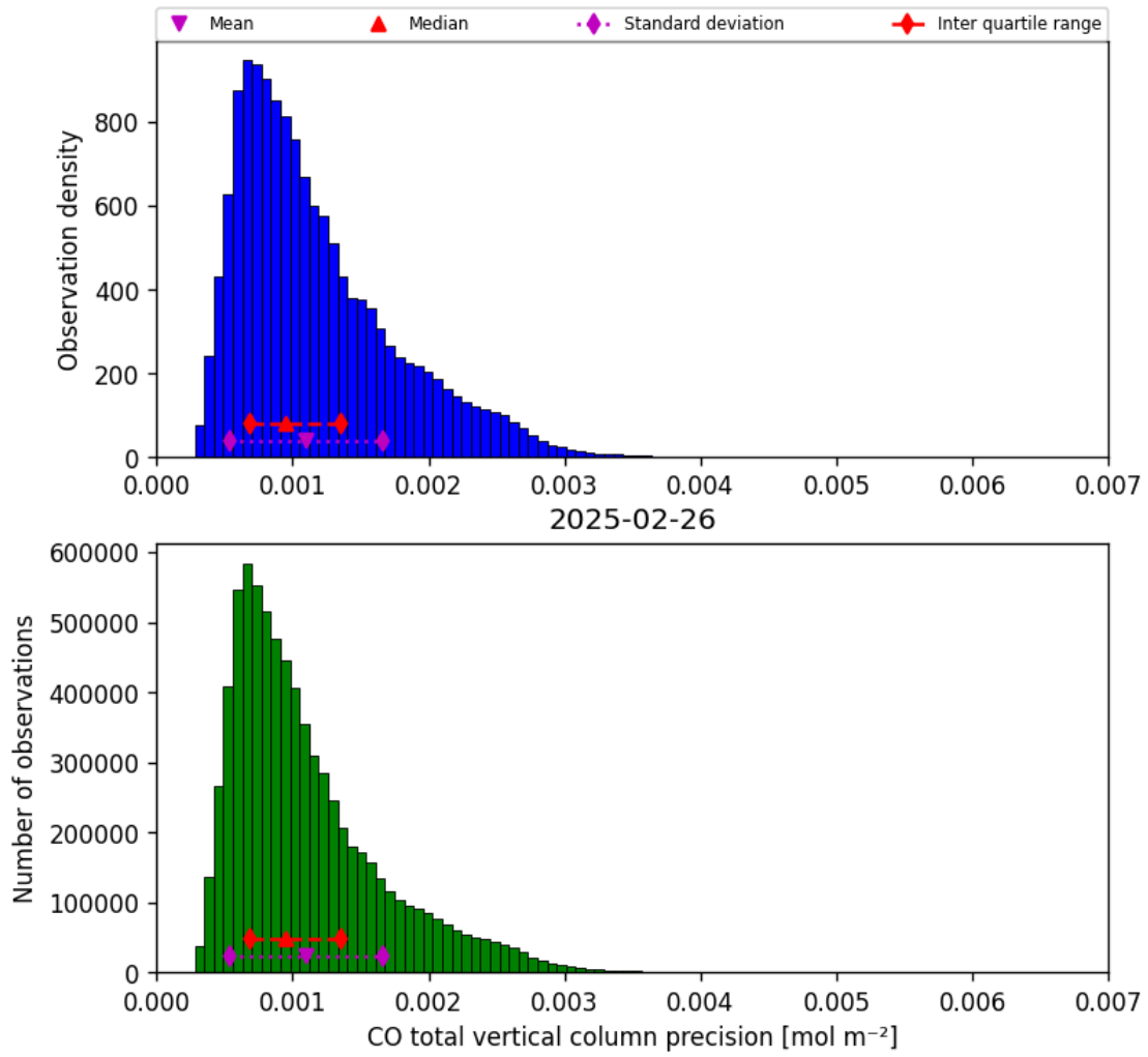
Figure 20: Histogram of “CO total vertical column precision” for 2025-02-25 to 2025-02-27
