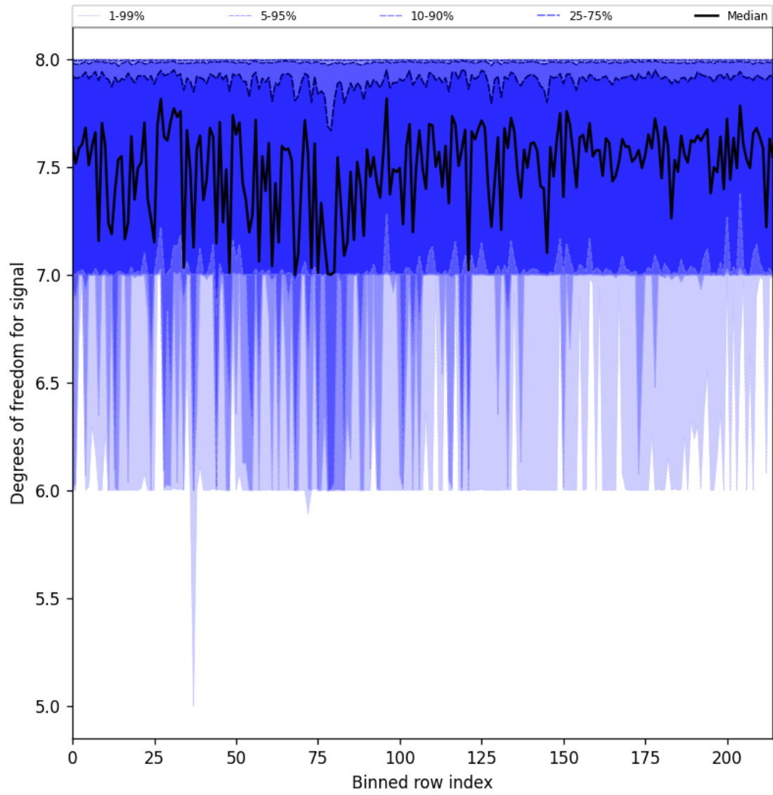
Figure 31: Along track statistics of “Degrees of freedom for signal” for 2025-02-25 to 2025-02-27
