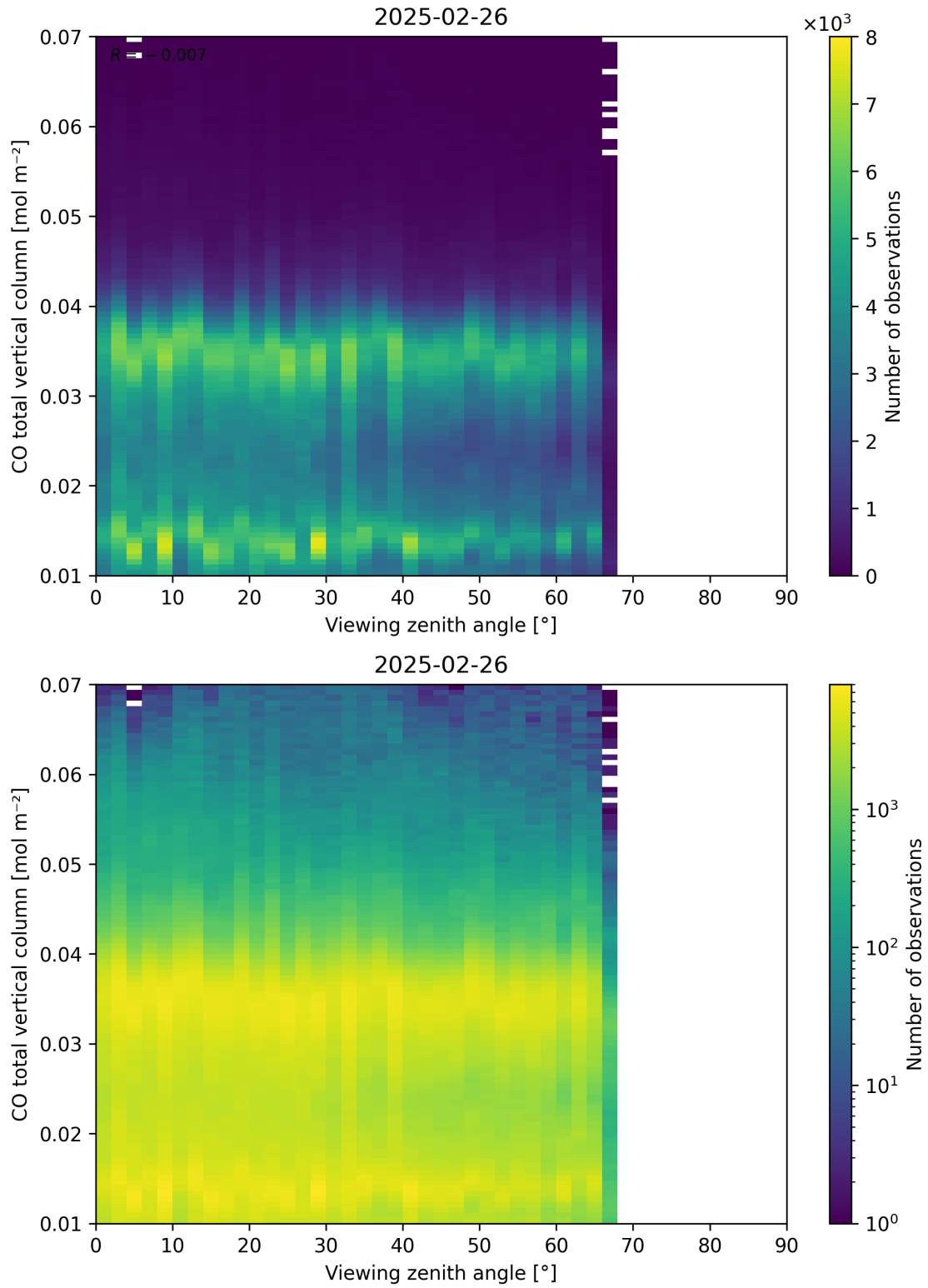
Figure 69: Scatter density plot of “Viewing zenith angle” against “CO total vertical column” for 2025-02-25 to 2025-02-27.
