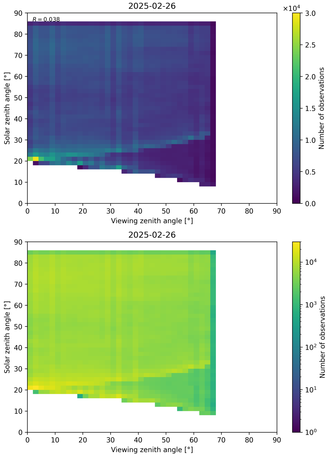
Figure 77: Scatter density plot of “Viewing zenith angle” against “Solar zenith angle” for 2025-02-25 to 2025-02-27.
