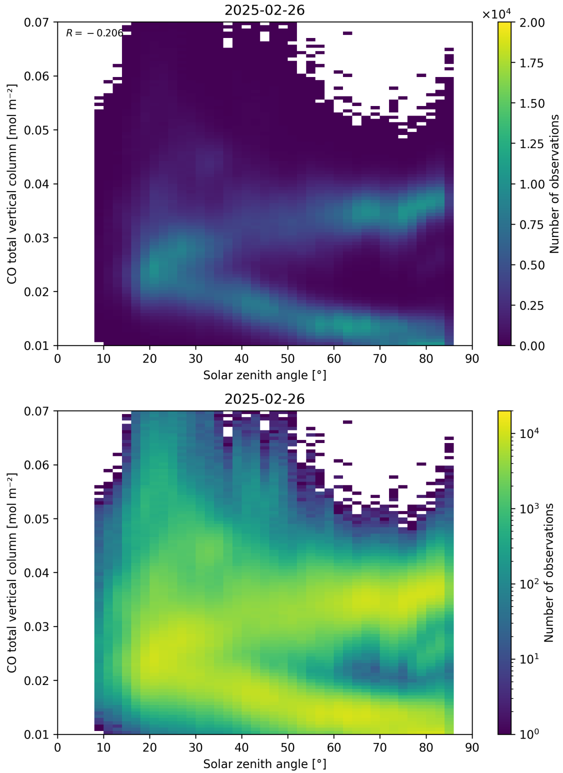
Figure 61: Scatter density plot of “Solar zenith angle” against “CO total vertical column” for 2025-02-25 to 2025-02-27.
