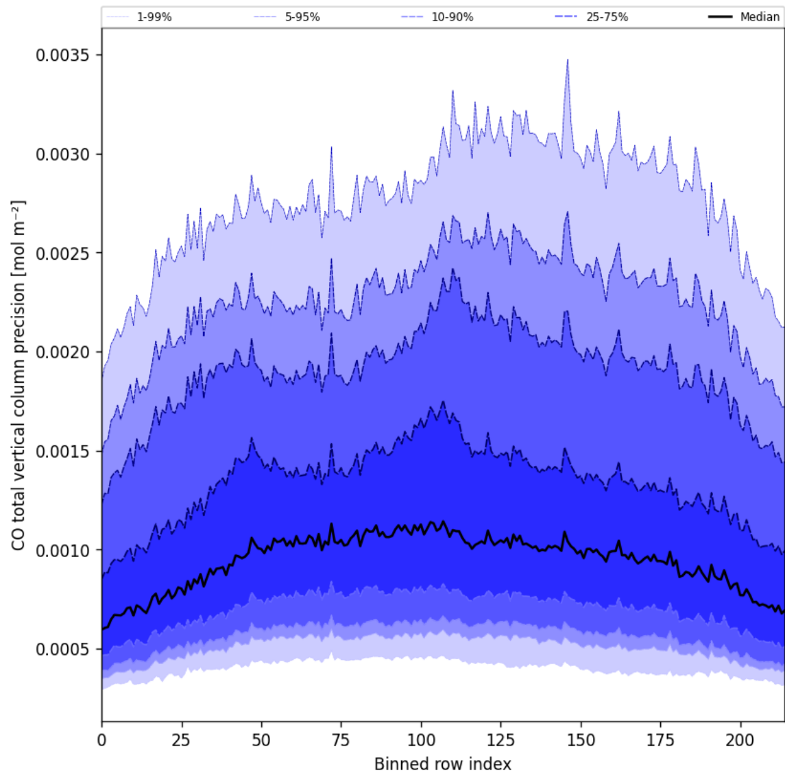
Figure 28: Along track statistics of “CO total vertical column precision” for 2025-02-25 to 2025-02-27
