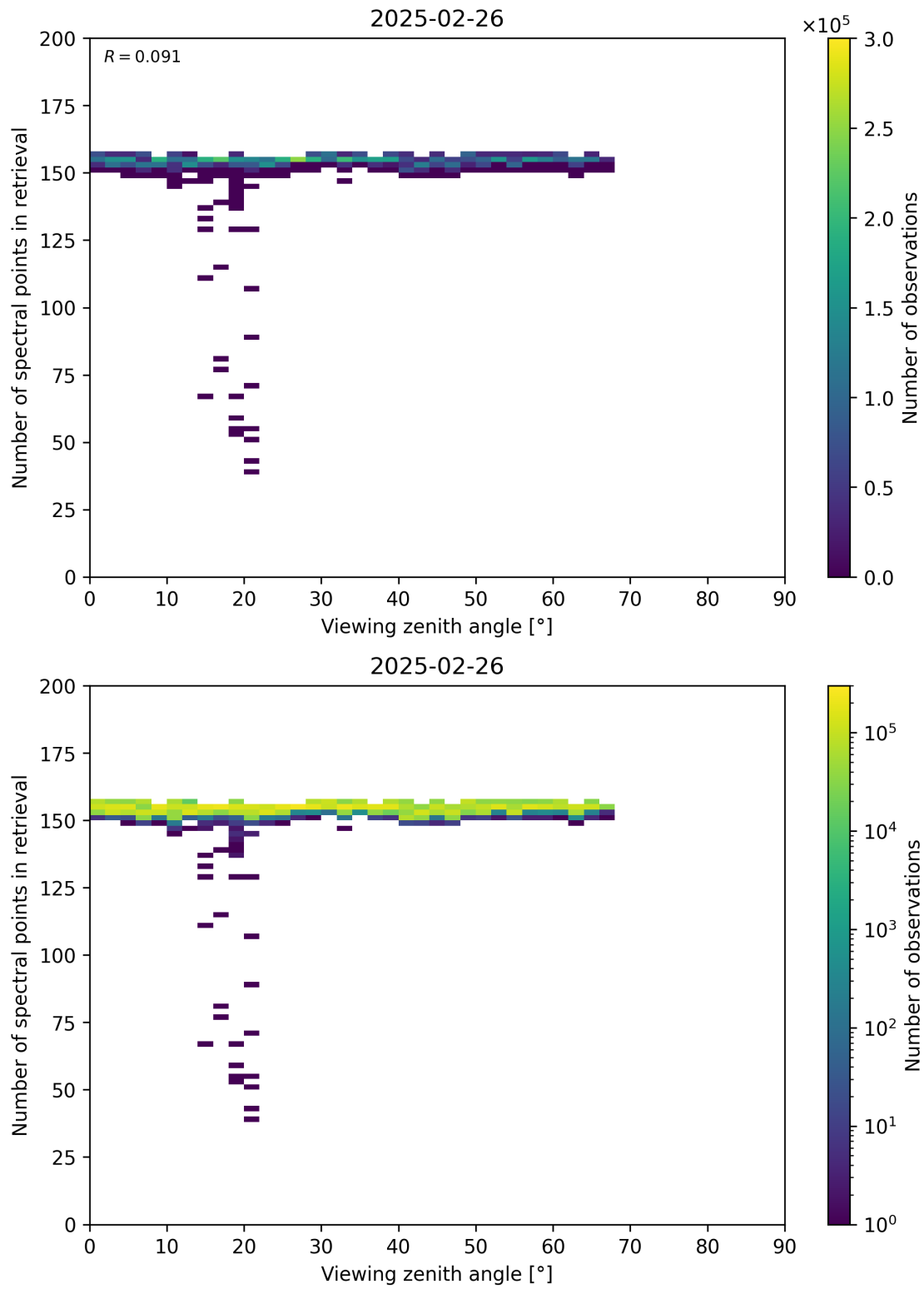
Figure 76: Scatter density plot of “Viewing zenith angle” against “Number of spectral points in retrieval” for 2025-02-25 to 2025-02-27.
