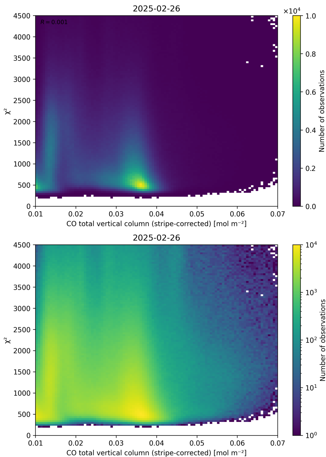
Figure 37: Scatter density plot of “CO total vertical column (stripe-corrected)” against “ \chi^2 ” for 2025-02-25 to 2025-02-27.
