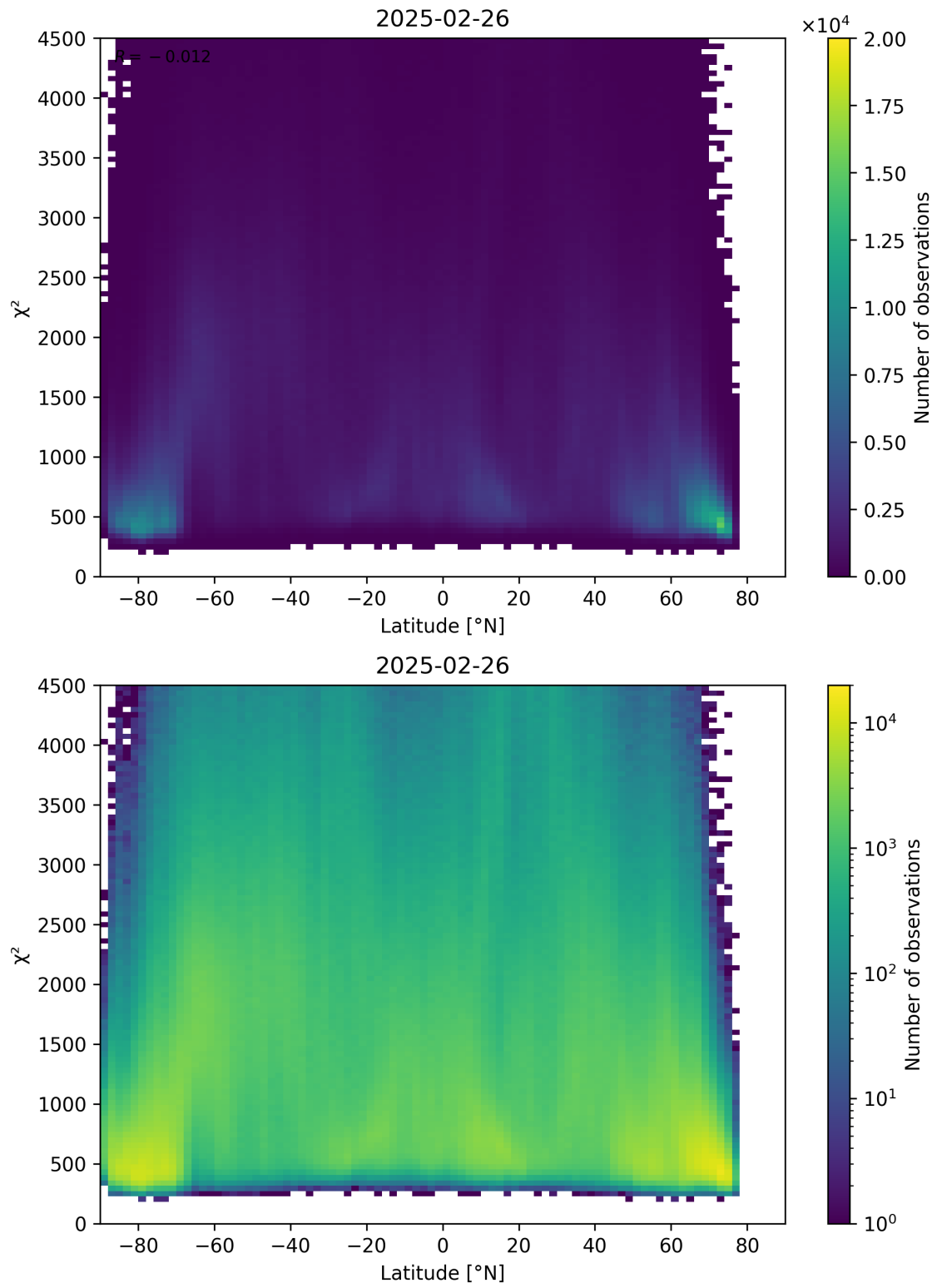
Figure 54: Scatter density plot of “Latitude” against “ \chi^2 ” for 2025-02-25 to 2025-02-27.
