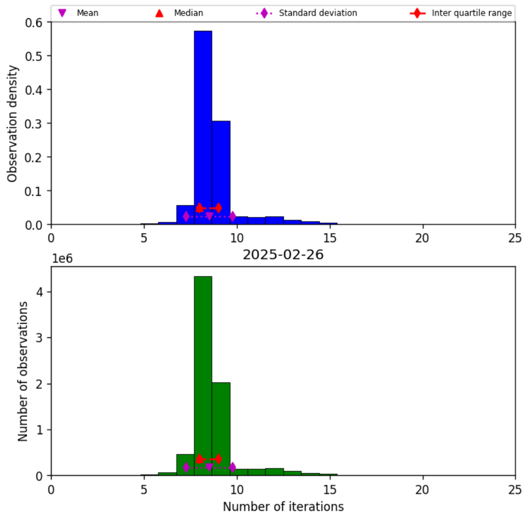
Figure 24: Histogram of “Number of iterations” for 2025-02-25 to 2025-02-27
