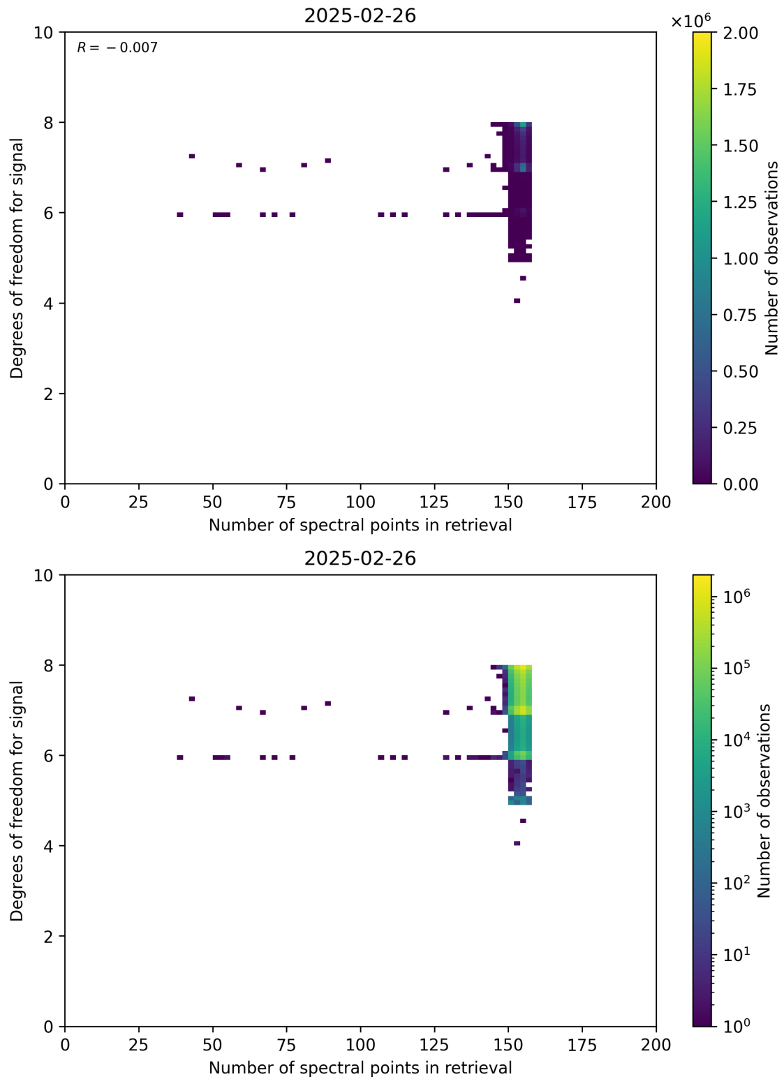
Figure 59: Scatter density plot of “Number of spectral points in retrieval” against “Degrees of freedom for signal” for 2025-02-25 to 2025-02-27.
