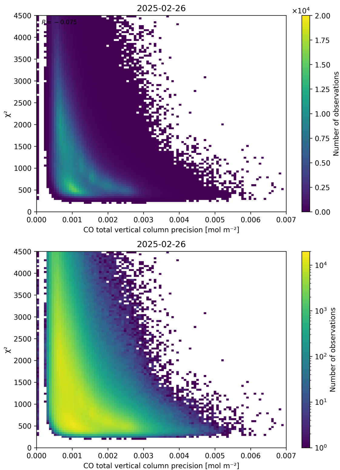
Figure 44: Scatter density plot of “CO total vertical column precision” against “ \chi^2 ” for 2025-02-25 to 2025-02-27.
