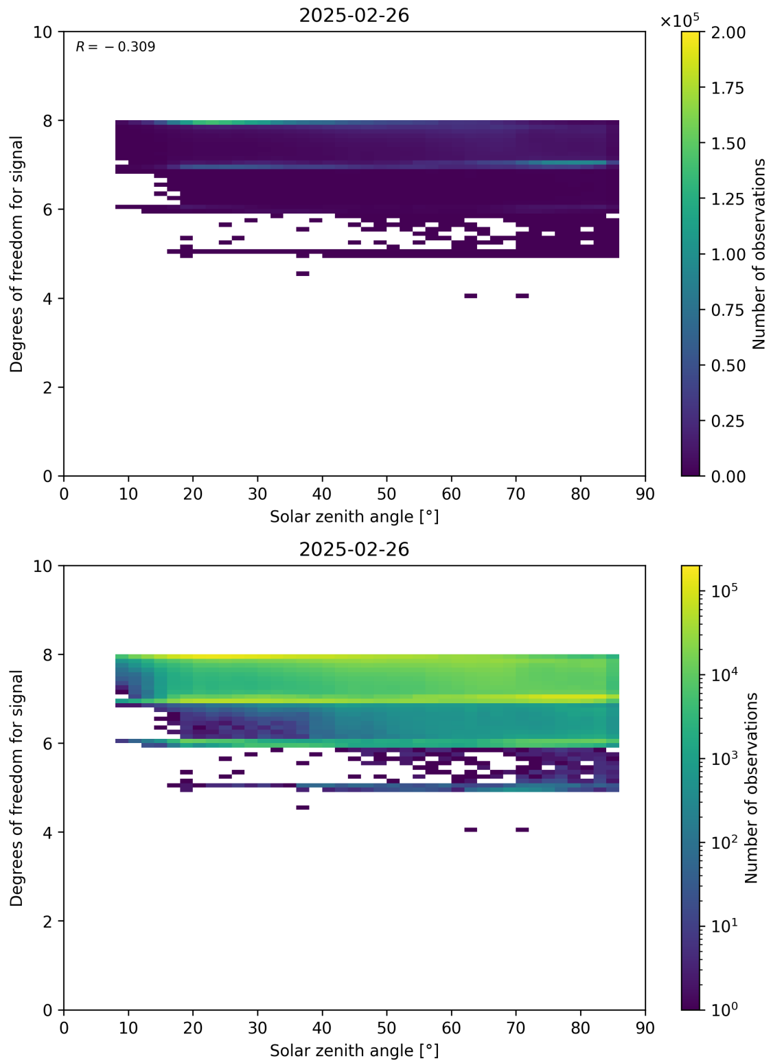
Figure 65: Scatter density plot of “Solar zenith angle” against “Degrees of freedom for signal” for 2025-02-25 to 2025-02-27.
