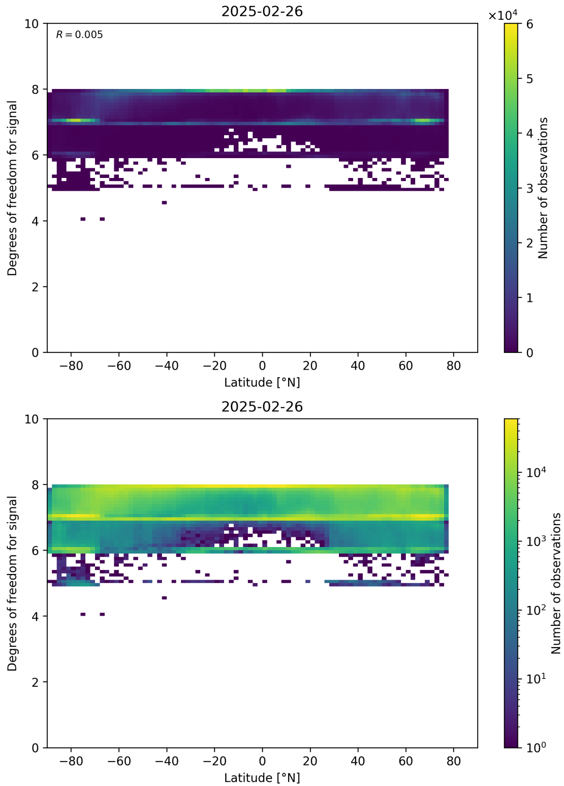
Figure 55: Scatter density plot of “Latitude” against “Degrees of freedom for signal” for 2025-02-25 to 2025-02-27.
