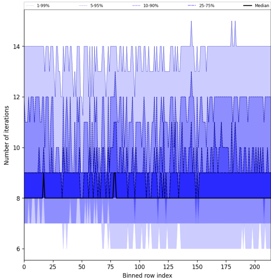
Figure 32: Along track statistics of “Number of iterations” for 2025-02-25 to 2025-02-27
