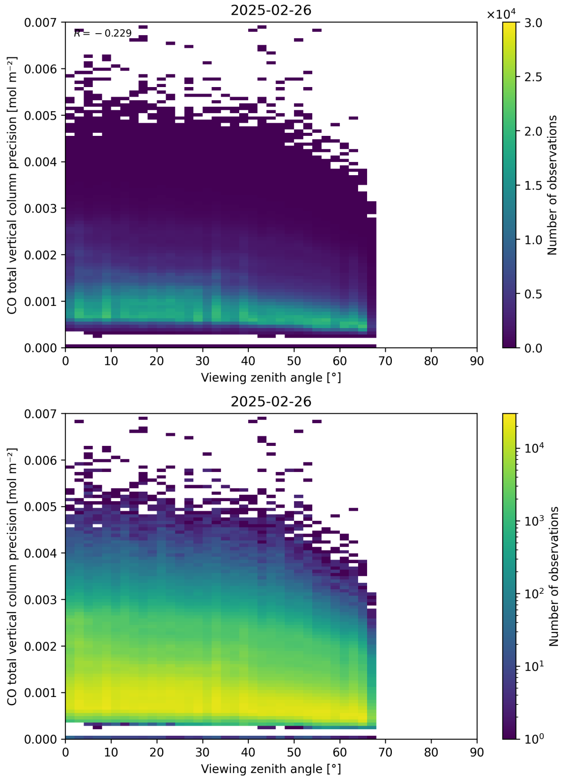
Figure 71: Scatter density plot of “Viewing zenith angle” against “CO total vertical column precision” for 2025-02-25 to 2025-02-27.
