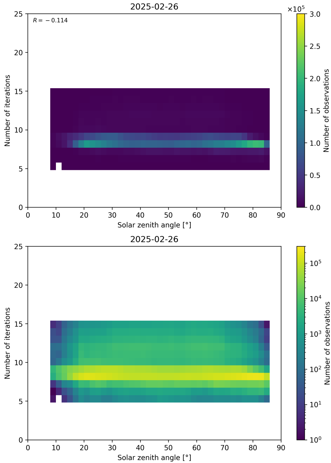
Figure 67: Scatter density plot of “Solar zenith angle” against “Number of iterations” for 2025-02-25 to 2025-02-27.
