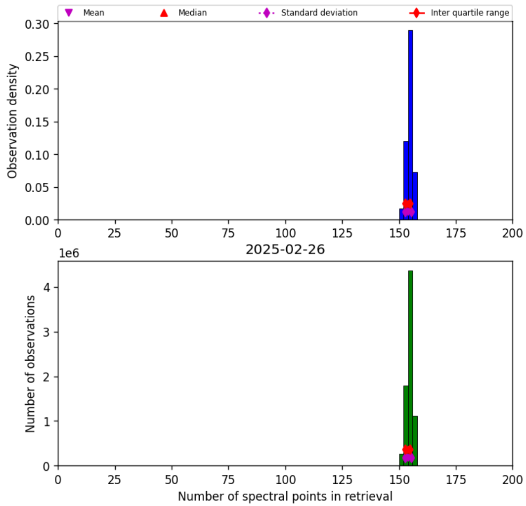
Figure 21: Histogram of “Number of spectral points in retrieval” for 2025-02-25 to 2025-02-27
