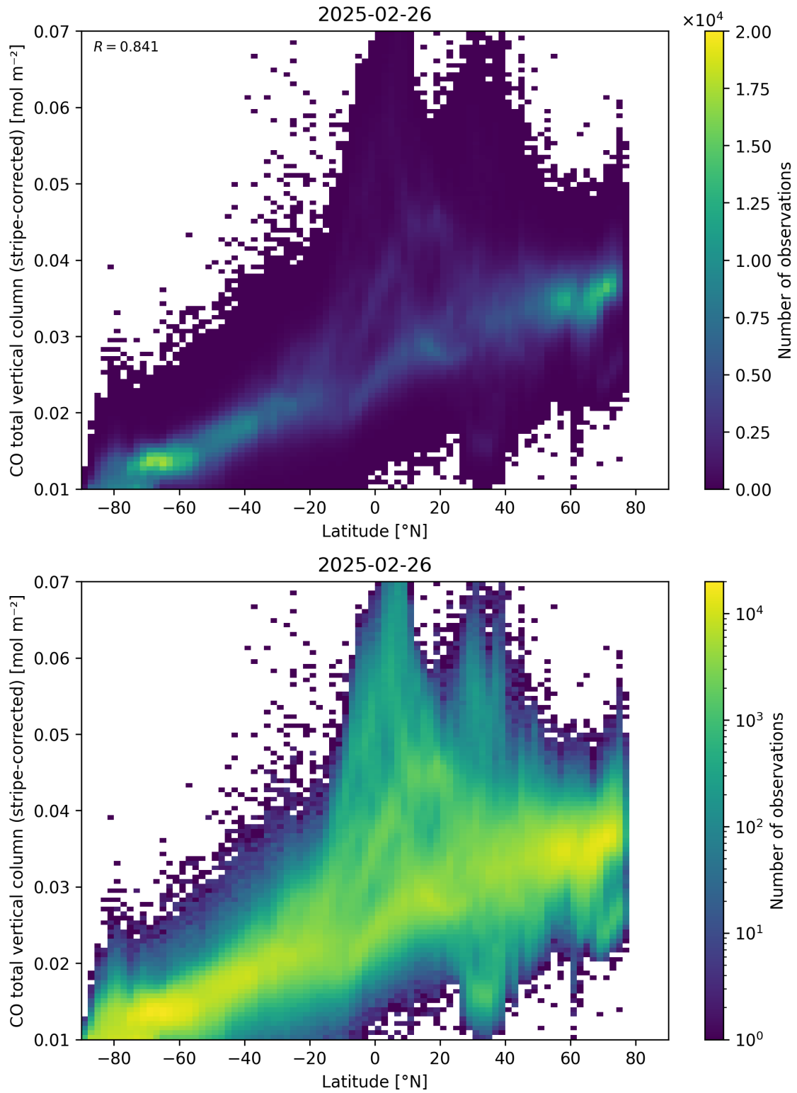
Figure 52: Scatter density plot of “Latitude” against “CO total vertical column (stripe-corrected)” for 2025-02-25 to 2025-02-27.
