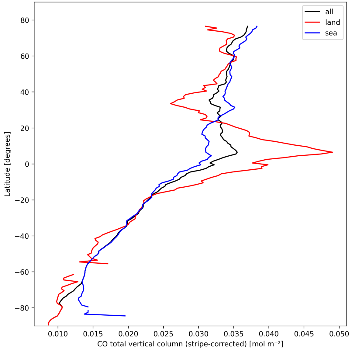
Figure 11: Zonal average of “CO total vertical column (stripe-corrected)” for 2025-02-25 to 2025-02-27.
