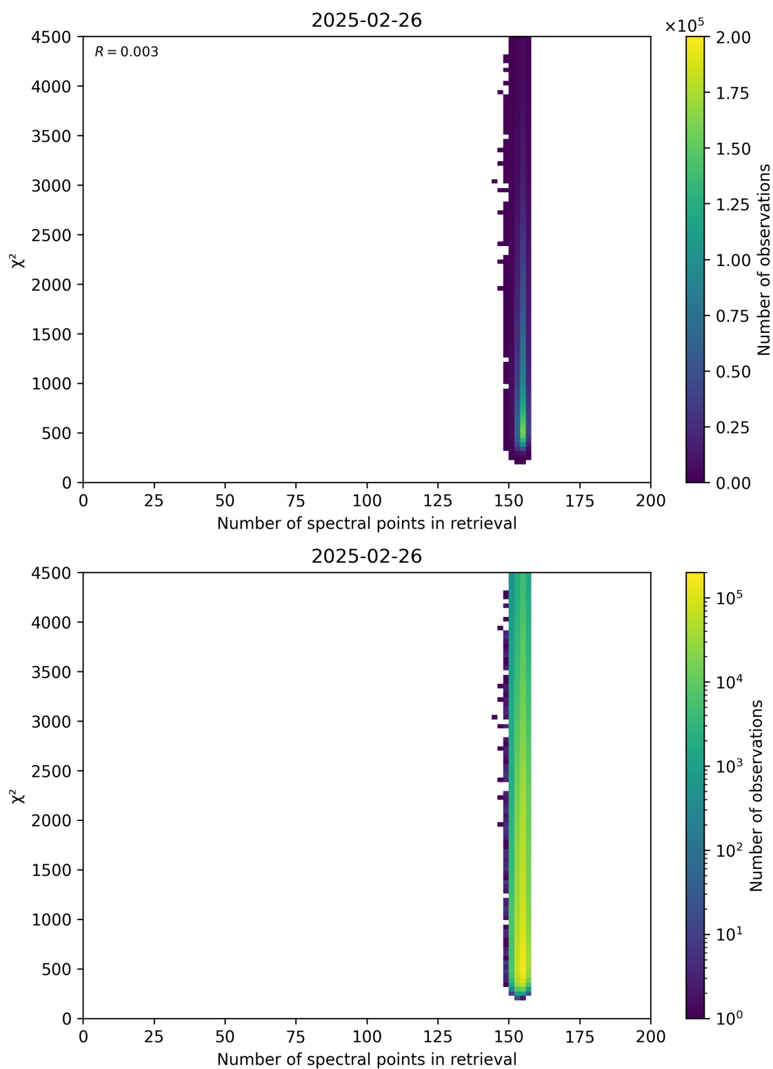
Figure 58: Scatter density plot of “Number of spectral points in retrieval” against “ \chi^2 ” for 2025-02-25 to 2025-02-27.
