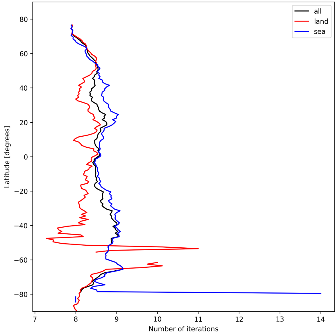
Figure 16: Zonal average of “Number of iterations” for 2025-02-25 to 2025-02-27.
