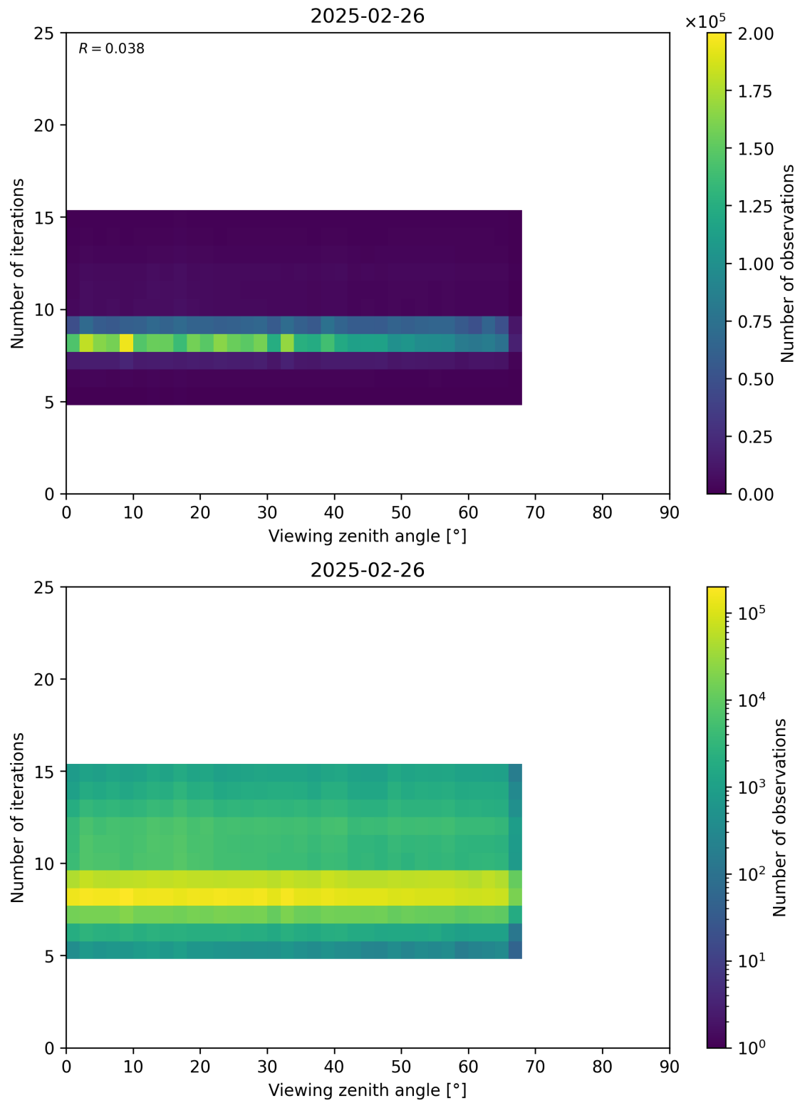
Figure 75: Scatter density plot of “Viewing zenith angle” against “Number of iterations” for 2025-02-25 to 2025-02-27.
