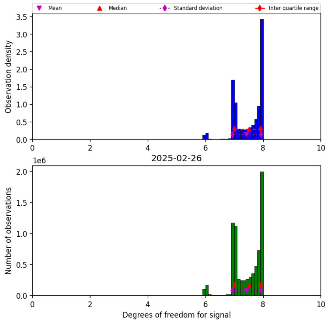
Figure 23: Histogram of “Degrees of freedom for signal” for 2025-02-25 to 2025-02-27
