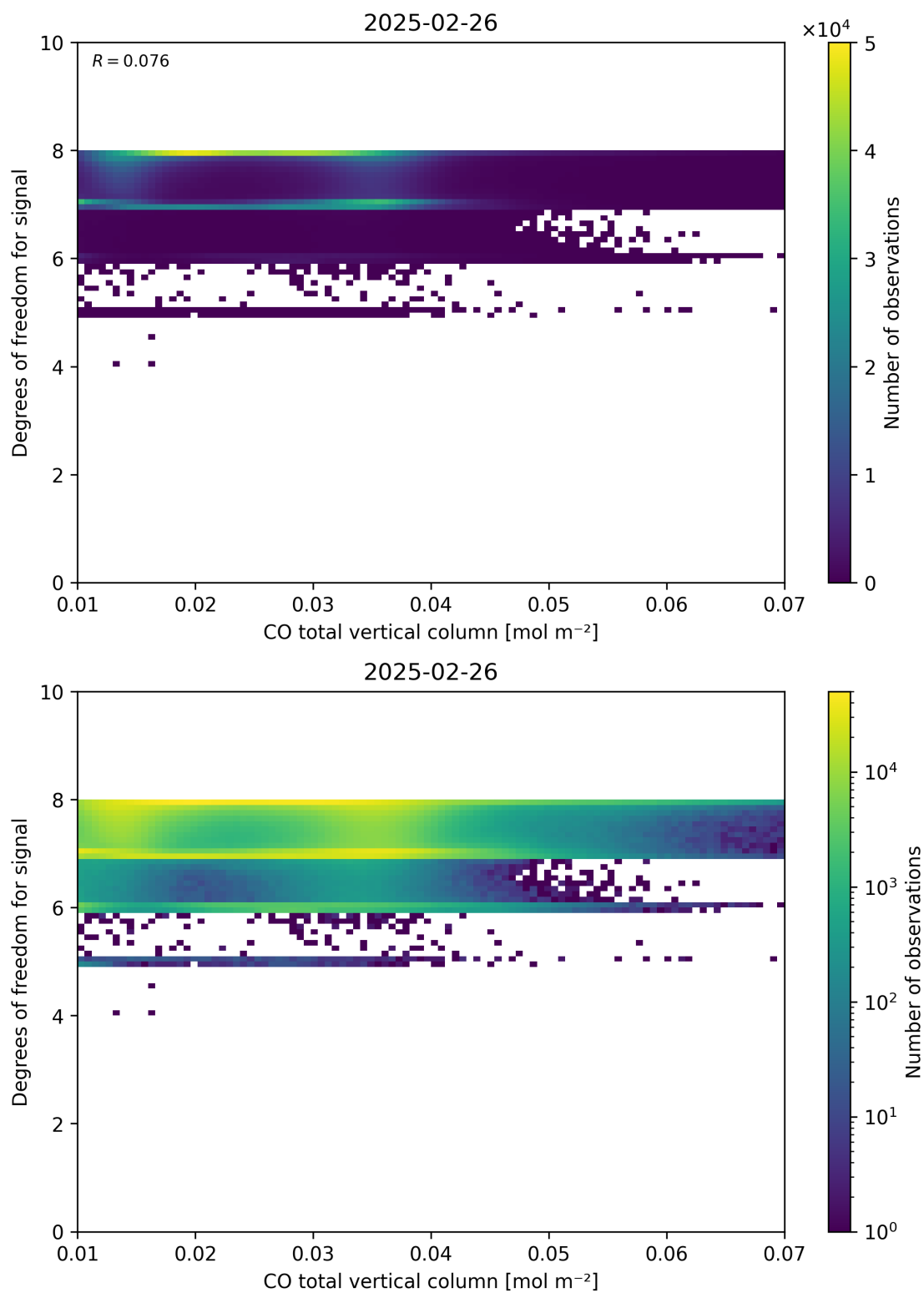
Figure 41: Scatter density plot of “CO total vertical column” against “Degrees of freedom for signal” for 2025-02-25 to 2025-02-27.
