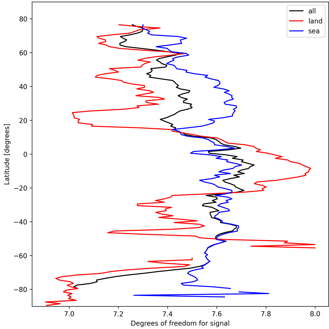
Figure 15: Zonal average of “Degrees of freedom for signal” for 2025-02-25 to 2025-02-27.
