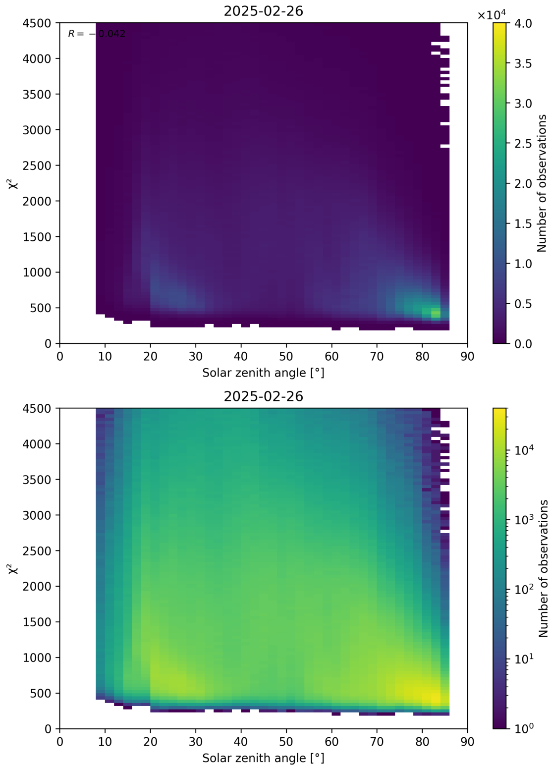
Figure 64: Scatter density plot of “Solar zenith angle” against “ \chi^2 ” for 2025-02-25 to 2025-02-27.
