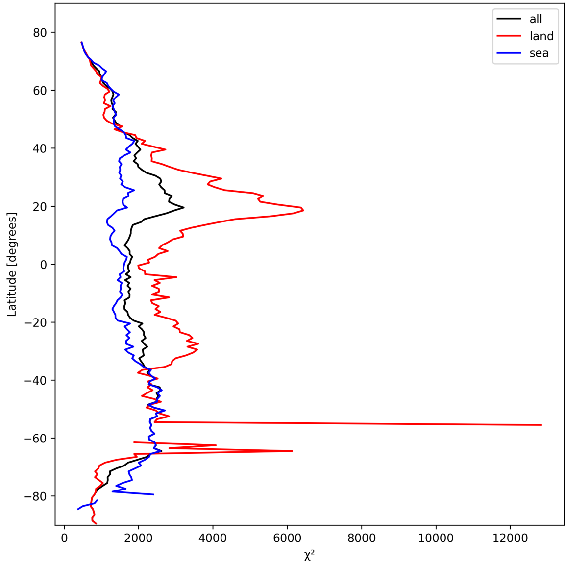
Figure 14: Zonal average of “ \chi^2 ” for 2025-02-25 to 2025-02-27.
