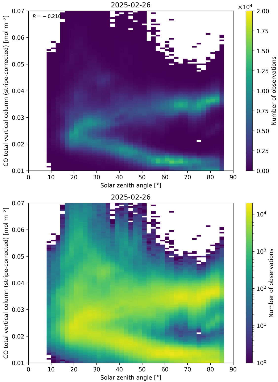
Figure 62: Scatter density plot of “Solar zenith angle” against “CO total vertical column (stripe-corrected)” for 2025-02-25 to 2025-02-27.
