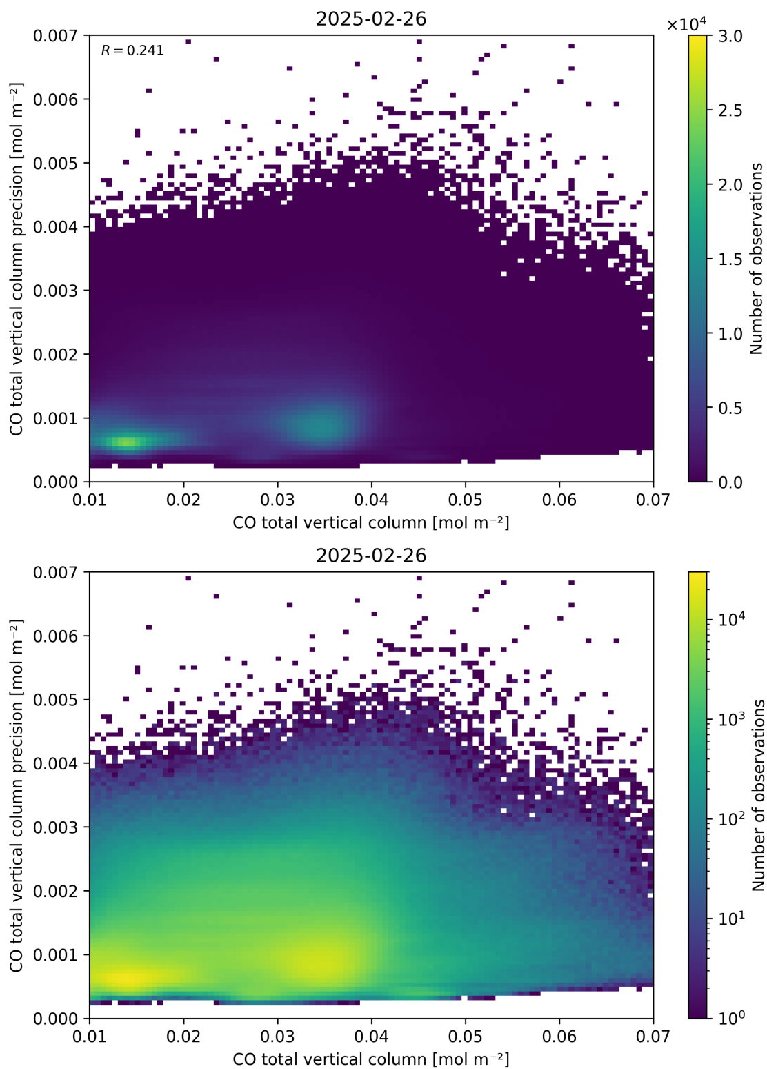
Figure 34: Scatter density plot of “CO total vertical column” against “CO total vertical column precision” for 2025-02-25 to 2025-02-27.
