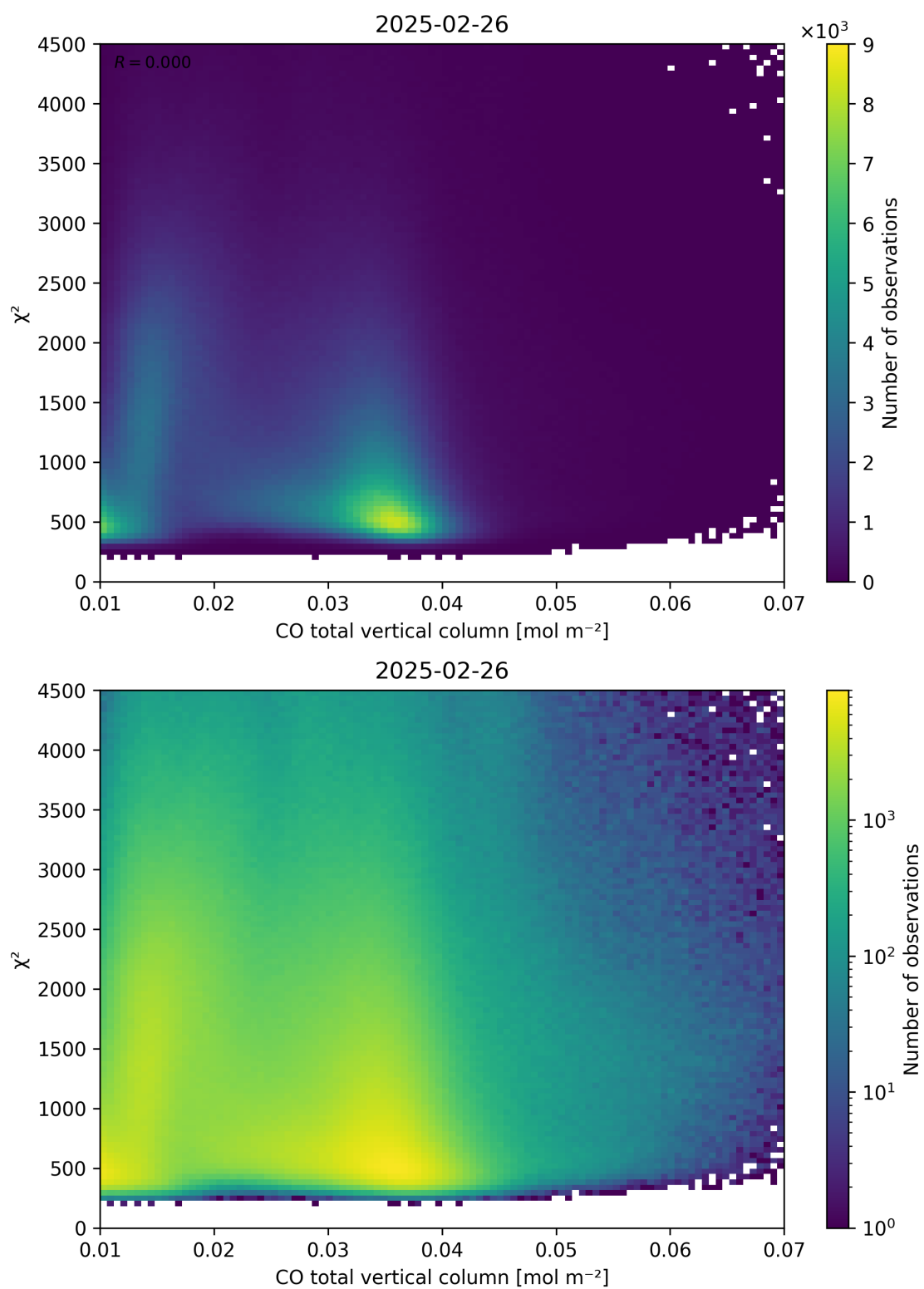
Figure 35: Scatter density plot of “CO total vertical column” against “ \chi^2 ” for 2025-02-25 to 2025-02-27.
