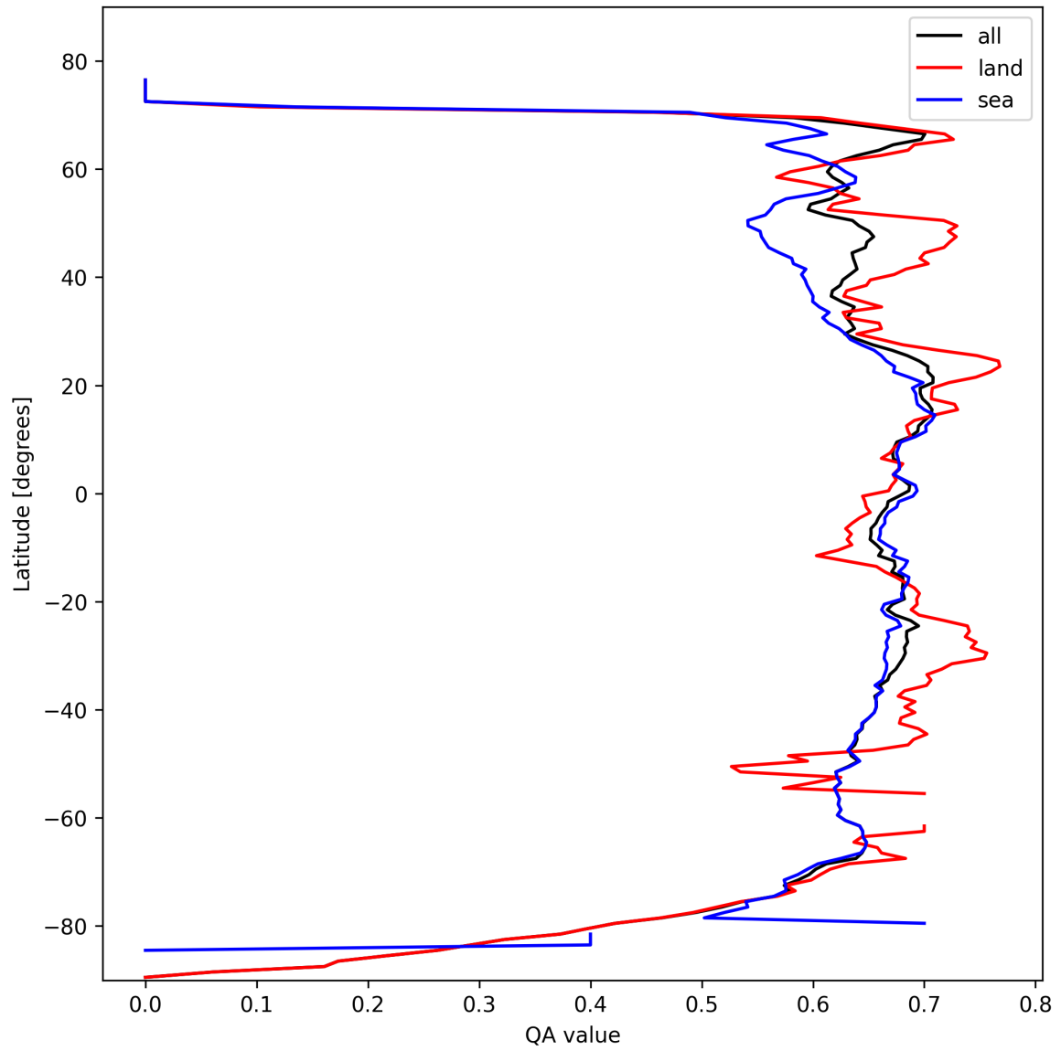
Figure 9: Zonal average of “QA value” for 2025-02-25 to 2025-02-27.
