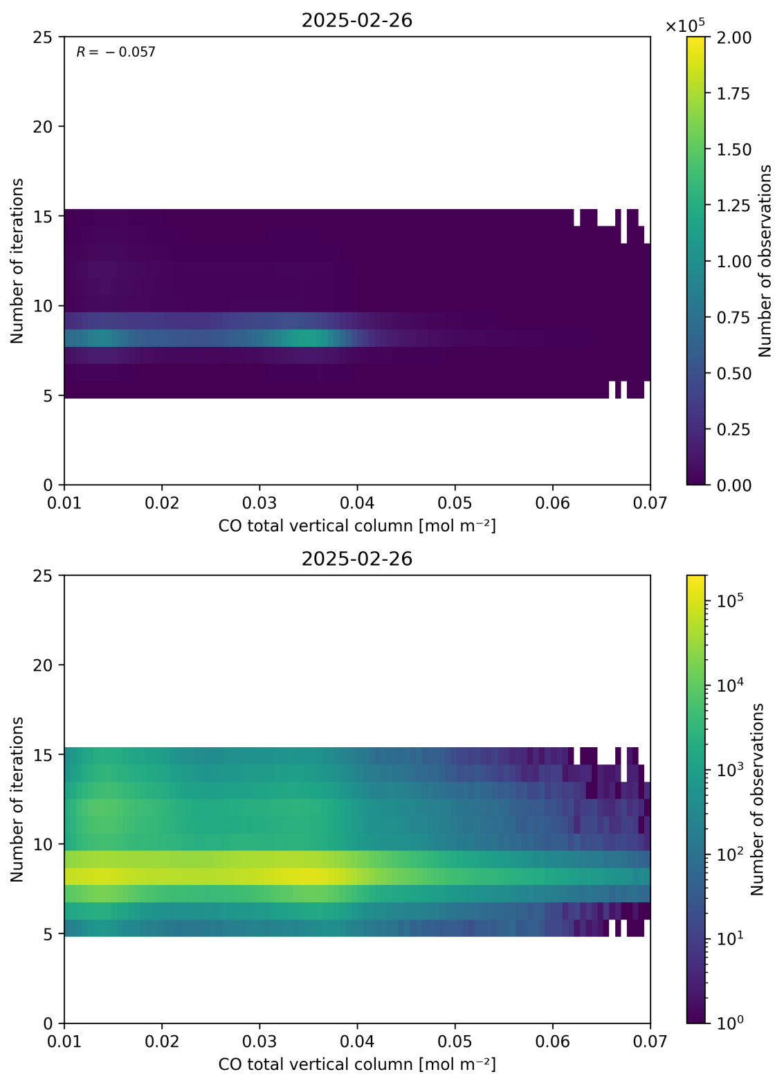
Figure 42: Scatter density plot of “CO total vertical column” against “Number of iterations” for 2025-02-25 to 2025-02-27.
