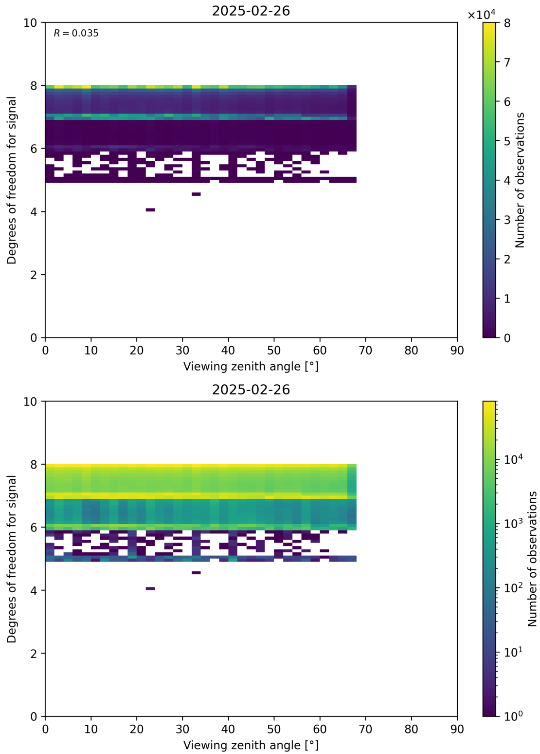
Figure 73: Scatter density plot of “Viewing zenith angle” against “Degrees of freedom for signal” for 2025-02-25 to 2025-02-27.
