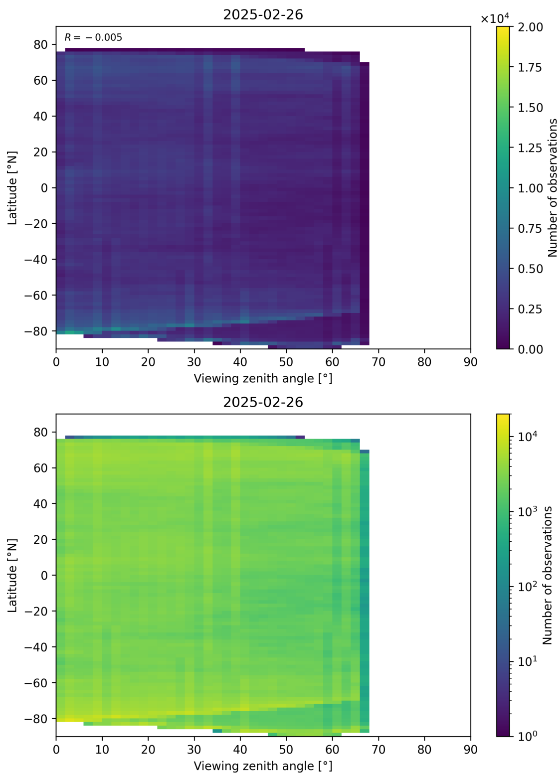
Figure 74: Scatter density plot of “Viewing zenith angle” against “Latitude” for 2025-02-25 to 2025-02-27.
