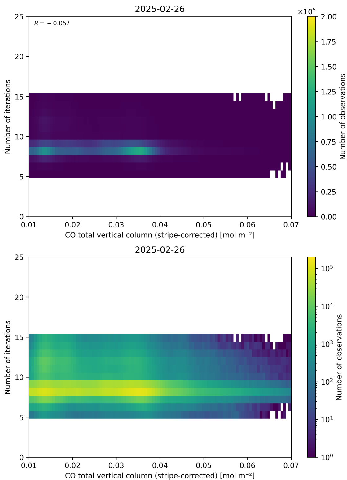
Figure 39: Scatter density plot of “CO total vertical column (stripe-corrected)” against “Number of iterations” for 2025-02-25 to 2025-02-27.
