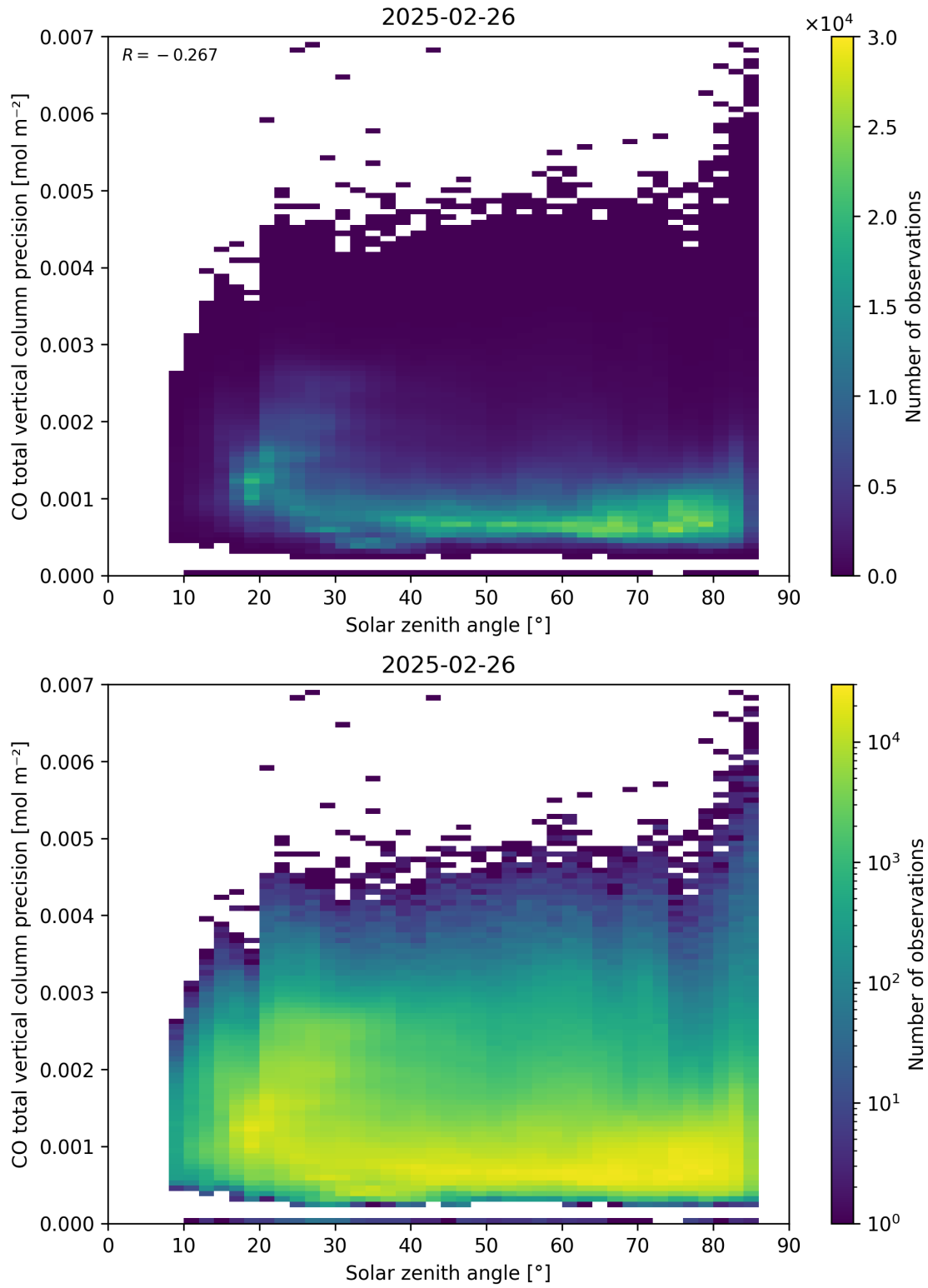
Figure 63: Scatter density plot of “Solar zenith angle” against “CO total vertical column precision” for 2025-02-25 to 2025-02-27.
