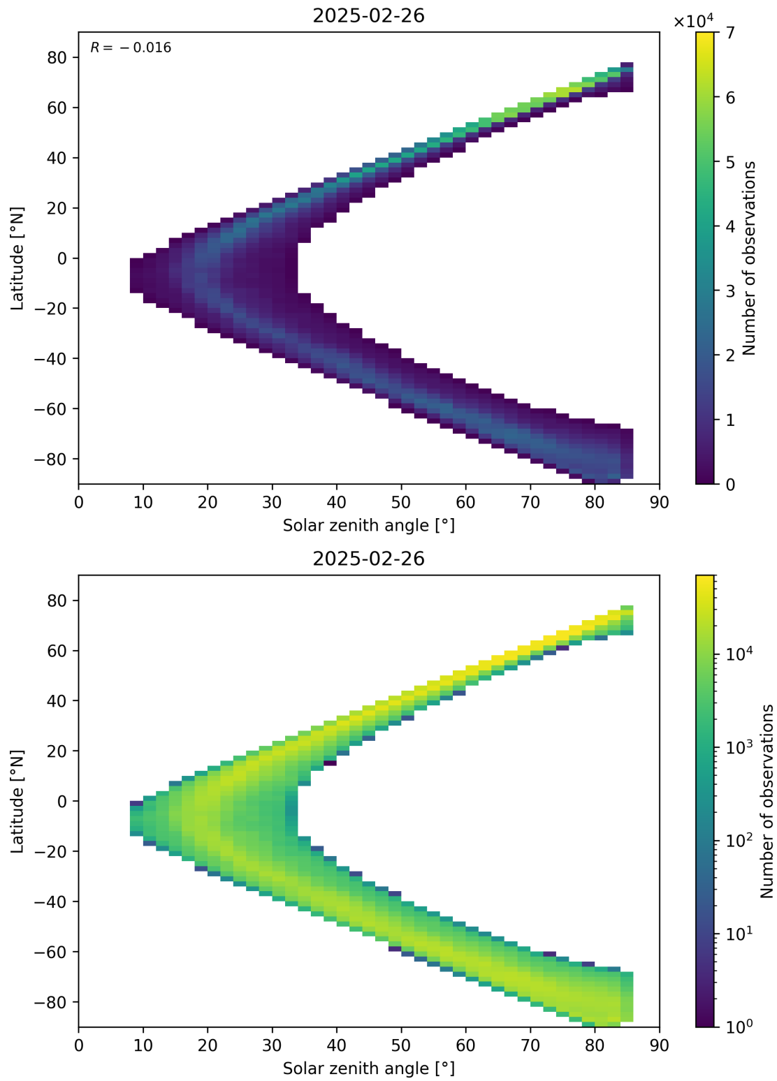
Figure 66: Scatter density plot of “Solar zenith angle” against “Latitude” for 2025-02-25 to 2025-02-27.
