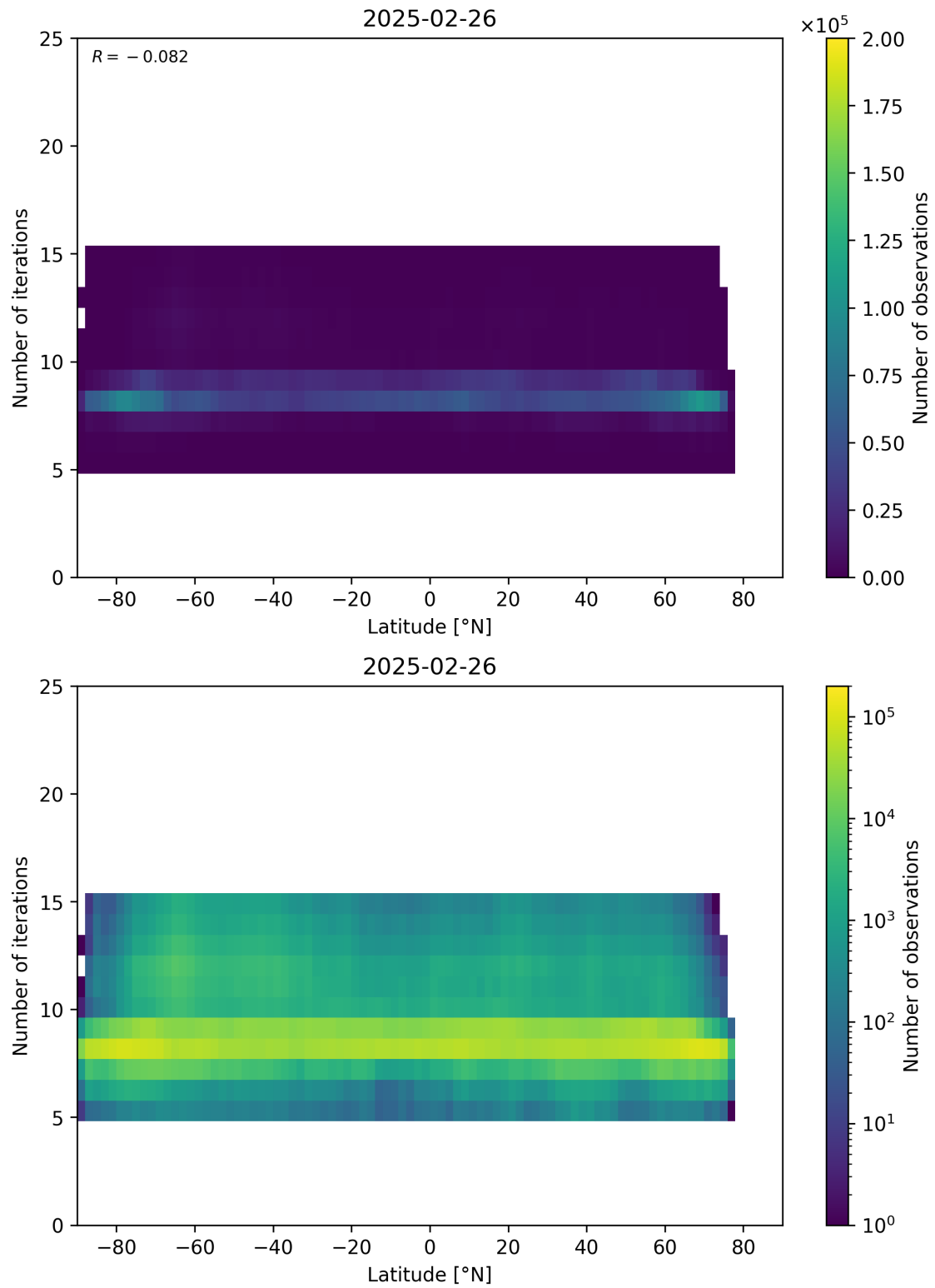
Figure 56: Scatter density plot of “Latitude” against “Number of iterations” for 2025-02-25 to 2025-02-27.
