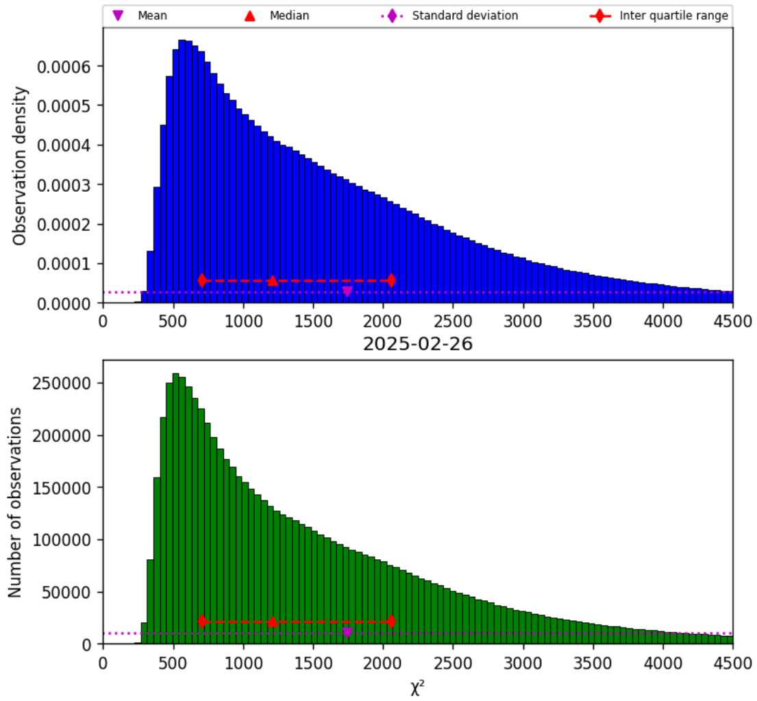
Figure 22: Histogram of “ \chi^2 ” for 2025-02-25 to 2025-02-27
