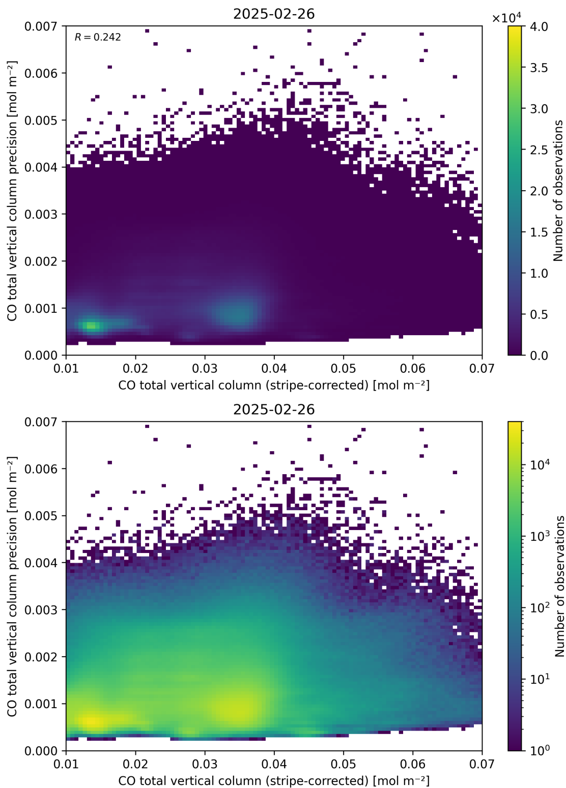
Figure 36: Scatter density plot of “CO total vertical column (stripe-corrected)” against “CO total vertical column precision” for 2025-02-25 to 2025-02-27.
