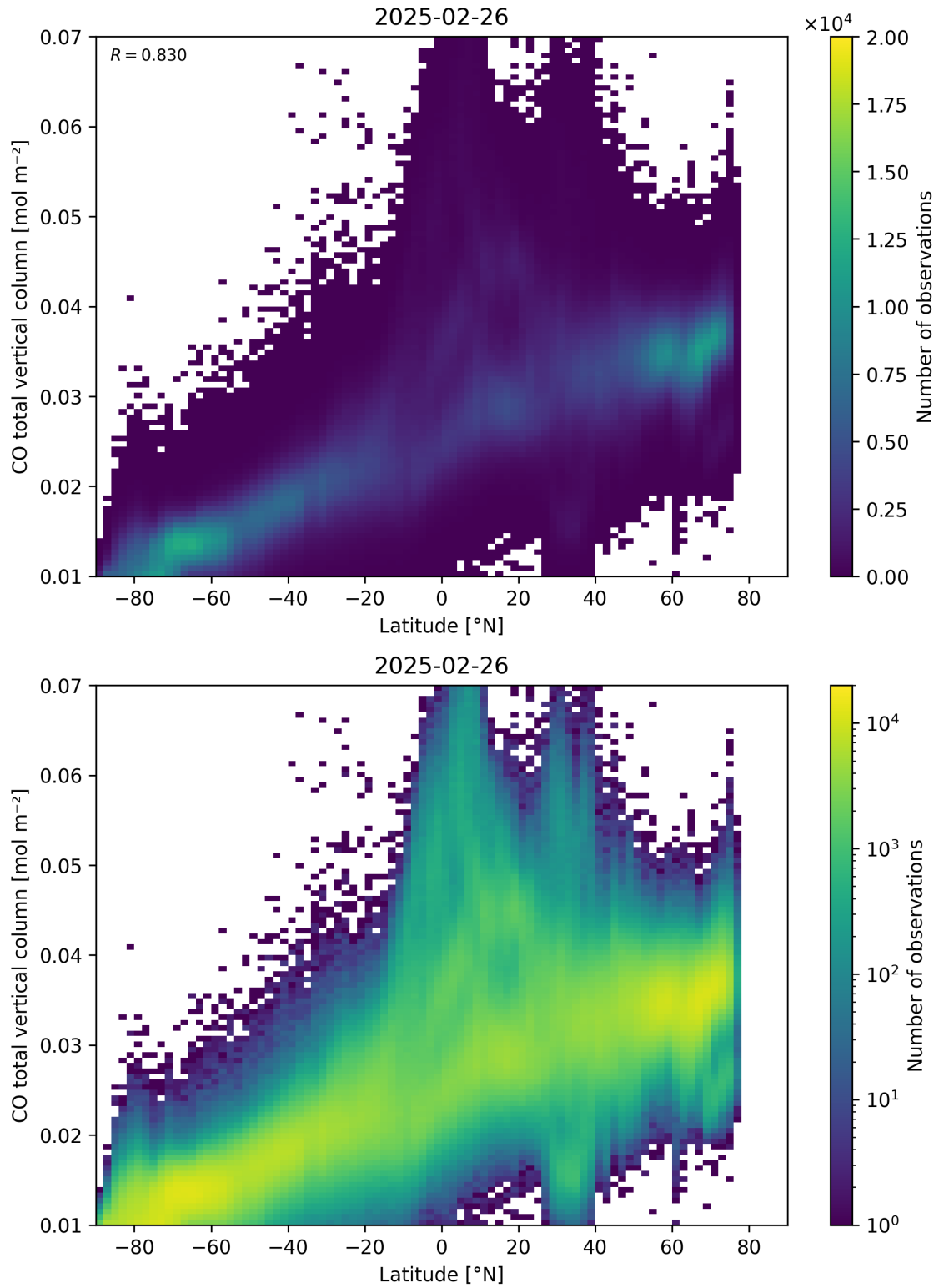
Figure 51: Scatter density plot of “Latitude” against “CO total vertical column” for 2025-02-25 to 2025-02-27.
