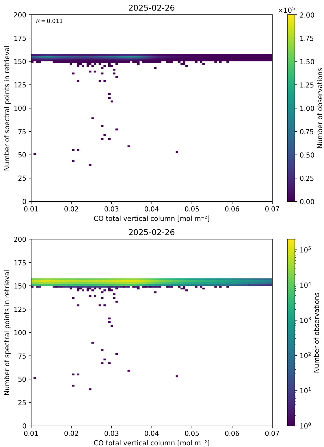
Figure 43: Scatter density plot of “CO total vertical column” against “Number of spectral points in retrieval” for 2025-02-25 to 2025-02-27.
