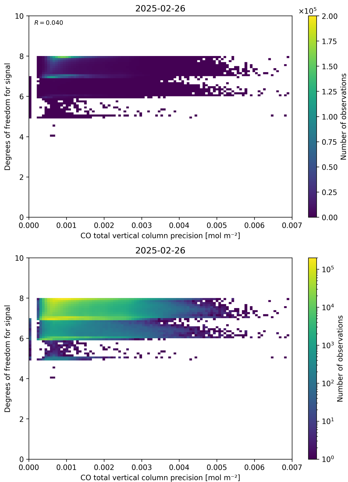
Figure 45: Scatter density plot of “CO total vertical column precision” against “Degrees of freedom for signal” for 2025-02-25 to 2025-02-27.
