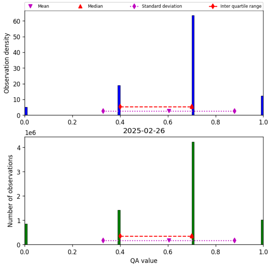
Figure 17: Histogram of “QA value” for 2025-02-25 to 2025-02-27
