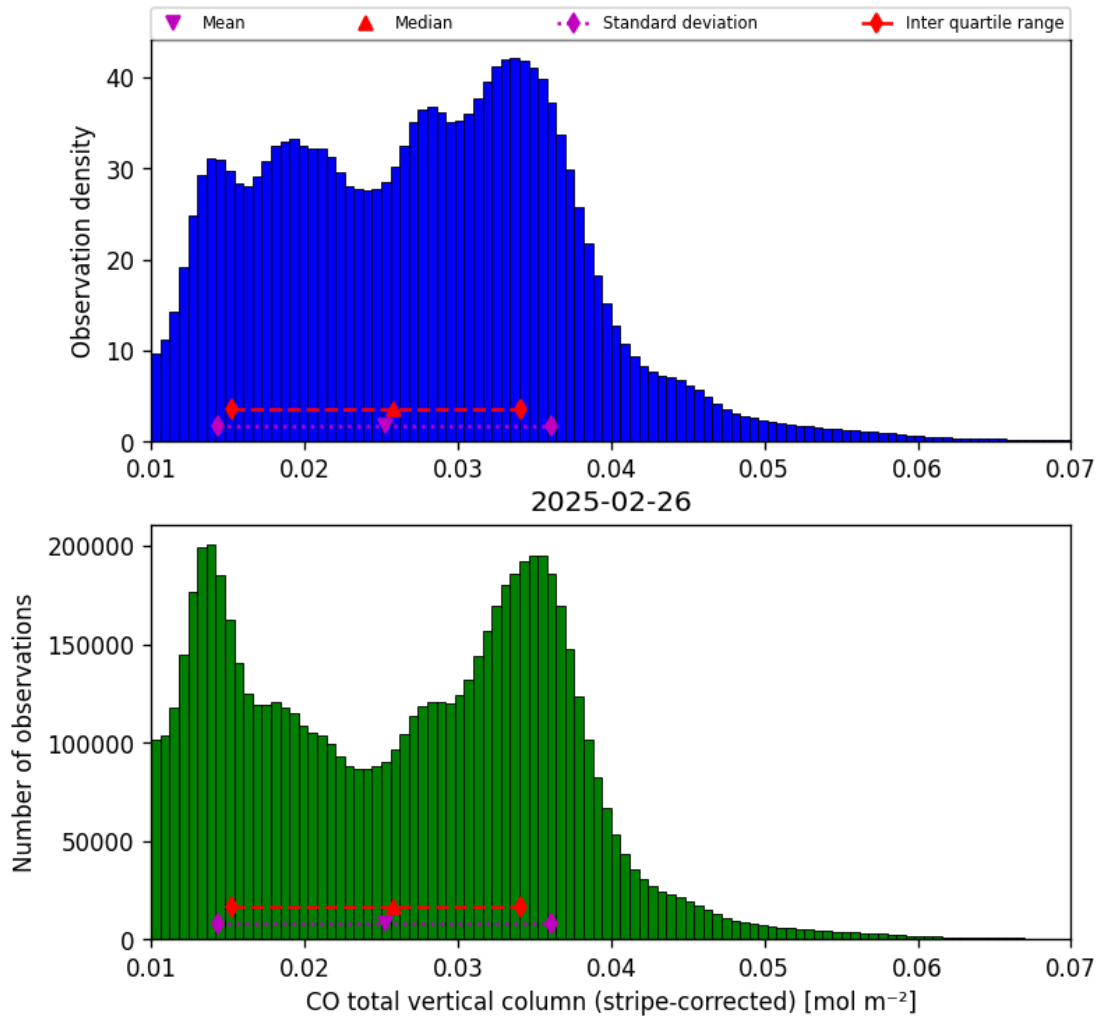
Figure 19: Histogram of “CO total vertical column (stripe-corrected)” for 2025-02-25 to 2025-02-27
