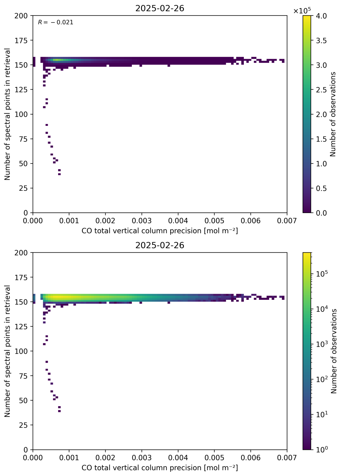
Figure 47: Scatter density plot of “CO total vertical column precision” against “Number of spectral points in retrieval” for 2025-02-25 to 2025-02-27.
