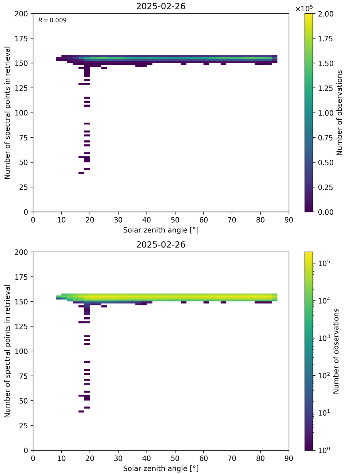
Figure 68: Scatter density plot of “Solar zenith angle” against “Number of spectral points in retrieval” for 2025-02-25 to 2025-02-27.
