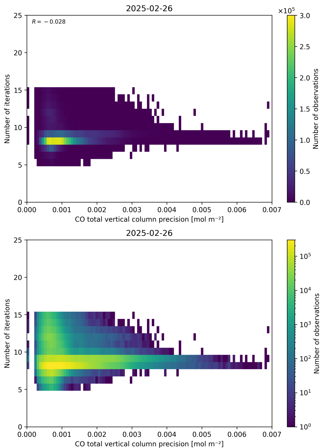
Figure 46: Scatter density plot of “CO total vertical column precision” against “Number of iterations” for 2025-02-25 to 2025-02-27.
