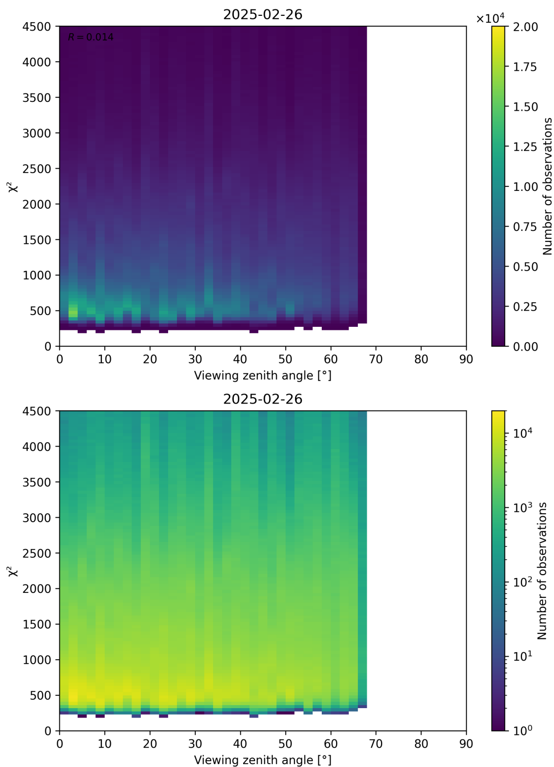
Figure 72: Scatter density plot of “Viewing zenith angle” against “ \chi^2 ” for 2025-02-25 to 2025-02-27.
