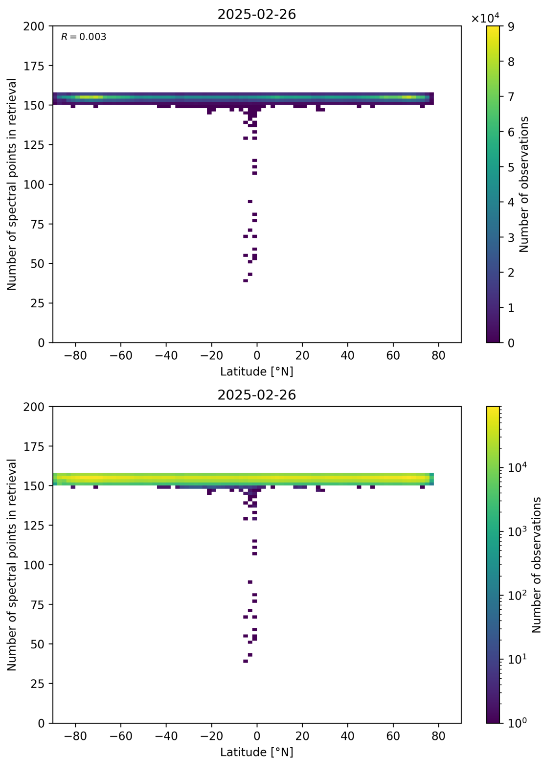
Figure 57: Scatter density plot of “Latitude” against “Number of spectral points in retrieval” for 2025-02-25 to 2025-02-27.
