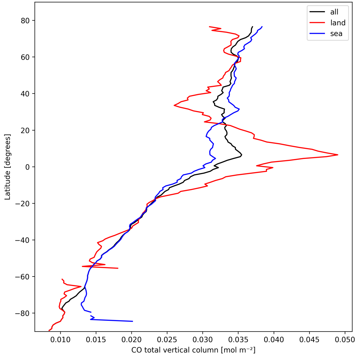
Figure 10: Zonal average of “CO total vertical column” for 2025-02-25 to 2025-02-27.
