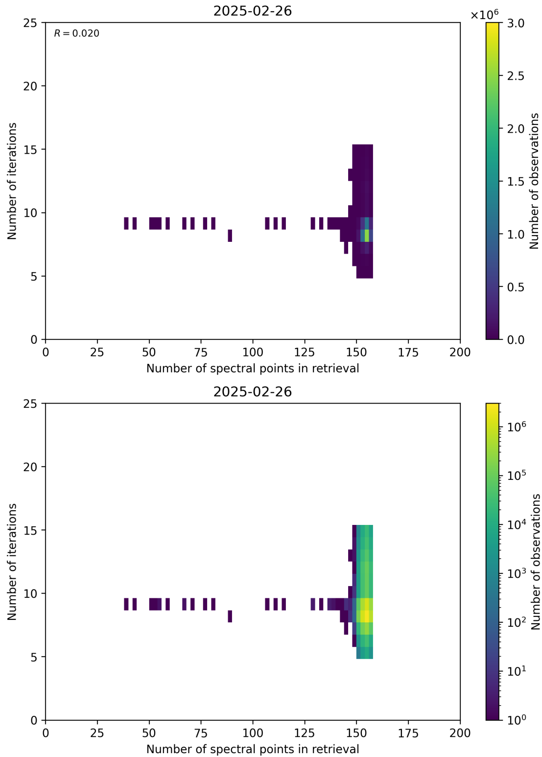
Figure 60: Scatter density plot of “Number of spectral points in retrieval” against “Number of iterations” for 2025-02-25 to 2025-02-27.
