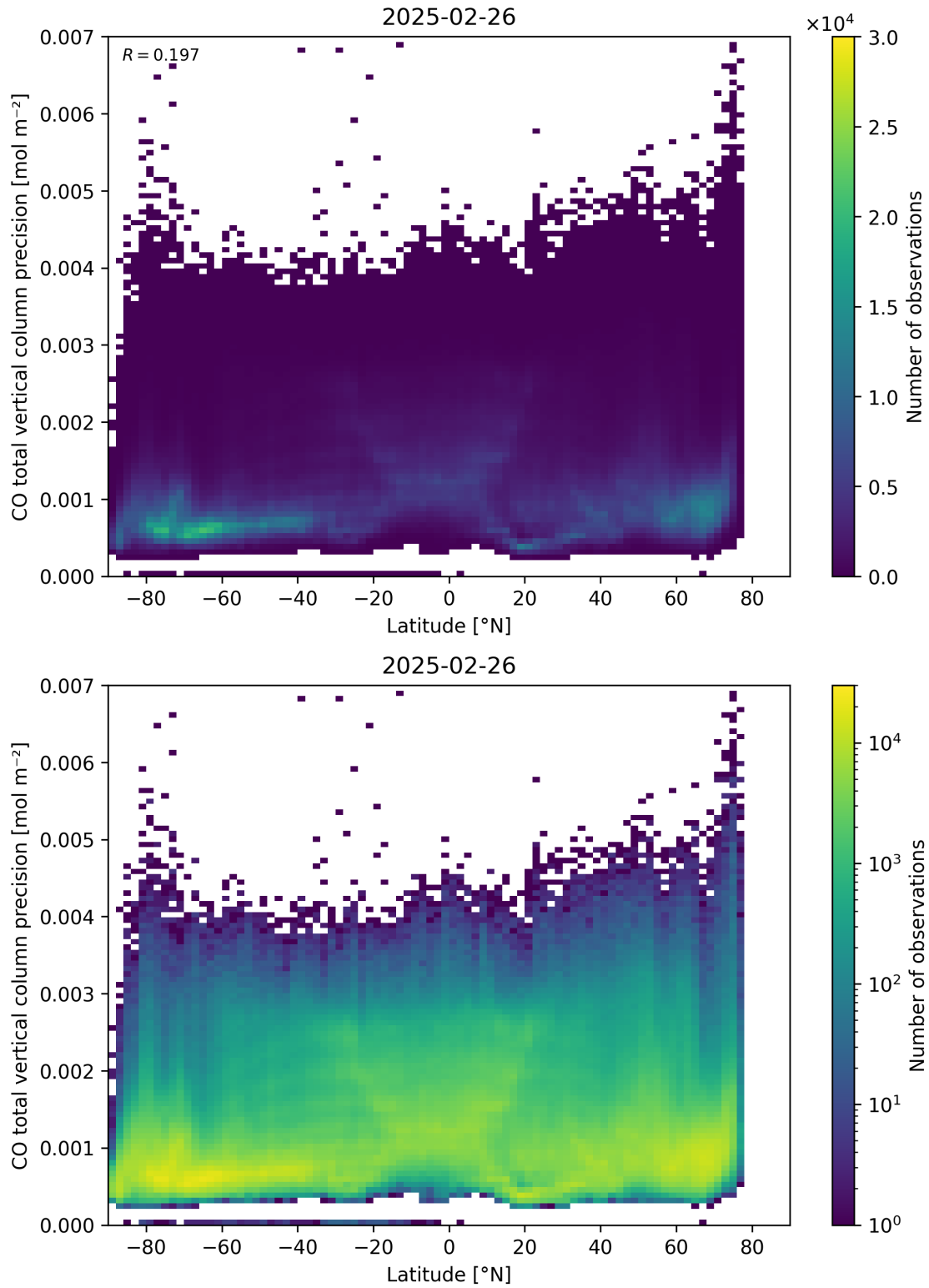
Figure 53: Scatter density plot of “Latitude” against “CO total vertical column precision” for 2025-02-25 to 2025-02-27.
