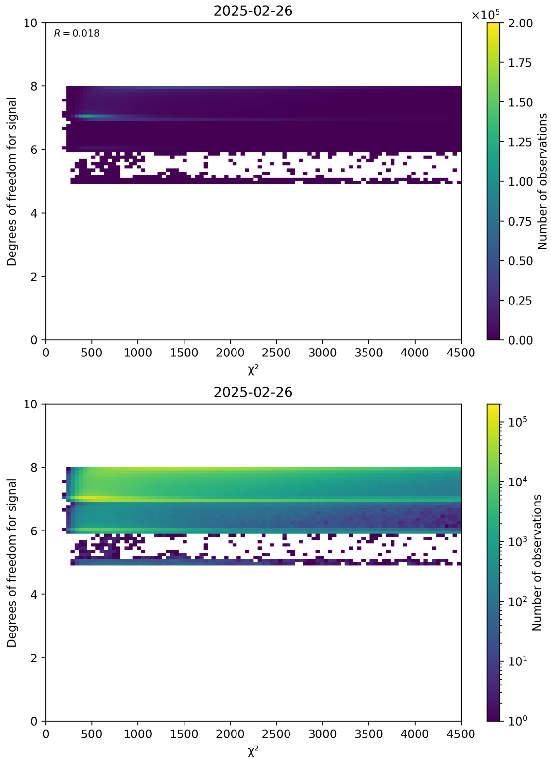
Figure 48: Scatter density plot of “ \chi^2 ” against “Degrees of freedom for signal” for 2025-02-25 to 2025-02-27.
