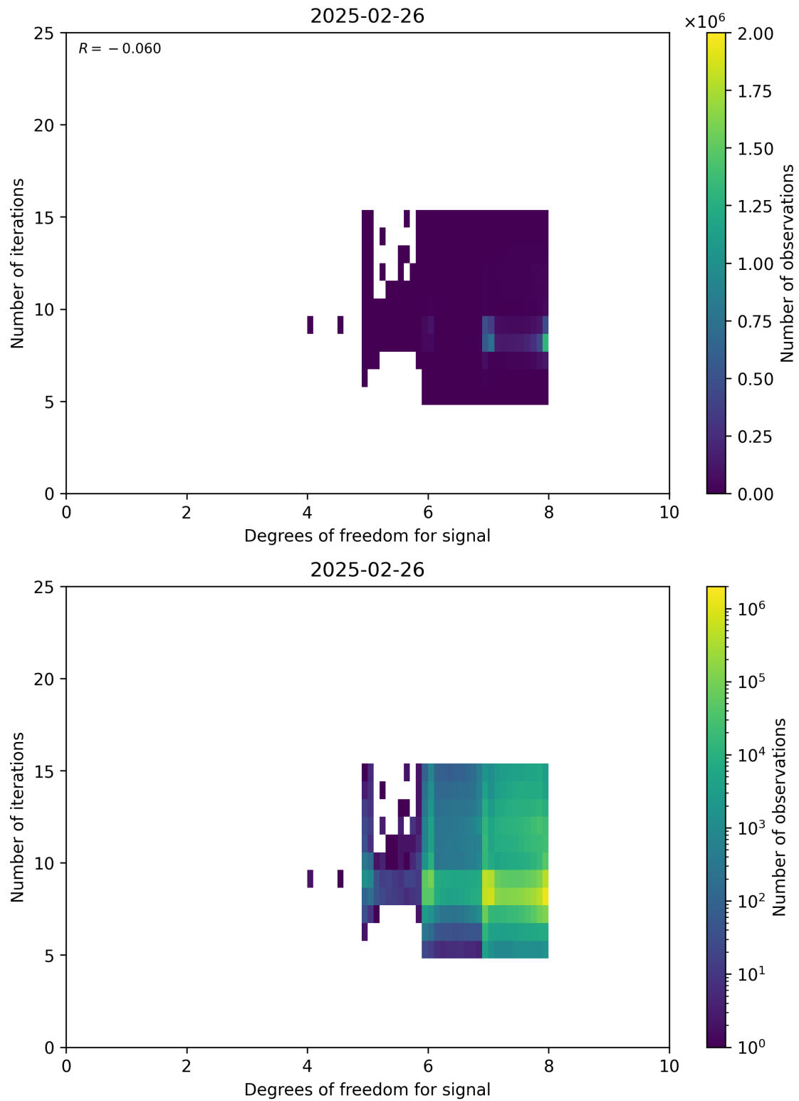
Figure 50: Scatter density plot of “Degrees of freedom for signal” against “Number of iterations” for 2025-02-25 to 2025-02-27.
