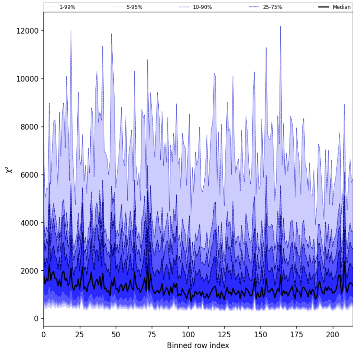
Figure 30: Along track statistics of “ \chi^2 ” for 2025-02-25 to 2025-02-27
