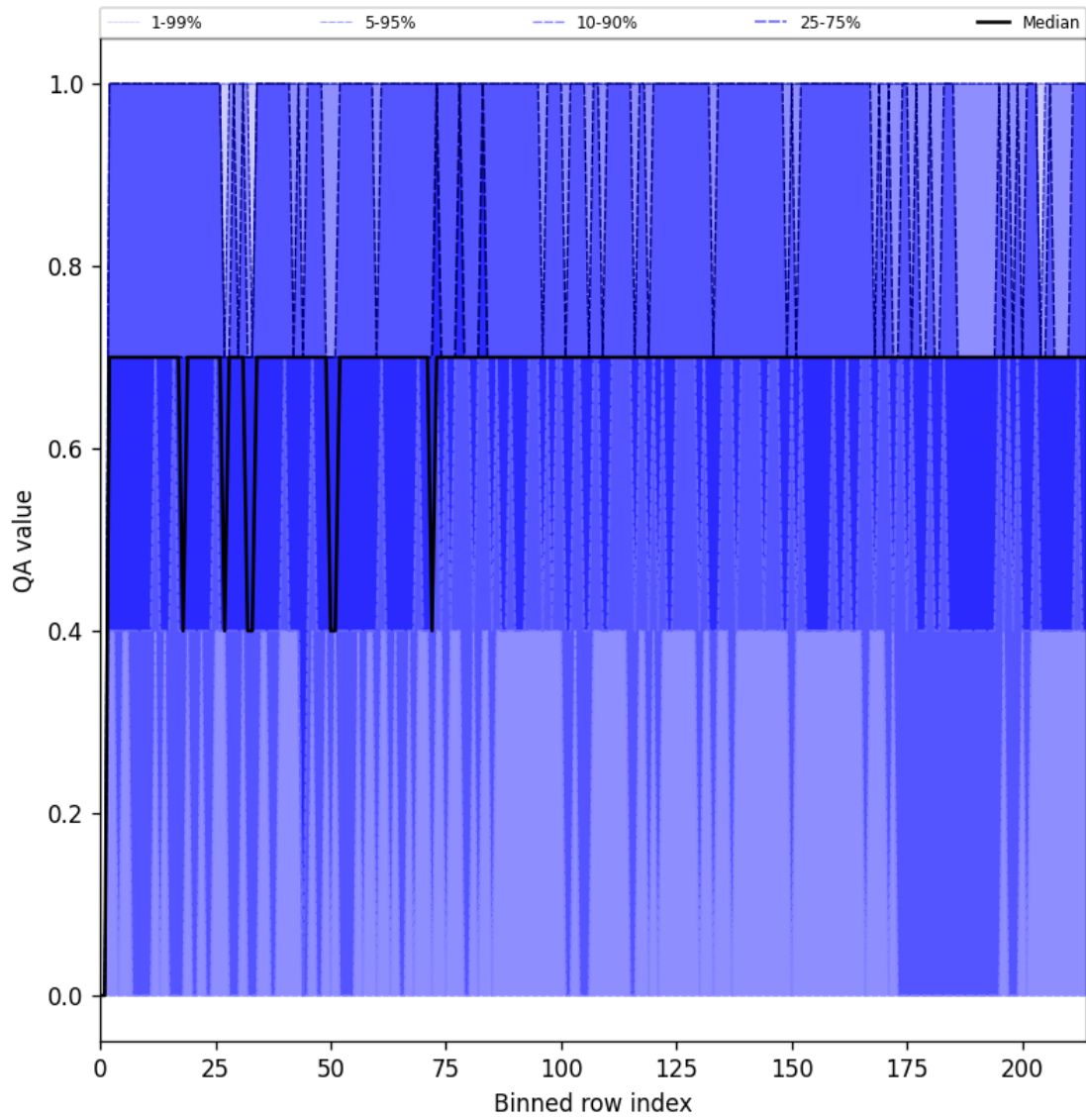
Figure 25: Along track statistics of “QA value” for 2025-02-25 to 2025-02-27
