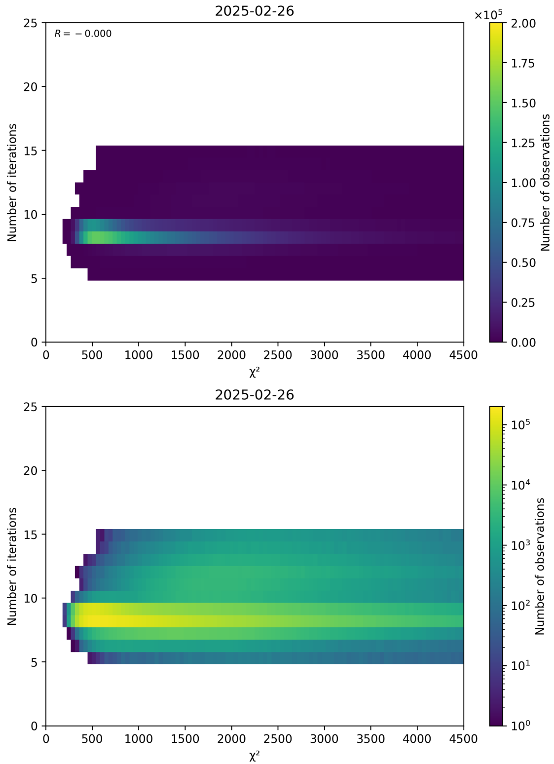
Figure 49: Scatter density plot of “ \chi^2 ” against “Number of iterations” for 2025-02-25 to 2025-02-27.
