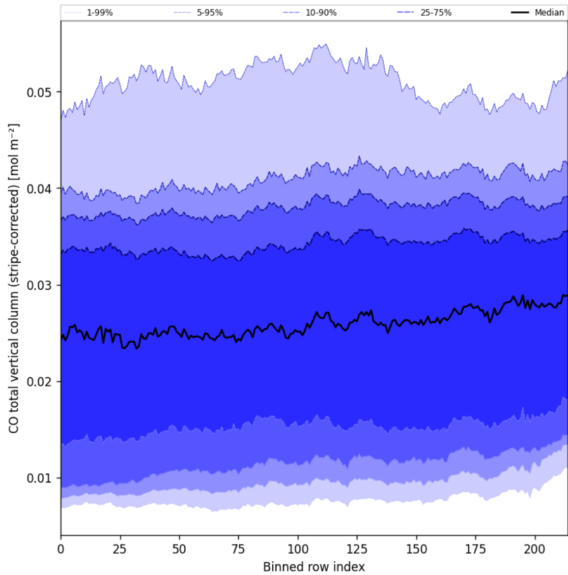
Figure 27: Along track statistics of “CO total vertical column (stripe-corrected)” for 2025-02-25 to 2025-02-27
