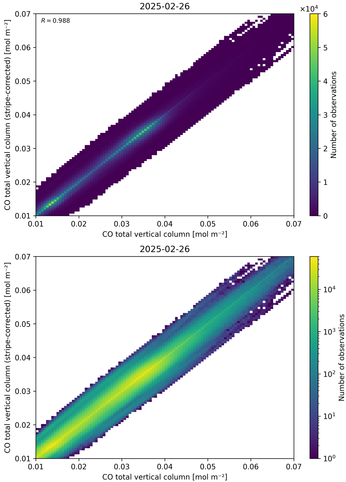
Figure 33: Scatter density plot of “CO total vertical column” against “CO total vertical column (stripe-corrected)” for 2025-02-25 to 2025-02-27.
