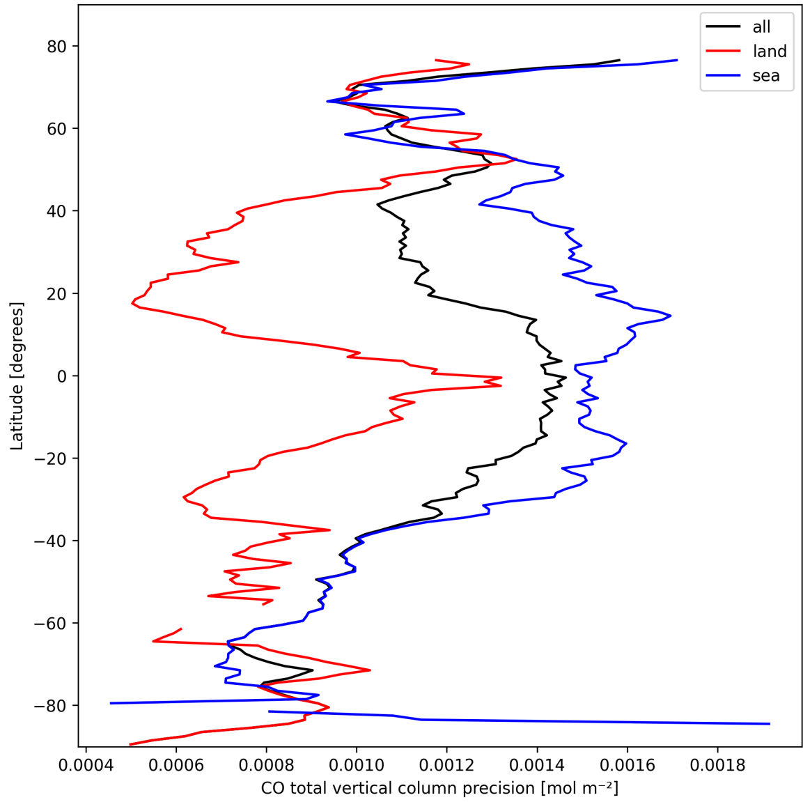
Figure 12: Zonal average of “CO total vertical column precision” for 2025-02-25 to 2025-02-27.
