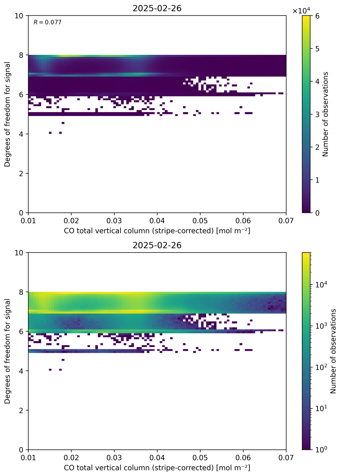
Figure 38: Scatter density plot of “CO total vertical column (stripe-corrected)” against “Degrees of freedom for signal” for 2025-02-25 to 2025-02-27.
