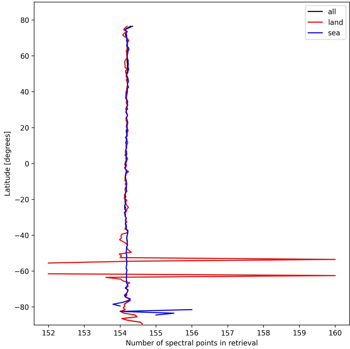
Figure 13: Zonal average of “Number of spectral points in retrieval” for 2025-02-25 to 2025-02-27.
