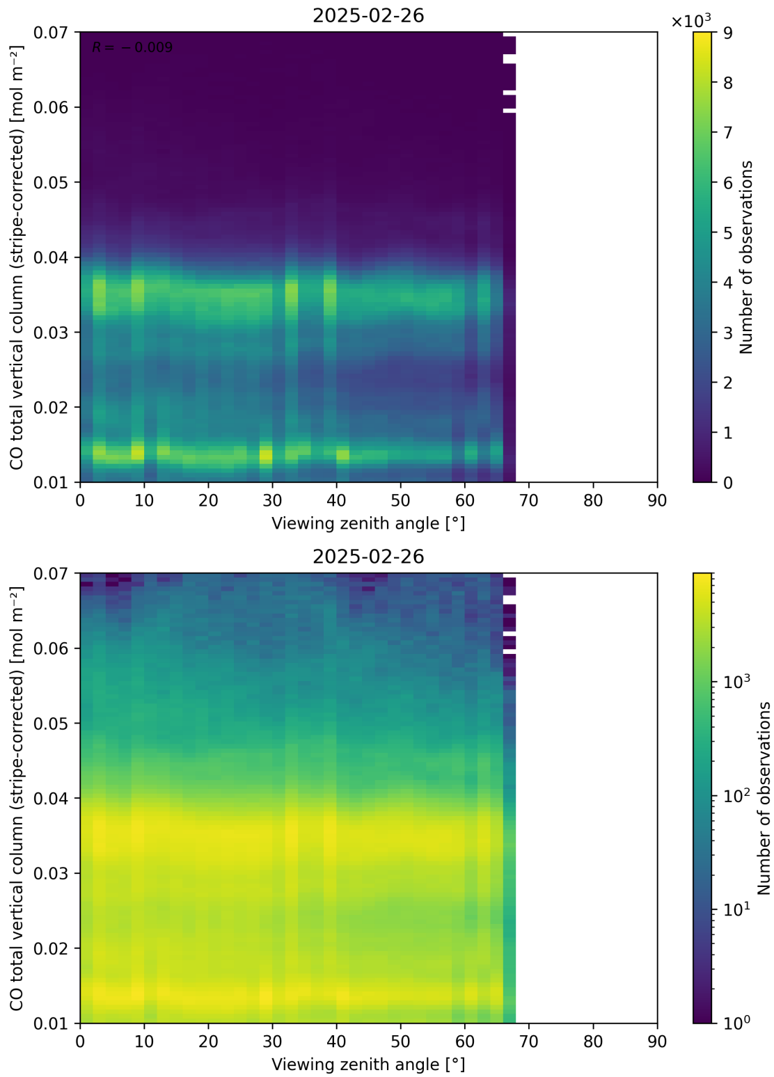
Figure 70: Scatter density plot of “Viewing zenith angle” against “CO total vertical column (stripe-corrected)” for 2025-02-25 to 2025-02-27.
