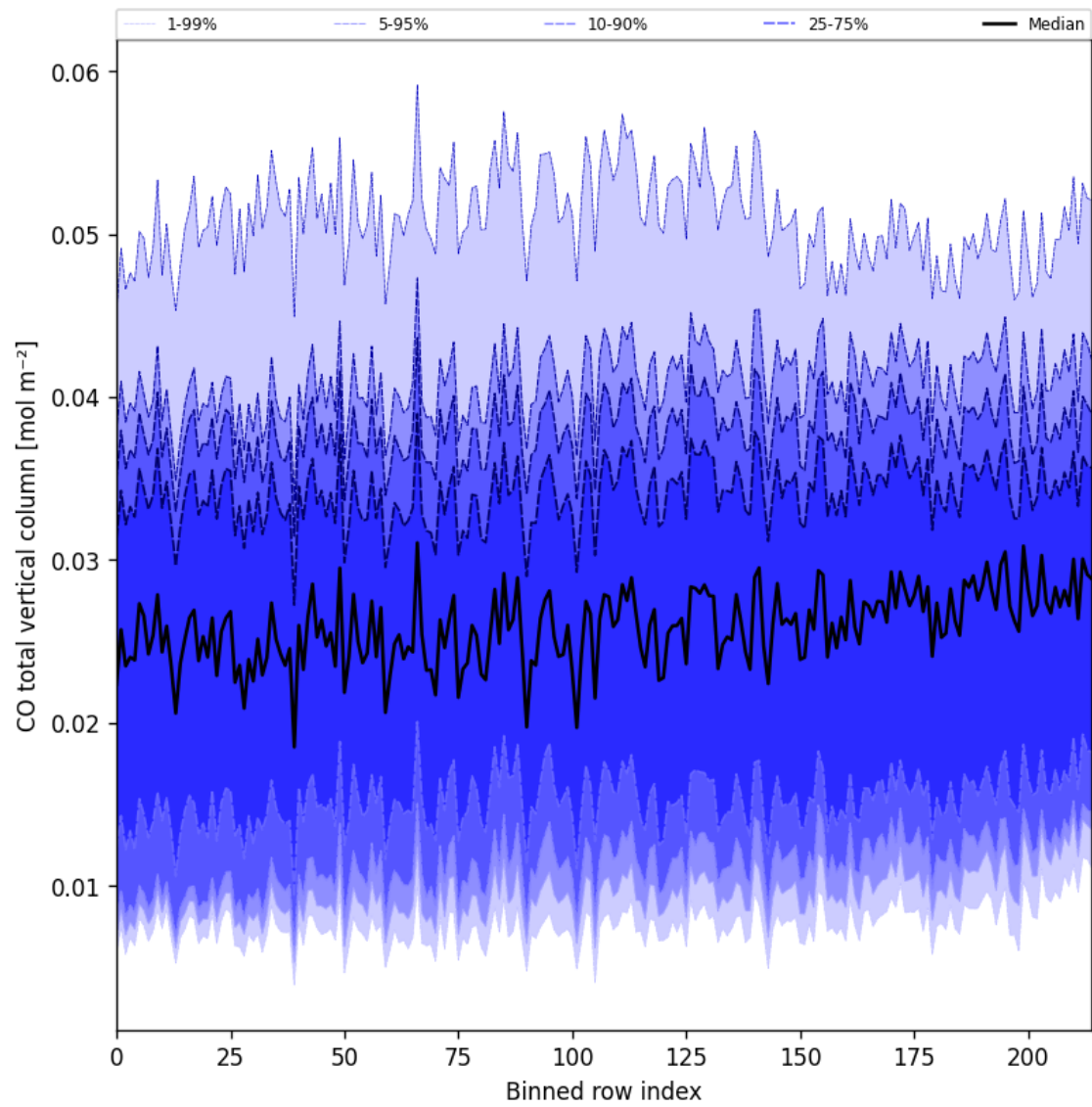
Figure 26: Along track statistics of “CO total vertical column” for 2025-02-25 to 2025-02-27
