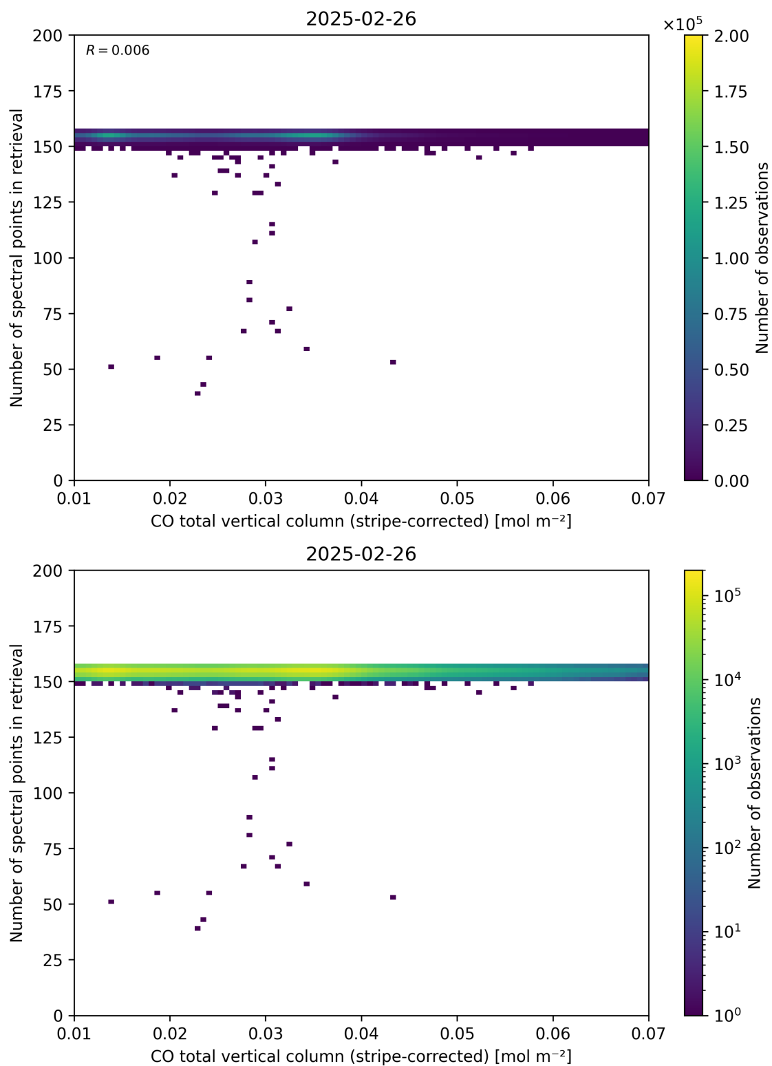
Figure 40: Scatter density plot of “CO total vertical column (stripe-corrected)” against “Number of spectral points in retrieval” for 2025-02-25 to 2025-02-27.
