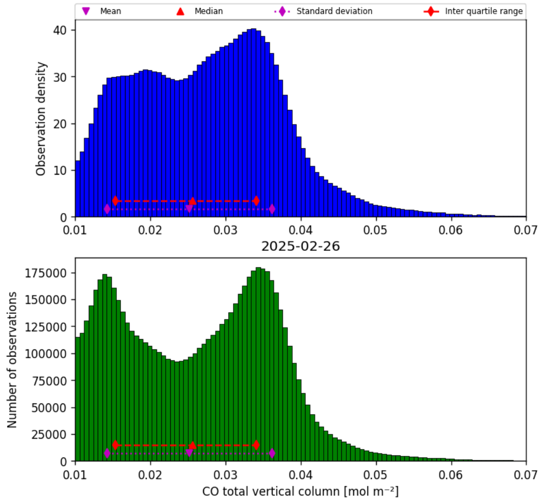
Figure 18: Histogram of “CO total vertical column” for 2025-02-25 to 2025-02-27
