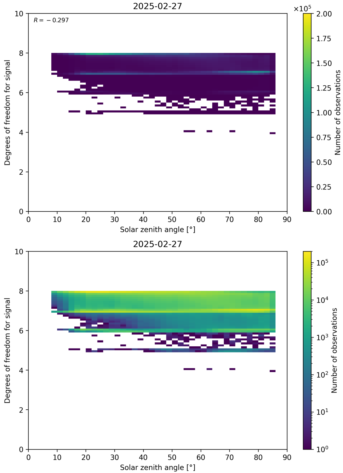
Figure 65: Scatter density plot of “Solar zenith angle” against “Degrees of freedom for signal” for 2025-02-26 to 2025-02-28.
