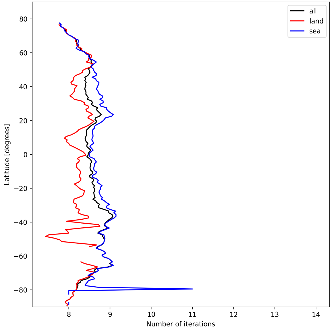
Figure 16: Zonal average of “Number of iterations” for 2025-02-26 to 2025-02-28.
