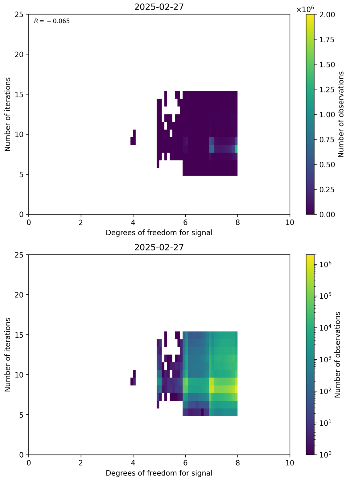
Figure 50: Scatter density plot of “Degrees of freedom for signal” against “Number of iterations” for 2025-02-26 to 2025-02-28.
