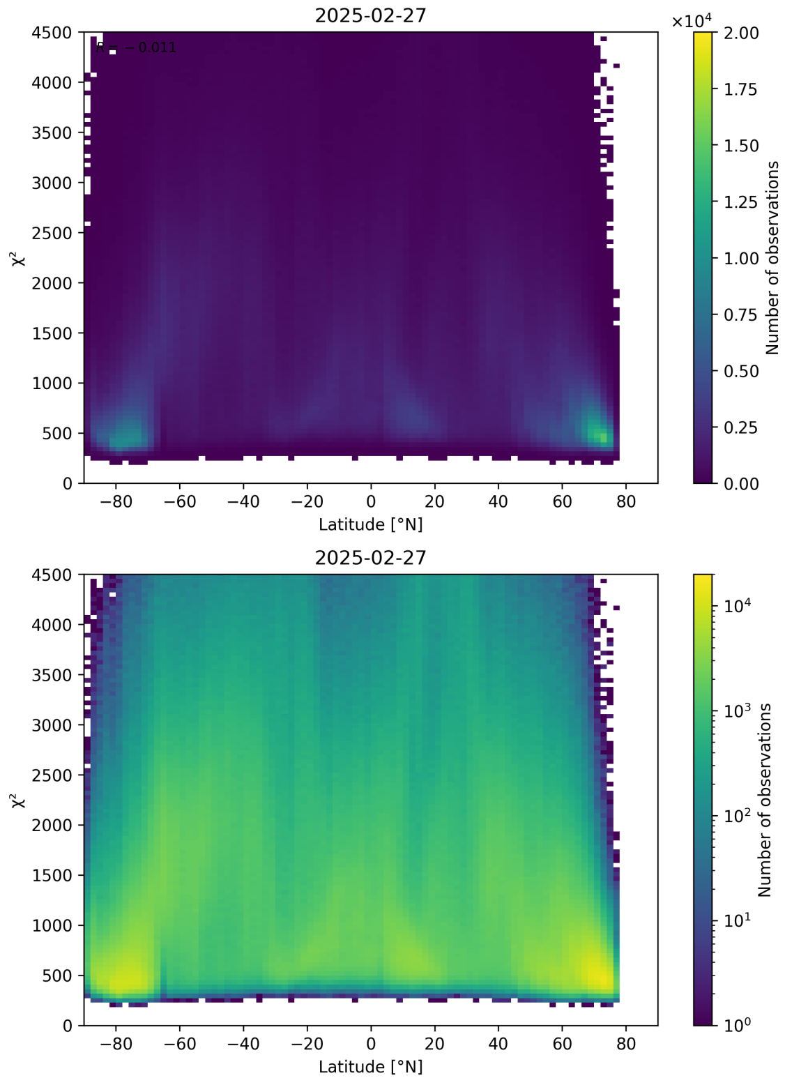
Figure 54: Scatter density plot of “Latitude” against “ \chi^2 ” for 2025-02-26 to 2025-02-28.
