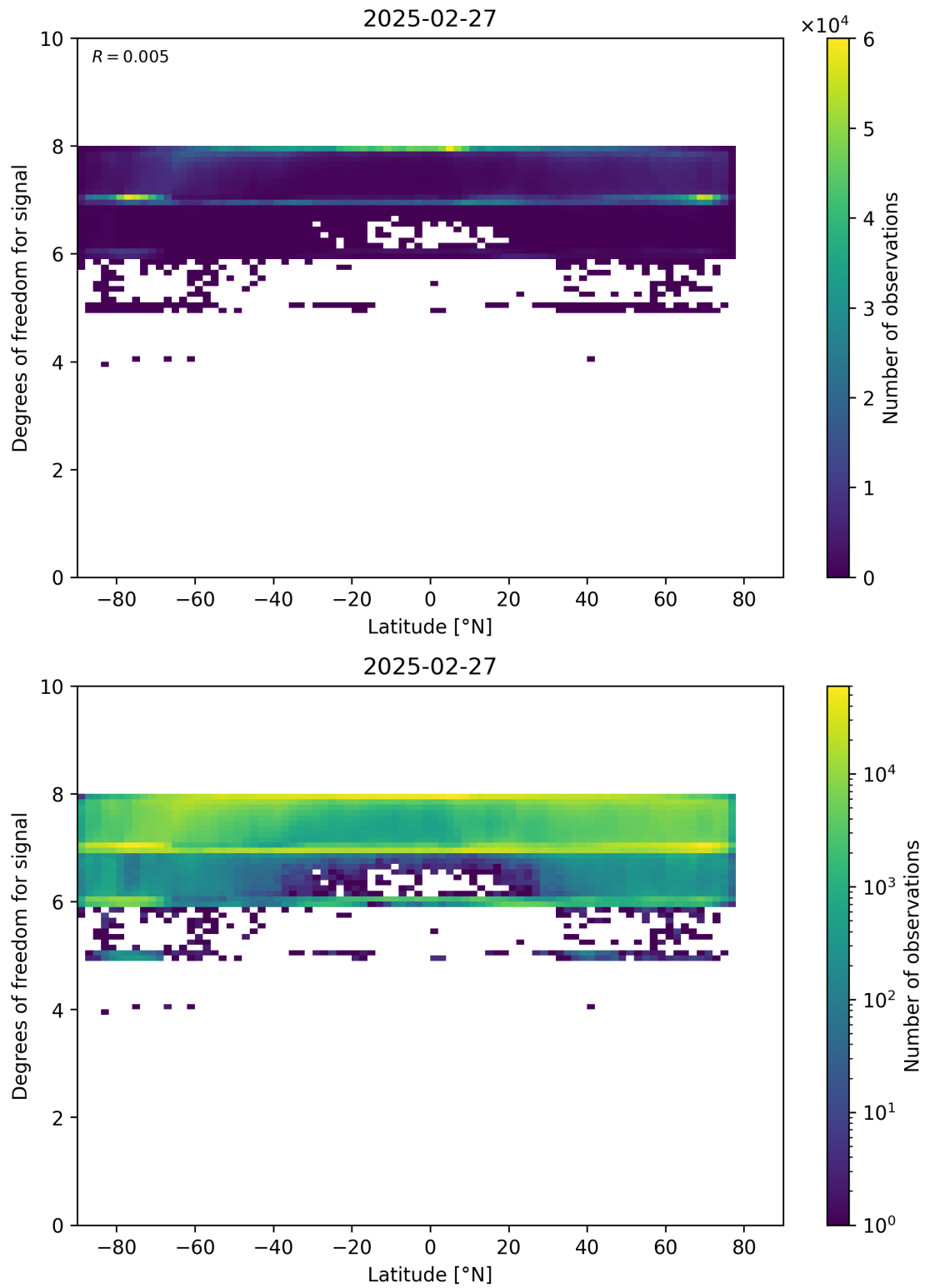
Figure 55: Scatter density plot of “Latitude” against “Degrees of freedom for signal” for 2025-02-26 to 2025-02-28.
