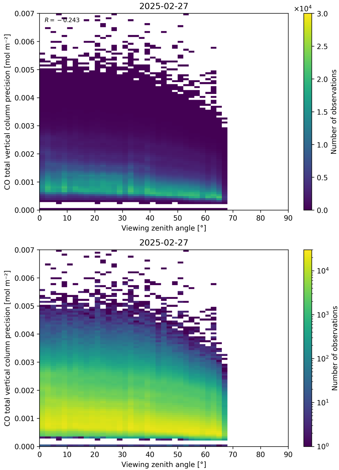
Figure 71: Scatter density plot of “Viewing zenith angle” against “CO total vertical column precision” for 2025-02-26 to 2025-02-28.
