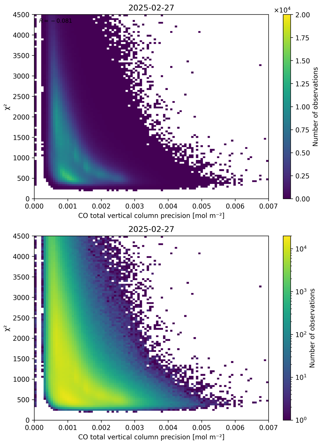
Figure 44: Scatter density plot of “CO total vertical column precision” against “ \chi^2 ” for 2025-02-26 to 2025-02-28.
