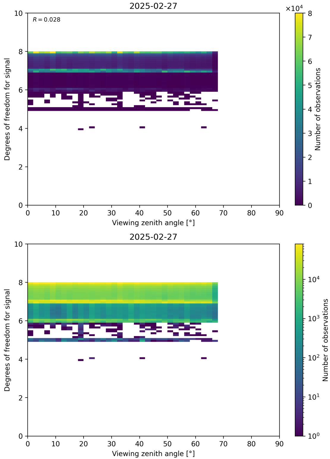
Figure 73: Scatter density plot of “Viewing zenith angle” against “Degrees of freedom for signal” for 2025-02-26 to 2025-02-28.
