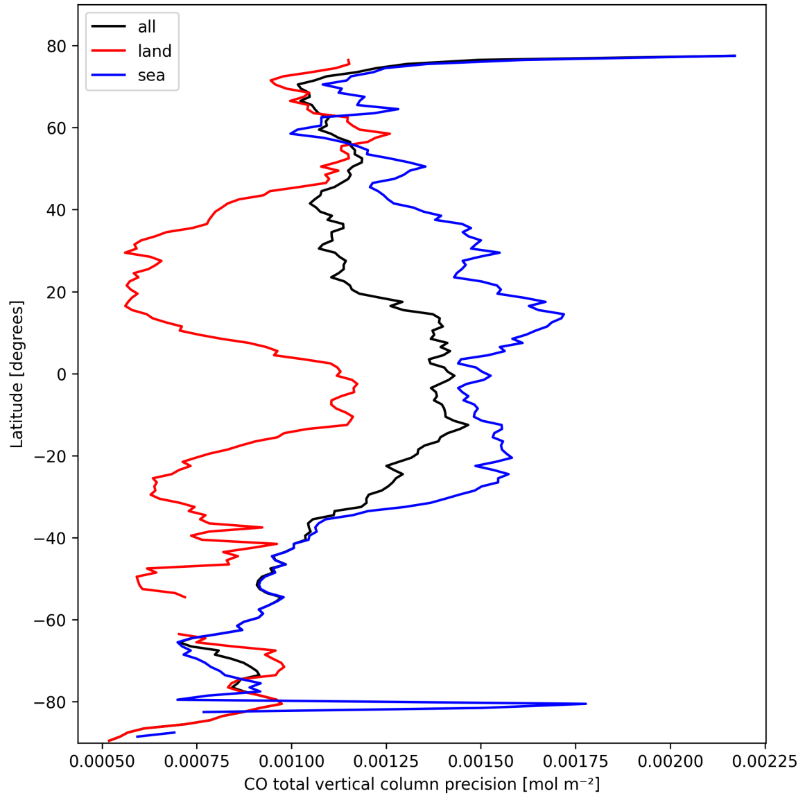
Figure 12: Zonal average of “CO total vertical column precision” for 2025-02-26 to 2025-02-28.
