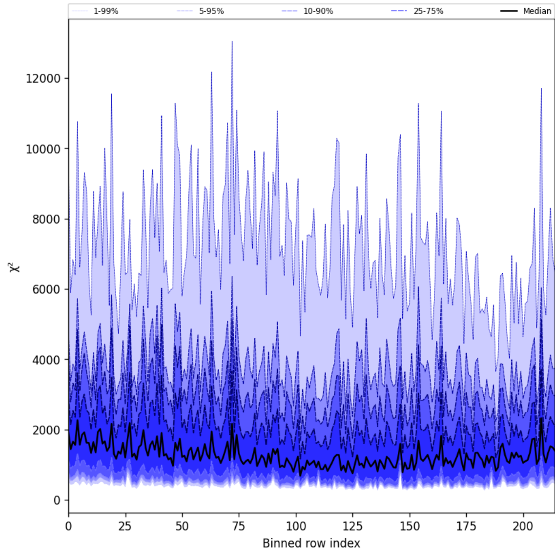
Figure 30: Along track statistics of “ \chi^2 ” for 2025-02-26 to 2025-02-28
