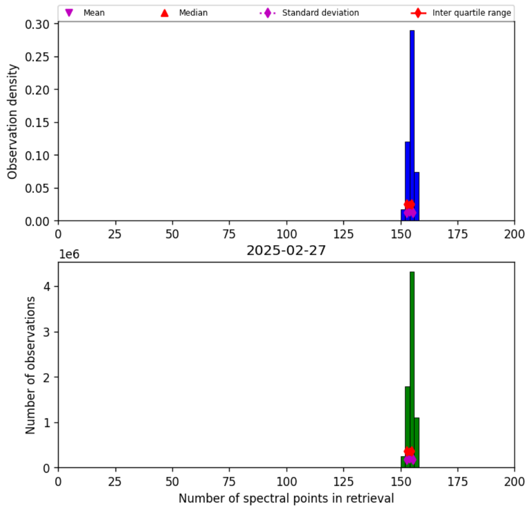
Figure 21: Histogram of “Number of spectral points in retrieval” for 2025-02-26 to 2025-02-28
