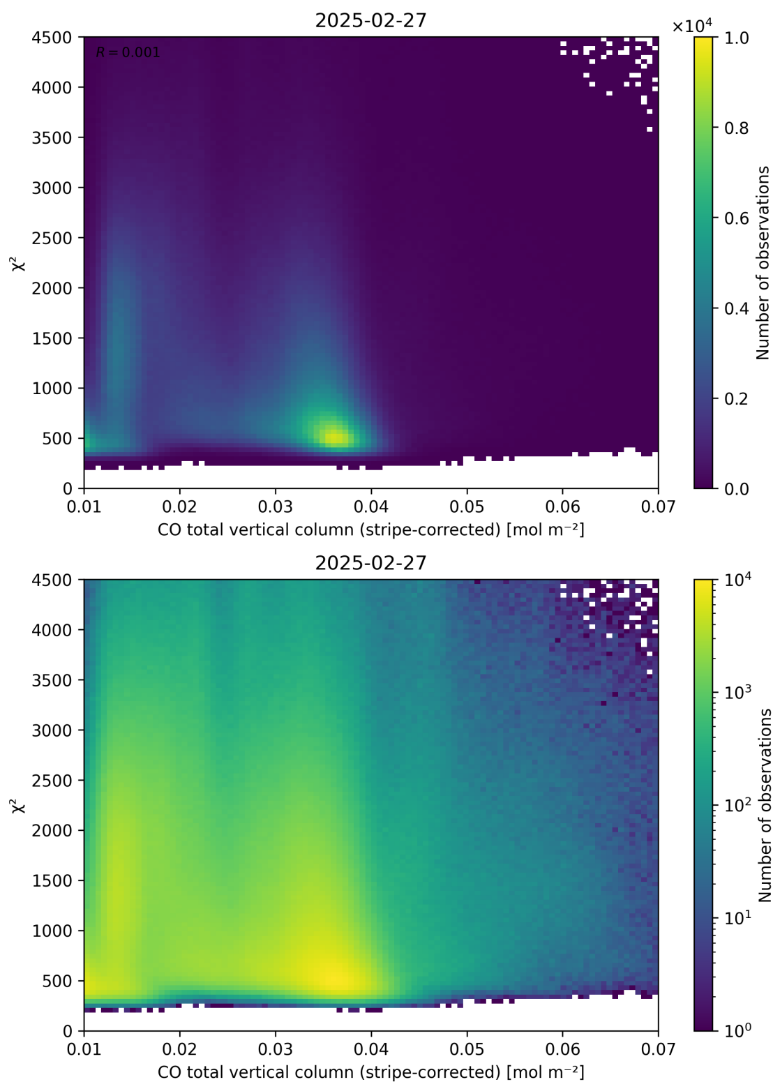
Figure 37: Scatter density plot of “CO total vertical column (stripe-corrected)” against “ \chi^2 ” for 2025-02-26 to 2025-02-28.
