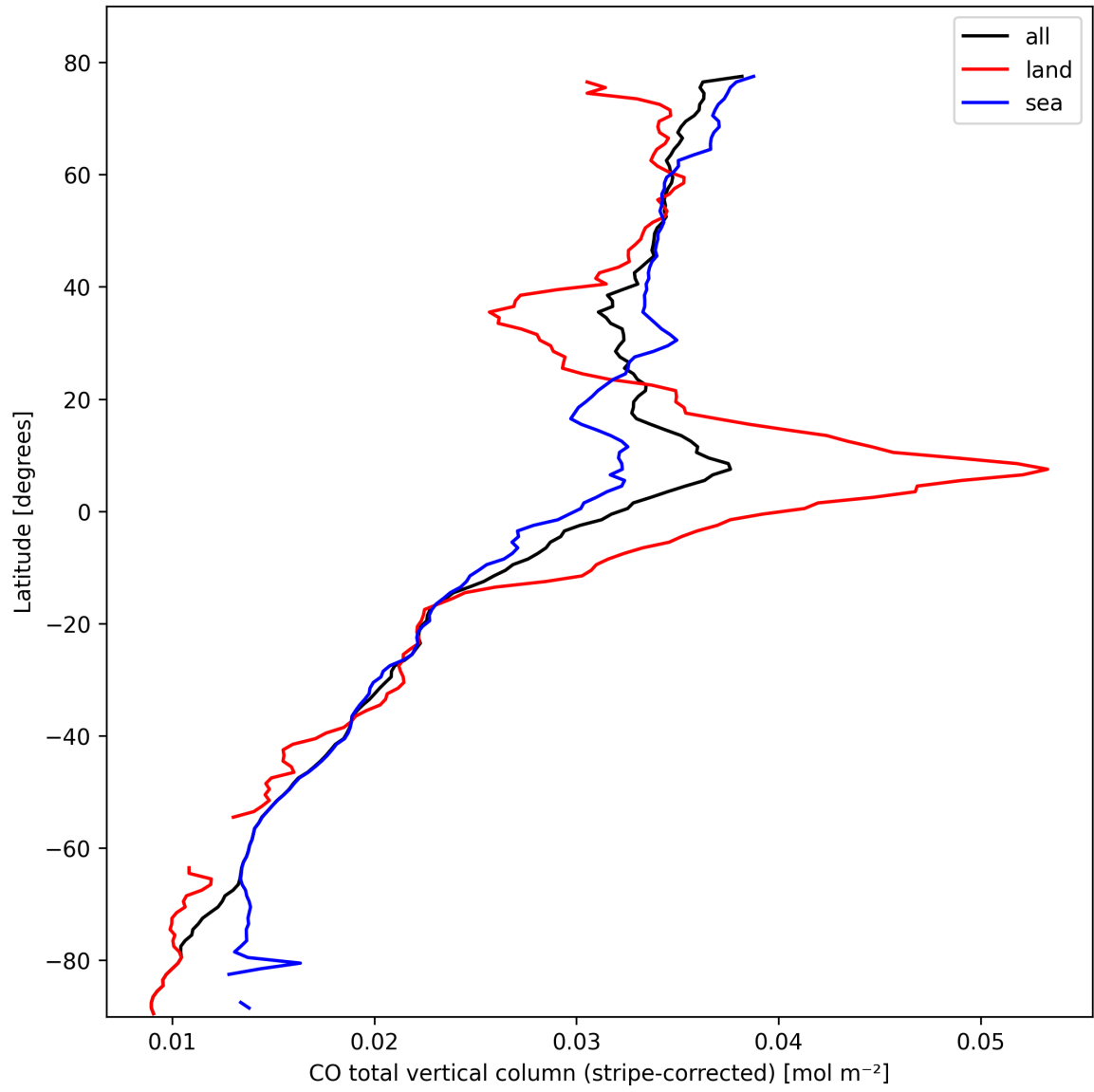
Figure 11: Zonal average of “CO total vertical column (stripe-corrected)” for 2025-02-26 to 2025-02-28.
