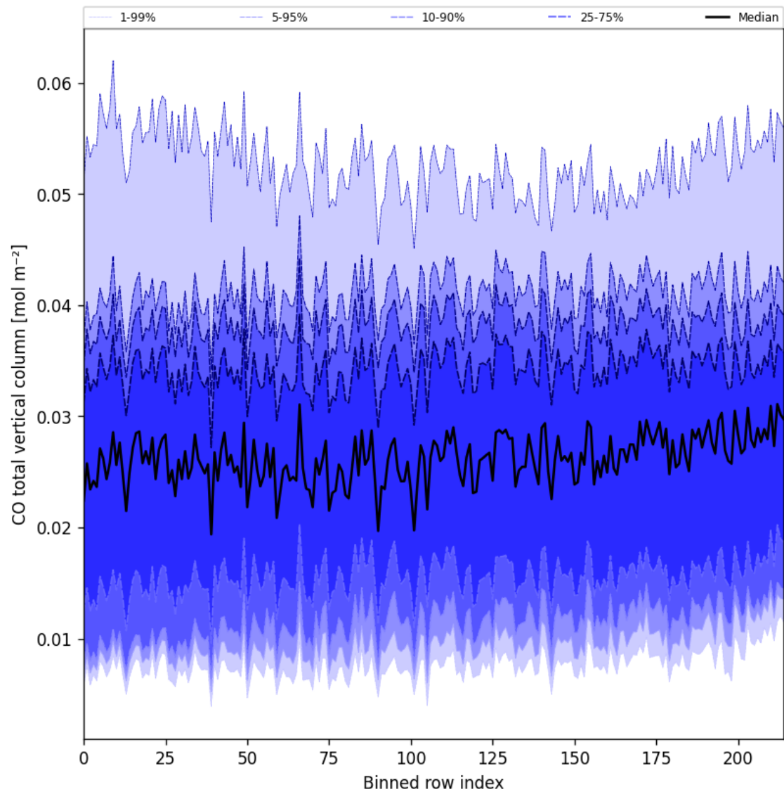
Figure 26: Along track statistics of “CO total vertical column” for 2025-02-26 to 2025-02-28
