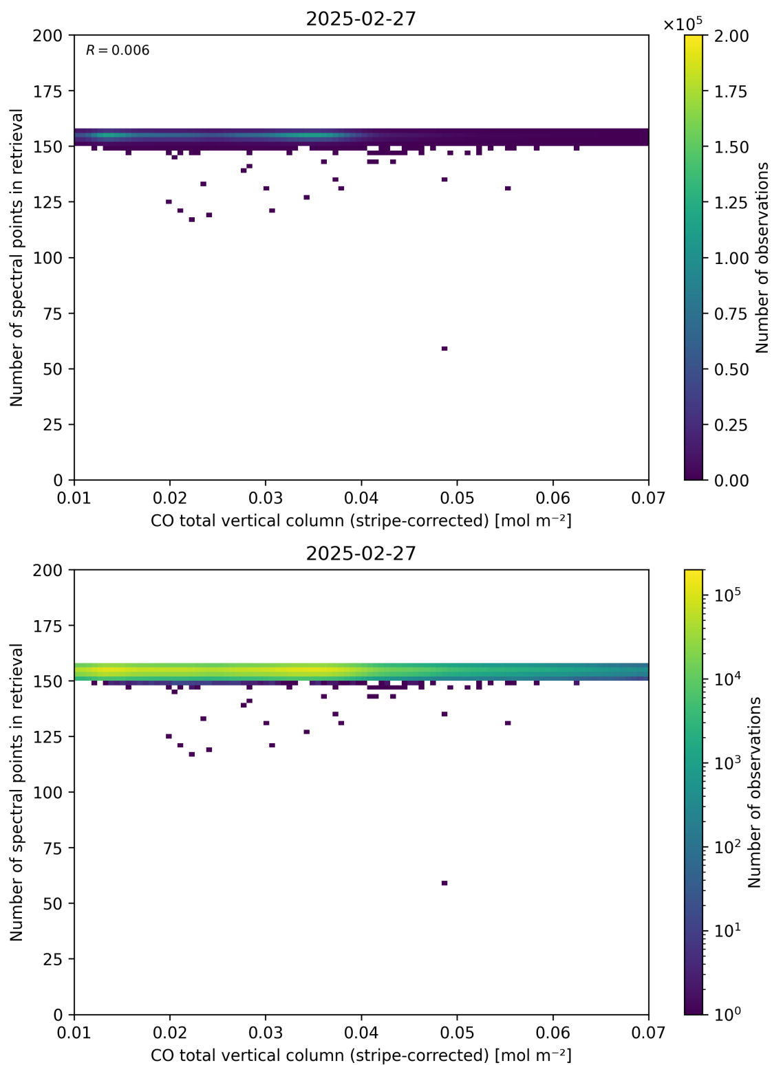
Figure 40: Scatter density plot of “CO total vertical column (stripe-corrected)” against “Number of spectral points in retrieval” for 2025-02-26 to 2025-02-28.
