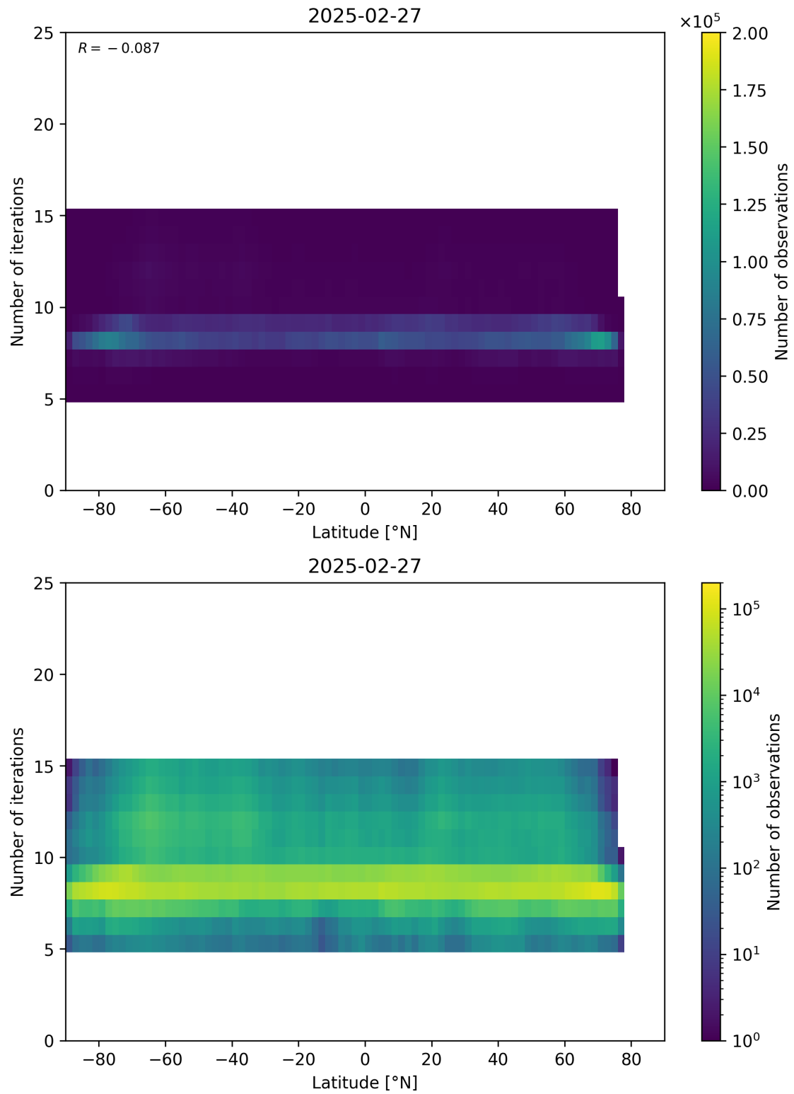
Figure 56: Scatter density plot of “Latitude” against “Number of iterations” for 2025-02-26 to 2025-02-28.
