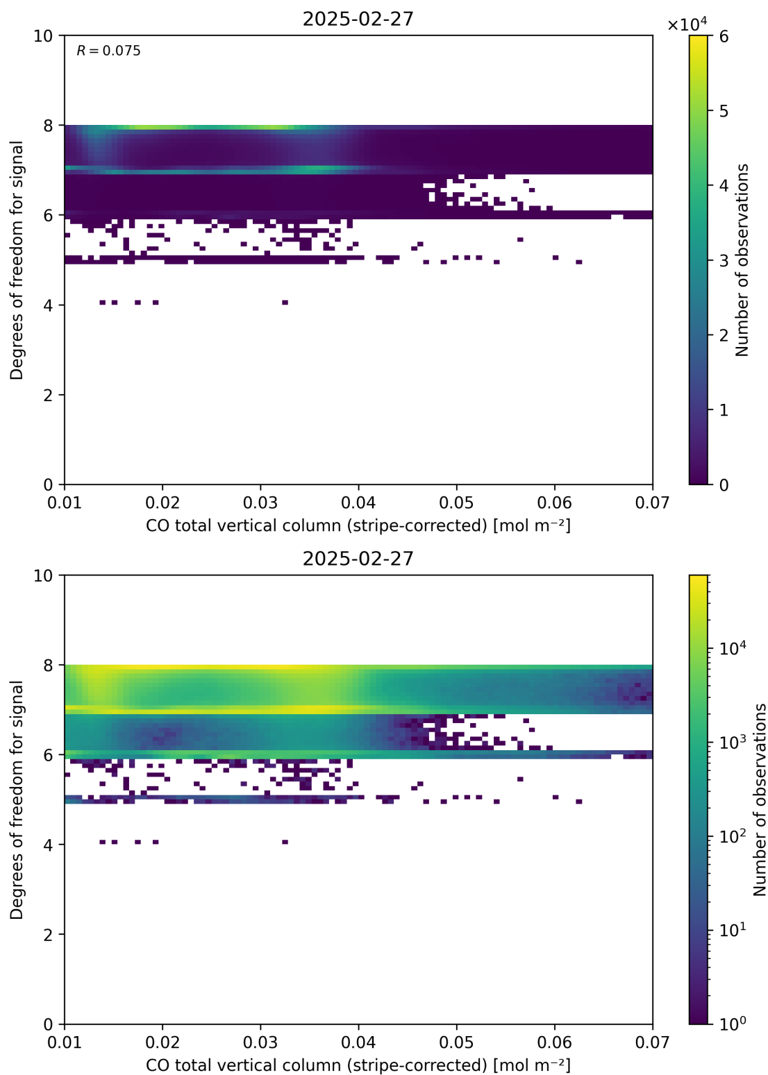
Figure 38: Scatter density plot of “CO total vertical column (stripe-corrected)” against “Degrees of freedom for signal” for 2025-02-26 to 2025-02-28.
