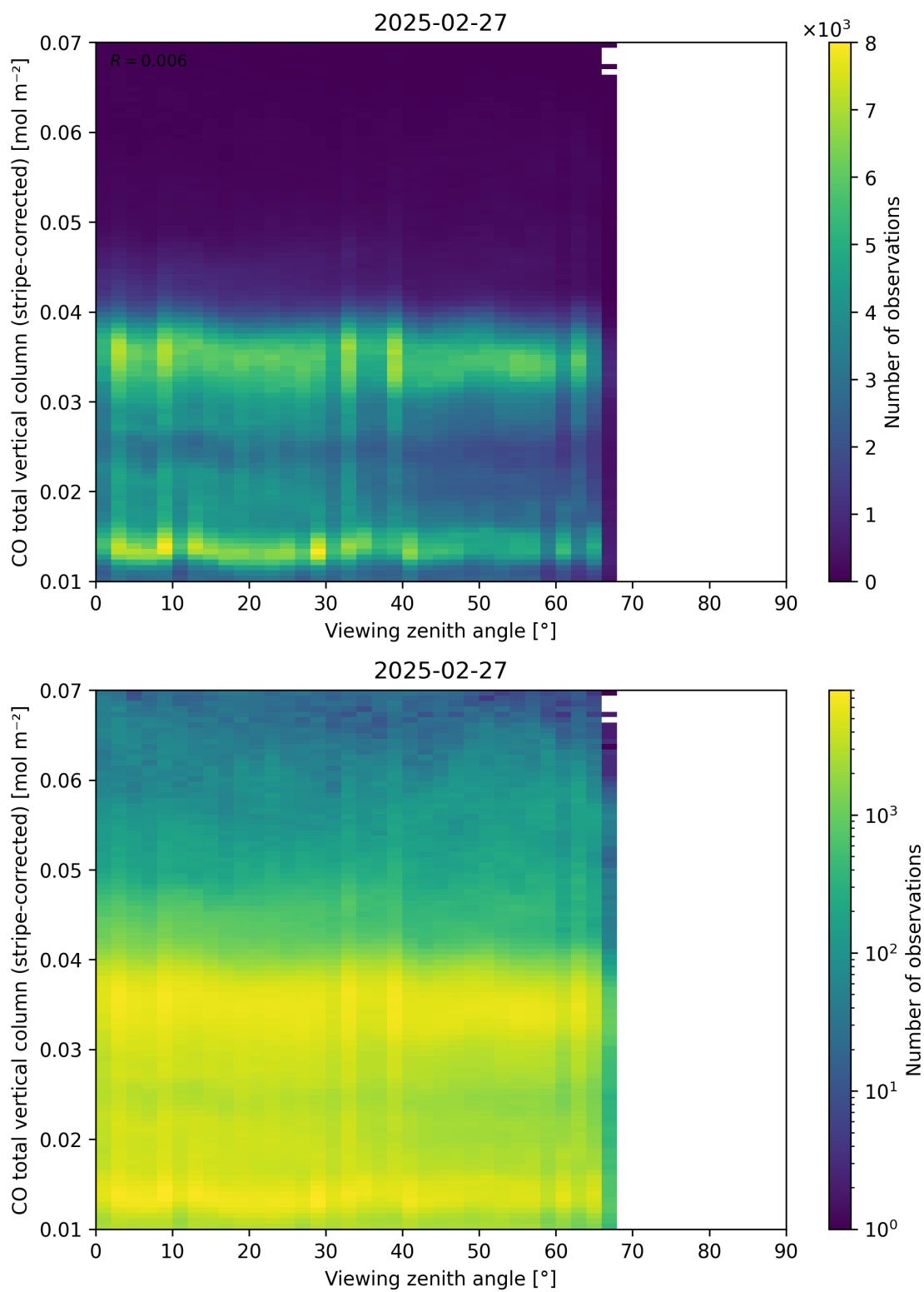
Figure 70: Scatter density plot of “Viewing zenith angle” against “CO total vertical column (stripe-corrected)” for 2025-02-26 to 2025-02-28.
