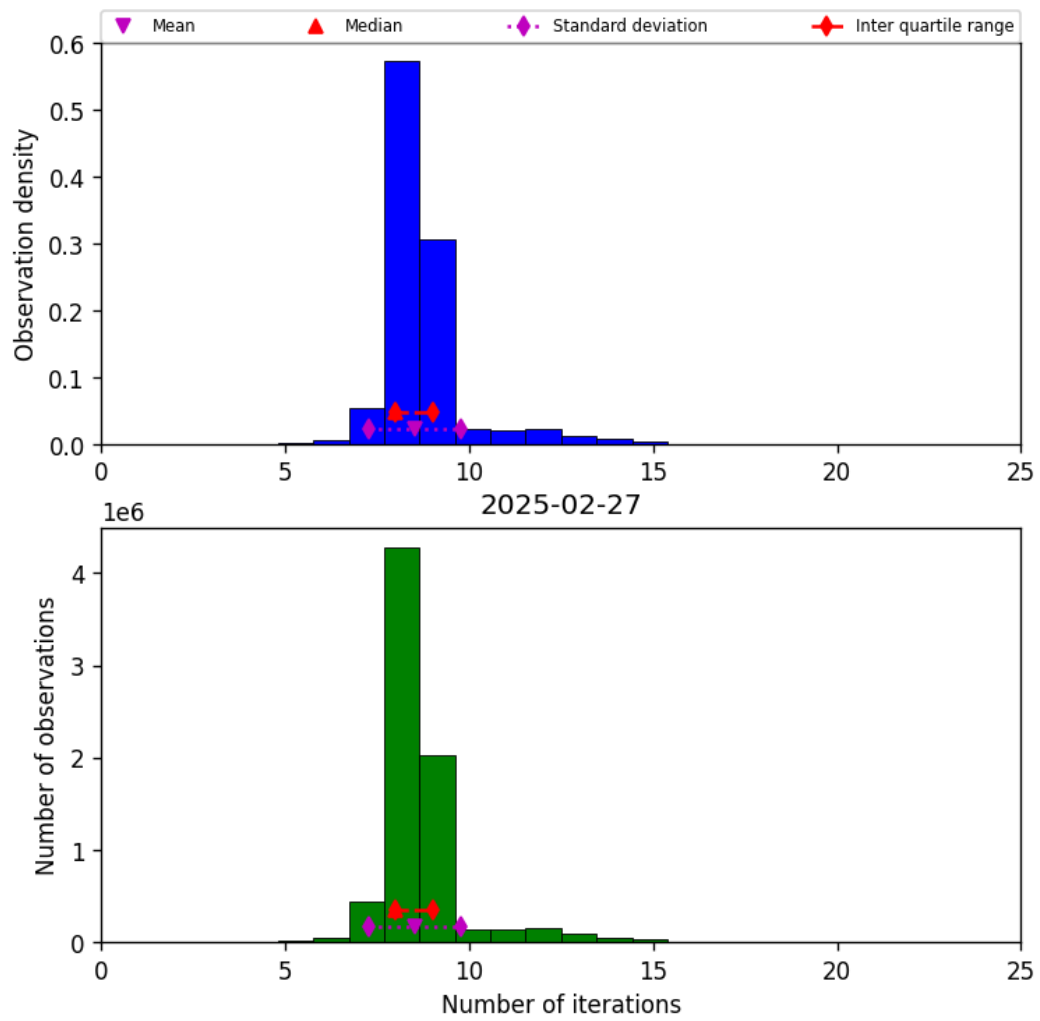
Figure 24: Histogram of “Number of iterations” for 2025-02-26 to 2025-02-28
