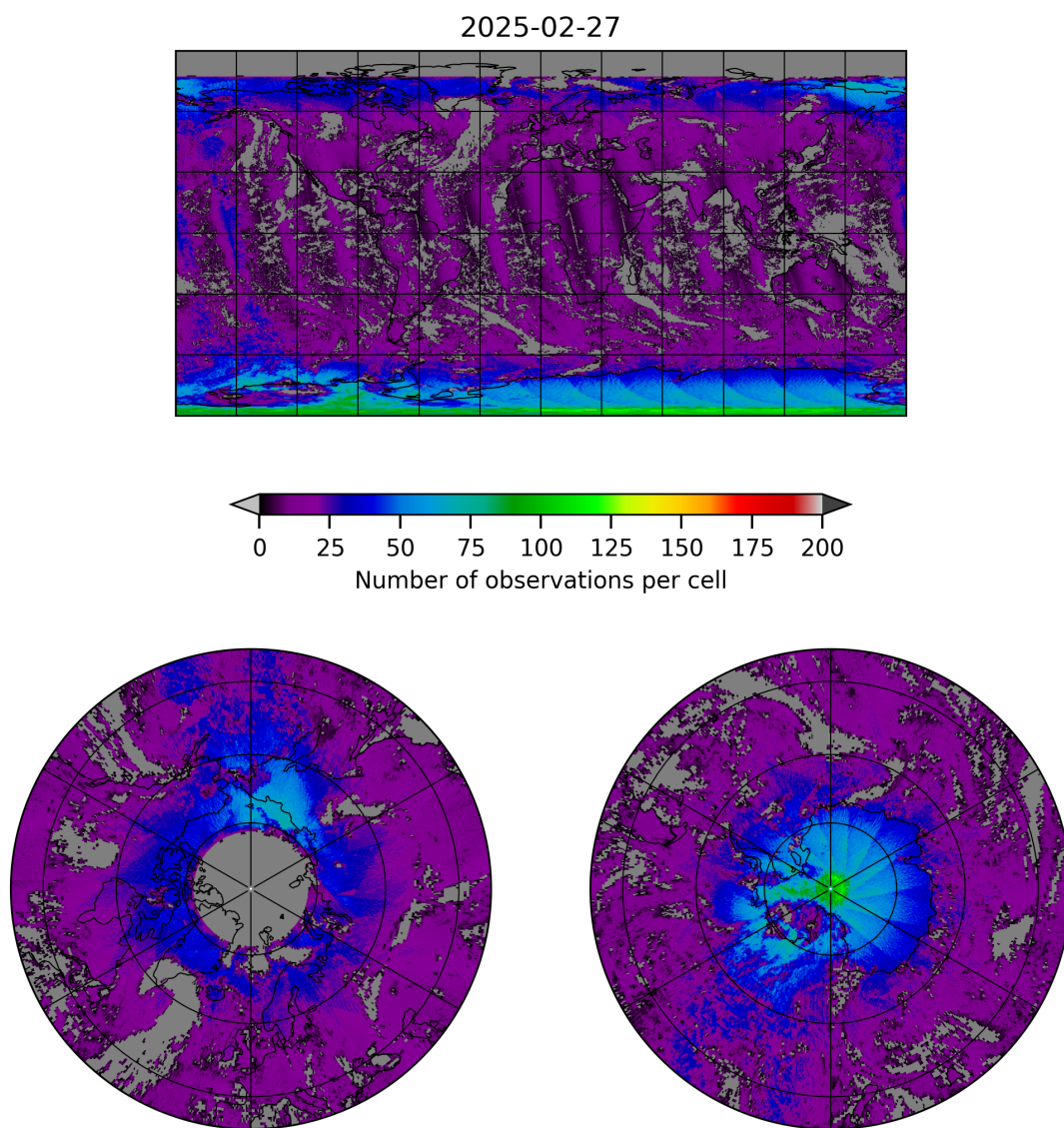
Figure 8: Map of the number of observations for 2025-02-26 to 2025-02-28
