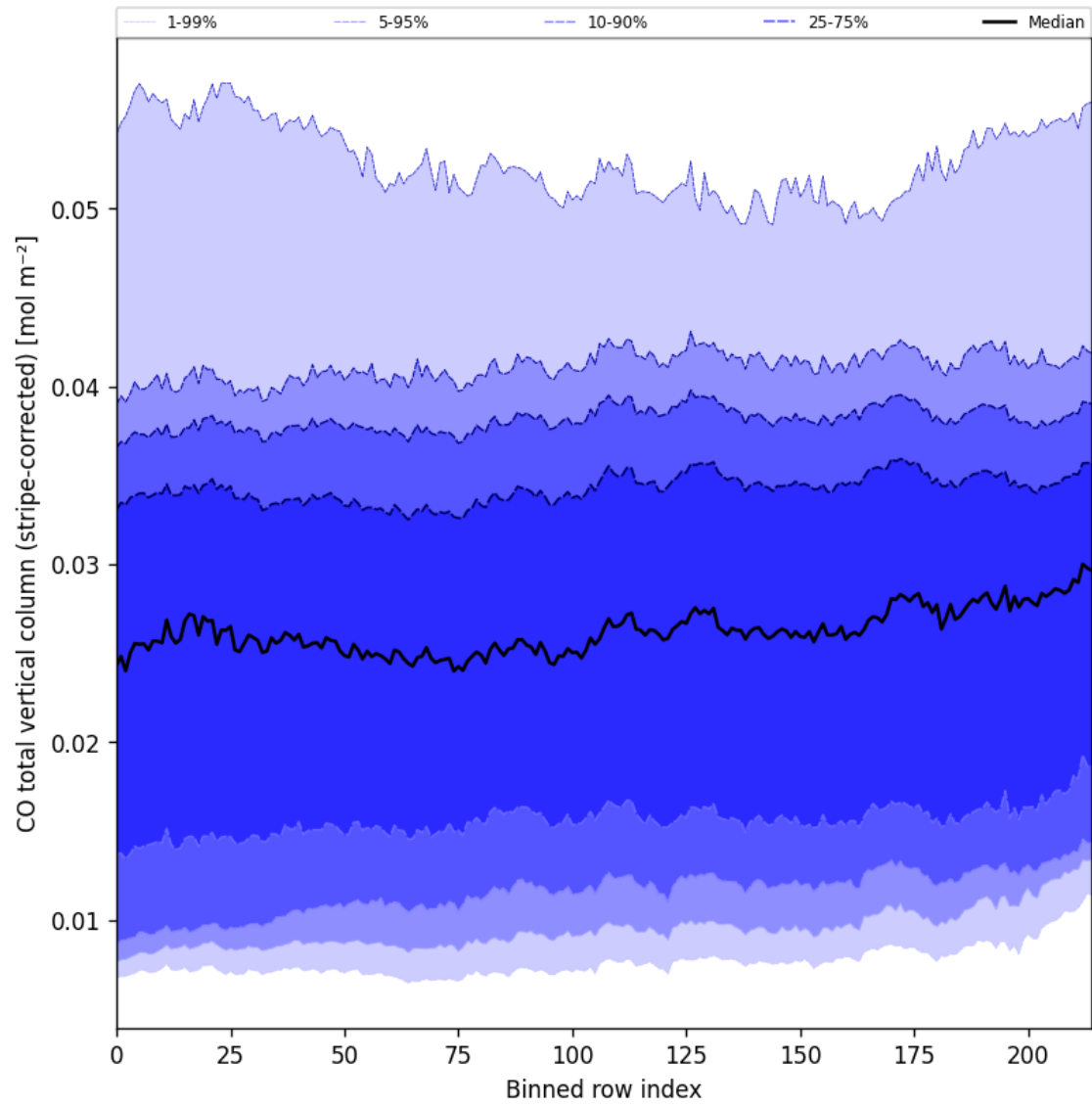
Figure 27: Along track statistics of “CO total vertical column (stripe-corrected)” for 2025-02-26 to 2025-02-28
