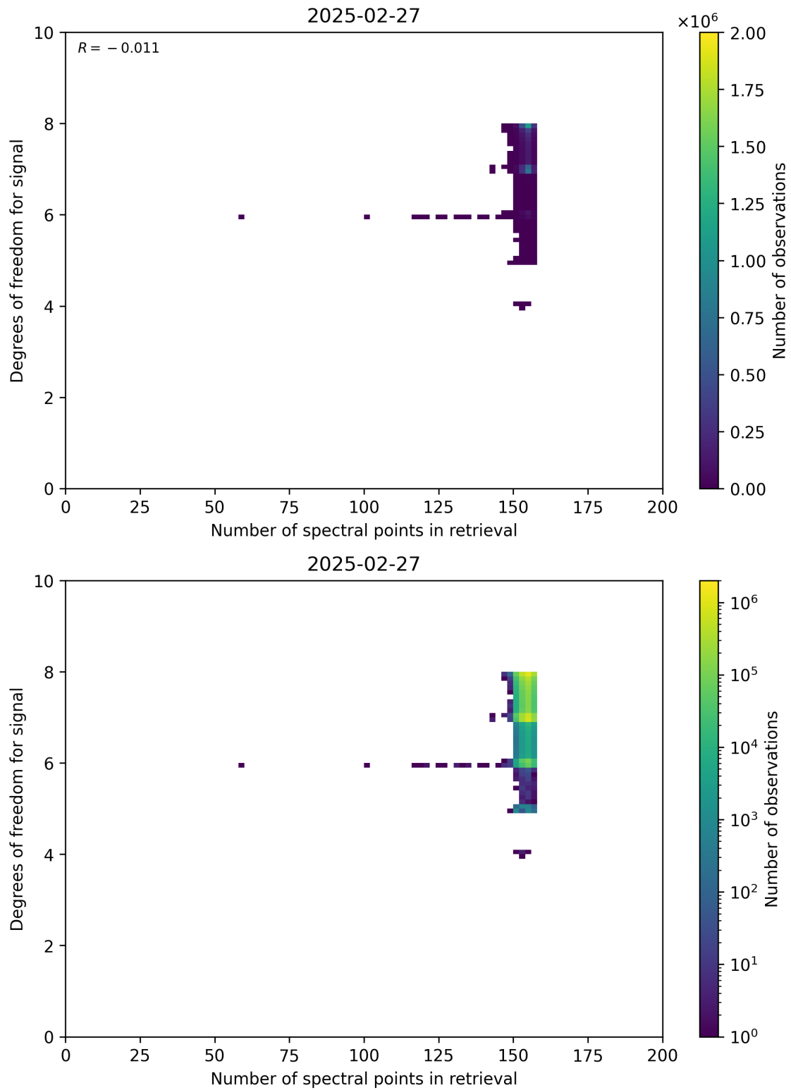
Figure 59: Scatter density plot of “Number of spectral points in retrieval” against “Degrees of freedom for signal” for 2025-02-26 to 2025-02-28.
