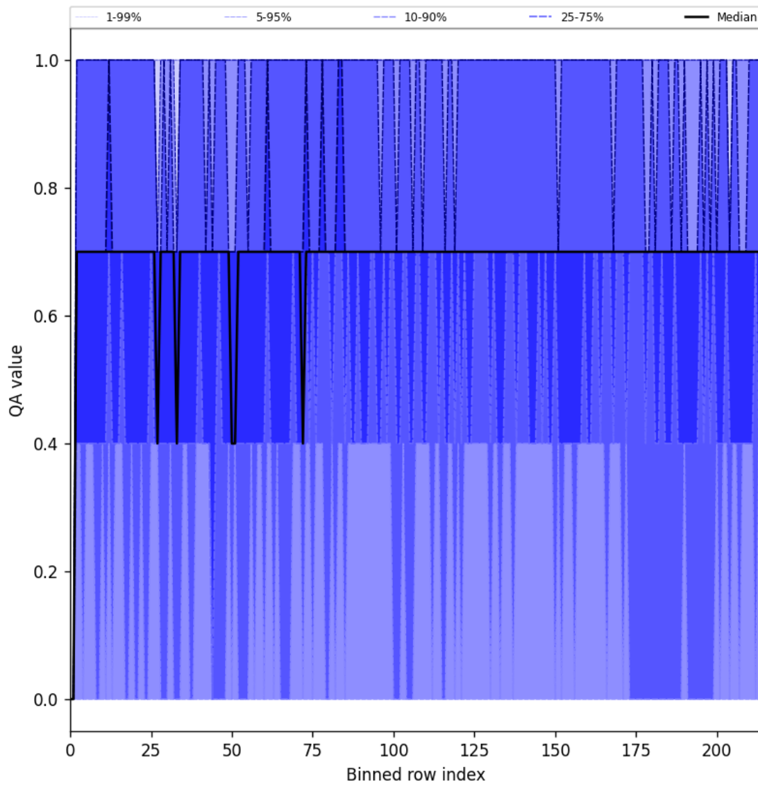
Figure 25: Along track statistics of “QA value” for 2025-02-26 to 2025-02-28
