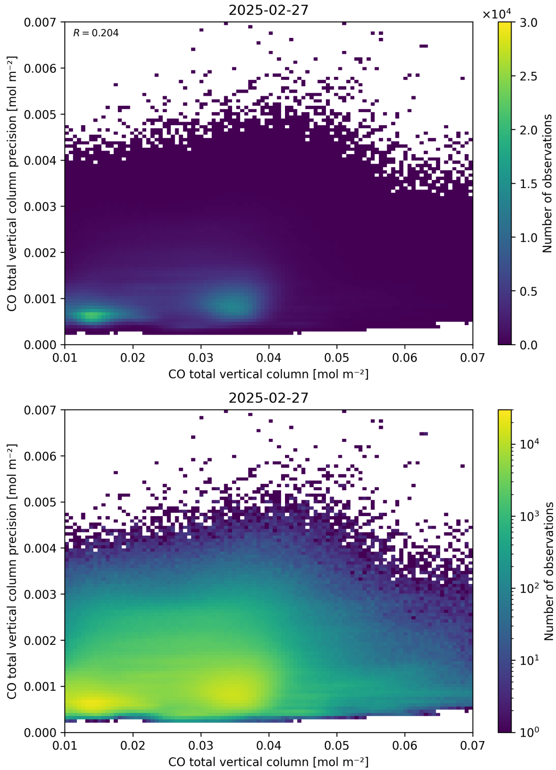
Figure 34: Scatter density plot of “CO total vertical column” against “CO total vertical column precision” for 2025-02-26 to 2025-02-28.
