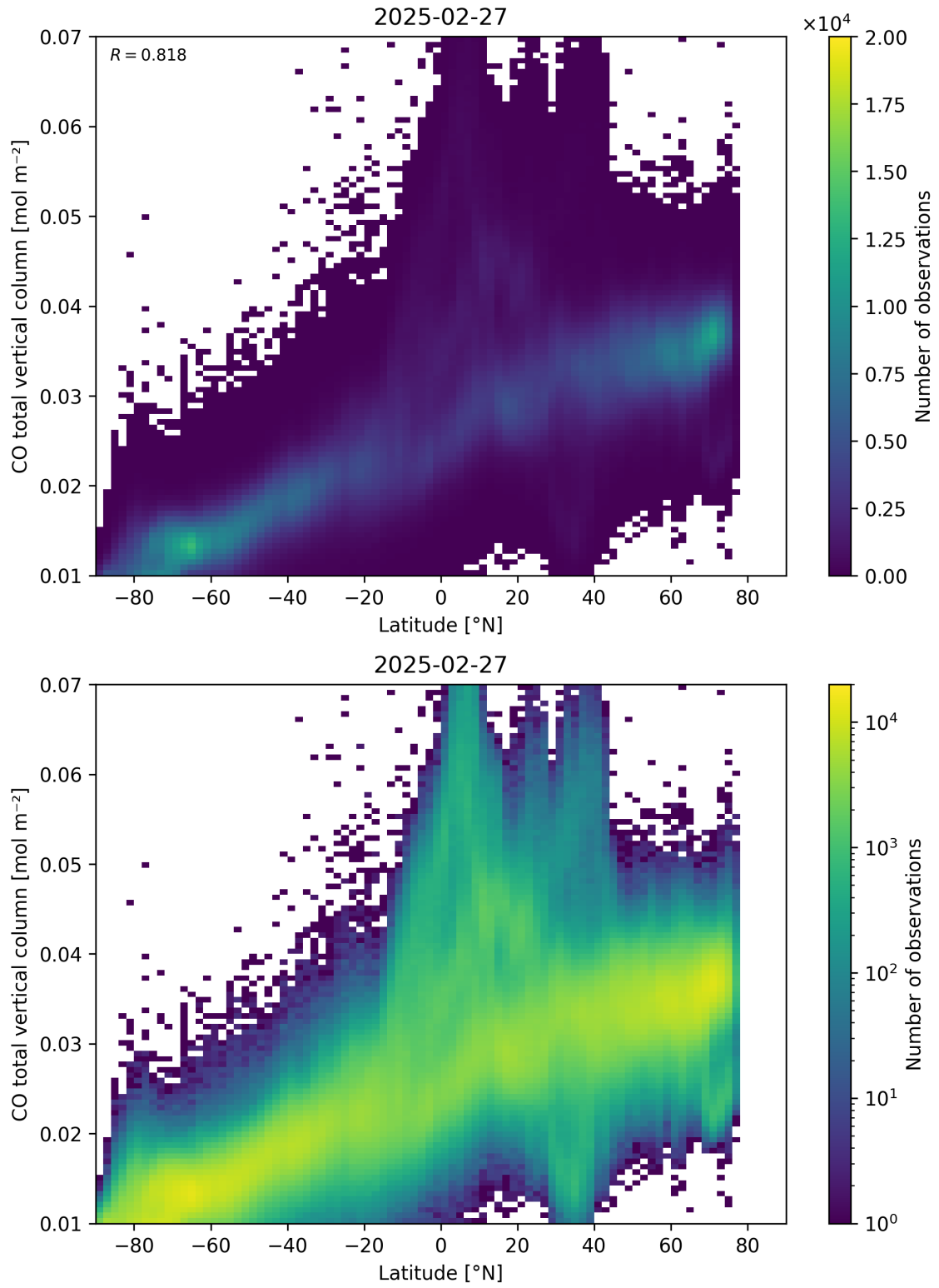
Figure 51: Scatter density plot of “Latitude” against “CO total vertical column” for 2025-02-26 to 2025-02-28.
