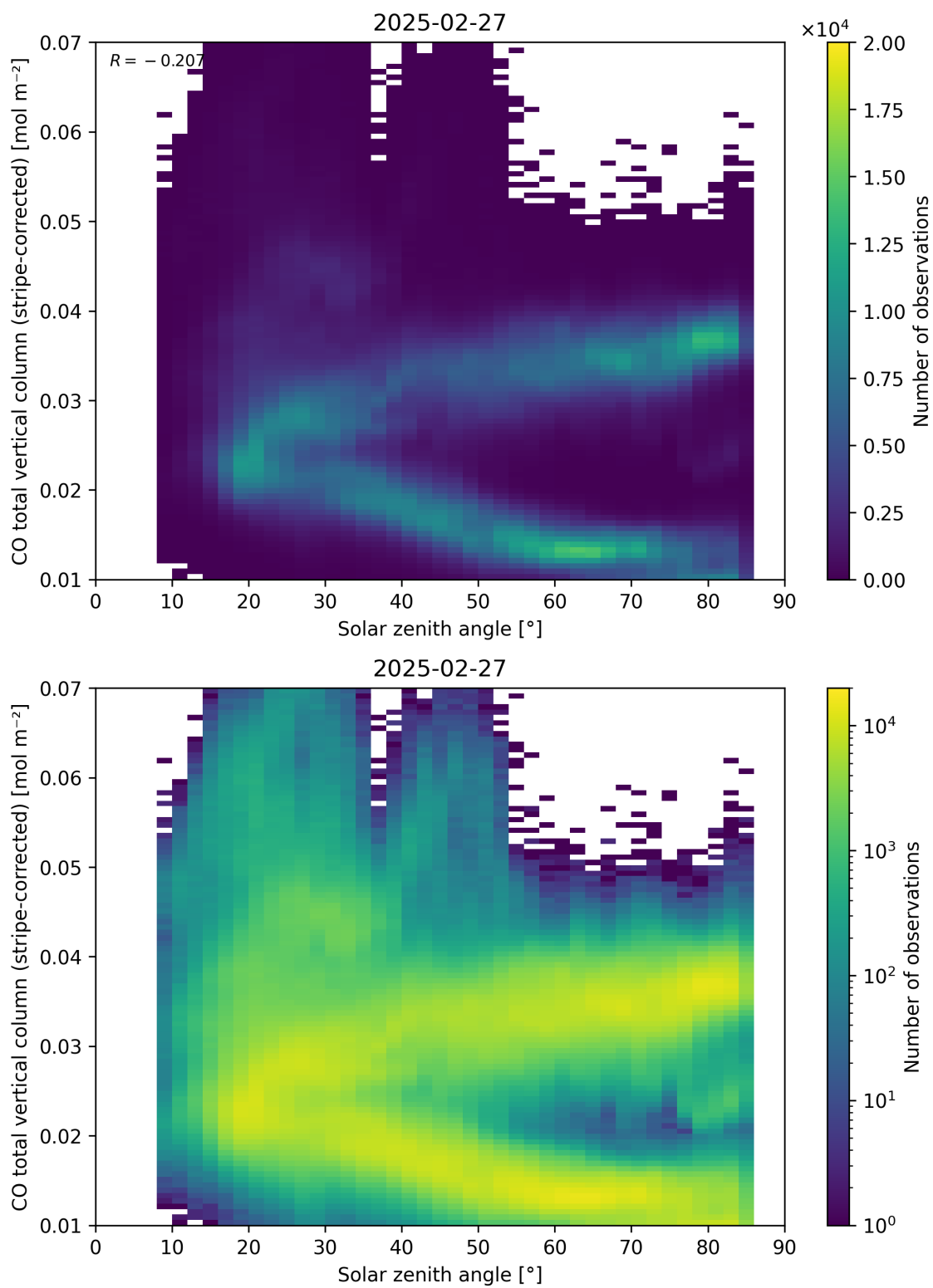
Figure 62: Scatter density plot of “Solar zenith angle” against “CO total vertical column (stripe-corrected)” for 2025-02-26 to 2025-02-28.
