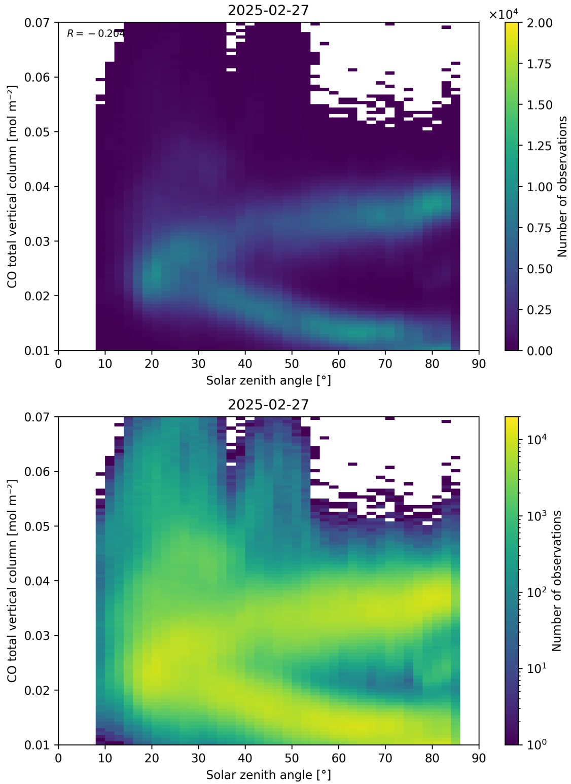
Figure 61: Scatter density plot of “Solar zenith angle” against “CO total vertical column” for 2025-02-26 to 2025-02-28.
