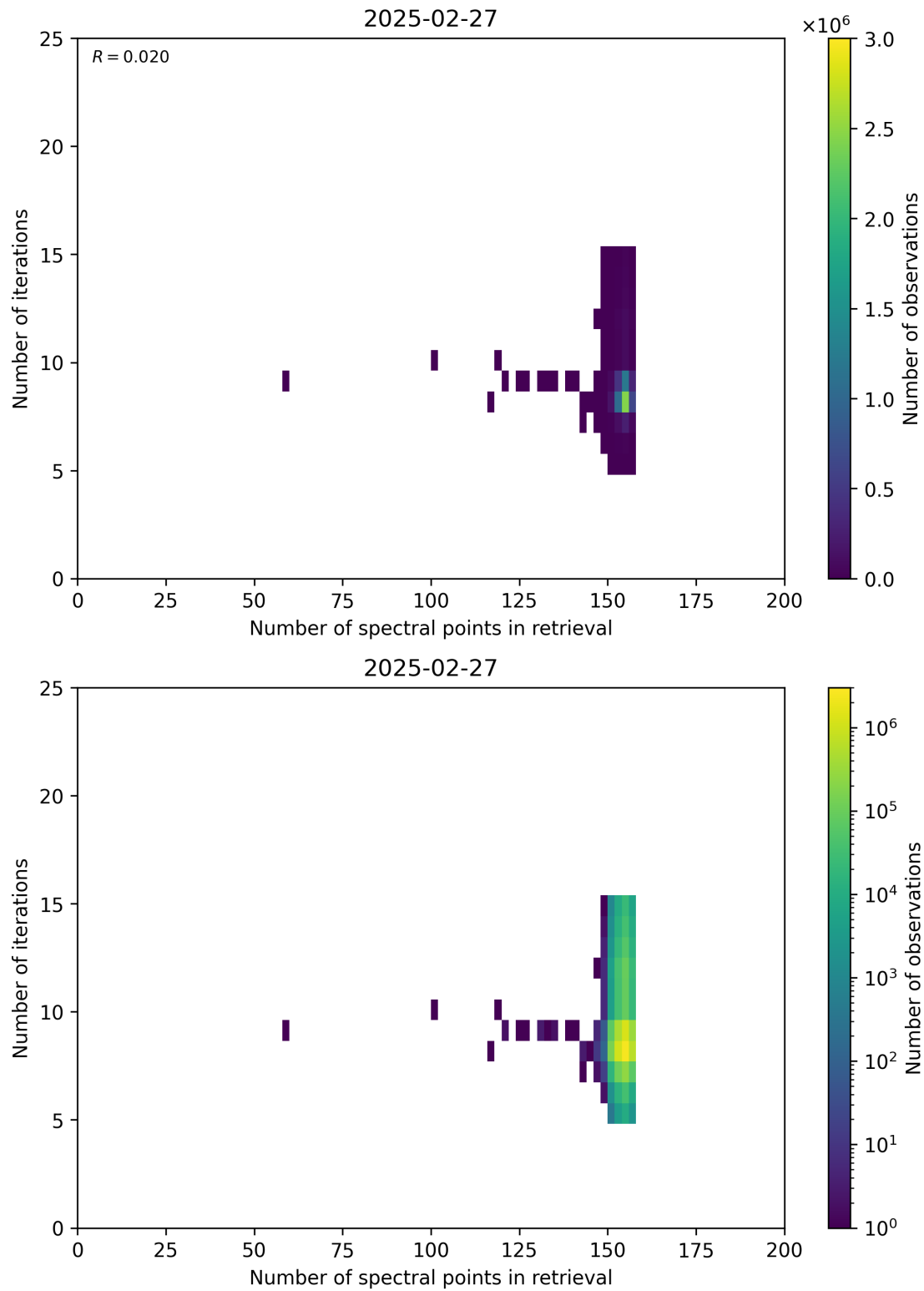
Figure 60: Scatter density plot of “Number of spectral points in retrieval” against “Number of iterations” for 2025-02-26 to 2025-02-28.
