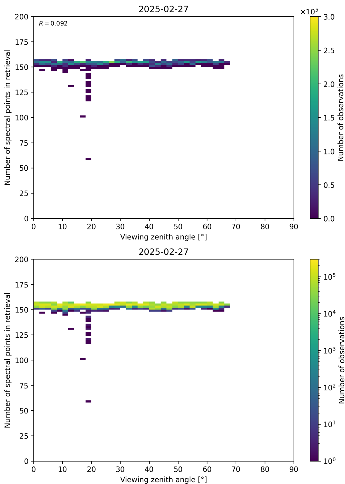
Figure 76: Scatter density plot of “Viewing zenith angle” against “Number of spectral points in retrieval” for 2025-02-26 to 2025-02-28.
