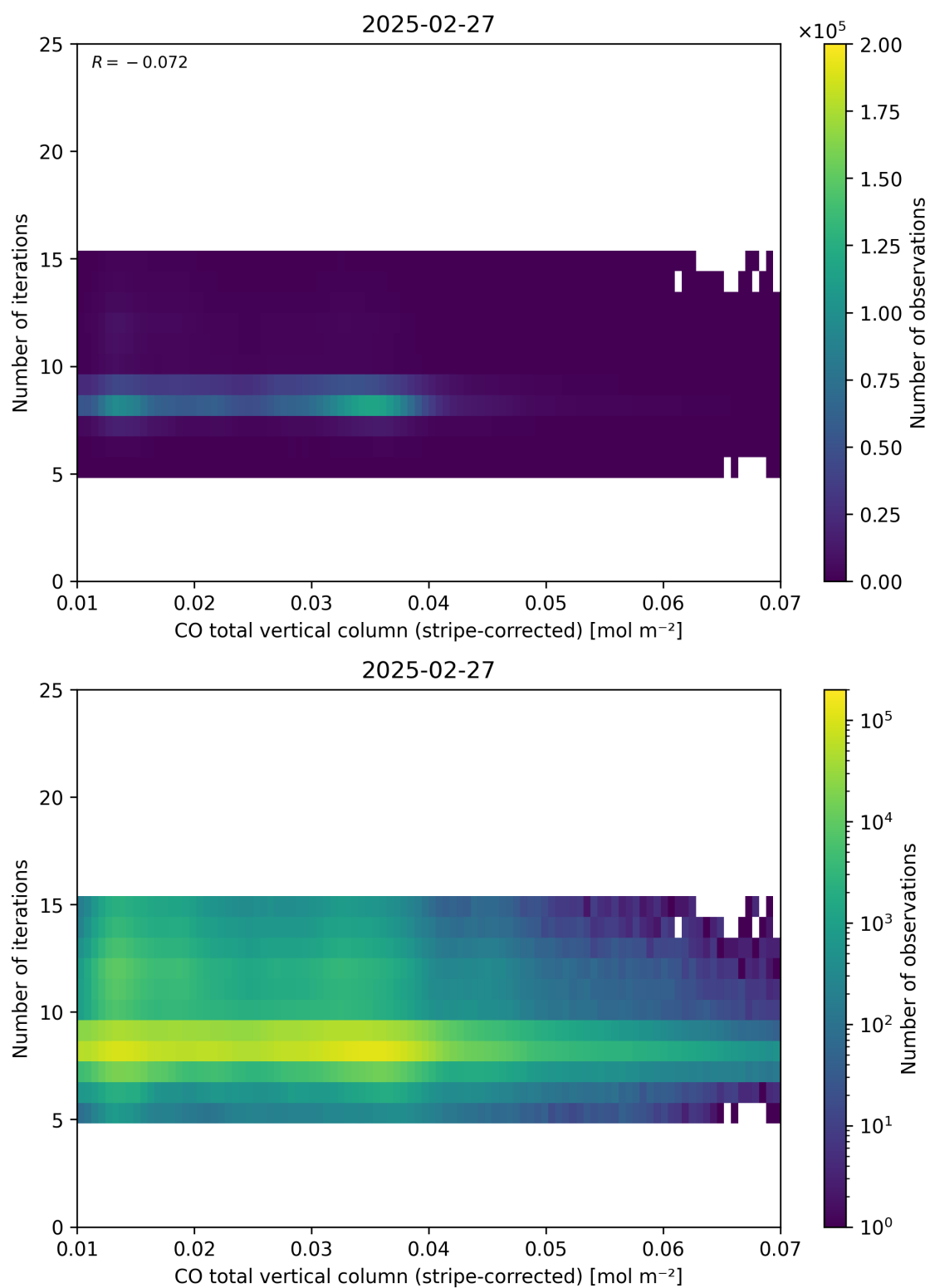
Figure 39: Scatter density plot of “CO total vertical column (stripe-corrected)” against “Number of iterations” for 2025-02-26 to 2025-02-28.
