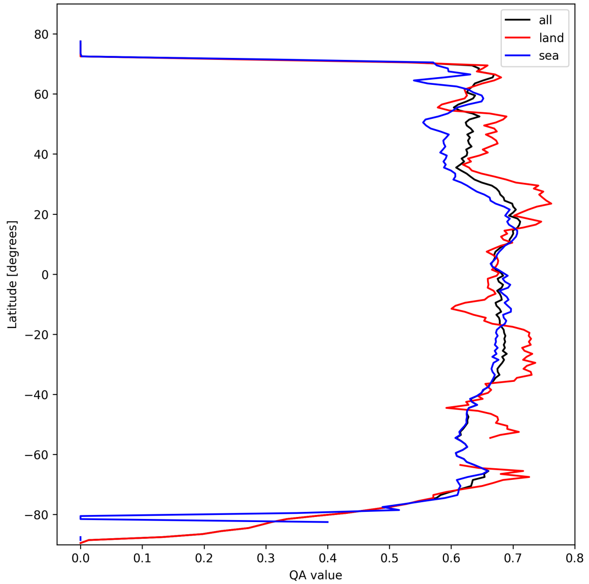
Figure 9: Zonal average of “QA value” for 2025-02-26 to 2025-02-28.
