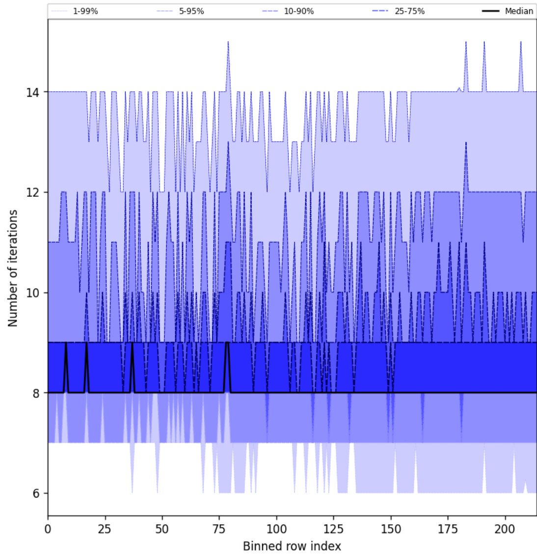
Figure 32: Along track statistics of “Number of iterations” for 2025-02-26 to 2025-02-28
