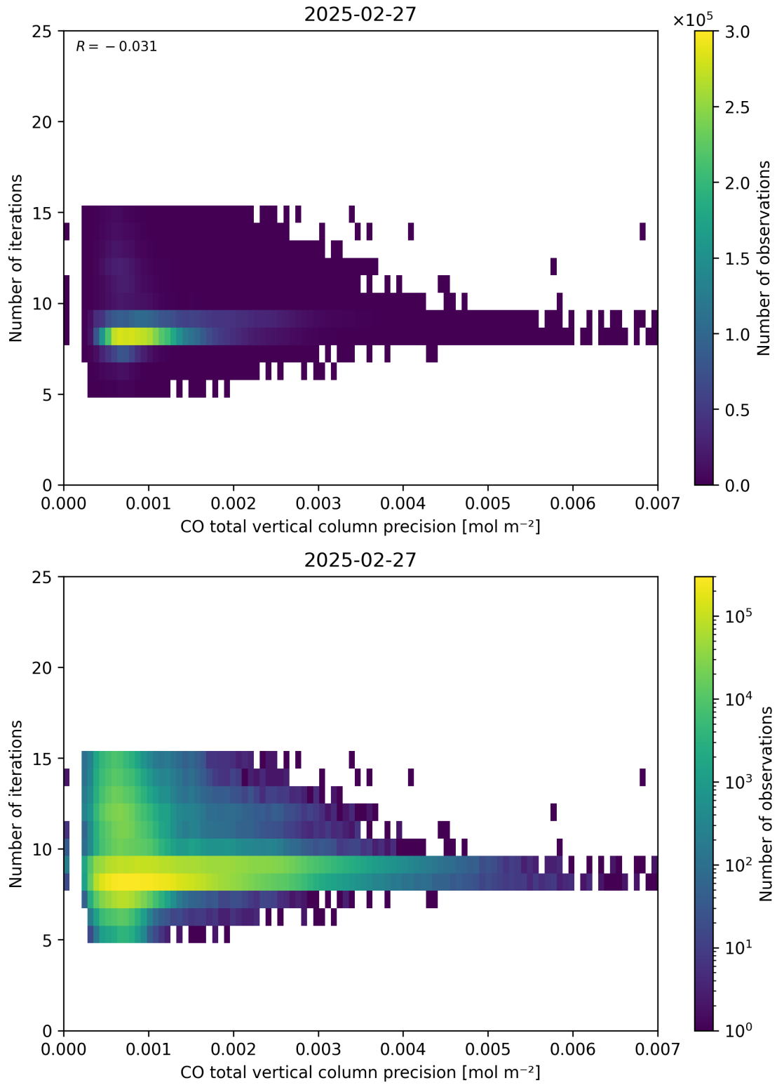
Figure 46: Scatter density plot of “CO total vertical column precision” against “Number of iterations” for 2025-02-26 to 2025-02-28.
