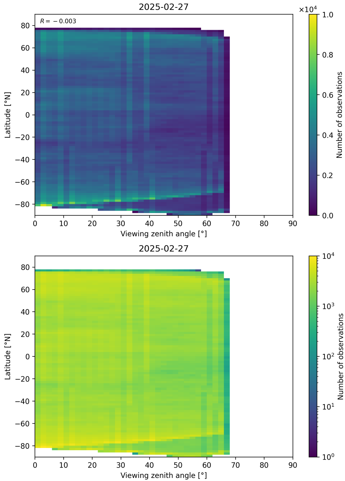
Figure 74: Scatter density plot of “Viewing zenith angle” against “Latitude” for 2025-02-26 to 2025-02-28.
