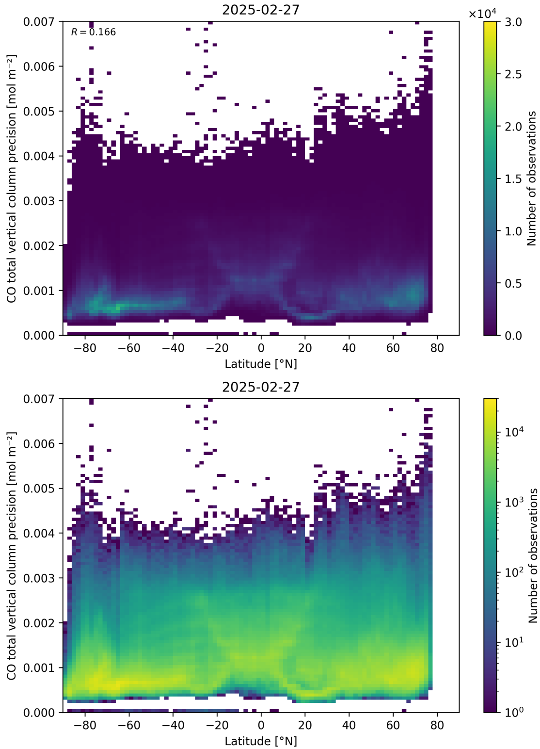
Figure 53: Scatter density plot of “Latitude” against “CO total vertical column precision” for 2025-02-26 to 2025-02-28.
