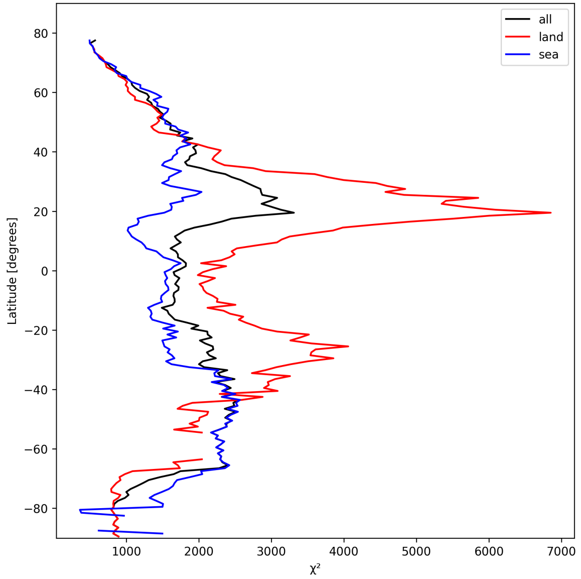
Figure 14: Zonal average of “ \chi^2 ” for 2025-02-26 to 2025-02-28.
