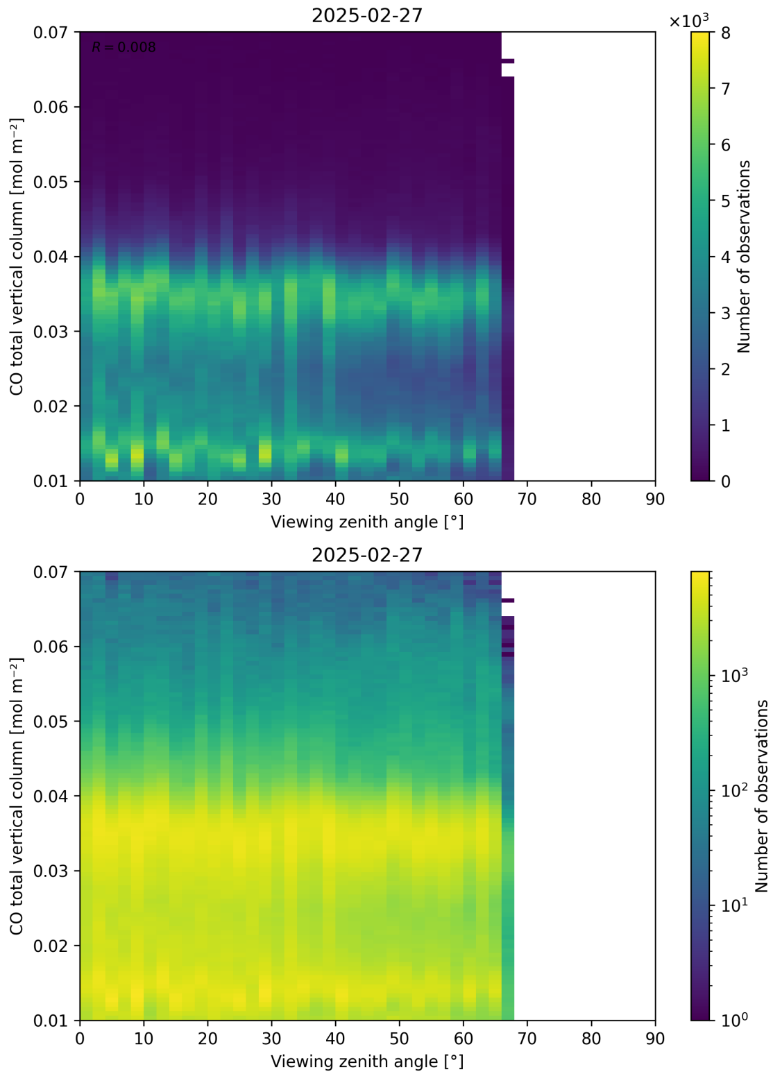
Figure 69: Scatter density plot of “Viewing zenith angle” against “CO total vertical column” for 2025-02-26 to 2025-02-28.
