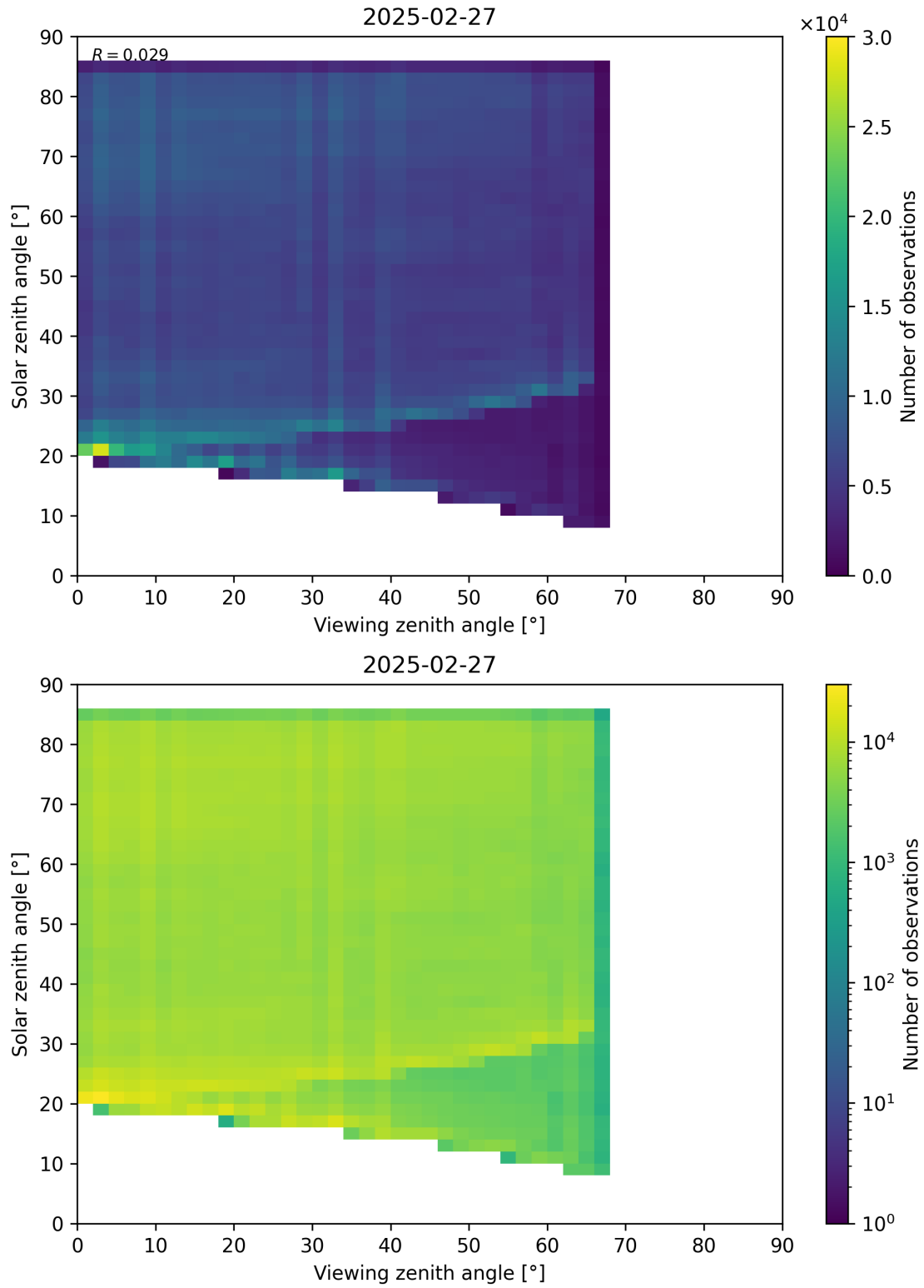
Figure 77: Scatter density plot of “Viewing zenith angle” against “Solar zenith angle” for 2025-02-26 to 2025-02-28.
