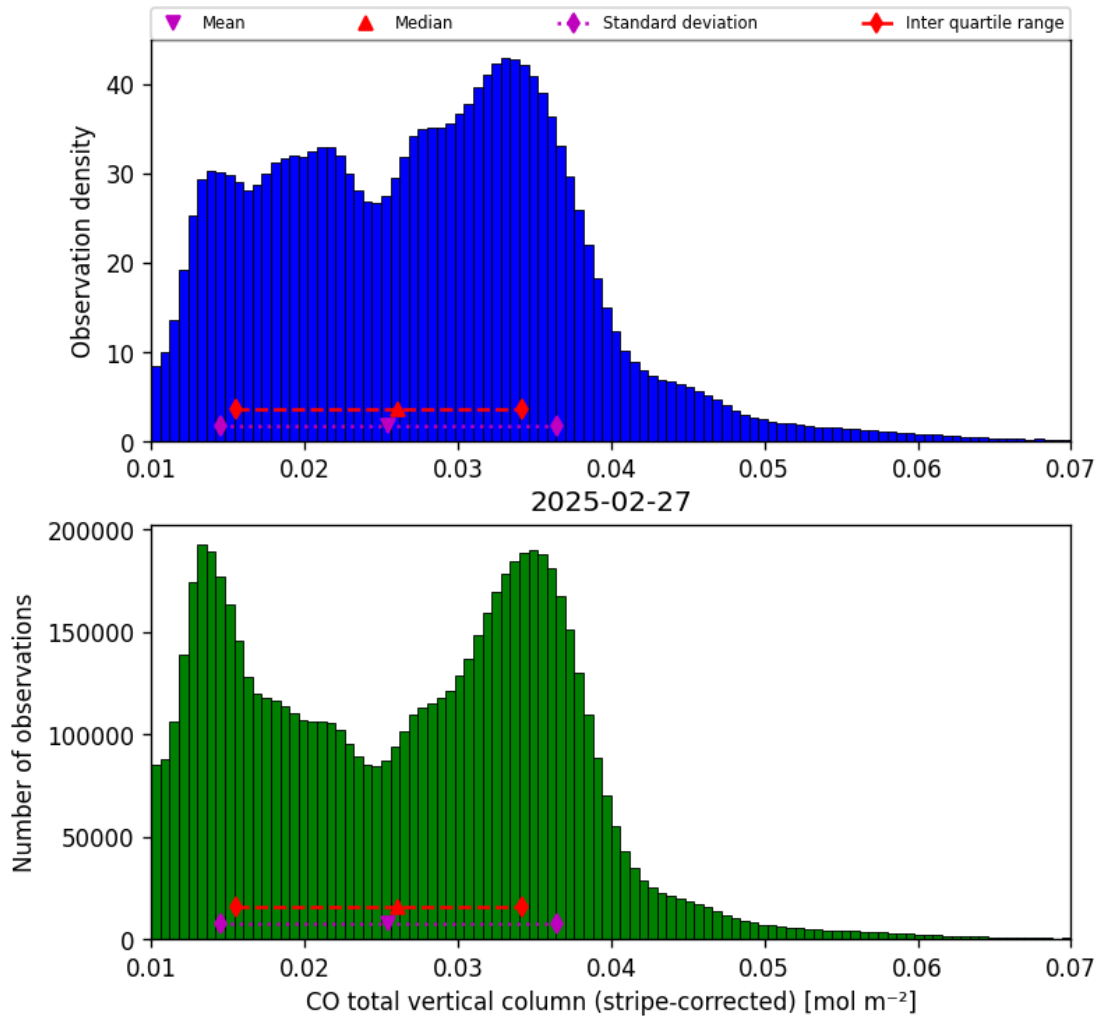
Figure 19: Histogram of “CO total vertical column (stripe-corrected)” for 2025-02-26 to 2025-02-28
