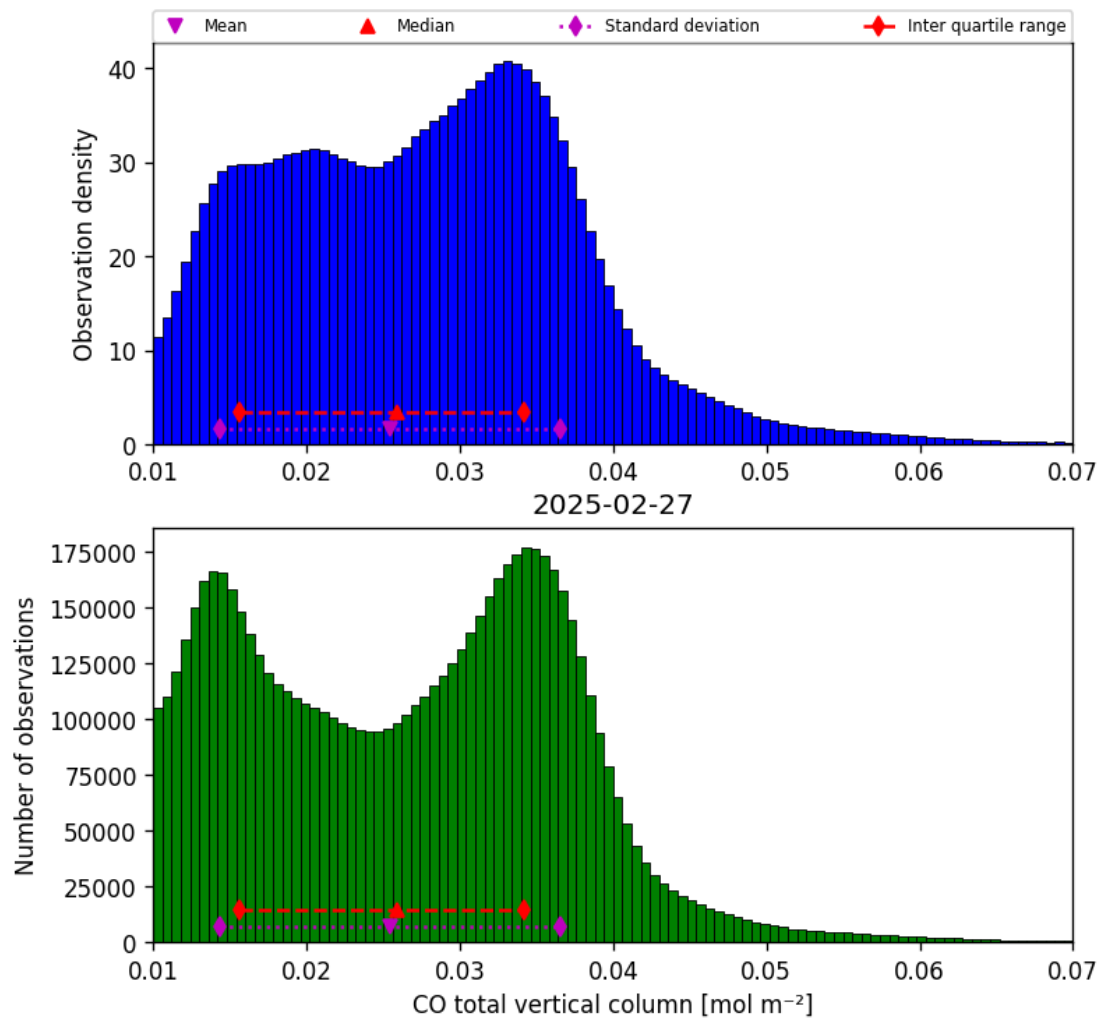
Figure 18: Histogram of “CO total vertical column” for 2025-02-26 to 2025-02-28
