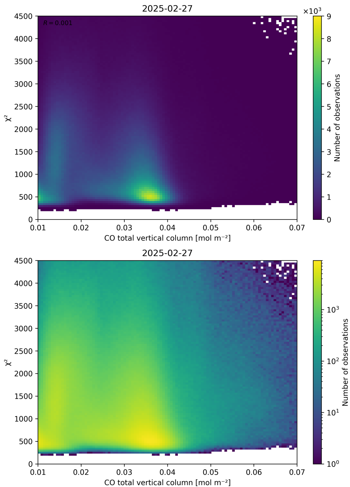
Figure 35: Scatter density plot of “CO total vertical column” against “ \chi^2 ” for 2025-02-26 to 2025-02-28.
