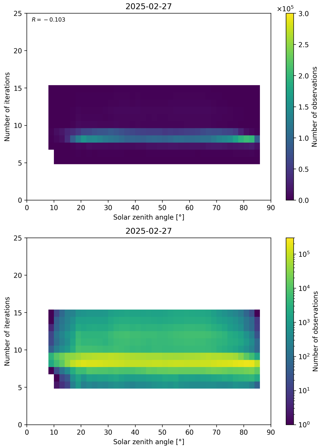
Figure 67: Scatter density plot of “Solar zenith angle” against “Number of iterations” for 2025-02-26 to 2025-02-28.
