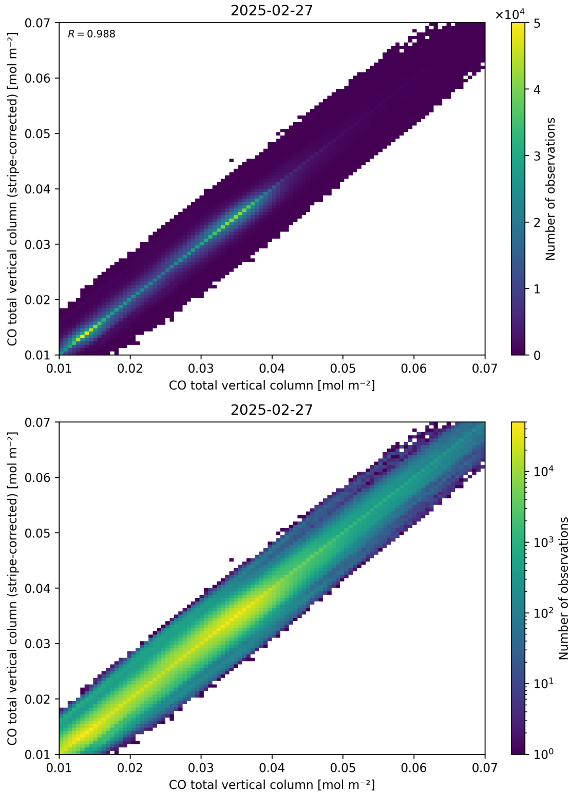
Figure 33: Scatter density plot of “CO total vertical column” against “CO total vertical column (stripe-corrected)” for 2025-02-26 to 2025-02-28.
