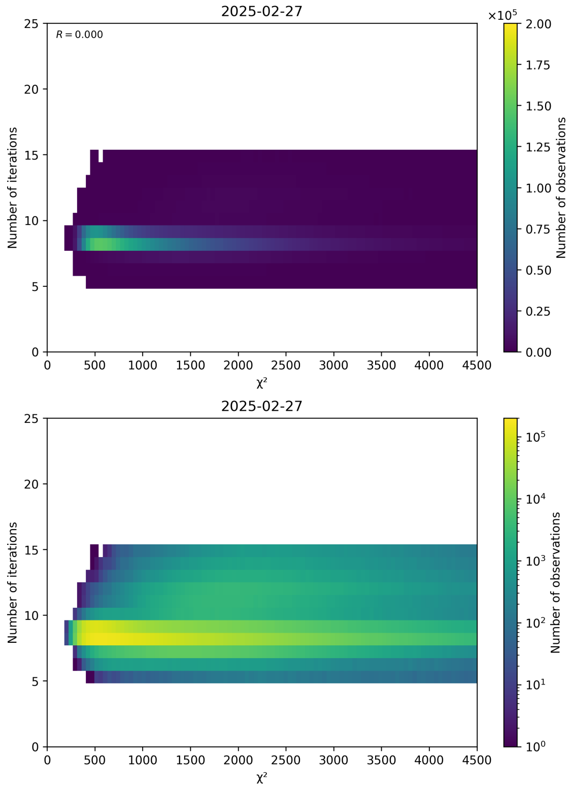
Figure 49: Scatter density plot of “ \chi^2 ” against “Number of iterations” for 2025-02-26 to 2025-02-28.
