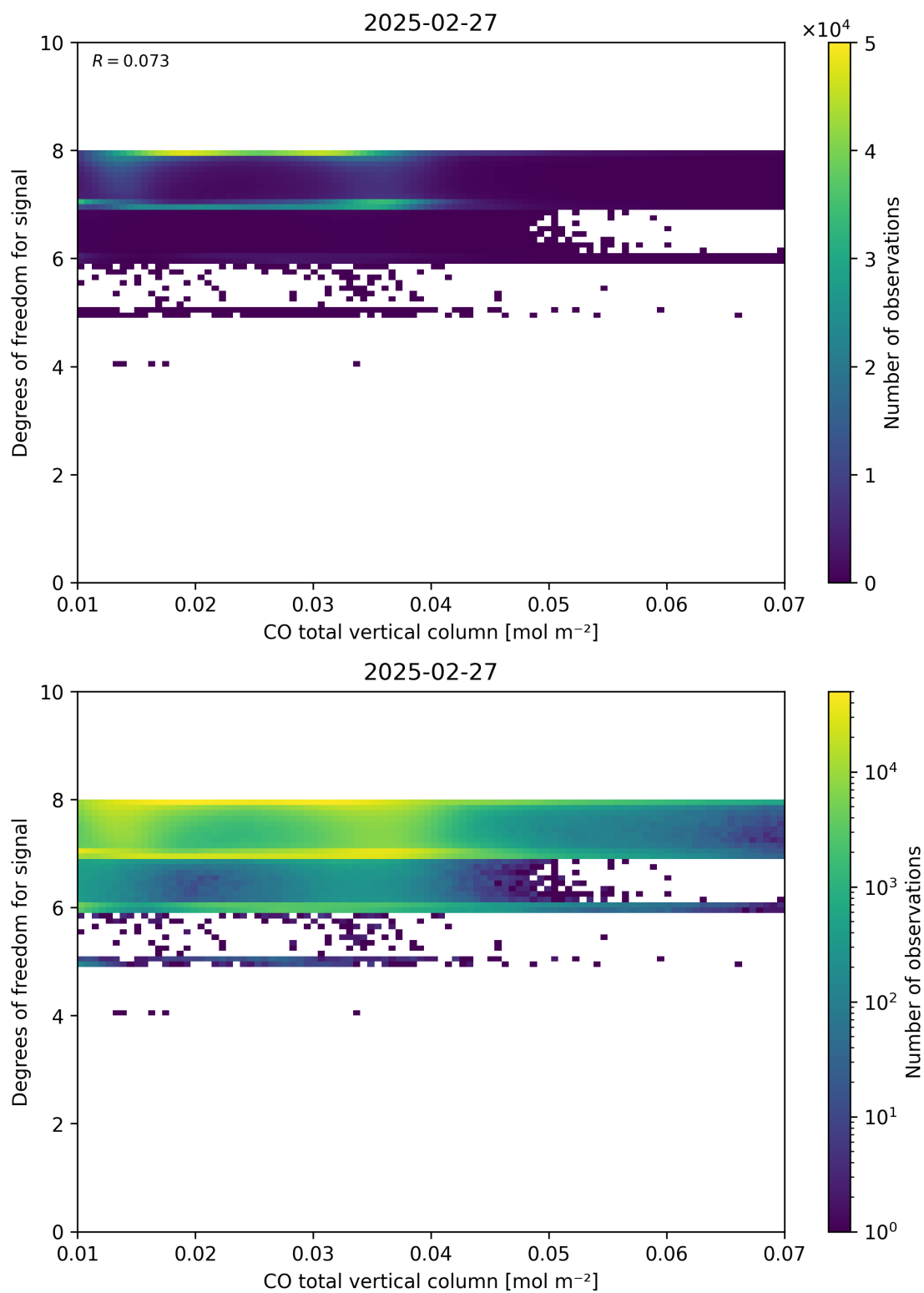
Figure 41: Scatter density plot of “CO total vertical column” against “Degrees of freedom for signal” for 2025-02-26 to 2025-02-28.
