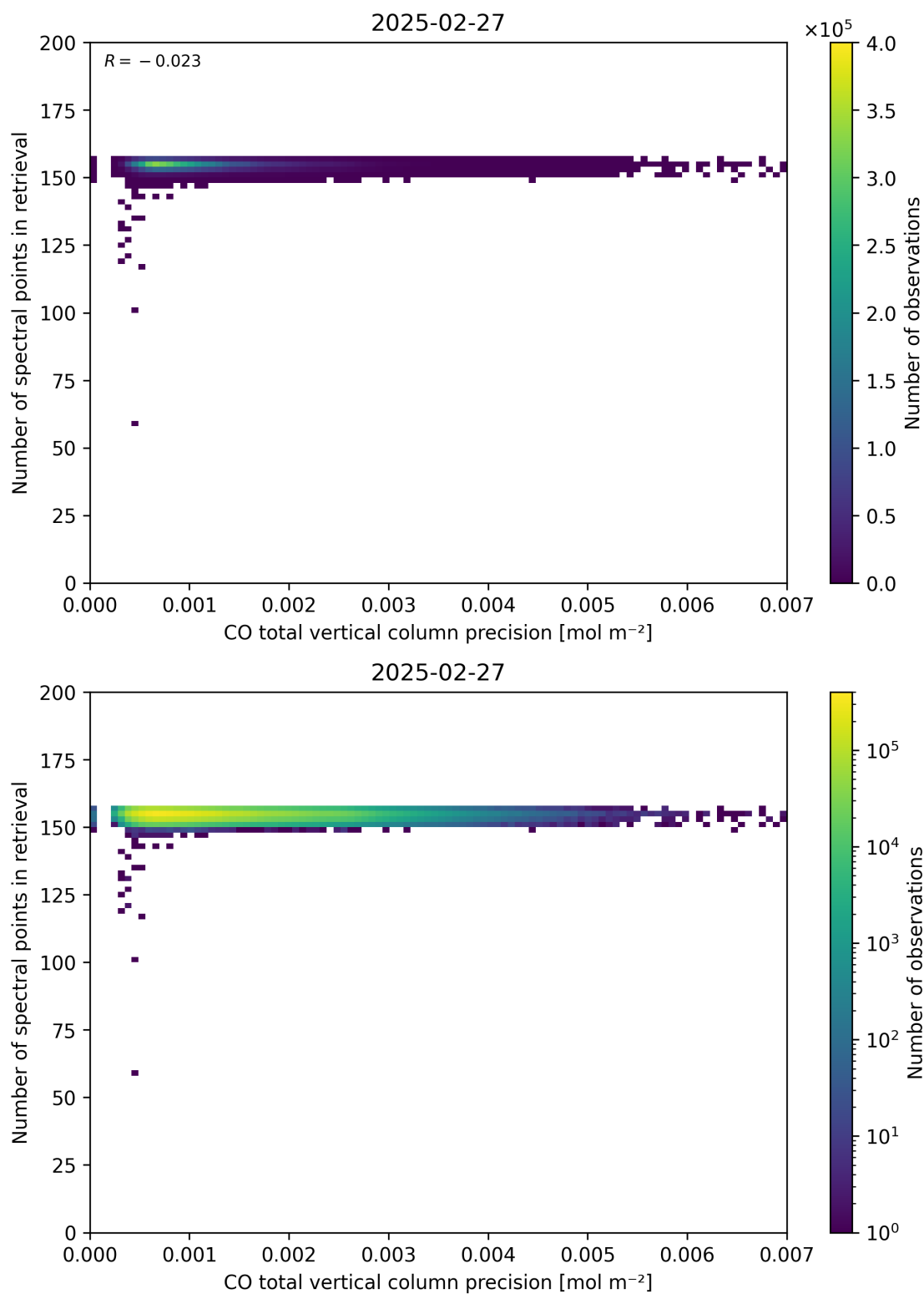
Figure 47: Scatter density plot of “CO total vertical column precision” against “Number of spectral points in retrieval” for 2025-02-26 to 2025-02-28.
