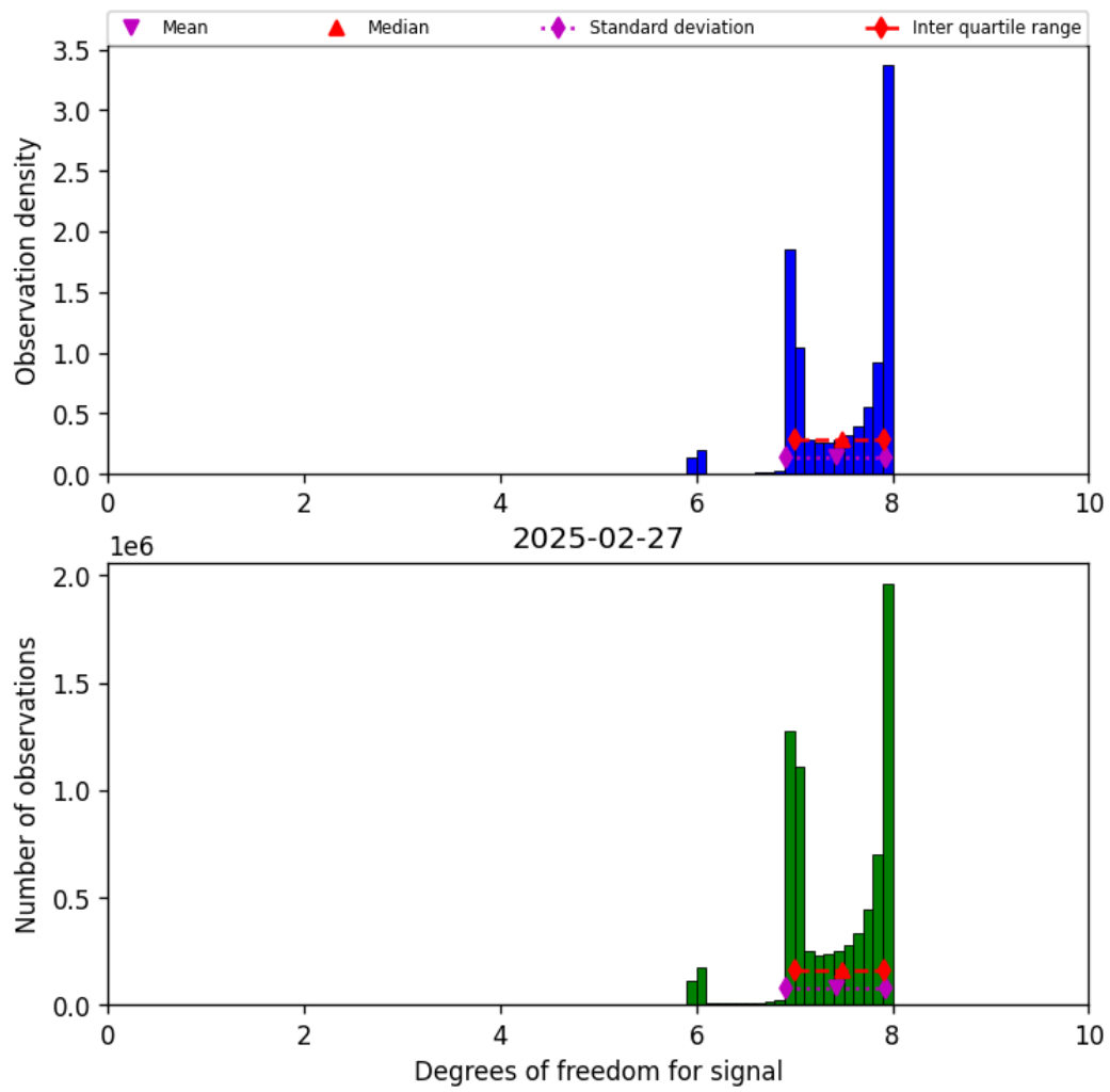
Figure 23: Histogram of “Degrees of freedom for signal” for 2025-02-26 to 2025-02-28
