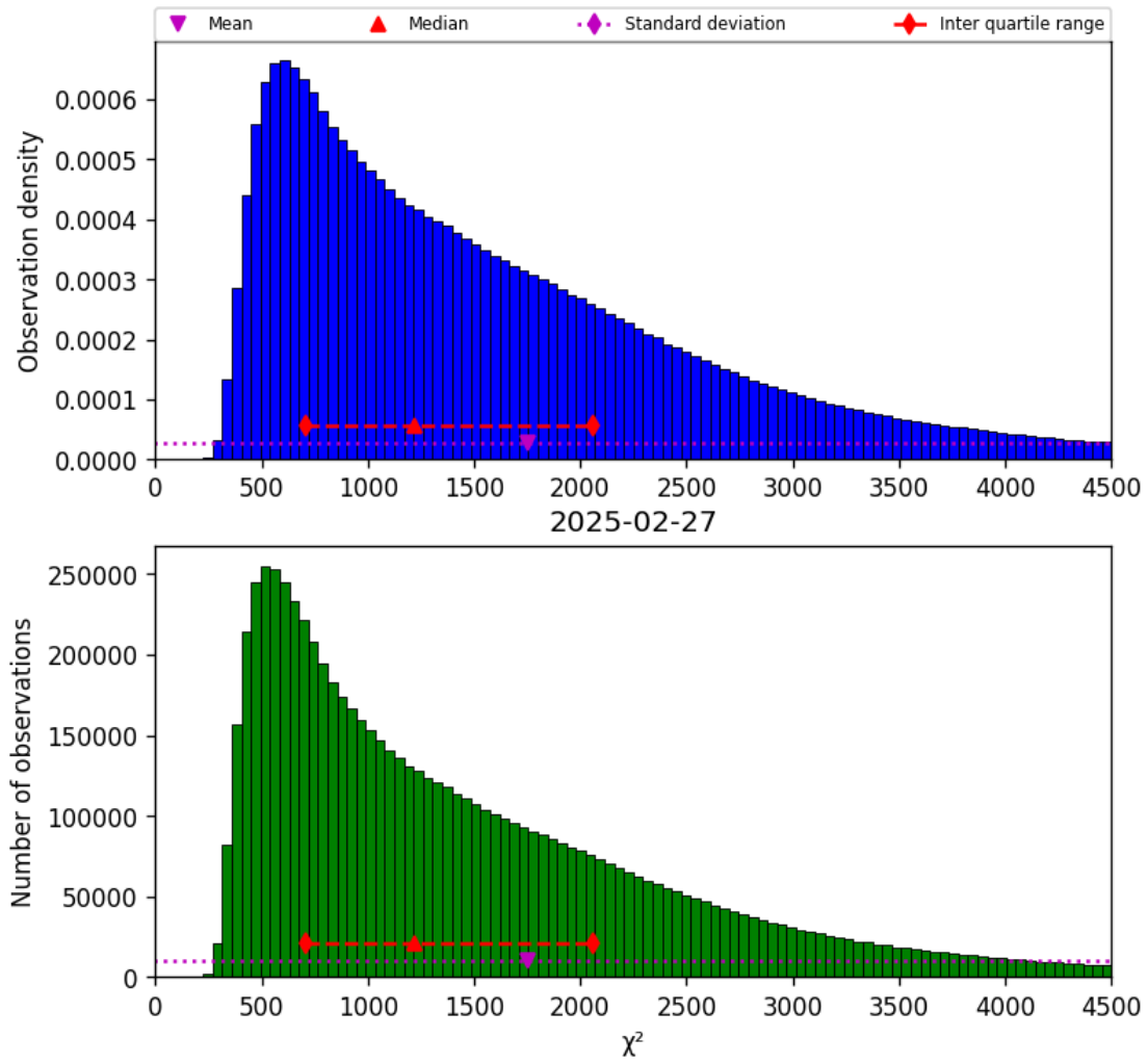
Figure 22: Histogram of “ \chi^2 ” for 2025-02-26 to 2025-02-28
