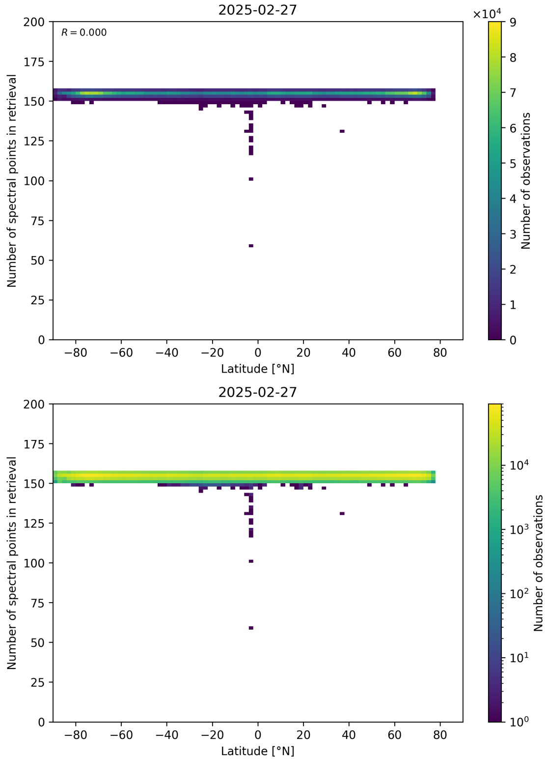
Figure 57: Scatter density plot of “Latitude” against “Number of spectral points in retrieval” for 2025-02-26 to 2025-02-28.
