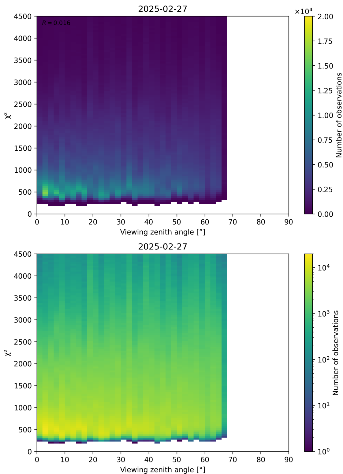
Figure 72: Scatter density plot of “Viewing zenith angle” against “ \chi^2 ” for 2025-02-26 to 2025-02-28.
