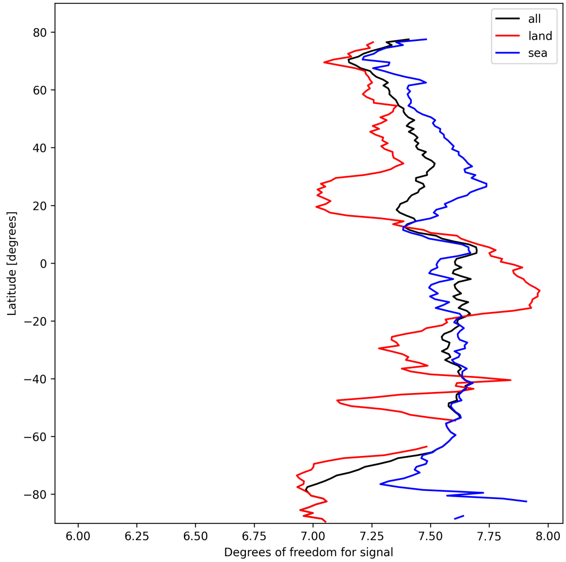
Figure 15: Zonal average of “Degrees of freedom for signal” for 2025-02-26 to 2025-02-28.
