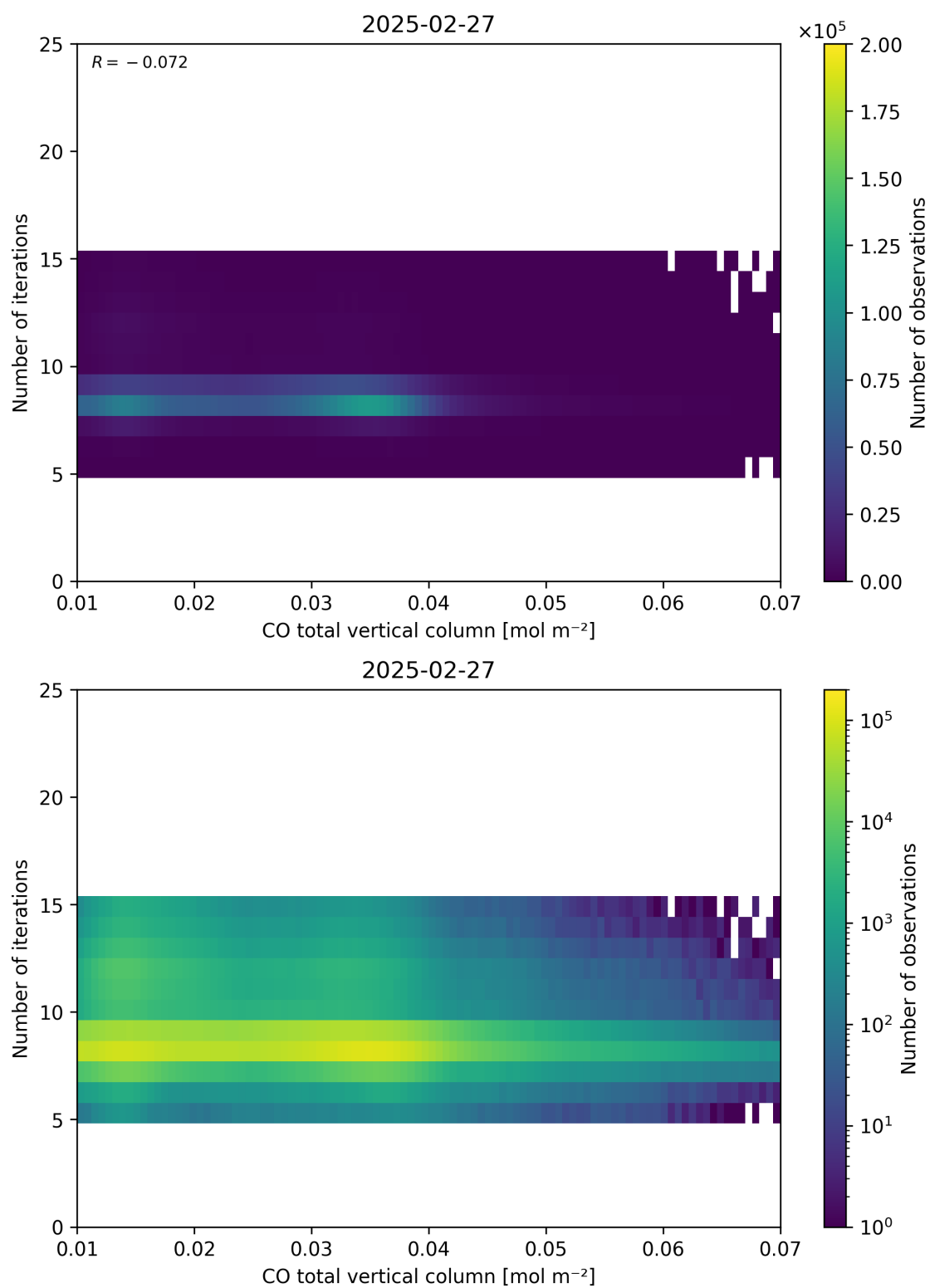
Figure 42: Scatter density plot of “CO total vertical column” against “Number of iterations” for 2025-02-26 to 2025-02-28.
