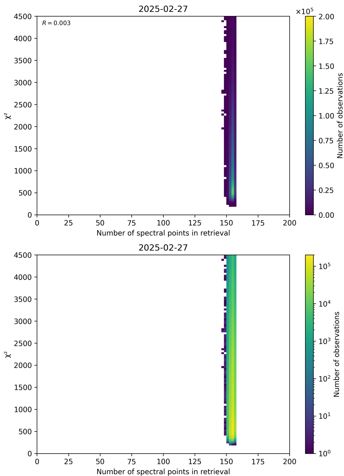
Figure 58: Scatter density plot of “Number of spectral points in retrieval” against “ \chi^2 ” for 2025-02-26 to 2025-02-28.
