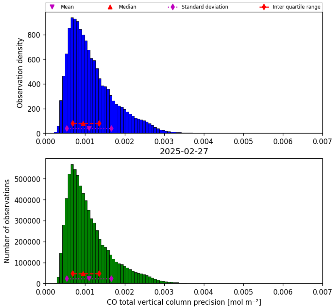
Figure 20: Histogram of “CO total vertical column precision” for 2025-02-26 to 2025-02-28
