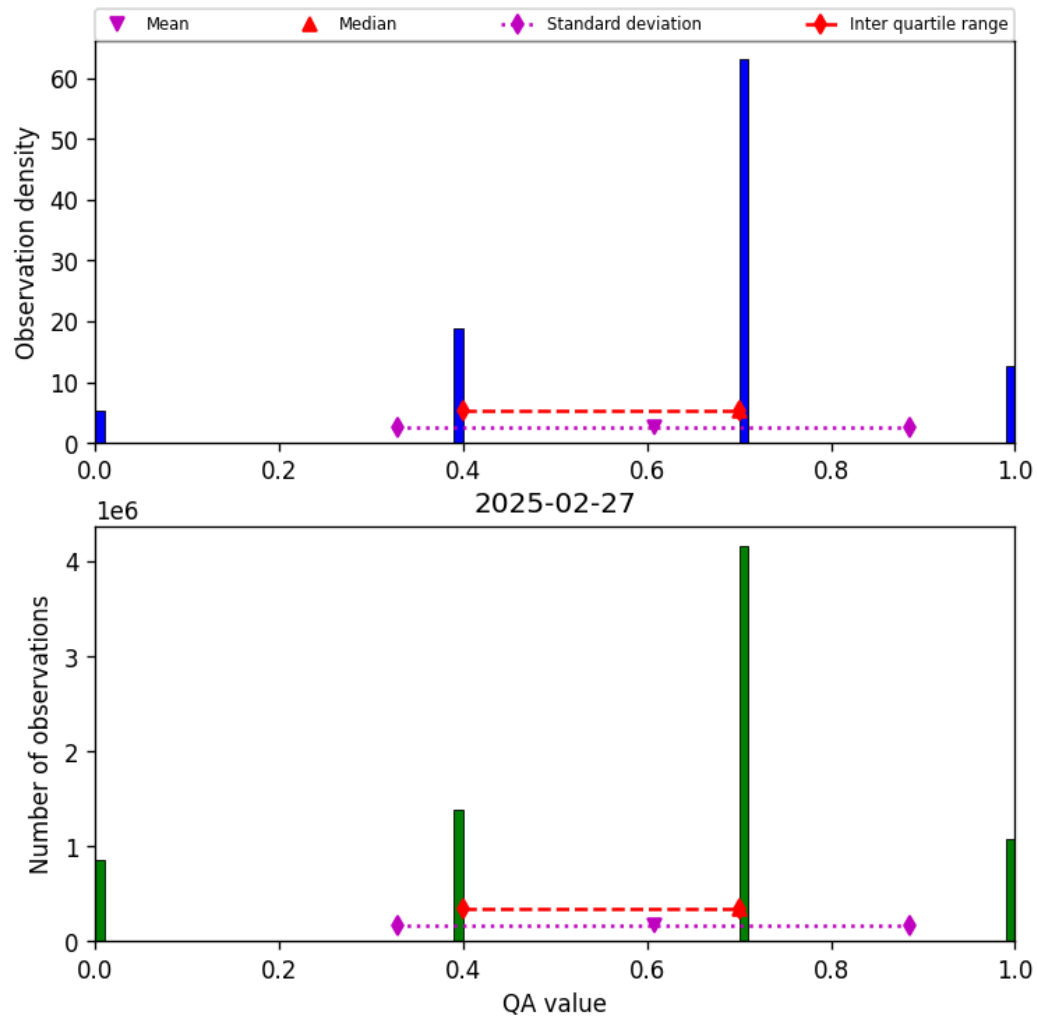
Figure 17: Histogram of “QA value” for 2025-02-26 to 2025-02-28
