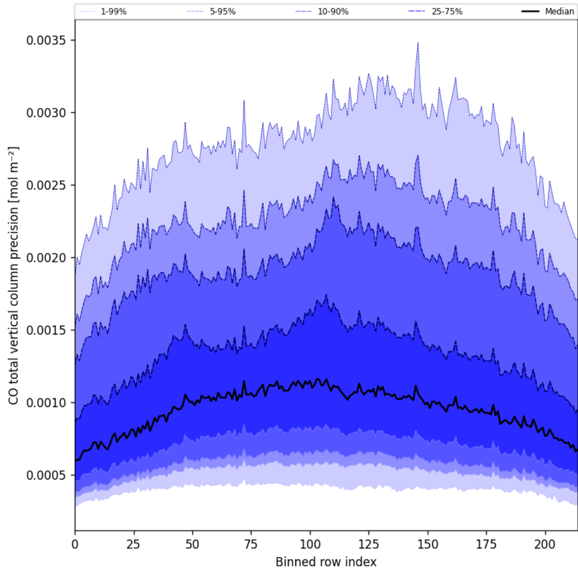
Figure 28: Along track statistics of “CO total vertical column precision” for 2025-02-26 to 2025-02-28
