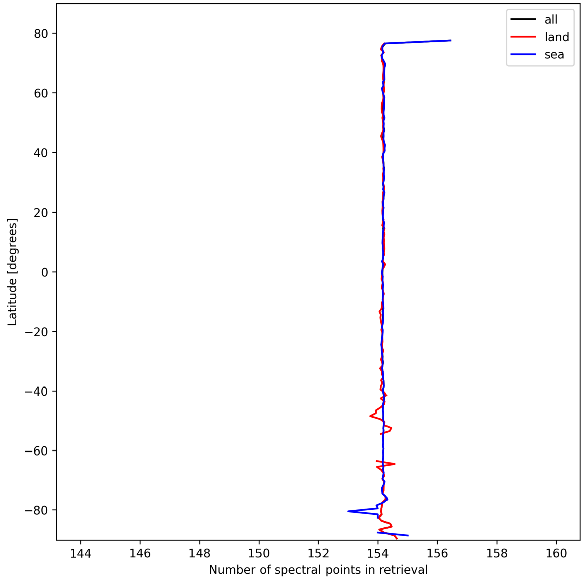
Figure 13: Zonal average of “Number of spectral points in retrieval” for 2025-02-26 to 2025-02-28.
