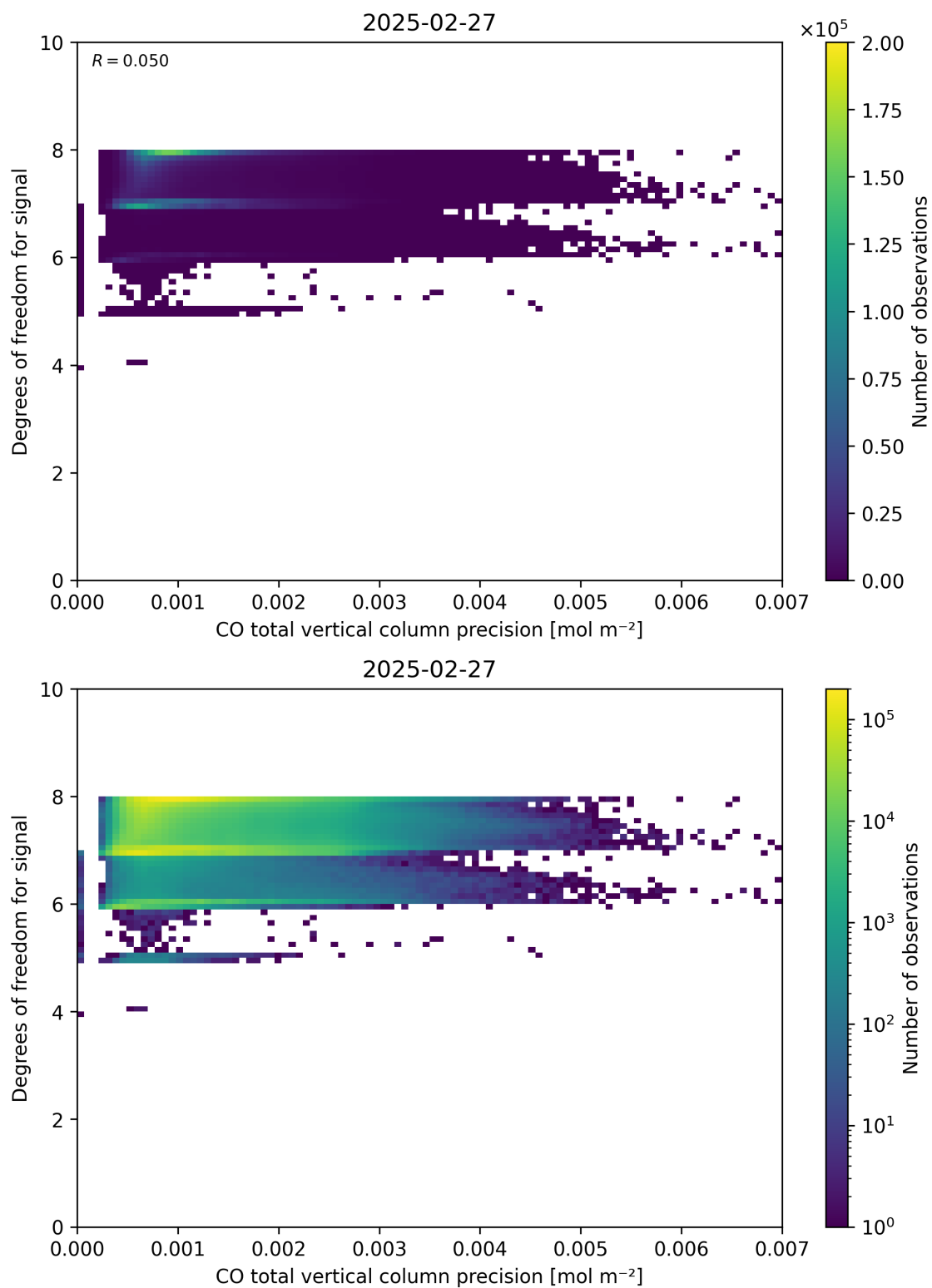
Figure 45: Scatter density plot of “CO total vertical column precision” against “Degrees of freedom for signal” for 2025-02-26 to 2025-02-28.
