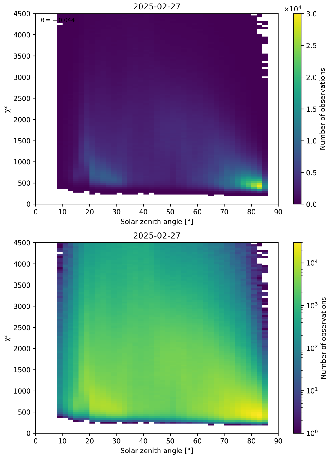
Figure 64: Scatter density plot of “Solar zenith angle” against “ \chi^2 ” for 2025-02-26 to 2025-02-28.
