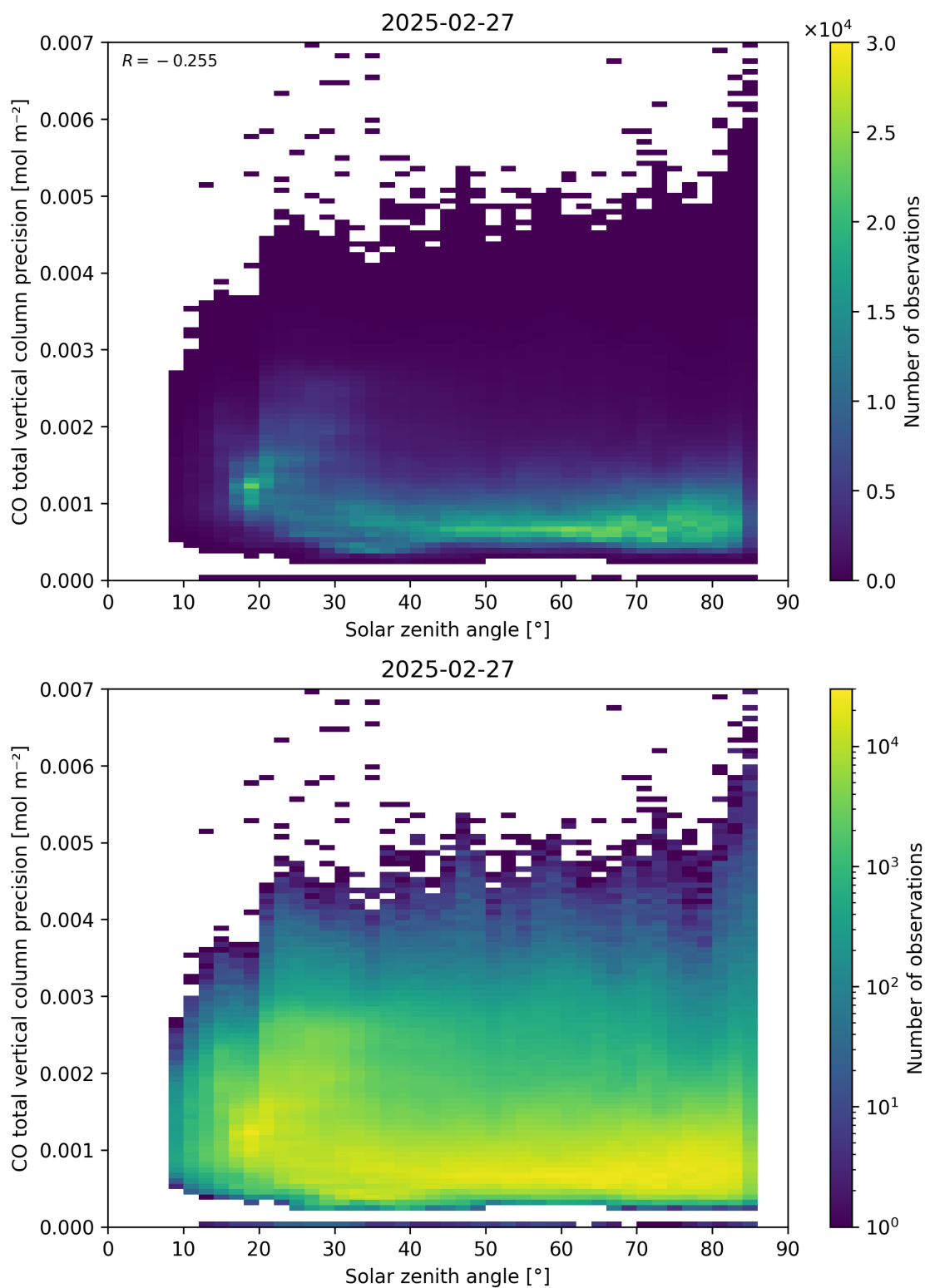
Figure 63: Scatter density plot of “Solar zenith angle” against “CO total vertical column precision” for 2025-02-26 to 2025-02-28.
