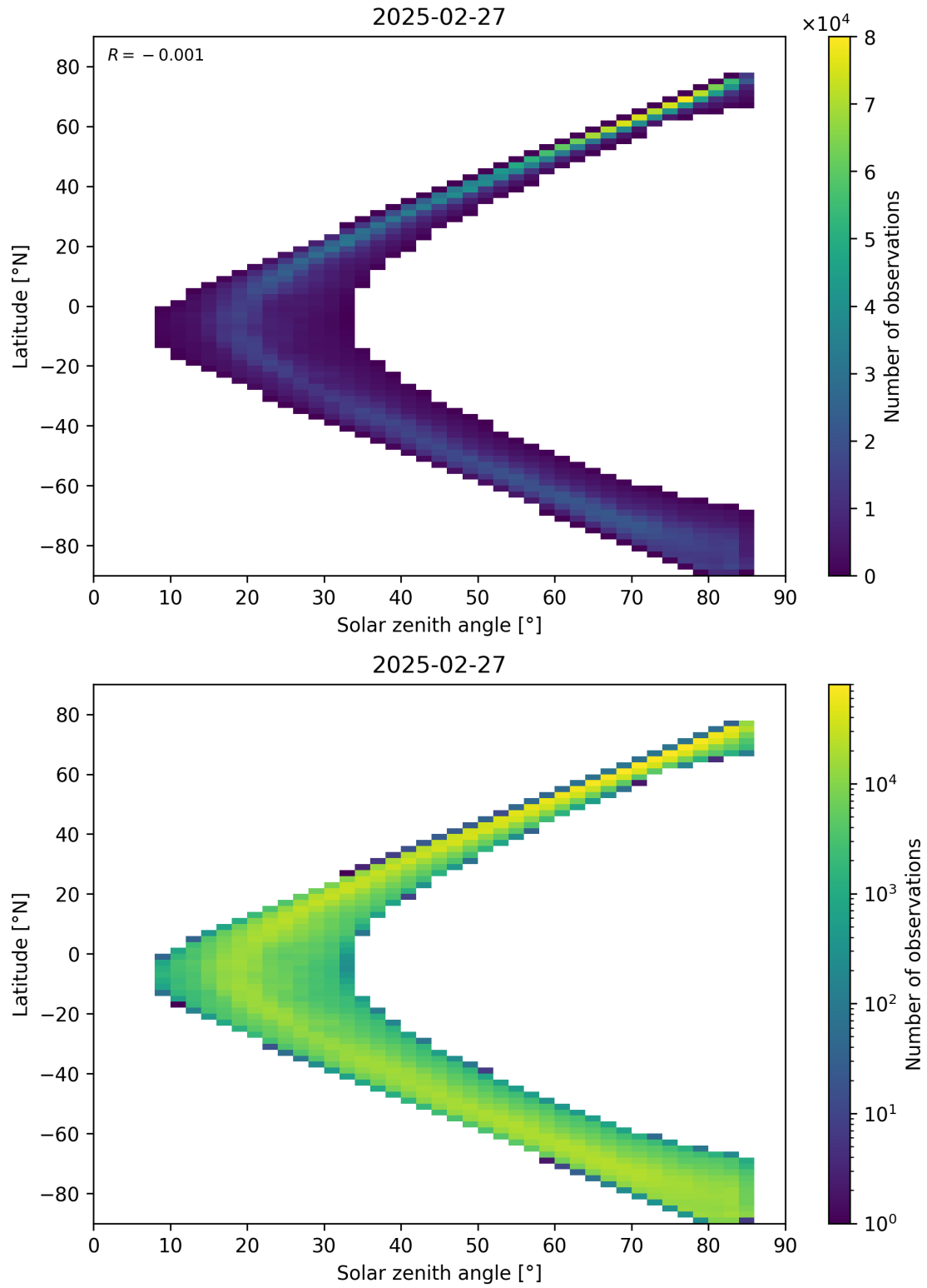
Figure 66: Scatter density plot of “Solar zenith angle” against “Latitude” for 2025-02-26 to 2025-02-28.
