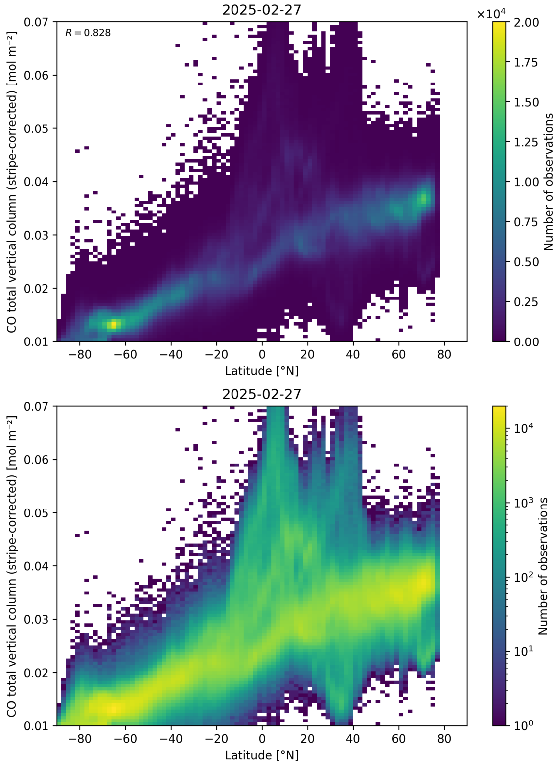
Figure 52: Scatter density plot of “Latitude” against “CO total vertical column (stripe-corrected)” for 2025-02-26 to 2025-02-28.
