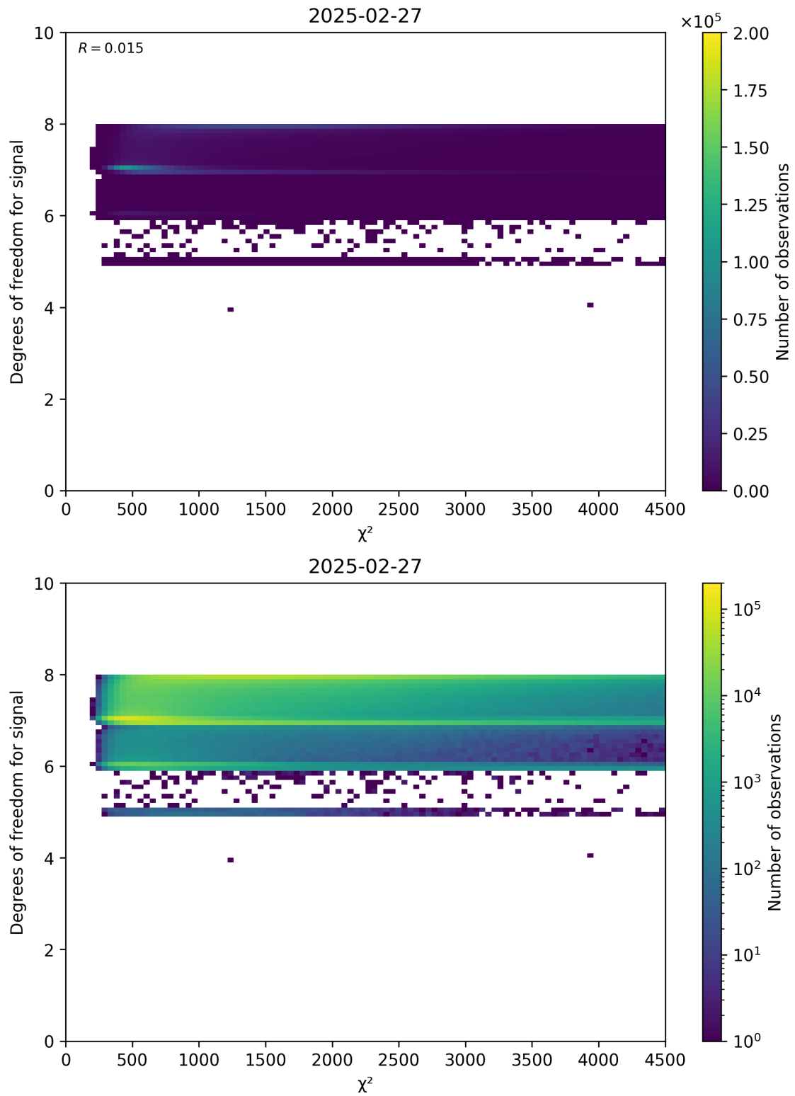
Figure 48: Scatter density plot of “ \chi^2 ” against “Degrees of freedom for signal” for 2025-02-26 to 2025-02-28.
