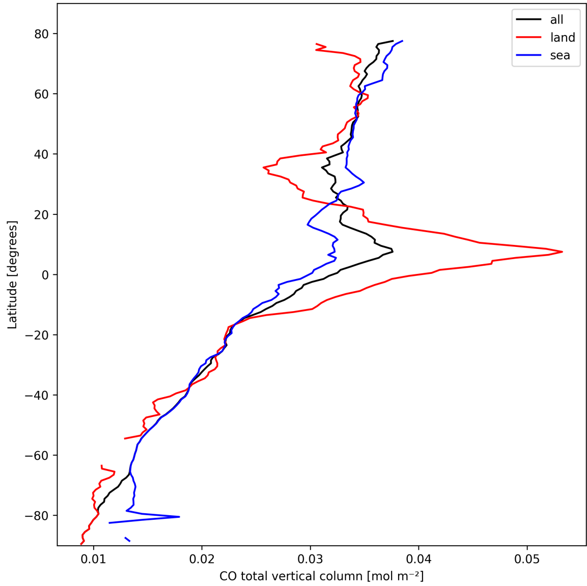
Figure 10: Zonal average of “CO total vertical column” for 2025-02-26 to 2025-02-28.
