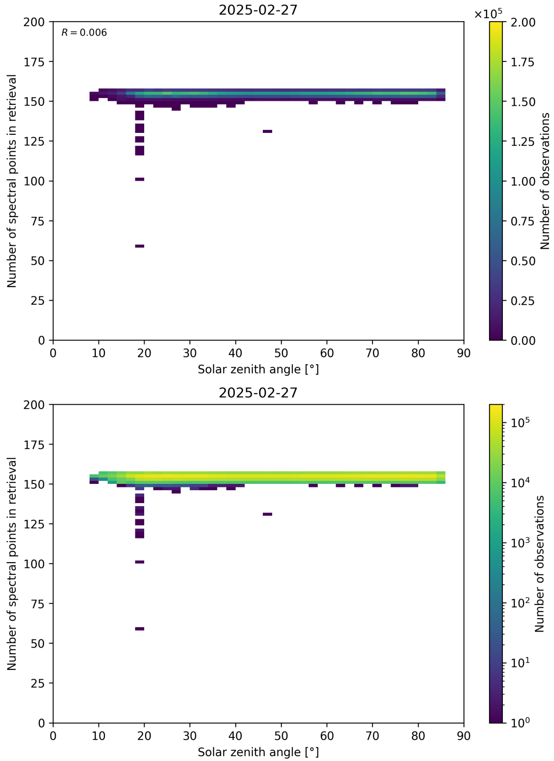
Figure 68: Scatter density plot of “Solar zenith angle” against “Number of spectral points in retrieval” for 2025-02-26 to 2025-02-28.
