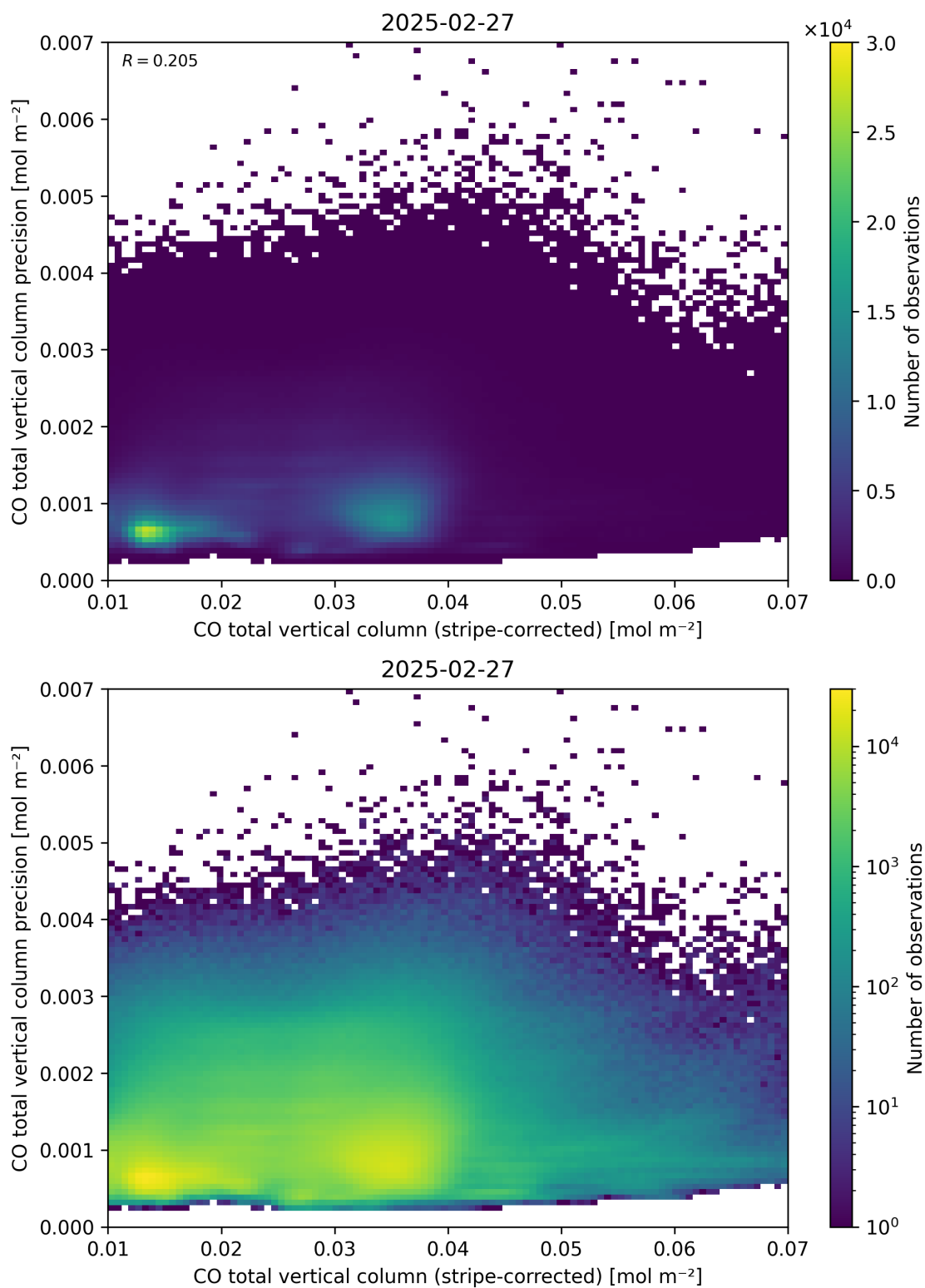
Figure 36: Scatter density plot of “CO total vertical column (stripe-corrected)” against “CO total vertical column precision” for 2025-02-26 to 2025-02-28.
