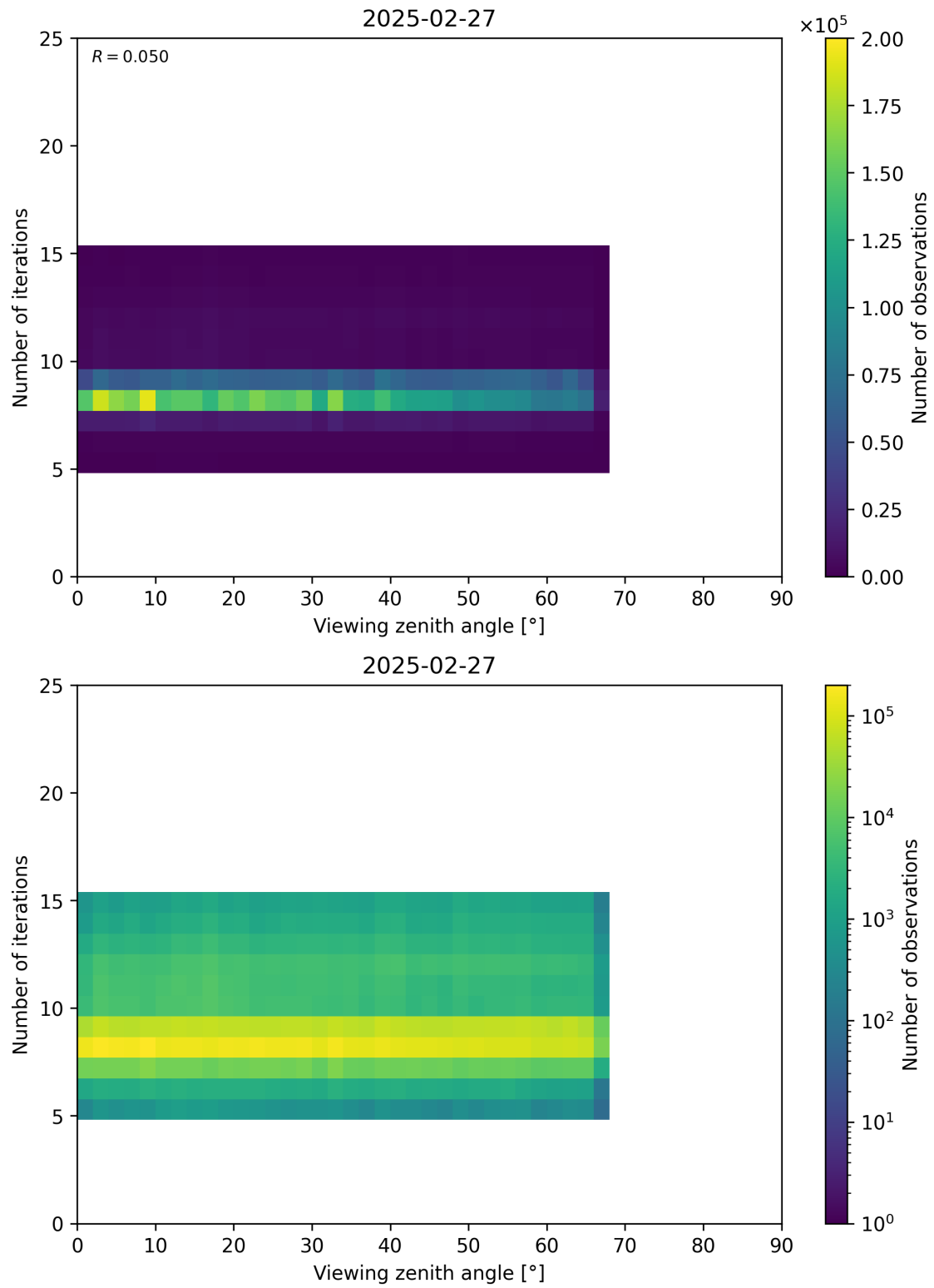
Figure 75: Scatter density plot of “Viewing zenith angle” against “Number of iterations” for 2025-02-26 to 2025-02-28.
