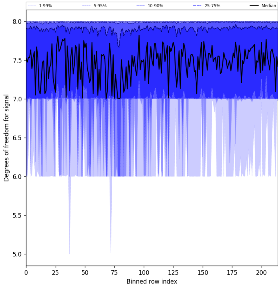
Figure 31: Along track statistics of “Degrees of freedom for signal” for 2025-02-26 to 2025-02-28
