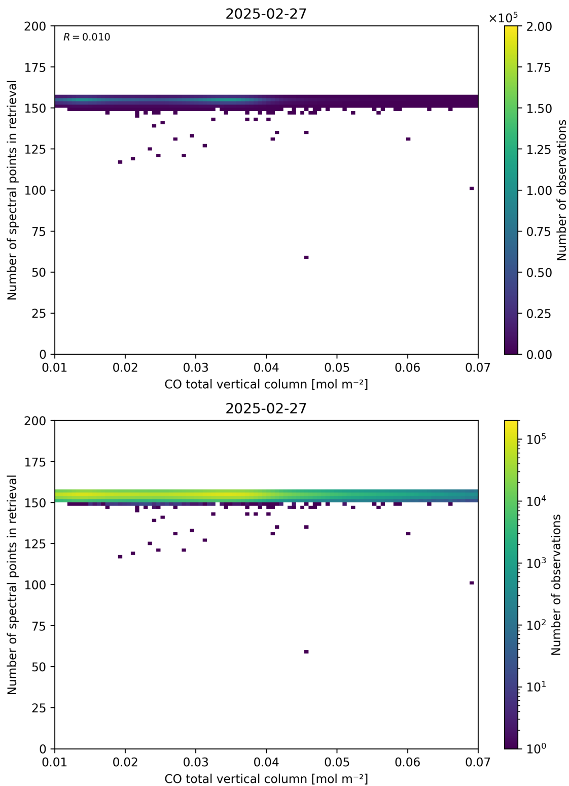
Figure 43: Scatter density plot of “CO total vertical column” against “Number of spectral points in retrieval” for 2025-02-26 to 2025-02-28.
