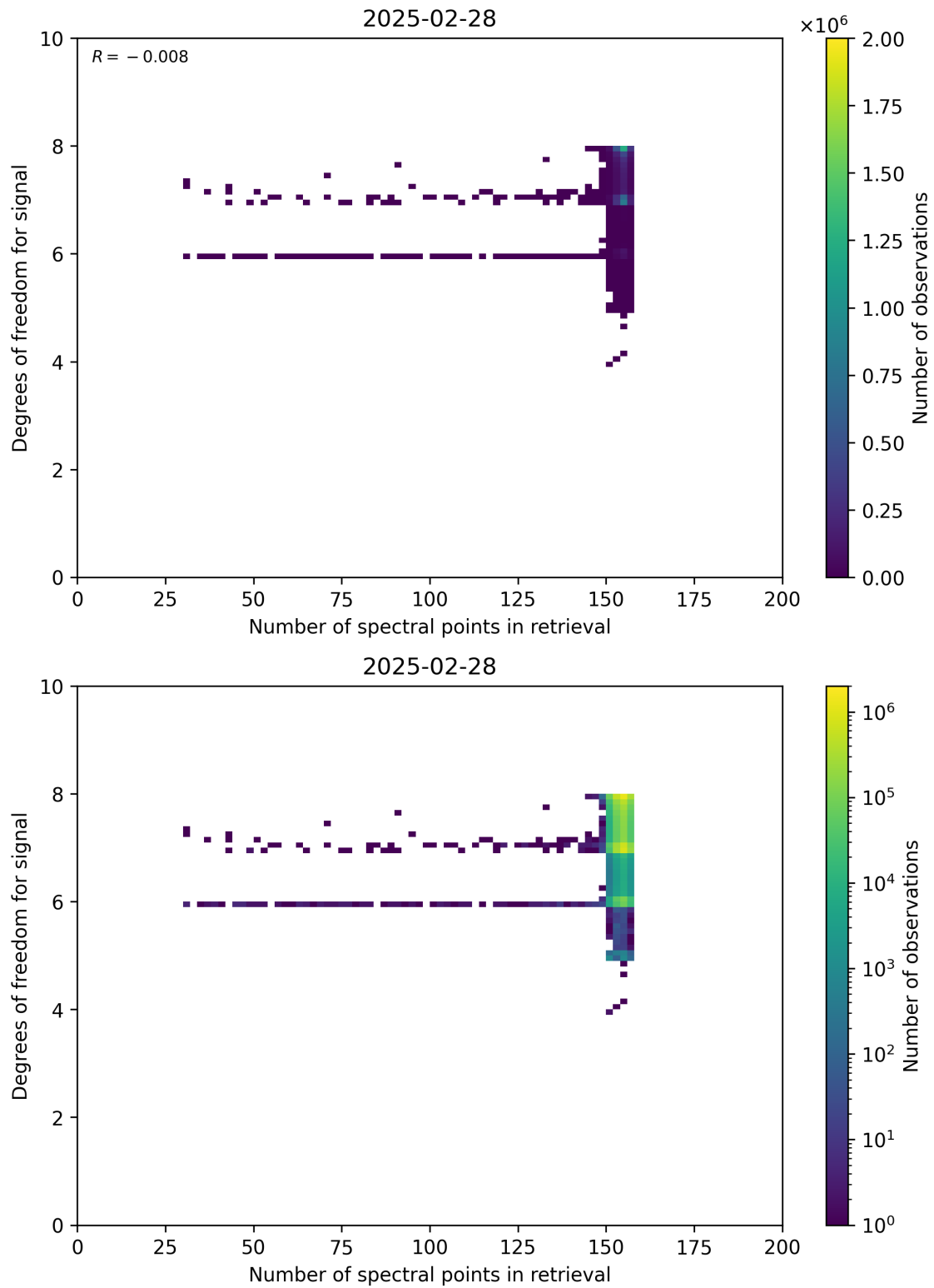
Figure 59: Scatter density plot of “Number of spectral points in retrieval” against “Degrees of freedom for signal” for 2025-02-27 to 2025-03-01.
