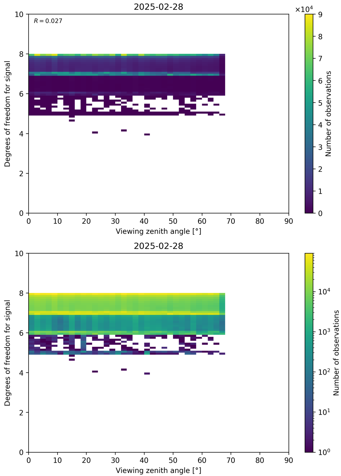
Figure 73: Scatter density plot of “Viewing zenith angle” against “Degrees of freedom for signal” for 2025-02-27 to 2025-03-01.
