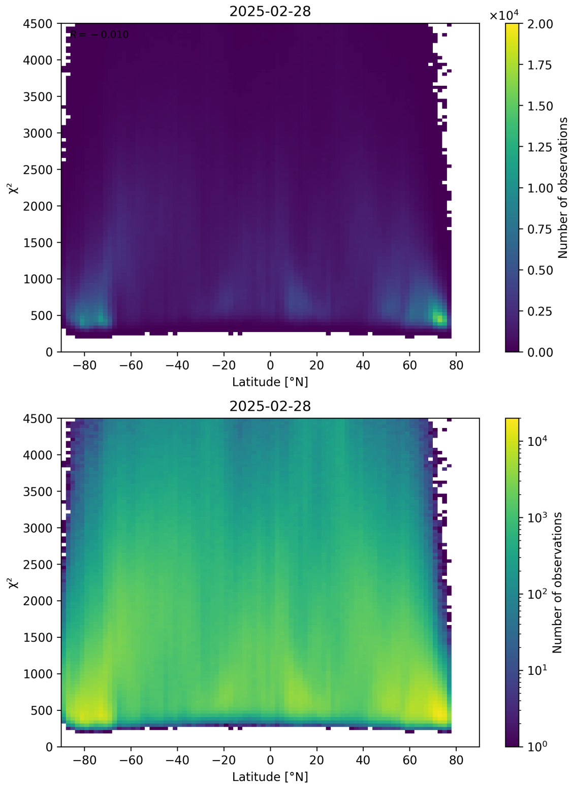
Figure 54: Scatter density plot of “Latitude” against “ \chi^2 ” for 2025-02-27 to 2025-03-01.
