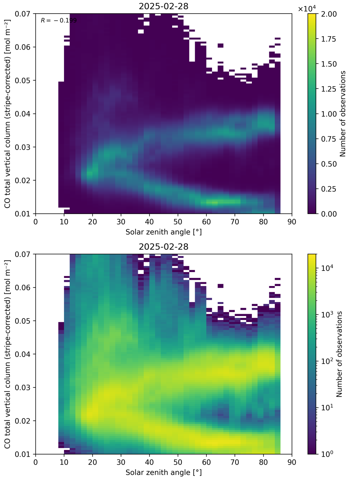
Figure 62: Scatter density plot of “Solar zenith angle” against “CO total vertical column (stripe-corrected)” for 2025-02-27 to 2025-03-01.
