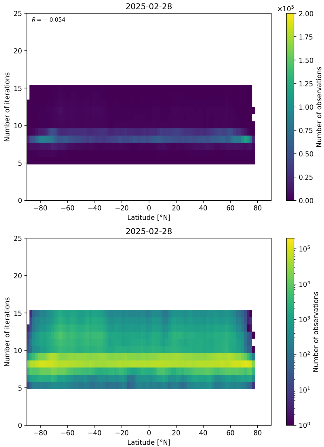
Figure 56: Scatter density plot of “Latitude” against “Number of iterations” for 2025-02-27 to 2025-03-01.
