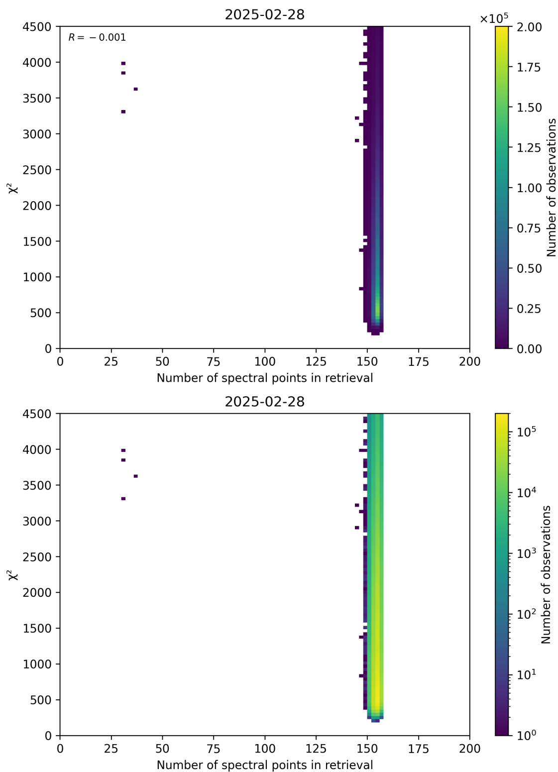
Figure 58: Scatter density plot of “Number of spectral points in retrieval” against “ \chi^2 ” for 2025-02-27 to 2025-03-01.
