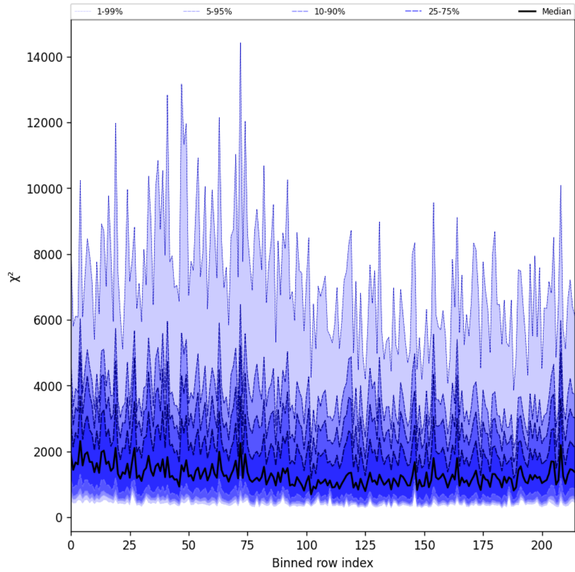
Figure 30: Along track statistics of “ \chi^2 ” for 2025-02-27 to 2025-03-01
