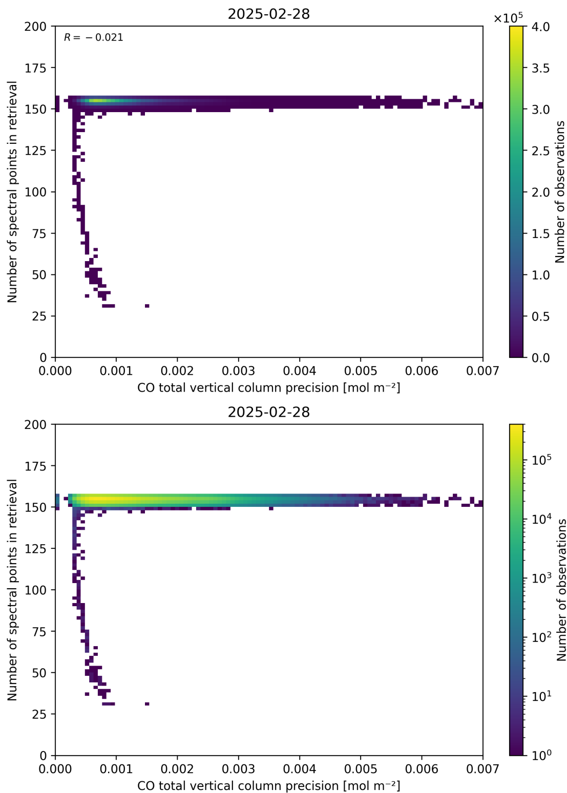
Figure 47: Scatter density plot of “CO total vertical column precision” against “Number of spectral points in retrieval” for 2025-02-27 to 2025-03-01.
