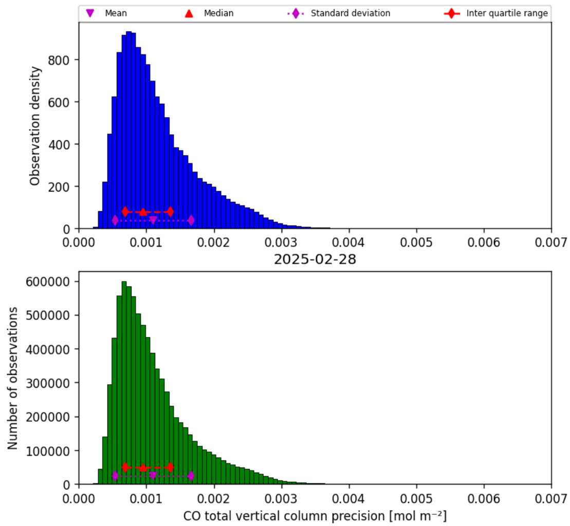
Figure 20: Histogram of “CO total vertical column precision” for 2025-02-27 to 2025-03-01
