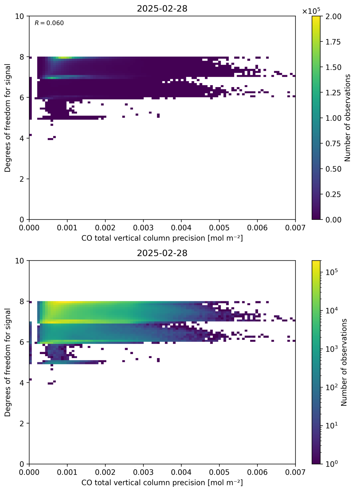
Figure 45: Scatter density plot of “CO total vertical column precision” against “Degrees of freedom for signal” for 2025-02-27 to 2025-03-01.
