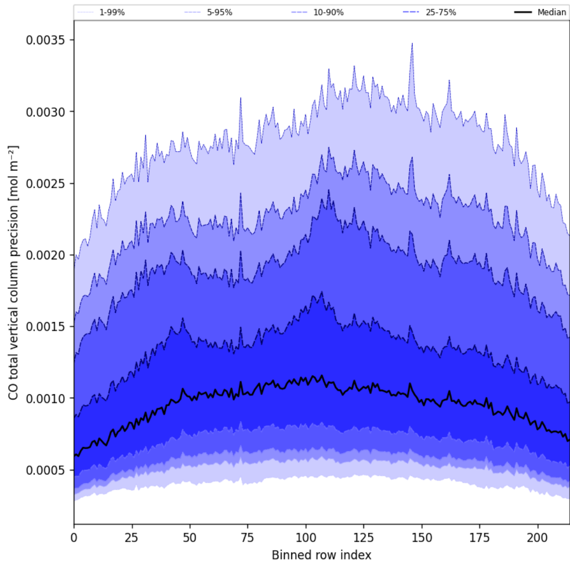
Figure 28: Along track statistics of “CO total vertical column precision” for 2025-02-27 to 2025-03-01
