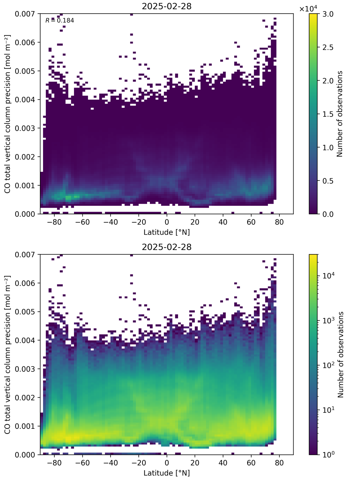
Figure 53: Scatter density plot of “Latitude” against “CO total vertical column precision” for 2025-02-27 to 2025-03-01.
