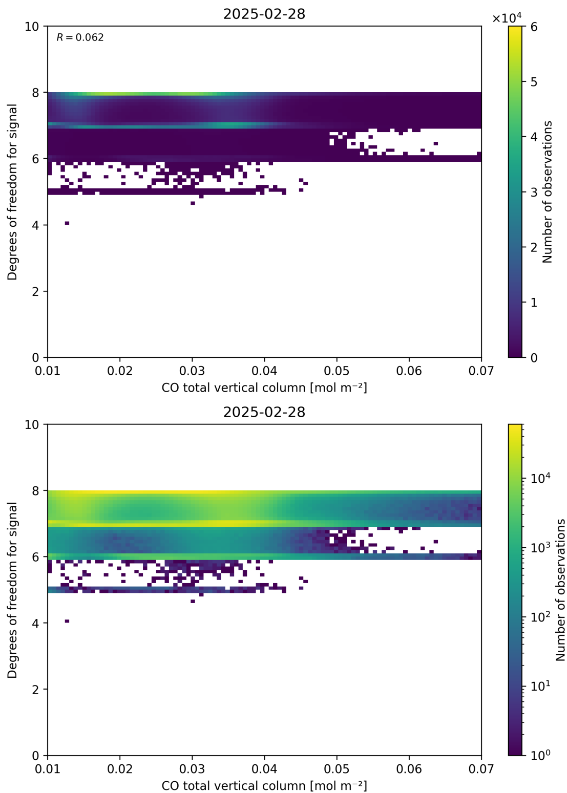
Figure 41: Scatter density plot of “CO total vertical column” against “Degrees of freedom for signal” for 2025-02-27 to 2025-03-01.
