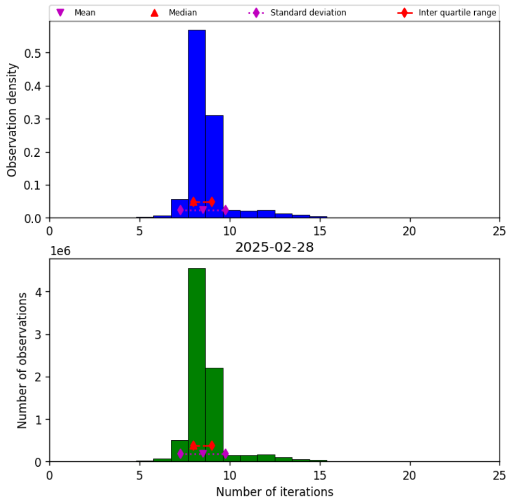
Figure 24: Histogram of “Number of iterations” for 2025-02-27 to 2025-03-01
