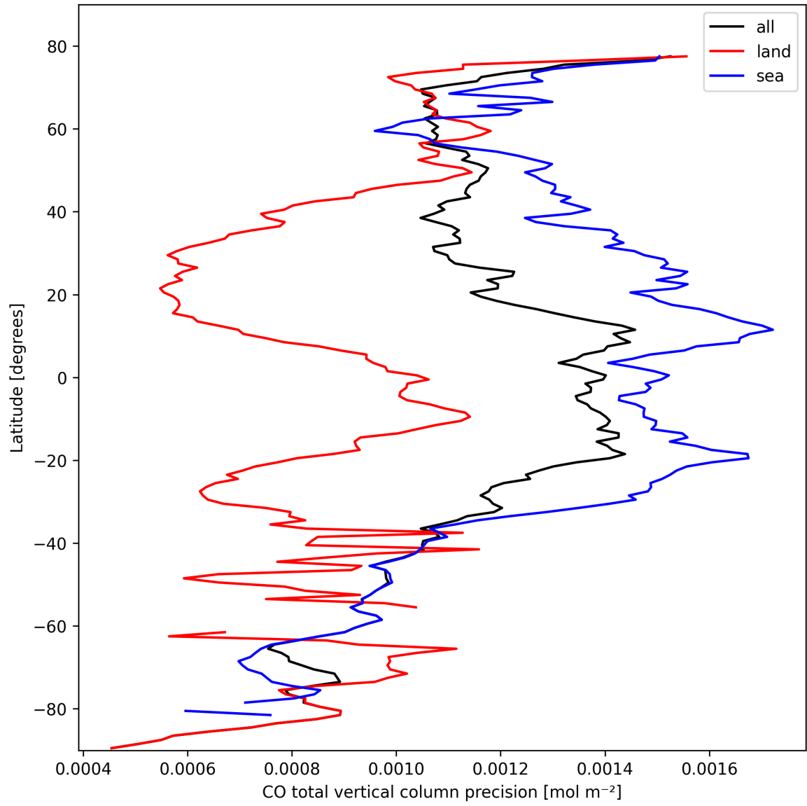
Figure 12: Zonal average of “CO total vertical column precision” for 2025-02-27 to 2025-03-01.
