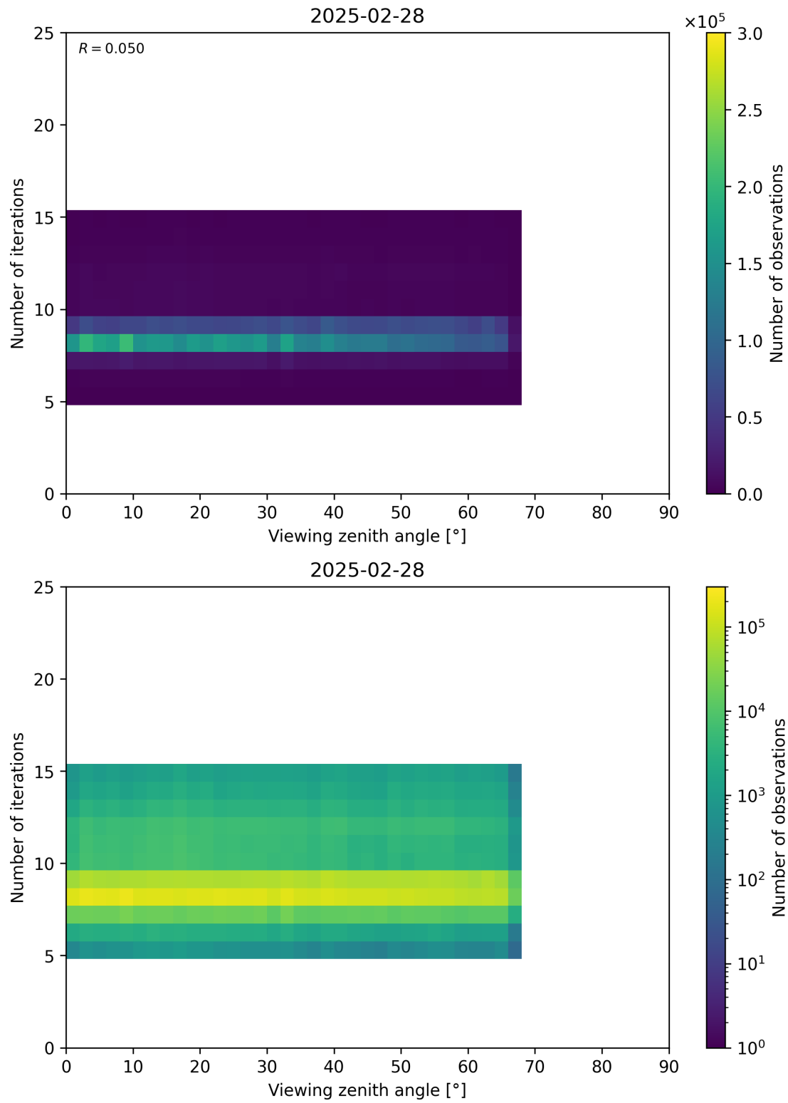
Figure 75: Scatter density plot of “Viewing zenith angle” against “Number of iterations” for 2025-02-27 to 2025-03-01.
