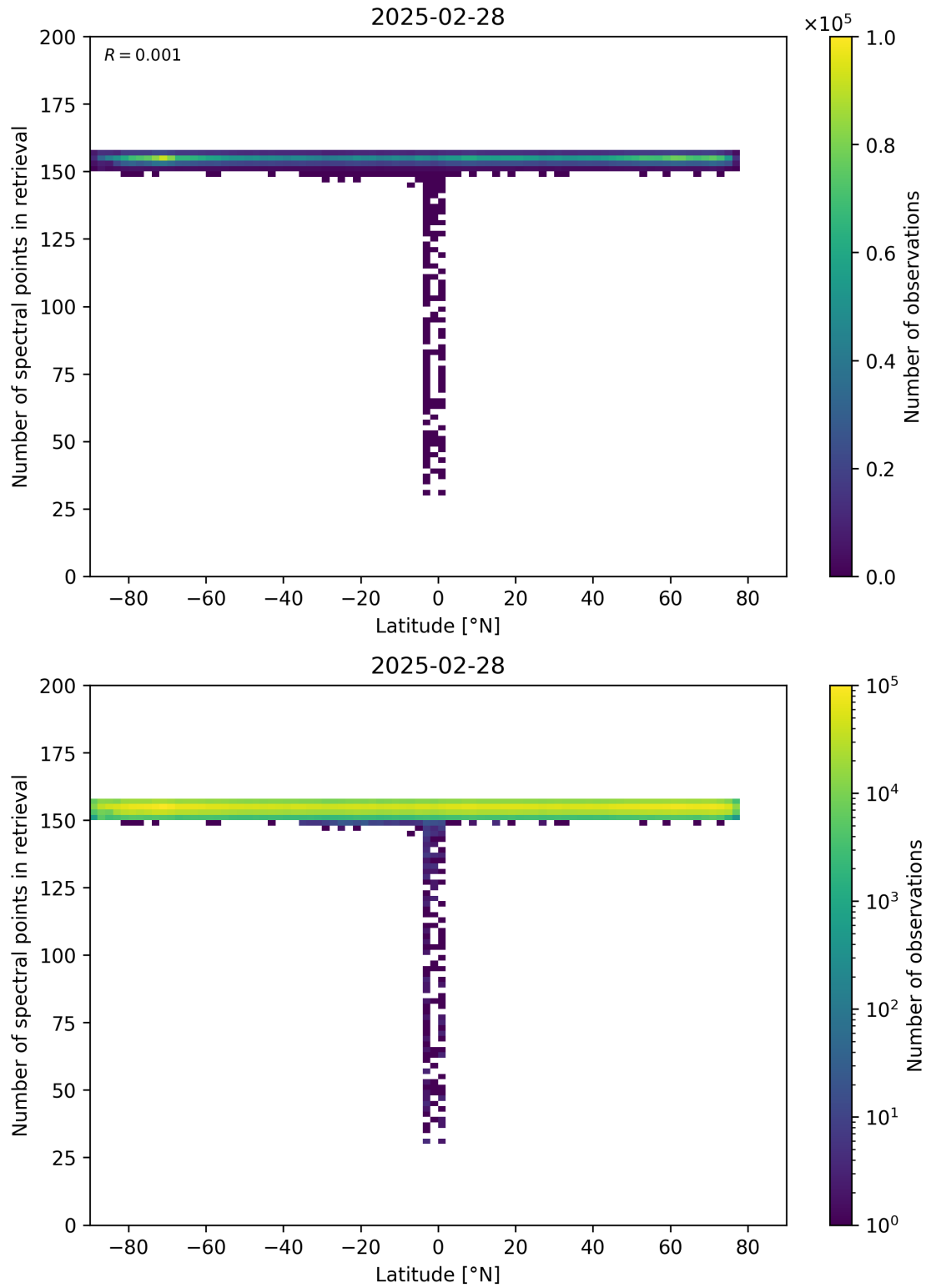
Figure 57: Scatter density plot of “Latitude” against “Number of spectral points in retrieval” for 2025-02-27 to 2025-03-01.
