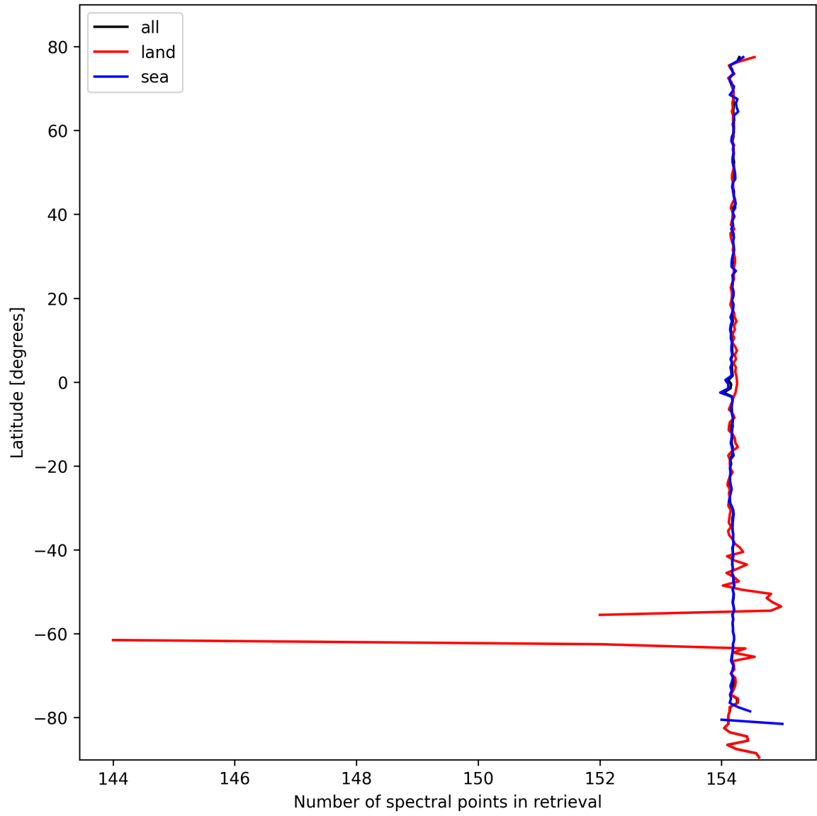
Figure 13: Zonal average of “Number of spectral points in retrieval” for 2025-02-27 to 2025-03-01.
