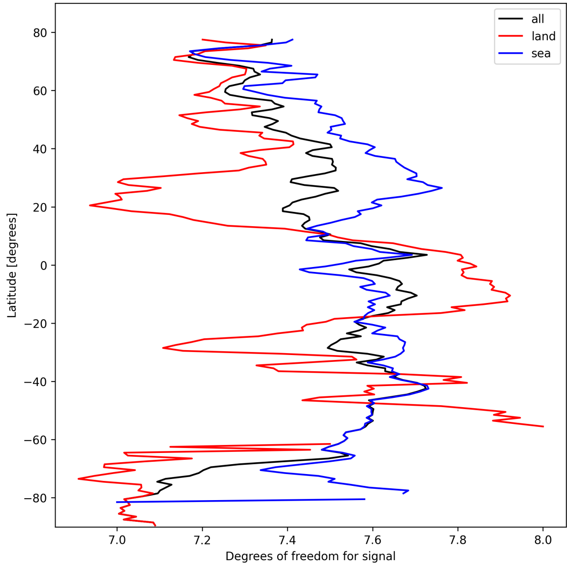
Figure 15: Zonal average of “Degrees of freedom for signal” for 2025-02-27 to 2025-03-01.
