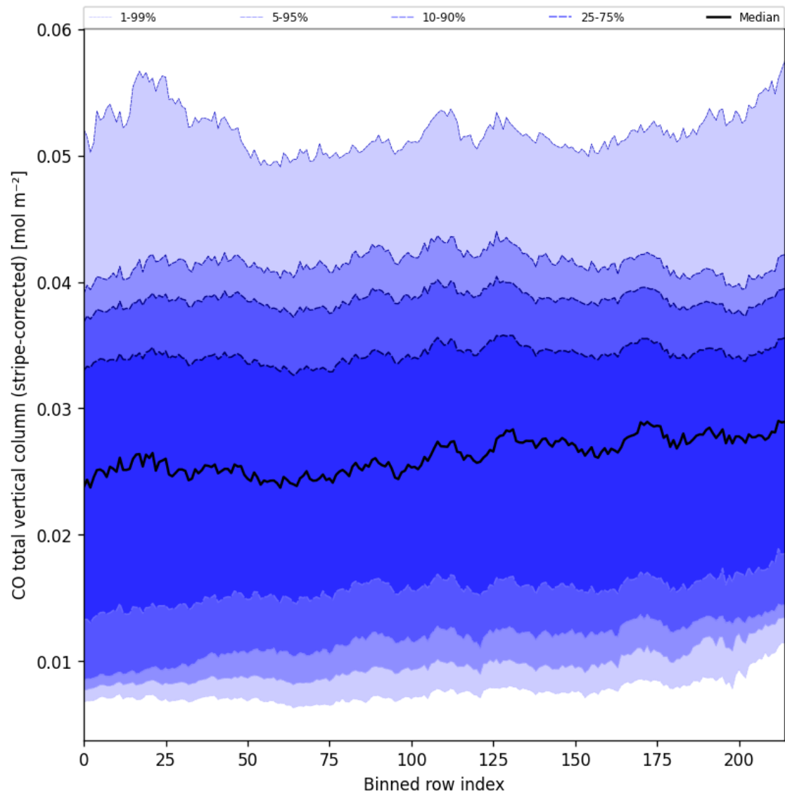
Figure 27: Along track statistics of “CO total vertical column (stripe-corrected)” for 2025-02-27 to 2025-03-01
