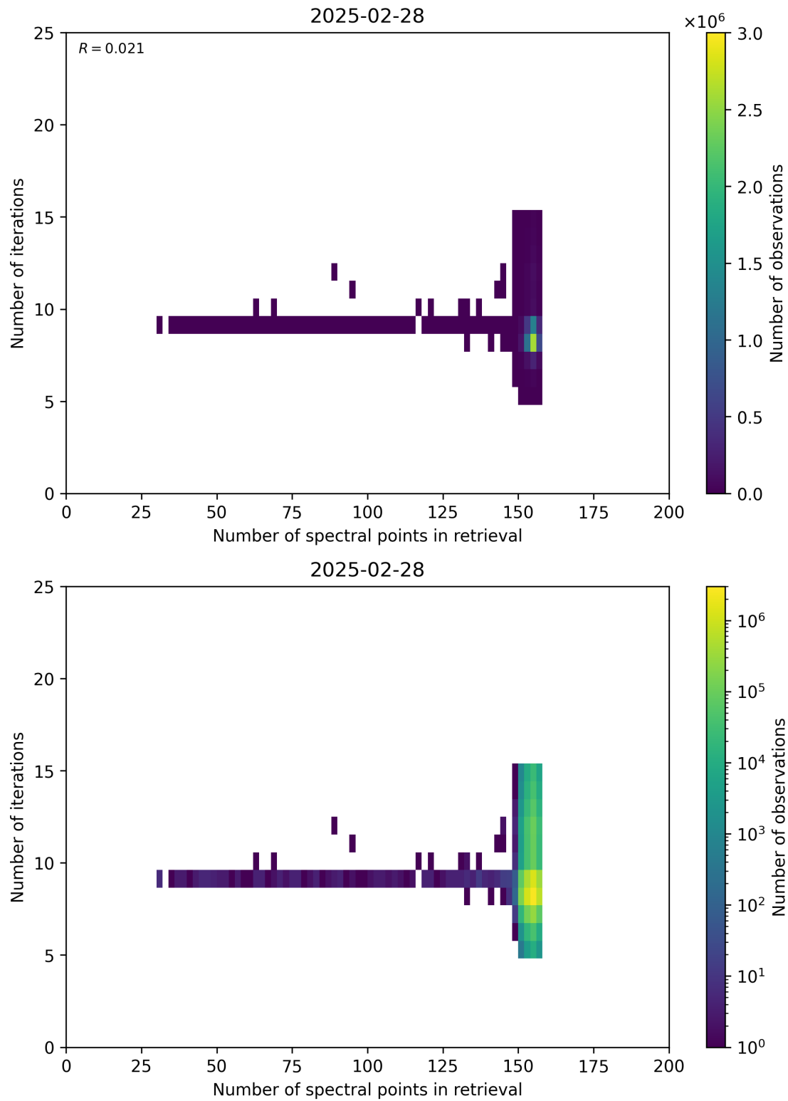
Figure 60: Scatter density plot of “Number of spectral points in retrieval” against “Number of iterations” for 2025-02-27 to 2025-03-01.
