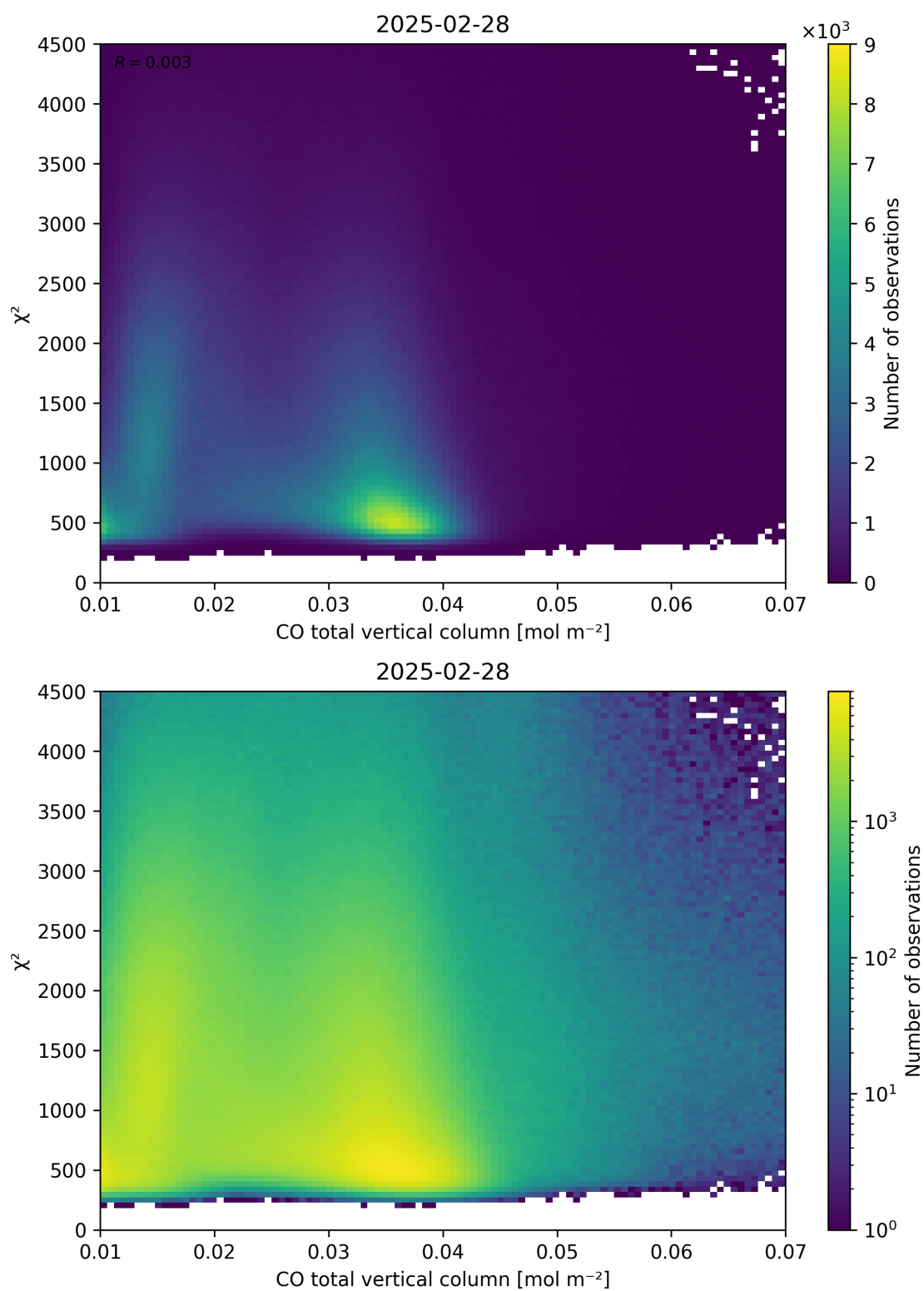
Figure 35: Scatter density plot of “CO total vertical column” against “ \chi^2 ” for 2025-02-27 to 2025-03-01.
