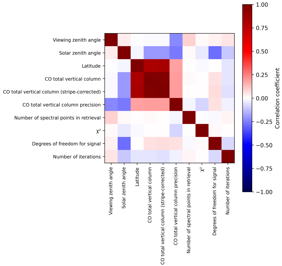
Figure 2: Map of correlation matrix for 2025-02-27 to 2025-03-01.
