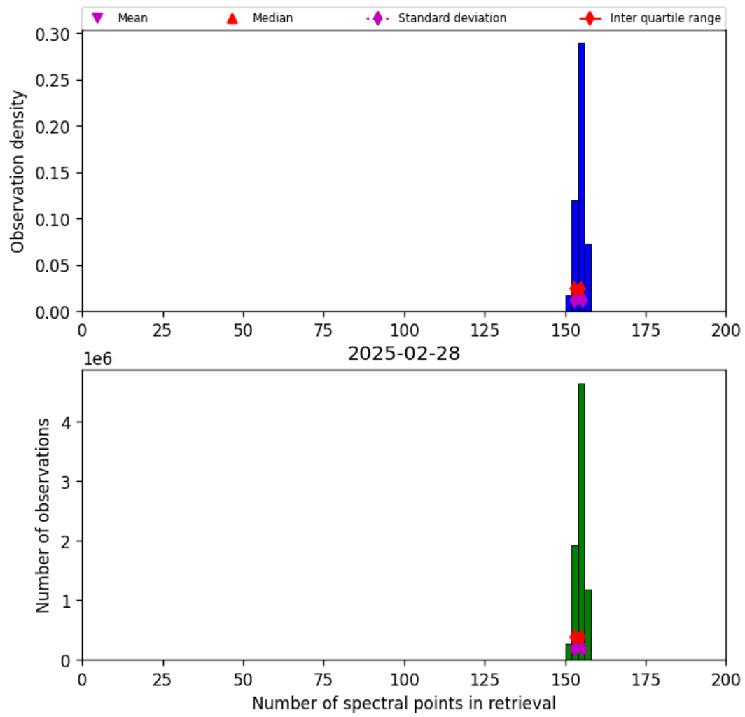
Figure 21: Histogram of “Number of spectral points in retrieval” for 2025-02-27 to 2025-03-01
