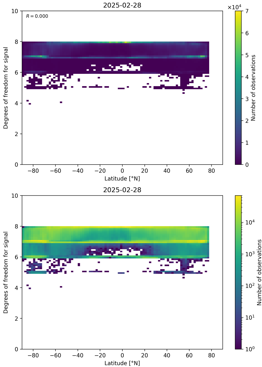
Figure 55: Scatter density plot of “Latitude” against “Degrees of freedom for signal” for 2025-02-27 to 2025-03-01.
