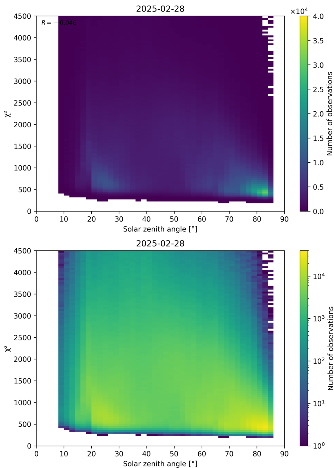
Figure 64: Scatter density plot of “Solar zenith angle” against “ \chi^2 ” for 2025-02-27 to 2025-03-01.
