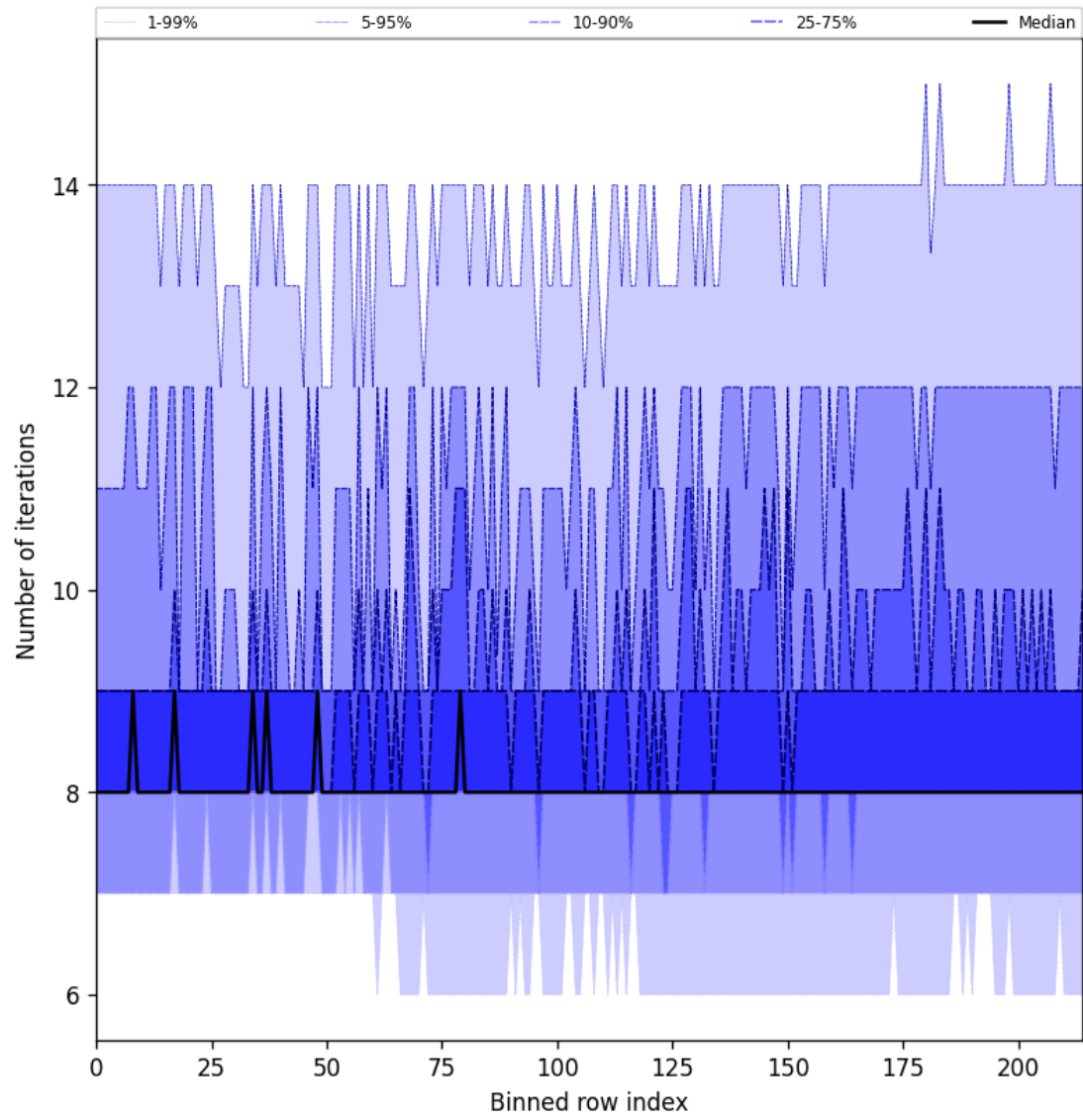
Figure 32: Along track statistics of “Number of iterations” for 2025-02-27 to 2025-03-01
