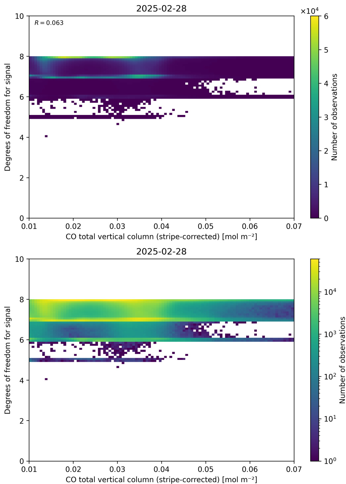
Figure 38: Scatter density plot of “CO total vertical column (stripe-corrected)” against “Degrees of freedom for signal” for 2025-02-27 to 2025-03-01.
