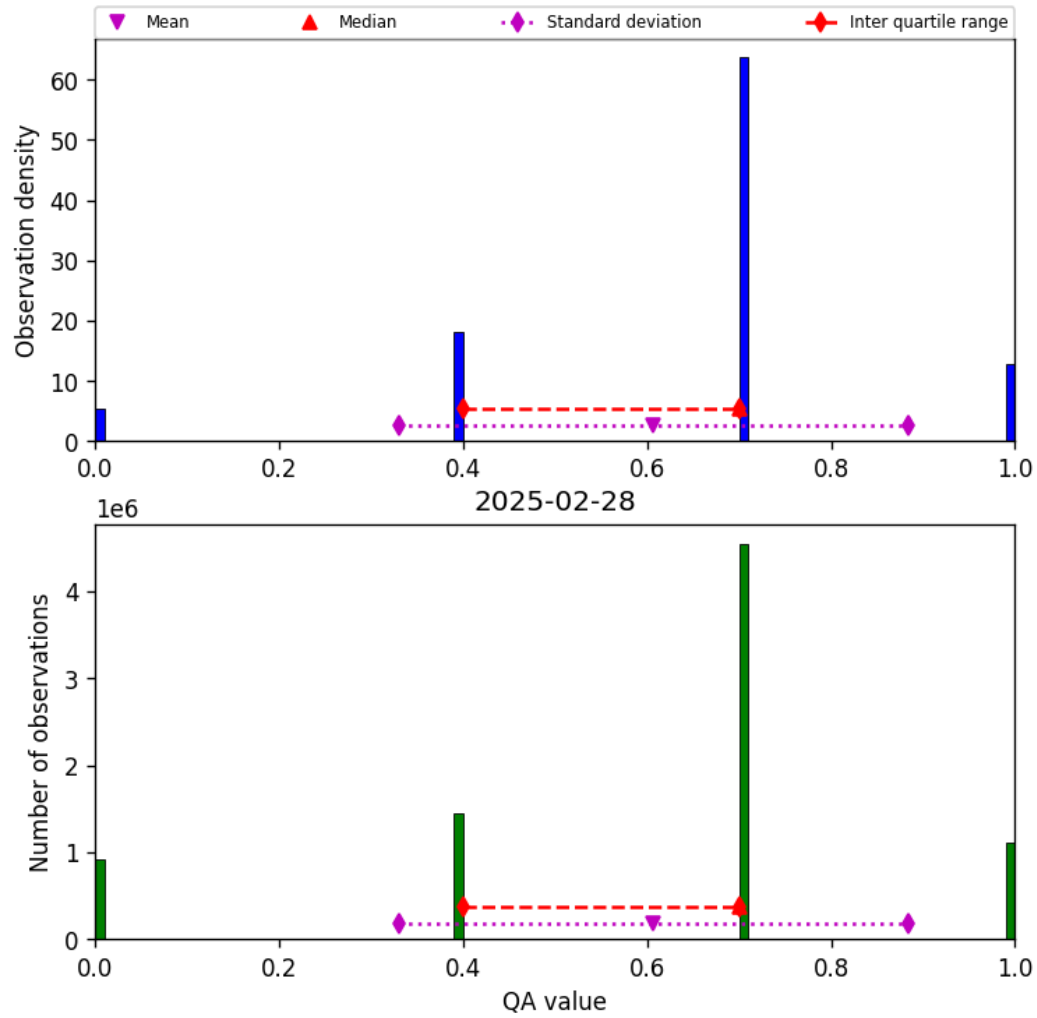
Figure 17: Histogram of “QA value” for 2025-02-27 to 2025-03-01
