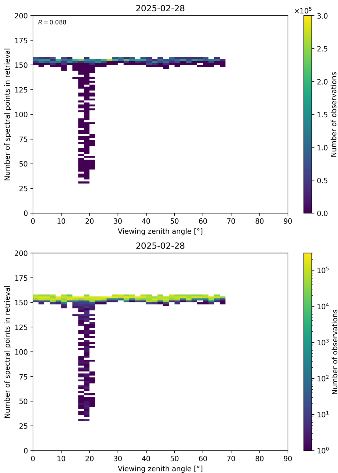
Figure 76: Scatter density plot of “Viewing zenith angle” against “Number of spectral points in retrieval” for 2025-02-27 to 2025-03-01.
