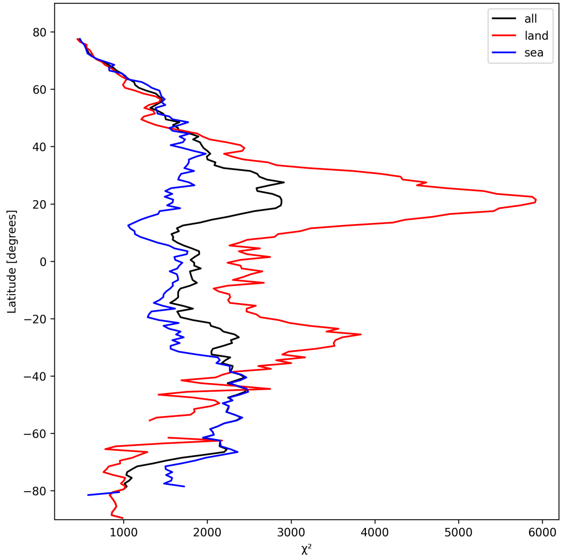
Figure 14: Zonal average of “ \chi^2 ” for 2025-02-27 to 2025-03-01.
