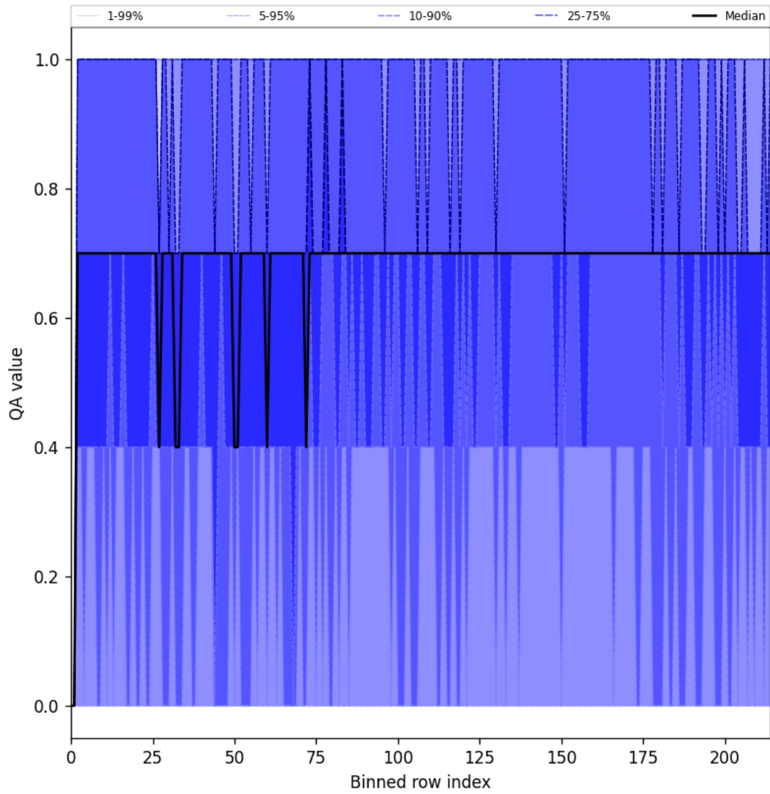
Figure 25: Along track statistics of “QA value” for 2025-02-27 to 2025-03-01
