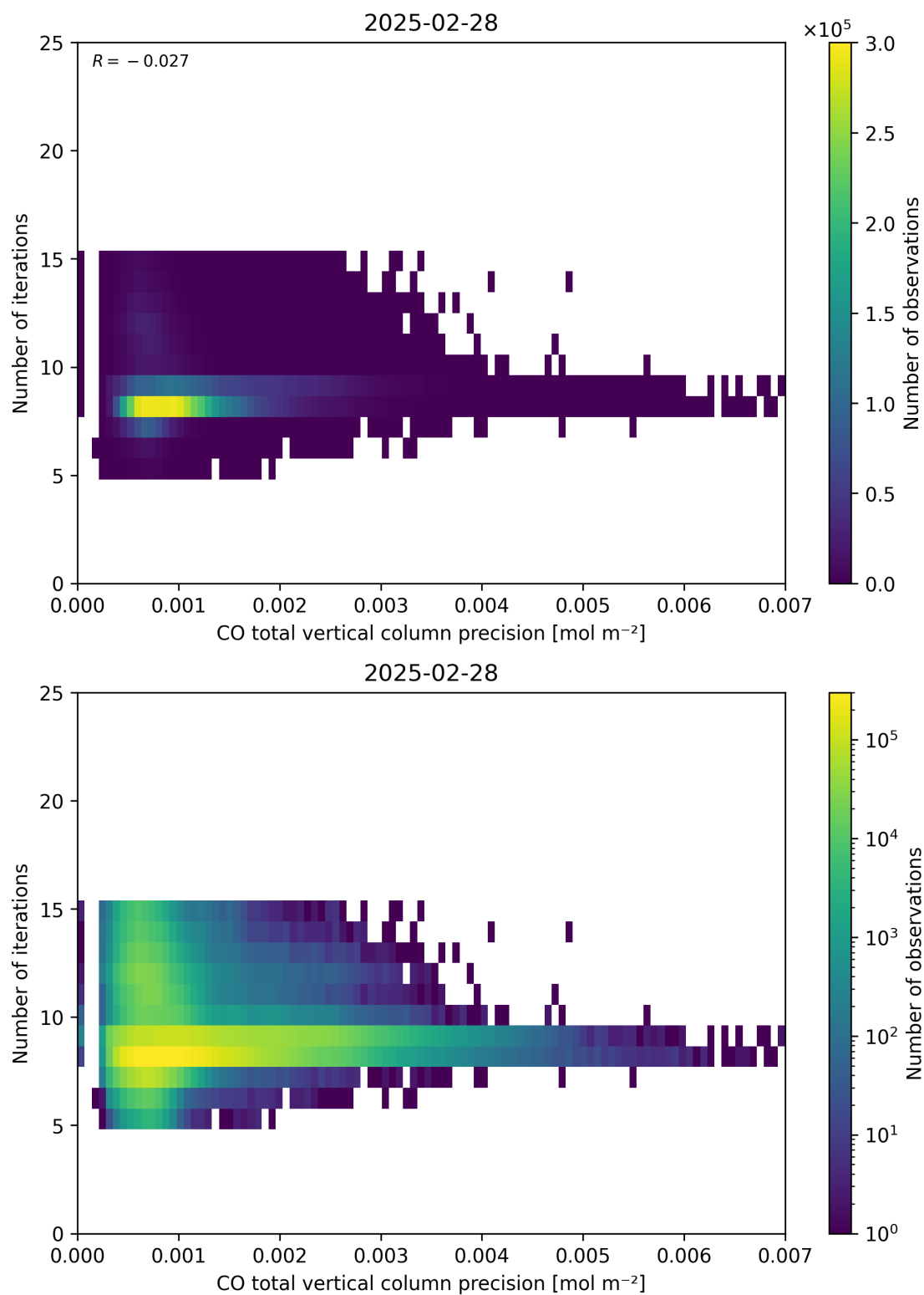
Figure 46: Scatter density plot of “CO total vertical column precision” against “Number of iterations” for 2025-02-27 to 2025-03-01.
