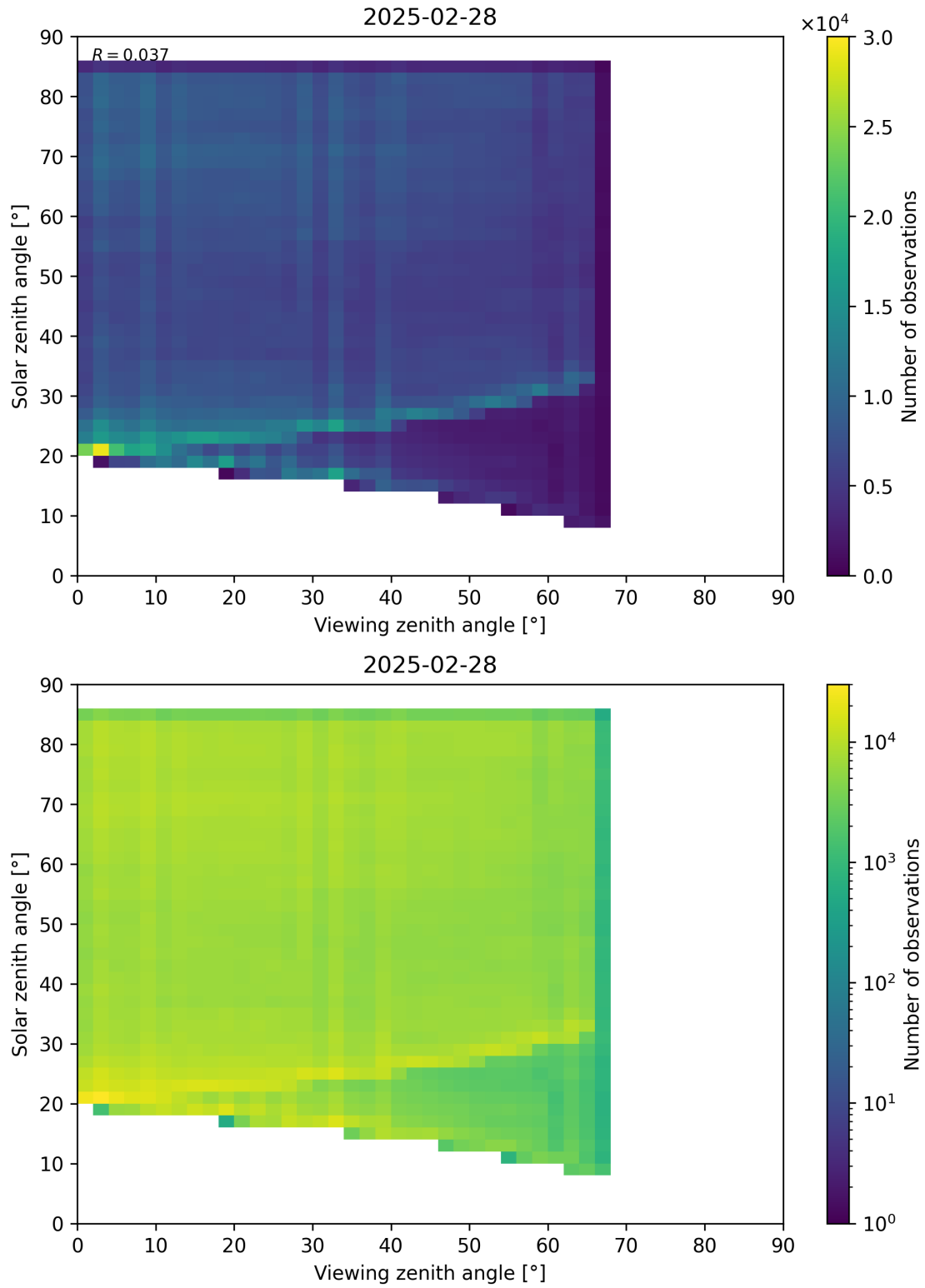
Figure 77: Scatter density plot of “Viewing zenith angle” against “Solar zenith angle” for 2025-02-27 to 2025-03-01.
