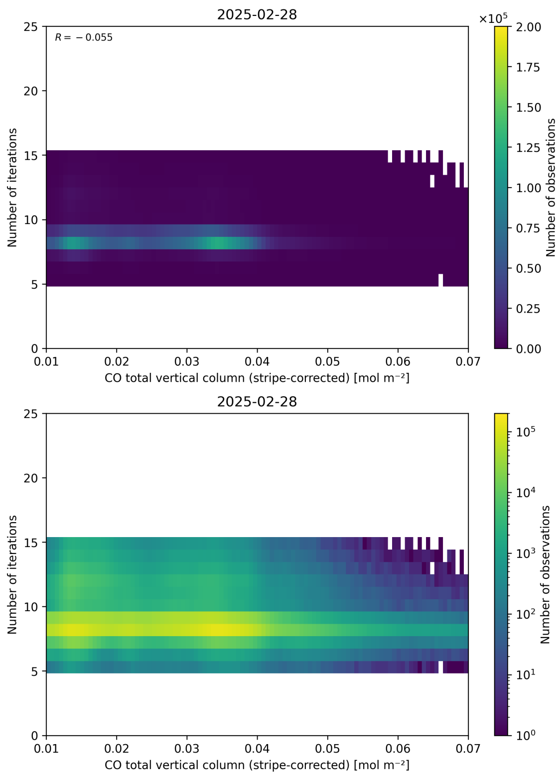
Figure 39: Scatter density plot of “CO total vertical column (stripe-corrected)” against “Number of iterations” for 2025-02-27 to 2025-03-01.
