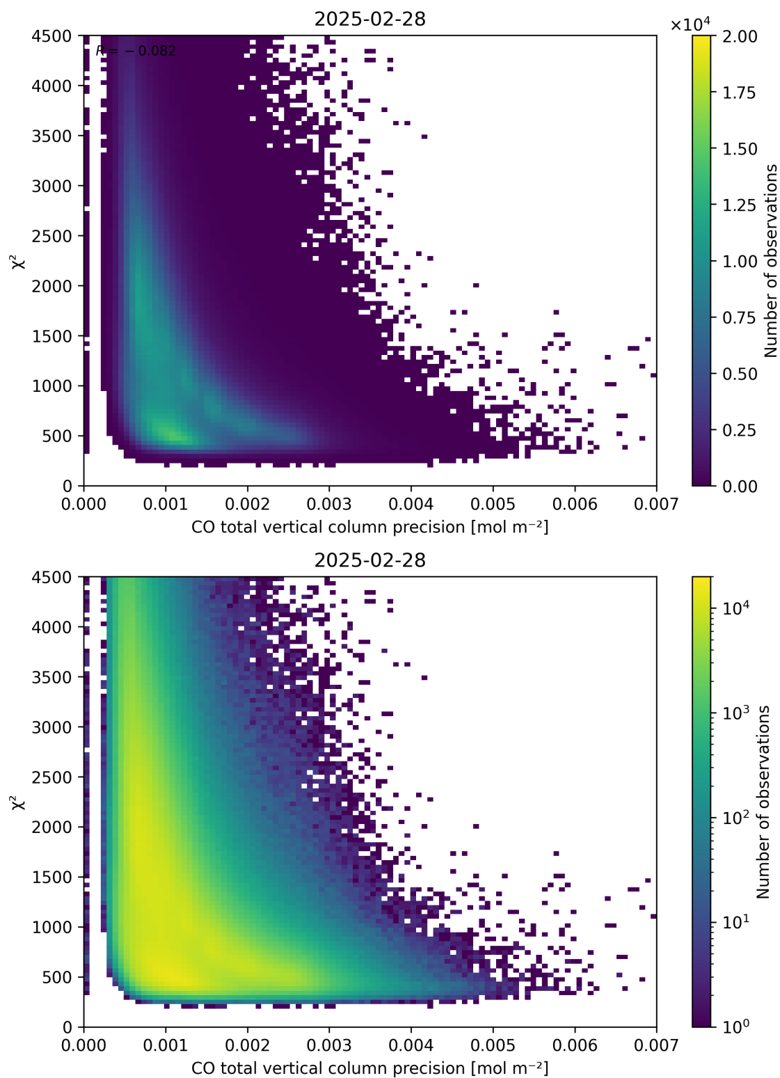
Figure 44: Scatter density plot of “CO total vertical column precision” against “ \chi^2 ” for 2025-02-27 to 2025-03-01.
