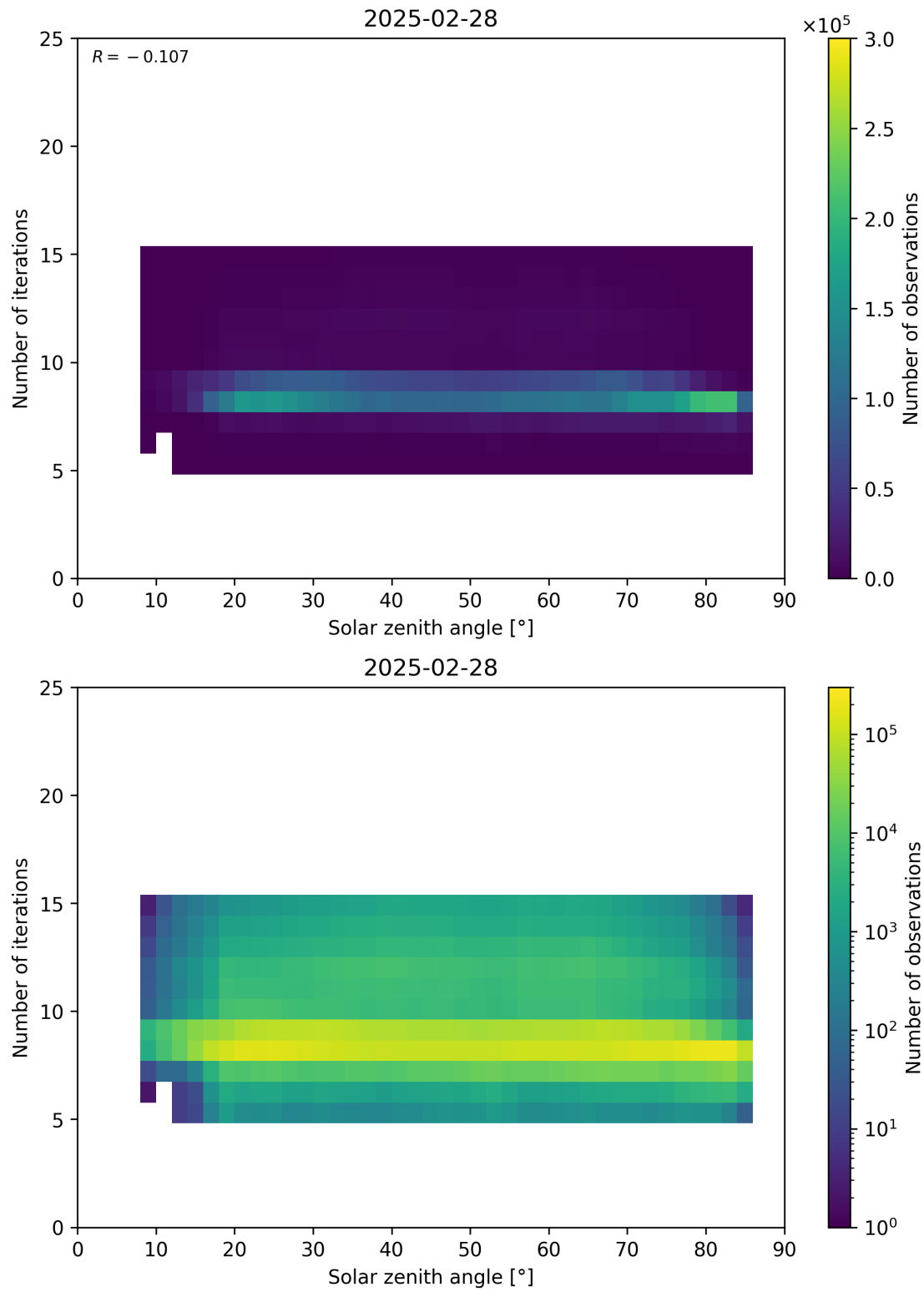
Figure 67: Scatter density plot of “Solar zenith angle” against “Number of iterations” for 2025-02-27 to 2025-03-01.
