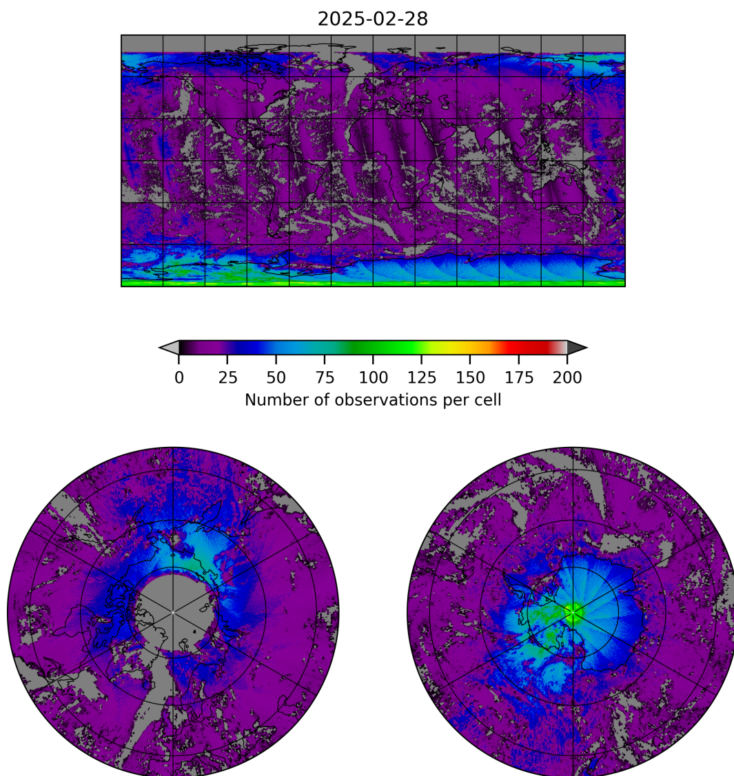
Figure 8: Map of the number of observations for 2025-02-27 to 2025-03-01
