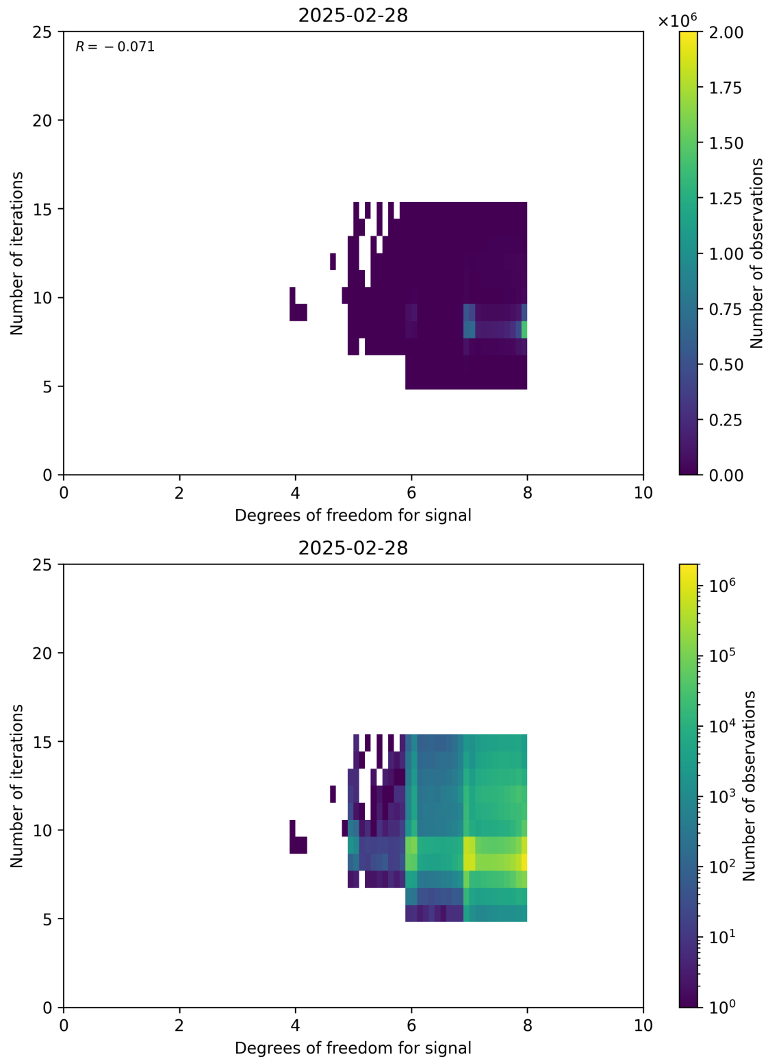
Figure 50: Scatter density plot of “Degrees of freedom for signal” against “Number of iterations” for 2025-02-27 to 2025-03-01.
