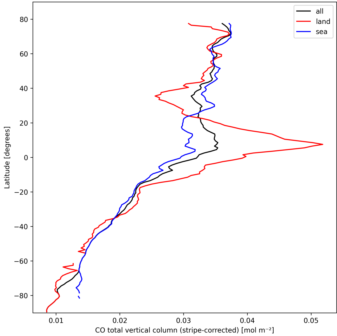
Figure 11: Zonal average of “CO total vertical column (stripe-corrected)” for 2025-02-27 to 2025-03-01.
