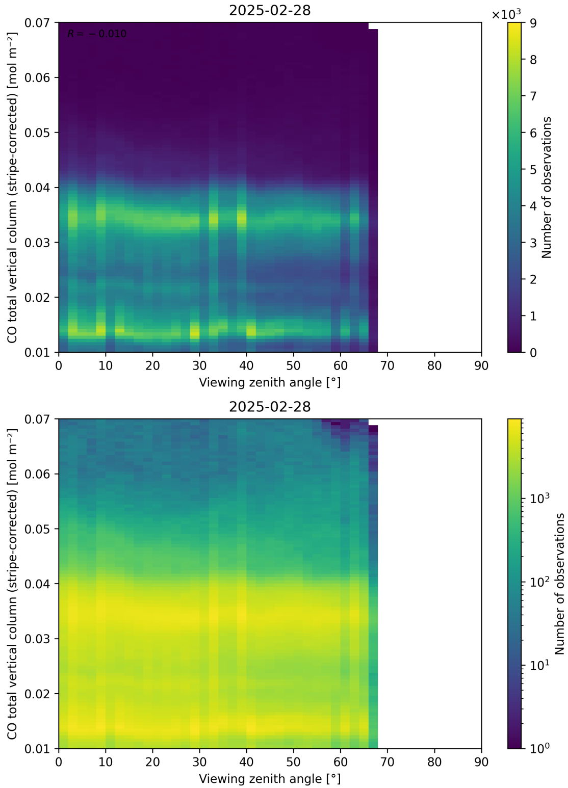
Figure 70: Scatter density plot of “Viewing zenith angle” against “CO total vertical column (stripe-corrected)” for 2025-02-27 to 2025-03-01.
