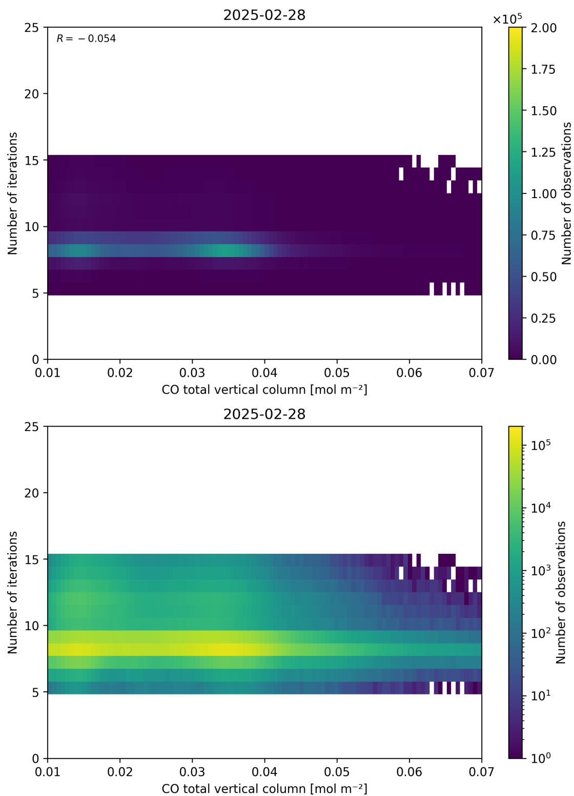
Figure 42: Scatter density plot of “CO total vertical column” against “Number of iterations” for 2025-02-27 to 2025-03-01.
