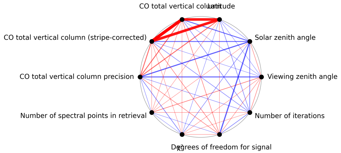
Figure 1: Map of correlation graph for 2025-02-27 to 2025-03-01.
