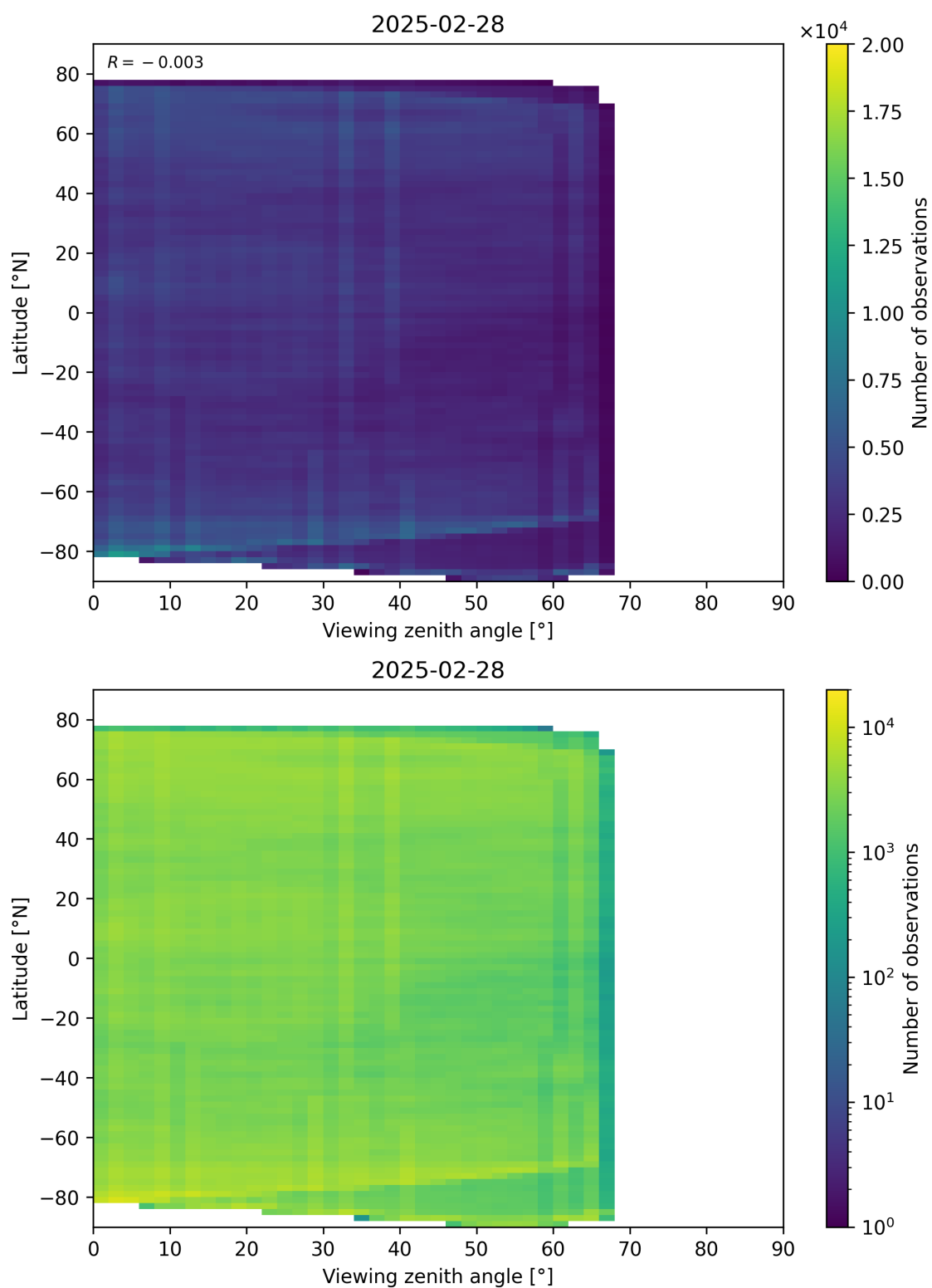
Figure 74: Scatter density plot of “Viewing zenith angle” against “Latitude” for 2025-02-27 to 2025-03-01.
