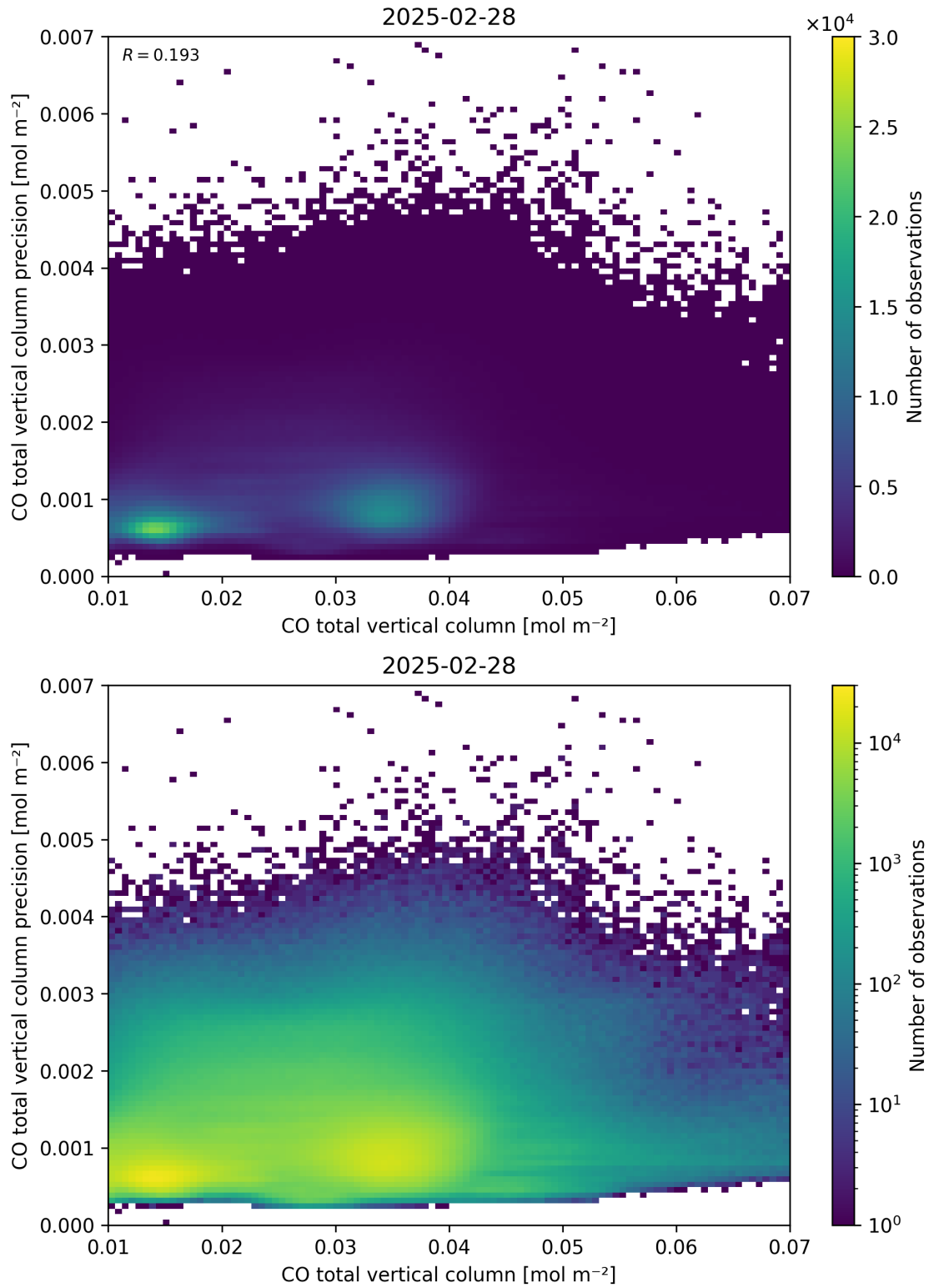
Figure 34: Scatter density plot of “CO total vertical column” against “CO total vertical column precision” for 2025-02-27 to 2025-03-01.
