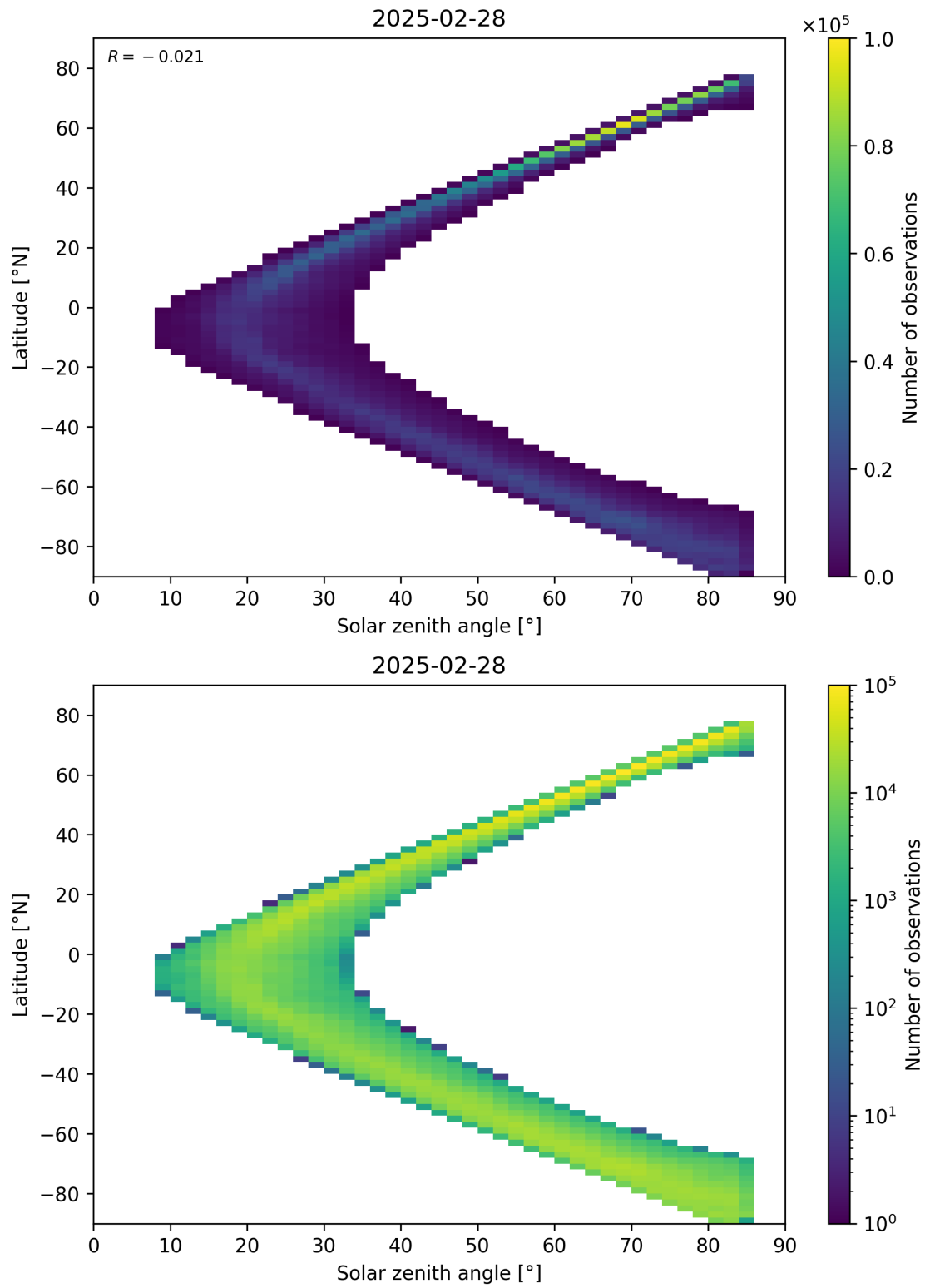
Figure 66: Scatter density plot of “Solar zenith angle” against “Latitude” for 2025-02-27 to 2025-03-01.
