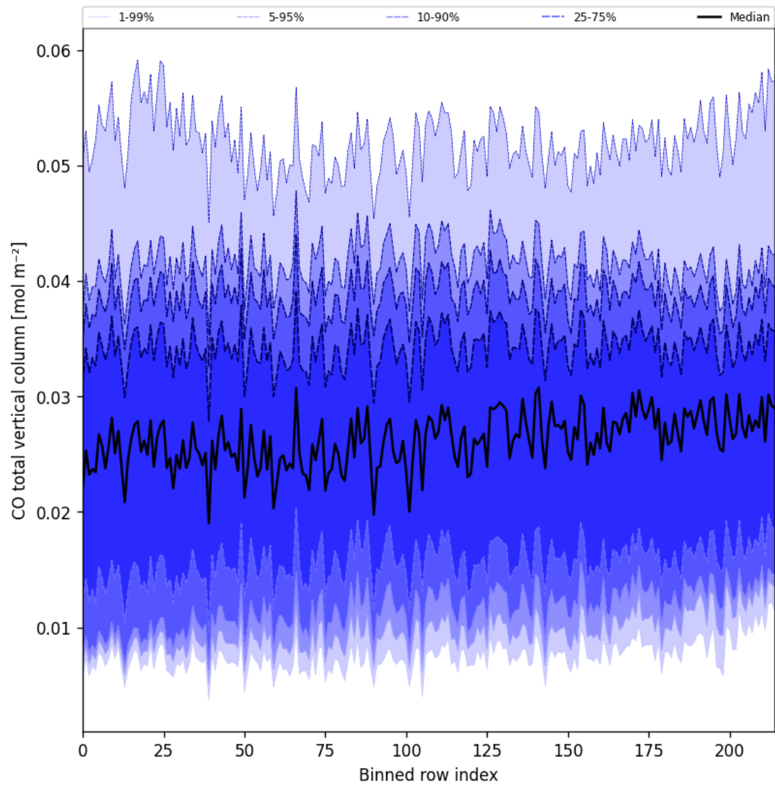
Figure 26: Along track statistics of “CO total vertical column” for 2025-02-27 to 2025-03-01
