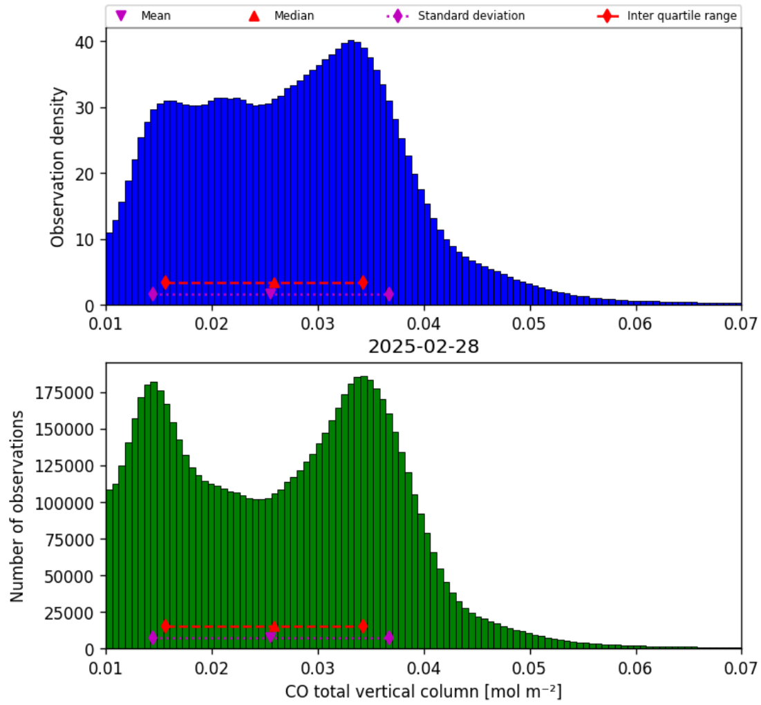
Figure 18: Histogram of “CO total vertical column” for 2025-02-27 to 2025-03-01
