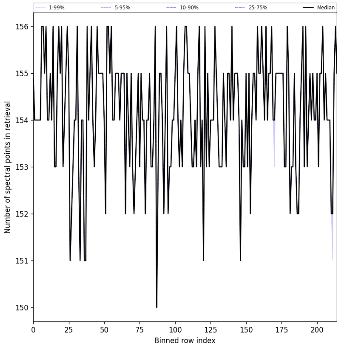
Figure 29: Along track statistics of “Number of spectral points in retrieval” for 2025-02-27 to 2025-03-01
