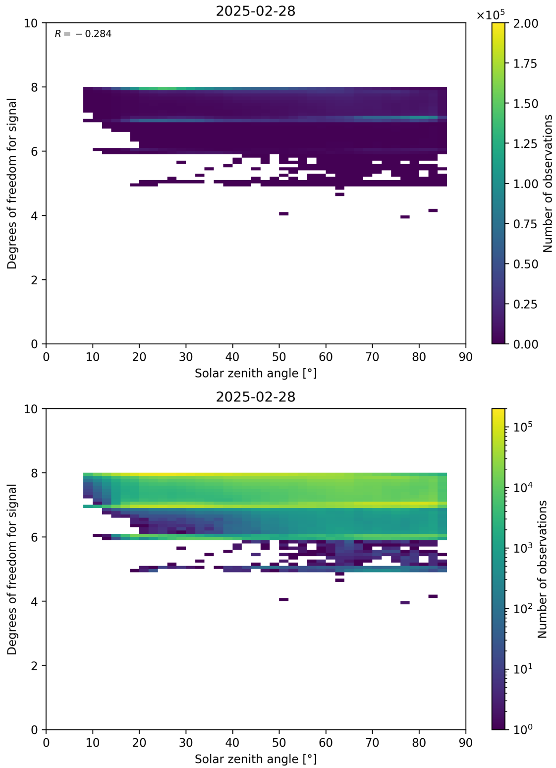
Figure 65: Scatter density plot of “Solar zenith angle” against “Degrees of freedom for signal” for 2025-02-27 to 2025-03-01.
