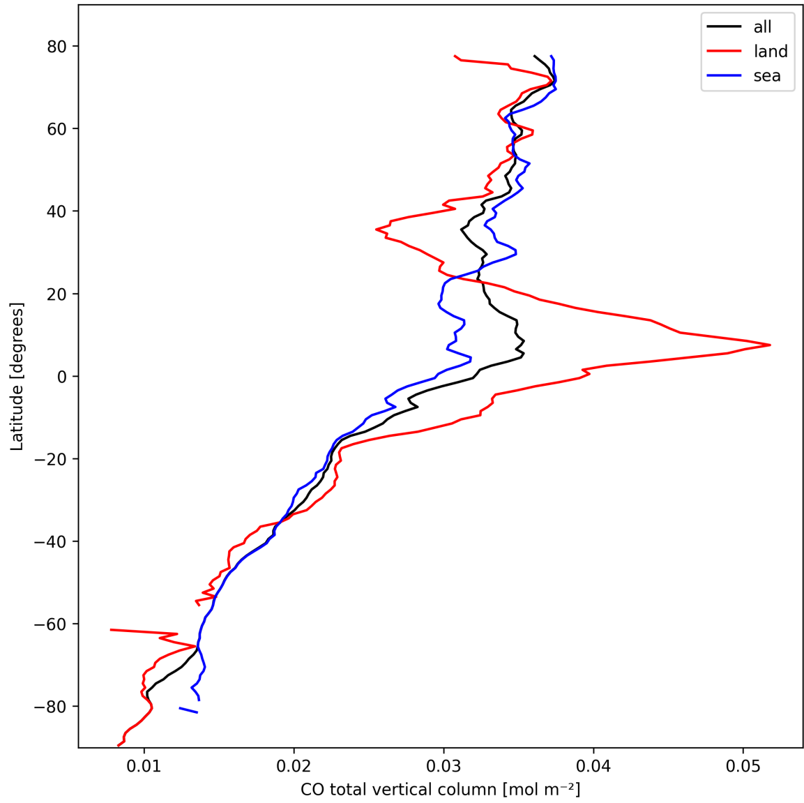
Figure 10: Zonal average of “CO total vertical column” for 2025-02-27 to 2025-03-01.
