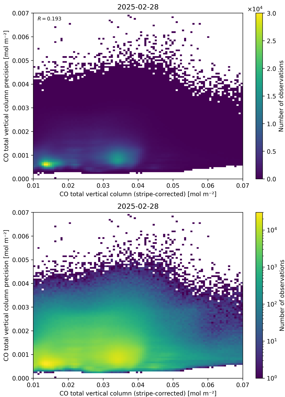
Figure 36: Scatter density plot of “CO total vertical column (stripe-corrected)” against “CO total vertical column precision” for 2025-02-27 to 2025-03-01.
