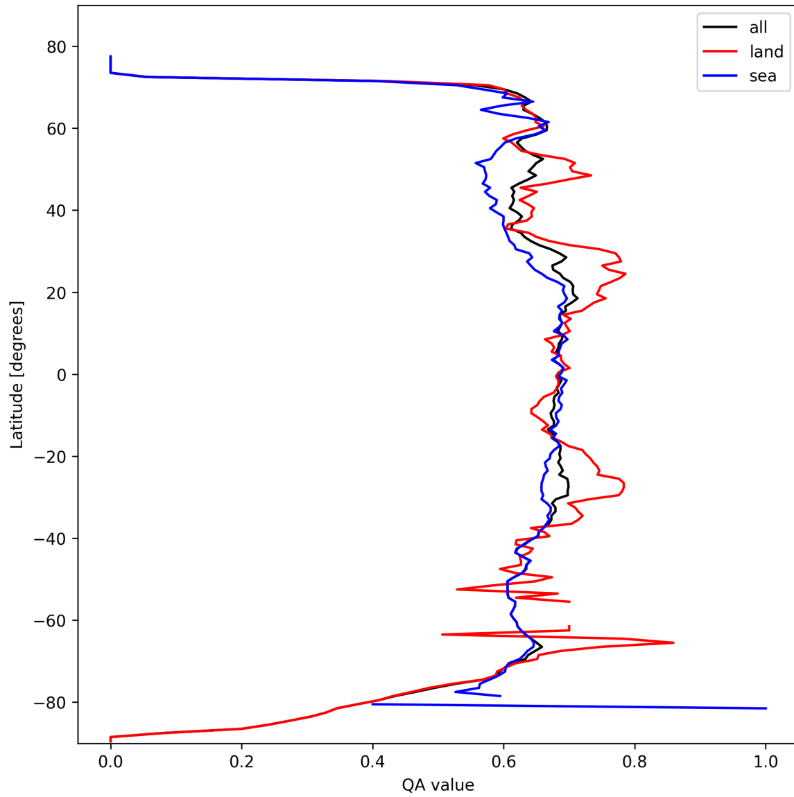
Figure 9: Zonal average of “QA value” for 2025-02-27 to 2025-03-01.
