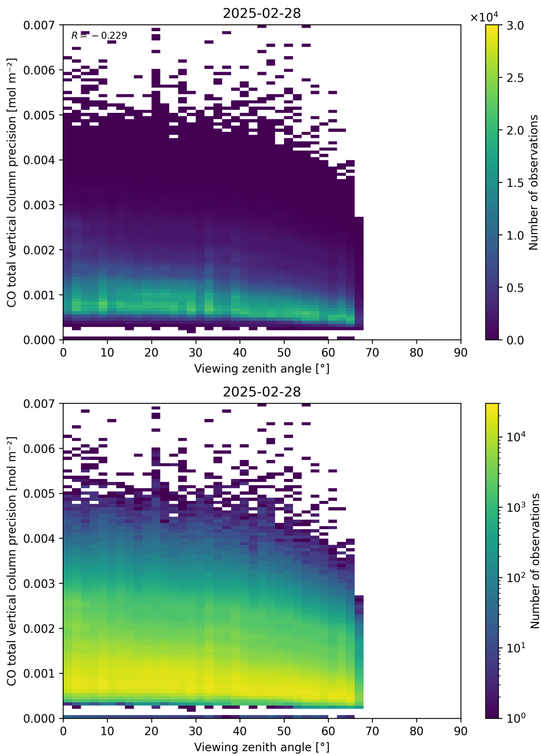
Figure 71: Scatter density plot of “Viewing zenith angle” against “CO total vertical column precision” for 2025-02-27 to 2025-03-01.
