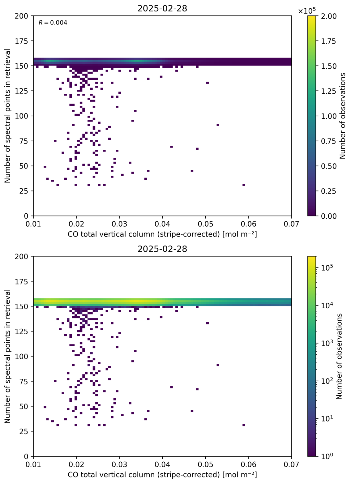
Figure 40: Scatter density plot of “CO total vertical column (stripe-corrected)” against “Number of spectral points in retrieval” for 2025-02-27 to 2025-03-01.
