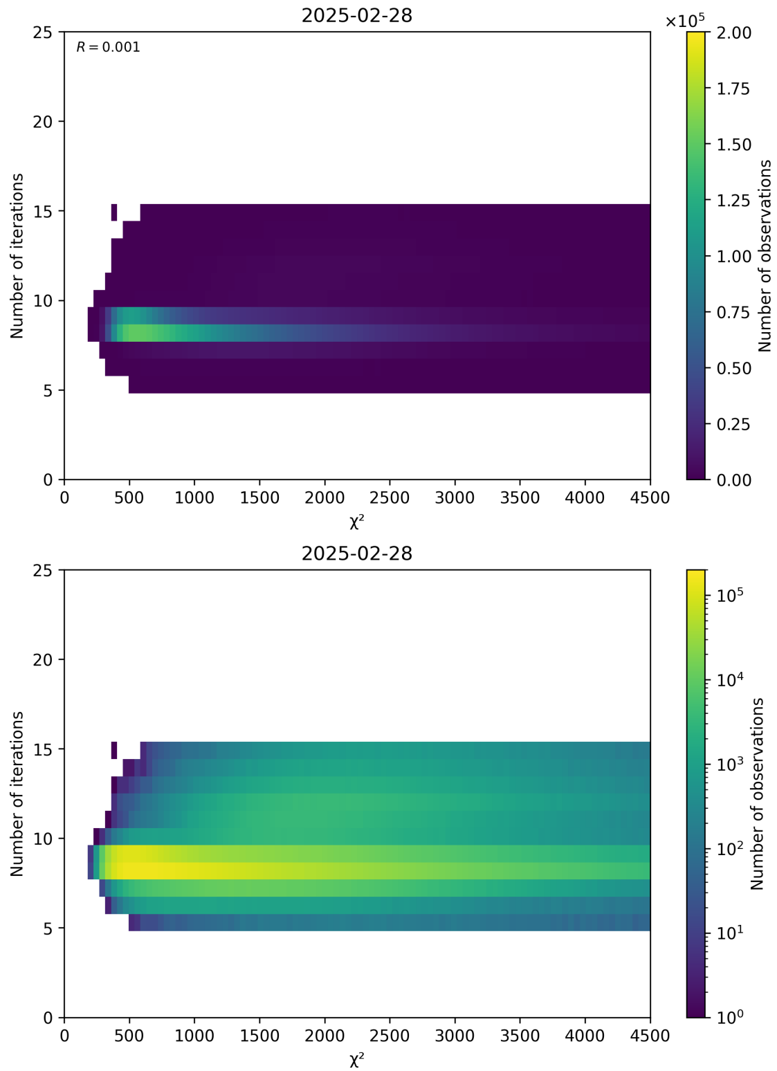
Figure 49: Scatter density plot of “ \chi^2 ” against “Number of iterations” for 2025-02-27 to 2025-03-01.
