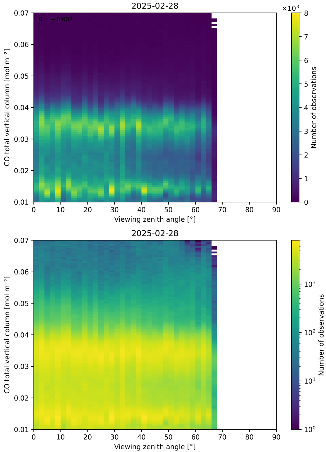
Figure 69: Scatter density plot of “Viewing zenith angle” against “CO total vertical column” for 2025-02-27 to 2025-03-01.
