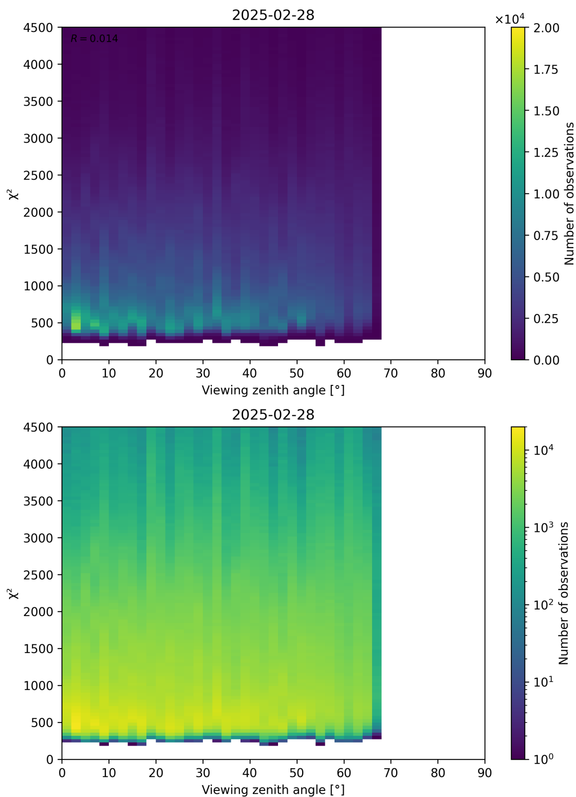
Figure 72: Scatter density plot of “Viewing zenith angle” against “ \chi^2 ” for 2025-02-27 to 2025-03-01.
