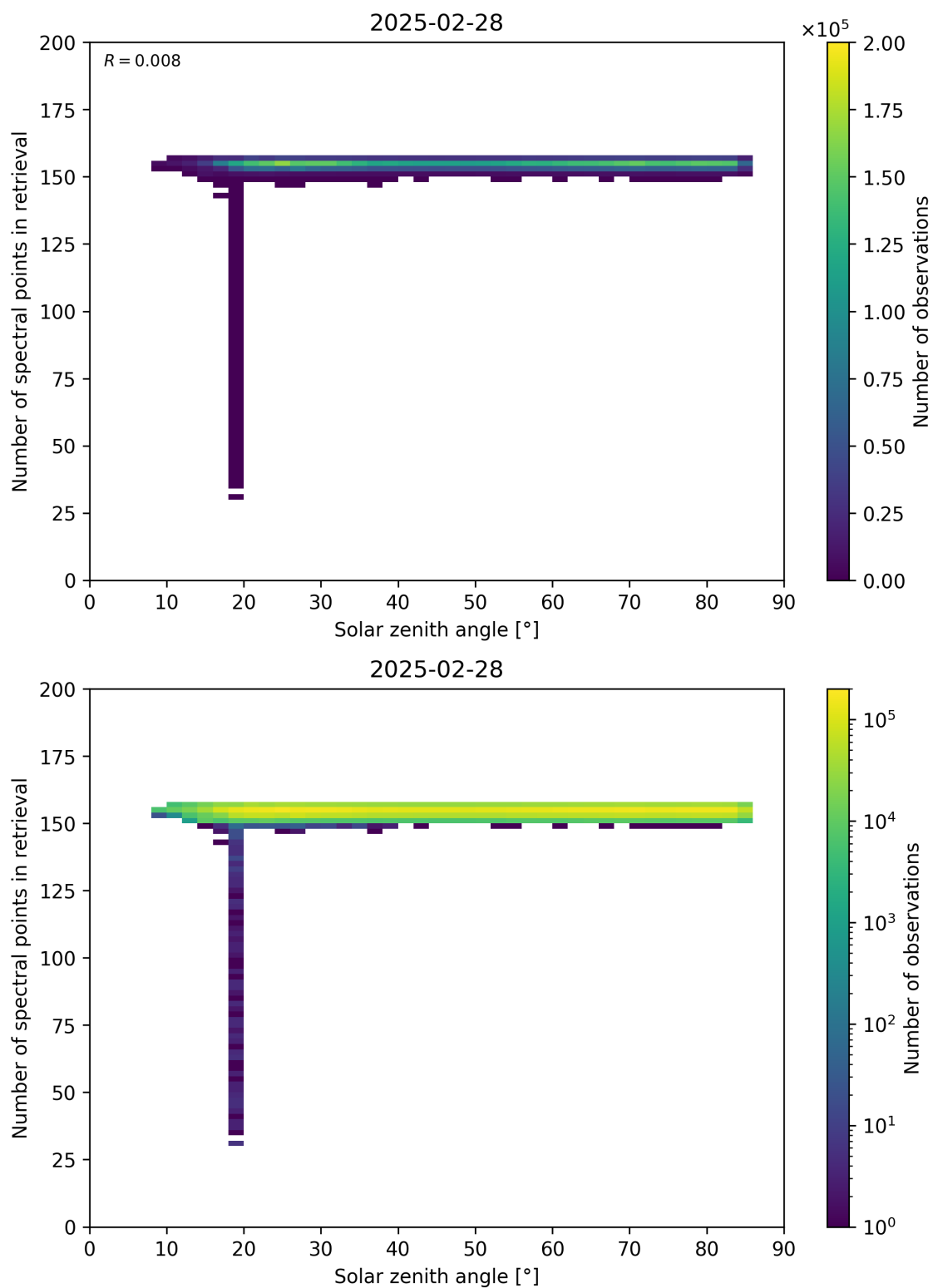
Figure 68: Scatter density plot of “Solar zenith angle” against “Number of spectral points in retrieval” for 2025-02-27 to 2025-03-01.
