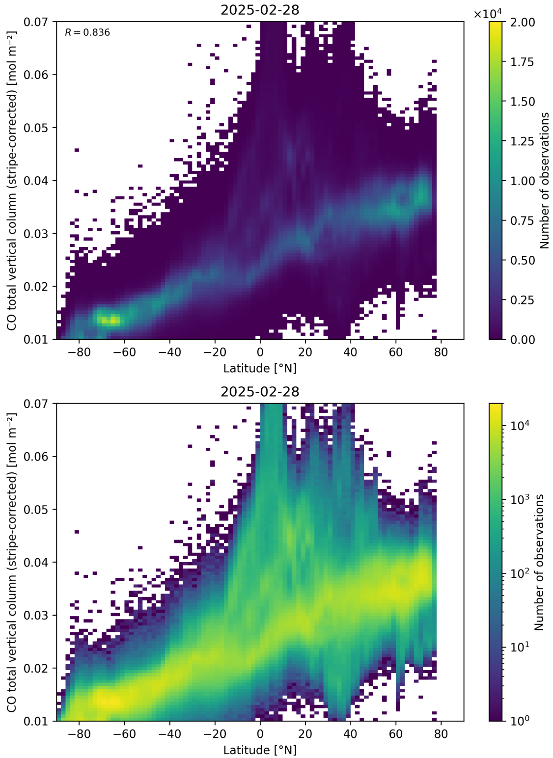
Figure 52: Scatter density plot of “Latitude” against “CO total vertical column (stripe-corrected)” for 2025-02-27 to 2025-03-01.
