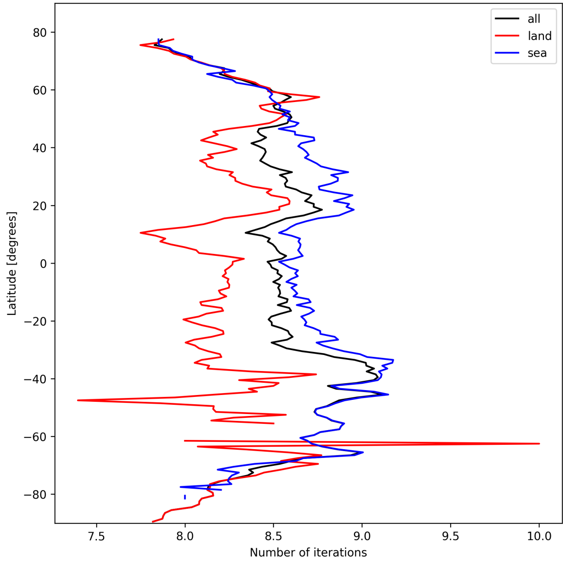
Figure 16: Zonal average of “Number of iterations” for 2025-02-27 to 2025-03-01.
