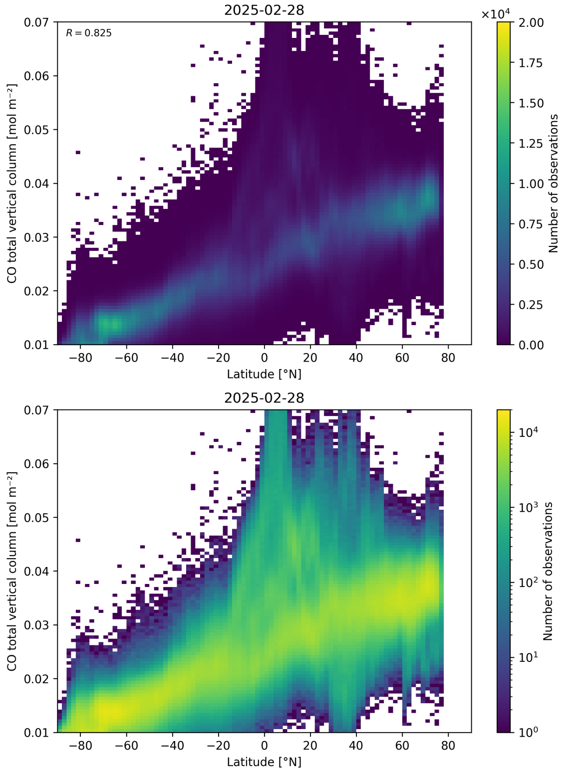
Figure 51: Scatter density plot of “Latitude” against “CO total vertical column” for 2025-02-27 to 2025-03-01.
