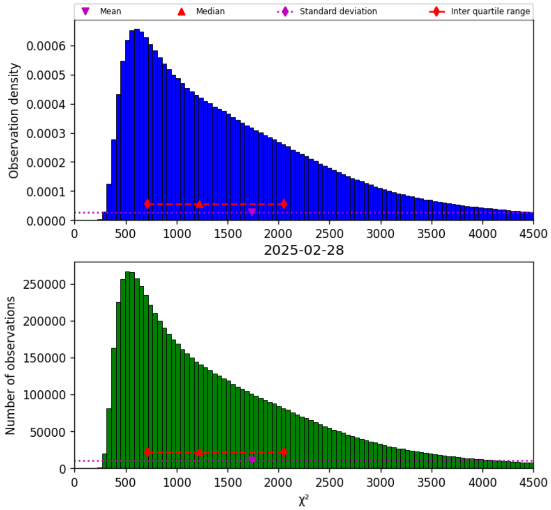
Figure 22: Histogram of “ \chi^2 ” for 2025-02-27 to 2025-03-01
