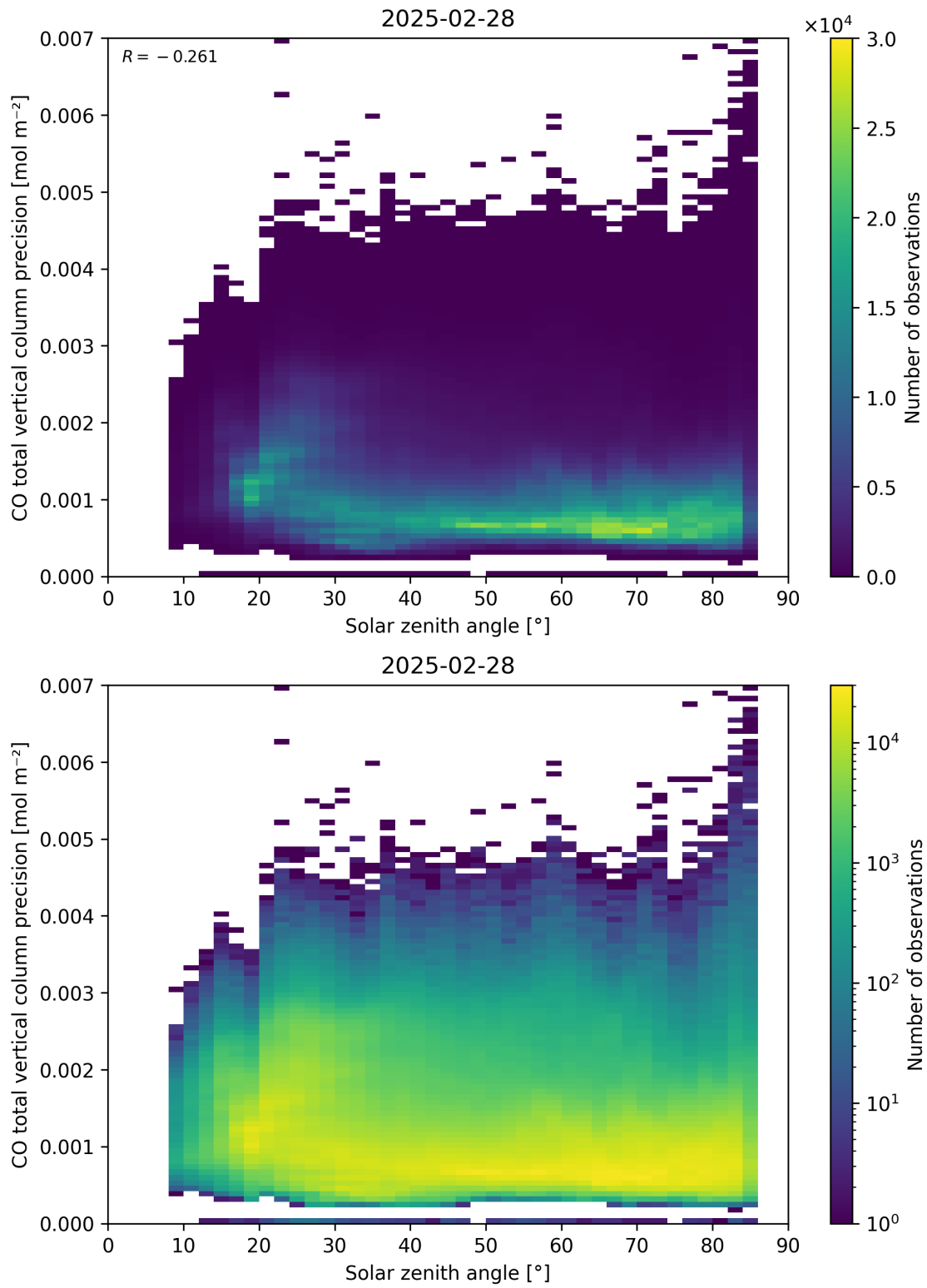
Figure 63: Scatter density plot of “Solar zenith angle” against “CO total vertical column precision” for 2025-02-27 to 2025-03-01.
