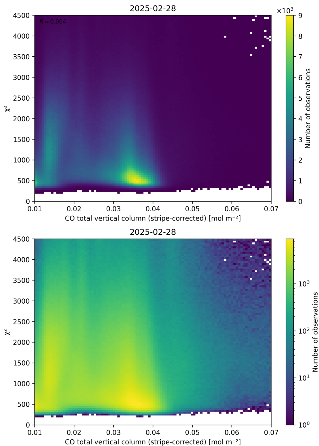
Figure 37: Scatter density plot of “CO total vertical column (stripe-corrected)” against “ \chi^2 ” for 2025-02-27 to 2025-03-01.
