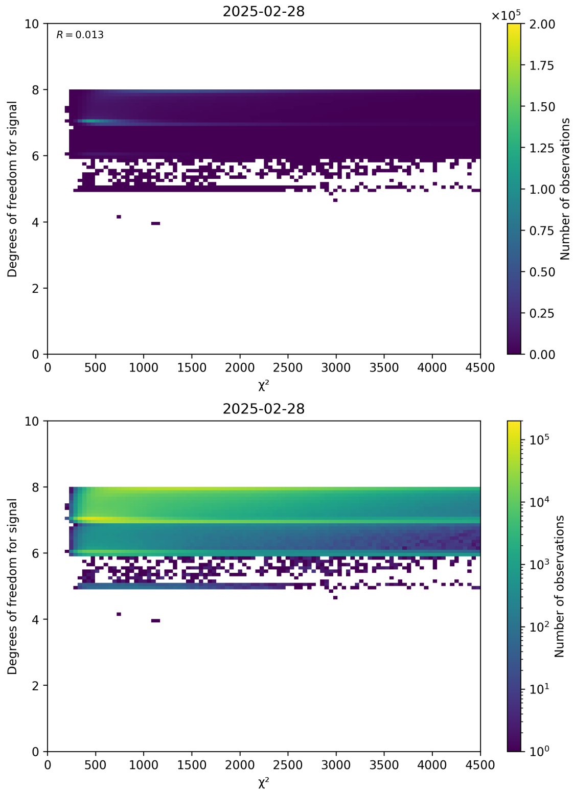
Figure 48: Scatter density plot of “ \chi^2 ” against “Degrees of freedom for signal” for 2025-02-27 to 2025-03-01.
