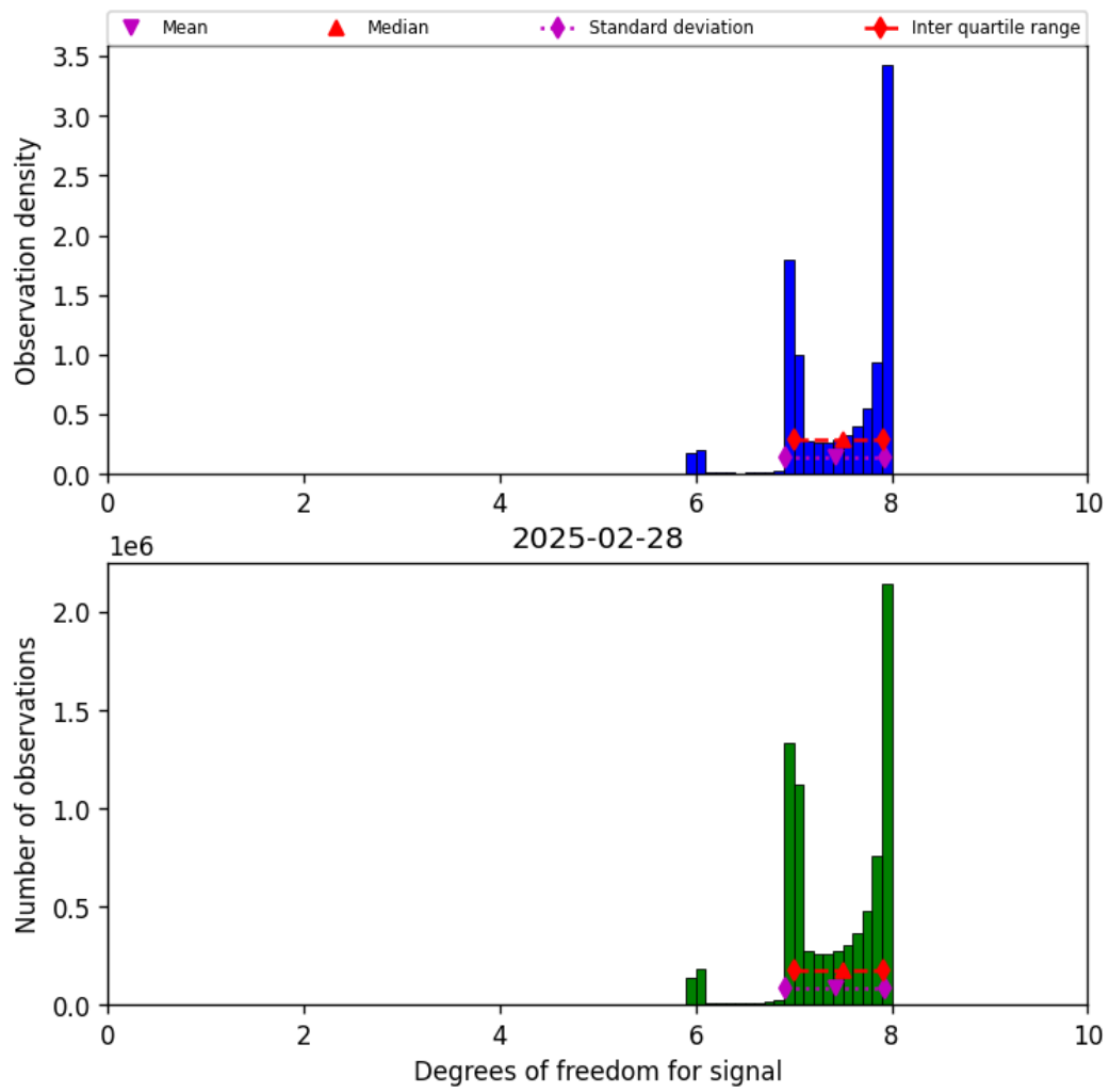
Figure 23: Histogram of “Degrees of freedom for signal” for 2025-02-27 to 2025-03-01
