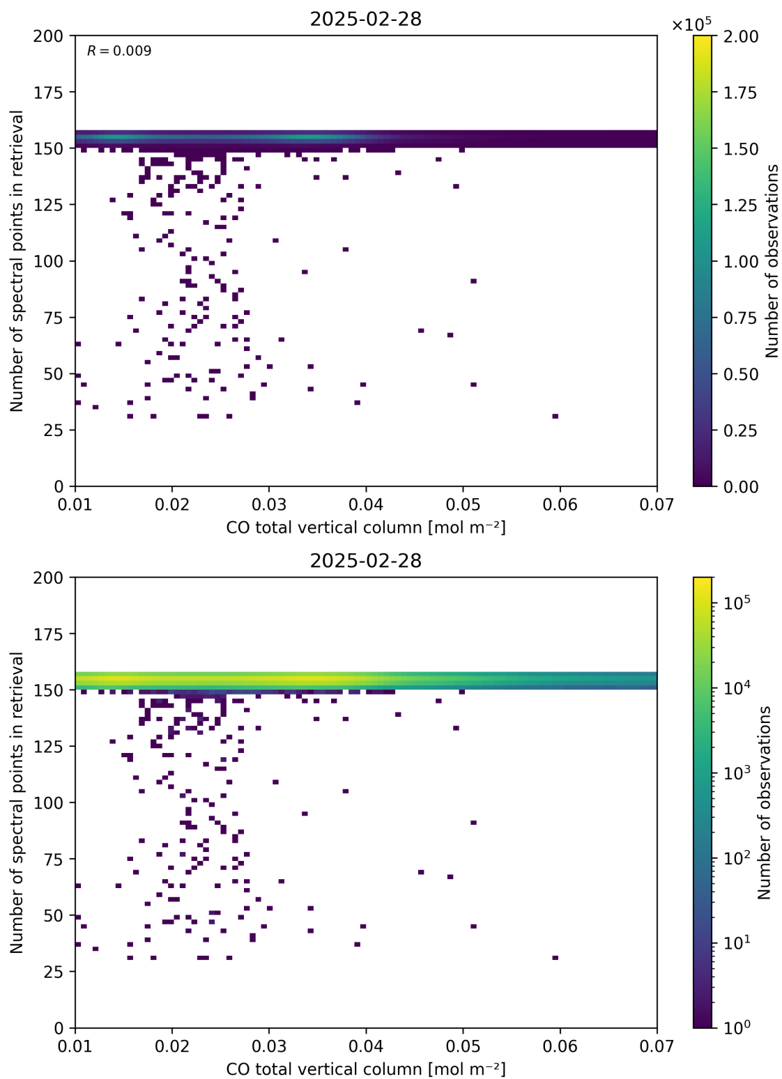
Figure 43: Scatter density plot of “CO total vertical column” against “Number of spectral points in retrieval” for 2025-02-27 to 2025-03-01.
