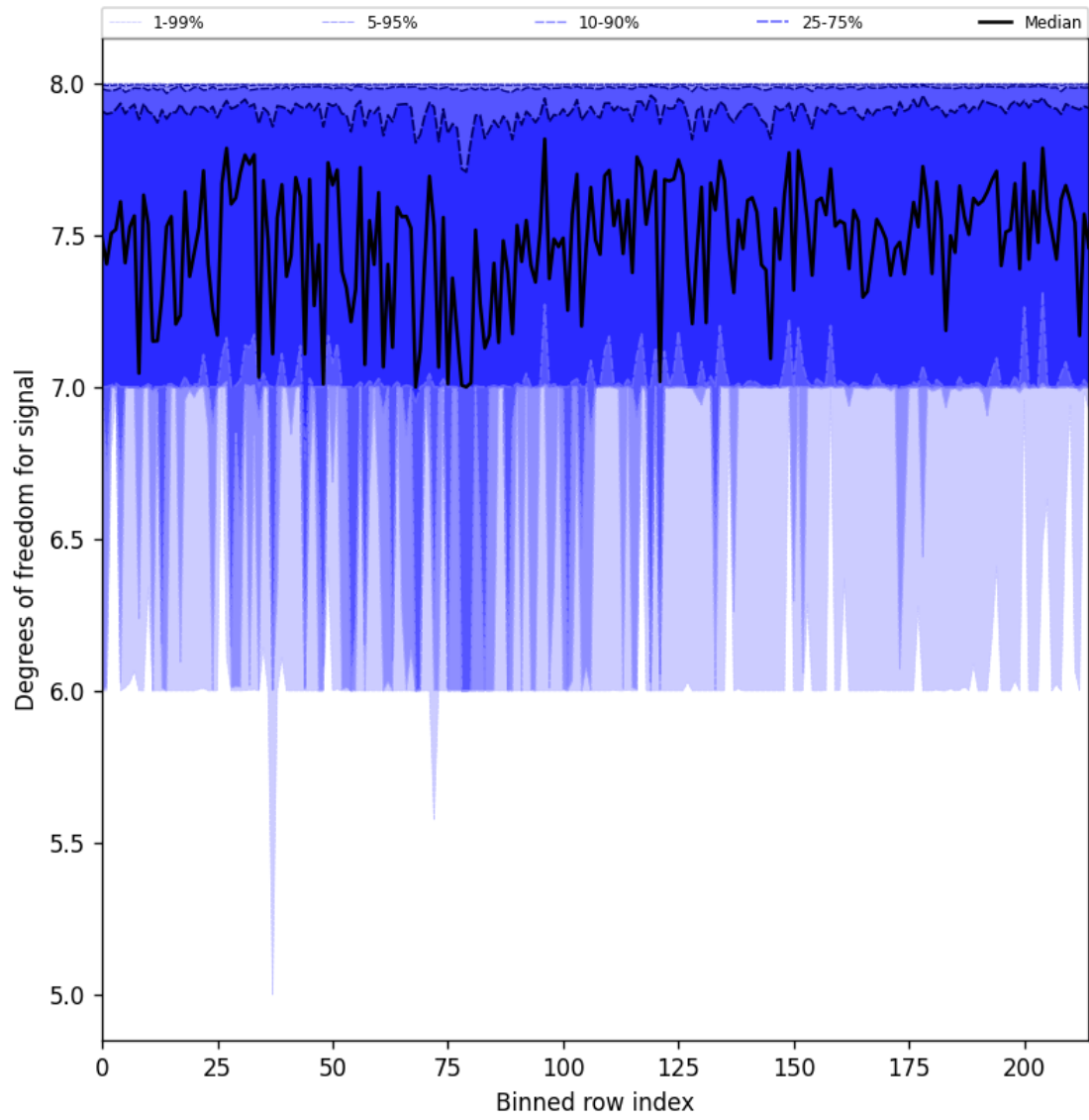
Figure 31: Along track statistics of “Degrees of freedom for signal” for 2025-02-27 to 2025-03-01
