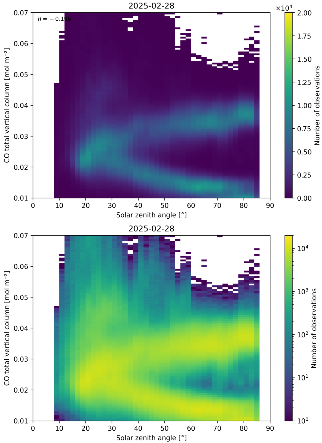
Figure 61: Scatter density plot of “Solar zenith angle” against “CO total vertical column” for 2025-02-27 to 2025-03-01.
