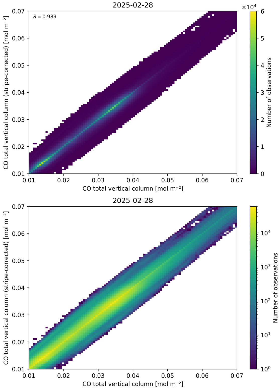
Figure 33: Scatter density plot of “CO total vertical column” against “CO total vertical column (stripe-corrected)” for 2025-02-27 to 2025-03-01.
