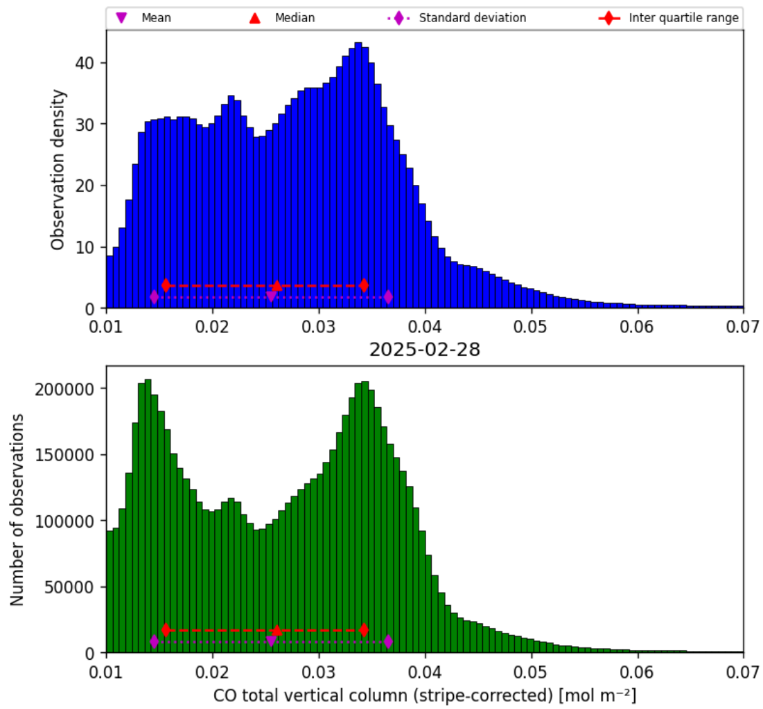
Figure 19: Histogram of “CO total vertical column (stripe-corrected)” for 2025-02-27 to 2025-03-01
