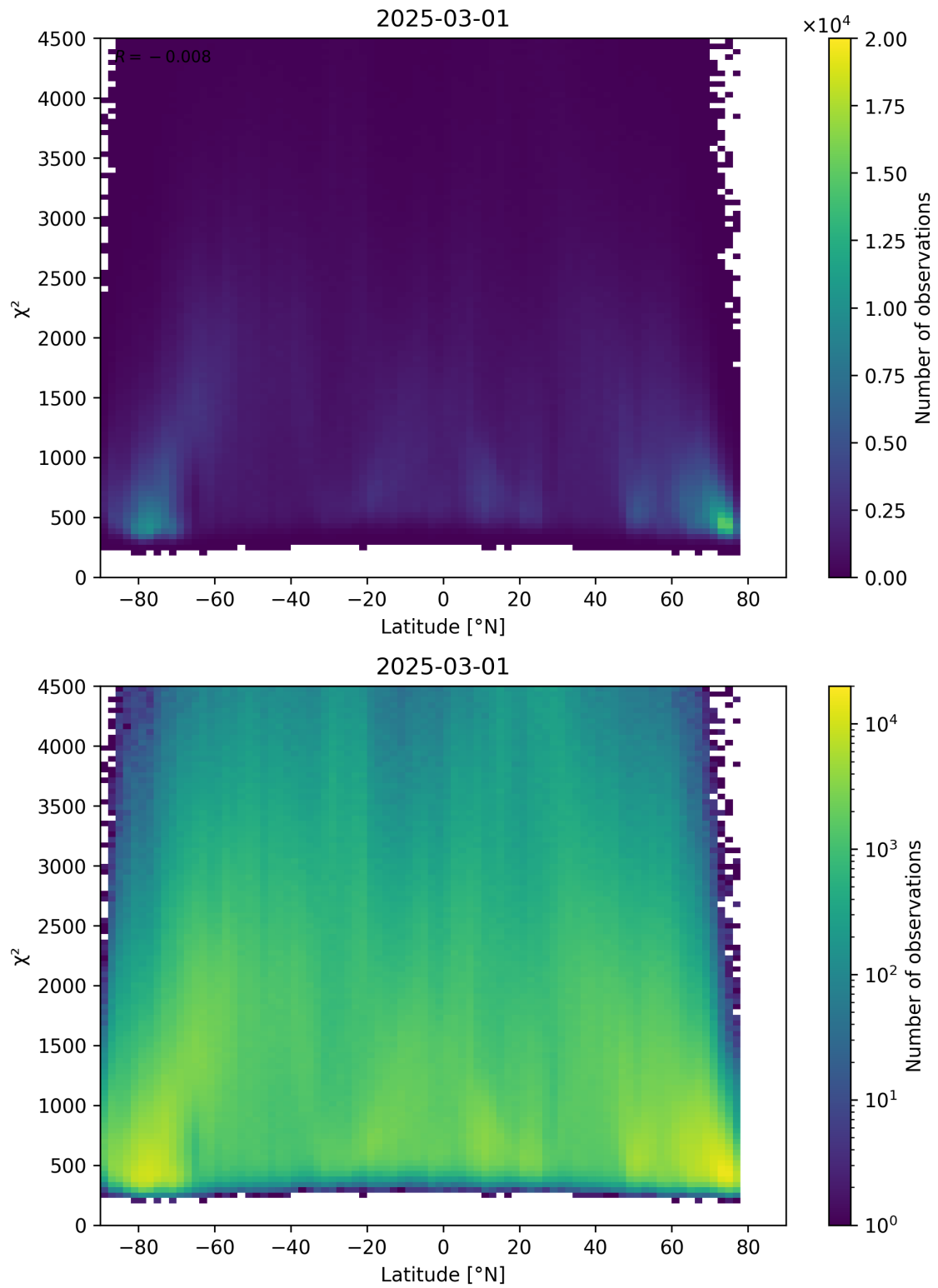
Figure 54: Scatter density plot of “Latitude” against “ \chi^2 ” for 2025-03-01 to 2025-03-02.
