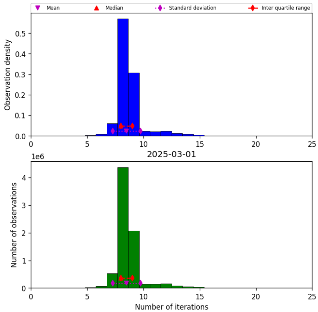
Figure 24: Histogram of “Number of iterations” for 2025-03-01 to 2025-03-02
