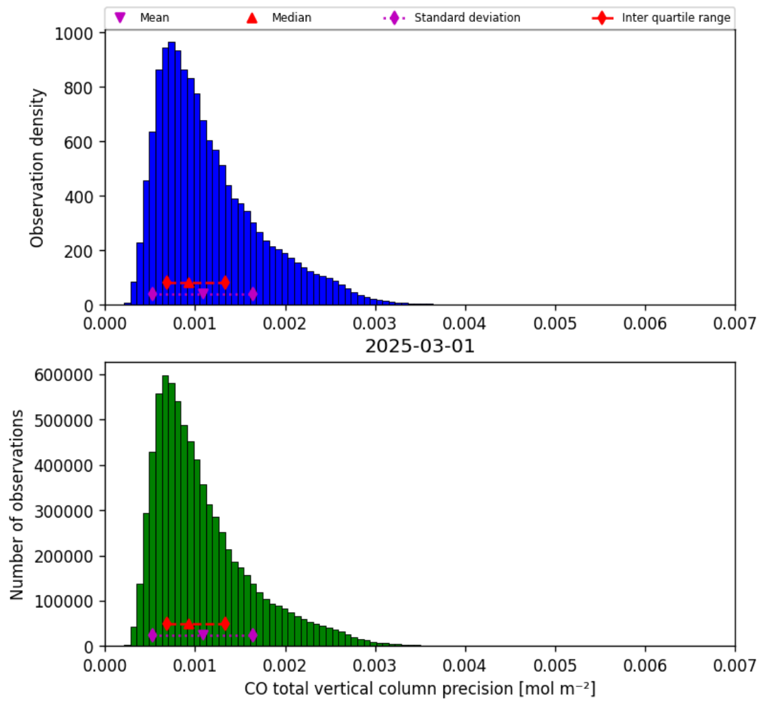
Figure 20: Histogram of “CO total vertical column precision” for 2025-03-01 to 2025-03-02
