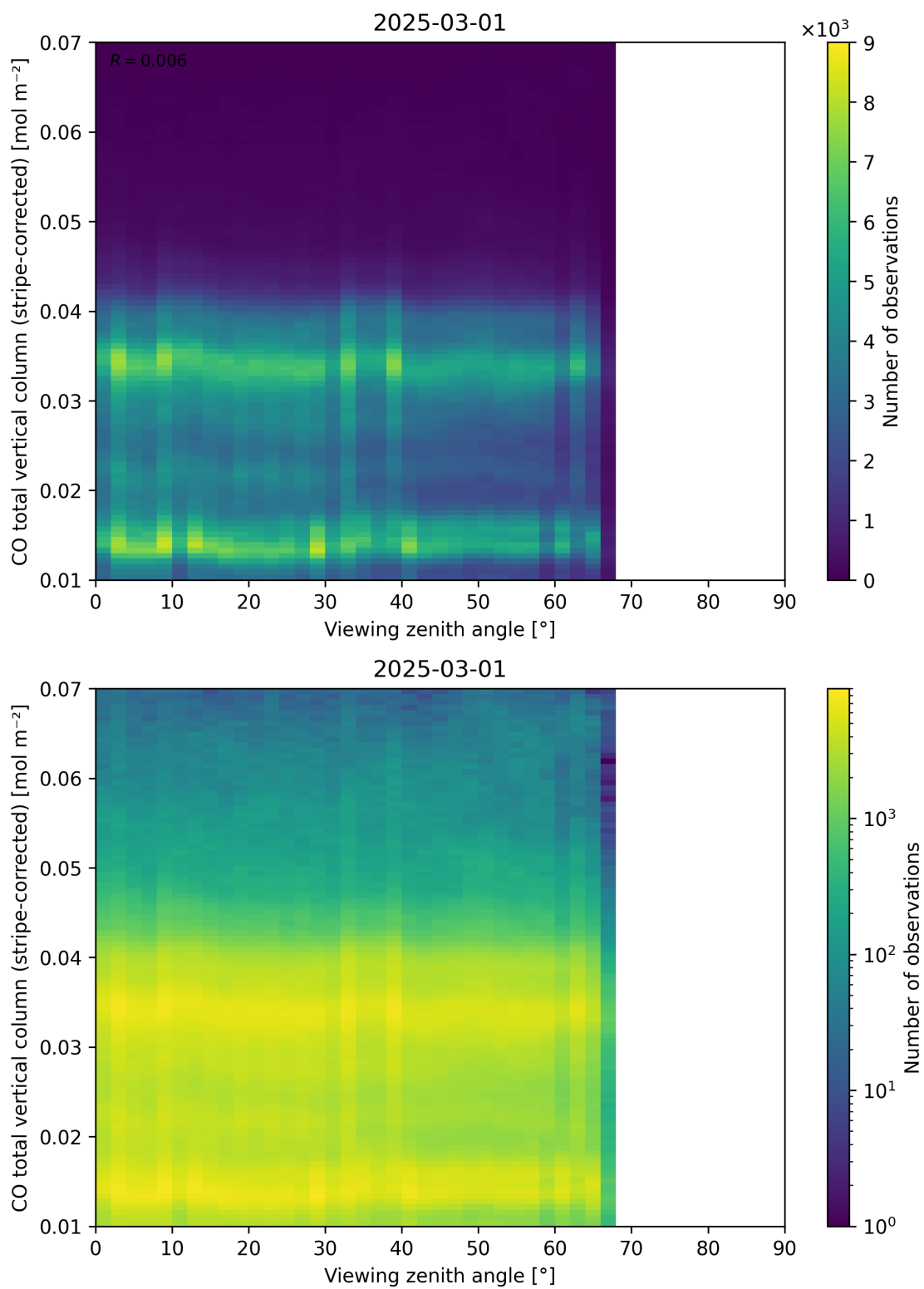
Figure 70: Scatter density plot of “Viewing zenith angle” against “CO total vertical column (stripe-corrected)” for 2025-03-01 to 2025-03-02.
