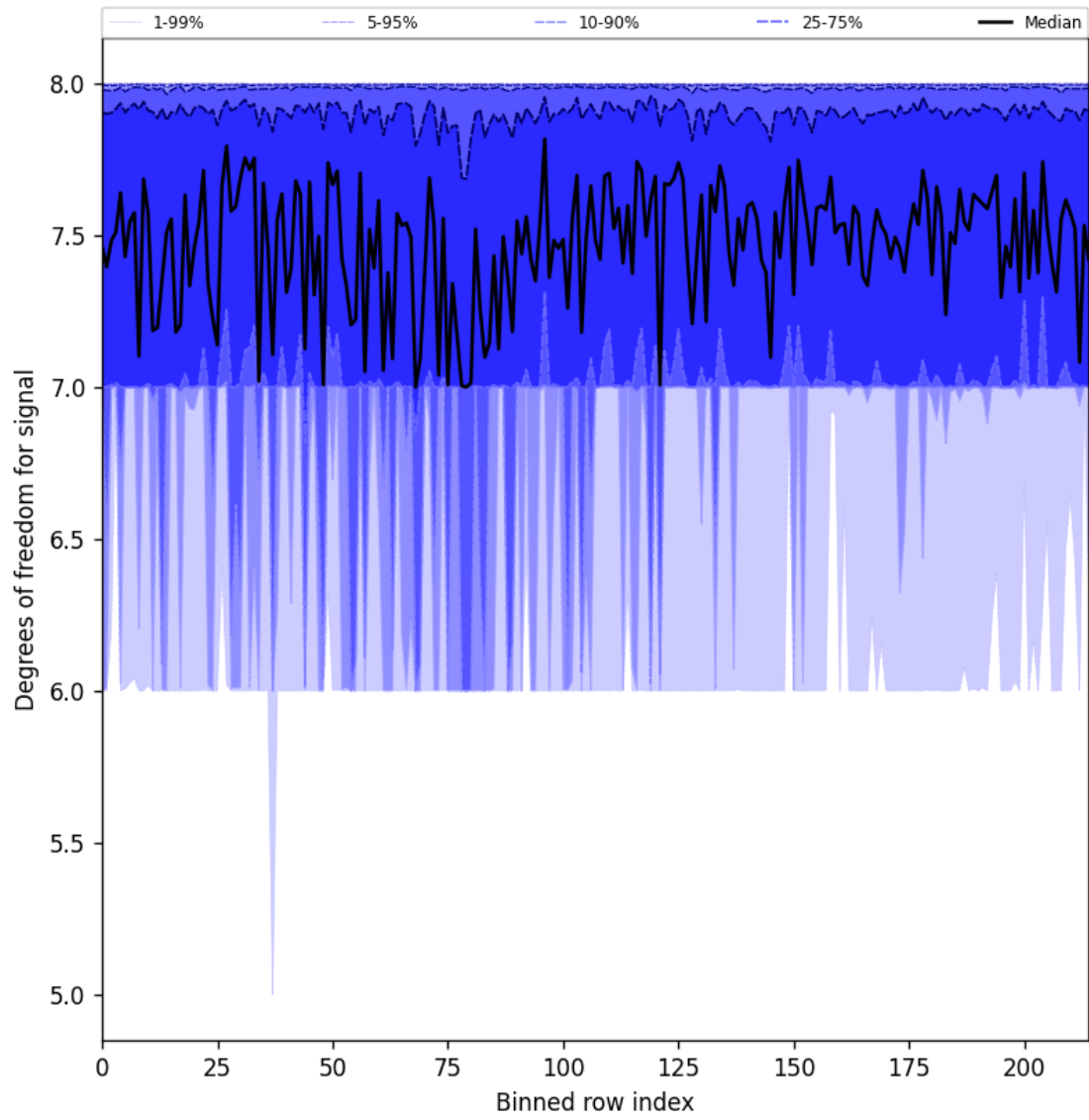
Figure 31: Along track statistics of “Degrees of freedom for signal” for 2025-03-01 to 2025-03-02
