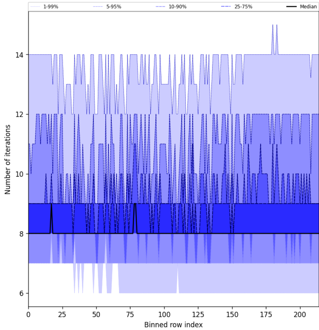
Figure 32: Along track statistics of “Number of iterations” for 2025-03-01 to 2025-03-02
