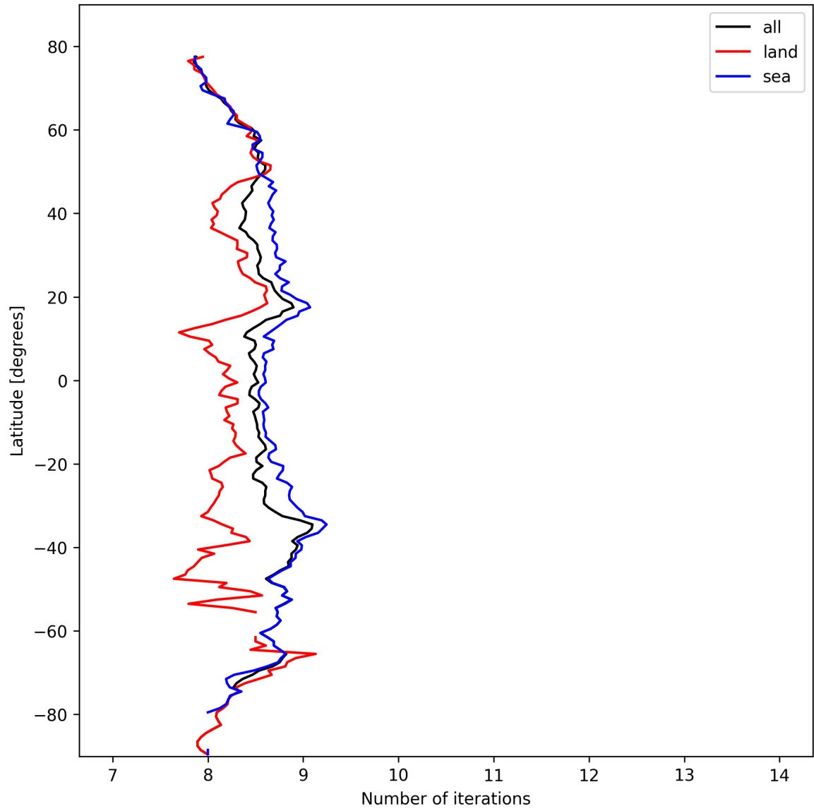
Figure 16: Zonal average of “Number of iterations” for 2025-03-01 to 2025-03-02.
