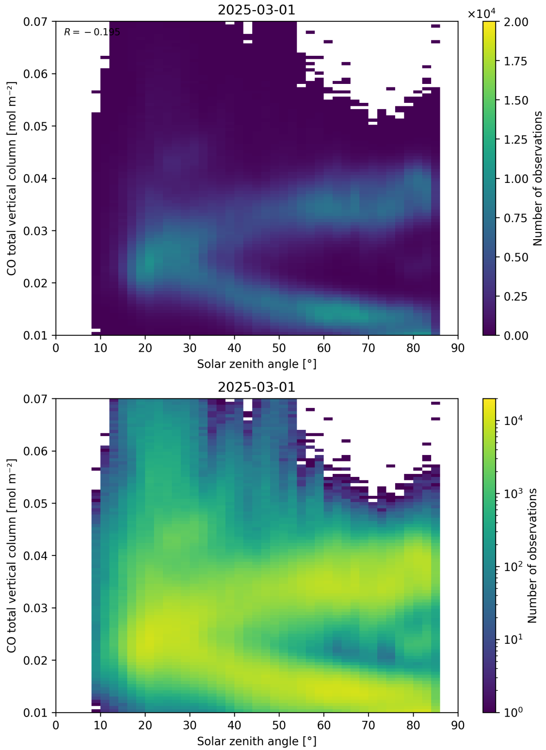
Figure 61: Scatter density plot of “Solar zenith angle” against “CO total vertical column” for 2025-03-01 to 2025-03-02.
