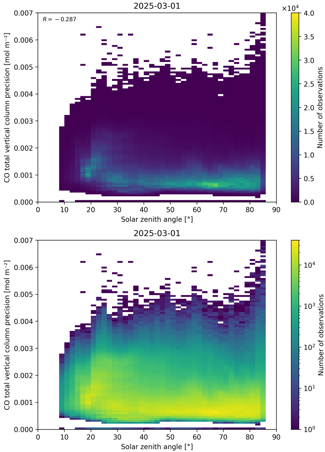
Figure 63: Scatter density plot of “Solar zenith angle” against “CO total vertical column precision” for 2025-03-01 to 2025-03-02.
