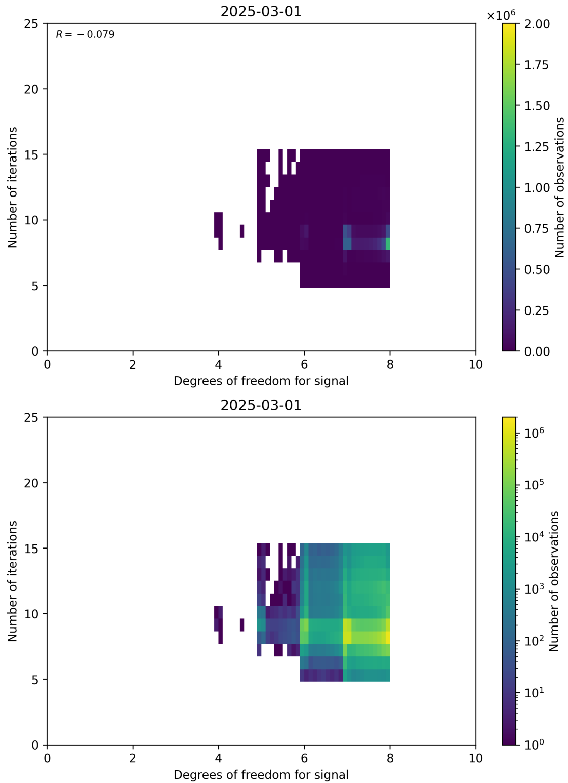
Figure 50: Scatter density plot of “Degrees of freedom for signal” against “Number of iterations” for 2025-03-01 to 2025-03-02.
