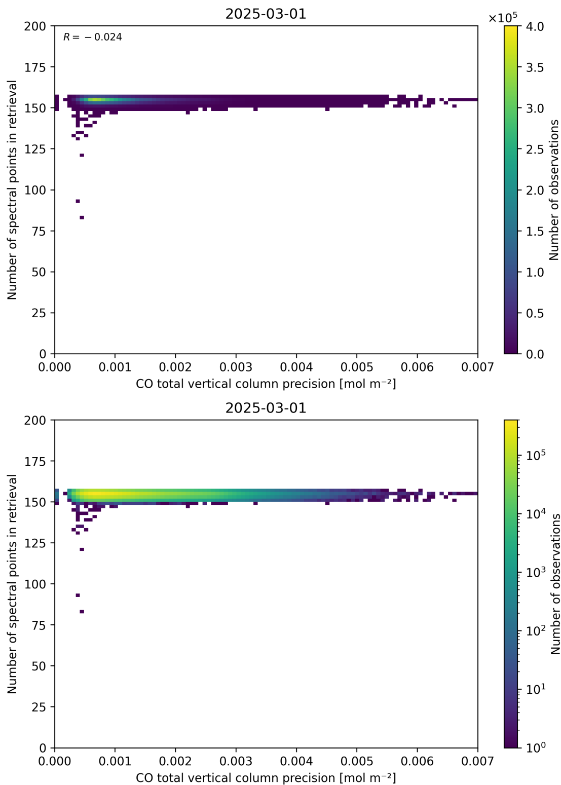
Figure 47: Scatter density plot of “CO total vertical column precision” against “Number of spectral points in retrieval” for 2025-03-01 to 2025-03-02.
