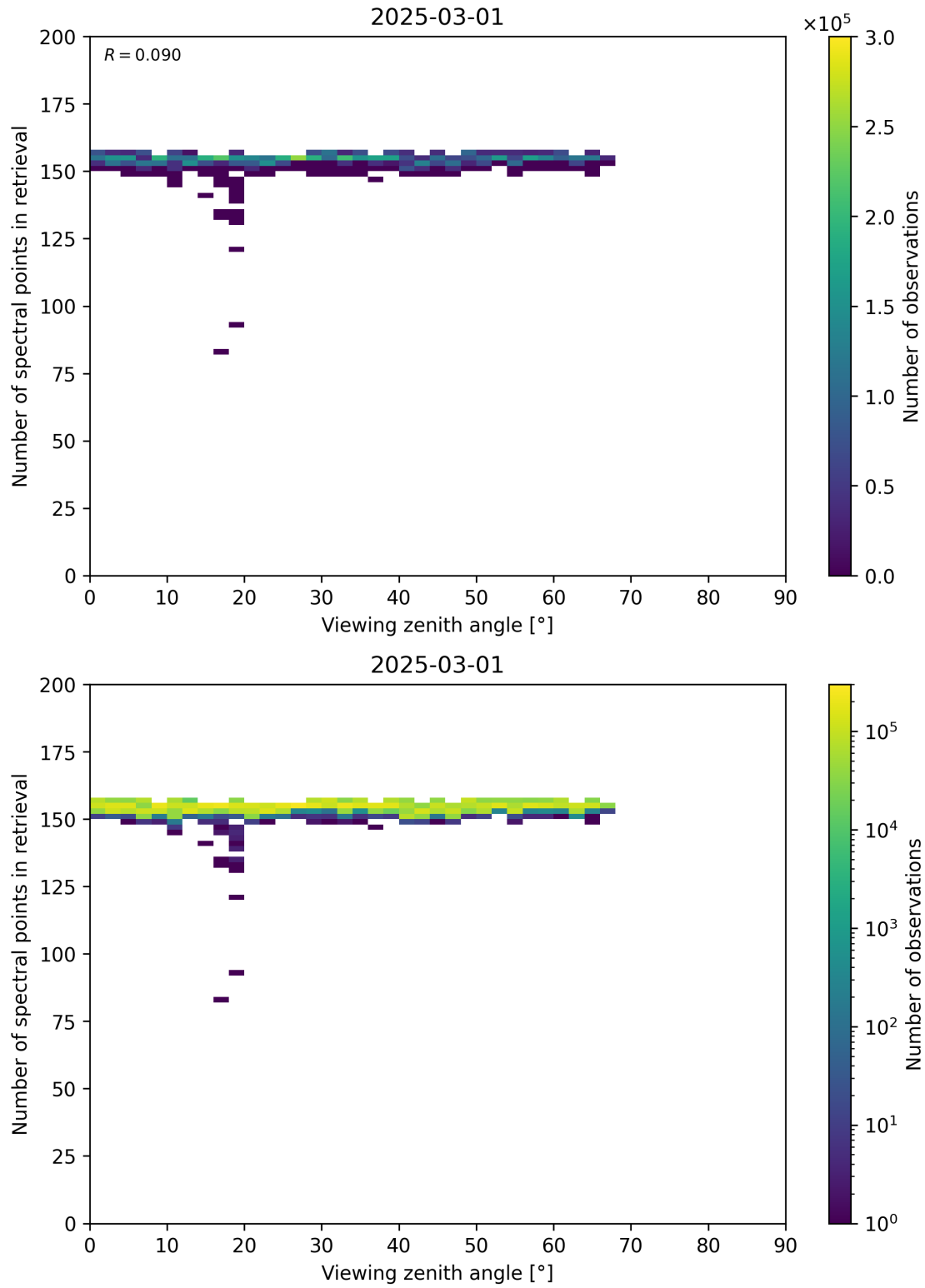
Figure 76: Scatter density plot of “Viewing zenith angle” against “Number of spectral points in retrieval” for 2025-03-01 to 2025-03-02.
