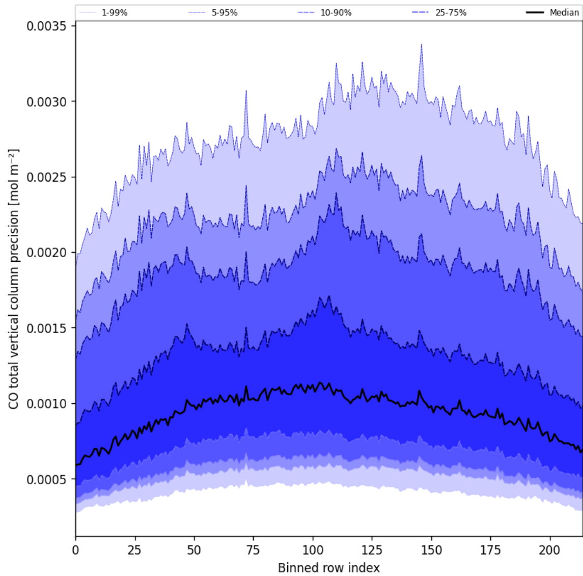
Figure 28: Along track statistics of “CO total vertical column precision” for 2025-03-01 to 2025-03-02
