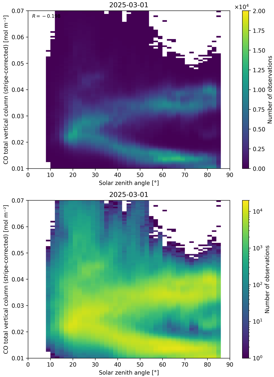
Figure 62: Scatter density plot of “Solar zenith angle” against “CO total vertical column (stripe-corrected)” for 2025-03-01 to 2025-03-02.
