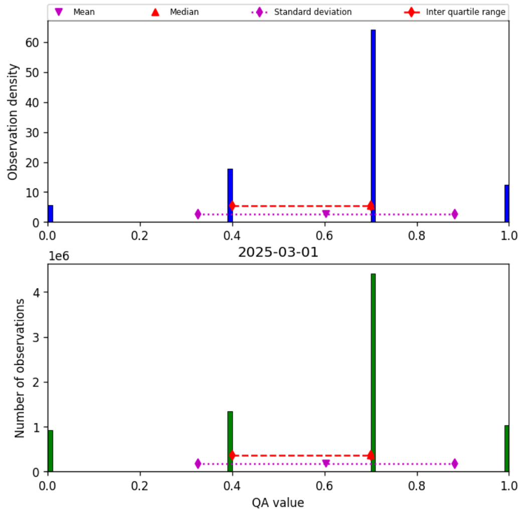
Figure 17: Histogram of “QA value” for 2025-03-01 to 2025-03-02
