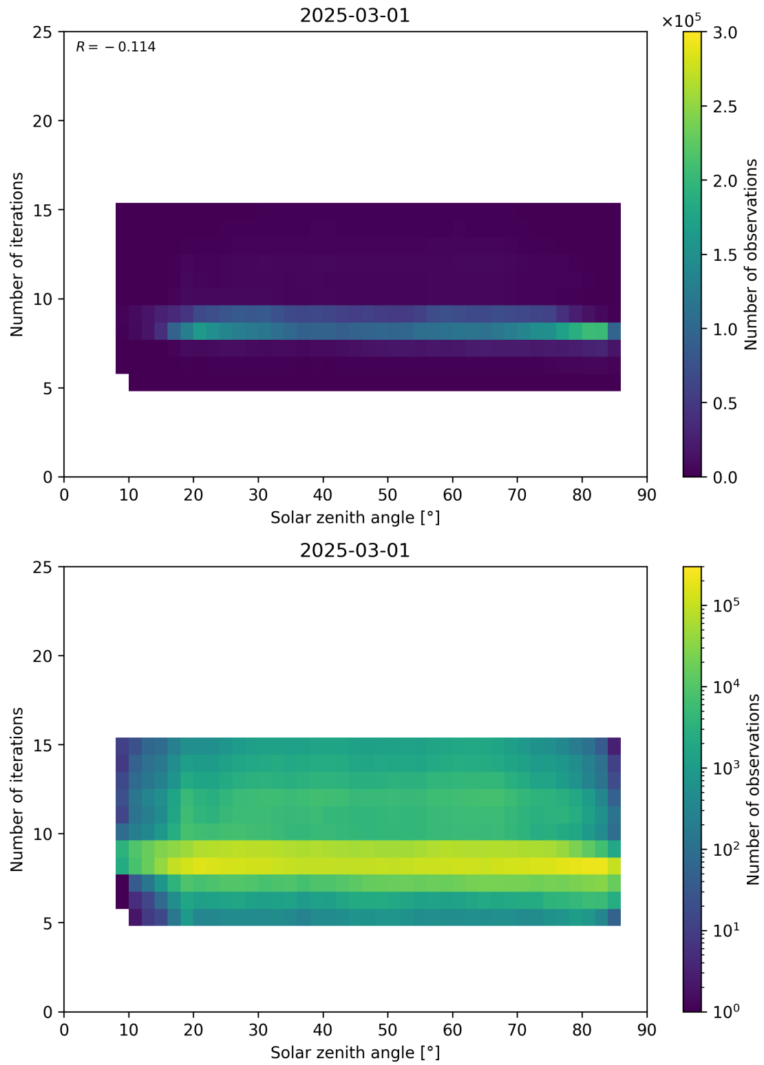
Figure 67: Scatter density plot of “Solar zenith angle” against “Number of iterations” for 2025-03-01 to 2025-03-02.
