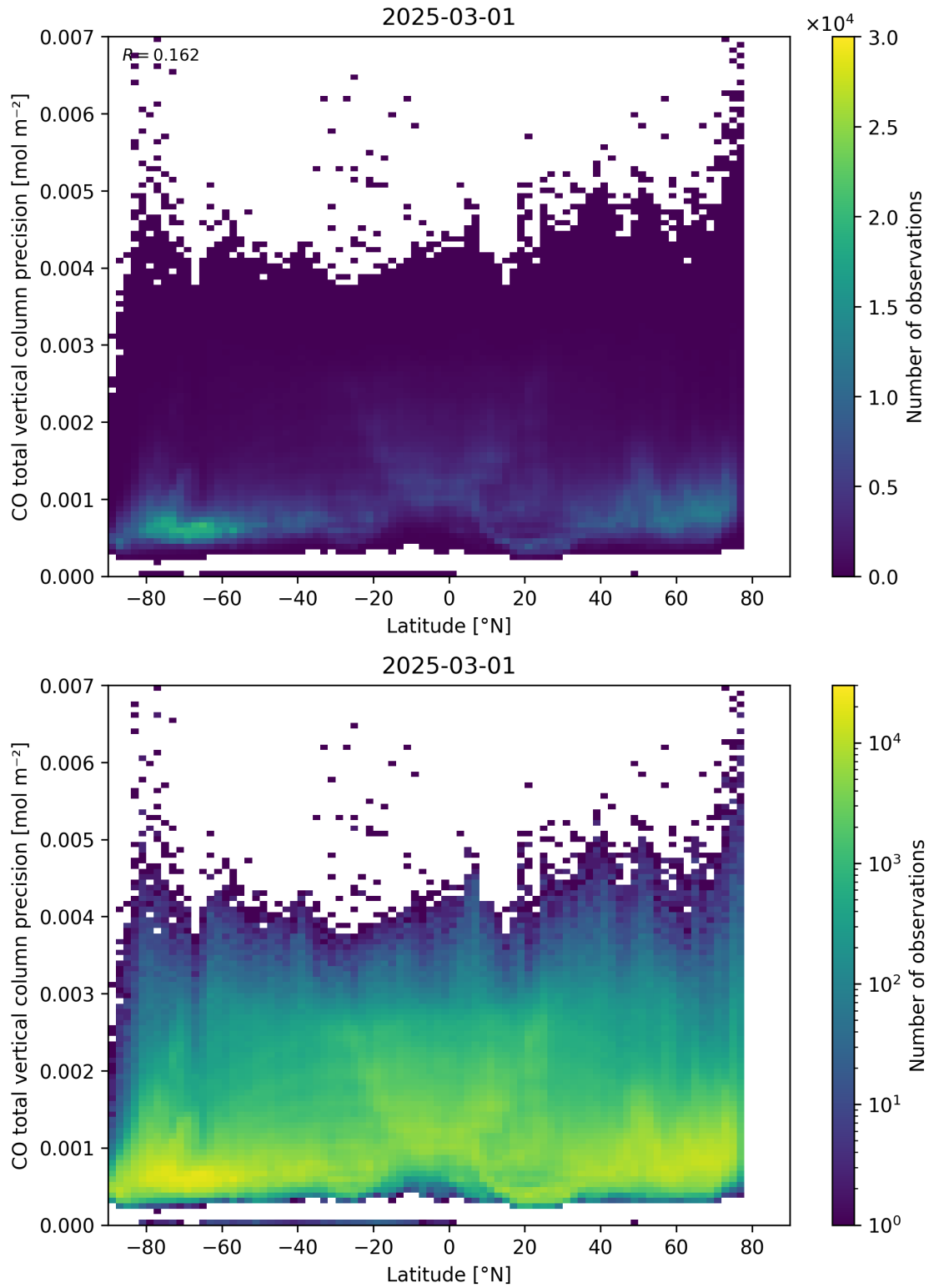
Figure 53: Scatter density plot of “Latitude” against “CO total vertical column precision” for 2025-03-01 to 2025-03-02.
