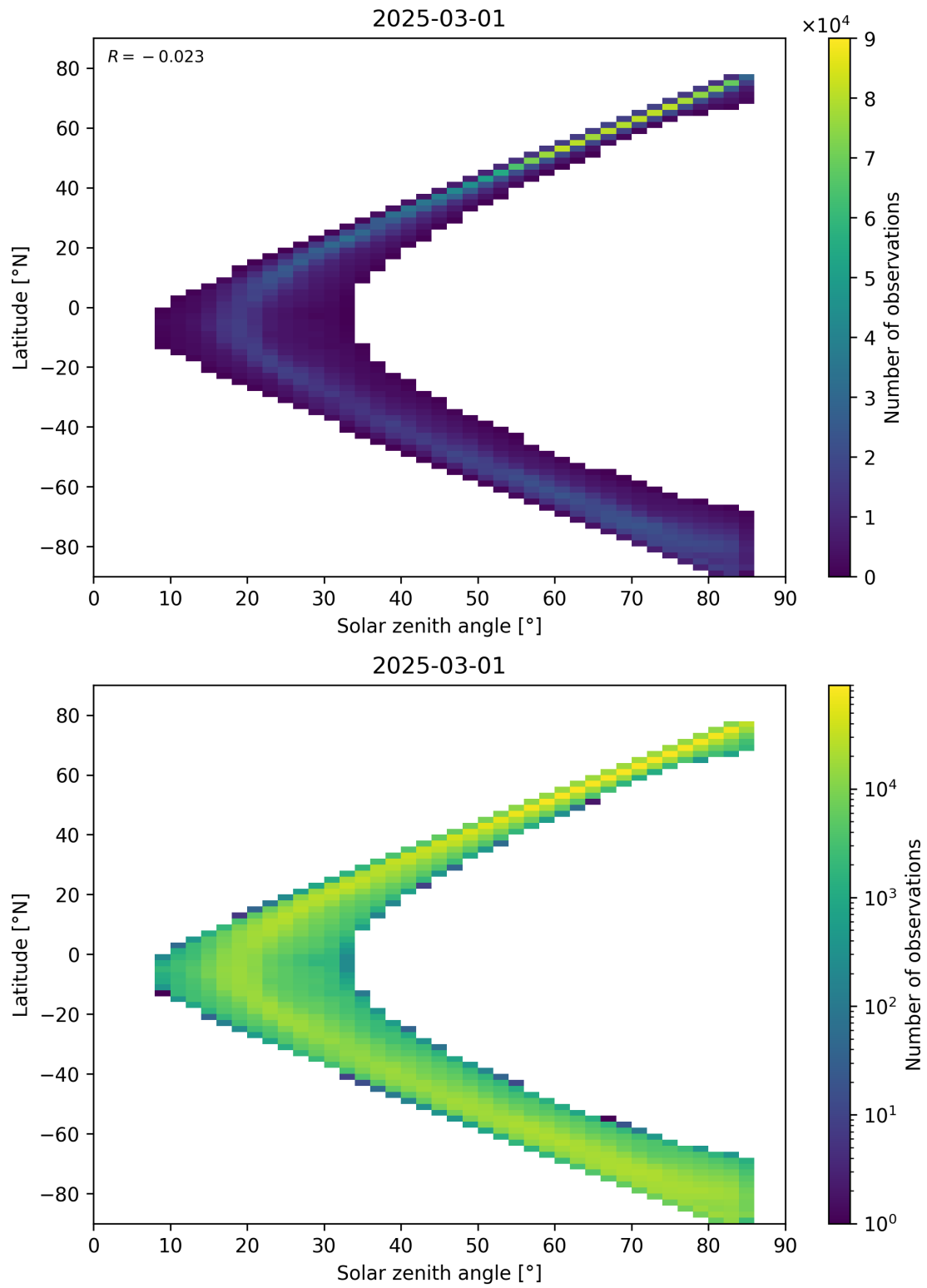
Figure 66: Scatter density plot of “Solar zenith angle” against “Latitude” for 2025-03-01 to 2025-03-02.
