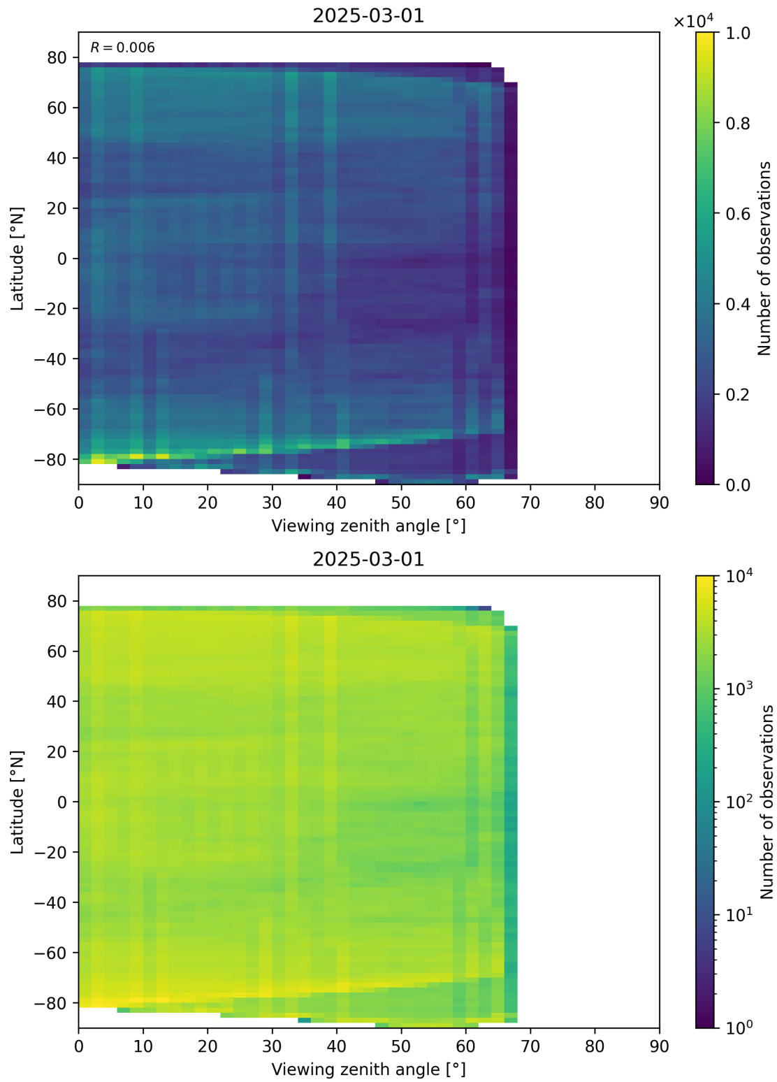
Figure 74: Scatter density plot of “Viewing zenith angle” against “Latitude” for 2025-03-01 to 2025-03-02.
