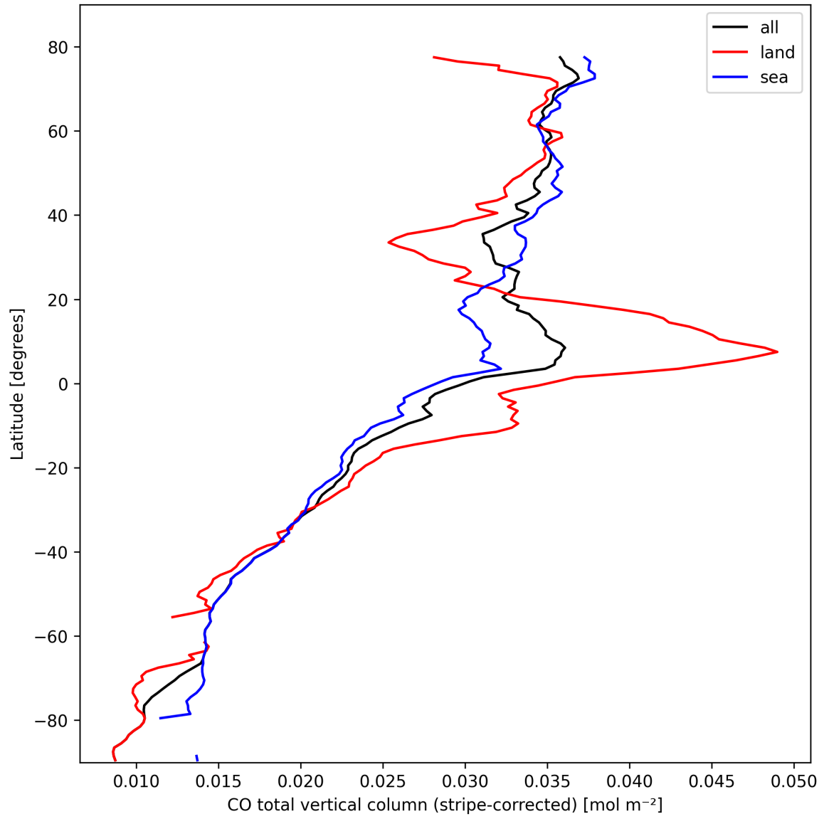
Figure 11: Zonal average of “CO total vertical column (stripe-corrected)” for 2025-03-01 to 2025-03-02.
