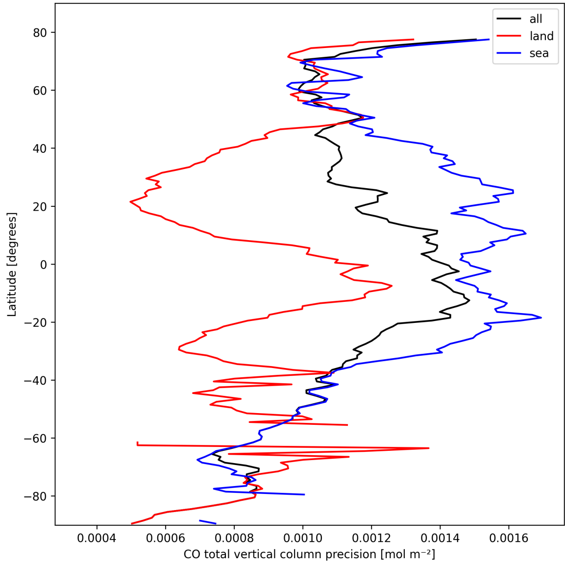
Figure 12: Zonal average of “CO total vertical column precision” for 2025-03-01 to 2025-03-02.
