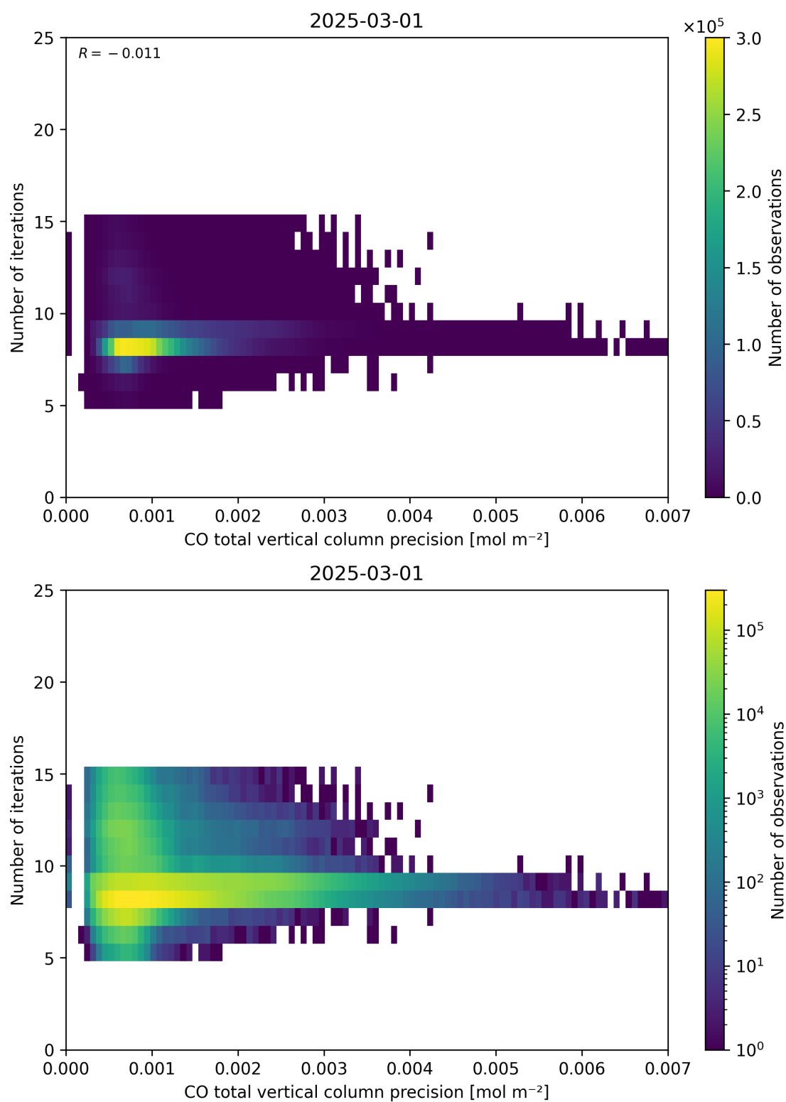
Figure 46: Scatter density plot of “CO total vertical column precision” against “Number of iterations” for 2025-03-01 to 2025-03-02.
