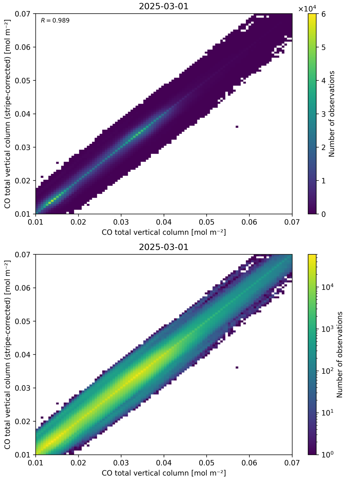
Figure 33: Scatter density plot of “CO total vertical column” against “CO total vertical column (stripe-corrected)” for 2025-03-01 to 2025-03-02.
