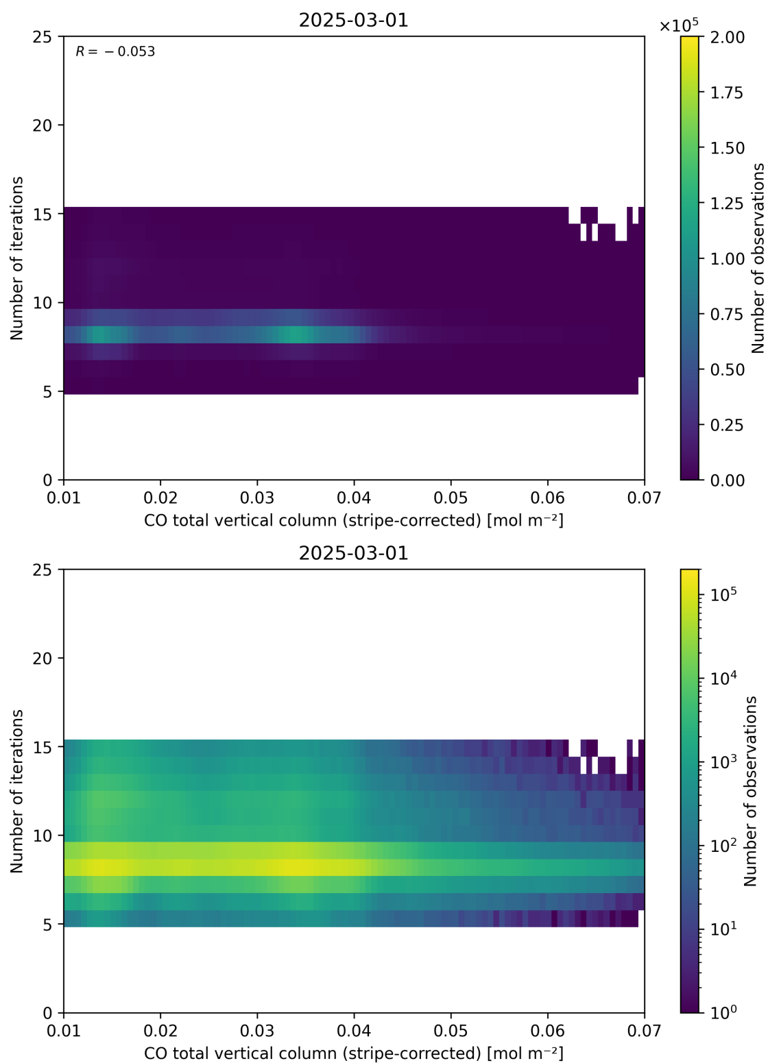
Figure 39: Scatter density plot of “CO total vertical column (stripe-corrected)” against “Number of iterations” for 2025-03-01 to 2025-03-02.
