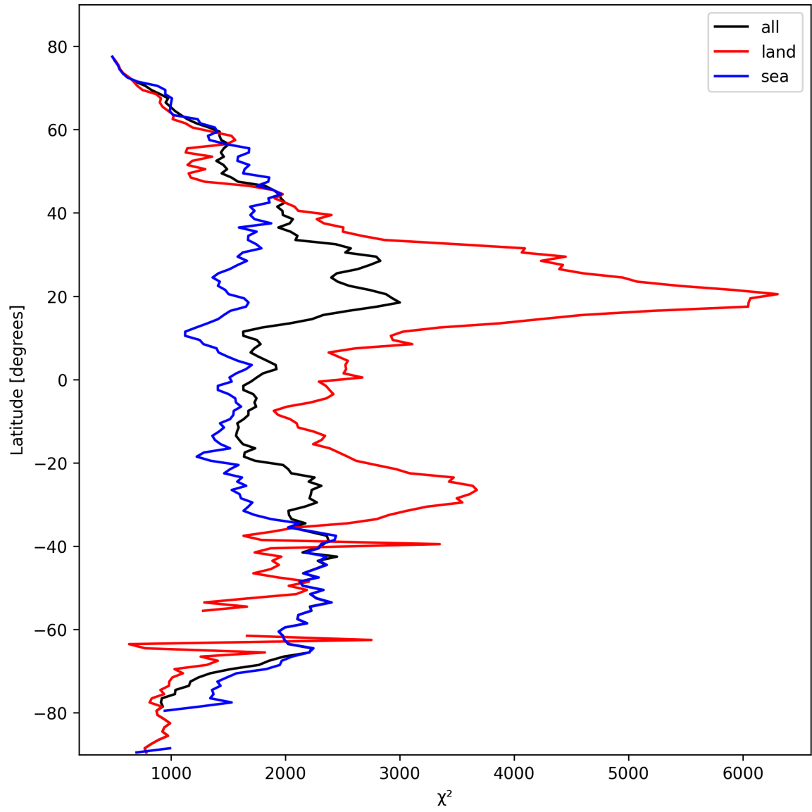
Figure 14: Zonal average of “ \chi^2 ” for 2025-03-01 to 2025-03-02.
