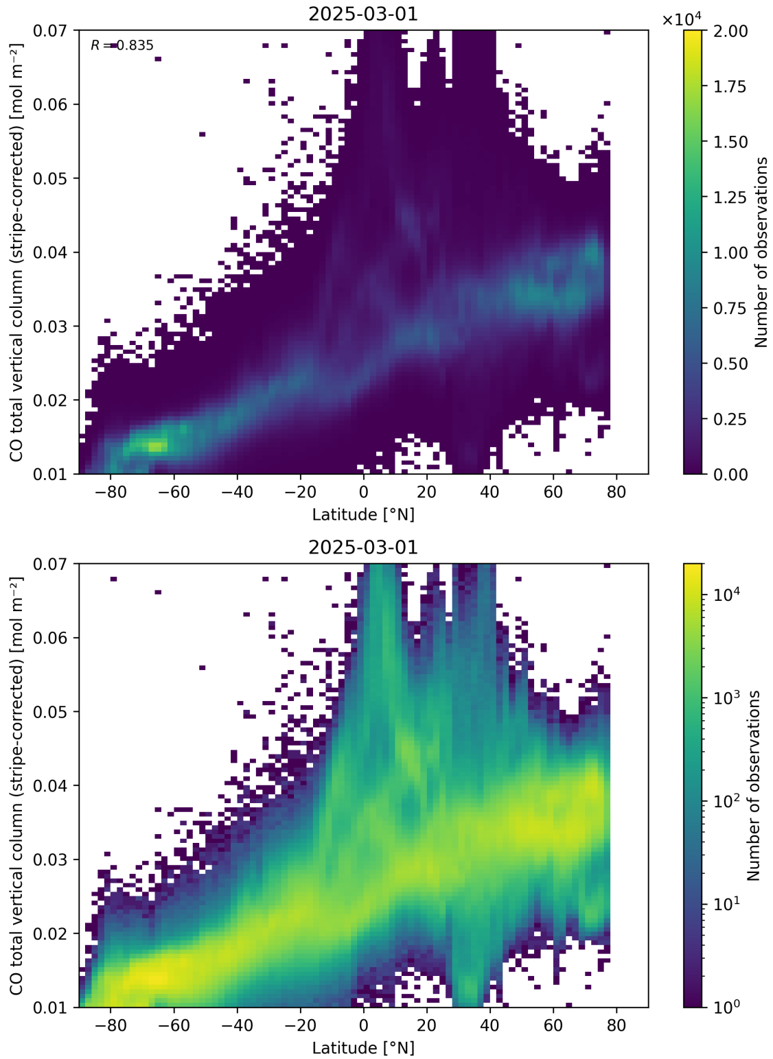
Figure 52: Scatter density plot of “Latitude” against “CO total vertical column (stripe-corrected)” for 2025-03-01 to 2025-03-02.
