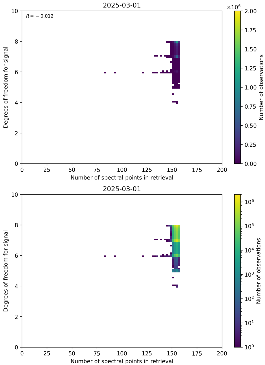
Figure 59: Scatter density plot of “Number of spectral points in retrieval” against “Degrees of freedom for signal” for 2025-03-01 to 2025-03-02.
