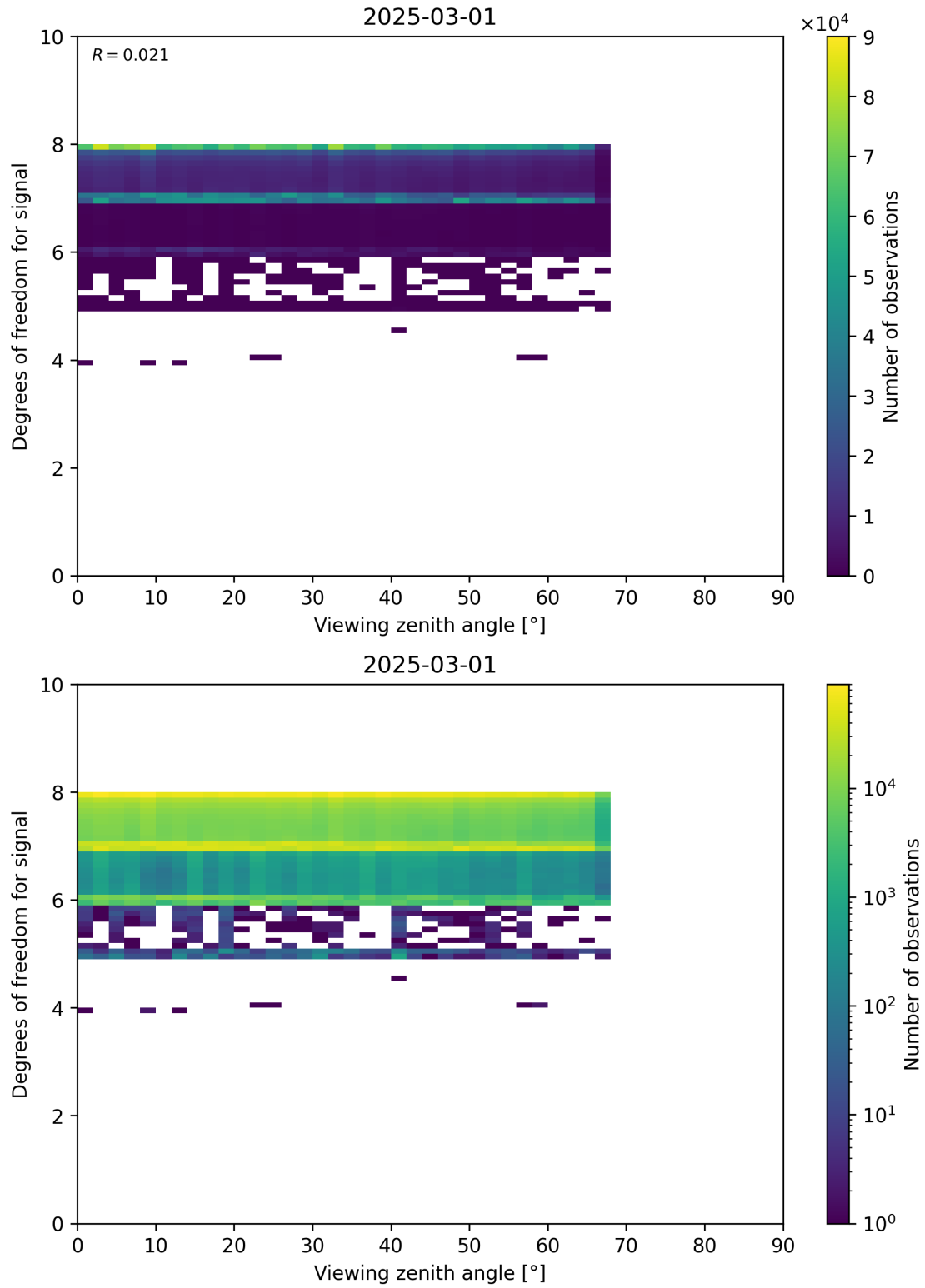
Figure 73: Scatter density plot of “Viewing zenith angle” against “Degrees of freedom for signal” for 2025-03-01 to 2025-03-02.
