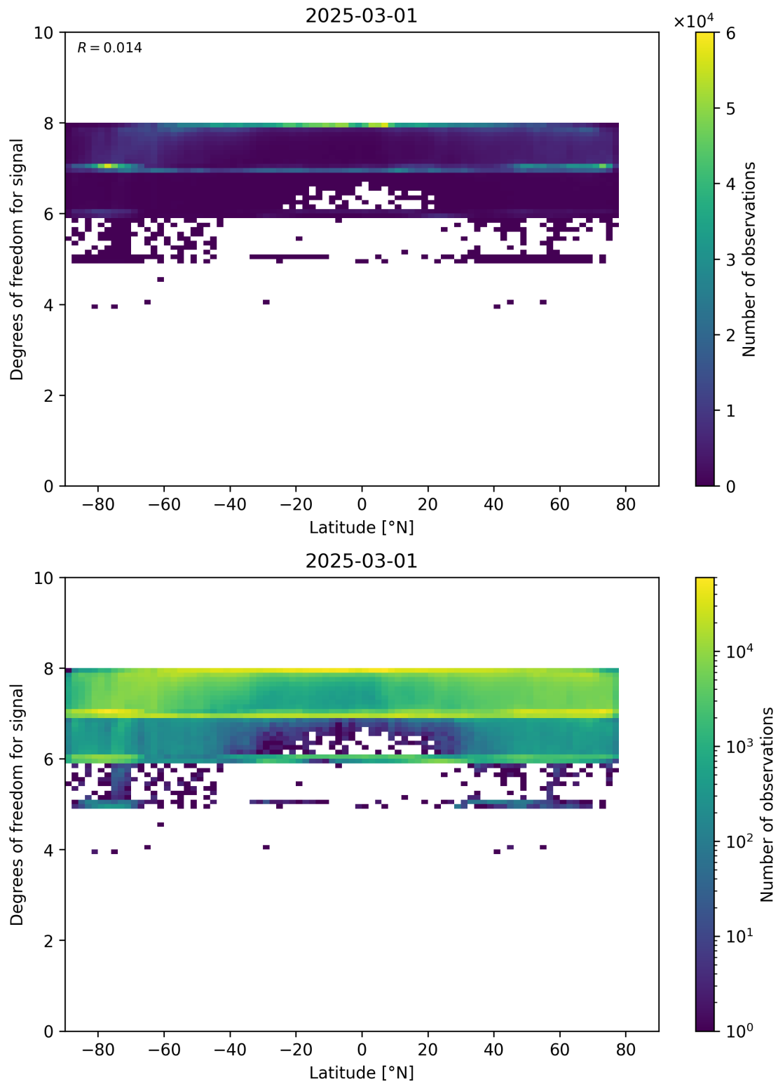
Figure 55: Scatter density plot of “Latitude” against “Degrees of freedom for signal” for 2025-03-01 to 2025-03-02.
