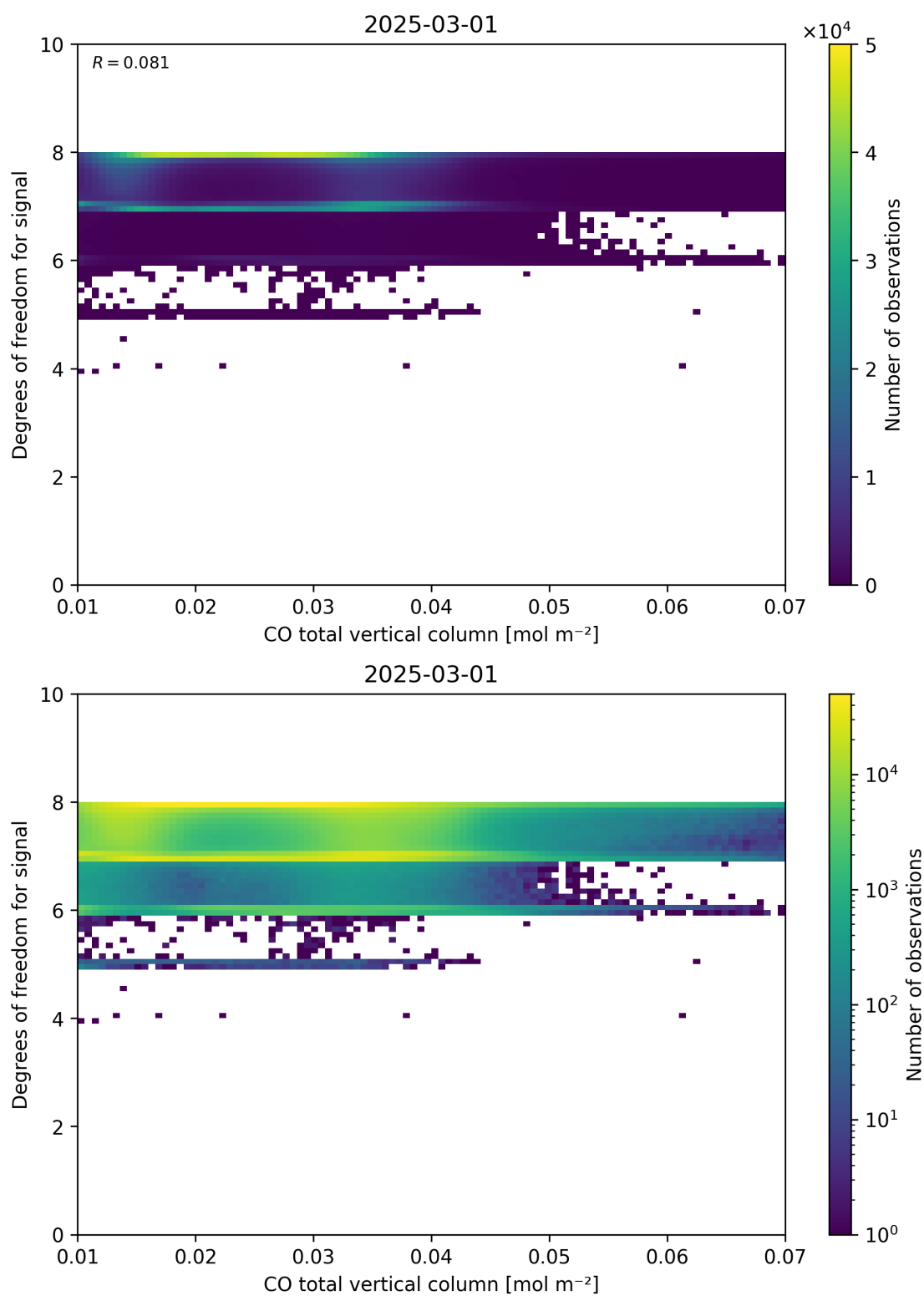
Figure 41: Scatter density plot of “CO total vertical column” against “Degrees of freedom for signal” for 2025-03-01 to 2025-03-02.
