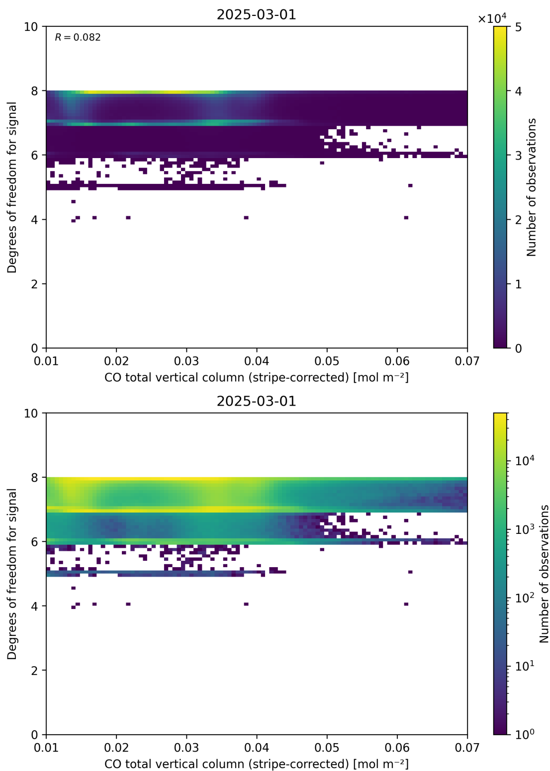
Figure 38: Scatter density plot of “CO total vertical column (stripe-corrected)” against “Degrees of freedom for signal” for 2025-03-01 to 2025-03-02.
