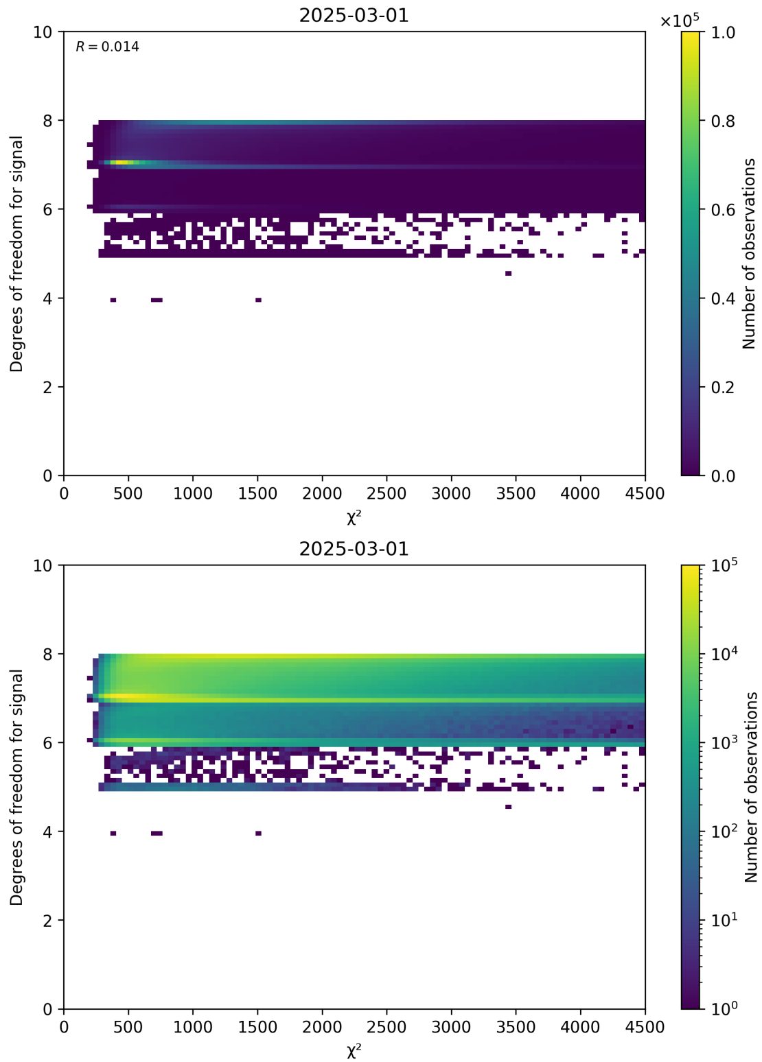
Figure 48: Scatter density plot of “ \chi^2 ” against “Degrees of freedom for signal” for 2025-03-01 to 2025-03-02.
