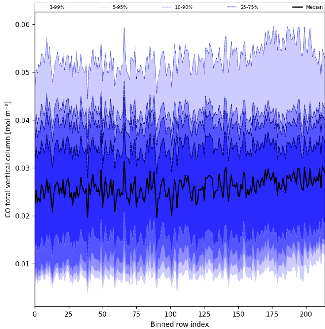
Figure 26: Along track statistics of “CO total vertical column” for 2025-03-01 to 2025-03-02
