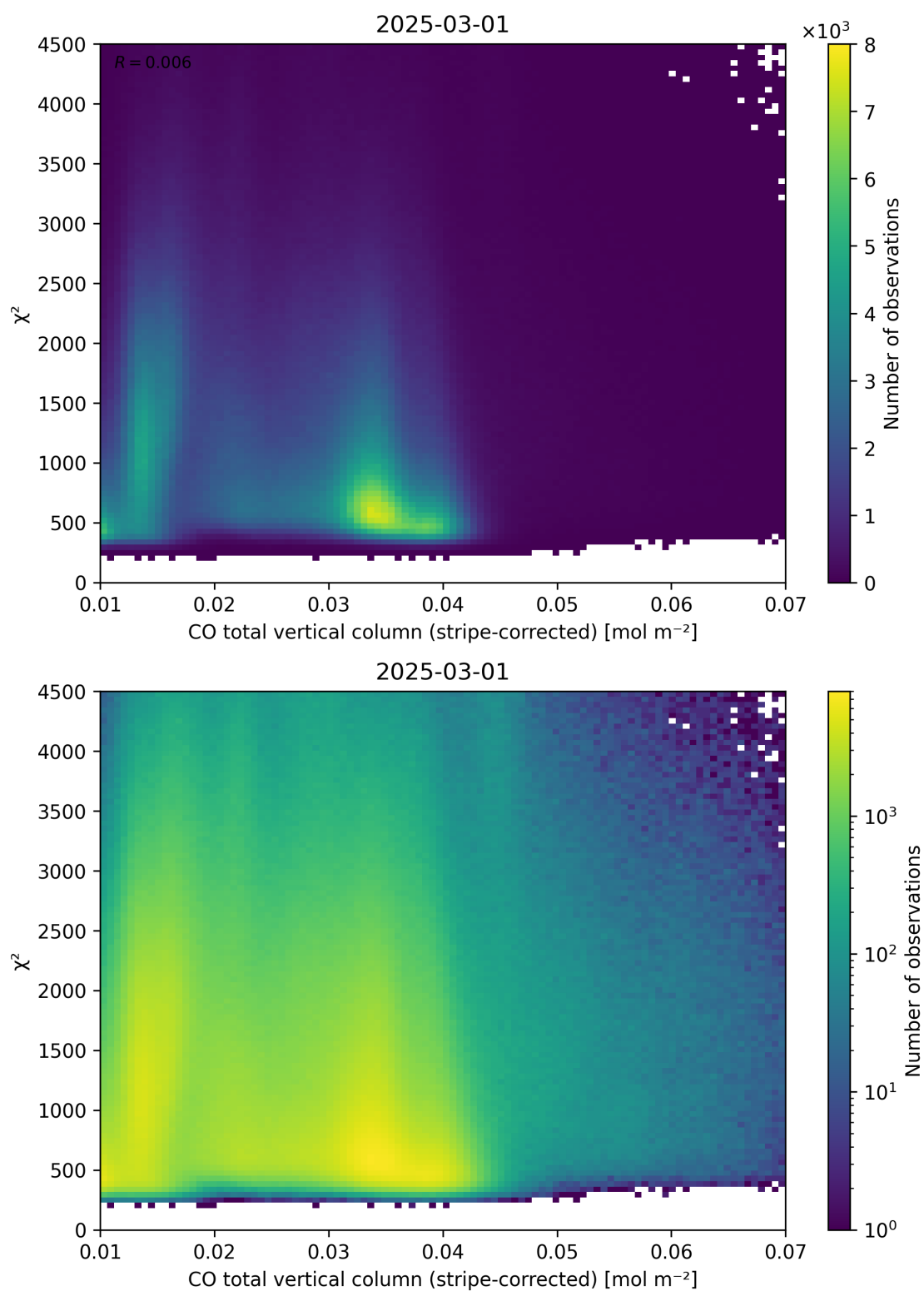
Figure 37: Scatter density plot of “CO total vertical column (stripe-corrected)” against “ \chi^2 ” for 2025-03-01 to 2025-03-02.
