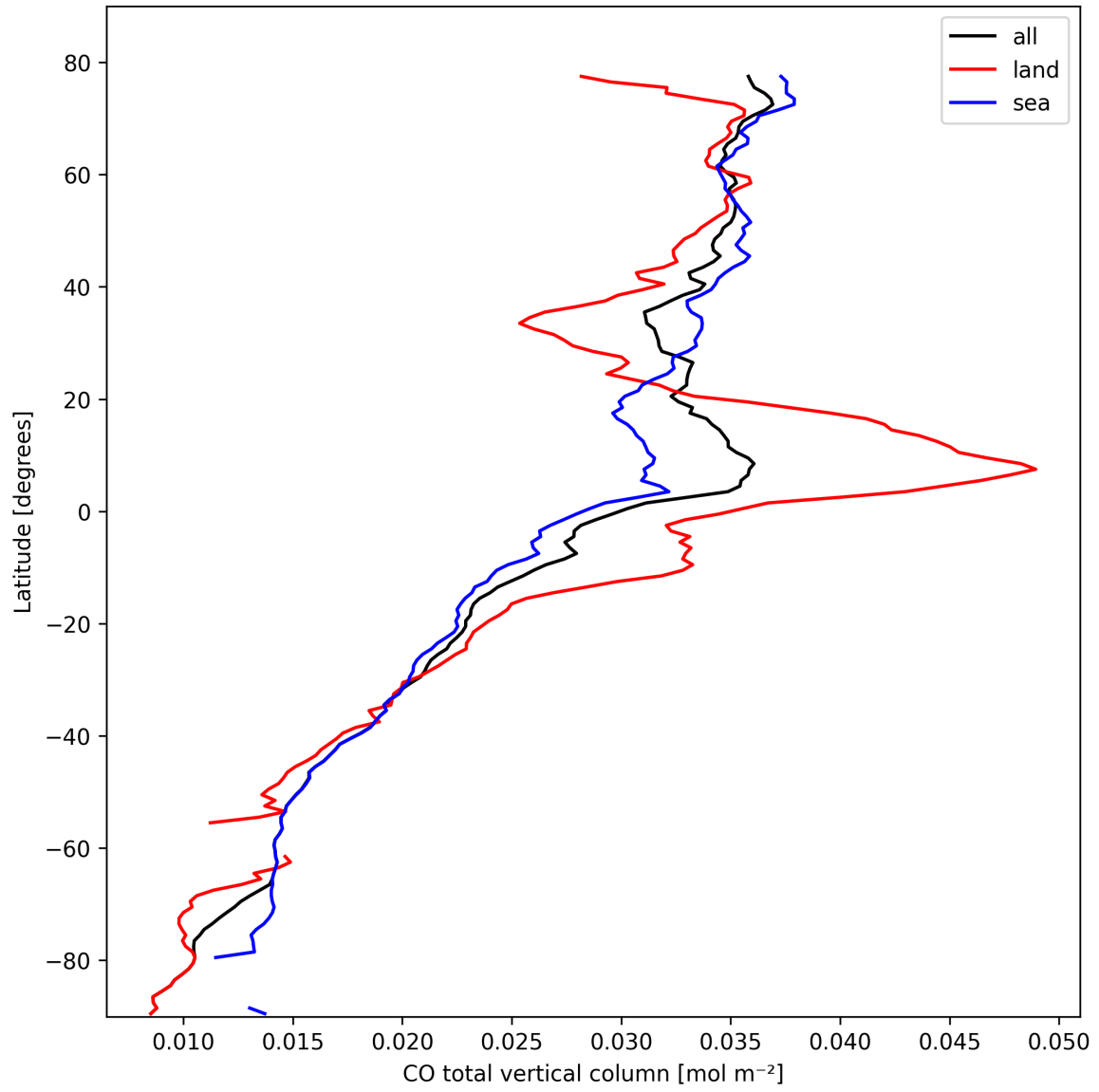
Figure 10: Zonal average of “CO total vertical column” for 2025-03-01 to 2025-03-02.
