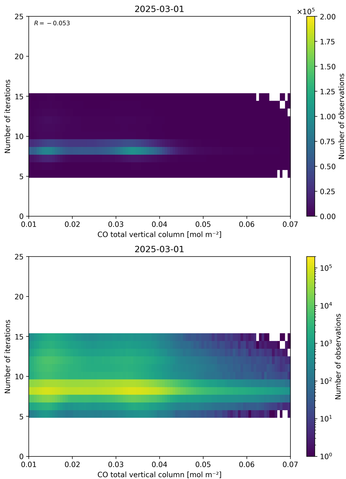
Figure 42: Scatter density plot of “CO total vertical column” against “Number of iterations” for 2025-03-01 to 2025-03-02.
