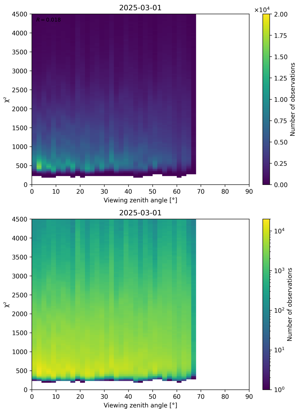
Figure 72: Scatter density plot of “Viewing zenith angle” against “ \chi^2 ” for 2025-03-01 to 2025-03-02.
