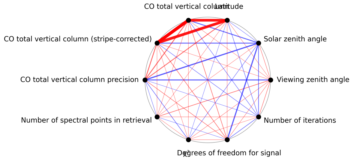
Figure 1: Map of correlation graph for 2025-03-01 to 2025-03-02.
