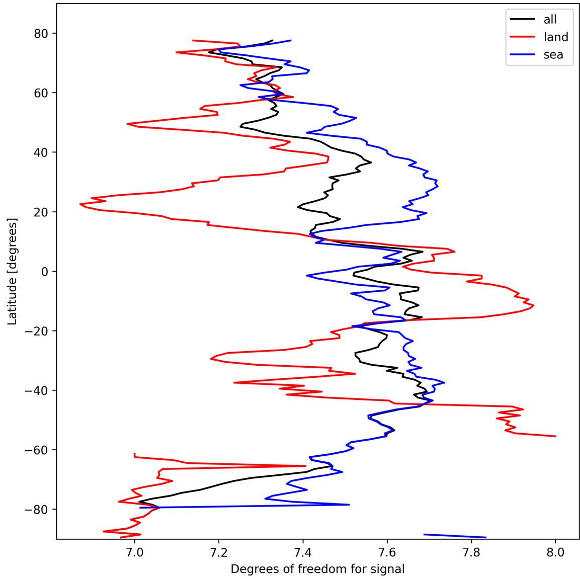
Figure 15: Zonal average of “Degrees of freedom for signal” for 2025-03-01 to 2025-03-02.
