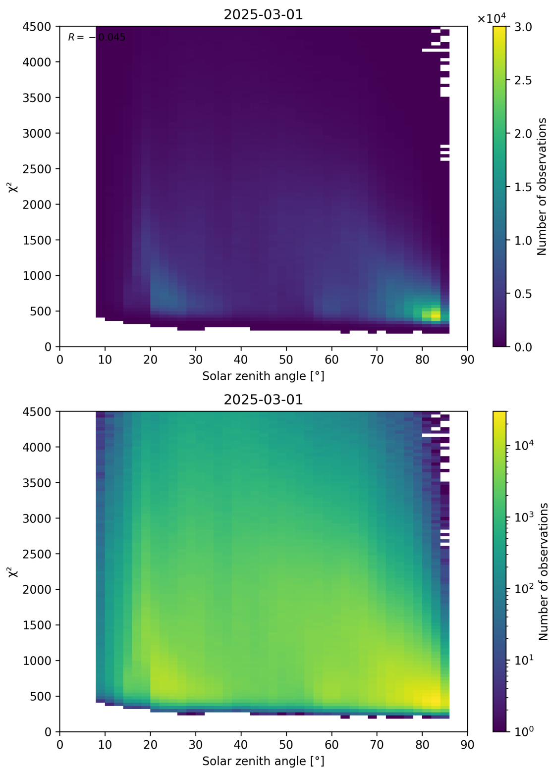
Figure 64: Scatter density plot of “Solar zenith angle” against “ \chi^2 ” for 2025-03-01 to 2025-03-02.
