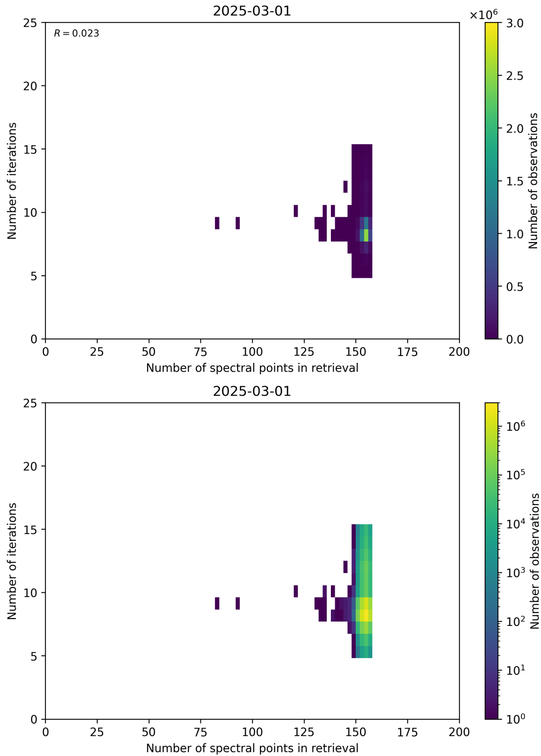
Figure 60: Scatter density plot of “Number of spectral points in retrieval” against “Number of iterations” for 2025-03-01 to 2025-03-02.
