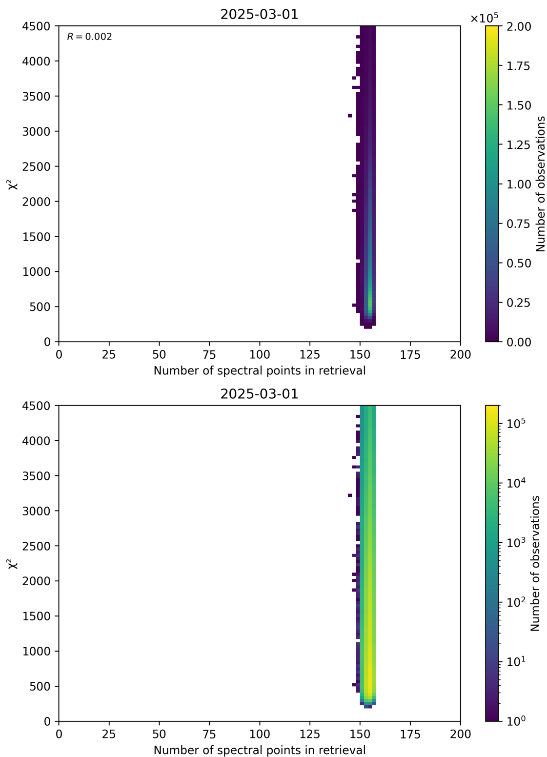
Figure 58: Scatter density plot of “Number of spectral points in retrieval” against “ \chi^2 ” for 2025-03-01 to 2025-03-02.
