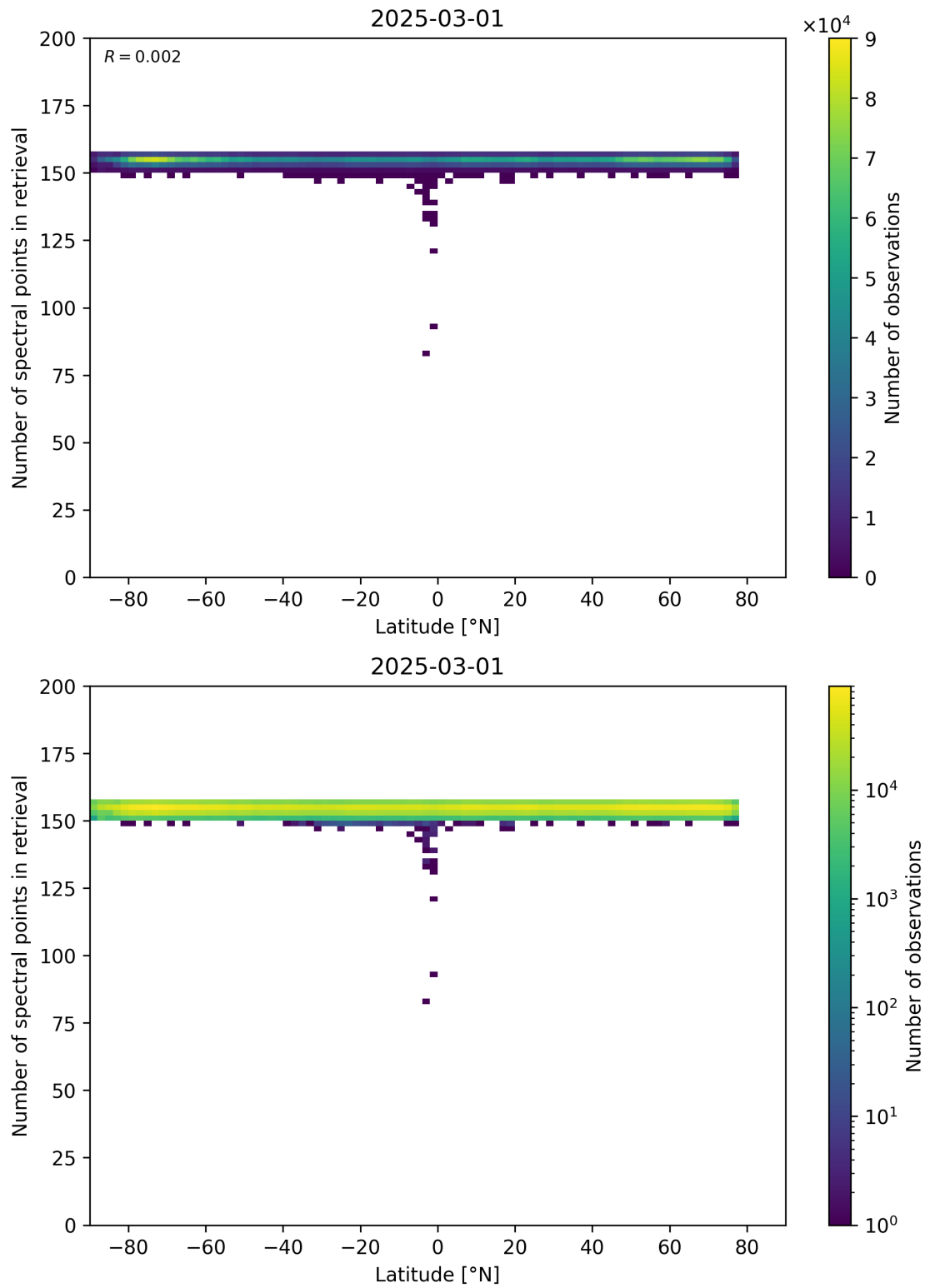
Figure 57: Scatter density plot of “Latitude” against “Number of spectral points in retrieval” for 2025-03-01 to 2025-03-02.
