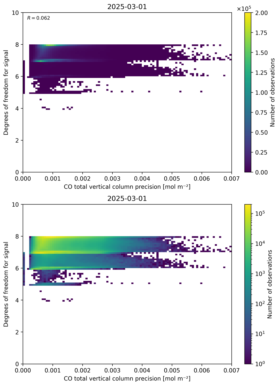
Figure 45: Scatter density plot of “CO total vertical column precision” against “Degrees of freedom for signal” for 2025-03-01 to 2025-03-02.
