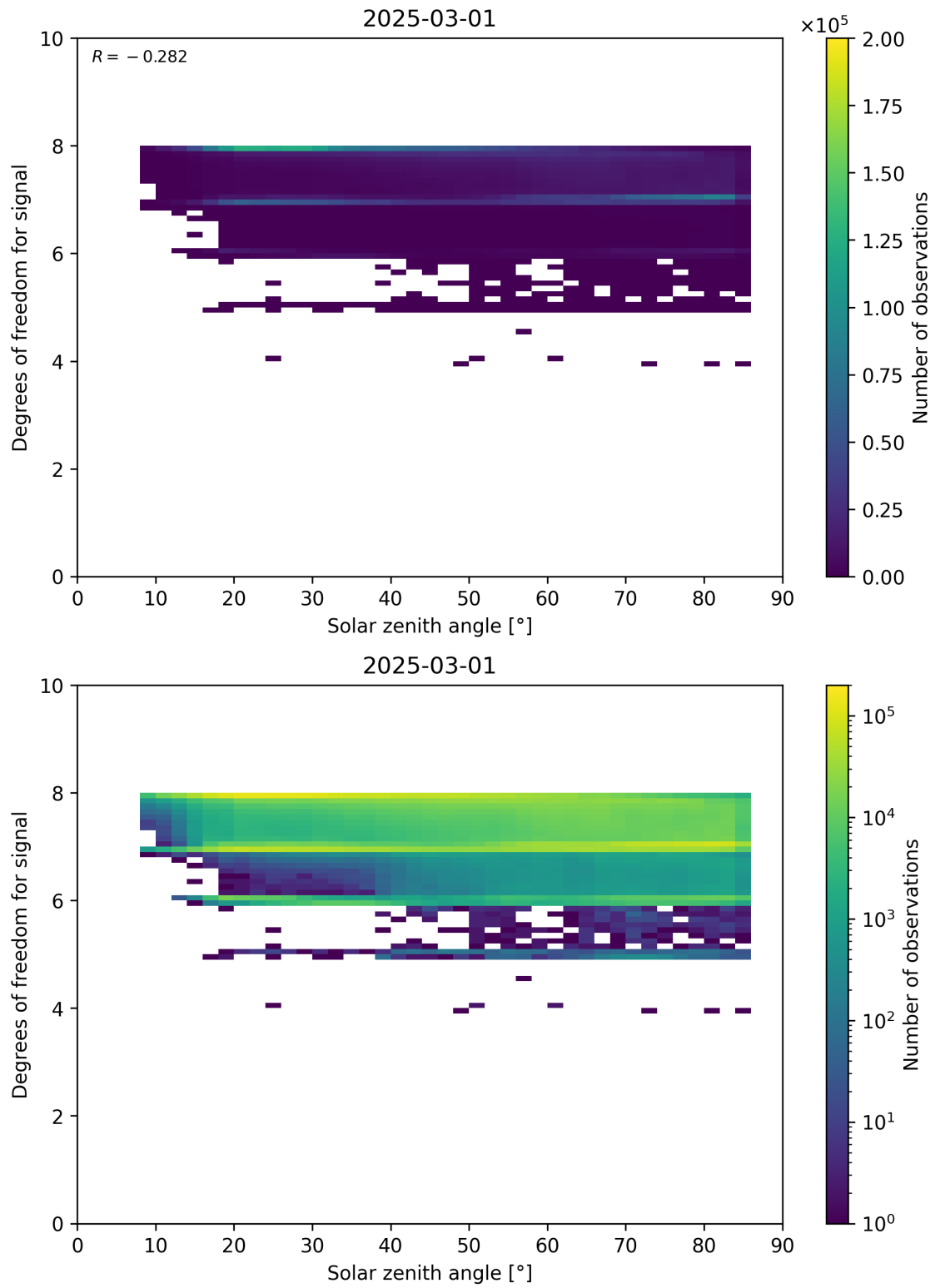
Figure 65: Scatter density plot of “Solar zenith angle” against “Degrees of freedom for signal” for 2025-03-01 to 2025-03-02.
