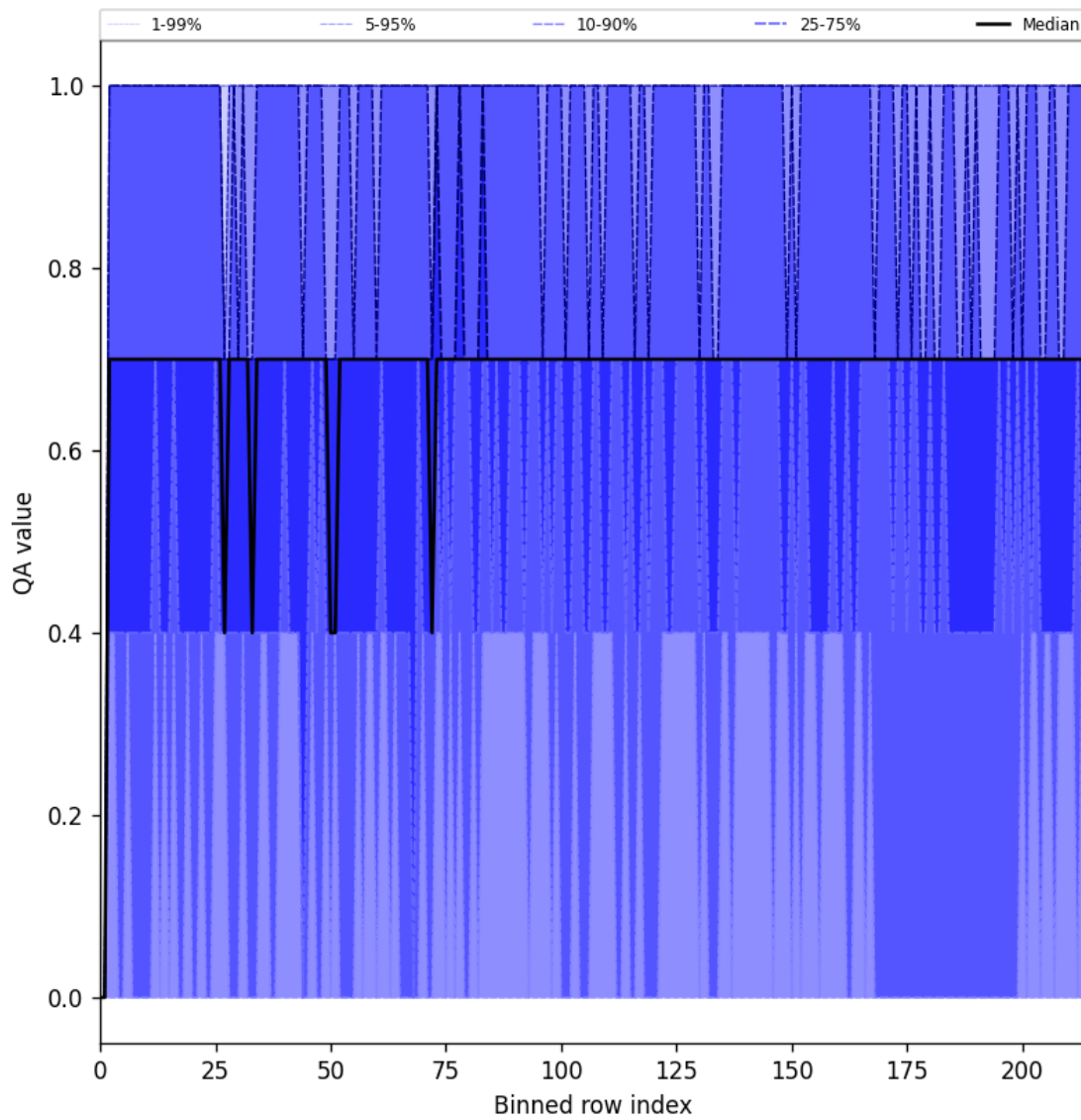
Figure 25: Along track statistics of “QA value” for 2025-03-01 to 2025-03-02
