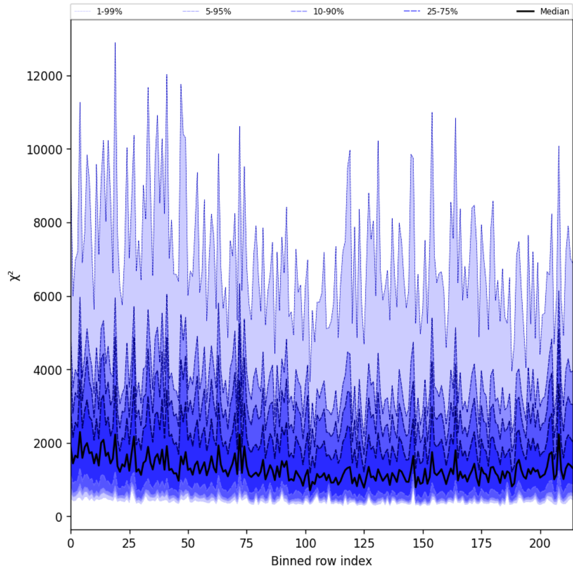
Figure 30: Along track statistics of “ \chi^2 ” for 2025-03-01 to 2025-03-02
