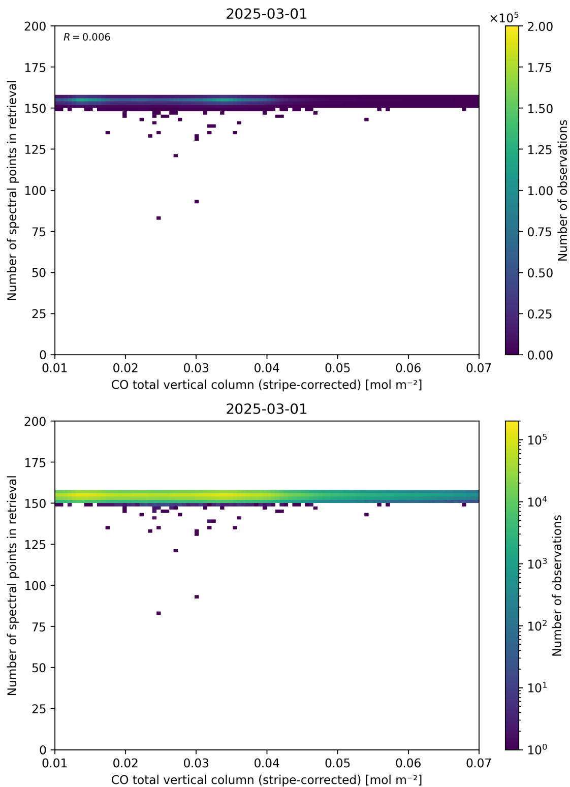
Figure 40: Scatter density plot of “CO total vertical column (stripe-corrected)” against “Number of spectral points in retrieval” for 2025-03-01 to 2025-03-02.
