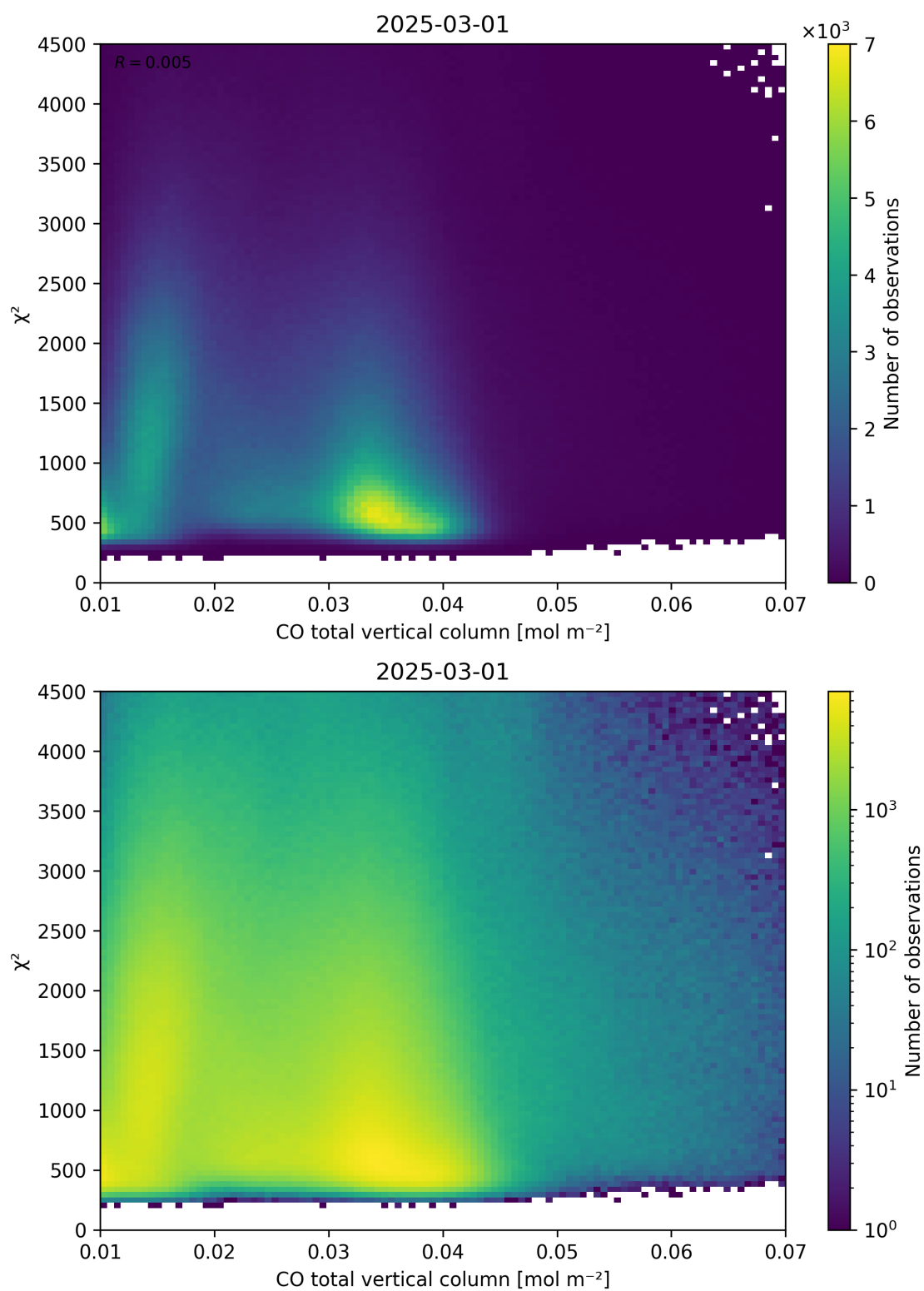
Figure 35: Scatter density plot of “CO total vertical column” against “ \chi^2 ” for 2025-03-01 to 2025-03-02.
