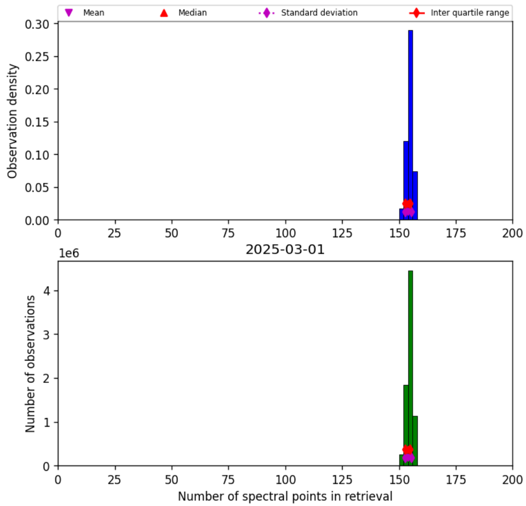
Figure 21: Histogram of “Number of spectral points in retrieval” for 2025-03-01 to 2025-03-02
