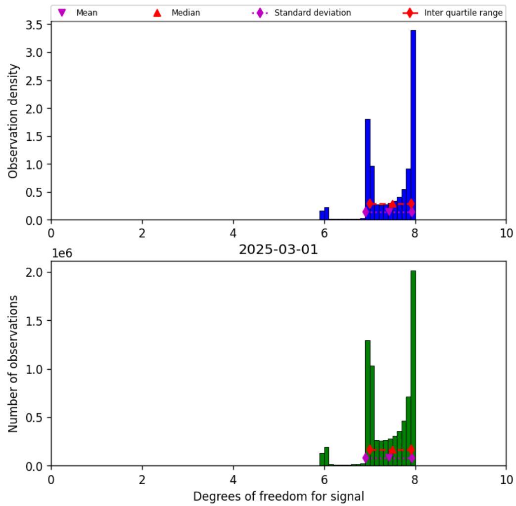
Figure 23: Histogram of “Degrees of freedom for signal” for 2025-03-01 to 2025-03-02
