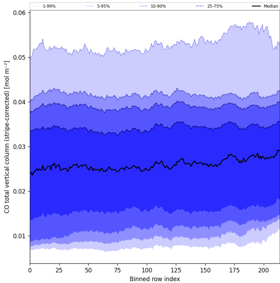
Figure 27: Along track statistics of “CO total vertical column (stripe-corrected)” for 2025-03-01 to 2025-03-02
