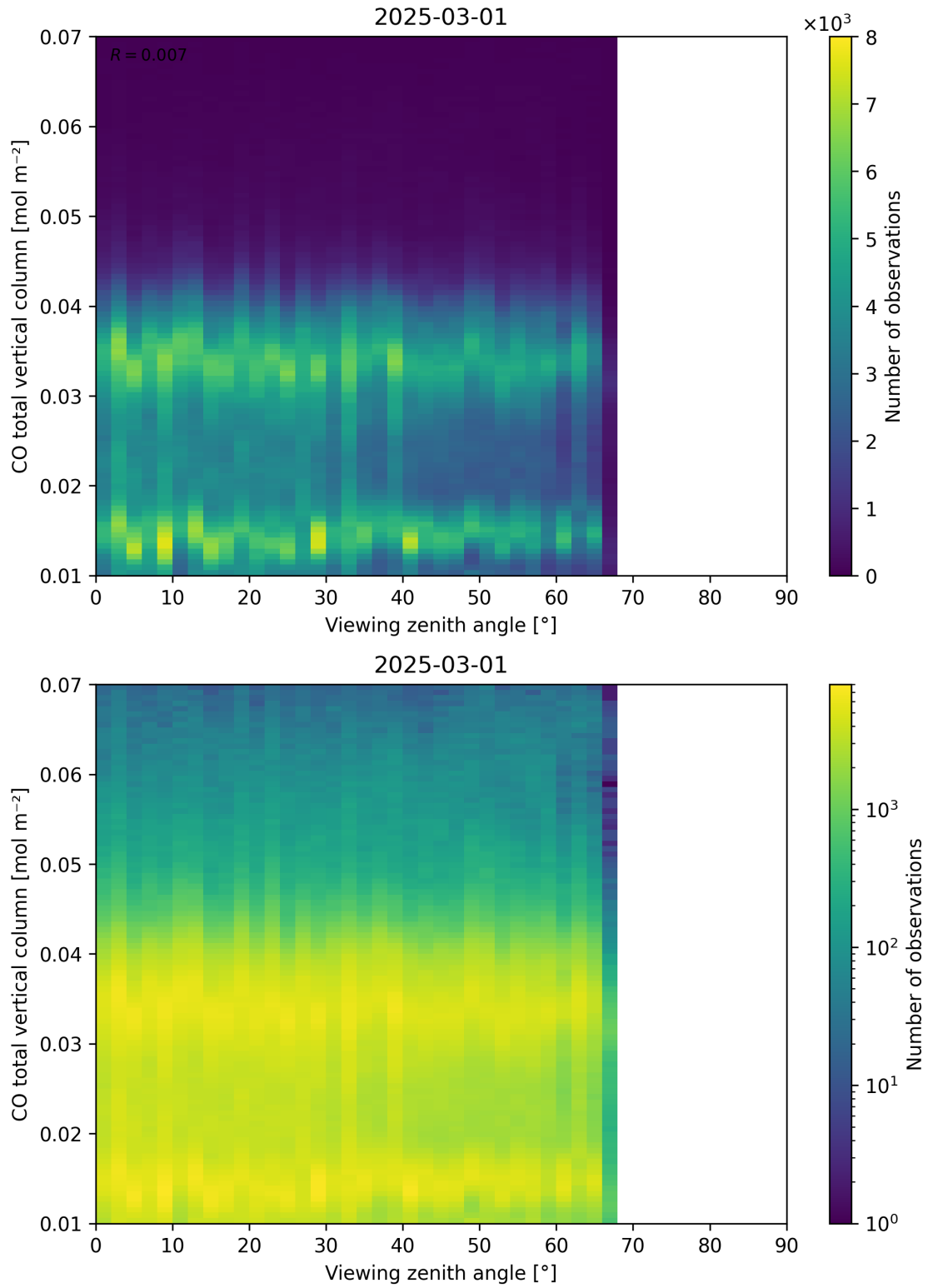
Figure 69: Scatter density plot of “Viewing zenith angle” against “CO total vertical column” for 2025-03-01 to 2025-03-02.
