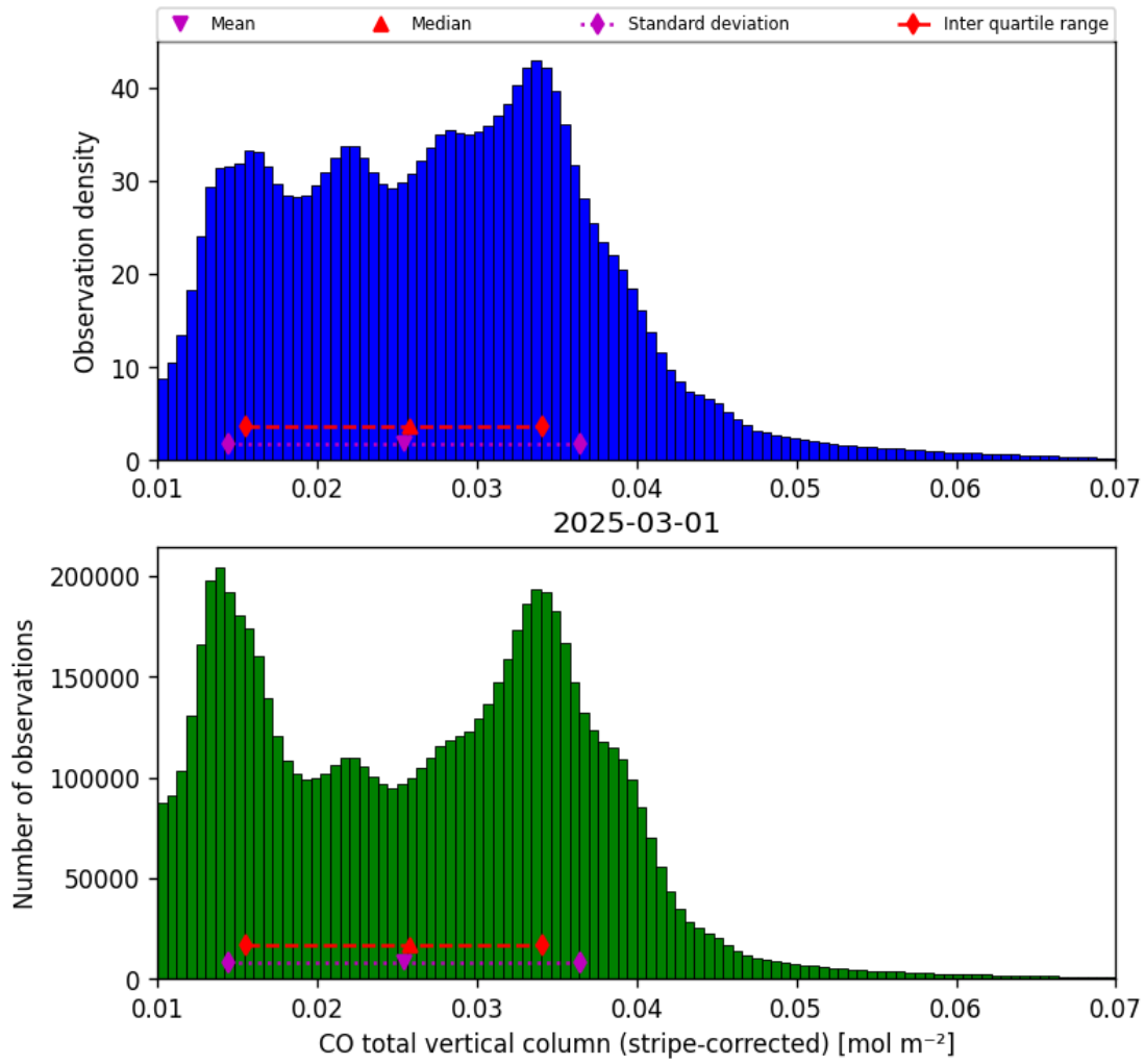
Figure 19: Histogram of “CO total vertical column (stripe-corrected)” for 2025-03-01 to 2025-03-02
