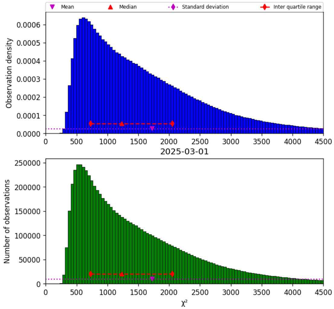
Figure 22: Histogram of “ \chi^2 ” for 2025-03-01 to 2025-03-02
