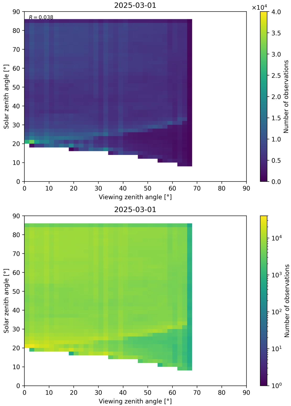
Figure 77: Scatter density plot of “Viewing zenith angle” against “Solar zenith angle” for 2025-03-01 to 2025-03-02.
