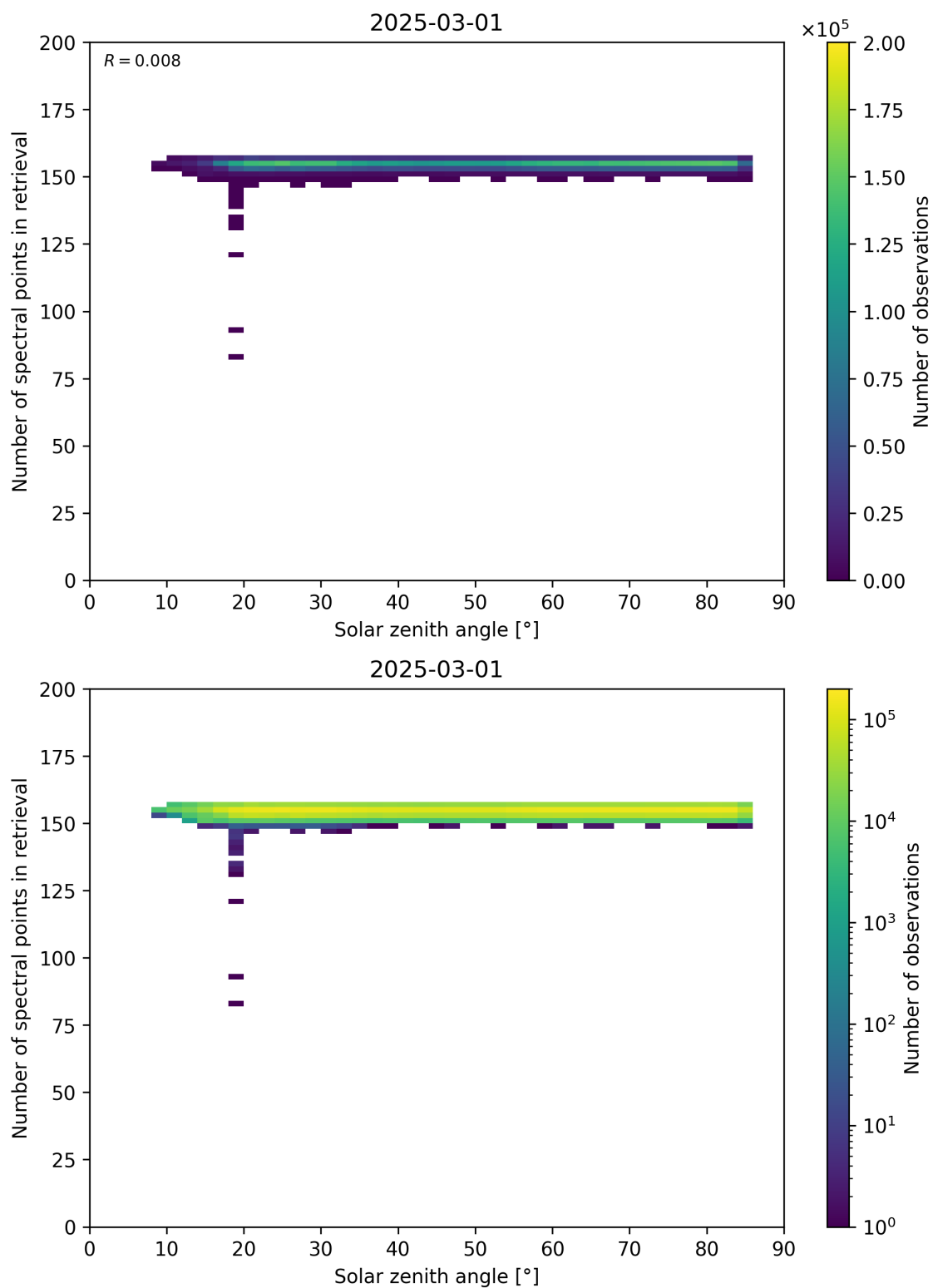
Figure 68: Scatter density plot of “Solar zenith angle” against “Number of spectral points in retrieval” for 2025-03-01 to 2025-03-02.
