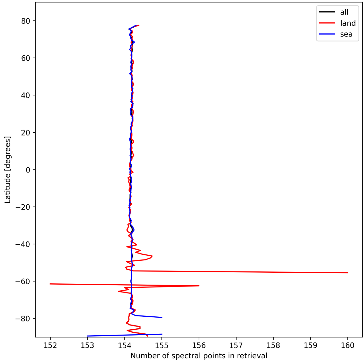
Figure 13: Zonal average of “Number of spectral points in retrieval” for 2025-03-01 to 2025-03-02.
