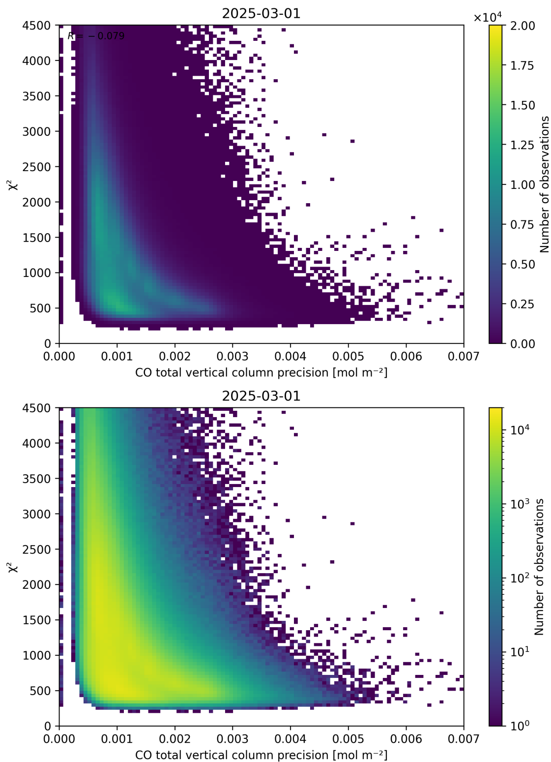
Figure 44: Scatter density plot of “CO total vertical column precision” against “ \chi^2 ” for 2025-03-01 to 2025-03-02.
