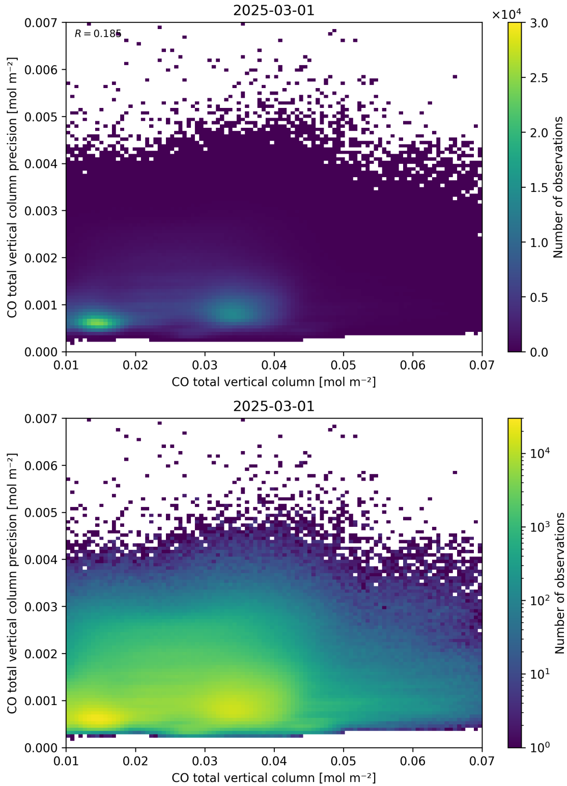
Figure 34: Scatter density plot of “CO total vertical column” against “CO total vertical column precision” for 2025-03-01 to 2025-03-02.
