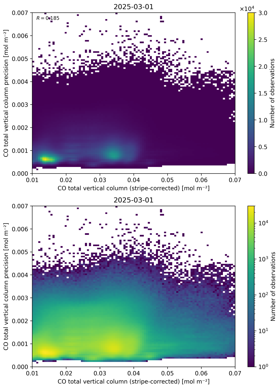
Figure 36: Scatter density plot of “CO total vertical column (stripe-corrected)” against “CO total vertical column precision” for 2025-03-01 to 2025-03-02.
