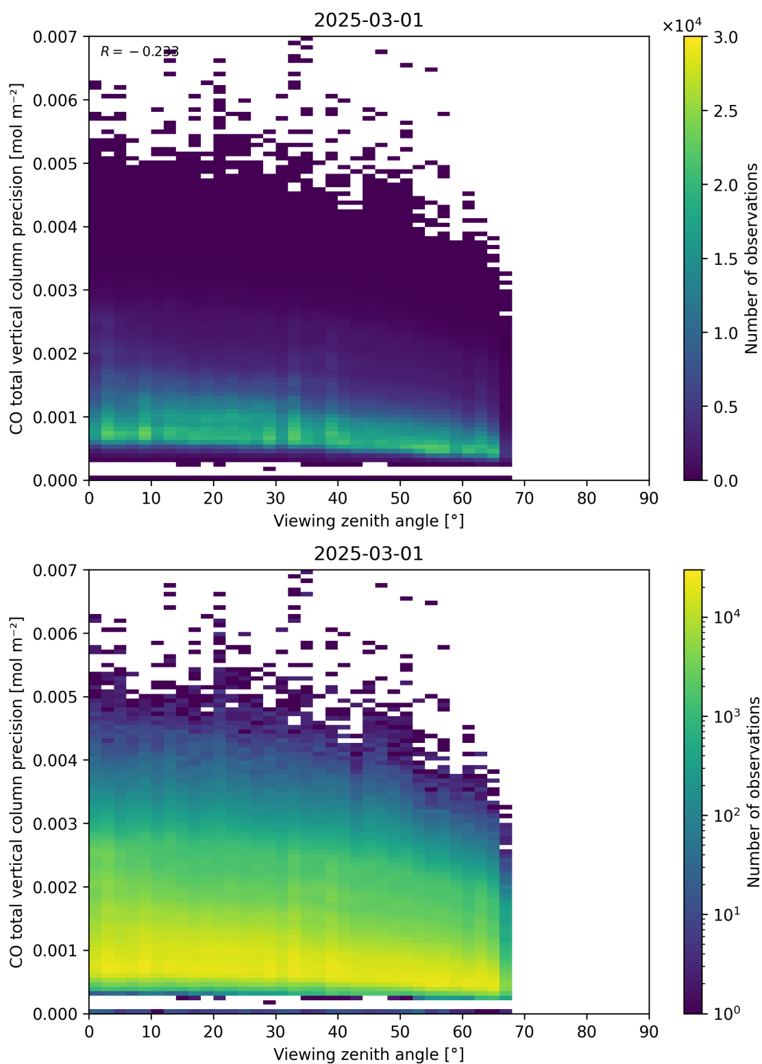
Figure 71: Scatter density plot of “Viewing zenith angle” against “CO total vertical column precision” for 2025-03-01 to 2025-03-02.
