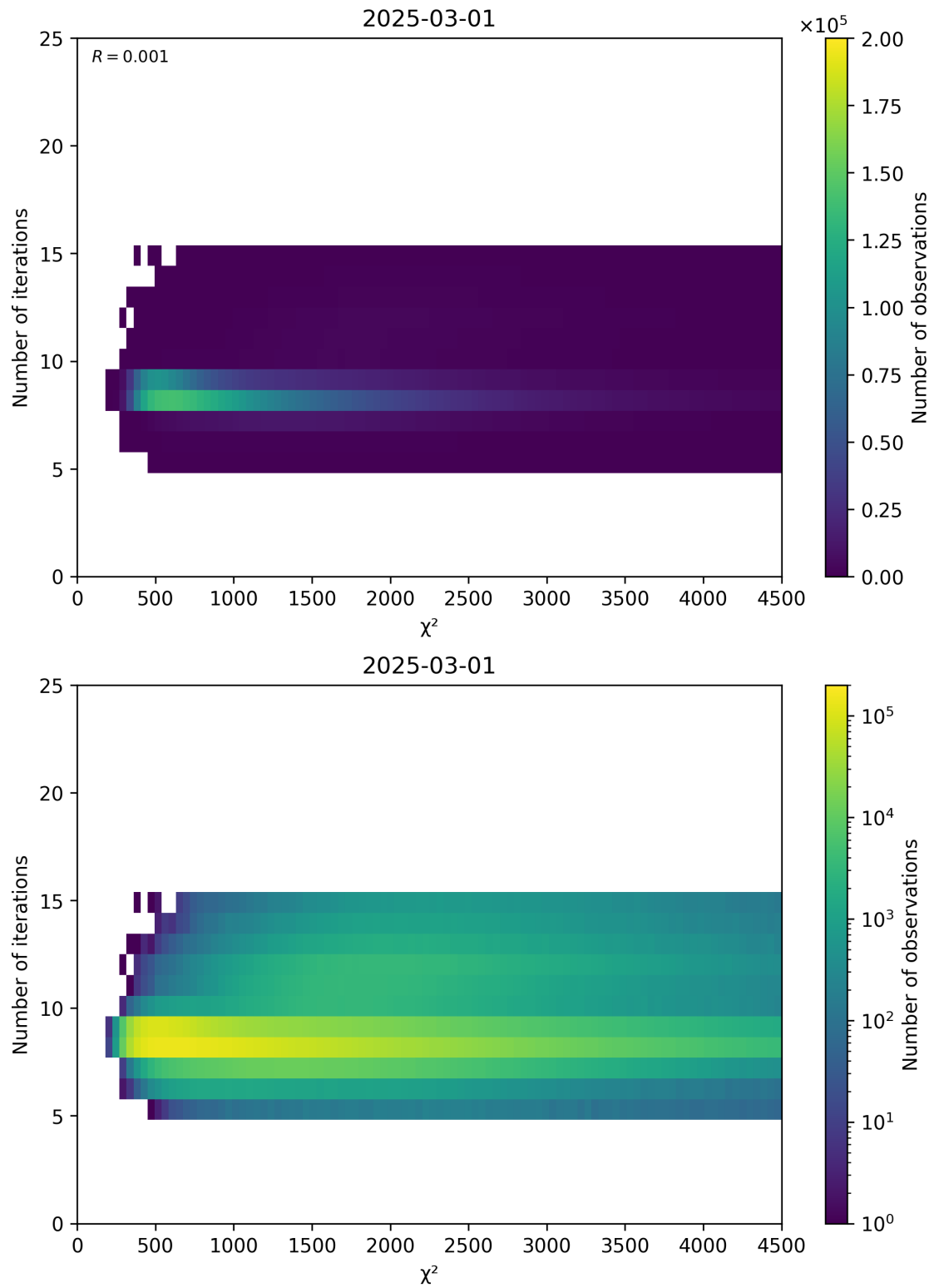
Figure 49: Scatter density plot of “ \chi^2 ” against “Number of iterations” for 2025-03-01 to 2025-03-02.
