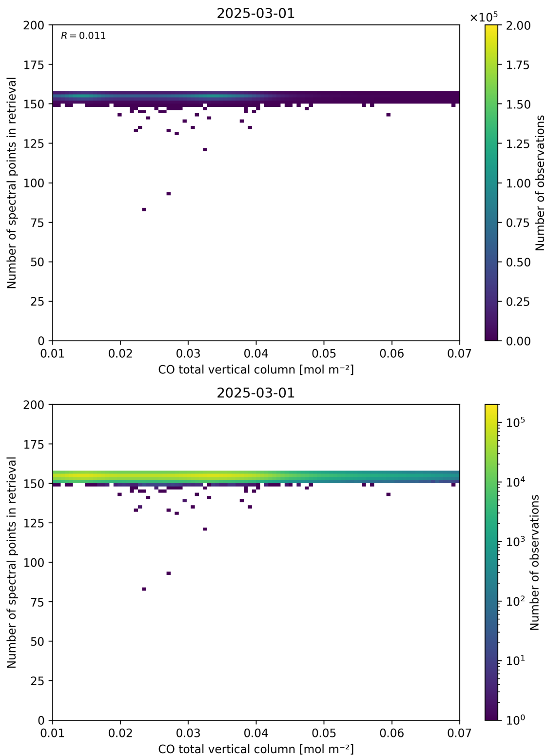
Figure 43: Scatter density plot of “CO total vertical column” against “Number of spectral points in retrieval” for 2025-03-01 to 2025-03-02.
