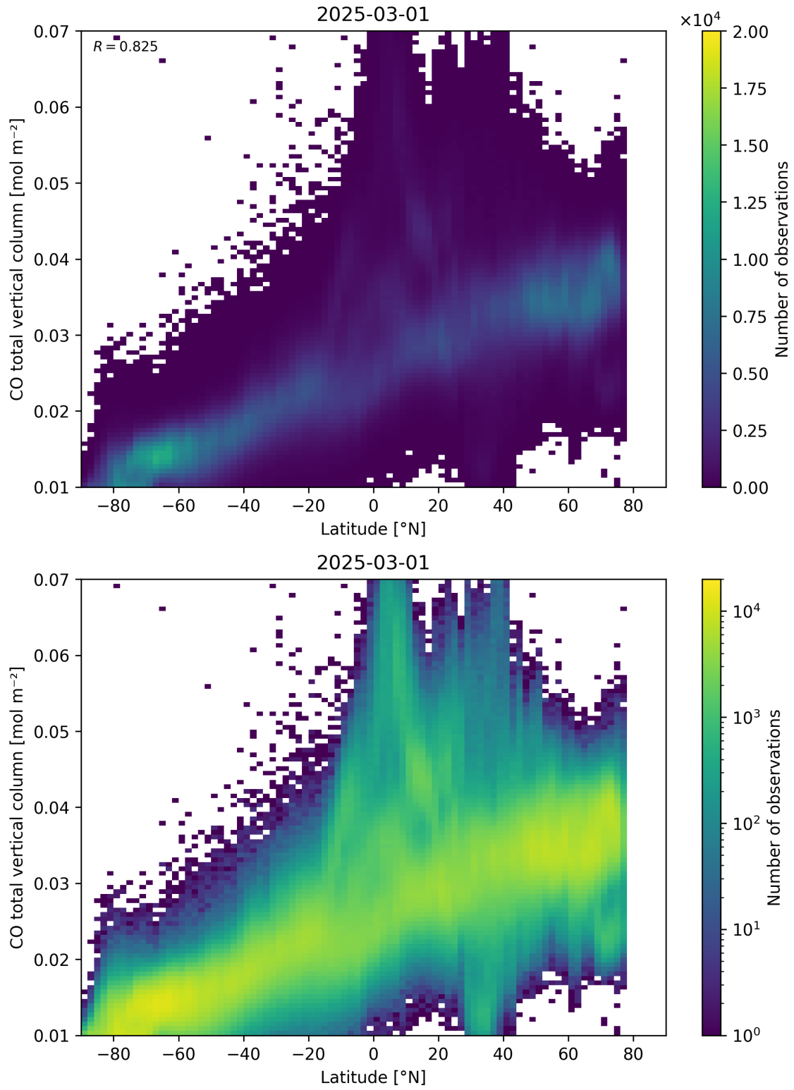
Figure 51: Scatter density plot of “Latitude” against “CO total vertical column” for 2025-03-01 to 2025-03-02.
