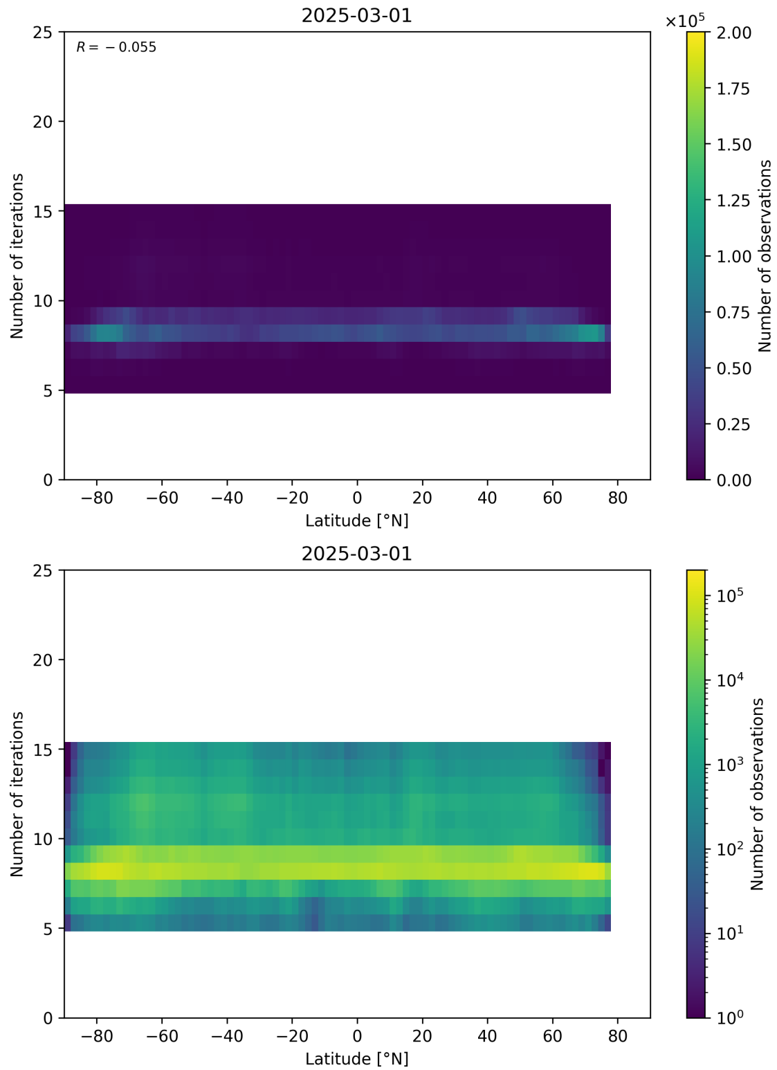
Figure 56: Scatter density plot of “Latitude” against “Number of iterations” for 2025-03-01 to 2025-03-02.
