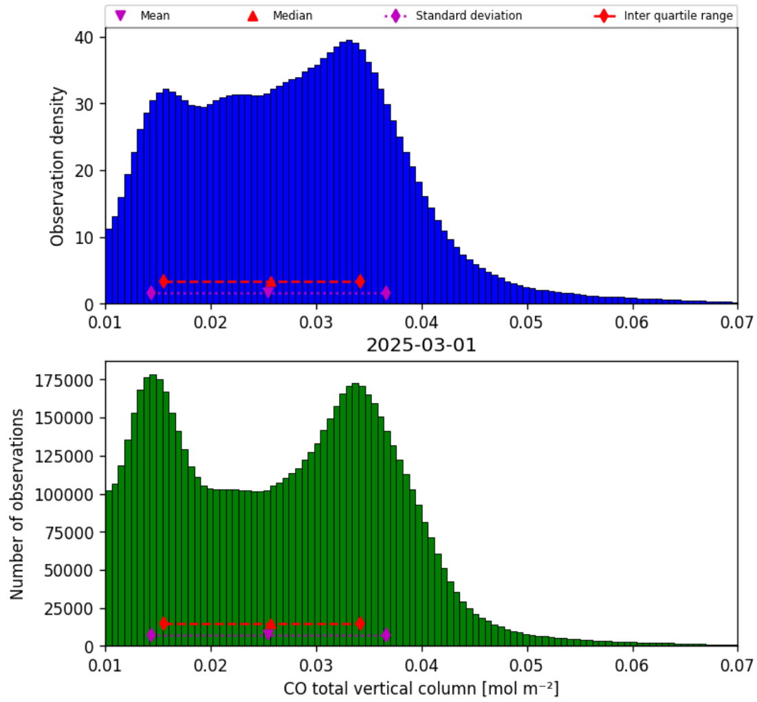
Figure 18: Histogram of “CO total vertical column” for 2025-03-01 to 2025-03-02
