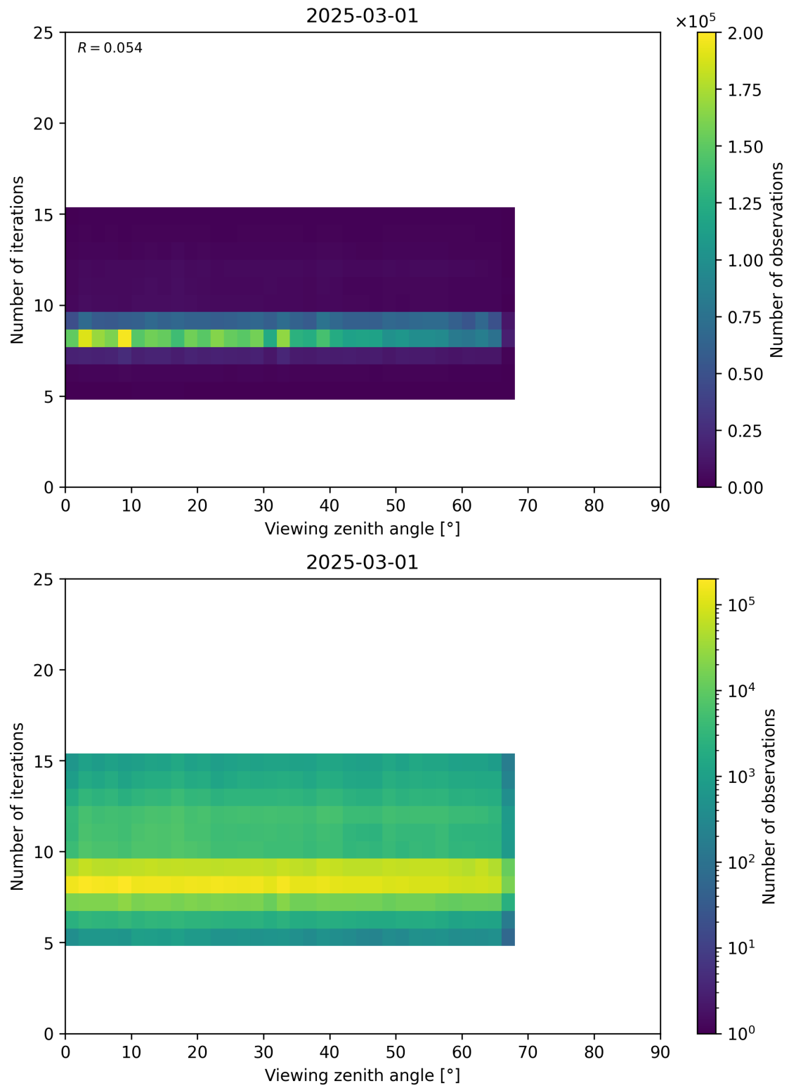
Figure 75: Scatter density plot of “Viewing zenith angle” against “Number of iterations” for 2025-03-01 to 2025-03-02.
