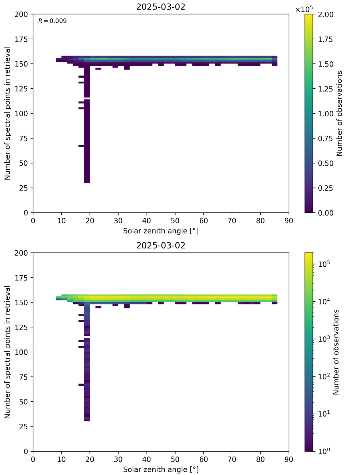
Figure 68: Scatter density plot of “Solar zenith angle” against “Number of spectral points in retrieval” for 2025-03-01 to 2025-03-03.
