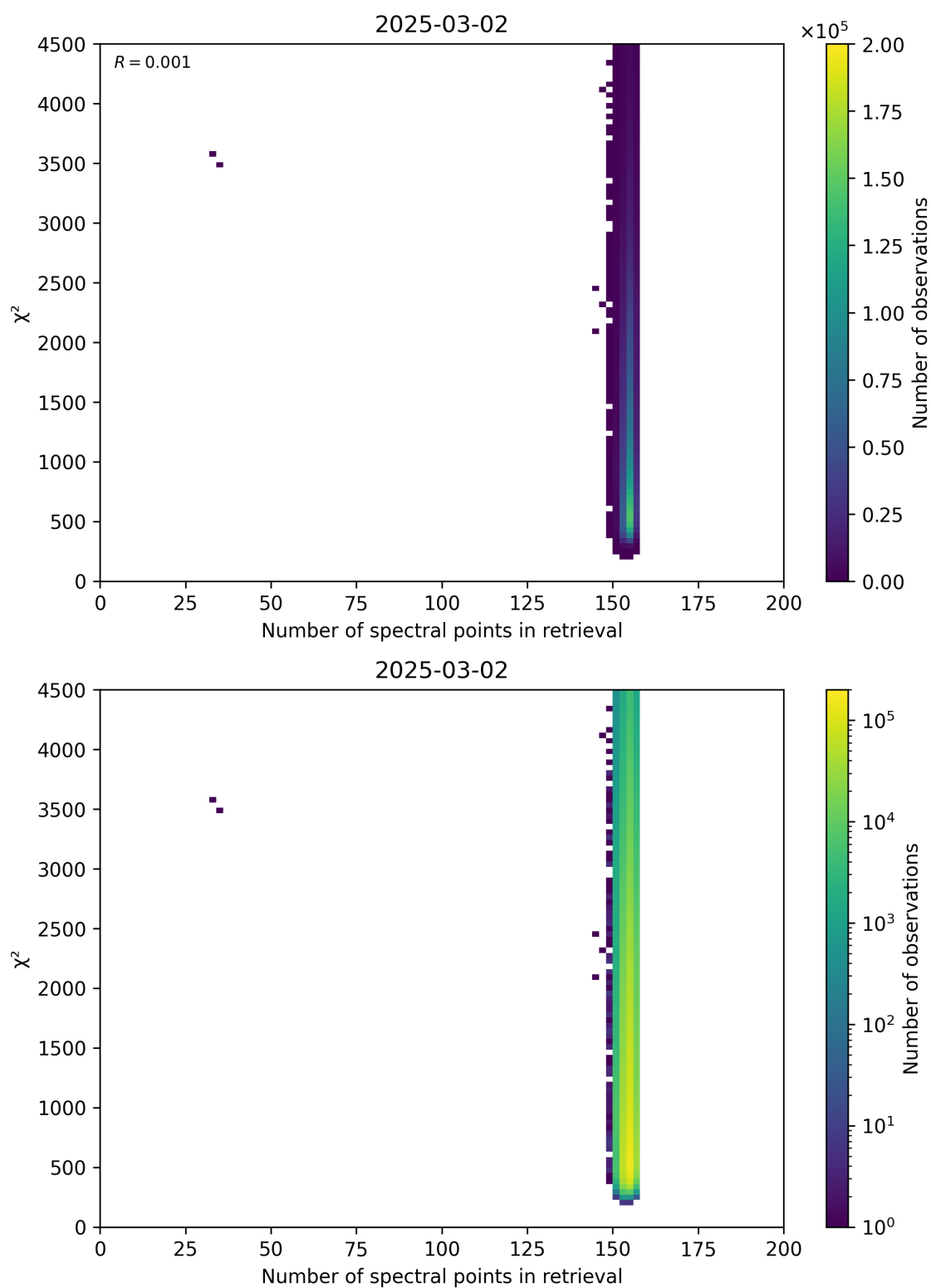
Figure 58: Scatter density plot of “Number of spectral points in retrieval” against “ \chi^2 ” for 2025-03-01 to 2025-03-03.
