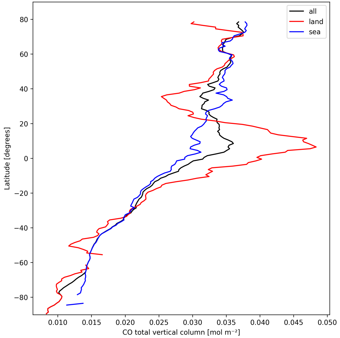
Figure 10: Zonal average of “CO total vertical column” for 2025-03-01 to 2025-03-03.
