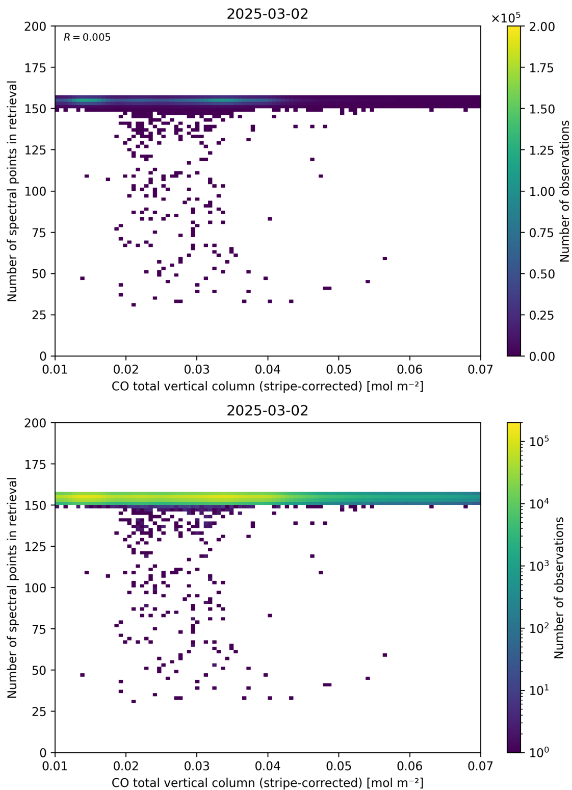
Figure 40: Scatter density plot of “CO total vertical column (stripe-corrected)” against “Number of spectral points in retrieval” for 2025-03-01 to 2025-03-03.
