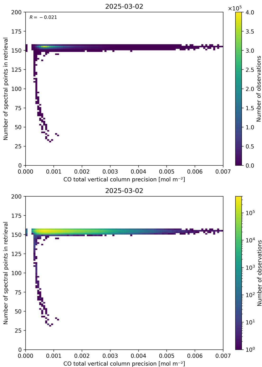
Figure 47: Scatter density plot of “CO total vertical column precision” against “Number of spectral points in retrieval” for 2025-03-01 to 2025-03-03.
