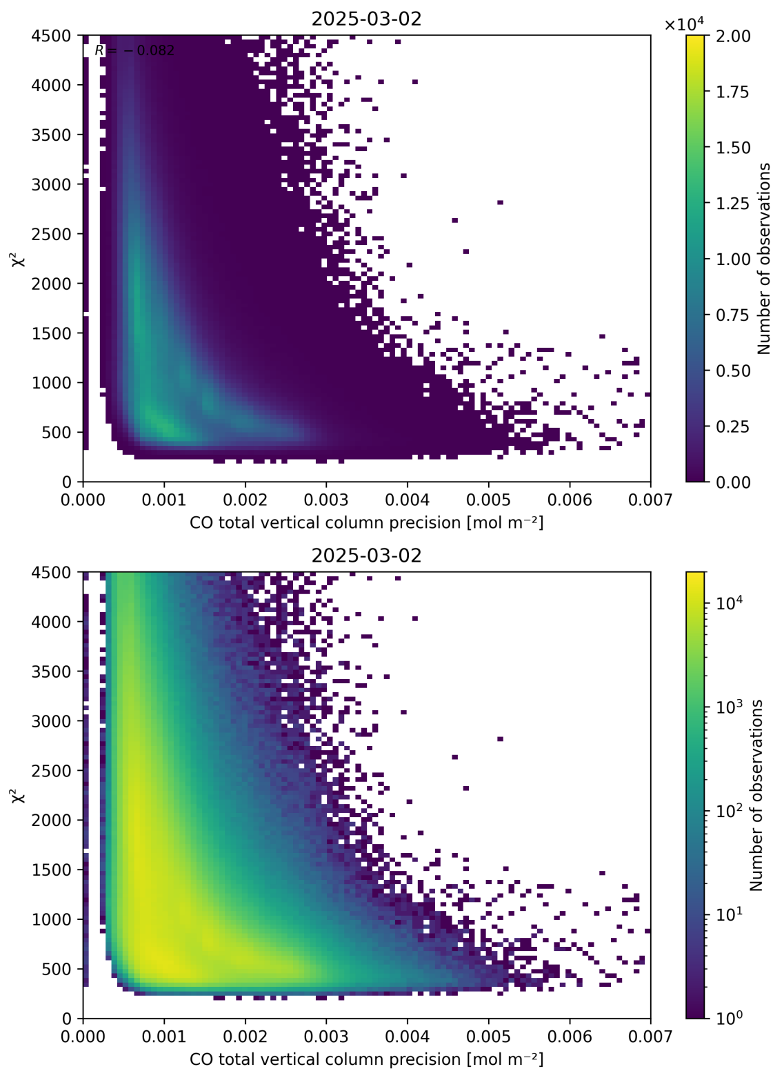
Figure 44: Scatter density plot of “CO total vertical column precision” against “ \chi^2 ” for 2025-03-01 to 2025-03-03.
