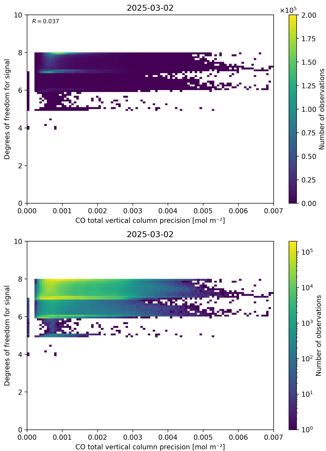
Figure 45: Scatter density plot of “CO total vertical column precision” against “Degrees of freedom for signal” for 2025-03-01 to 2025-03-03.
