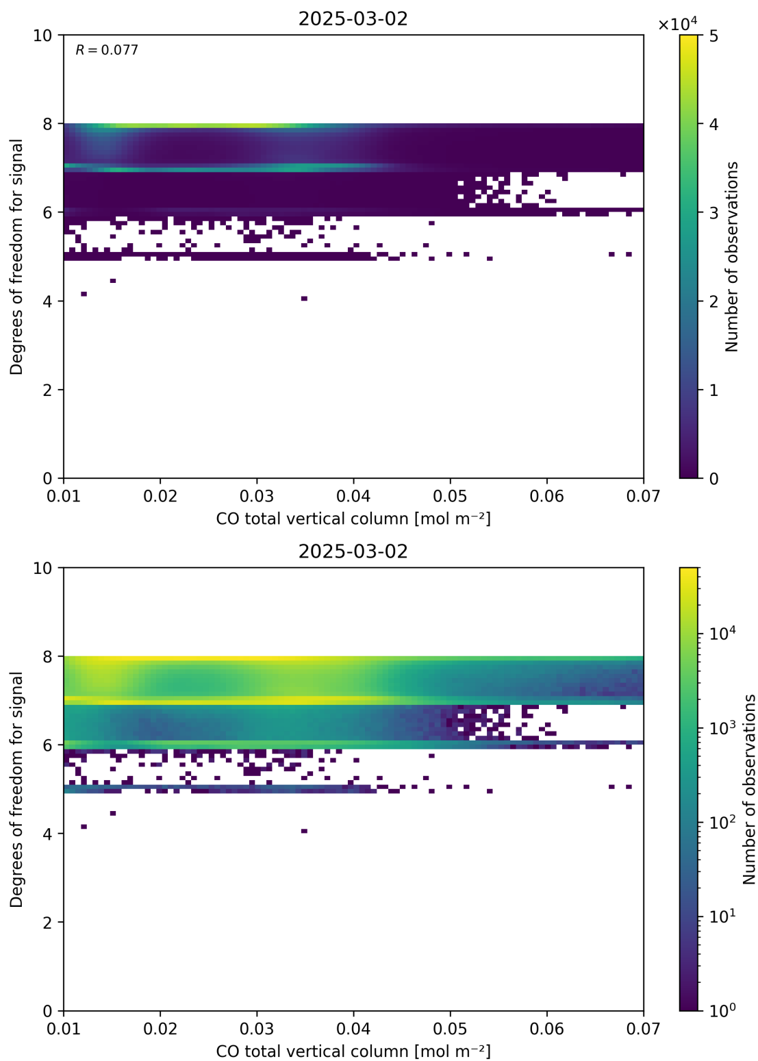
Figure 41: Scatter density plot of “CO total vertical column” against “Degrees of freedom for signal” for 2025-03-01 to 2025-03-03.
