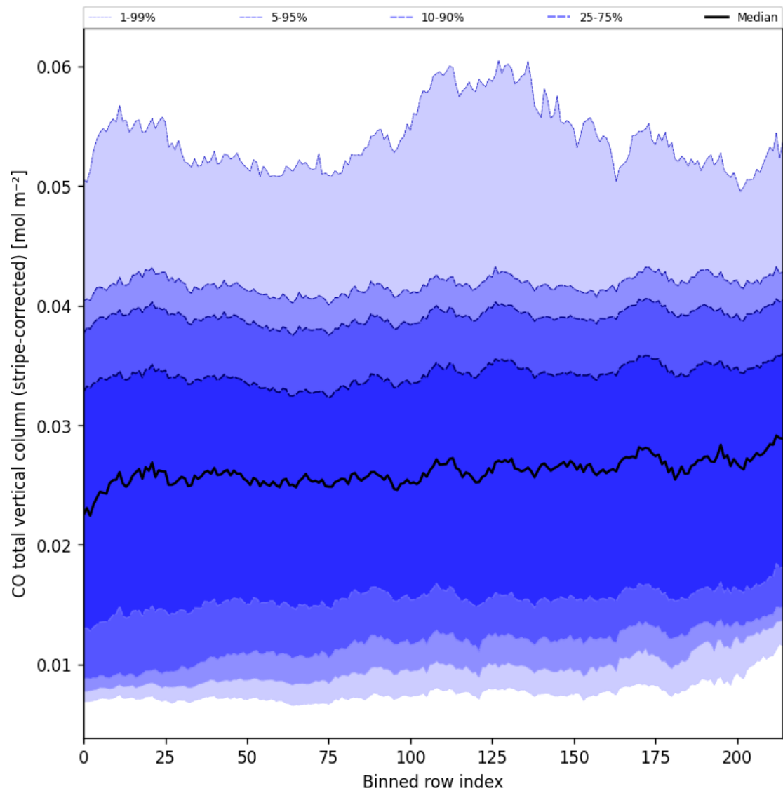
Figure 27: Along track statistics of “CO total vertical column (stripe-corrected)” for 2025-03-01 to 2025-03-03
