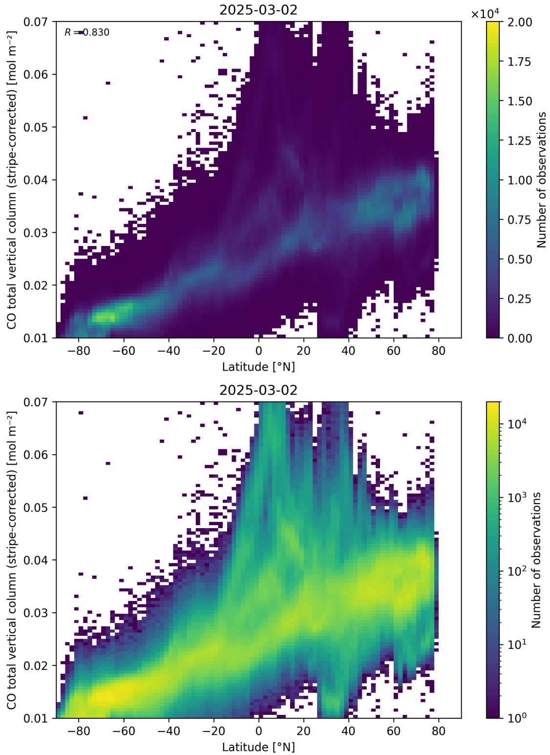
Figure 52: Scatter density plot of “Latitude” against “CO total vertical column (stripe-corrected)” for 2025-03-01 to 2025-03-03.
