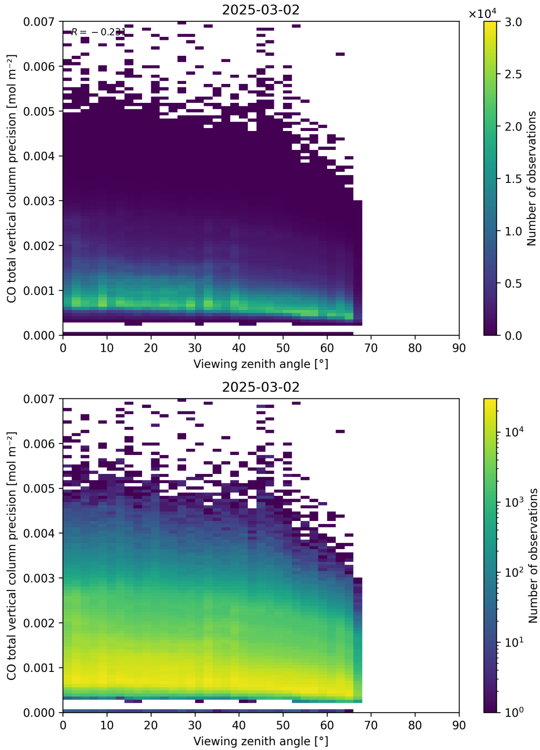
Figure 71: Scatter density plot of “Viewing zenith angle” against “CO total vertical column precision” for 2025-03-01 to 2025-03-03.
