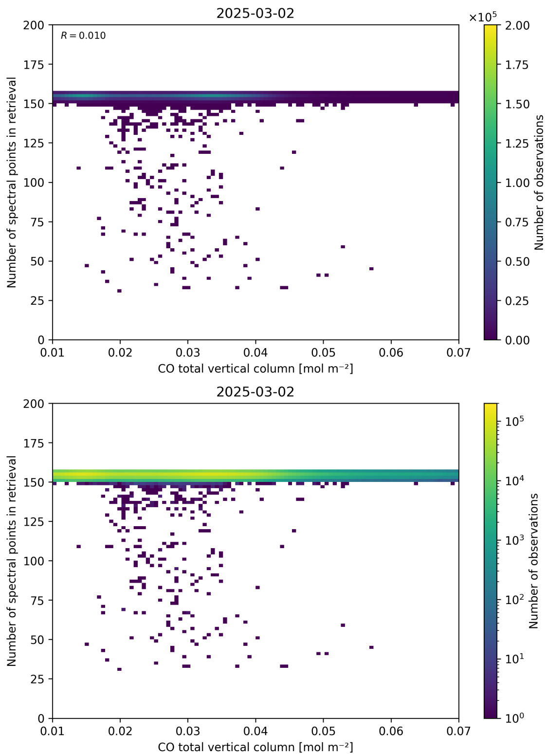
Figure 43: Scatter density plot of “CO total vertical column” against “Number of spectral points in retrieval” for 2025-03-01 to 2025-03-03.
