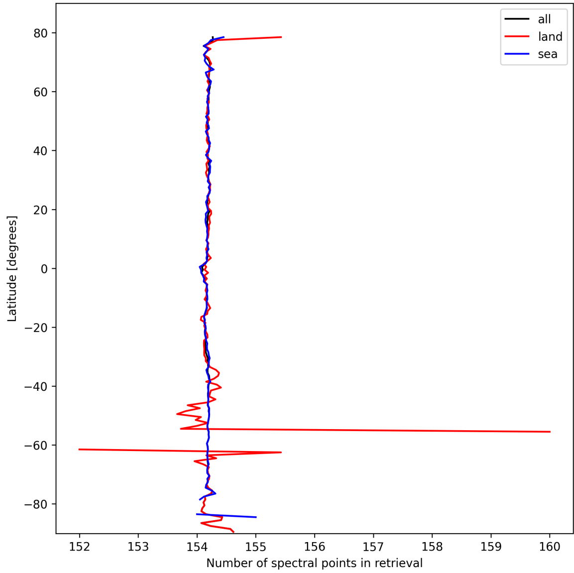
Figure 13: Zonal average of “Number of spectral points in retrieval” for 2025-03-01 to 2025-03-03.
