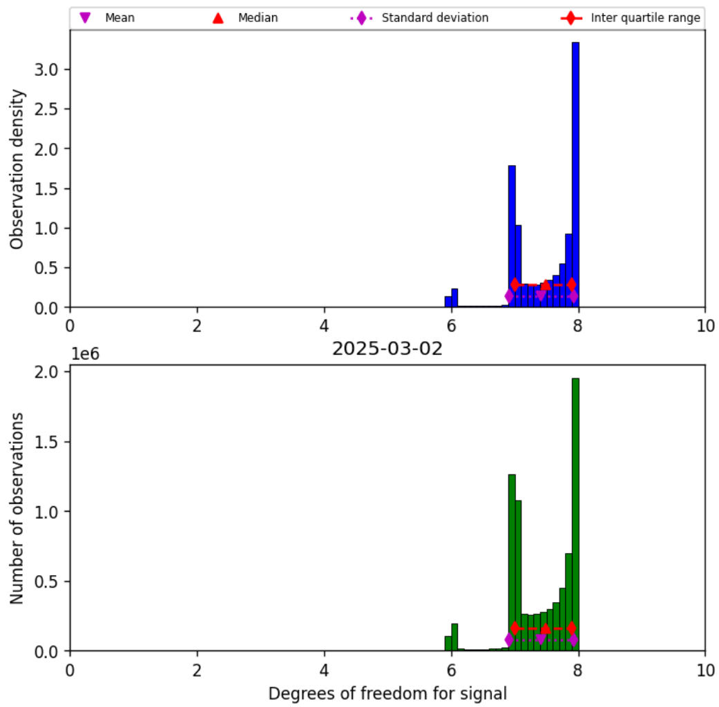
Figure 23: Histogram of “Degrees of freedom for signal” for 2025-03-01 to 2025-03-03
