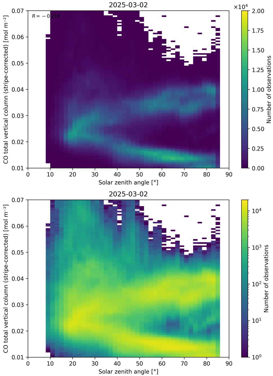
Figure 62: Scatter density plot of “Solar zenith angle” against “CO total vertical column (stripe-corrected)” for 2025-03-01 to 2025-03-03.
