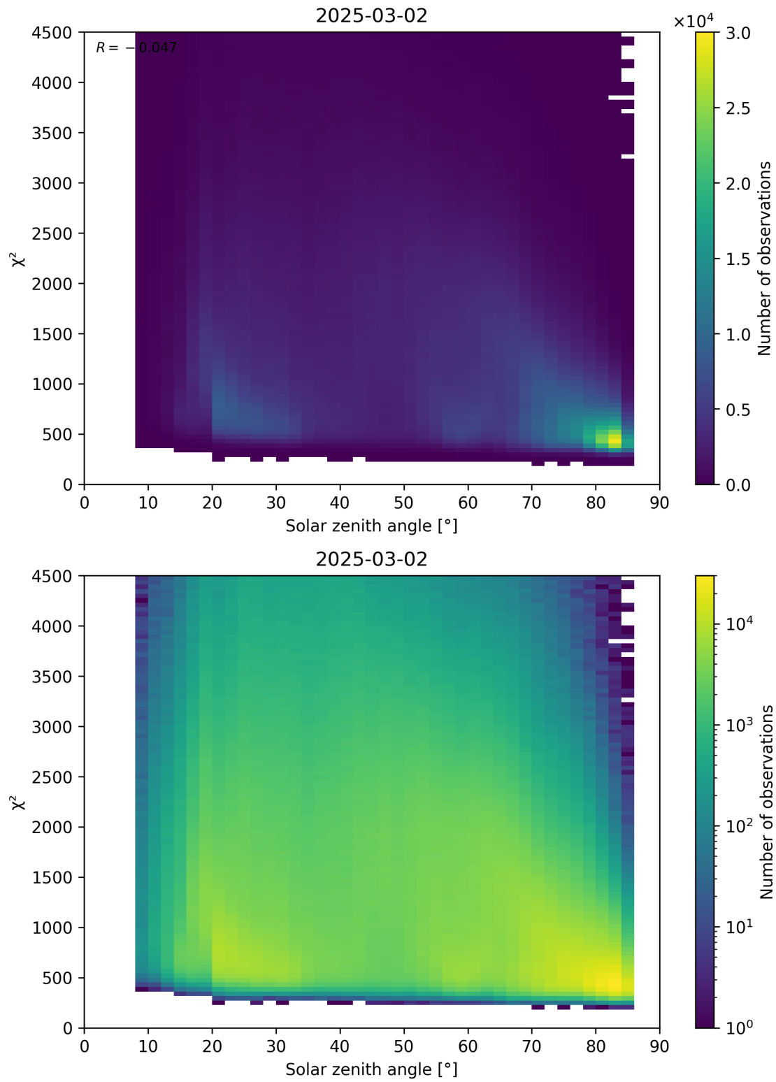
Figure 64: Scatter density plot of “Solar zenith angle” against “ \chi^2 ” for 2025-03-01 to 2025-03-03.
