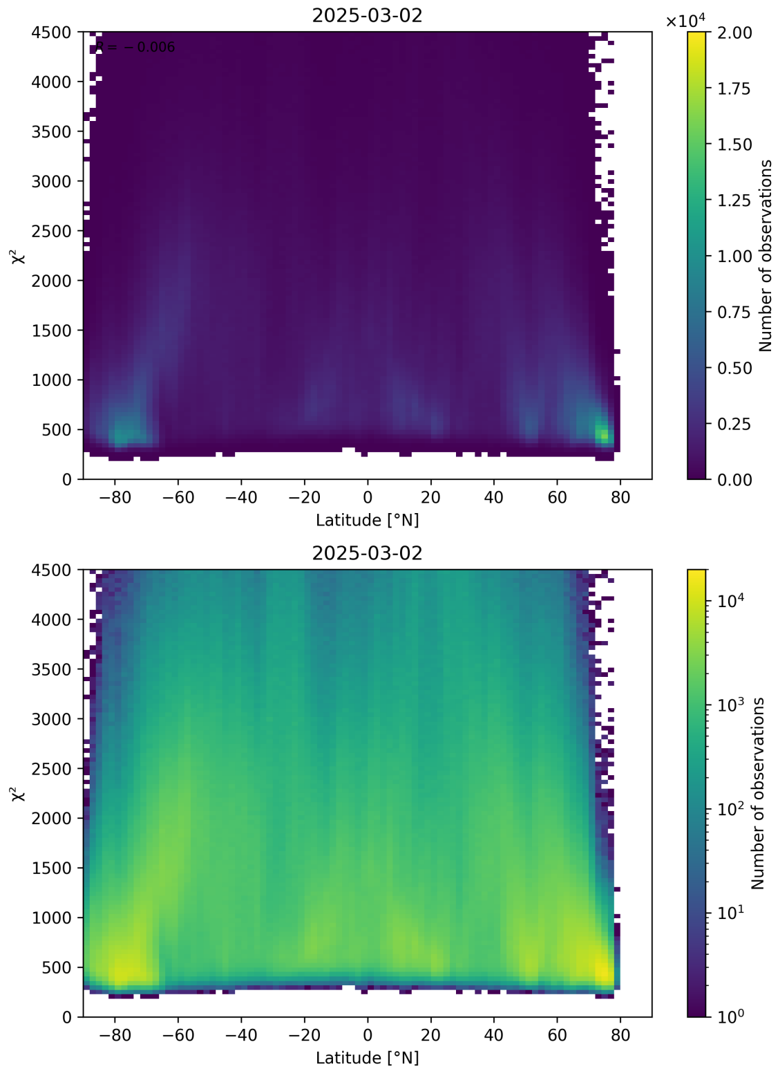
Figure 54: Scatter density plot of “Latitude” against “ \chi^2 ” for 2025-03-01 to 2025-03-03.
