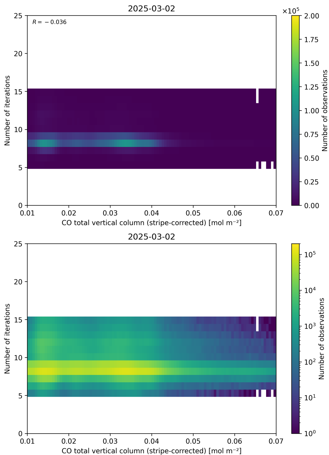
Figure 39: Scatter density plot of “CO total vertical column (stripe-corrected)” against “Number of iterations” for 2025-03-01 to 2025-03-03.
