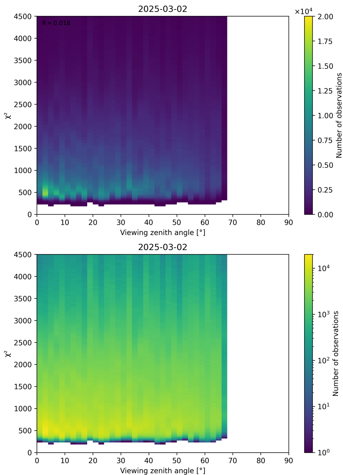
Figure 72: Scatter density plot of “Viewing zenith angle” against “ \chi^2 ” for 2025-03-01 to 2025-03-03.
