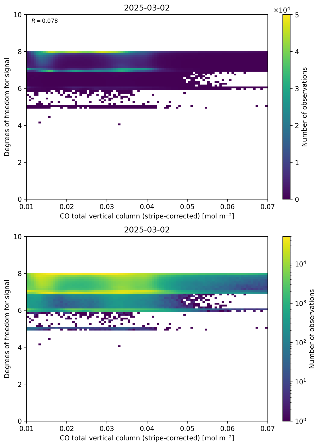
Figure 38: Scatter density plot of “CO total vertical column (stripe-corrected)” against “Degrees of freedom for signal” for 2025-03-01 to 2025-03-03.
