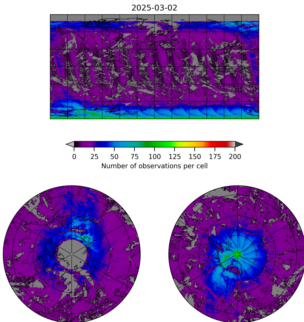
Figure 8: Map of the number of observations for 2025-03-01 to 2025-03-03
