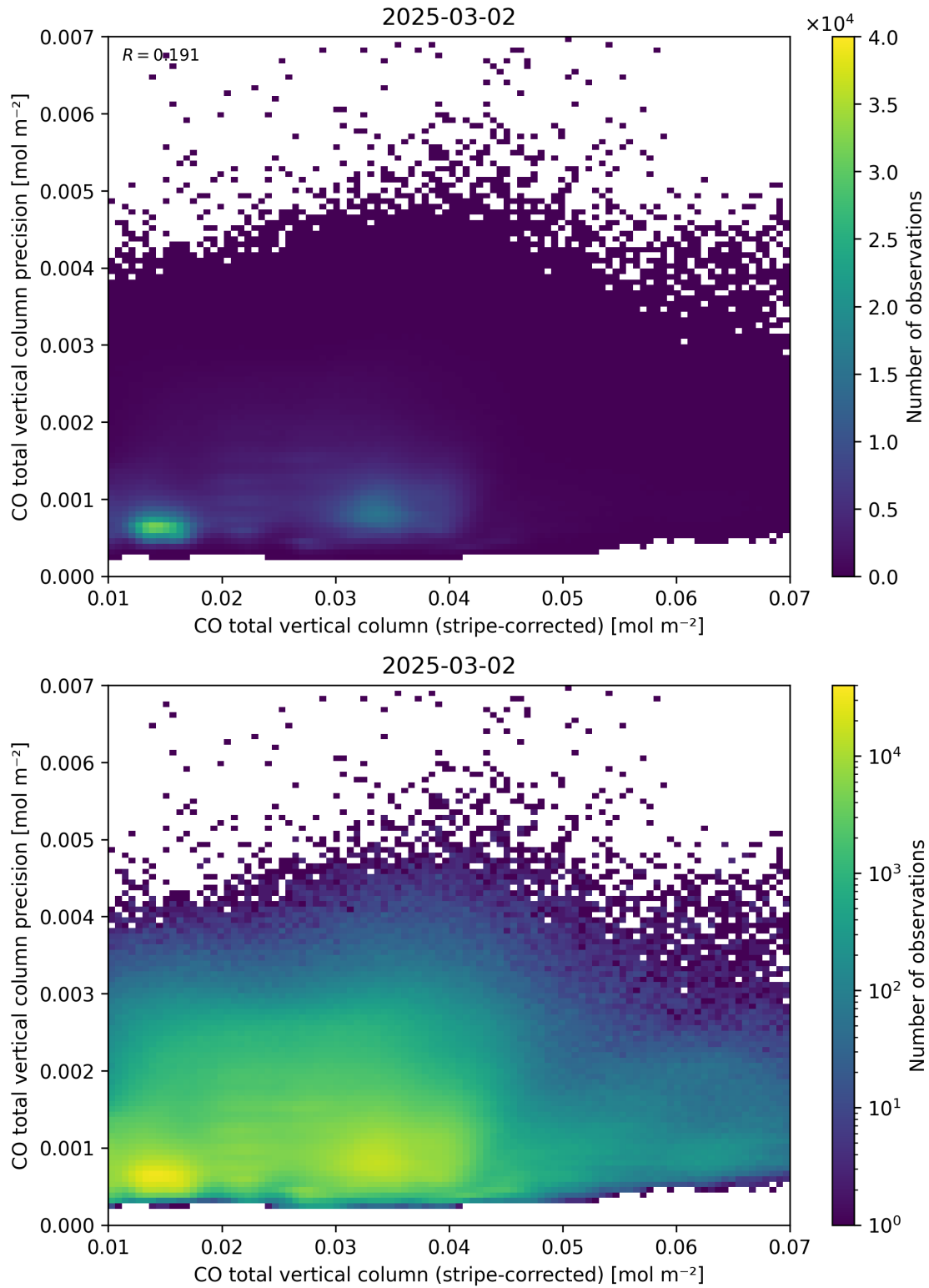
Figure 36: Scatter density plot of “CO total vertical column (stripe-corrected)” against “CO total vertical column precision” for 2025-03-01 to 2025-03-03.
