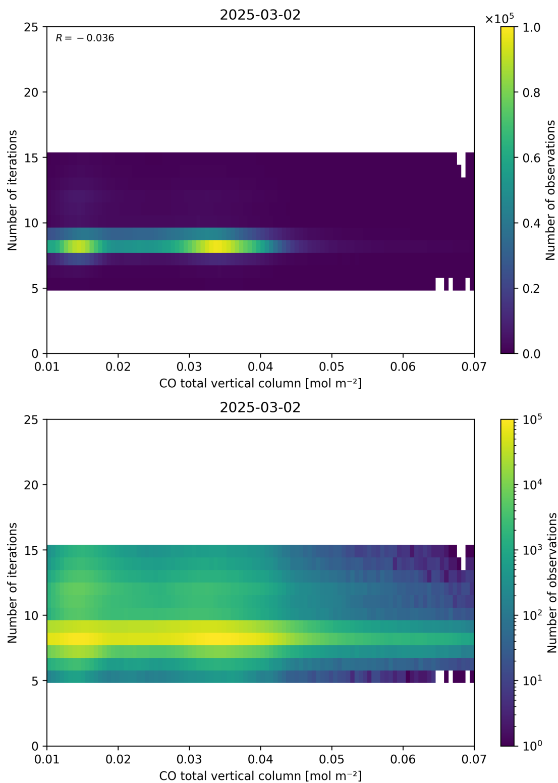
Figure 42: Scatter density plot of “CO total vertical column” against “Number of iterations” for 2025-03-01 to 2025-03-03.
