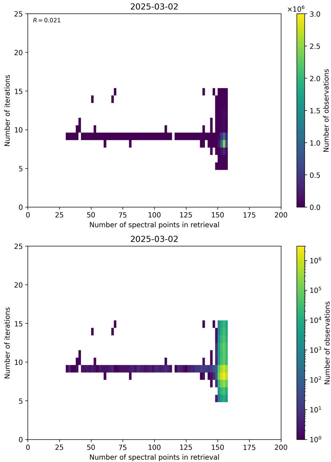
Figure 60: Scatter density plot of “Number of spectral points in retrieval” against “Number of iterations” for 2025-03-01 to 2025-03-03.
