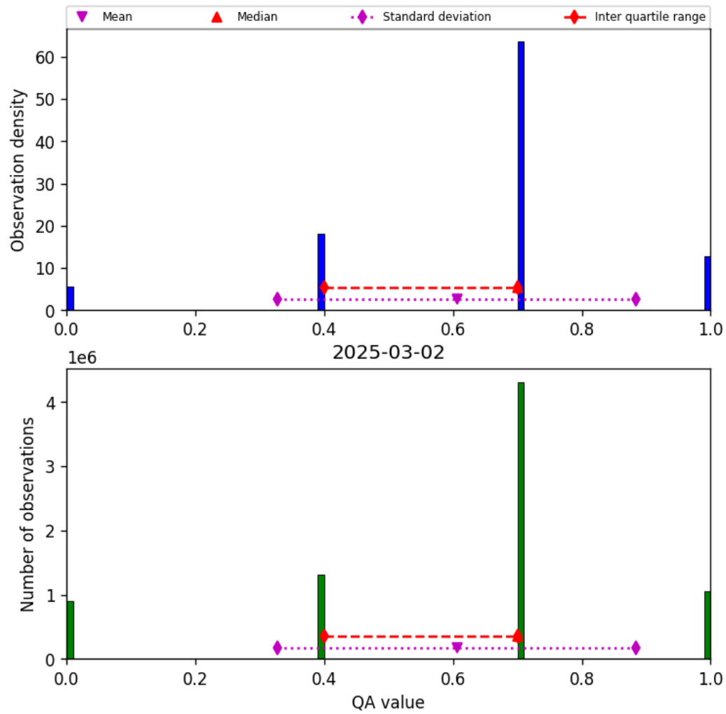
Figure 17: Histogram of “QA value” for 2025-03-01 to 2025-03-03
