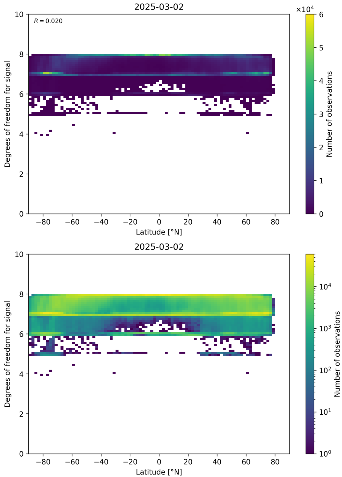
Figure 55: Scatter density plot of “Latitude” against “Degrees of freedom for signal” for 2025-03-01 to 2025-03-03.
