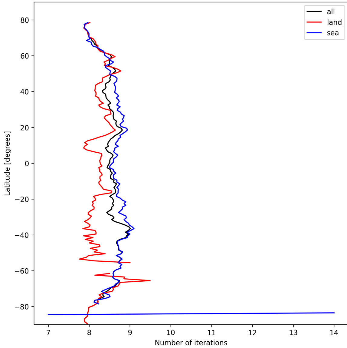
Figure 16: Zonal average of “Number of iterations” for 2025-03-01 to 2025-03-03.
