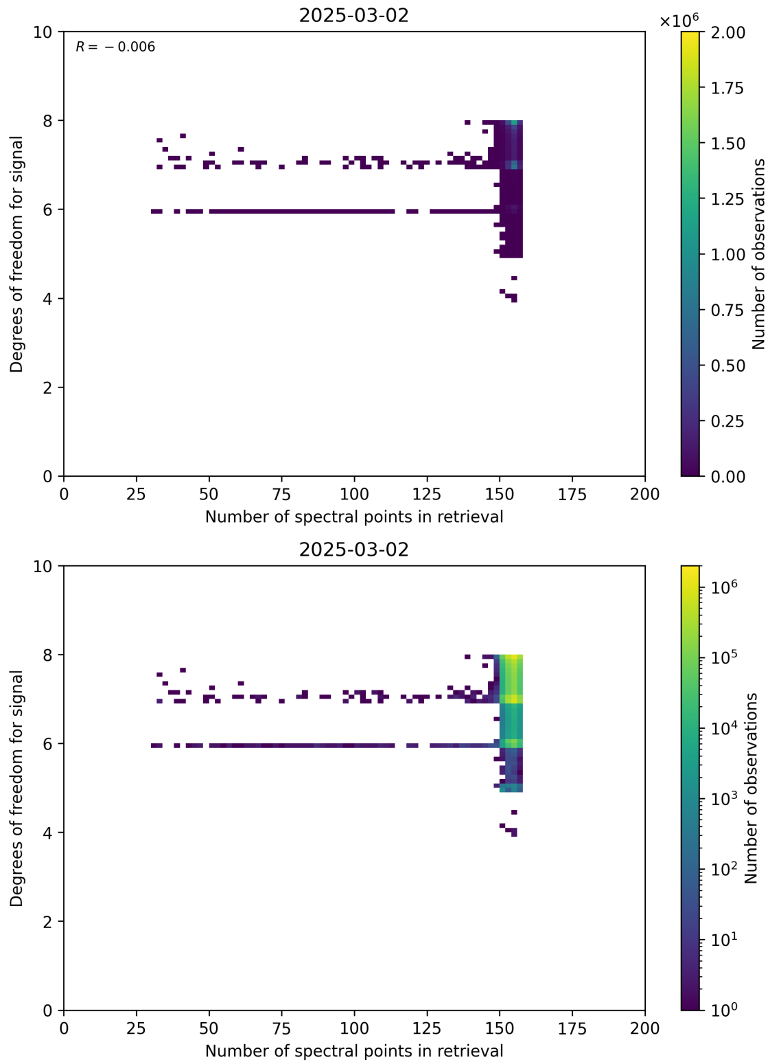
Figure 59: Scatter density plot of “Number of spectral points in retrieval” against “Degrees of freedom for signal” for 2025-03-01 to 2025-03-03.
