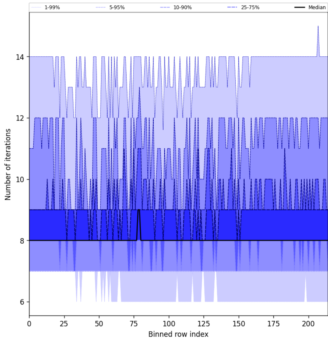
Figure 32: Along track statistics of “Number of iterations” for 2025-03-01 to 2025-03-03
