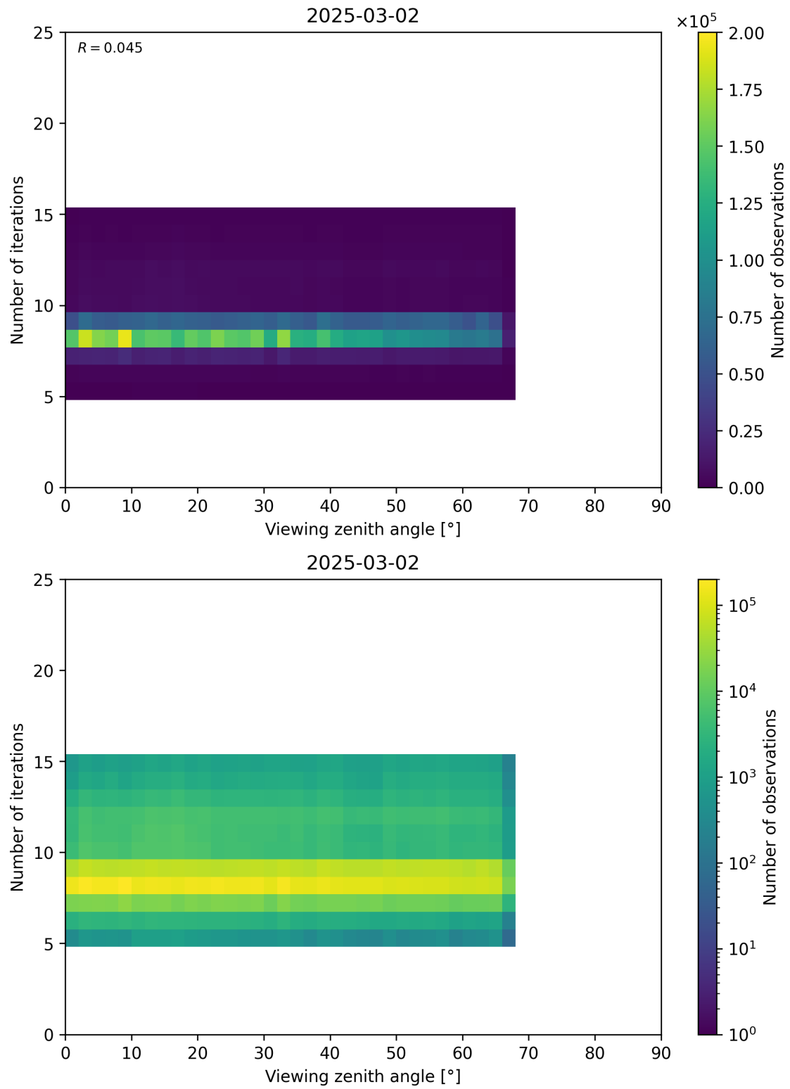
Figure 75: Scatter density plot of “Viewing zenith angle” against “Number of iterations” for 2025-03-01 to 2025-03-03.
