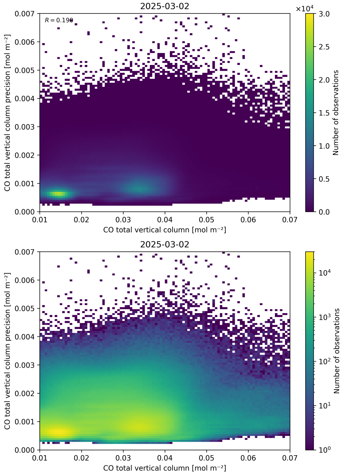
Figure 34: Scatter density plot of “CO total vertical column” against “CO total vertical column precision” for 2025-03-01 to 2025-03-03.
