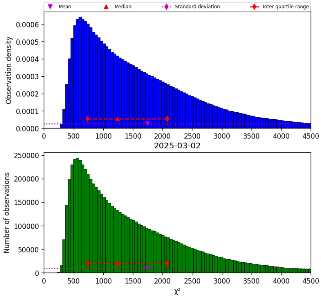
Figure 22: Histogram of " \chi^2 " for 2025-03-01 to 2025-03-03
