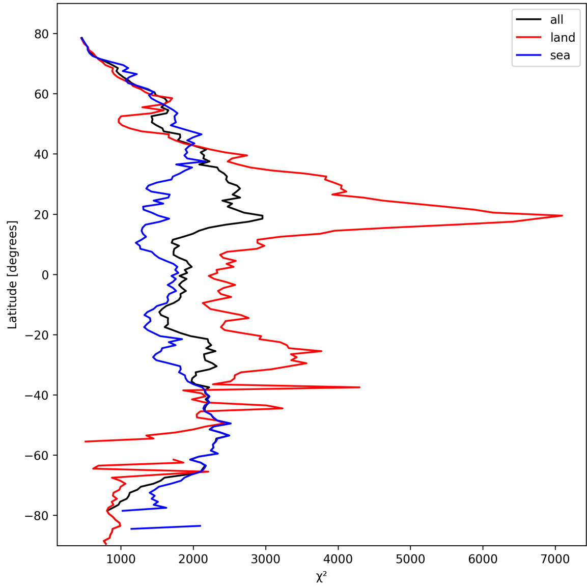
Figure 14: Zonal average of “ \chi^2 ” for 2025-03-01 to 2025-03-03.
