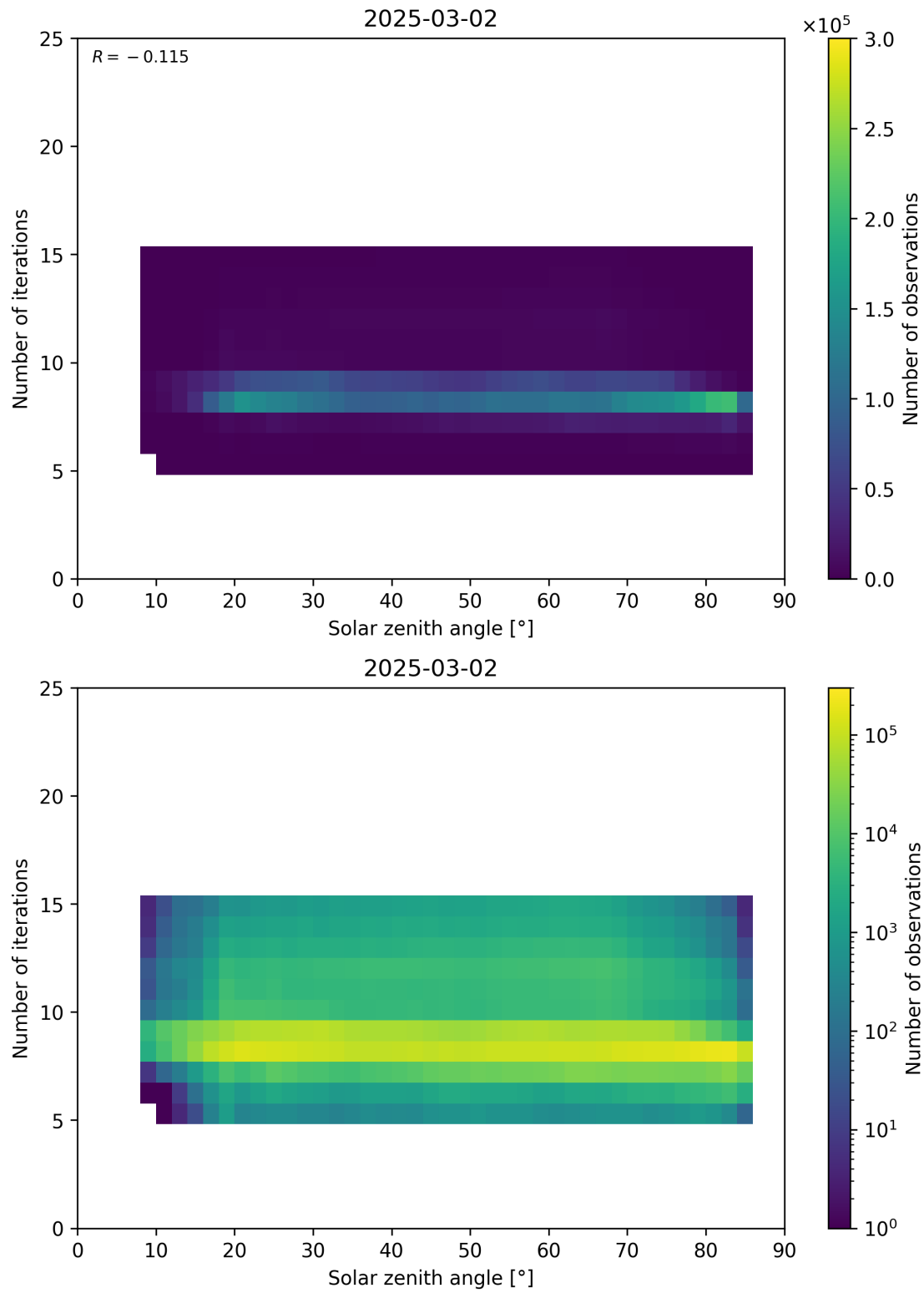
Figure 67: Scatter density plot of “Solar zenith angle” against “Number of iterations” for 2025-03-01 to 2025-03-03.
