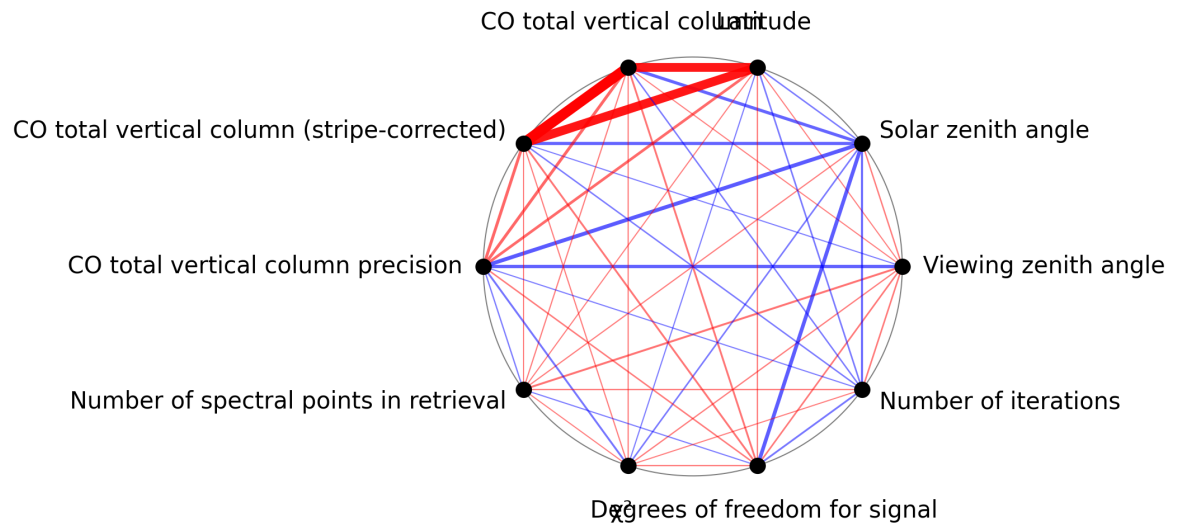
Figure 1: Map of correlation graph for 2025-03-01 to 2025-03-03.
