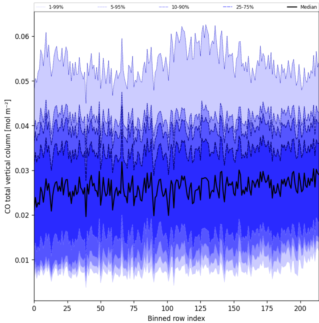
Figure 26: Along track statistics of “CO total vertical column” for 2025-03-01 to 2025-03-03
