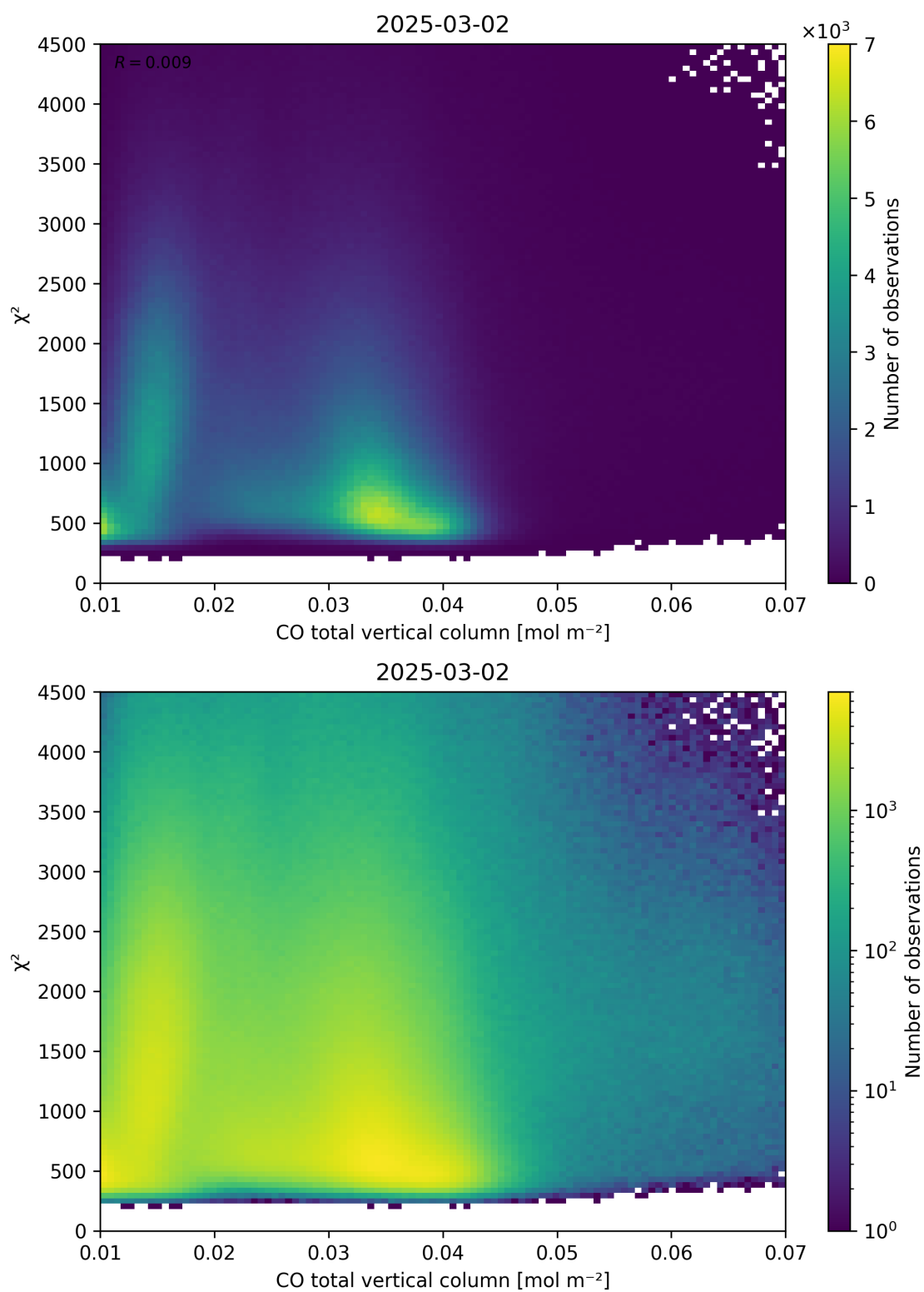
Figure 35: Scatter density plot of “CO total vertical column” against “ \chi^2 ” for 2025-03-01 to 2025-03-03.
