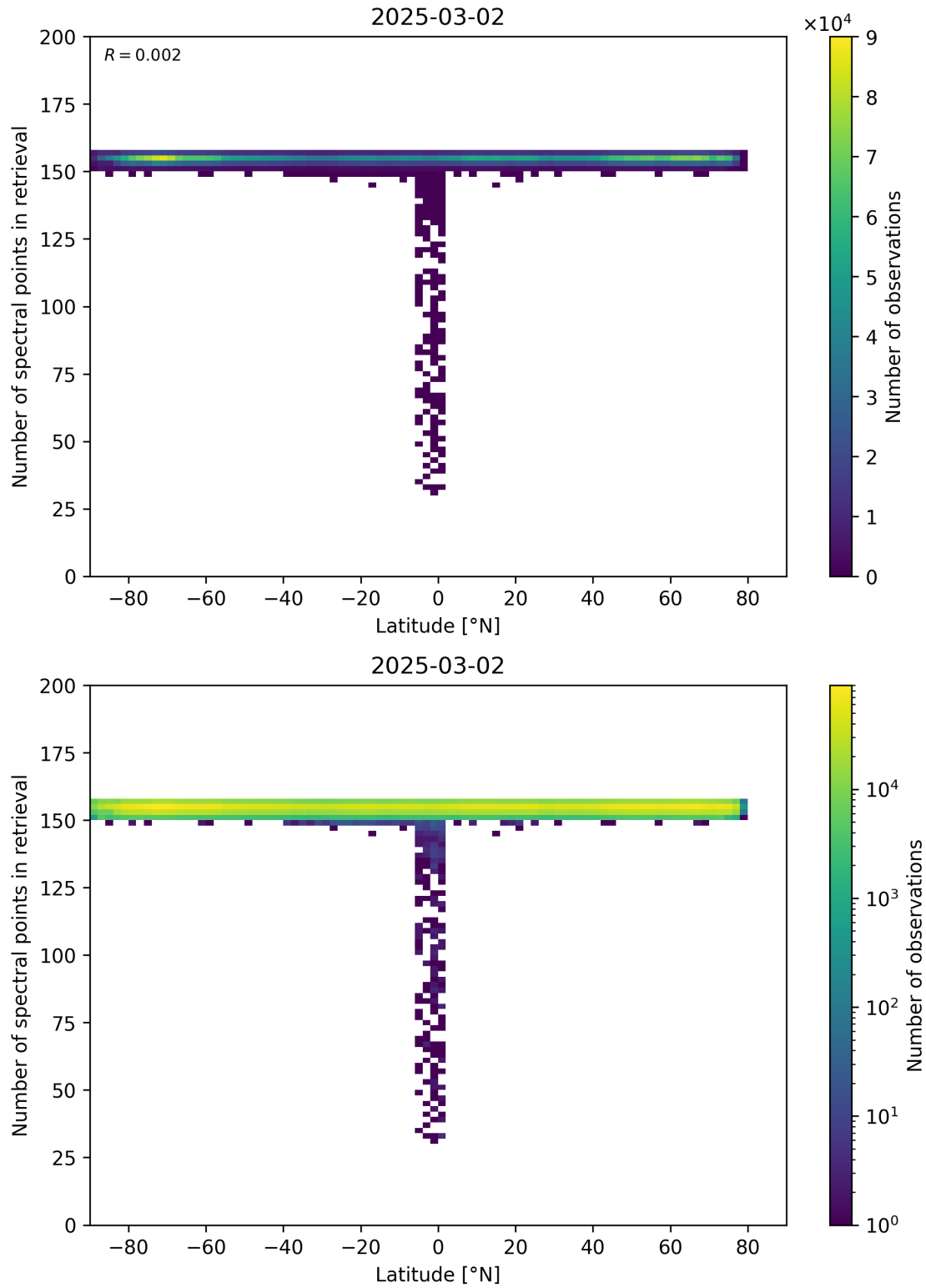
Figure 57: Scatter density plot of “Latitude” against “Number of spectral points in retrieval” for 2025-03-01 to 2025-03-03.
