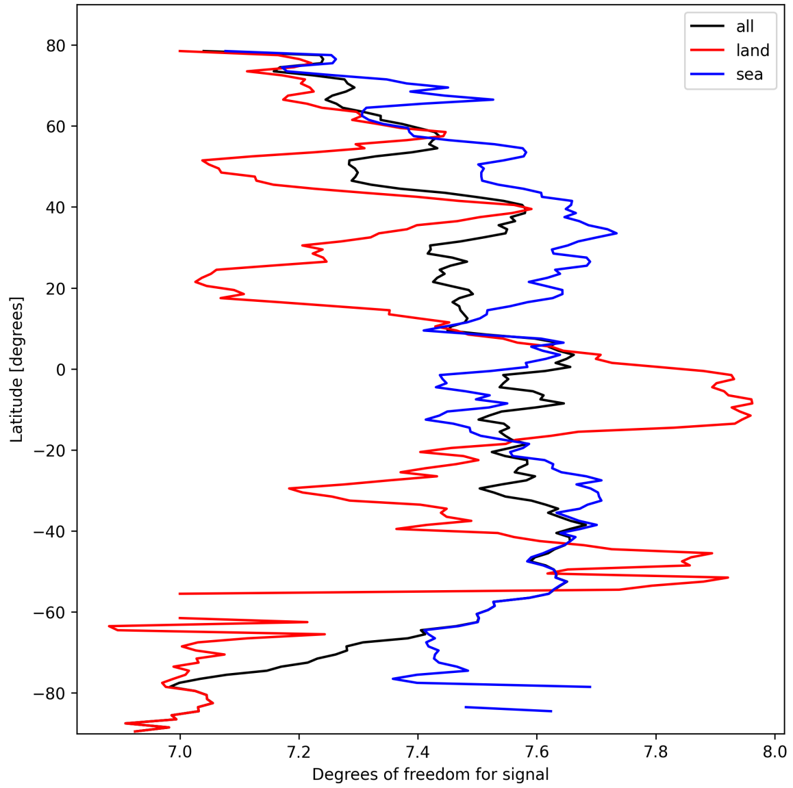
Figure 15: Zonal average of “Degrees of freedom for signal” for 2025-03-01 to 2025-03-03.
