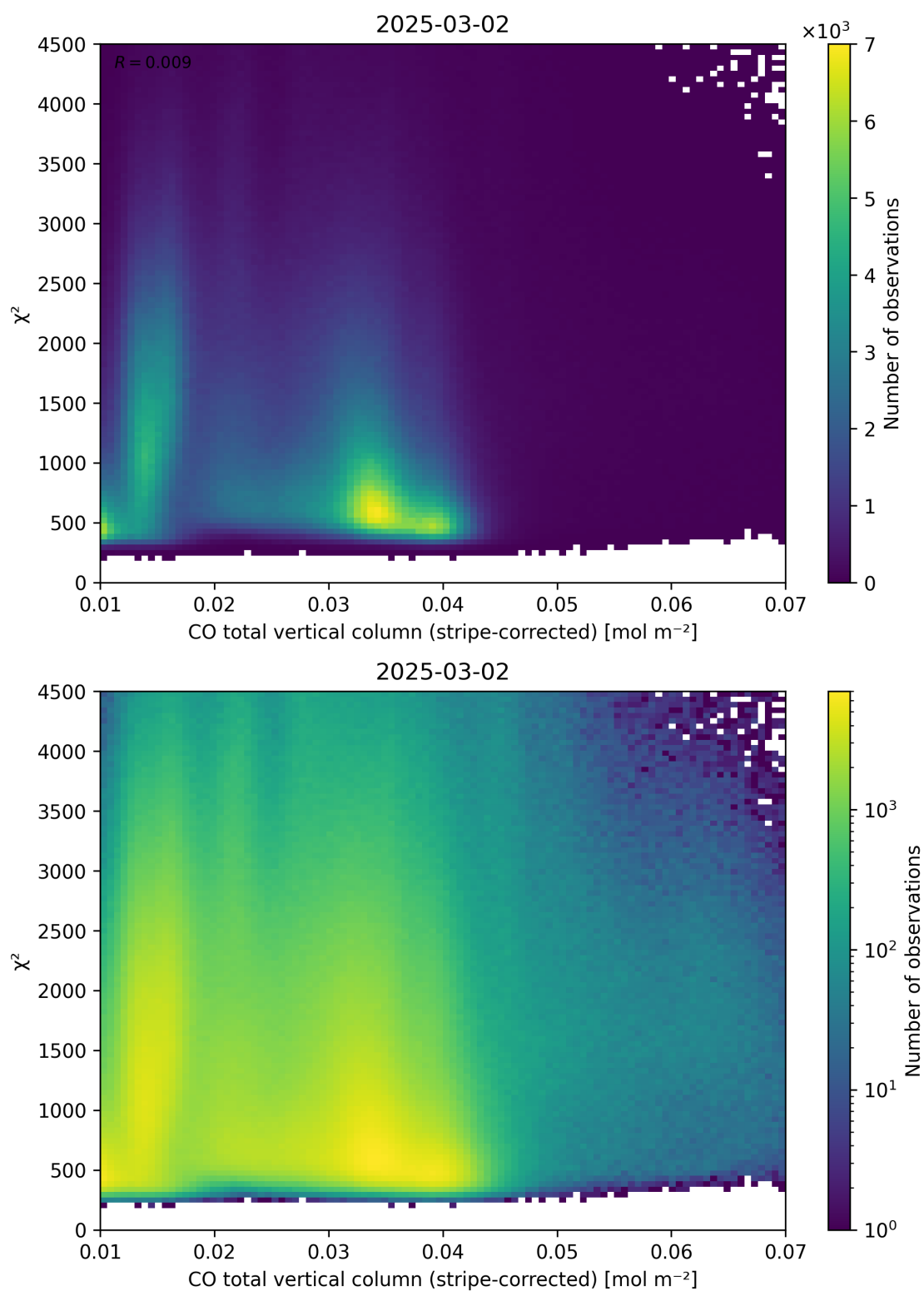
Figure 37: Scatter density plot of “CO total vertical column (stripe-corrected)” against “ \chi^2 ” for 2025-03-01 to 2025-03-03.
