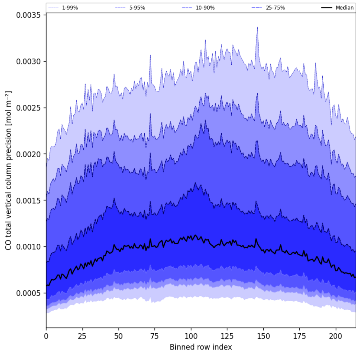
Figure 28: Along track statistics of “CO total vertical column precision” for 2025-03-01 to 2025-03-03
