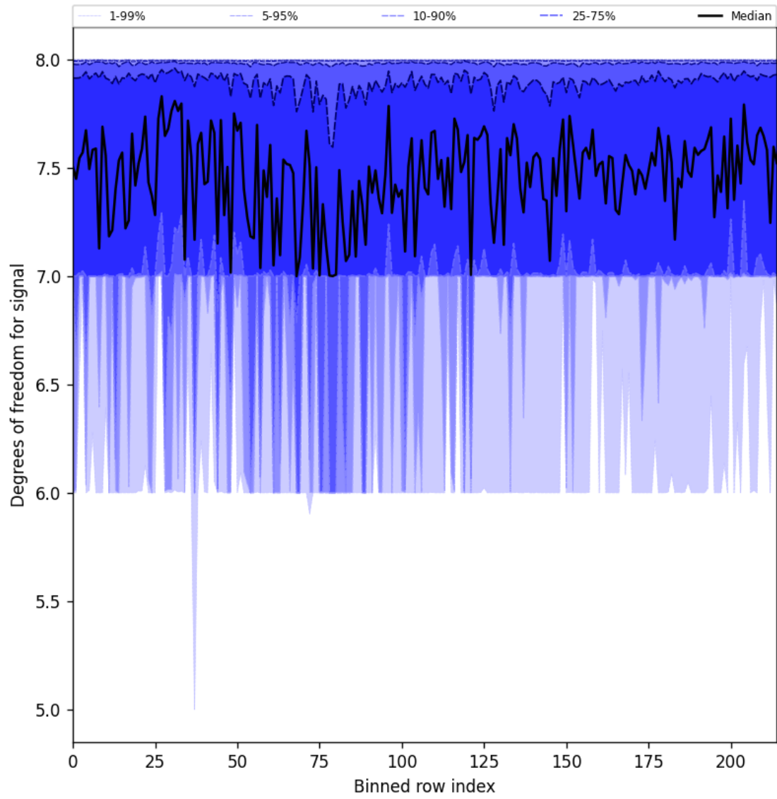
Figure 31: Along track statistics of “Degrees of freedom for signal” for 2025-03-01 to 2025-03-03
