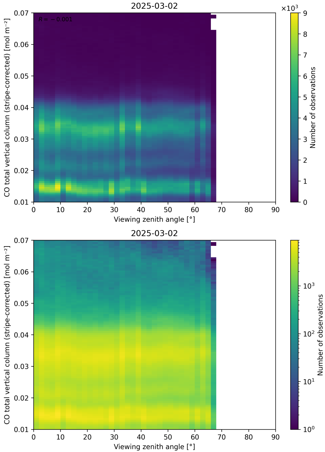
Figure 70: Scatter density plot of “Viewing zenith angle” against “CO total vertical column (stripe-corrected)” for 2025-03-01 to 2025-03-03.
