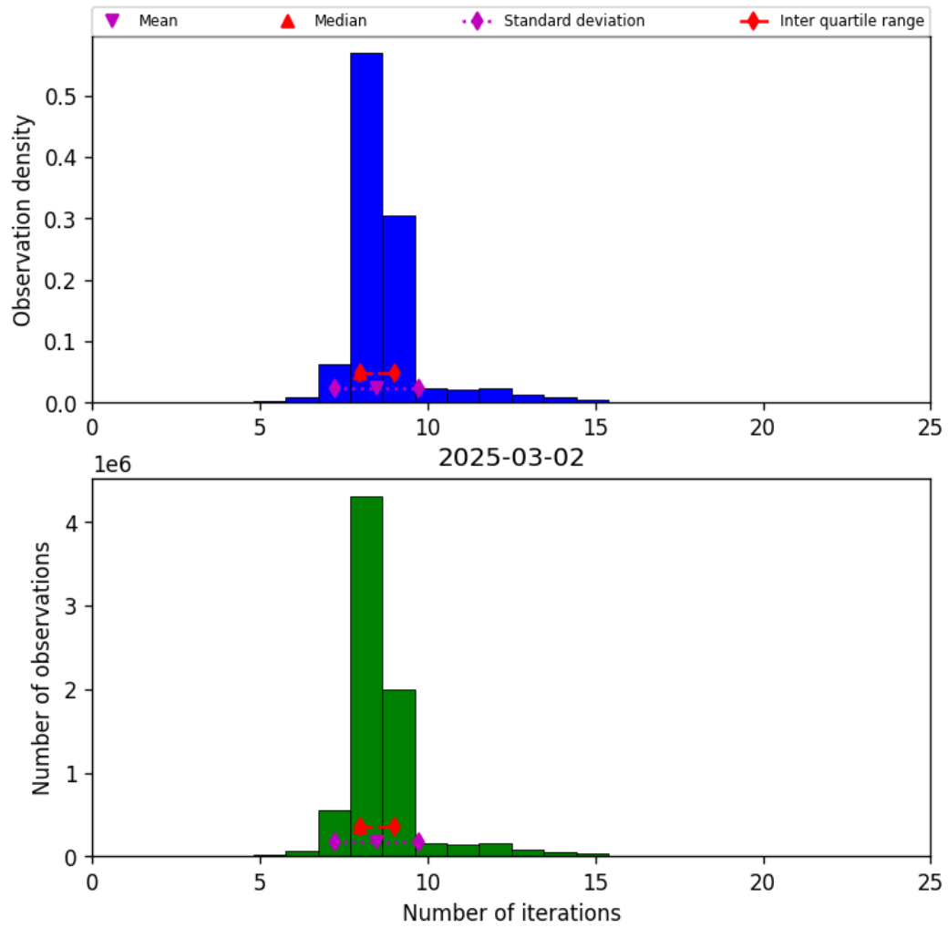
Figure 24: Histogram of “Number of iterations” for 2025-03-01 to 2025-03-03
