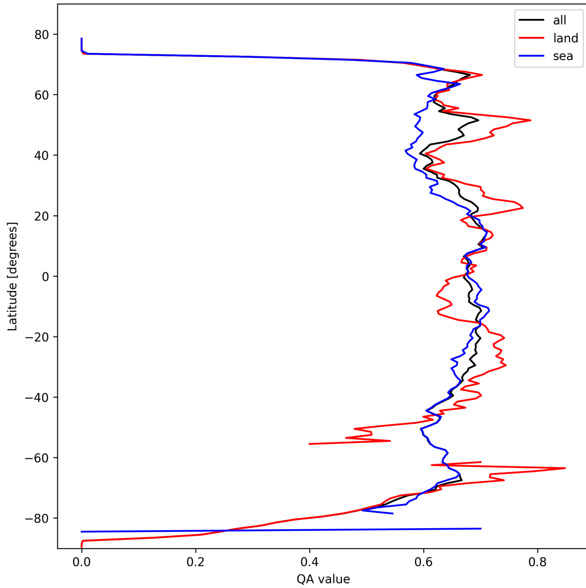
Figure 9: Zonal average of “QA value” for 2025-03-01 to 2025-03-03.
