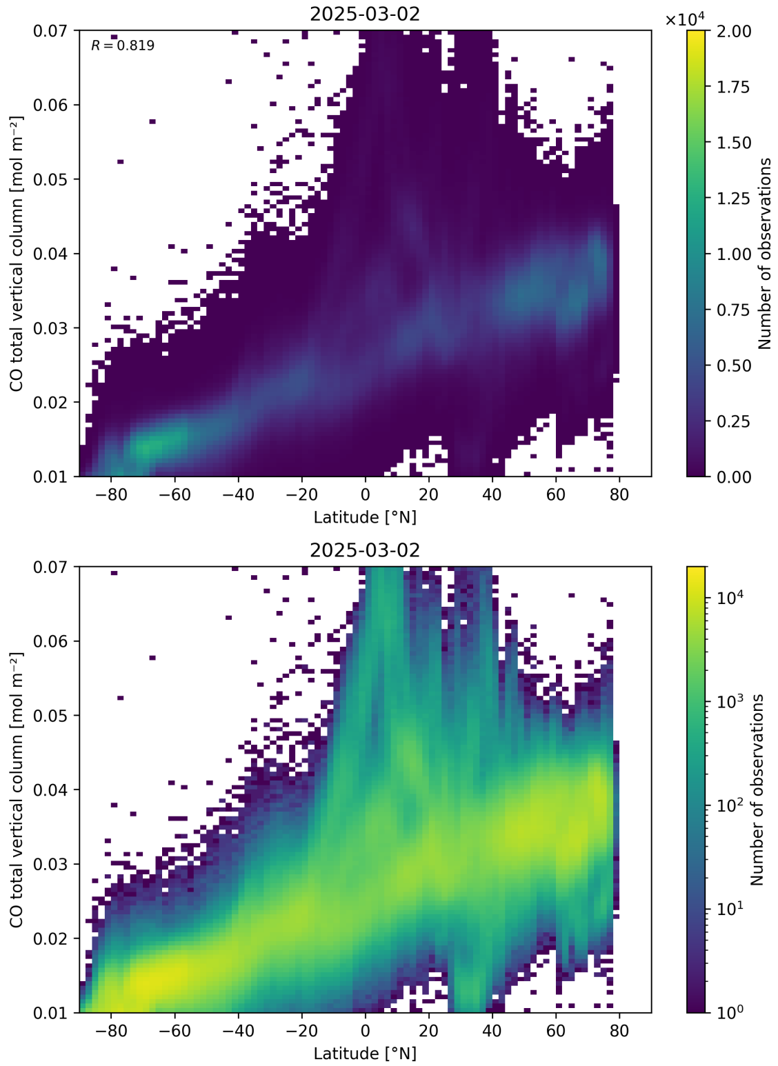
Figure 51: Scatter density plot of “Latitude” against “CO total vertical column” for 2025-03-01 to 2025-03-03.
