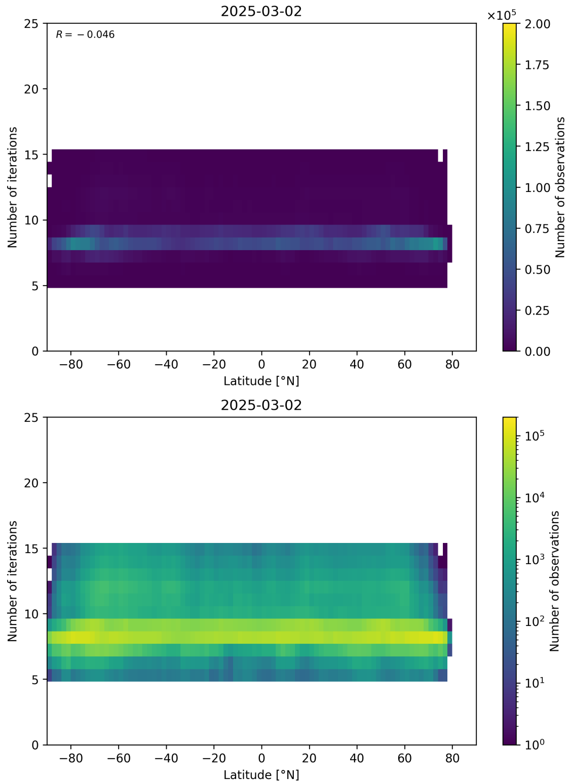
Figure 56: Scatter density plot of “Latitude” against “Number of iterations” for 2025-03-01 to 2025-03-03.
