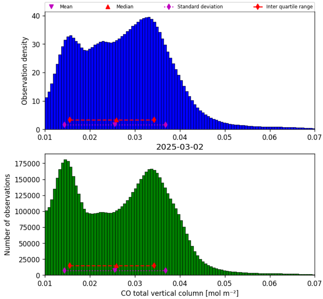
Figure 18: Histogram of “CO total vertical column” for 2025-03-01 to 2025-03-03
