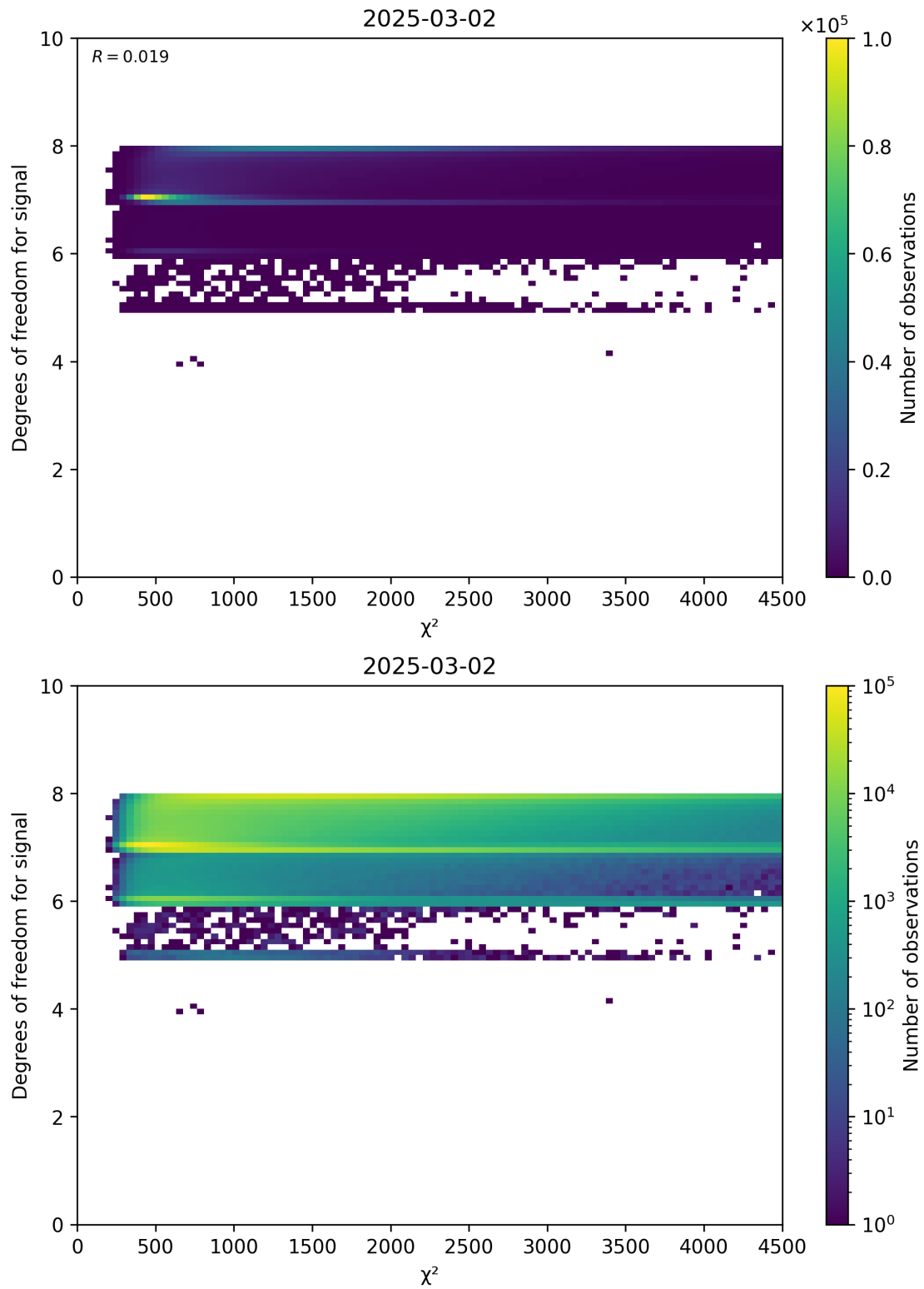
Figure 48: Scatter density plot of “ \chi^2 ” against “Degrees of freedom for signal” for 2025-03-01 to 2025-03-03.
