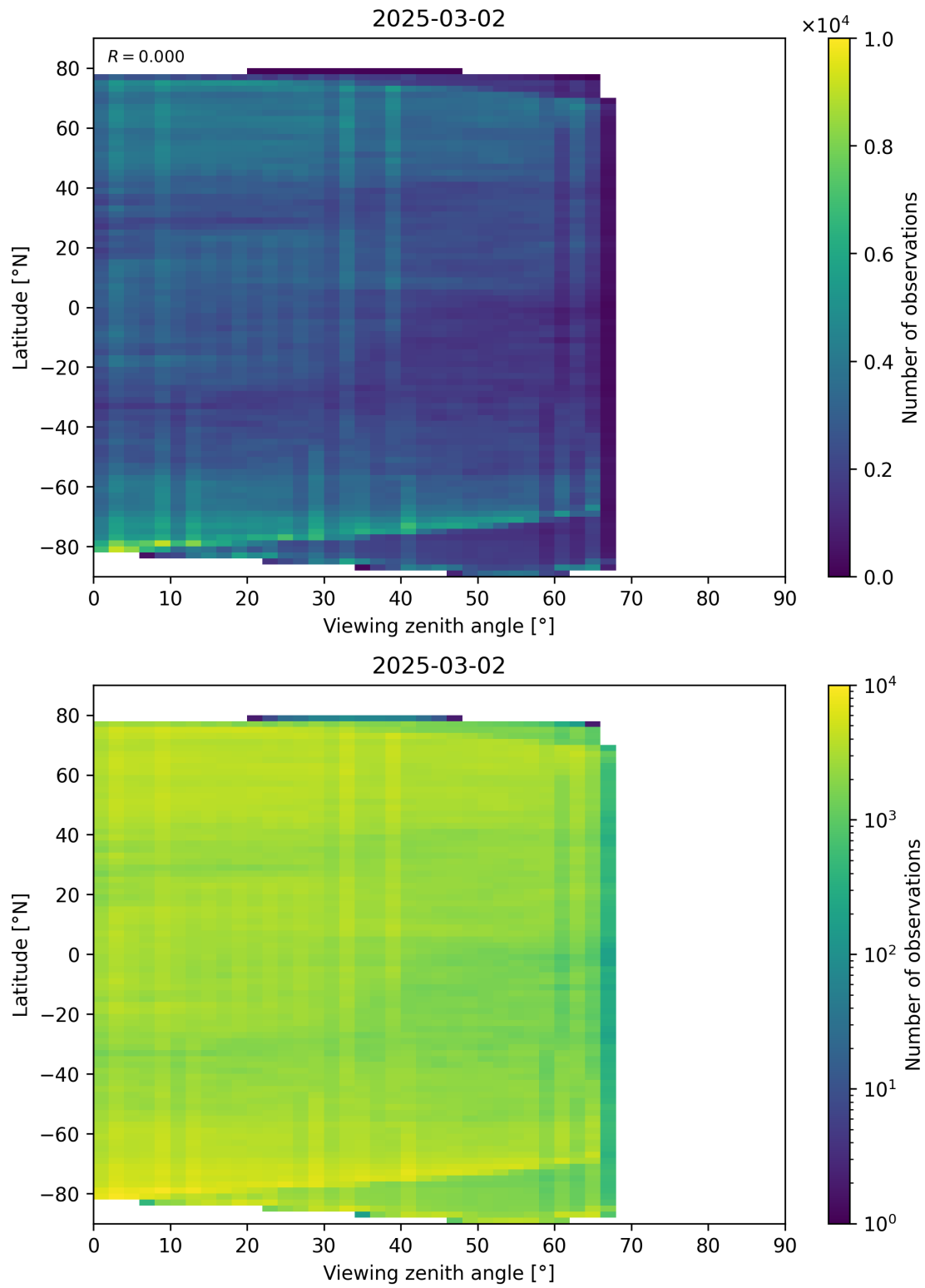
Figure 74: Scatter density plot of “Viewing zenith angle” against “Latitude” for 2025-03-01 to 2025-03-03.
