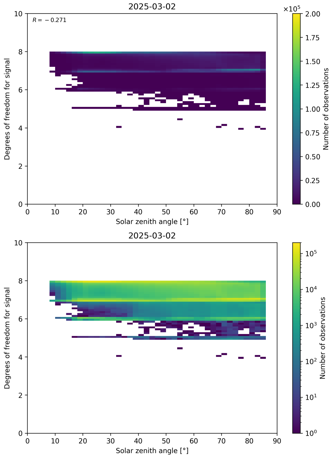
Figure 65: Scatter density plot of “Solar zenith angle” against “Degrees of freedom for signal” for 2025-03-01 to 2025-03-03.
