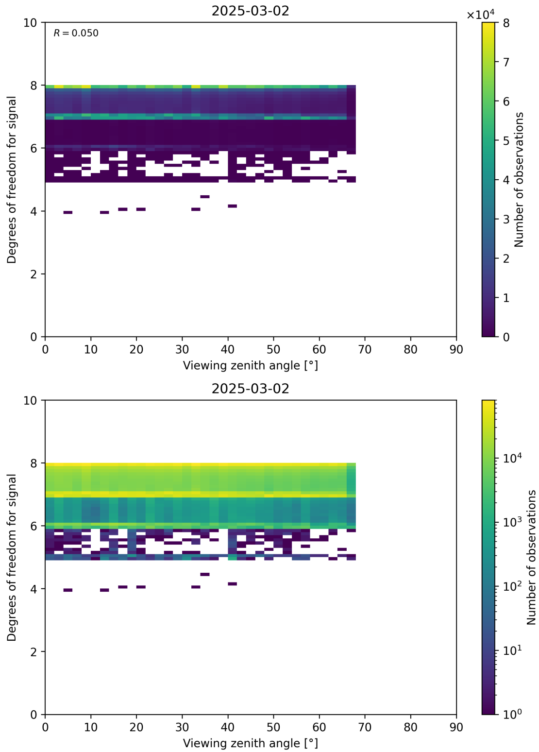
Figure 73: Scatter density plot of “Viewing zenith angle” against “Degrees of freedom for signal” for 2025-03-01 to 2025-03-03.
