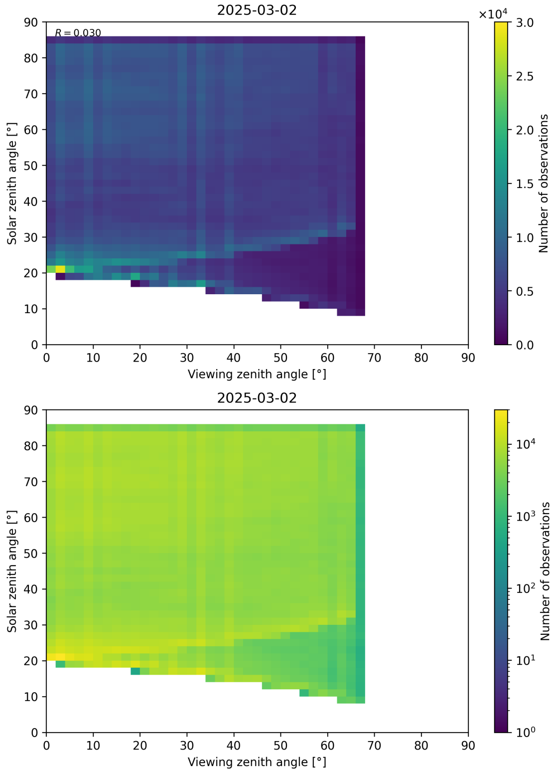
Figure 77: Scatter density plot of “Viewing zenith angle” against “Solar zenith angle” for 2025-03-01 to 2025-03-03.
