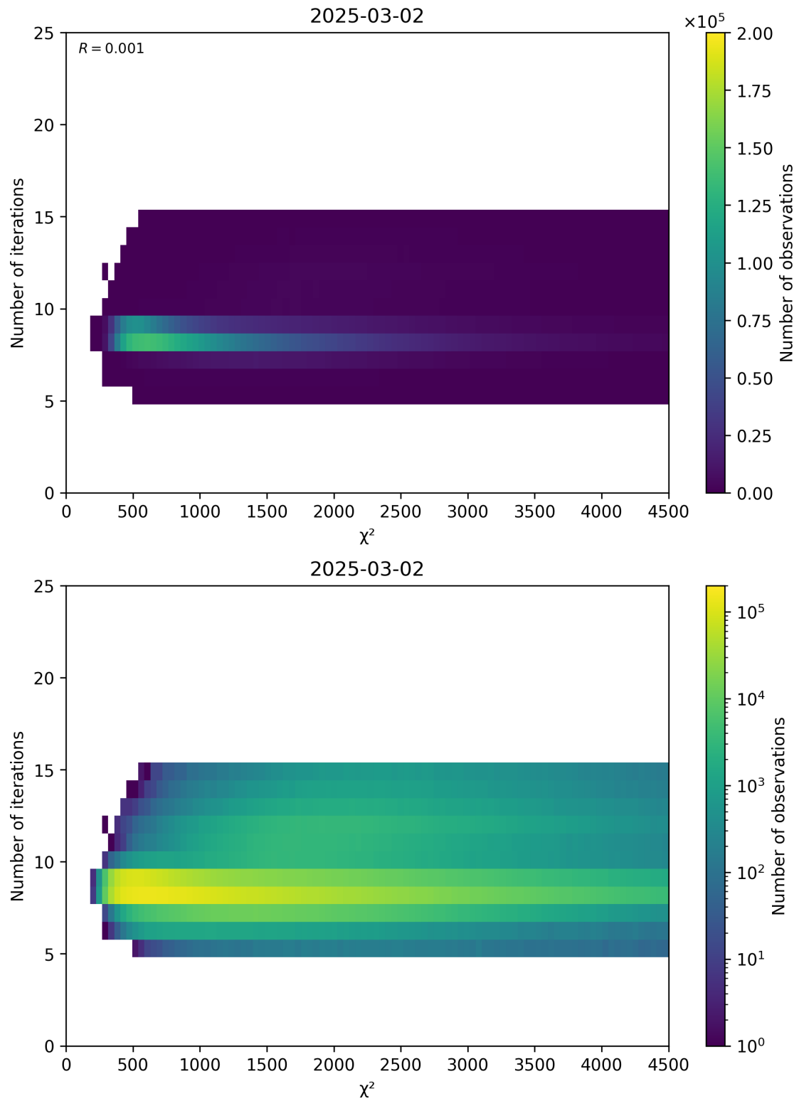
Figure 49: Scatter density plot of “ \chi^2 ” against “Number of iterations” for 2025-03-01 to 2025-03-03.
