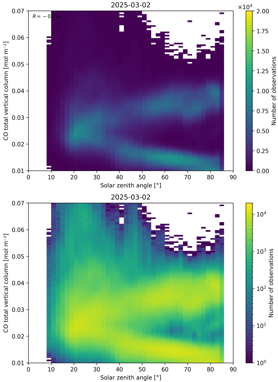
Figure 61: Scatter density plot of “Solar zenith angle” against “CO total vertical column” for 2025-03-01 to 2025-03-03.
