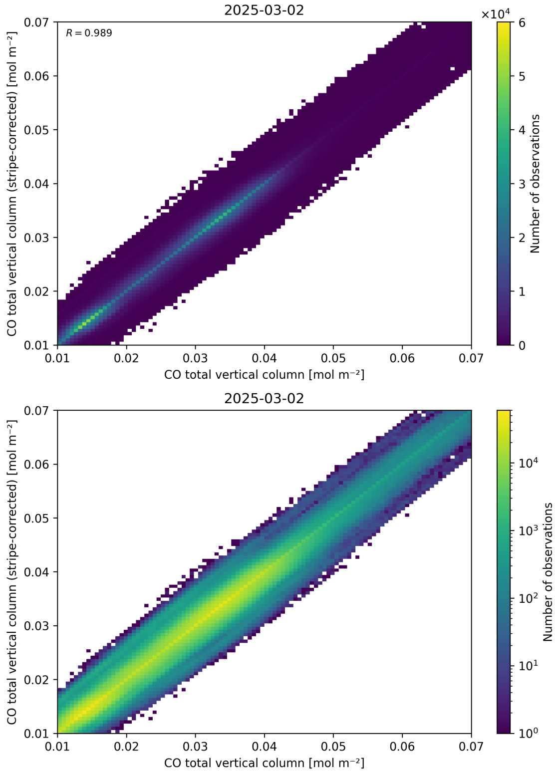
Figure 33: Scatter density plot of “CO total vertical column” against “CO total vertical column (stripe-corrected)” for 2025-03-01 to 2025-03-03.
