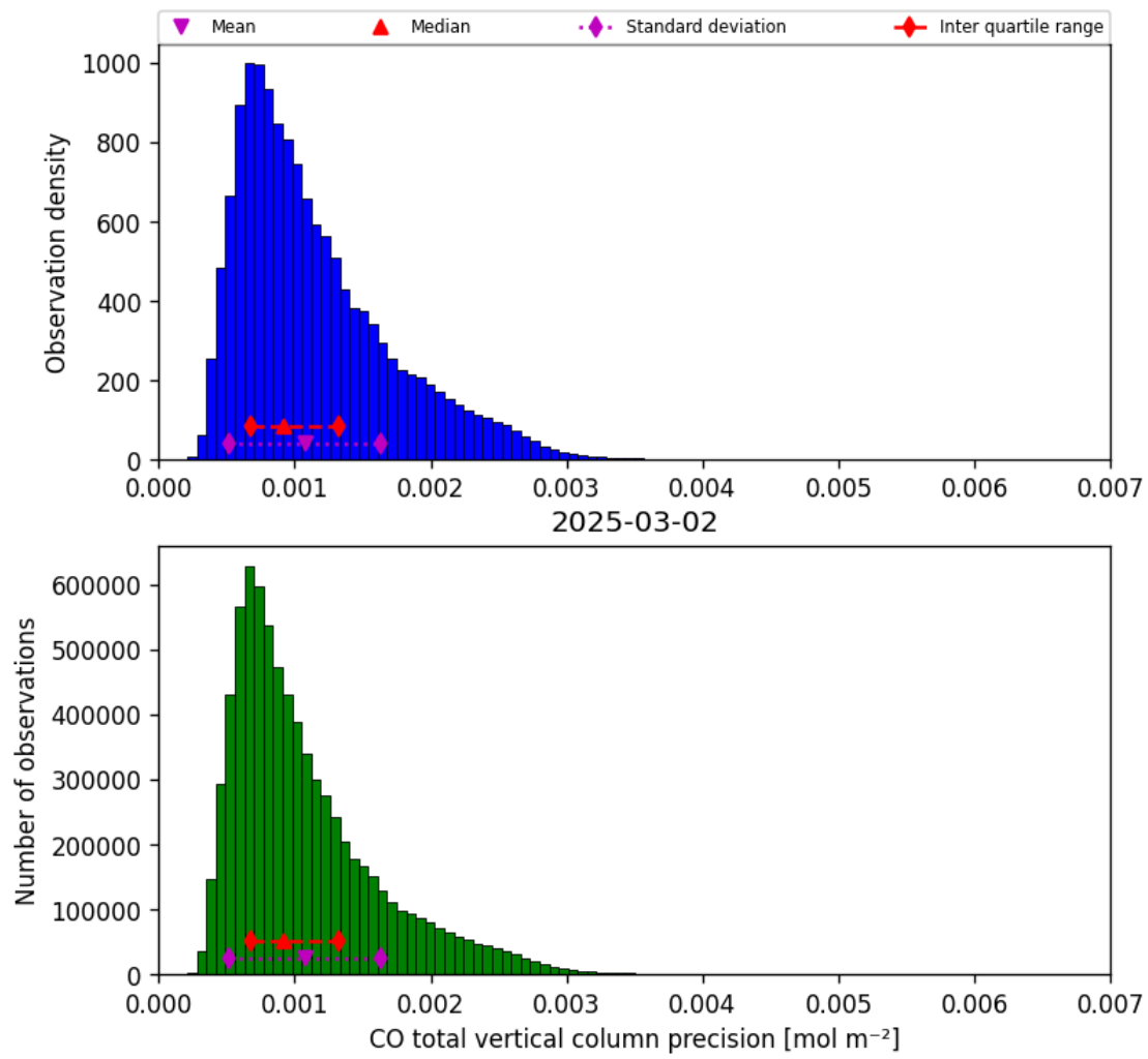
Figure 20: Histogram of “CO total vertical column precision” for 2025-03-01 to 2025-03-03
