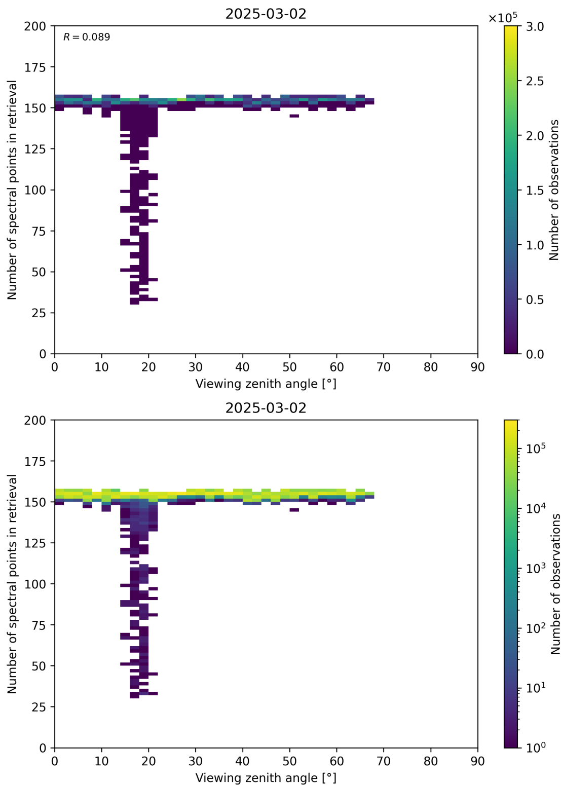
Figure 76: Scatter density plot of “Viewing zenith angle” against “Number of spectral points in retrieval” for 2025-03-01 to 2025-03-03.
