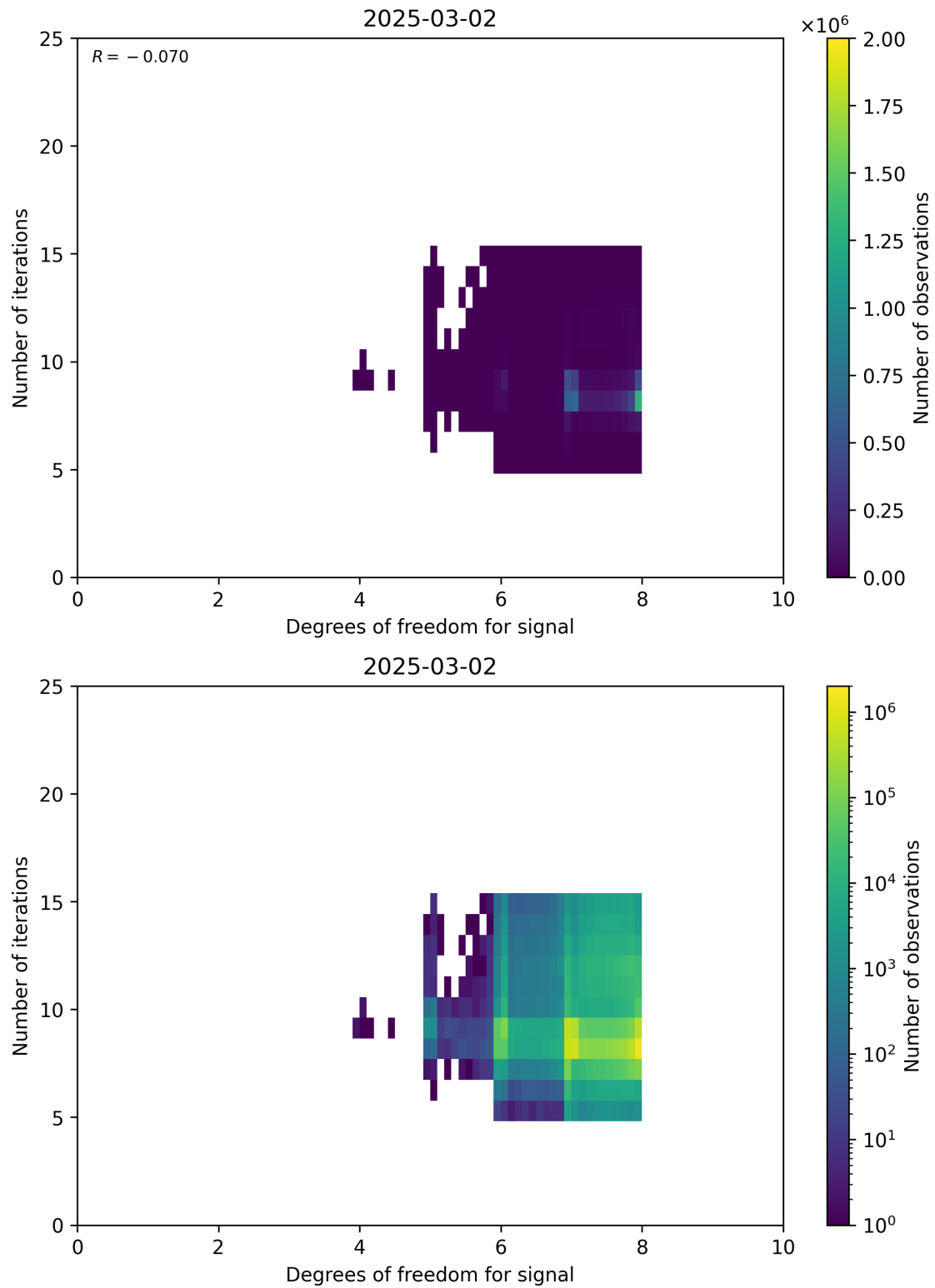
Figure 50: Scatter density plot of “Degrees of freedom for signal” against “Number of iterations” for 2025-03-01 to 2025-03-03.
