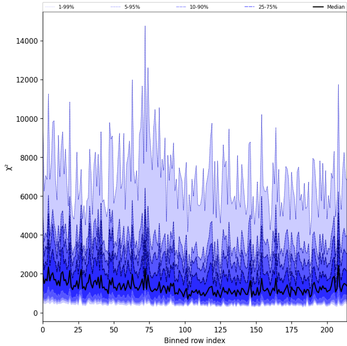
Figure 30: Along track statistics of “ \chi^2 ” for 2025-03-01 to 2025-03-03
