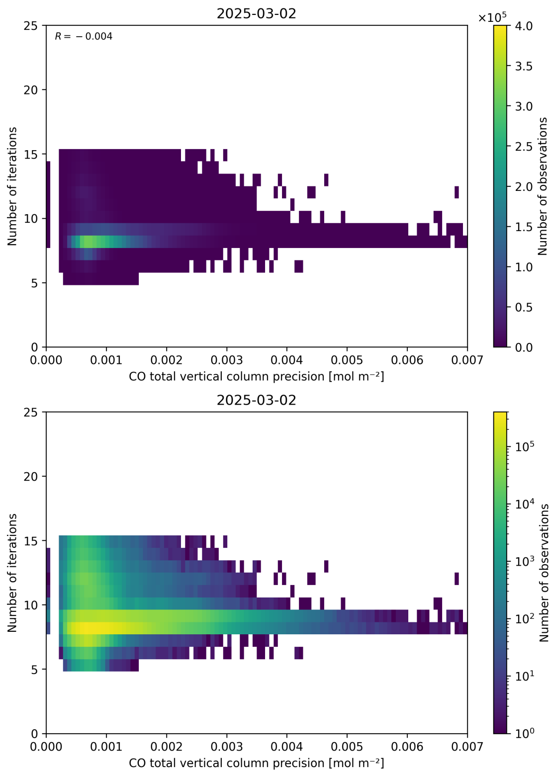
Figure 46: Scatter density plot of “CO total vertical column precision” against “Number of iterations” for 2025-03-01 to 2025-03-03.
