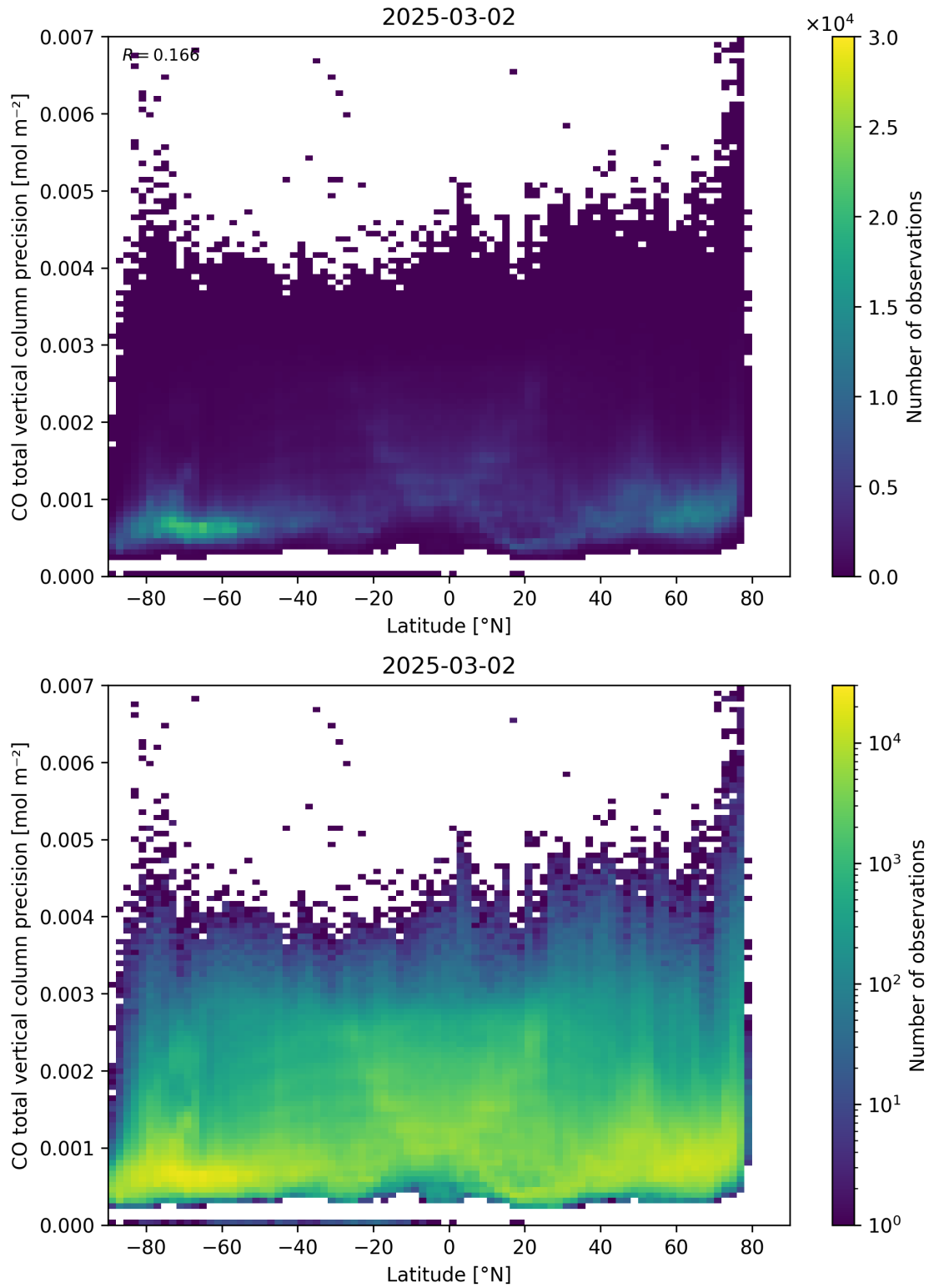
Figure 53: Scatter density plot of “Latitude” against “CO total vertical column precision” for 2025-03-01 to 2025-03-03.
