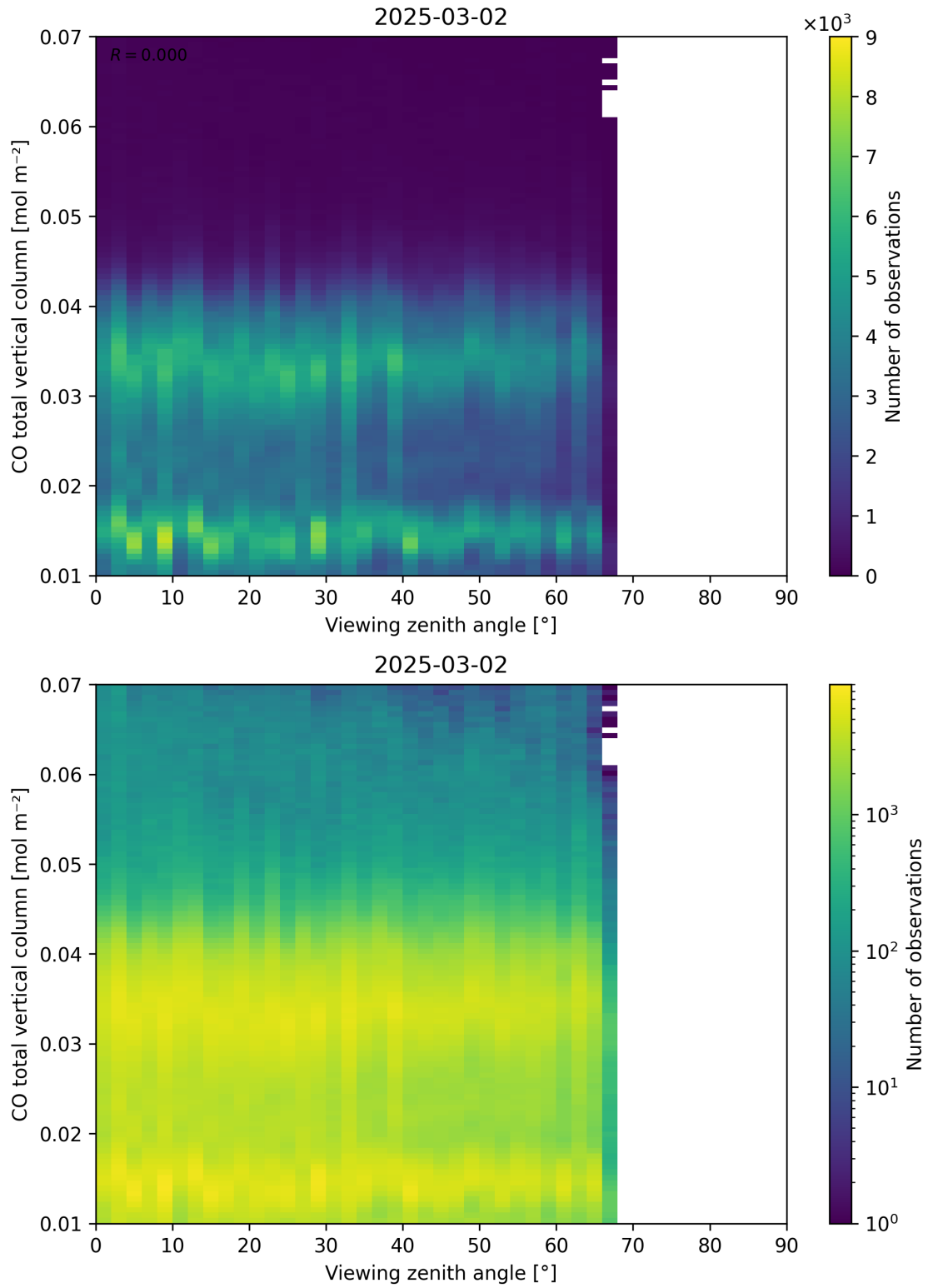
Figure 69: Scatter density plot of “Viewing zenith angle” against “CO total vertical column” for 2025-03-01 to 2025-03-03.
