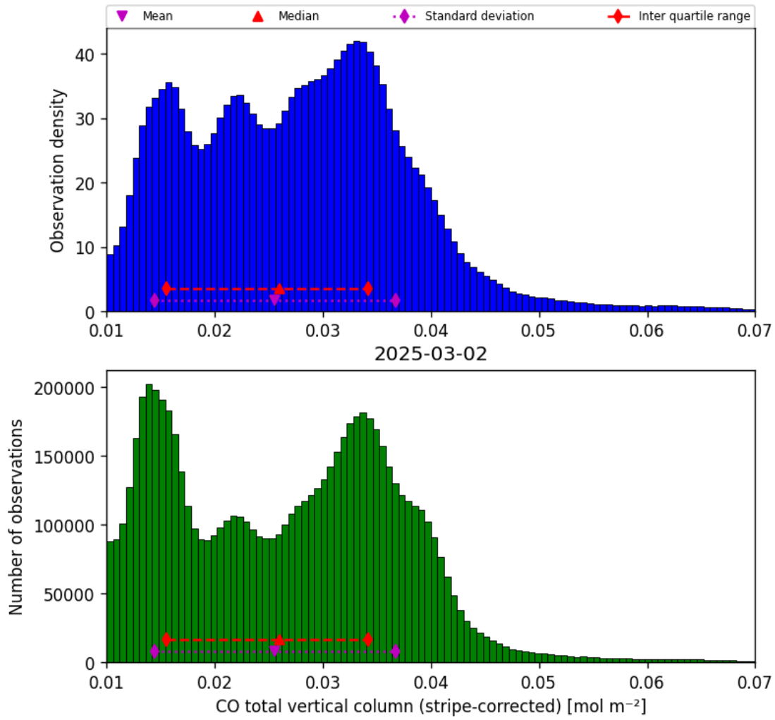
Figure 19: Histogram of “CO total vertical column (stripe-corrected)” for 2025-03-01 to 2025-03-03
