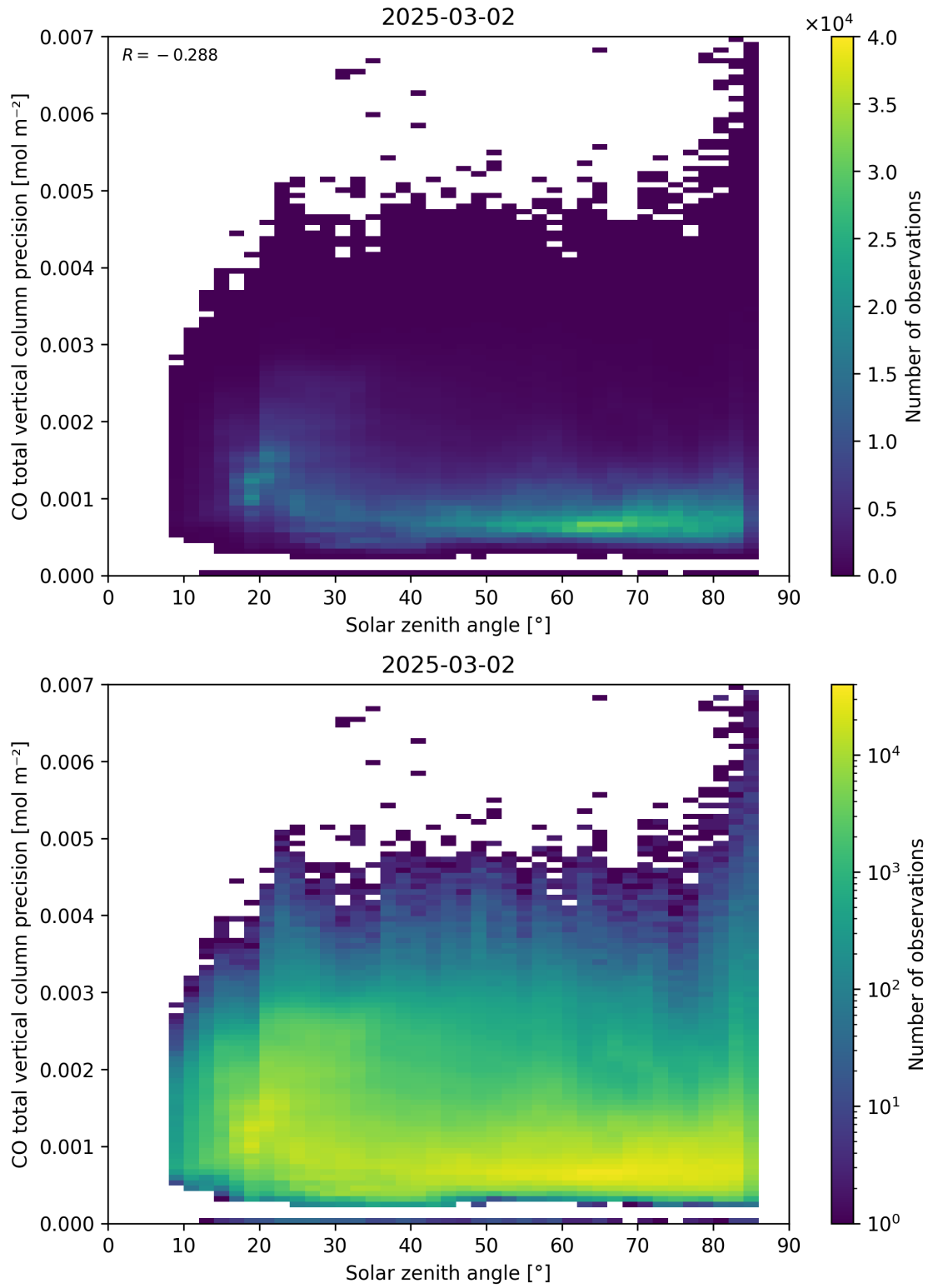
Figure 63: Scatter density plot of “Solar zenith angle” against “CO total vertical column precision” for 2025-03-01 to 2025-03-03.
