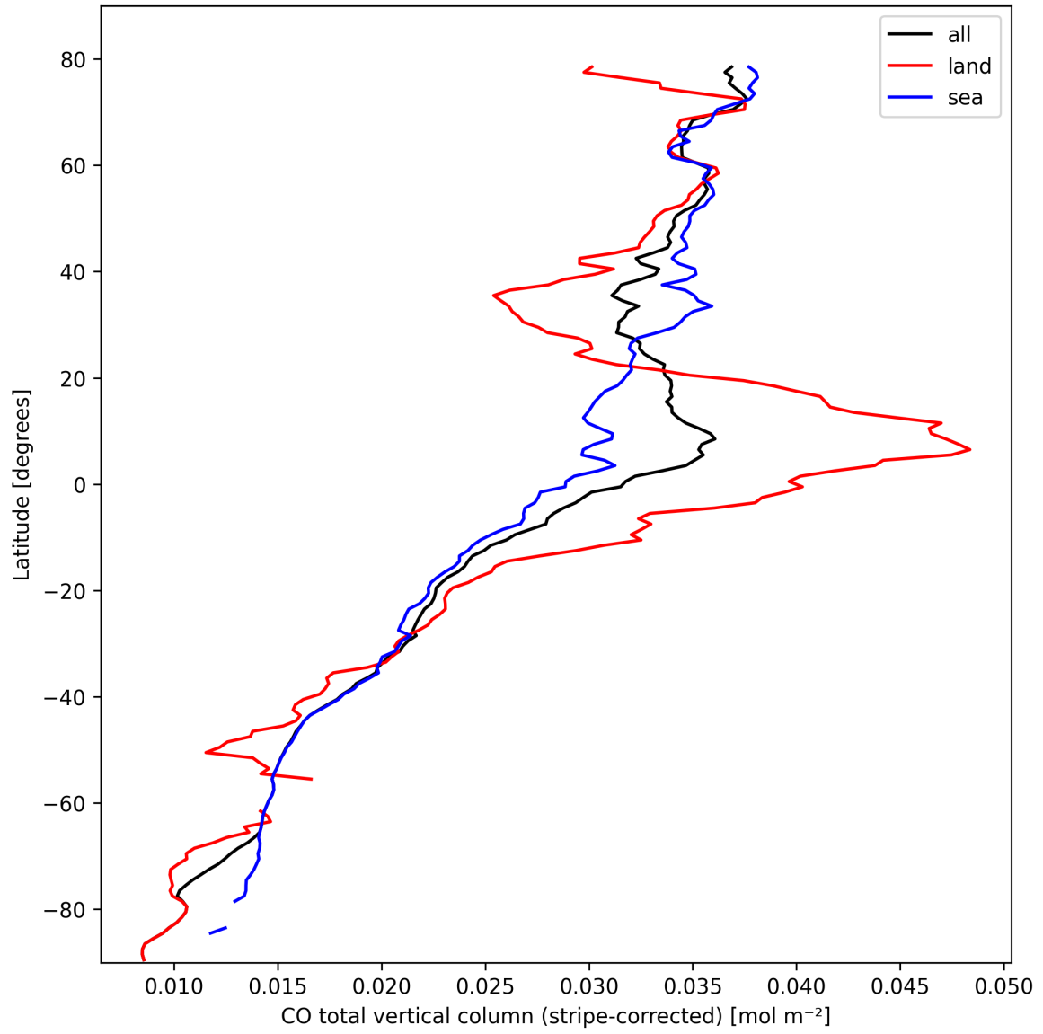
Figure 11: Zonal average of “CO total vertical column (stripe-corrected)” for 2025-03-01 to 2025-03-03.
