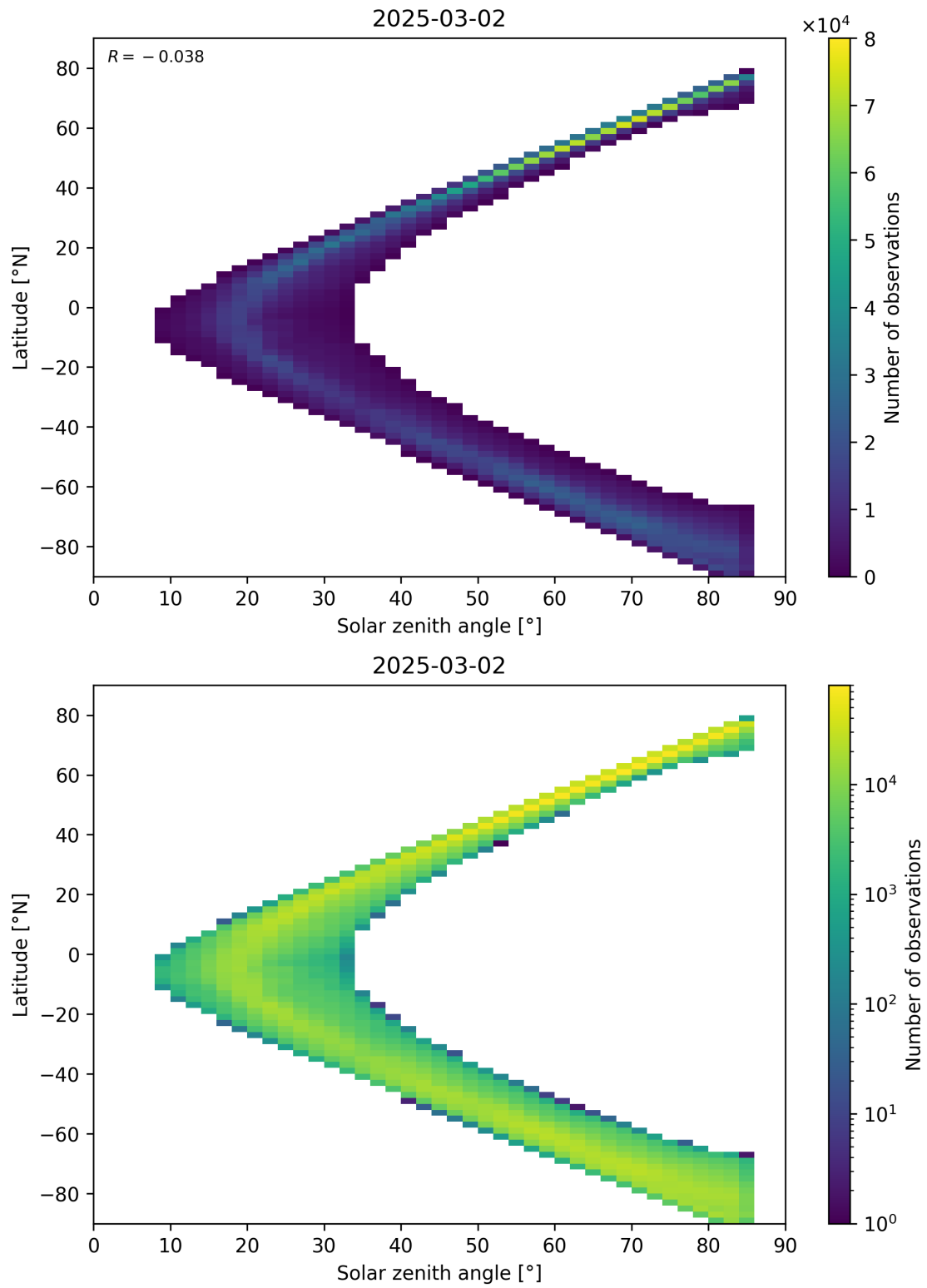
Figure 66: Scatter density plot of “Solar zenith angle” against “Latitude” for 2025-03-01 to 2025-03-03.
