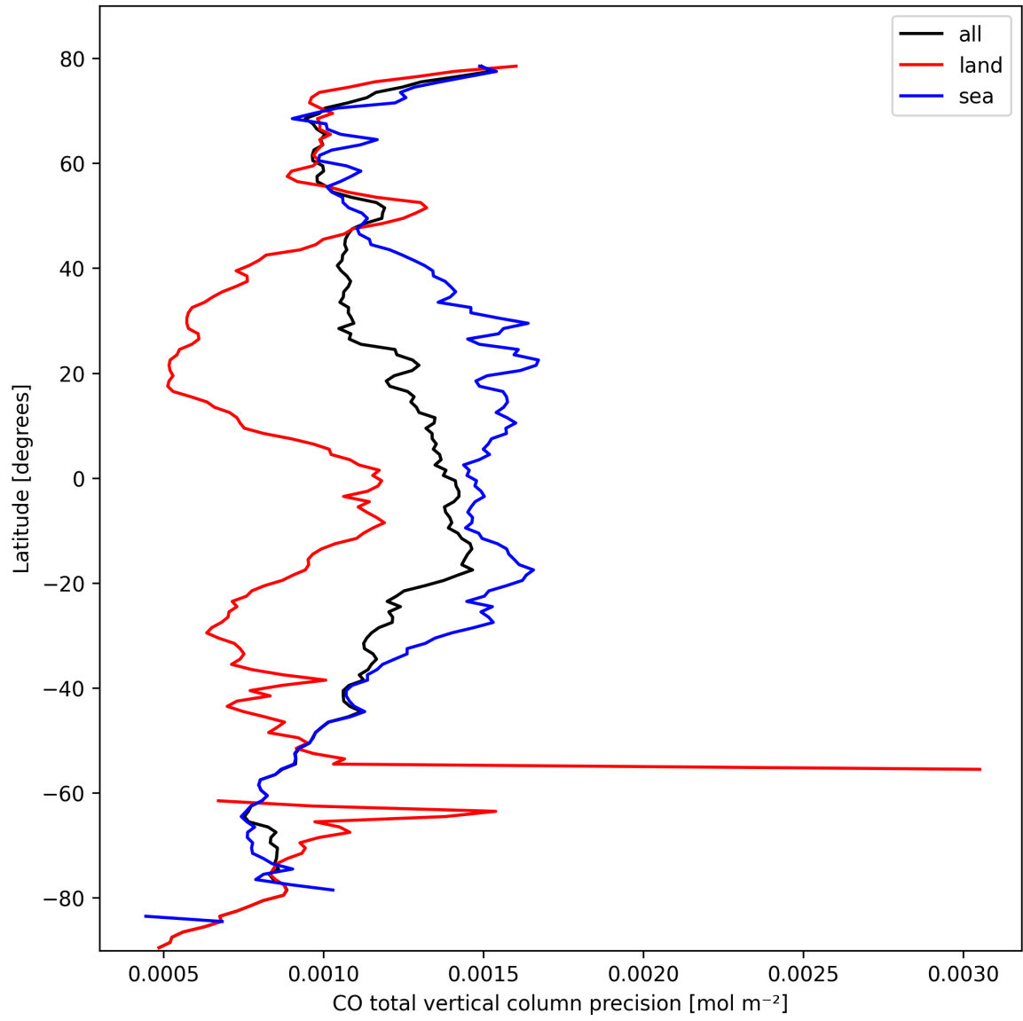
Figure 12: Zonal average of “CO total vertical column precision” for 2025-03-01 to 2025-03-03.
