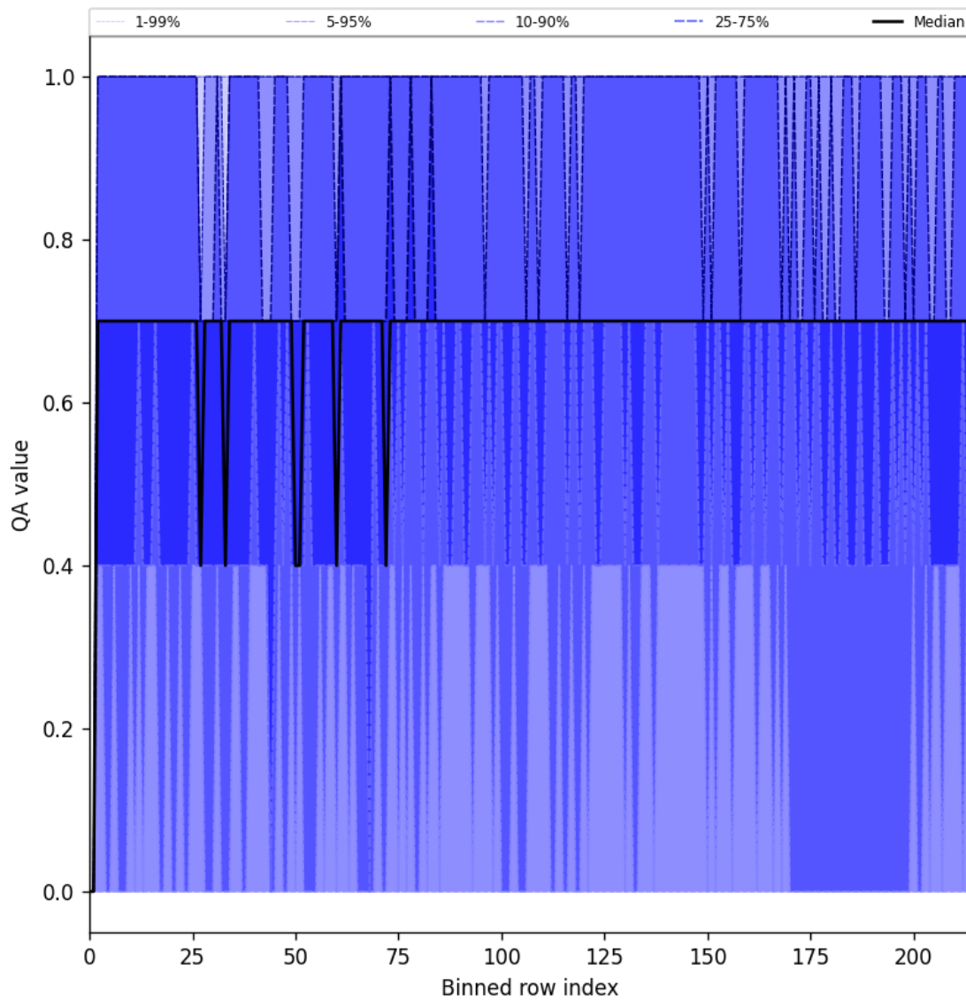
Figure 25: Along track statistics of “QA value” for 2025-03-01 to 2025-03-03
