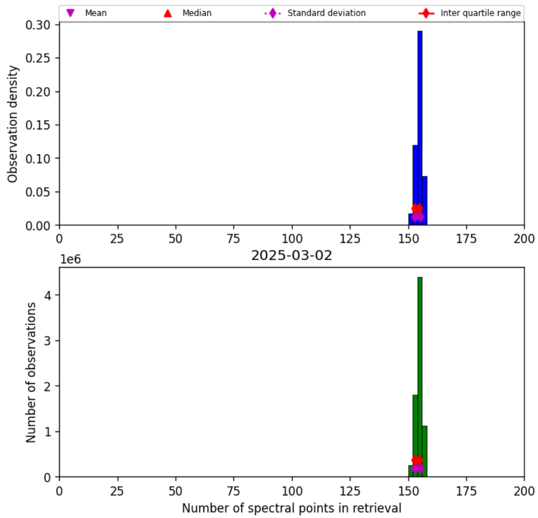
Figure 21: Histogram of “Number of spectral points in retrieval” for 2025-03-01 to 2025-03-03
