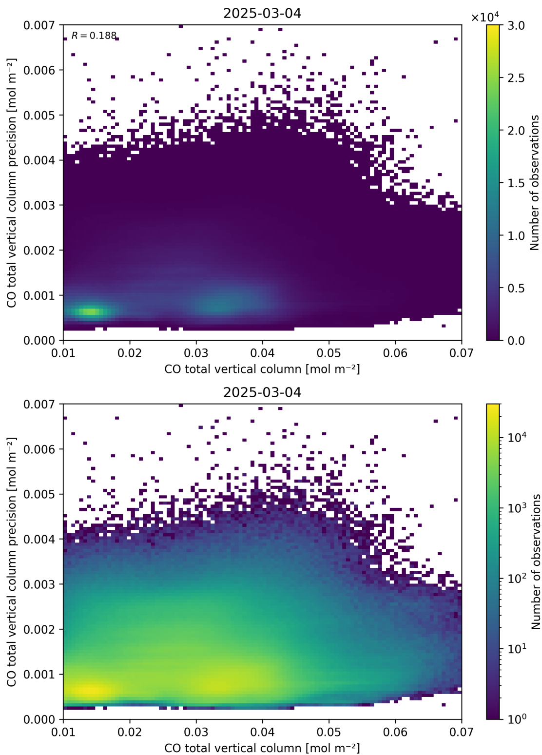
Figure 34: Scatter density plot of “CO total vertical column” against “CO total vertical column precision” for 2025-03-03 to 2025-03-05.
