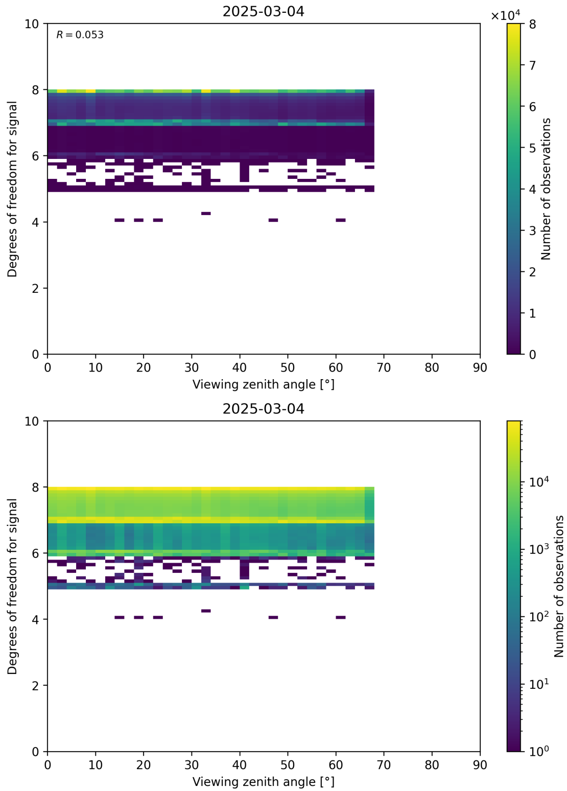
Figure 73: Scatter density plot of “Viewing zenith angle” against “Degrees of freedom for signal” for 2025-03-03 to 2025-03-05.
