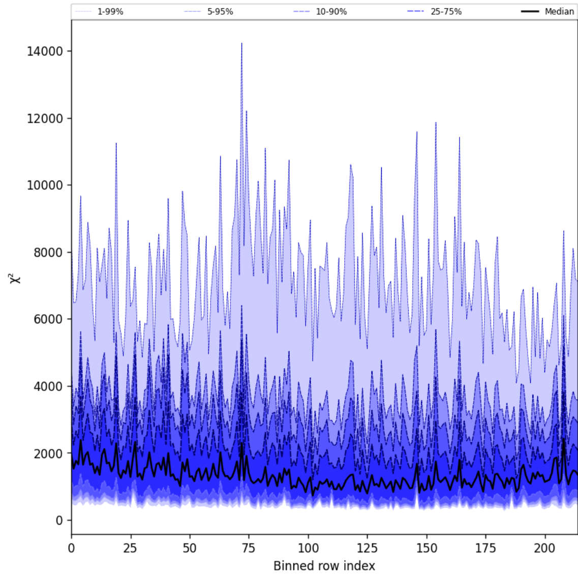
Figure 30: Along track statistics of “ \chi^2 ” for 2025-03-03 to 2025-03-05
