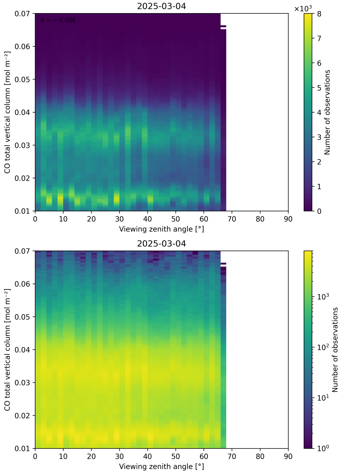
Figure 69: Scatter density plot of “Viewing zenith angle” against “CO total vertical column” for 2025-03-03 to 2025-03-05.
