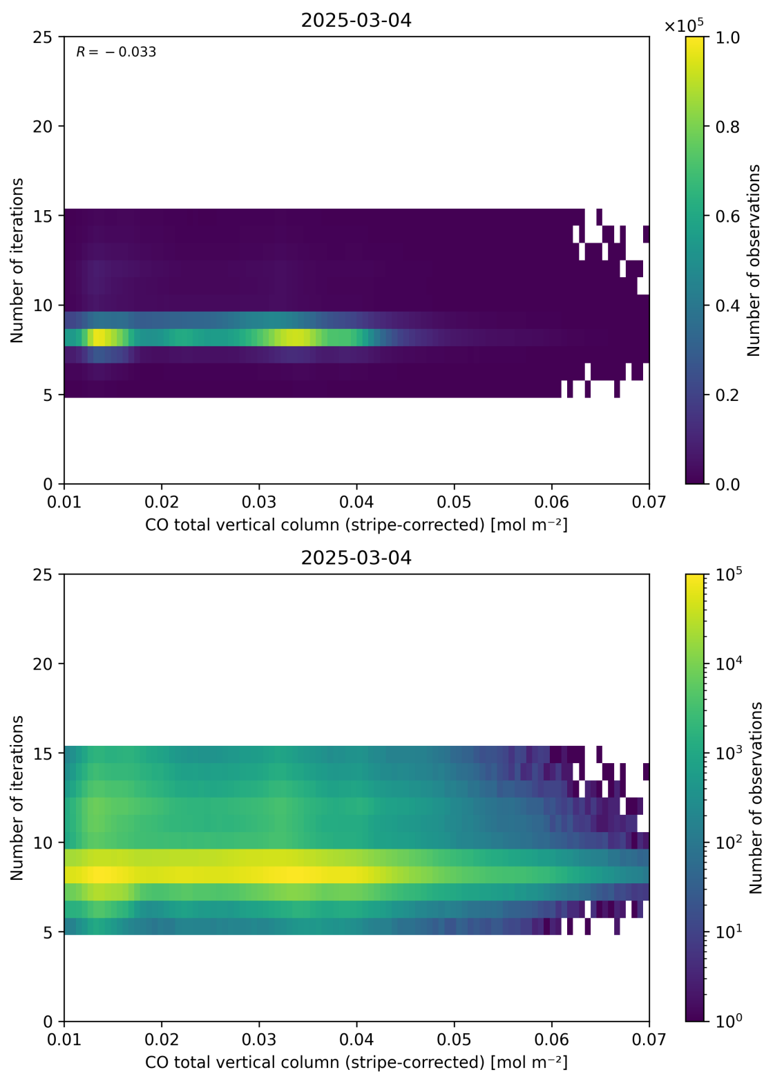
Figure 39: Scatter density plot of “CO total vertical column (stripe-corrected)” against “Number of iterations” for 2025-03-03 to 2025-03-05.
