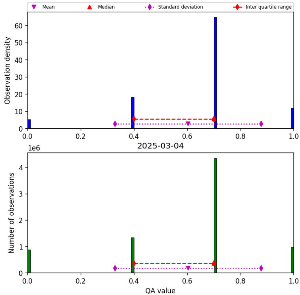
Figure 17: Histogram of “QA value” for 2025-03-03 to 2025-03-05
