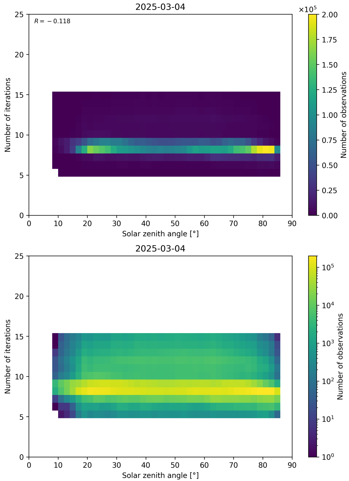
Figure 67: Scatter density plot of “Solar zenith angle” against “Number of iterations” for 2025-03-03 to 2025-03-05.
