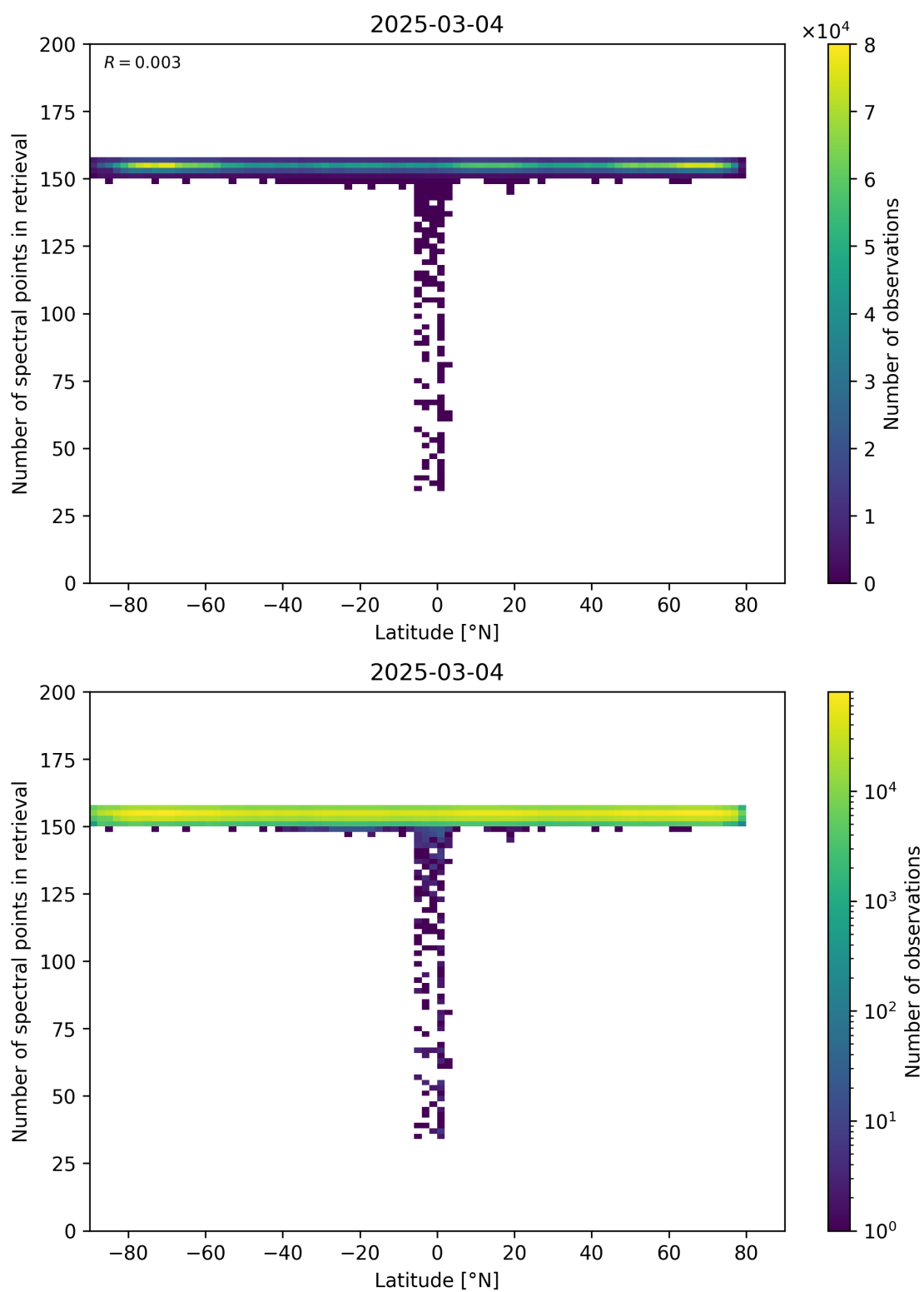
Figure 57: Scatter density plot of “Latitude” against “Number of spectral points in retrieval” for 2025-03-03 to 2025-03-05.
