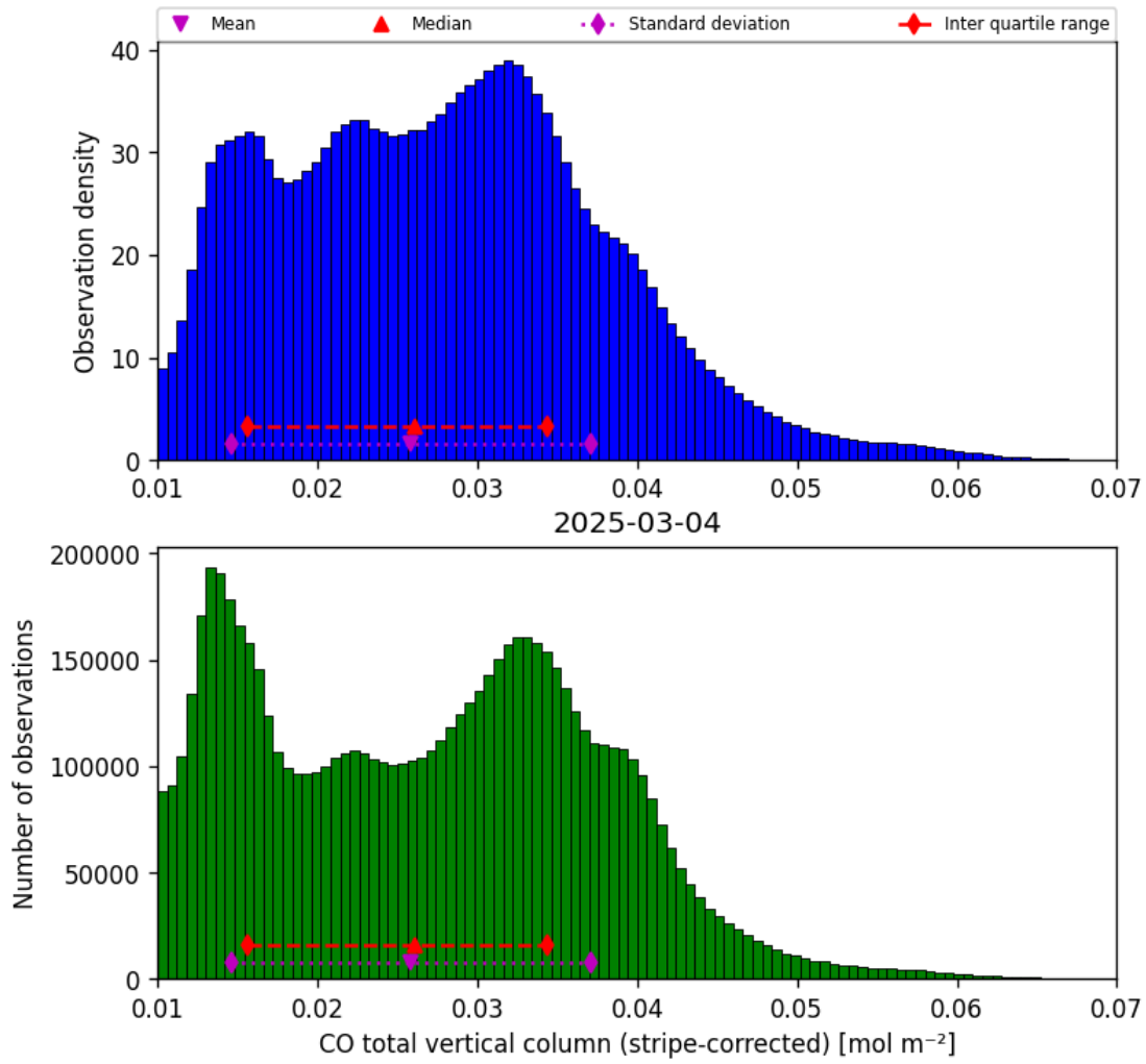
Figure 19: Histogram of “CO total vertical column (stripe-corrected)” for 2025-03-03 to 2025-03-05
