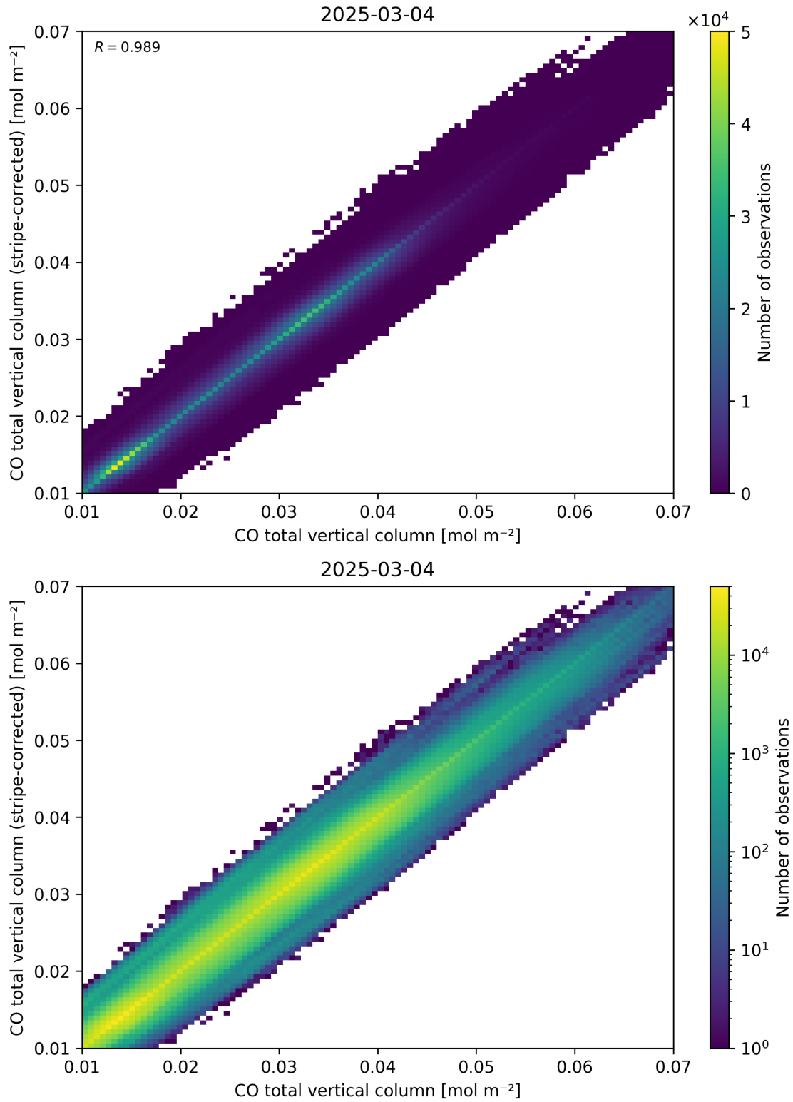
Figure 33: Scatter density plot of “CO total vertical column” against “CO total vertical column (stripe-corrected)” for 2025-03-03 to 2025-03-05.
