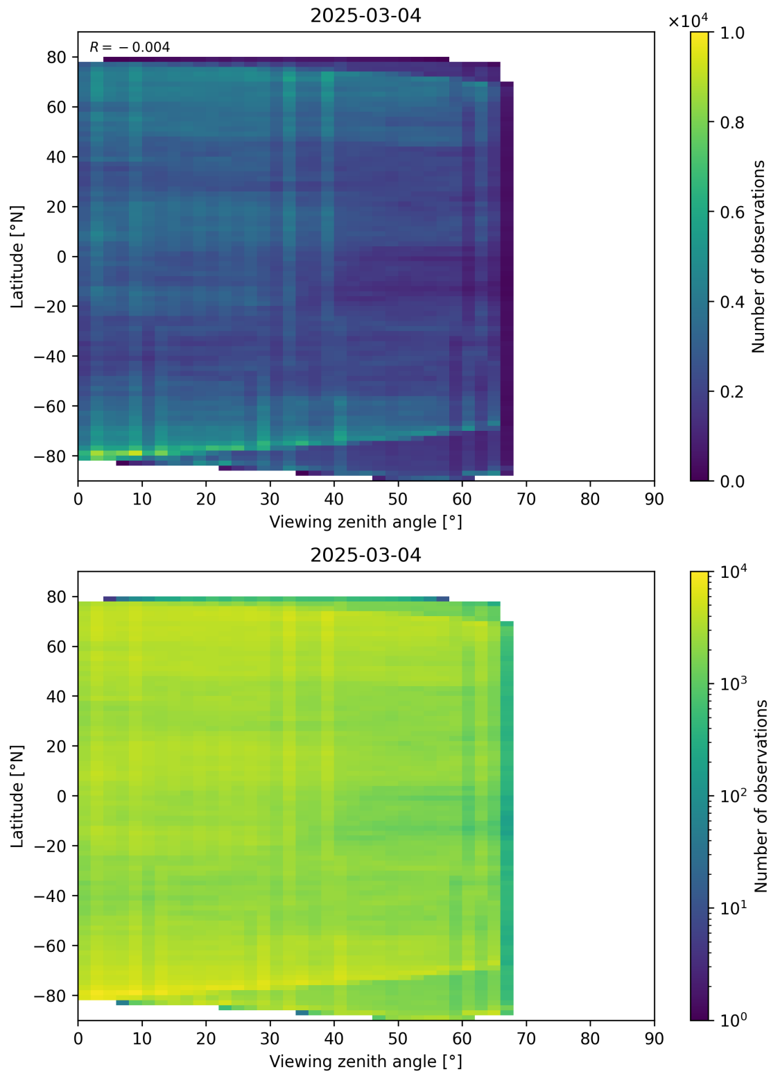
Figure 74: Scatter density plot of “Viewing zenith angle” against “Latitude” for 2025-03-03 to 2025-03-05.
