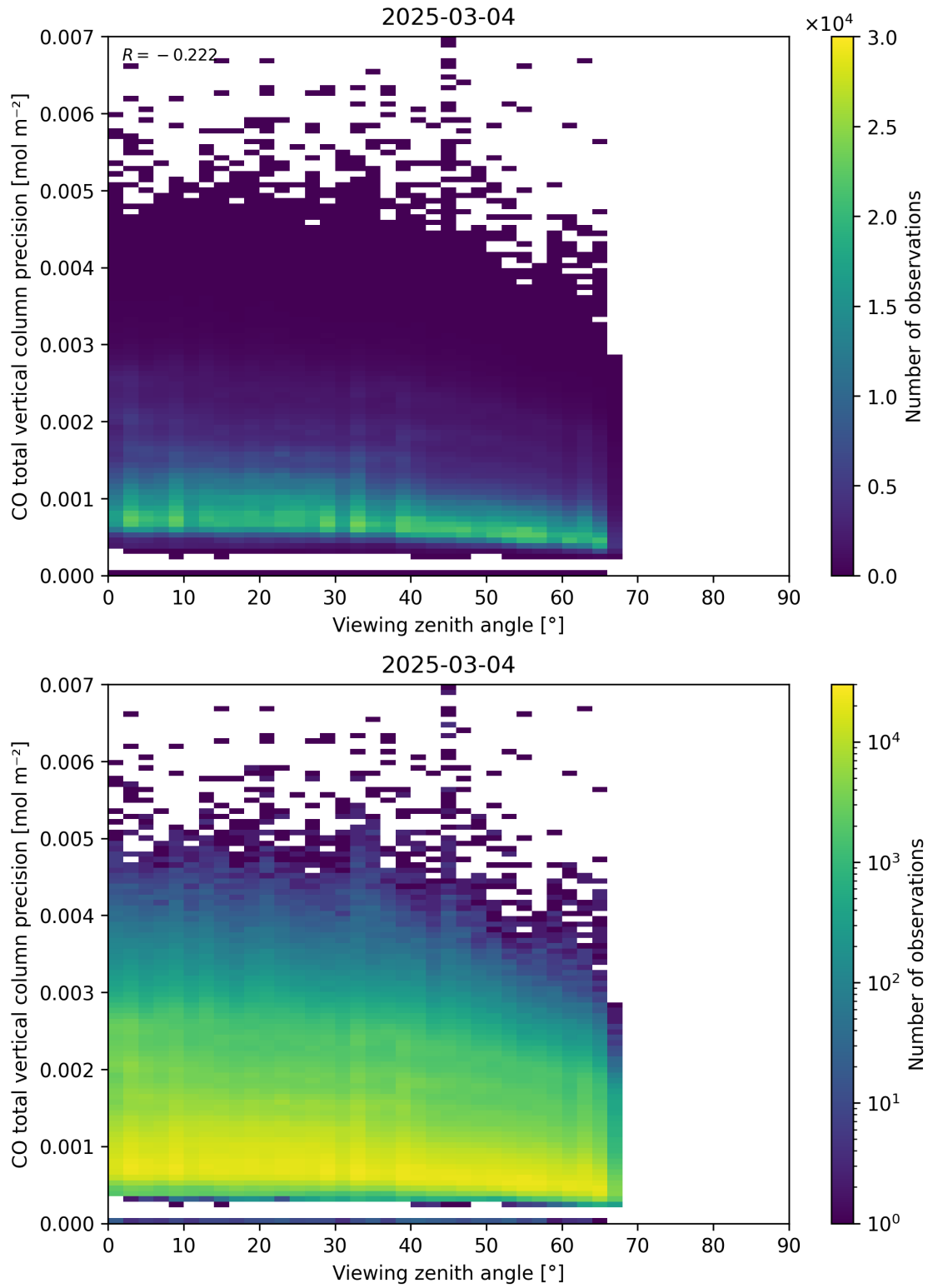
Figure 71: Scatter density plot of “Viewing zenith angle” against “CO total vertical column precision” for 2025-03-03 to 2025-03-05.
