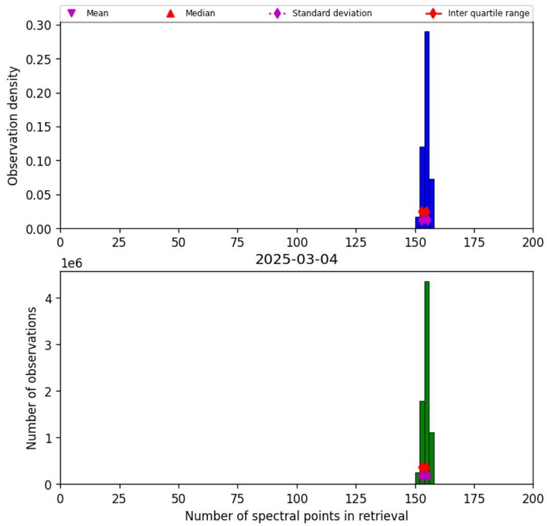
Figure 21: Histogram of “Number of spectral points in retrieval” for 2025-03-03 to 2025-03-05
