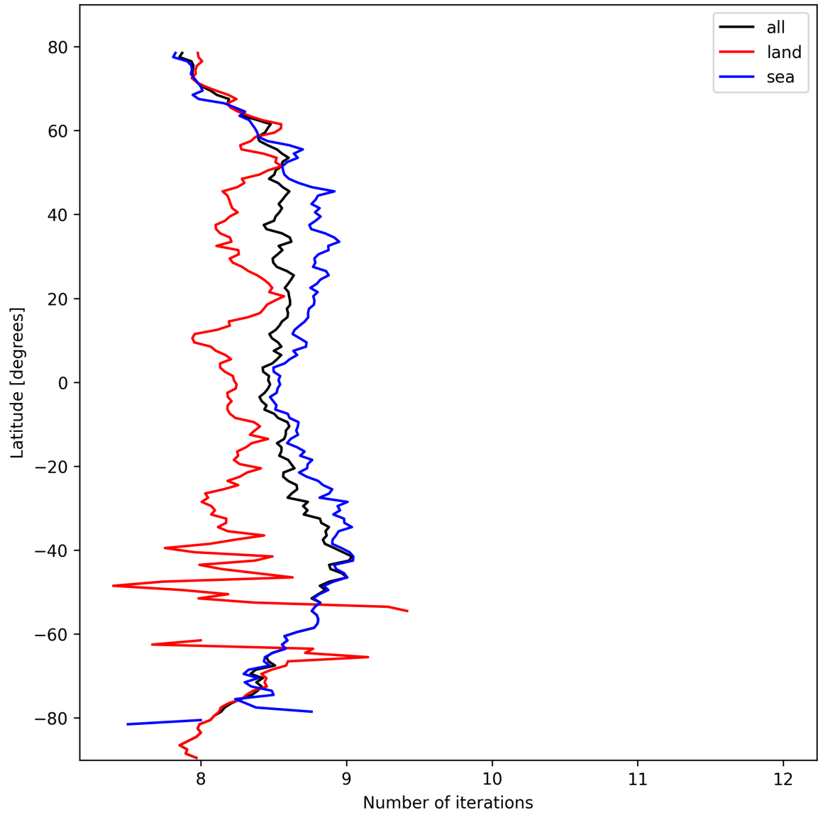
Figure 16: Zonal average of “Number of iterations” for 2025-03-03 to 2025-03-05.
