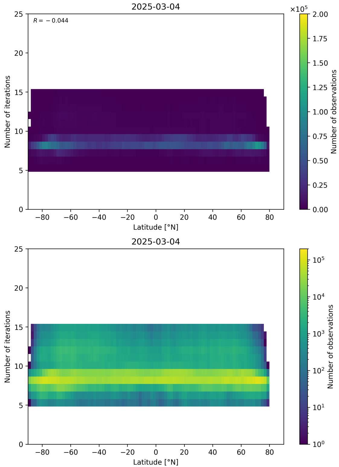
Figure 56: Scatter density plot of “Latitude” against “Number of iterations” for 2025-03-03 to 2025-03-05.
