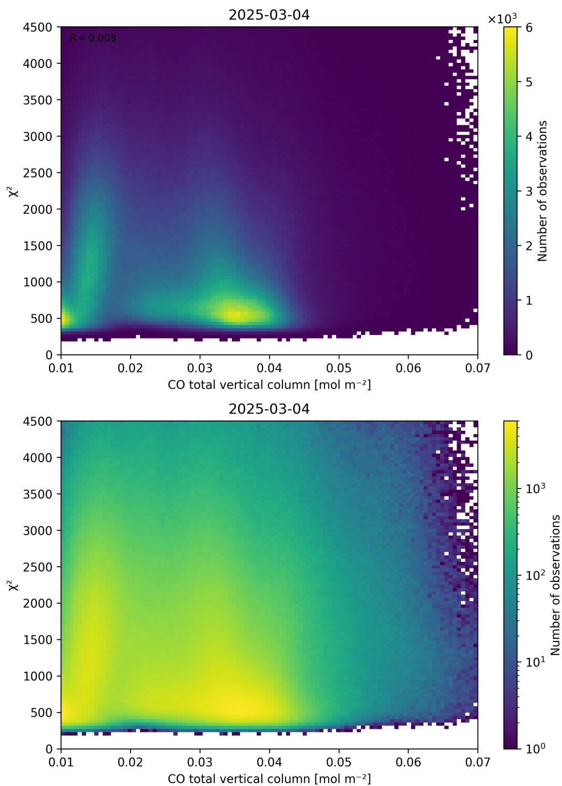
Figure 35: Scatter density plot of “CO total vertical column” against “ \chi^2 ” for 2025-03-03 to 2025-03-05.
