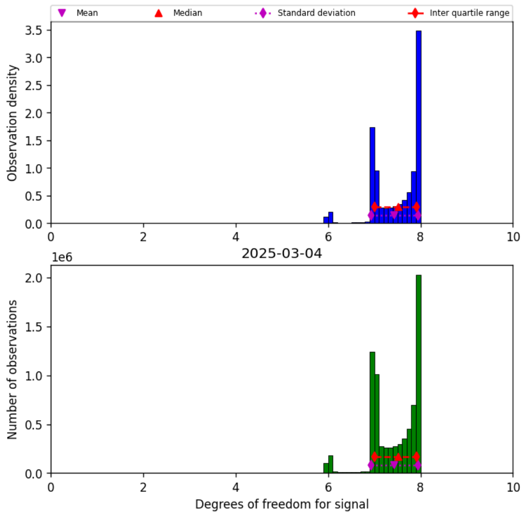
Figure 23: Histogram of “Degrees of freedom for signal” for 2025-03-03 to 2025-03-05
