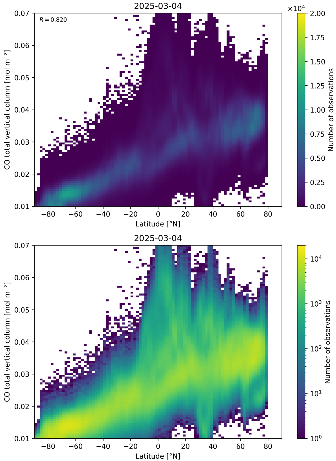
Figure 51: Scatter density plot of “Latitude” against “CO total vertical column” for 2025-03-03 to 2025-03-05.
