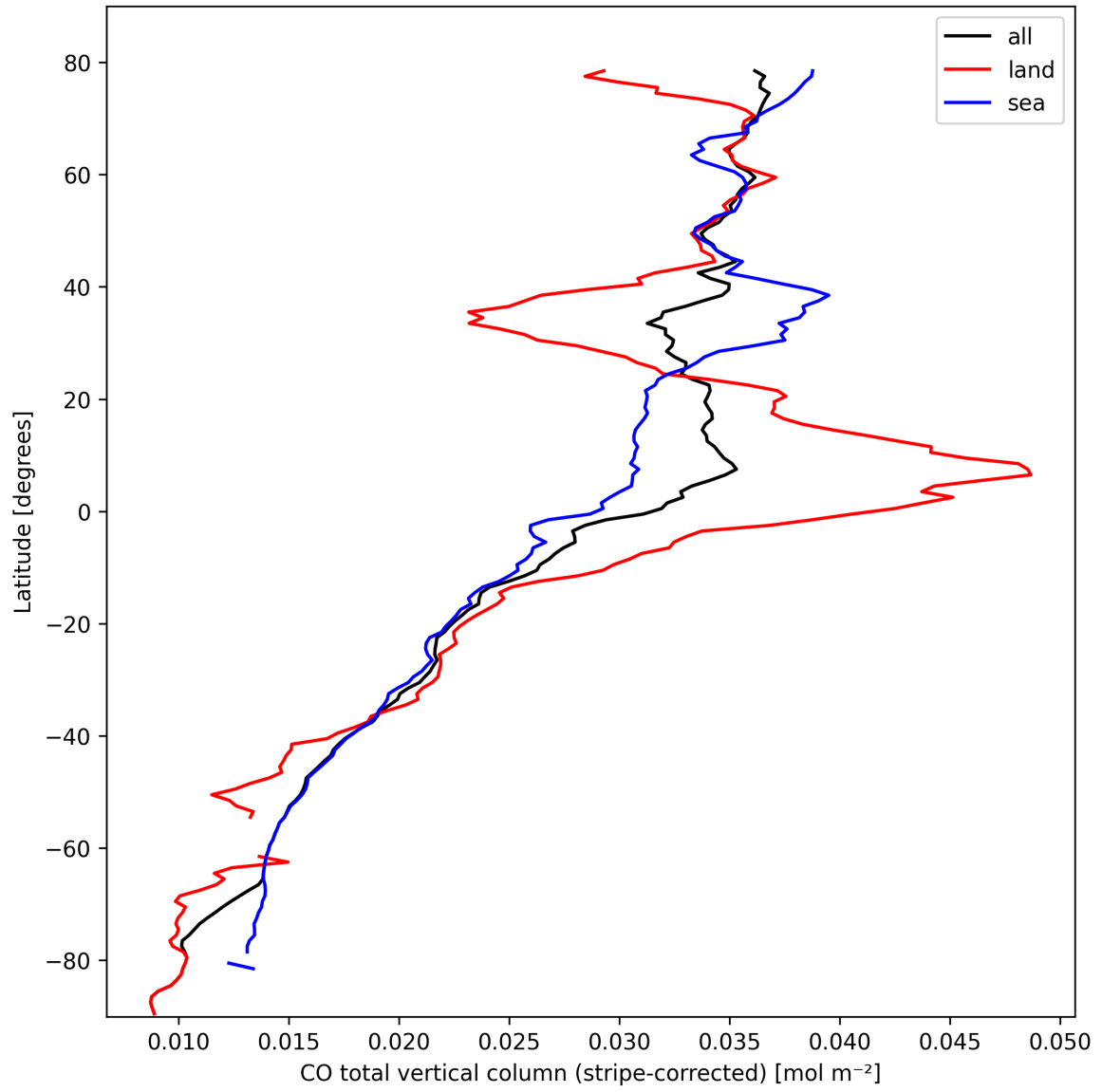
Figure 11: Zonal average of “CO total vertical column (stripe-corrected)” for 2025-03-03 to 2025-03-05.
