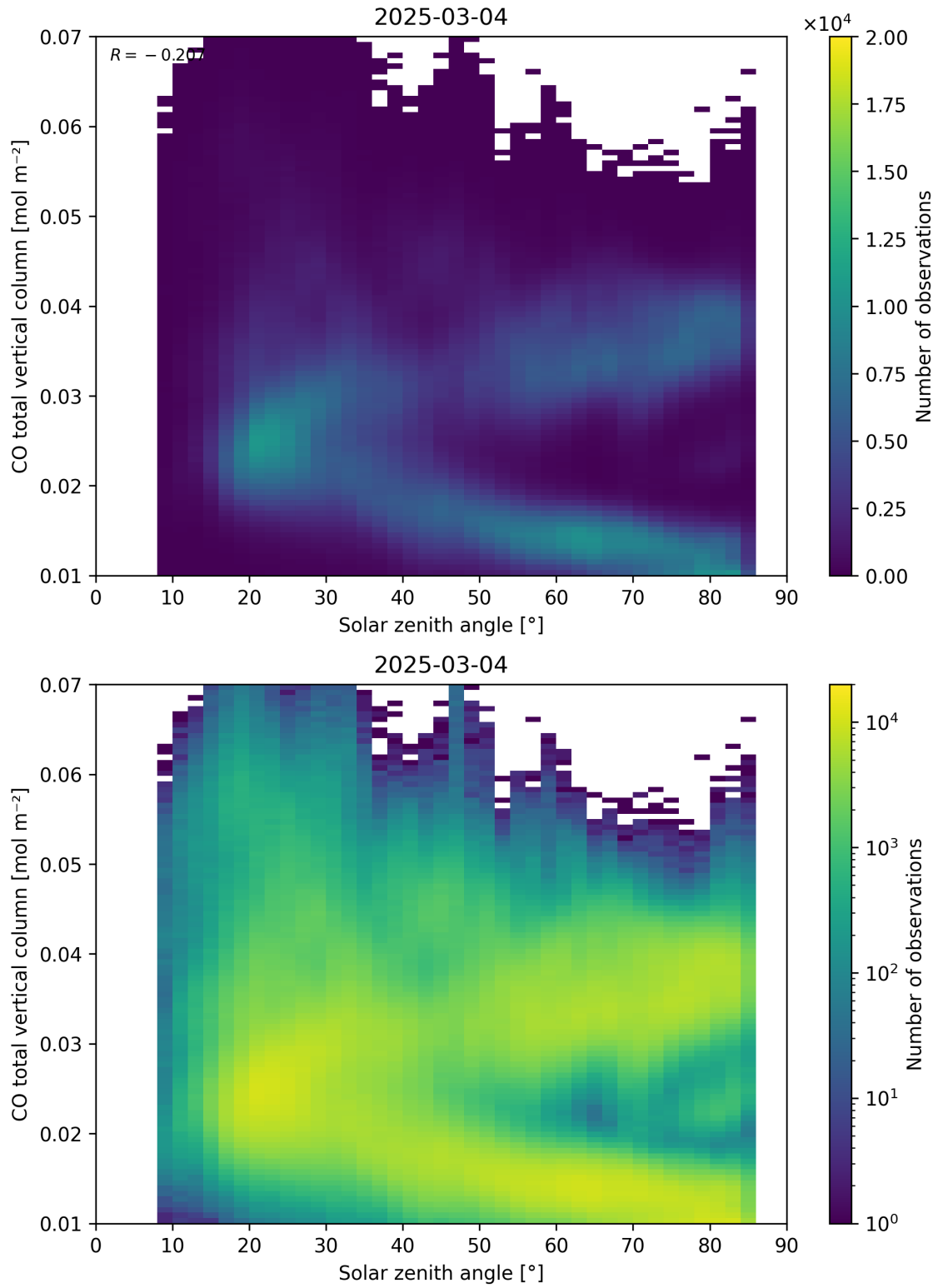
Figure 61: Scatter density plot of “Solar zenith angle” against “CO total vertical column” for 2025-03-03 to 2025-03-05.
