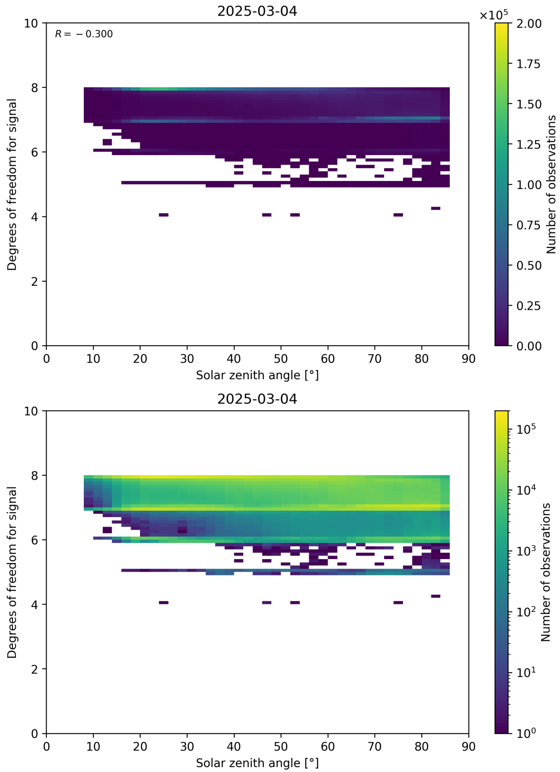
Figure 65: Scatter density plot of “Solar zenith angle” against “Degrees of freedom for signal” for 2025-03-03 to 2025-03-05.
