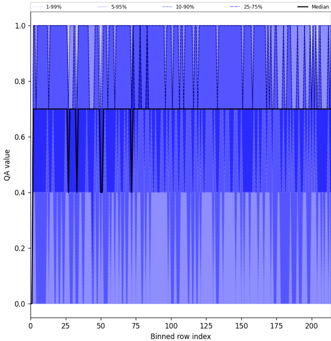
Figure 25: Along track statistics of “QA value” for 2025-03-03 to 2025-03-05
