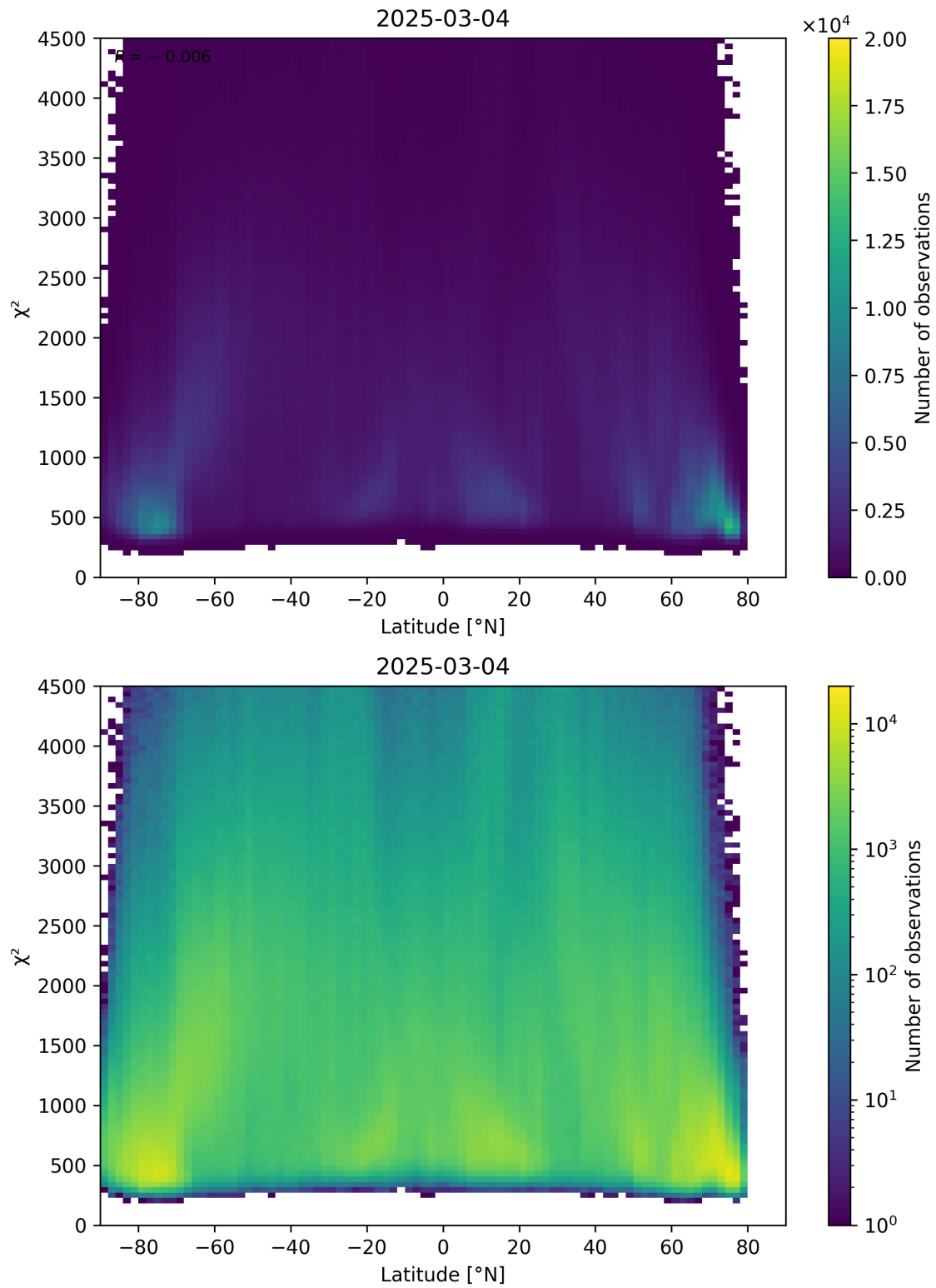
Figure 54: Scatter density plot of “Latitude” against “ \chi^2 ” for 2025-03-03 to 2025-03-05.
