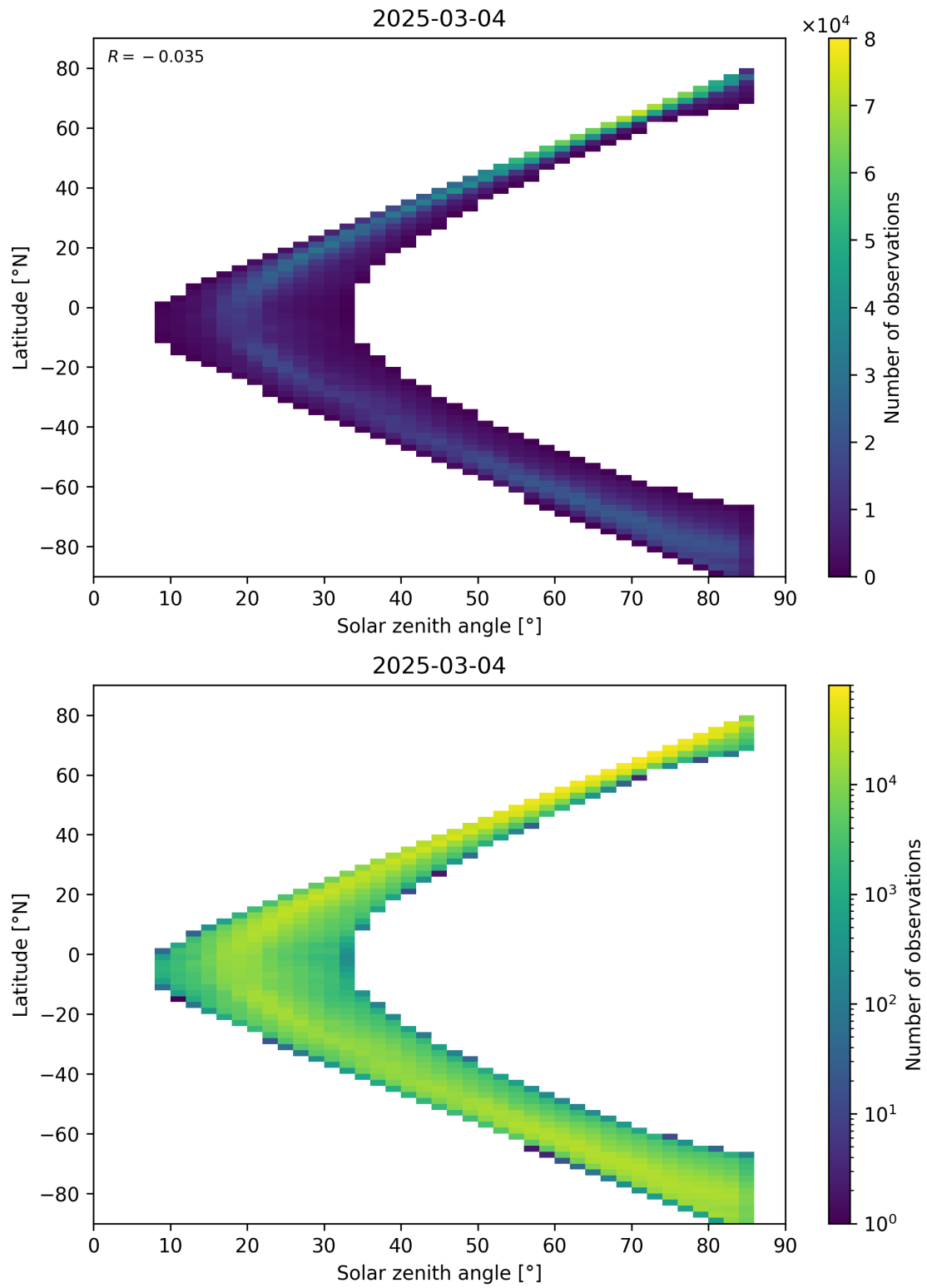
Figure 66: Scatter density plot of “Solar zenith angle” against “Latitude” for 2025-03-03 to 2025-03-05.
