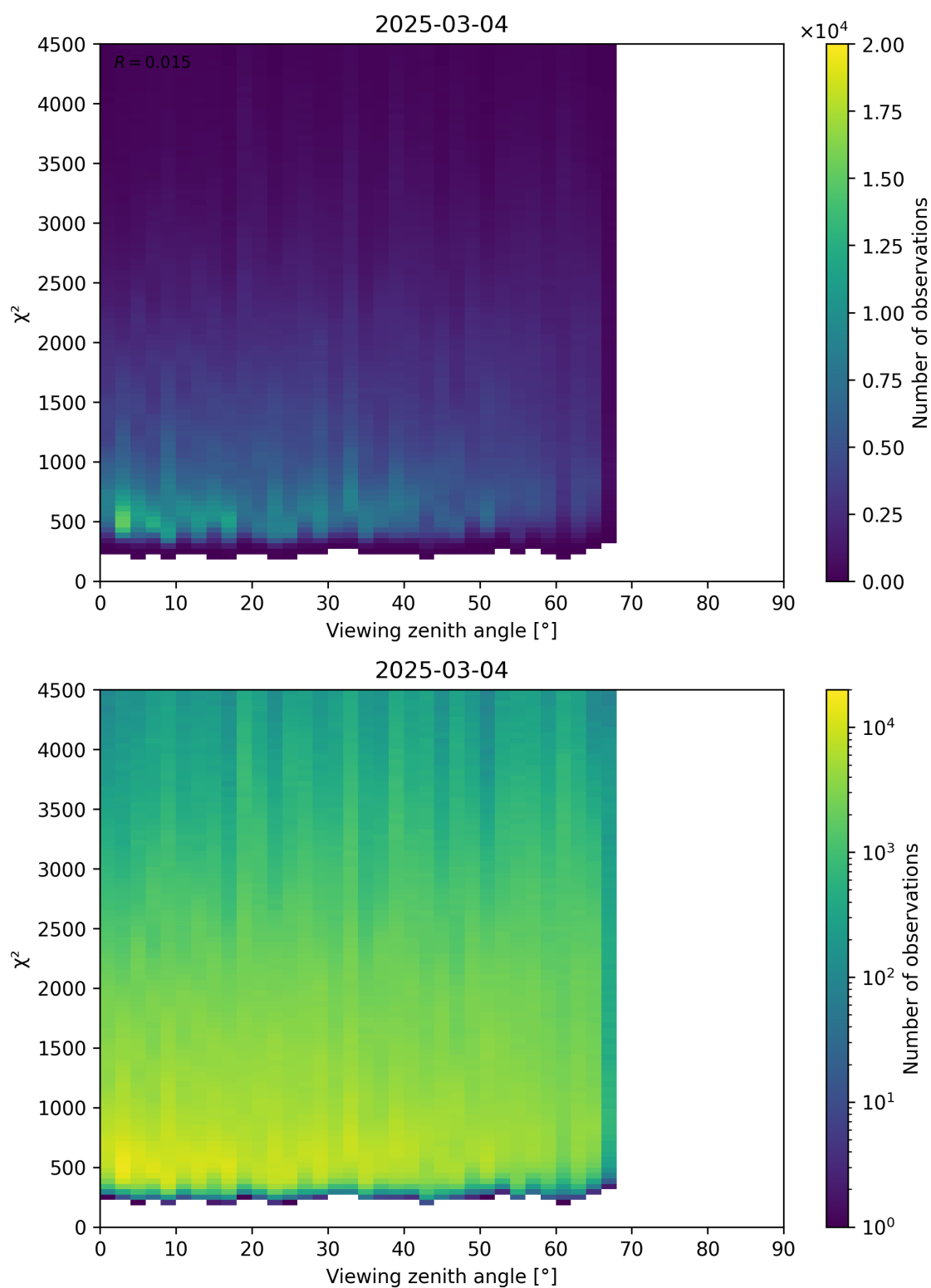
Figure 72: Scatter density plot of “Viewing zenith angle” against “ \chi^2 ” for 2025-03-03 to 2025-03-05.
