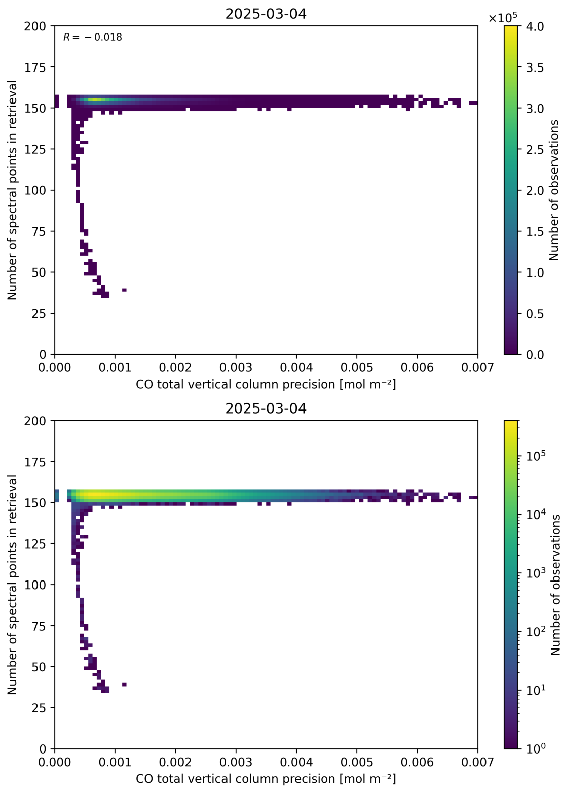
Figure 47: Scatter density plot of “CO total vertical column precision” against “Number of spectral points in retrieval” for 2025-03-03 to 2025-03-05.
