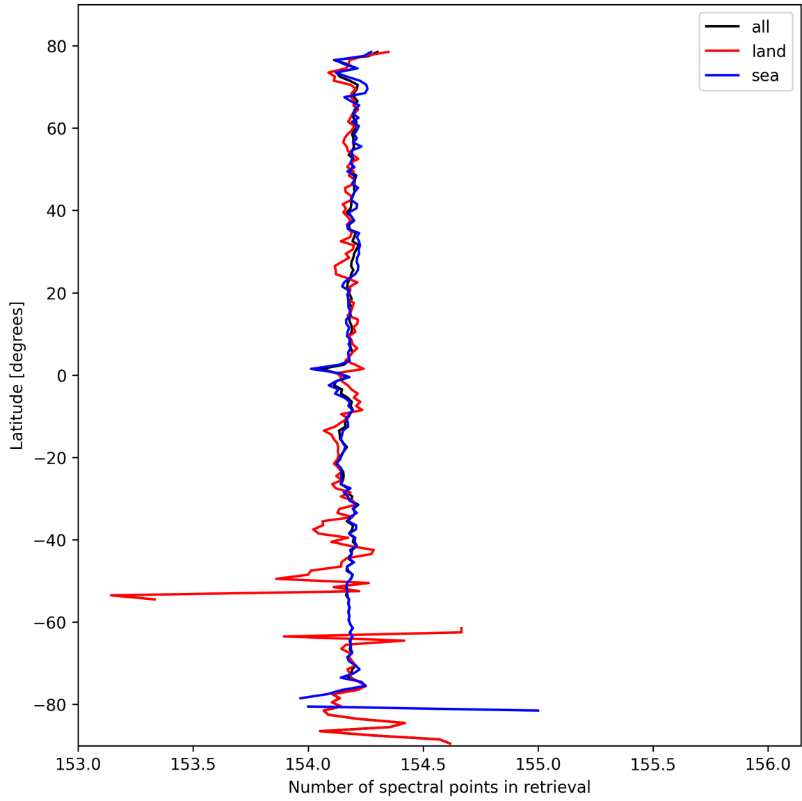
Figure 13: Zonal average of “Number of spectral points in retrieval” for 2025-03-03 to 2025-03-05.
