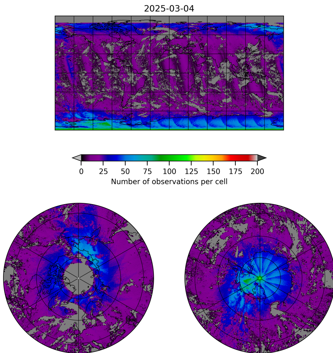
Figure 8: Map of the number of observations for 2025-03-03 to 2025-03-05
