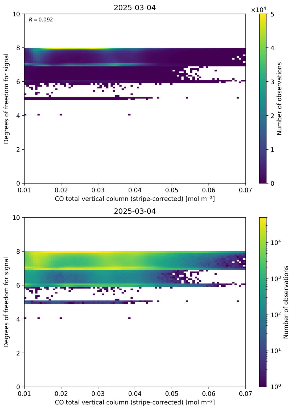
Figure 38: Scatter density plot of “CO total vertical column (stripe-corrected)” against “Degrees of freedom for signal” for 2025-03-03 to 2025-03-05.
