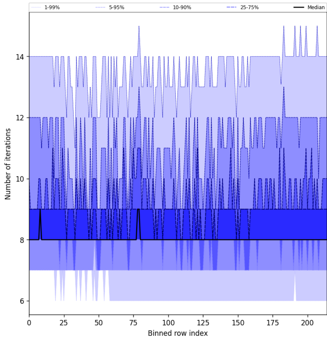
Figure 32: Along track statistics of “Number of iterations” for 2025-03-03 to 2025-03-05
