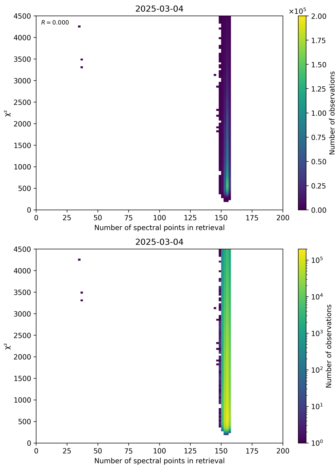
Figure 58: Scatter density plot of “Number of spectral points in retrieval” against “ \chi^2 ” for 2025-03-03 to 2025-03-05.
