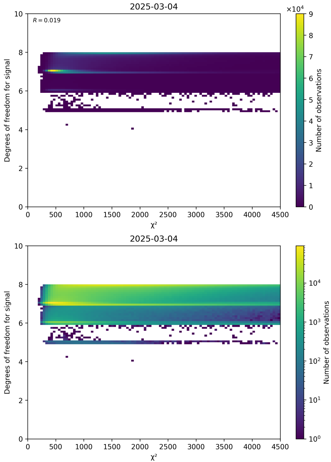
Figure 48: Scatter density plot of “ \chi^2 ” against “Degrees of freedom for signal” for 2025-03-03 to 2025-03-05.
