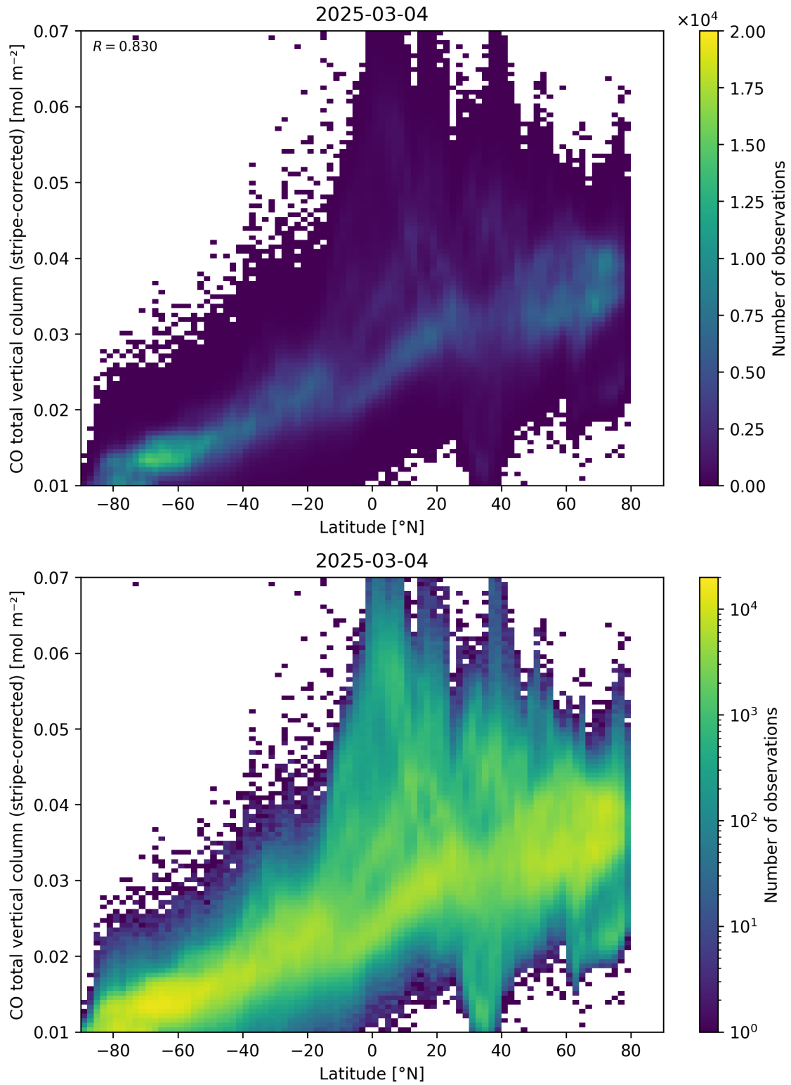
Figure 52: Scatter density plot of “Latitude” against “CO total vertical column (stripe-corrected)” for 2025-03-03 to 2025-03-05.
