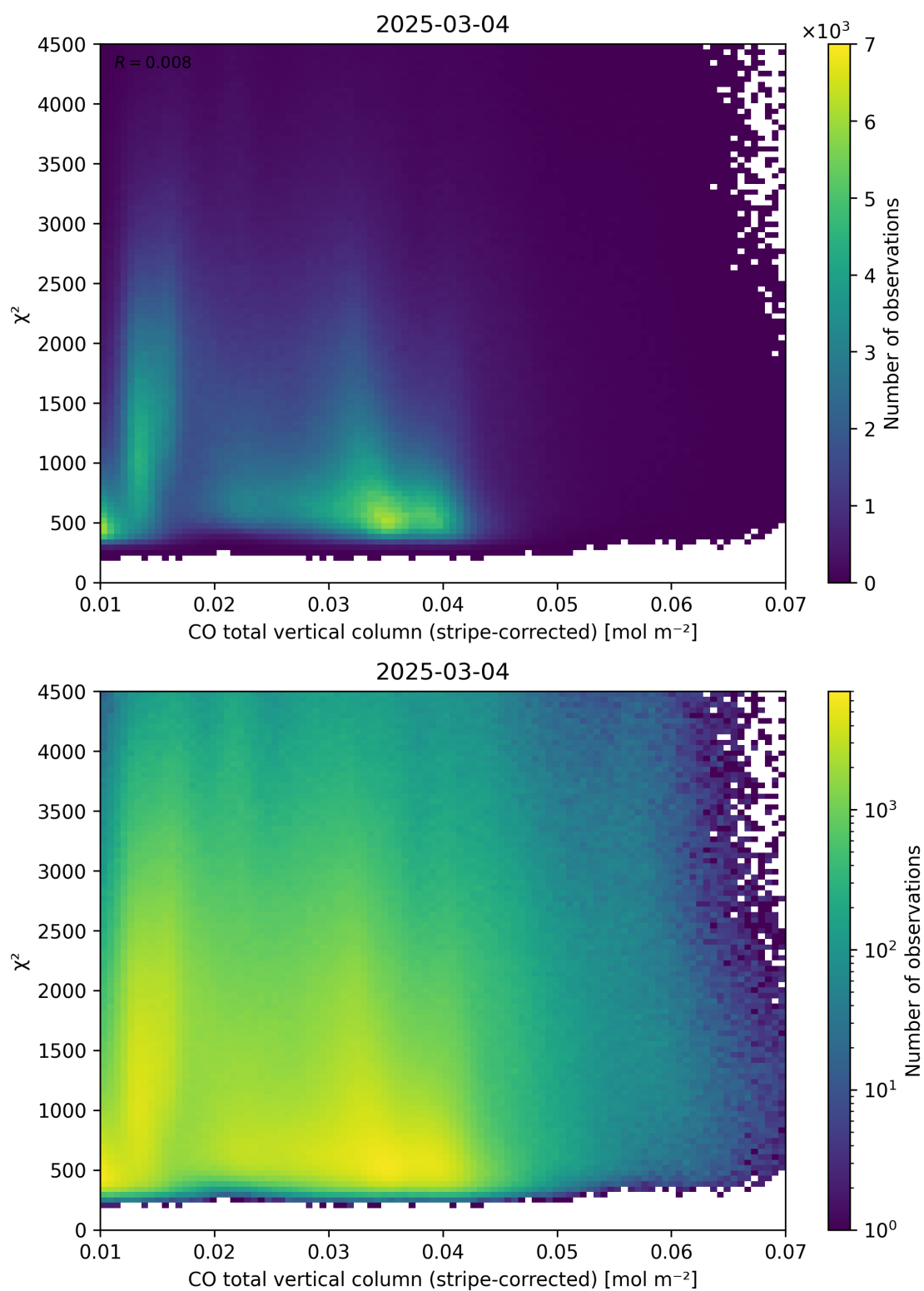
Figure 37: Scatter density plot of “CO total vertical column (stripe-corrected)” against “ \chi^2 ” for 2025-03-03 to 2025-03-05.
