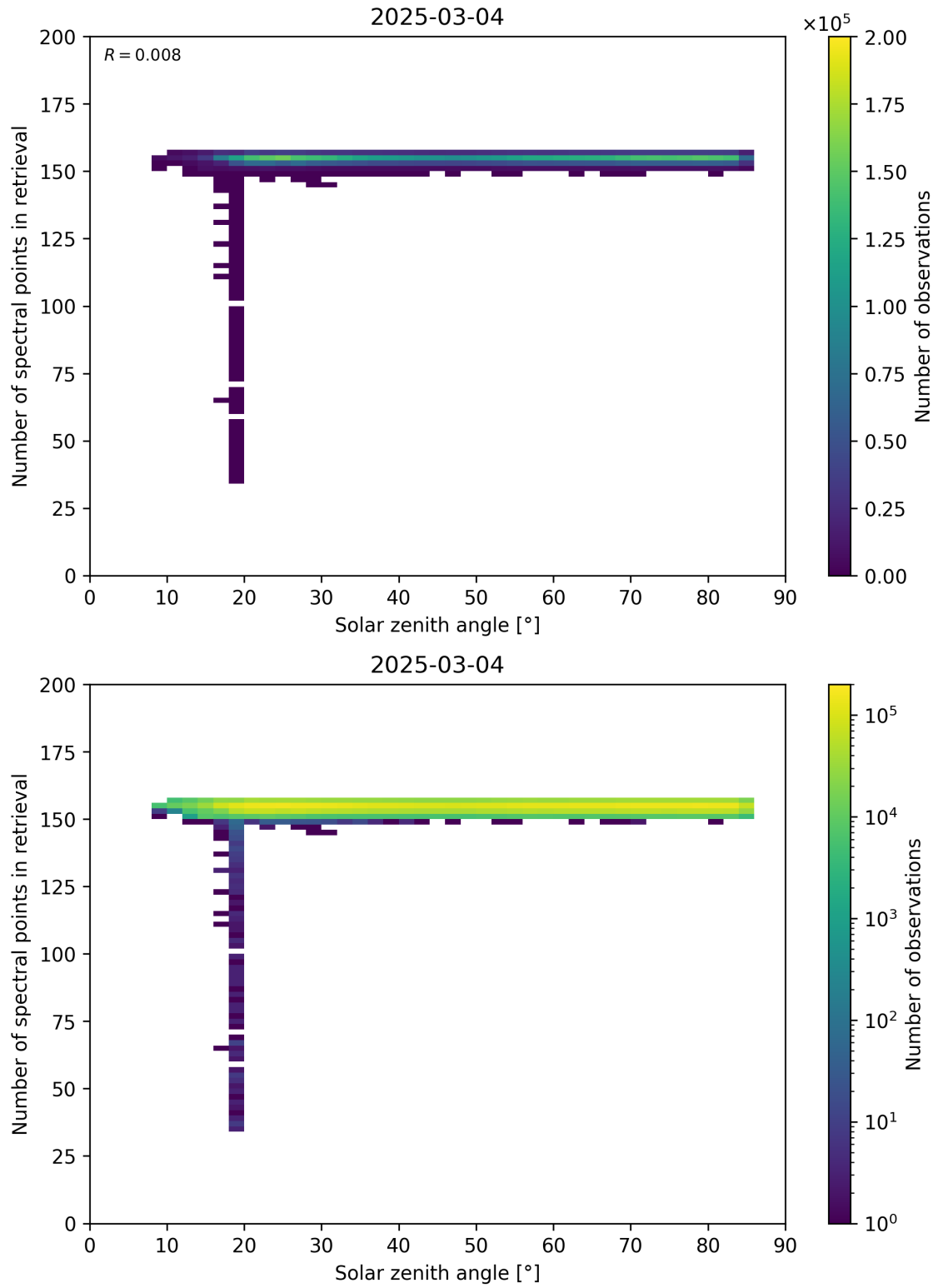
Figure 68: Scatter density plot of “Solar zenith angle” against “Number of spectral points in retrieval” for 2025-03-03 to 2025-03-05.
