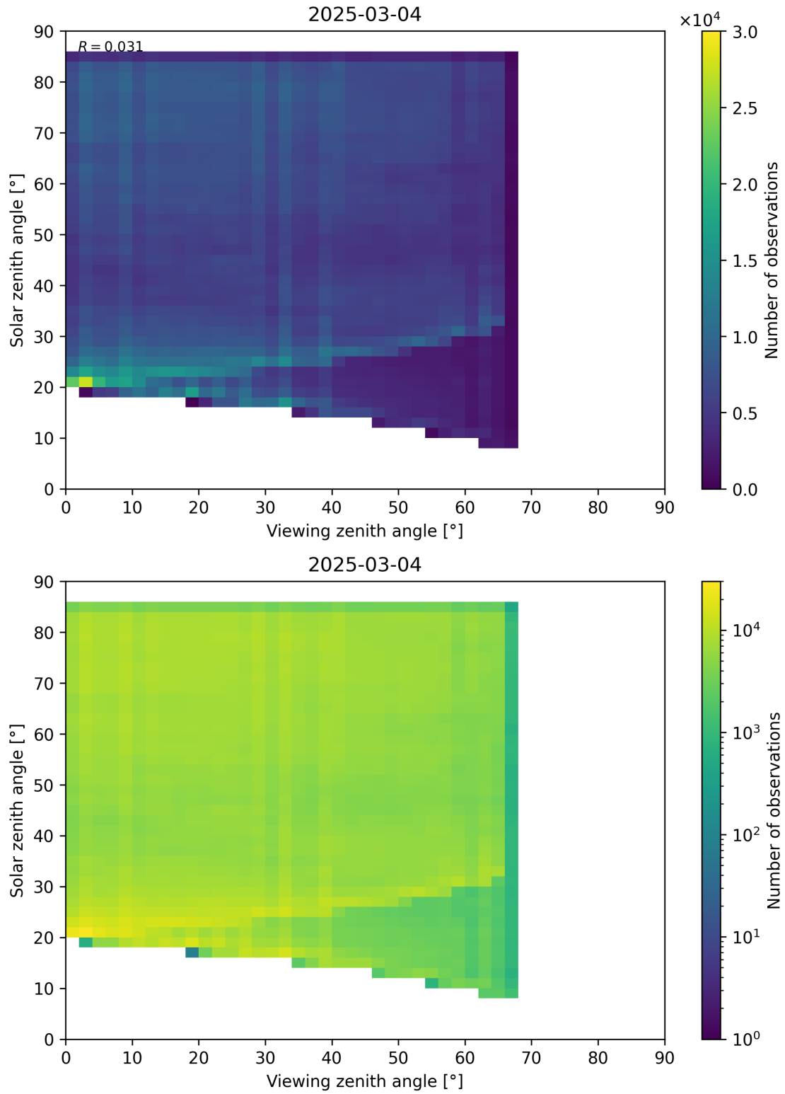
Figure 77: Scatter density plot of “Viewing zenith angle” against “Solar zenith angle” for 2025-03-03 to 2025-03-05.
