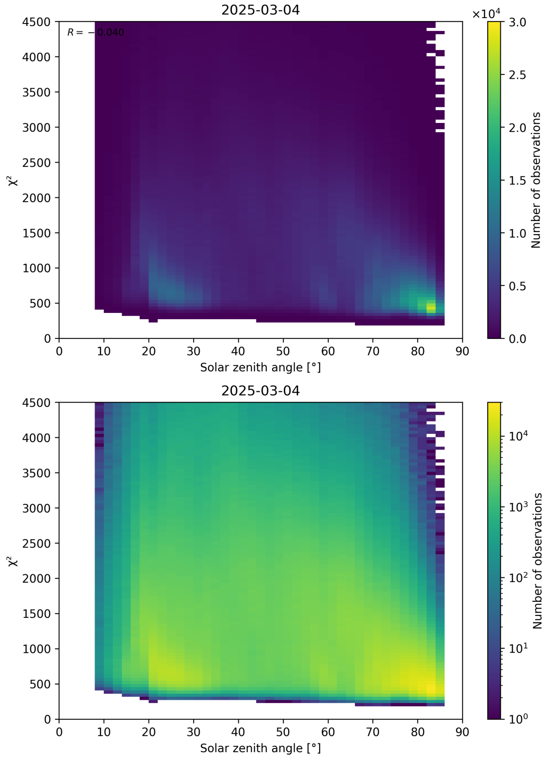
Figure 64: Scatter density plot of “Solar zenith angle” against “ \chi^2 ” for 2025-03-03 to 2025-03-05.
