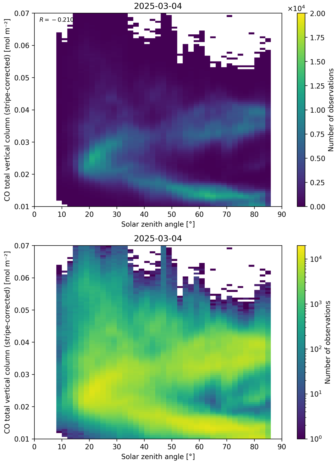
Figure 62: Scatter density plot of “Solar zenith angle” against “CO total vertical column (stripe-corrected)” for 2025-03-03 to 2025-03-05.
