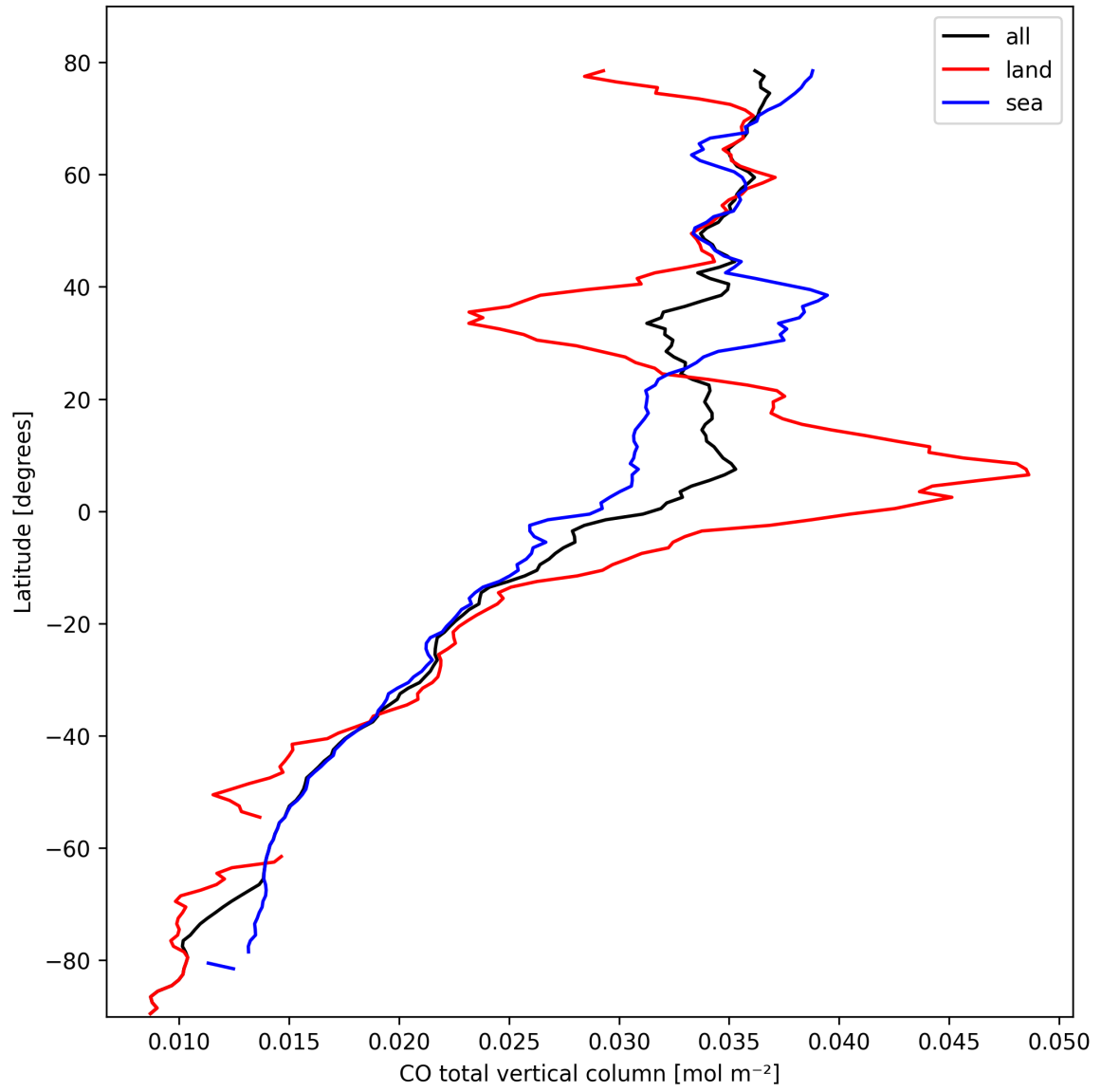
Figure 10: Zonal average of “CO total vertical column” for 2025-03-03 to 2025-03-05.
