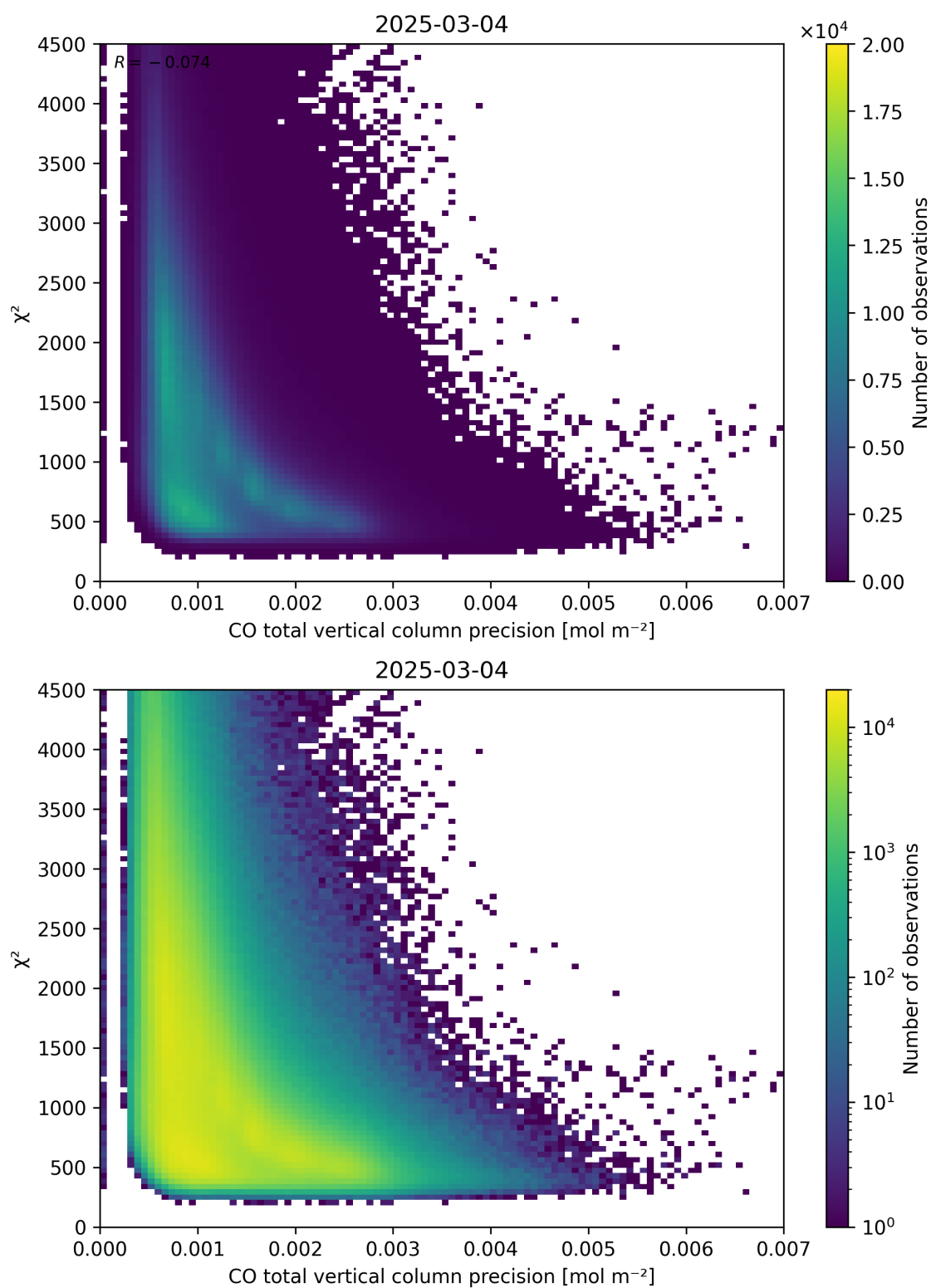
Figure 44: Scatter density plot of “CO total vertical column precision” against “ \chi^2 ” for 2025-03-03 to 2025-03-05.
