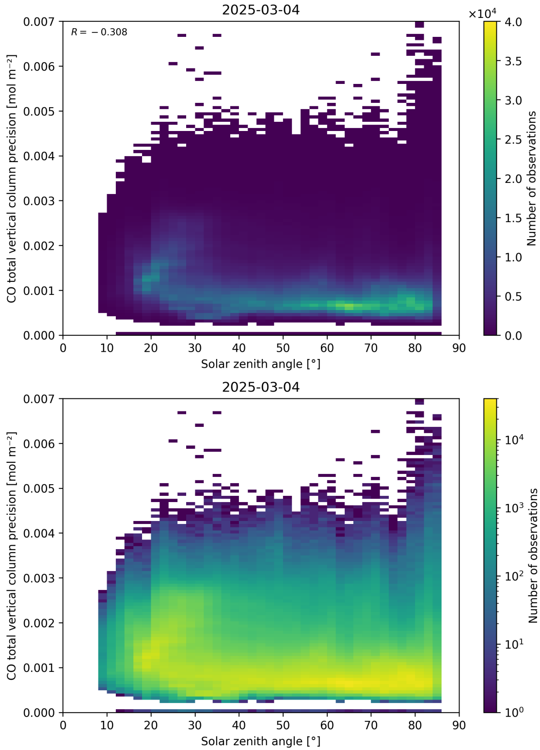
Figure 63: Scatter density plot of “Solar zenith angle” against “CO total vertical column precision” for 2025-03-03 to 2025-03-05.
