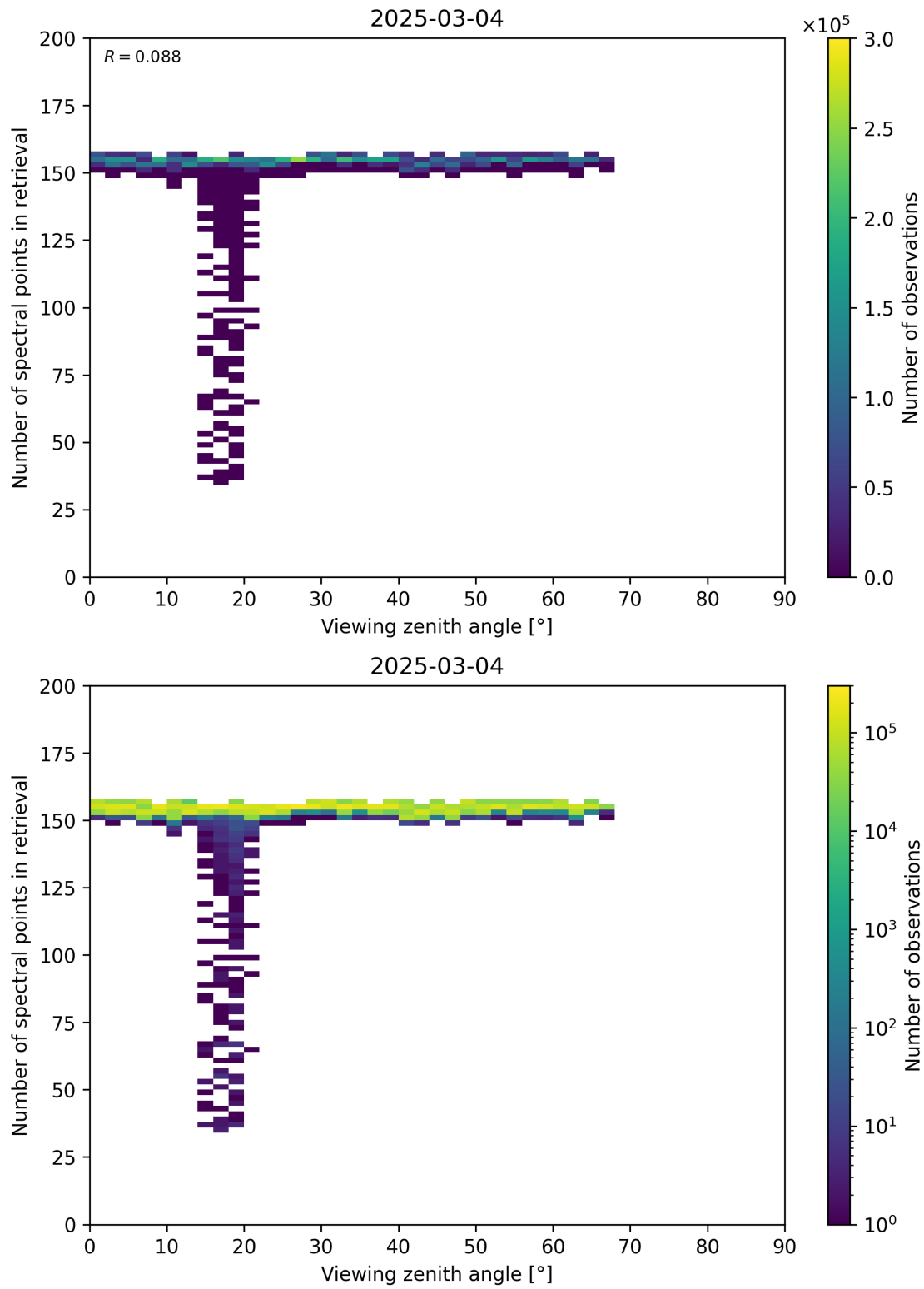
Figure 76: Scatter density plot of “Viewing zenith angle” against “Number of spectral points in retrieval” for 2025-03-03 to 2025-03-05.
