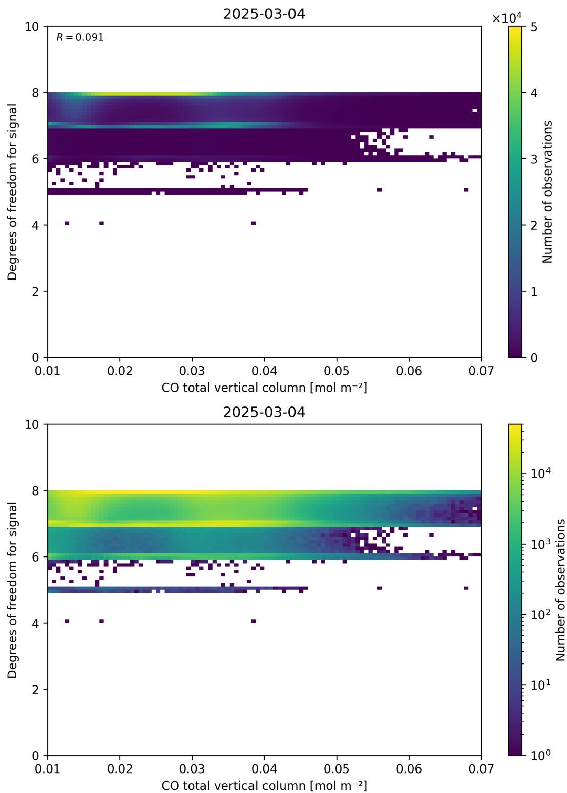
Figure 41: Scatter density plot of “CO total vertical column” against “Degrees of freedom for signal” for 2025-03-03 to 2025-03-05.
