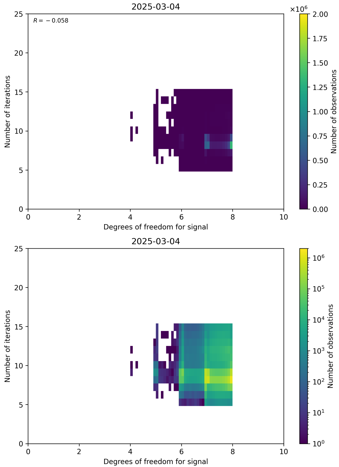
Figure 50: Scatter density plot of “Degrees of freedom for signal” against “Number of iterations” for 2025-03-03 to 2025-03-05.
