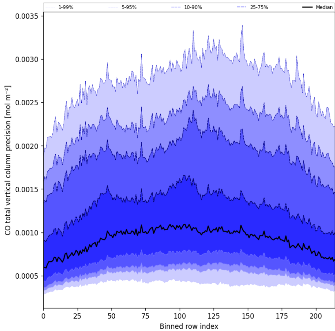
Figure 28: Along track statistics of “CO total vertical column precision” for 2025-03-03 to 2025-03-05
