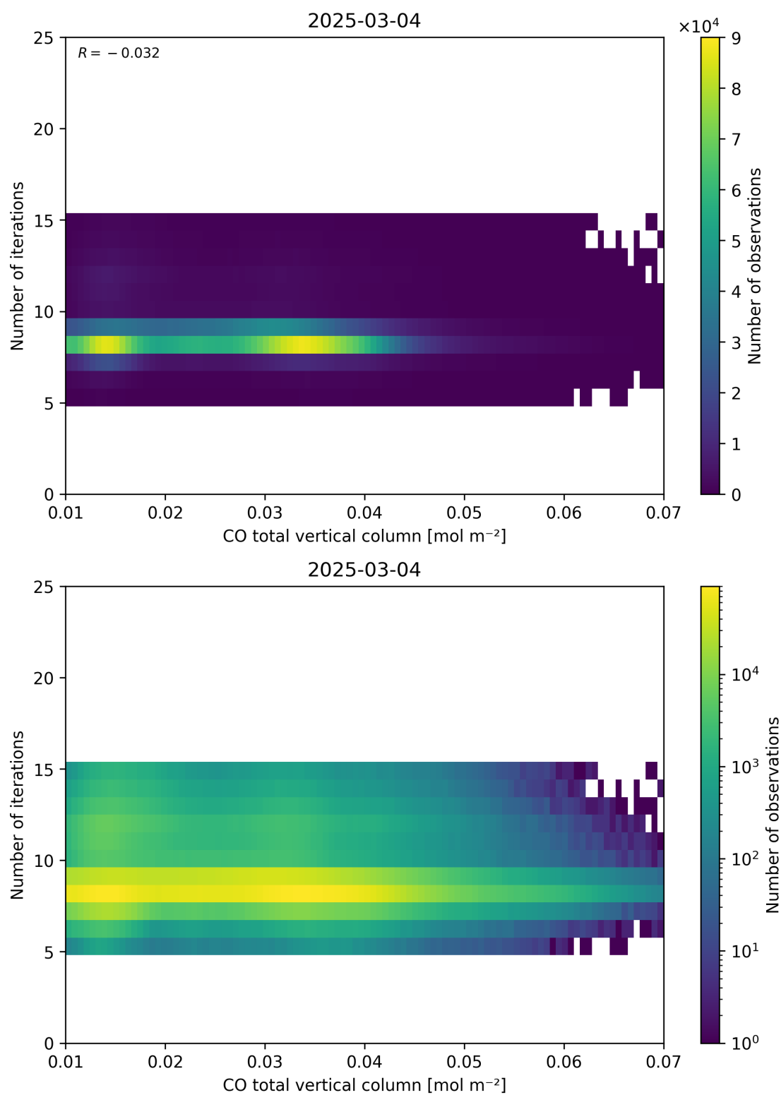
Figure 42: Scatter density plot of “CO total vertical column” against “Number of iterations” for 2025-03-03 to 2025-03-05.
