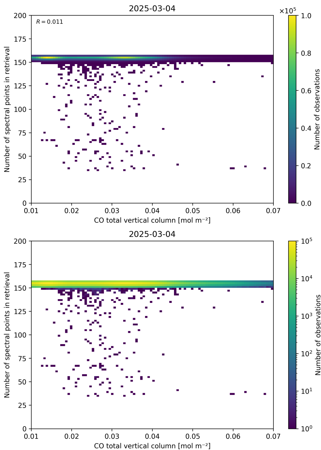
Figure 43: Scatter density plot of “CO total vertical column” against “Number of spectral points in retrieval” for 2025-03-03 to 2025-03-05.
