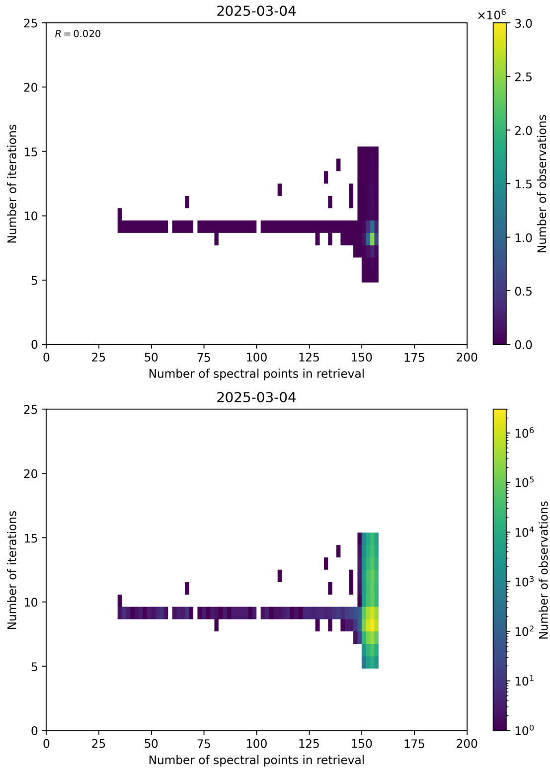
Figure 60: Scatter density plot of “Number of spectral points in retrieval” against “Number of iterations” for 2025-03-03 to 2025-03-05.
