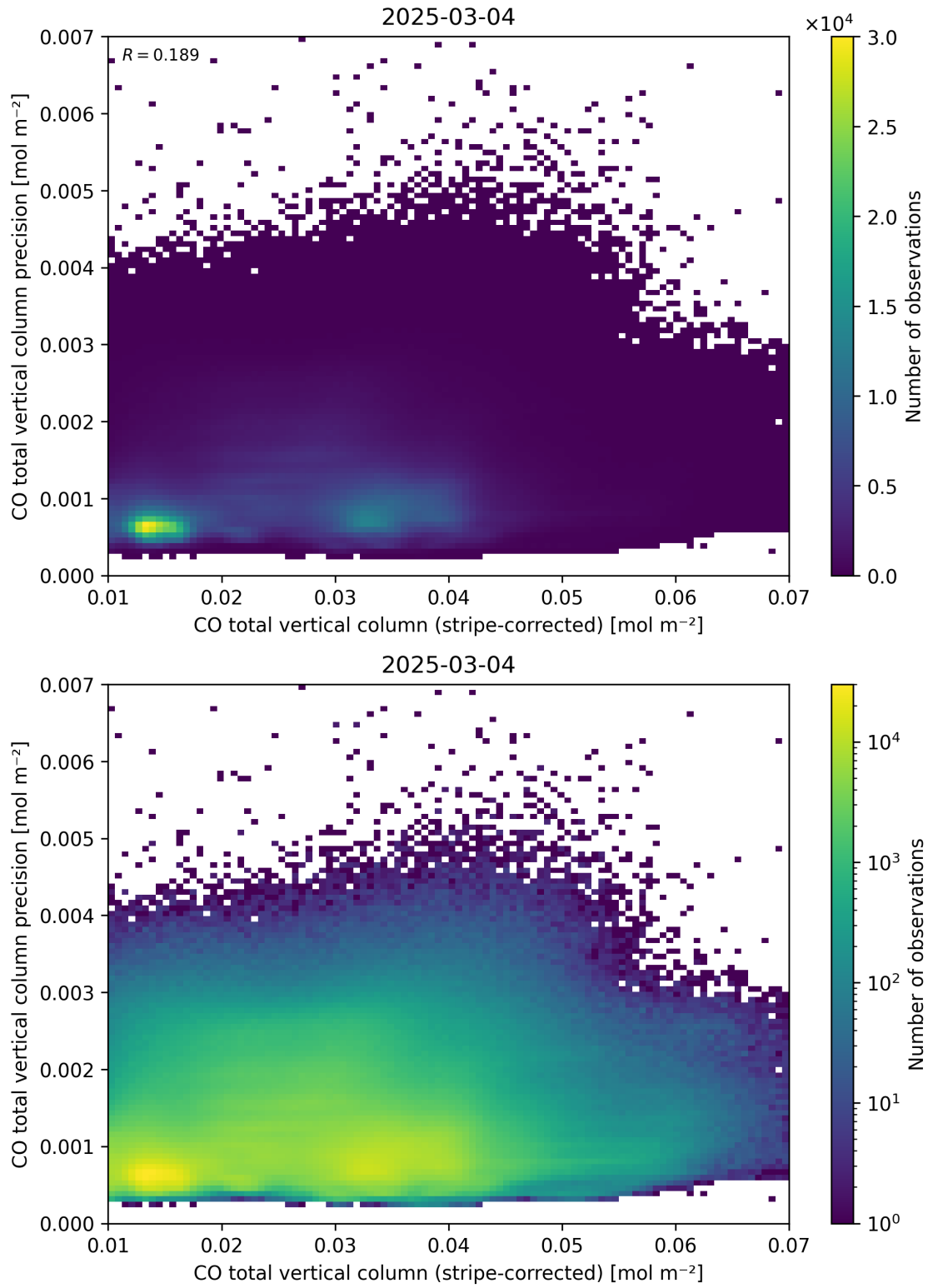
Figure 36: Scatter density plot of “CO total vertical column (stripe-corrected)” against “CO total vertical column precision” for 2025-03-03 to 2025-03-05.
