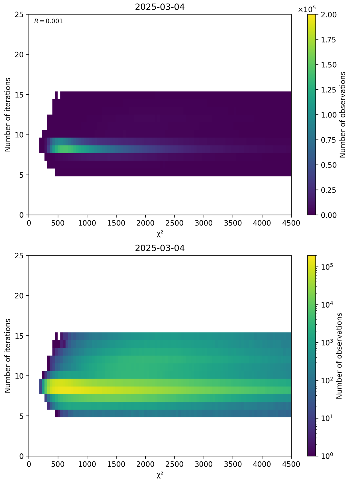
Figure 49: Scatter density plot of “ \chi^2 ” against “Number of iterations” for 2025-03-03 to 2025-03-05.
