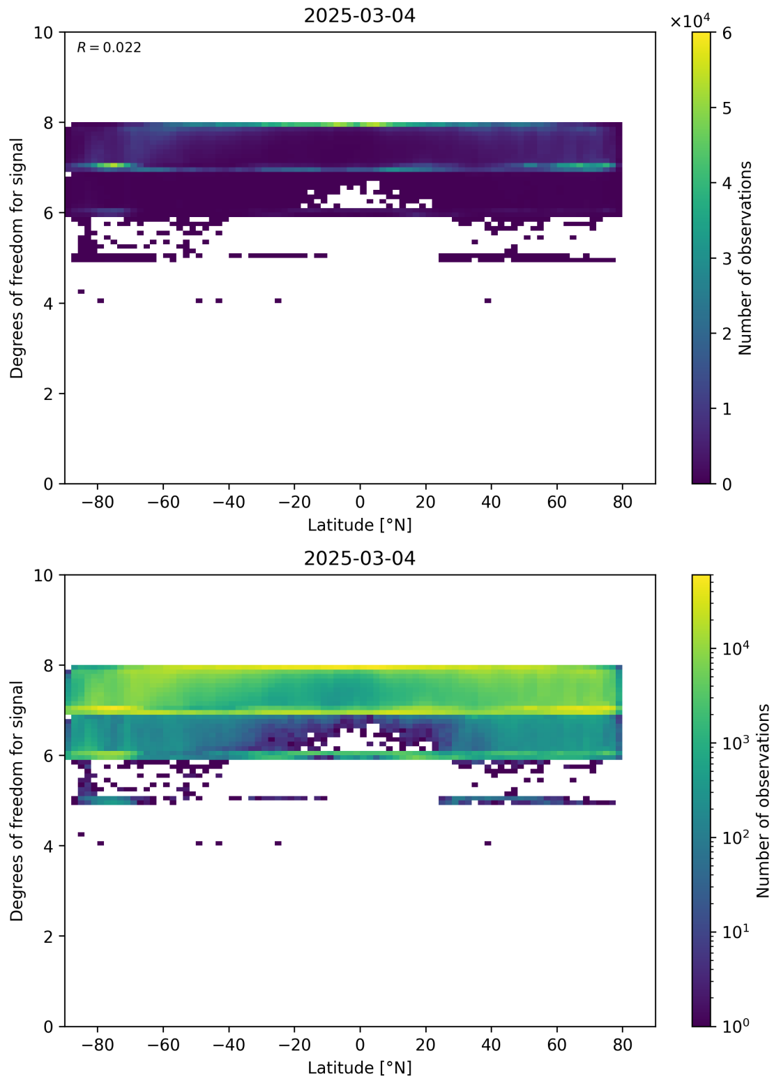
Figure 55: Scatter density plot of “Latitude” against “Degrees of freedom for signal” for 2025-03-03 to 2025-03-05.
