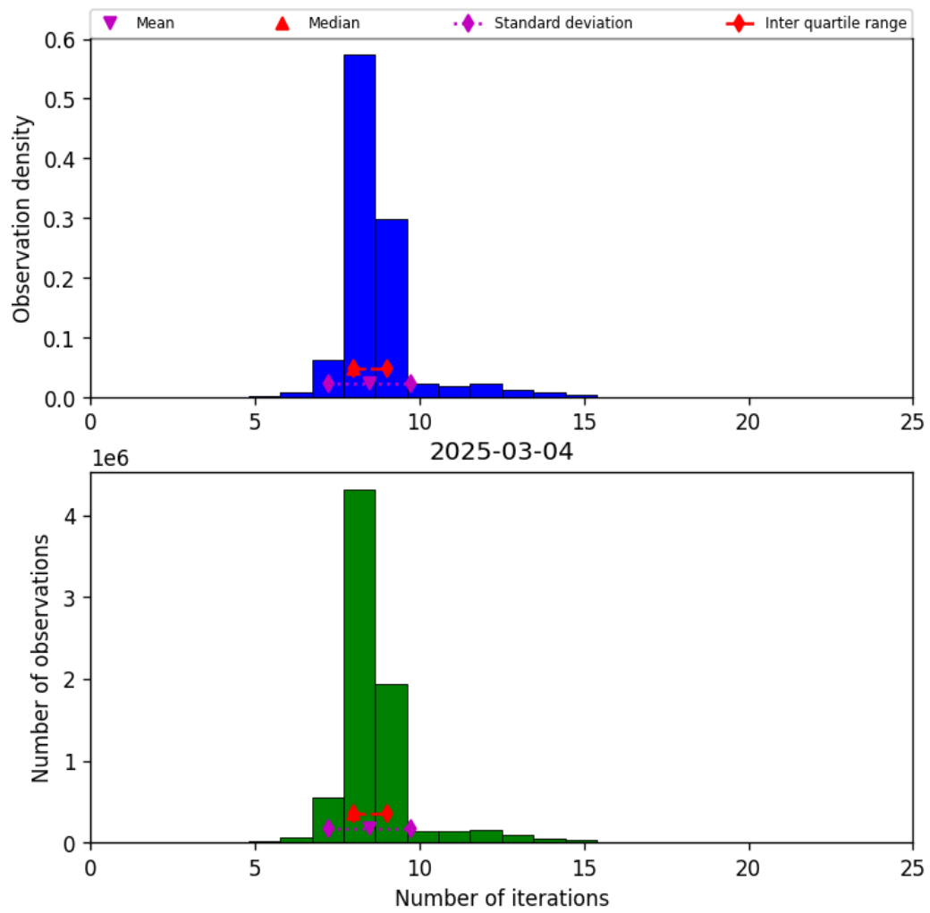
Figure 24: Histogram of “Number of iterations” for 2025-03-03 to 2025-03-05
