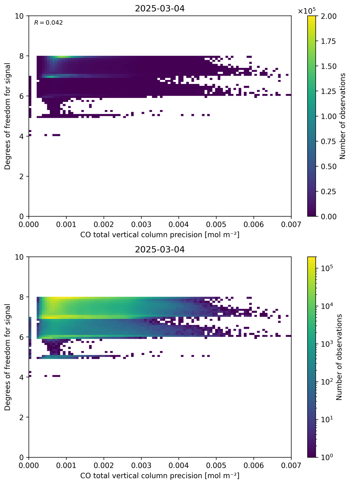
Figure 45: Scatter density plot of “CO total vertical column precision” against “Degrees of freedom for signal” for 2025-03-03 to 2025-03-05.
