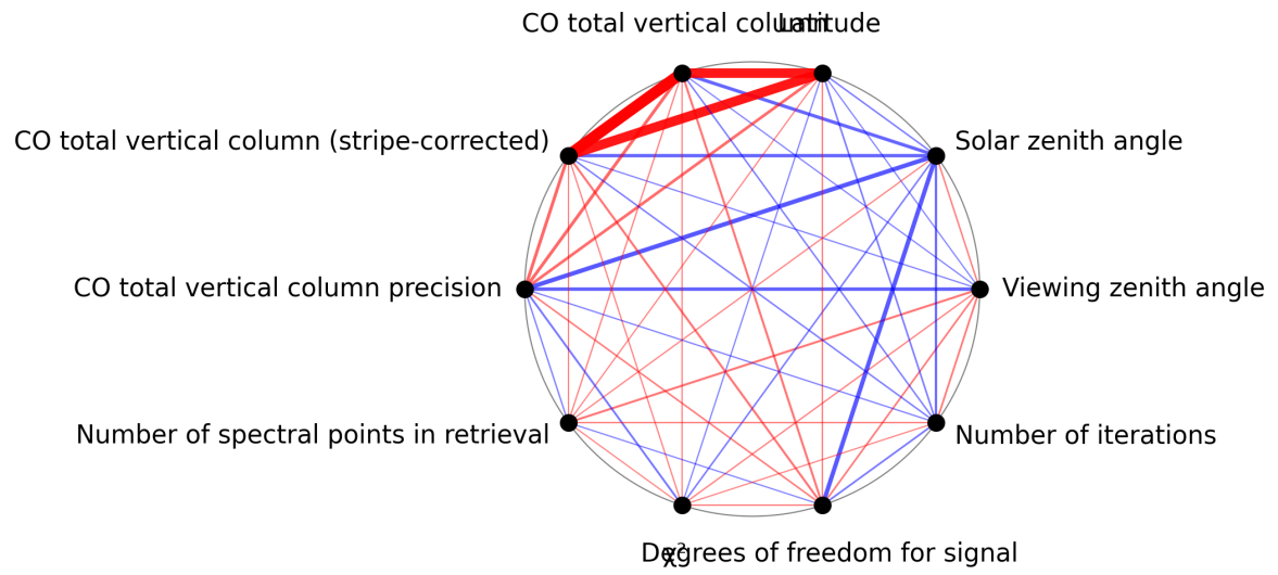
Figure 1: Map of correlation graph for 2025-03-03 to 2025-03-05.
