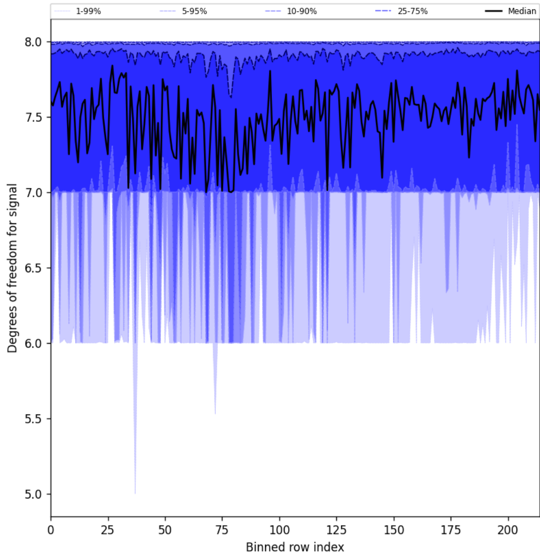
Figure 31: Along track statistics of “Degrees of freedom for signal” for 2025-03-03 to 2025-03-05
