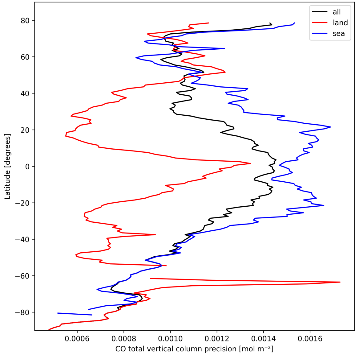
Figure 12: Zonal average of "CO total vertical column precision" for 2025-03-03 to 2025-03-05.
