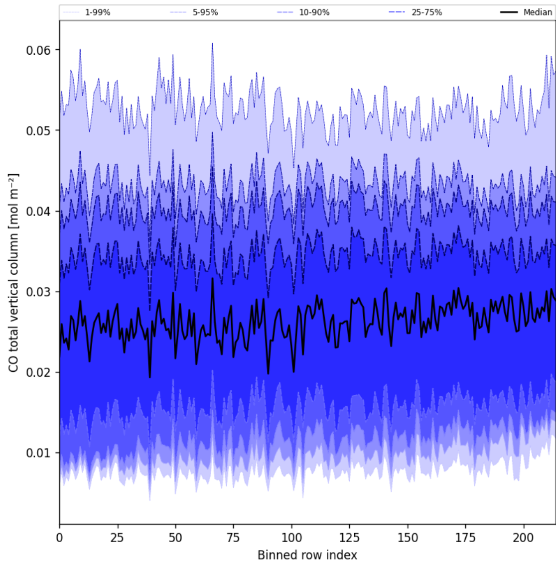
Figure 26: Along track statistics of “CO total vertical column” for 2025-03-03 to 2025-03-05
