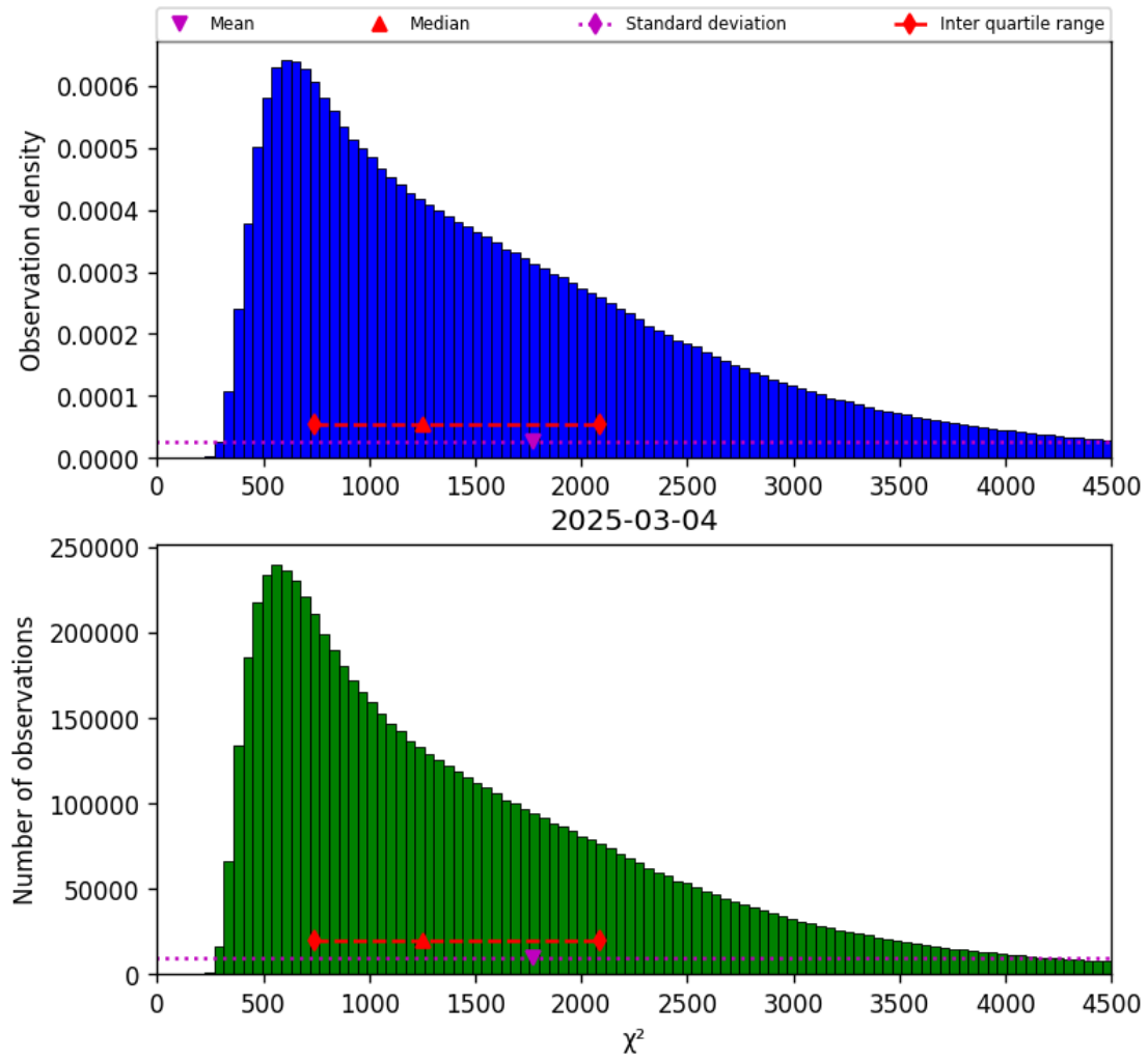
Figure 22: Histogram of “ \chi^2 ” for 2025-03-03 to 2025-03-05
