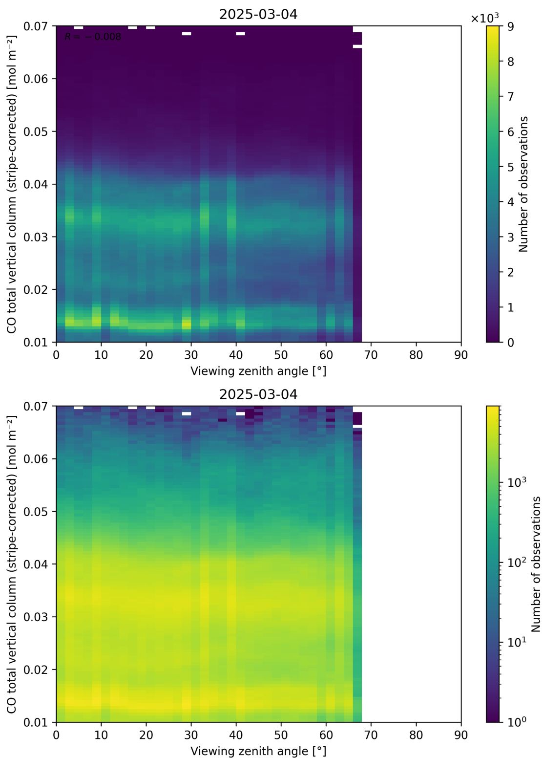
Figure 70: Scatter density plot of “Viewing zenith angle” against “CO total vertical column (stripe-corrected)” for 2025-03-03 to 2025-03-05.
