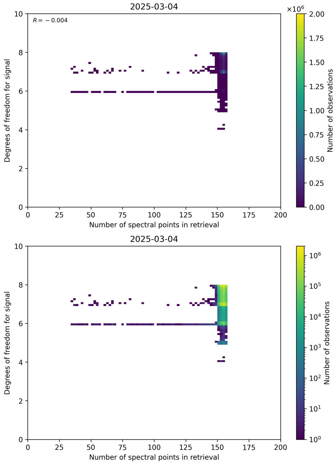
Figure 59: Scatter density plot of “Number of spectral points in retrieval” against “Degrees of freedom for signal” for 2025-03-03 to 2025-03-05.
