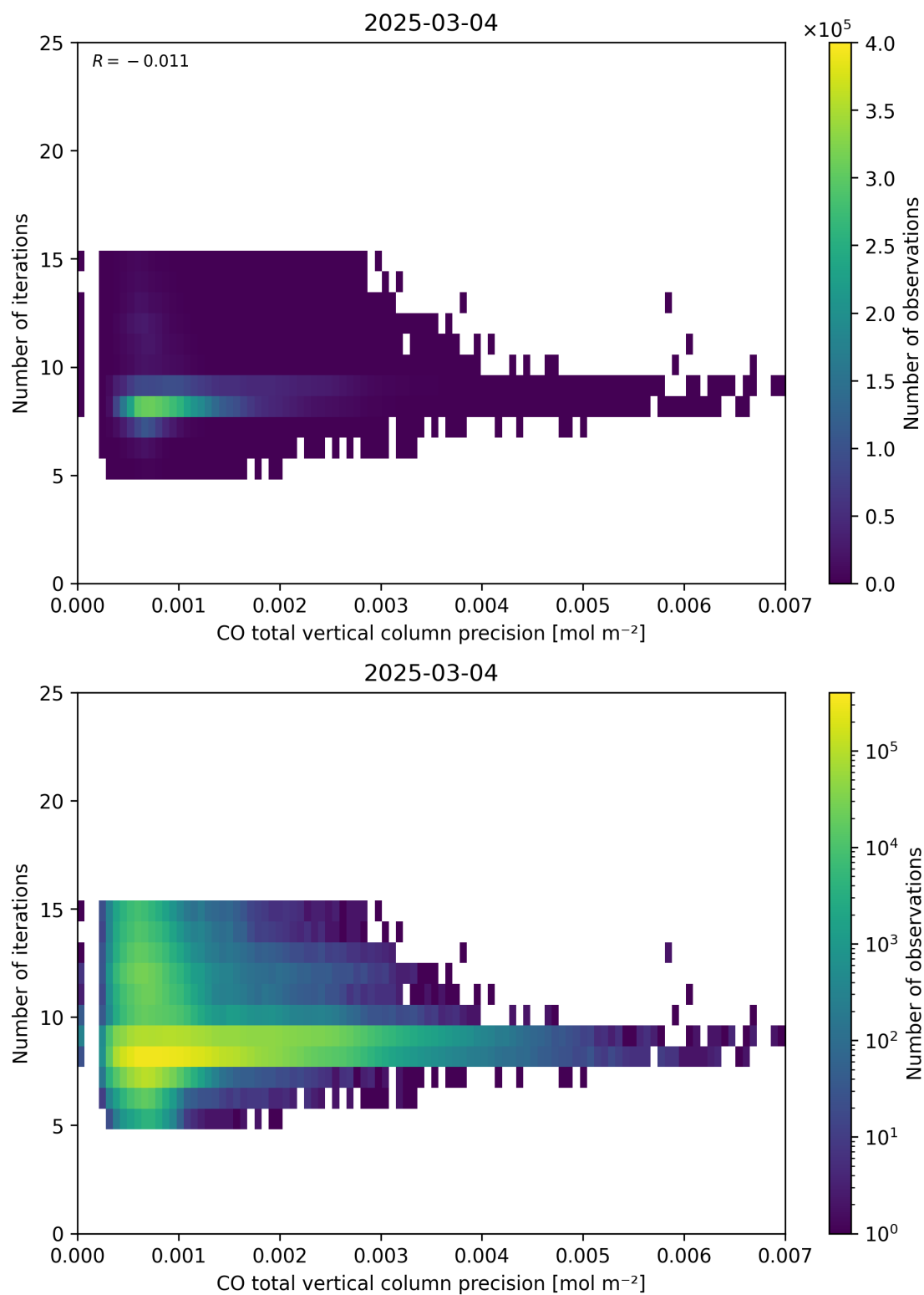
Figure 46: Scatter density plot of “CO total vertical column precision” against “Number of iterations” for 2025-03-03 to 2025-03-05.
