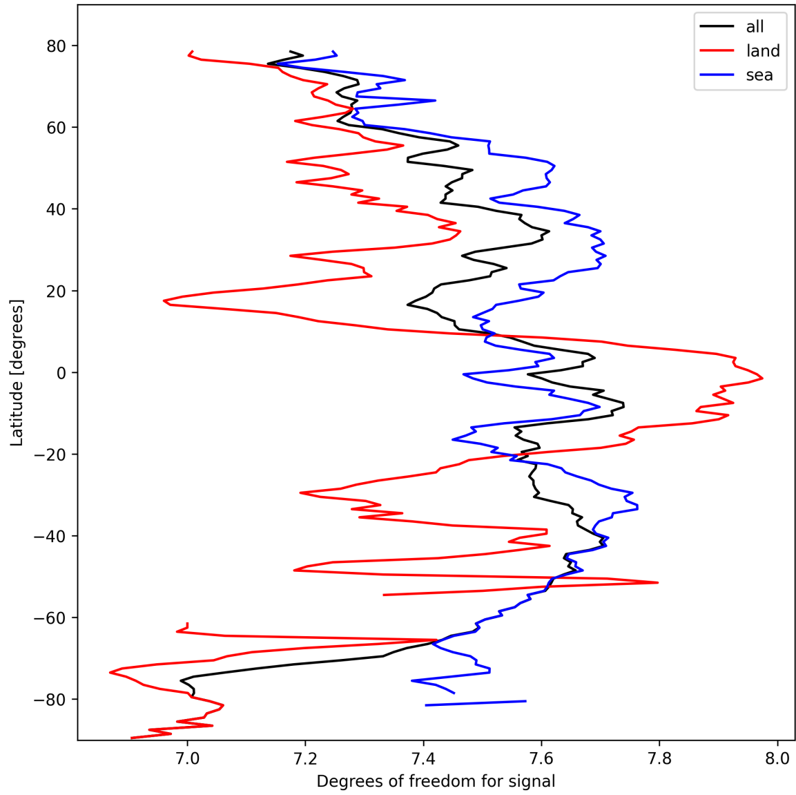
Figure 15: Zonal average of “Degrees of freedom for signal” for 2025-03-03 to 2025-03-05.
