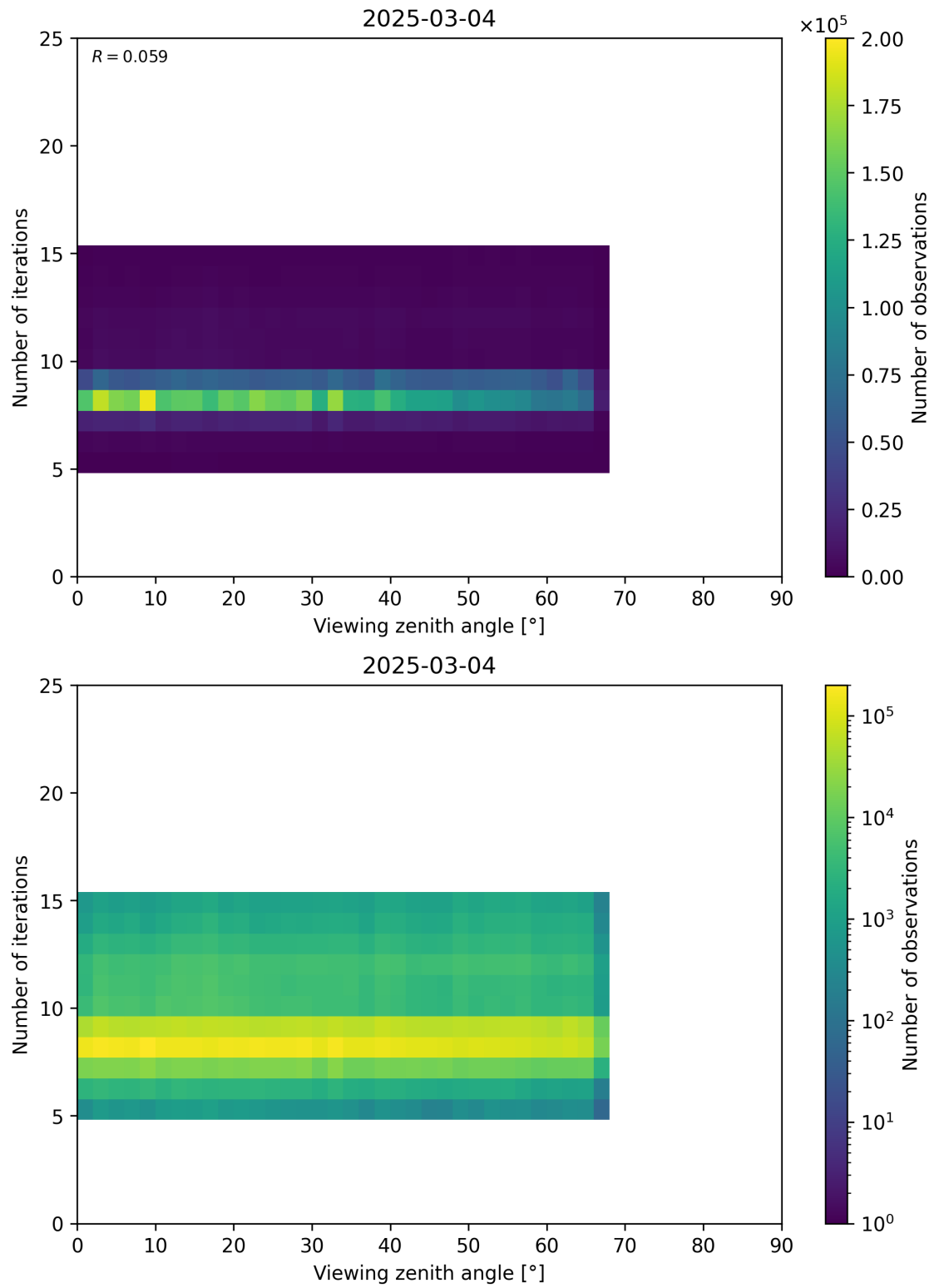
Figure 75: Scatter density plot of “Viewing zenith angle” against “Number of iterations” for 2025-03-03 to 2025-03-05.
