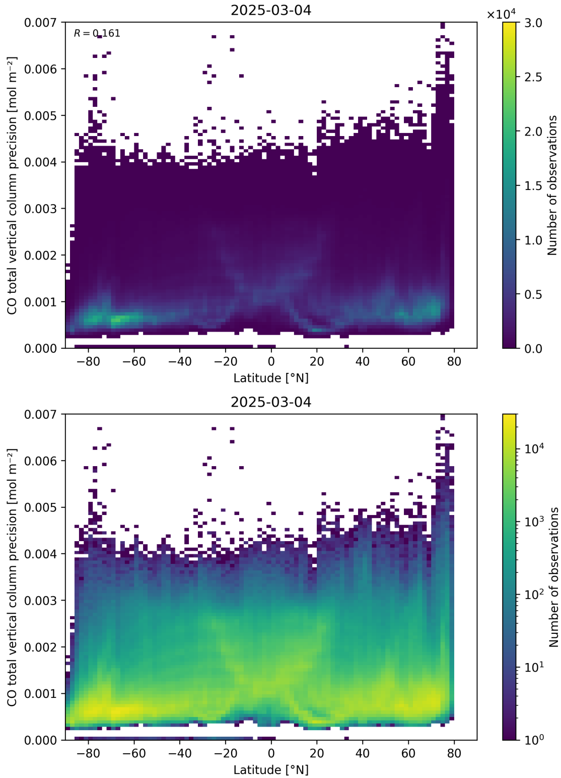
Figure 53: Scatter density plot of “Latitude” against “CO total vertical column precision” for 2025-03-03 to 2025-03-05.
