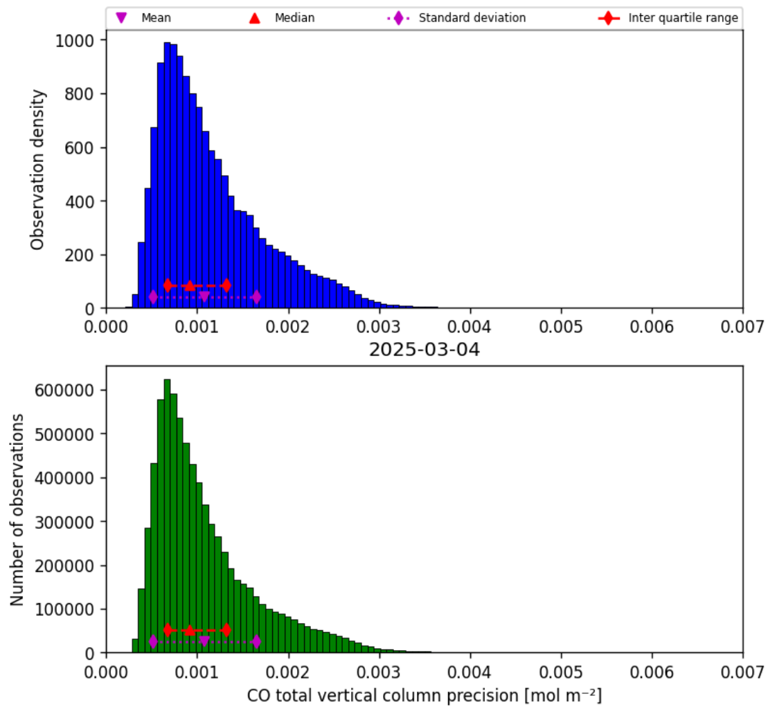
Figure 20: Histogram of “CO total vertical column precision” for 2025-03-03 to 2025-03-05
