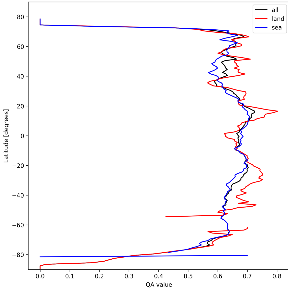
Figure 9: Zonal average of “QA value” for 2025-03-03 to 2025-03-05.
