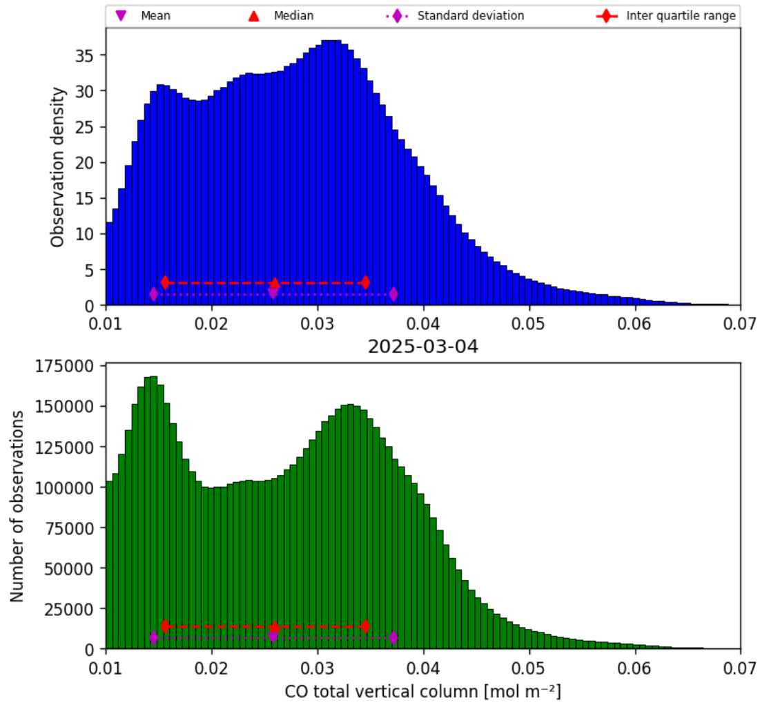
Figure 18: Histogram of “CO total vertical column” for 2025-03-03 to 2025-03-05
