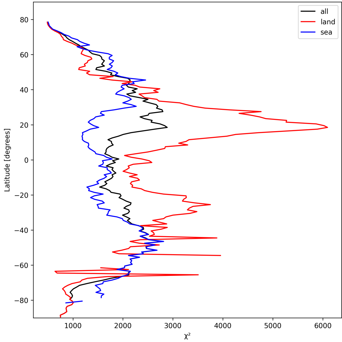
Figure 14: Zonal average of “ \chi^2 ” for 2025-03-03 to 2025-03-05.
