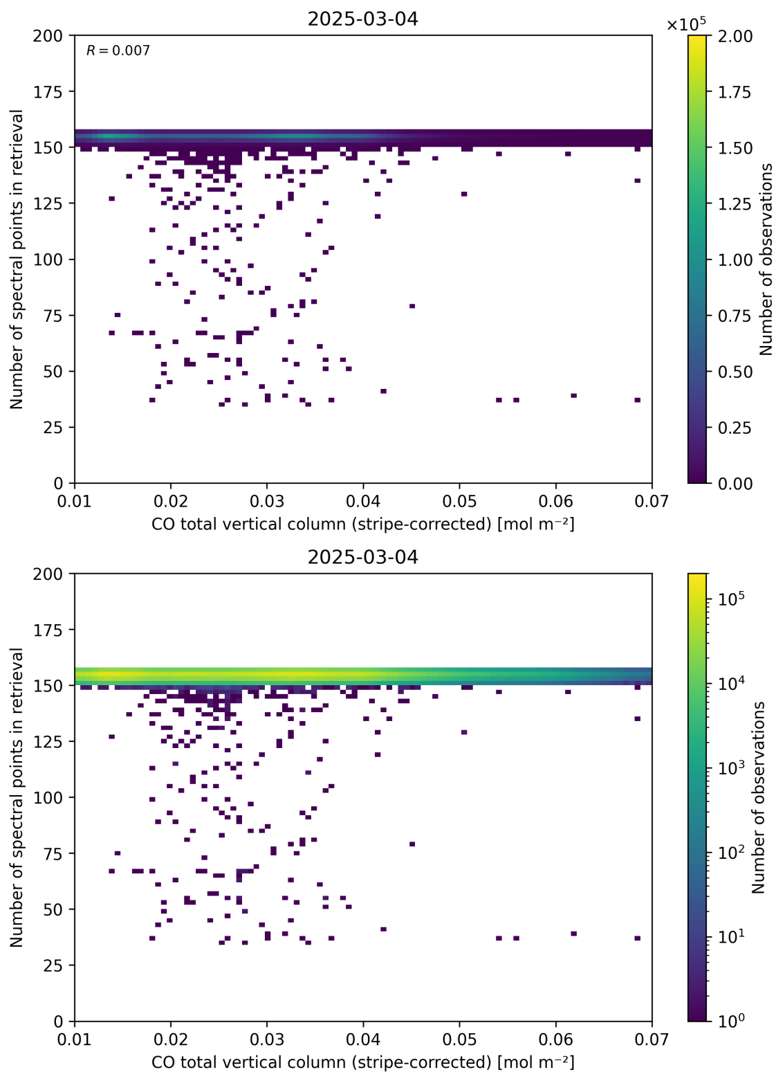
Figure 40: Scatter density plot of “CO total vertical column (stripe-corrected)” against “Number of spectral points in retrieval” for 2025-03-03 to 2025-03-05.
