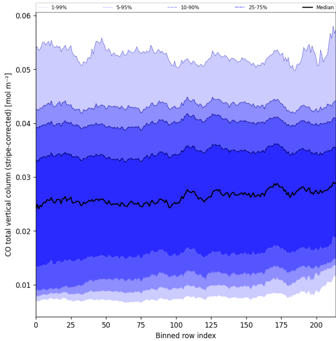
Figure 27: Along track statistics of “CO total vertical column (stripe-corrected)” for 2025-03-03 to 2025-03-05
