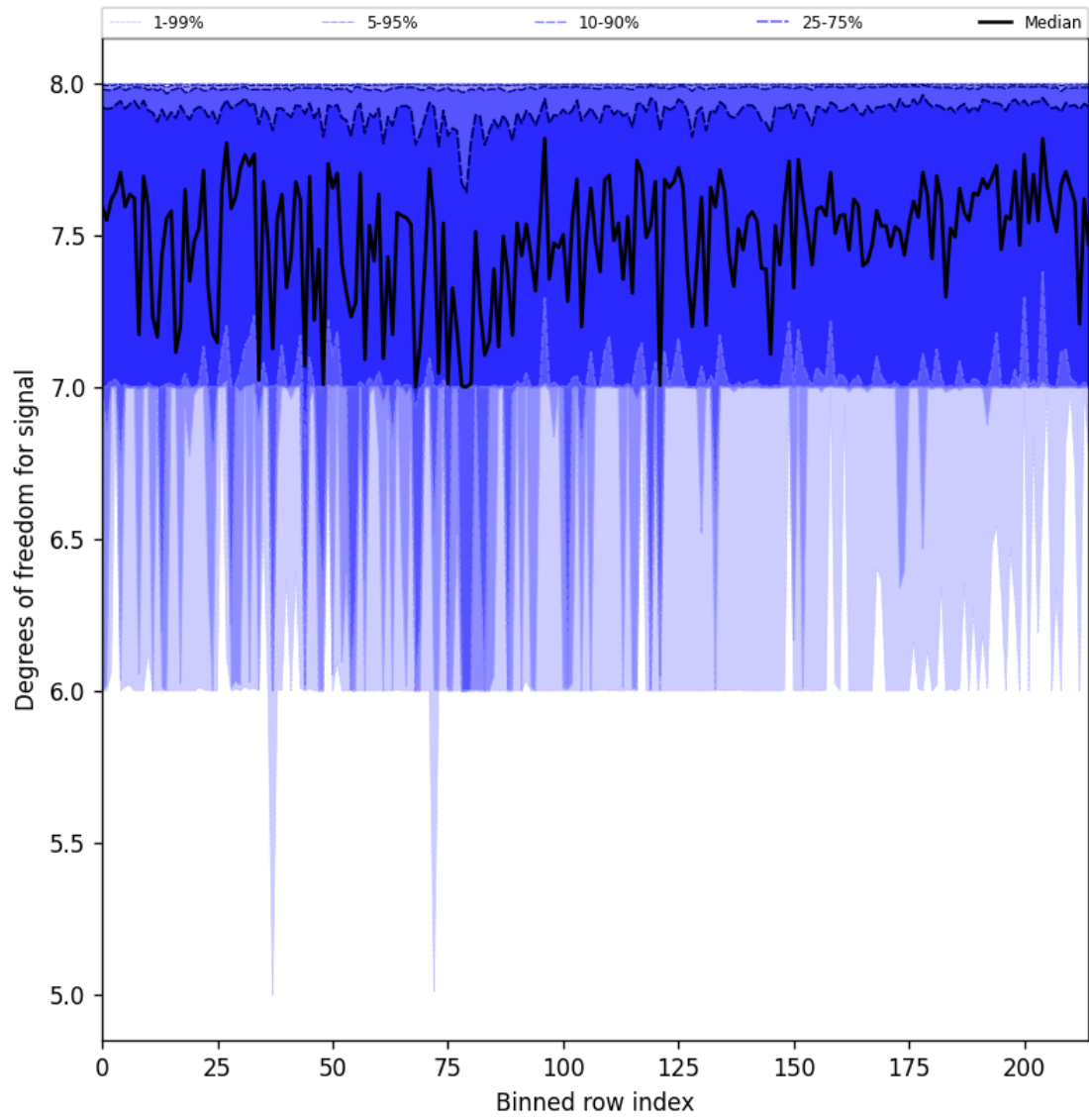
Figure 31: Along track statistics of “Degrees of freedom for signal” for 2025-03-04 to 2025-03-06
