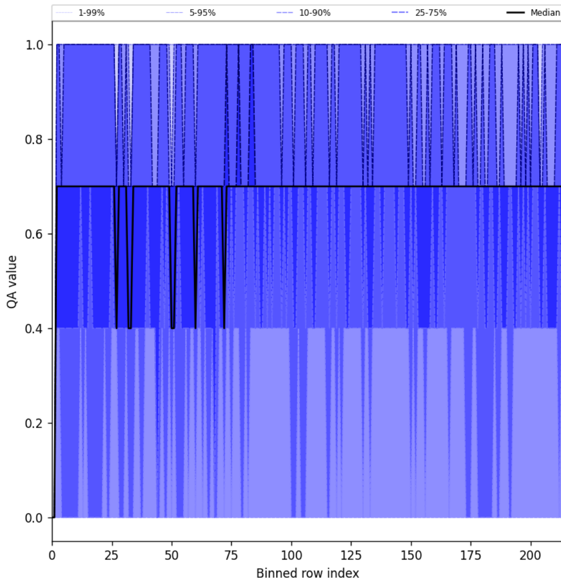
Figure 25: Along track statistics of “QA value” for 2025-03-04 to 2025-03-06
