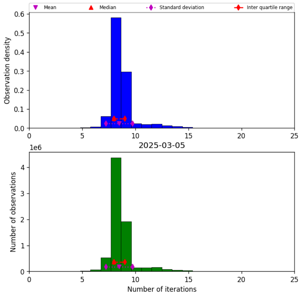
Figure 24: Histogram of “Number of iterations” for 2025-03-04 to 2025-03-06
