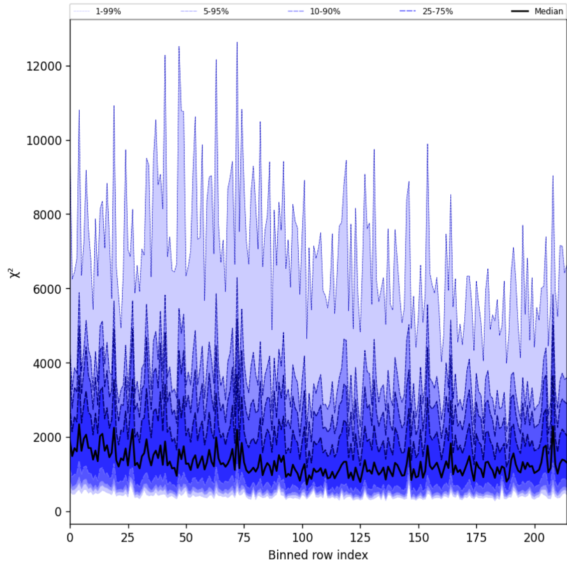
Figure 30: Along track statistics of “ \chi^2 ” for 2025-03-04 to 2025-03-06
