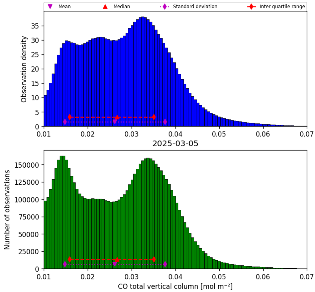
Figure 18: Histogram of “CO total vertical column” for 2025-03-04 to 2025-03-06
