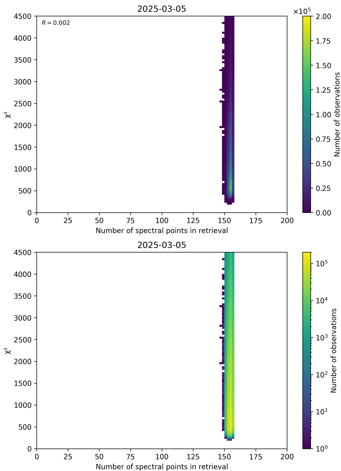
Figure 58: Scatter density plot of “Number of spectral points in retrieval” against “ \chi^2 ” for 2025-03-04 to 2025-03-06.
