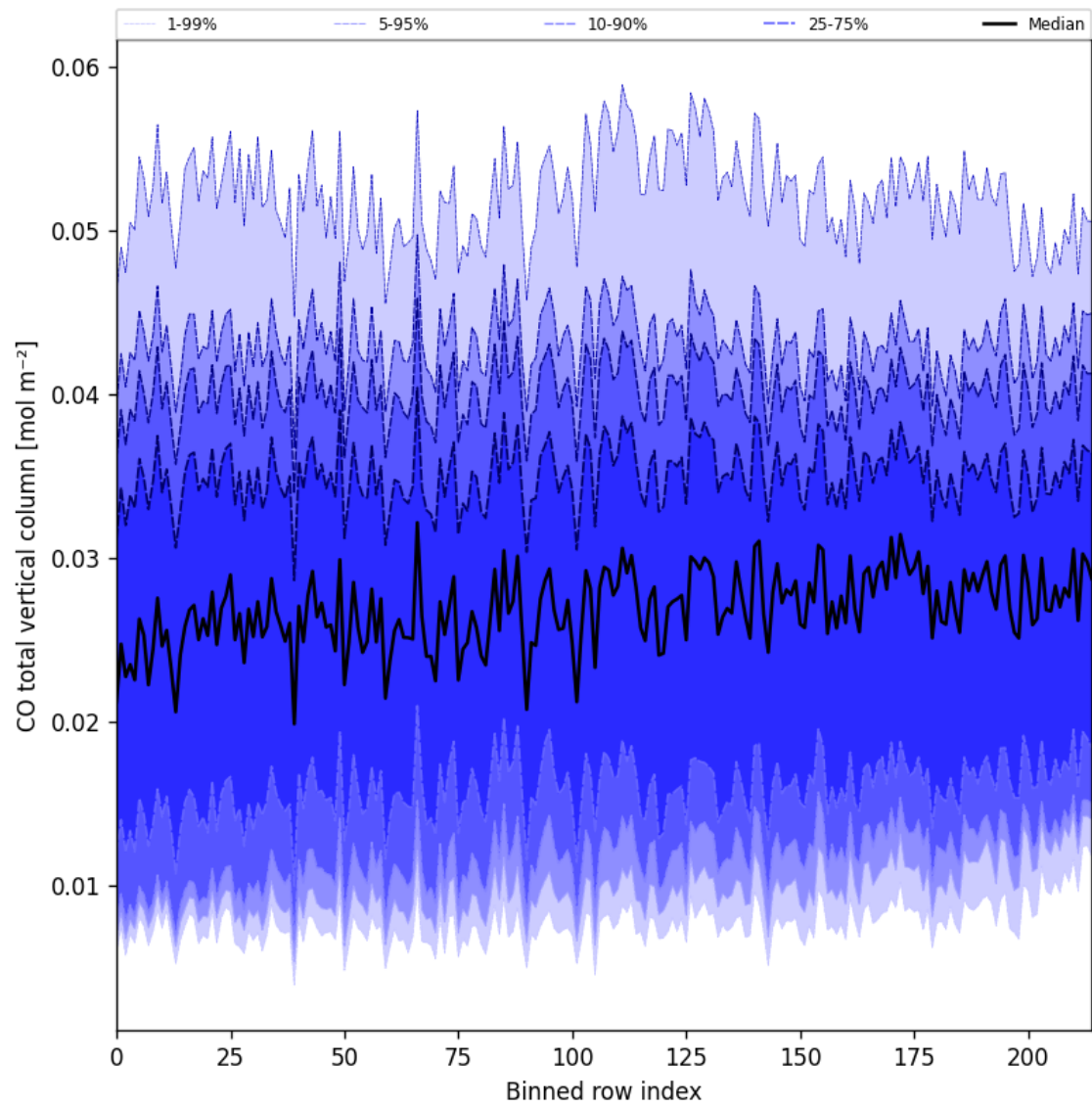
Figure 26: Along track statistics of “CO total vertical column” for 2025-03-04 to 2025-03-06
