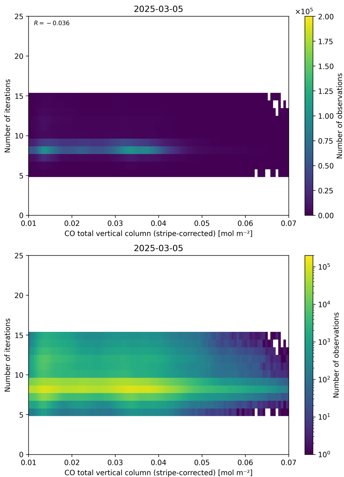
Figure 39: Scatter density plot of “CO total vertical column (stripe-corrected)” against “Number of iterations” for 2025-03-04 to 2025-03-06.
