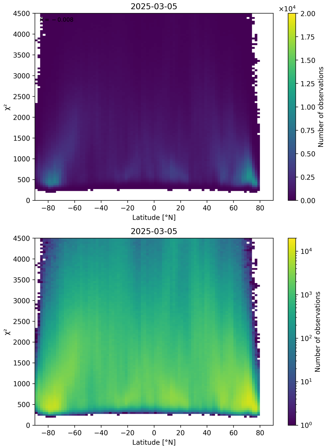
Figure 54: Scatter density plot of “Latitude” against “ \chi^2 ” for 2025-03-04 to 2025-03-06.
