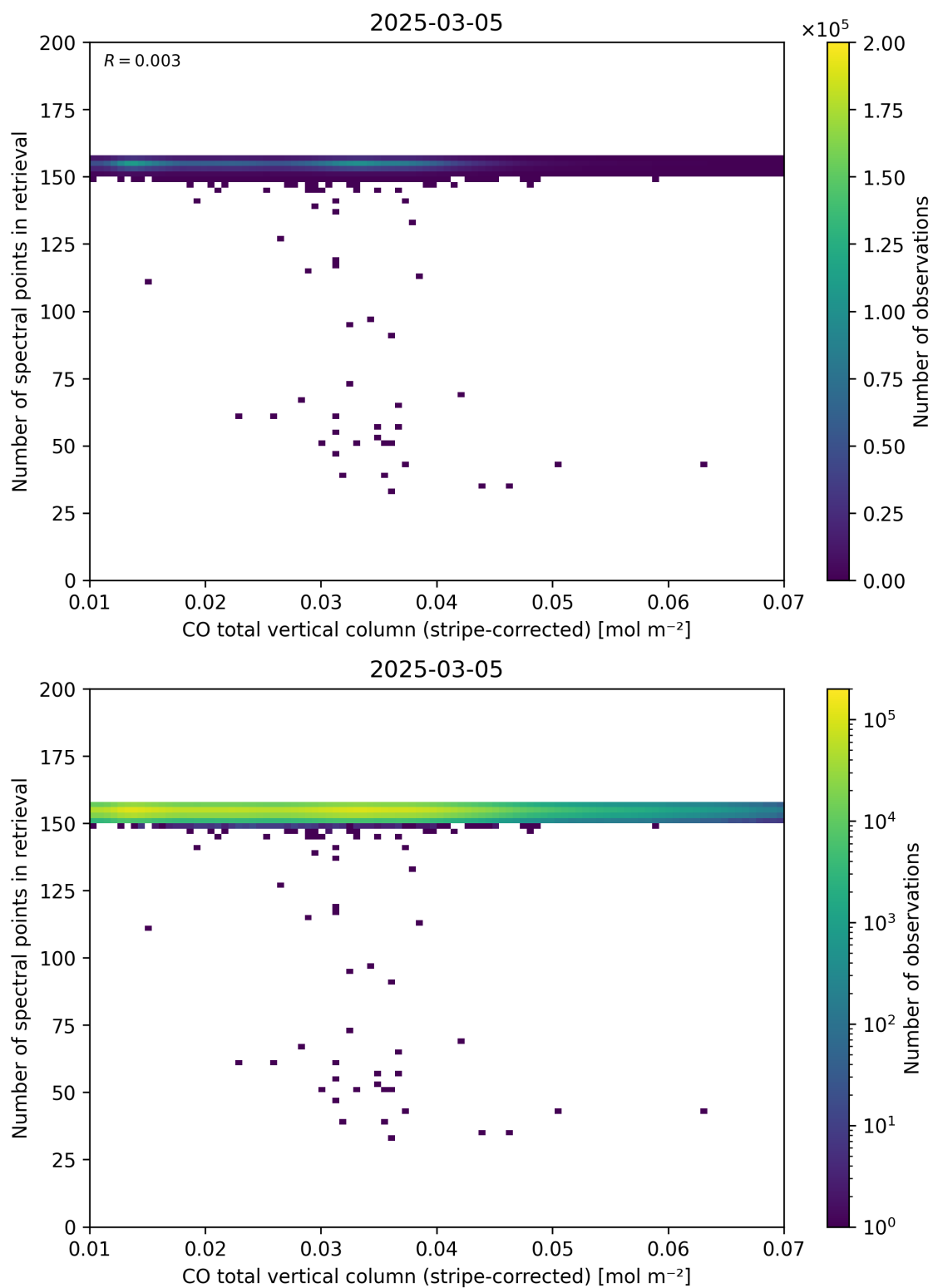
Figure 40: Scatter density plot of “CO total vertical column (stripe-corrected)” against “Number of spectral points in retrieval” for 2025-03-04 to 2025-03-06.
