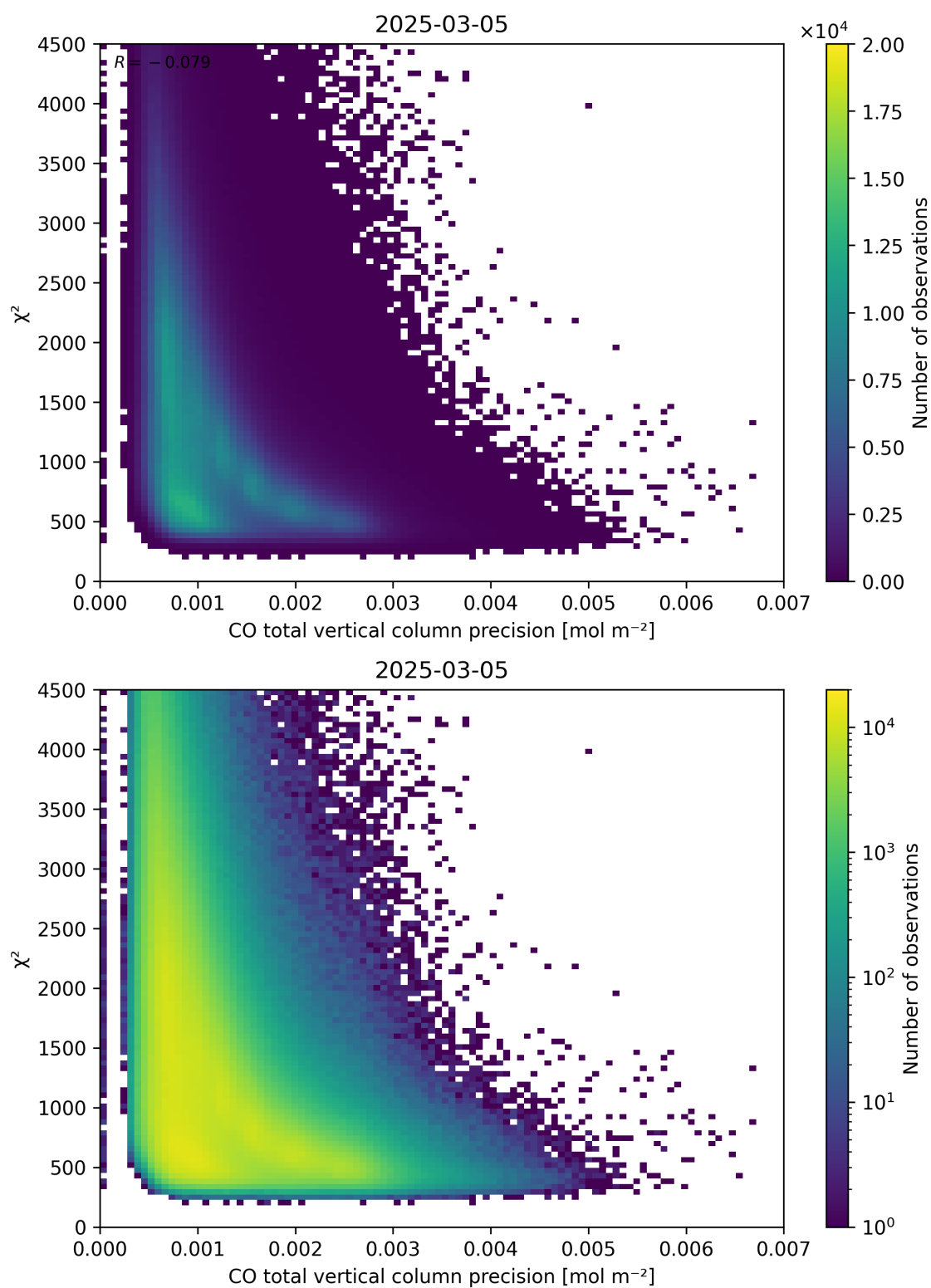
Figure 44: Scatter density plot of “CO total vertical column precision” against “ \chi^2 ” for 2025-03-04 to 2025-03-06.
