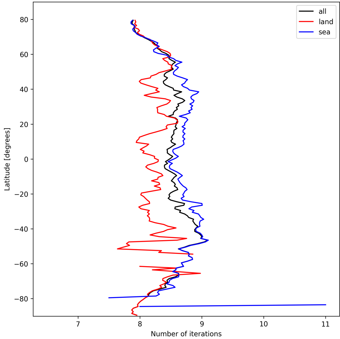
Figure 16: Zonal average of “Number of iterations” for 2025-03-04 to 2025-03-06.
