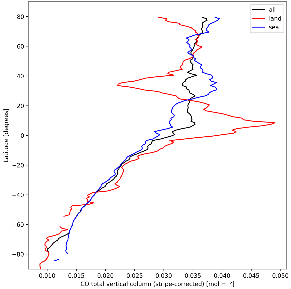
Figure 11: Zonal average of “CO total vertical column (stripe-corrected)” for 2025-03-04 to 2025-03-06.
