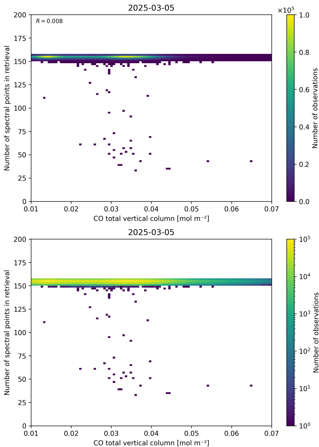
Figure 43: Scatter density plot of “CO total vertical column” against “Number of spectral points in retrieval” for 2025-03-04 to 2025-03-06.
