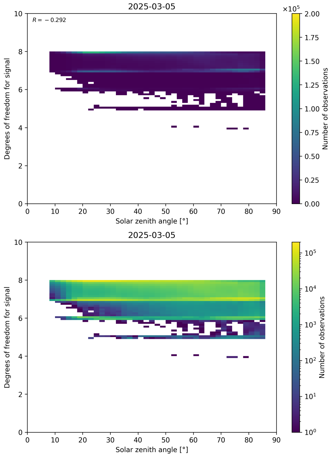
Figure 65: Scatter density plot of “Solar zenith angle” against “Degrees of freedom for signal” for 2025-03-04 to 2025-03-06.
