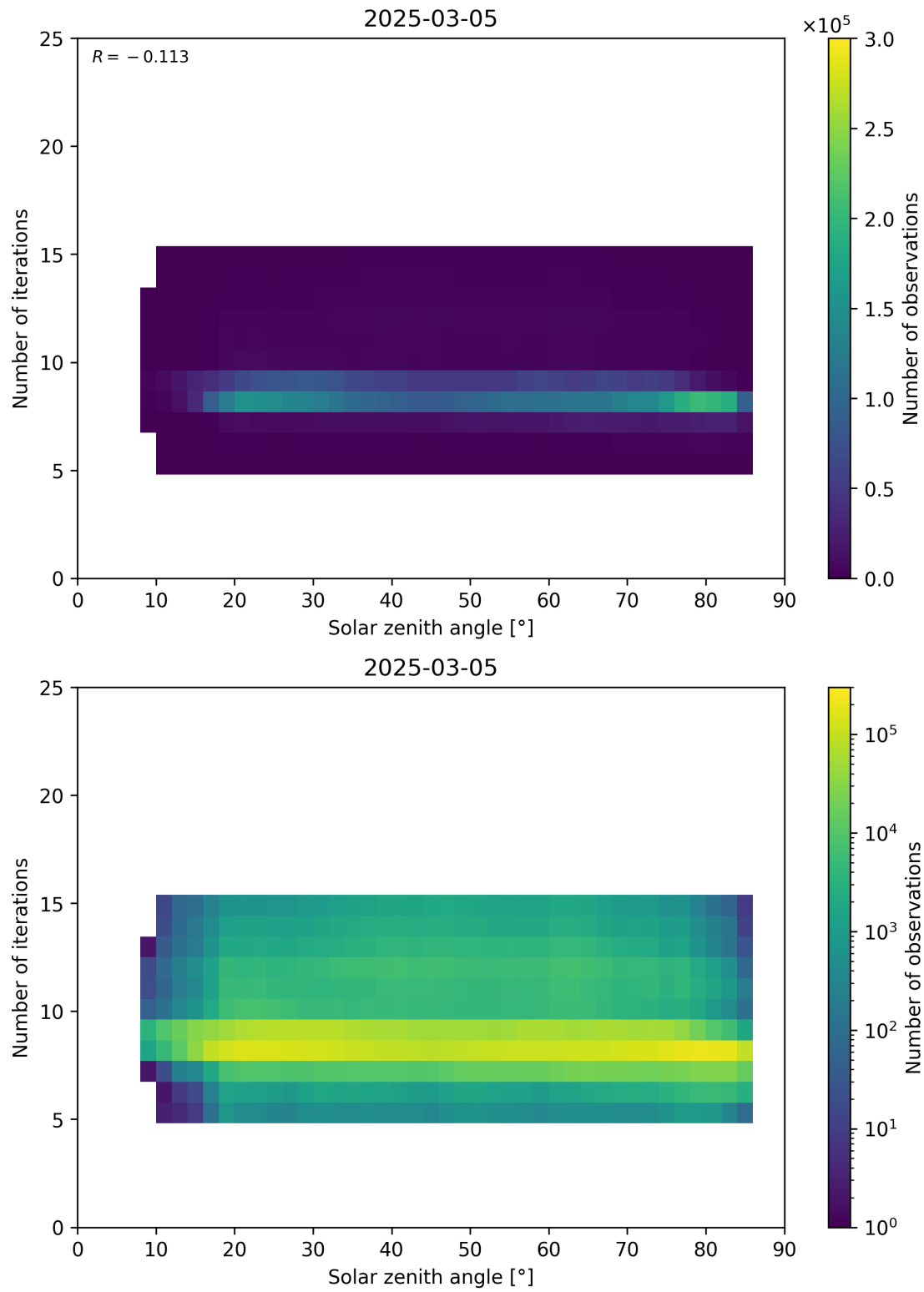
Figure 67: Scatter density plot of “Solar zenith angle” against “Number of iterations” for 2025-03-04 to 2025-03-06.
