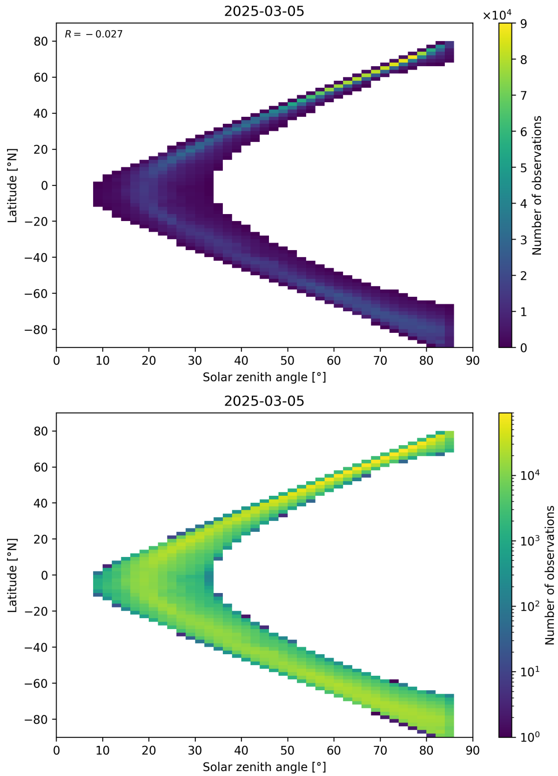
Figure 66: Scatter density plot of “Solar zenith angle” against “Latitude” for 2025-03-04 to 2025-03-06.
