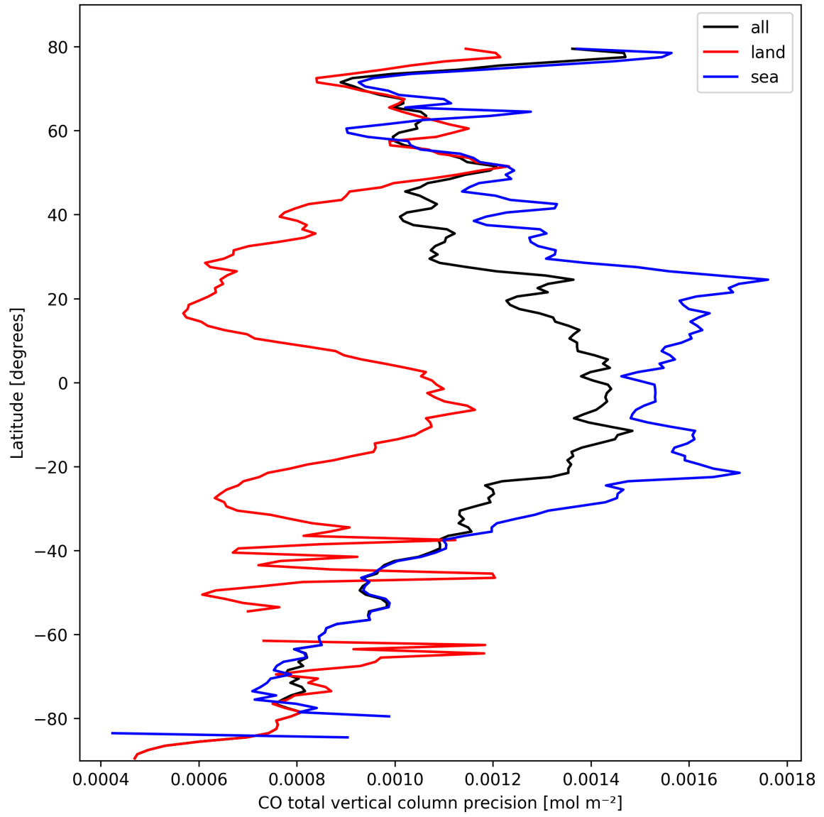
Figure 12: Zonal average of "CO total vertical column precision" for 2025-03-04 to 2025-03-06.
