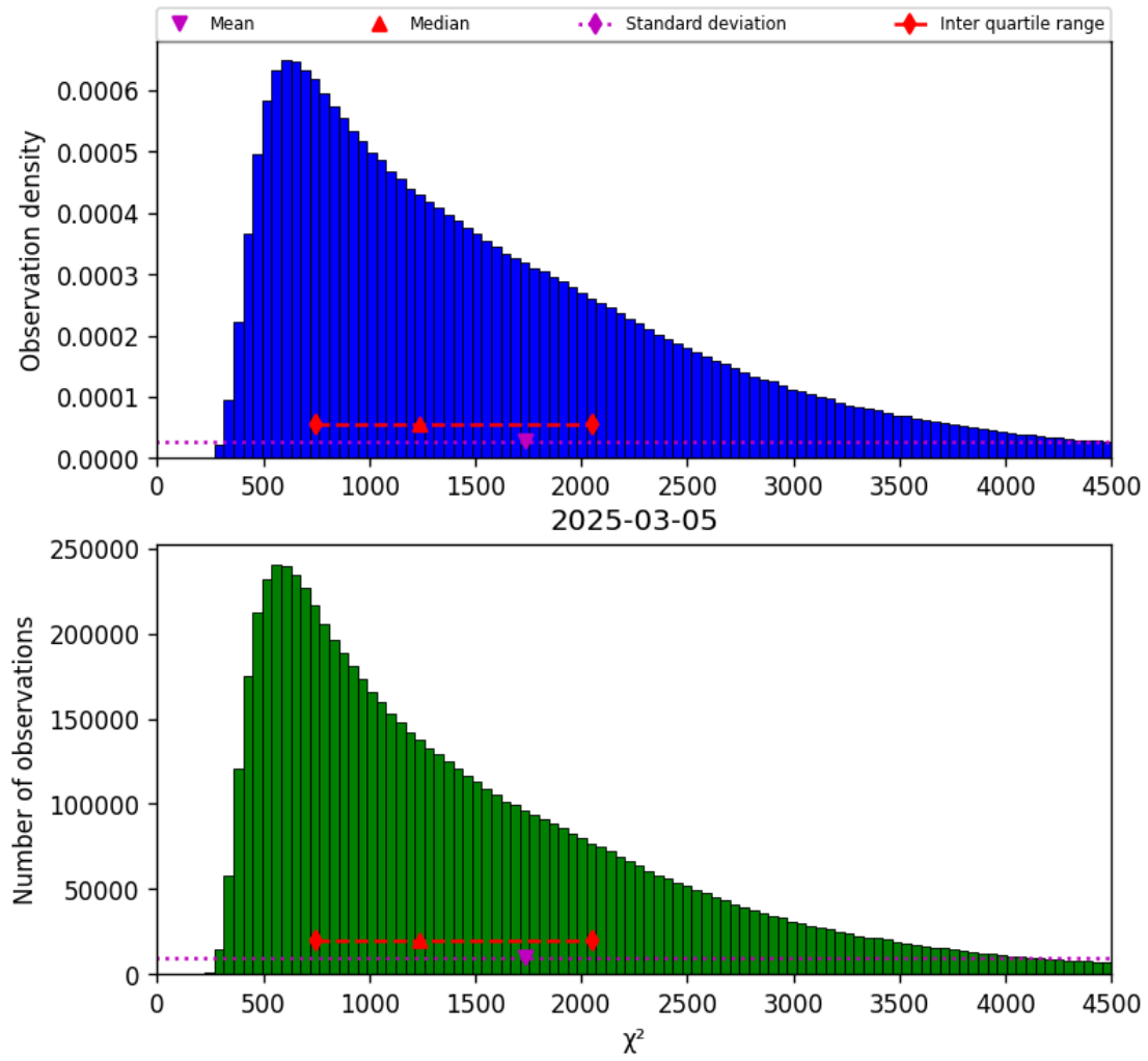
Figure 22: Histogram of “ \chi^2 ” for 2025-03-04 to 2025-03-06
