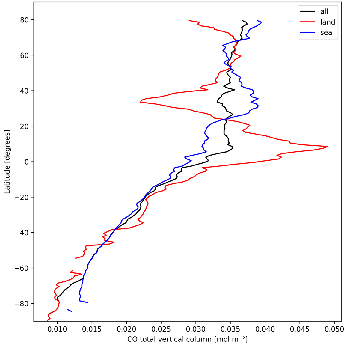
Figure 10: Zonal average of “CO total vertical column” for 2025-03-04 to 2025-03-06.
