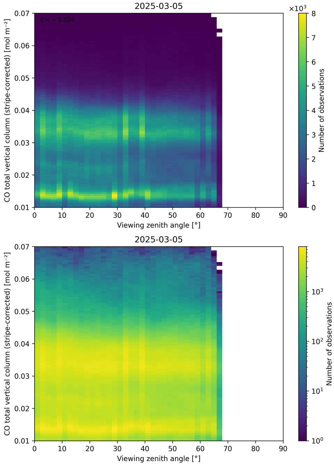
Figure 70: Scatter density plot of “Viewing zenith angle” against “CO total vertical column (stripe-corrected)” for 2025-03-04 to 2025-03-06.
