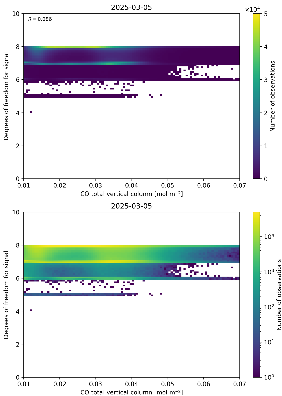
Figure 41: Scatter density plot of “CO total vertical column” against “Degrees of freedom for signal” for 2025-03-04 to 2025-03-06.
