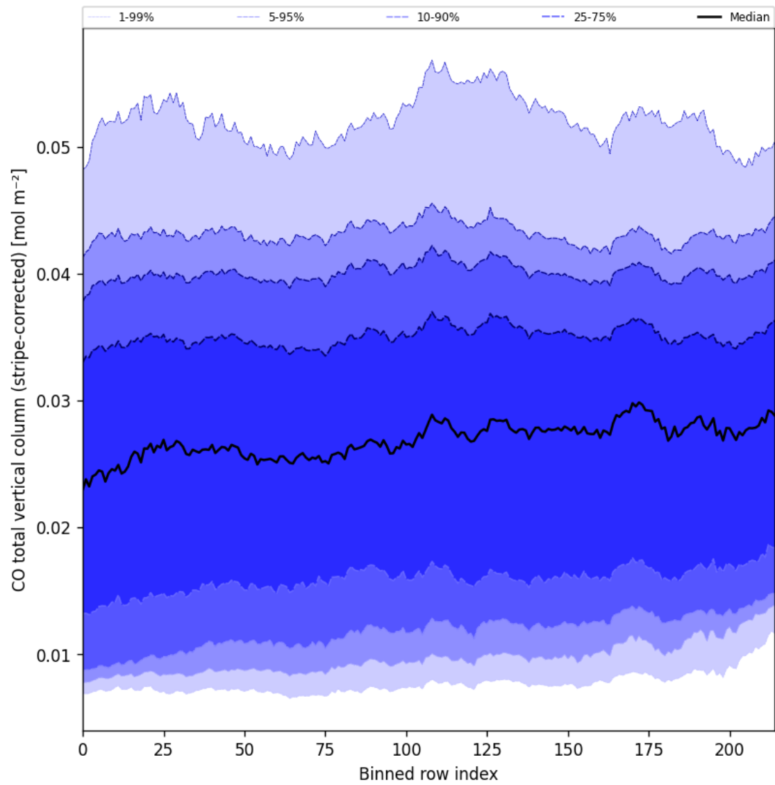
Figure 27: Along track statistics of “CO total vertical column (stripe-corrected)” for 2025-03-04 to 2025-03-06
