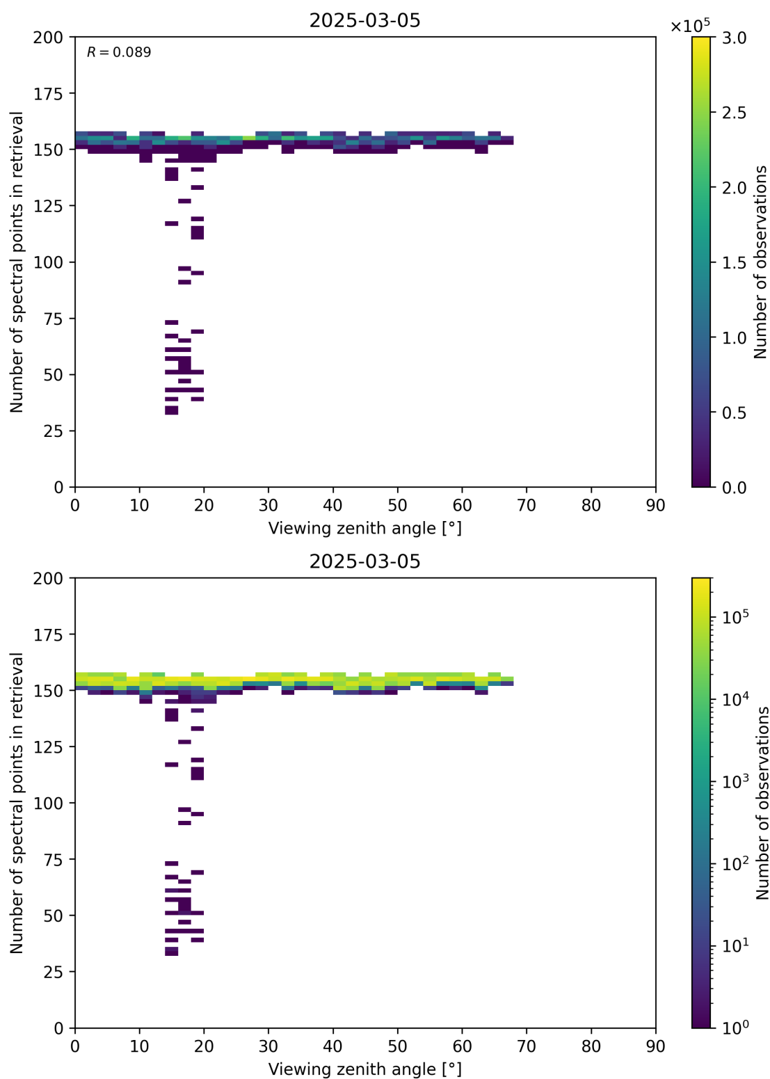
Figure 76: Scatter density plot of “Viewing zenith angle” against “Number of spectral points in retrieval” for 2025-03-04 to 2025-03-06.
