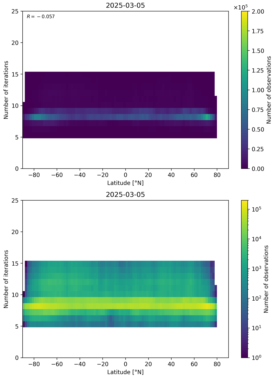
Figure 56: Scatter density plot of “Latitude” against “Number of iterations” for 2025-03-04 to 2025-03-06.
