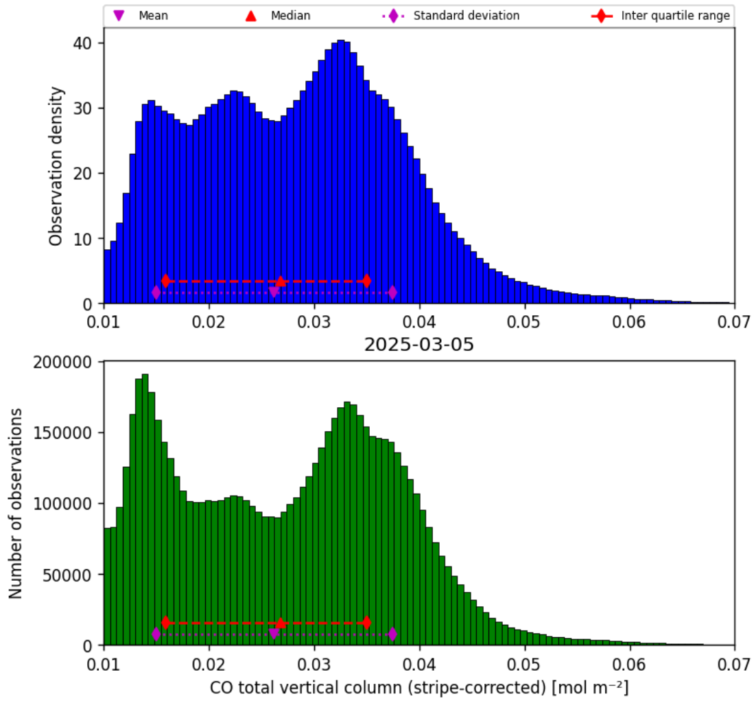
Figure 19: Histogram of “CO total vertical column (stripe-corrected)” for 2025-03-04 to 2025-03-06
