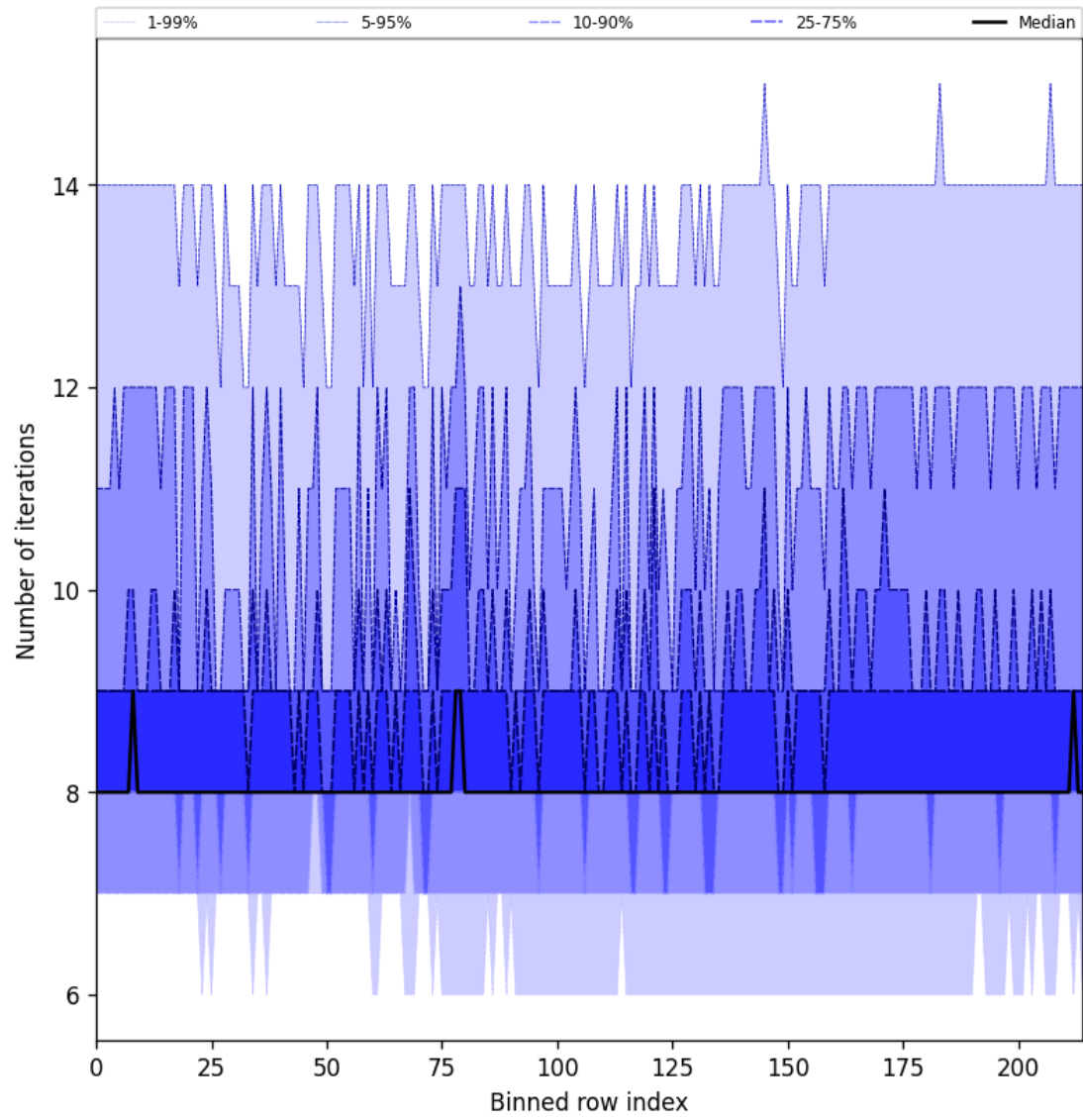
Figure 32: Along track statistics of “Number of iterations” for 2025-03-04 to 2025-03-06
