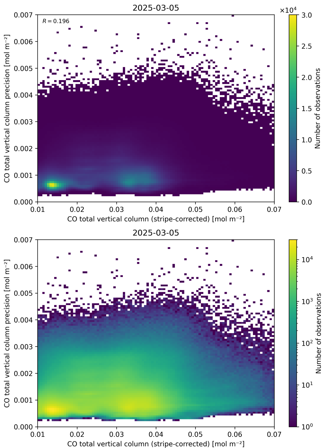
Figure 36: Scatter density plot of “CO total vertical column (stripe-corrected)” against “CO total vertical column precision” for 2025-03-04 to 2025-03-06.
