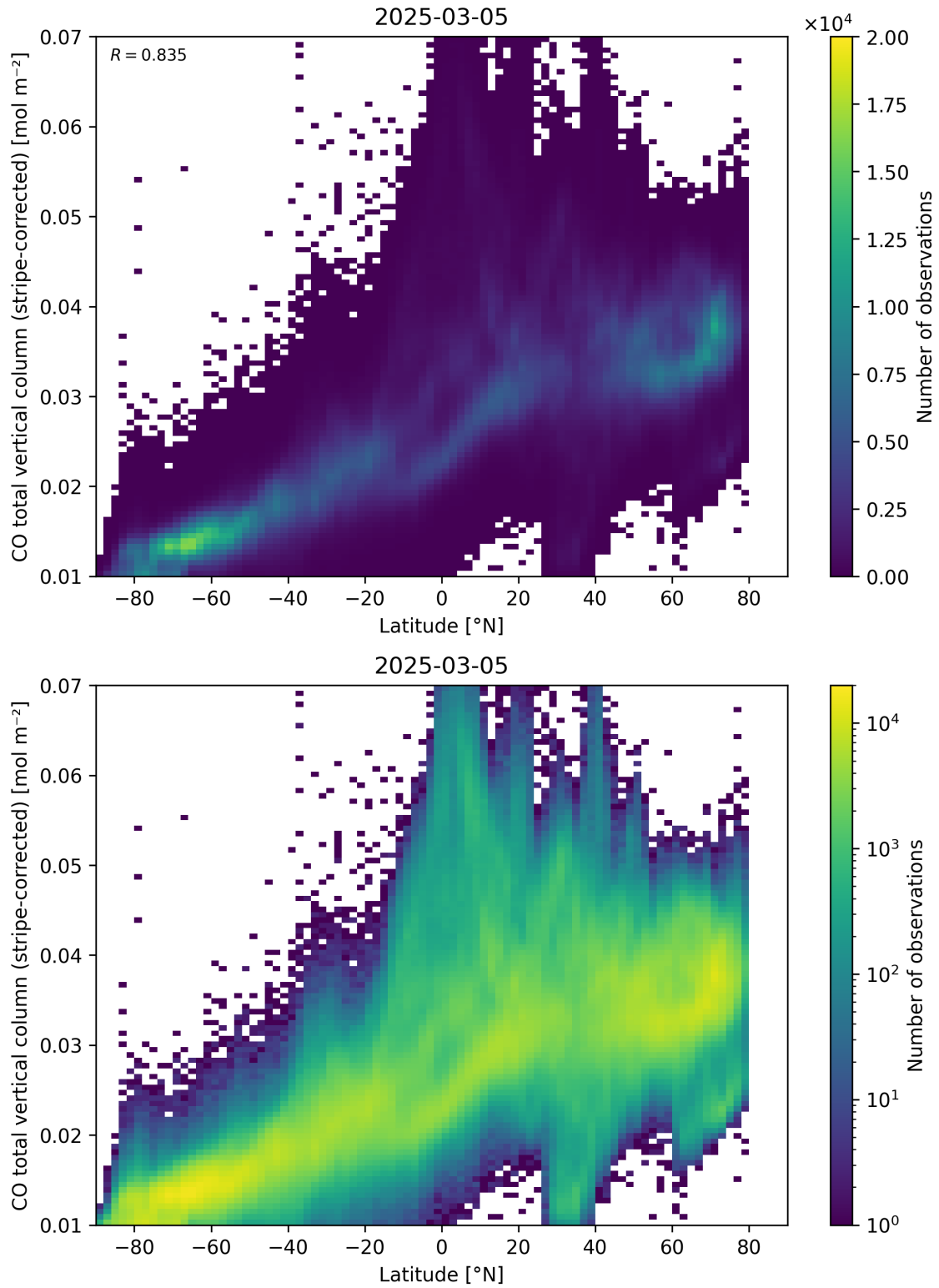
Figure 52: Scatter density plot of “Latitude” against “CO total vertical column (stripe-corrected)” for 2025-03-04 to 2025-03-06.
