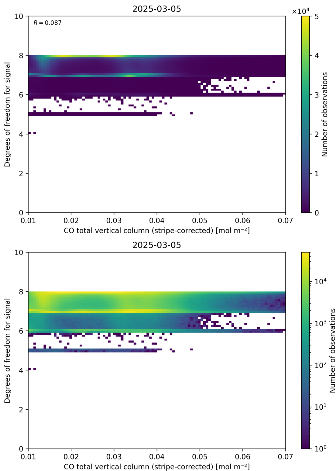
Figure 38: Scatter density plot of “CO total vertical column (stripe-corrected)” against “Degrees of freedom for signal” for 2025-03-04 to 2025-03-06.
