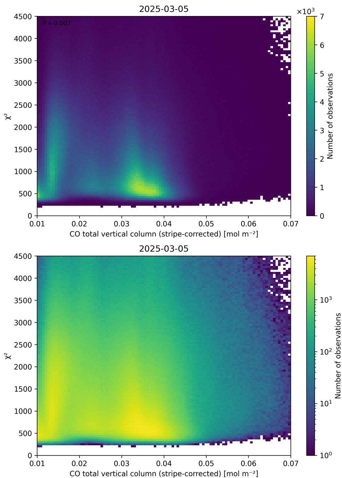
Figure 37: Scatter density plot of “CO total vertical column (stripe-corrected)” against “ \chi^2 ” for 2025-03-04 to 2025-03-06.
