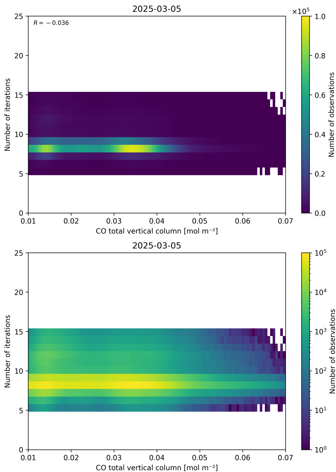
Figure 42: Scatter density plot of “CO total vertical column” against “Number of iterations” for 2025-03-04 to 2025-03-06.
