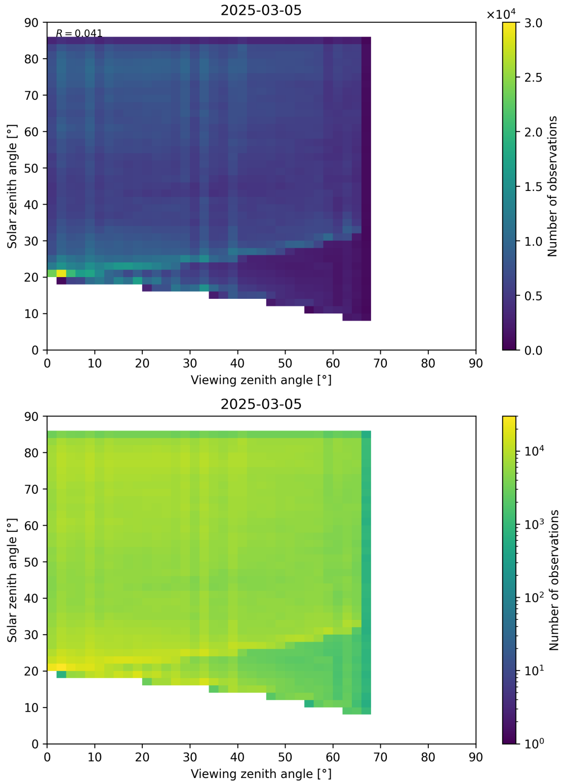
Figure 77: Scatter density plot of “Viewing zenith angle” against “Solar zenith angle” for 2025-03-04 to 2025-03-06.
