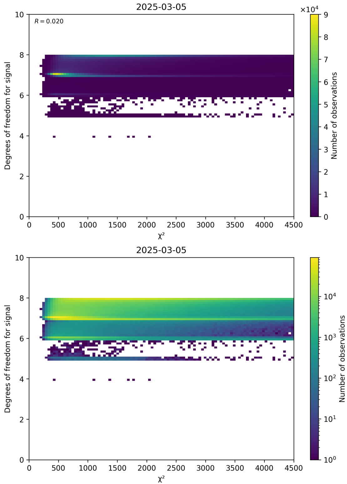
Figure 48: Scatter density plot of “ \chi^2 ” against “Degrees of freedom for signal” for 2025-03-04 to 2025-03-06.
