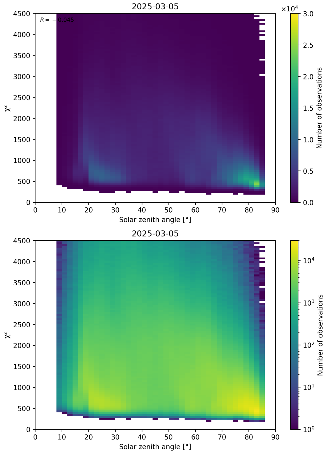
Figure 64: Scatter density plot of “Solar zenith angle” against “ \chi^2 ” for 2025-03-04 to 2025-03-06.
