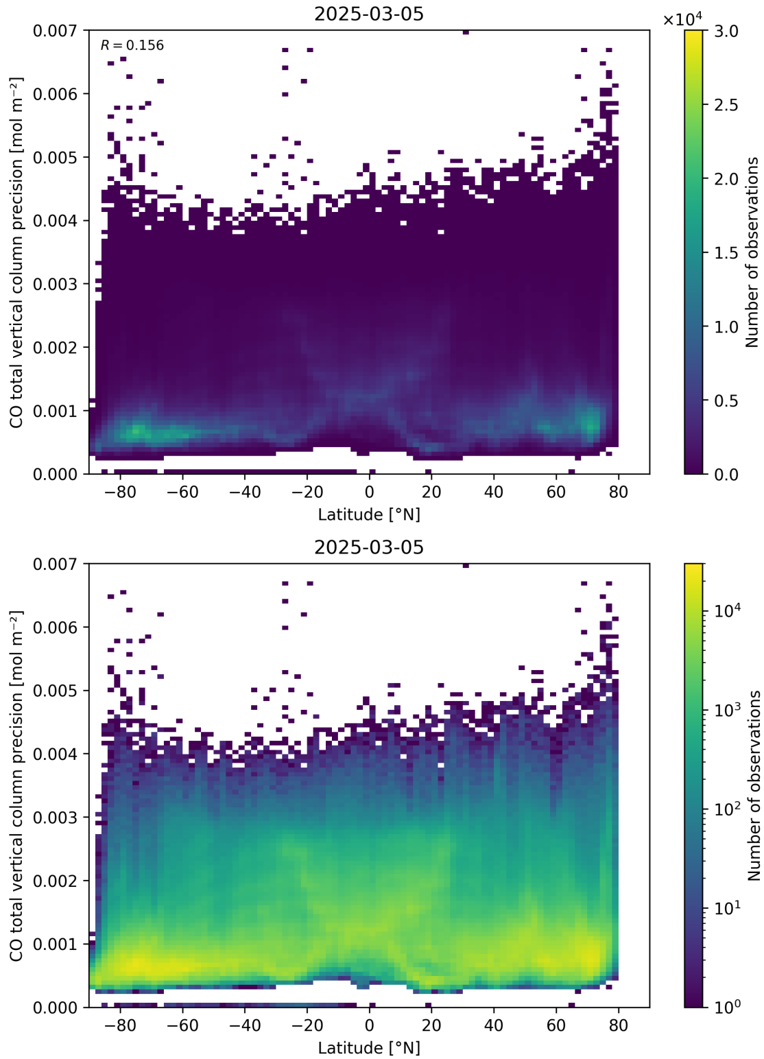
Figure 53: Scatter density plot of “Latitude” against “CO total vertical column precision” for 2025-03-04 to 2025-03-06.
