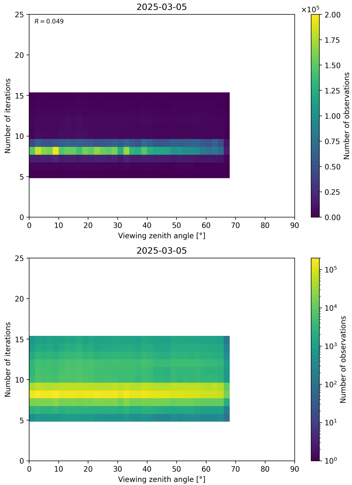
Figure 75: Scatter density plot of “Viewing zenith angle” against “Number of iterations” for 2025-03-04 to 2025-03-06.
