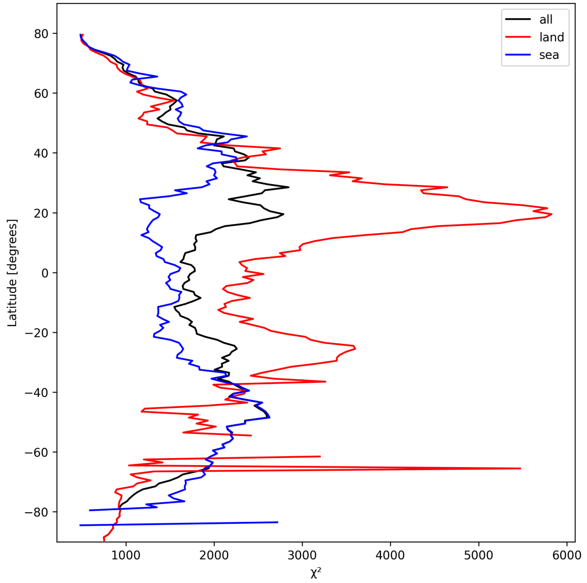
Figure 14: Zonal average of “ \chi^2 ” for 2025-03-04 to 2025-03-06.
