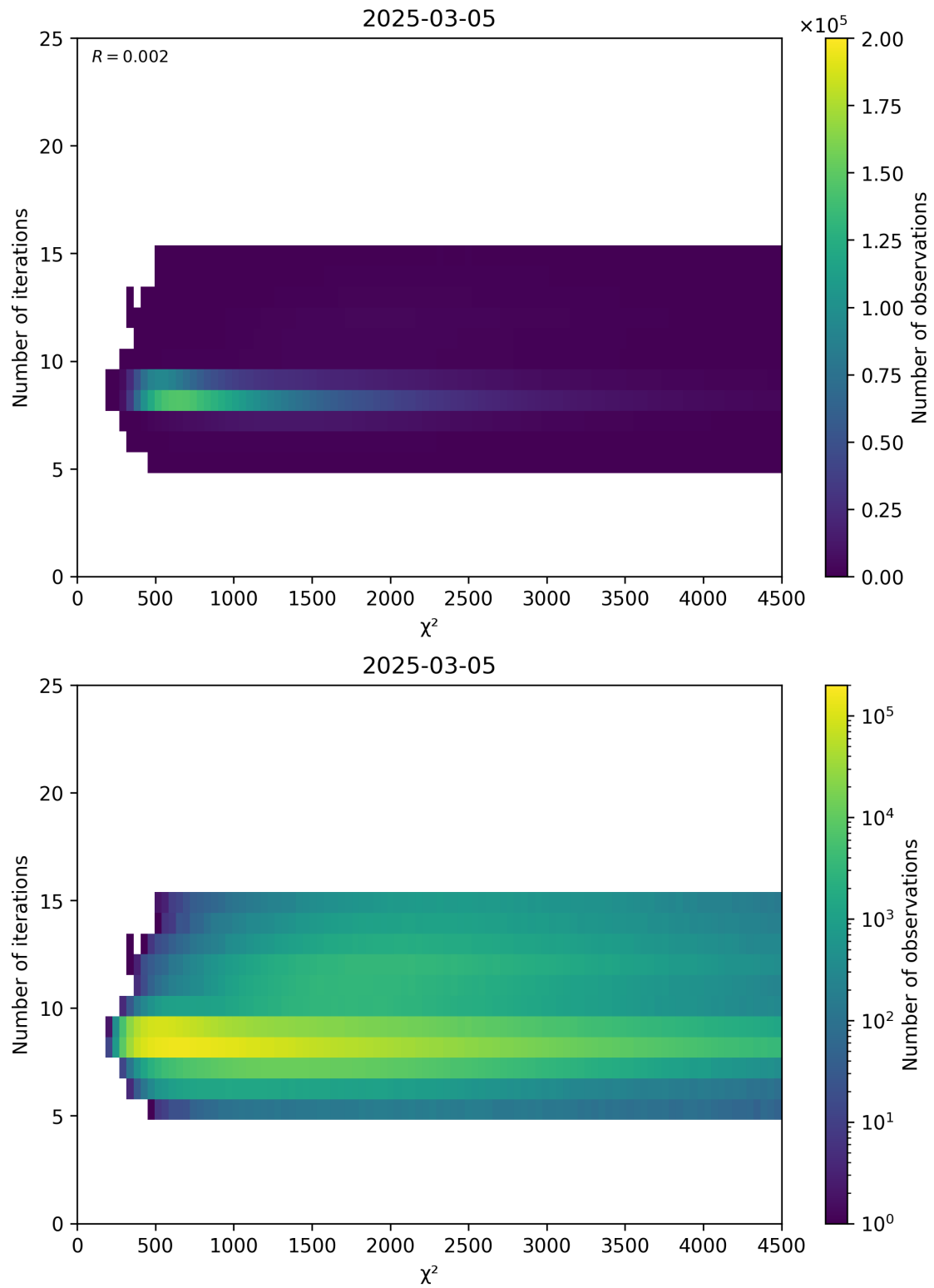
Figure 49: Scatter density plot of “ \chi^2 ” against “Number of iterations” for 2025-03-04 to 2025-03-06.
