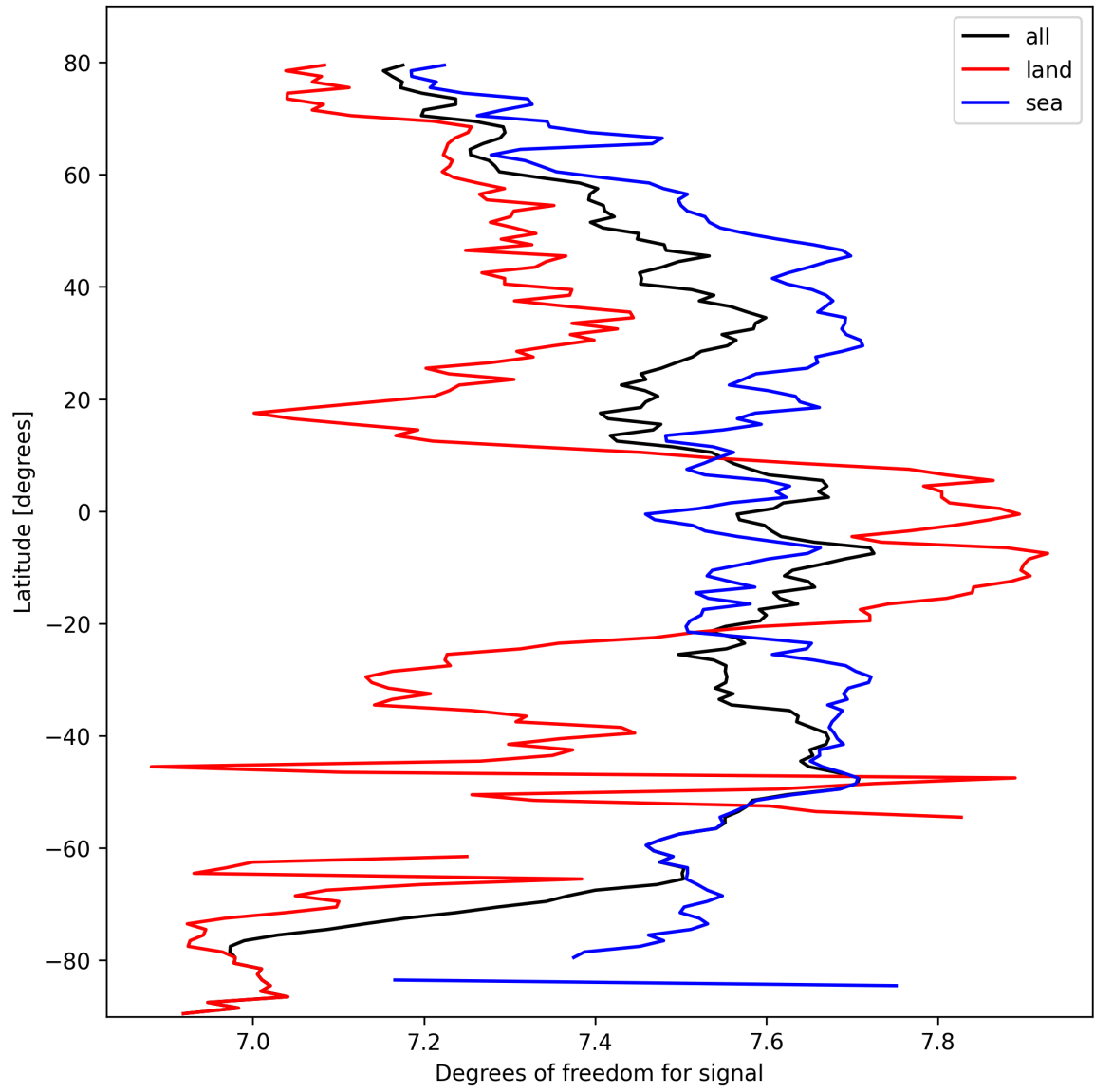
Figure 15: Zonal average of “Degrees of freedom for signal” for 2025-03-04 to 2025-03-06.
