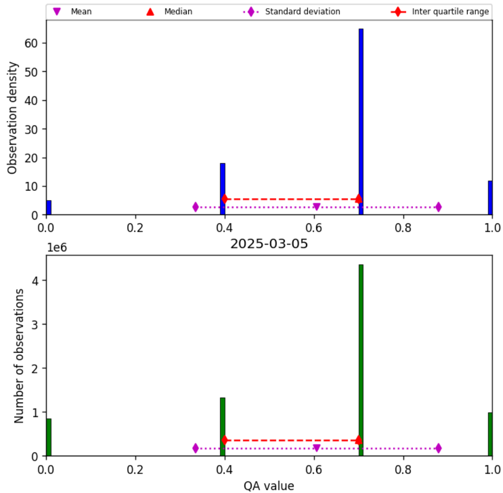
Figure 17: Histogram of “QA value” for 2025-03-04 to 2025-03-06
