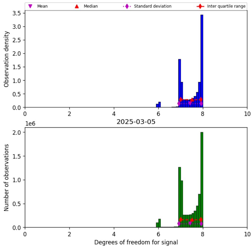
Figure 23: Histogram of “Degrees of freedom for signal” for 2025-03-04 to 2025-03-06
