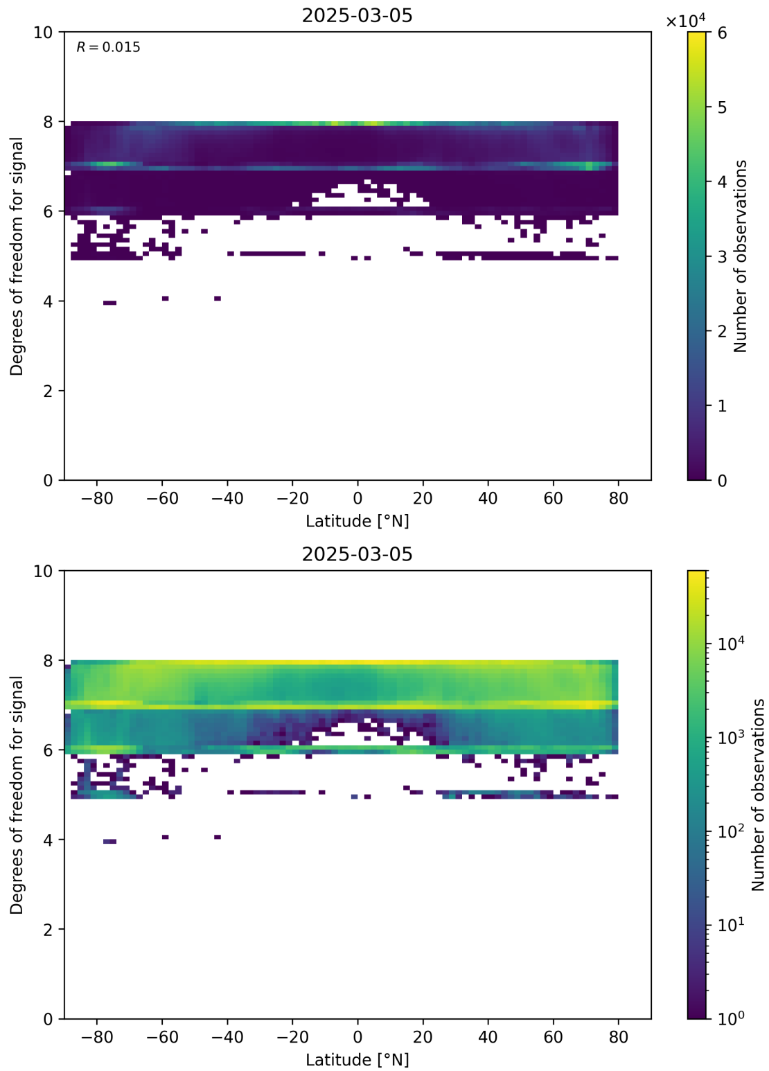
Figure 55: Scatter density plot of “Latitude” against “Degrees of freedom for signal” for 2025-03-04 to 2025-03-06.
