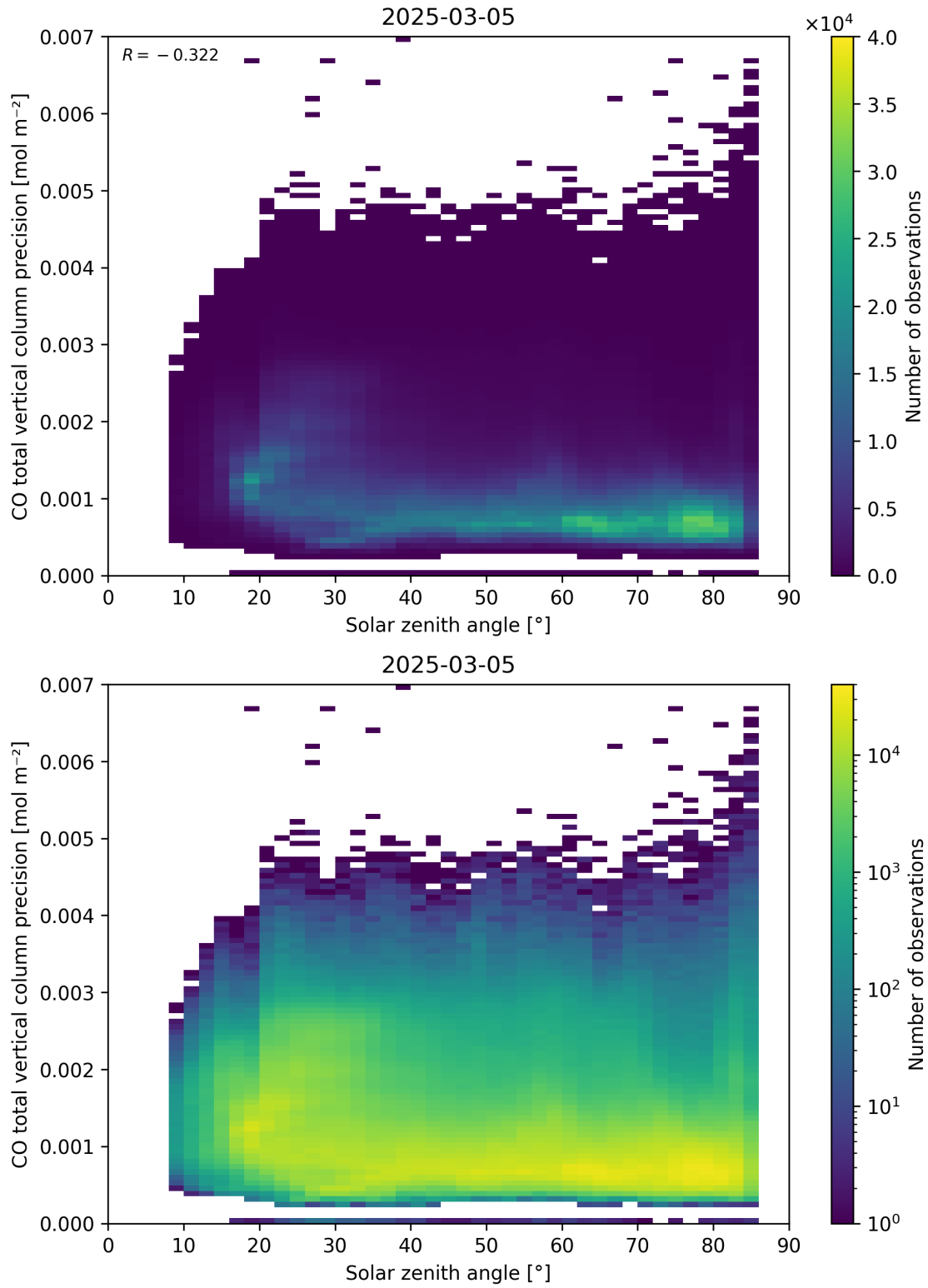
Figure 63: Scatter density plot of “Solar zenith angle” against “CO total vertical column precision” for 2025-03-04 to 2025-03-06.
