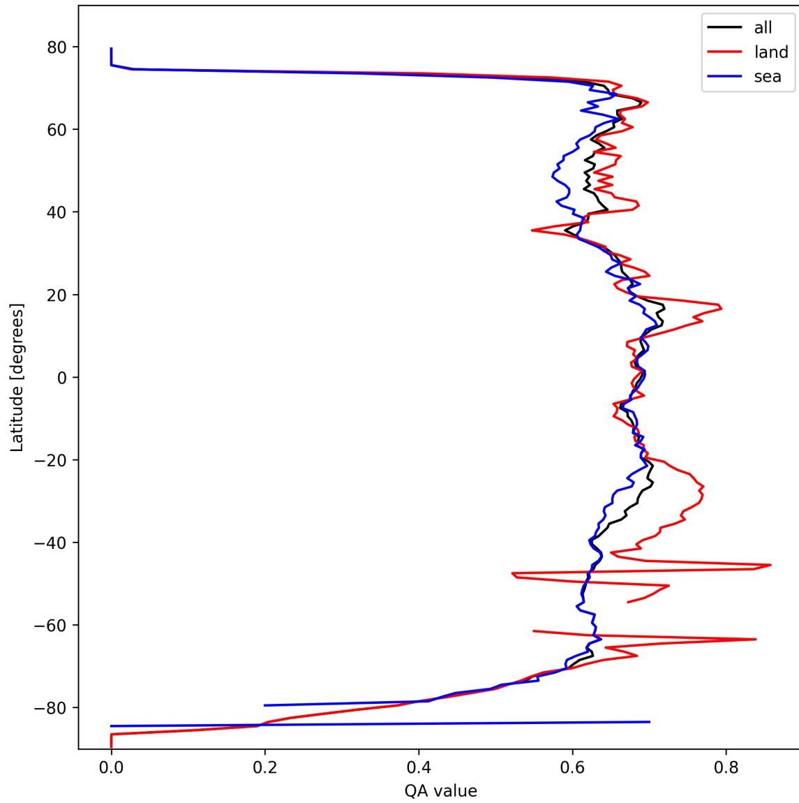
Figure 9: Zonal average of “QA value” for 2025-03-04 to 2025-03-06.
