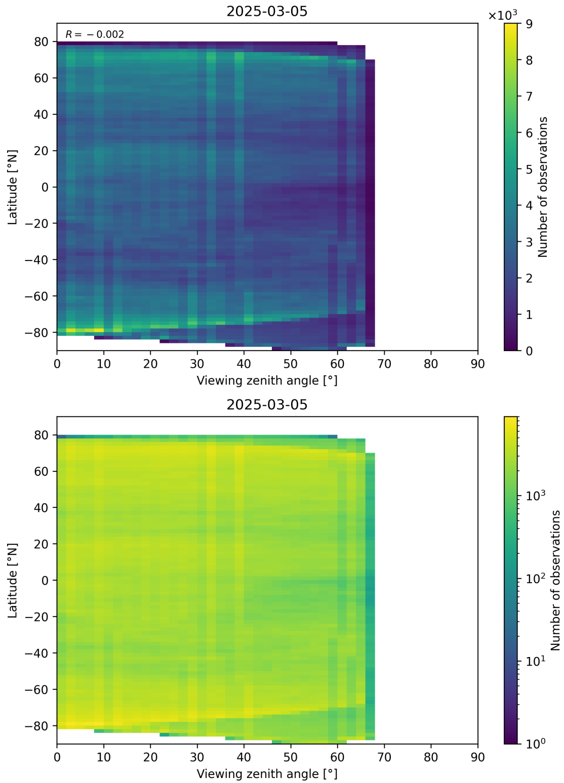
Figure 74: Scatter density plot of “Viewing zenith angle” against “Latitude” for 2025-03-04 to 2025-03-06.
