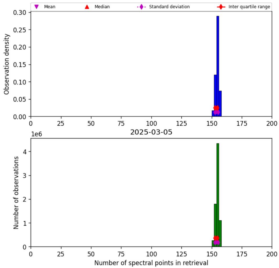
Figure 21: Histogram of “Number of spectral points in retrieval” for 2025-03-04 to 2025-03-06
