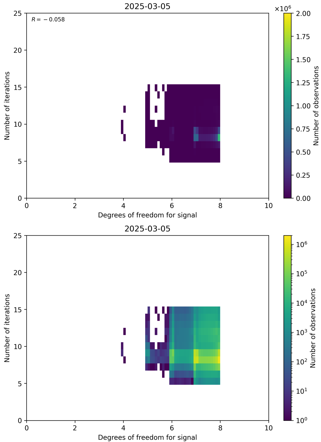
Figure 50: Scatter density plot of “Degrees of freedom for signal” against “Number of iterations” for 2025-03-04 to 2025-03-06.
