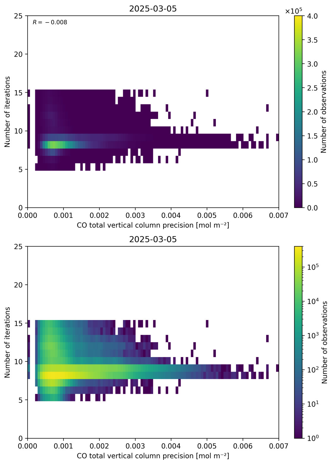
Figure 46: Scatter density plot of “CO total vertical column precision” against “Number of iterations” for 2025-03-04 to 2025-03-06.
