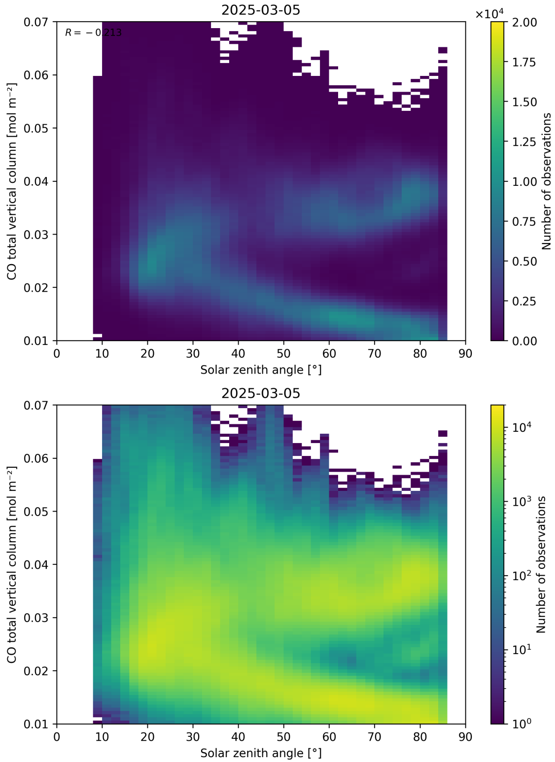
Figure 61: Scatter density plot of “Solar zenith angle” against “CO total vertical column” for 2025-03-04 to 2025-03-06.
