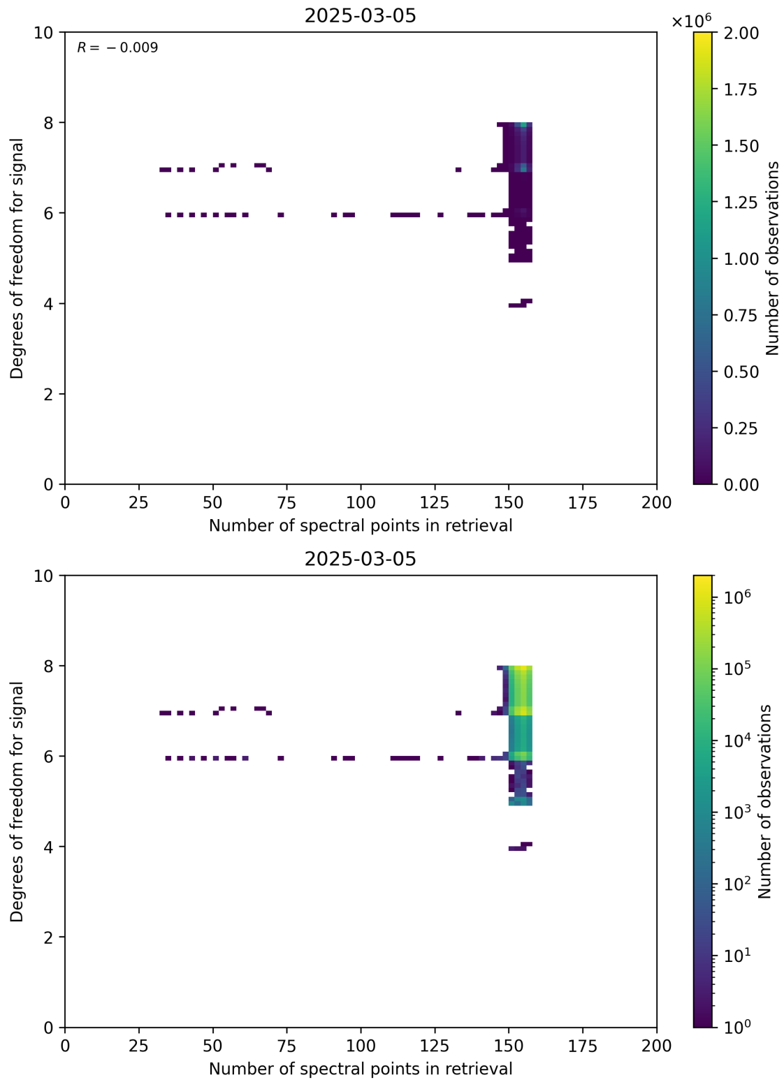
Figure 59: Scatter density plot of “Number of spectral points in retrieval” against “Degrees of freedom for signal” for 2025-03-04 to 2025-03-06.
