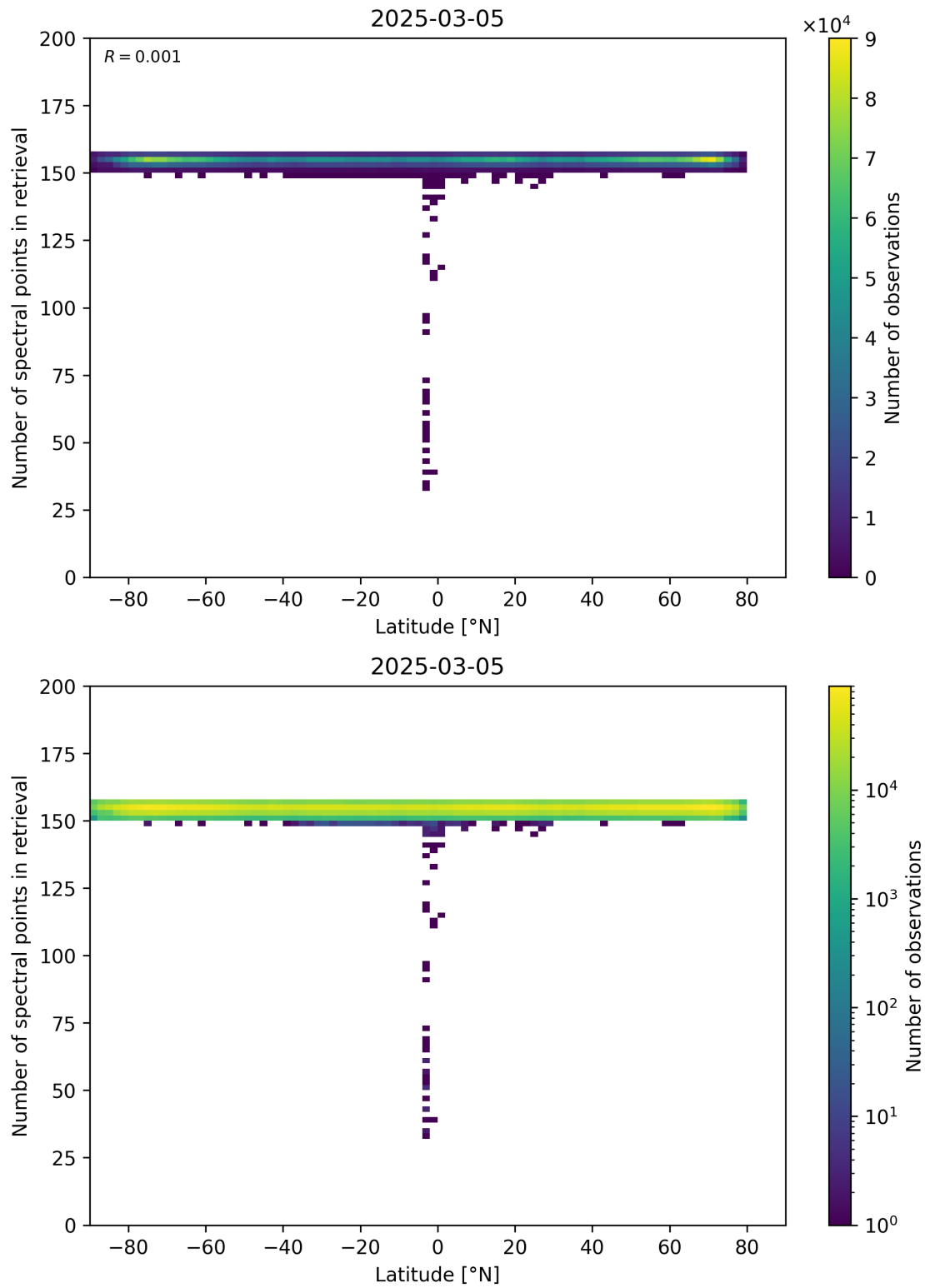
Figure 57: Scatter density plot of “Latitude” against “Number of spectral points in retrieval” for 2025-03-04 to 2025-03-06.
