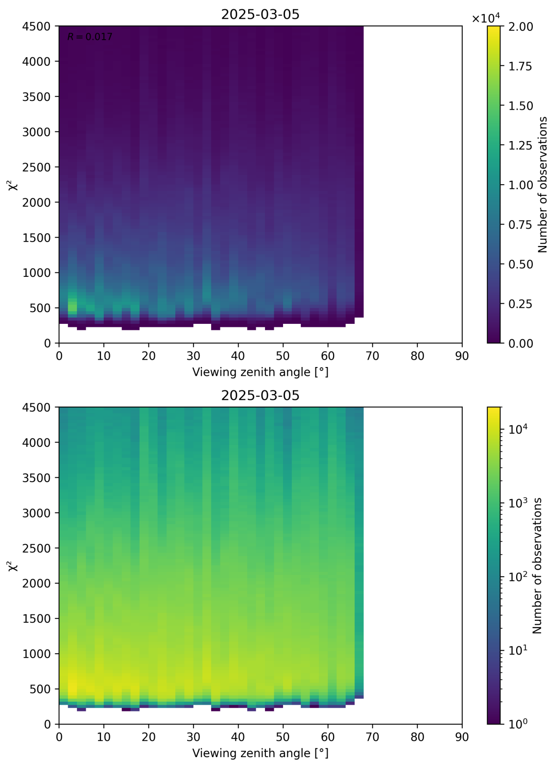
Figure 72: Scatter density plot of “Viewing zenith angle” against “ \chi^2 ” for 2025-03-04 to 2025-03-06.
