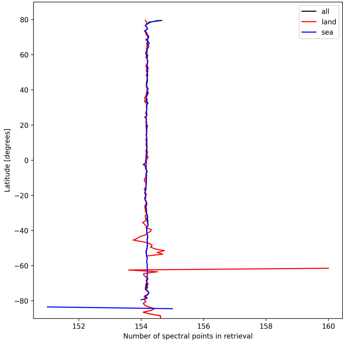
Figure 13: Zonal average of “Number of spectral points in retrieval” for 2025-03-04 to 2025-03-06.
