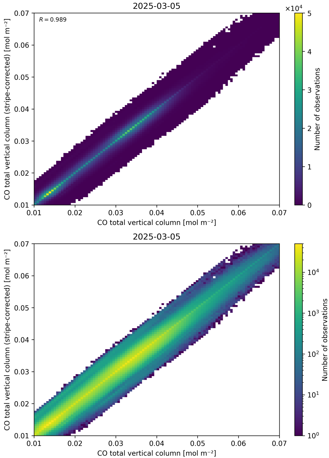
Figure 33: Scatter density plot of “CO total vertical column” against “CO total vertical column (stripe-corrected)” for 2025-03-04 to 2025-03-06.
