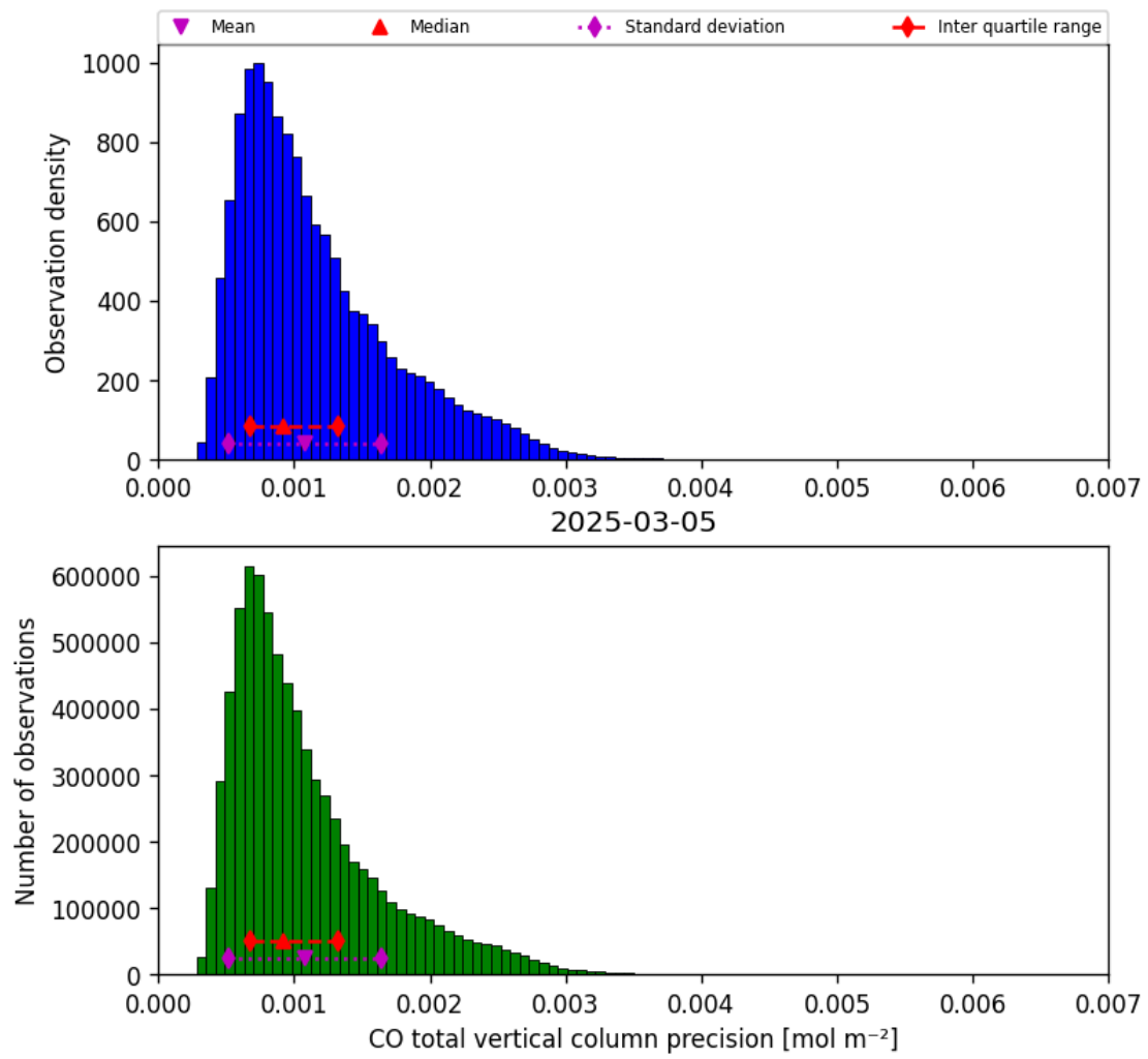
Figure 20: Histogram of “CO total vertical column precision” for 2025-03-04 to 2025-03-06
