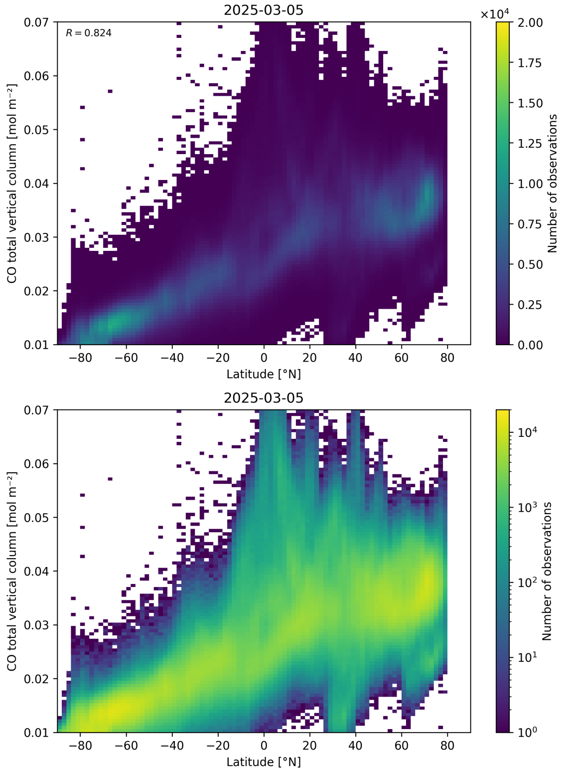
Figure 51: Scatter density plot of “Latitude” against “CO total vertical column” for 2025-03-04 to 2025-03-06.
