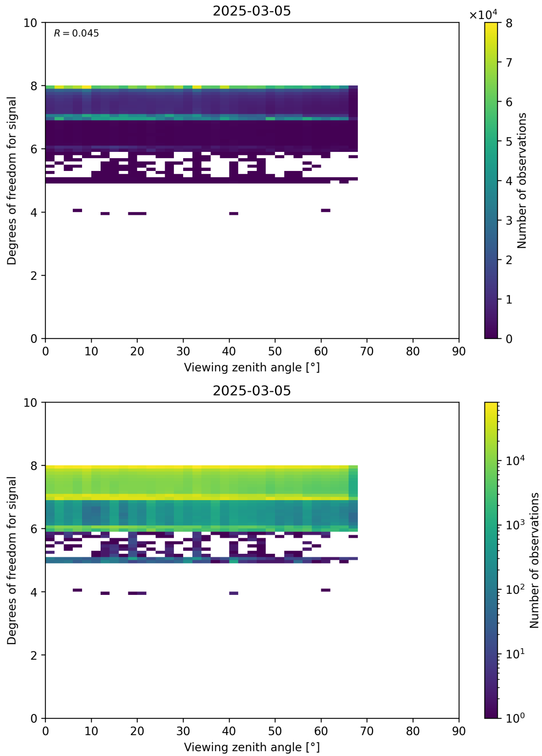
Figure 73: Scatter density plot of “Viewing zenith angle” against “Degrees of freedom for signal” for 2025-03-04 to 2025-03-06.
