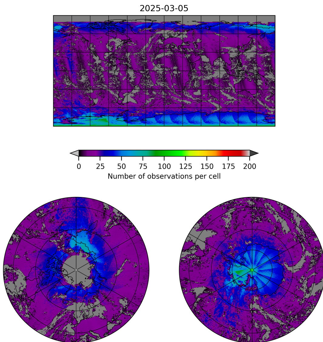
Figure 8: Map of the number of observations for 2025-03-04 to 2025-03-06
