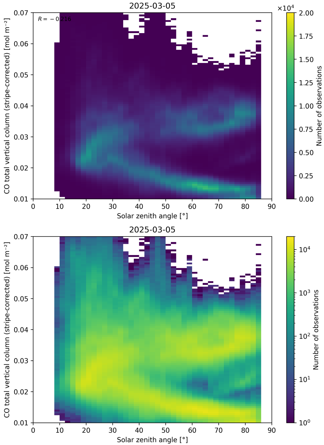
Figure 62: Scatter density plot of “Solar zenith angle” against “CO total vertical column (stripe-corrected)” for 2025-03-04 to 2025-03-06.
