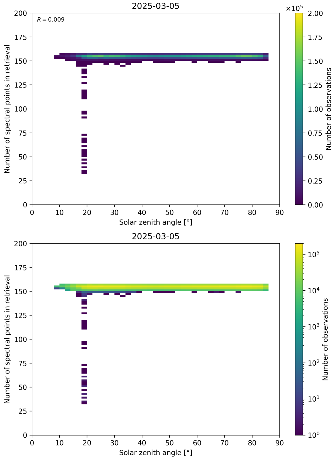
Figure 68: Scatter density plot of “Solar zenith angle” against “Number of spectral points in retrieval” for 2025-03-04 to 2025-03-06.
