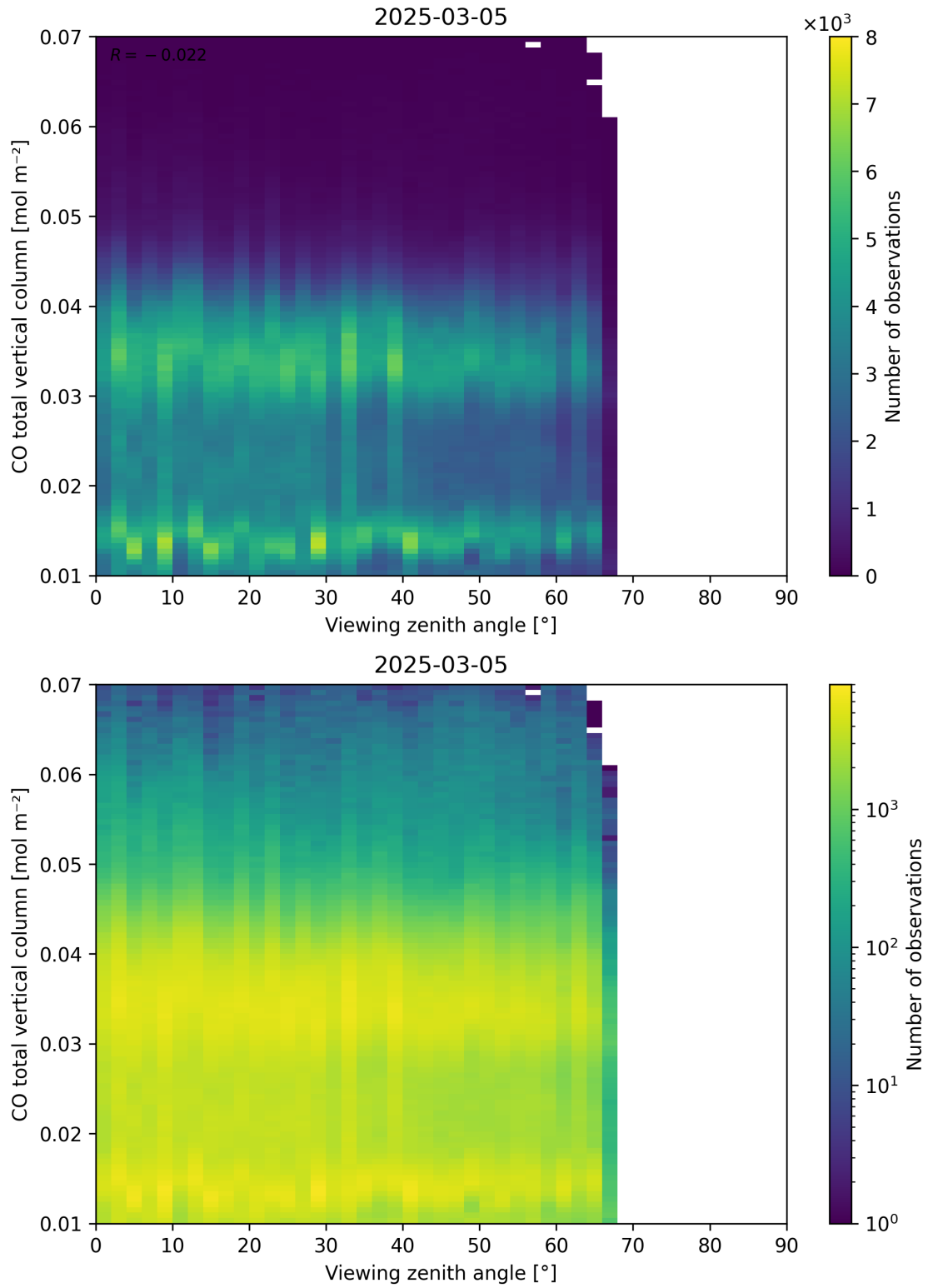
Figure 69: Scatter density plot of “Viewing zenith angle” against “CO total vertical column” for 2025-03-04 to 2025-03-06.
