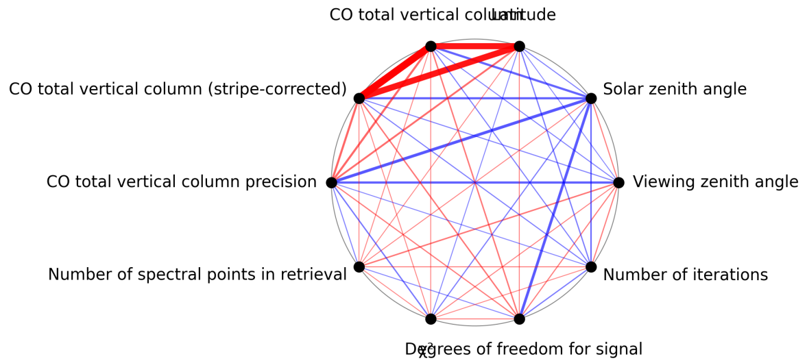
Figure 1: Map of correlation graph for 2025-03-04 to 2025-03-06.
