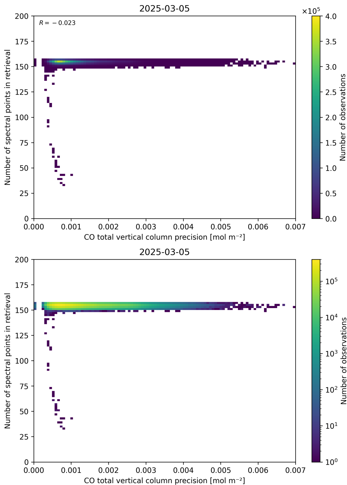
Figure 47: Scatter density plot of “CO total vertical column precision” against “Number of spectral points in retrieval” for 2025-03-04 to 2025-03-06.
