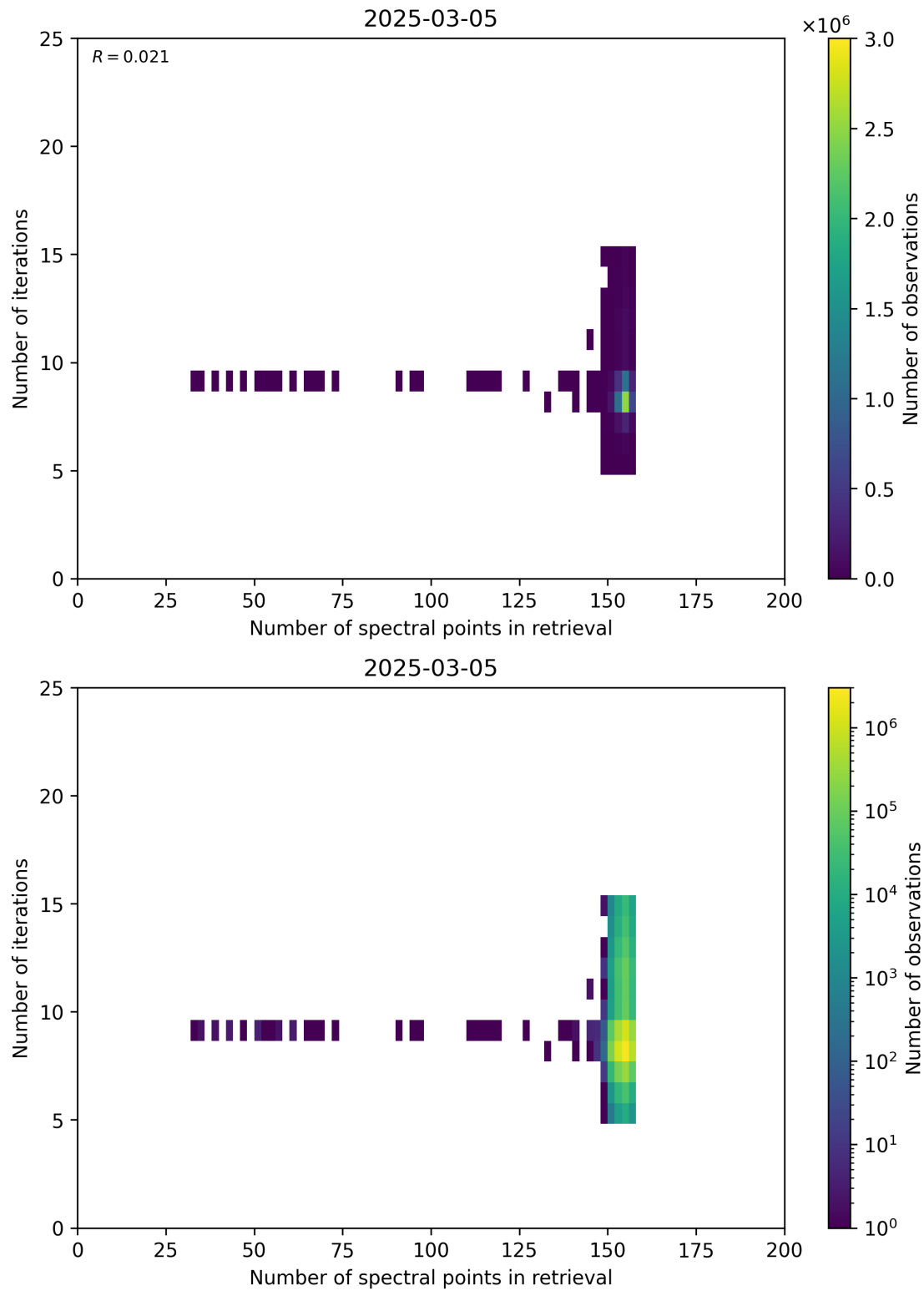
Figure 60: Scatter density plot of “Number of spectral points in retrieval” against “Number of iterations” for 2025-03-04 to 2025-03-06.
