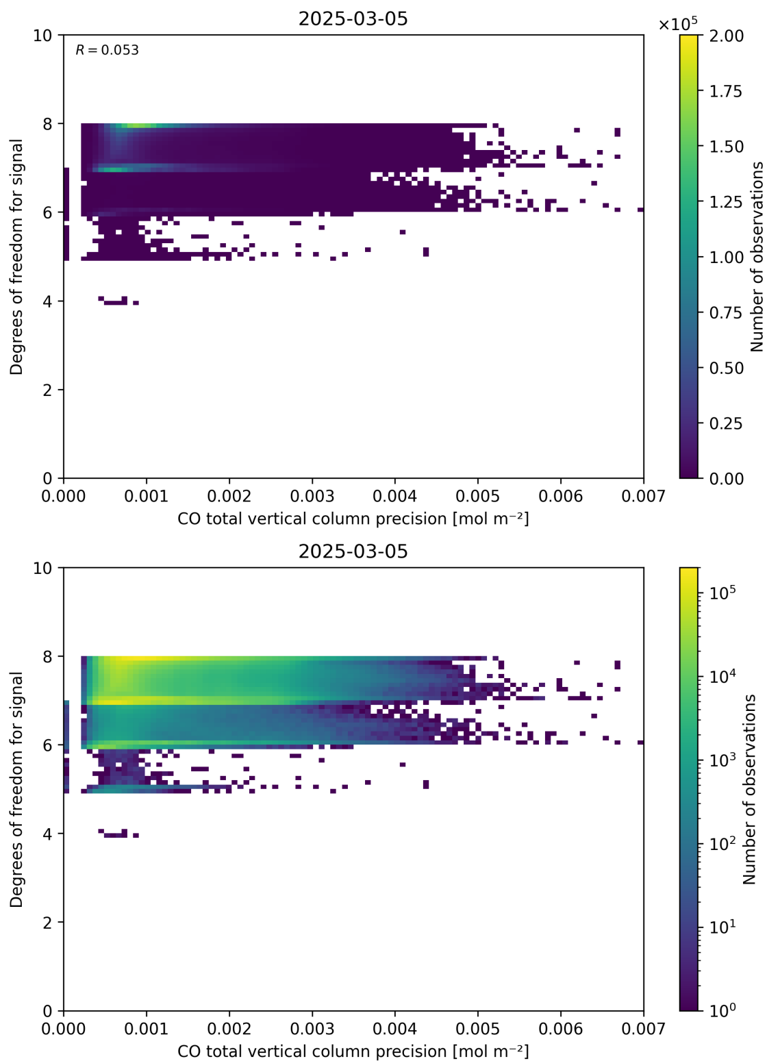
Figure 45: Scatter density plot of “CO total vertical column precision” against “Degrees of freedom for signal” for 2025-03-04 to 2025-03-06.
