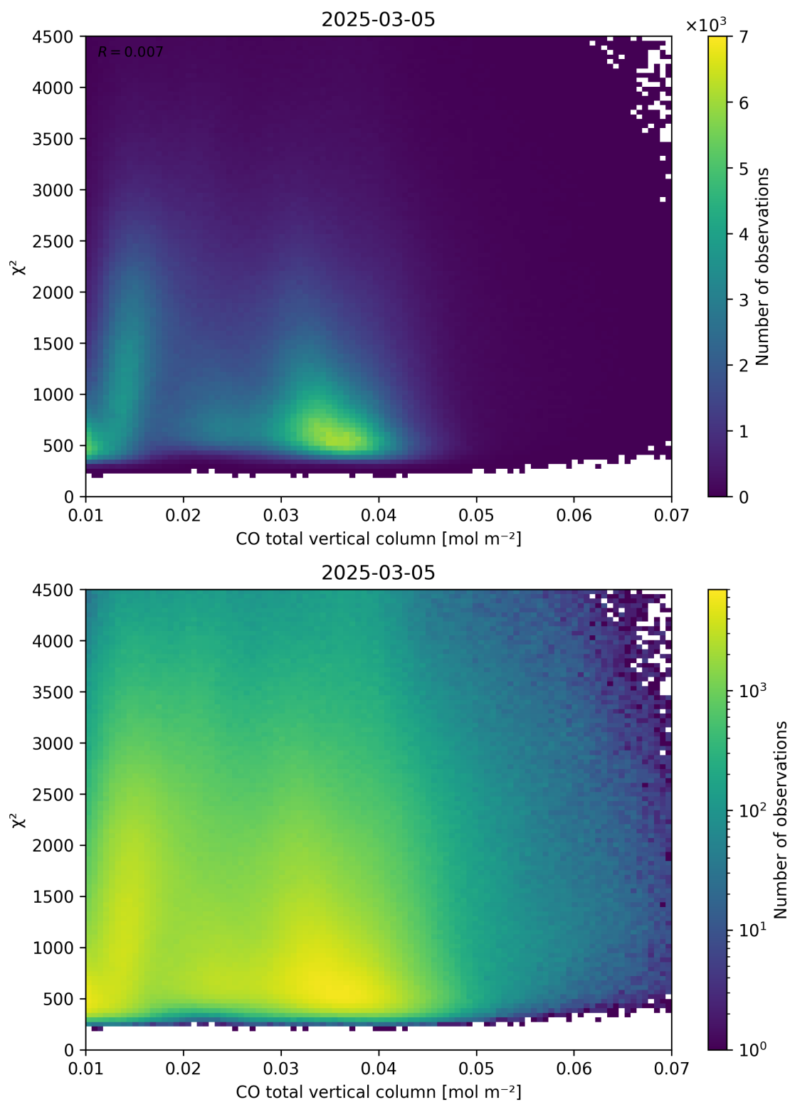
Figure 35: Scatter density plot of “CO total vertical column” against “ \chi^2 ” for 2025-03-04 to 2025-03-06.
