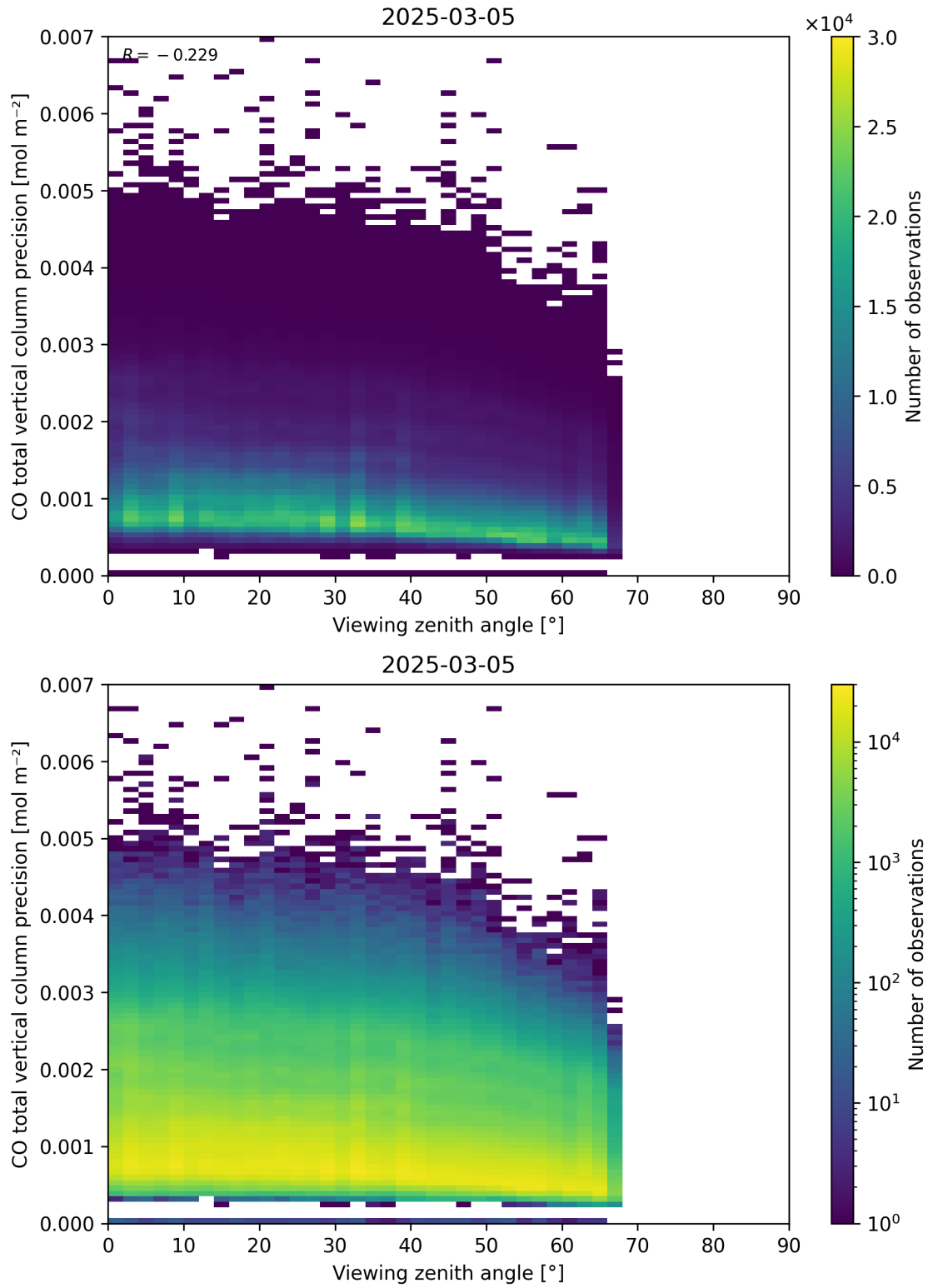
Figure 71: Scatter density plot of “Viewing zenith angle” against “CO total vertical column precision” for 2025-03-04 to 2025-03-06.
