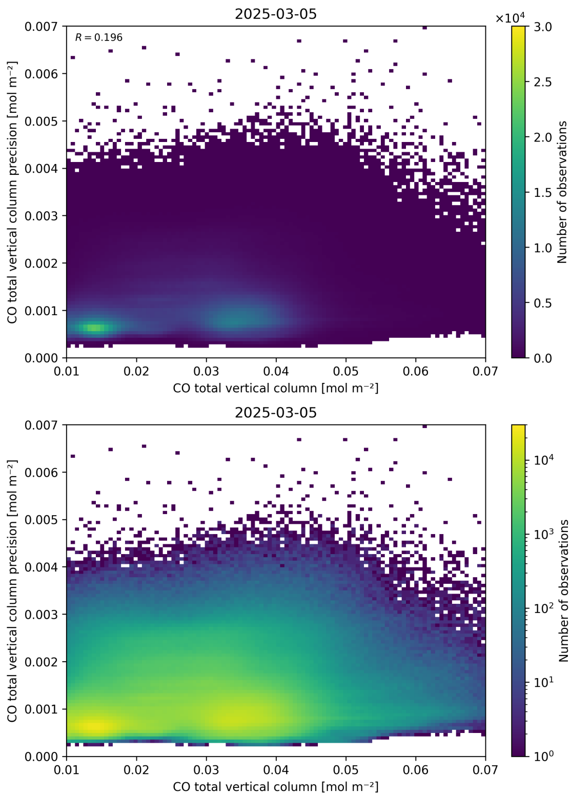
Figure 34: Scatter density plot of “CO total vertical column” against “CO total vertical column precision” for 2025-03-04 to 2025-03-06.
