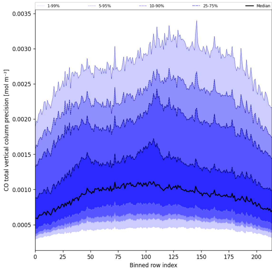
Figure 28: Along track statistics of “CO total vertical column precision” for 2025-03-04 to 2025-03-06
