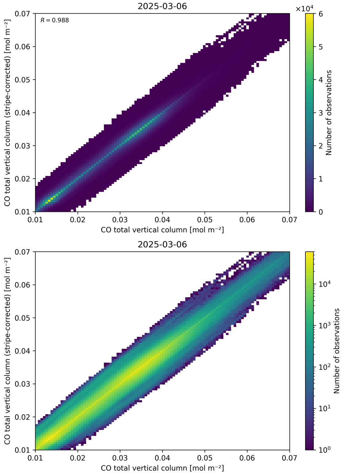
Figure 33: Scatter density plot of “CO total vertical column” against “CO total vertical column (stripe-corrected)” for 2025-03-05 to 2025-03-07.
