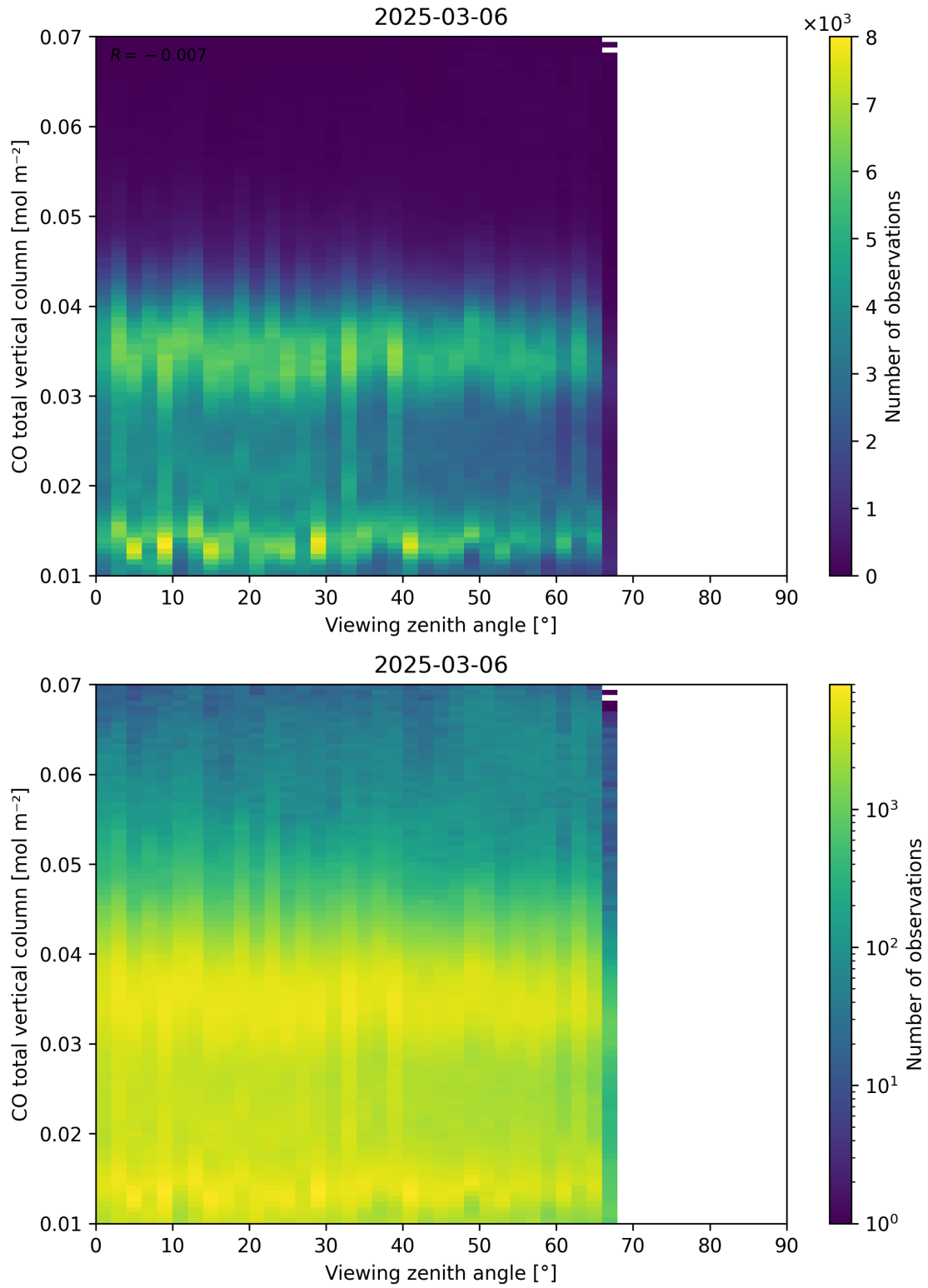
Figure 69: Scatter density plot of “Viewing zenith angle” against “CO total vertical column” for 2025-03-05 to 2025-03-07.
