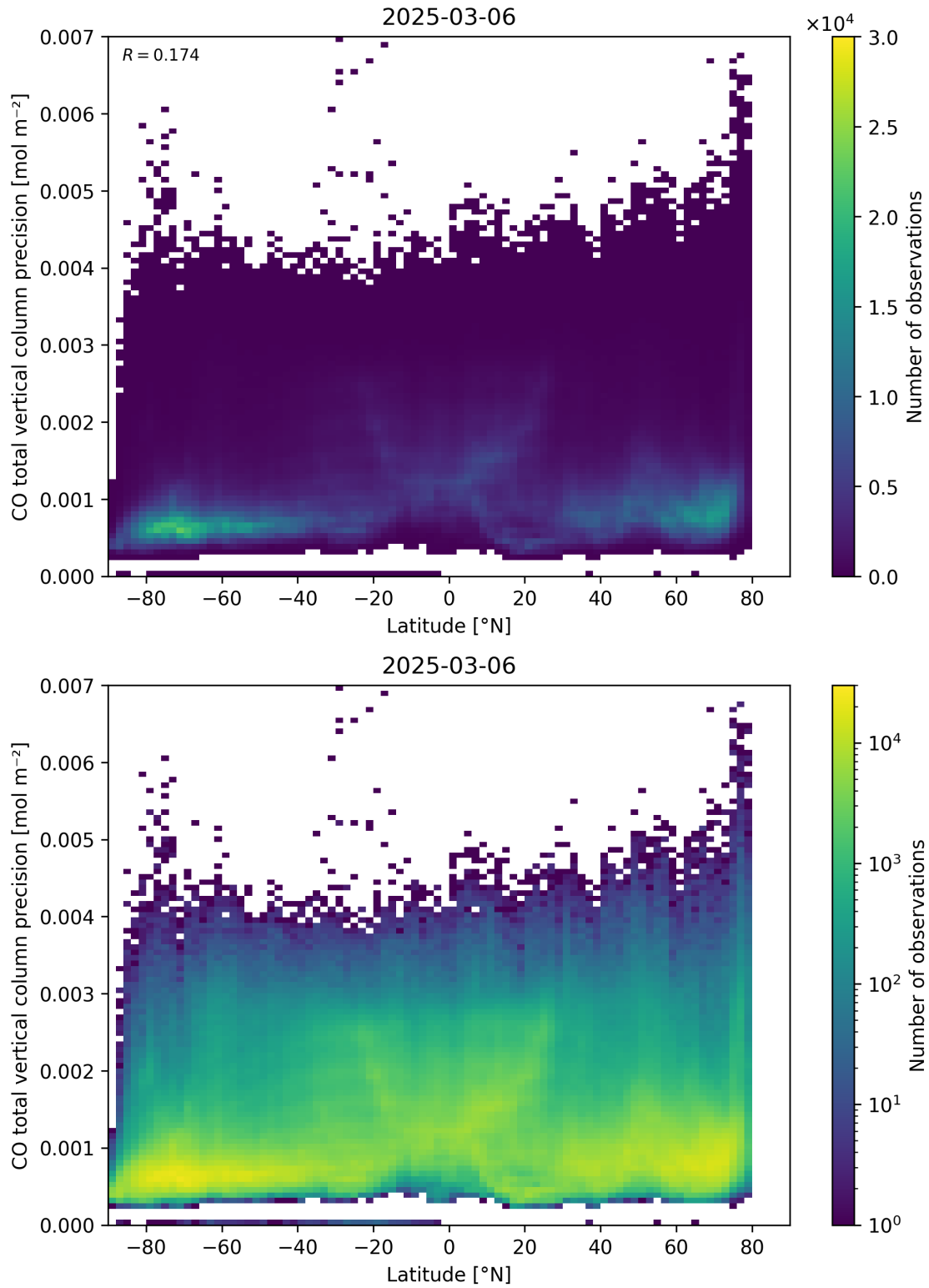
Figure 53: Scatter density plot of “Latitude” against “CO total vertical column precision” for 2025-03-05 to 2025-03-07.
