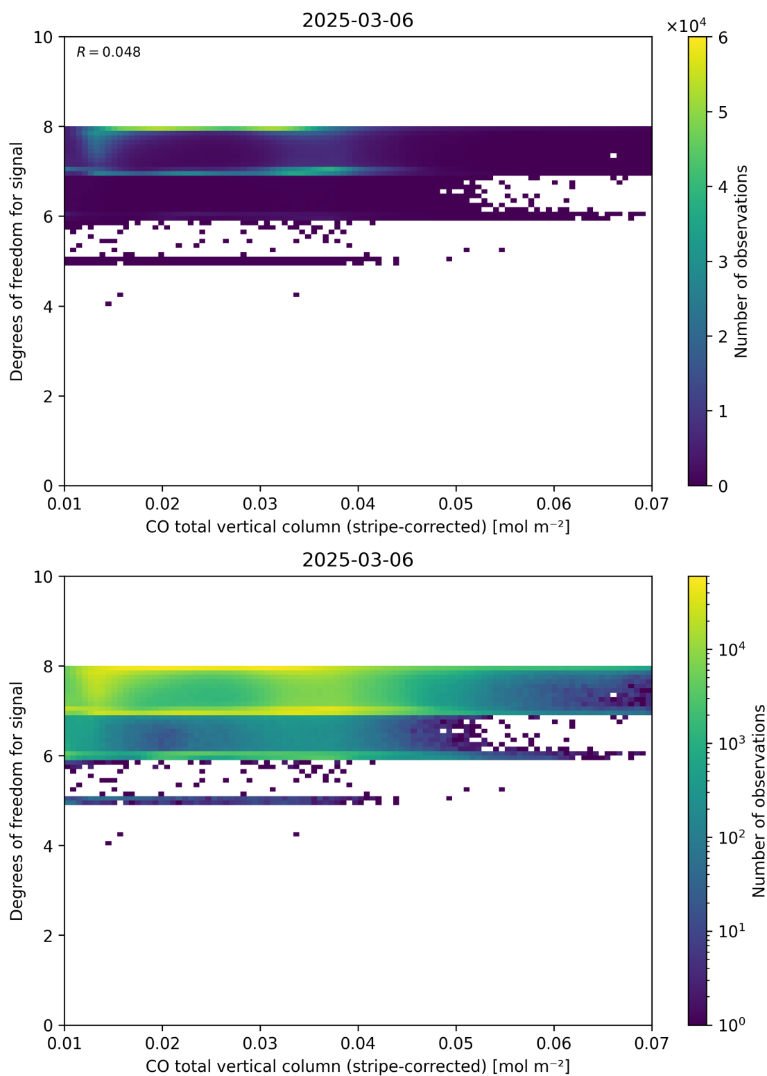
Figure 38: Scatter density plot of “CO total vertical column (stripe-corrected)” against “Degrees of freedom for signal” for 2025-03-05 to 2025-03-07.
