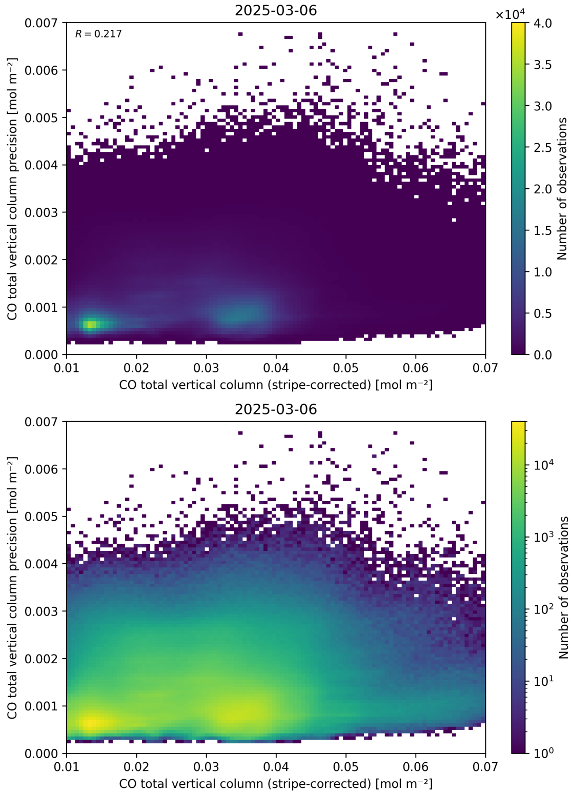
Figure 36: Scatter density plot of “CO total vertical column (stripe-corrected)” against “CO total vertical column precision” for 2025-03-05 to 2025-03-07.
