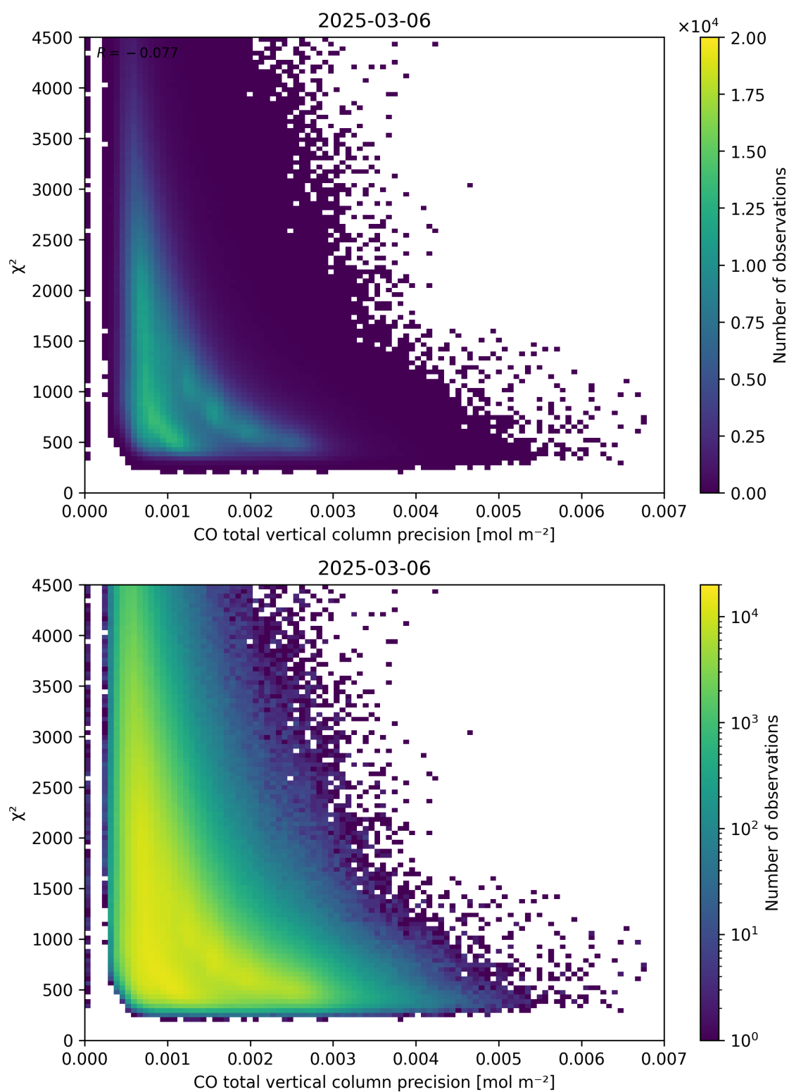
Figure 44: Scatter density plot of “CO total vertical column precision” against “ \chi^2 ” for 2025-03-05 to 2025-03-07.
