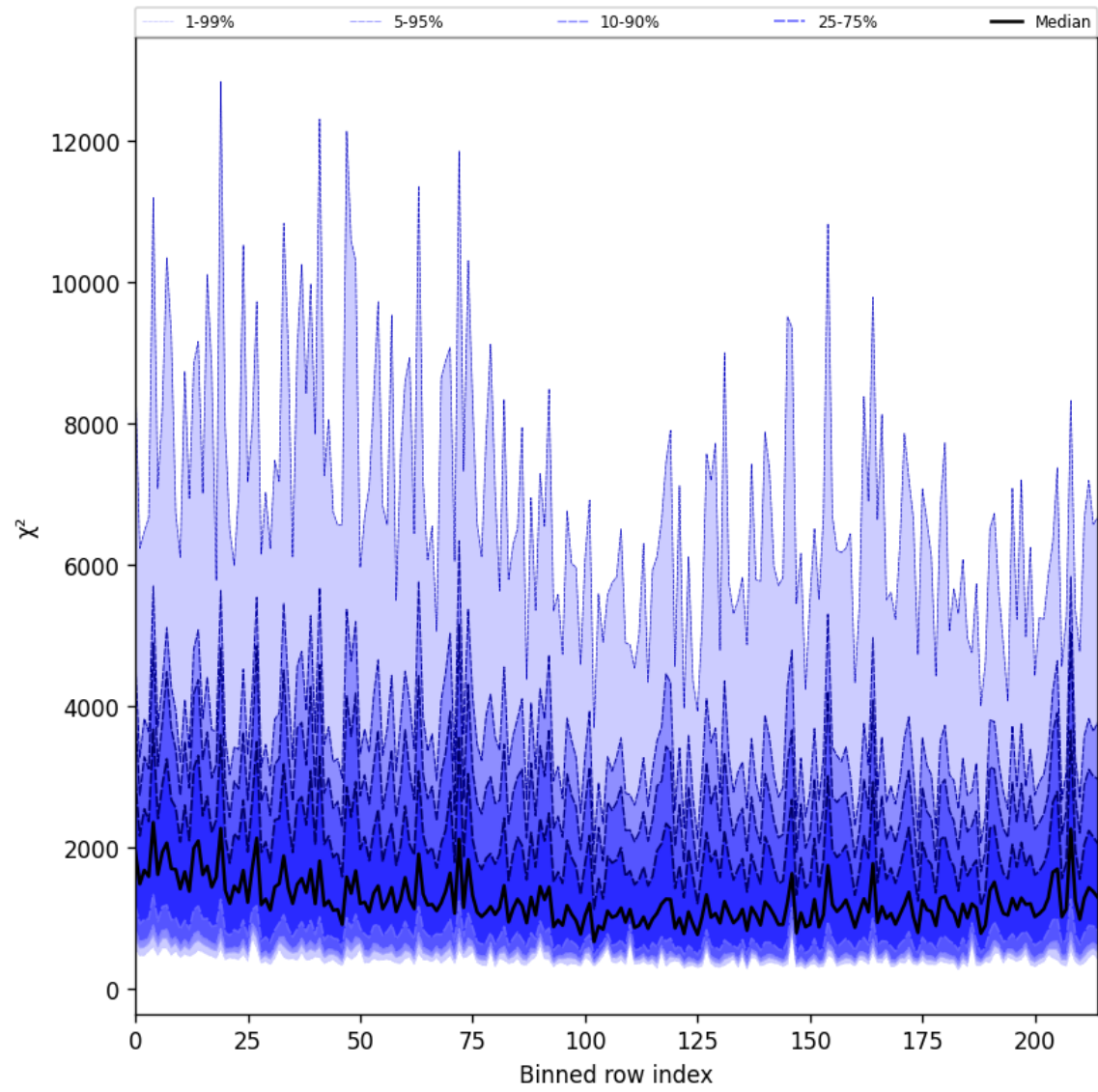
Figure 30: Along track statistics of “ \chi^2 ” for 2025-03-05 to 2025-03-07
