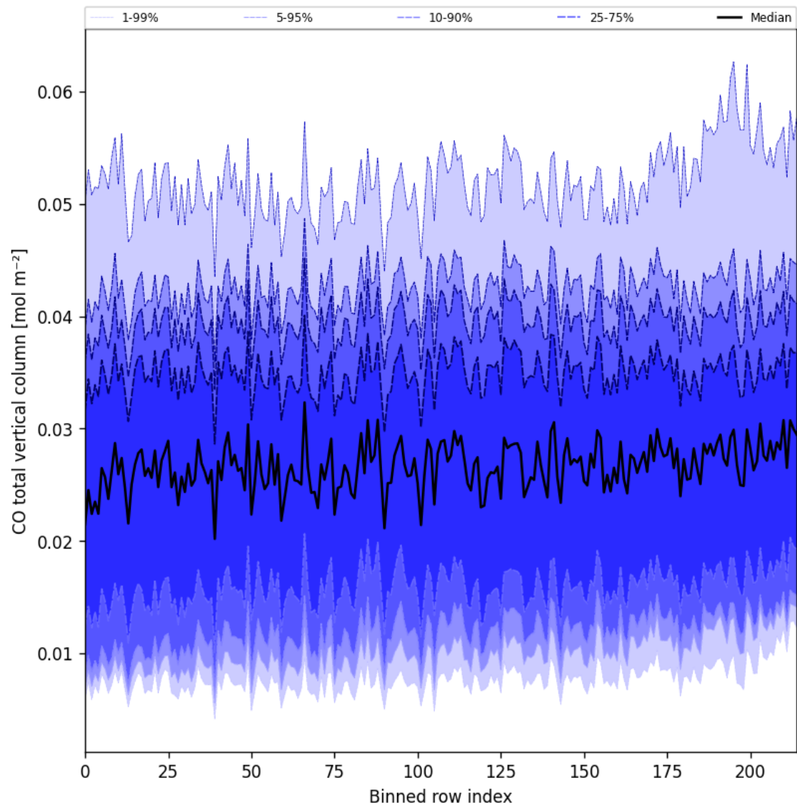
Figure 26: Along track statistics of “CO total vertical column” for 2025-03-05 to 2025-03-07
