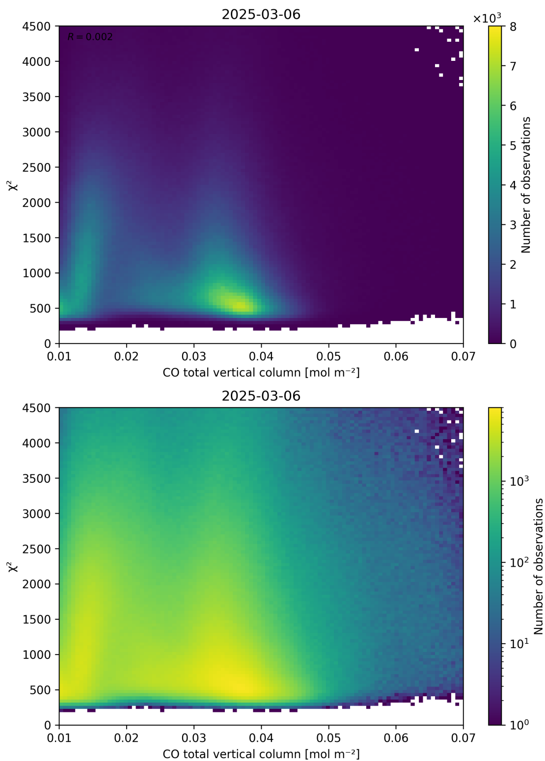
Figure 35: Scatter density plot of “CO total vertical column” against “ \chi^2 ” for 2025-03-05 to 2025-03-07.
