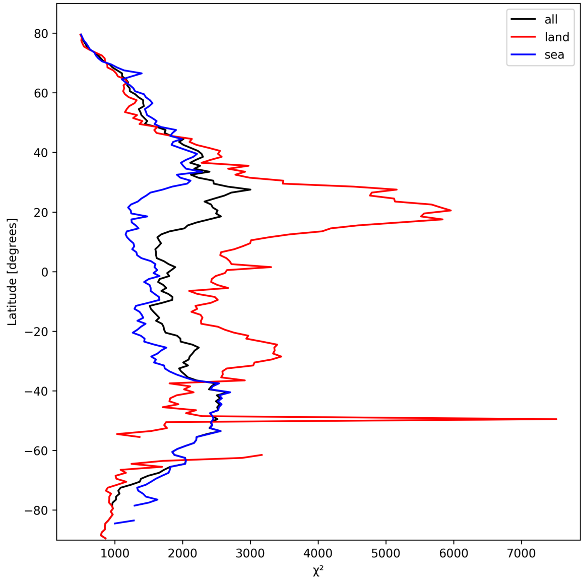
Figure 14: Zonal average of “ \chi^2 ” for 2025-03-05 to 2025-03-07.
