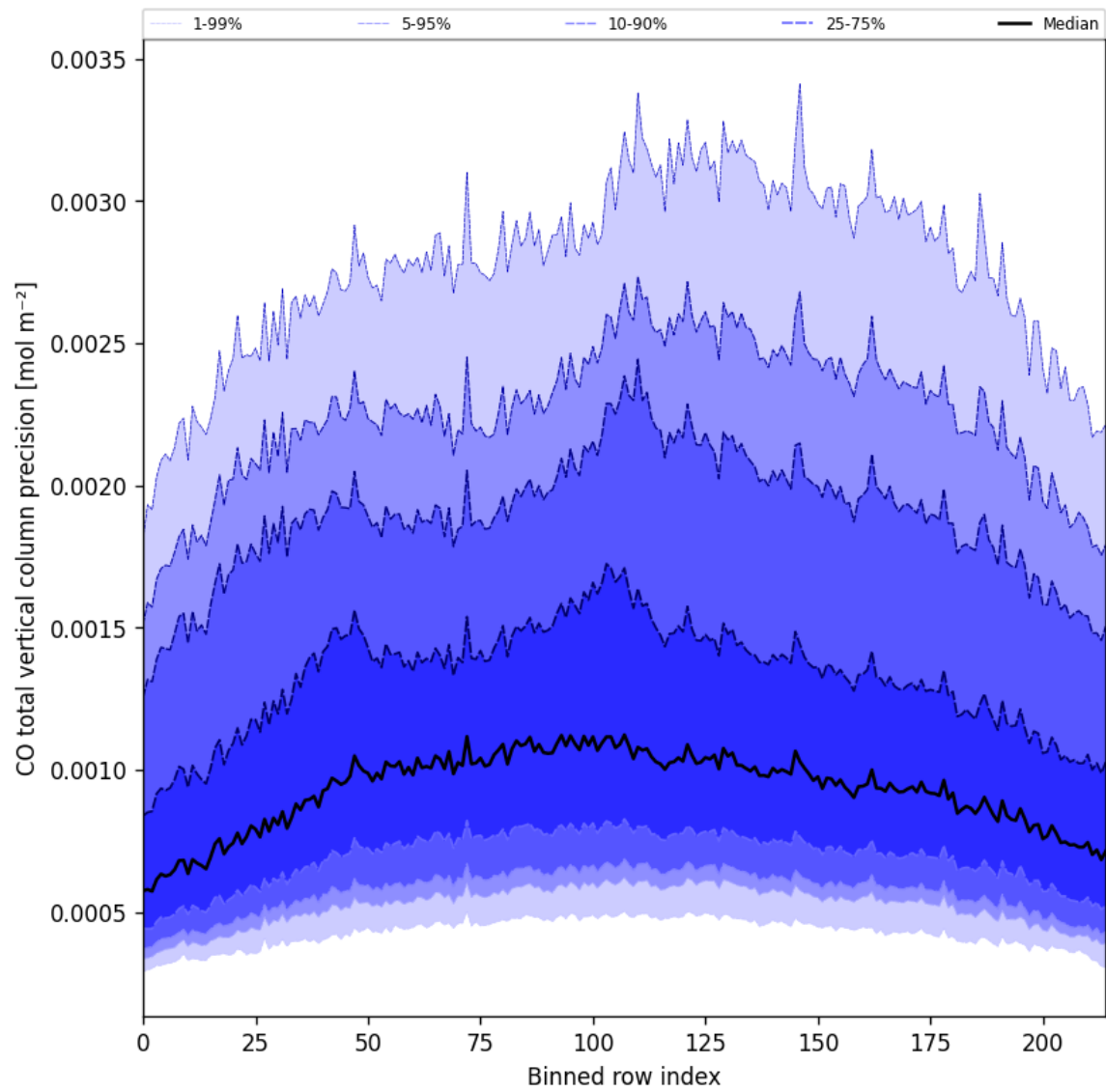
Figure 28: Along track statistics of “CO total vertical column precision” for 2025-03-05 to 2025-03-07
