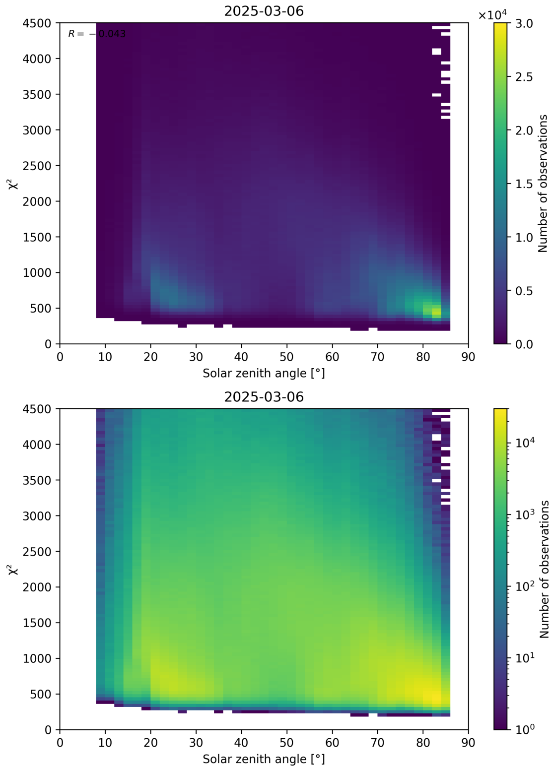
Figure 64: Scatter density plot of “Solar zenith angle” against “ \chi^2 ” for 2025-03-05 to 2025-03-07.
