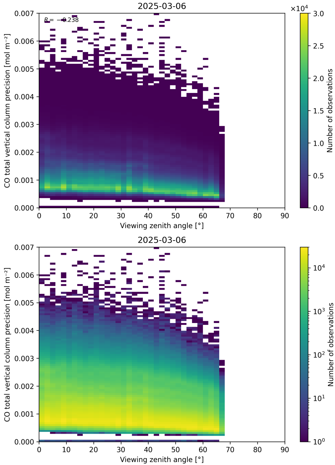
Figure 71: Scatter density plot of “Viewing zenith angle” against “CO total vertical column precision” for 2025-03-05 to 2025-03-07.
