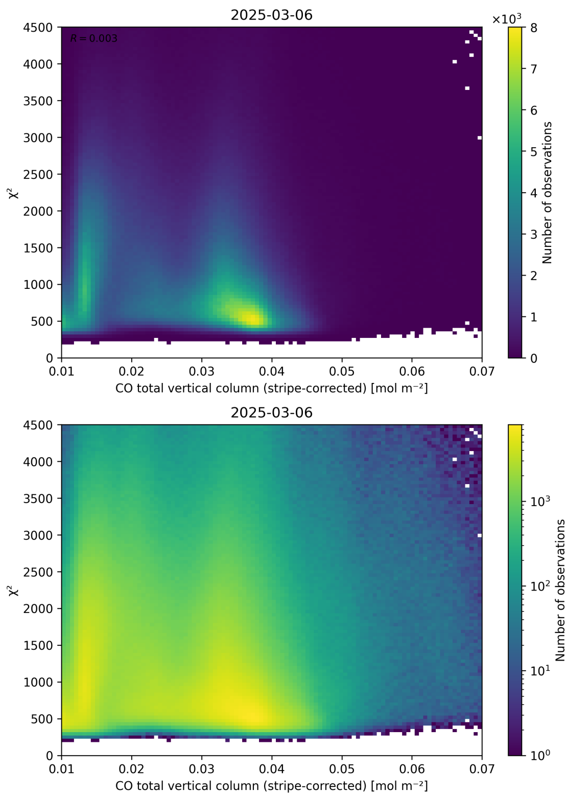
Figure 37: Scatter density plot of “CO total vertical column (stripe-corrected)” against “ \chi^2 ” for 2025-03-05 to 2025-03-07.
