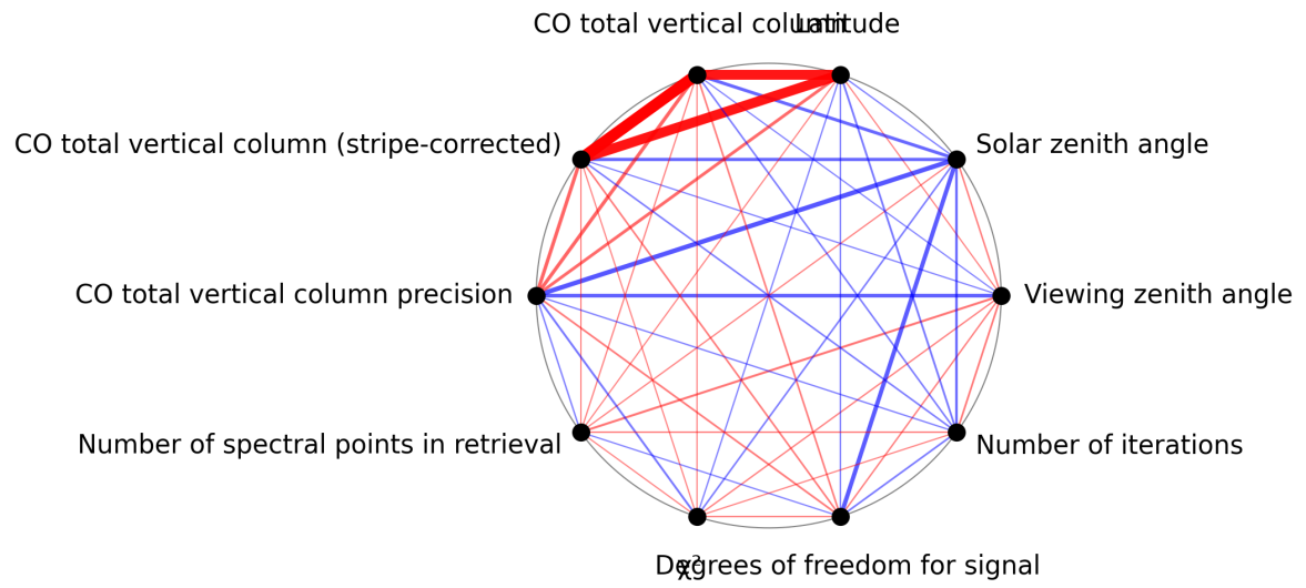
Figure 1: Map of correlation graph for 2025-03-05 to 2025-03-07.
