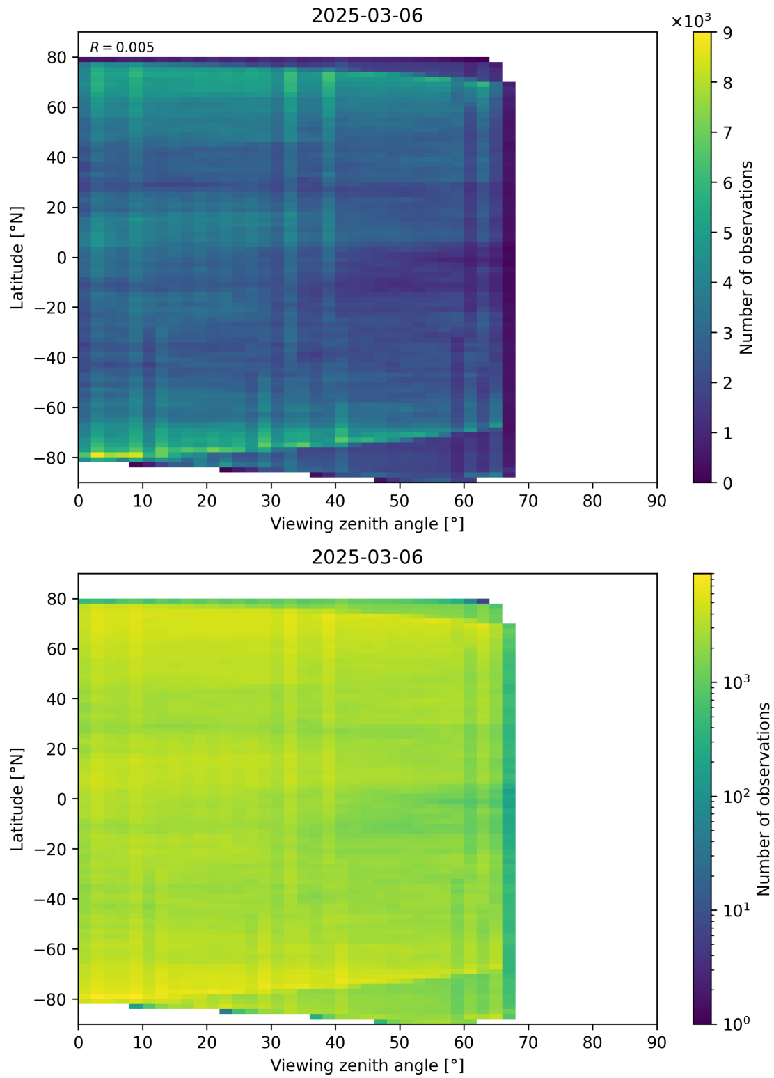
Figure 74: Scatter density plot of “Viewing zenith angle” against “Latitude” for 2025-03-05 to 2025-03-07.
