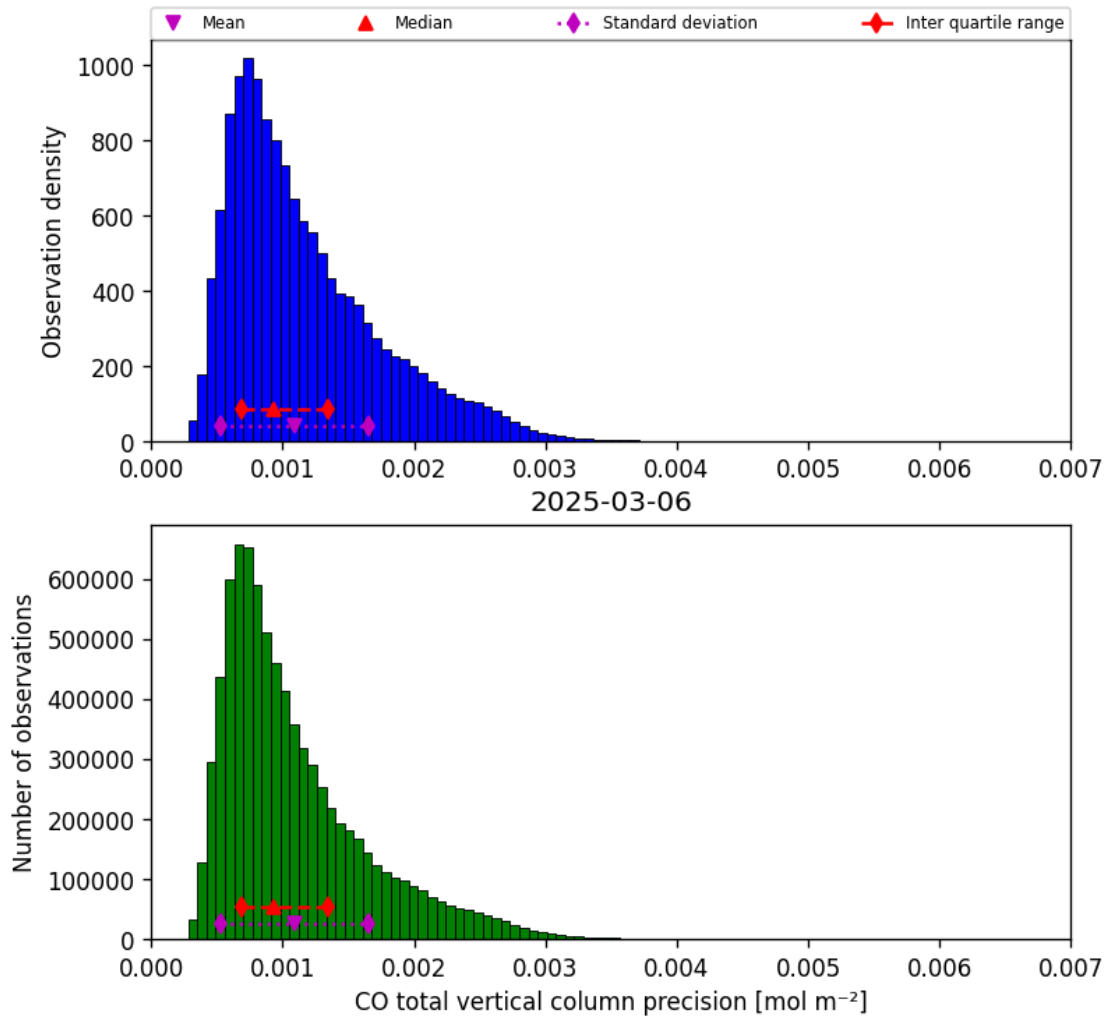
Figure 20: Histogram of “CO total vertical column precision” for 2025-03-05 to 2025-03-07
