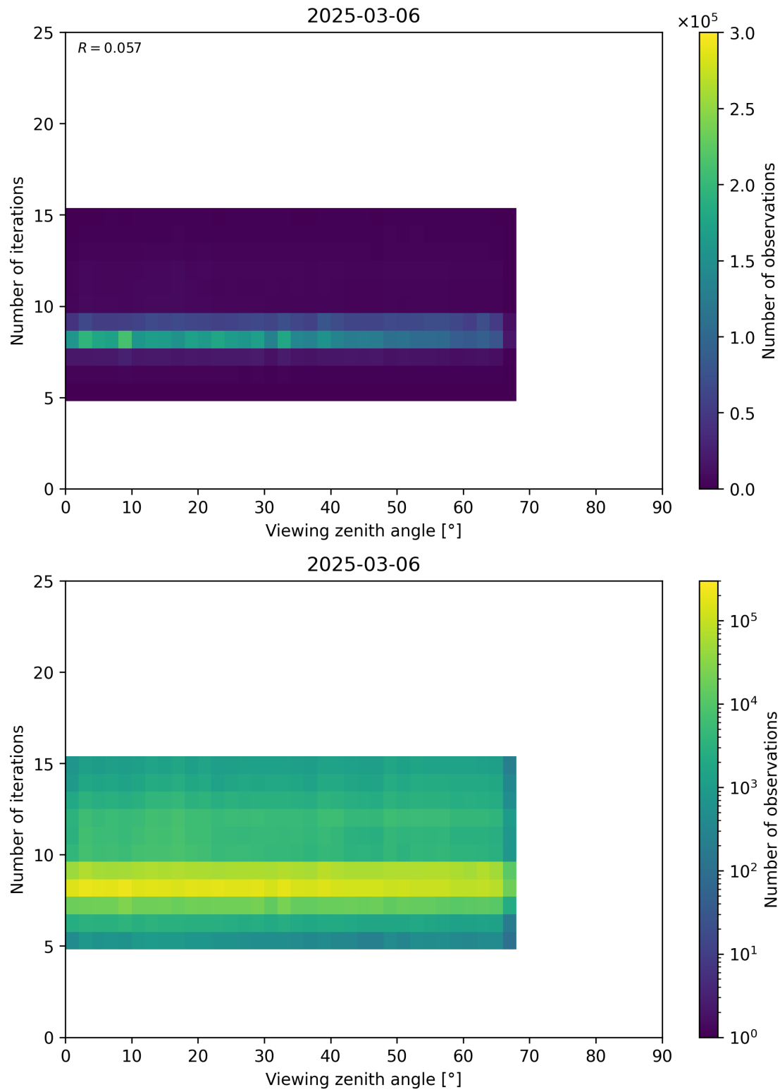
Figure 75: Scatter density plot of “Viewing zenith angle” against “Number of iterations” for 2025-03-05 to 2025-03-07.
