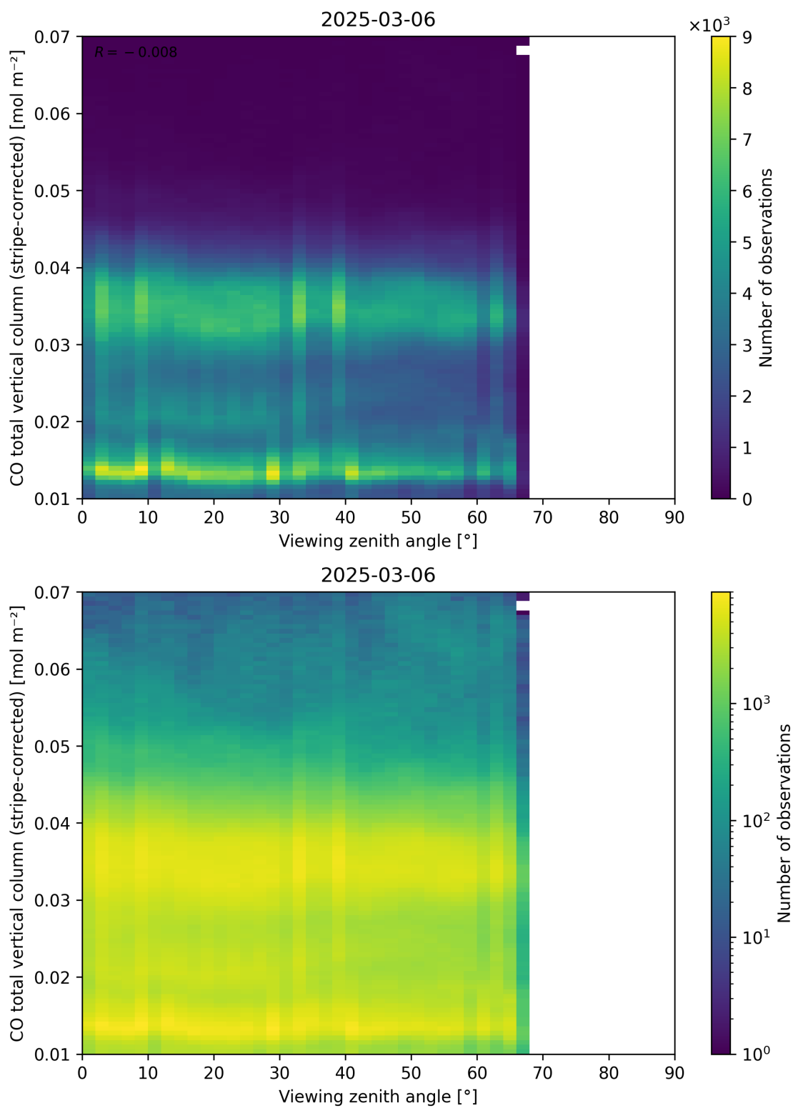
Figure 70: Scatter density plot of “Viewing zenith angle” against “CO total vertical column (stripe-corrected)” for 2025-03-05 to 2025-03-07.
