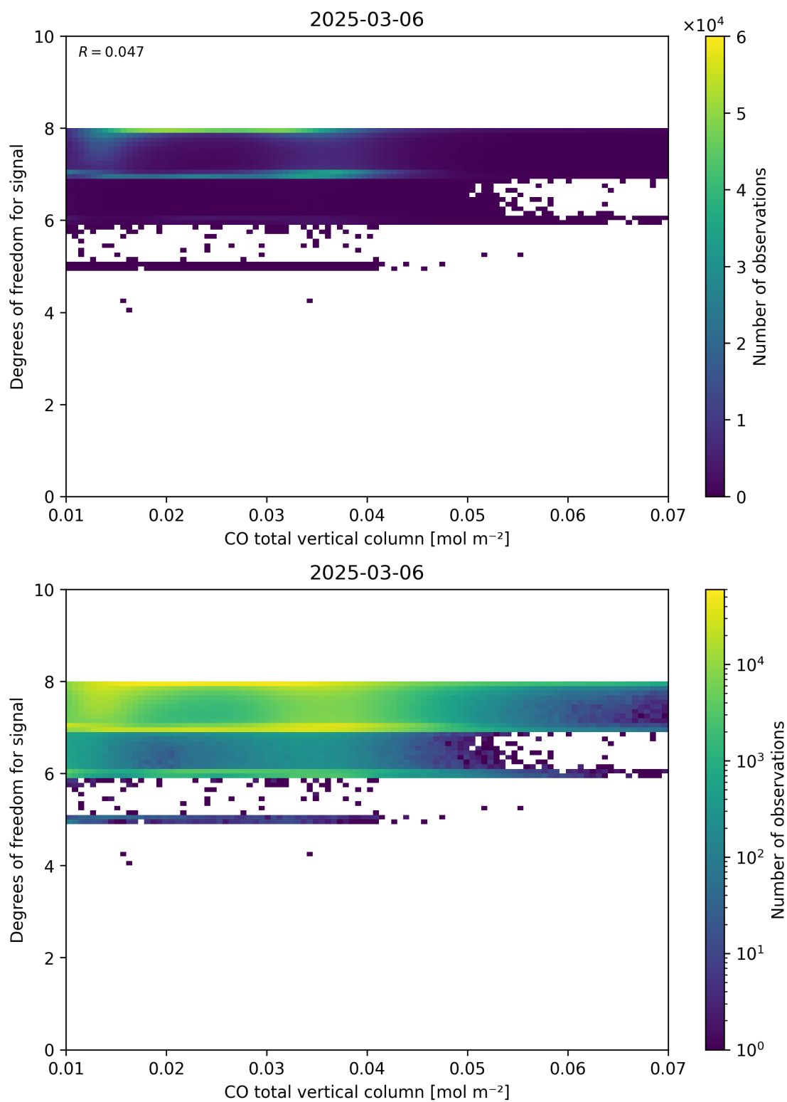
Figure 41: Scatter density plot of “CO total vertical column” against “Degrees of freedom for signal” for 2025-03-05 to 2025-03-07.
