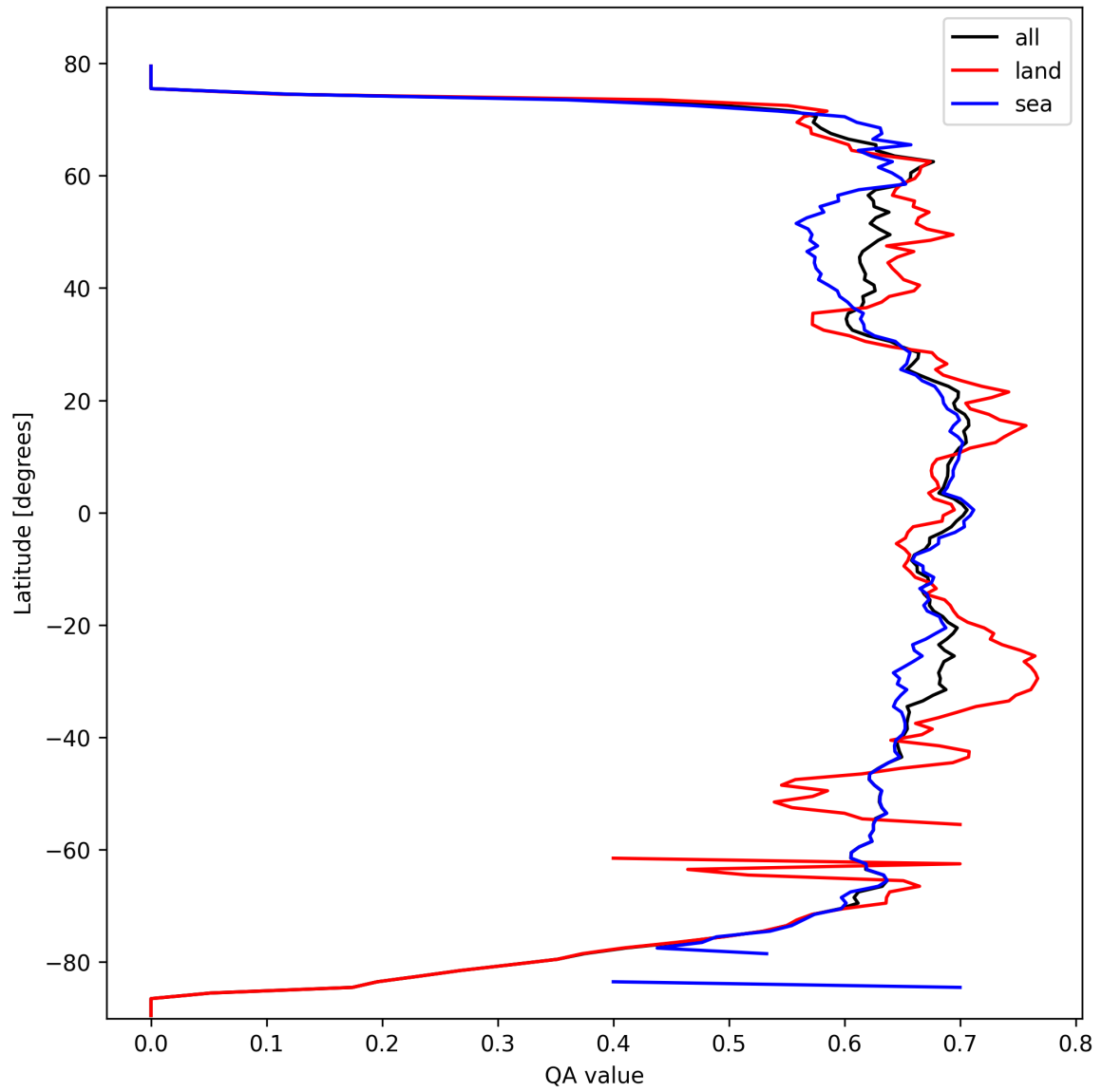
Figure 9: Zonal average of “QA value” for 2025-03-05 to 2025-03-07.
