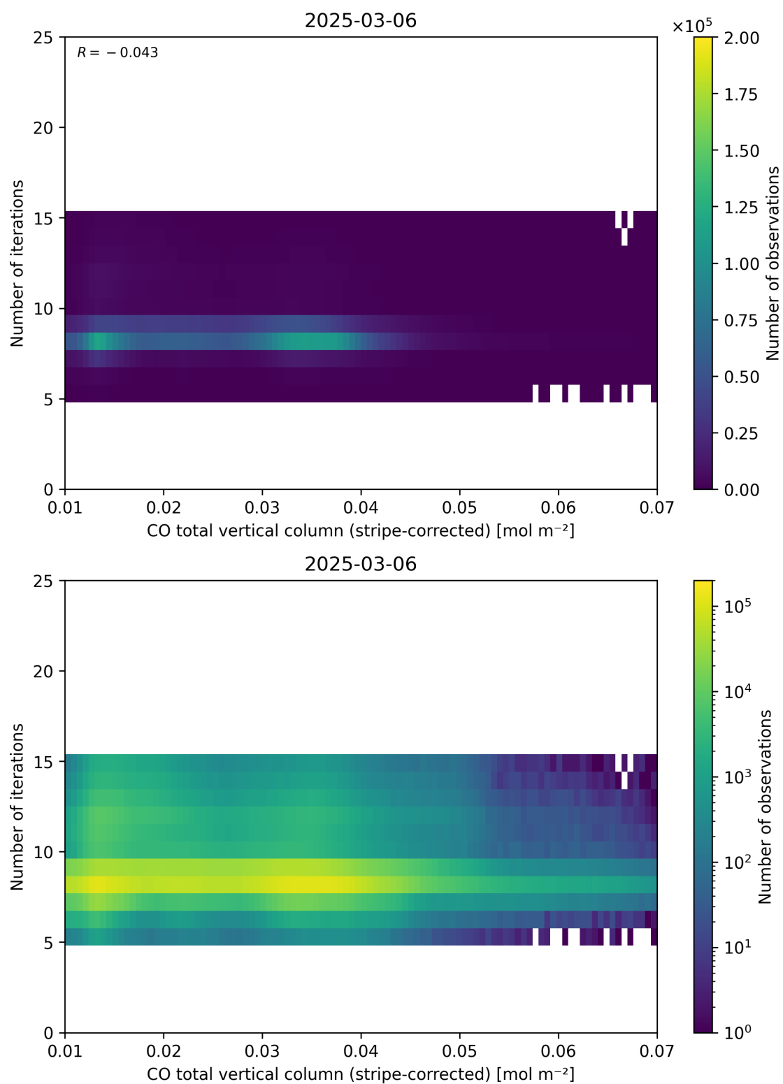
Figure 39: Scatter density plot of “CO total vertical column (stripe-corrected)” against “Number of iterations” for 2025-03-05 to 2025-03-07.
