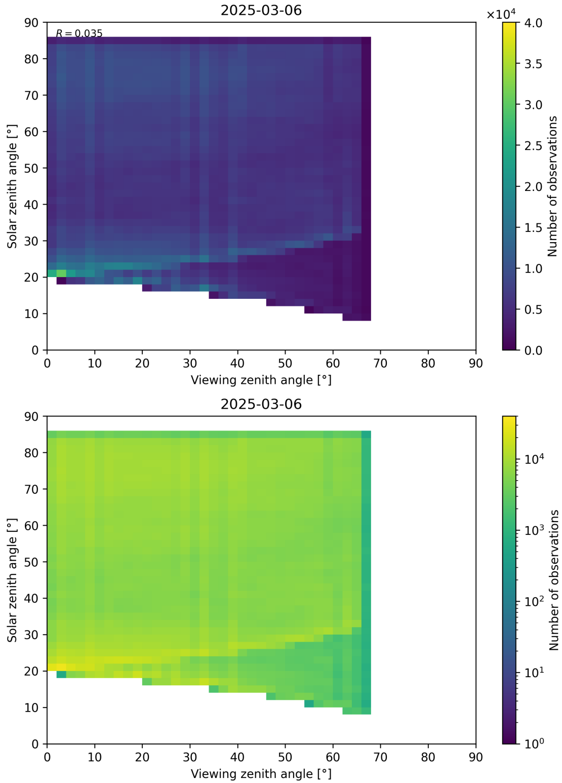
Figure 77: Scatter density plot of “Viewing zenith angle” against “Solar zenith angle” for 2025-03-05 to 2025-03-07.
