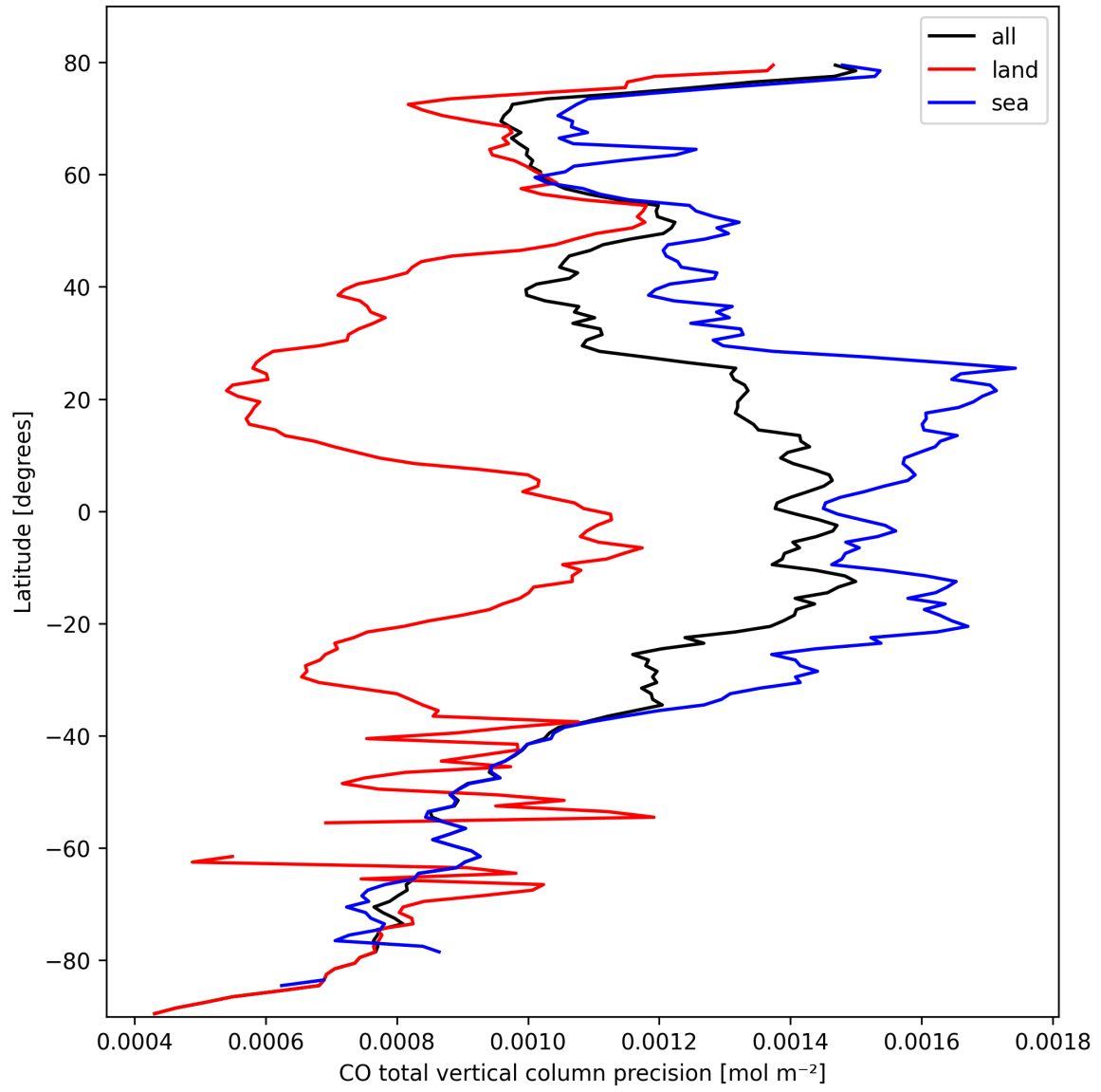
Figure 12: Zonal average of “CO total vertical column precision” for 2025-03-05 to 2025-03-07.
