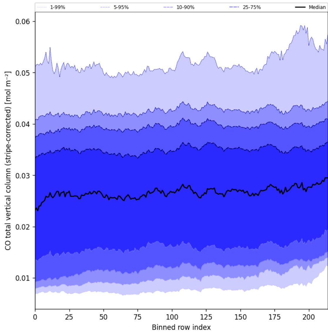
Figure 27: Along track statistics of “CO total vertical column (stripe-corrected)” for 2025-03-05 to 2025-03-07
