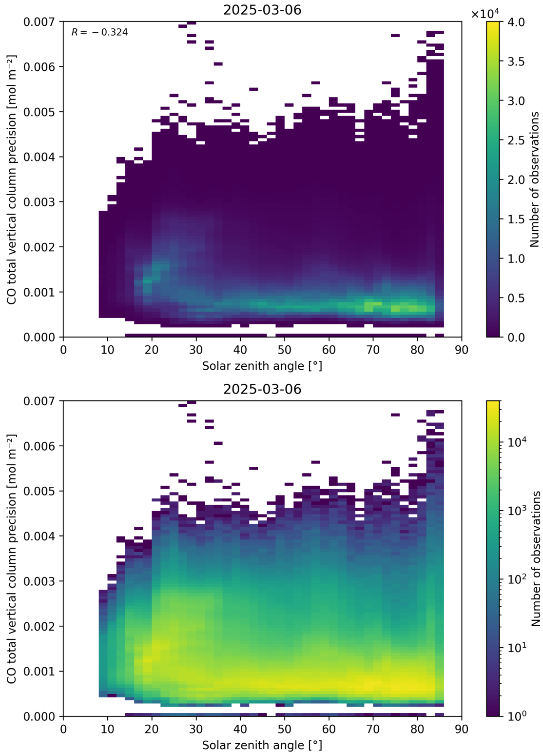
Figure 63: Scatter density plot of “Solar zenith angle” against “CO total vertical column precision” for 2025-03-05 to 2025-03-07.
