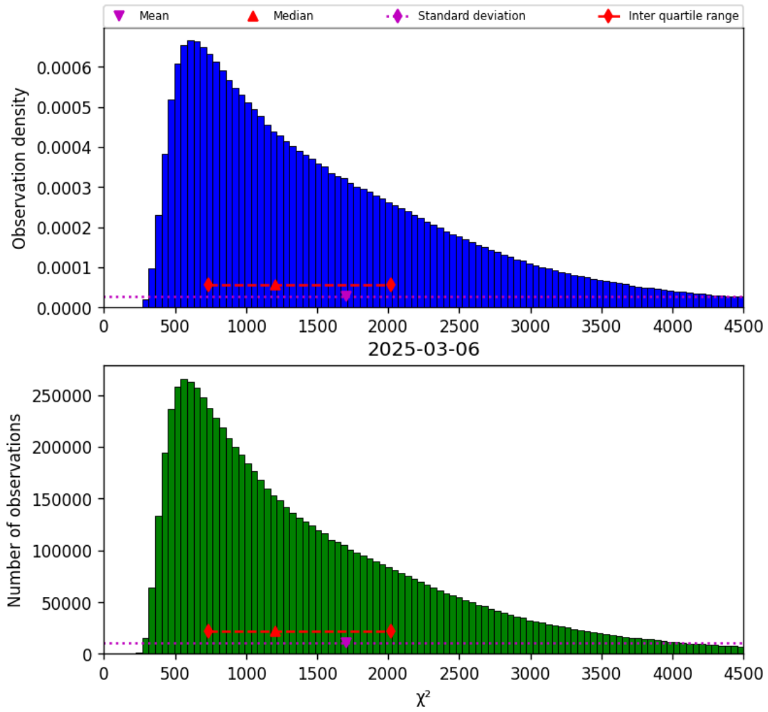
Figure 22: Histogram of “ \chi^2 ” for 2025-03-05 to 2025-03-07
