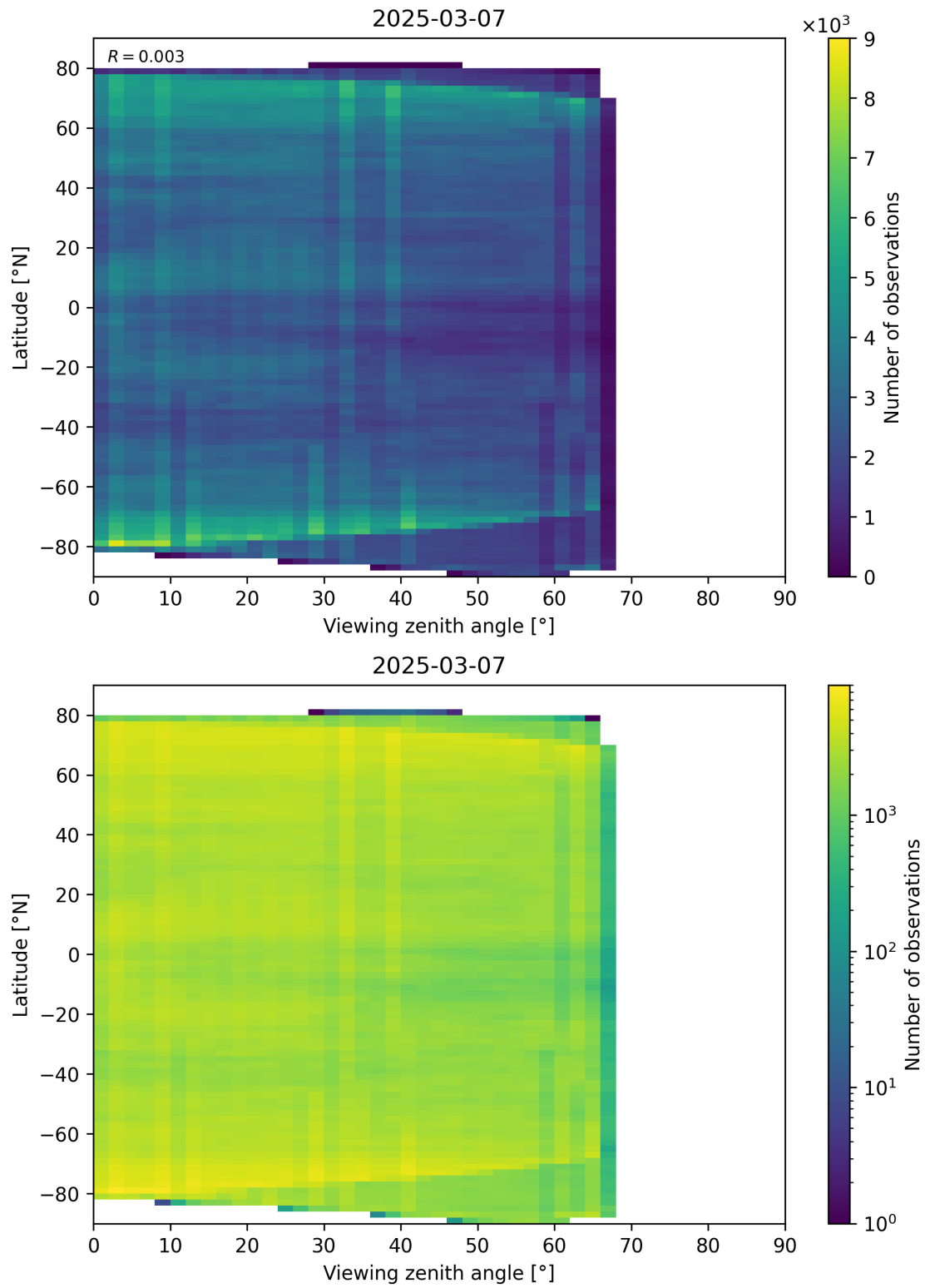
Figure 74: Scatter density plot of “Viewing zenith angle” against “Latitude” for 2025-03-07 to 2025-03-08.
