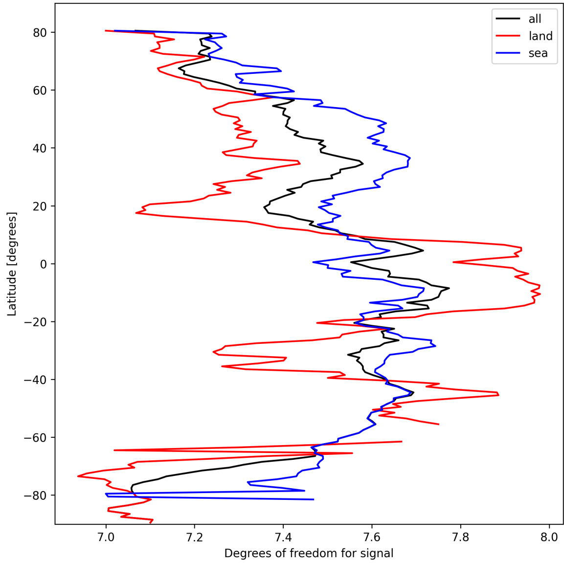
Figure 15: Zonal average of “Degrees of freedom for signal” for 2025-03-07 to 2025-03-08.
