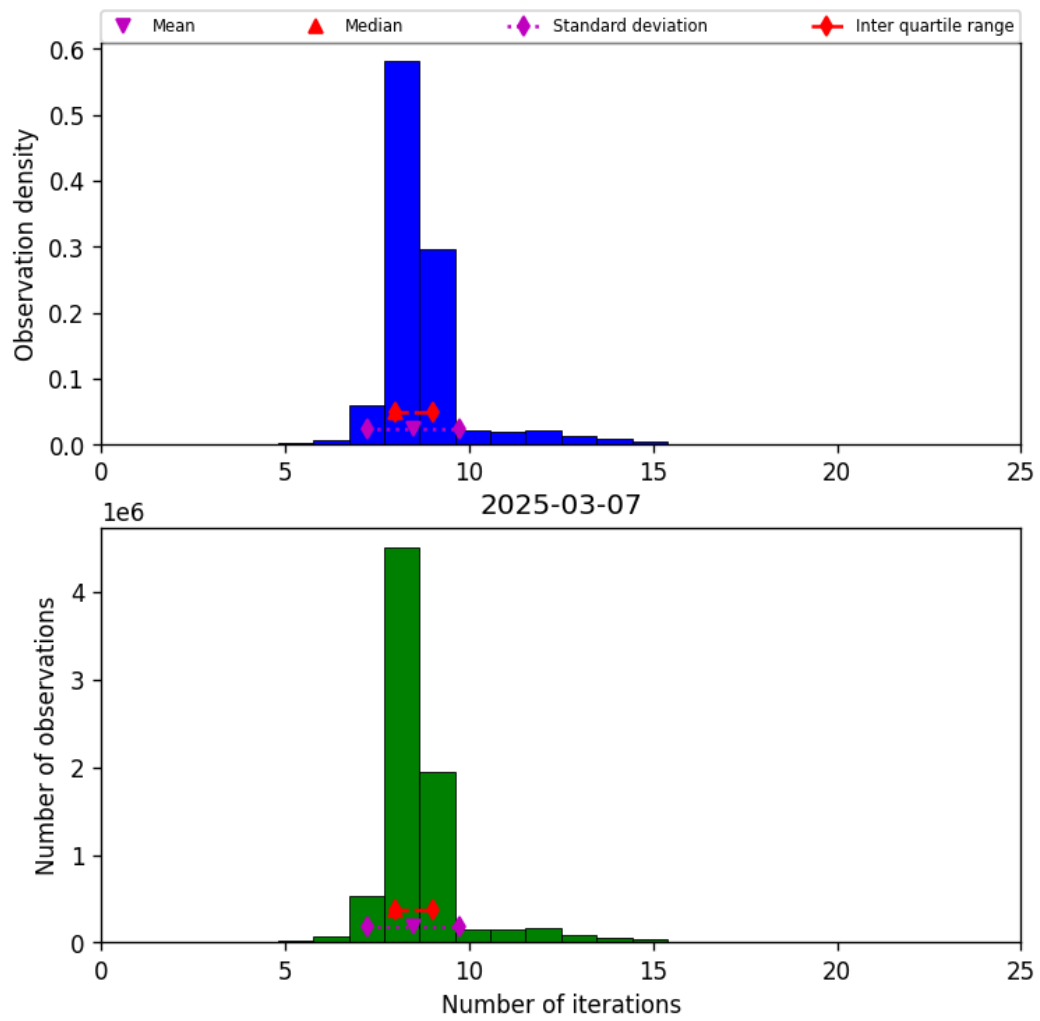
Figure 24: Histogram of “Number of iterations” for 2025-03-07 to 2025-03-08
