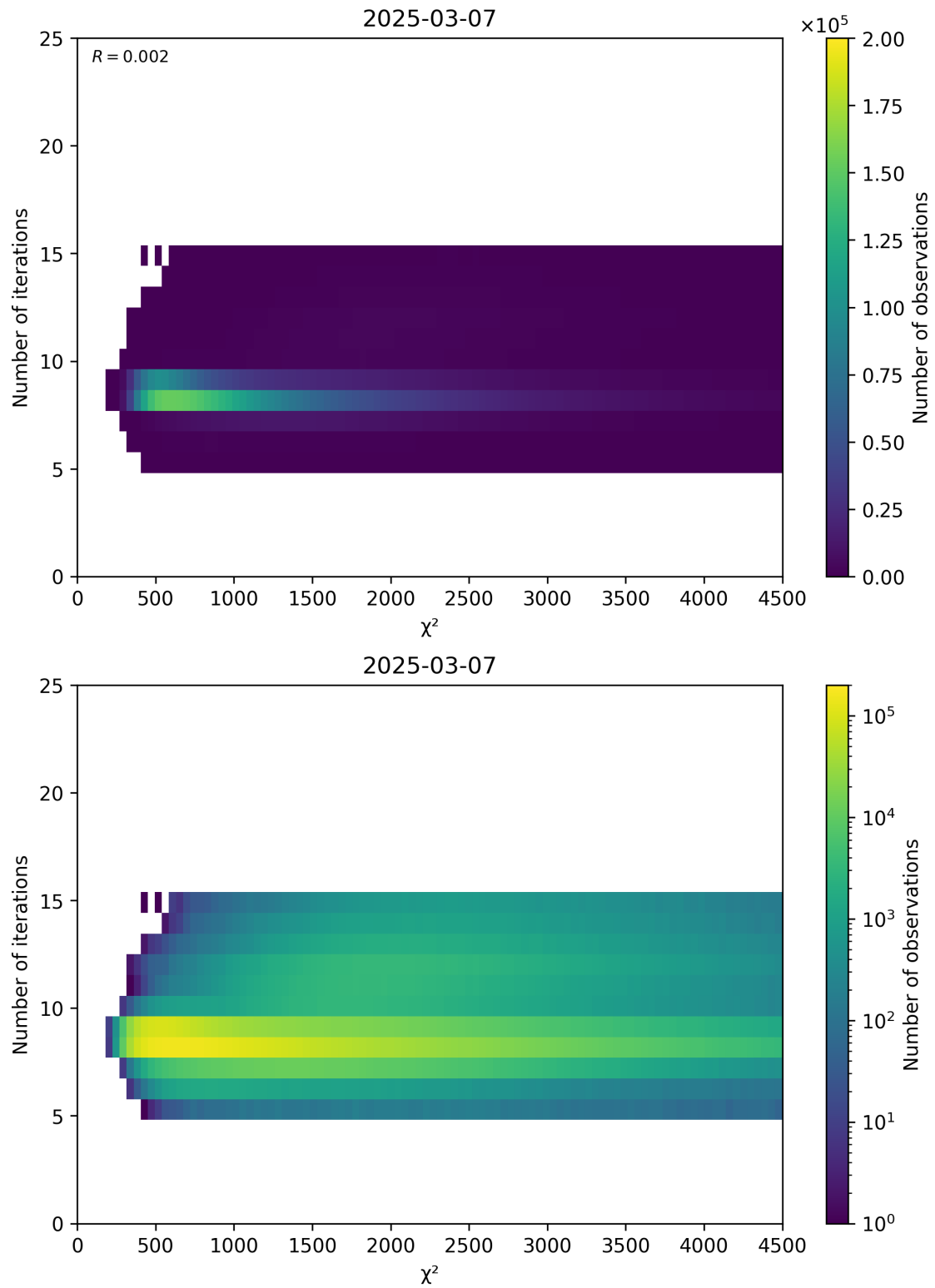
Figure 49: Scatter density plot of “ \chi^2 ” against “Number of iterations” for 2025-03-07 to 2025-03-08.
