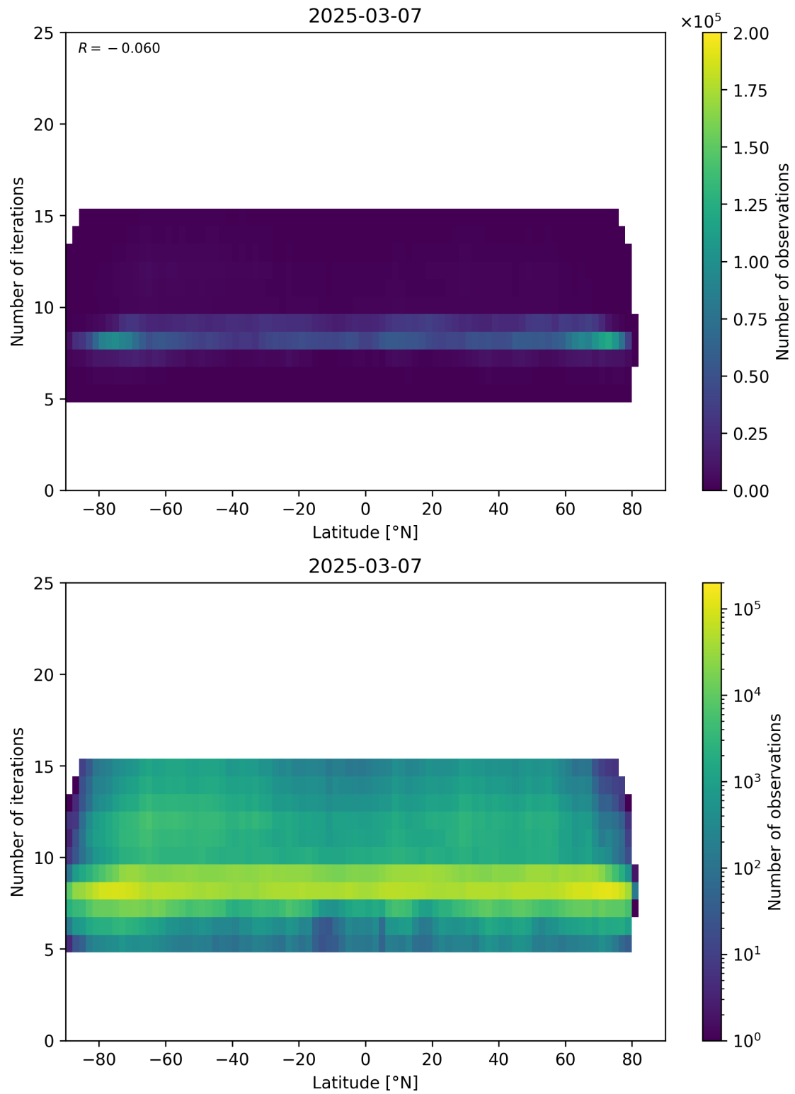
Figure 56: Scatter density plot of “Latitude” against “Number of iterations” for 2025-03-07 to 2025-03-08.
