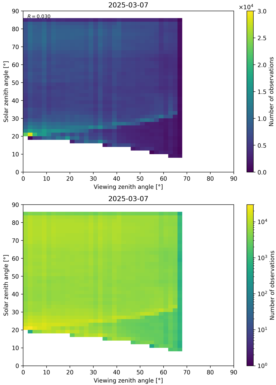
Figure 77: Scatter density plot of “Viewing zenith angle” against “Solar zenith angle” for 2025-03-07 to 2025-03-08.
