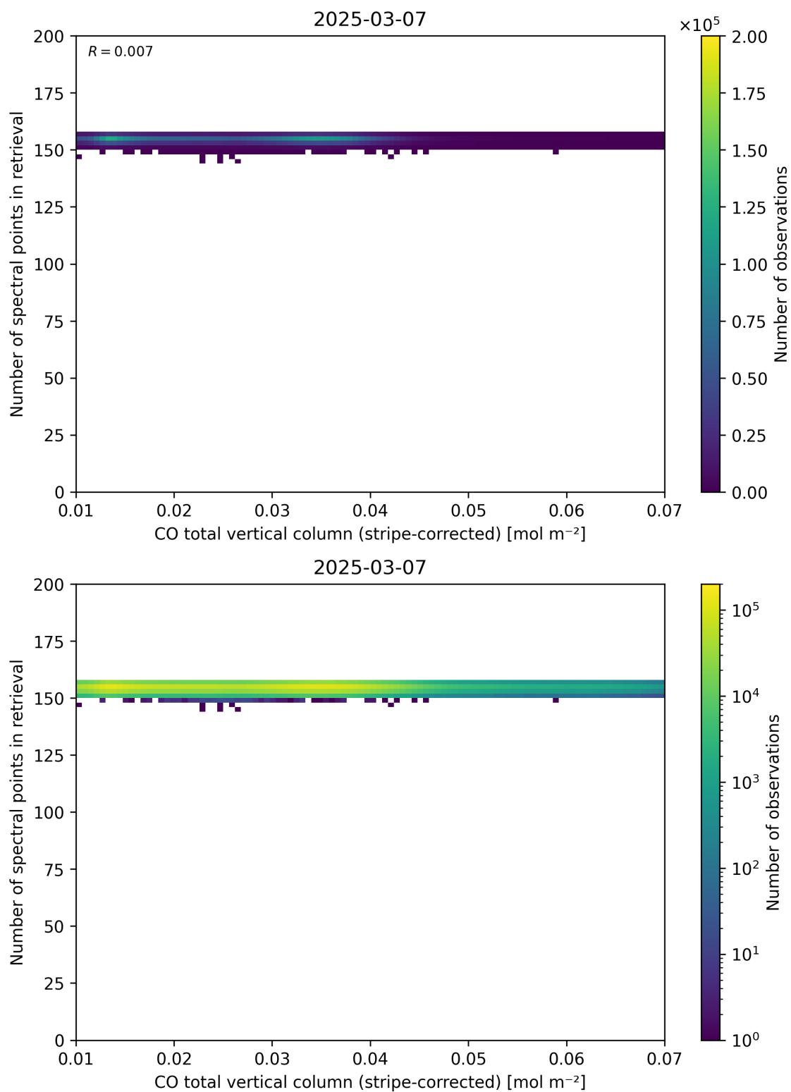
Figure 40: Scatter density plot of “CO total vertical column (stripe-corrected)” against “Number of spectral points in retrieval” for 2025-03-07 to 2025-03-08.
