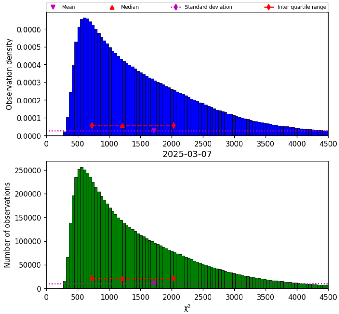
Figure 22: Histogram of " \chi^2 " for 2025-03-07 to 2025-03-08
