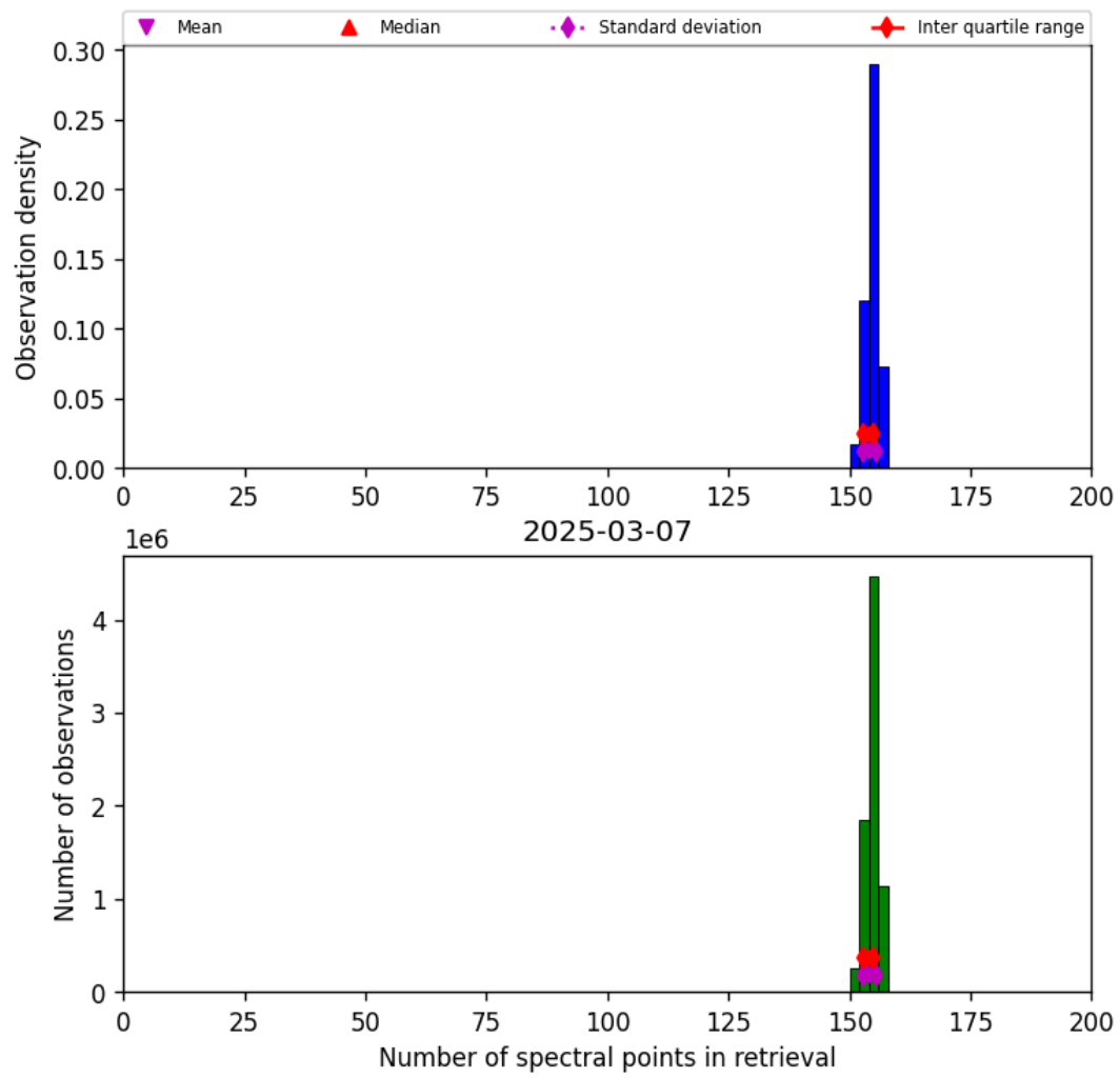
Figure 21: Histogram of “Number of spectral points in retrieval” for 2025-03-07 to 2025-03-08
