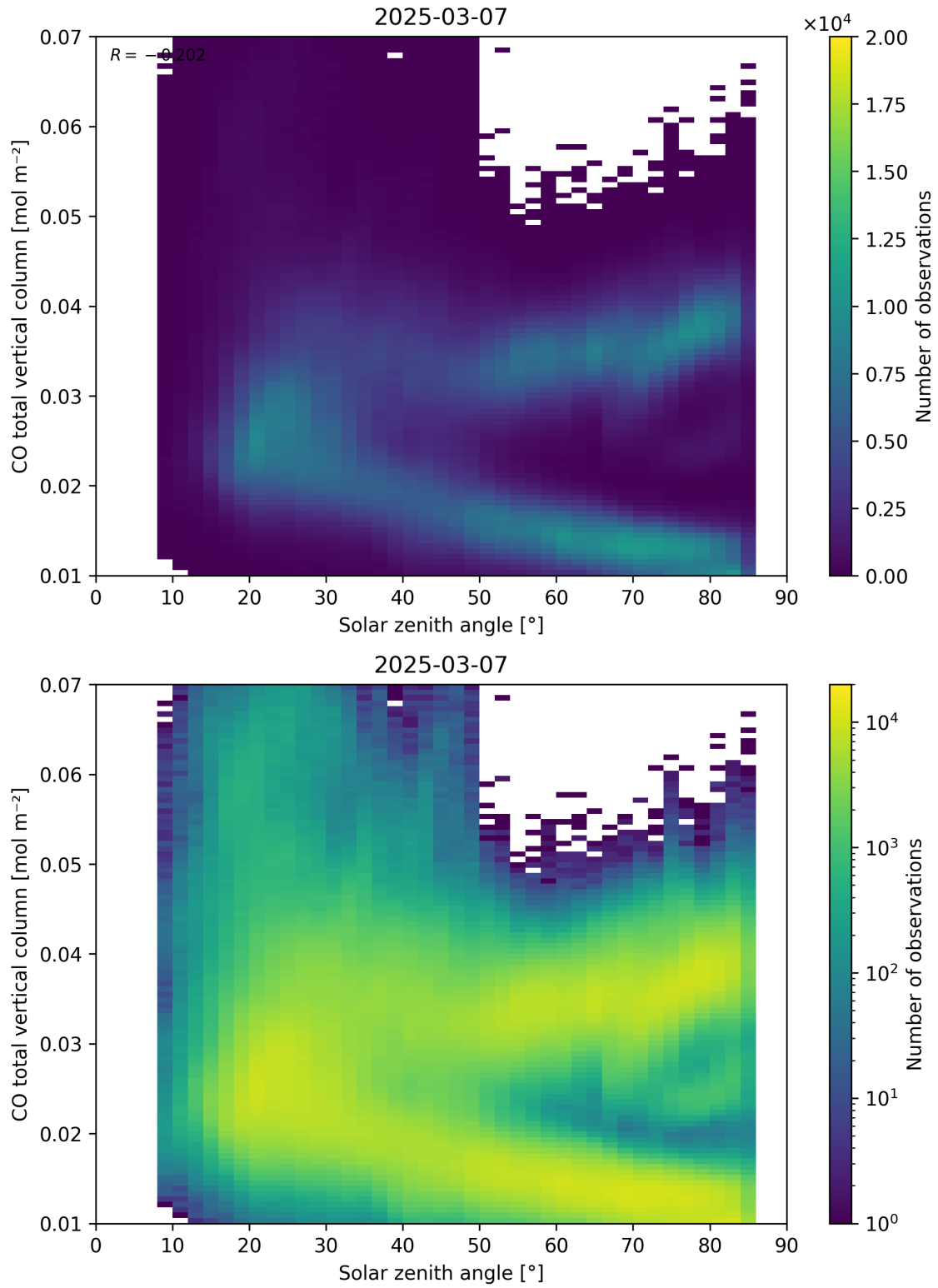
Figure 61: Scatter density plot of “Solar zenith angle” against “CO total vertical column” for 2025-03-07 to 2025-03-08.
