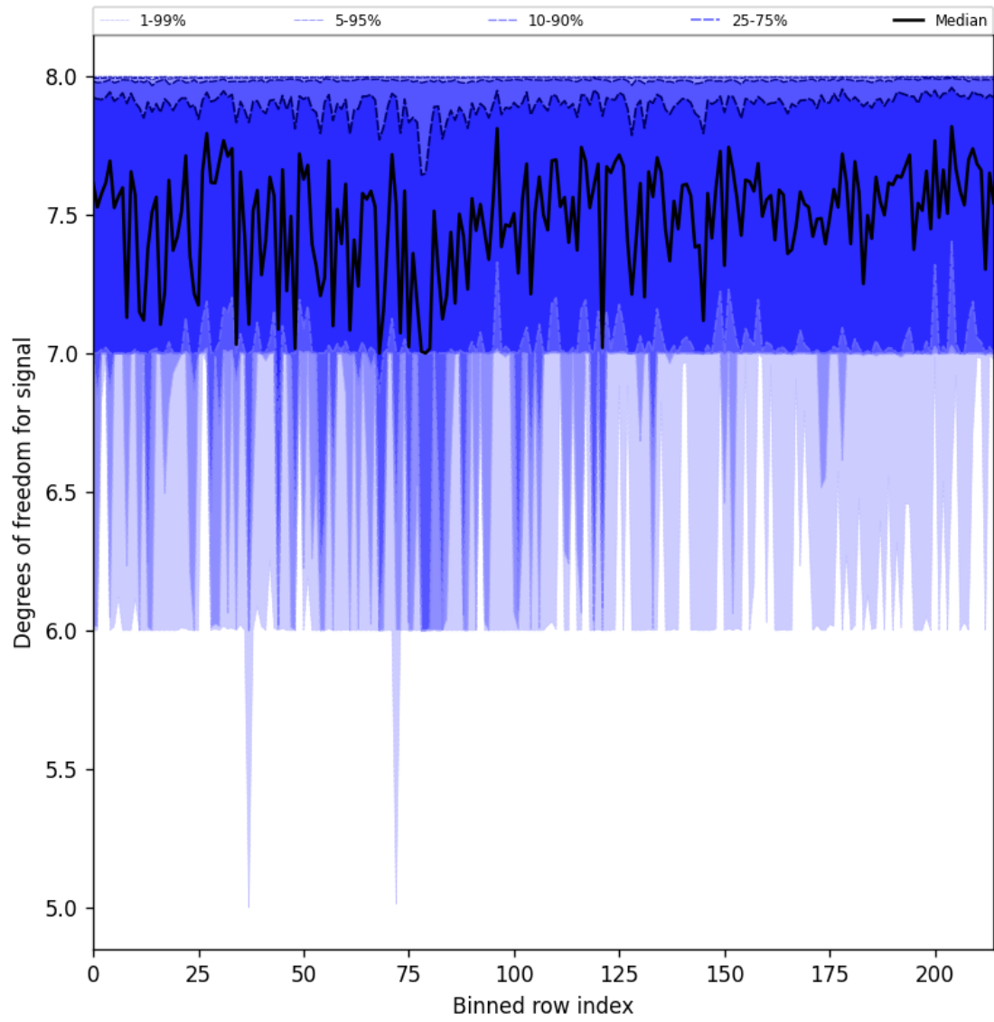
Figure 31: Along track statistics of “Degrees of freedom for signal” for 2025-03-07 to 2025-03-08
