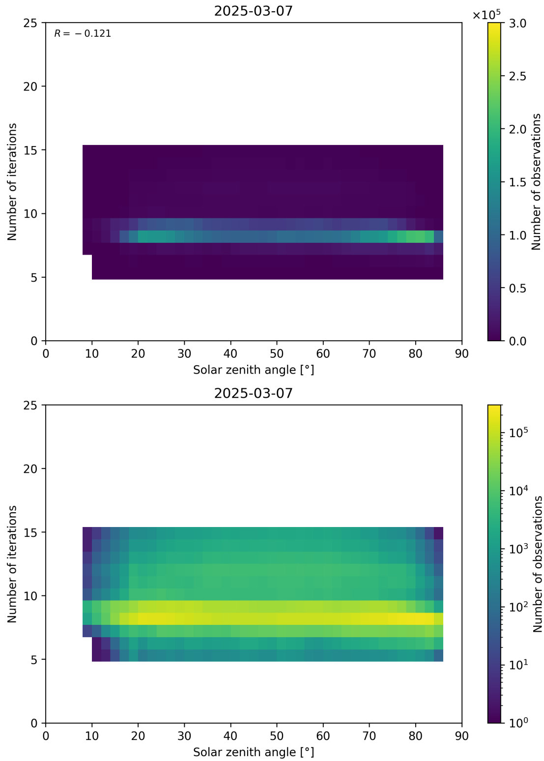
Figure 67: Scatter density plot of “Solar zenith angle” against “Number of iterations” for 2025-03-07 to 2025-03-08.
