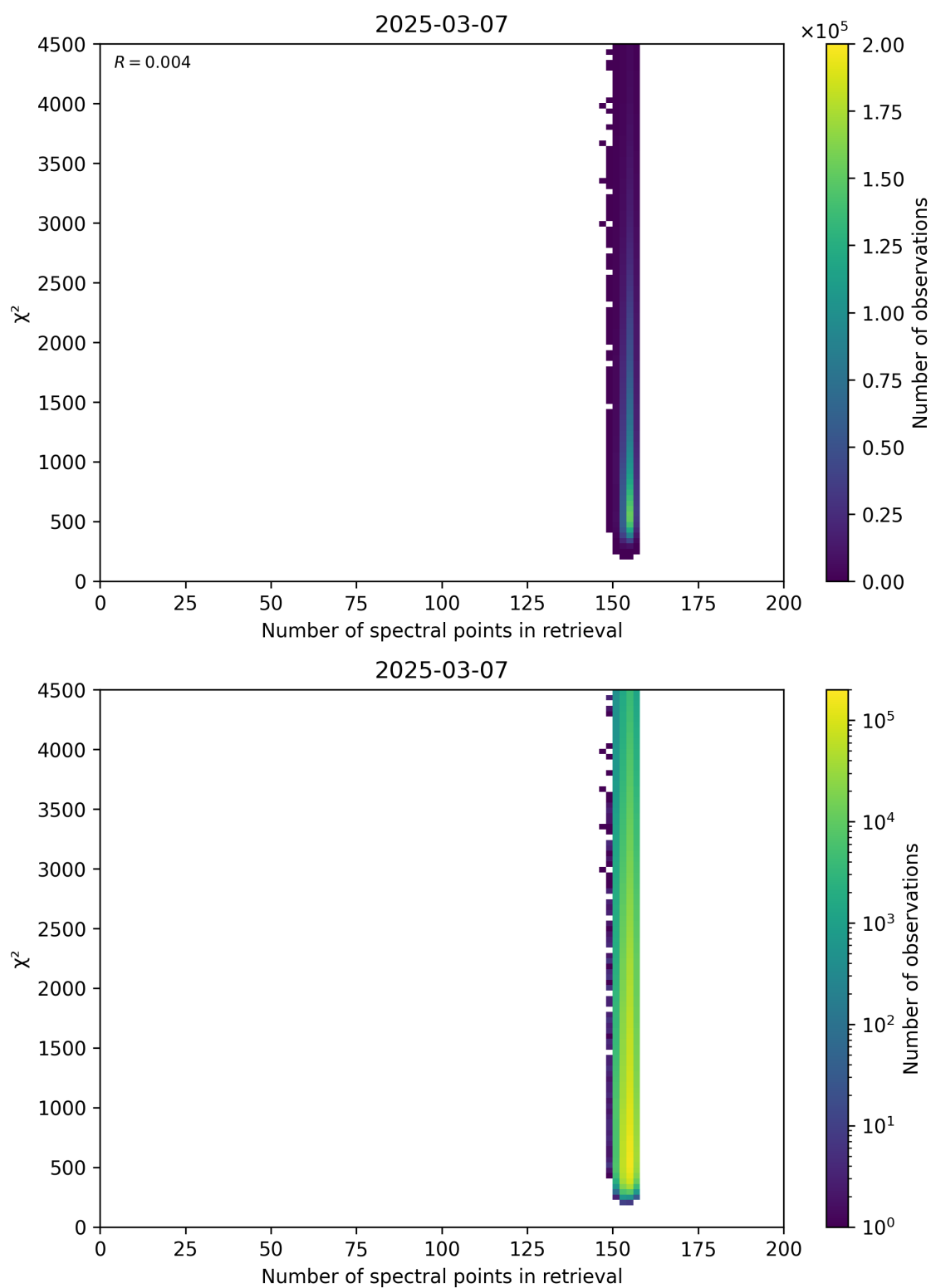
Figure 58: Scatter density plot of “Number of spectral points in retrieval” against “ \chi^2 ” for 2025-03-07 to 2025-03-08.
