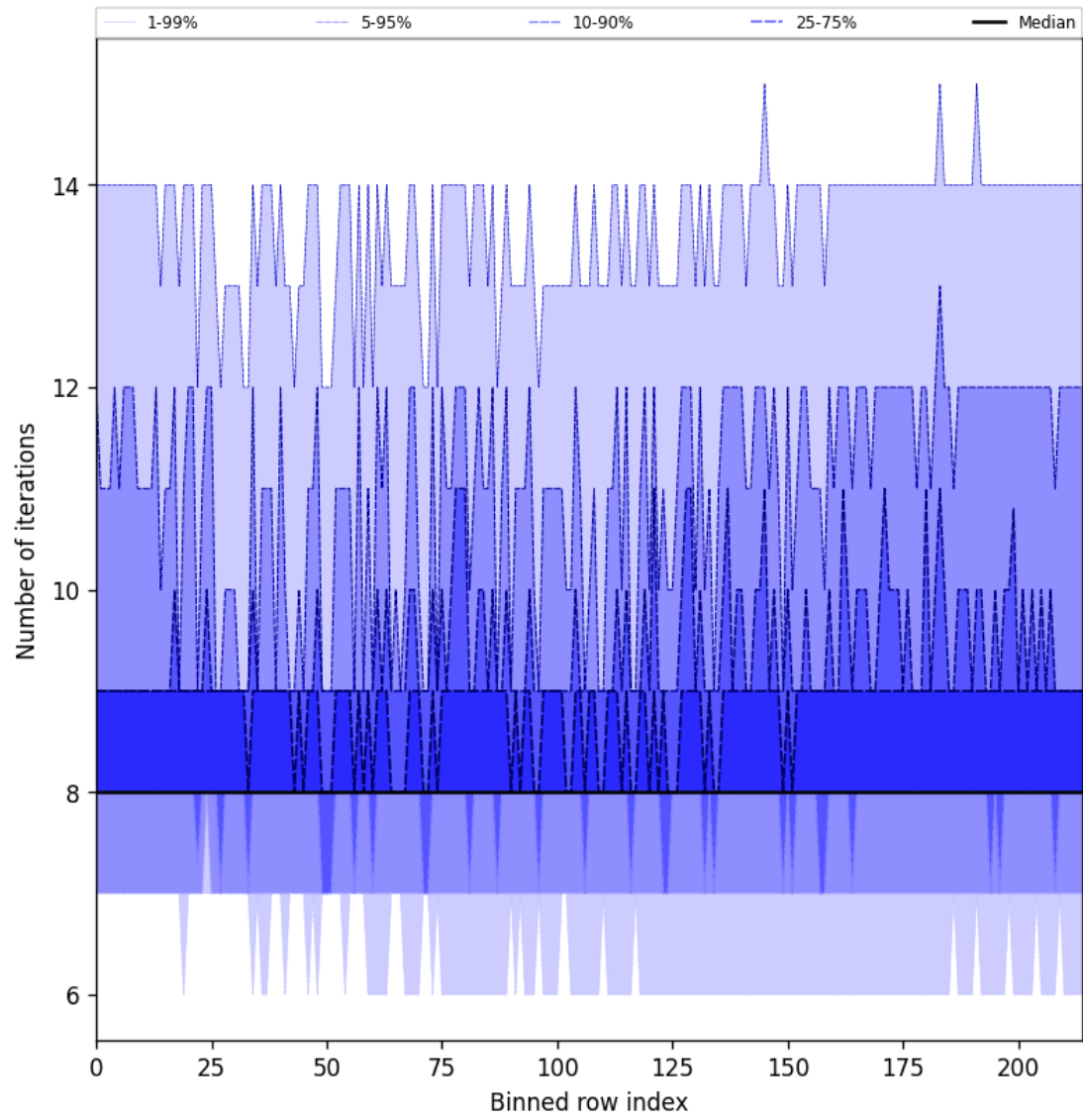
Figure 32: Along track statistics of “Number of iterations” for 2025-03-07 to 2025-03-08
