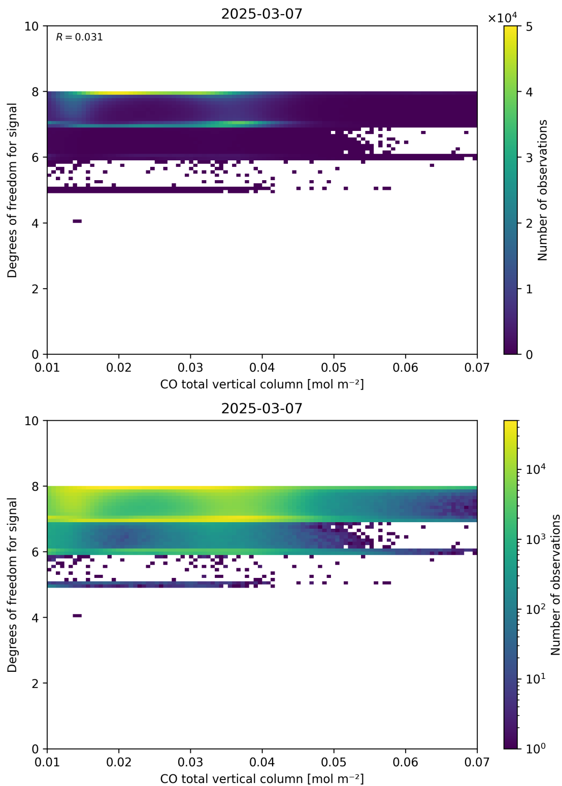
Figure 41: Scatter density plot of “CO total vertical column” against “Degrees of freedom for signal” for 2025-03-07 to 2025-03-08.
