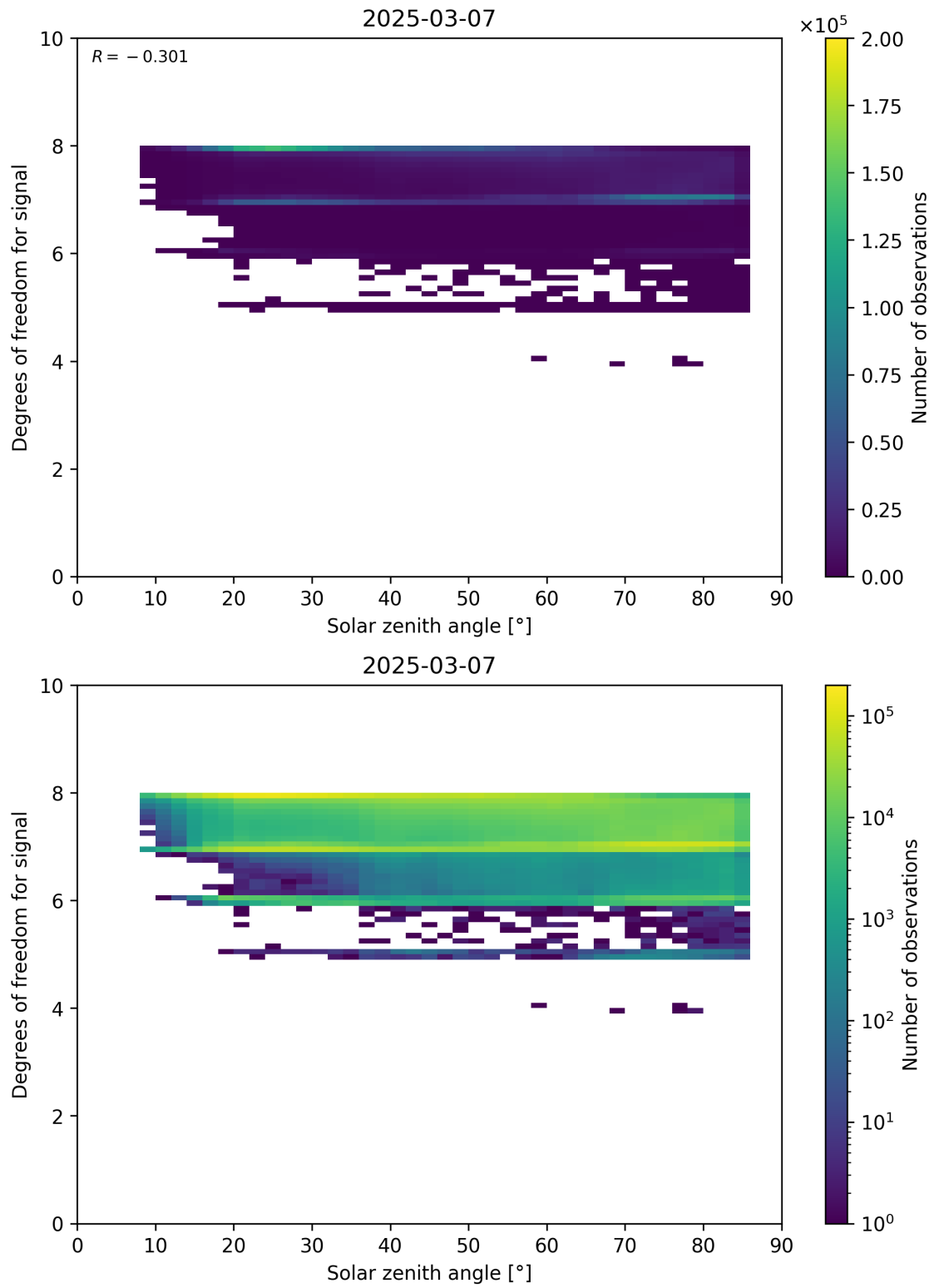
Figure 65: Scatter density plot of “Solar zenith angle” against “Degrees of freedom for signal” for 2025-03-07 to 2025-03-08.
