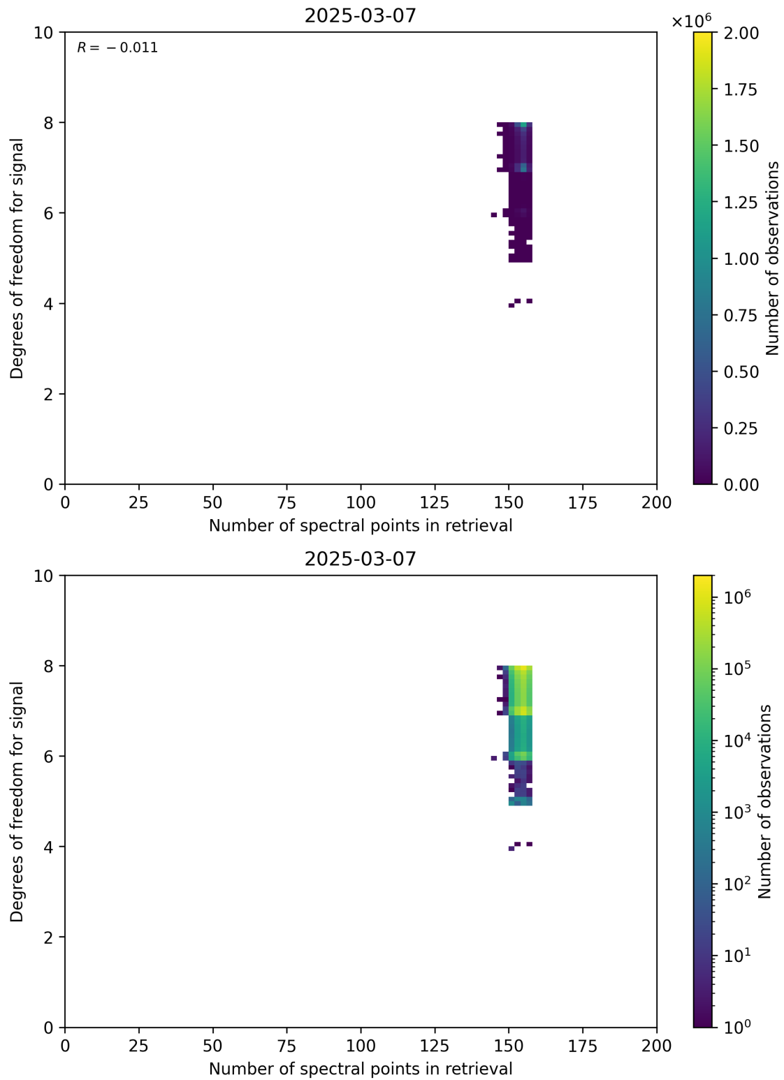
Figure 59: Scatter density plot of “Number of spectral points in retrieval” against “Degrees of freedom for signal” for 2025-03-07 to 2025-03-08.
