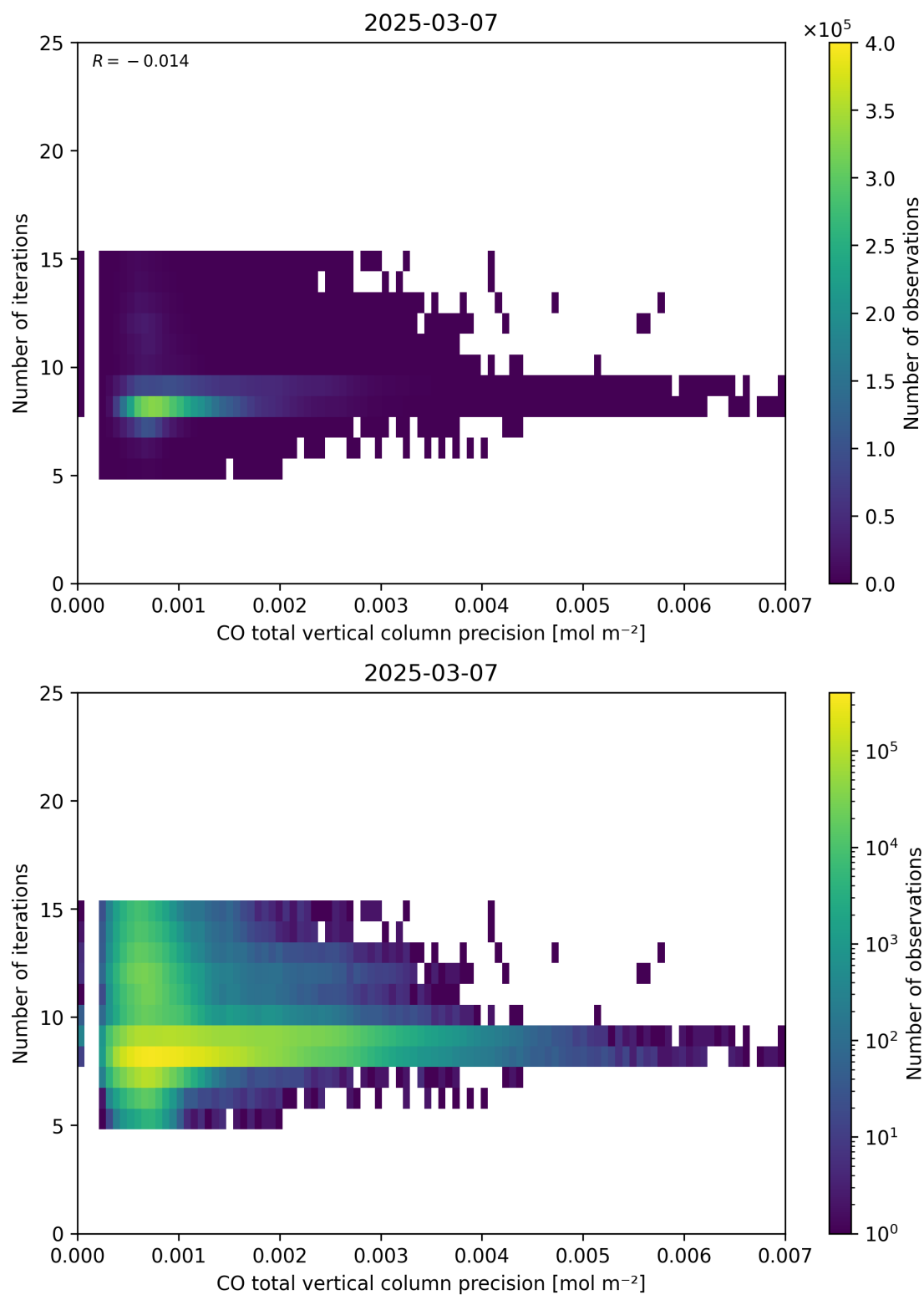
Figure 46: Scatter density plot of “CO total vertical column precision” against “Number of iterations” for 2025-03-07 to 2025-03-08.
