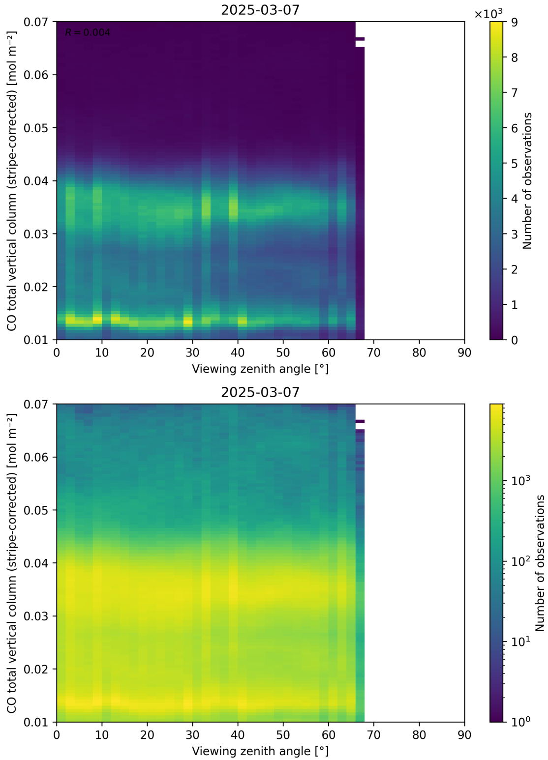
Figure 70: Scatter density plot of “Viewing zenith angle” against “CO total vertical column (stripe-corrected)” for 2025-03-07 to 2025-03-08.
