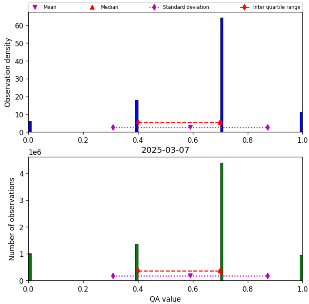
Figure 17: Histogram of “QA value” for 2025-03-07 to 2025-03-08
