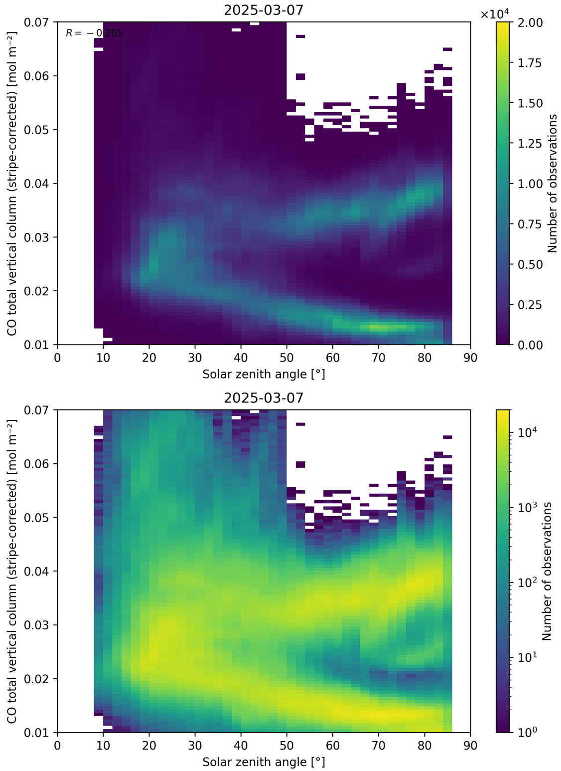
Figure 62: Scatter density plot of “Solar zenith angle” against “CO total vertical column (stripe-corrected)” for 2025-03-07 to 2025-03-08.
