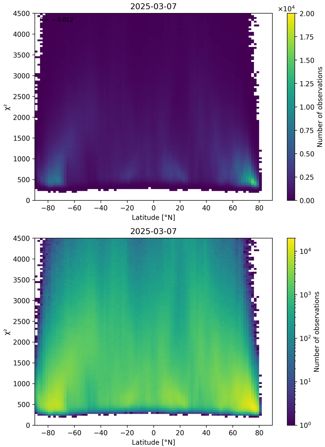
Figure 54: Scatter density plot of “Latitude” against “ \chi^2 ” for 2025-03-07 to 2025-03-08.
