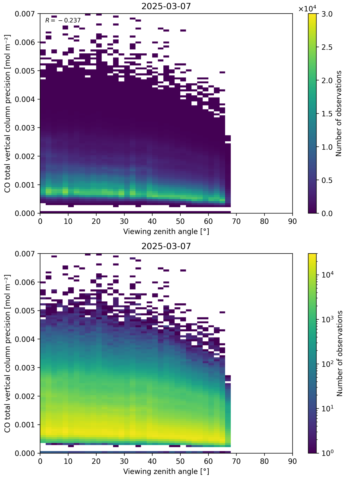
Figure 71: Scatter density plot of “Viewing zenith angle” against “CO total vertical column precision” for 2025-03-07 to 2025-03-08.
