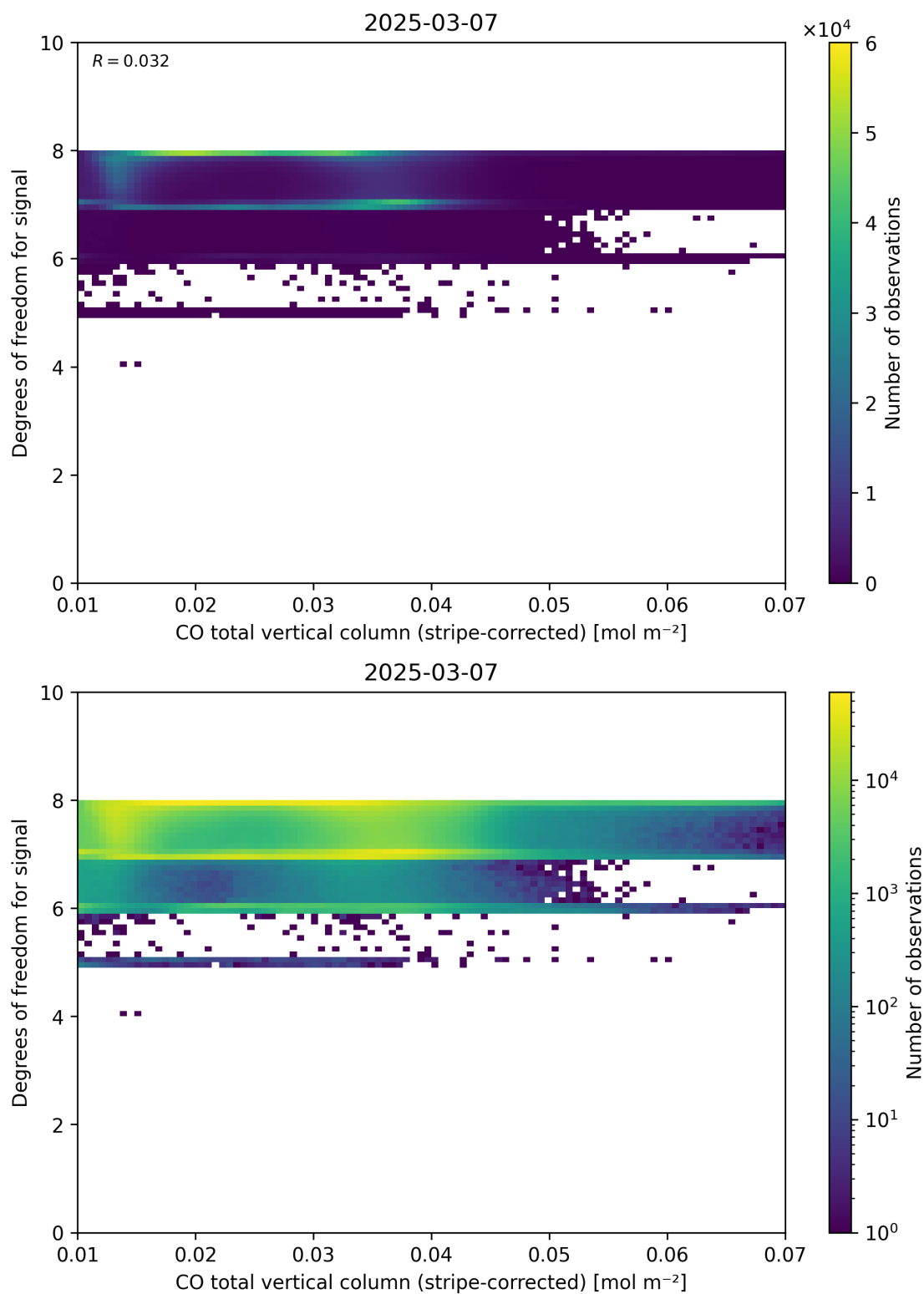
Figure 38: Scatter density plot of “CO total vertical column (stripe-corrected)” against “Degrees of freedom for signal” for 2025-03-07 to 2025-03-08.
