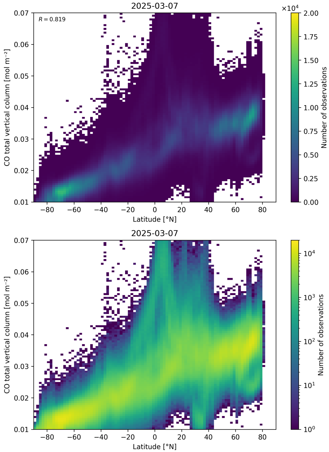
Figure 51: Scatter density plot of “Latitude” against “CO total vertical column” for 2025-03-07 to 2025-03-08.
