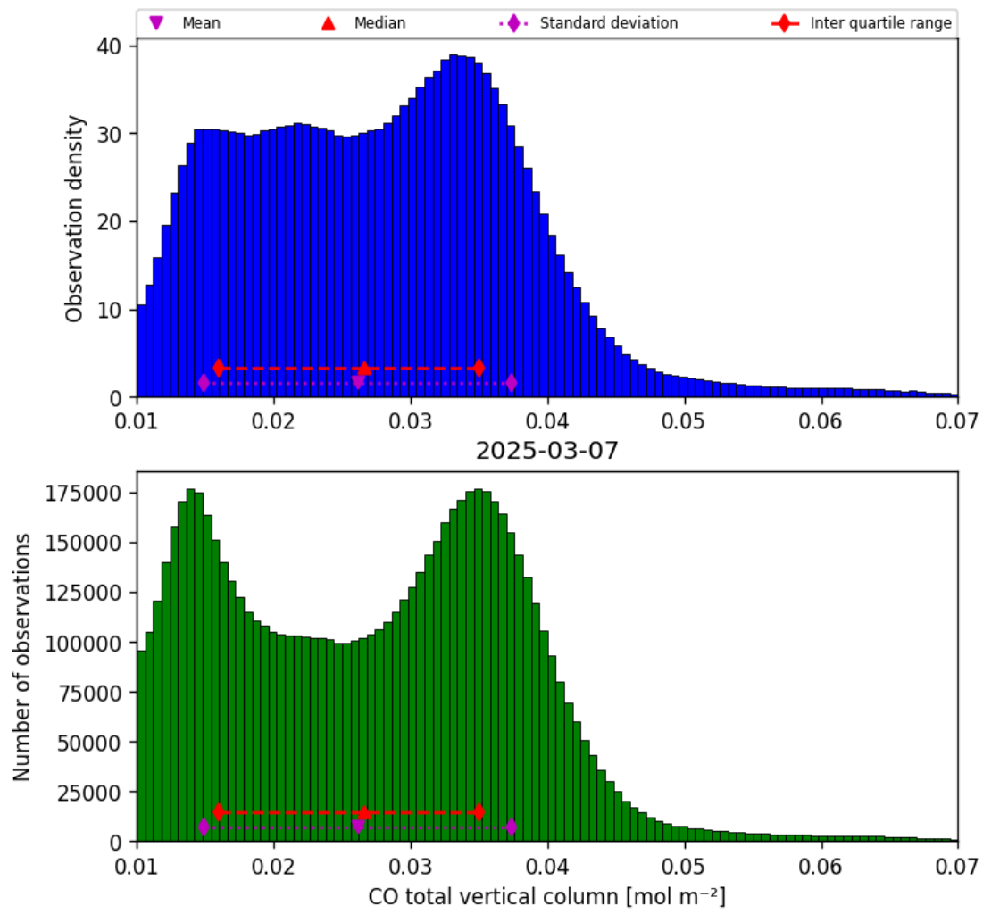
Figure 18: Histogram of “CO total vertical column” for 2025-03-07 to 2025-03-08
