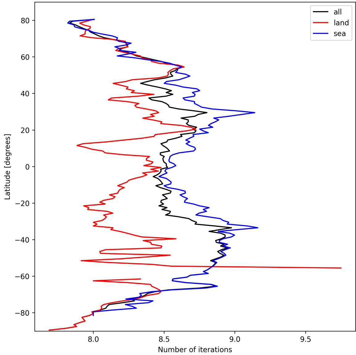
Figure 16: Zonal average of “Number of iterations” for 2025-03-07 to 2025-03-08.
