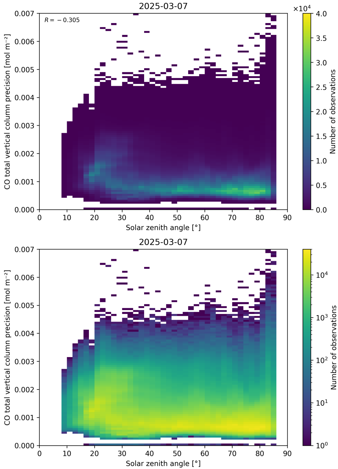
Figure 63: Scatter density plot of “Solar zenith angle” against “CO total vertical column precision” for 2025-03-07 to 2025-03-08.
