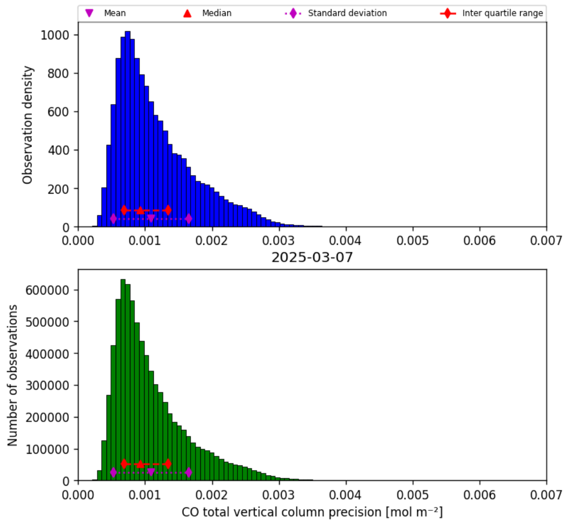
Figure 20: Histogram of “CO total vertical column precision” for 2025-03-07 to 2025-03-08
