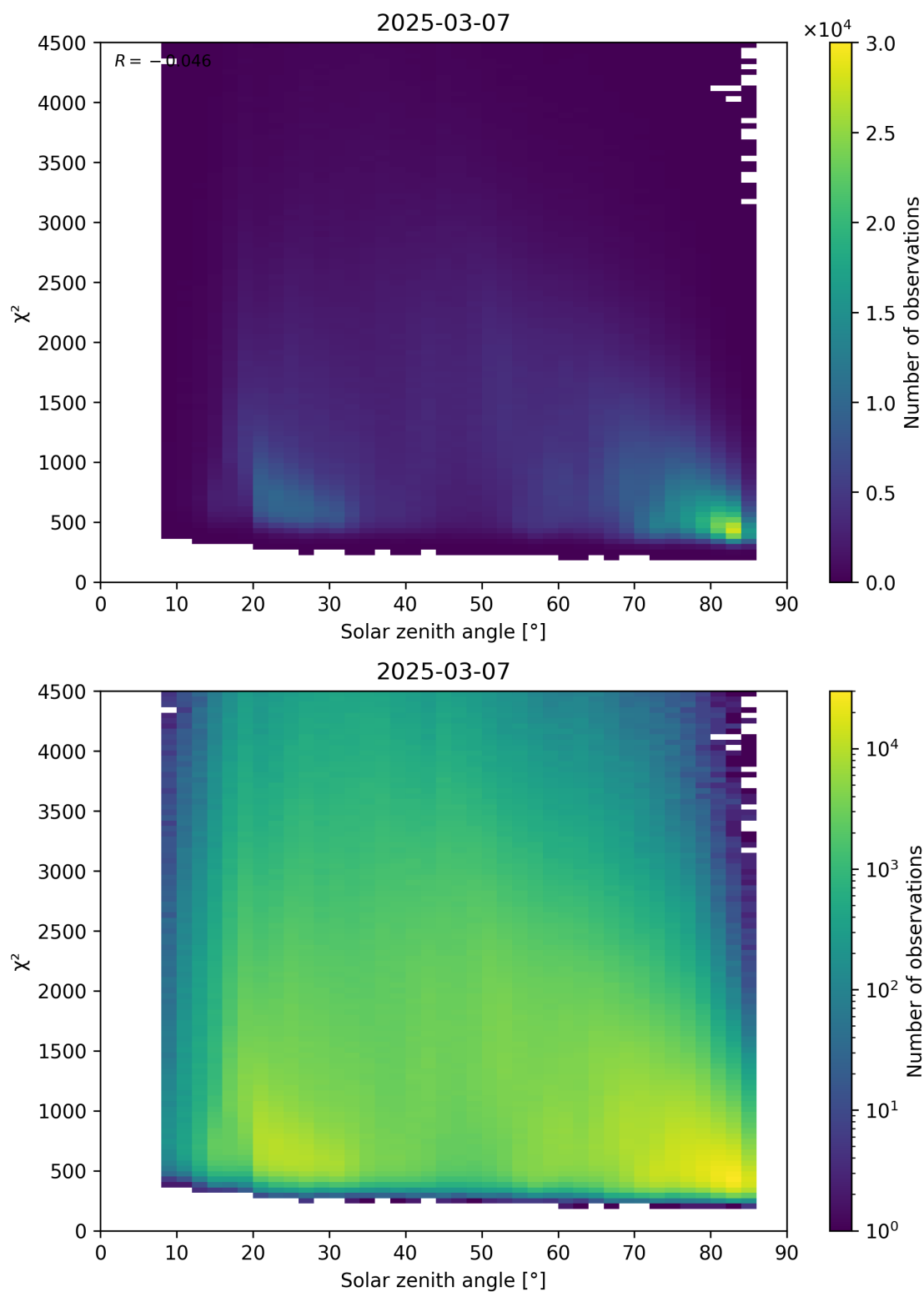
Figure 64: Scatter density plot of “Solar zenith angle” against “ \chi^2 ” for 2025-03-07 to 2025-03-08.
