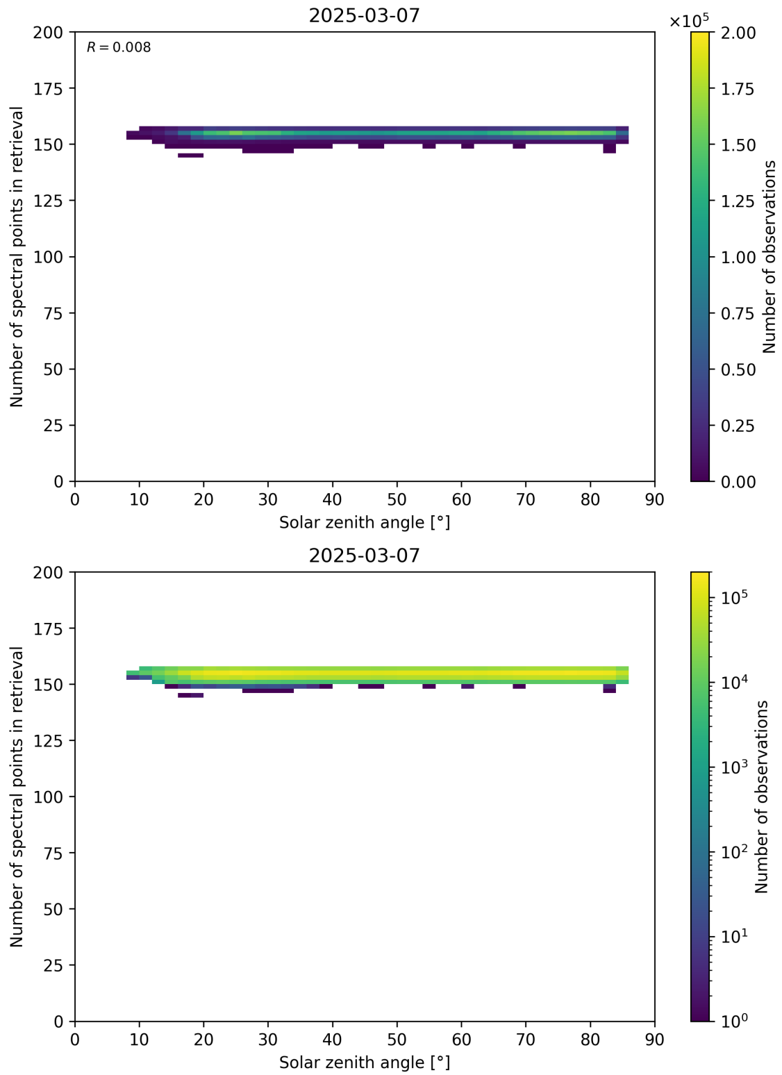
Figure 68: Scatter density plot of “Solar zenith angle” against “Number of spectral points in retrieval” for 2025-03-07 to 2025-03-08.
