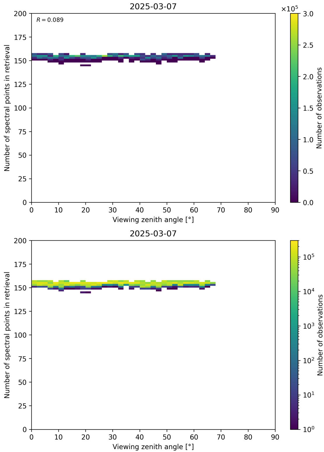
Figure 76: Scatter density plot of “Viewing zenith angle” against “Number of spectral points in retrieval” for 2025-03-07 to 2025-03-08.
