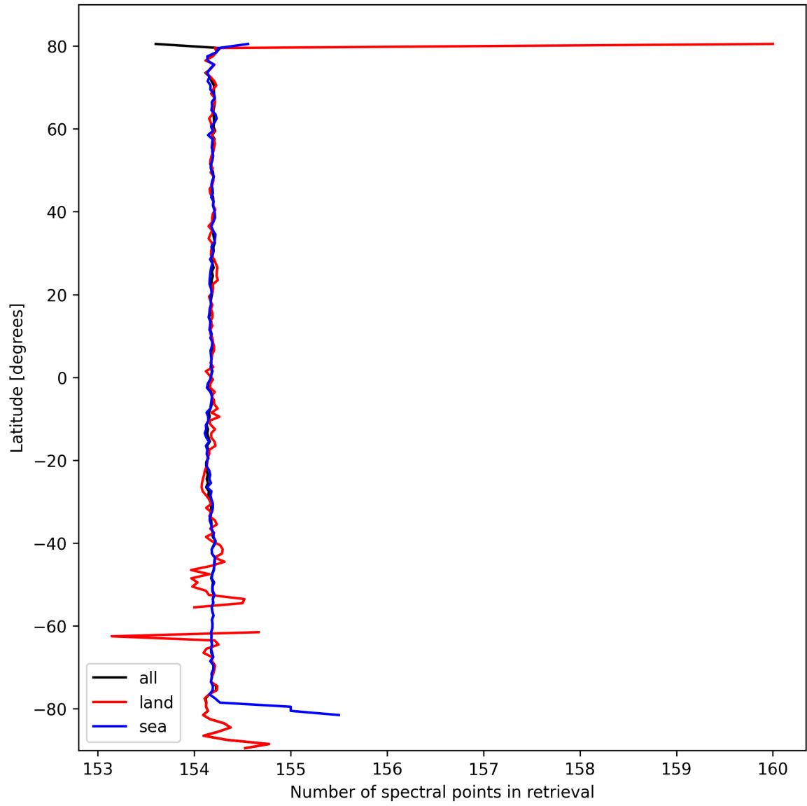
Figure 13: Zonal average of “Number of spectral points in retrieval” for 2025-03-07 to 2025-03-08.
