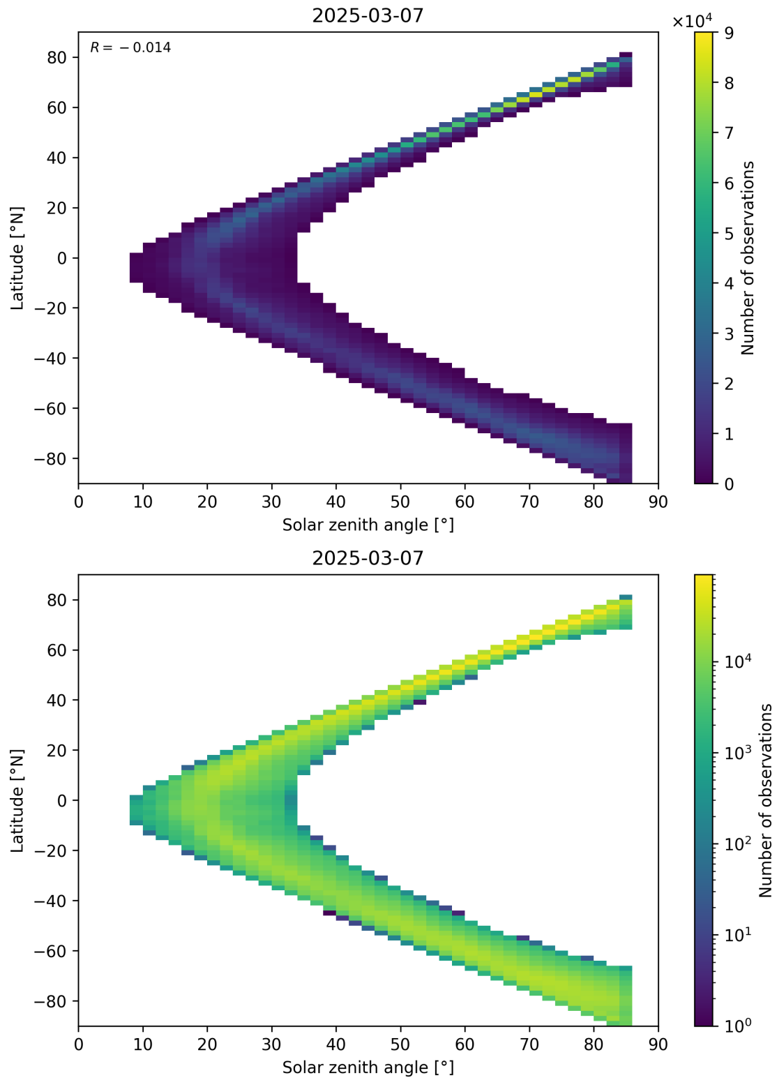
Figure 66: Scatter density plot of “Solar zenith angle” against “Latitude” for 2025-03-07 to 2025-03-08.
