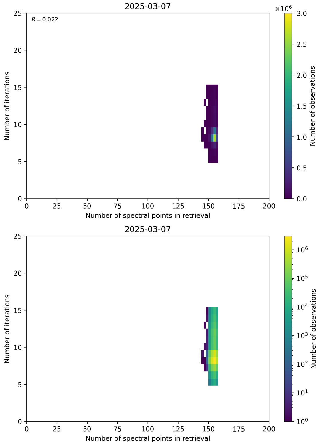
Figure 60: Scatter density plot of “Number of spectral points in retrieval” against “Number of iterations” for 2025-03-07 to 2025-03-08.
