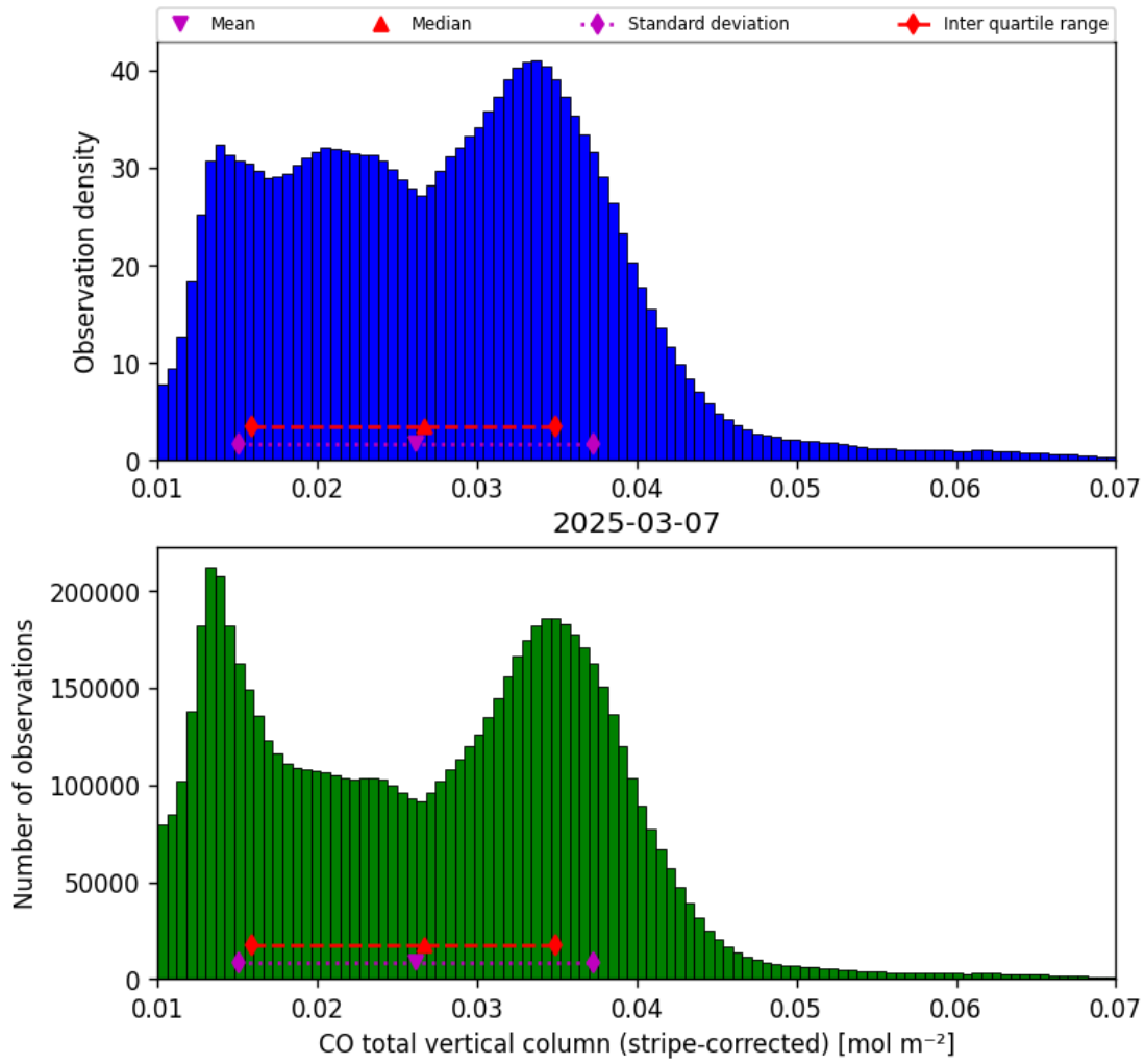
Figure 19: Histogram of “CO total vertical column (stripe-corrected)” for 2025-03-07 to 2025-03-08
