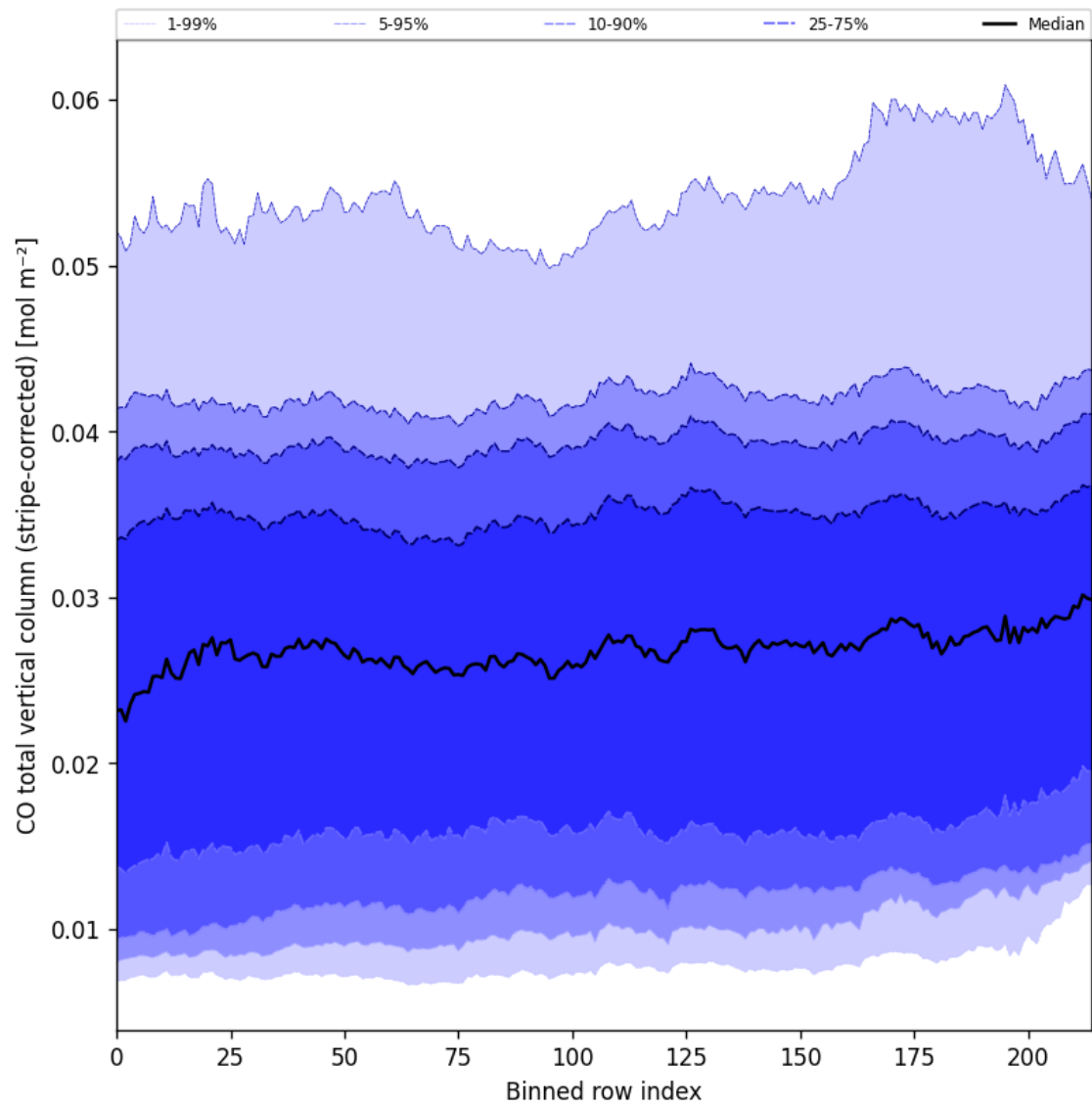
Figure 27: Along track statistics of “CO total vertical column (stripe-corrected)” for 2025-03-07 to 2025-03-08
