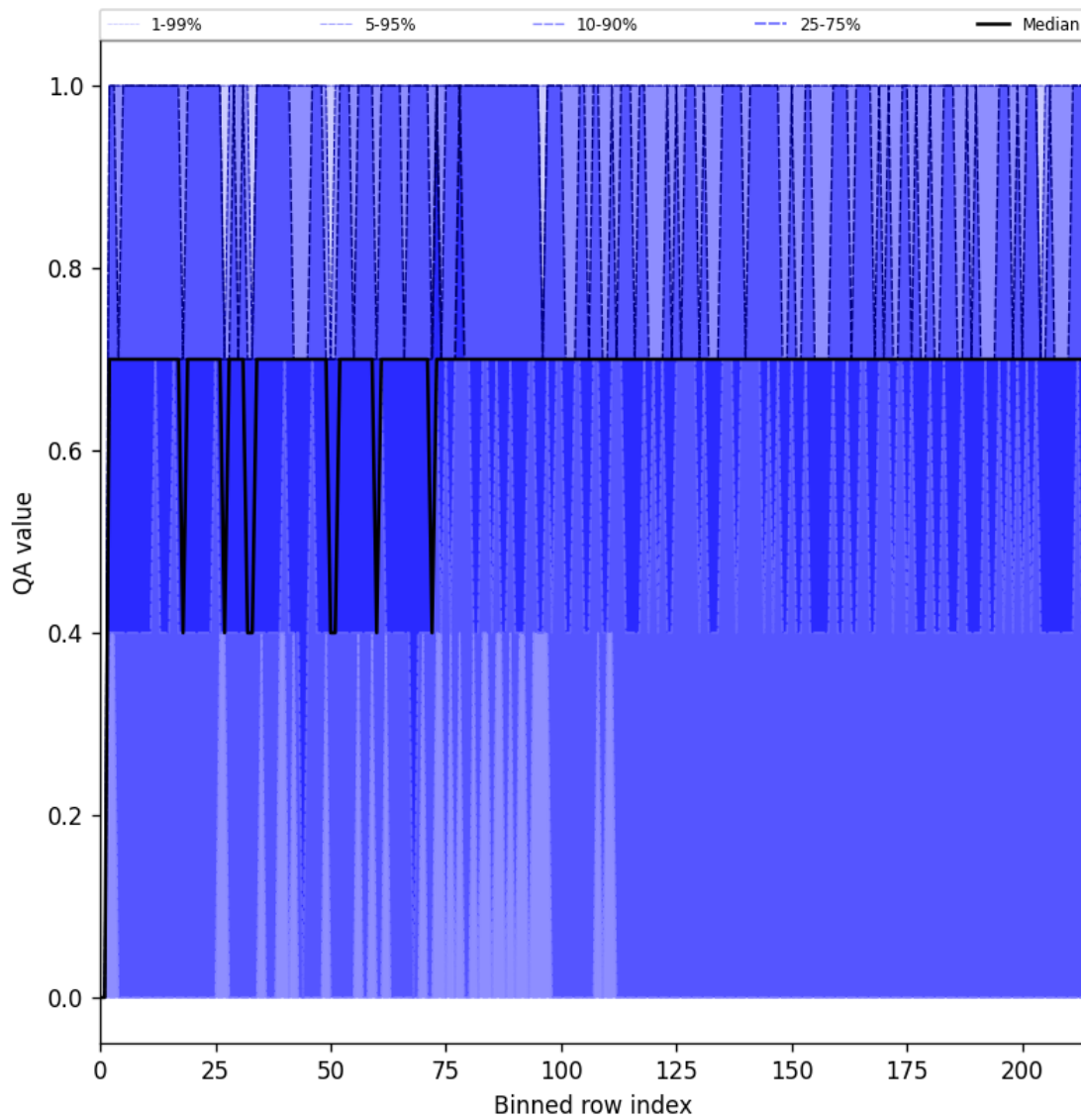
Figure 25: Along track statistics of “QA value” for 2025-03-07 to 2025-03-08
