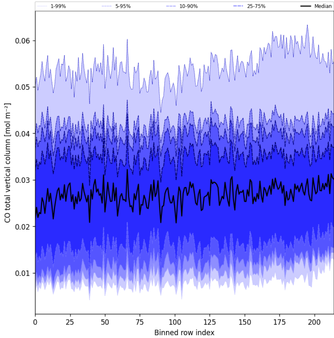
Figure 26: Along track statistics of “CO total vertical column” for 2025-03-07 to 2025-03-08
