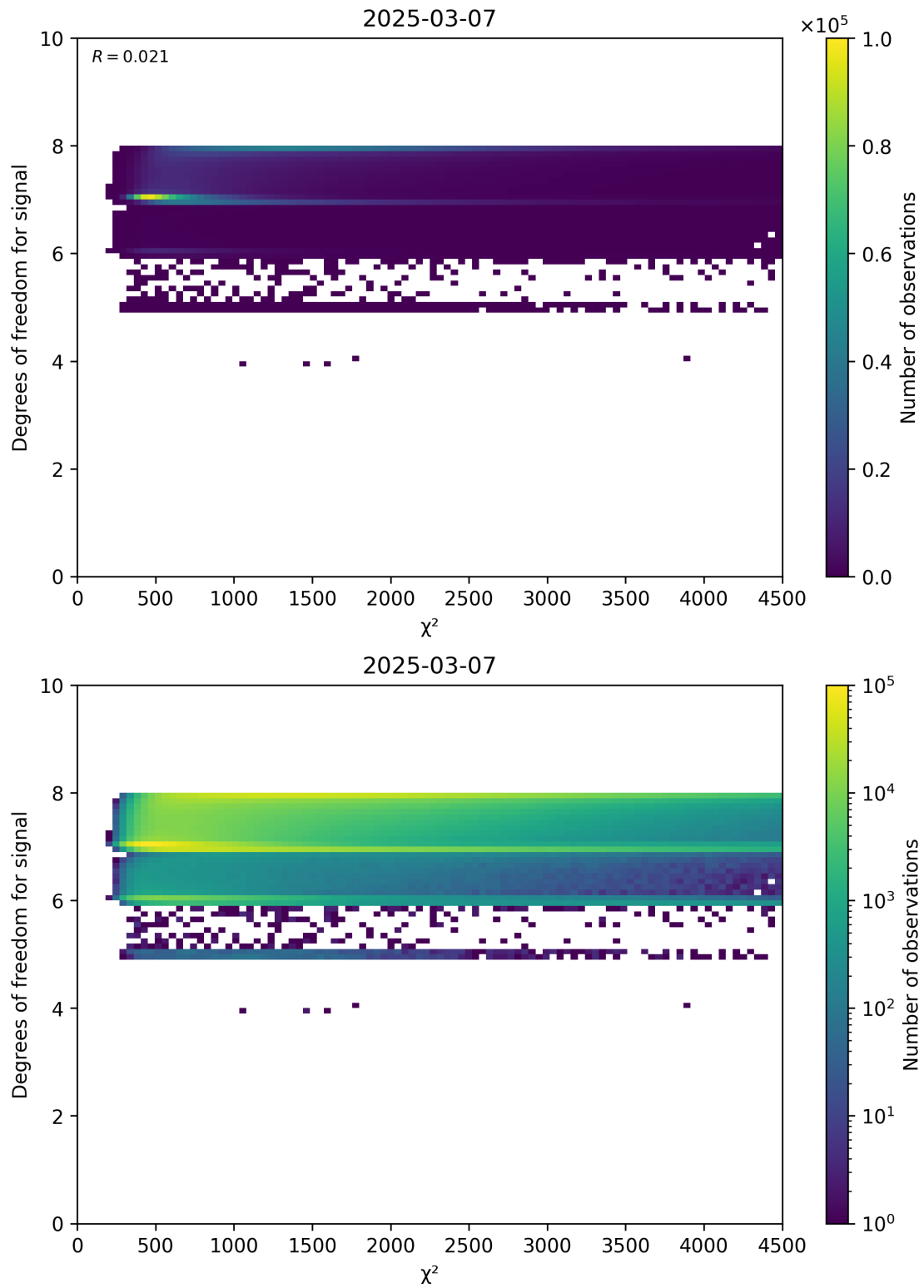
Figure 48: Scatter density plot of “ \chi^2 ” against “Degrees of freedom for signal” for 2025-03-07 to 2025-03-08.
