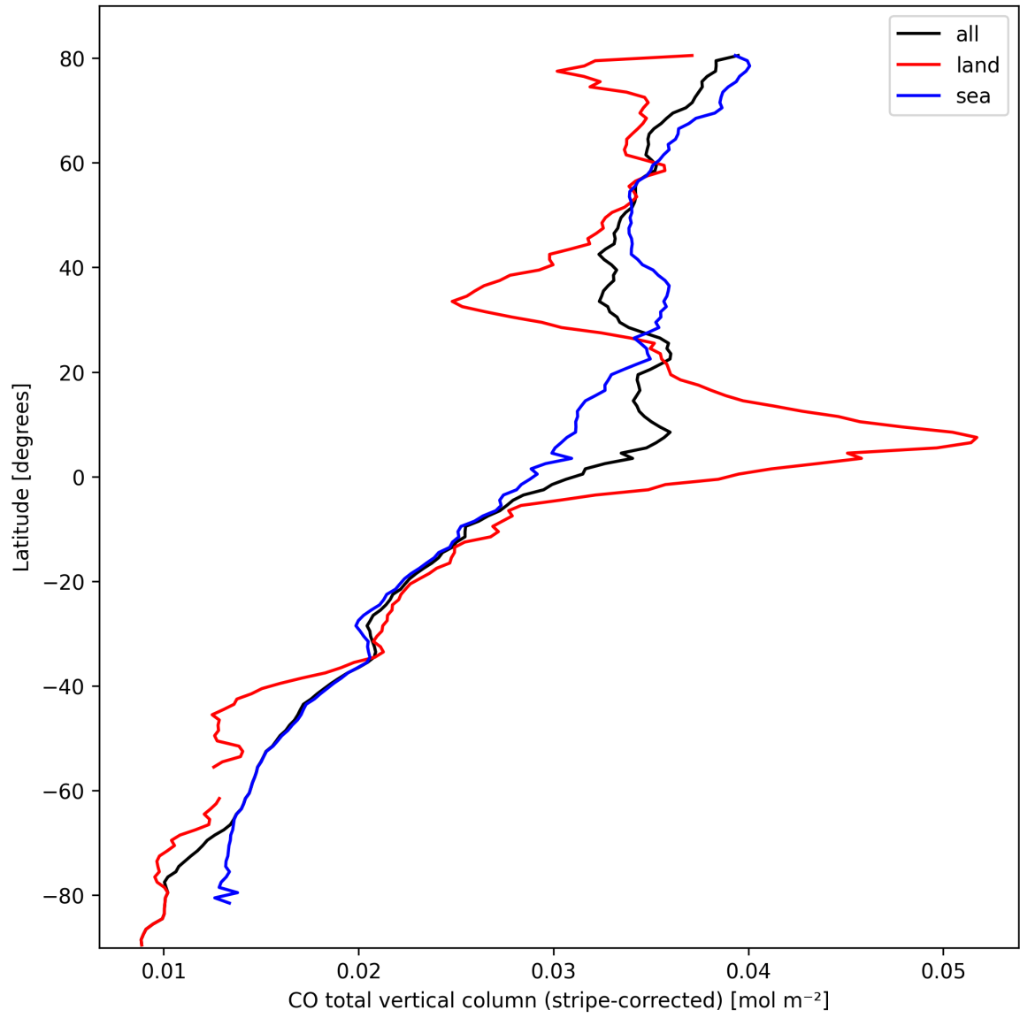
Figure 11: Zonal average of “CO total vertical column (stripe-corrected)” for 2025-03-07 to 2025-03-08.
