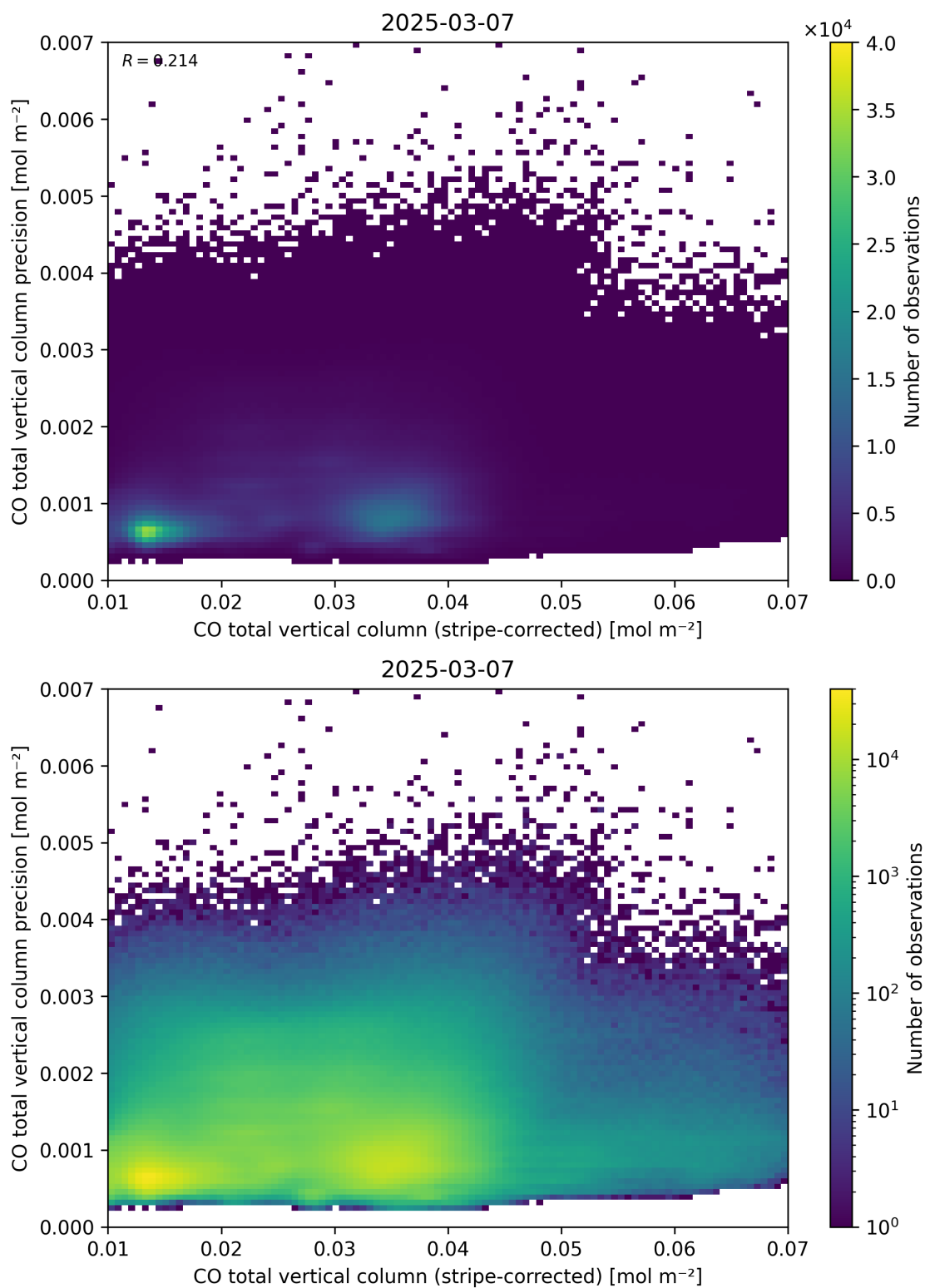
Figure 36: Scatter density plot of “CO total vertical column (stripe-corrected)” against “CO total vertical column precision” for 2025-03-07 to 2025-03-08.
