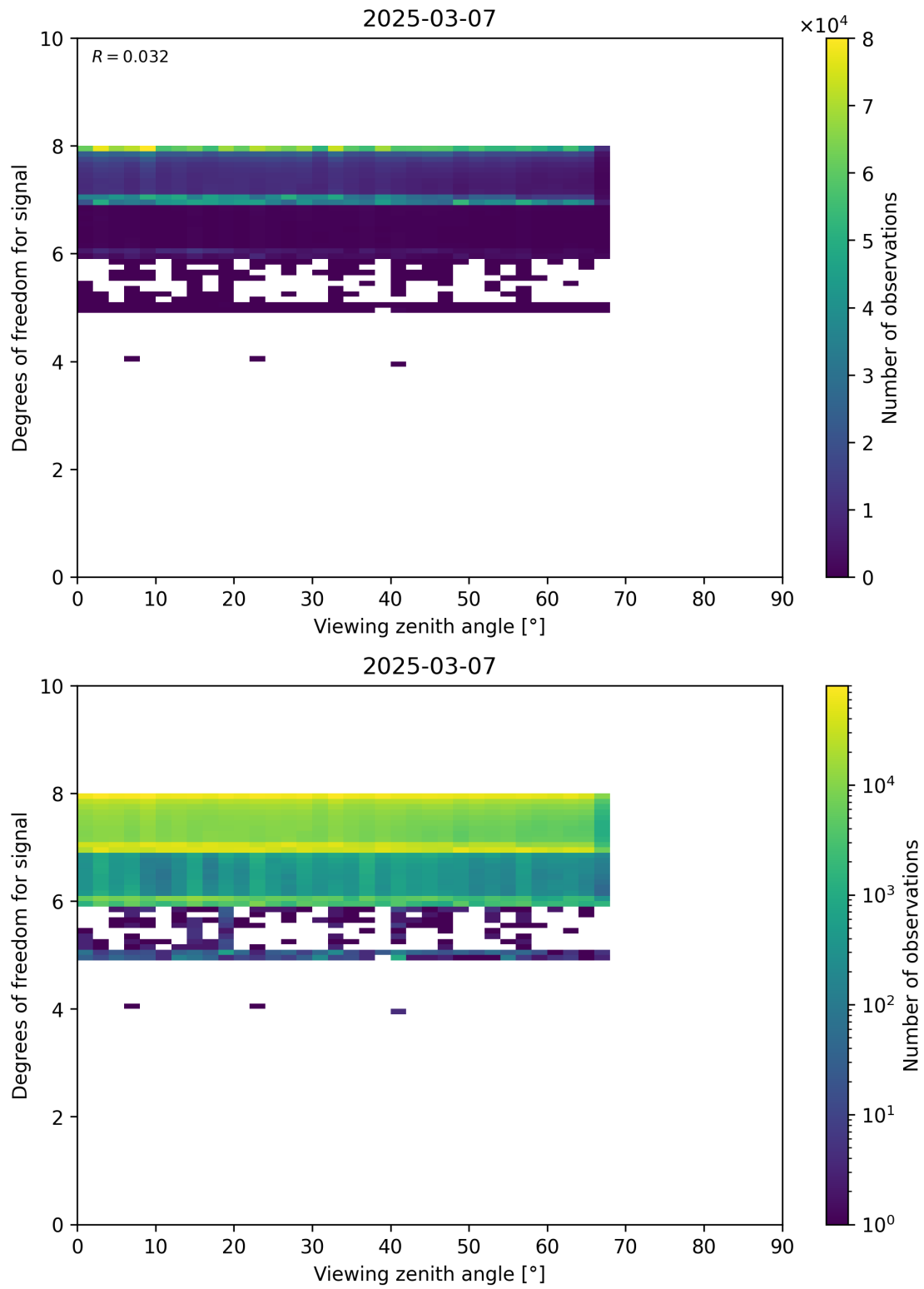
Figure 73: Scatter density plot of “Viewing zenith angle” against “Degrees of freedom for signal” for 2025-03-07 to 2025-03-08.
