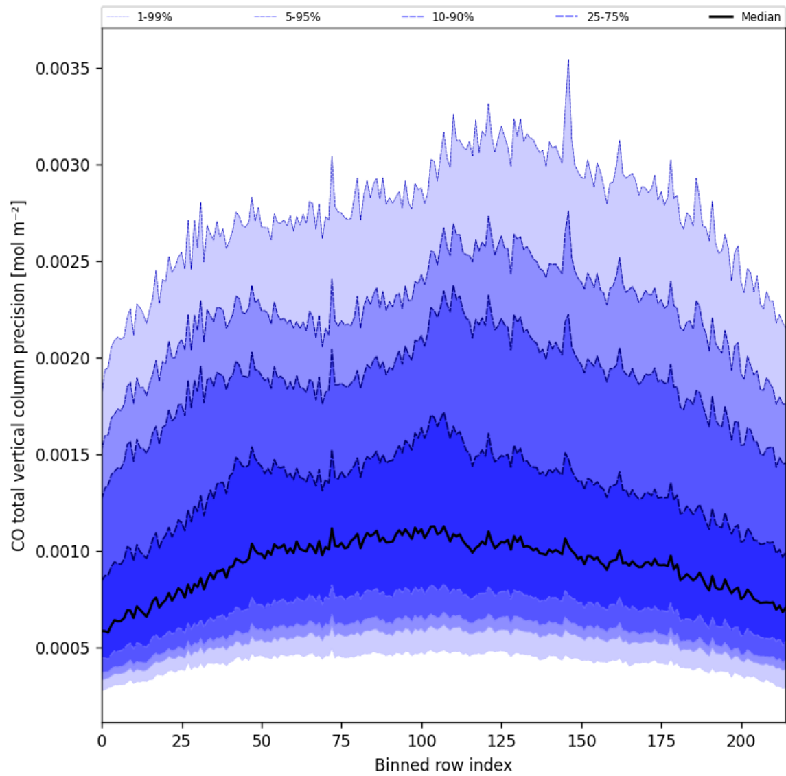
Figure 28: Along track statistics of “CO total vertical column precision” for 2025-03-07 to 2025-03-08
