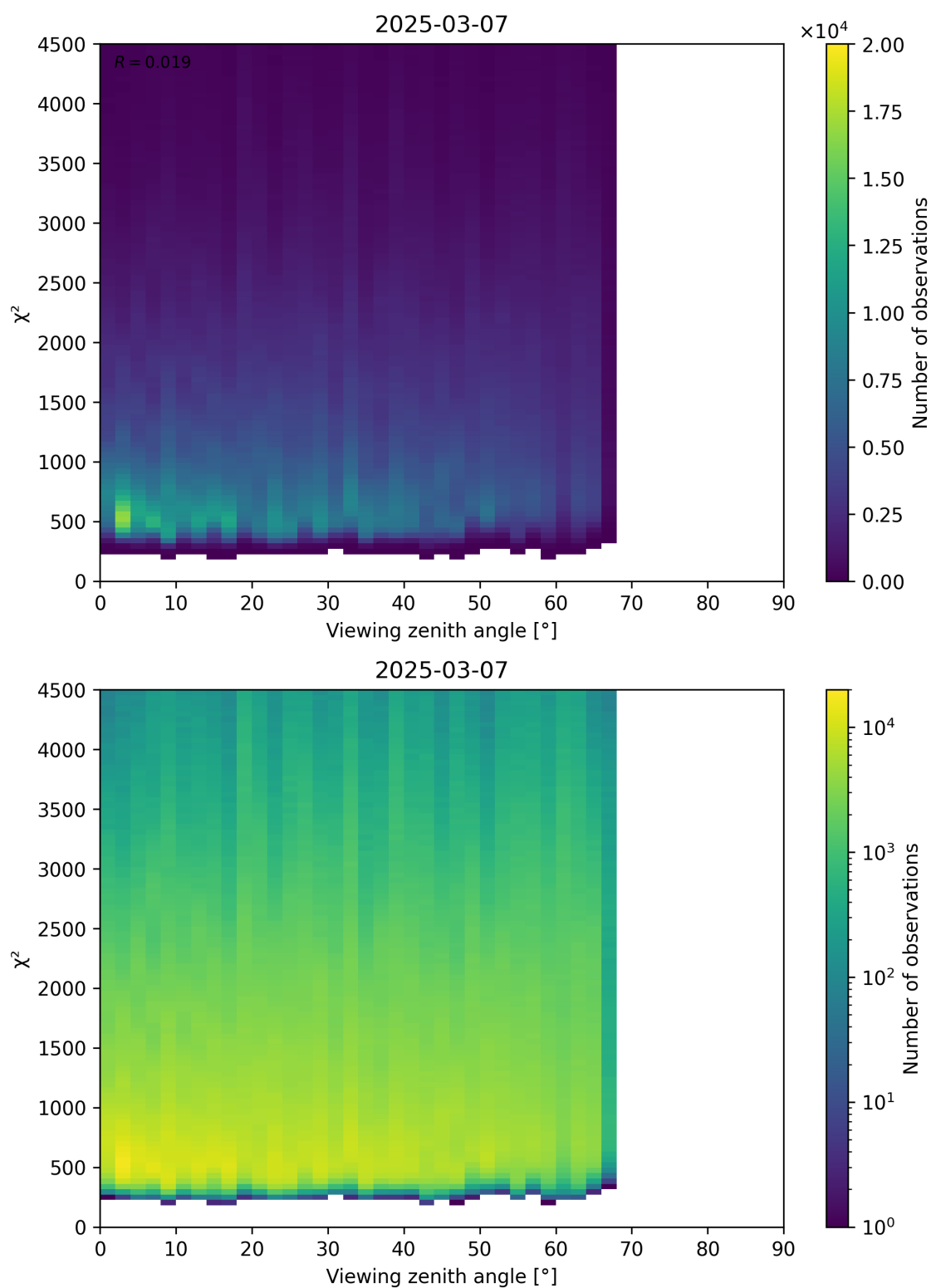
Figure 72: Scatter density plot of “Viewing zenith angle” against “ \chi^2 ” for 2025-03-07 to 2025-03-08.
