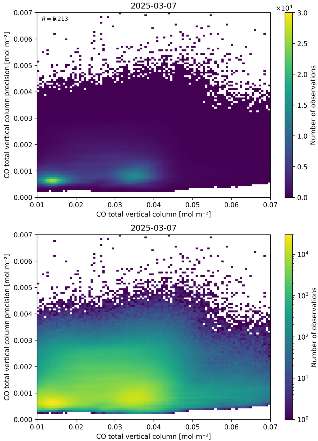
Figure 34: Scatter density plot of “CO total vertical column” against “CO total vertical column precision” for 2025-03-07 to 2025-03-08.
