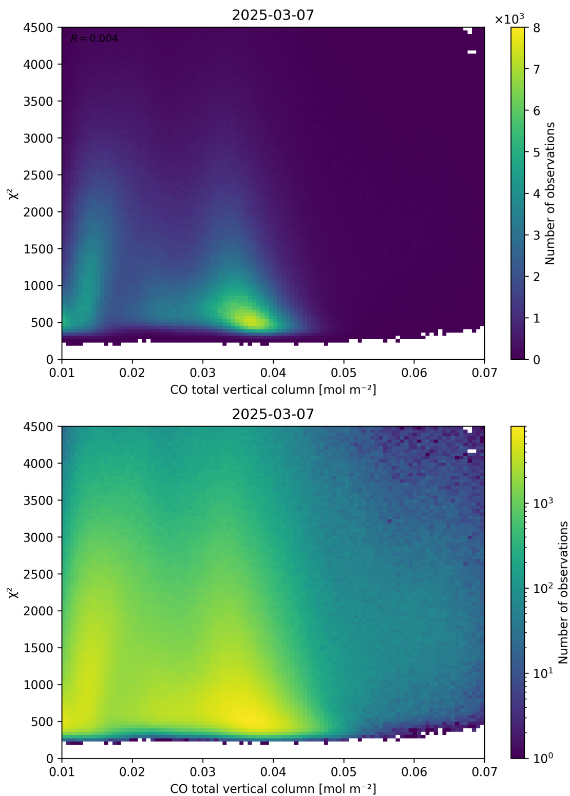
Figure 35: Scatter density plot of “CO total vertical column” against “ \chi^2 ” for 2025-03-07 to 2025-03-08.
