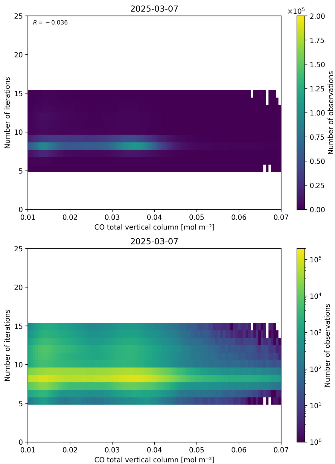
Figure 42: Scatter density plot of “CO total vertical column” against “Number of iterations” for 2025-03-07 to 2025-03-08.
