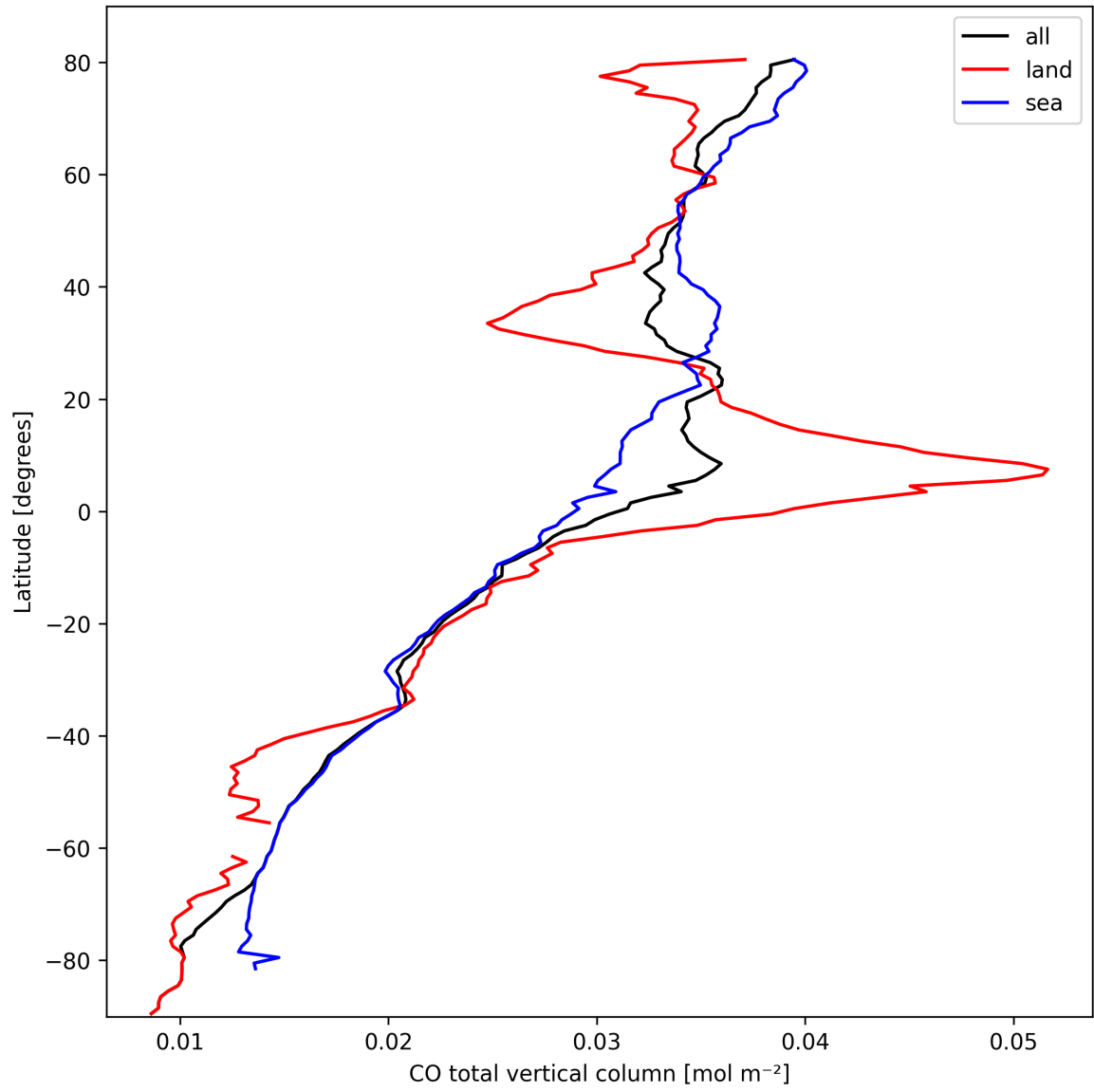
Figure 10: Zonal average of “CO total vertical column” for 2025-03-07 to 2025-03-08.
