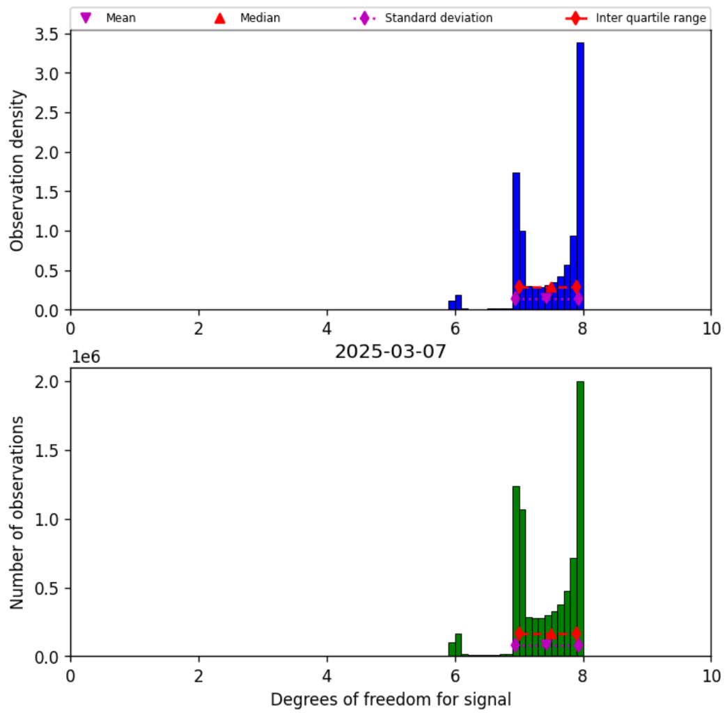
Figure 23: Histogram of “Degrees of freedom for signal” for 2025-03-07 to 2025-03-08
