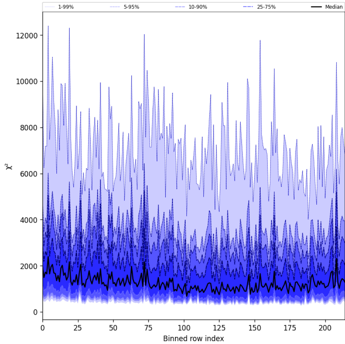
Figure 30: Along track statistics of “ \chi^2 ” for 2025-03-07 to 2025-03-08
