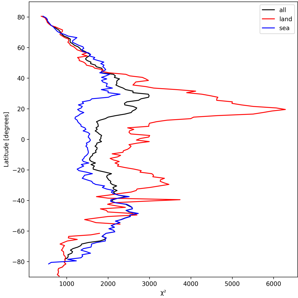
Figure 14: Zonal average of “ \chi^2 ” for 2025-03-07 to 2025-03-08.
