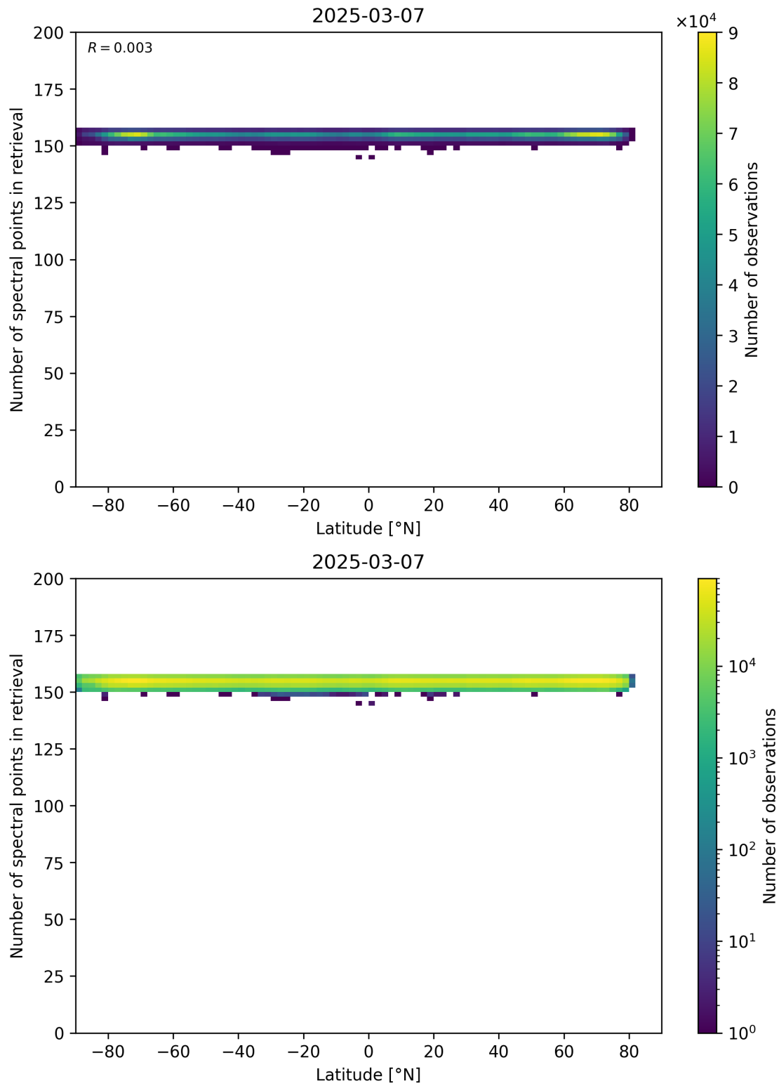
Figure 57: Scatter density plot of “Latitude” against “Number of spectral points in retrieval” for 2025-03-07 to 2025-03-08.
