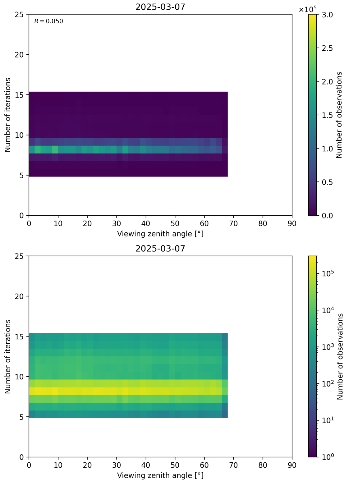
Figure 75: Scatter density plot of “Viewing zenith angle” against “Number of iterations” for 2025-03-07 to 2025-03-08.
