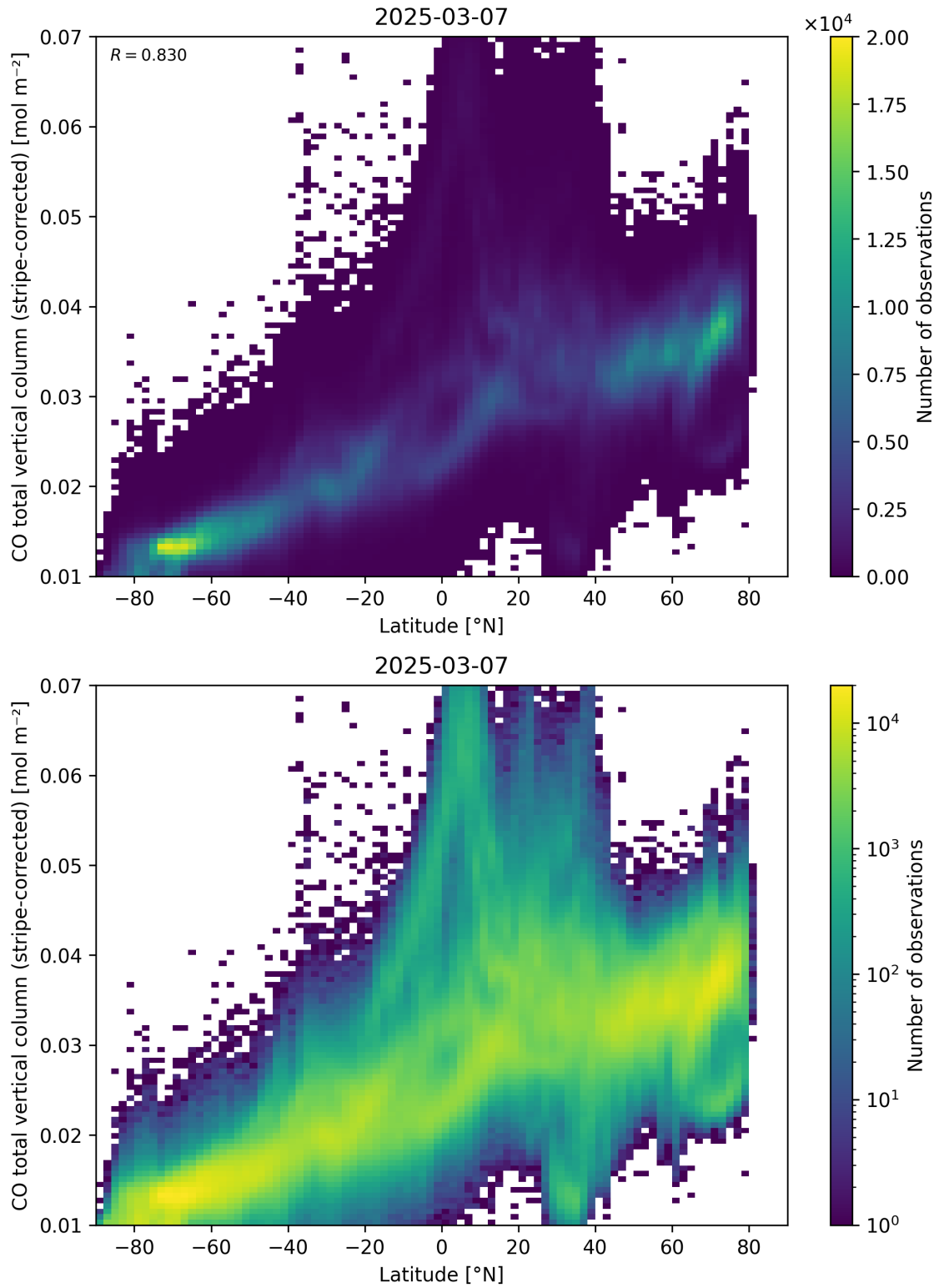
Figure 52: Scatter density plot of “Latitude” against “CO total vertical column (stripe-corrected)” for 2025-03-07 to 2025-03-08.
