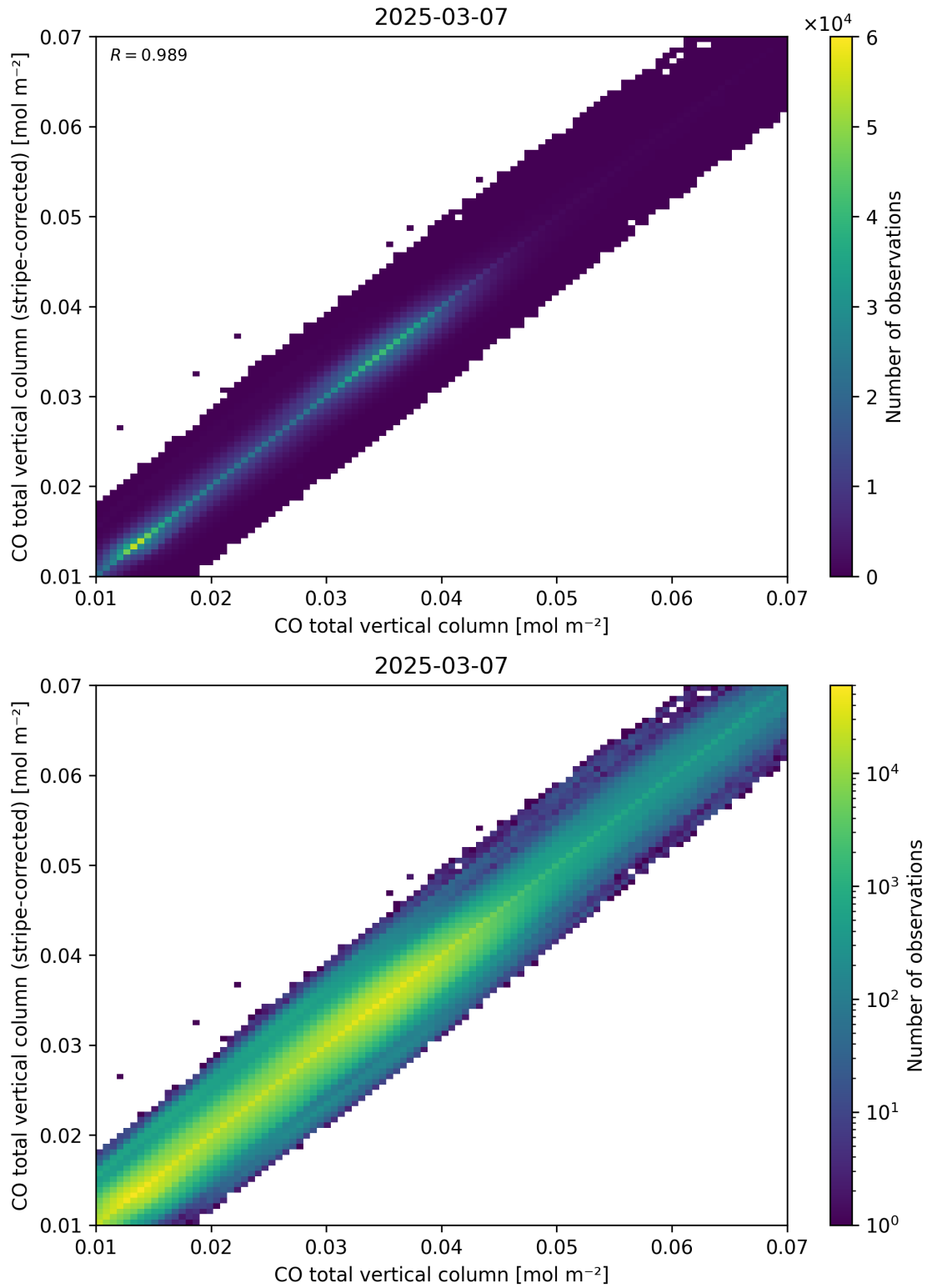
Figure 33: Scatter density plot of “CO total vertical column” against “CO total vertical column (stripe-corrected)” for 2025-03-07 to 2025-03-08.
