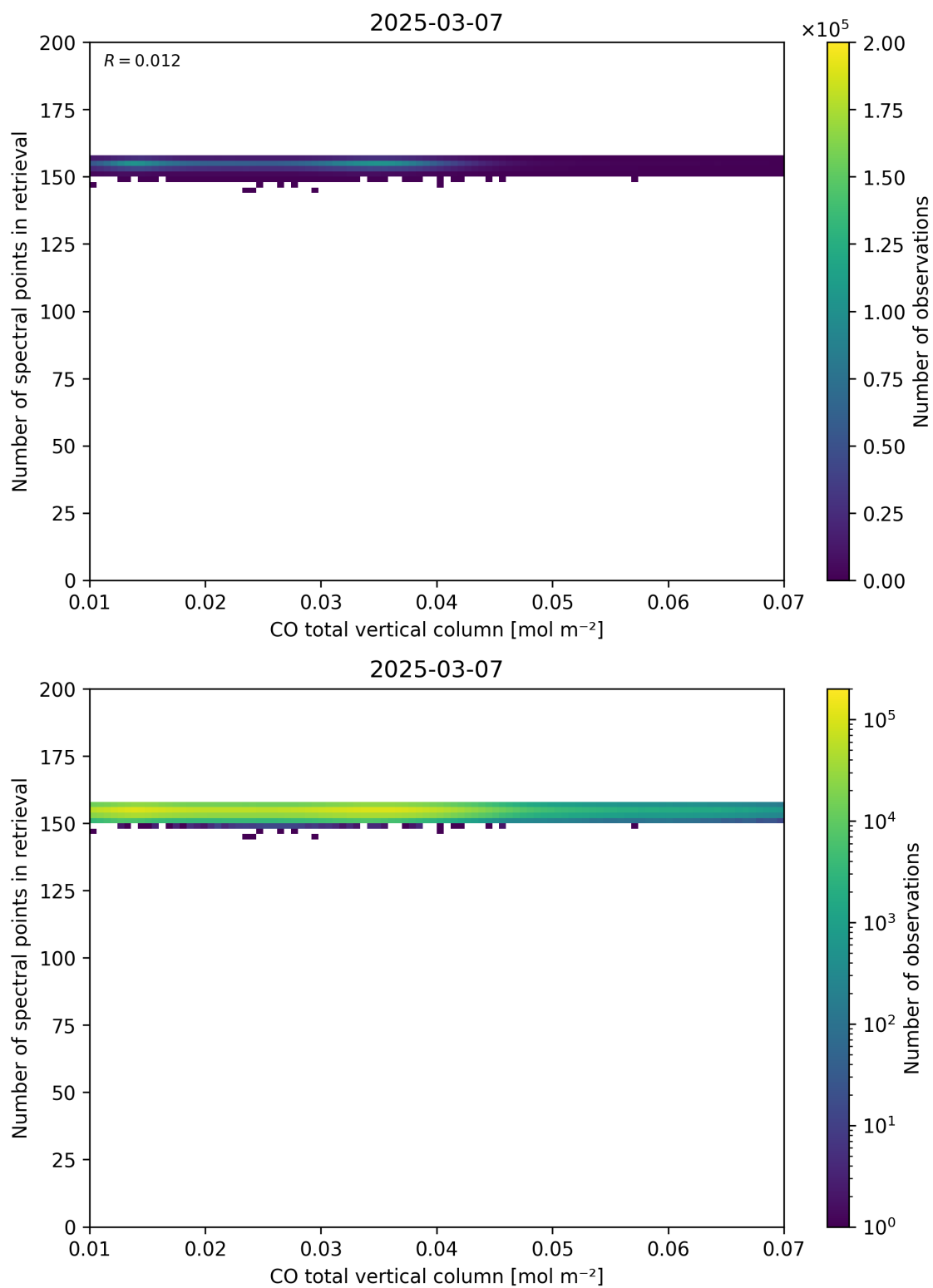
Figure 43: Scatter density plot of “CO total vertical column” against “Number of spectral points in retrieval” for 2025-03-07 to 2025-03-08.
