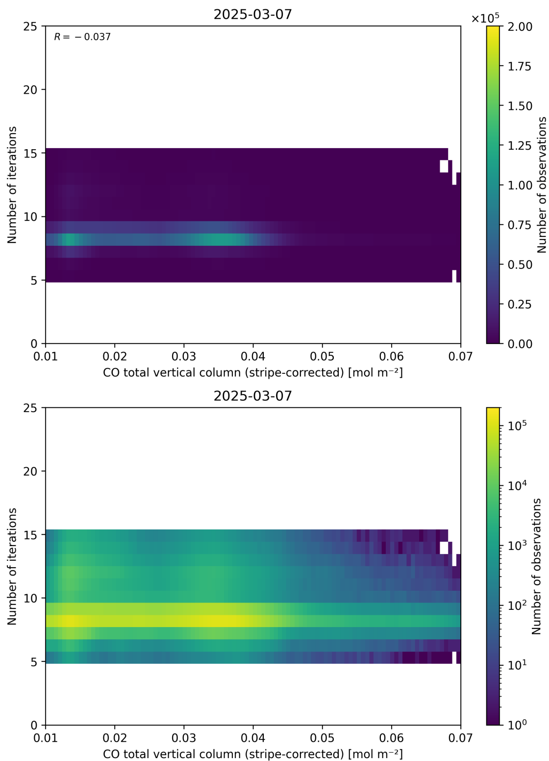
Figure 39: Scatter density plot of “CO total vertical column (stripe-corrected)” against “Number of iterations” for 2025-03-07 to 2025-03-08.
