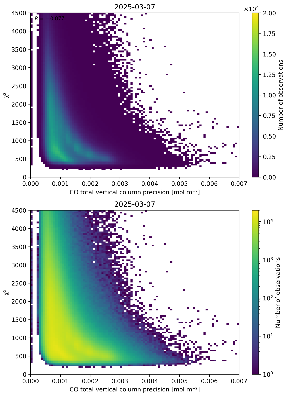
Figure 44: Scatter density plot of “CO total vertical column precision” against “ \chi^2 ” for 2025-03-07 to 2025-03-08.
