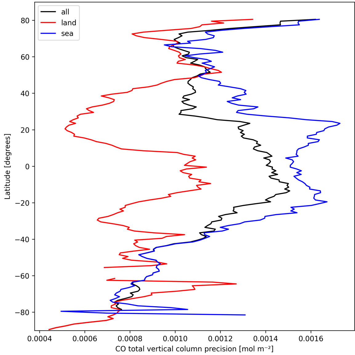
Figure 12: Zonal average of “CO total vertical column precision” for 2025-03-07 to 2025-03-08.
