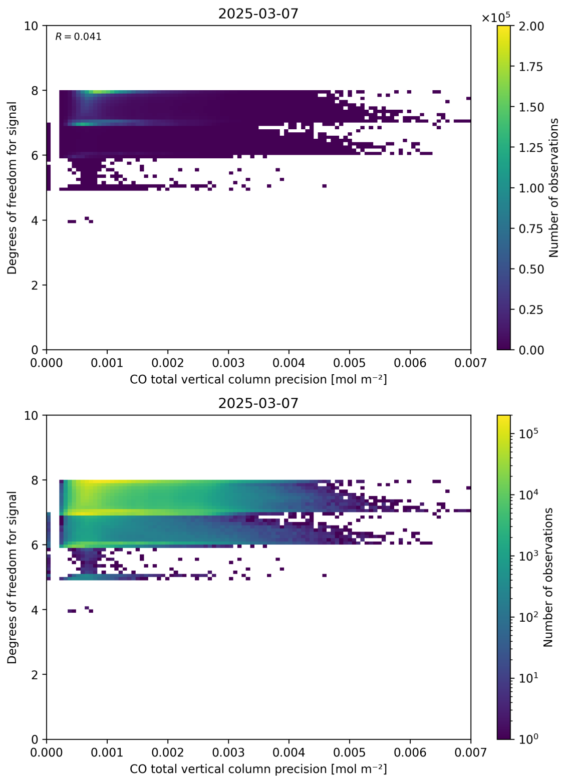
Figure 45: Scatter density plot of “CO total vertical column precision” against “Degrees of freedom for signal” for 2025-03-07 to 2025-03-08.
