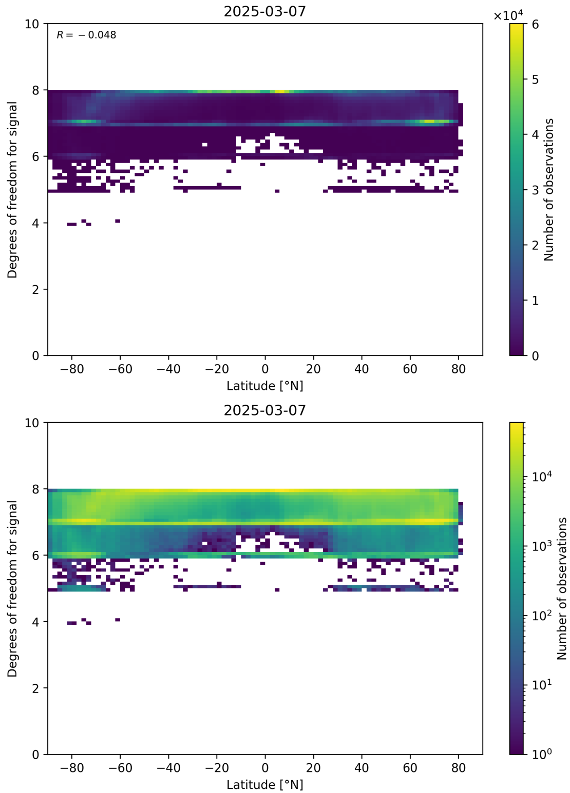
Figure 55: Scatter density plot of “Latitude” against “Degrees of freedom for signal” for 2025-03-07 to 2025-03-08.
