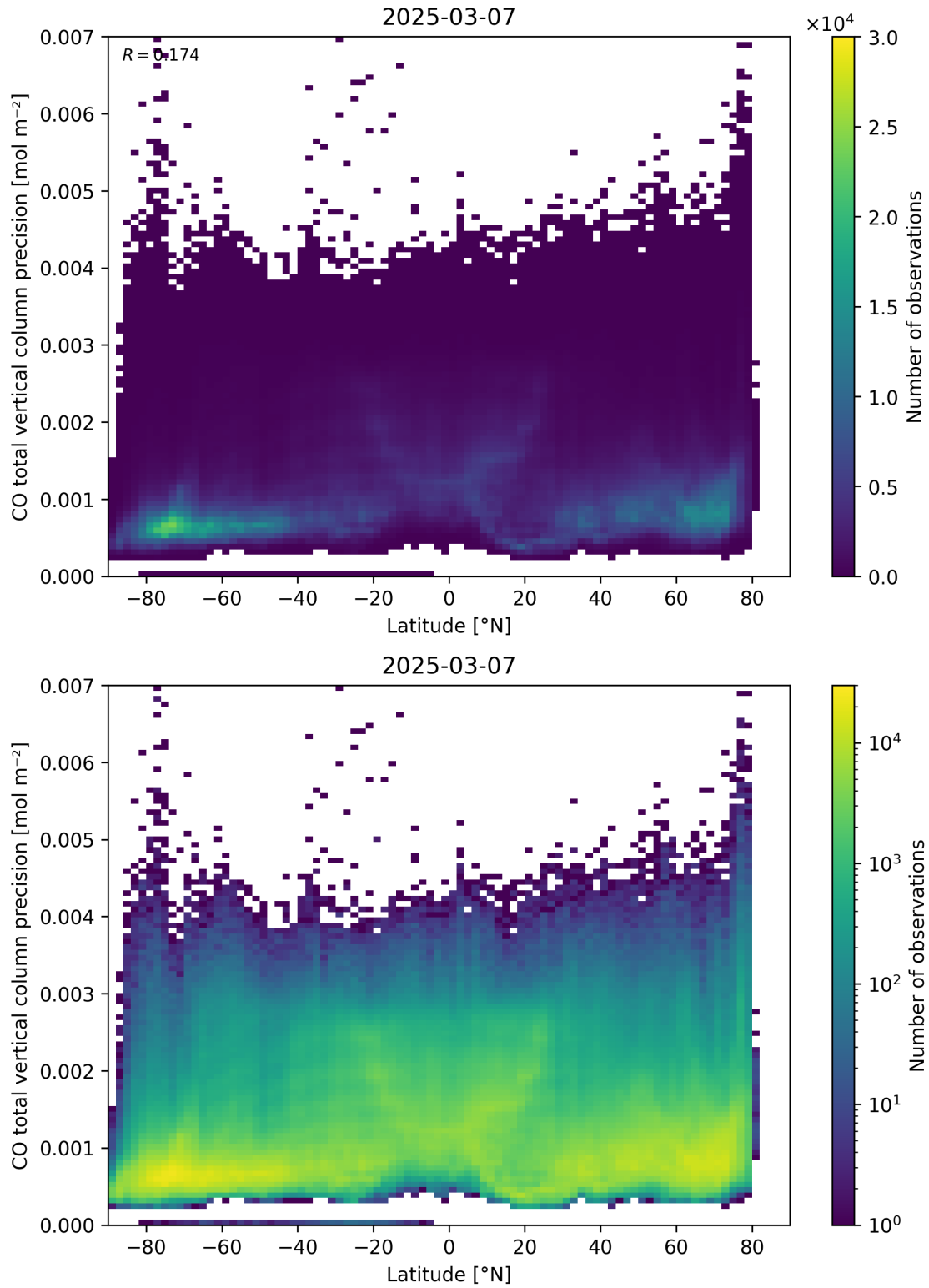
Figure 53: Scatter density plot of “Latitude” against “CO total vertical column precision” for 2025-03-07 to 2025-03-08.
