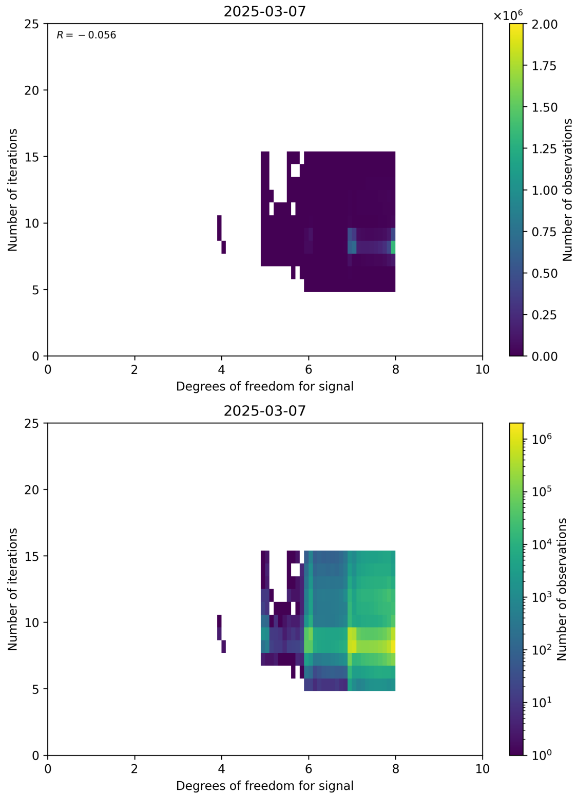
Figure 50: Scatter density plot of “Degrees of freedom for signal” against “Number of iterations” for 2025-03-07 to 2025-03-08.
