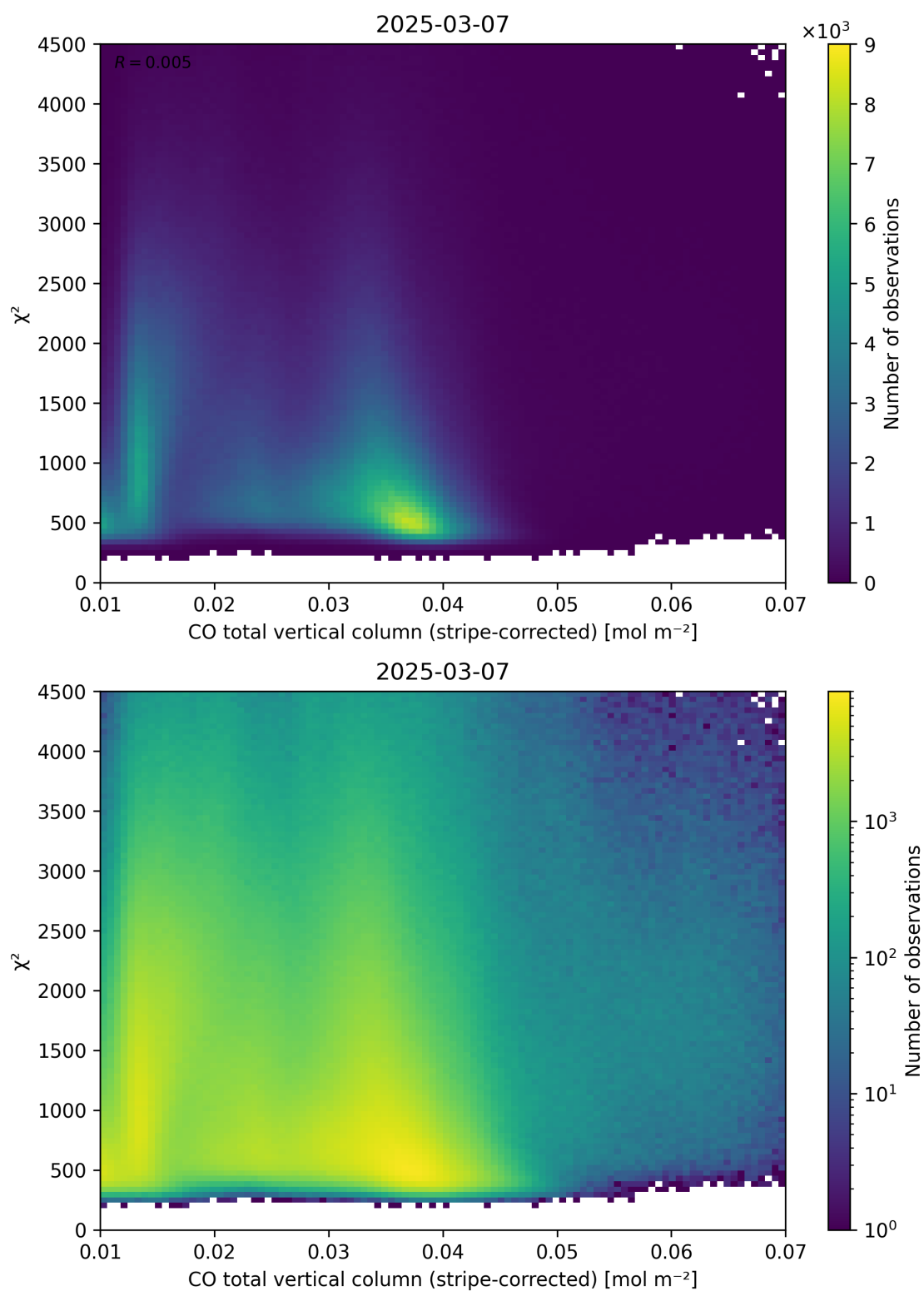
Figure 37: Scatter density plot of “CO total vertical column (stripe-corrected)” against “ \chi^2 ” for 2025-03-07 to 2025-03-08.
