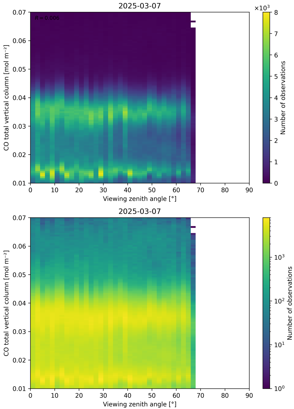
Figure 69: Scatter density plot of “Viewing zenith angle” against “CO total vertical column” for 2025-03-07 to 2025-03-08.
