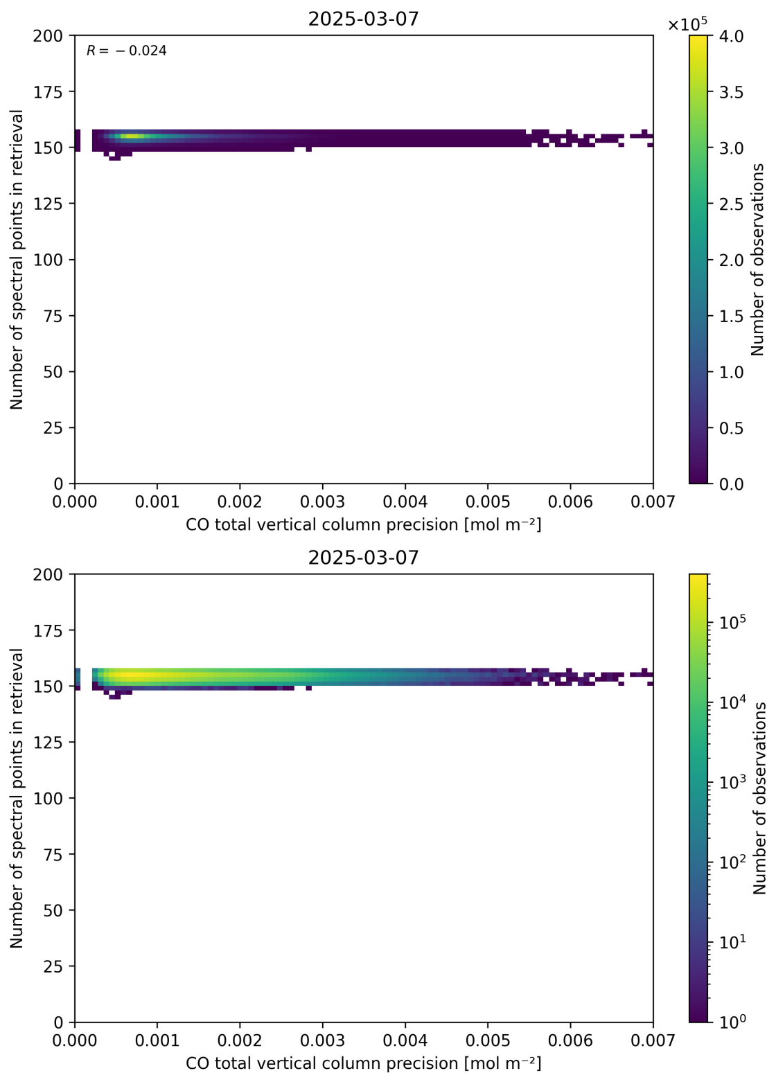
Figure 47: Scatter density plot of “CO total vertical column precision” against “Number of spectral points in retrieval” for 2025-03-07 to 2025-03-08.
