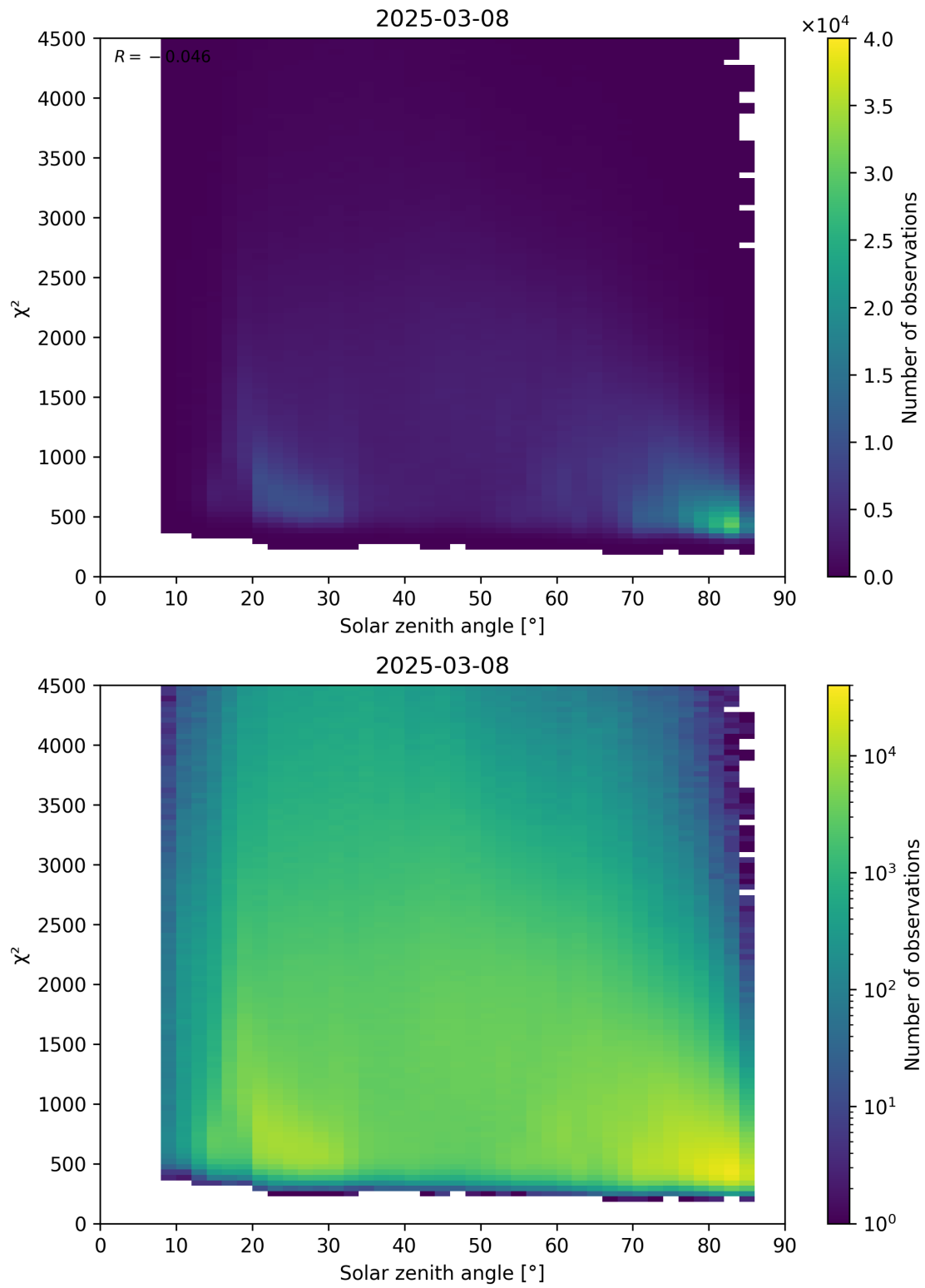
Figure 64: Scatter density plot of “Solar zenith angle” against “ \chi^2 ” for 2025-03-07 to 2025-03-09.
