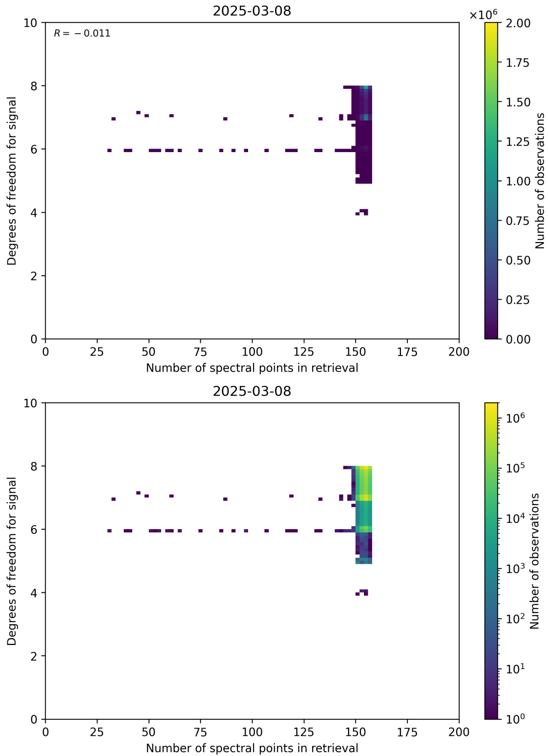
Figure 59: Scatter density plot of “Number of spectral points in retrieval” against “Degrees of freedom for signal” for 2025-03-07 to 2025-03-09.
