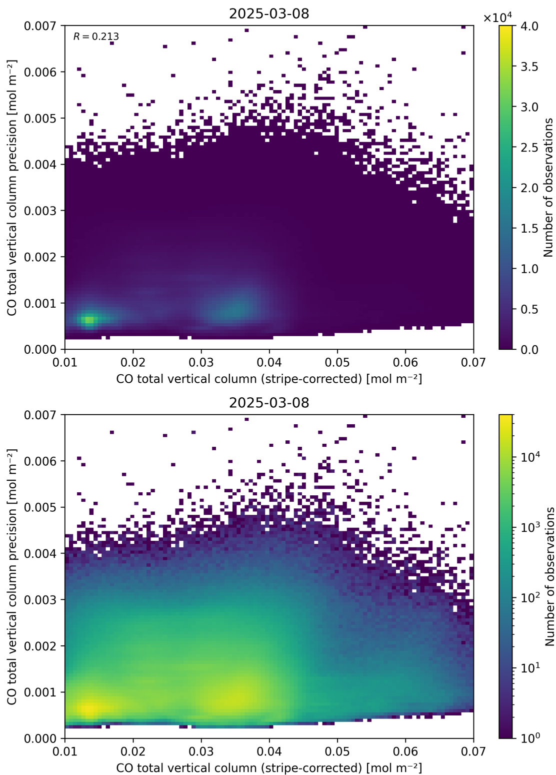
Figure 36: Scatter density plot of “CO total vertical column (stripe-corrected)” against “CO total vertical column precision” for 2025-03-07 to 2025-03-09.
