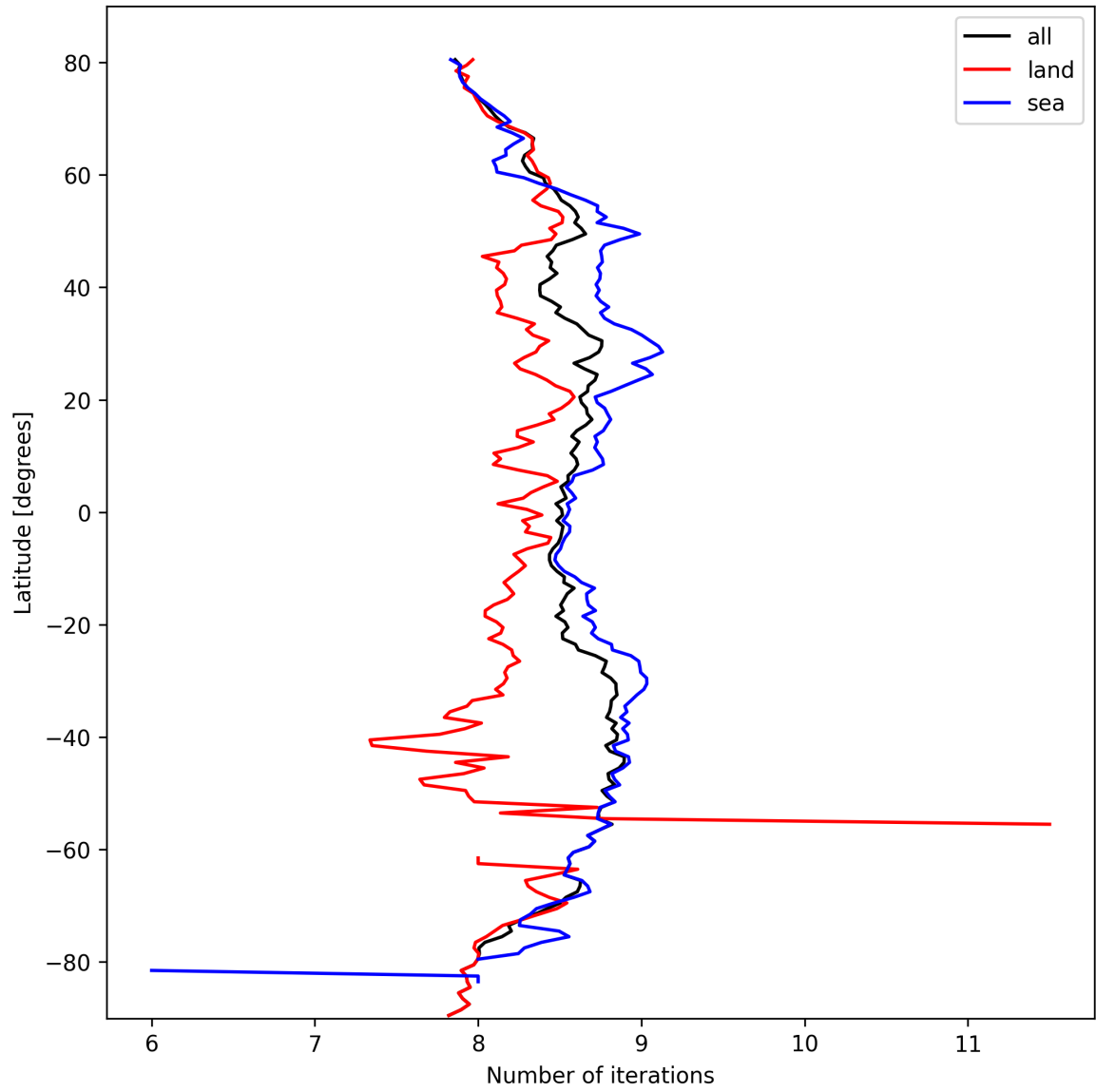
Figure 16: Zonal average of “Number of iterations” for 2025-03-07 to 2025-03-09.
