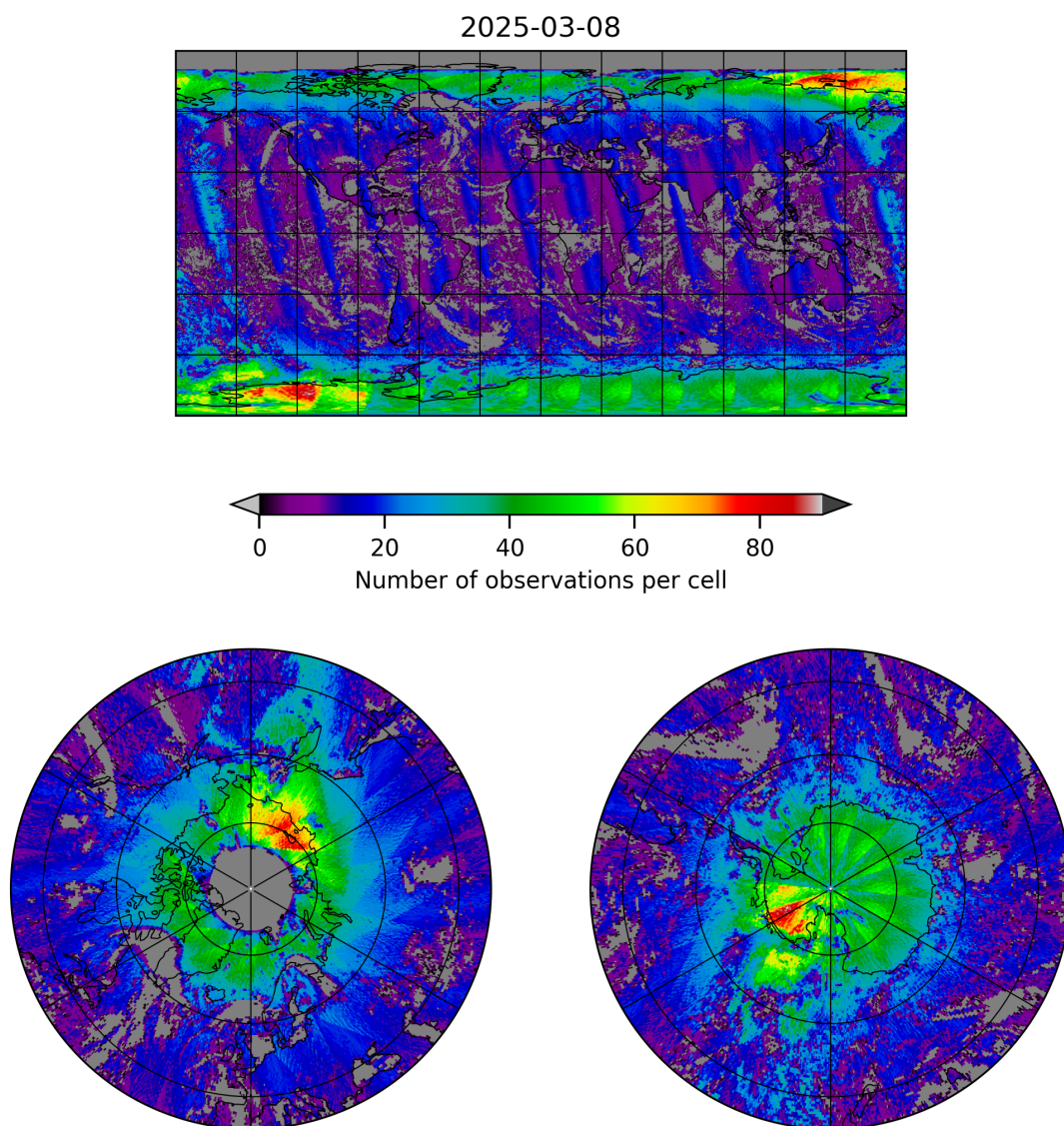
Figure 8: Map of the number of observations for 2025-03-07 to 2025-03-09
