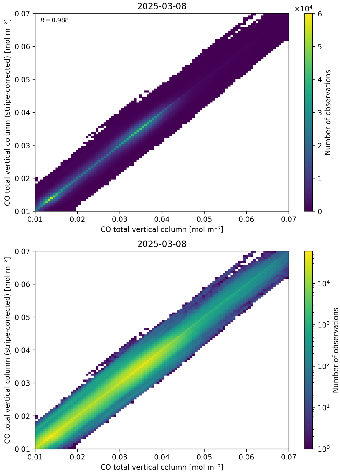
Figure 33: Scatter density plot of “CO total vertical column” against “CO total vertical column (stripe-corrected)” for 2025-03-07 to 2025-03-09.
