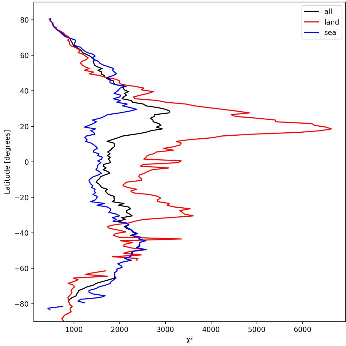
Figure 14: Zonal average of “ \chi^2 ” for 2025-03-07 to 2025-03-09.
