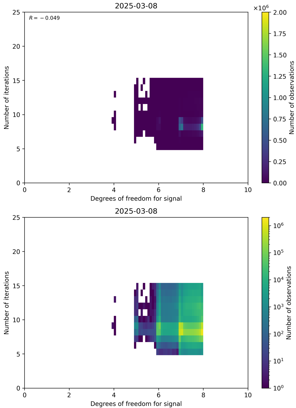
Figure 50: Scatter density plot of “Degrees of freedom for signal” against “Number of iterations” for 2025-03-07 to 2025-03-09.
