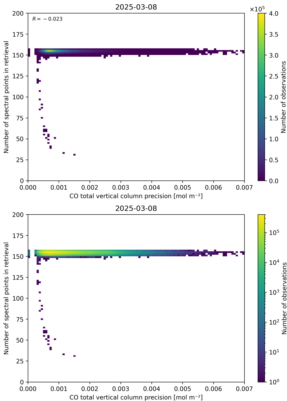
Figure 47: Scatter density plot of “CO total vertical column precision” against “Number of spectral points in retrieval” for 2025-03-07 to 2025-03-09.
