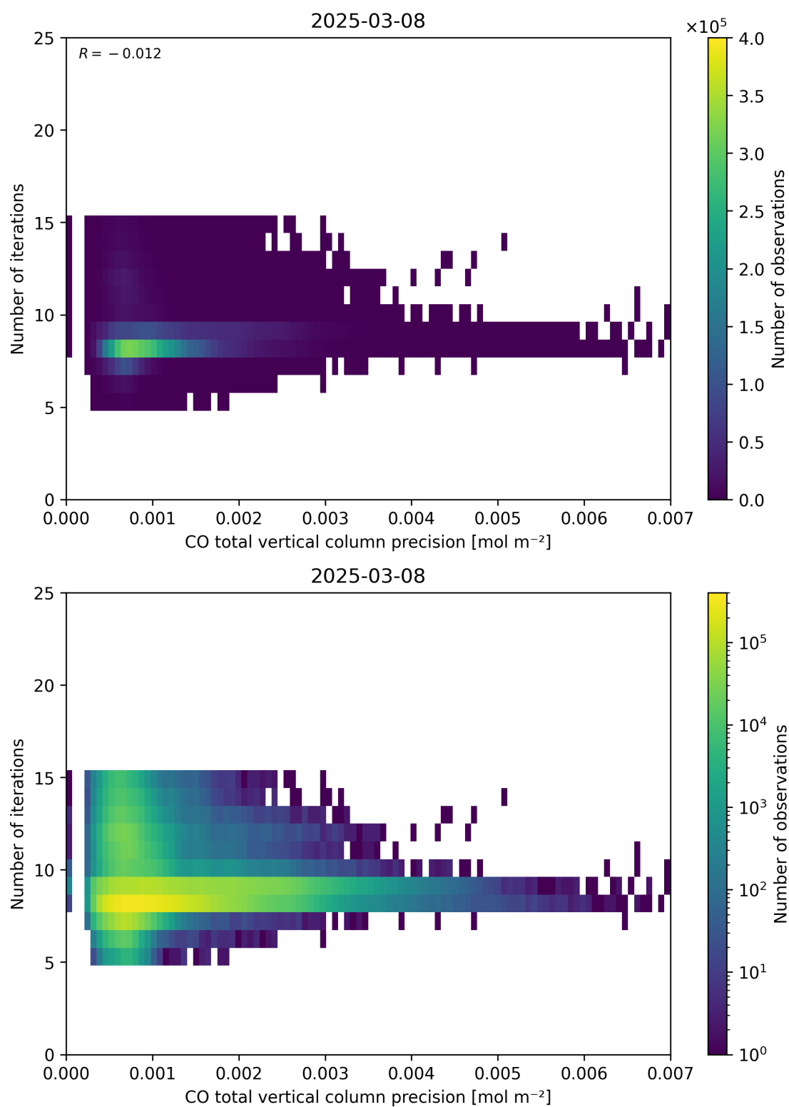
Figure 46: Scatter density plot of “CO total vertical column precision” against “Number of iterations” for 2025-03-07 to 2025-03-09.
