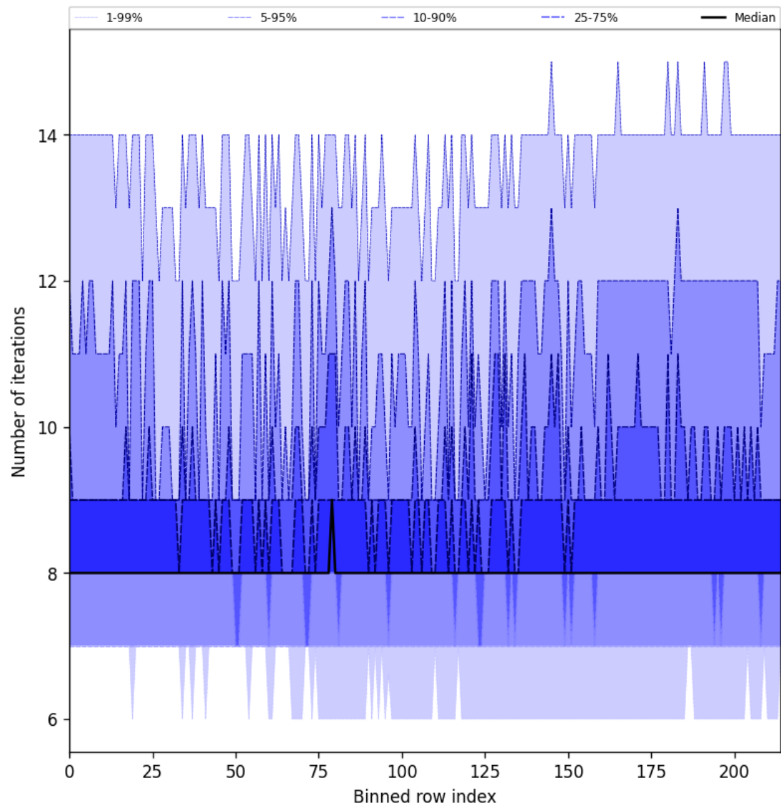
Figure 32: Along track statistics of “Number of iterations” for 2025-03-07 to 2025-03-09
