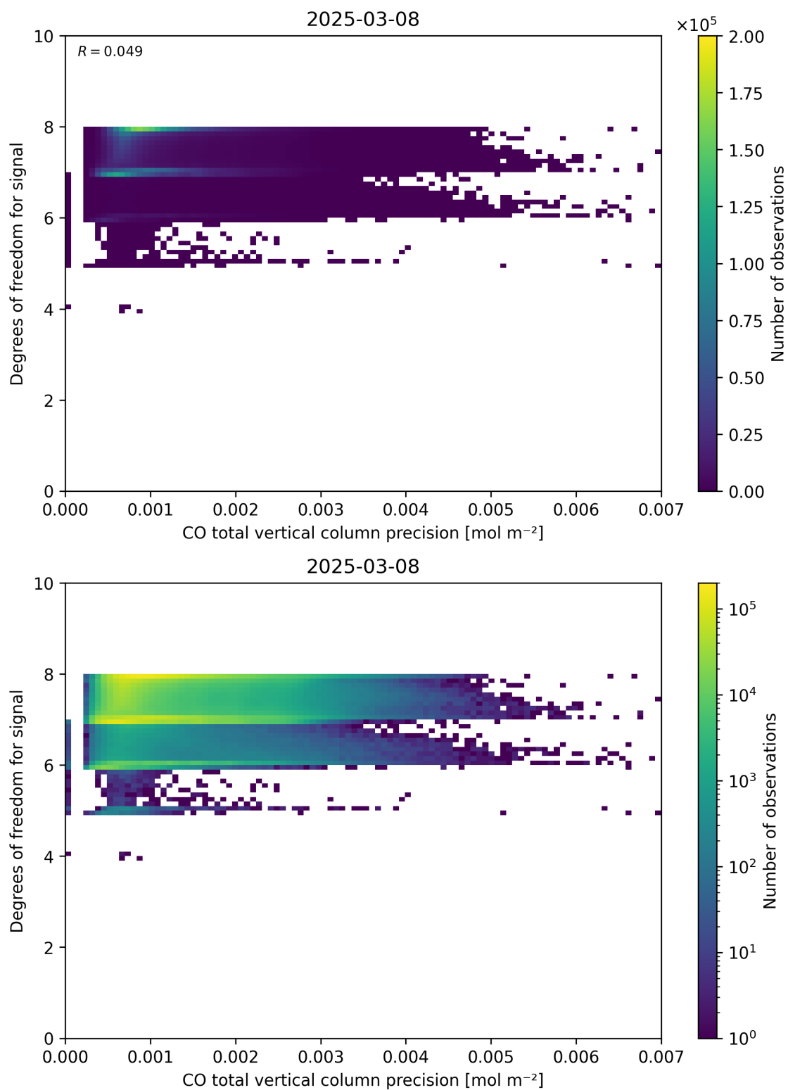
Figure 45: Scatter density plot of “CO total vertical column precision” against “Degrees of freedom for signal” for 2025-03-07 to 2025-03-09.
