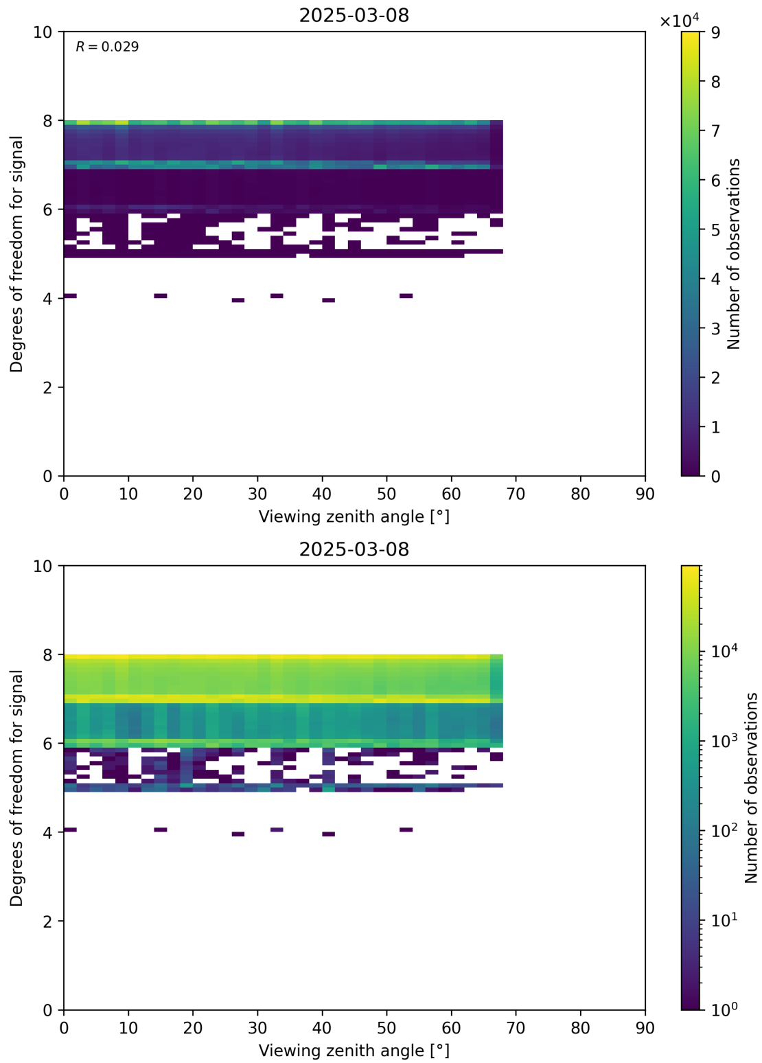
Figure 73: Scatter density plot of “Viewing zenith angle” against “Degrees of freedom for signal” for 2025-03-07 to 2025-03-09.
