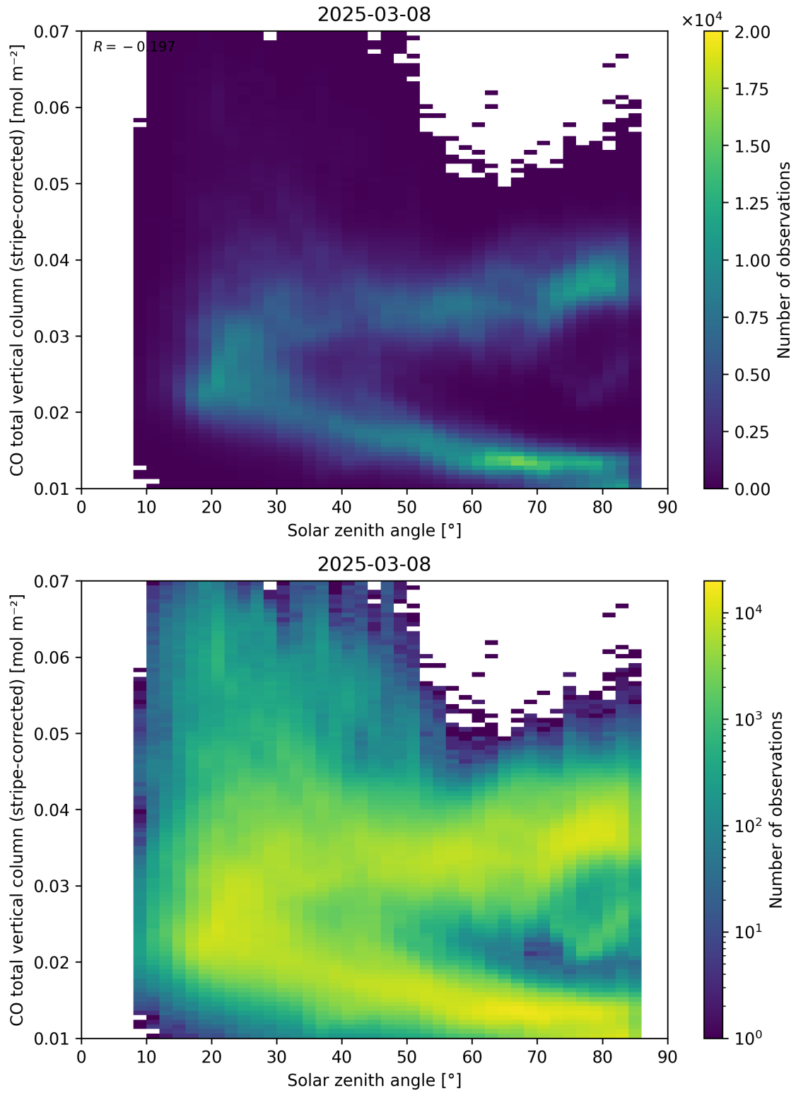
Figure 62: Scatter density plot of “Solar zenith angle” against “CO total vertical column (stripe-corrected)” for 2025-03-07 to 2025-03-09.
