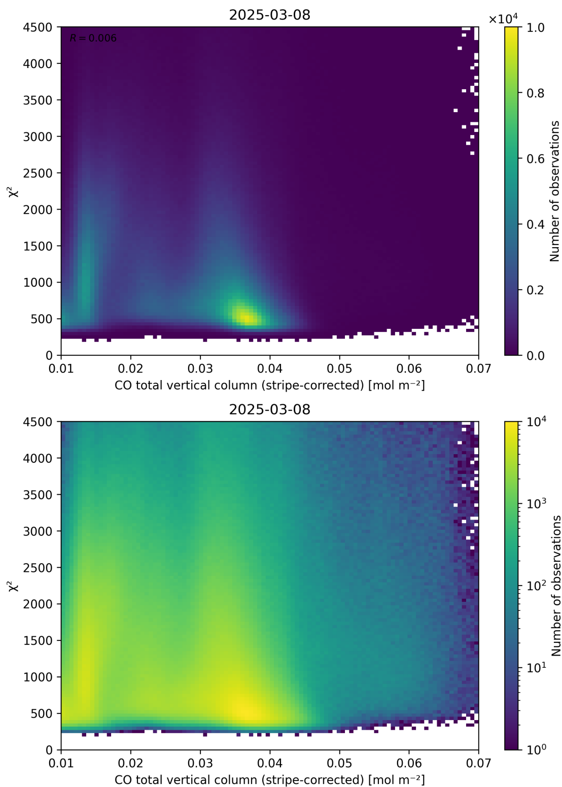
Figure 37: Scatter density plot of “CO total vertical column (stripe-corrected)” against “ \chi^2 ” for 2025-03-07 to 2025-03-09.
