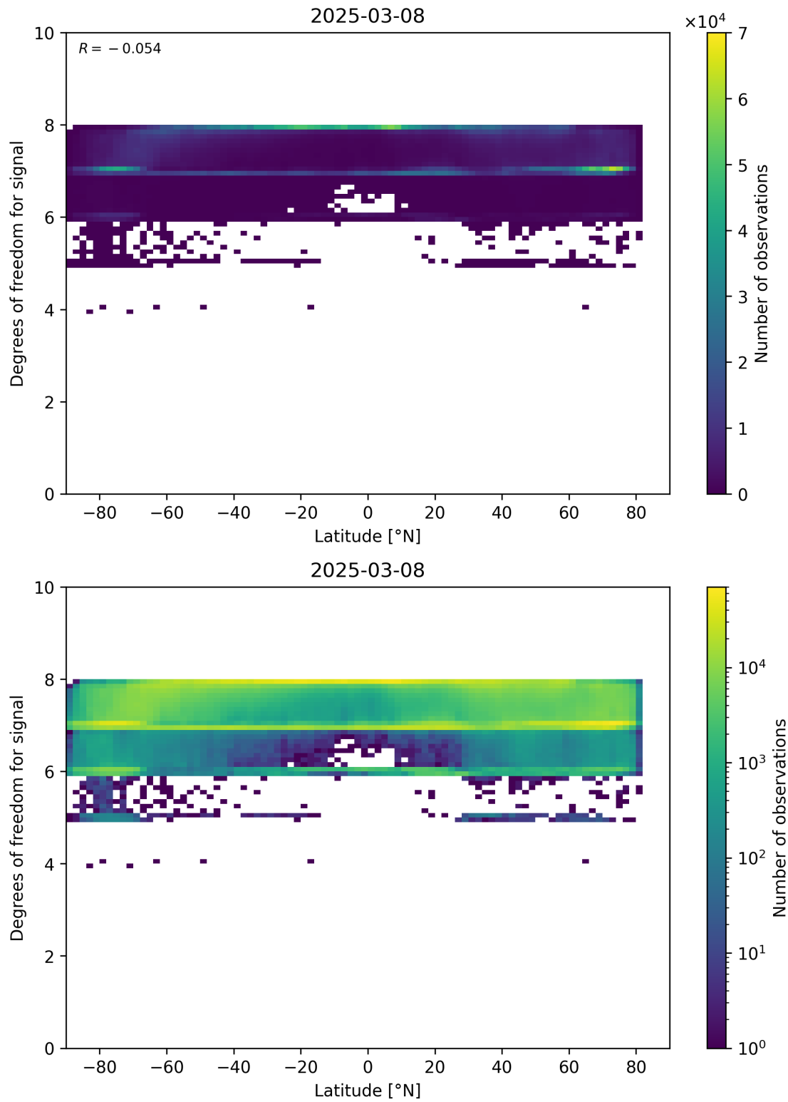
Figure 55: Scatter density plot of “Latitude” against “Degrees of freedom for signal” for 2025-03-07 to 2025-03-09.
