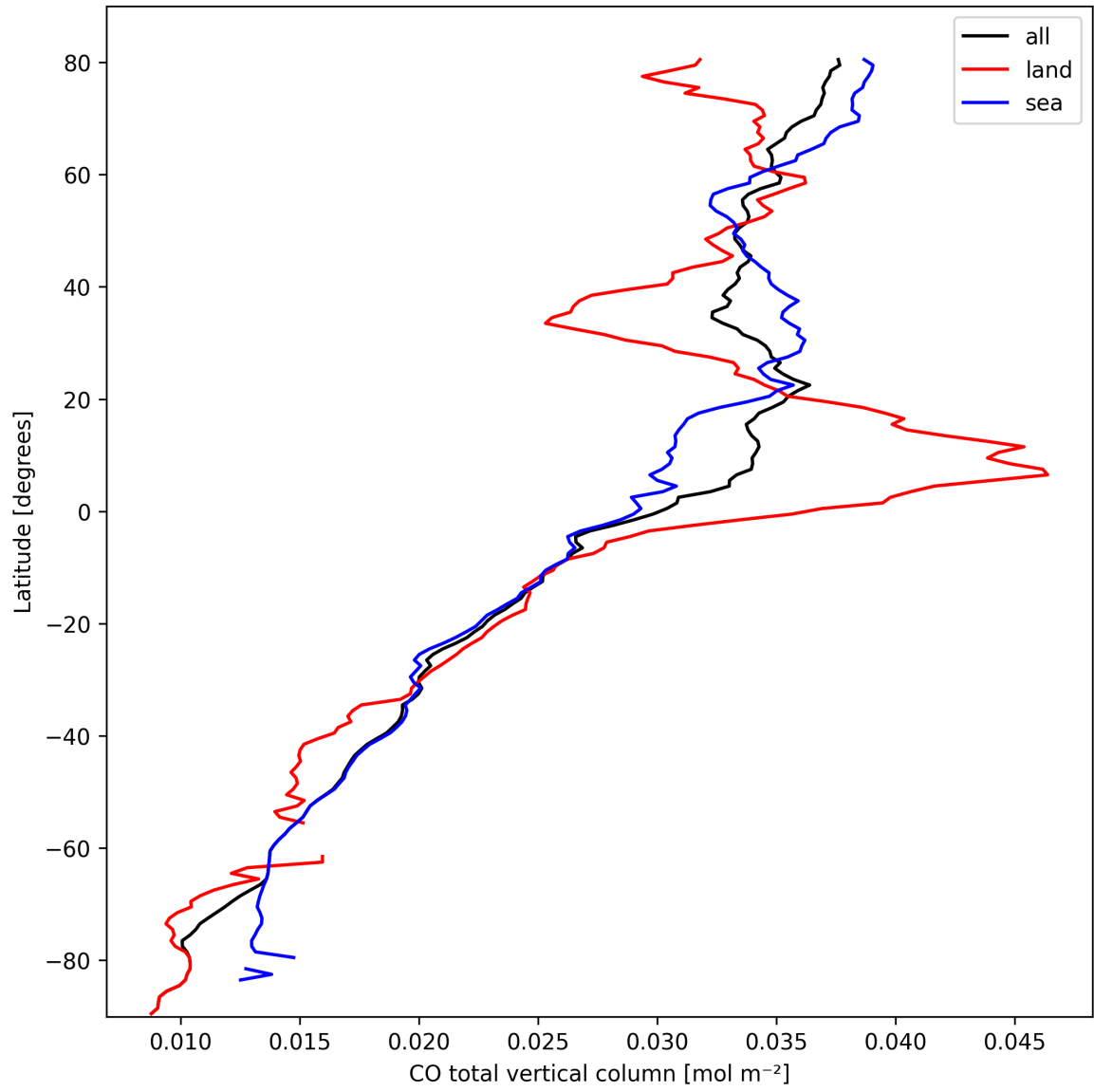
Figure 10: Zonal average of “CO total vertical column” for 2025-03-07 to 2025-03-09.
