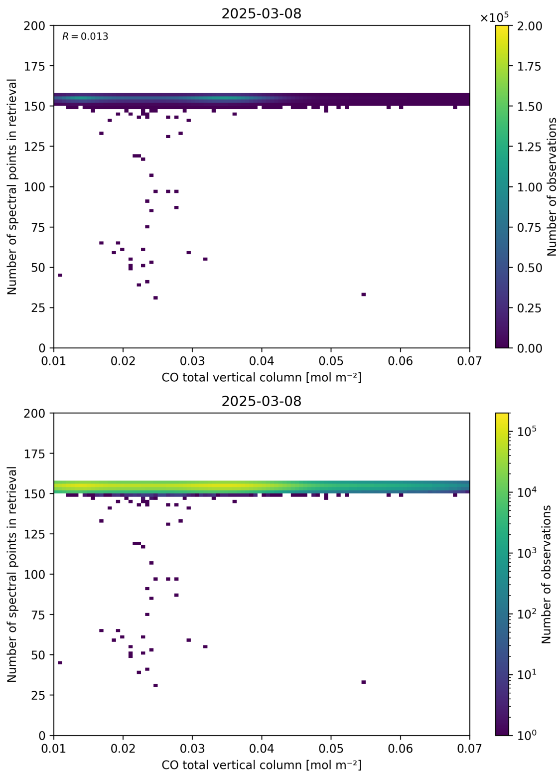
Figure 43: Scatter density plot of “CO total vertical column” against “Number of spectral points in retrieval” for 2025-03-07 to 2025-03-09.
