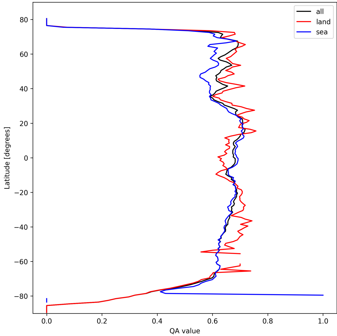
Figure 9: Zonal average of “QA value” for 2025-03-07 to 2025-03-09.
