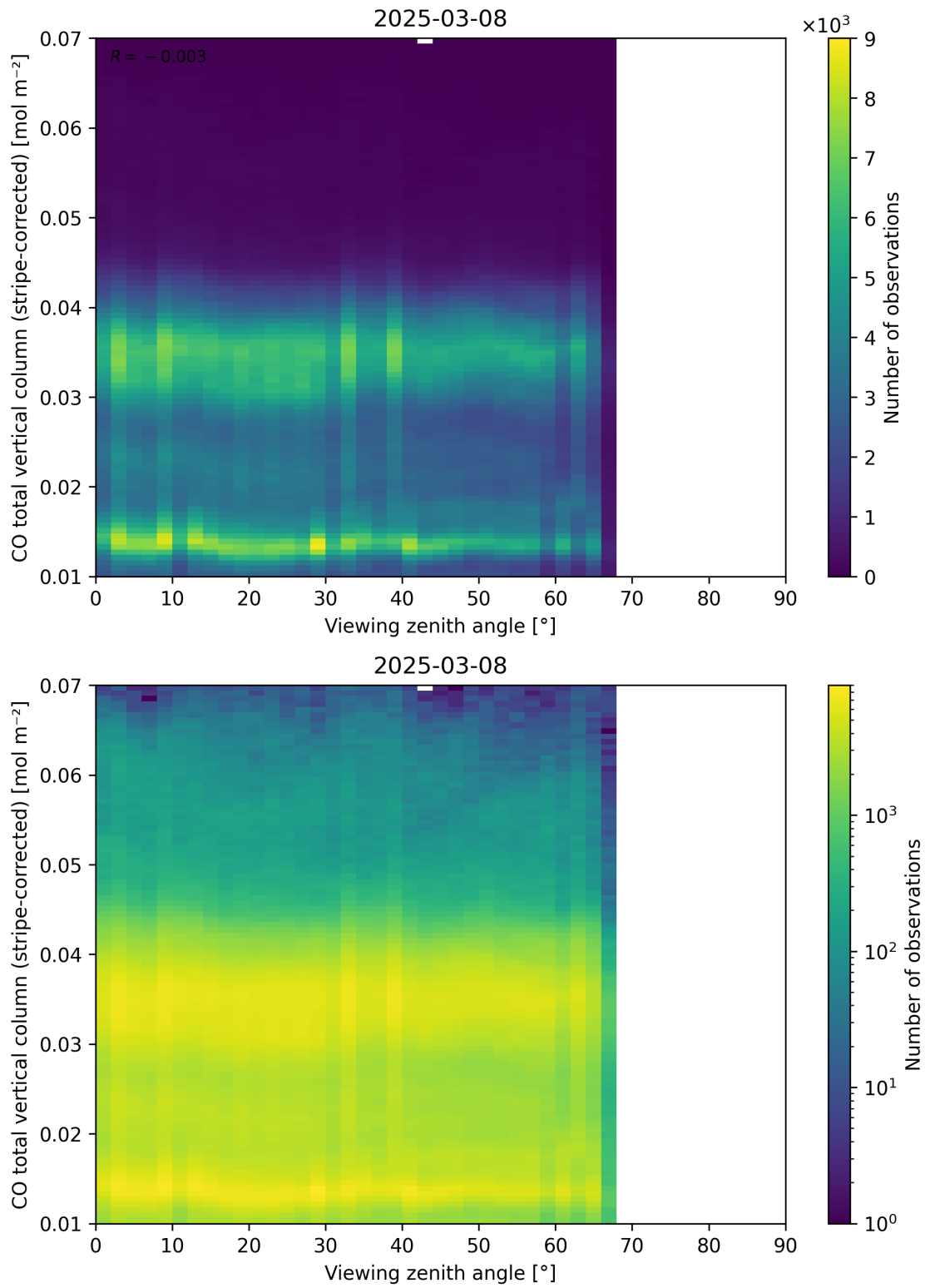
Figure 70: Scatter density plot of “Viewing zenith angle” against “CO total vertical column (stripe-corrected)” for 2025-03-07 to 2025-03-09.
