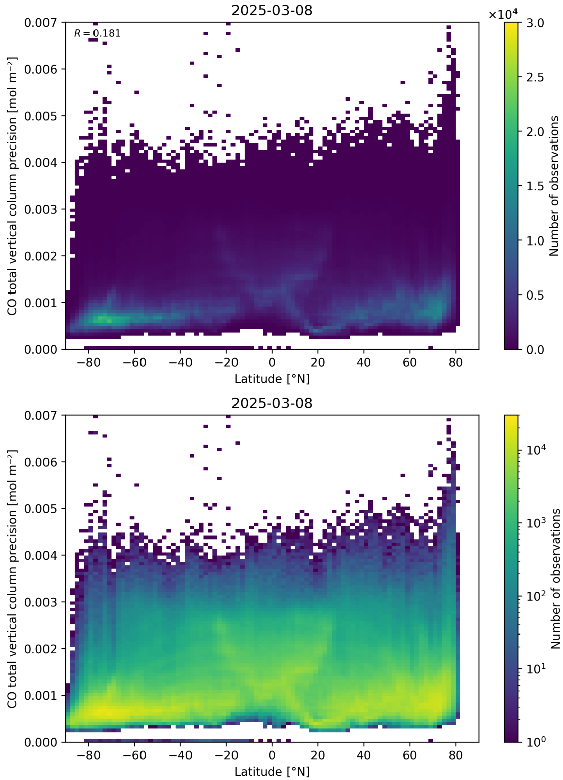
Figure 53: Scatter density plot of “Latitude” against “CO total vertical column precision” for 2025-03-07 to 2025-03-09.
