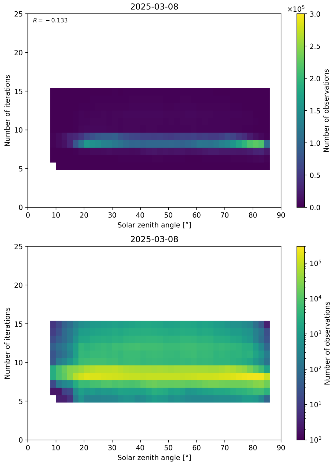
Figure 67: Scatter density plot of “Solar zenith angle” against “Number of iterations” for 2025-03-07 to 2025-03-09.
