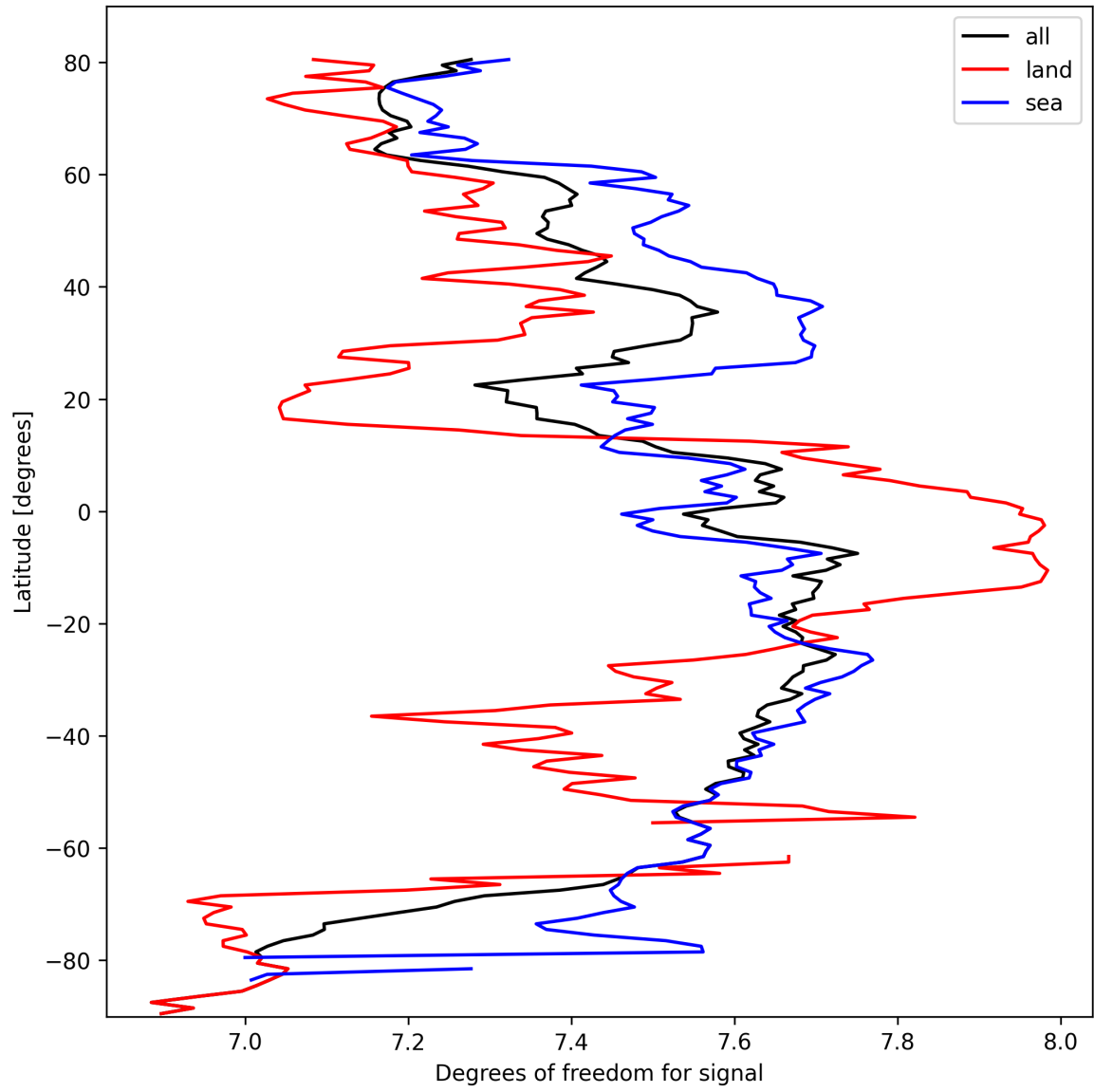
Figure 15: Zonal average of “Degrees of freedom for signal” for 2025-03-07 to 2025-03-09.
