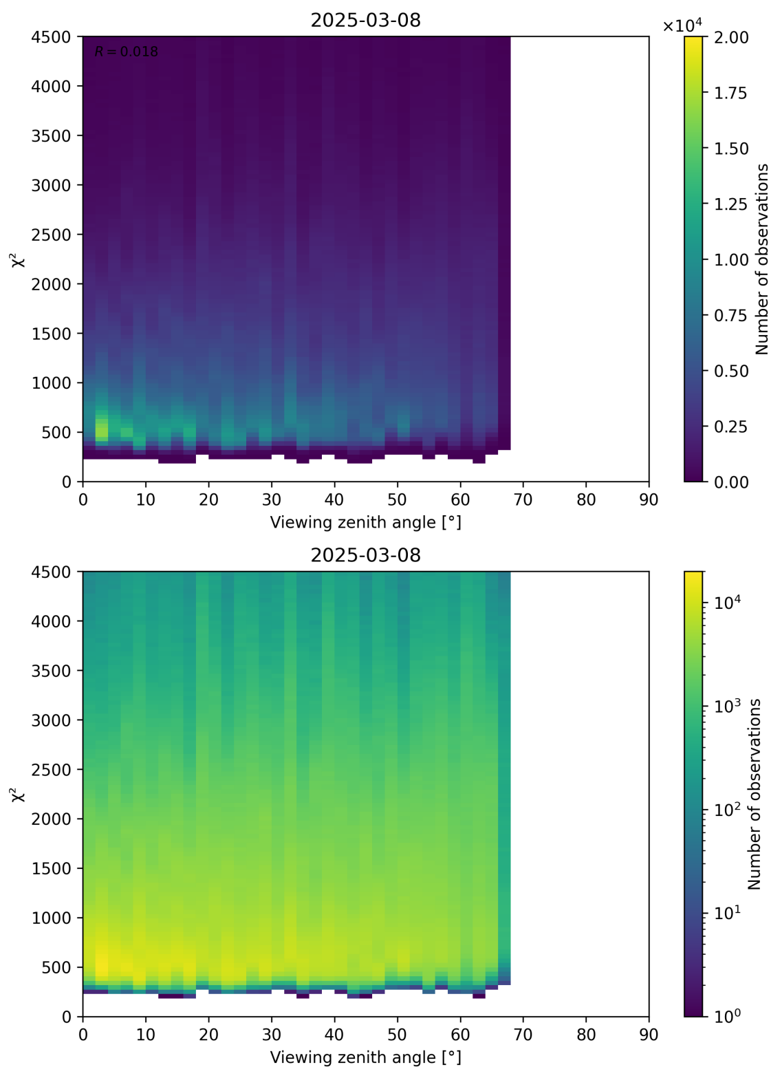
Figure 72: Scatter density plot of “Viewing zenith angle” against “ \chi^2 ” for 2025-03-07 to 2025-03-09.
