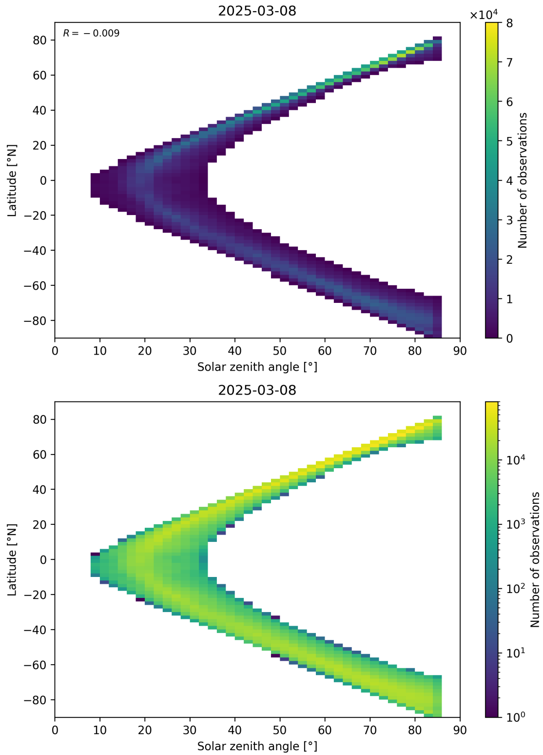
Figure 66: Scatter density plot of “Solar zenith angle” against “Latitude” for 2025-03-07 to 2025-03-09.
