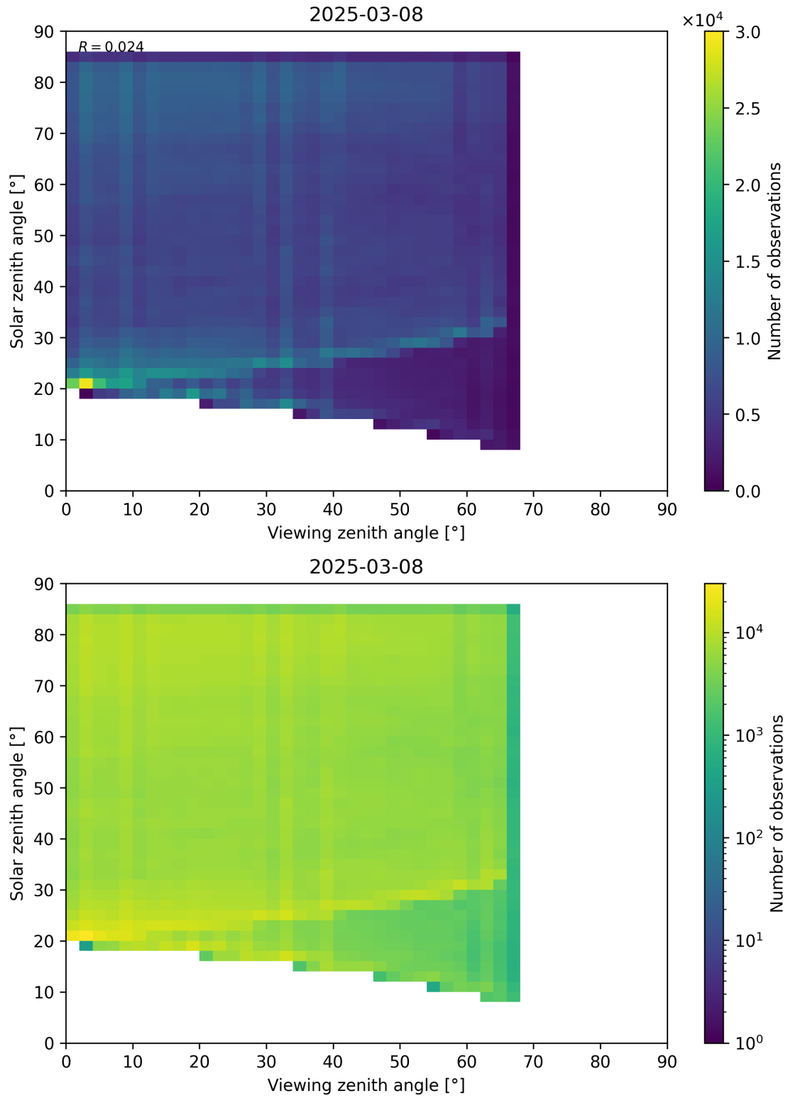
Figure 77: Scatter density plot of “Viewing zenith angle” against “Solar zenith angle” for 2025-03-07 to 2025-03-09.
