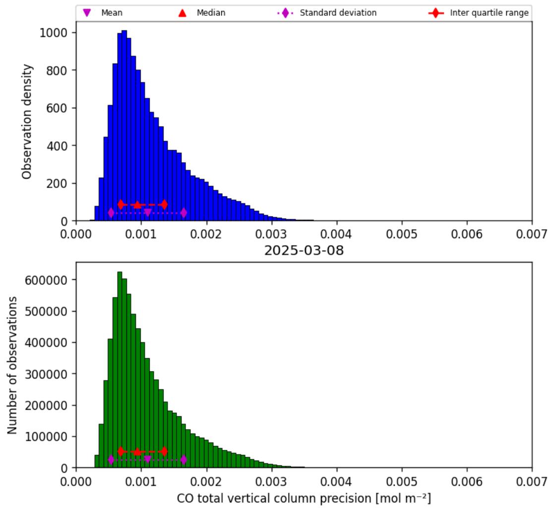
Figure 20: Histogram of “CO total vertical column precision” for 2025-03-07 to 2025-03-09
