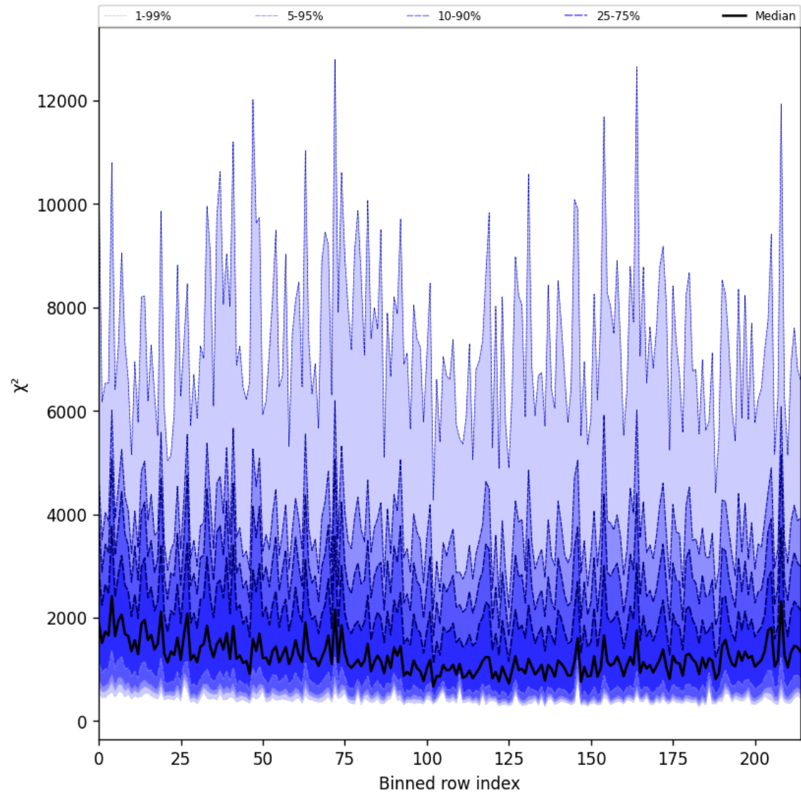
Figure 30: Along track statistics of “ \chi^2 ” for 2025-03-07 to 2025-03-09
