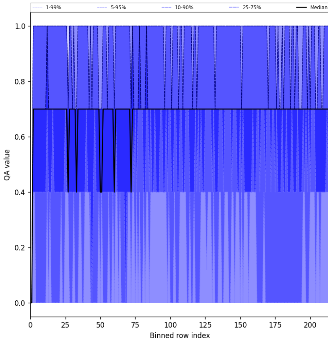
Figure 25: Along track statistics of “QA value” for 2025-03-07 to 2025-03-09
