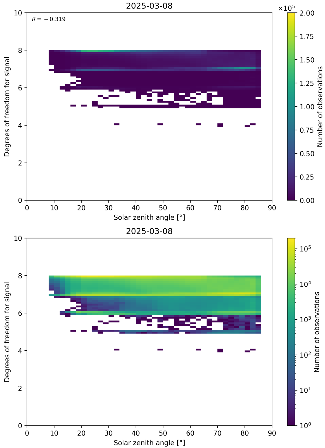
Figure 65: Scatter density plot of “Solar zenith angle” against “Degrees of freedom for signal” for 2025-03-07 to 2025-03-09.
