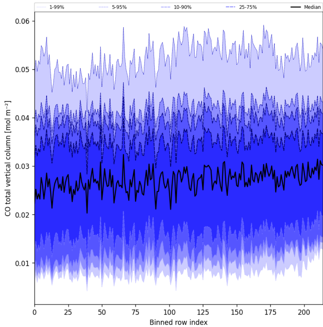
Figure 26: Along track statistics of “CO total vertical column” for 2025-03-07 to 2025-03-09
