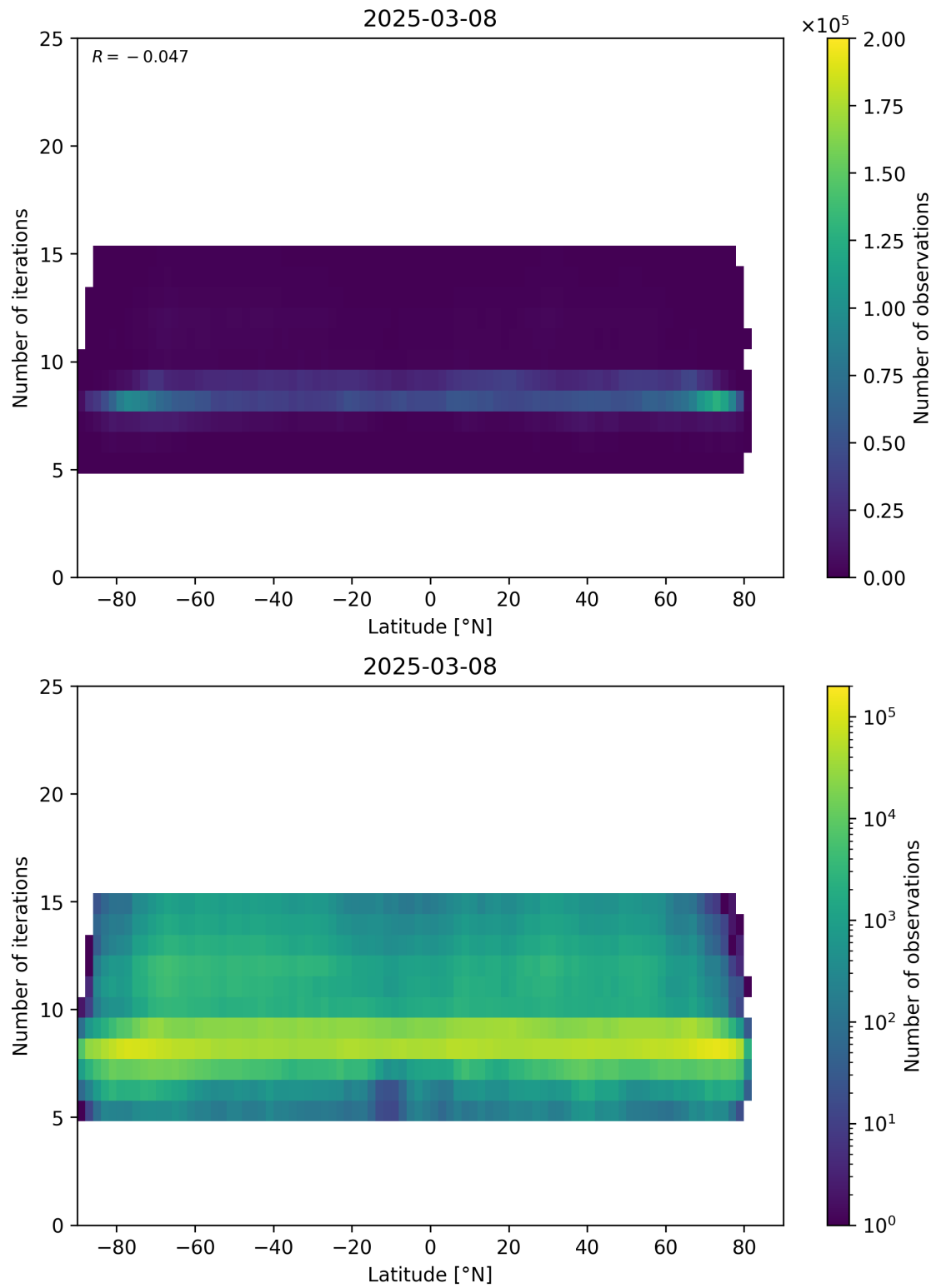
Figure 56: Scatter density plot of “Latitude” against “Number of iterations” for 2025-03-07 to 2025-03-09.
