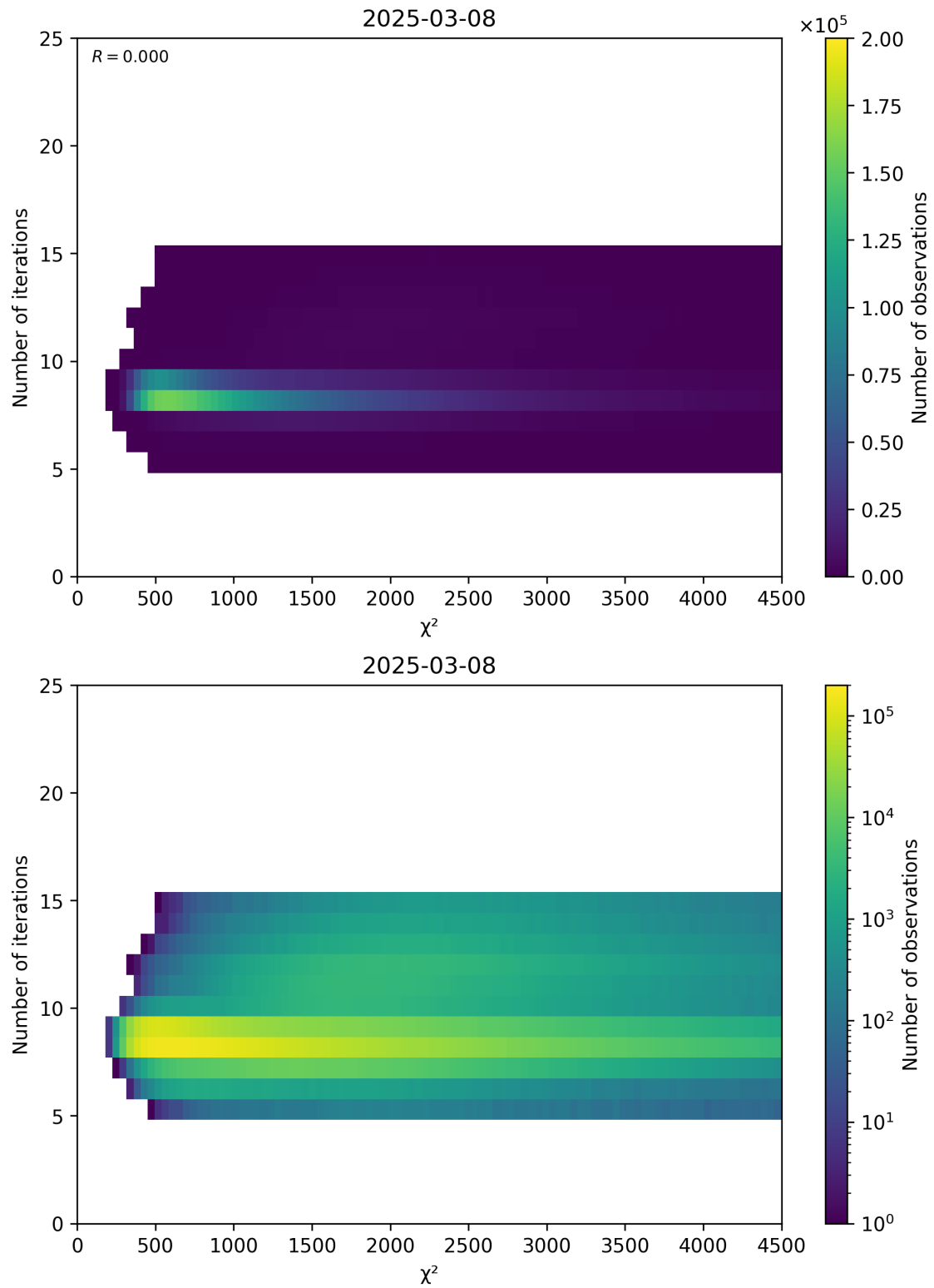
Figure 49: Scatter density plot of “ \chi^2 ” against “Number of iterations” for 2025-03-07 to 2025-03-09.
