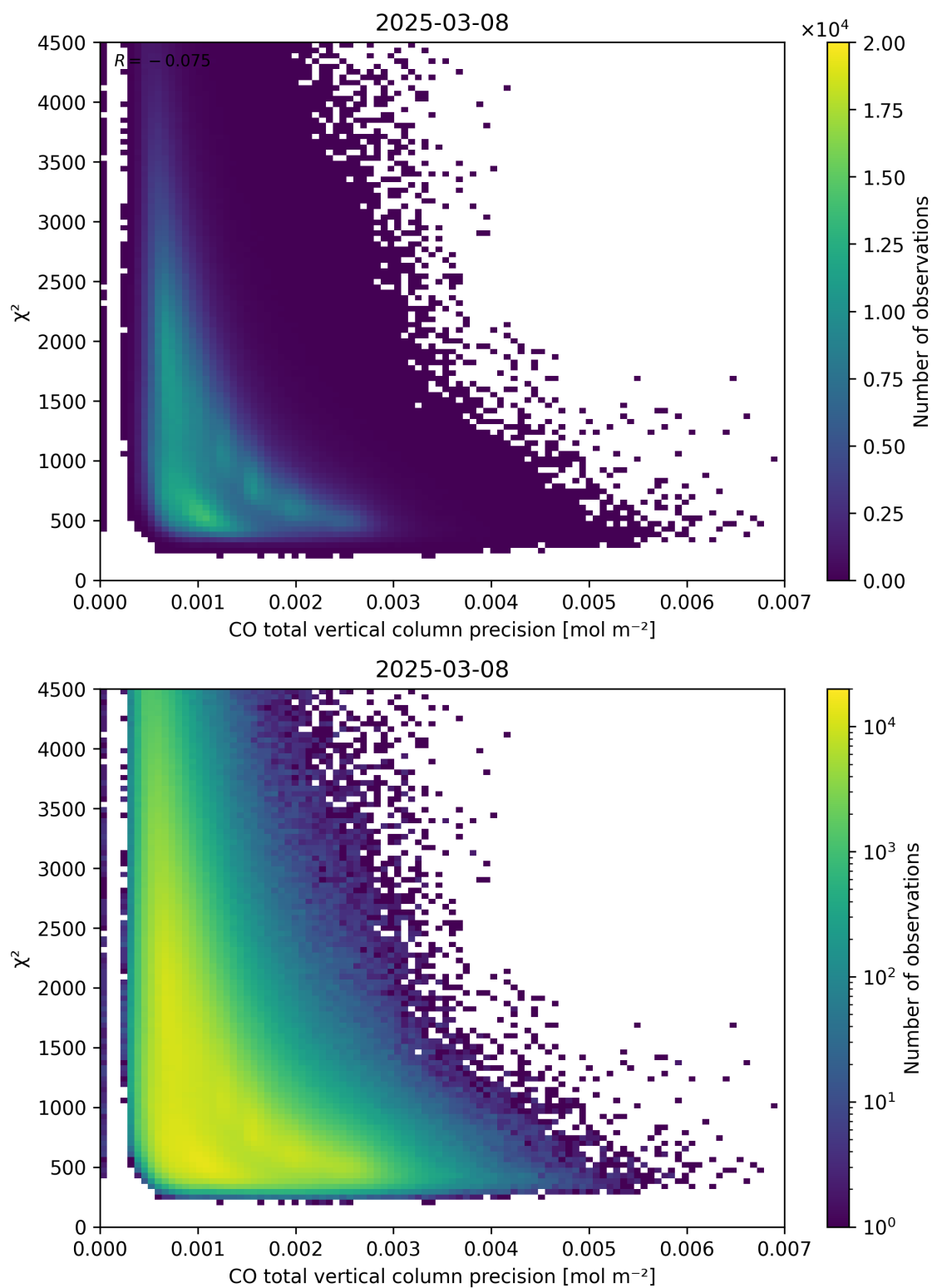
Figure 44: Scatter density plot of “CO total vertical column precision” against “ \chi^2 ” for 2025-03-07 to 2025-03-09.
