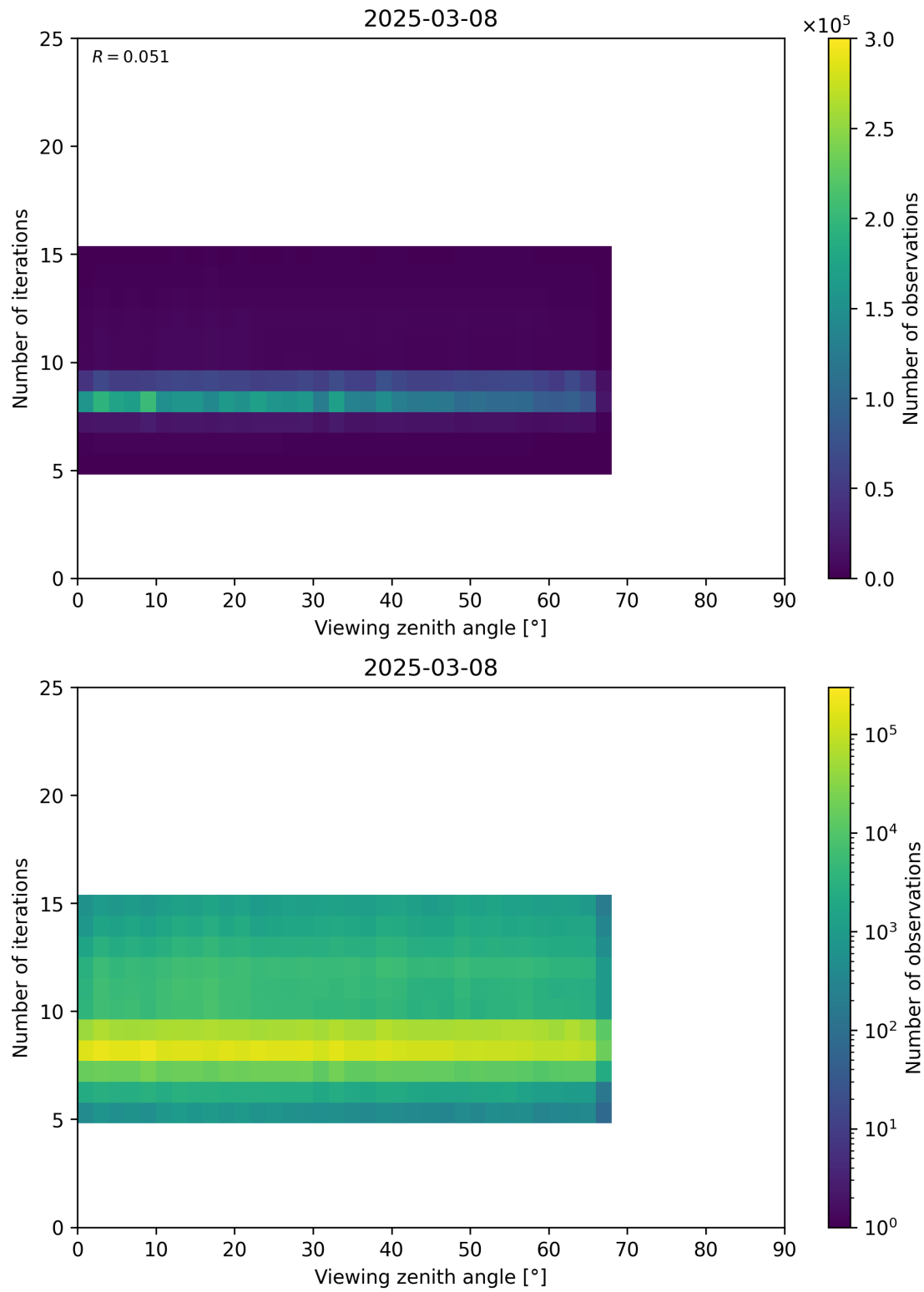
Figure 75: Scatter density plot of “Viewing zenith angle” against “Number of iterations” for 2025-03-07 to 2025-03-09.
