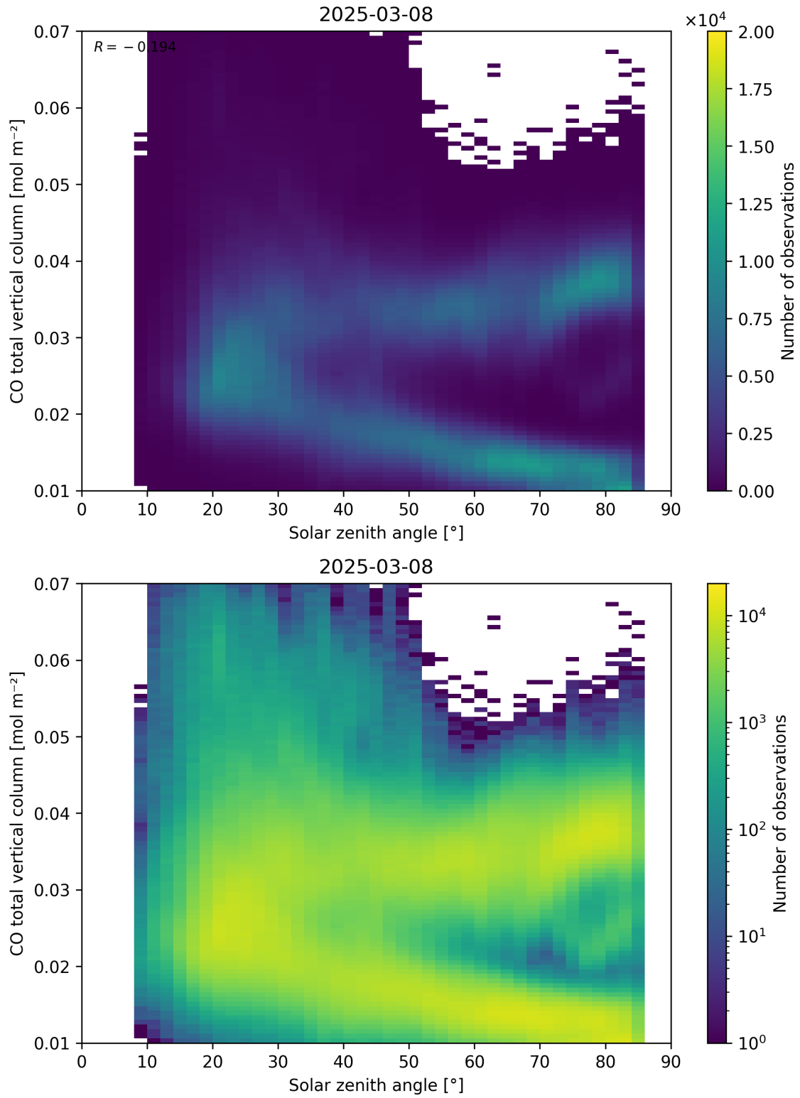
Figure 61: Scatter density plot of “Solar zenith angle” against “CO total vertical column” for 2025-03-07 to 2025-03-09.
