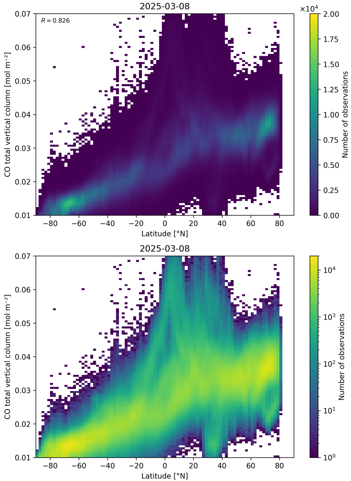
Figure 51: Scatter density plot of “Latitude” against “CO total vertical column” for 2025-03-07 to 2025-03-09.
