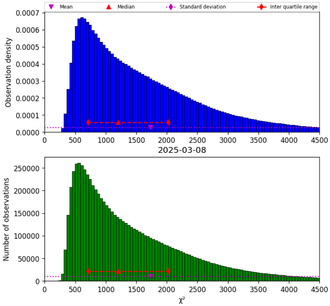
Figure 22: Histogram of “ \chi^2 ” for 2025-03-07 to 2025-03-09
