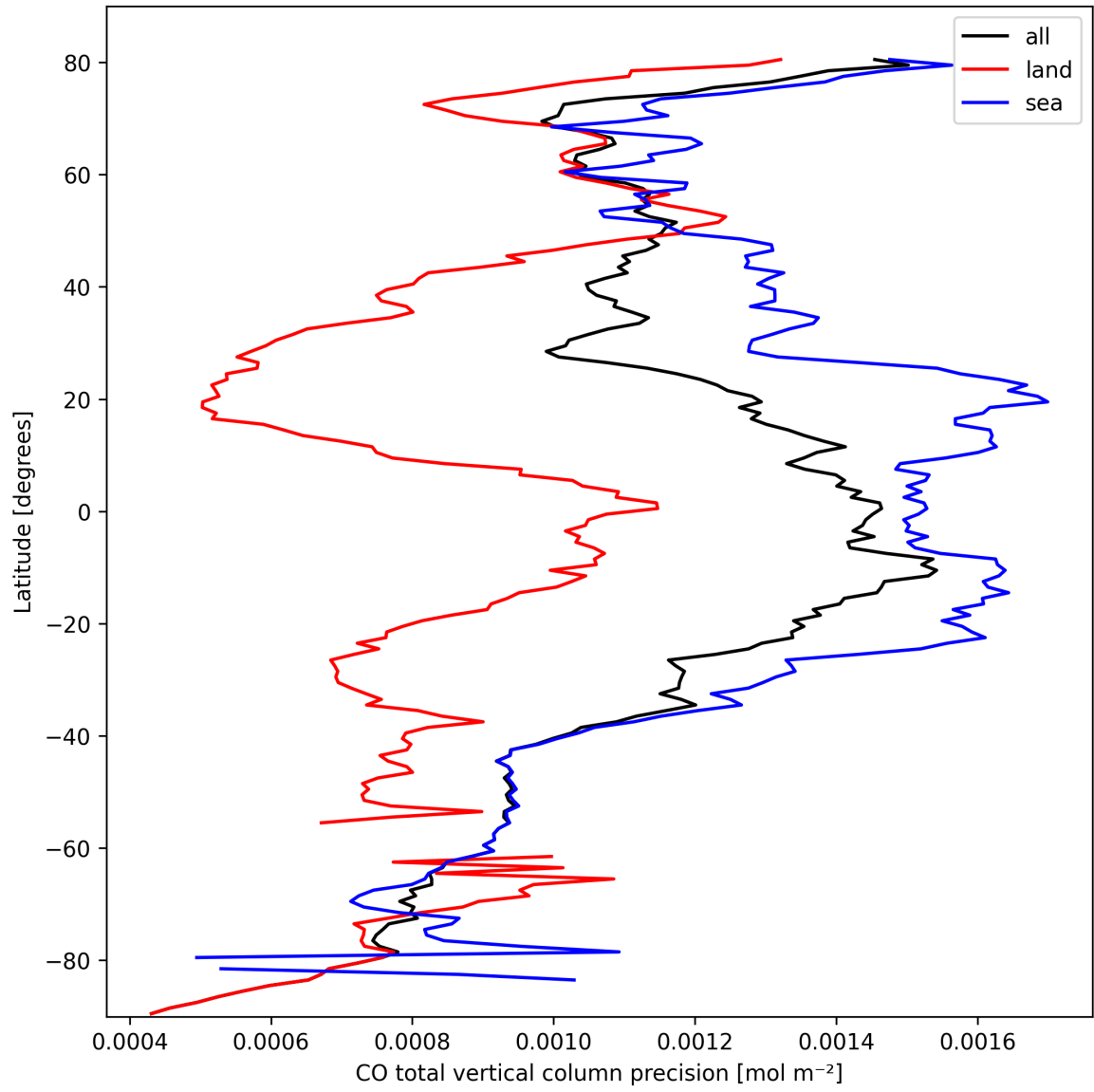
Figure 12: Zonal average of “CO total vertical column precision” for 2025-03-07 to 2025-03-09.
