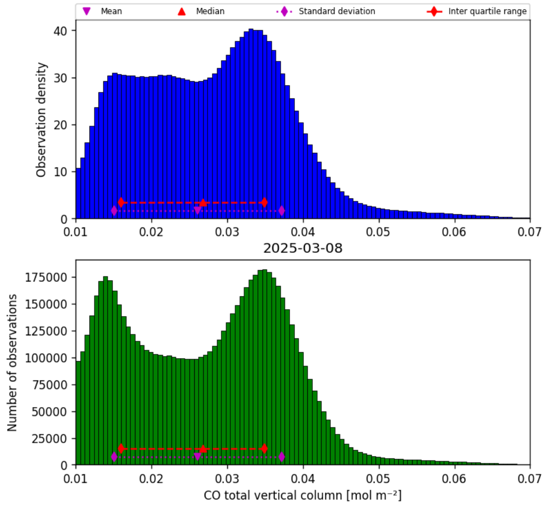
Figure 18: Histogram of “CO total vertical column” for 2025-03-07 to 2025-03-09
