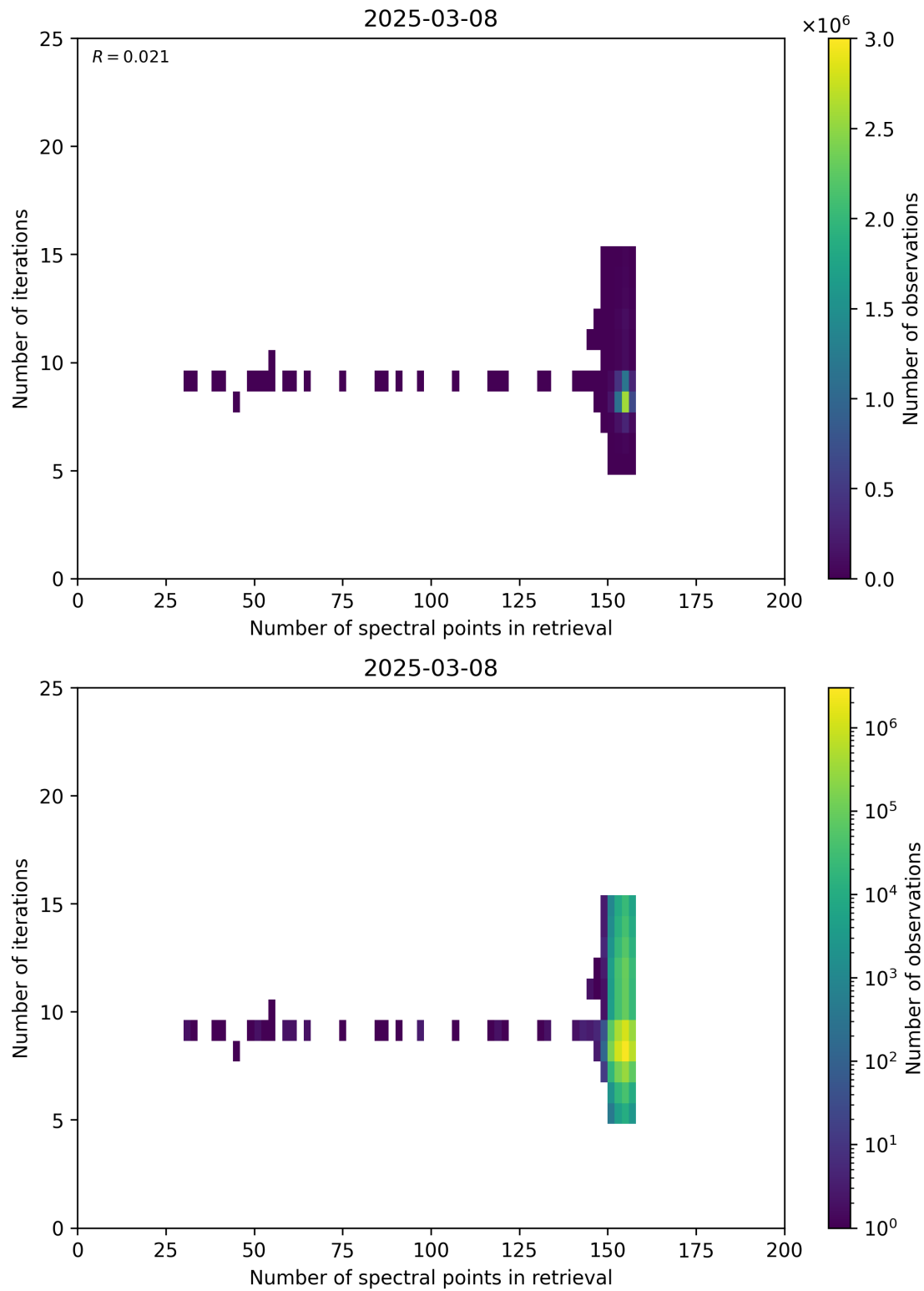
Figure 60: Scatter density plot of “Number of spectral points in retrieval” against “Number of iterations” for 2025-03-07 to 2025-03-09.
