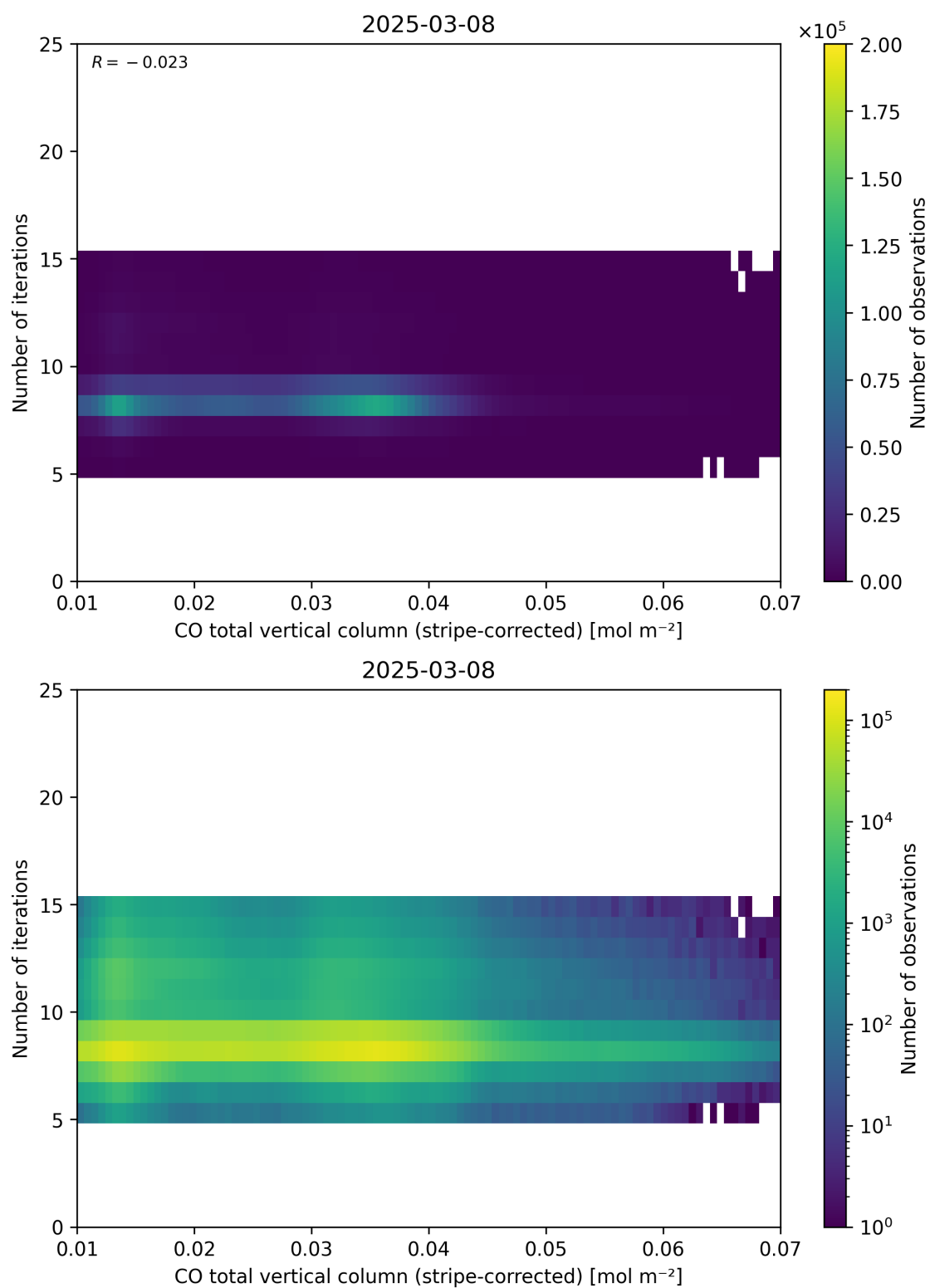
Figure 39: Scatter density plot of “CO total vertical column (stripe-corrected)” against “Number of iterations” for 2025-03-07 to 2025-03-09.
