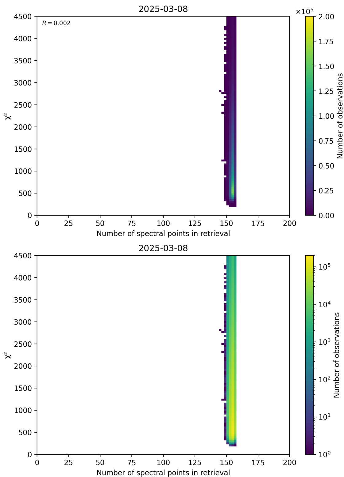
Figure 58: Scatter density plot of “Number of spectral points in retrieval” against “ \chi^2 ” for 2025-03-07 to 2025-03-09.
