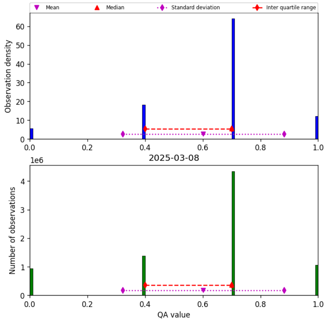
Figure 17: Histogram of “QA value” for 2025-03-07 to 2025-03-09
