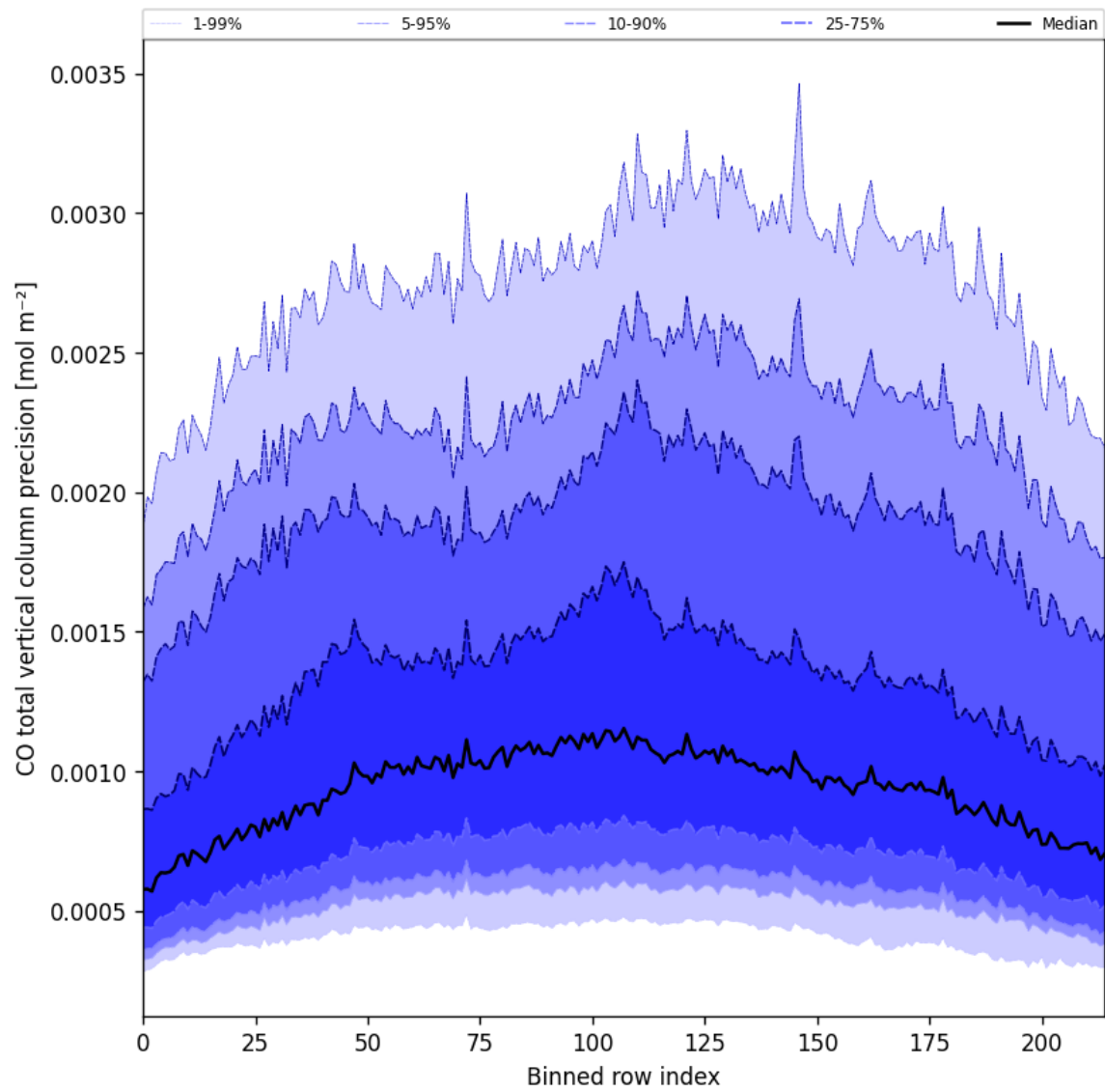
Figure 28: Along track statistics of “CO total vertical column precision” for 2025-03-07 to 2025-03-09
