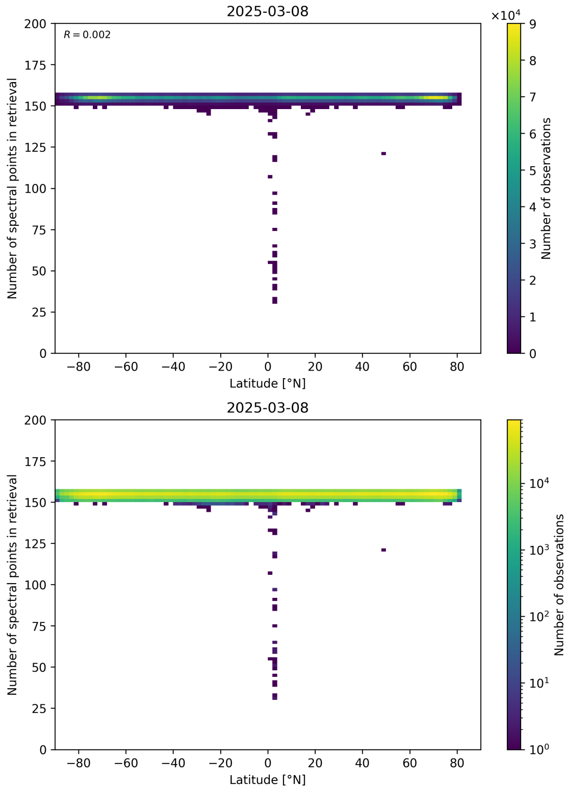
Figure 57: Scatter density plot of “Latitude” against “Number of spectral points in retrieval” for 2025-03-07 to 2025-03-09.
