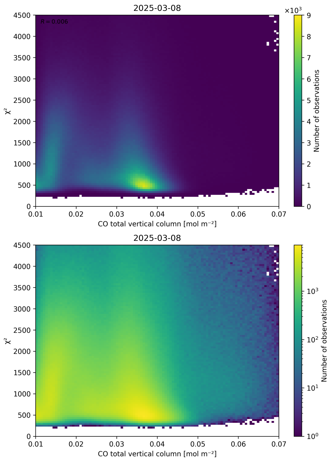
Figure 35: Scatter density plot of “CO total vertical column” against “ \chi^2 ” for 2025-03-07 to 2025-03-09.
