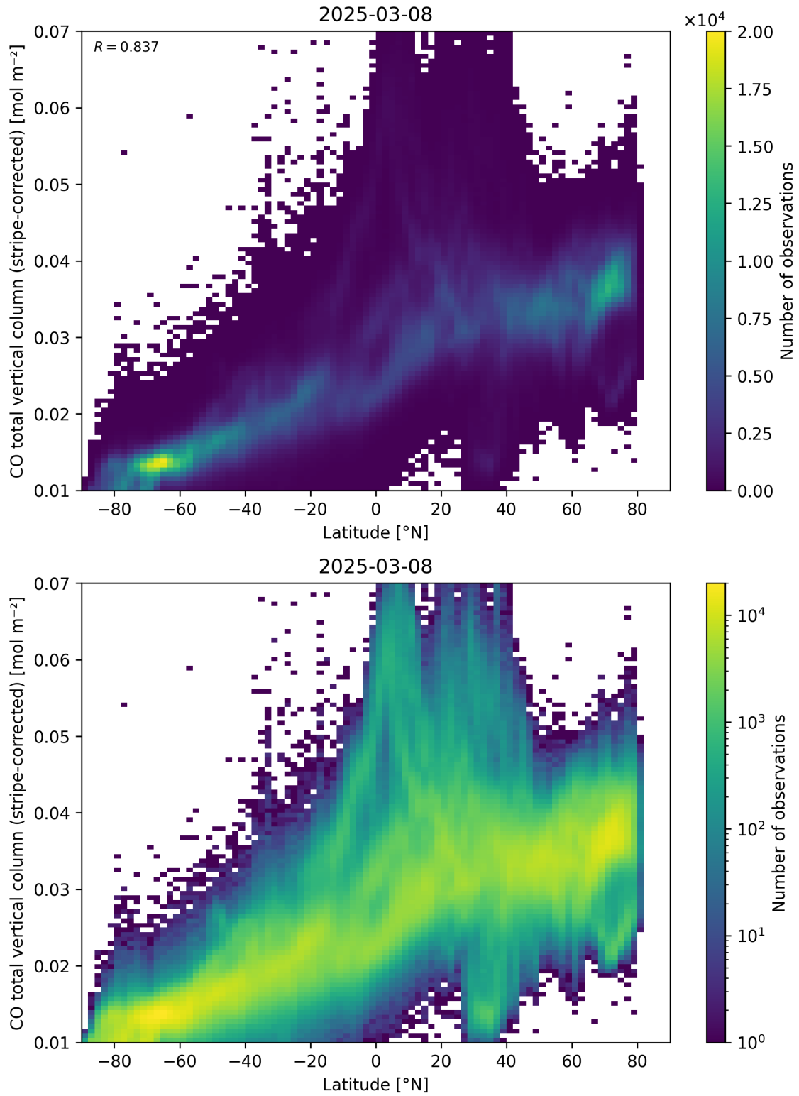
Figure 52: Scatter density plot of “Latitude” against “CO total vertical column (stripe-corrected)” for 2025-03-07 to 2025-03-09.
