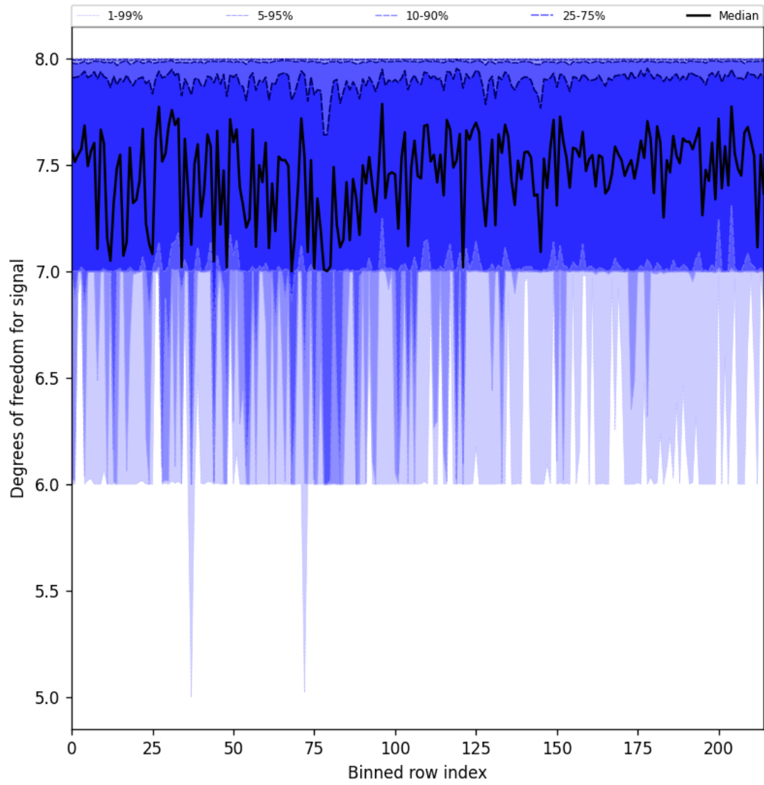
Figure 31: Along track statistics of “Degrees of freedom for signal” for 2025-03-07 to 2025-03-09
