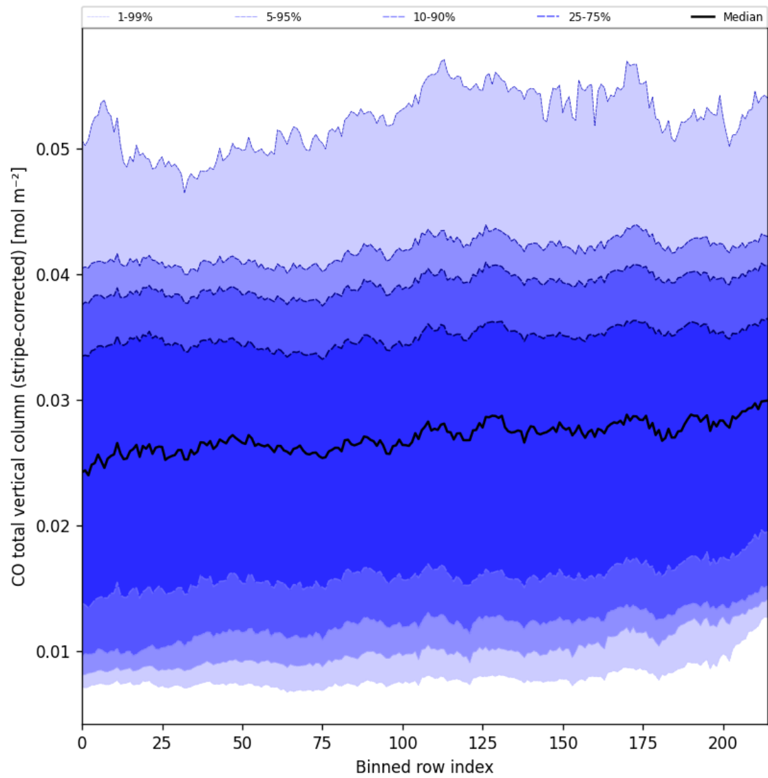
Figure 27: Along track statistics of “CO total vertical column (stripe-corrected)” for 2025-03-07 to 2025-03-09
