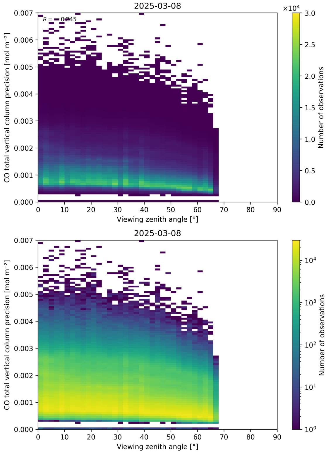
Figure 71: Scatter density plot of “Viewing zenith angle” against “CO total vertical column precision” for 2025-03-07 to 2025-03-09.
