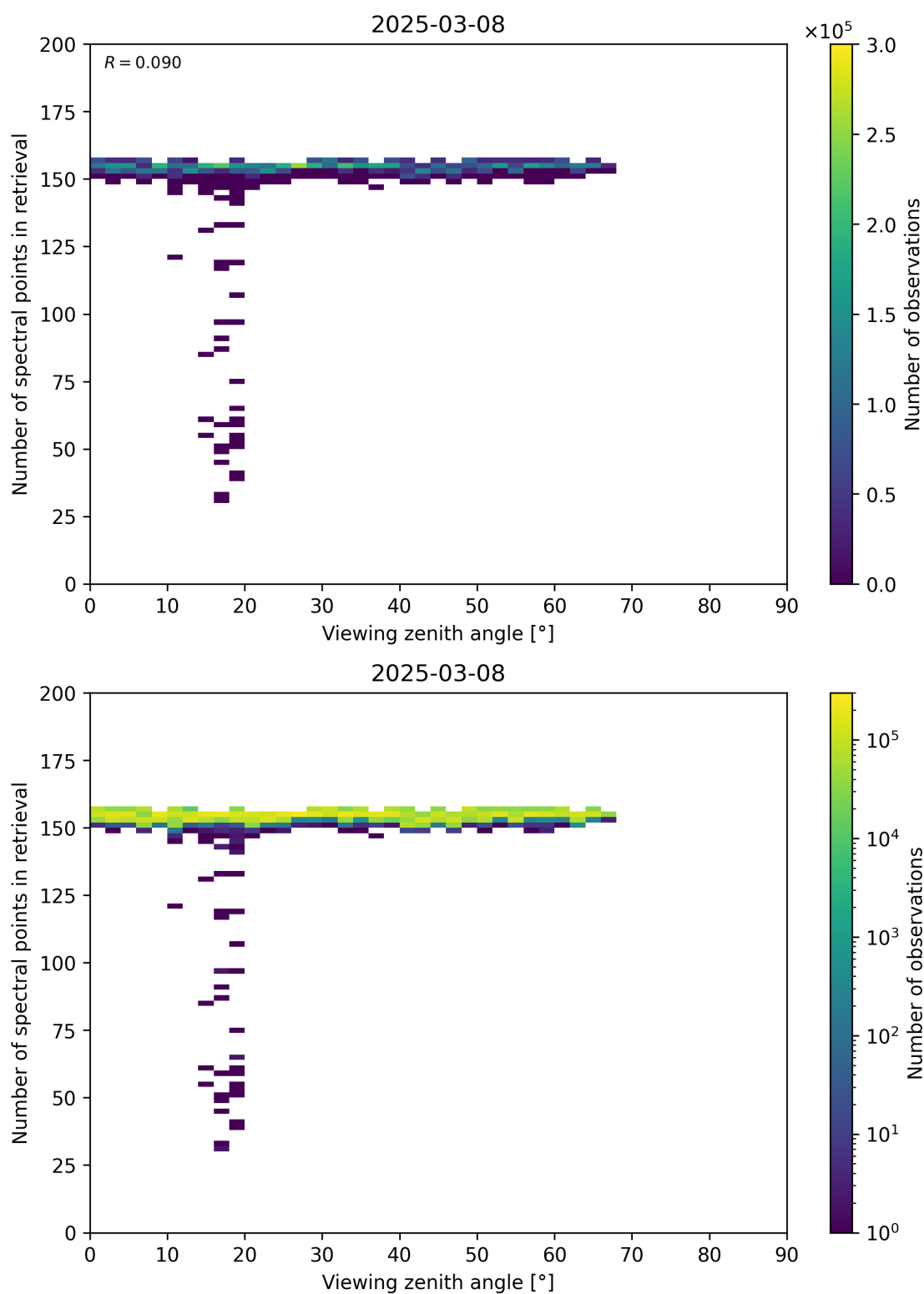
Figure 76: Scatter density plot of “Viewing zenith angle” against “Number of spectral points in retrieval” for 2025-03-07 to 2025-03-09.
