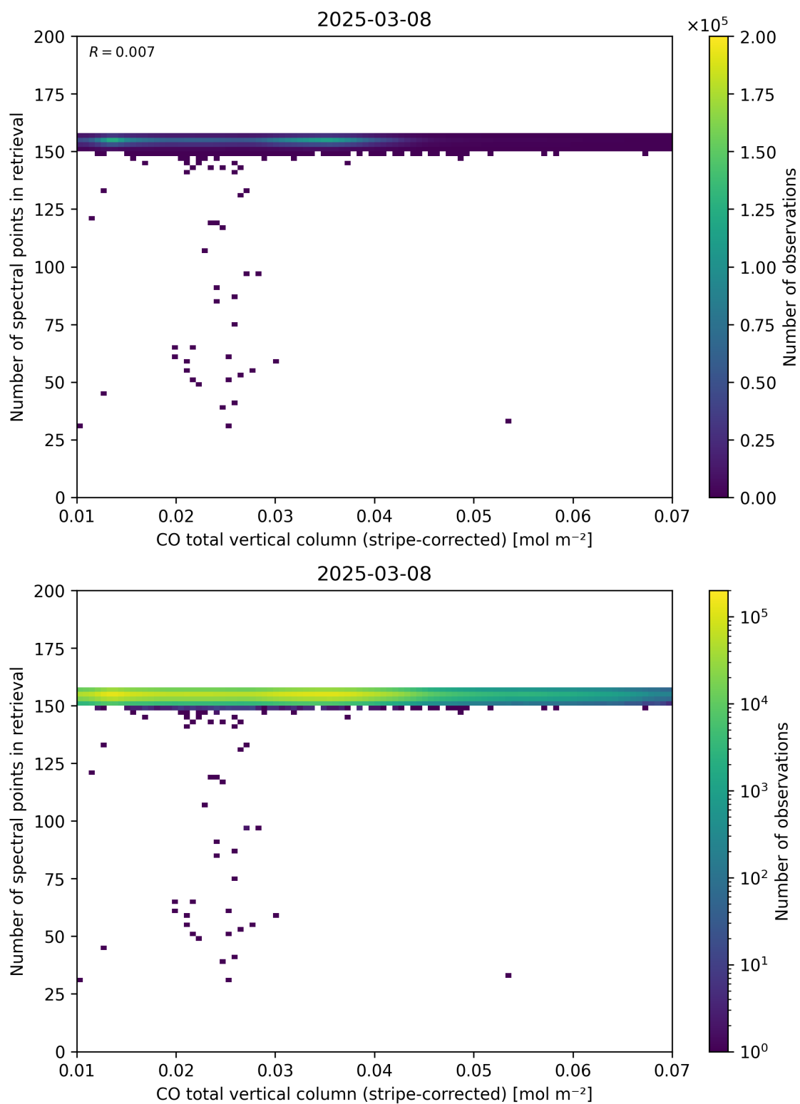
Figure 40: Scatter density plot of “CO total vertical column (stripe-corrected)” against “Number of spectral points in retrieval” for 2025-03-07 to 2025-03-09.
