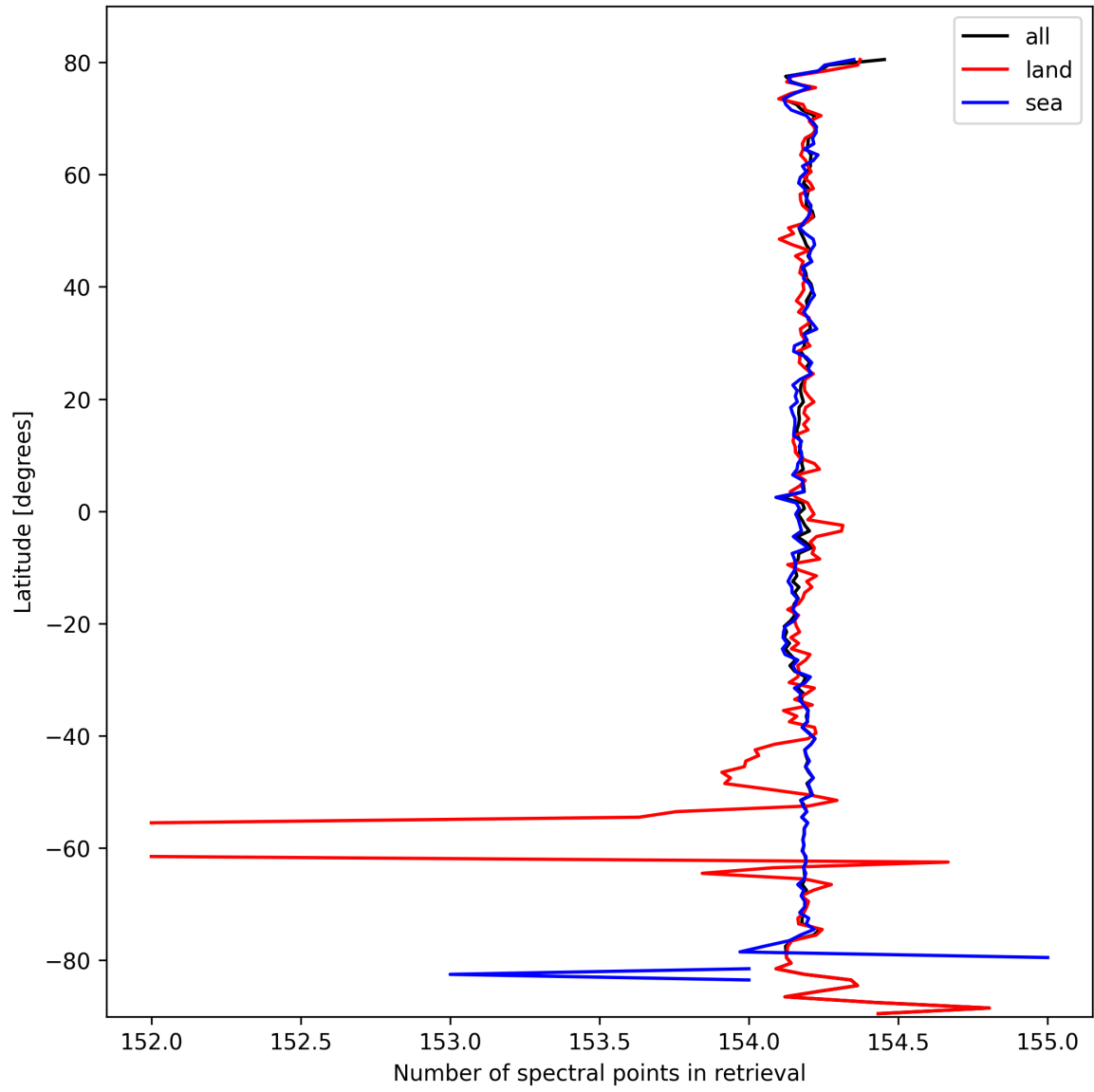
Figure 13: Zonal average of “Number of spectral points in retrieval” for 2025-03-07 to 2025-03-09.
