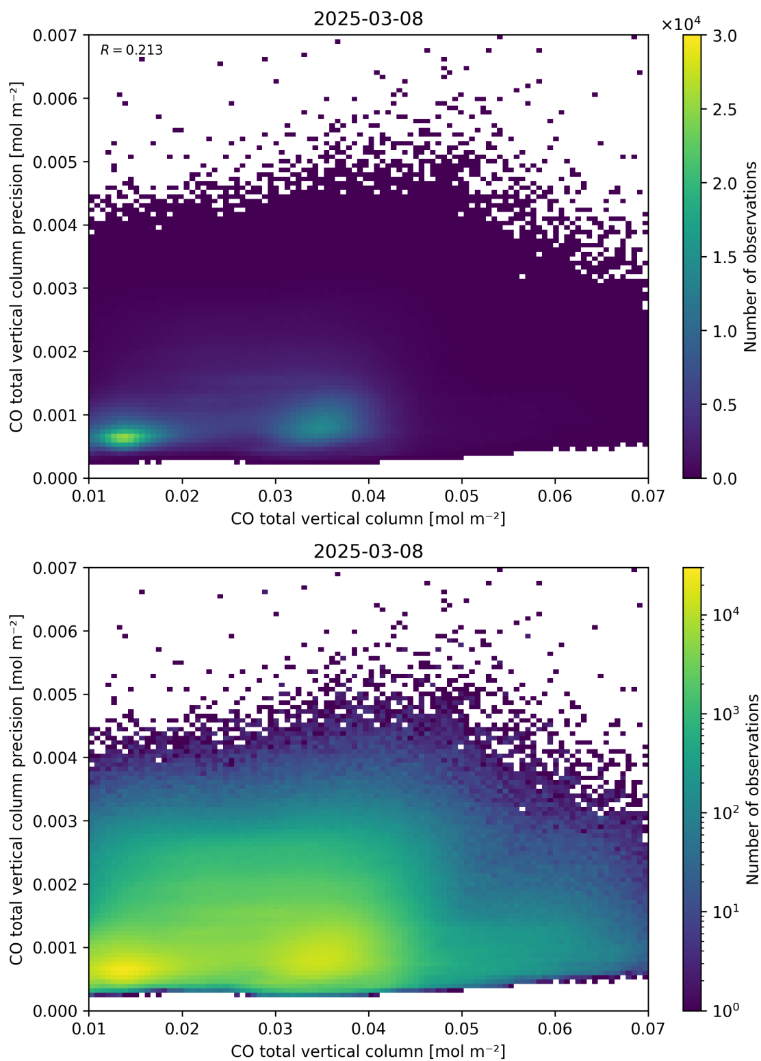
Figure 34: Scatter density plot of “CO total vertical column” against “CO total vertical column precision” for 2025-03-07 to 2025-03-09.
