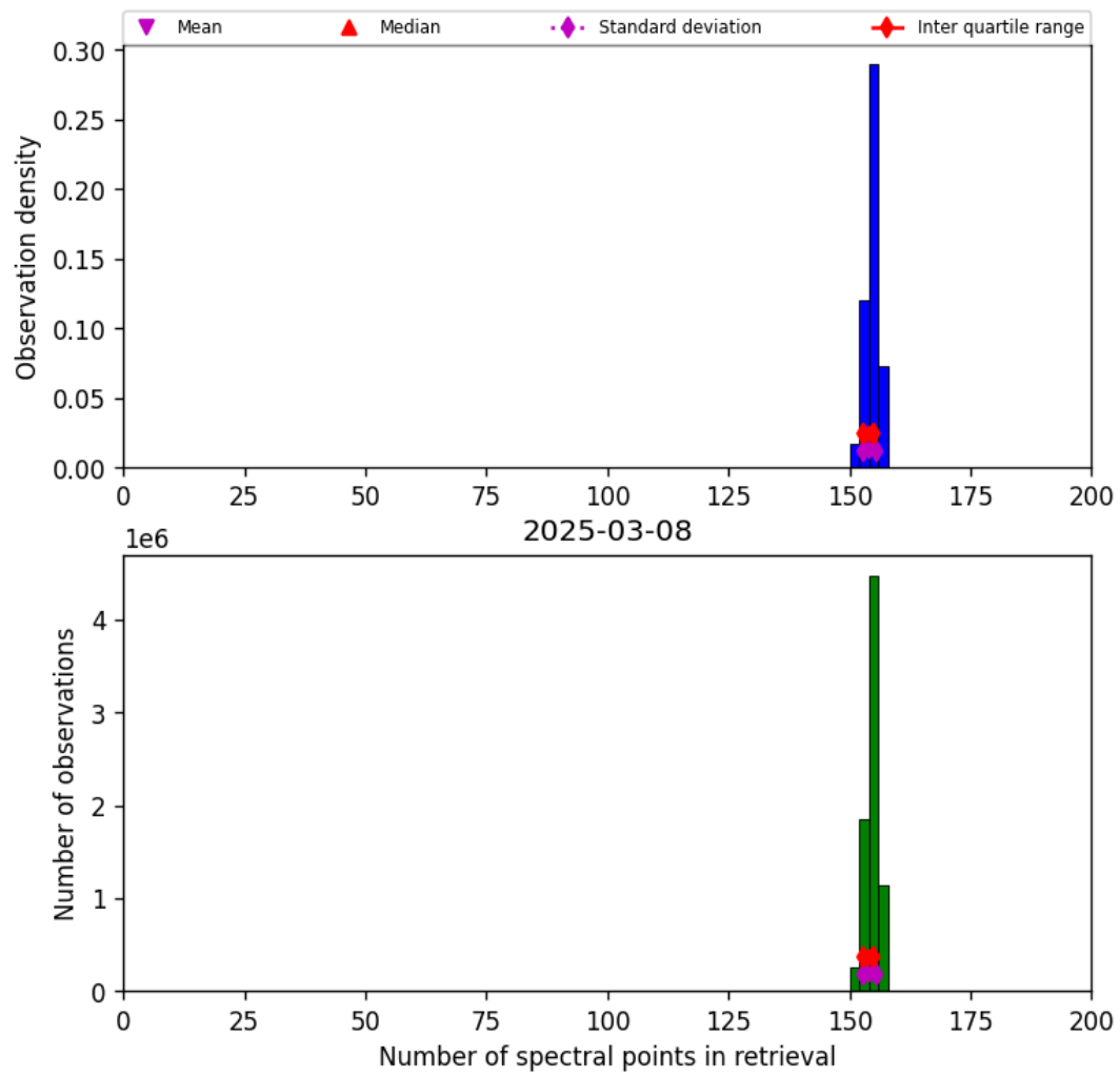
Figure 21: Histogram of “Number of spectral points in retrieval” for 2025-03-07 to 2025-03-09
