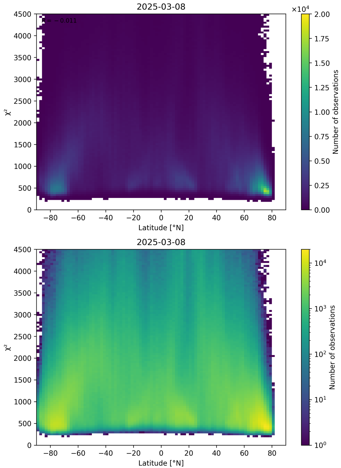
Figure 54: Scatter density plot of “Latitude” against “ \chi^2 ” for 2025-03-07 to 2025-03-09.
