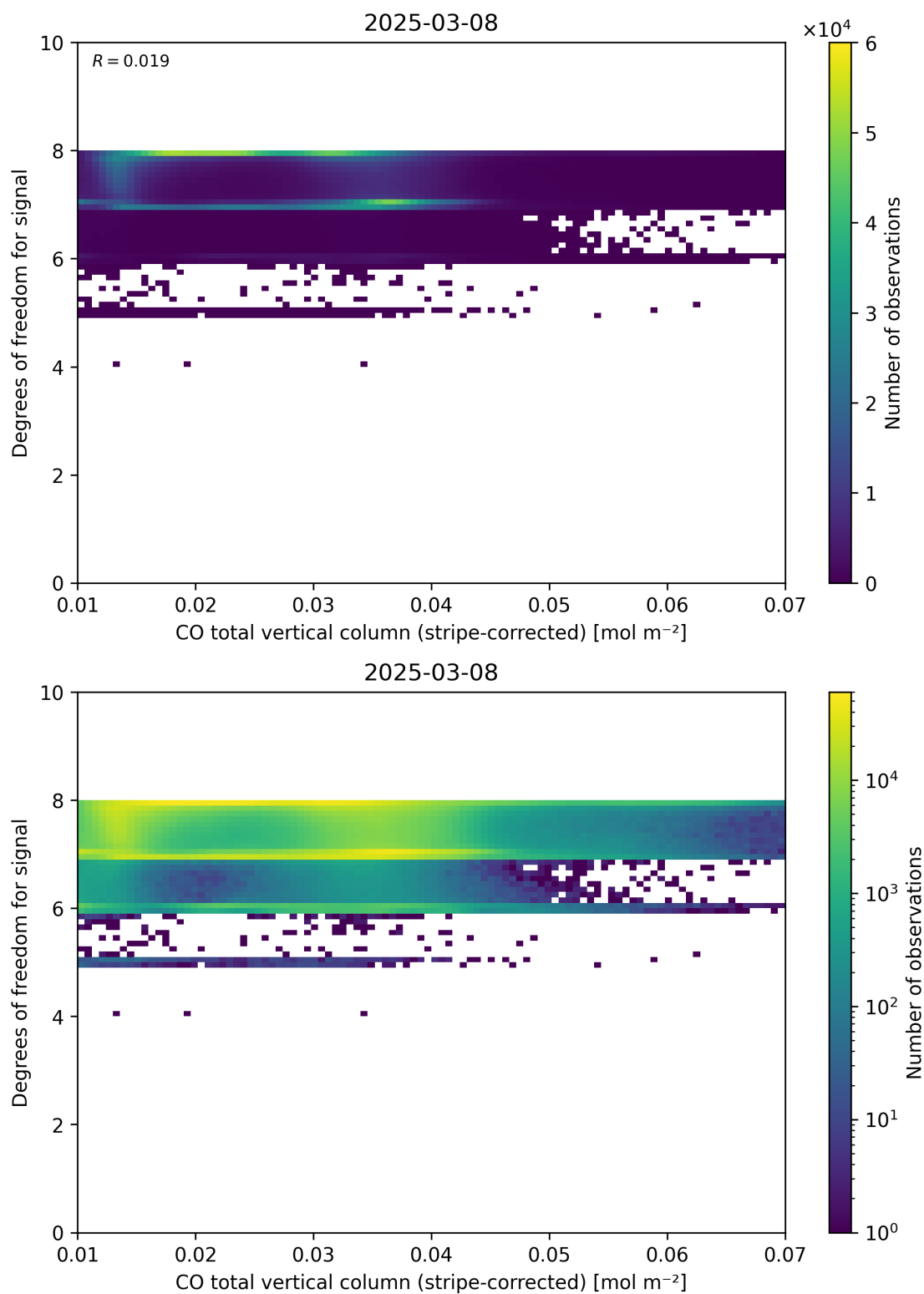
Figure 38: Scatter density plot of “CO total vertical column (stripe-corrected)” against “Degrees of freedom for signal” for 2025-03-07 to 2025-03-09.
