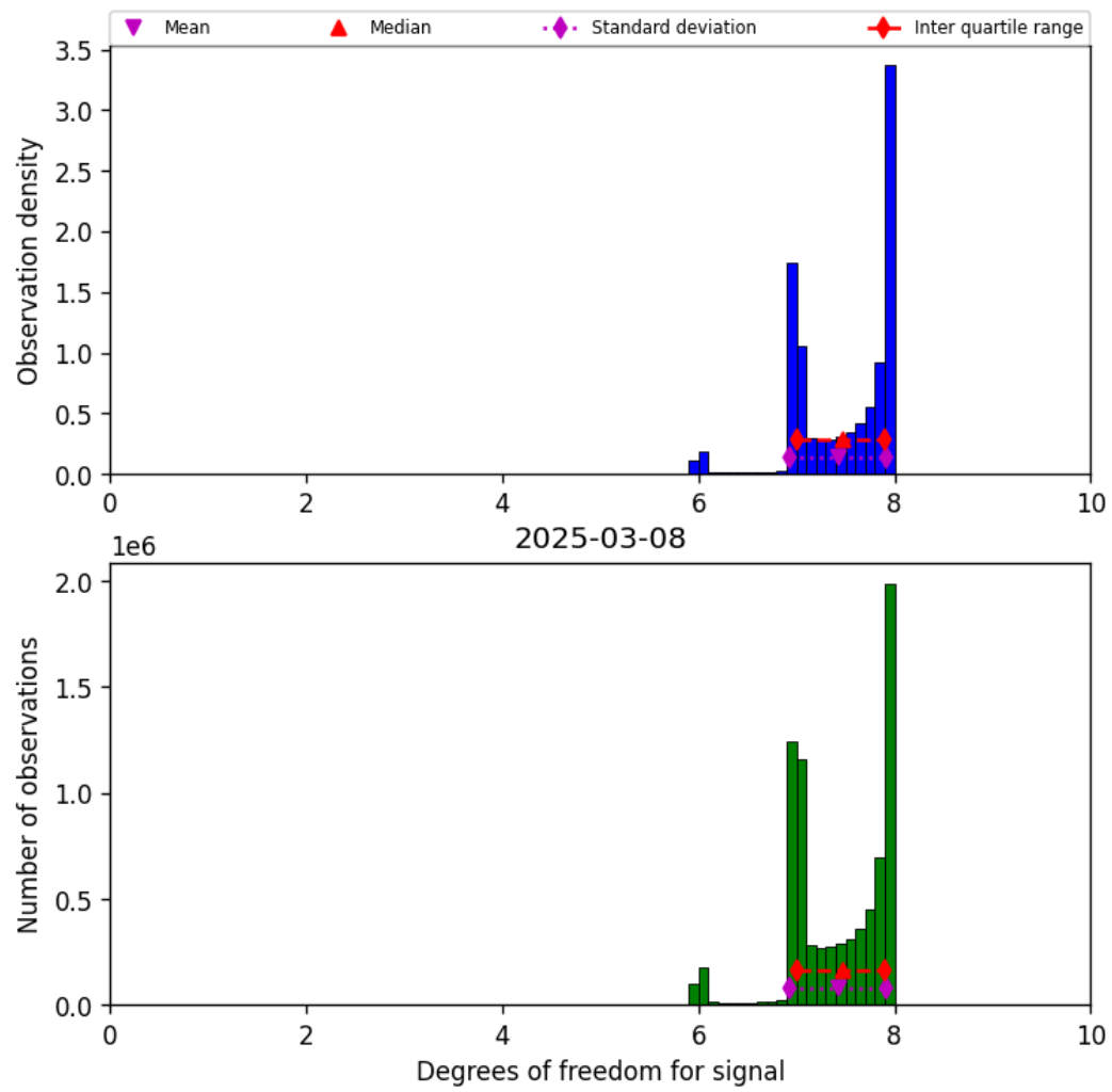
Figure 23: Histogram of “Degrees of freedom for signal” for 2025-03-07 to 2025-03-09
