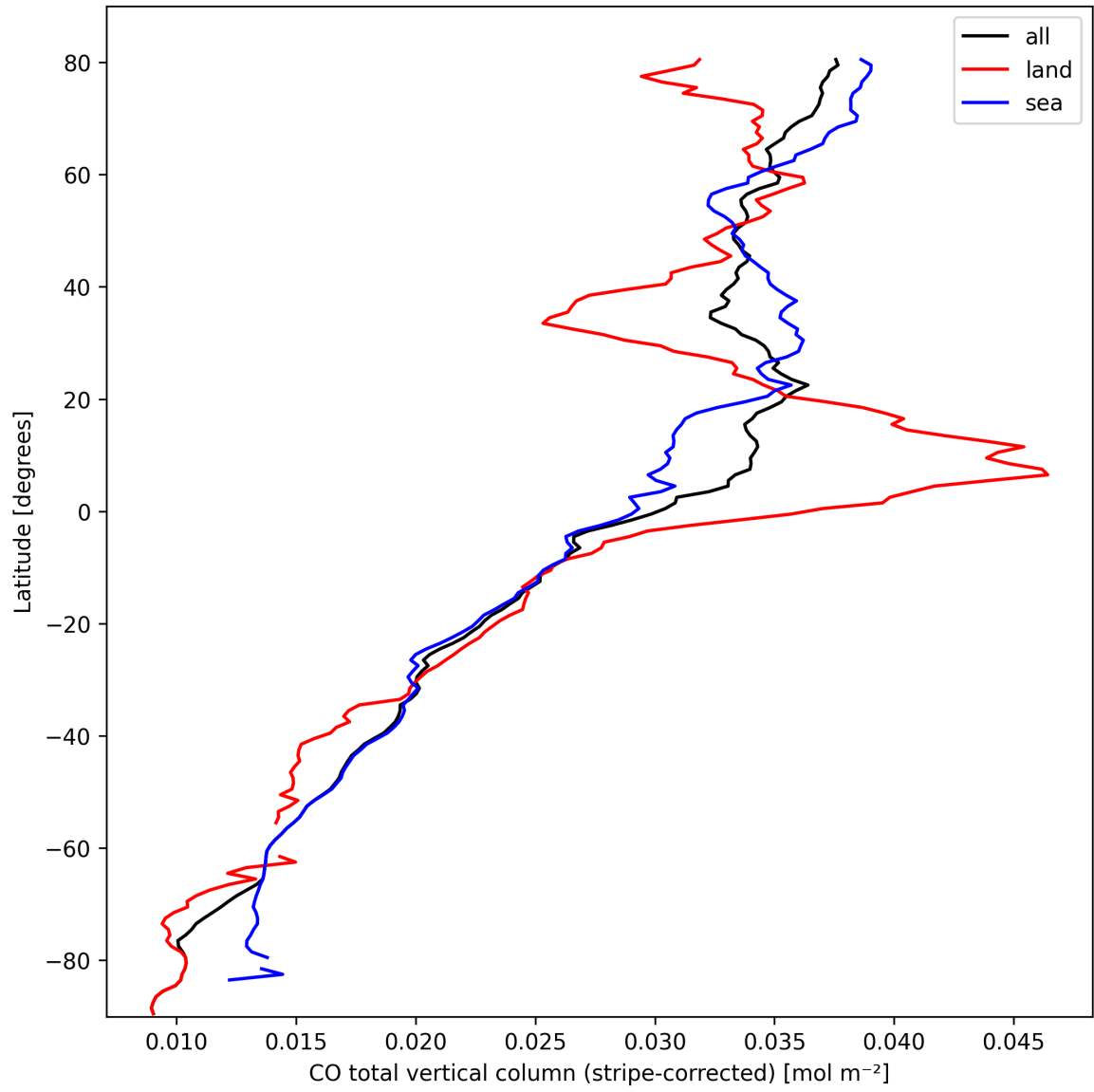
Figure 11: Zonal average of “CO total vertical column (stripe-corrected)” for 2025-03-07 to 2025-03-09.
