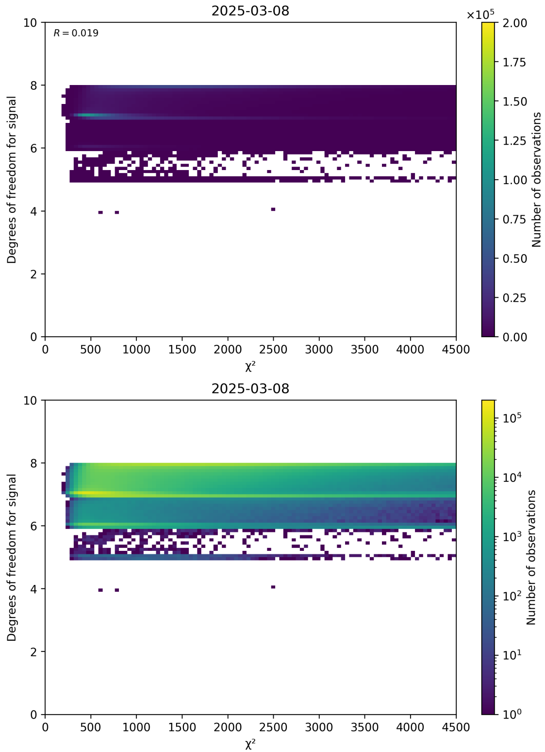
Figure 48: Scatter density plot of “ \chi^2 ” against “Degrees of freedom for signal” for 2025-03-07 to 2025-03-09.
