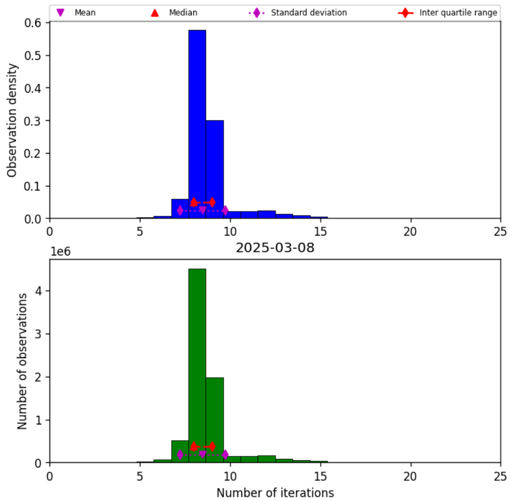
Figure 24: Histogram of “Number of iterations” for 2025-03-07 to 2025-03-09
