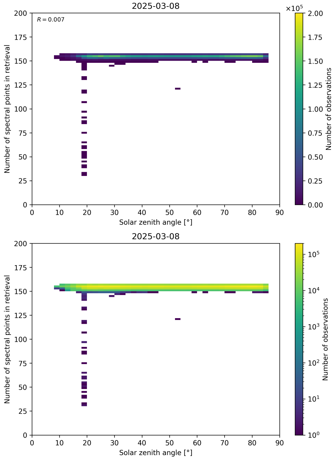
Figure 68: Scatter density plot of “Solar zenith angle” against “Number of spectral points in retrieval” for 2025-03-07 to 2025-03-09.
