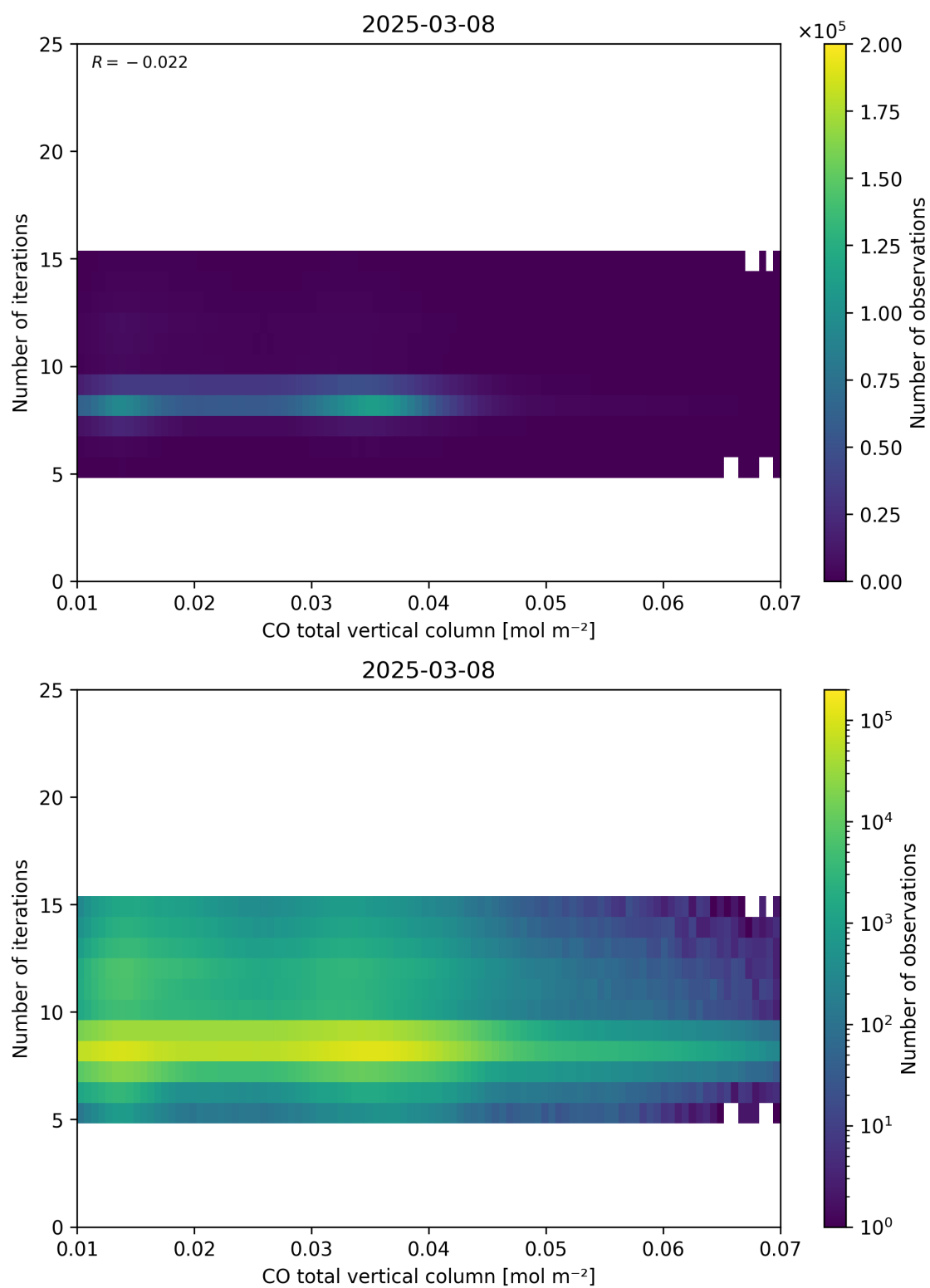
Figure 42: Scatter density plot of “CO total vertical column” against “Number of iterations” for 2025-03-07 to 2025-03-09.
