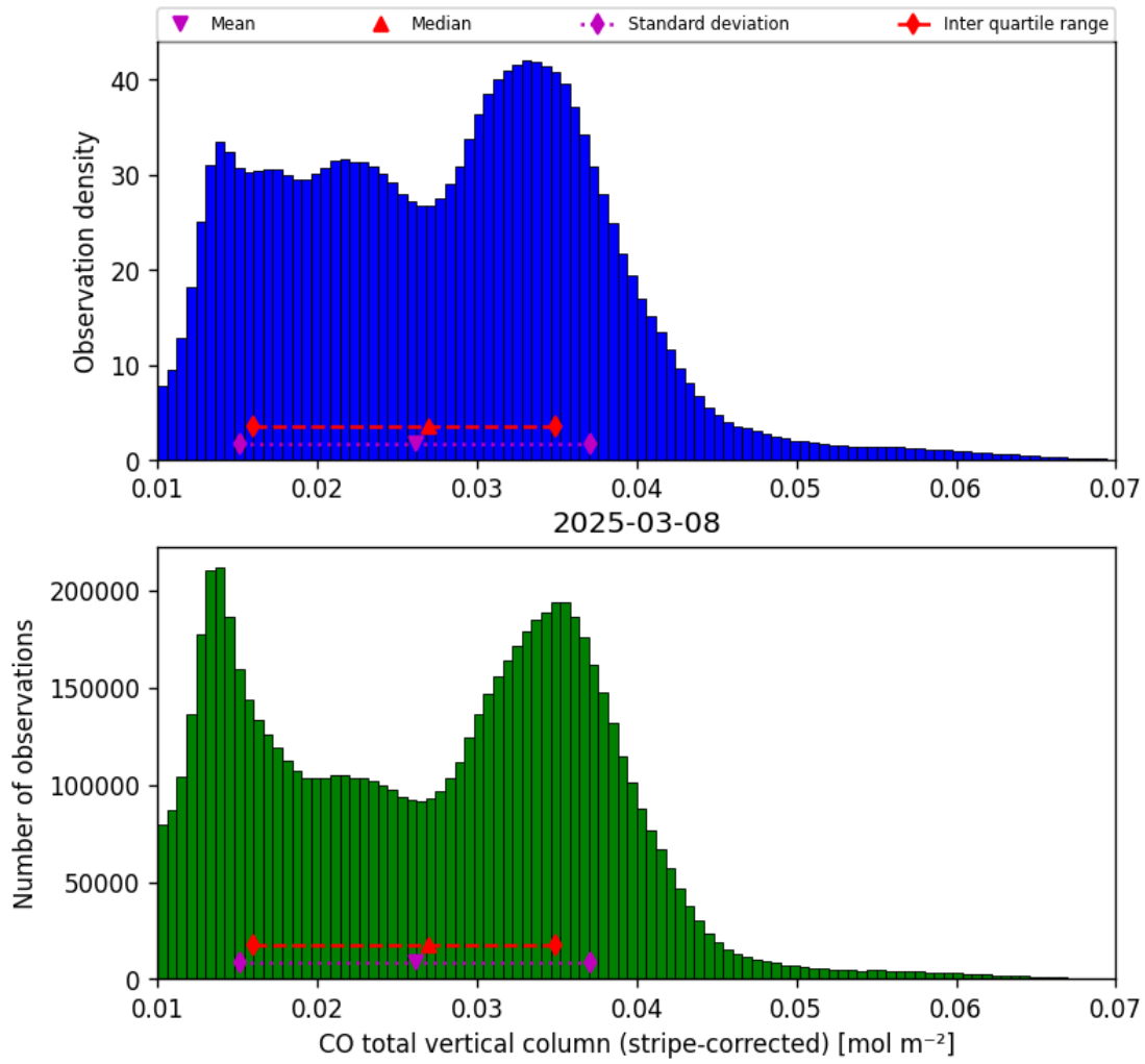
Figure 19: Histogram of “CO total vertical column (stripe-corrected)” for 2025-03-07 to 2025-03-09
