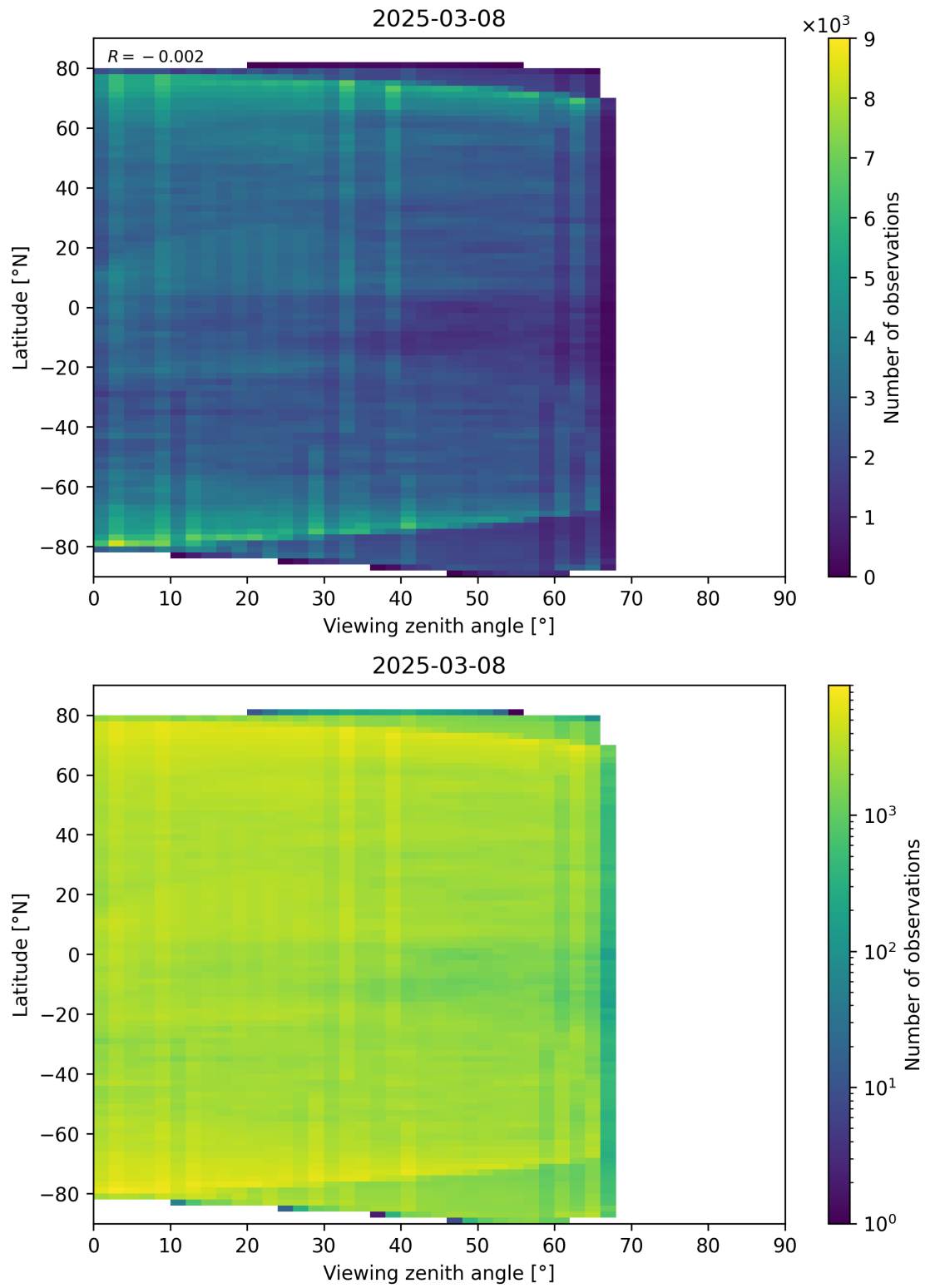
Figure 74: Scatter density plot of “Viewing zenith angle” against “Latitude” for 2025-03-07 to 2025-03-09.
