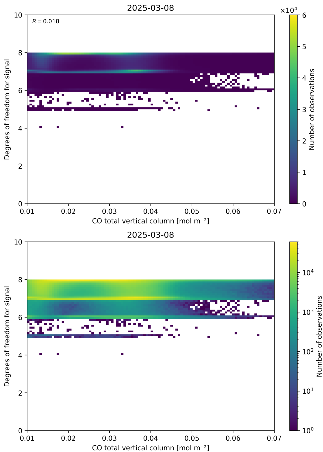
Figure 41: Scatter density plot of “CO total vertical column” against “Degrees of freedom for signal” for 2025-03-07 to 2025-03-09.
