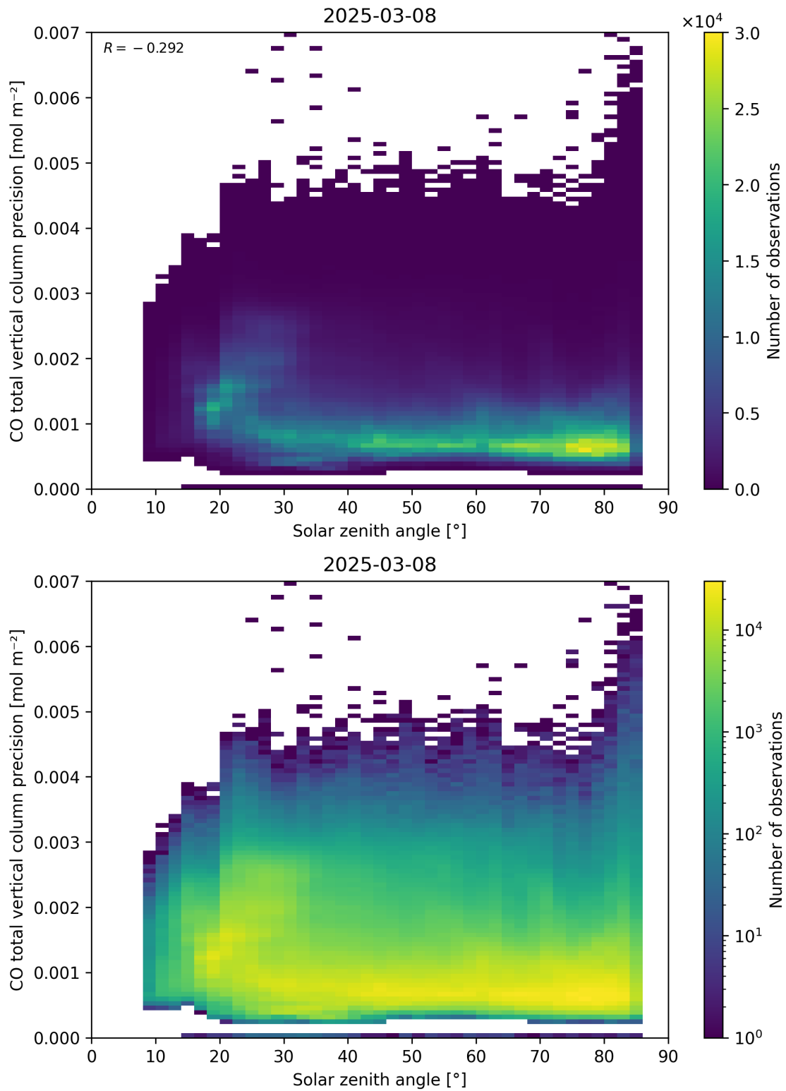
Figure 63: Scatter density plot of “Solar zenith angle” against “CO total vertical column precision” for 2025-03-07 to 2025-03-09.
