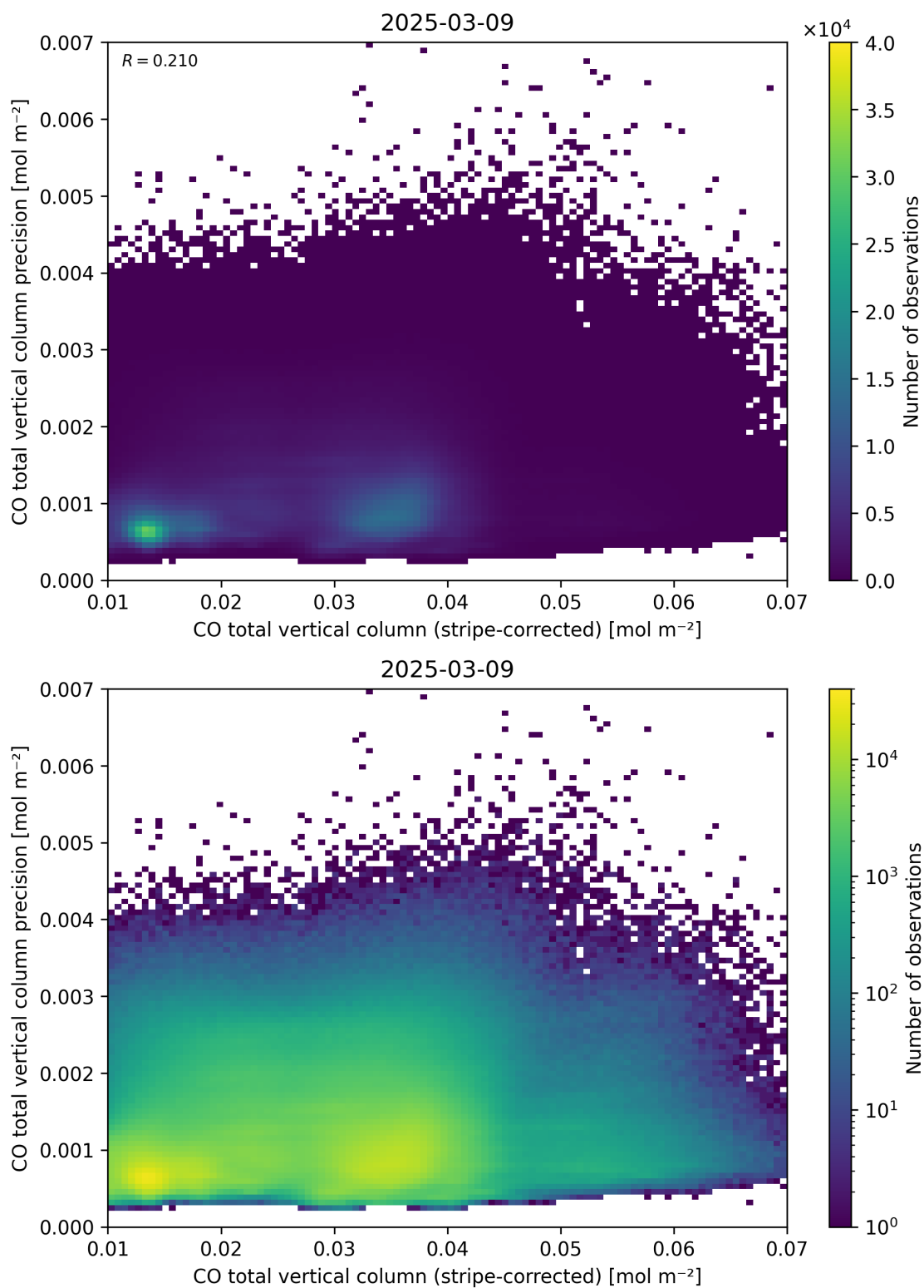
Figure 36: Scatter density plot of “CO total vertical column (stripe-corrected)” against “CO total vertical column precision” for 2025-03-08 to 2025-03-10.
