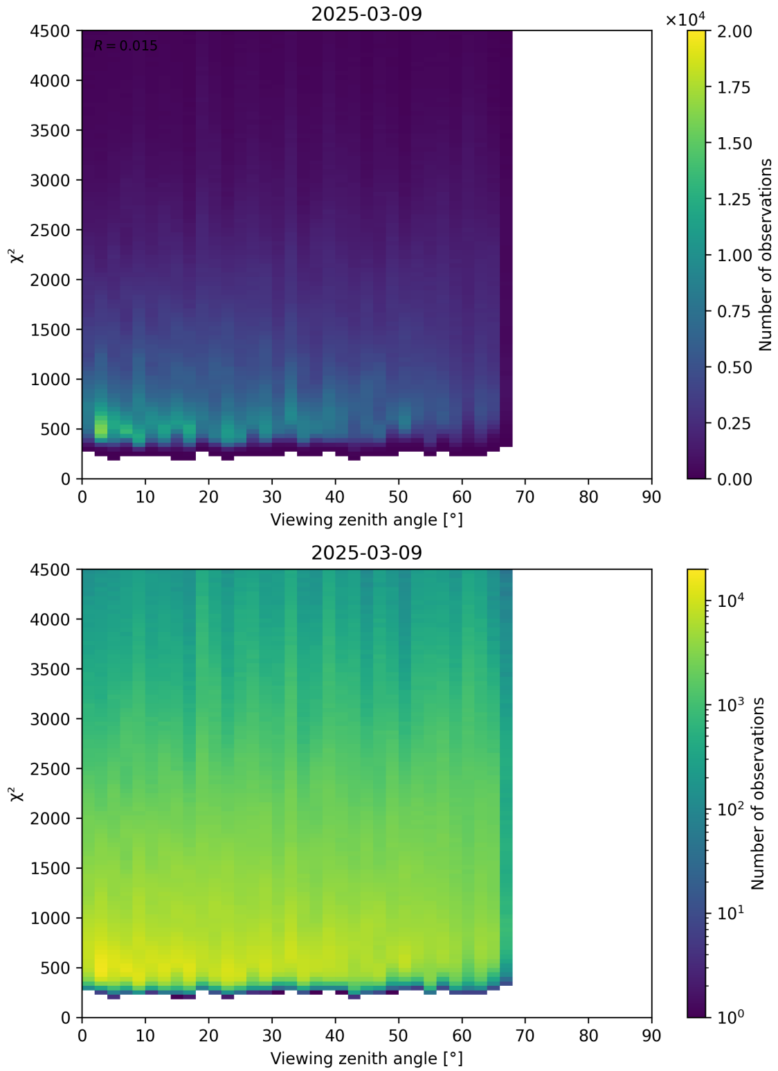
Figure 72: Scatter density plot of “Viewing zenith angle” against “ \chi^2 ” for 2025-03-08 to 2025-03-10.
