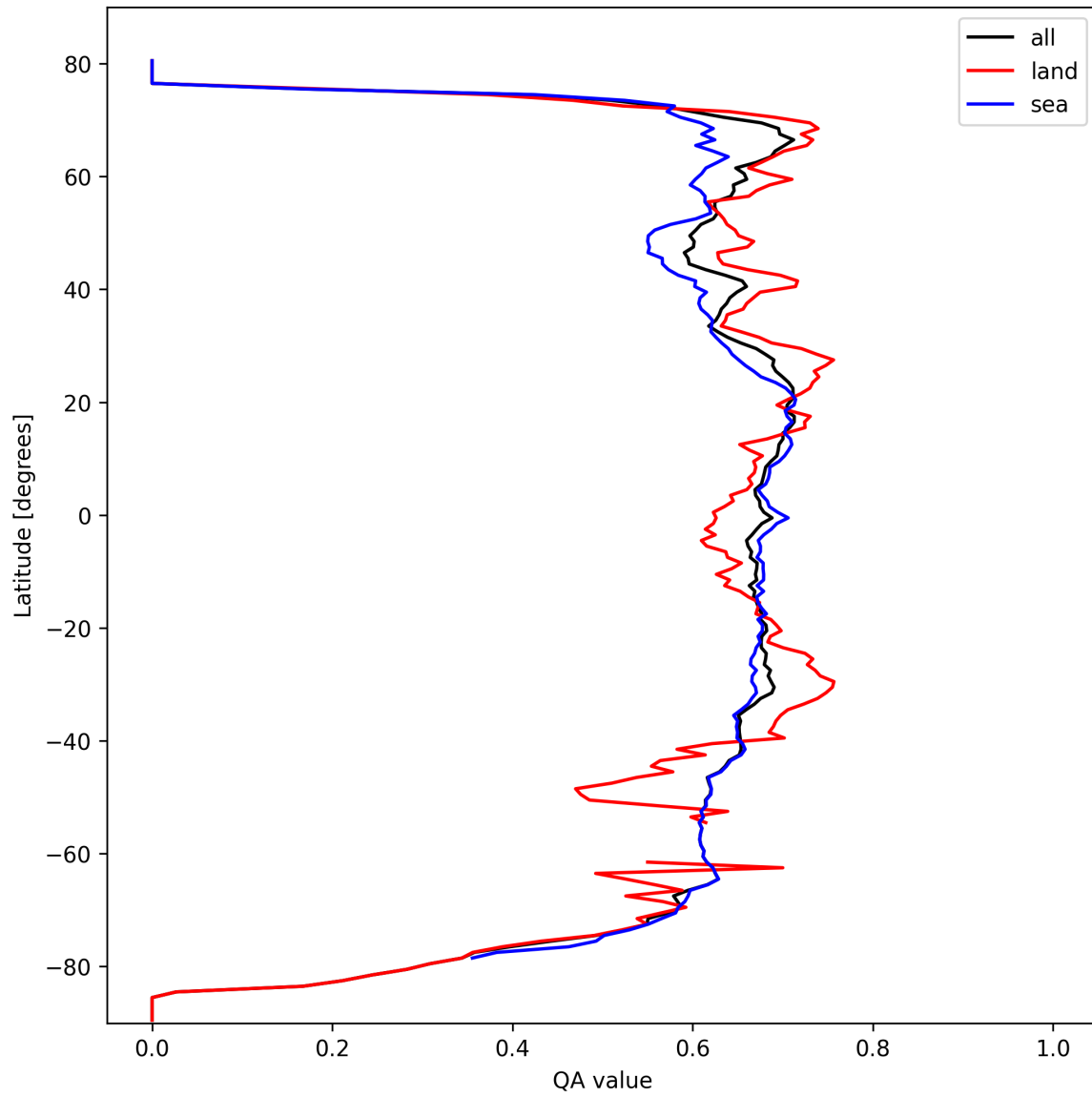
Figure 9: Zonal average of “QA value” for 2025-03-08 to 2025-03-10.
