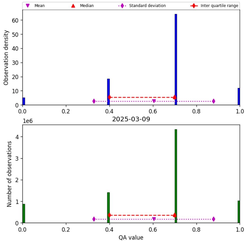
Figure 17: Histogram of “QA value” for 2025-03-08 to 2025-03-10
