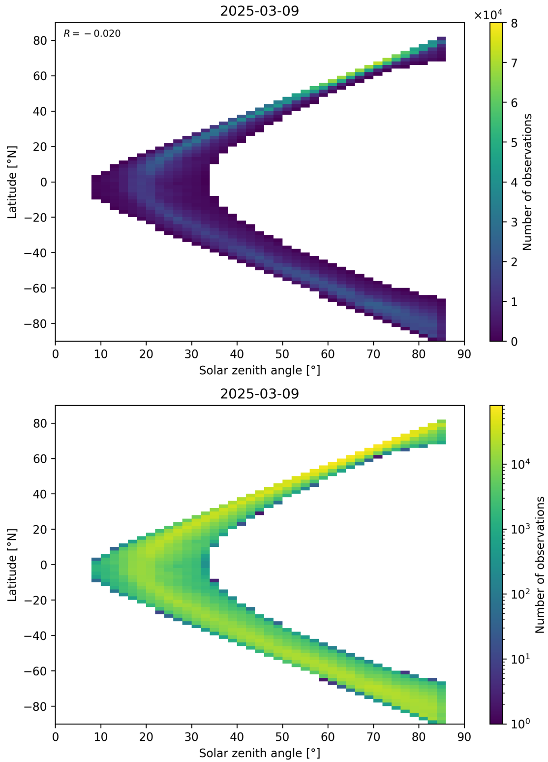
Figure 66: Scatter density plot of “Solar zenith angle” against “Latitude” for 2025-03-08 to 2025-03-10.
