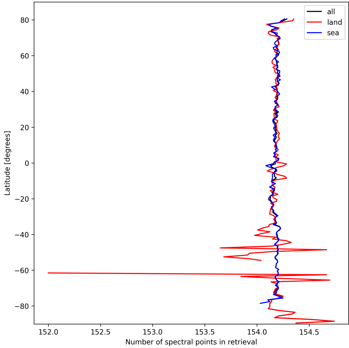
Figure 13: Zonal average of “Number of spectral points in retrieval” for 2025-03-08 to 2025-03-10.
