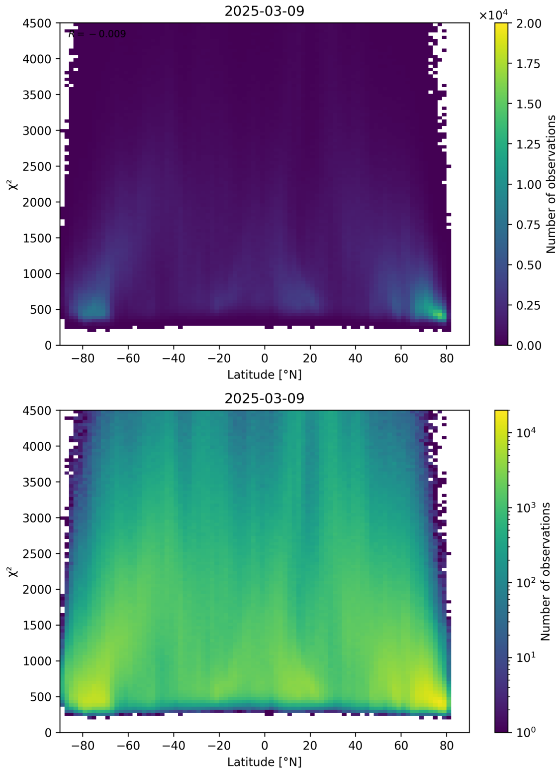
Figure 54: Scatter density plot of “Latitude” against “ \chi^2 ” for 2025-03-08 to 2025-03-10.
