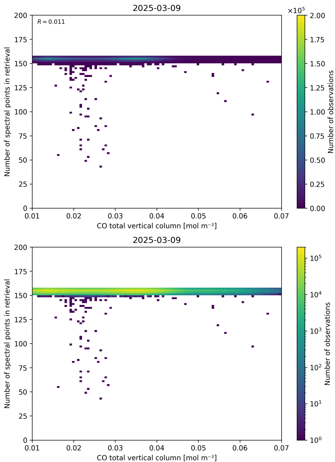
Figure 43: Scatter density plot of “CO total vertical column” against “Number of spectral points in retrieval” for 2025-03-08 to 2025-03-10.
