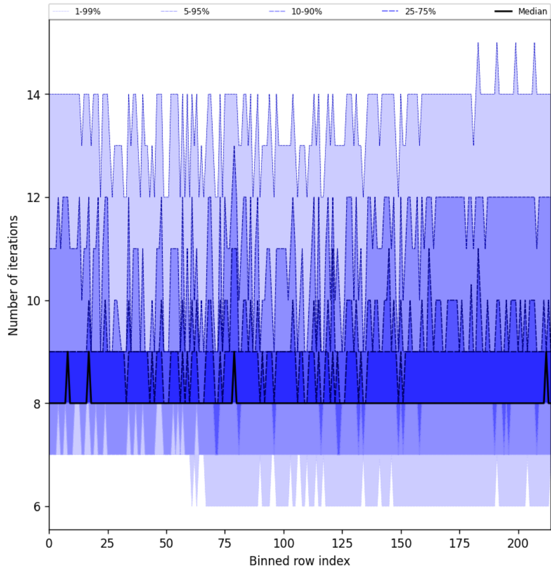
Figure 32: Along track statistics of “Number of iterations” for 2025-03-08 to 2025-03-10
