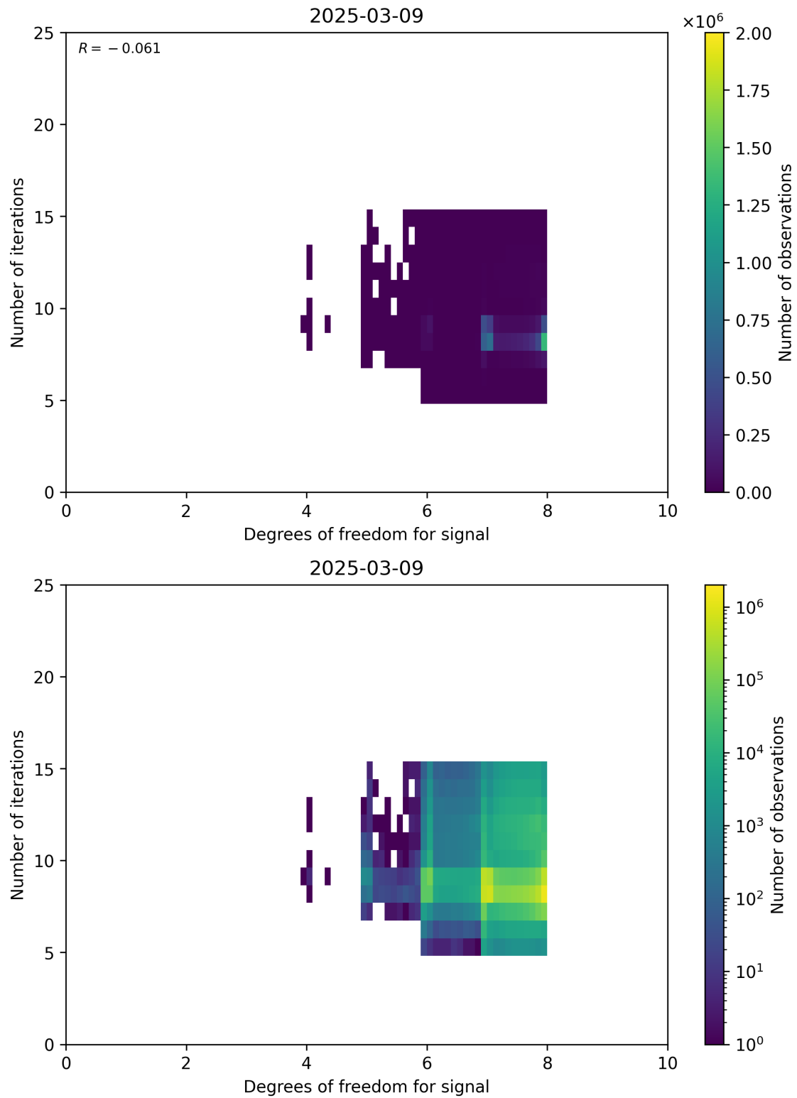
Figure 50: Scatter density plot of “Degrees of freedom for signal” against “Number of iterations” for 2025-03-08 to 2025-03-10.
