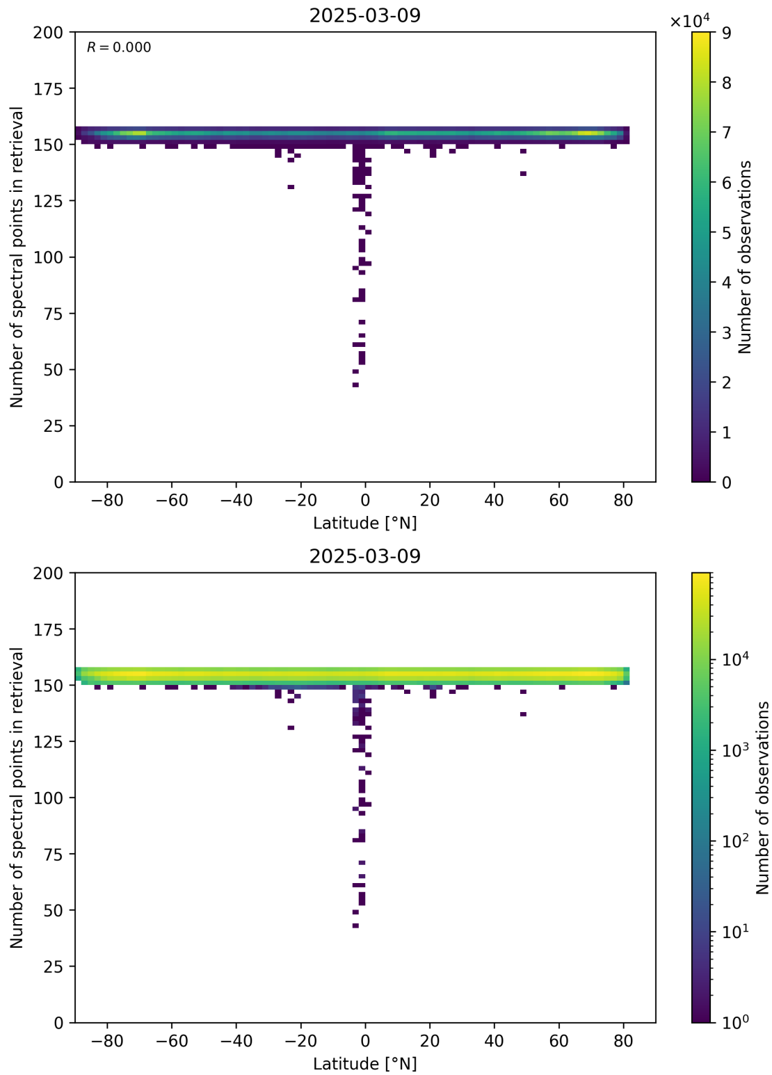
Figure 57: Scatter density plot of “Latitude” against “Number of spectral points in retrieval” for 2025-03-08 to 2025-03-10.
