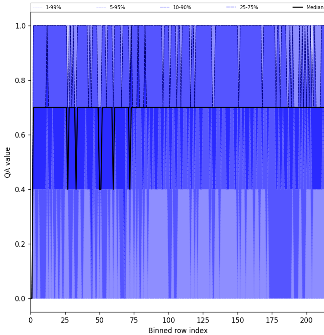
Figure 25: Along track statistics of “QA value” for 2025-03-08 to 2025-03-10
