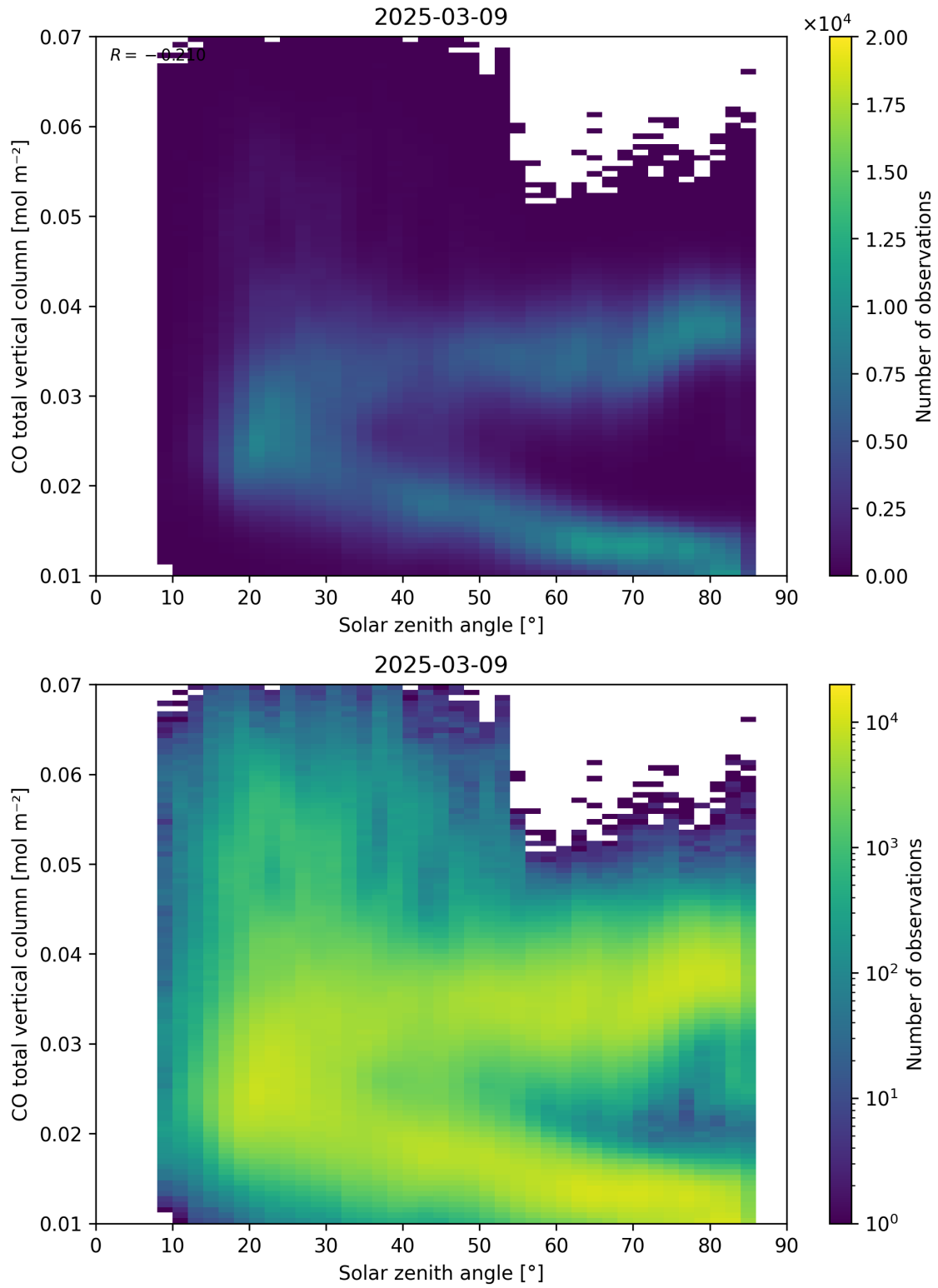
Figure 61: Scatter density plot of “Solar zenith angle” against “CO total vertical column” for 2025-03-08 to 2025-03-10.
