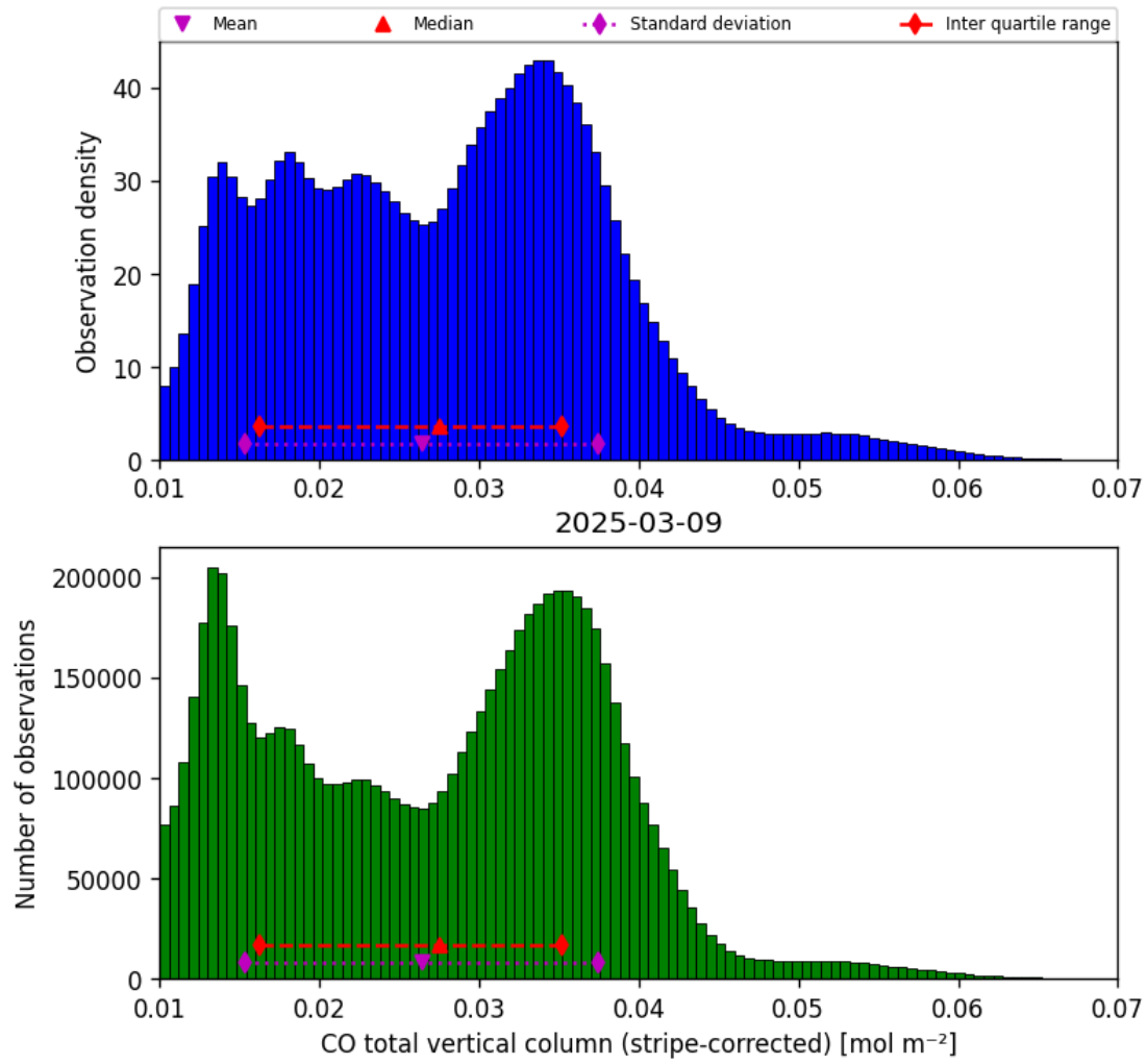
Figure 19: Histogram of “CO total vertical column (stripe-corrected)” for 2025-03-08 to 2025-03-10
