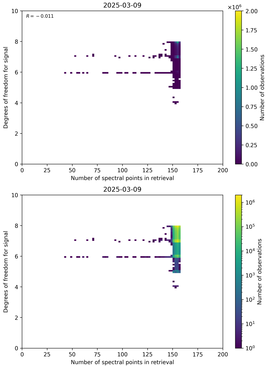
Figure 59: Scatter density plot of “Number of spectral points in retrieval” against “Degrees of freedom for signal” for 2025-03-08 to 2025-03-10.
