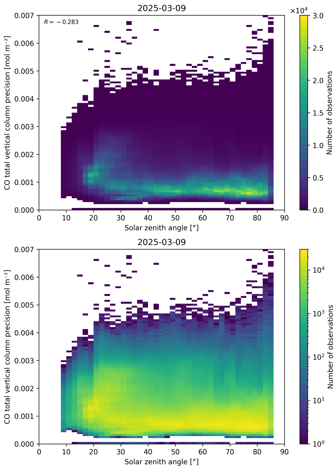
Figure 63: Scatter density plot of “Solar zenith angle” against “CO total vertical column precision” for 2025-03-08 to 2025-03-10.
