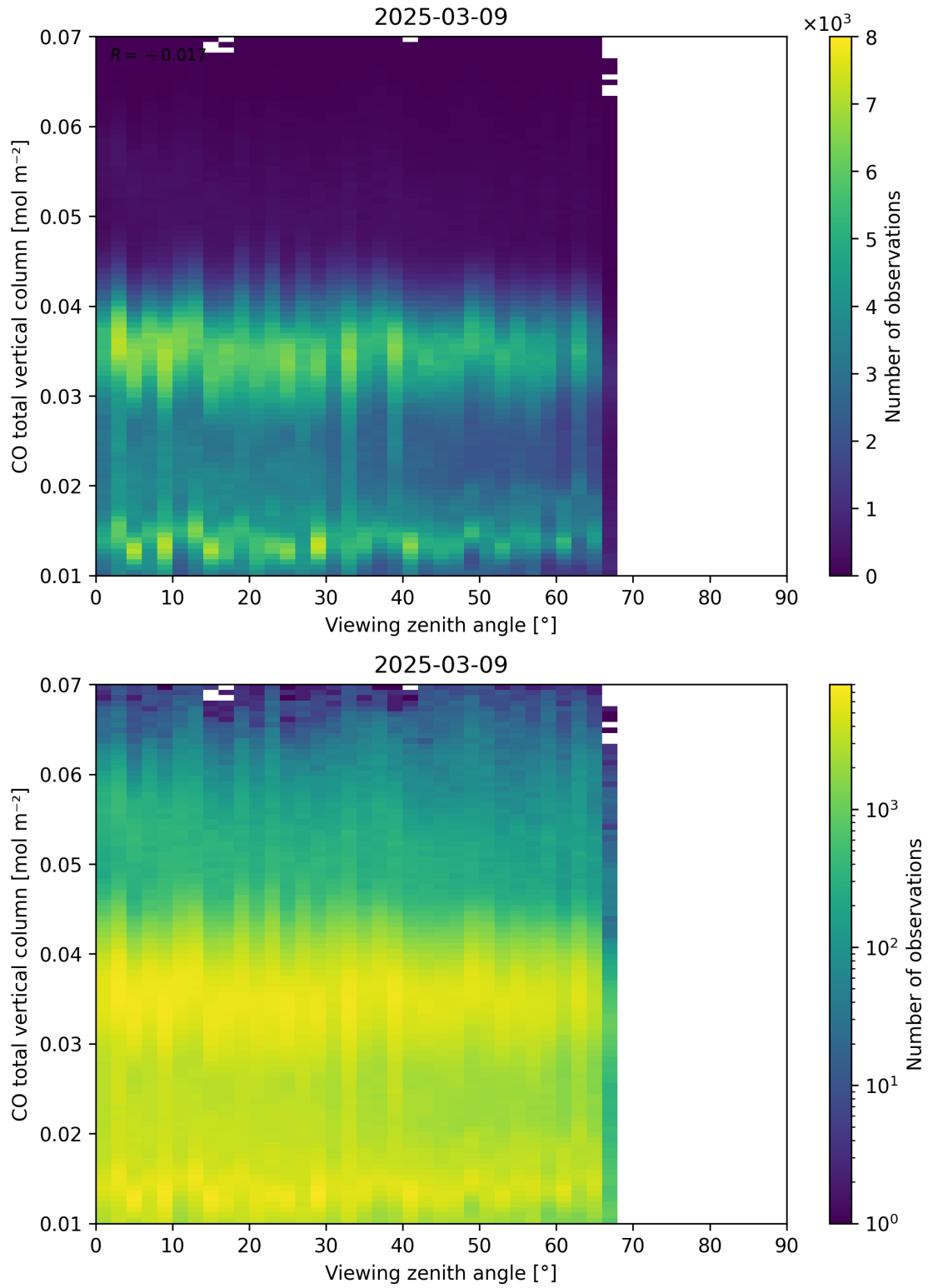
Figure 69: Scatter density plot of “Viewing zenith angle” against “CO total vertical column” for 2025-03-08 to 2025-03-10.
