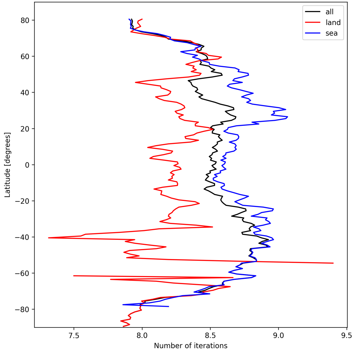
Figure 16: Zonal average of “Number of iterations” for 2025-03-08 to 2025-03-10.
