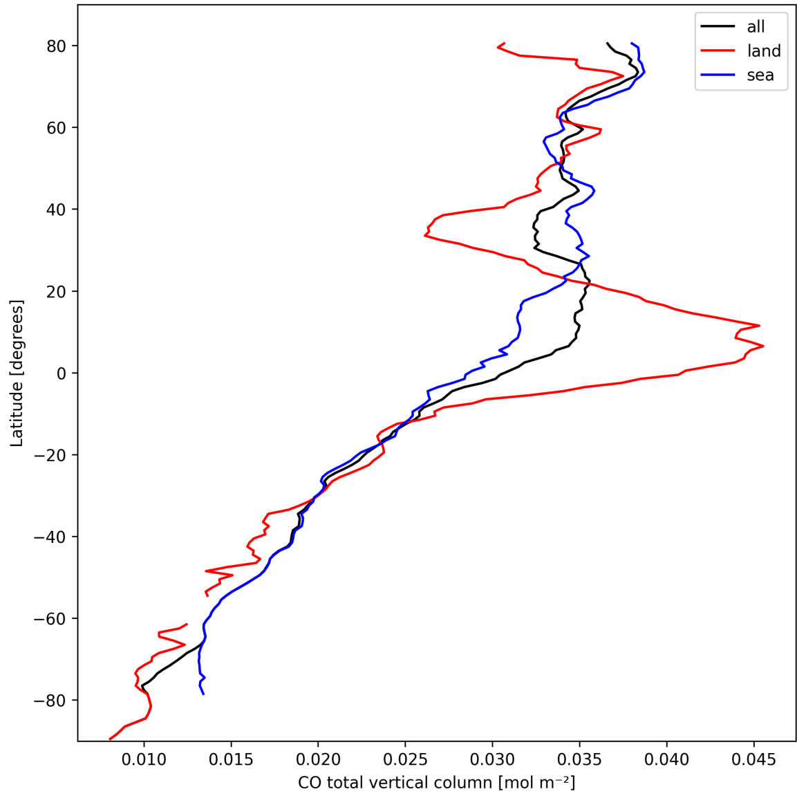
Figure 10: Zonal average of “CO total vertical column” for 2025-03-08 to 2025-03-10.
