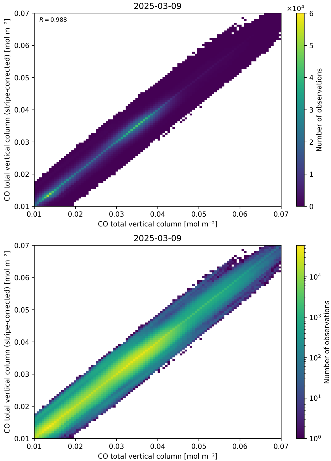
Figure 33: Scatter density plot of “CO total vertical column” against “CO total vertical column (stripe-corrected)” for 2025-03-08 to 2025-03-10.
