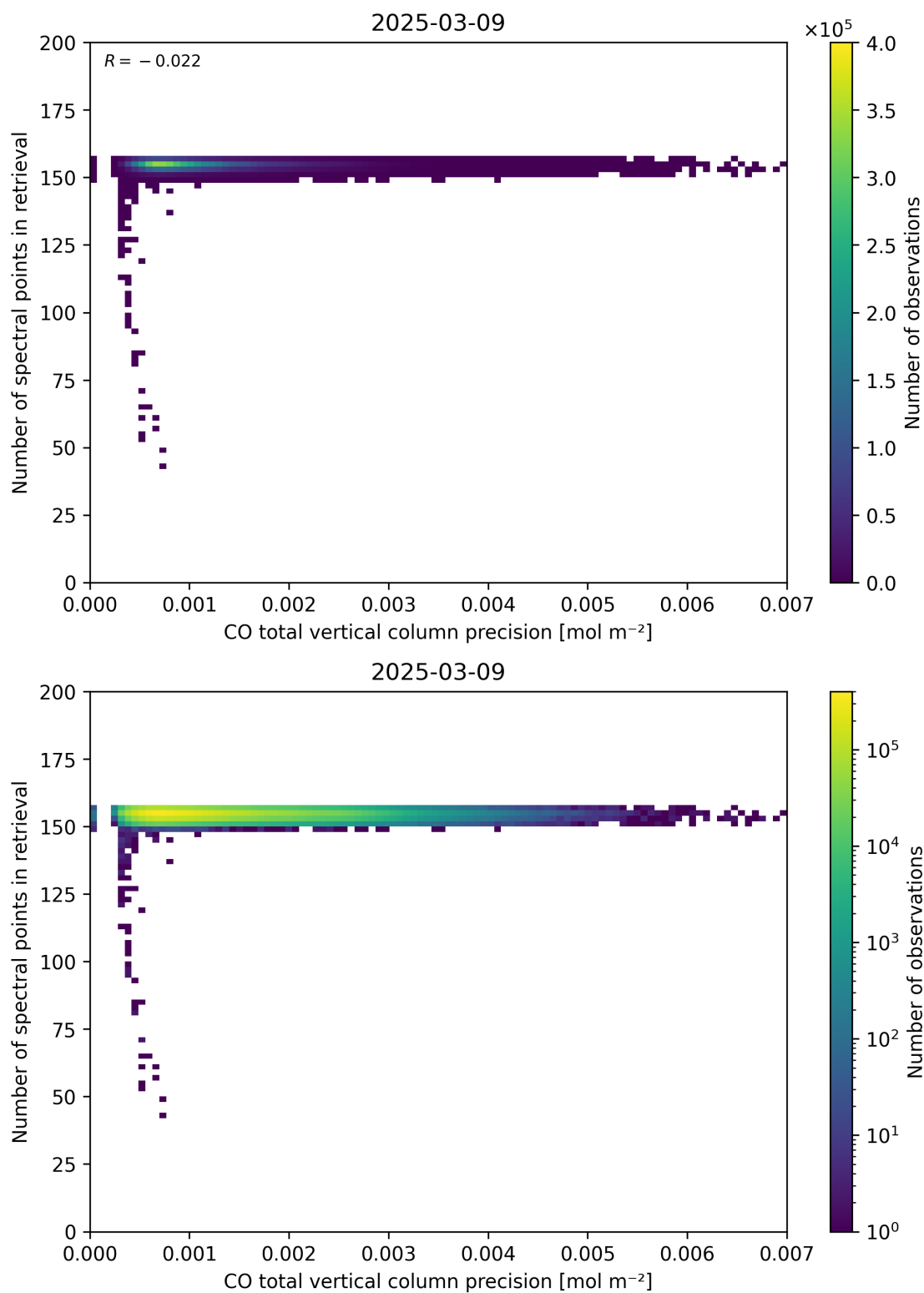
Figure 47: Scatter density plot of “CO total vertical column precision” against “Number of spectral points in retrieval” for 2025-03-08 to 2025-03-10.
