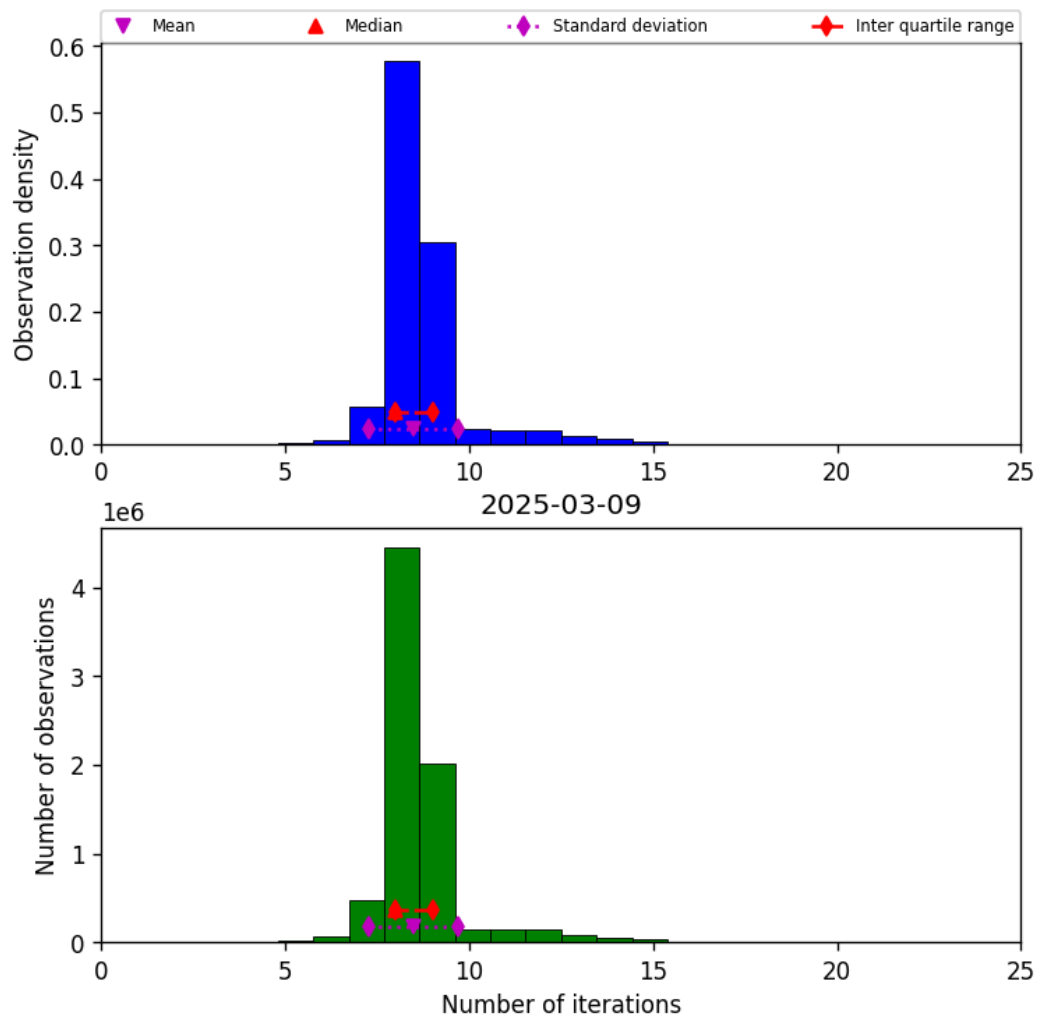
Figure 24: Histogram of “Number of iterations” for 2025-03-08 to 2025-03-10
