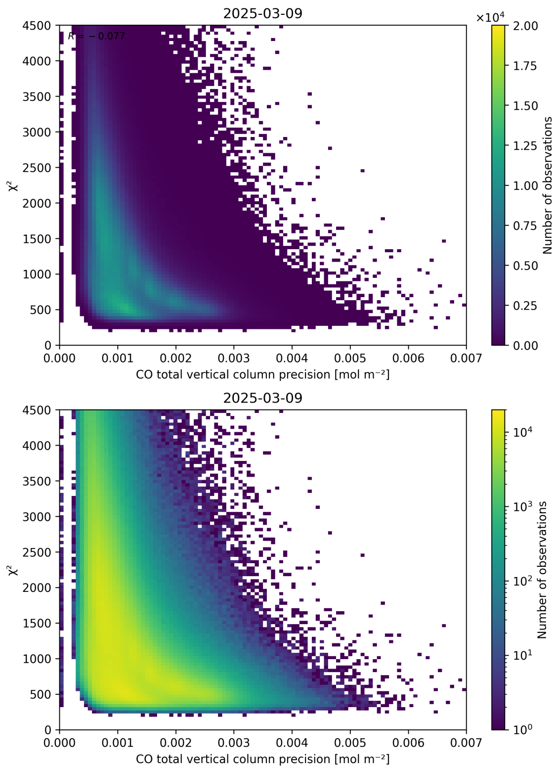
Figure 44: Scatter density plot of “CO total vertical column precision” against “ \chi^2 ” for 2025-03-08 to 2025-03-10.
