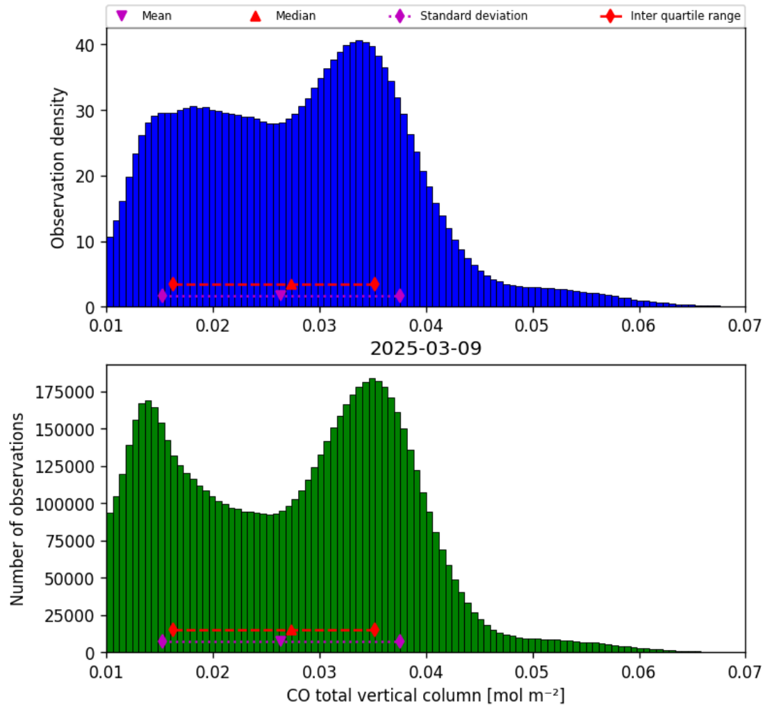
Figure 18: Histogram of “CO total vertical column” for 2025-03-08 to 2025-03-10
