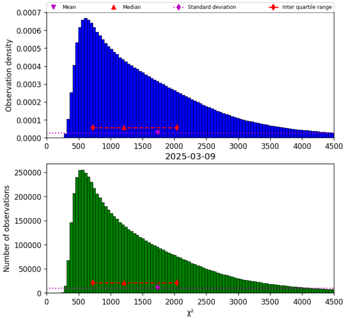
Figure 22: Histogram of “ \chi^2 ” for 2025-03-08 to 2025-03-10
