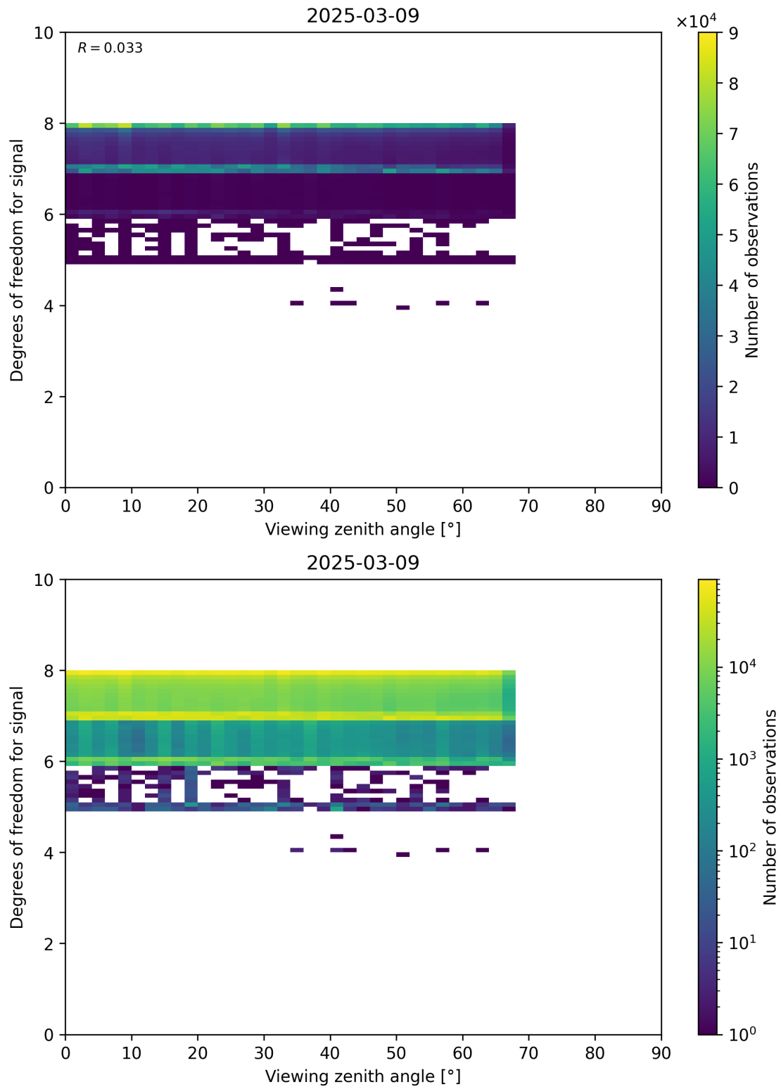
Figure 73: Scatter density plot of “Viewing zenith angle” against “Degrees of freedom for signal” for 2025-03-08 to 2025-03-10.
