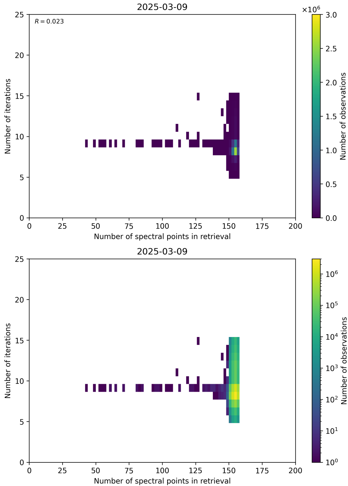
Figure 60: Scatter density plot of “Number of spectral points in retrieval” against “Number of iterations” for 2025-03-08 to 2025-03-10.
