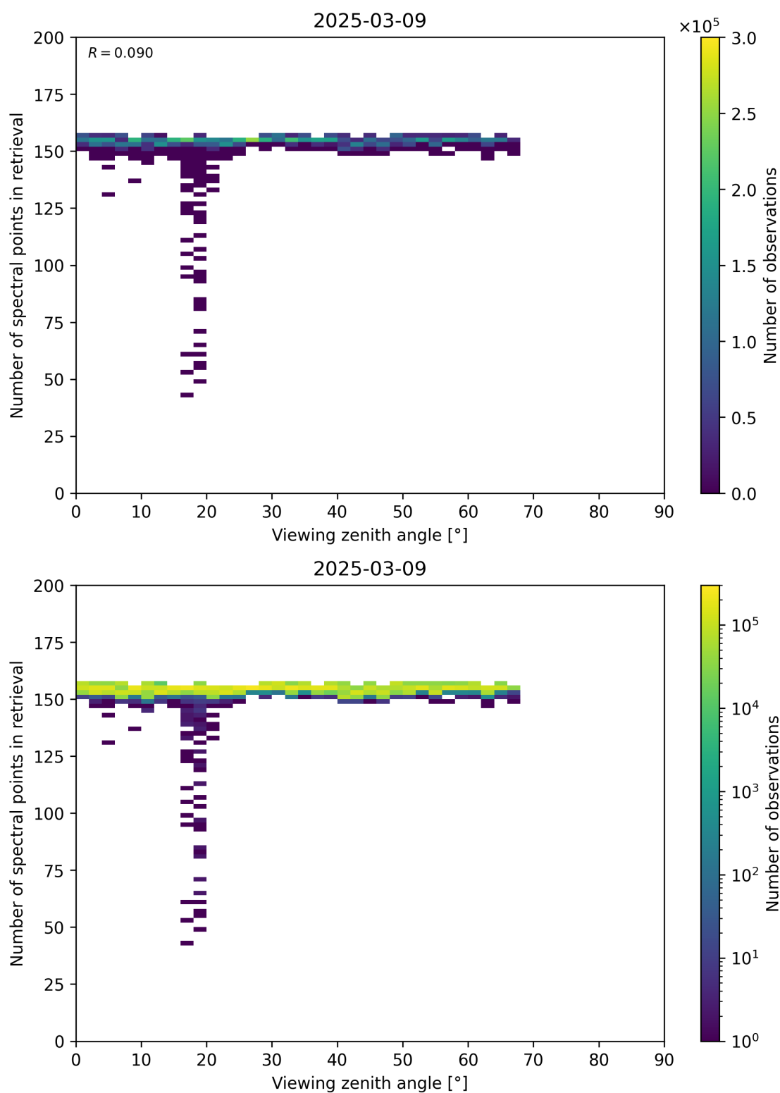
Figure 76: Scatter density plot of “Viewing zenith angle” against “Number of spectral points in retrieval” for 2025-03-08 to 2025-03-10.
