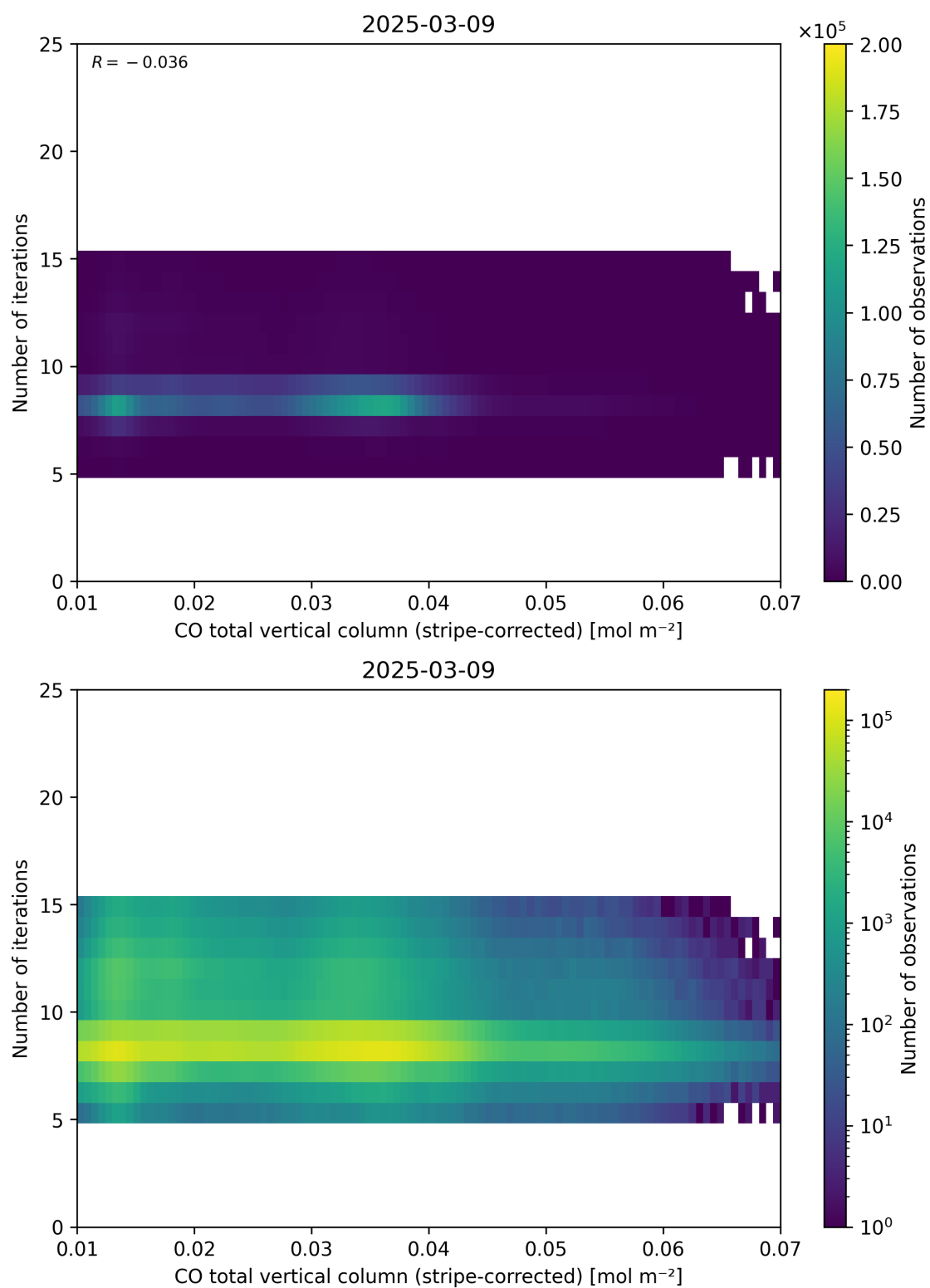
Figure 39: Scatter density plot of “CO total vertical column (stripe-corrected)” against “Number of iterations” for 2025-03-08 to 2025-03-10.
