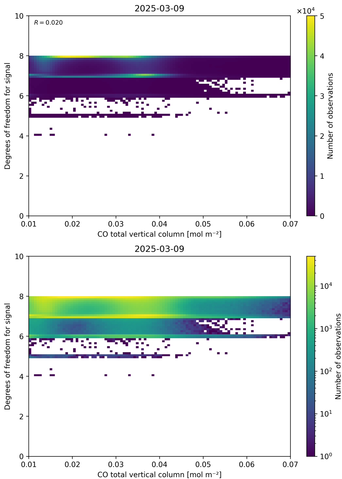
Figure 41: Scatter density plot of “CO total vertical column” against “Degrees of freedom for signal” for 2025-03-08 to 2025-03-10.
