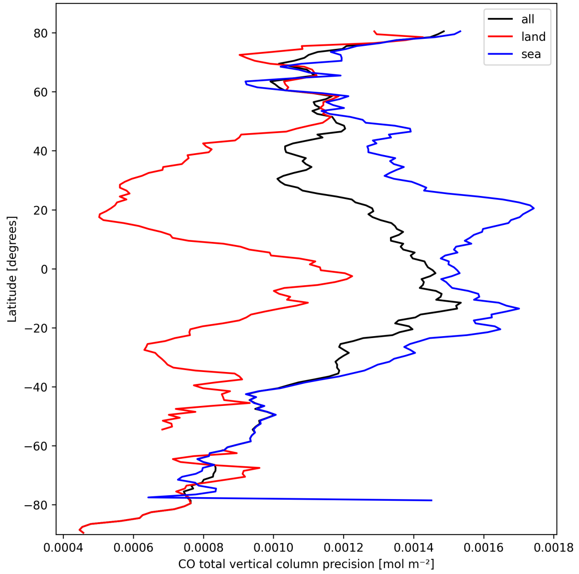
Figure 12: Zonal average of “CO total vertical column precision” for 2025-03-08 to 2025-03-10.
