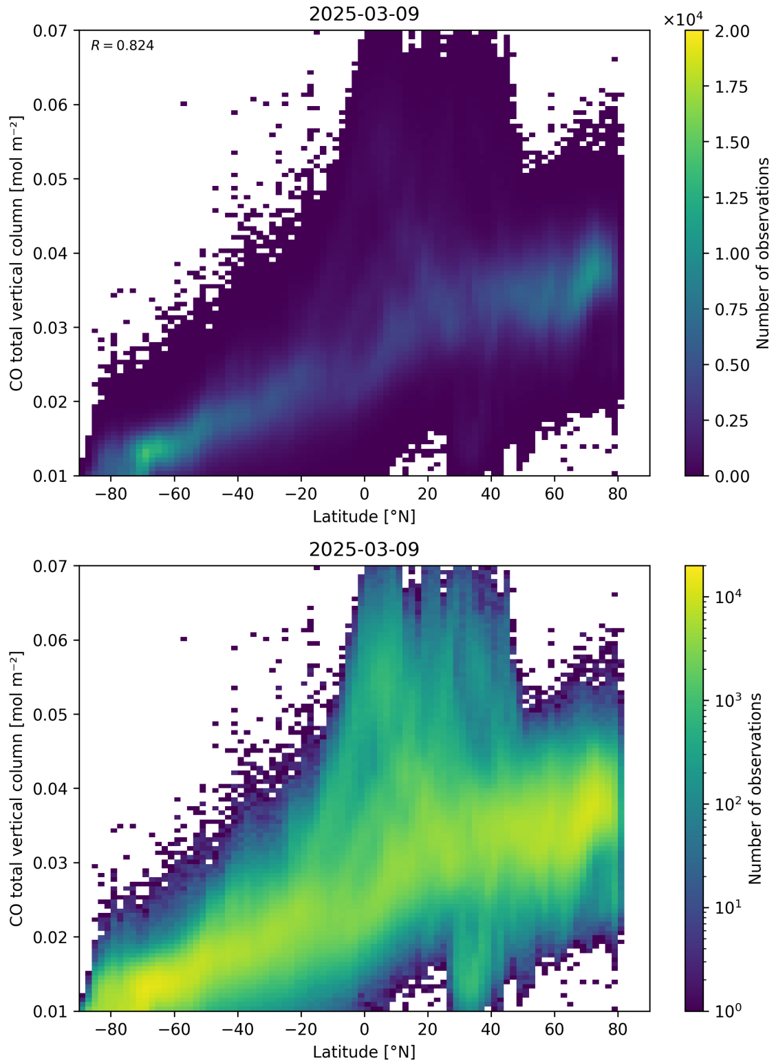
Figure 51: Scatter density plot of “Latitude” against “CO total vertical column” for 2025-03-08 to 2025-03-10.
