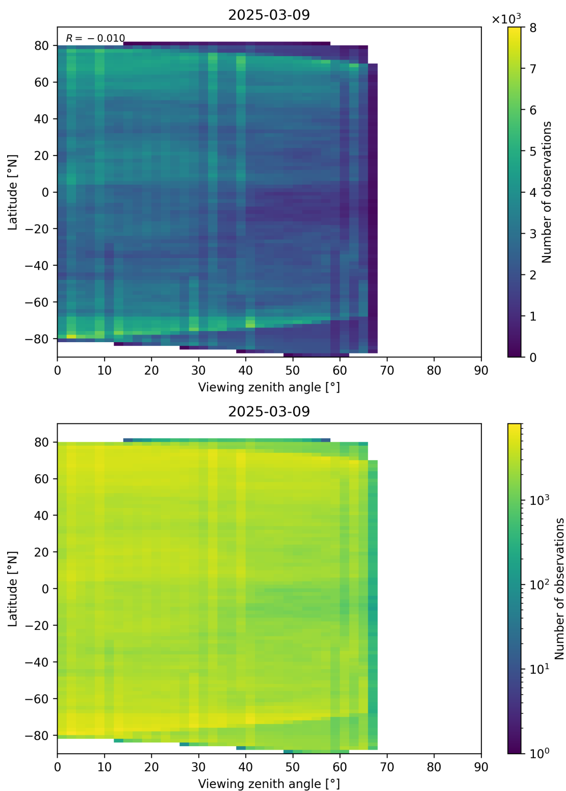
Figure 74: Scatter density plot of “Viewing zenith angle” against “Latitude” for 2025-03-08 to 2025-03-10.
