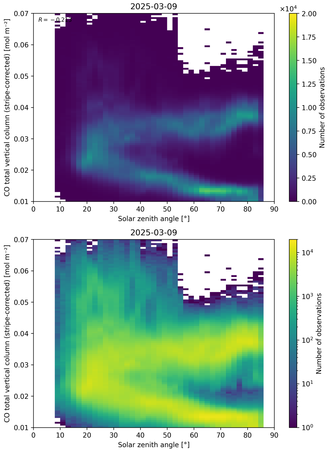
Figure 62: Scatter density plot of “Solar zenith angle” against “CO total vertical column (stripe-corrected)” for 2025-03-08 to 2025-03-10.
