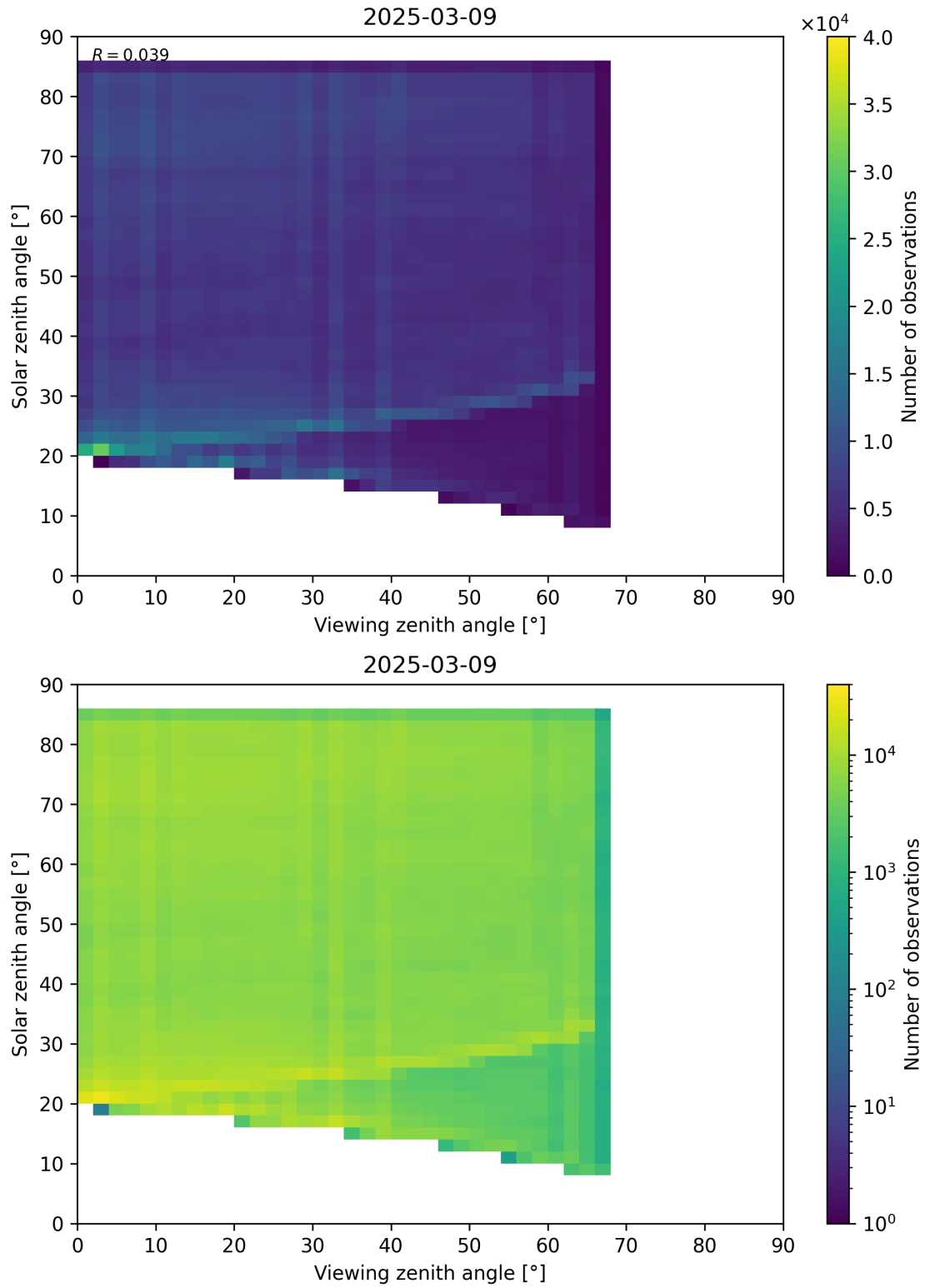
Figure 77: Scatter density plot of “Viewing zenith angle” against “Solar zenith angle” for 2025-03-08 to 2025-03-10.
