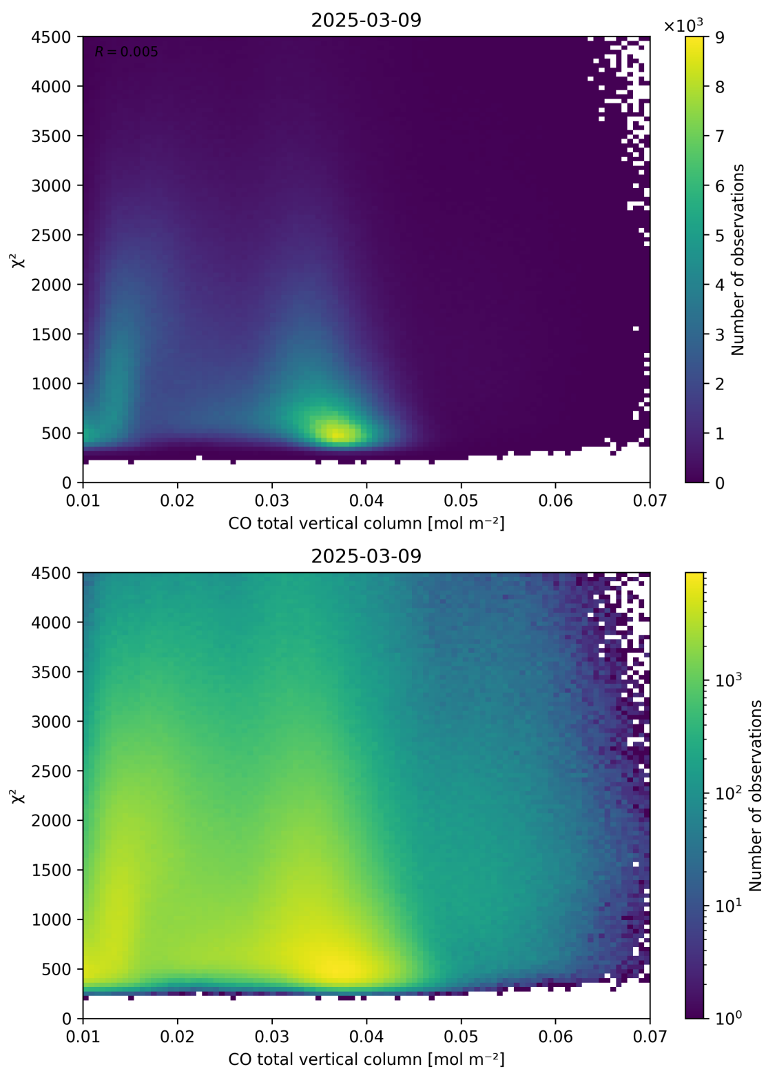
Figure 35: Scatter density plot of “CO total vertical column” against “ \chi^2 ” for 2025-03-08 to 2025-03-10.
