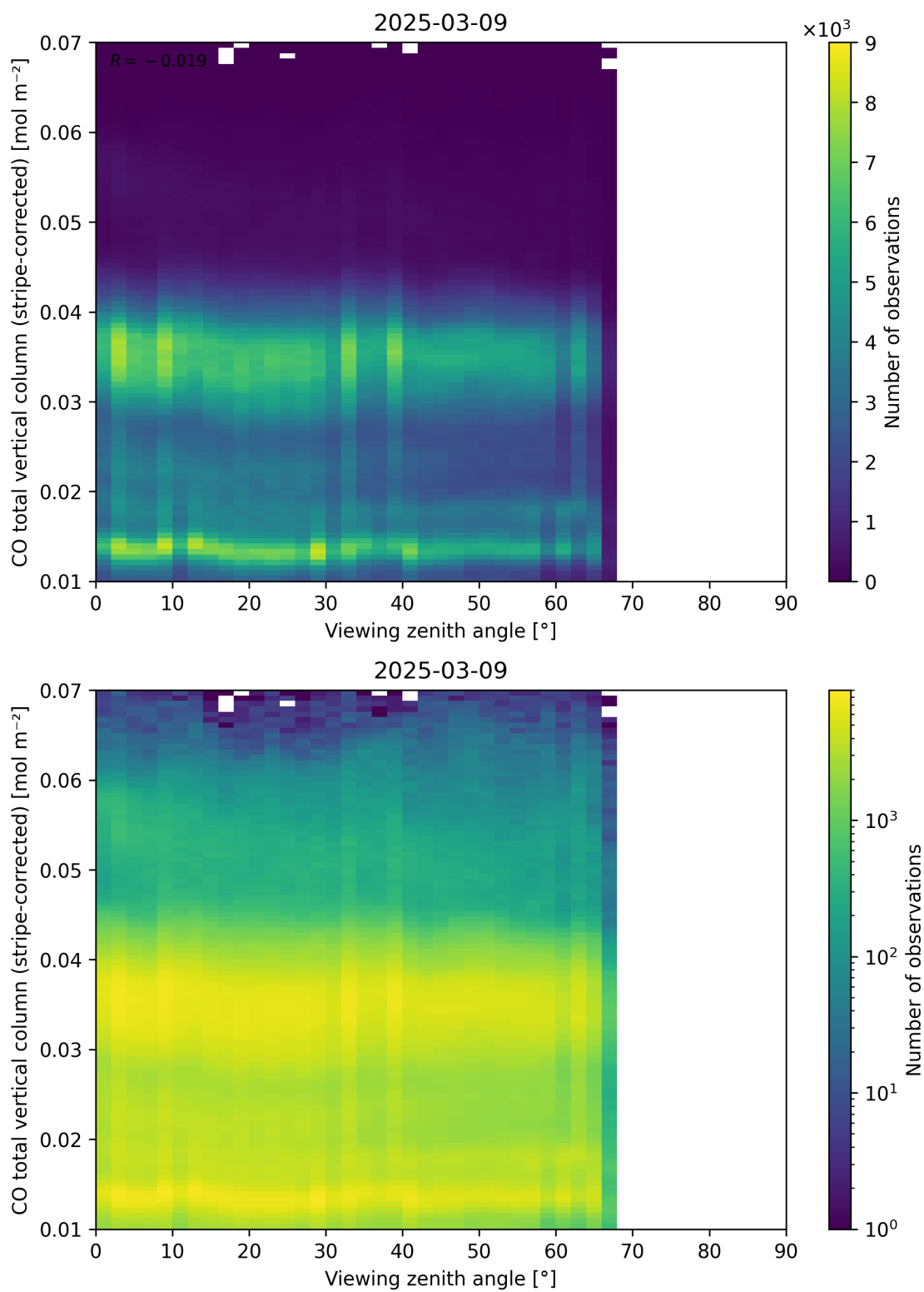
Figure 70: Scatter density plot of “Viewing zenith angle” against “CO total vertical column (stripe-corrected)” for 2025-03-08 to 2025-03-10.
