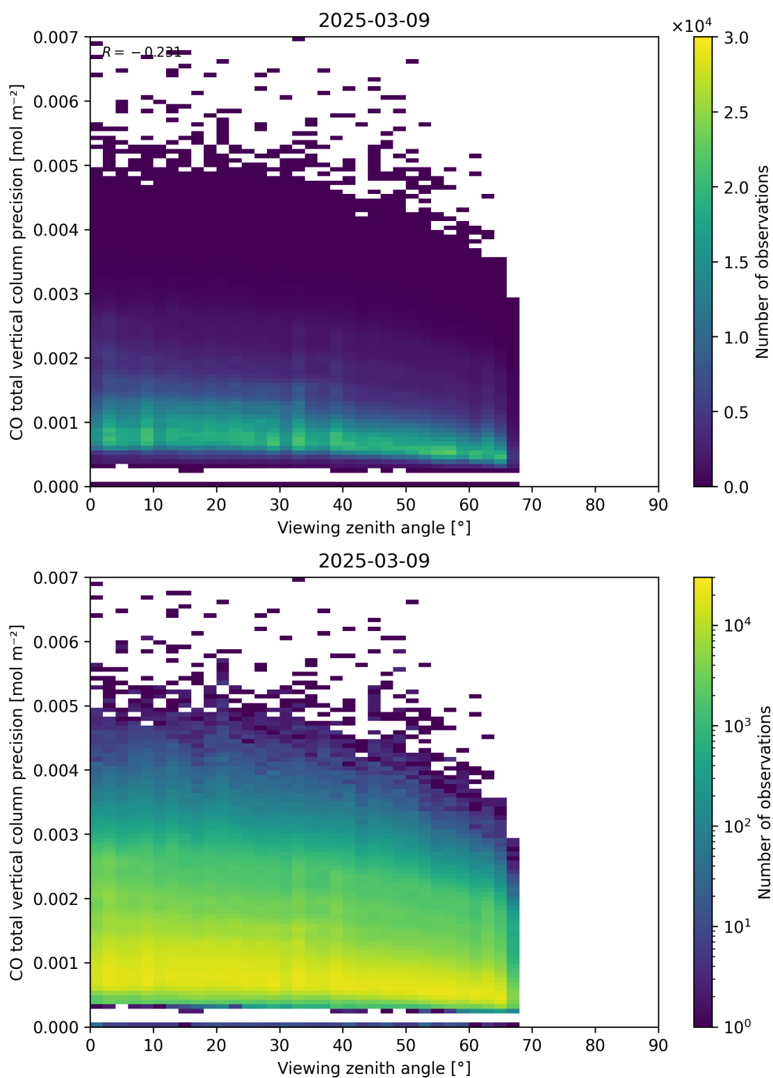
Figure 71: Scatter density plot of “Viewing zenith angle” against “CO total vertical column precision” for 2025-03-08 to 2025-03-10.
