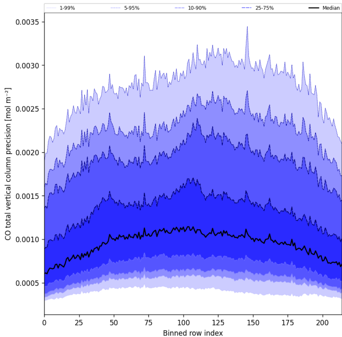
Figure 28: Along track statistics of “CO total vertical column precision” for 2025-03-08 to 2025-03-10
