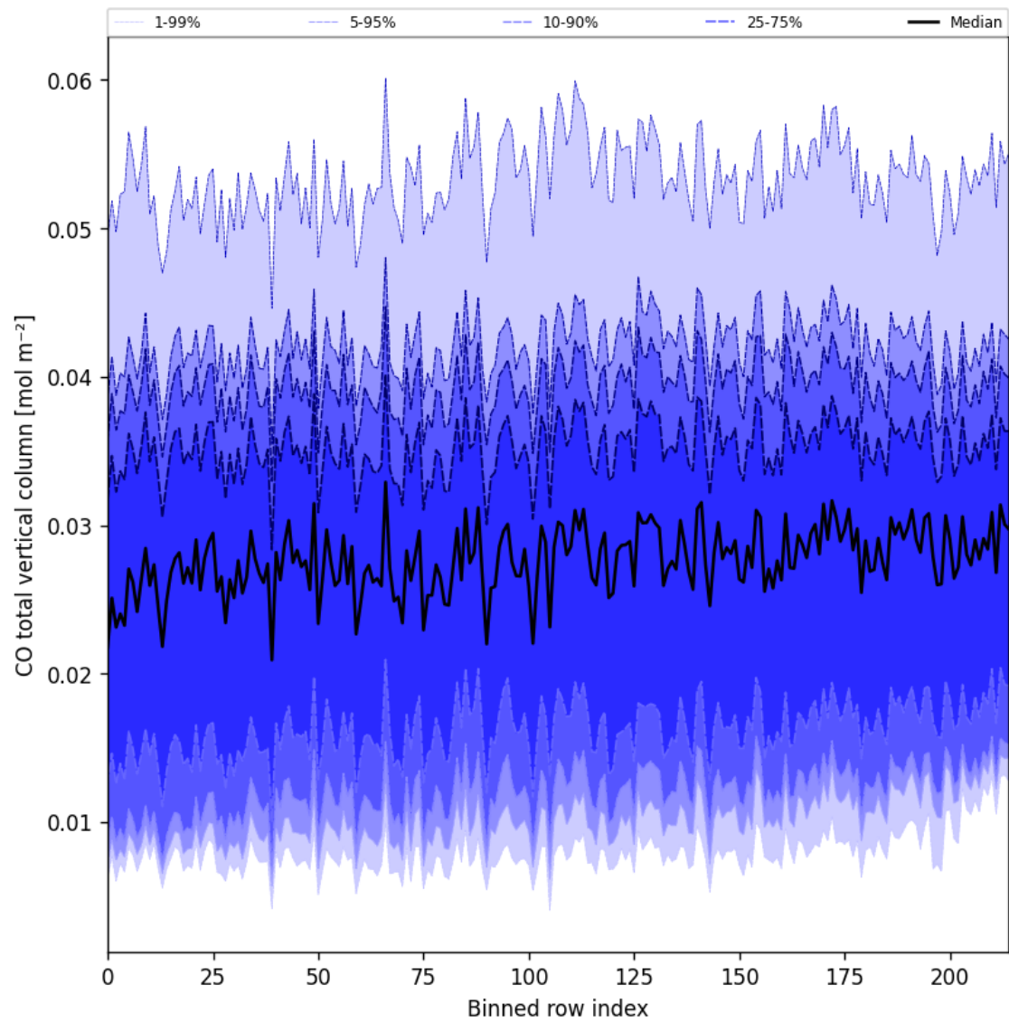
Figure 26: Along track statistics of “CO total vertical column” for 2025-03-08 to 2025-03-10
