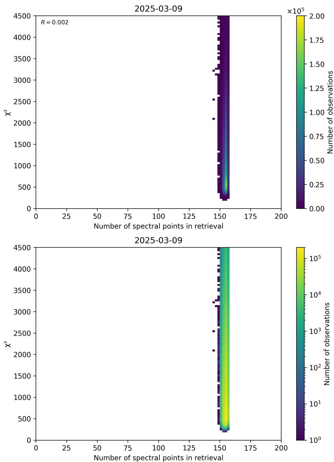
Figure 58: Scatter density plot of “Number of spectral points in retrieval” against “ \chi^2 ” for 2025-03-08 to 2025-03-10.
