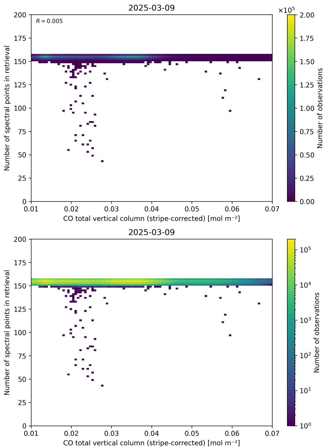
Figure 40: Scatter density plot of “CO total vertical column (stripe-corrected)” against “Number of spectral points in retrieval” for 2025-03-08 to 2025-03-10.
