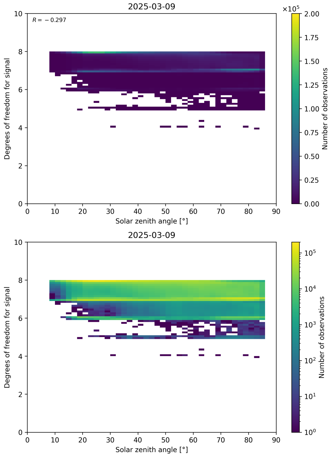
Figure 65: Scatter density plot of “Solar zenith angle” against “Degrees of freedom for signal” for 2025-03-08 to 2025-03-10.
