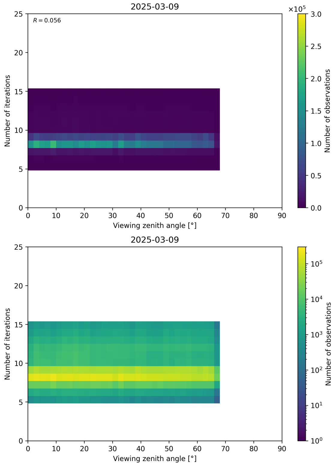
Figure 75: Scatter density plot of “Viewing zenith angle” against “Number of iterations” for 2025-03-08 to 2025-03-10.
