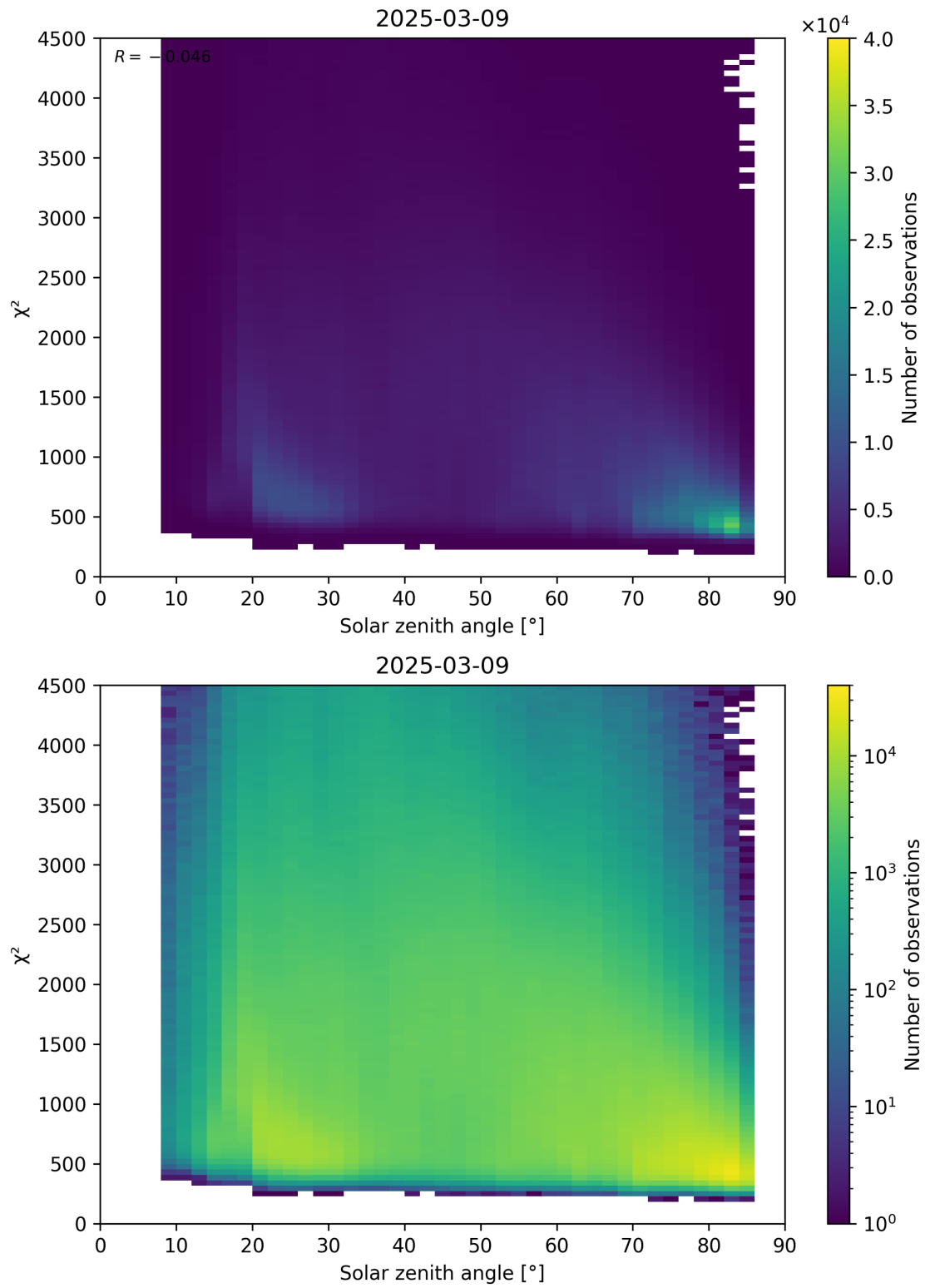
Figure 64: Scatter density plot of “Solar zenith angle” against “ \chi^2 ” for 2025-03-08 to 2025-03-10.
