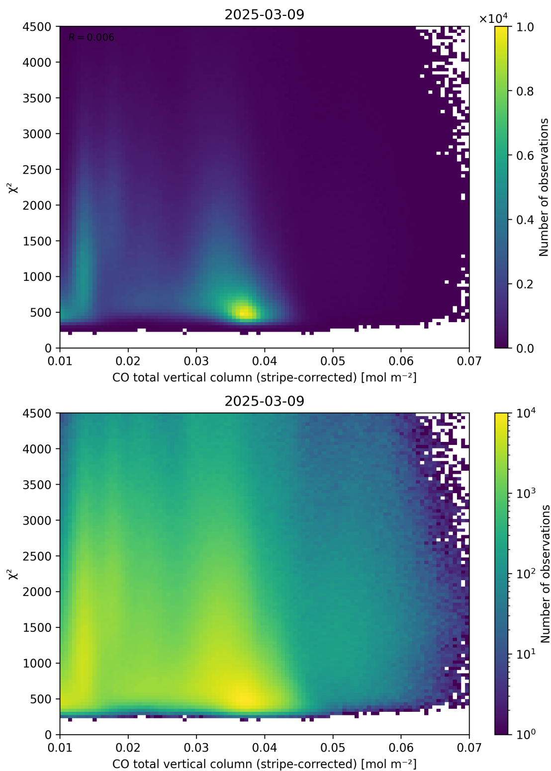
Figure 37: Scatter density plot of “CO total vertical column (stripe-corrected)” against “ \chi^2 ” for 2025-03-08 to 2025-03-10.
