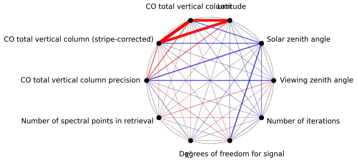
Figure 1: Map of correlation graph for 2025-03-08 to 2025-03-10.
