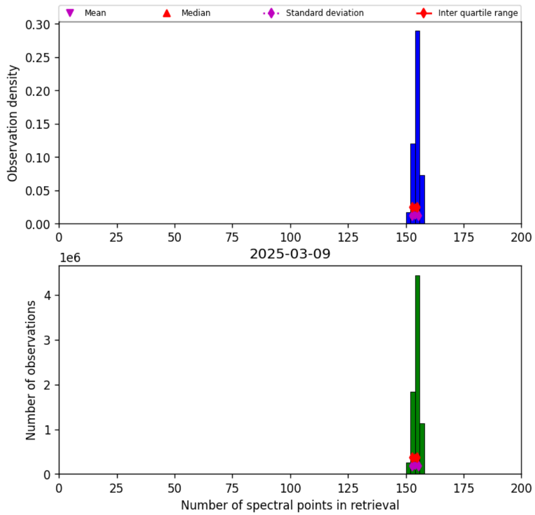
Figure 21: Histogram of “Number of spectral points in retrieval” for 2025-03-08 to 2025-03-10
