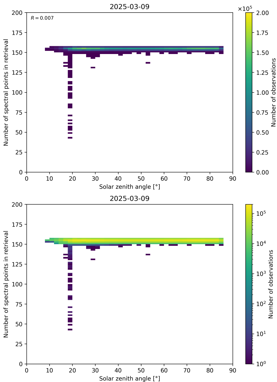
Figure 68: Scatter density plot of “Solar zenith angle” against “Number of spectral points in retrieval” for 2025-03-08 to 2025-03-10.
