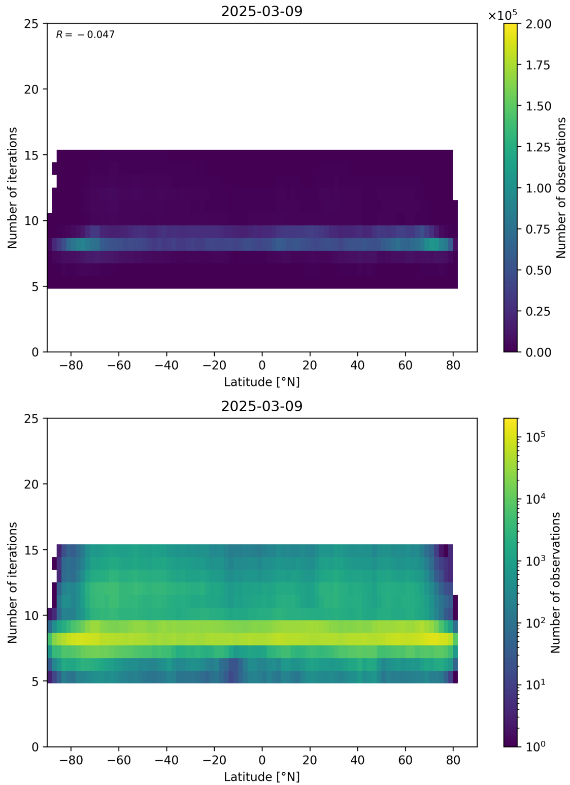
Figure 56: Scatter density plot of “Latitude” against “Number of iterations” for 2025-03-08 to 2025-03-10.
