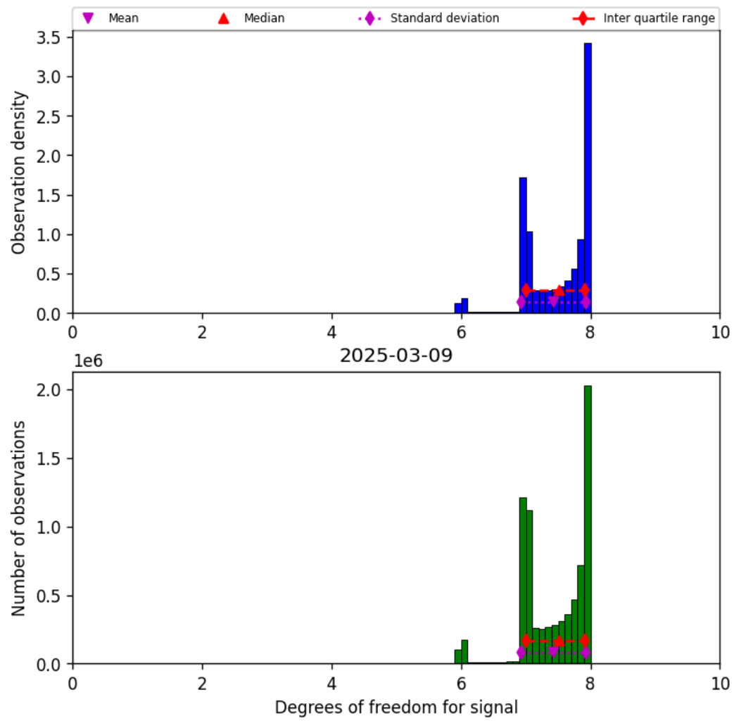
Figure 23: Histogram of “Degrees of freedom for signal” for 2025-03-08 to 2025-03-10
