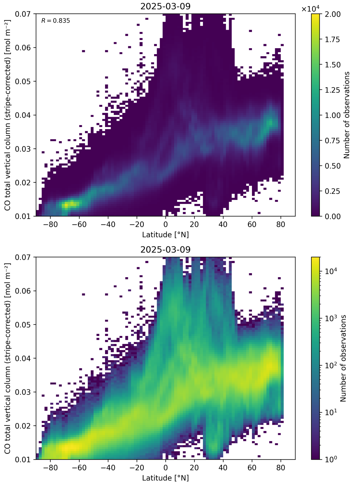
Figure 52: Scatter density plot of “Latitude” against “CO total vertical column (stripe-corrected)” for 2025-03-08 to 2025-03-10.
