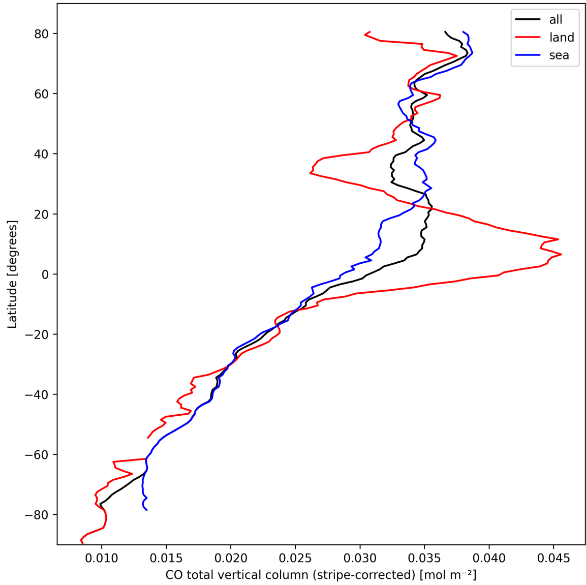
Figure 11: Zonal average of “CO total vertical column (stripe-corrected)” for 2025-03-08 to 2025-03-10.
