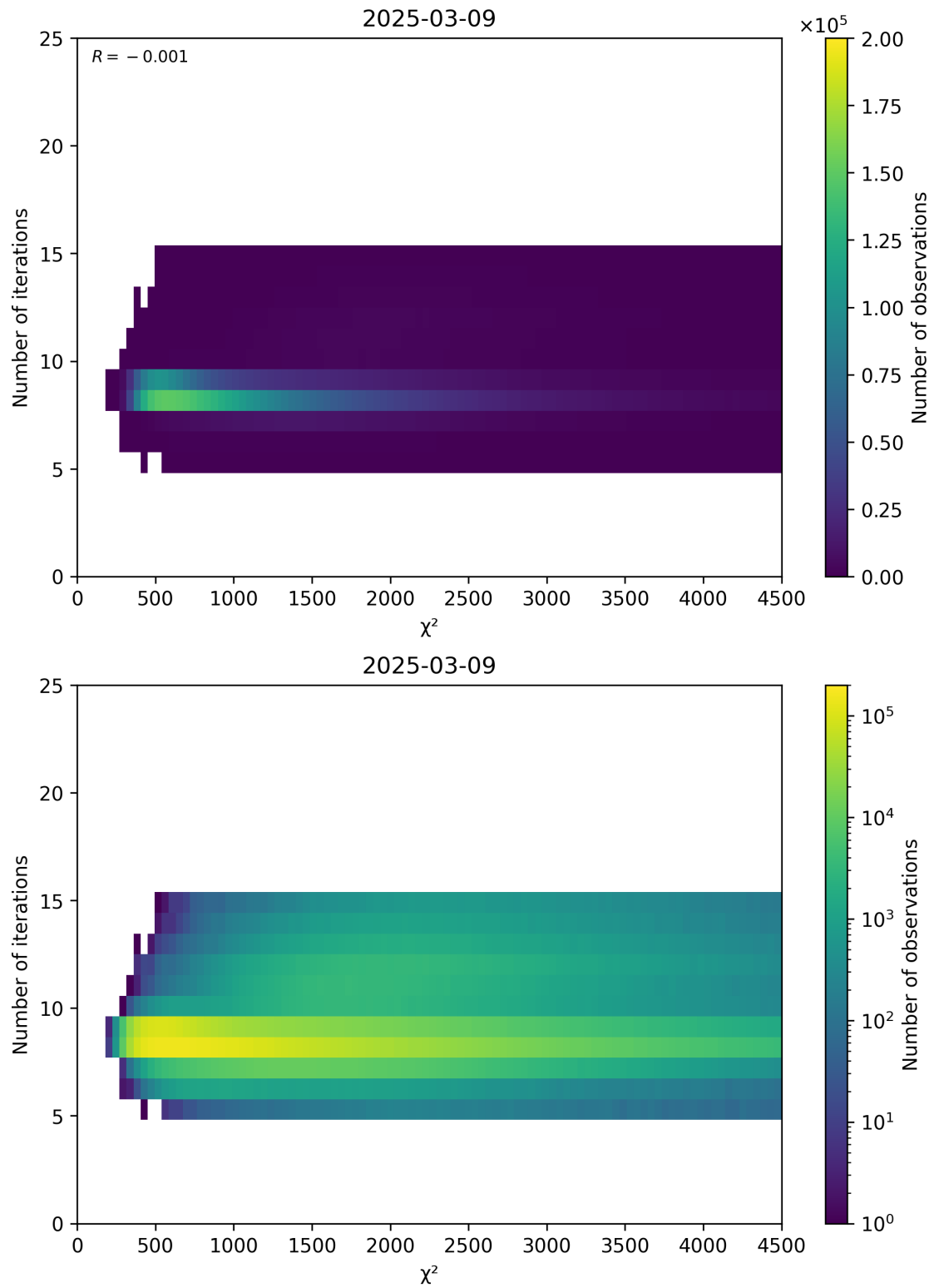
Figure 49: Scatter density plot of “ \chi^2 ” against “Number of iterations” for 2025-03-08 to 2025-03-10.
