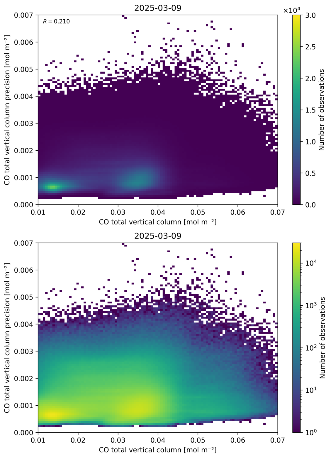
Figure 34: Scatter density plot of “CO total vertical column” against “CO total vertical column precision” for 2025-03-08 to 2025-03-10.
