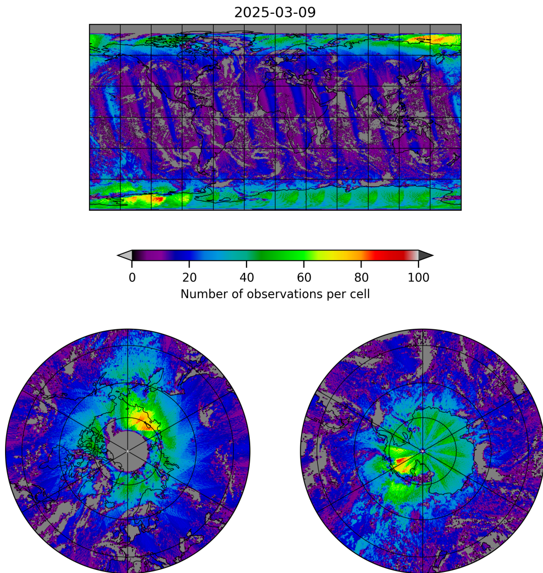
Figure 8: Map of the number of observations for 2025-03-08 to 2025-03-10
