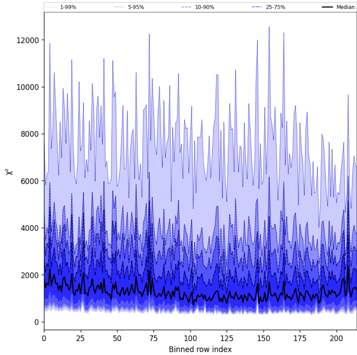
Figure 30: Along track statistics of “ \chi^2 ” for 2025-03-08 to 2025-03-10
