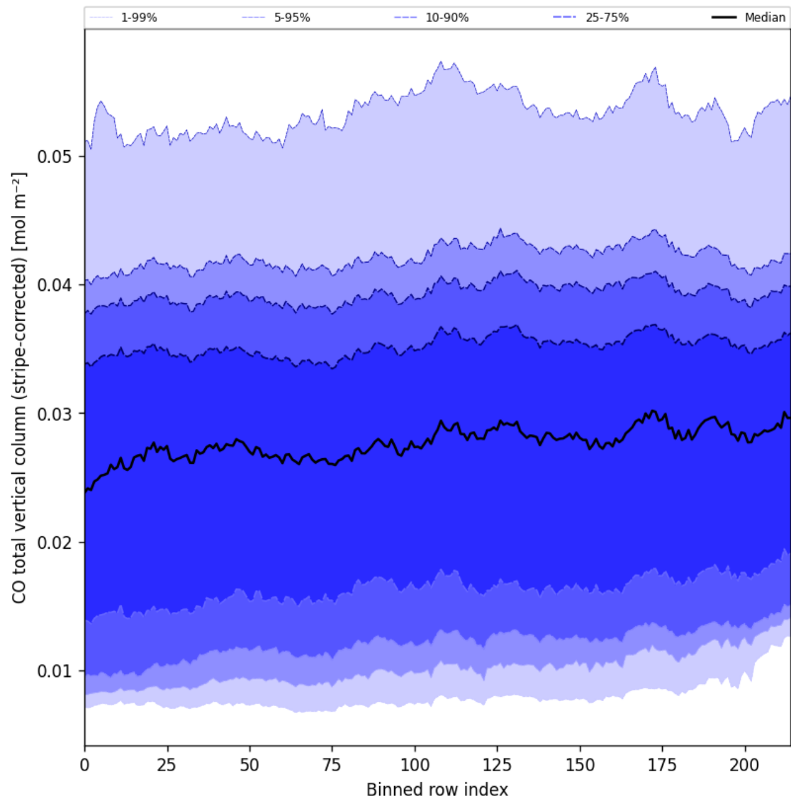
Figure 27: Along track statistics of “CO total vertical column (stripe-corrected)” for 2025-03-08 to 2025-03-10
