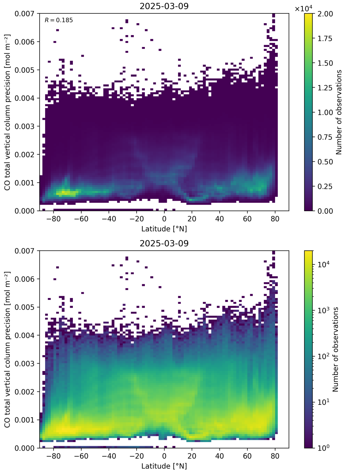
Figure 53: Scatter density plot of “Latitude” against “CO total vertical column precision” for 2025-03-08 to 2025-03-10.
