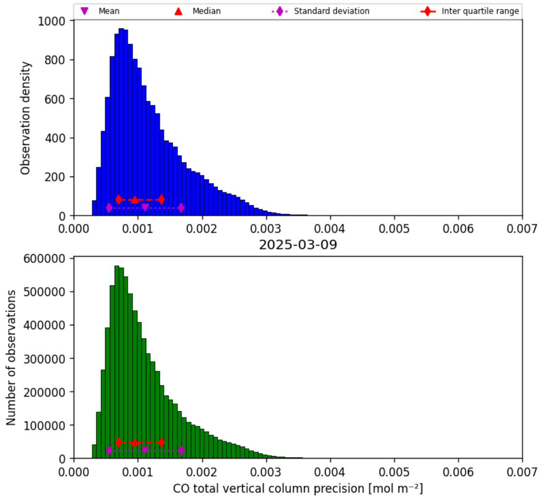
Figure 20: Histogram of “CO total vertical column precision” for 2025-03-08 to 2025-03-10
