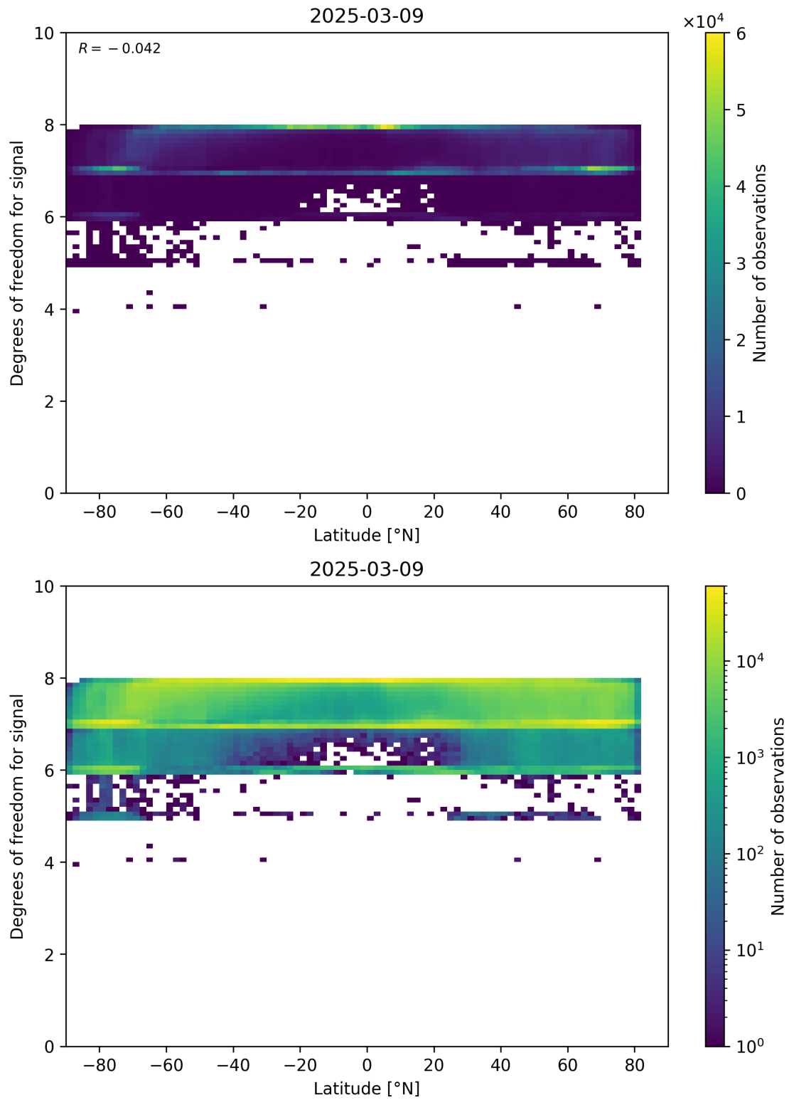
Figure 55: Scatter density plot of “Latitude” against “Degrees of freedom for signal” for 2025-03-08 to 2025-03-10.
