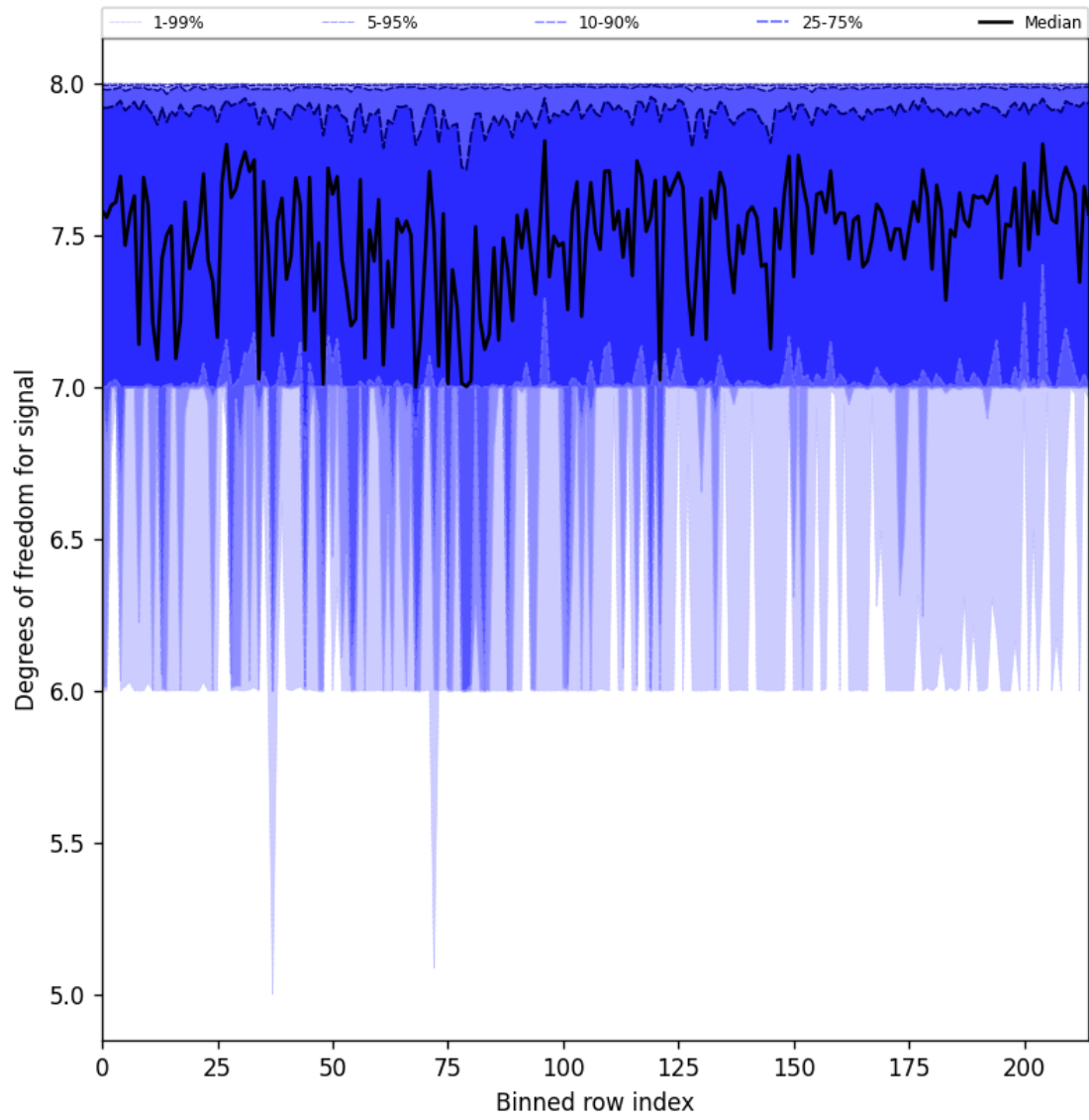
Figure 31: Along track statistics of “Degrees of freedom for signal” for 2025-03-08 to 2025-03-10
