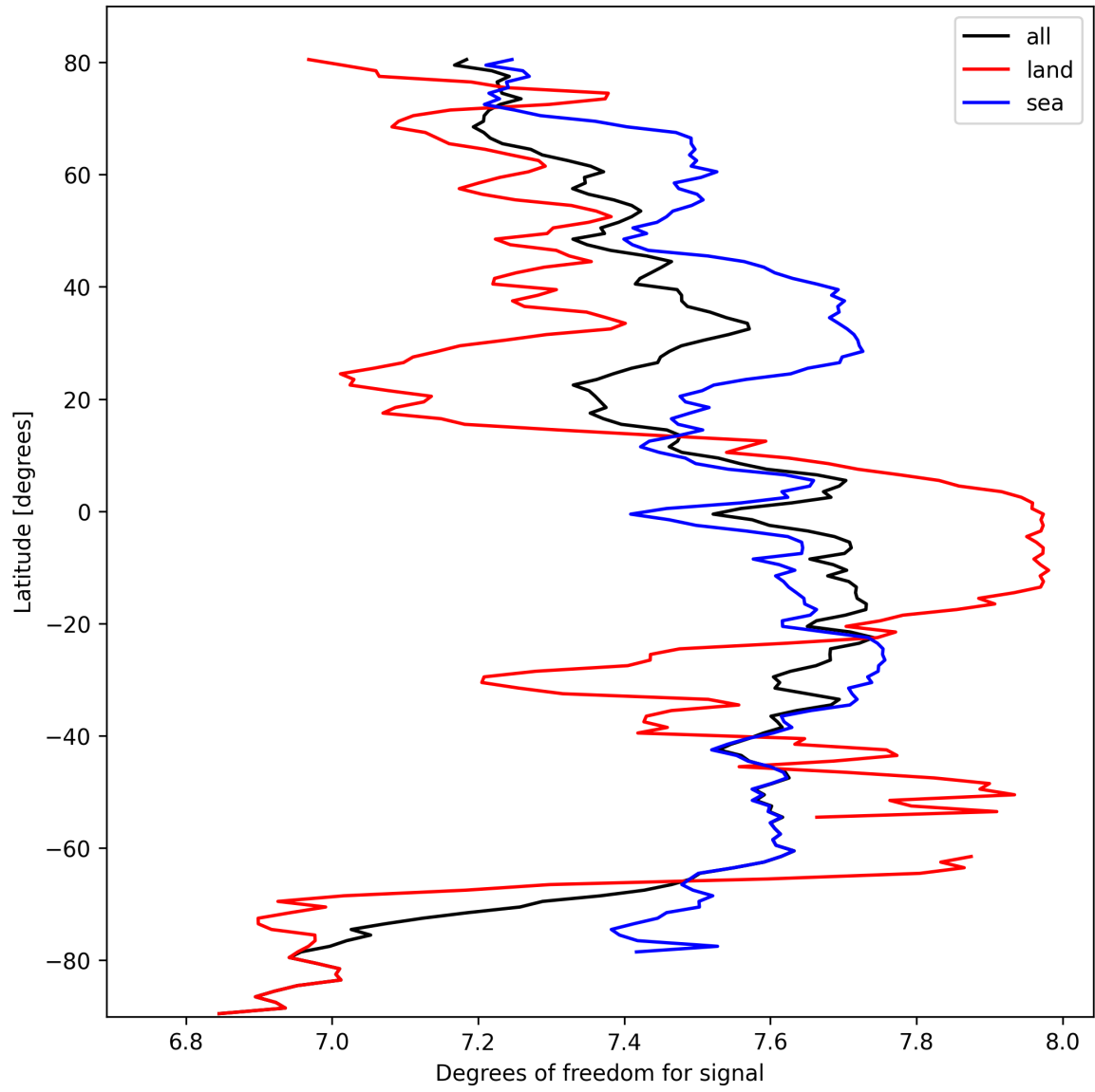
Figure 15: Zonal average of “Degrees of freedom for signal” for 2025-03-08 to 2025-03-10.
