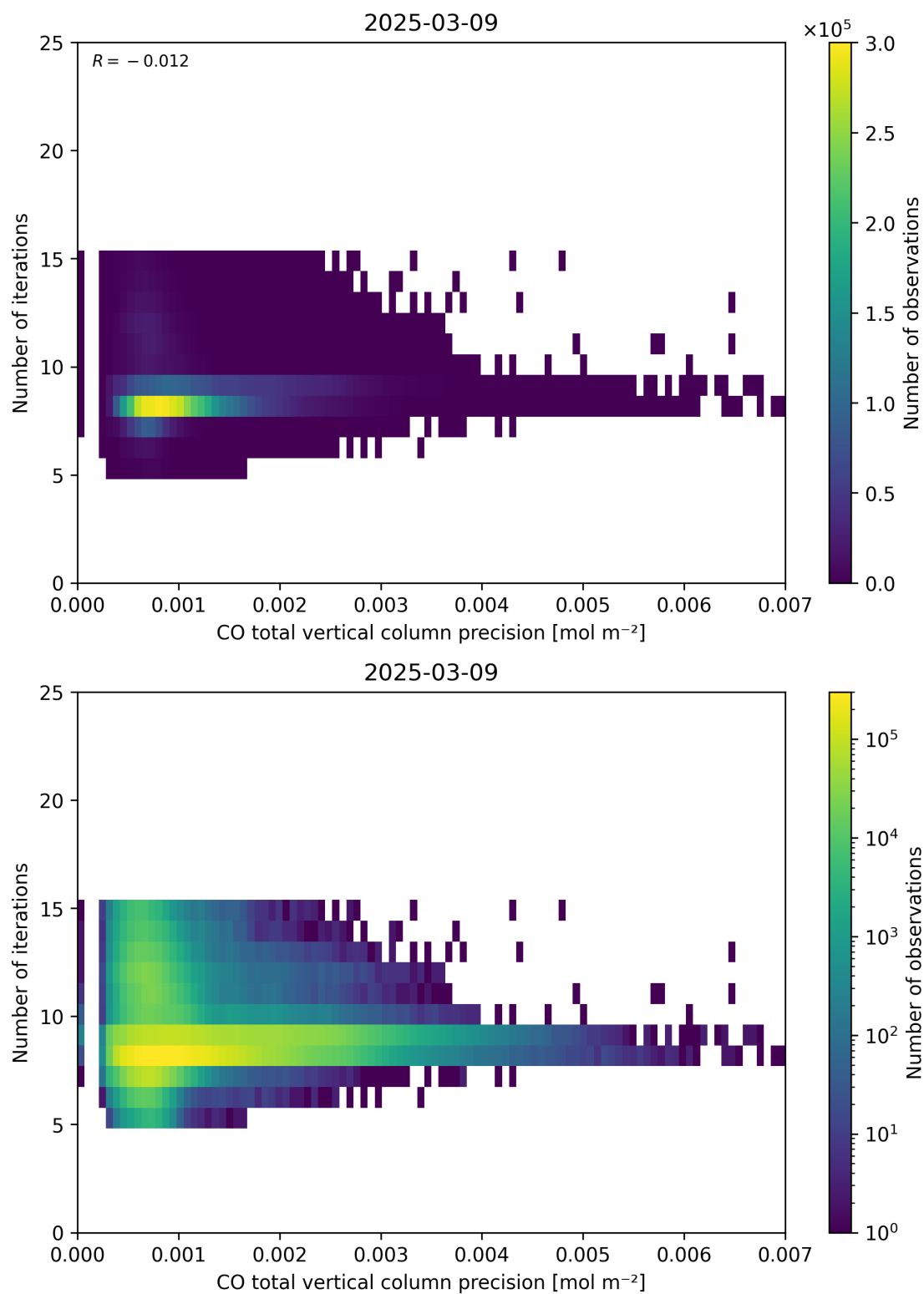
Figure 46: Scatter density plot of “CO total vertical column precision” against “Number of iterations” for 2025-03-08 to 2025-03-10.
