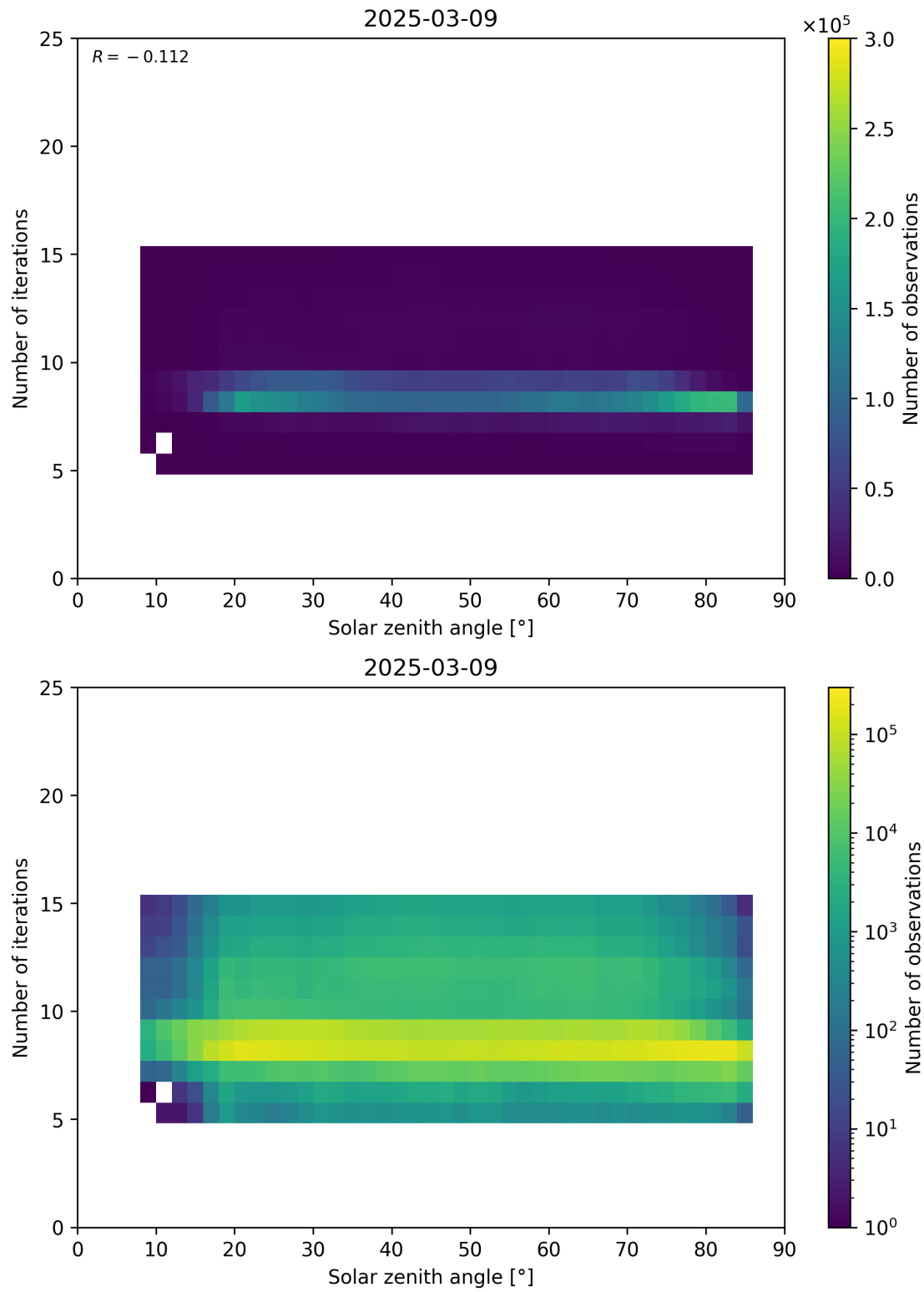
Figure 67: Scatter density plot of “Solar zenith angle” against “Number of iterations” for 2025-03-08 to 2025-03-10.
