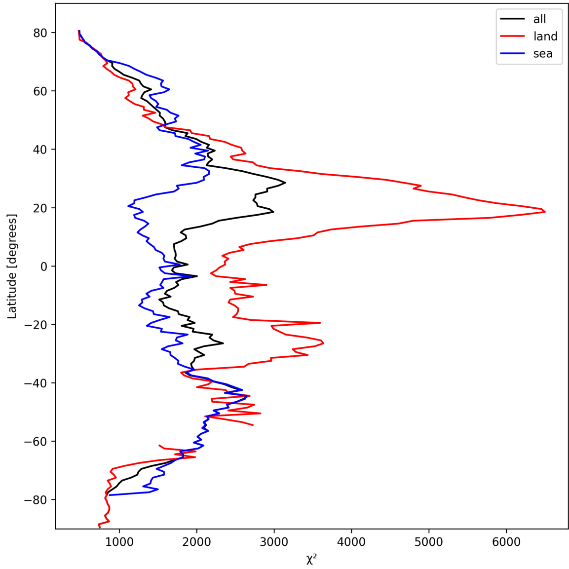
Figure 14: Zonal average of “ \chi^2 ” for 2025-03-08 to 2025-03-10.
