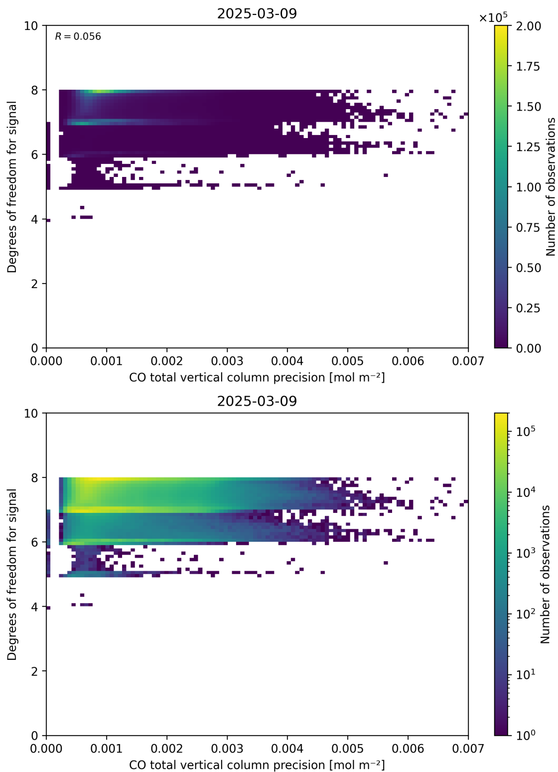
Figure 45: Scatter density plot of “CO total vertical column precision” against “Degrees of freedom for signal” for 2025-03-08 to 2025-03-10.
