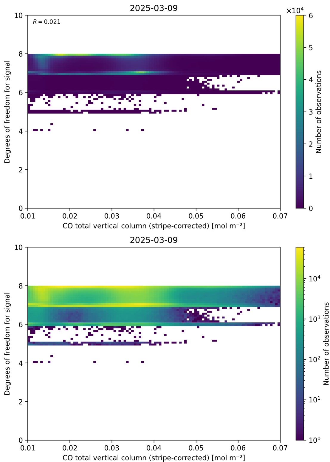
Figure 38: Scatter density plot of “CO total vertical column (stripe-corrected)” against “Degrees of freedom for signal” for 2025-03-08 to 2025-03-10.
