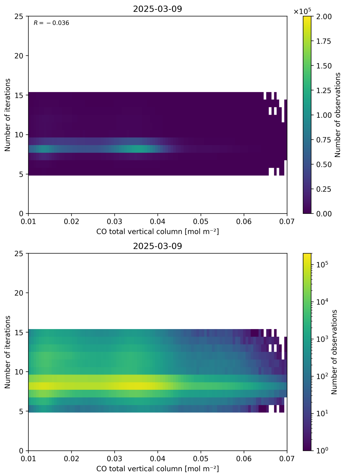
Figure 42: Scatter density plot of “CO total vertical column” against “Number of iterations” for 2025-03-08 to 2025-03-10.
