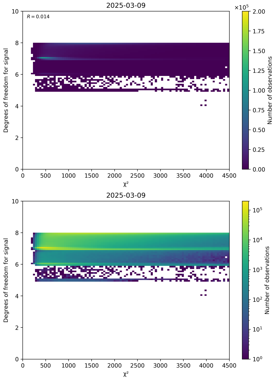
Figure 48: Scatter density plot of “ \chi^2 ” against “Degrees of freedom for signal” for 2025-03-08 to 2025-03-10.
