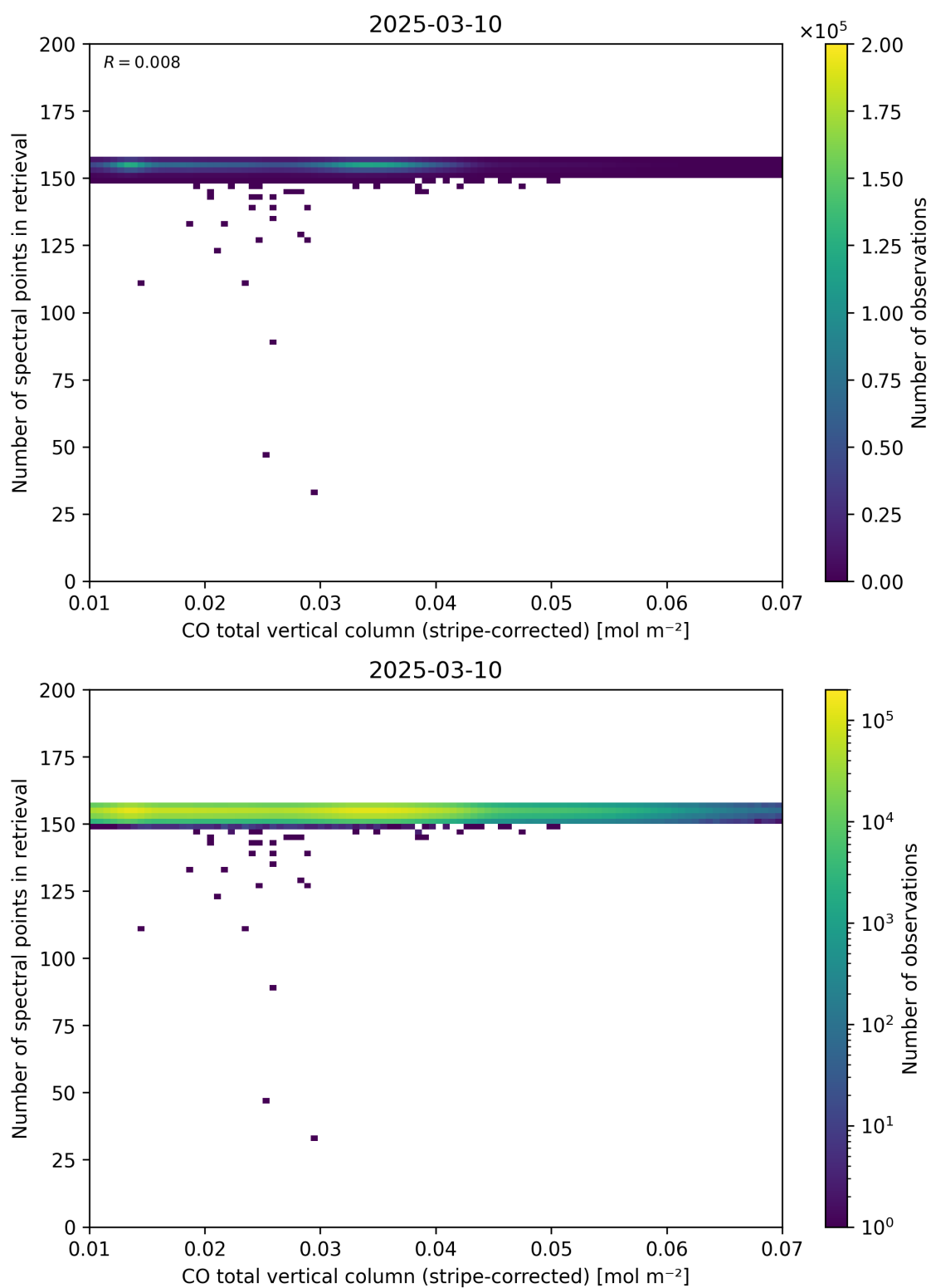
Figure 40: Scatter density plot of “CO total vertical column (stripe-corrected)” against “Number of spectral points in retrieval” for 2025-03-09 to 2025-03-11.
