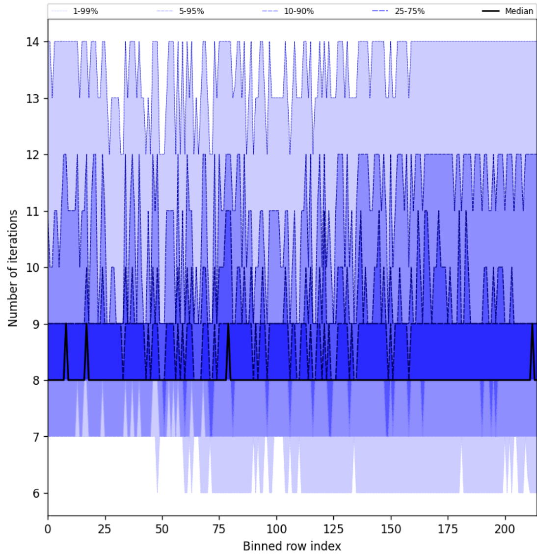
Figure 32: Along track statistics of “Number of iterations” for 2025-03-09 to 2025-03-11
