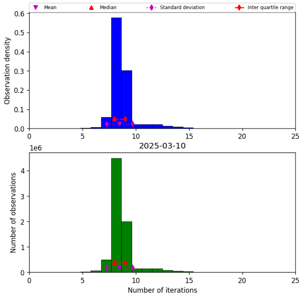
Figure 24: Histogram of “Number of iterations” for 2025-03-09 to 2025-03-11
