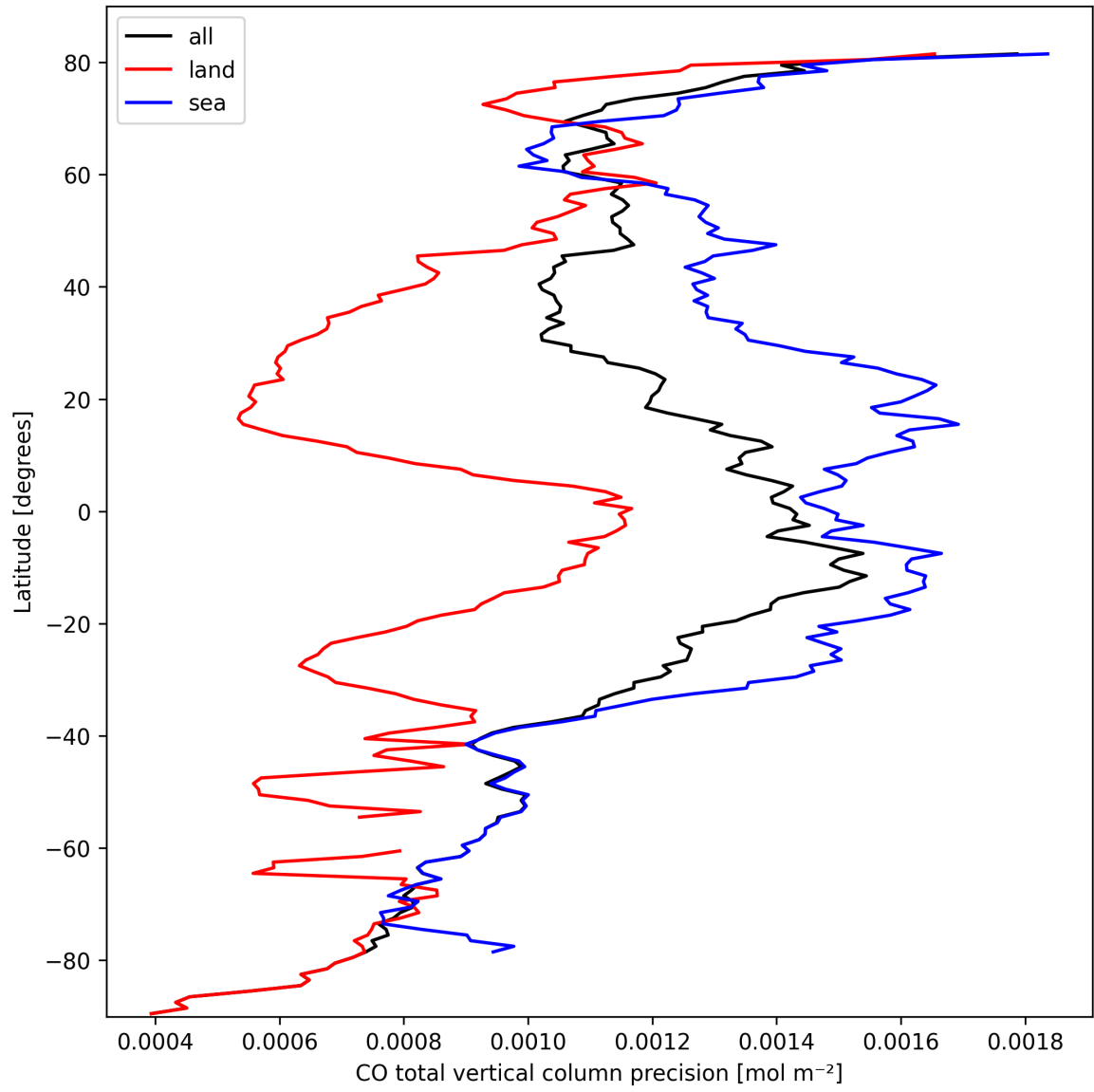
Figure 12: Zonal average of “CO total vertical column precision” for 2025-03-09 to 2025-03-11.
