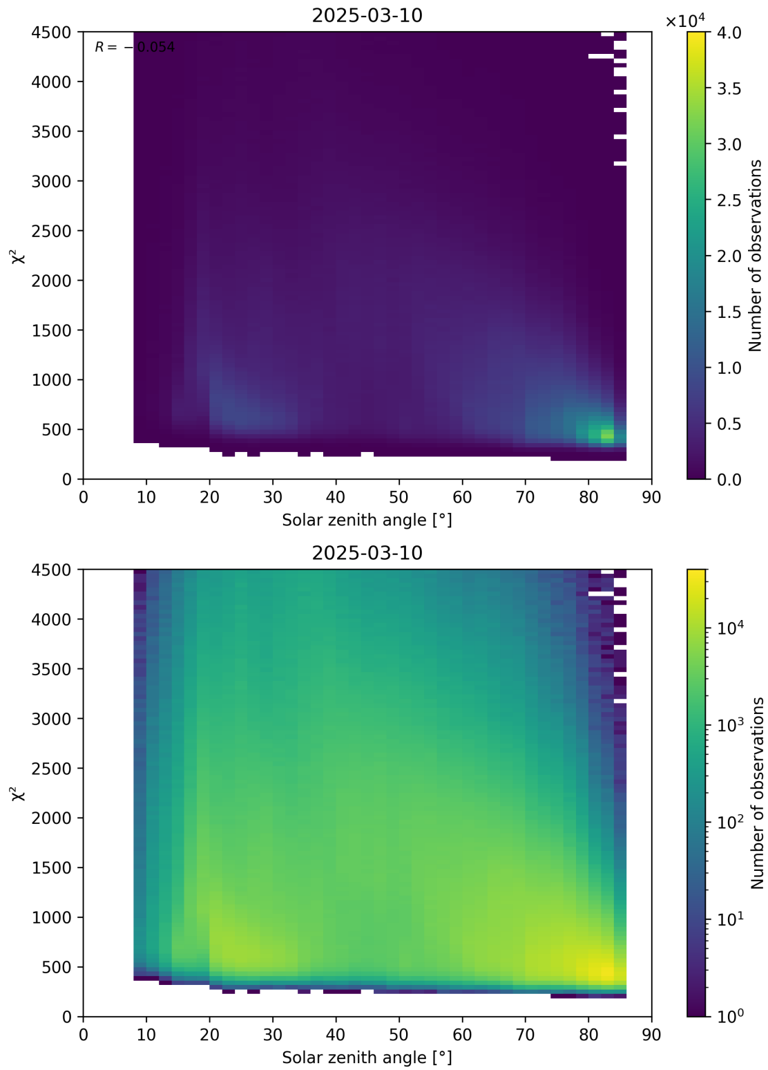
Figure 64: Scatter density plot of “Solar zenith angle” against “ \chi^2 ” for 2025-03-09 to 2025-03-11.
