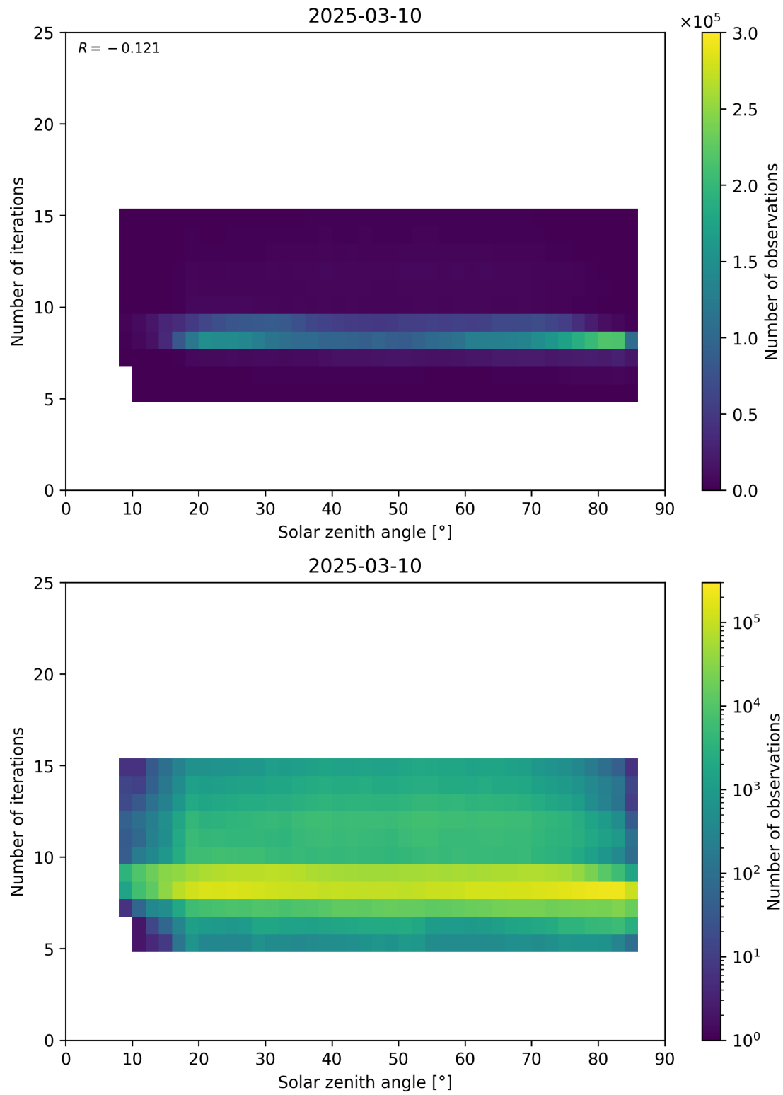
Figure 67: Scatter density plot of “Solar zenith angle” against “Number of iterations” for 2025-03-09 to 2025-03-11.
