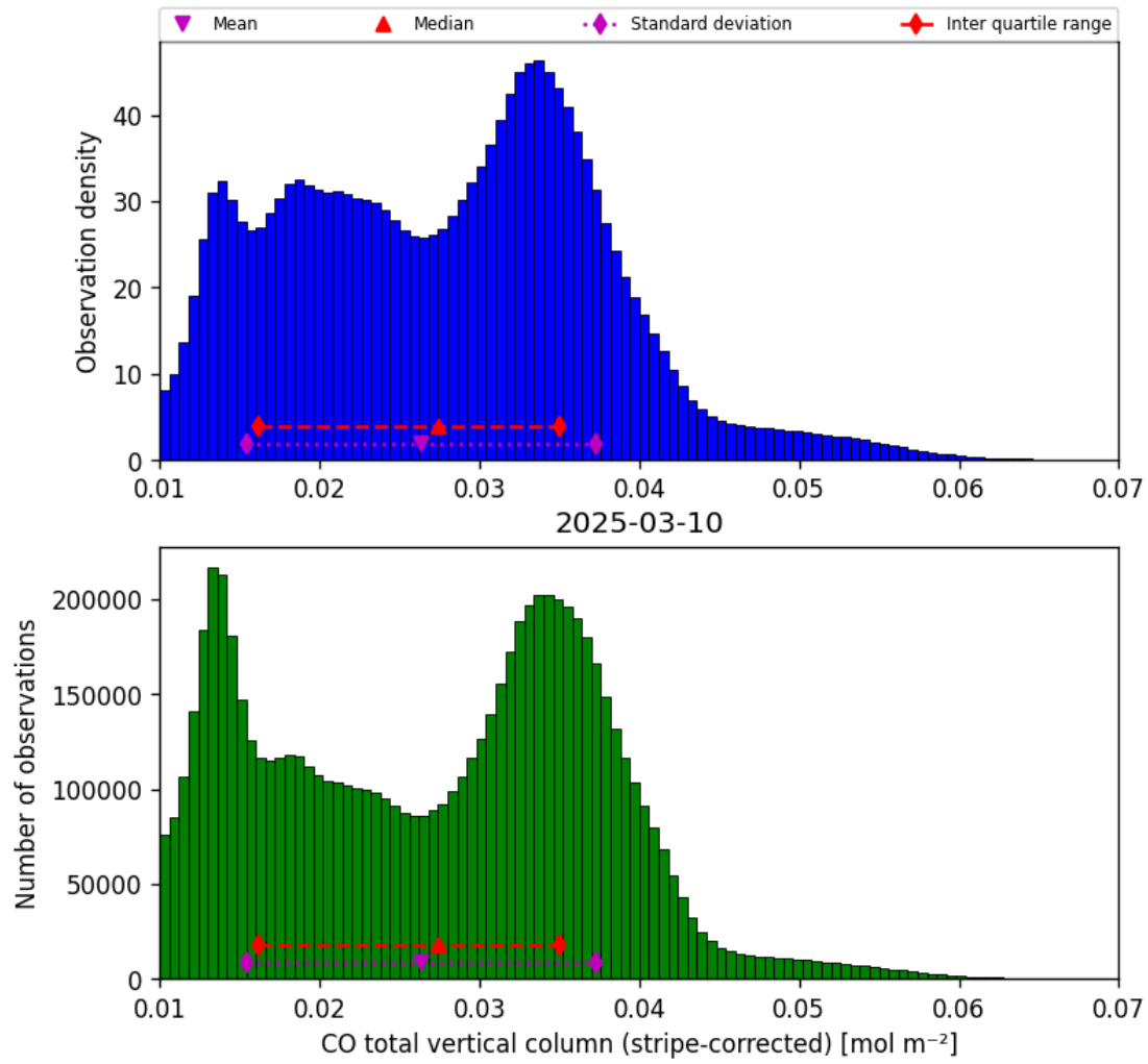
Figure 19: Histogram of “CO total vertical column (stripe-corrected)” for 2025-03-09 to 2025-03-11
