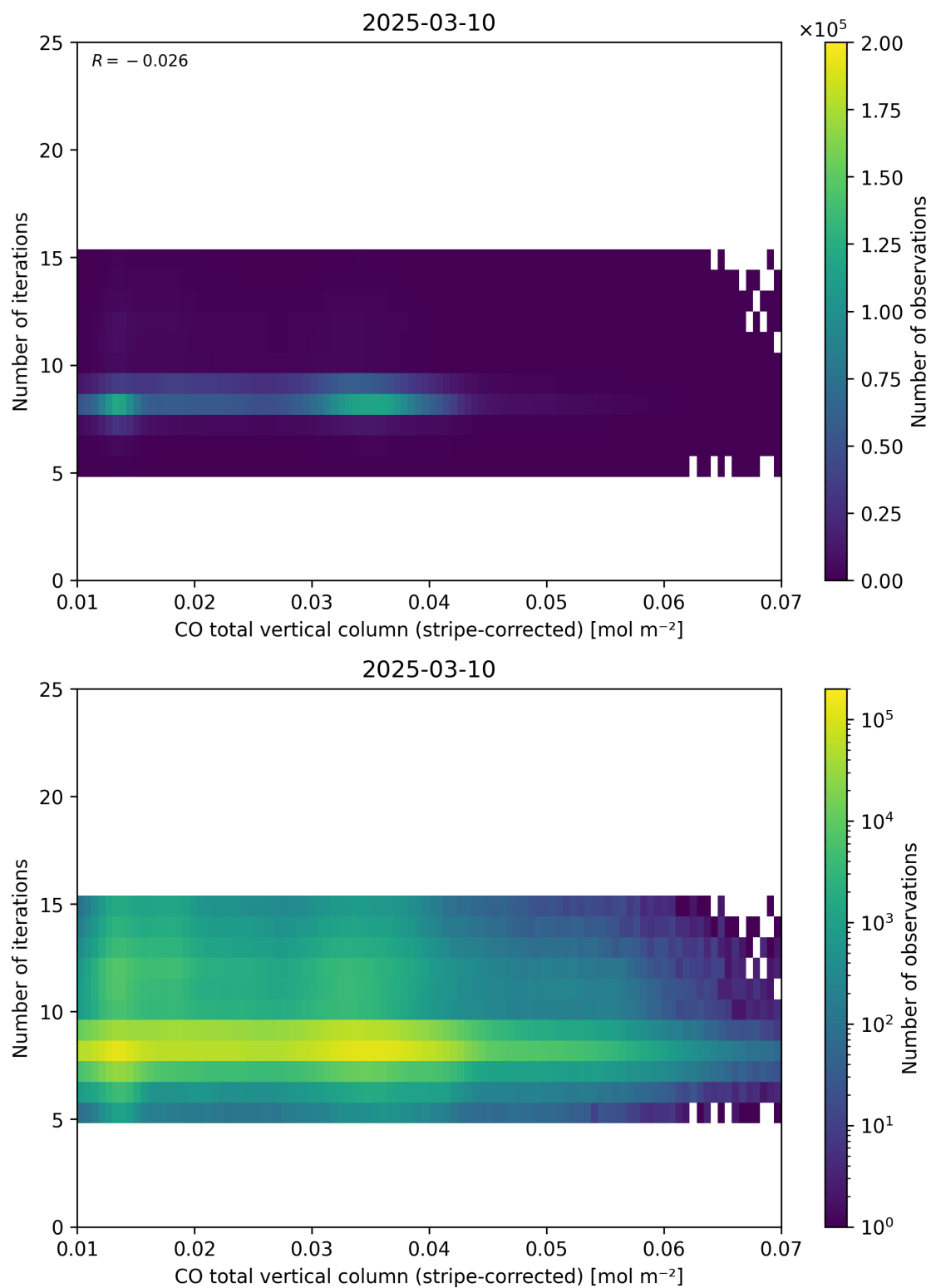
Figure 39: Scatter density plot of “CO total vertical column (stripe-corrected)” against “Number of iterations” for 2025-03-09 to 2025-03-11.
