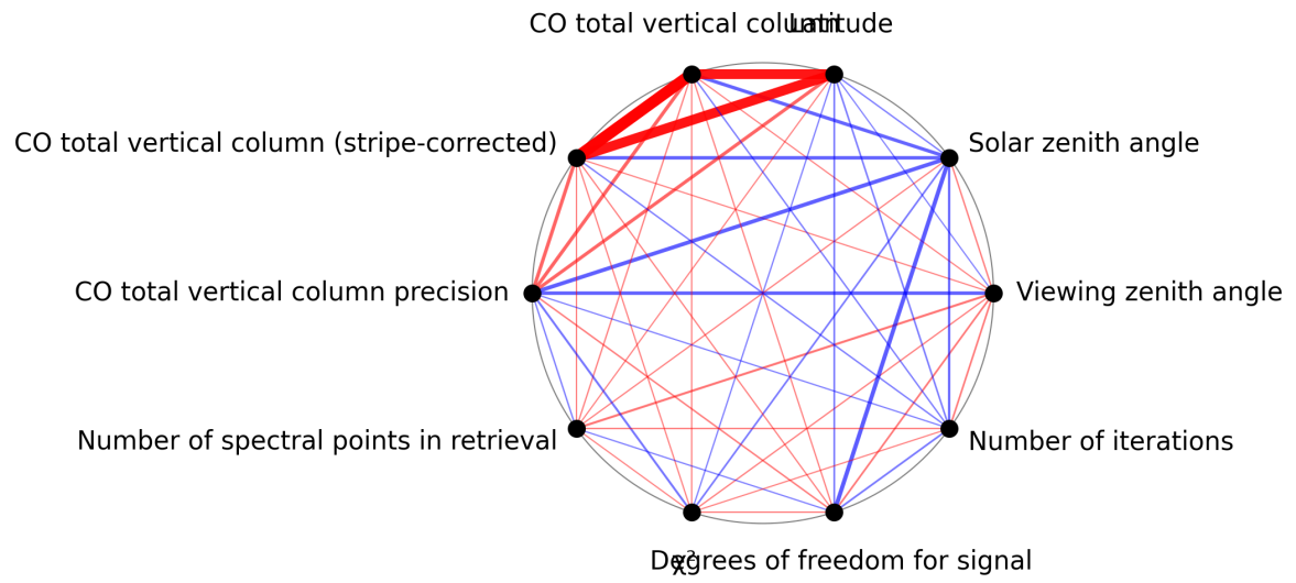
Figure 1: Map of correlation graph for 2025-03-09 to 2025-03-11.
