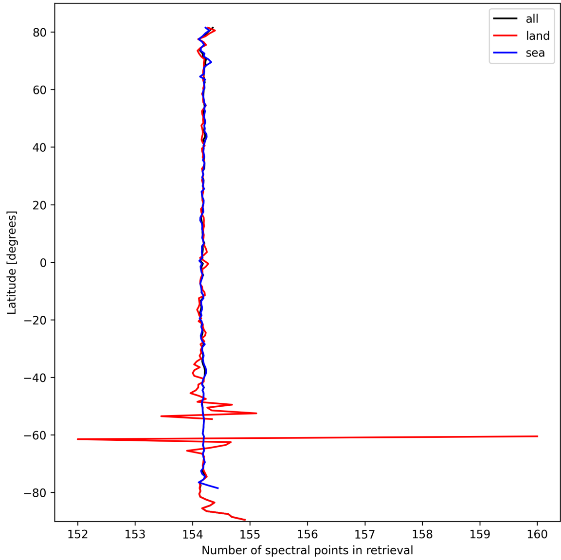
Figure 13: Zonal average of “Number of spectral points in retrieval” for 2025-03-09 to 2025-03-11.
