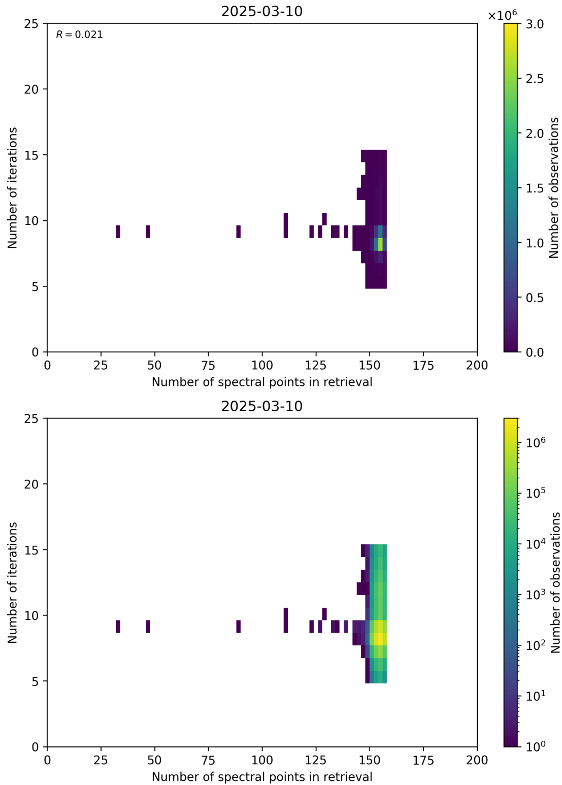
Figure 60: Scatter density plot of “Number of spectral points in retrieval” against “Number of iterations” for 2025-03-09 to 2025-03-11.
