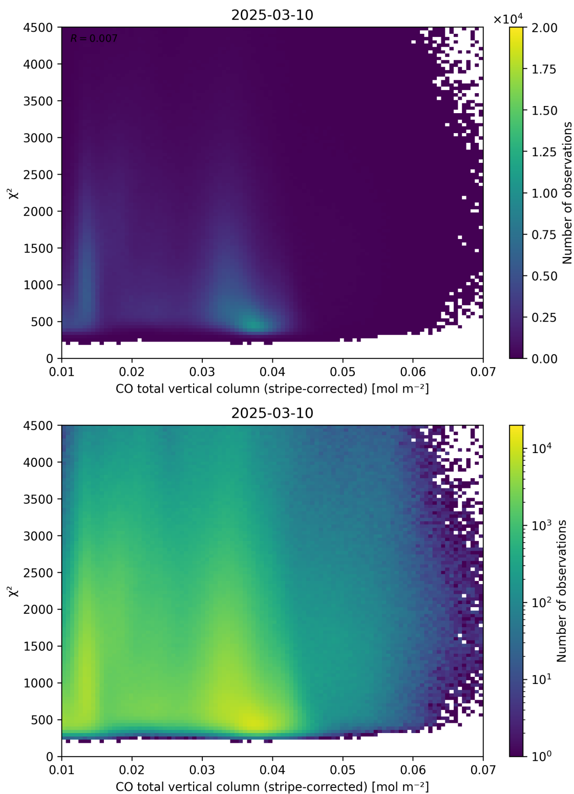
Figure 37: Scatter density plot of “CO total vertical column (stripe-corrected)” against “ \chi^2 ” for 2025-03-09 to 2025-03-11.
