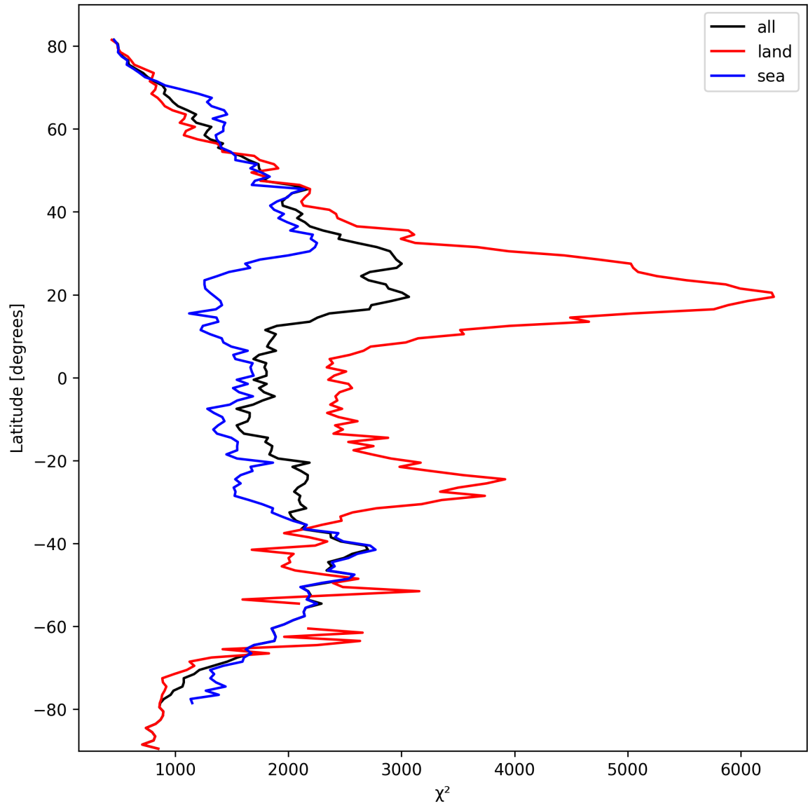
Figure 14: Zonal average of “ \chi^2 ” for 2025-03-09 to 2025-03-11.
