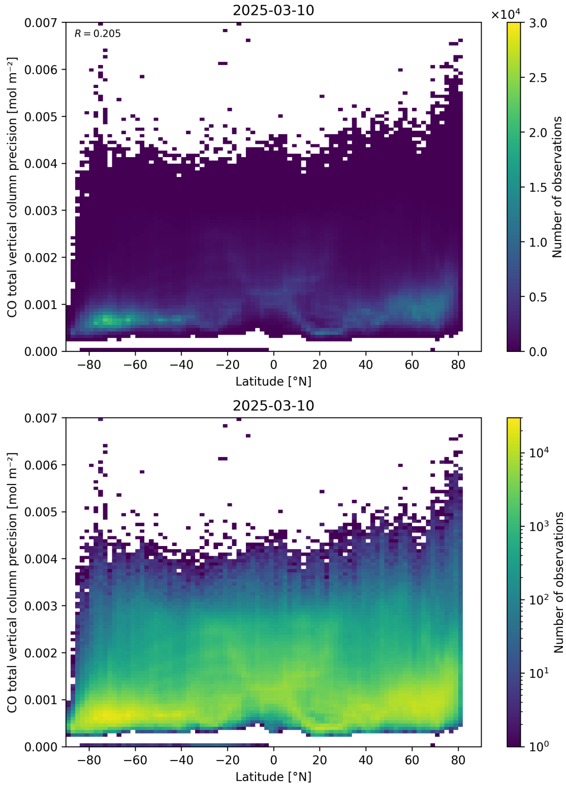
Figure 53: Scatter density plot of “Latitude” against “CO total vertical column precision” for 2025-03-09 to 2025-03-11.
