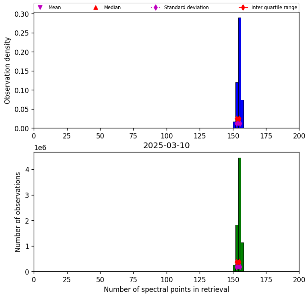
Figure 21: Histogram of “Number of spectral points in retrieval” for 2025-03-09 to 2025-03-11
