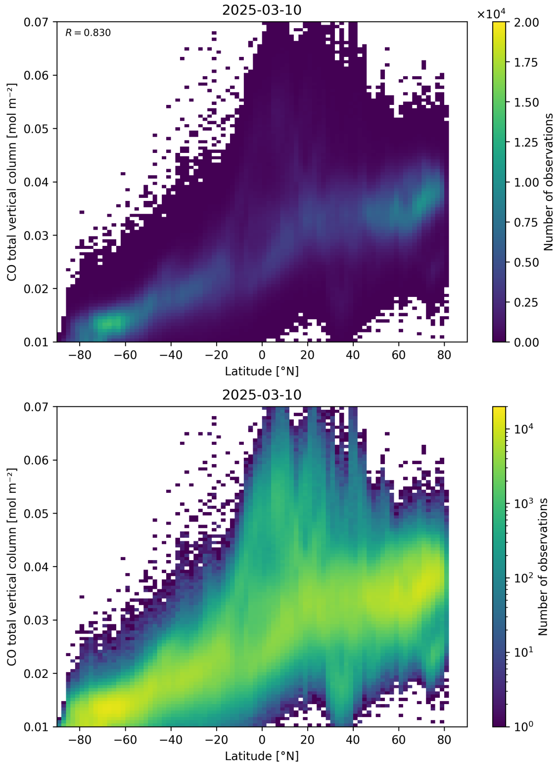
Figure 51: Scatter density plot of “Latitude” against “CO total vertical column” for 2025-03-09 to 2025-03-11.
