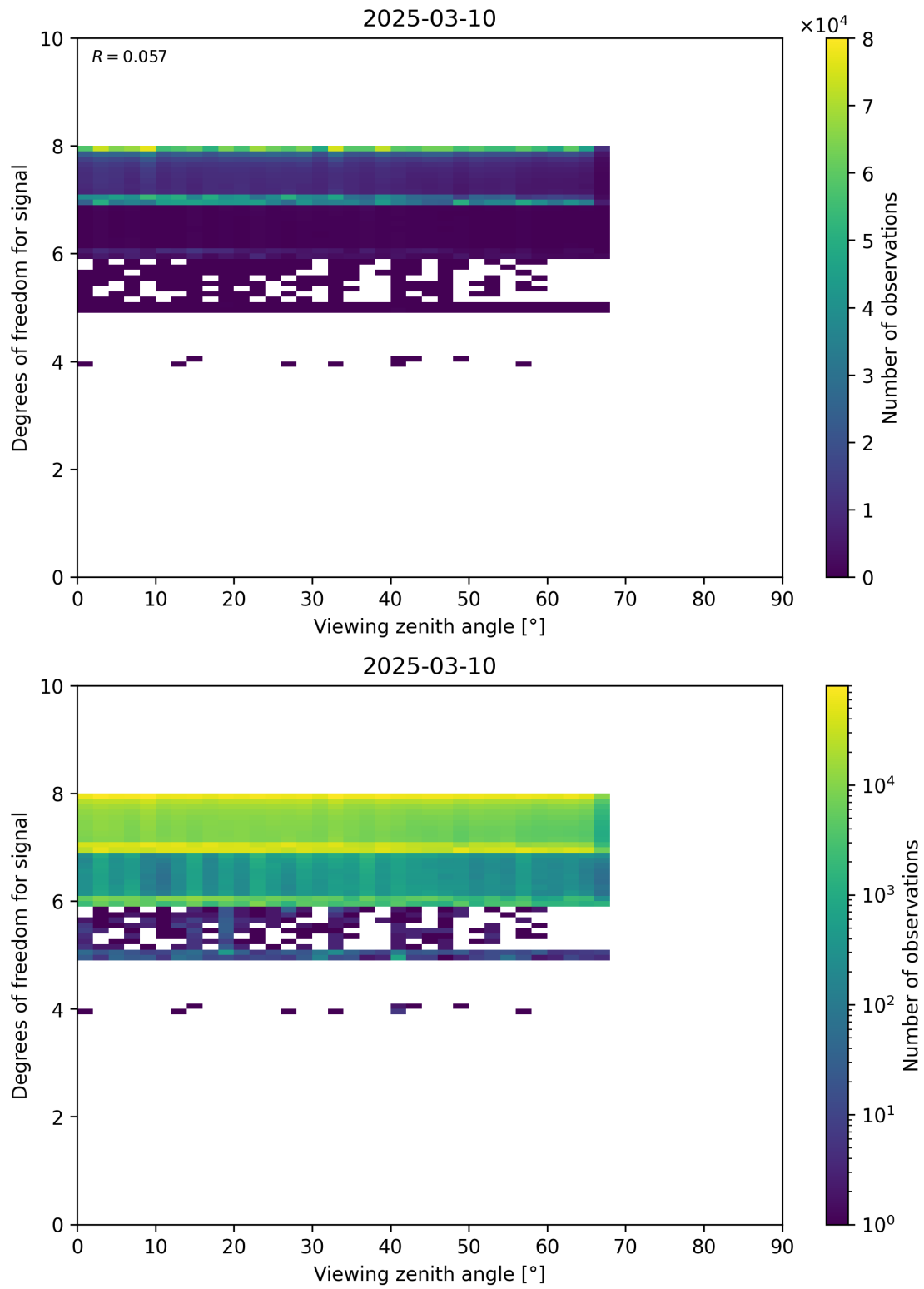
Figure 73: Scatter density plot of “Viewing zenith angle” against “Degrees of freedom for signal” for 2025-03-09 to 2025-03-11.
