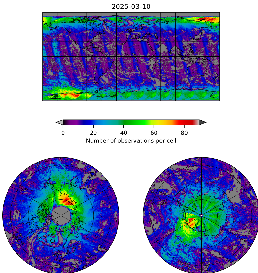
Figure 8: Map of the number of observations for 2025-03-09 to 2025-03-11
