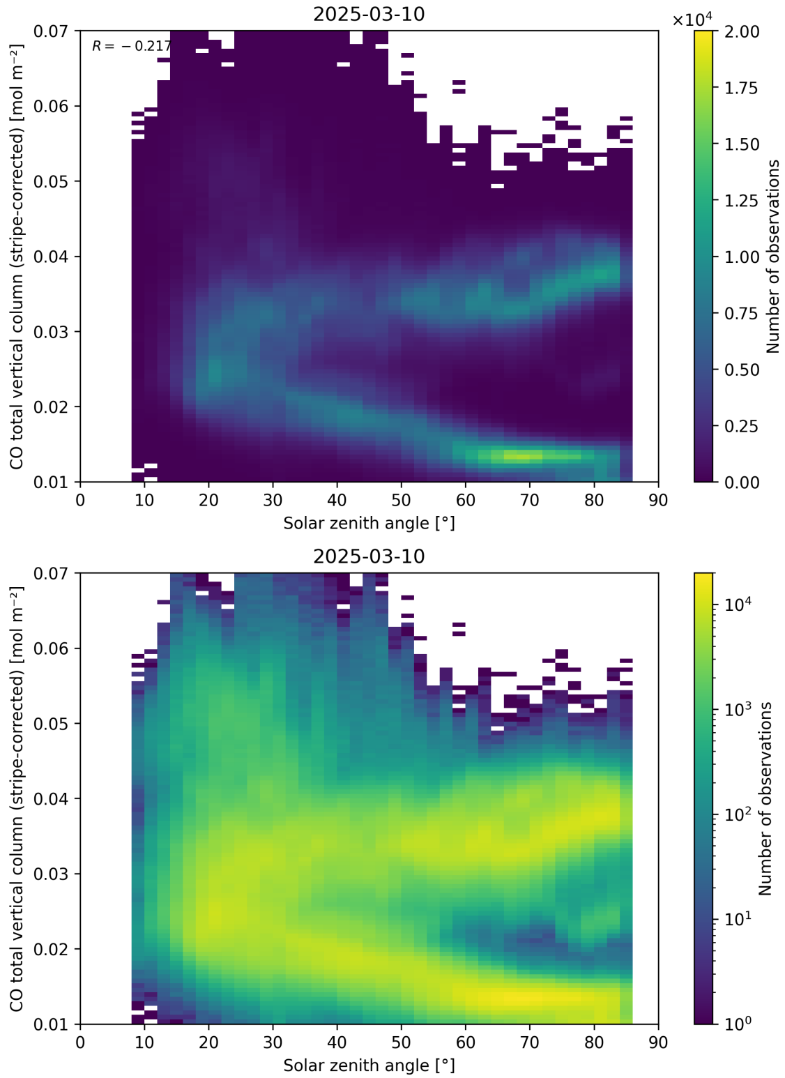
Figure 62: Scatter density plot of “Solar zenith angle” against “CO total vertical column (stripe-corrected)” for 2025-03-09 to 2025-03-11.
