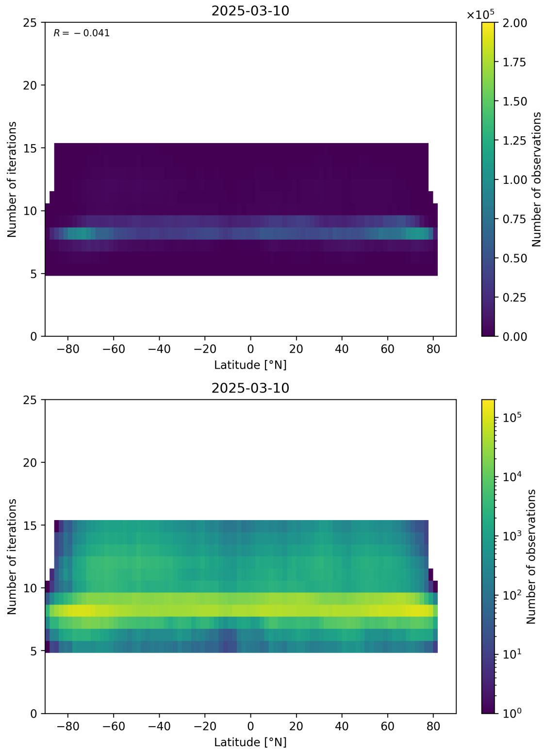
Figure 56: Scatter density plot of “Latitude” against “Number of iterations” for 2025-03-09 to 2025-03-11.
