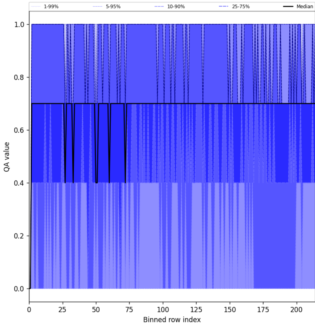
Figure 25: Along track statistics of “QA value” for 2025-03-09 to 2025-03-11
