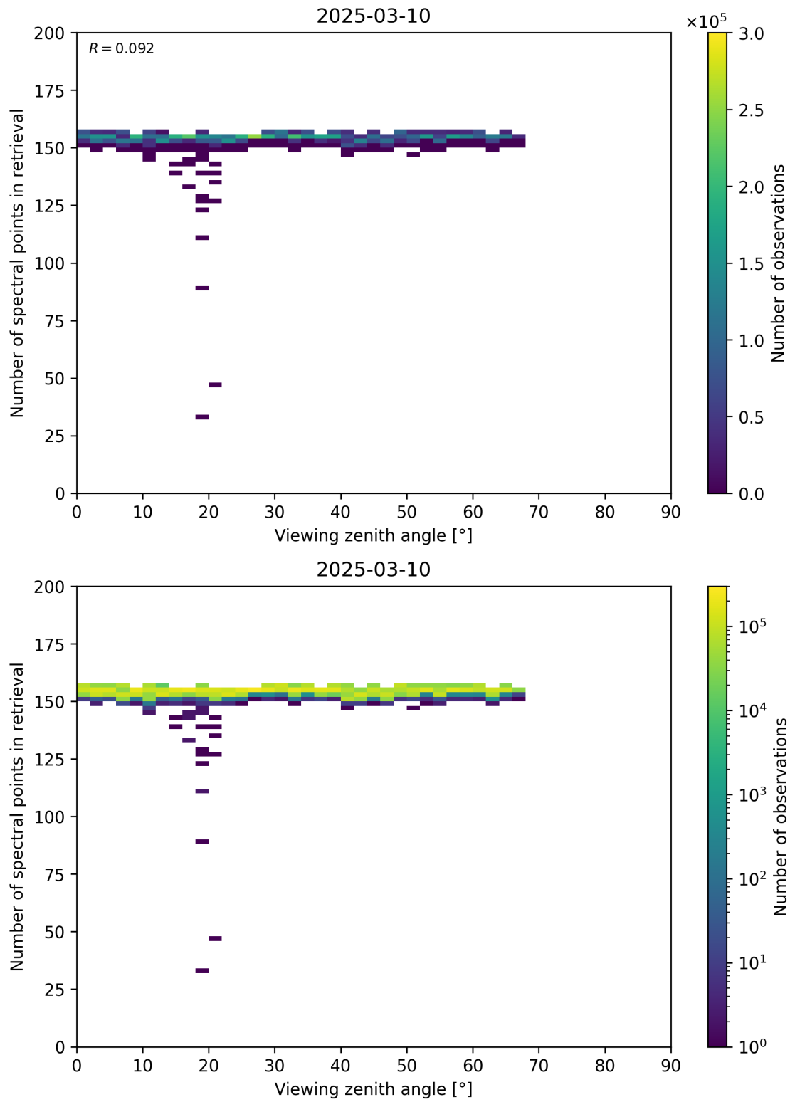
Figure 76: Scatter density plot of “Viewing zenith angle” against “Number of spectral points in retrieval” for 2025-03-09 to 2025-03-11.
