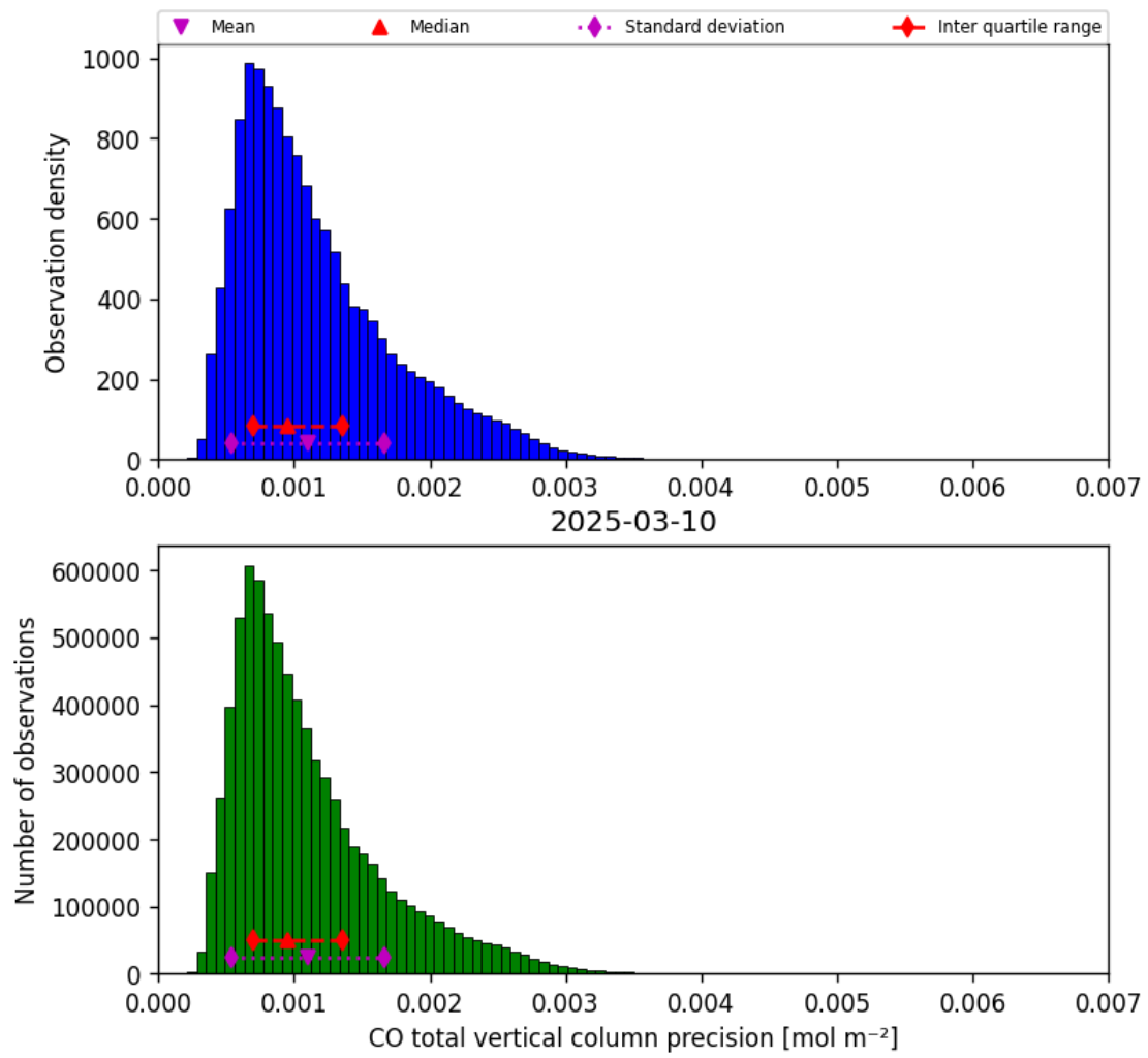
Figure 20: Histogram of “CO total vertical column precision” for 2025-03-09 to 2025-03-11
