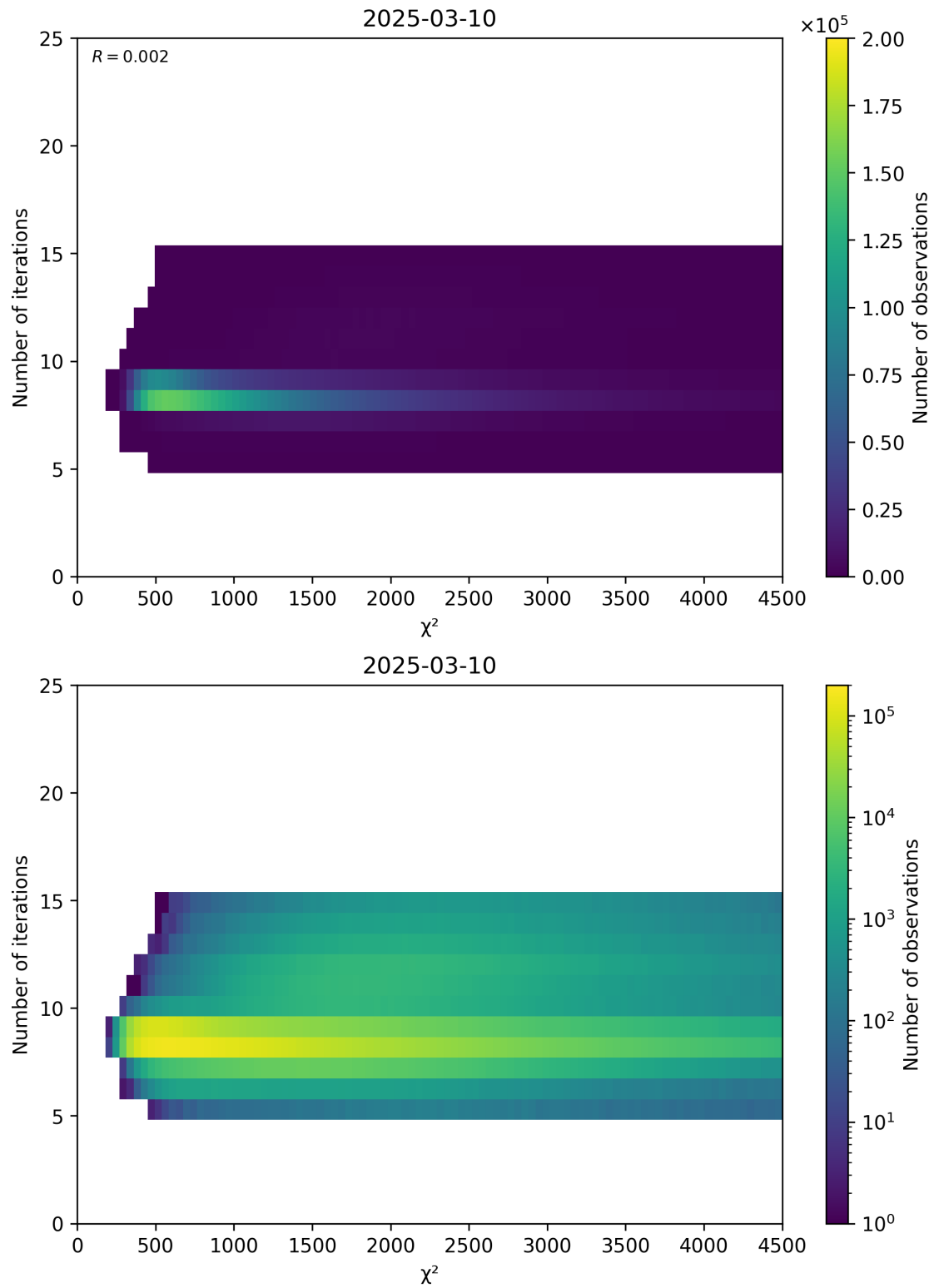
Figure 49: Scatter density plot of “ \chi^2 ” against “Number of iterations” for 2025-03-09 to 2025-03-11.
