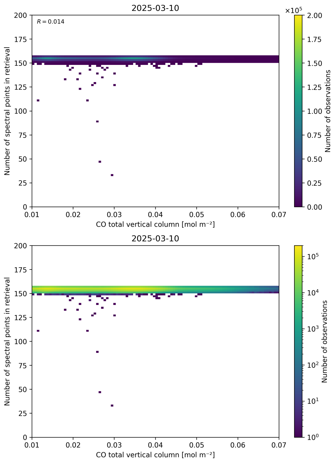
Figure 43: Scatter density plot of “CO total vertical column” against “Number of spectral points in retrieval” for 2025-03-09 to 2025-03-11.
