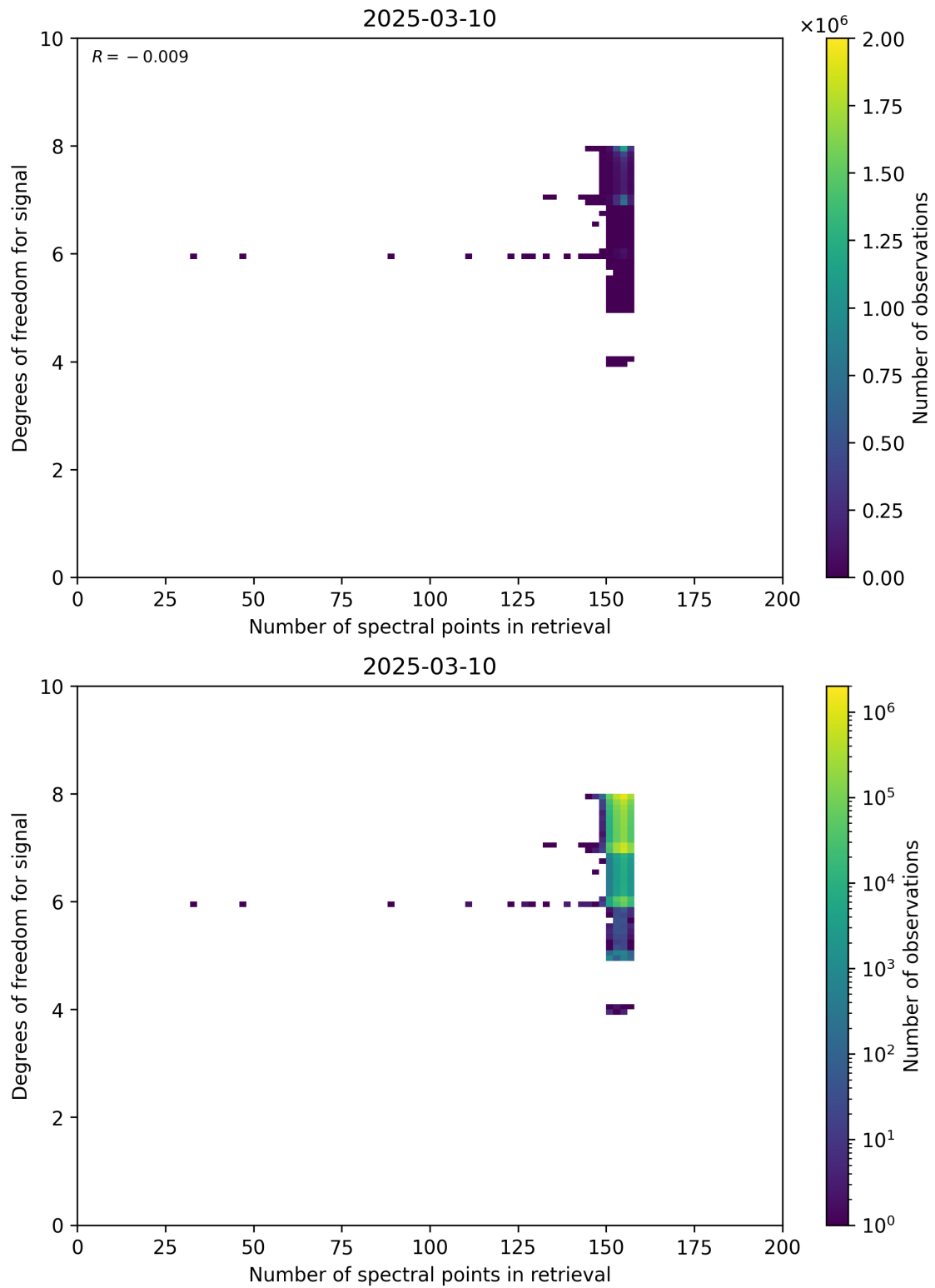
Figure 59: Scatter density plot of “Number of spectral points in retrieval” against “Degrees of freedom for signal” for 2025-03-09 to 2025-03-11.
