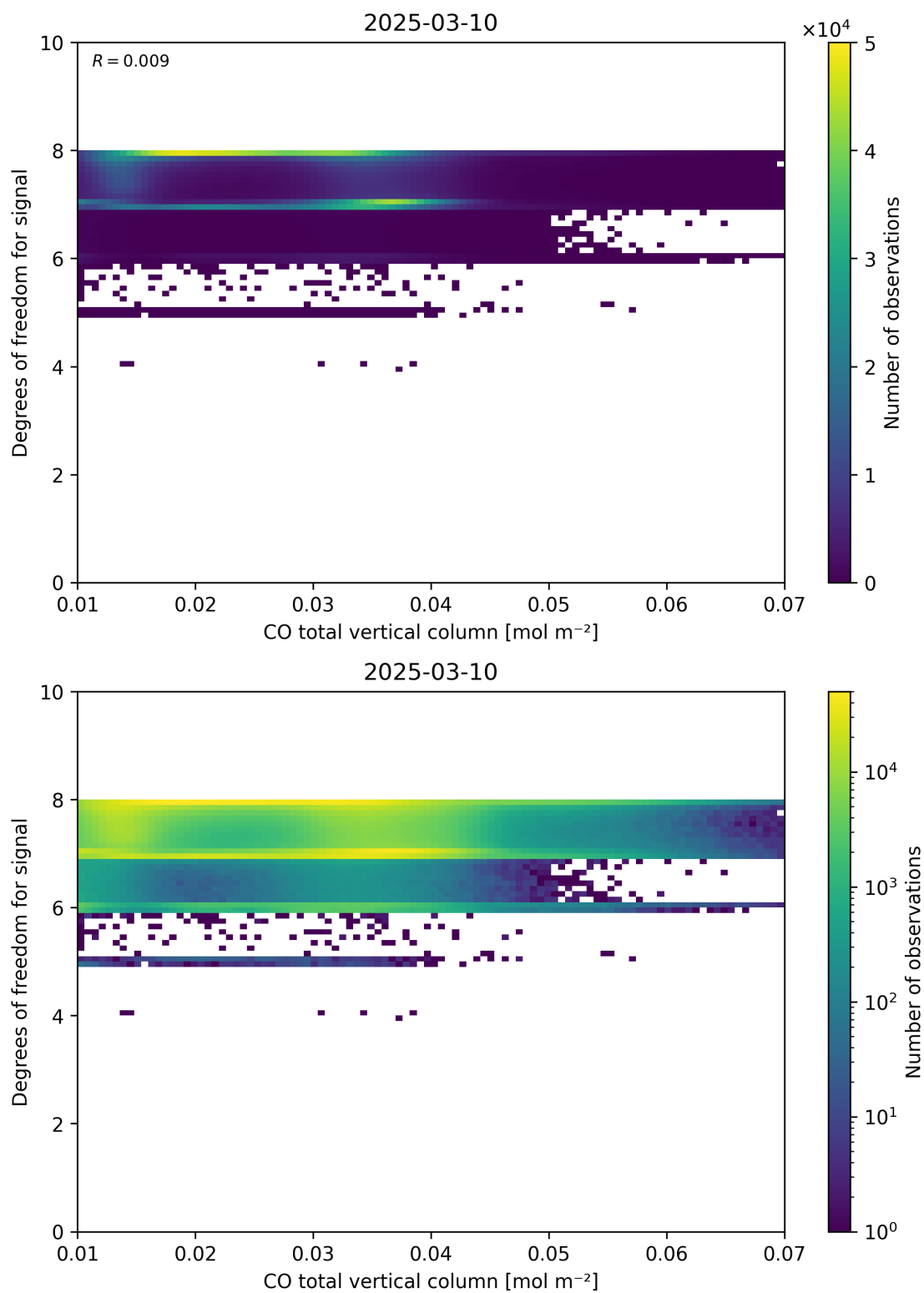
Figure 41: Scatter density plot of “CO total vertical column” against “Degrees of freedom for signal” for 2025-03-09 to 2025-03-11.
