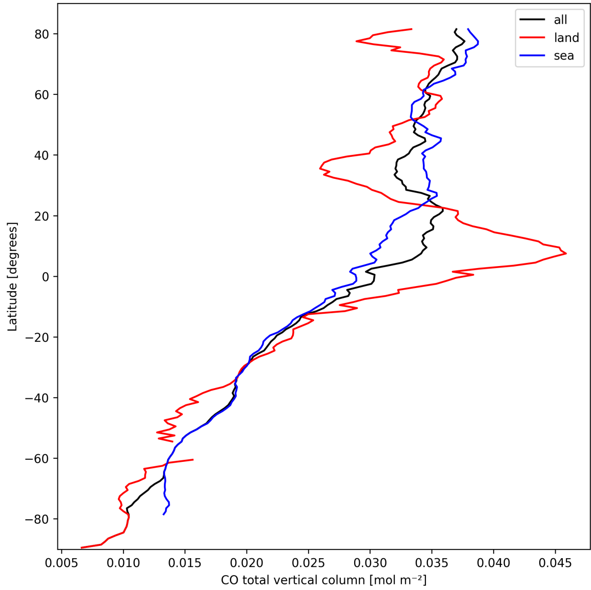
Figure 10: Zonal average of “CO total vertical column” for 2025-03-09 to 2025-03-11.
