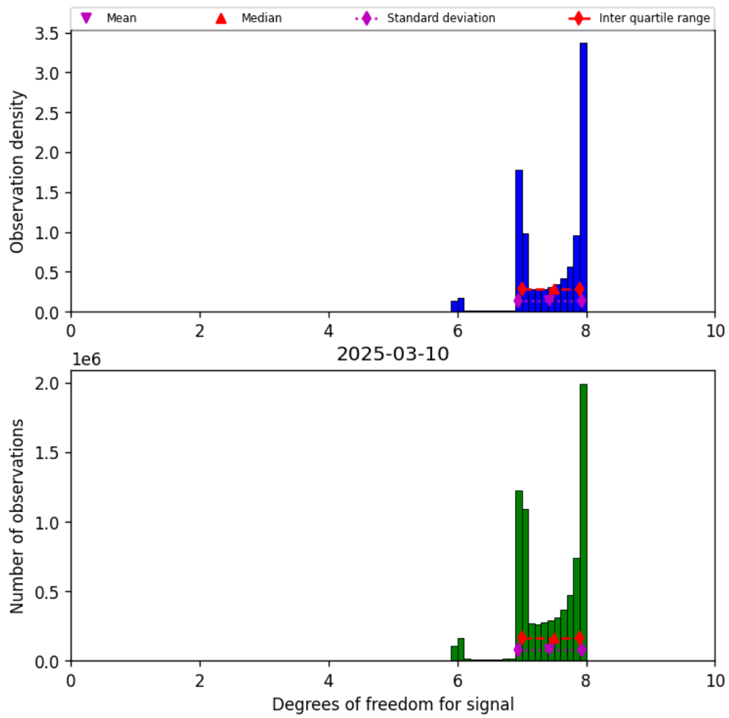
Figure 23: Histogram of “Degrees of freedom for signal” for 2025-03-09 to 2025-03-11
