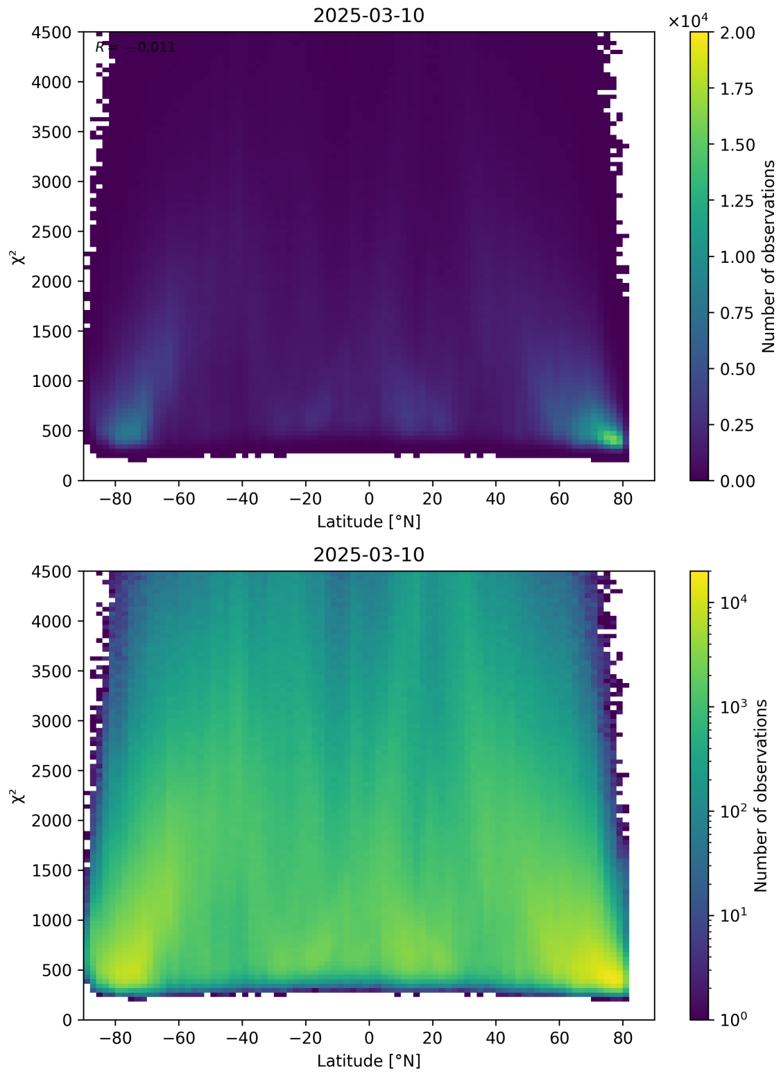
Figure 54: Scatter density plot of “Latitude” against “ \chi^2 ” for 2025-03-09 to 2025-03-11.
