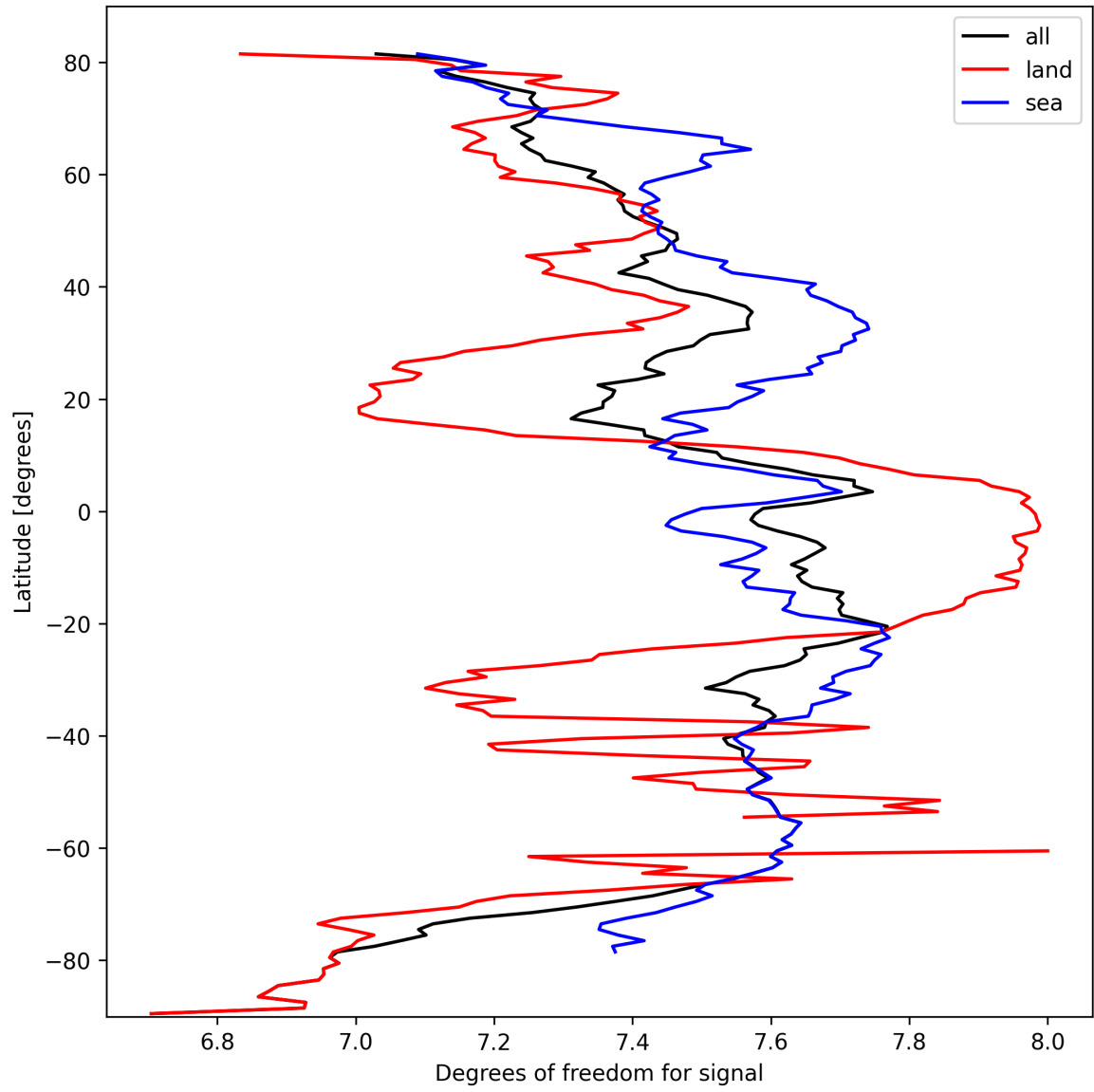
Figure 15: Zonal average of “Degrees of freedom for signal” for 2025-03-09 to 2025-03-11.
