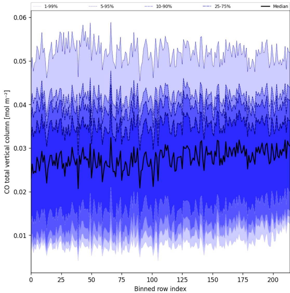
Figure 26: Along track statistics of “CO total vertical column” for 2025-03-09 to 2025-03-11
