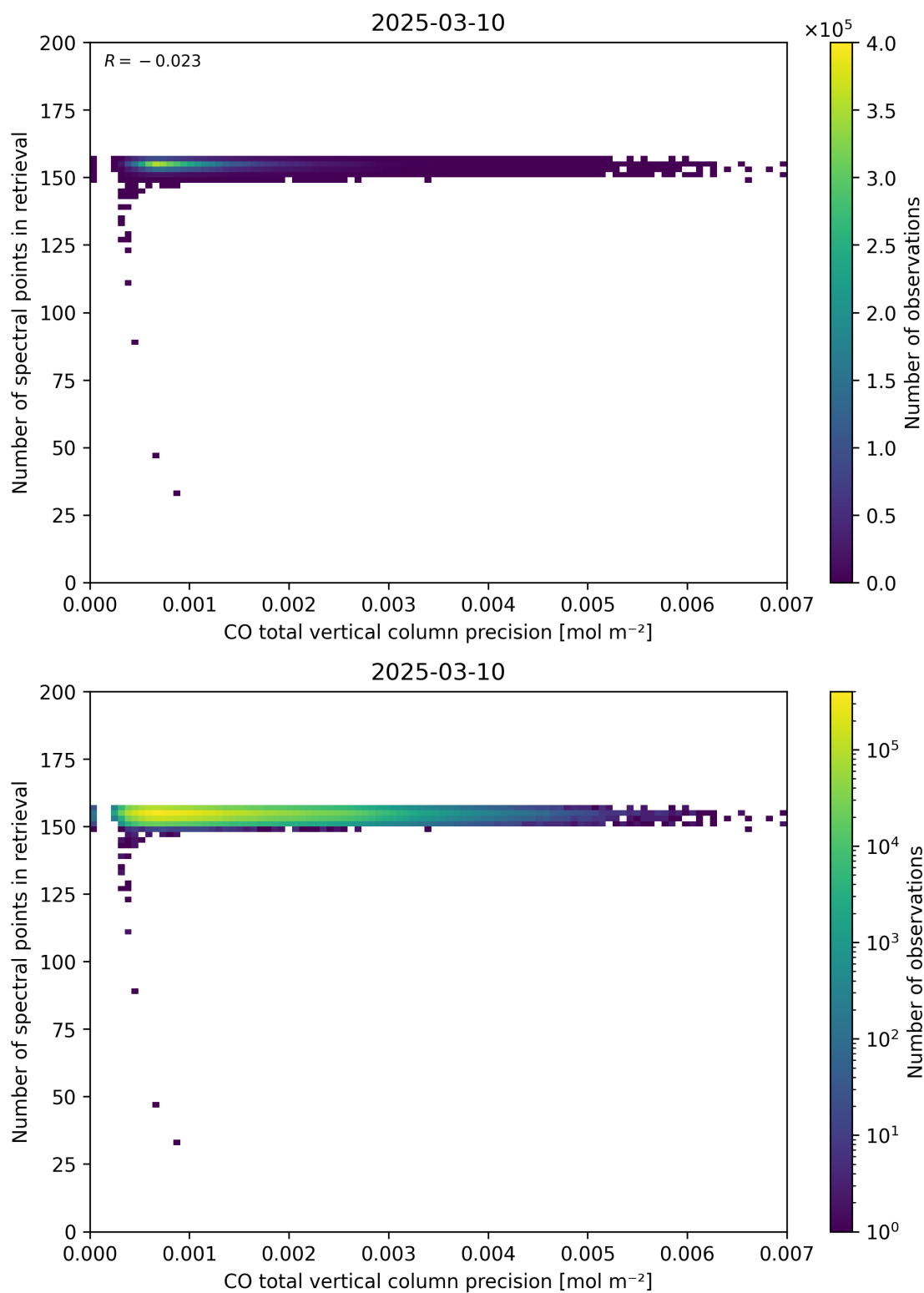
Figure 47: Scatter density plot of “CO total vertical column precision” against “Number of spectral points in retrieval” for 2025-03-09 to 2025-03-11.
