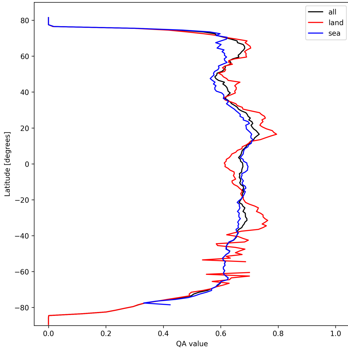
Figure 9: Zonal average of “QA value” for 2025-03-09 to 2025-03-11.
