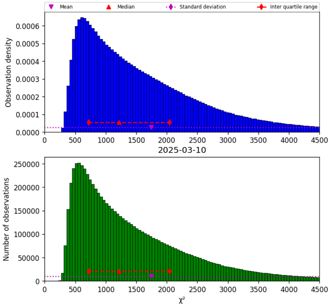
Figure 22: Histogram of “ \chi^2 ” for 2025-03-09 to 2025-03-11
