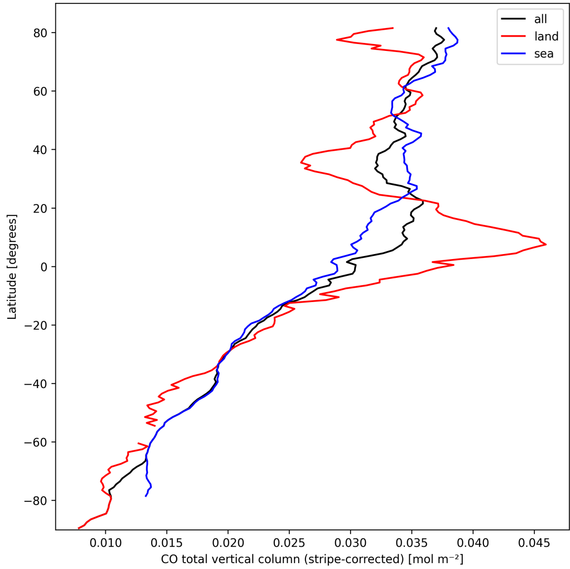
Figure 11: Zonal average of “CO total vertical column (stripe-corrected)” for 2025-03-09 to 2025-03-11.
