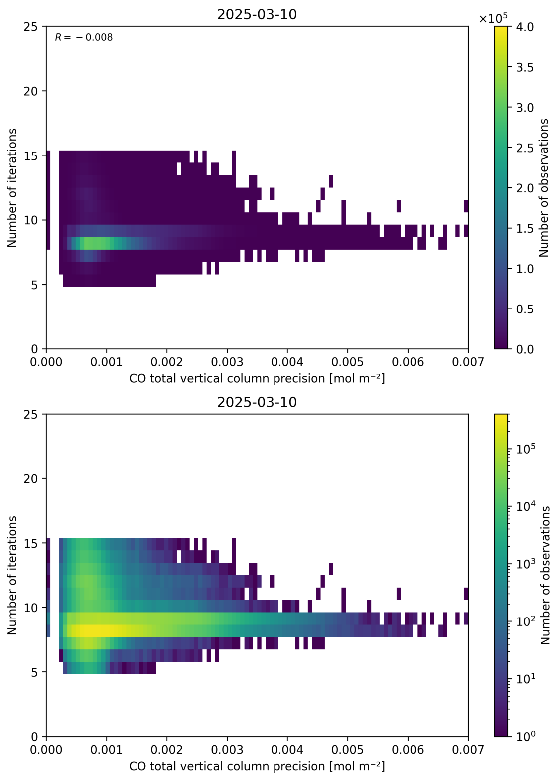
Figure 46: Scatter density plot of “CO total vertical column precision” against “Number of iterations” for 2025-03-09 to 2025-03-11.
