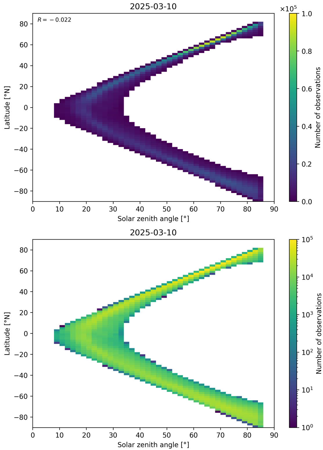
Figure 66: Scatter density plot of “Solar zenith angle” against “Latitude” for 2025-03-09 to 2025-03-11.
