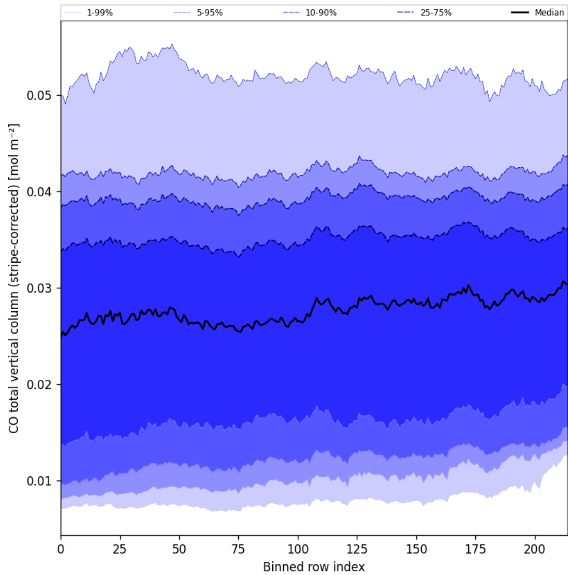
Figure 27: Along track statistics of “CO total vertical column (stripe-corrected)” for 2025-03-09 to 2025-03-11
