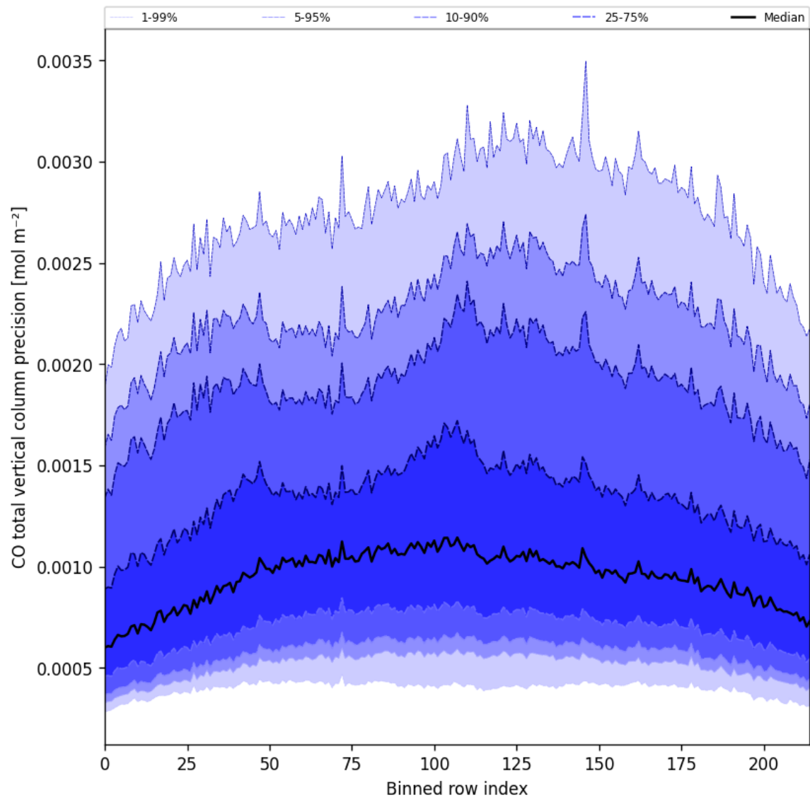
Figure 28: Along track statistics of “CO total vertical column precision” for 2025-03-09 to 2025-03-11
