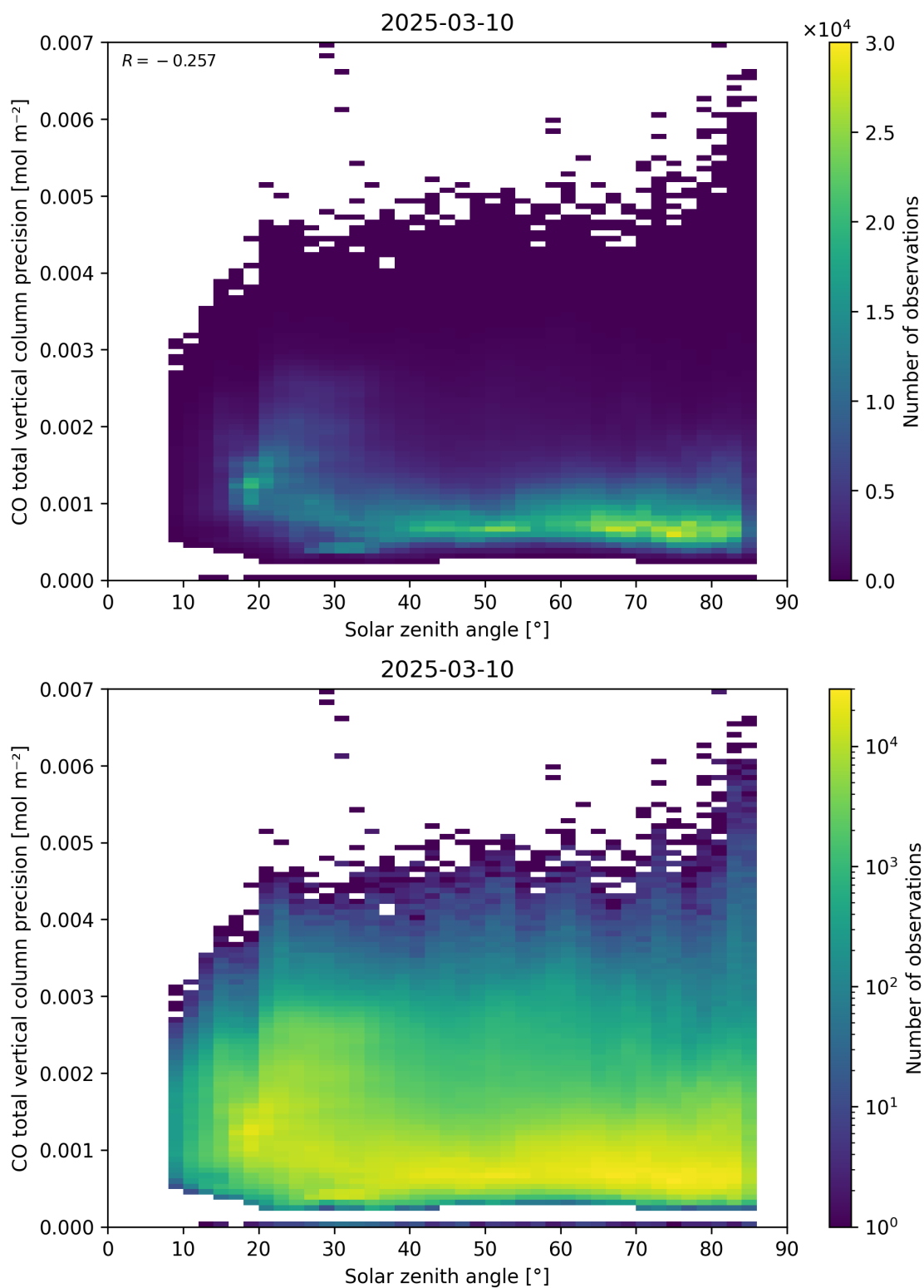
Figure 63: Scatter density plot of “Solar zenith angle” against “CO total vertical column precision” for 2025-03-09 to 2025-03-11.
