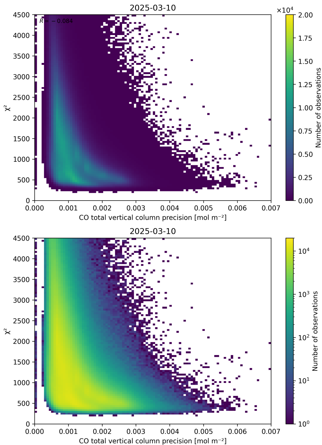
Figure 44: Scatter density plot of “CO total vertical column precision” against “ \chi^2 ” for 2025-03-09 to 2025-03-11.
