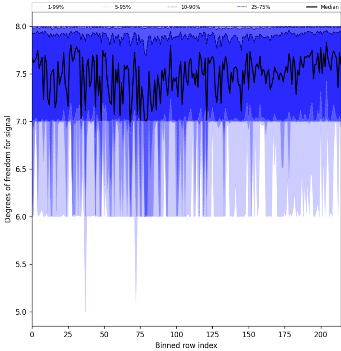
Figure 31: Along track statistics of “Degrees of freedom for signal” for 2025-03-09 to 2025-03-11
