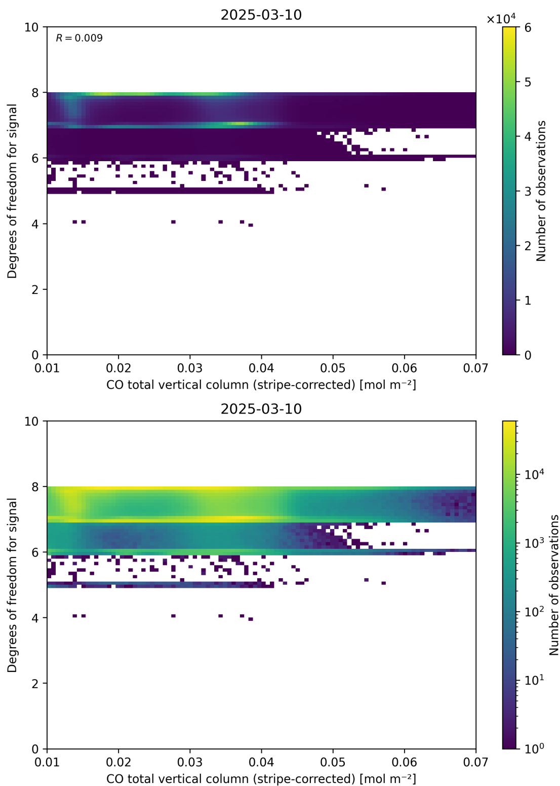
Figure 38: Scatter density plot of “CO total vertical column (stripe-corrected)” against “Degrees of freedom for signal” for 2025-03-09 to 2025-03-11.
