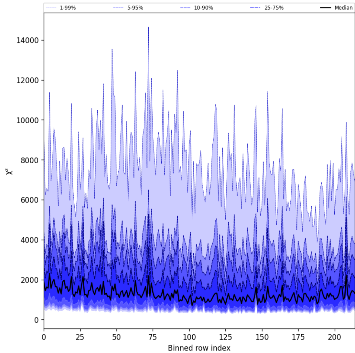
Figure 30: Along track statistics of “ \chi^2 ” for 2025-03-09 to 2025-03-11
