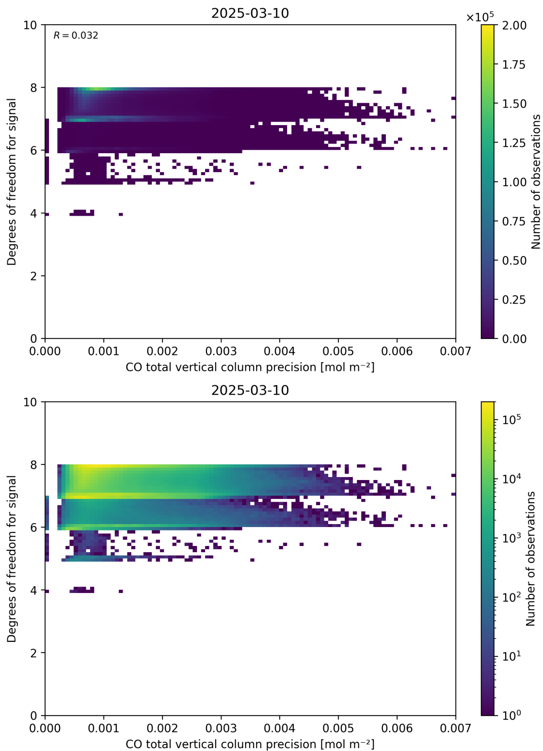
Figure 45: Scatter density plot of “CO total vertical column precision” against “Degrees of freedom for signal” for 2025-03-09 to 2025-03-11.
