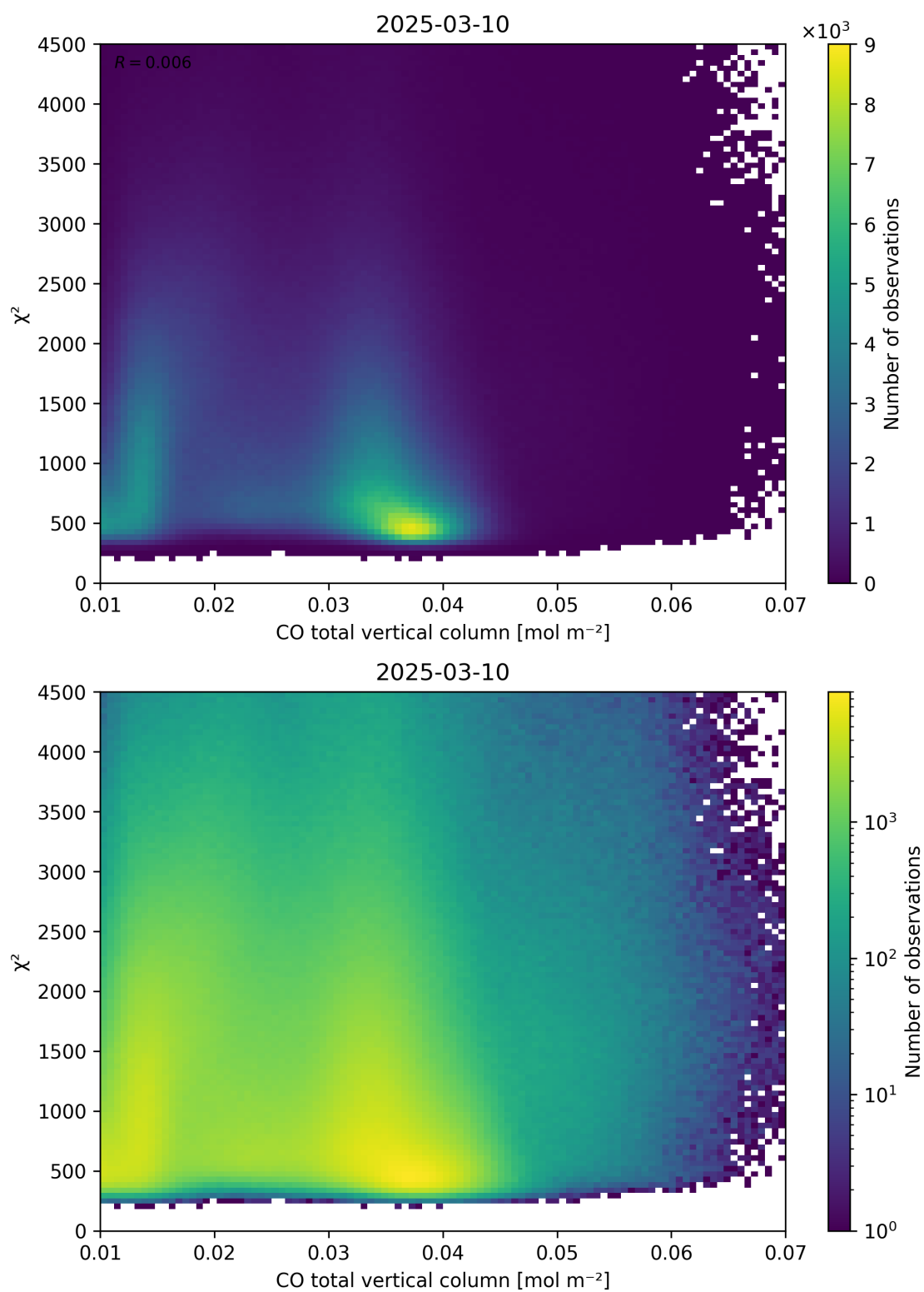
Figure 35: Scatter density plot of “CO total vertical column” against “ \chi^2 ” for 2025-03-09 to 2025-03-11.
