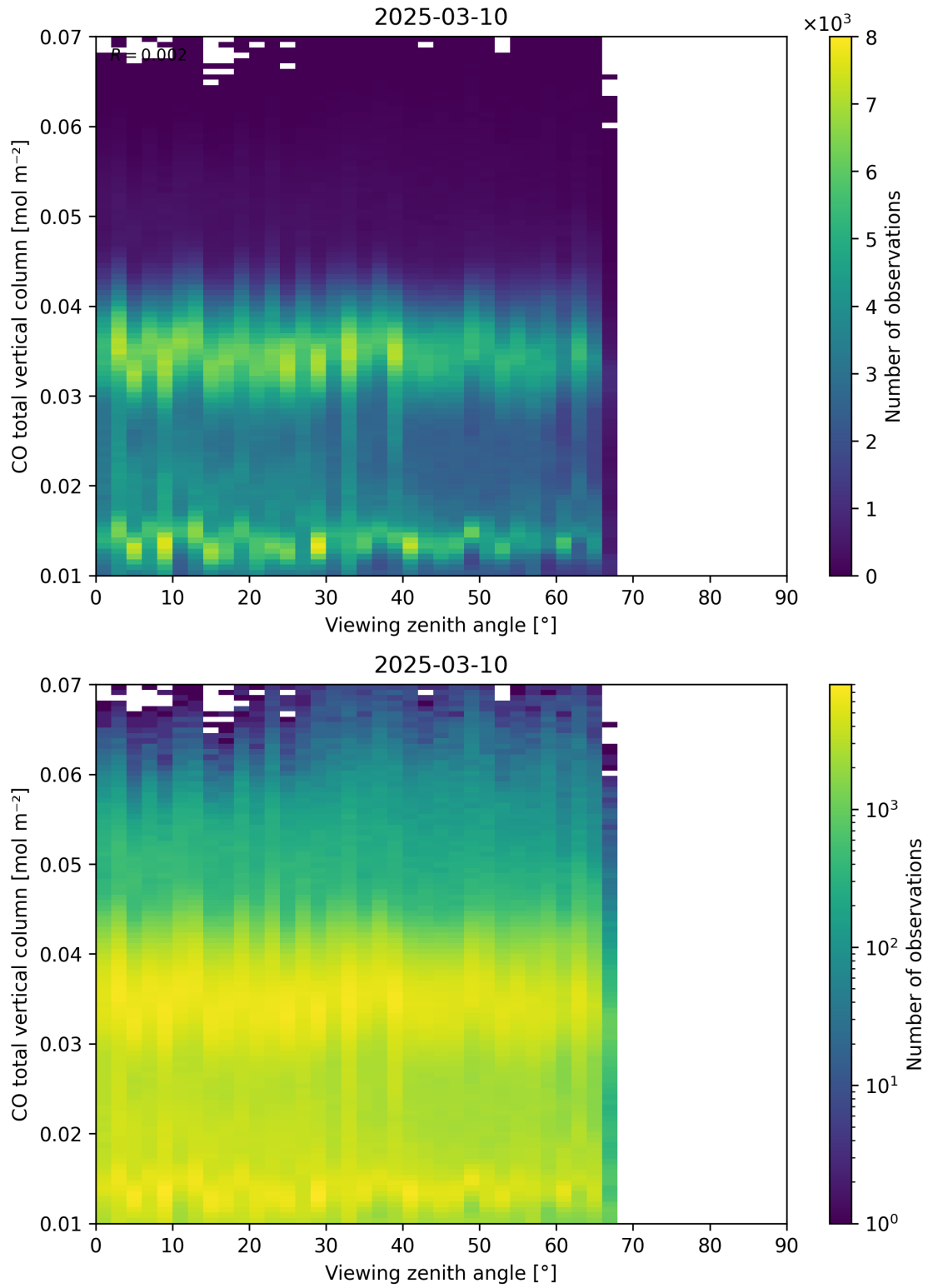
Figure 69: Scatter density plot of “Viewing zenith angle” against “CO total vertical column” for 2025-03-09 to 2025-03-11.
