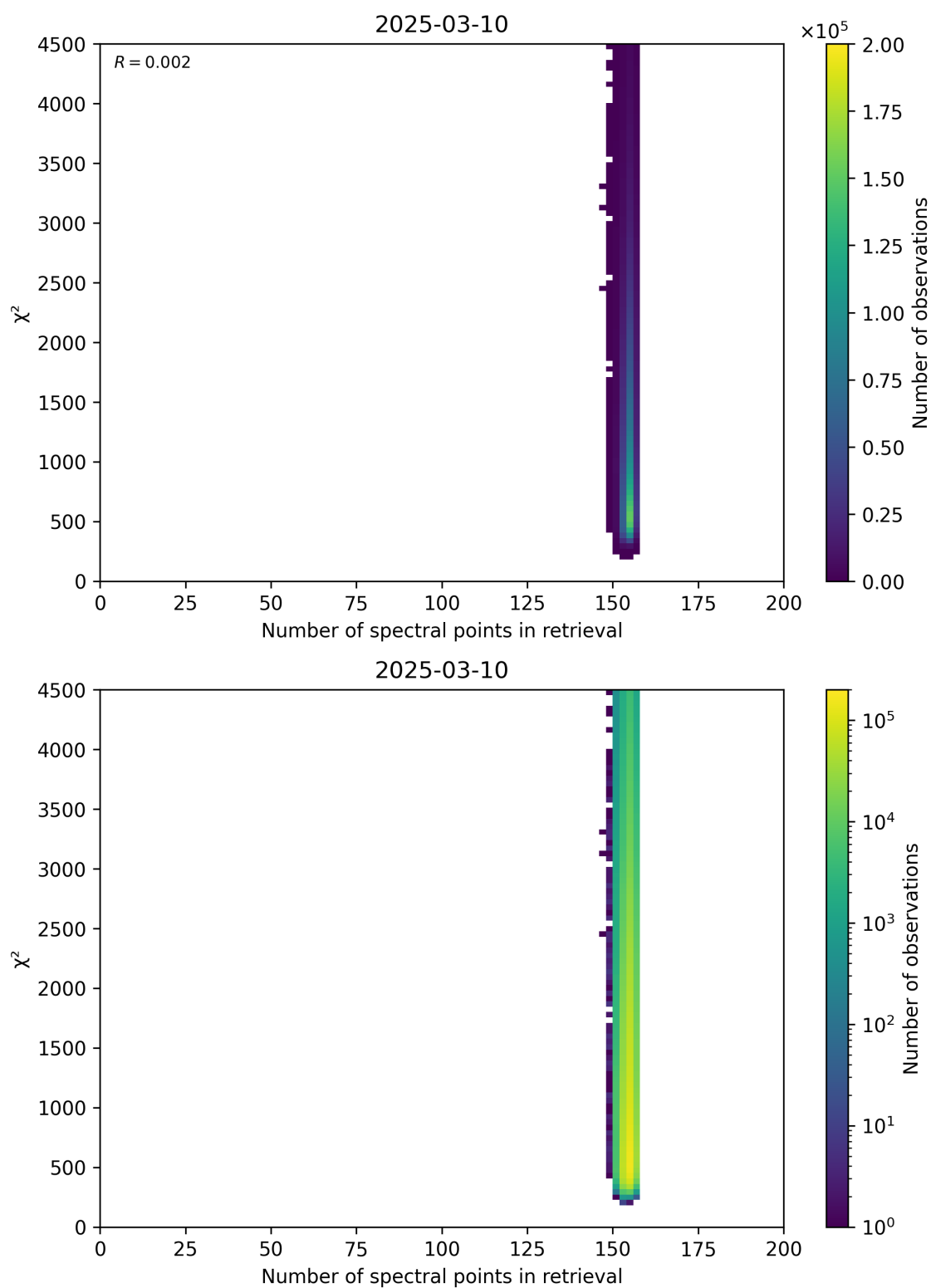
Figure 58: Scatter density plot of “Number of spectral points in retrieval” against “ \chi^2 ” for 2025-03-09 to 2025-03-11.
