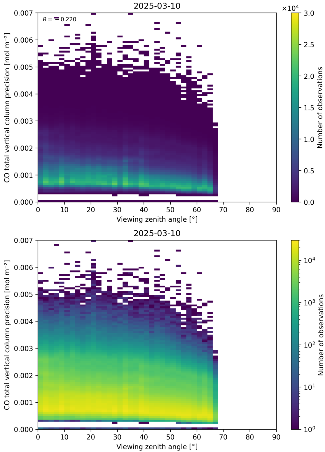
Figure 71: Scatter density plot of “Viewing zenith angle” against “CO total vertical column precision” for 2025-03-09 to 2025-03-11.
