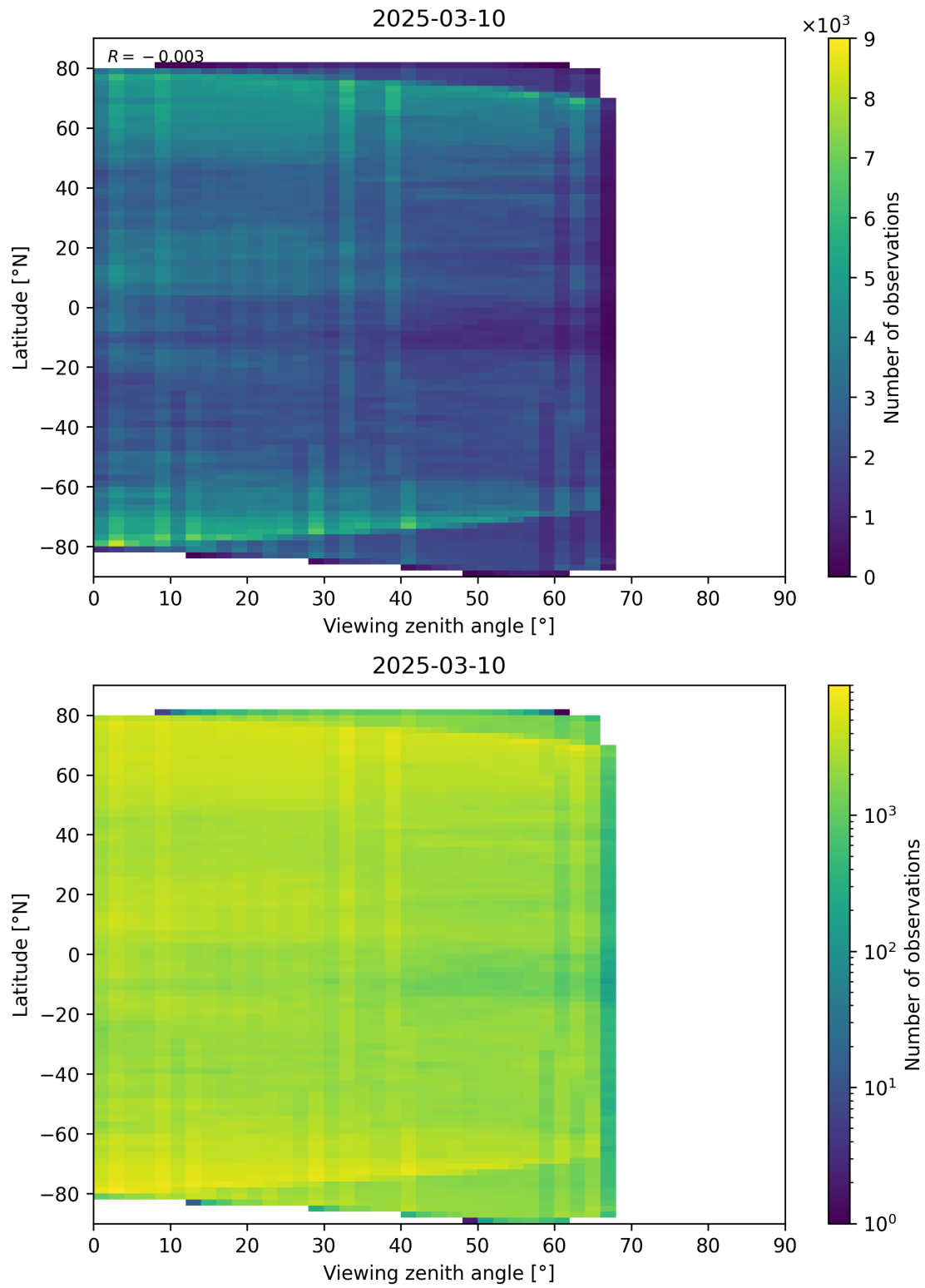
Figure 74: Scatter density plot of “Viewing zenith angle” against “Latitude” for 2025-03-09 to 2025-03-11.
