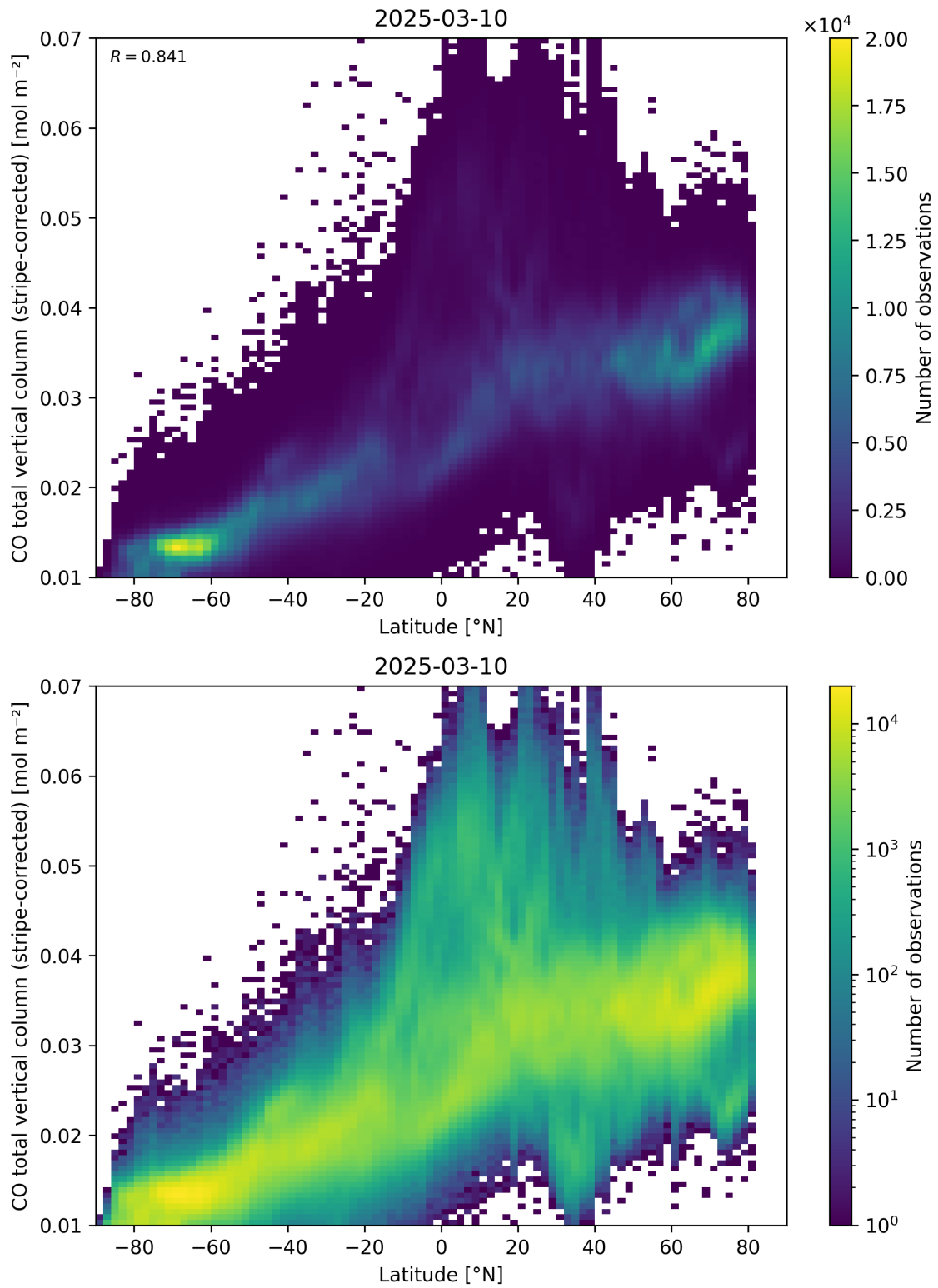
Figure 52: Scatter density plot of “Latitude” against “CO total vertical column (stripe-corrected)” for 2025-03-09 to 2025-03-11.
