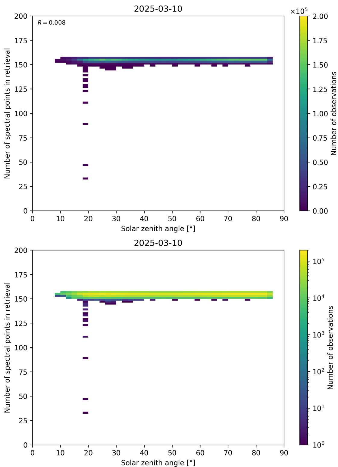
Figure 68: Scatter density plot of “Solar zenith angle” against “Number of spectral points in retrieval” for 2025-03-09 to 2025-03-11.
