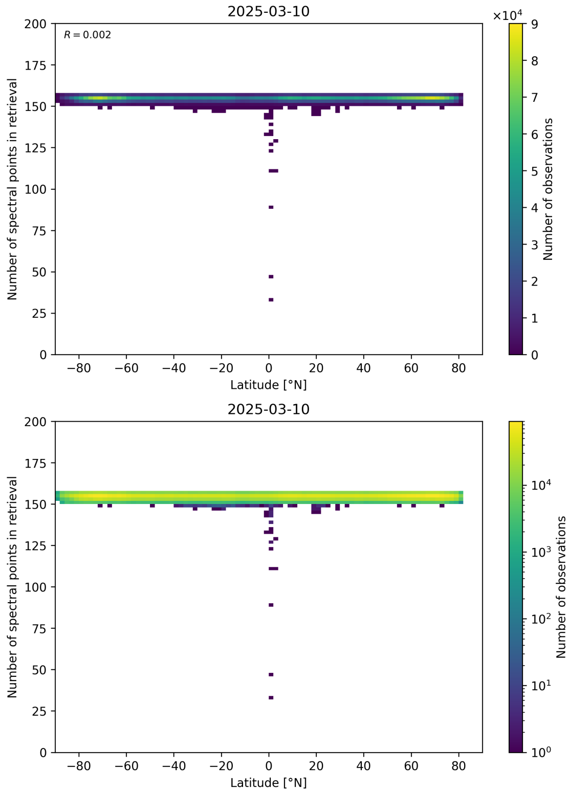
Figure 57: Scatter density plot of “Latitude” against “Number of spectral points in retrieval” for 2025-03-09 to 2025-03-11.
