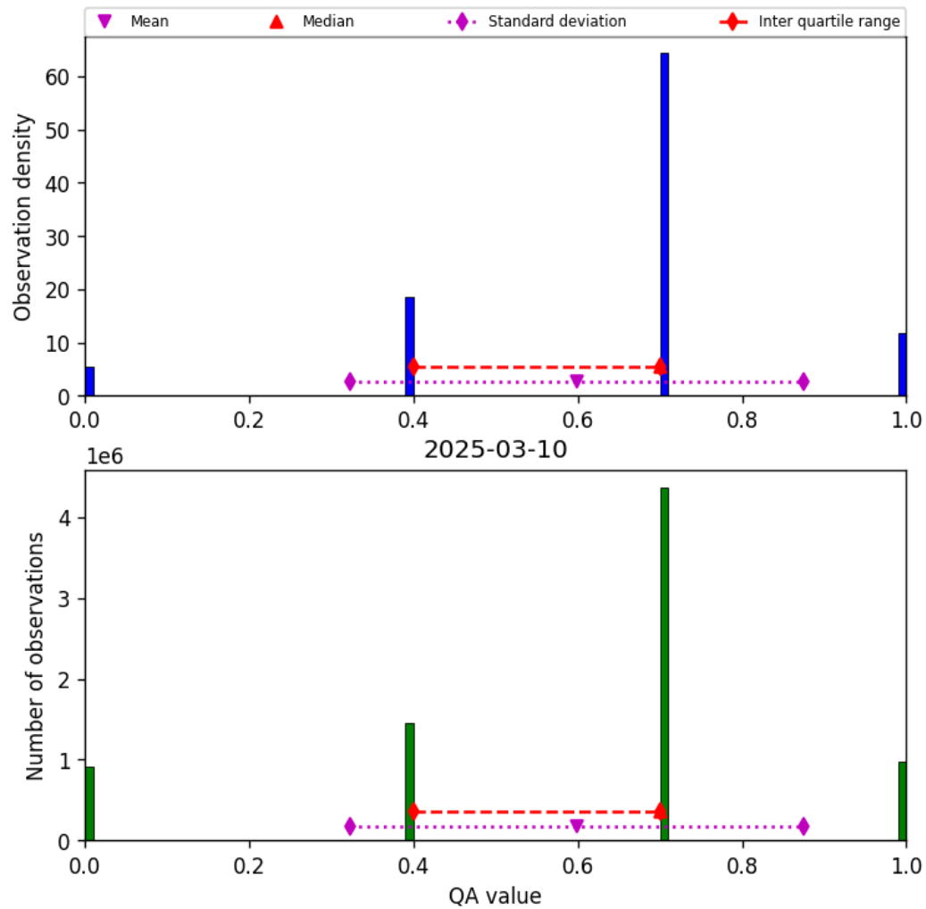
Figure 17: Histogram of “QA value” for 2025-03-09 to 2025-03-11
