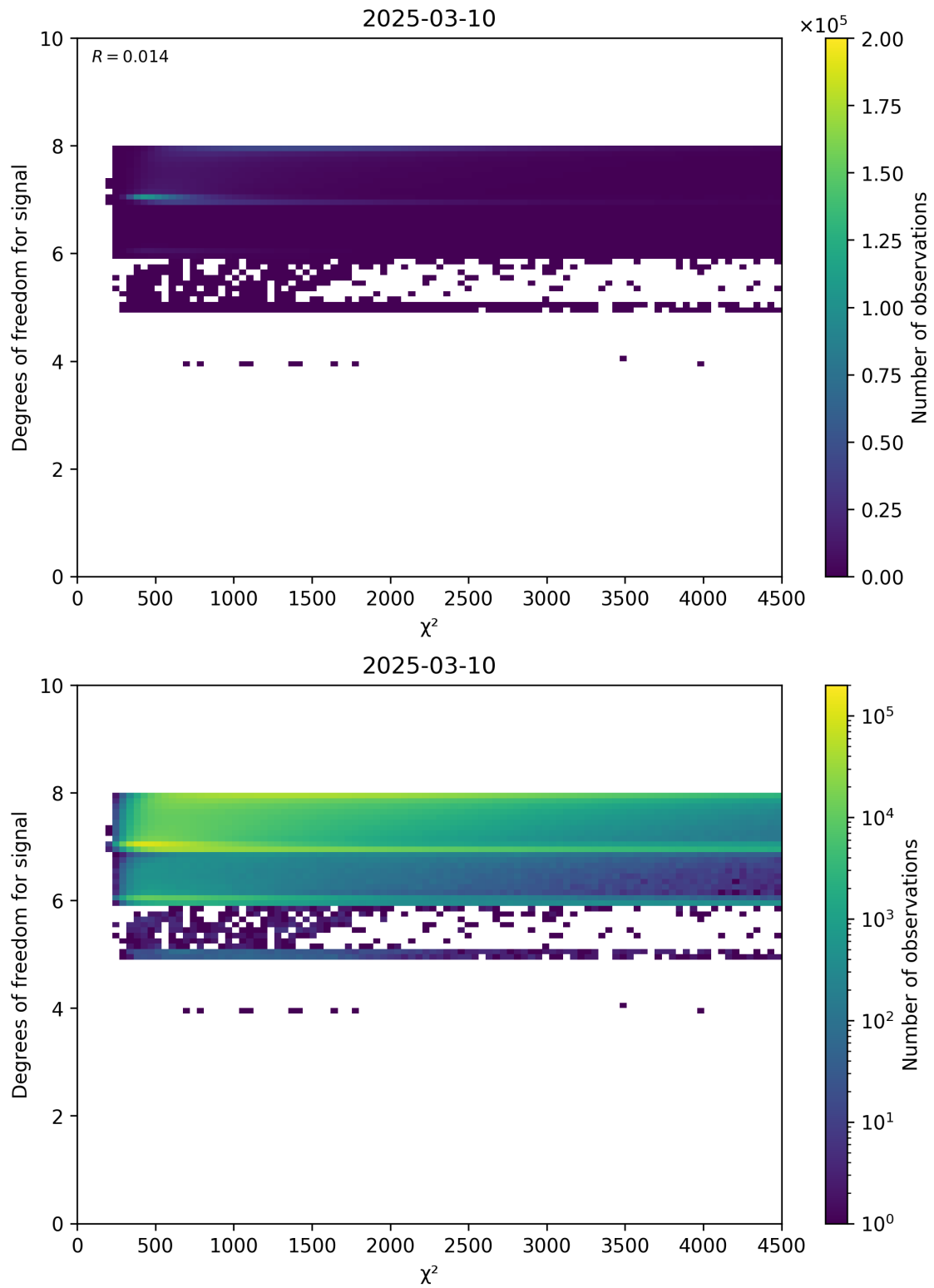
Figure 48: Scatter density plot of “ \chi^2 ” against “Degrees of freedom for signal” for 2025-03-09 to 2025-03-11.
