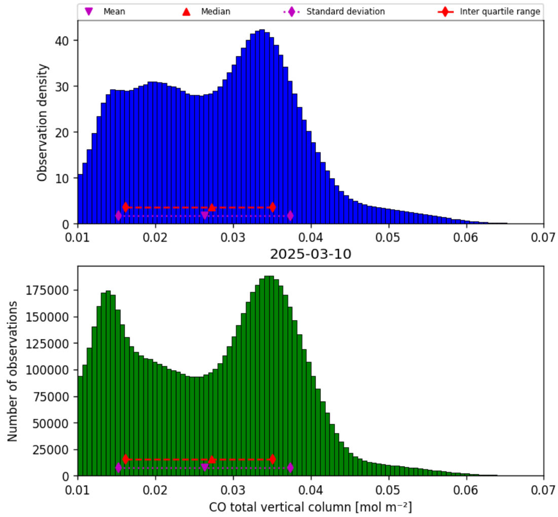
Figure 18: Histogram of “CO total vertical column” for 2025-03-09 to 2025-03-11
