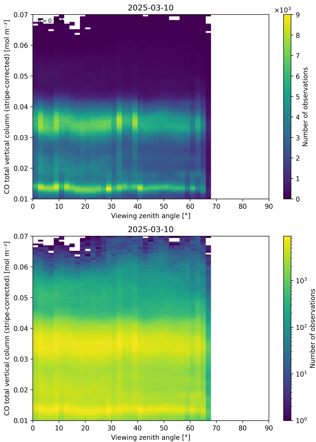
Figure 70: Scatter density plot of “Viewing zenith angle” against “CO total vertical column (stripe-corrected)” for 2025-03-09 to 2025-03-11.
