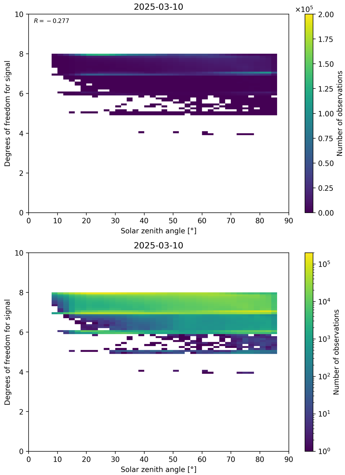
Figure 65: Scatter density plot of “Solar zenith angle” against “Degrees of freedom for signal” for 2025-03-09 to 2025-03-11.
