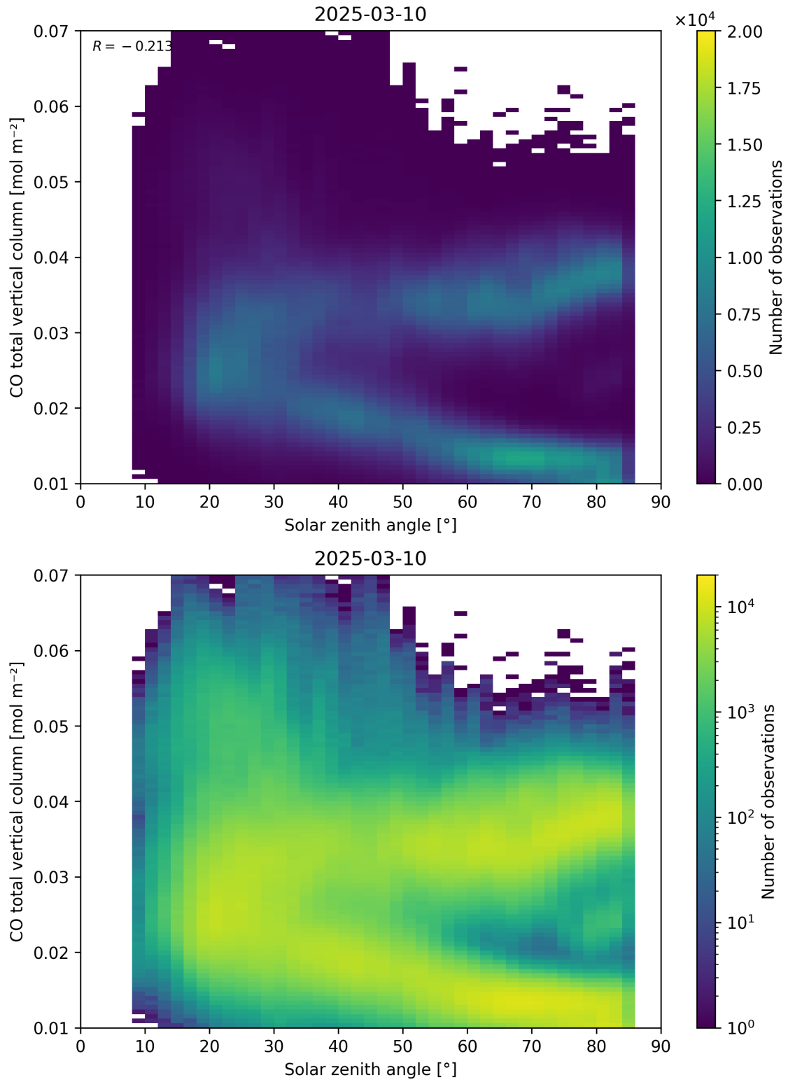
Figure 61: Scatter density plot of “Solar zenith angle” against “CO total vertical column” for 2025-03-09 to 2025-03-11.
