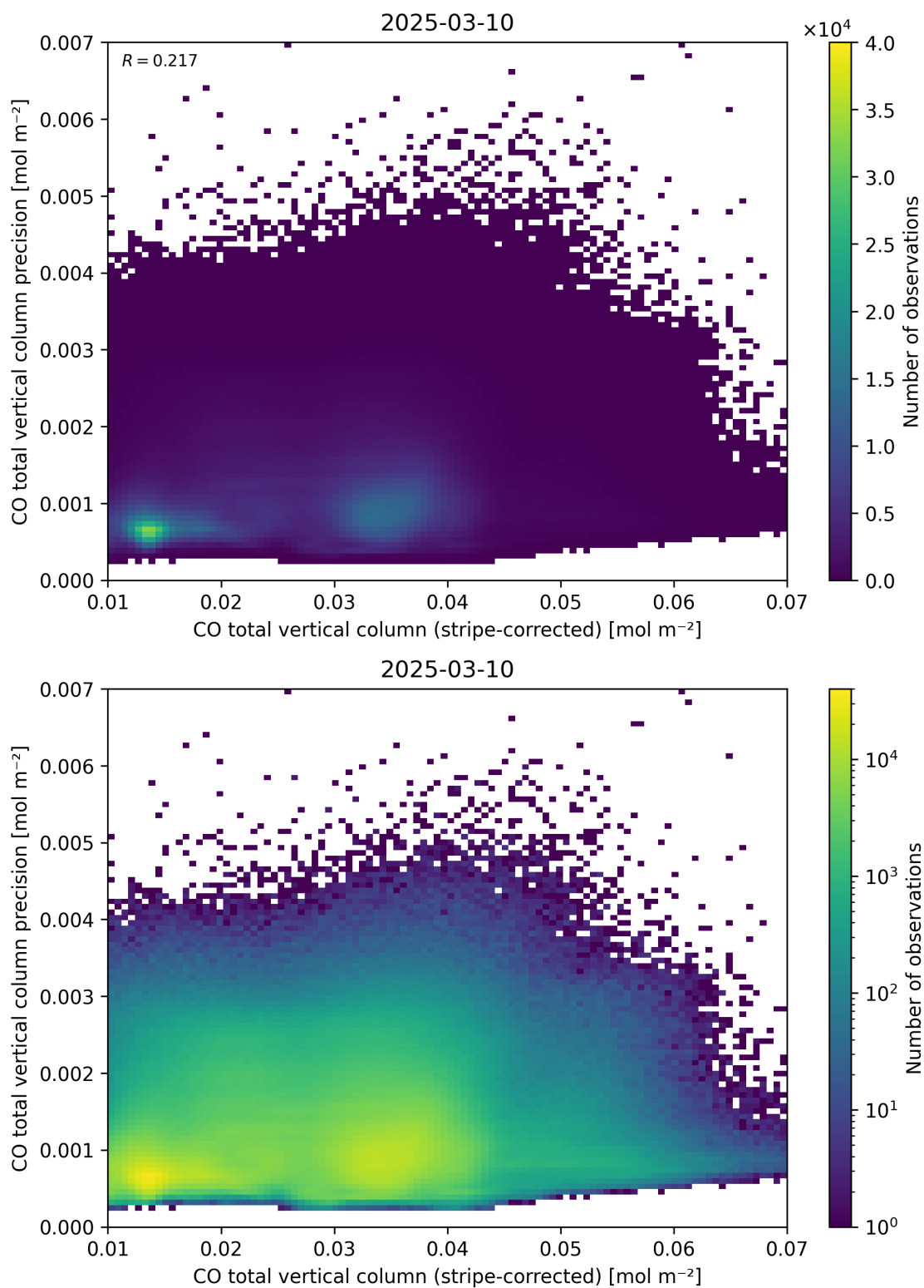
Figure 36: Scatter density plot of “CO total vertical column (stripe-corrected)” against “CO total vertical column precision” for 2025-03-09 to 2025-03-11.
