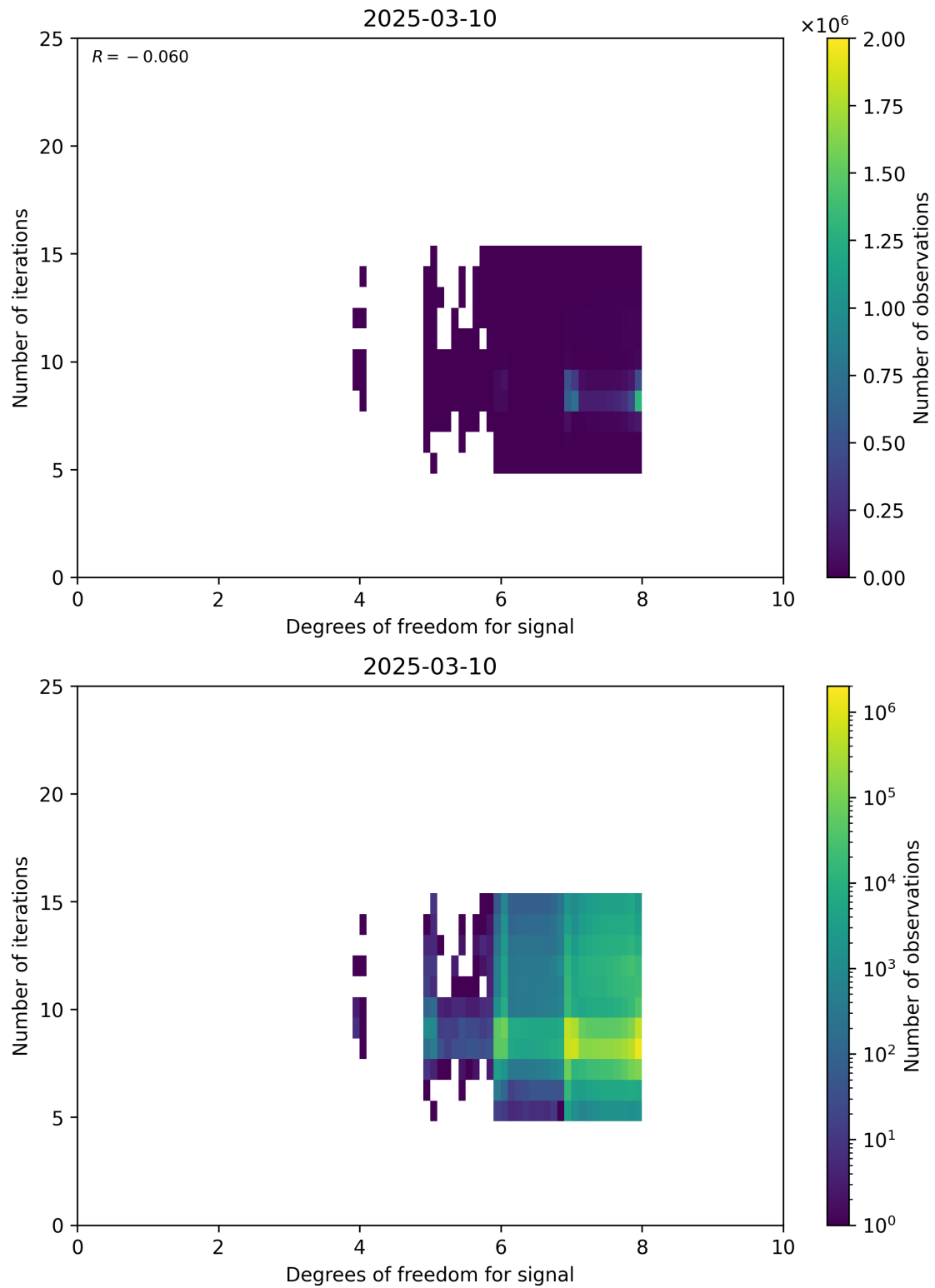
Figure 50: Scatter density plot of “Degrees of freedom for signal” against “Number of iterations” for 2025-03-09 to 2025-03-11.
