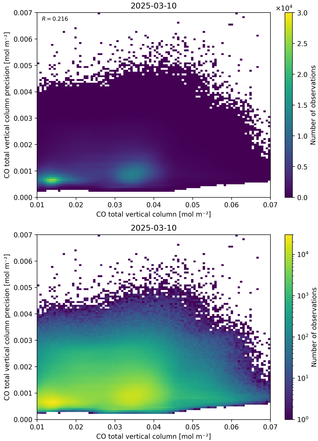
Figure 34: Scatter density plot of “CO total vertical column” against “CO total vertical column precision” for 2025-03-09 to 2025-03-11.
