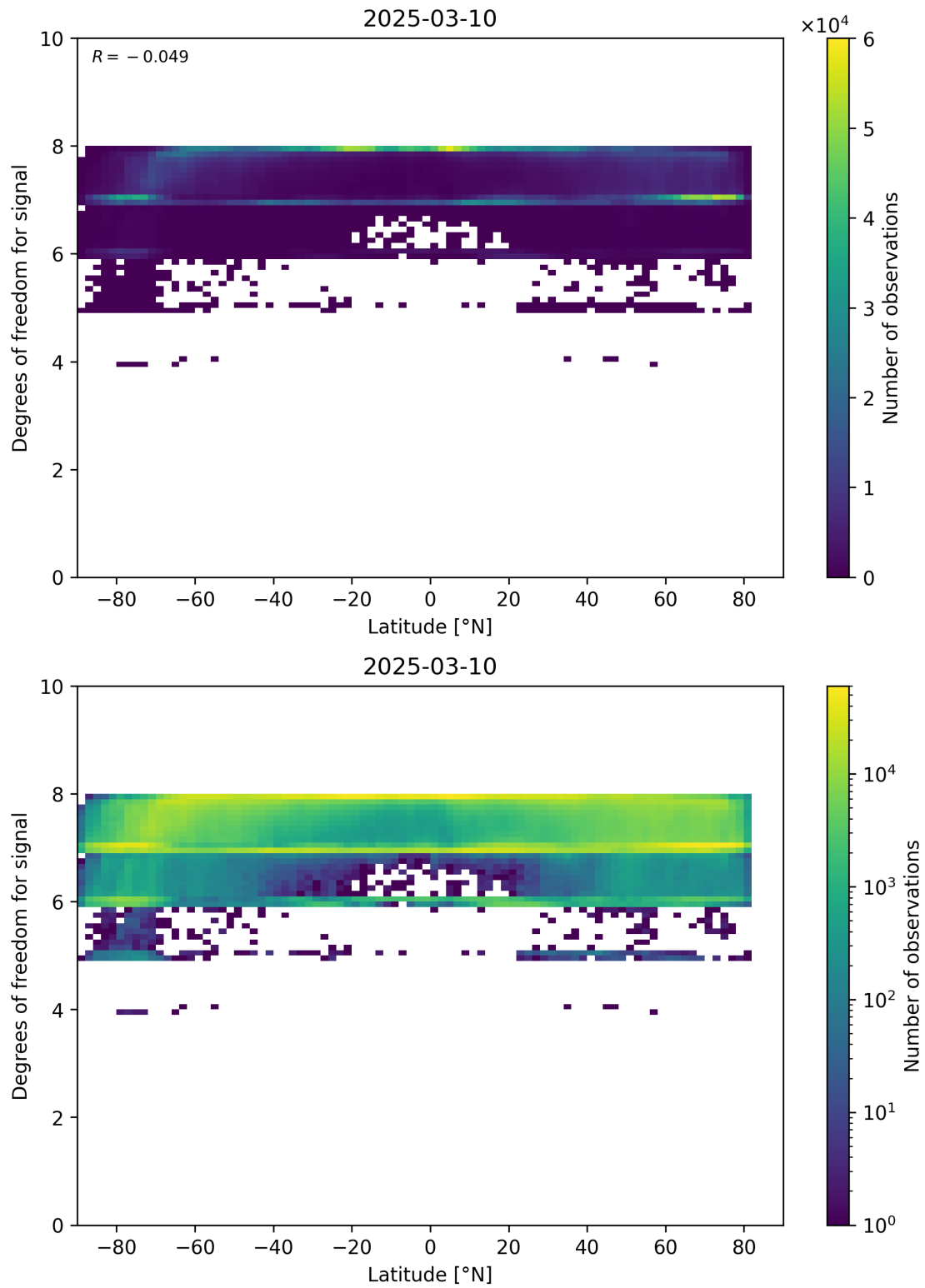
Figure 55: Scatter density plot of “Latitude” against “Degrees of freedom for signal” for 2025-03-09 to 2025-03-11.
