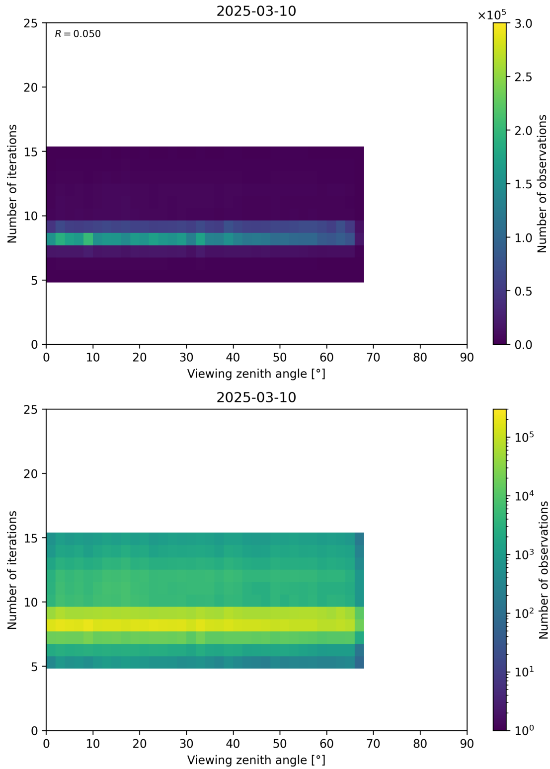
Figure 75: Scatter density plot of “Viewing zenith angle” against “Number of iterations” for 2025-03-09 to 2025-03-11.
