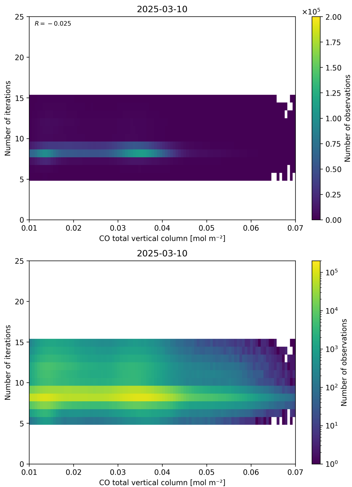
Figure 42: Scatter density plot of “CO total vertical column” against “Number of iterations” for 2025-03-09 to 2025-03-11.
