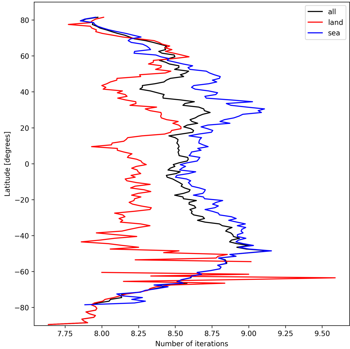
Figure 16: Zonal average of “Number of iterations” for 2025-03-09 to 2025-03-11.
