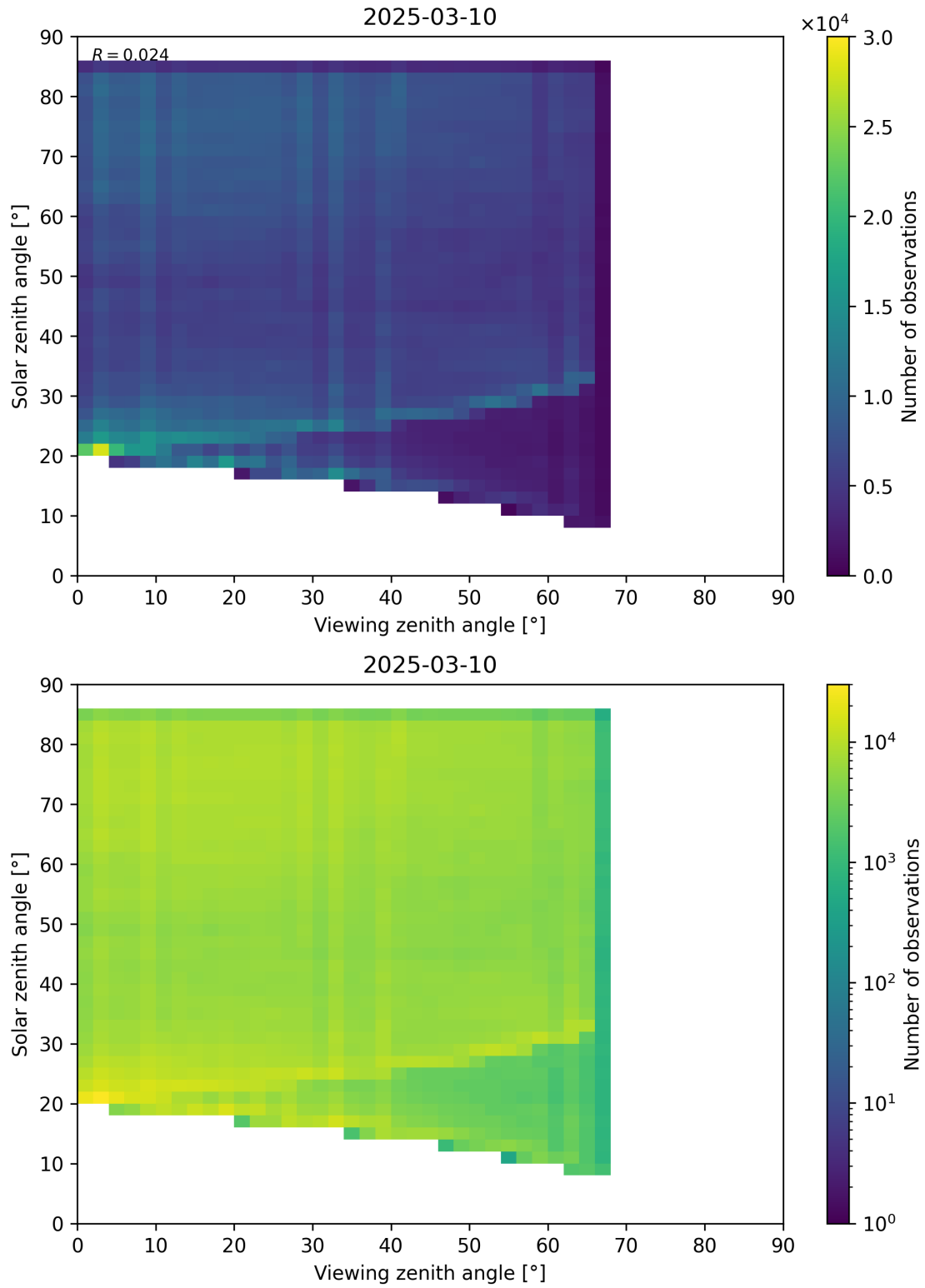
Figure 77: Scatter density plot of “Viewing zenith angle” against “Solar zenith angle” for 2025-03-09 to 2025-03-11.
