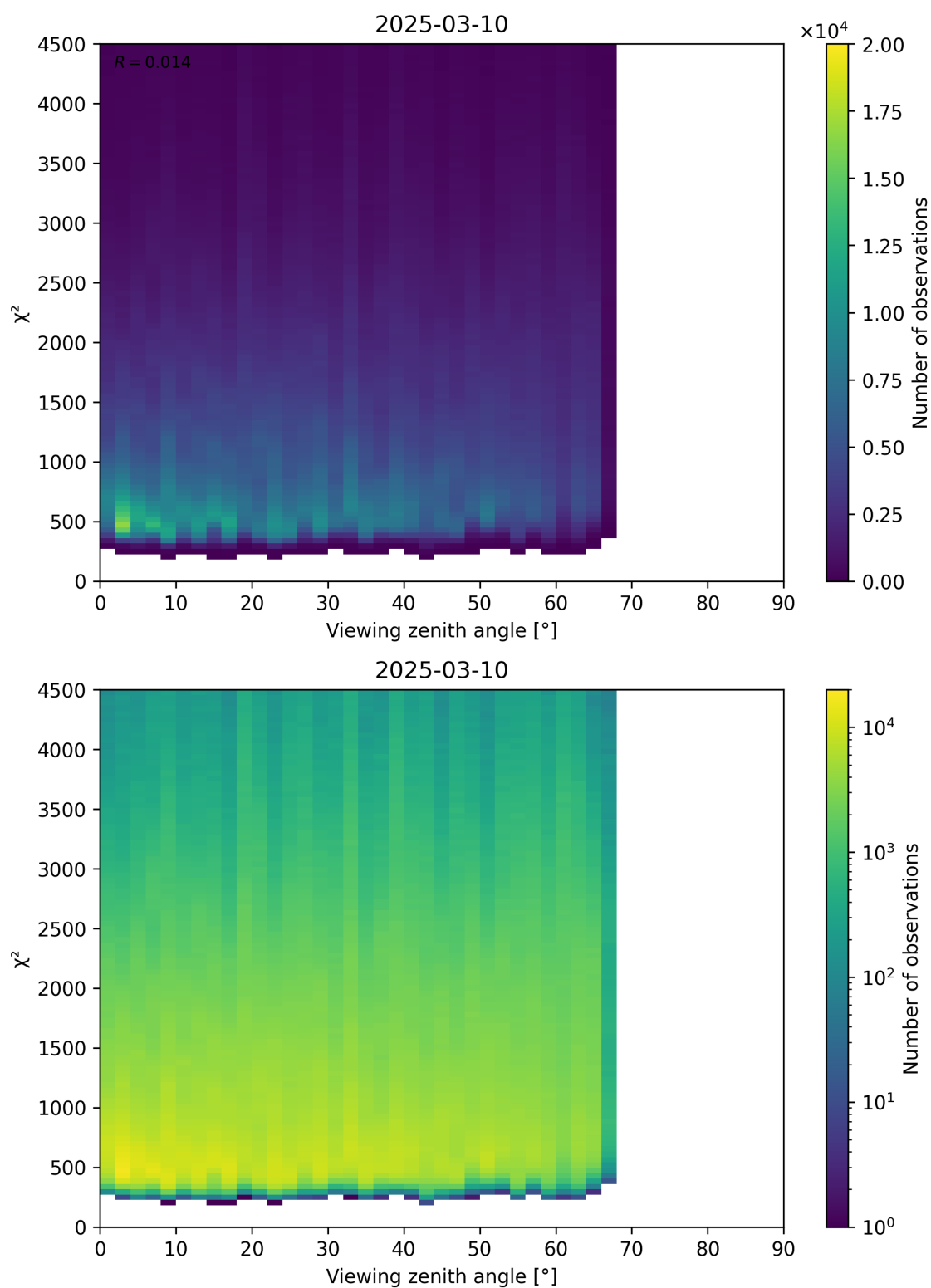
Figure 72: Scatter density plot of “Viewing zenith angle” against “ \chi^2 ” for 2025-03-09 to 2025-03-11.
