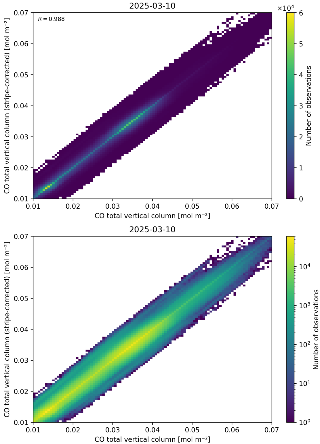
Figure 33: Scatter density plot of “CO total vertical column” against “CO total vertical column (stripe-corrected)” for 2025-03-09 to 2025-03-11.
