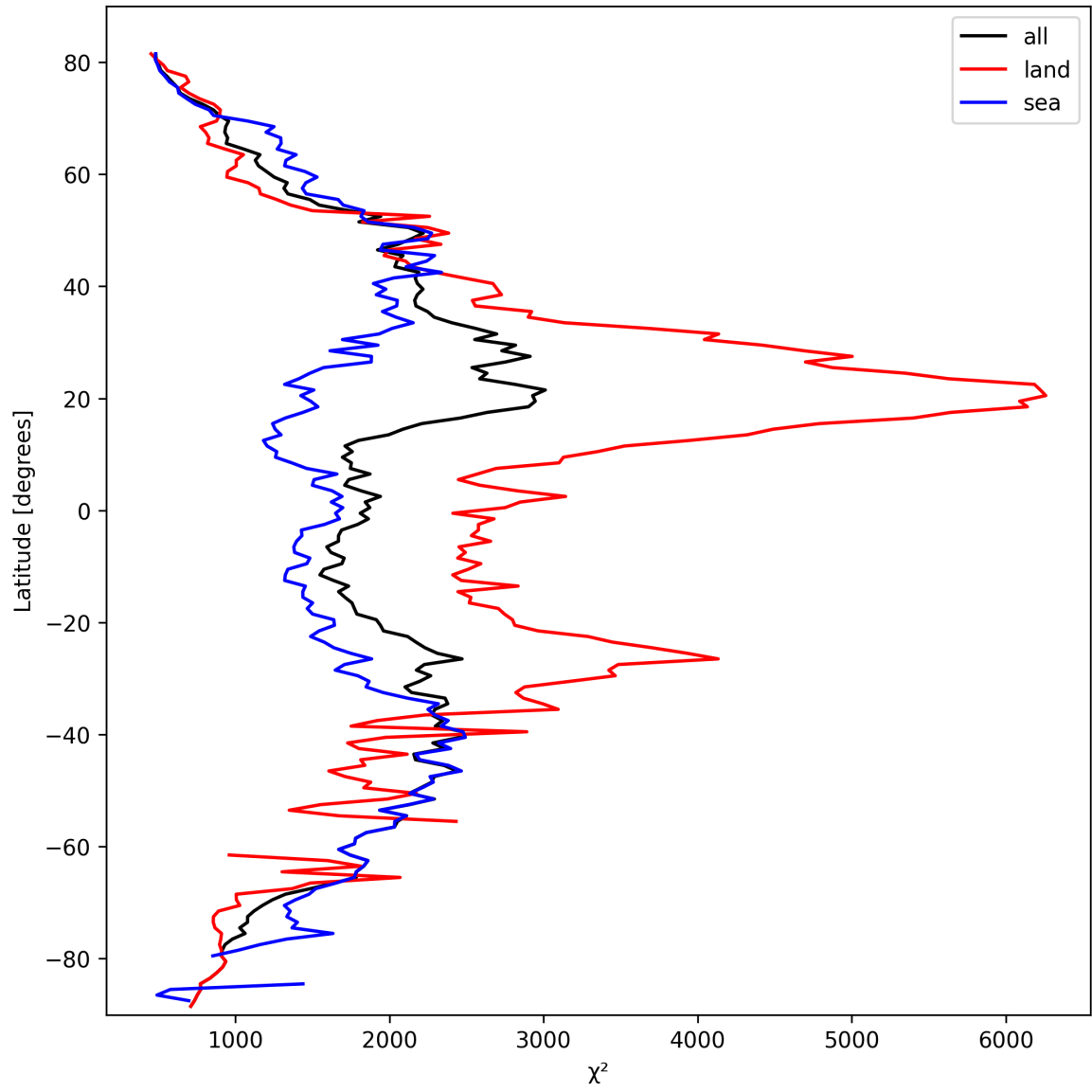
Figure 14: Zonal average of “ \chi^2 ” for 2025-03-10 to 2025-03-12.
