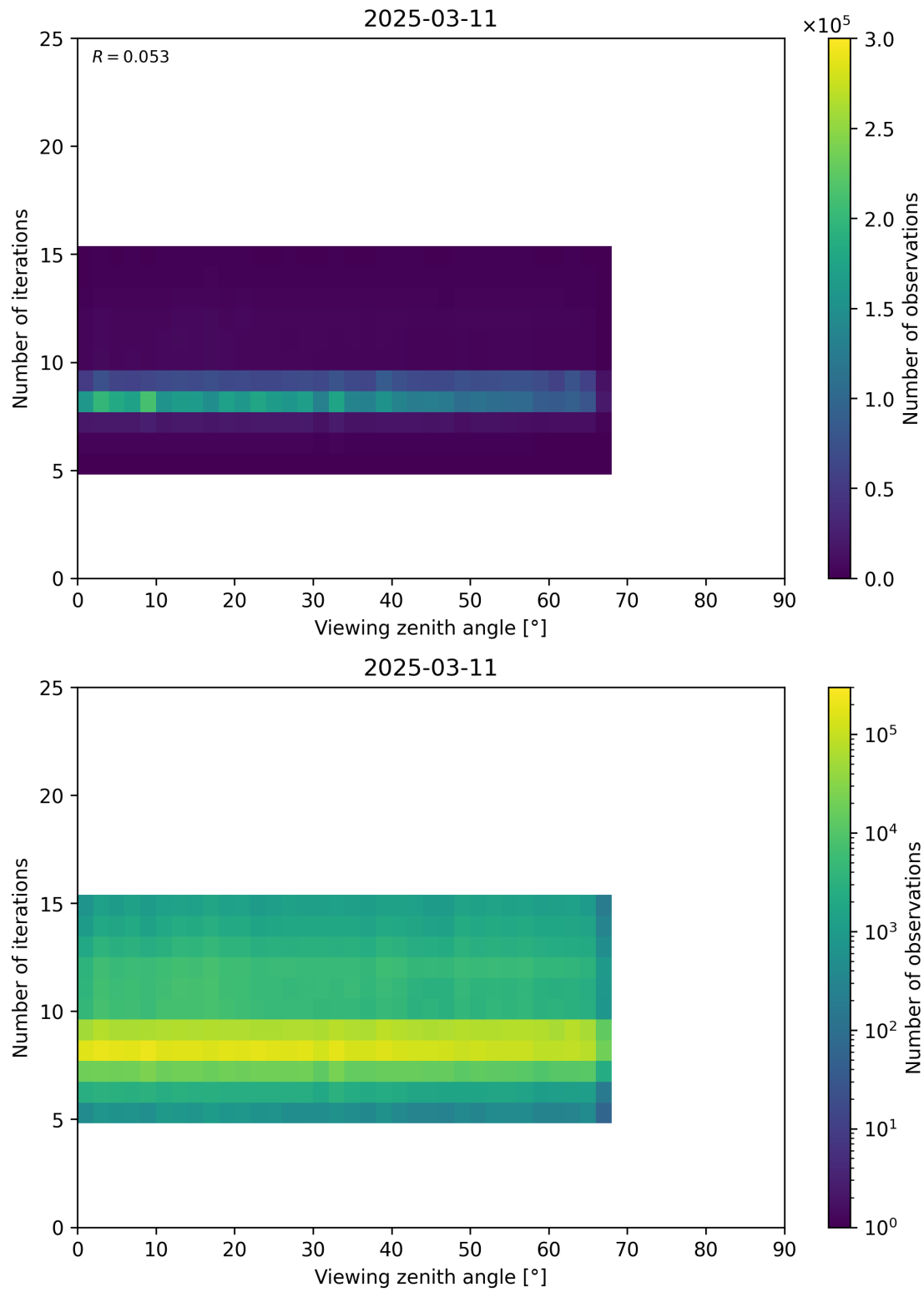
Figure 75: Scatter density plot of “Viewing zenith angle” against “Number of iterations” for 2025-03-10 to 2025-03-12.
