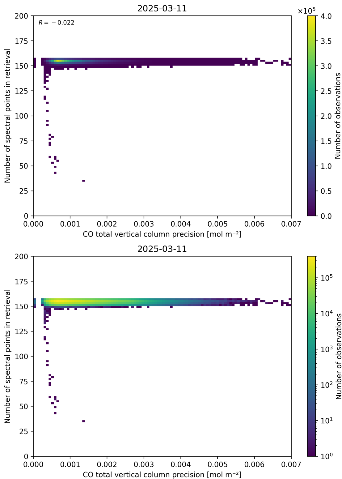
Figure 47: Scatter density plot of “CO total vertical column precision” against “Number of spectral points in retrieval” for 2025-03-10 to 2025-03-12.
