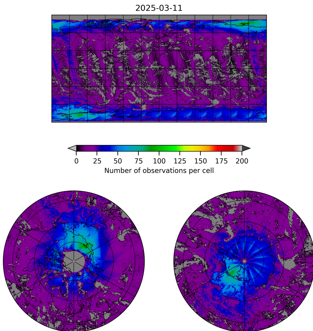
Figure 8: Map of the number of observations for 2025-03-10 to 2025-03-12
