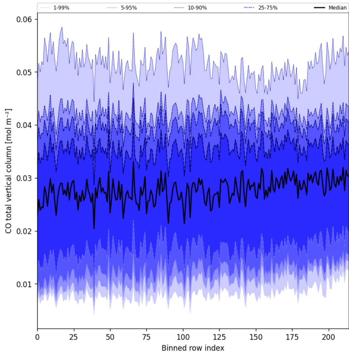
Figure 26: Along track statistics of "CO total vertical column" for 2025-03-10 to 2025-03-12
