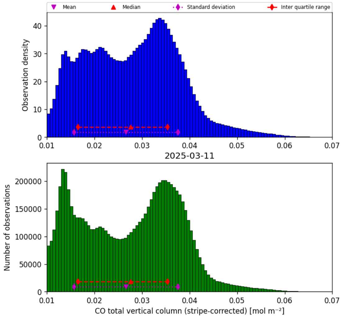
Figure 19: Histogram of “CO total vertical column (stripe-corrected)” for 2025-03-10 to 2025-03-12
