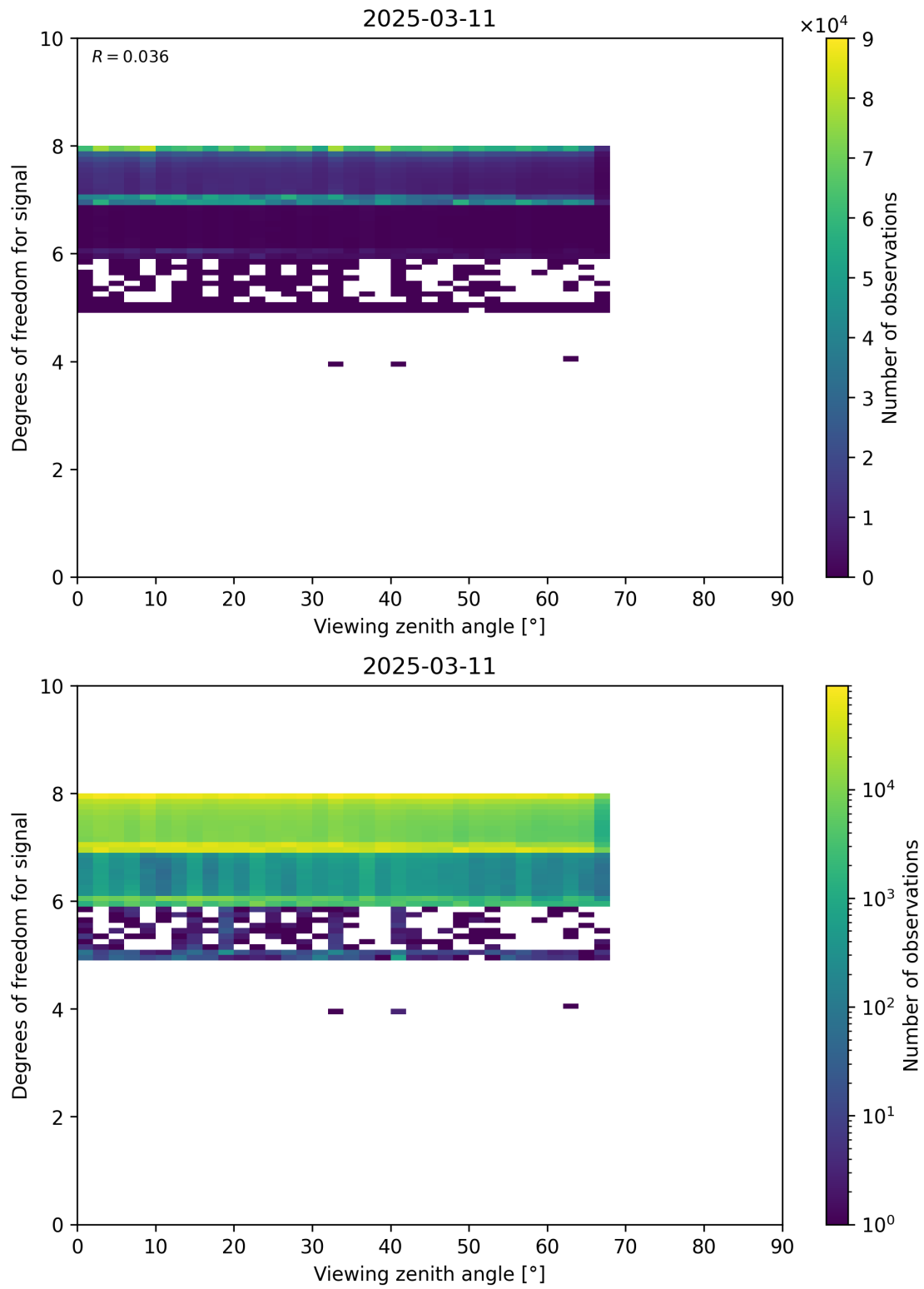
Figure 73: Scatter density plot of “Viewing zenith angle” against “Degrees of freedom for signal” for 2025-03-10 to 2025-03-12.
