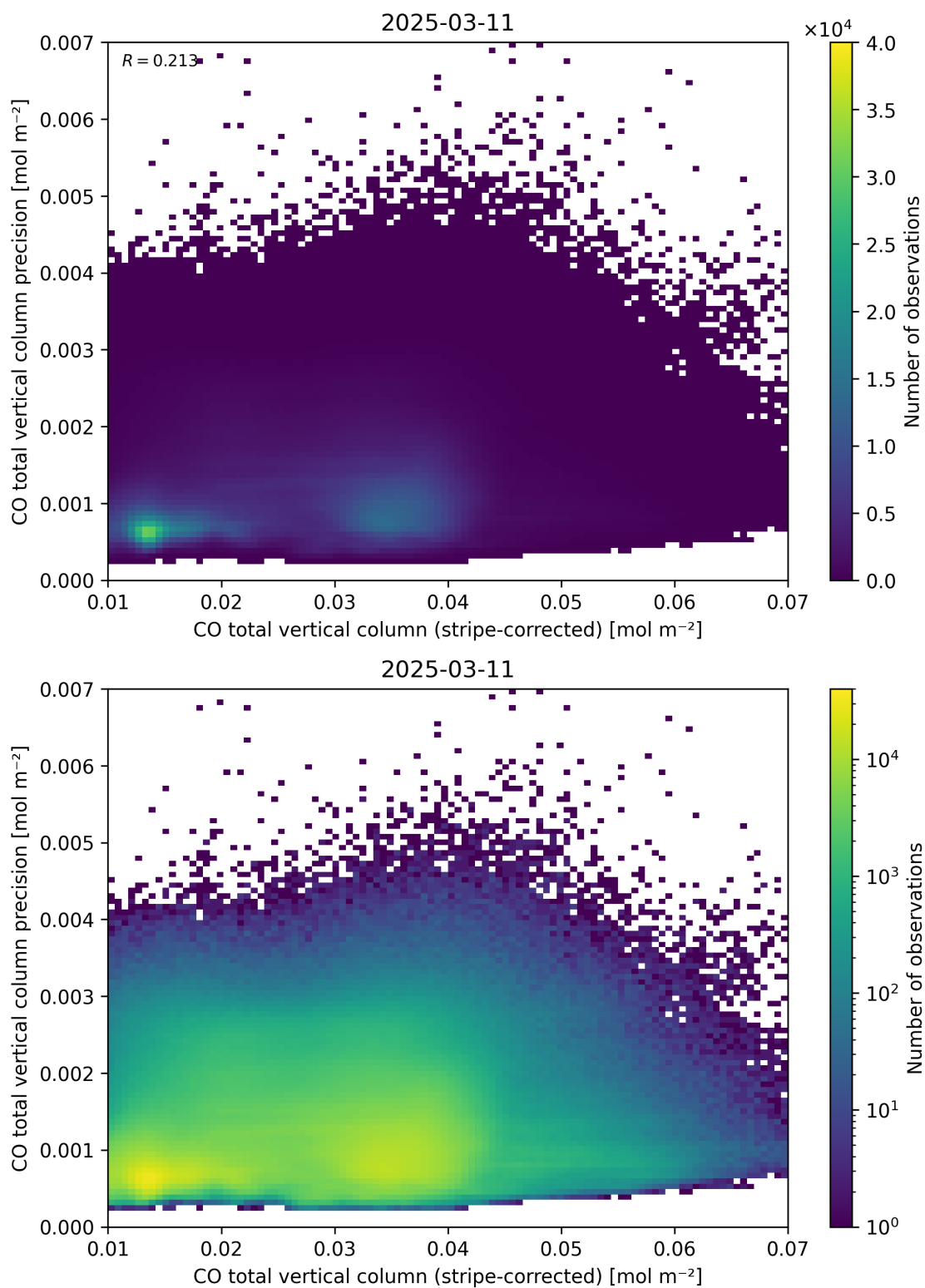
Figure 36: Scatter density plot of “CO total vertical column (stripe-corrected)” against “CO total vertical column precision” for 2025-03-10 to 2025-03-12.
