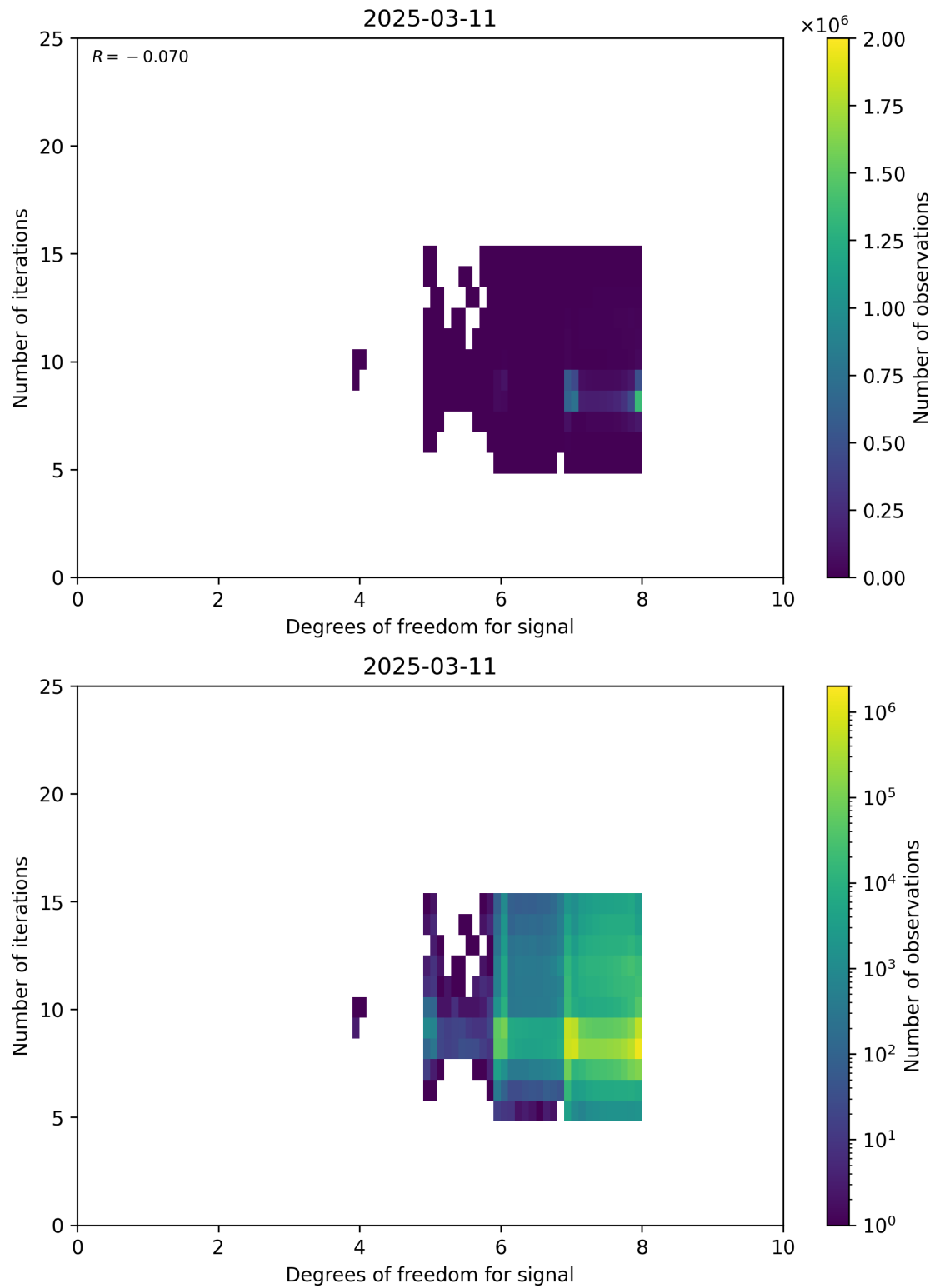
Figure 50: Scatter density plot of “Degrees of freedom for signal” against “Number of iterations” for 2025-03-10 to 2025-03-12.
