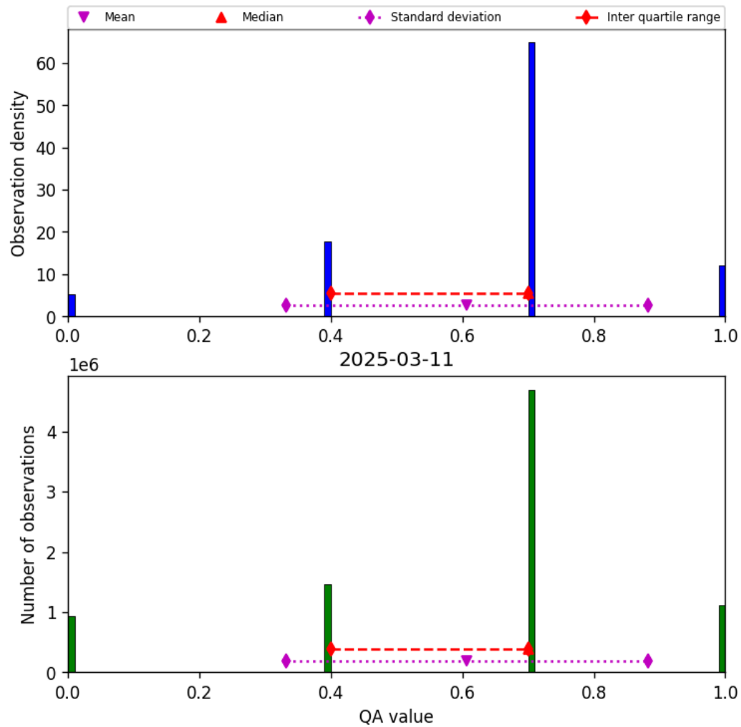
Figure 17: Histogram of “QA value” for 2025-03-10 to 2025-03-12
