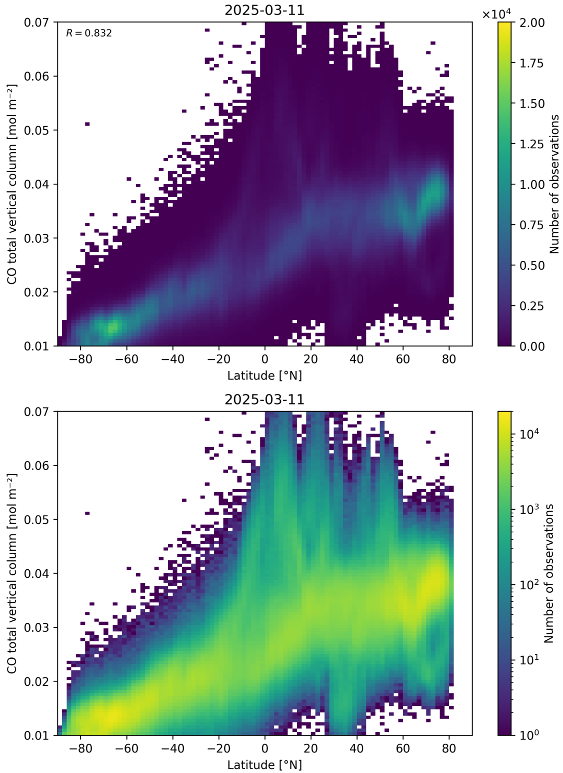
Figure 51: Scatter density plot of “Latitude” against “CO total vertical column” for 2025-03-10 to 2025-03-12.
