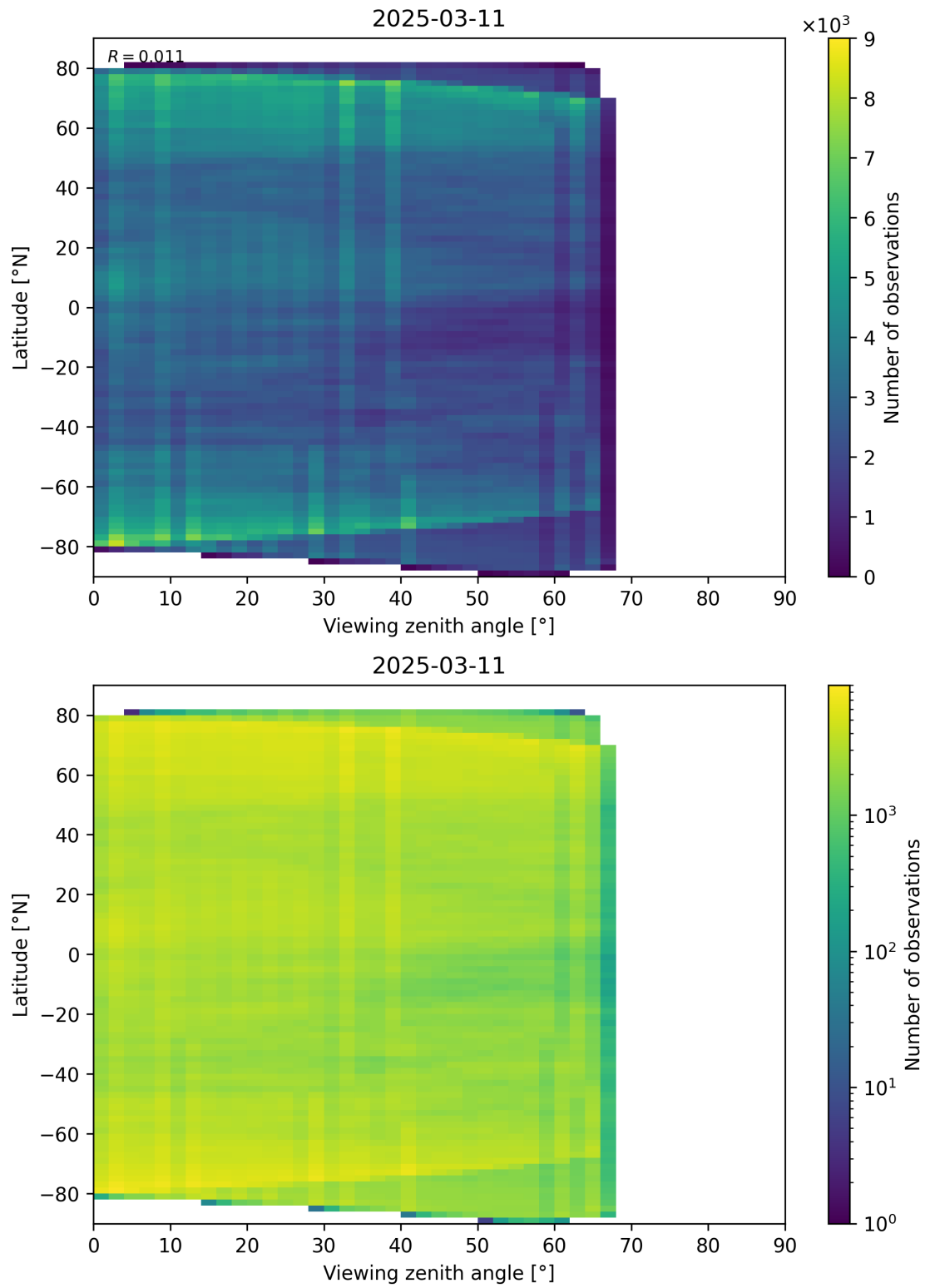
Figure 74: Scatter density plot of “Viewing zenith angle” against “Latitude” for 2025-03-10 to 2025-03-12.
