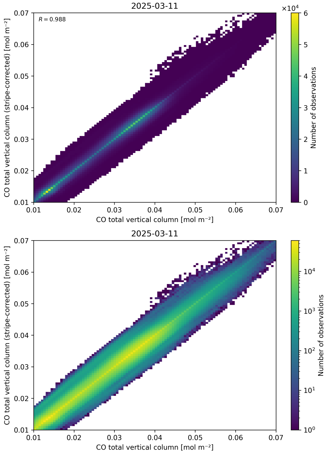
Figure 33: Scatter density plot of “CO total vertical column” against “CO total vertical column (stripe-corrected)” for 2025-03-10 to 2025-03-12.
