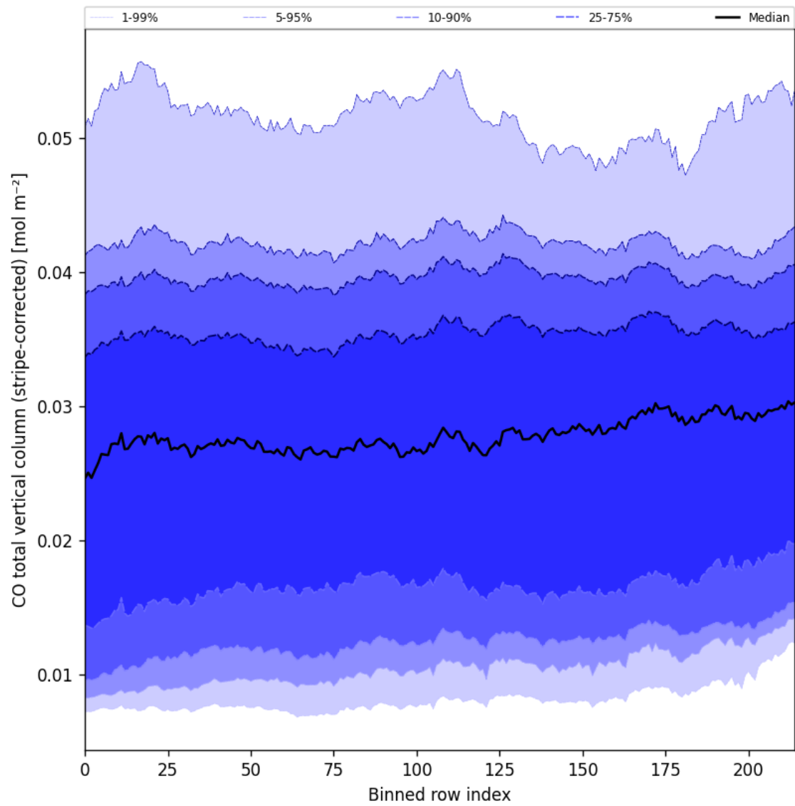
Figure 27: Along track statistics of “CO total vertical column (stripe-corrected)” for 2025-03-10 to 2025-03-12
