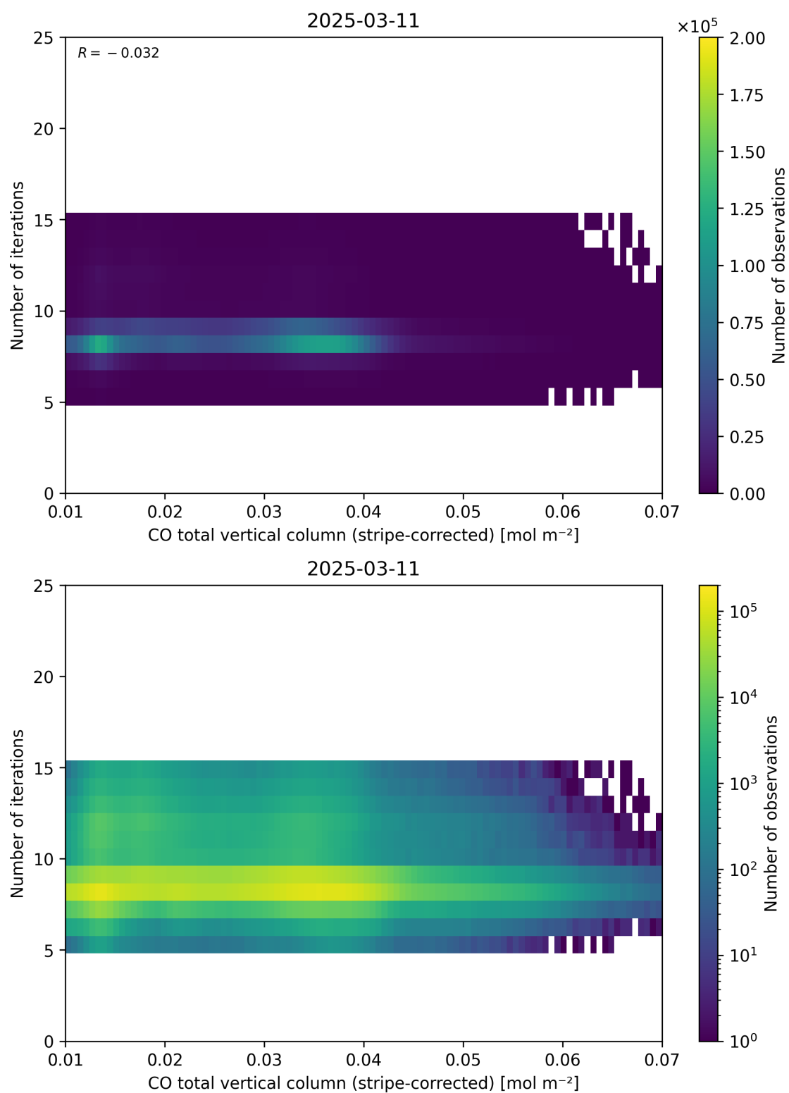
Figure 39: Scatter density plot of “CO total vertical column (stripe-corrected)” against “Number of iterations” for 2025-03-10 to 2025-03-12.
