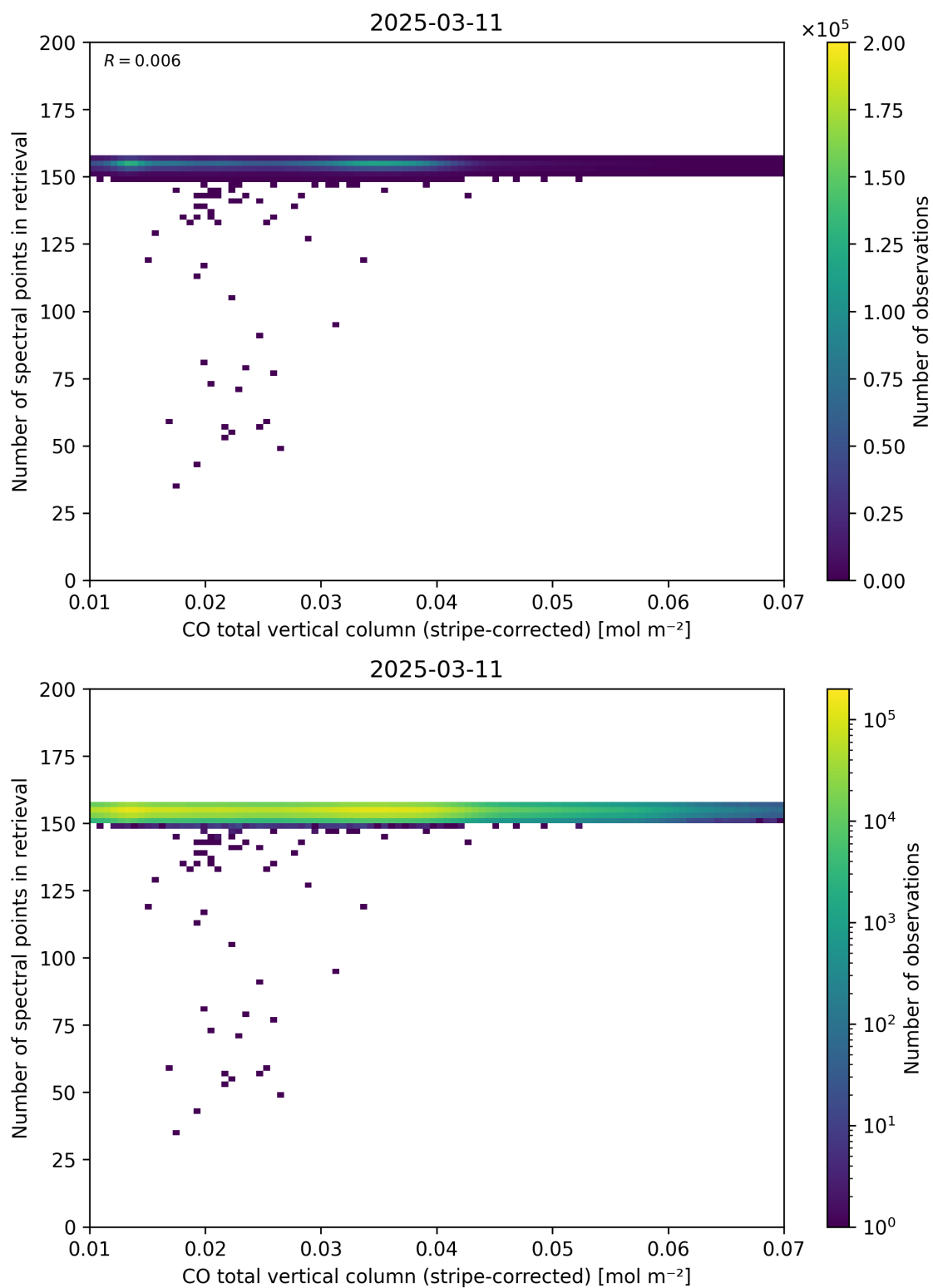
Figure 40: Scatter density plot of “CO total vertical column (stripe-corrected)” against “Number of spectral points in retrieval” for 2025-03-10 to 2025-03-12.
