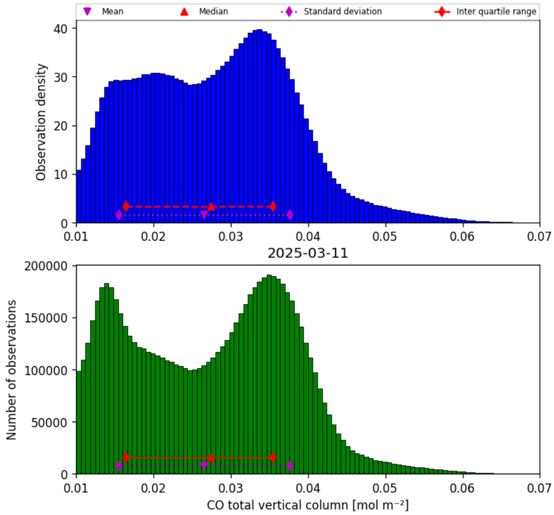
Figure 18: Histogram of “CO total vertical column” for 2025-03-10 to 2025-03-12
