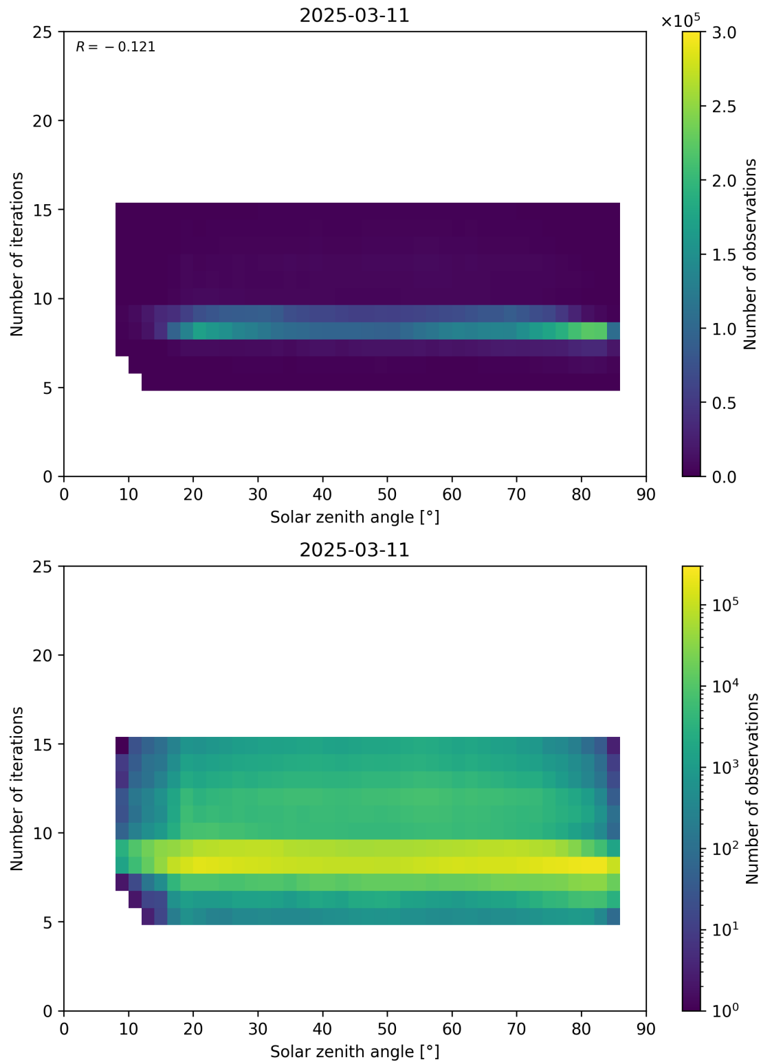
Figure 67: Scatter density plot of “Solar zenith angle” against “Number of iterations” for 2025-03-10 to 2025-03-12.
