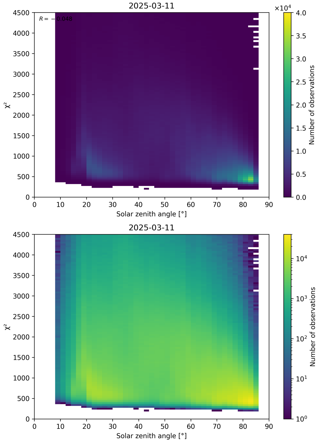
Figure 64: Scatter density plot of “Solar zenith angle” against “ \chi^2 ” for 2025-03-10 to 2025-03-12.
