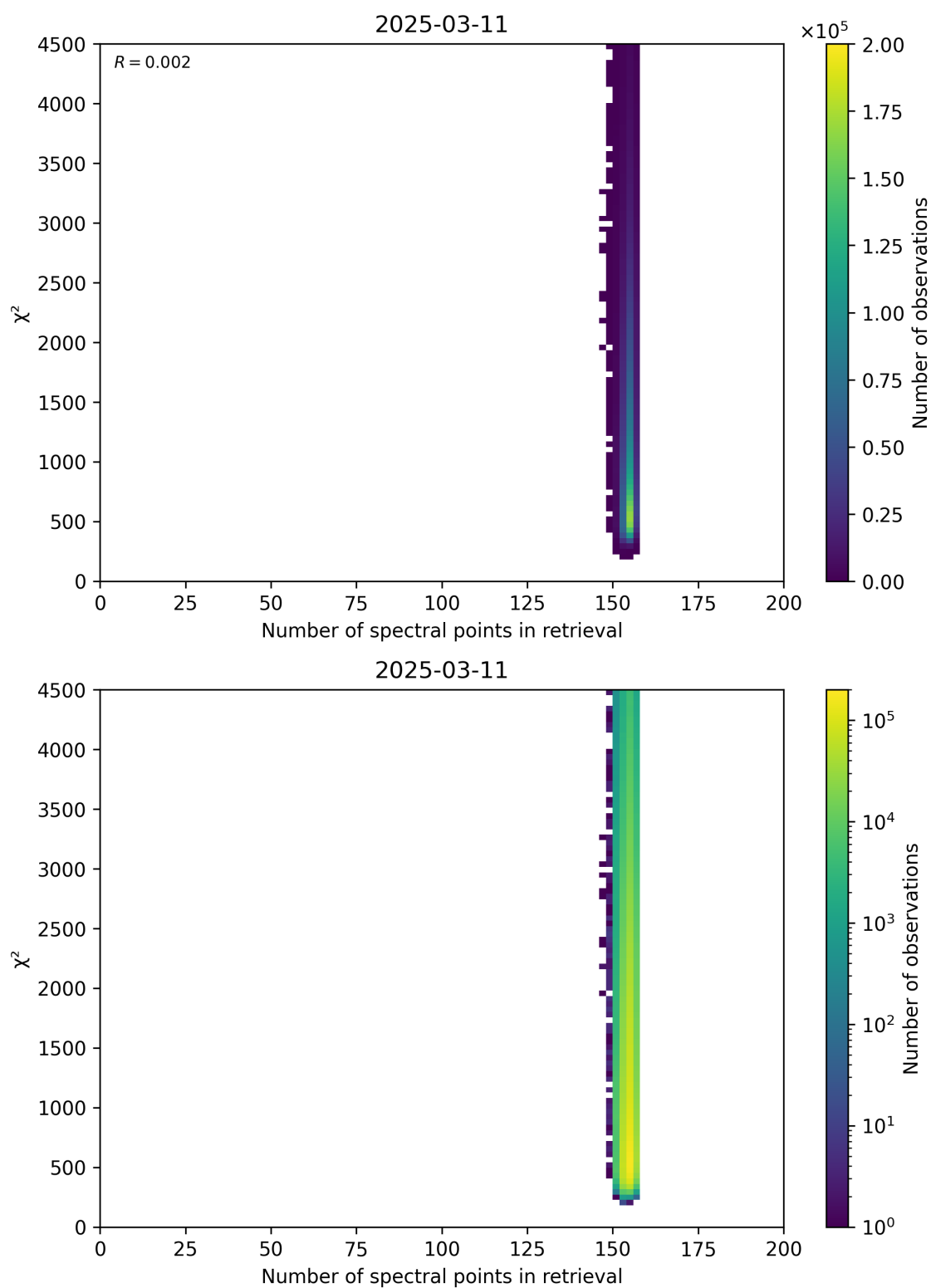
Figure 58: Scatter density plot of “Number of spectral points in retrieval” against “ \chi^2 ” for 2025-03-10 to 2025-03-12.
