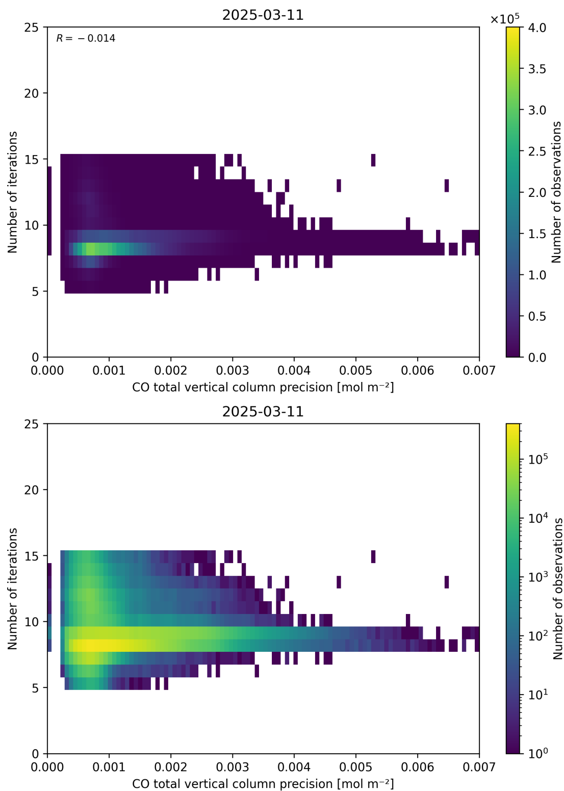
Figure 46: Scatter density plot of “CO total vertical column precision” against “Number of iterations” for 2025-03-10 to 2025-03-12.
