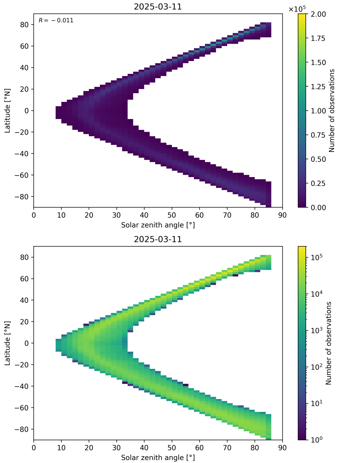
Figure 66: Scatter density plot of “Solar zenith angle” against “Latitude” for 2025-03-10 to 2025-03-12.
