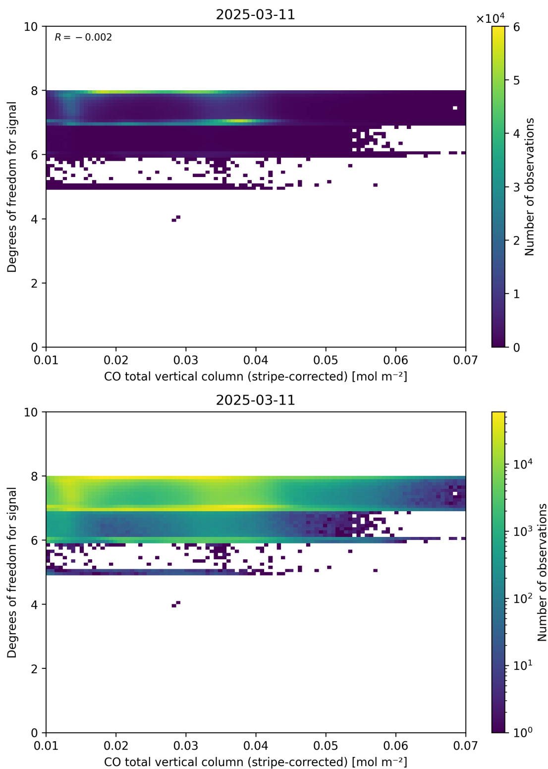
Figure 38: Scatter density plot of “CO total vertical column (stripe-corrected)” against “Degrees of freedom for signal” for 2025-03-10 to 2025-03-12.
