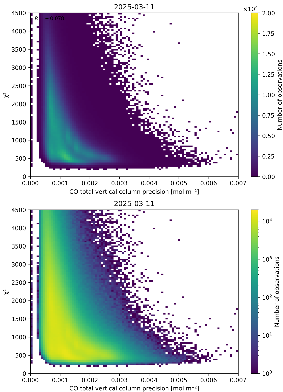
Figure 44: Scatter density plot of “CO total vertical column precision” against “ \chi^2 ” for 2025-03-10 to 2025-03-12.
