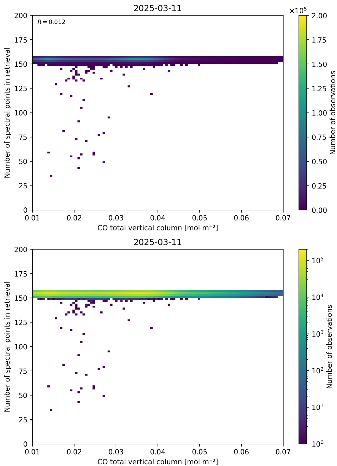
Figure 43: Scatter density plot of “CO total vertical column” against “Number of spectral points in retrieval” for 2025-03-10 to 2025-03-12.
