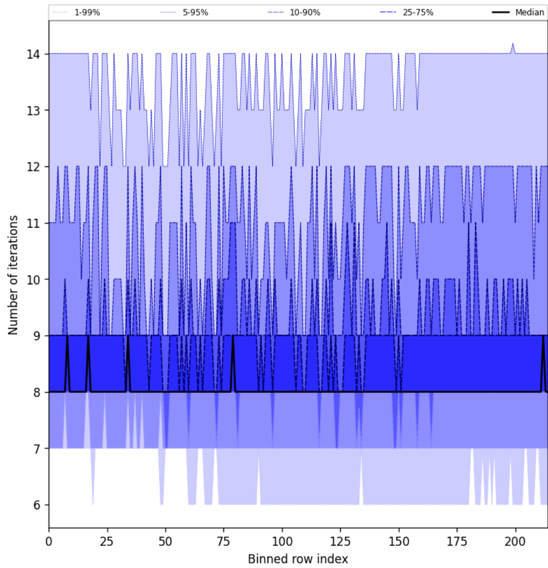
Figure 32: Along track statistics of “Number of iterations” for 2025-03-10 to 2025-03-12
