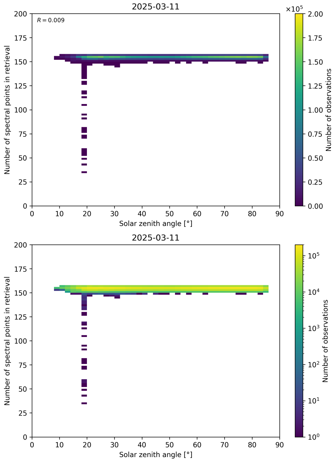
Figure 68: Scatter density plot of “Solar zenith angle” against “Number of spectral points in retrieval” for 2025-03-10 to 2025-03-12.
