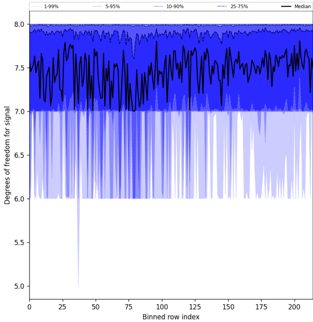
Figure 31: Along track statistics of “Degrees of freedom for signal” for 2025-03-10 to 2025-03-12
