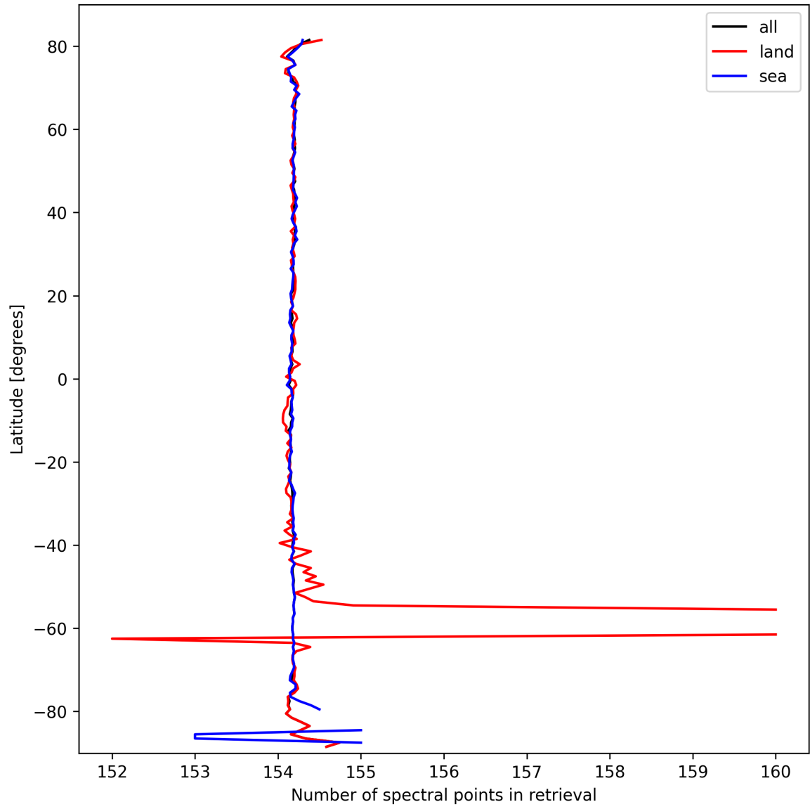
Figure 13: Zonal average of “Number of spectral points in retrieval” for 2025-03-10 to 2025-03-12.
