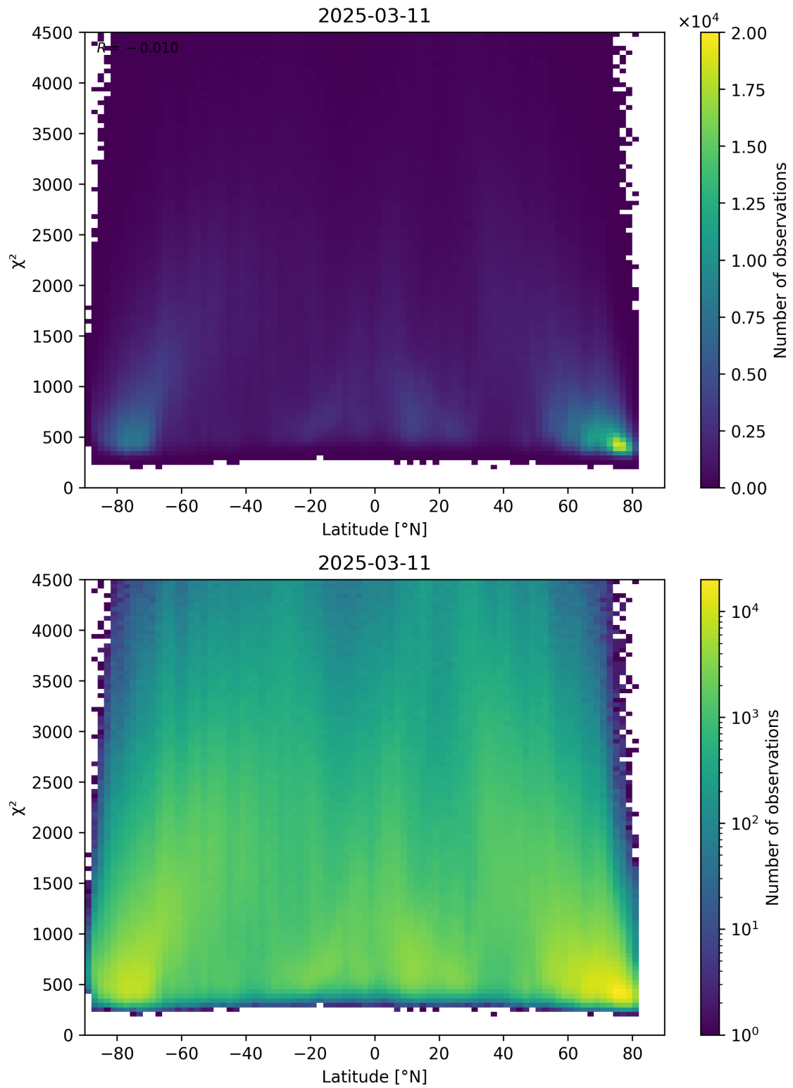
Figure 54: Scatter density plot of “Latitude” against “ \chi^2 ” for 2025-03-10 to 2025-03-12.
