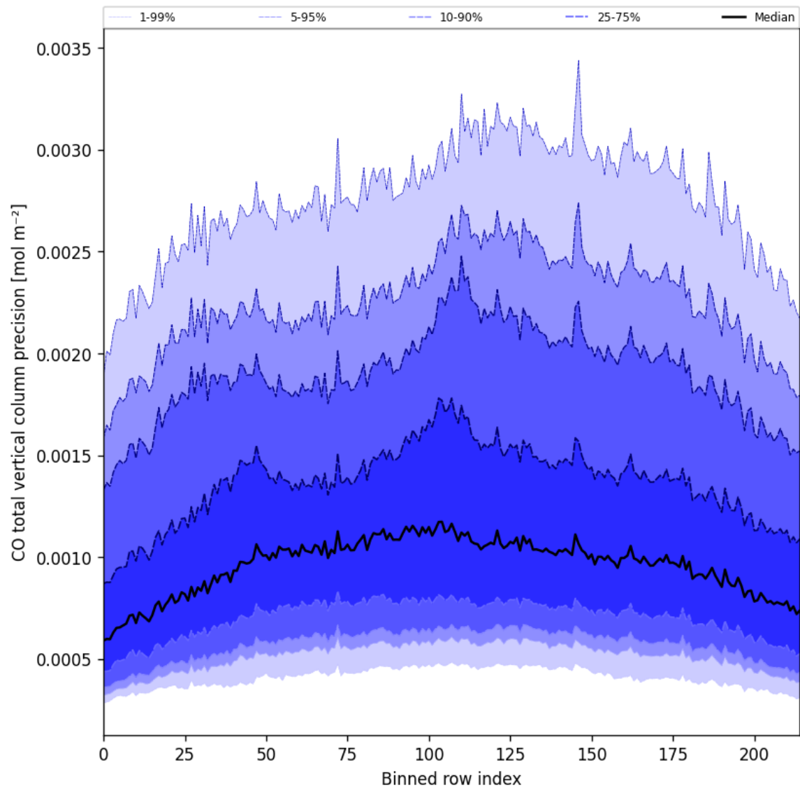
Figure 28: Along track statistics of “CO total vertical column precision” for 2025-03-10 to 2025-03-12
