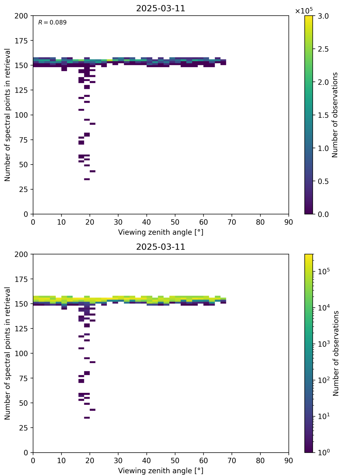
Figure 76: Scatter density plot of “Viewing zenith angle” against “Number of spectral points in retrieval” for 2025-03-10 to 2025-03-12.
