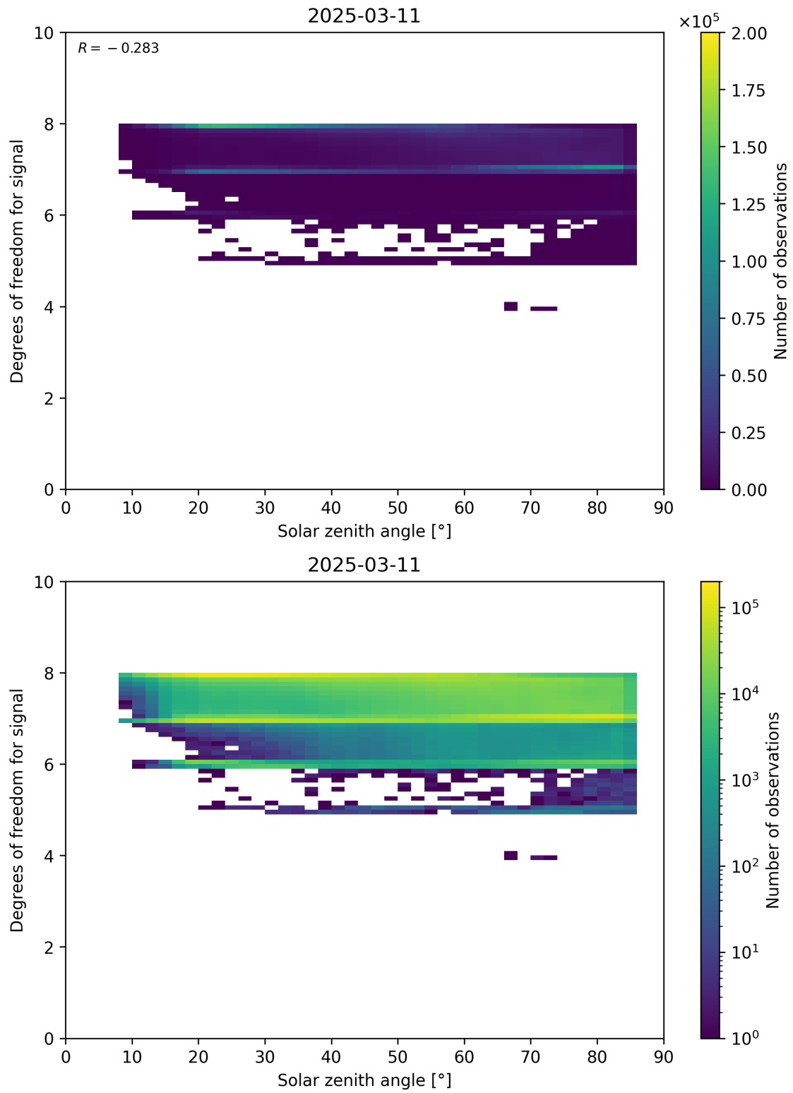
Figure 65: Scatter density plot of “Solar zenith angle” against “Degrees of freedom for signal” for 2025-03-10 to 2025-03-12.
