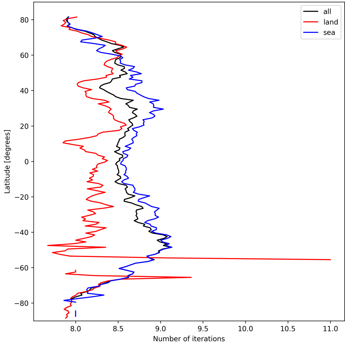
Figure 16: Zonal average of “Number of iterations” for 2025-03-10 to 2025-03-12.
