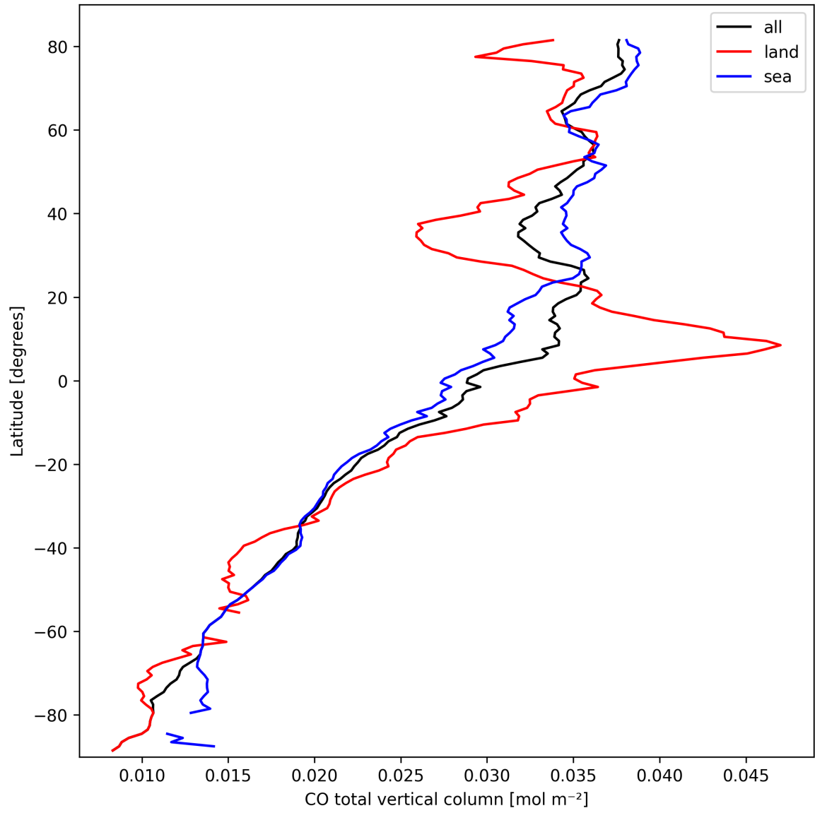
Figure 10: Zonal average of “CO total vertical column” for 2025-03-10 to 2025-03-12.
