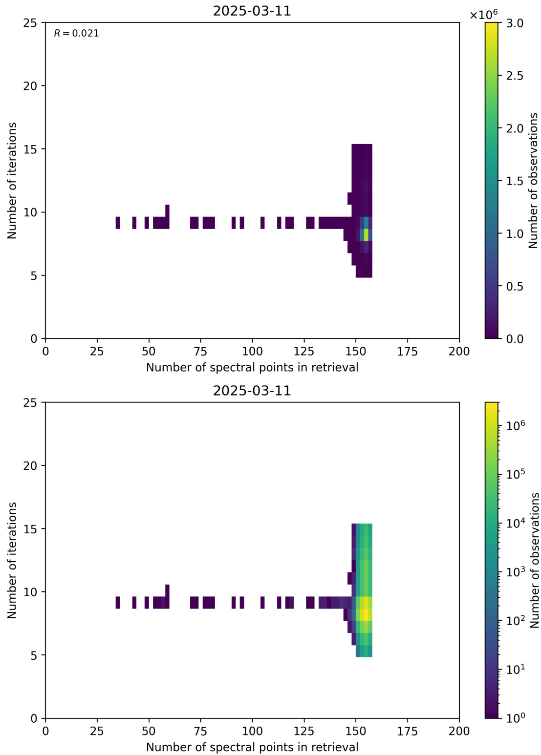
Figure 60: Scatter density plot of “Number of spectral points in retrieval” against “Number of iterations” for 2025-03-10 to 2025-03-12.
