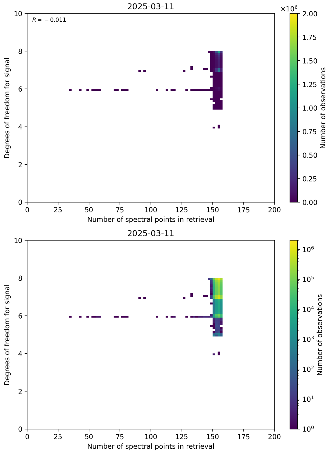
Figure 59: Scatter density plot of “Number of spectral points in retrieval” against “Degrees of freedom for signal” for 2025-03-10 to 2025-03-12.
