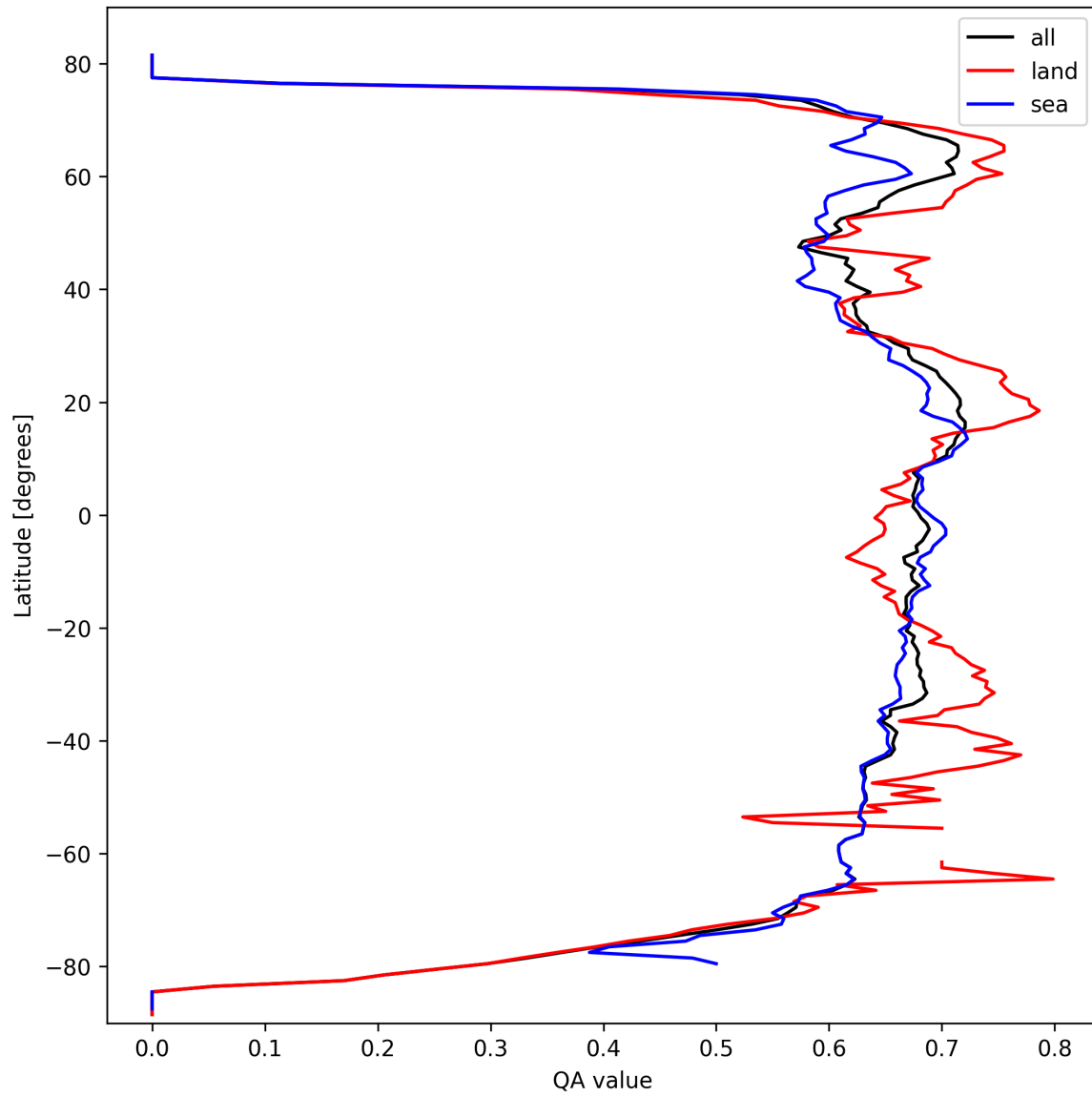
Figure 9: Zonal average of “QA value” for 2025-03-10 to 2025-03-12.
