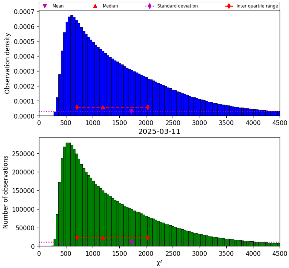
Figure 22: Histogram of “ \chi^2 ” for 2025-03-10 to 2025-03-12
