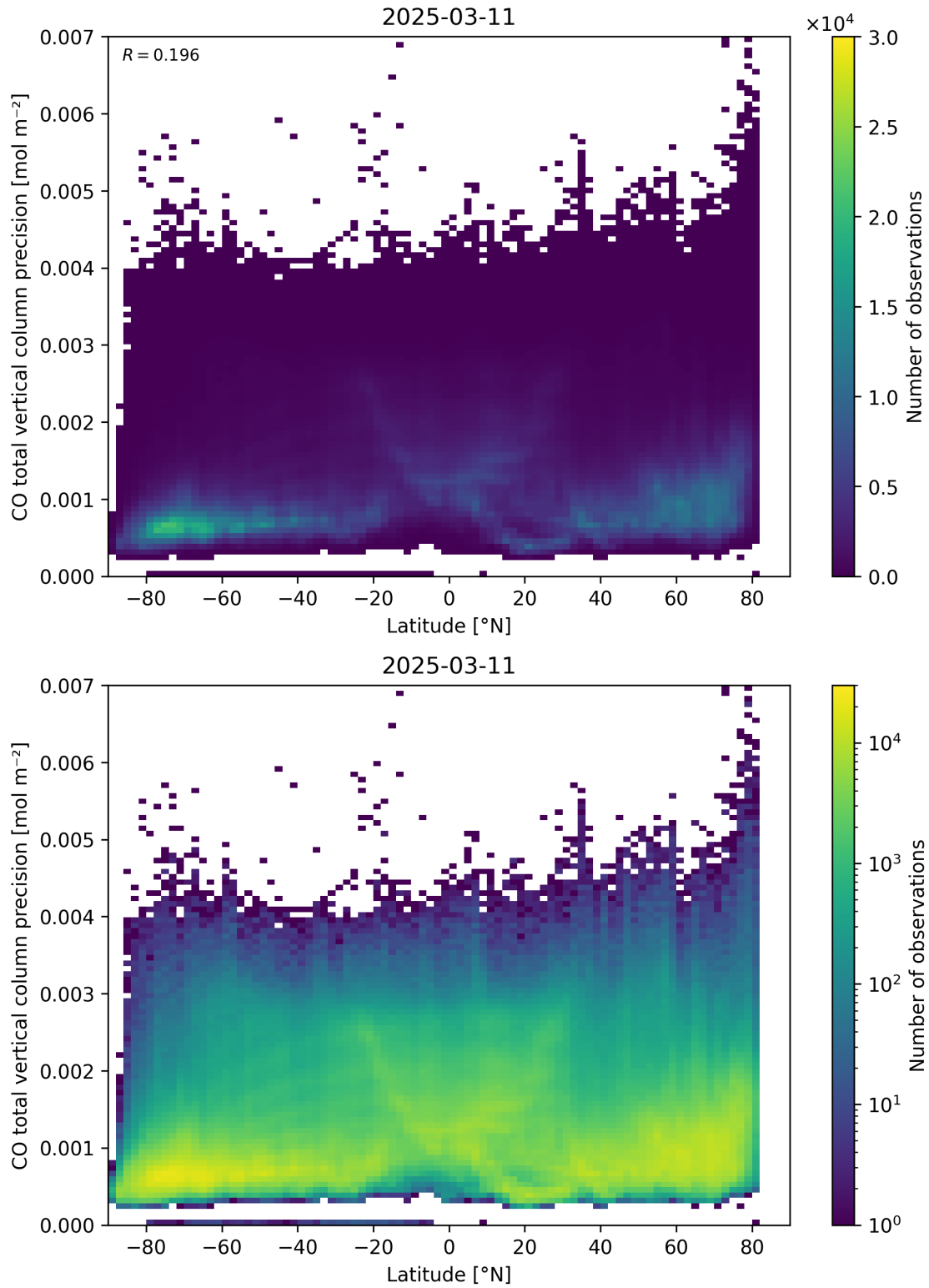
Figure 53: Scatter density plot of “Latitude” against “CO total vertical column precision” for 2025-03-10 to 2025-03-12.
