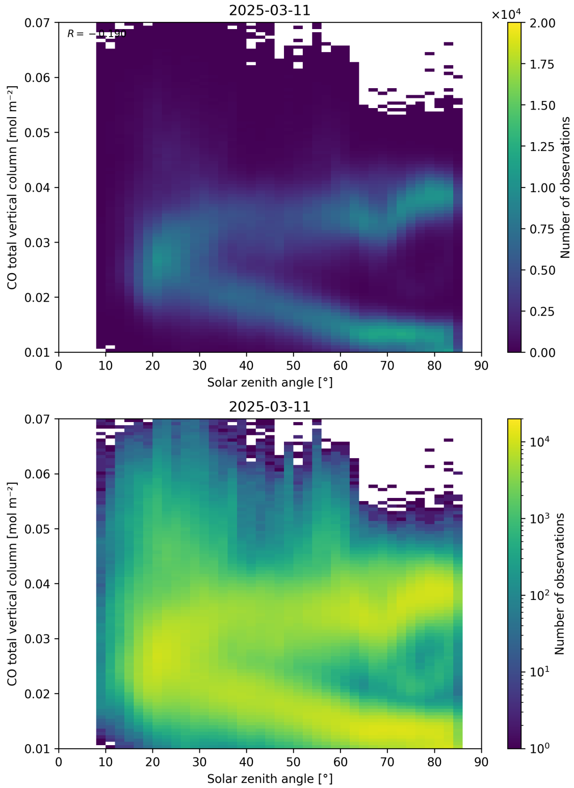
Figure 61: Scatter density plot of “Solar zenith angle” against “CO total vertical column” for 2025-03-10 to 2025-03-12.
