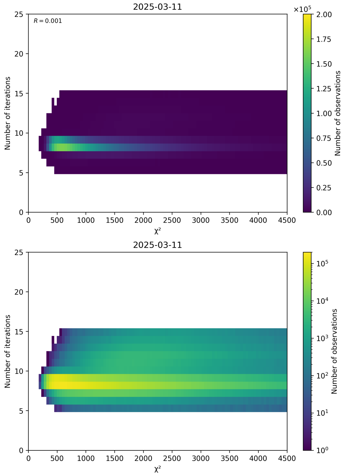
Figure 49: Scatter density plot of “ \chi^2 ” against “Number of iterations” for 2025-03-10 to 2025-03-12.
