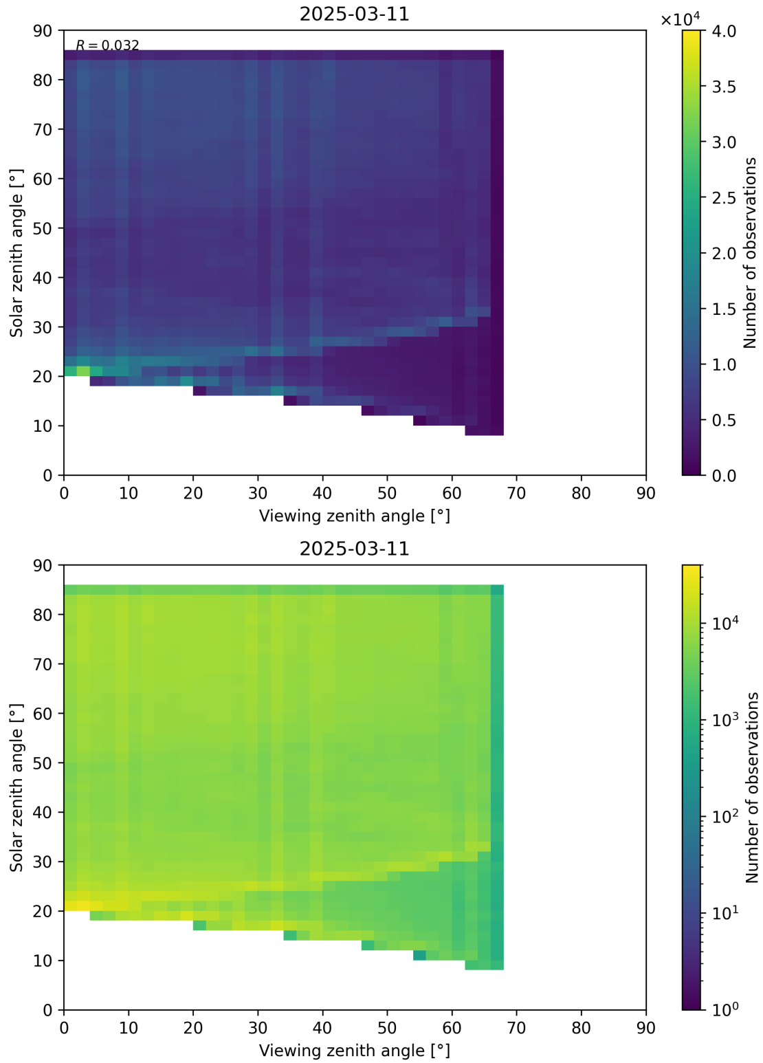
Figure 77: Scatter density plot of “Viewing zenith angle” against “Solar zenith angle” for 2025-03-10 to 2025-03-12.
