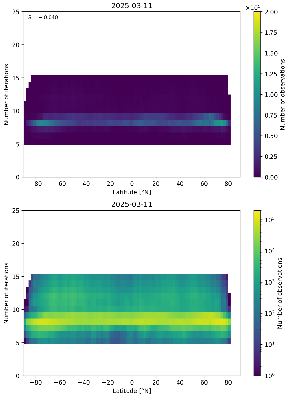
Figure 56: Scatter density plot of “Latitude” against “Number of iterations” for 2025-03-10 to 2025-03-12.
