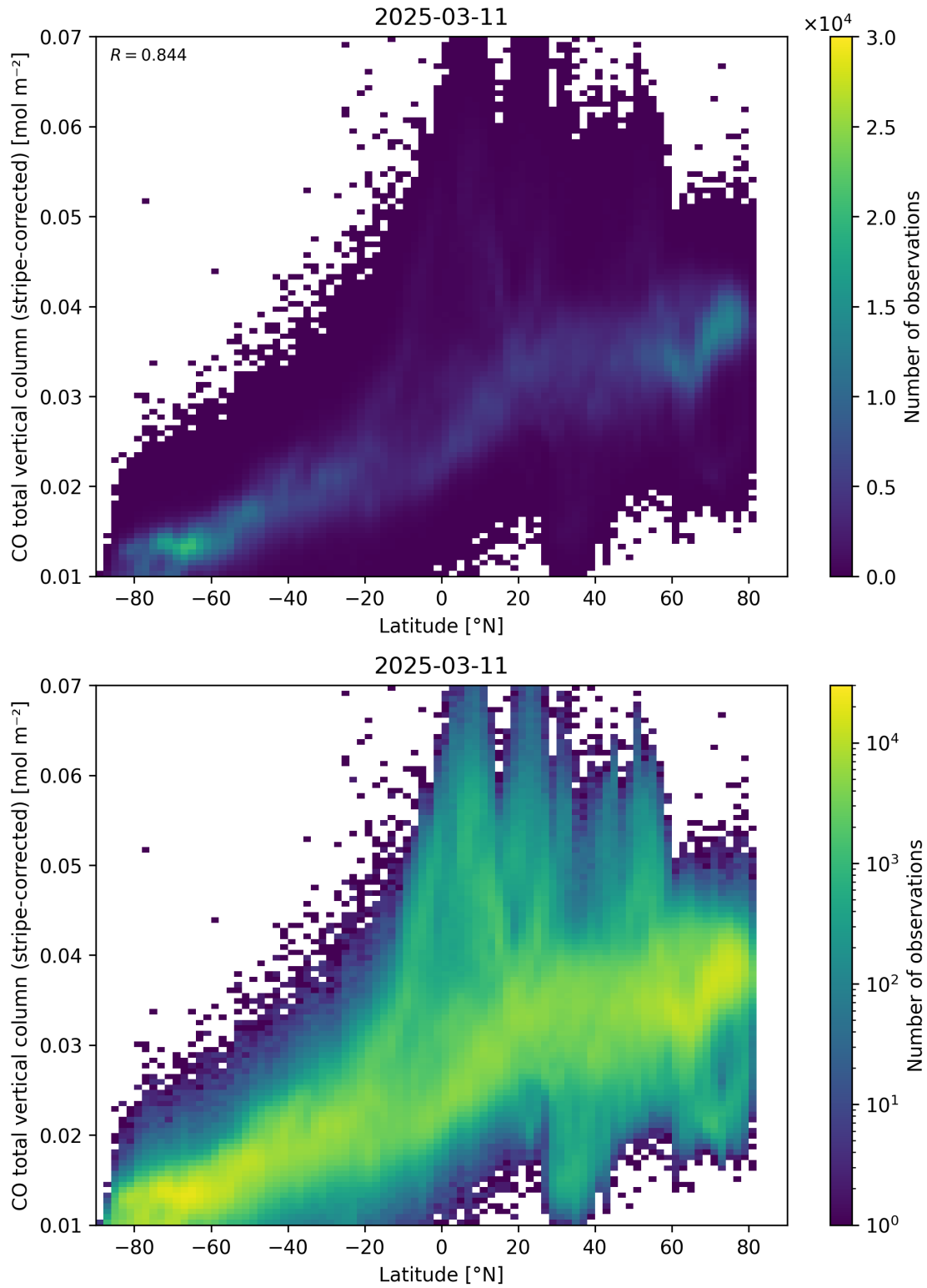
Figure 52: Scatter density plot of “Latitude” against “CO total vertical column (stripe-corrected)” for 2025-03-10 to 2025-03-12.
