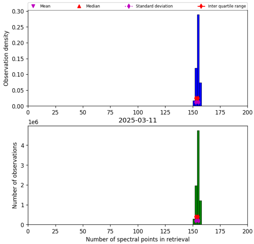
Figure 21: Histogram of “Number of spectral points in retrieval” for 2025-03-10 to 2025-03-12
