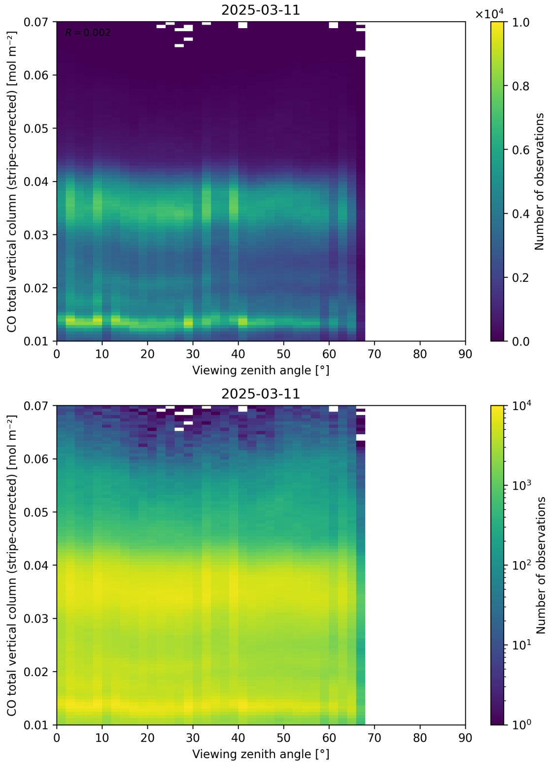
Figure 70: Scatter density plot of “Viewing zenith angle” against “CO total vertical column (stripe-corrected)” for 2025-03-10 to 2025-03-12.
