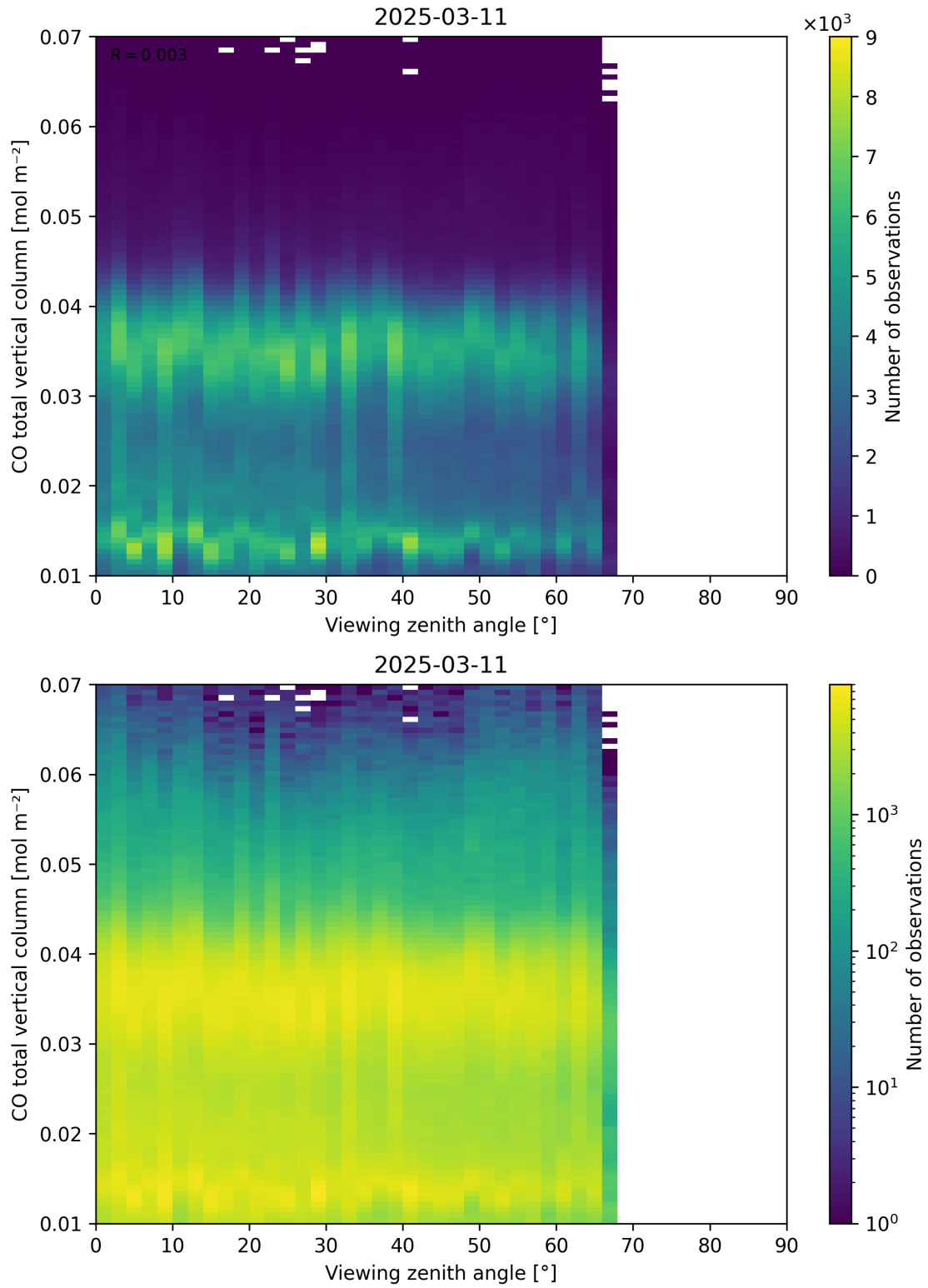
Figure 69: Scatter density plot of “Viewing zenith angle” against “CO total vertical column” for 2025-03-10 to 2025-03-12.
