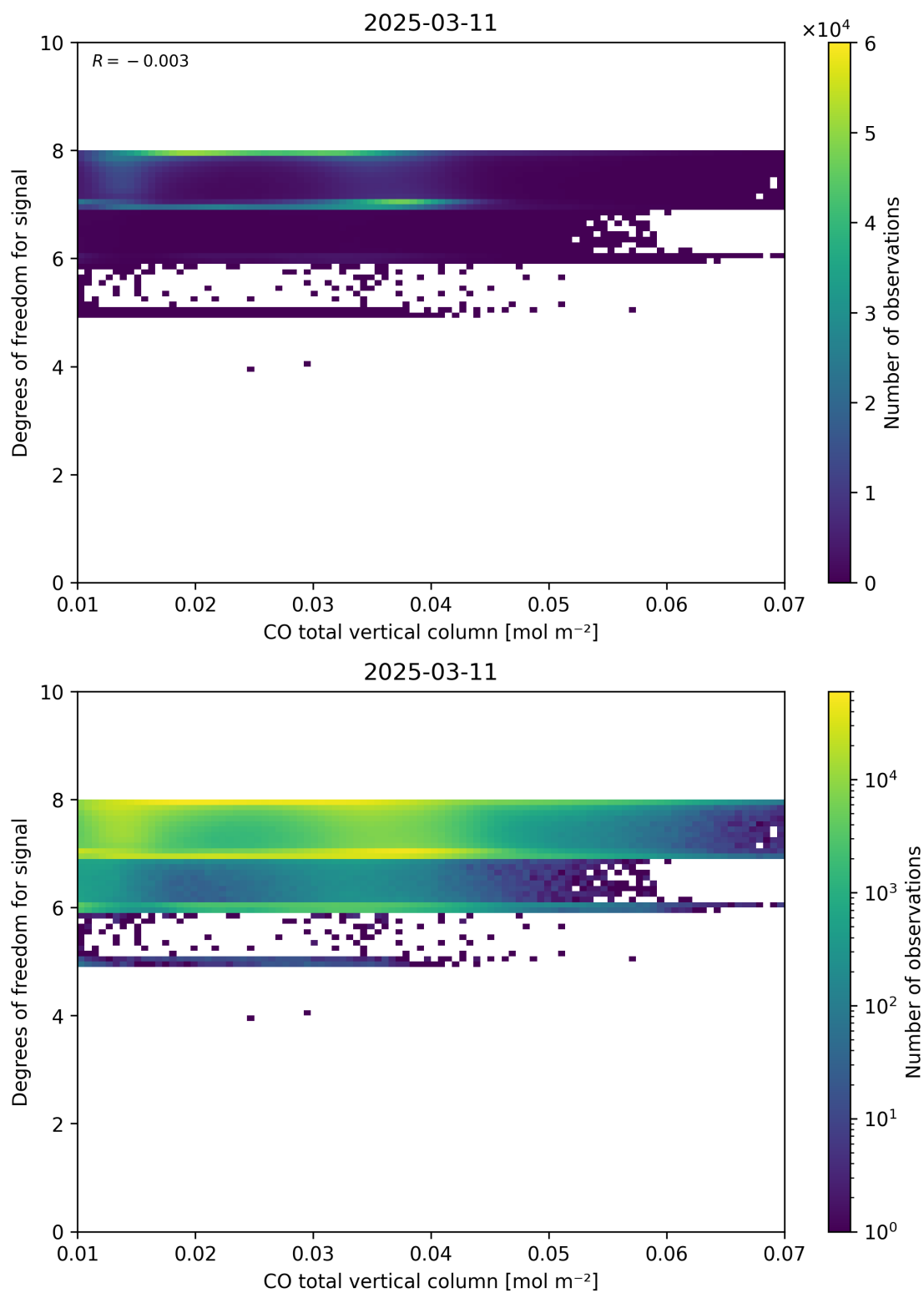
Figure 41: Scatter density plot of “CO total vertical column” against “Degrees of freedom for signal” for 2025-03-10 to 2025-03-12.
