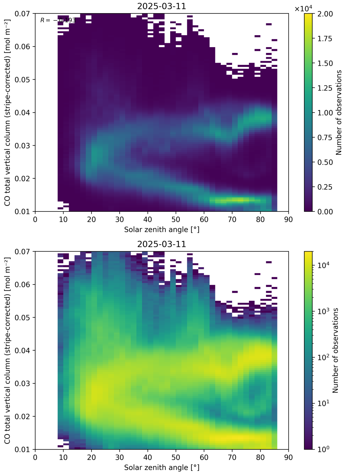
Figure 62: Scatter density plot of “Solar zenith angle” against “CO total vertical column (stripe-corrected)” for 2025-03-10 to 2025-03-12.
