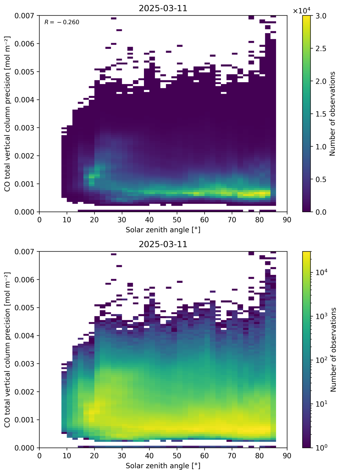
Figure 63: Scatter density plot of “Solar zenith angle” against “CO total vertical column precision” for 2025-03-10 to 2025-03-12.
