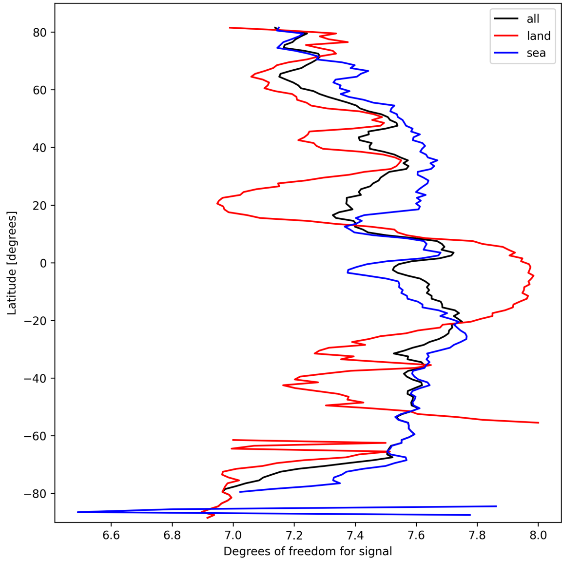
Figure 15: Zonal average of “Degrees of freedom for signal” for 2025-03-10 to 2025-03-12.
