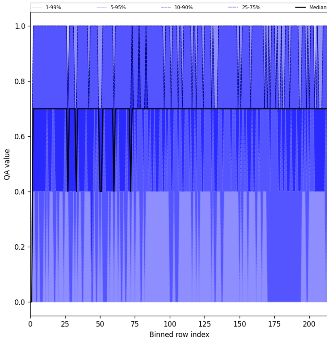
Figure 25: Along track statistics of “QA value” for 2025-03-10 to 2025-03-12
