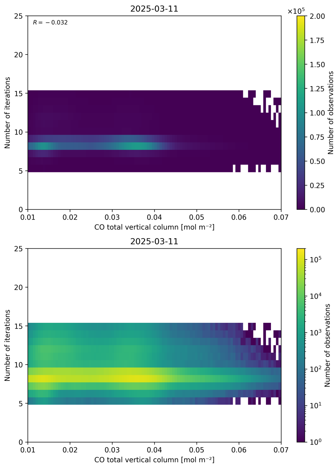
Figure 42: Scatter density plot of “CO total vertical column” against “Number of iterations” for 2025-03-10 to 2025-03-12.
