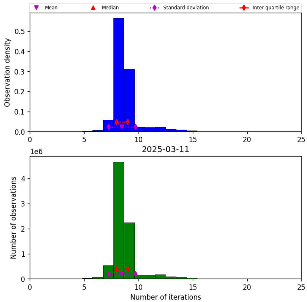
Figure 24: Histogram of “Number of iterations” for 2025-03-10 to 2025-03-12
