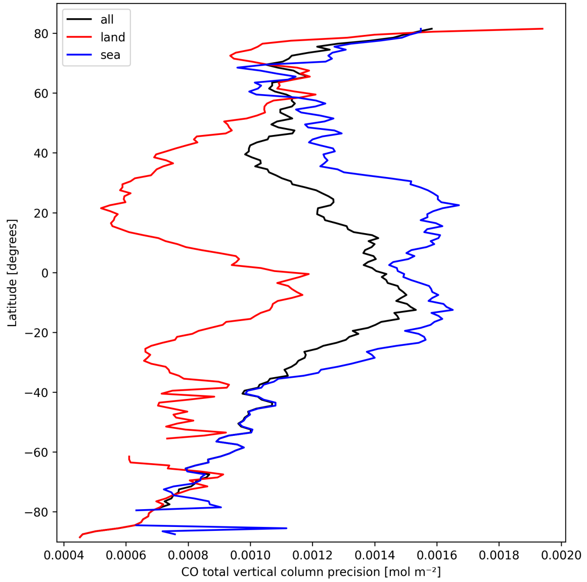
Figure 12: Zonal average of “CO total vertical column precision” for 2025-03-10 to 2025-03-12.
