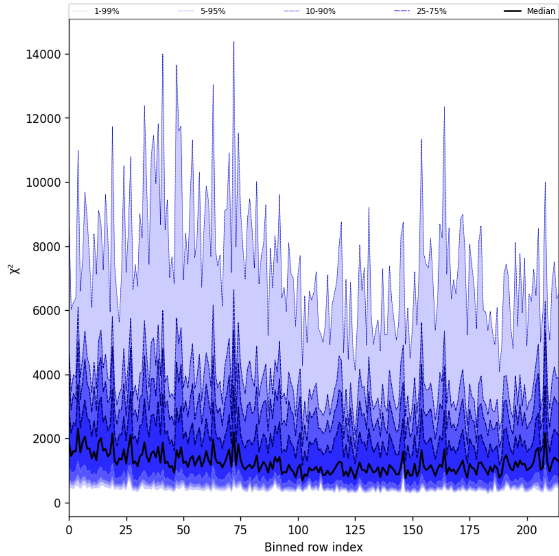
Figure 30: Along track statistics of “ \chi^2 ” for 2025-03-10 to 2025-03-12
