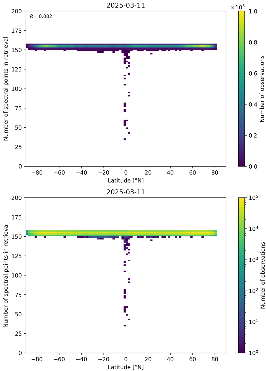
Figure 57: Scatter density plot of “Latitude” against “Number of spectral points in retrieval” for 2025-03-10 to 2025-03-12.
