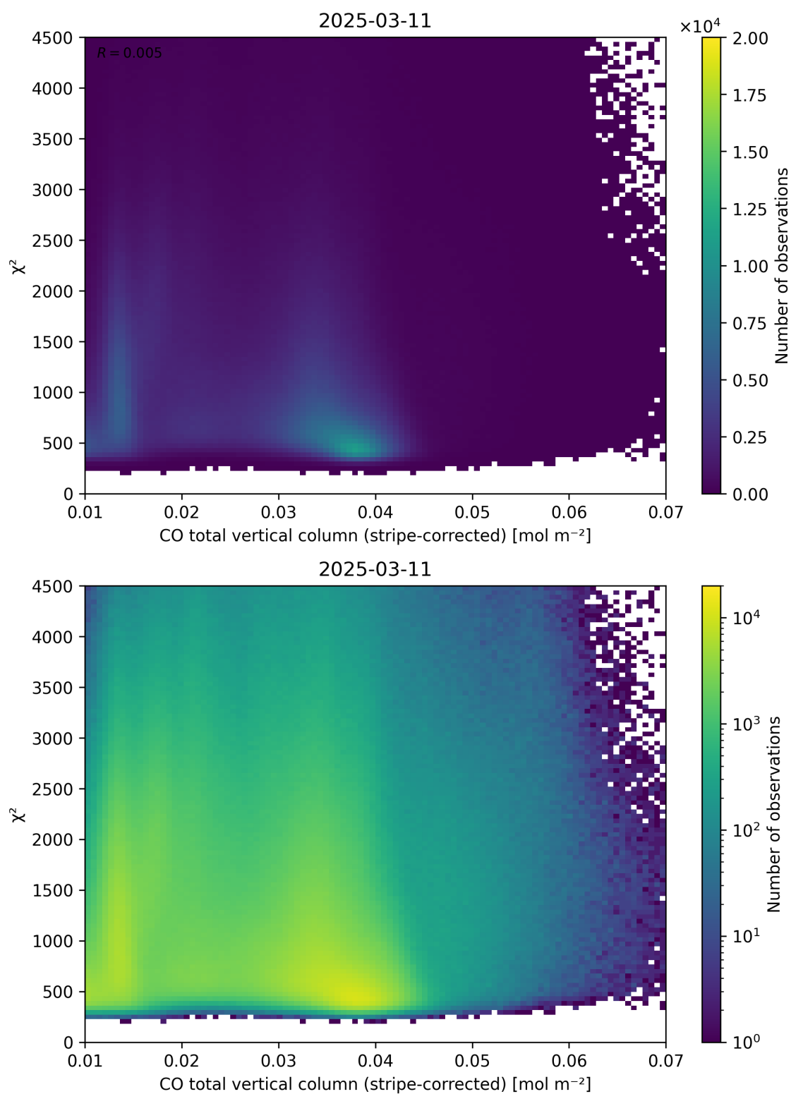
Figure 37: Scatter density plot of “CO total vertical column (stripe-corrected)” against “ \chi^2 ” for 2025-03-10 to 2025-03-12.
