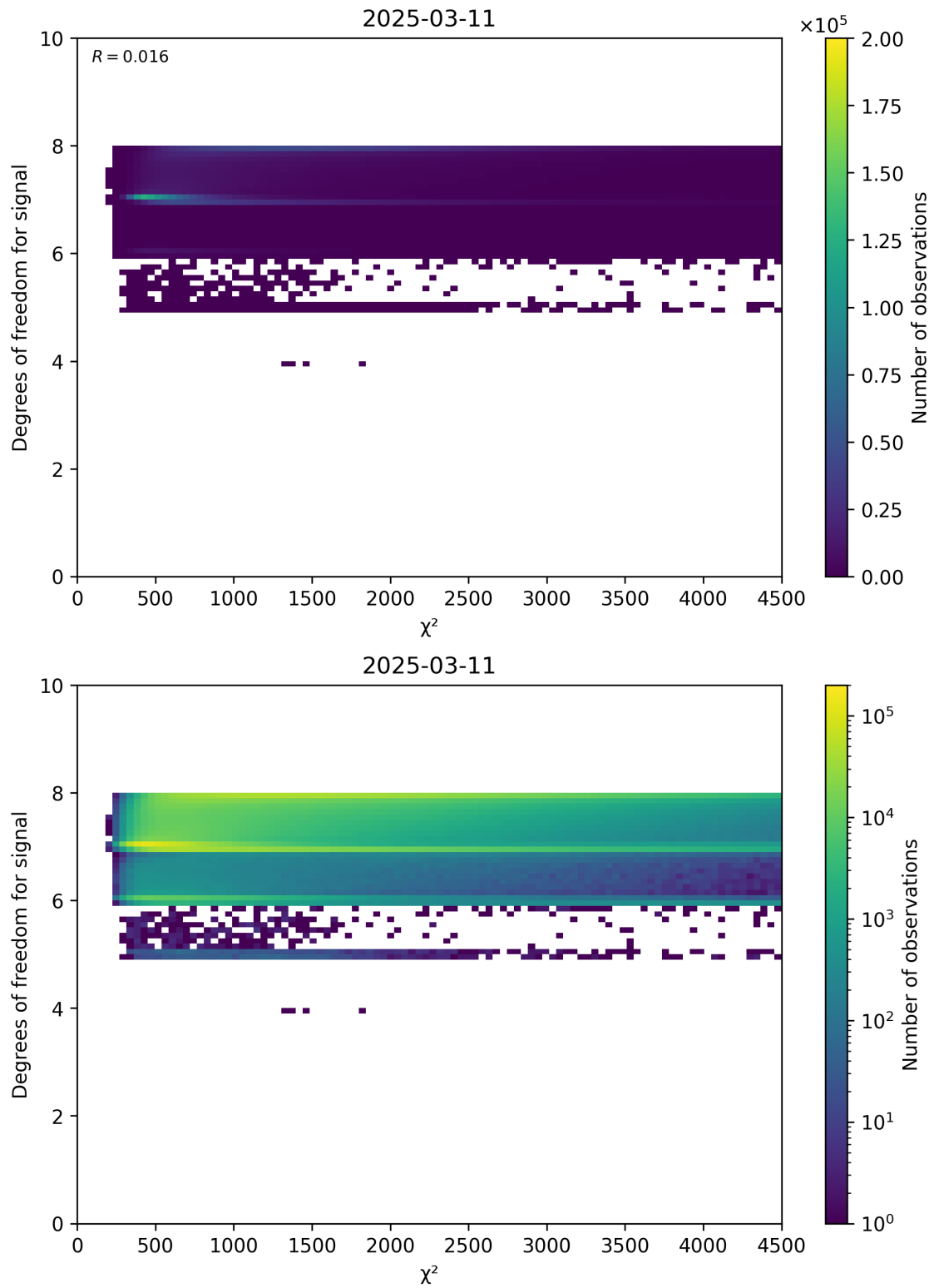
Figure 48: Scatter density plot of “ \chi^2 ” against “Degrees of freedom for signal” for 2025-03-10 to 2025-03-12.
