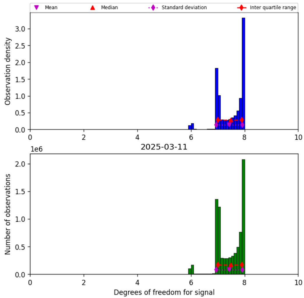
Figure 23: Histogram of “Degrees of freedom for signal” for 2025-03-10 to 2025-03-12
