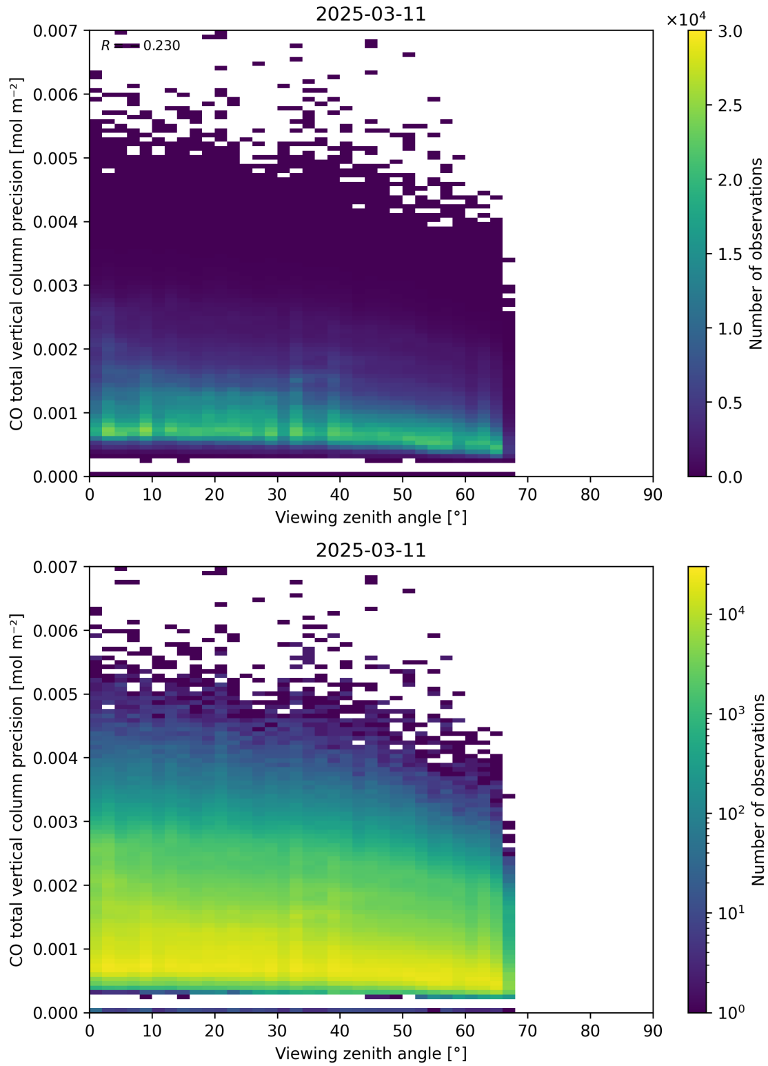
Figure 71: Scatter density plot of “Viewing zenith angle” against “CO total vertical column precision” for 2025-03-10 to 2025-03-12.
