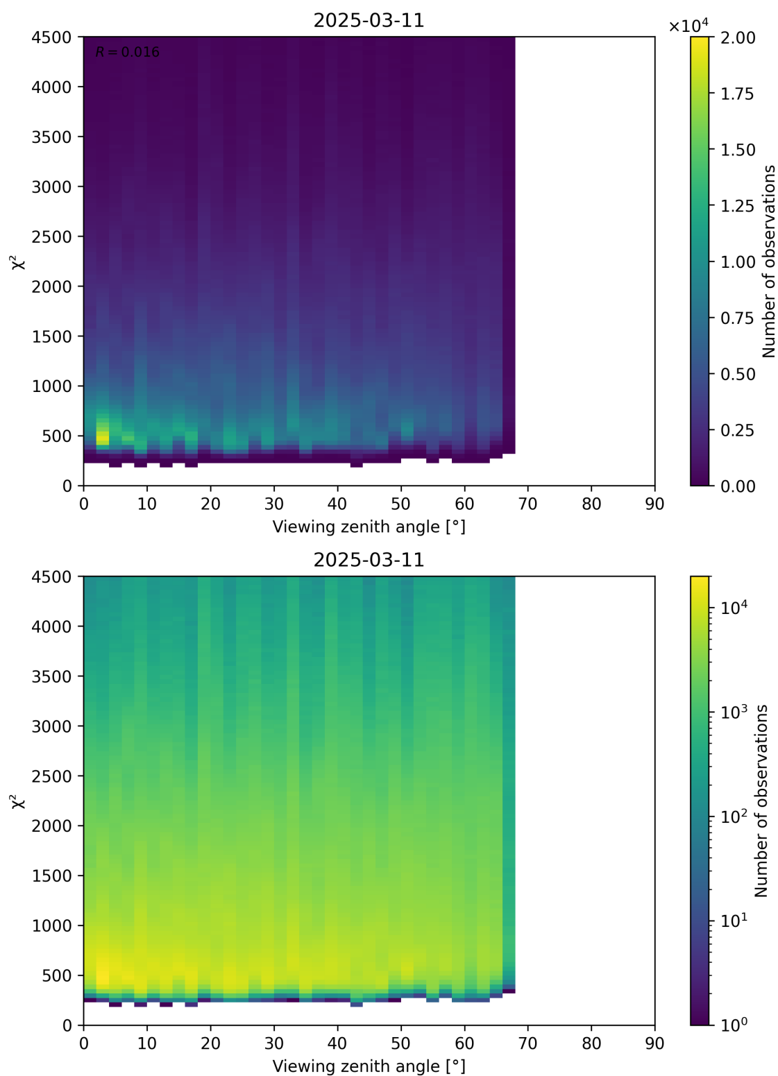
Figure 72: Scatter density plot of “Viewing zenith angle” against “ \chi^2 ” for 2025-03-10 to 2025-03-12.
