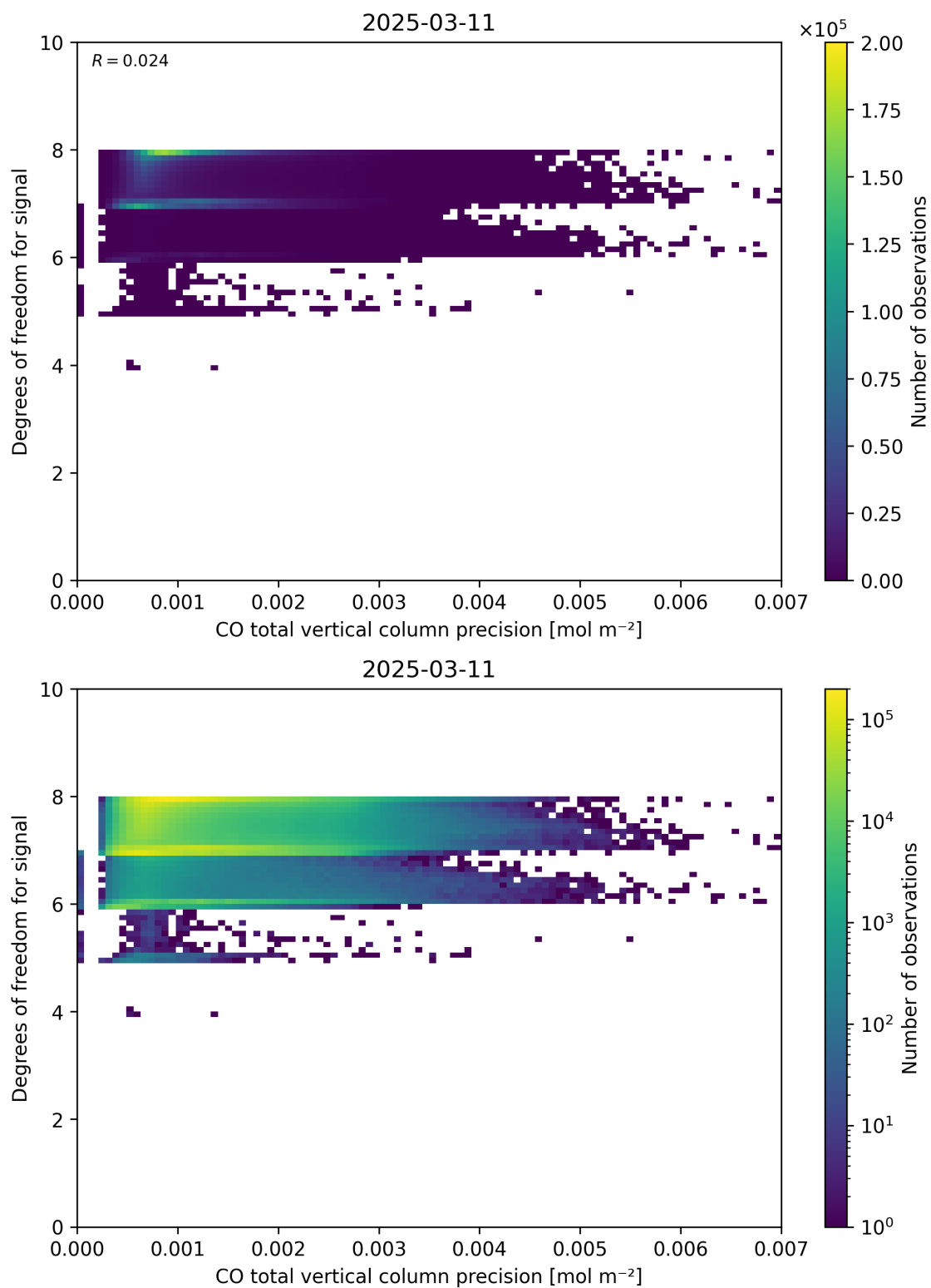
Figure 45: Scatter density plot of “CO total vertical column precision” against “Degrees of freedom for signal” for 2025-03-10 to 2025-03-12.
