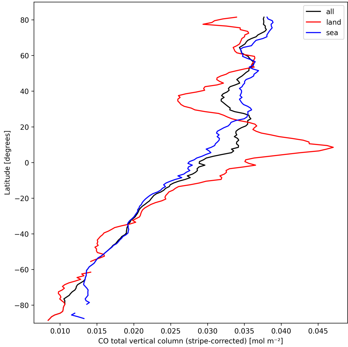
Figure 11: Zonal average of “CO total vertical column (stripe-corrected)” for 2025-03-10 to 2025-03-12.
