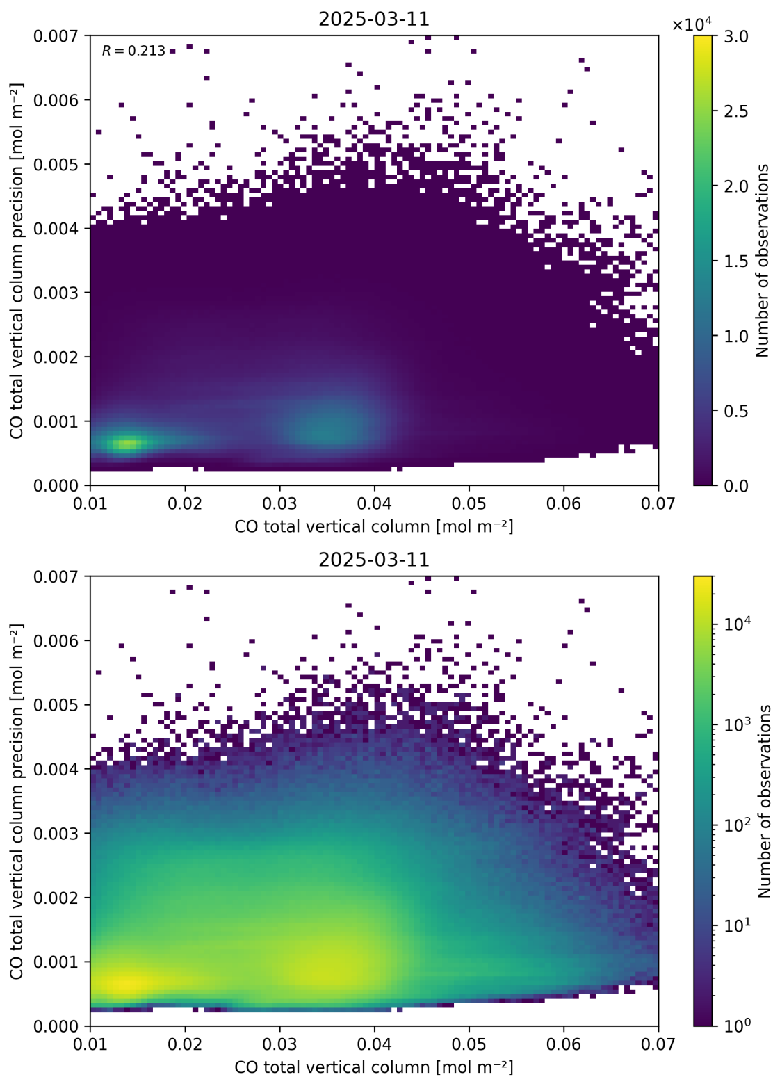
Figure 34: Scatter density plot of “CO total vertical column” against “CO total vertical column precision” for 2025-03-10 to 2025-03-12.
