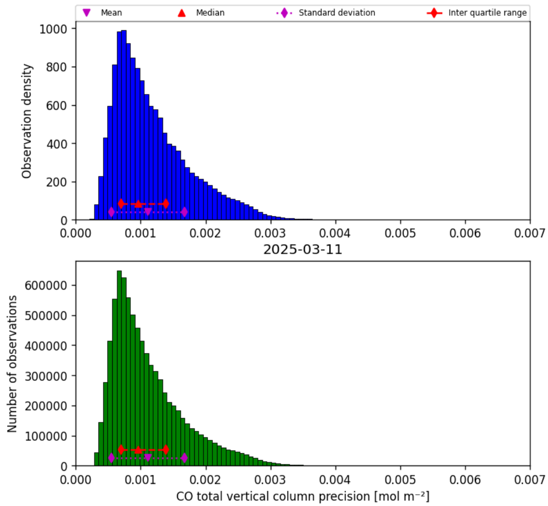
Figure 20: Histogram of “CO total vertical column precision” for 2025-03-10 to 2025-03-12
