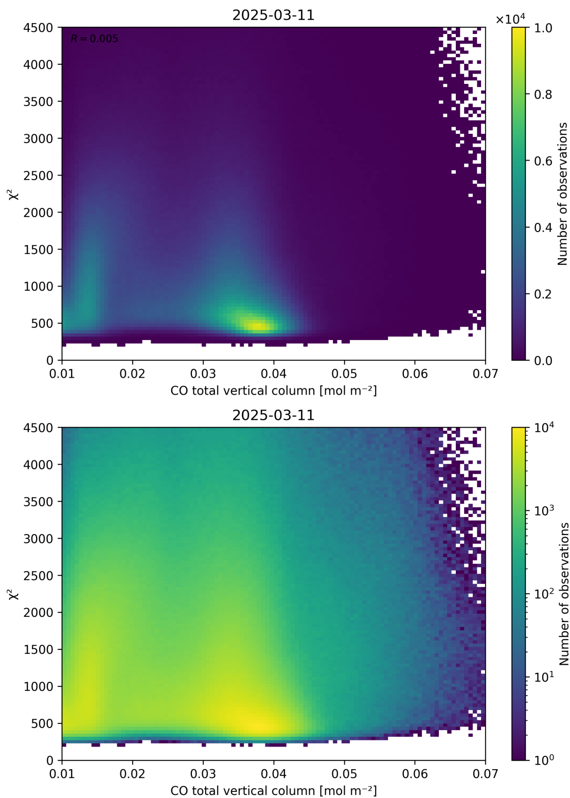
Figure 35: Scatter density plot of “CO total vertical column” against “ \chi^2 ” for 2025-03-10 to 2025-03-12.
