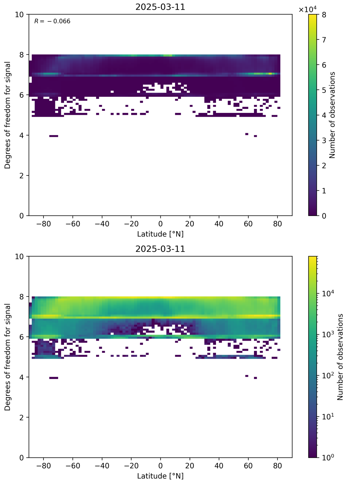
Figure 55: Scatter density plot of “Latitude” against “Degrees of freedom for signal” for 2025-03-10 to 2025-03-12.
