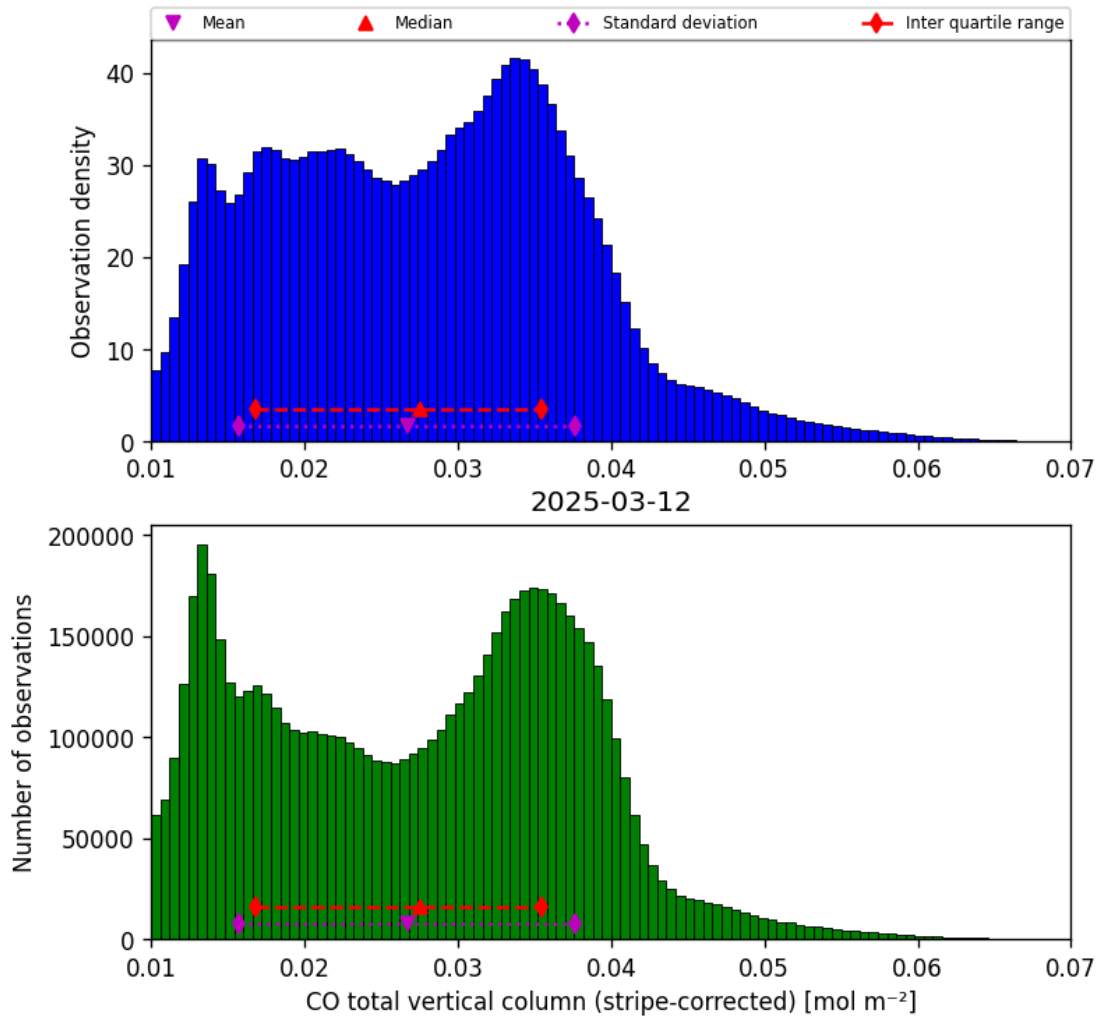
Figure 19: Histogram of “CO total vertical column (stripe-corrected)” for 2025-03-12 to 2025-03-13
