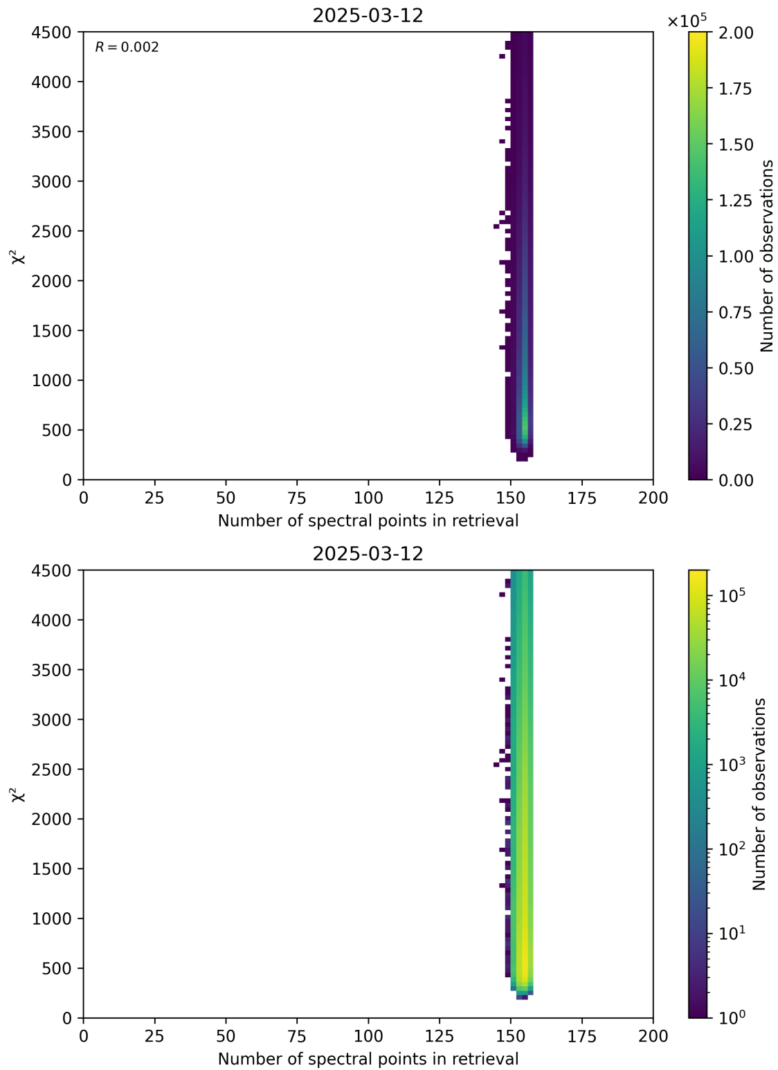
Figure 58: Scatter density plot of “Number of spectral points in retrieval” against “ \chi^2 ” for 2025-03-12 to 2025-03-13.
