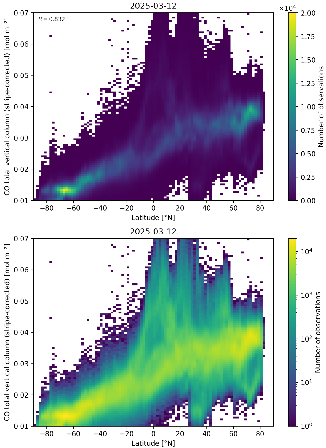
Figure 52: Scatter density plot of “Latitude” against “CO total vertical column (stripe-corrected)” for 2025-03-12 to 2025-03-13.
