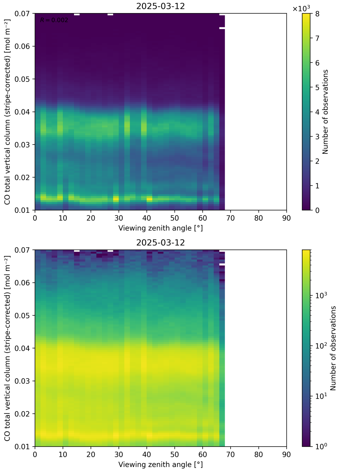
Figure 70: Scatter density plot of “Viewing zenith angle” against “CO total vertical column (stripe-corrected)” for 2025-03-12 to 2025-03-13.
