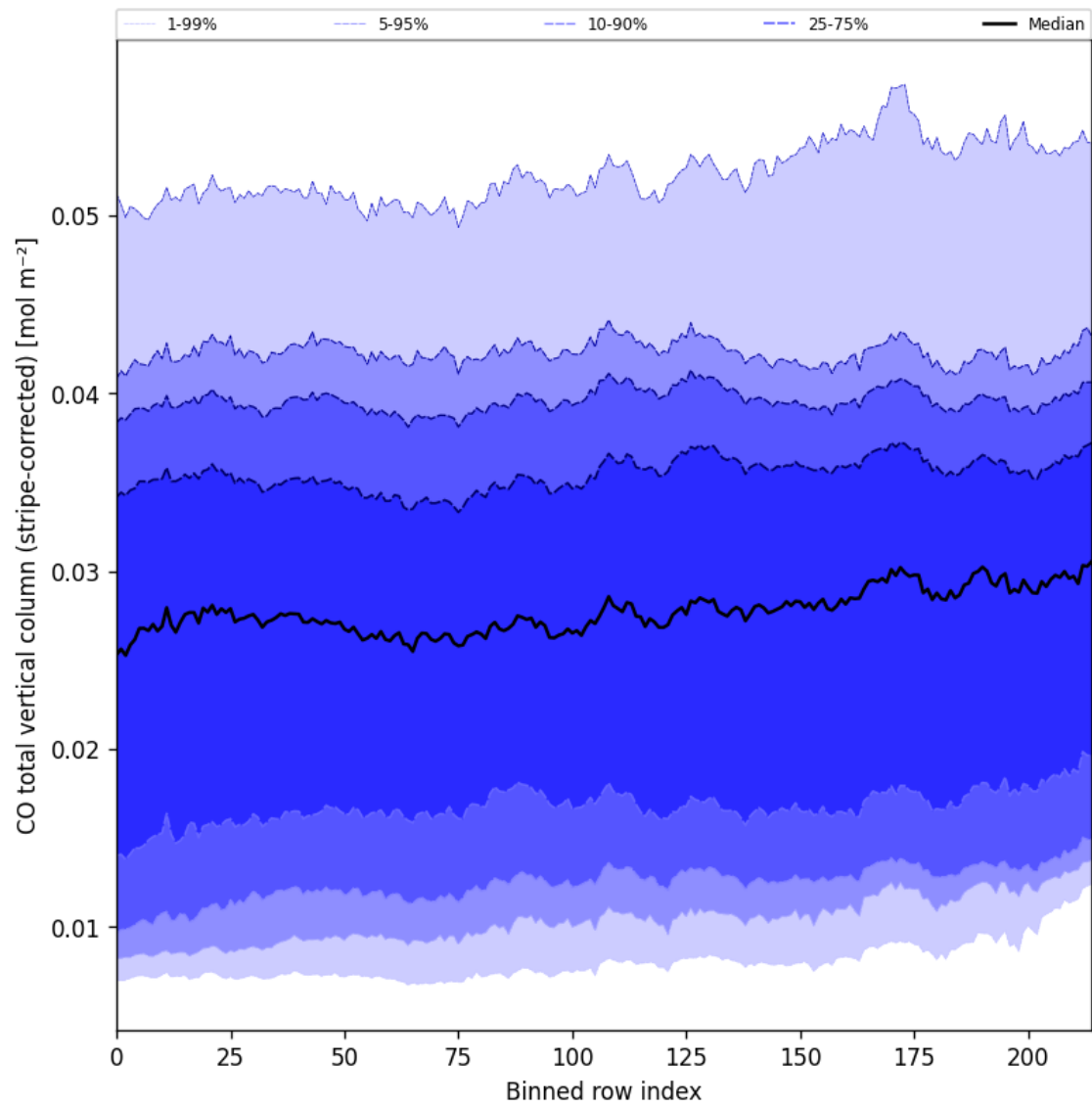
Figure 27: Along track statistics of “CO total vertical column (stripe-corrected)” for 2025-03-12 to 2025-03-13
