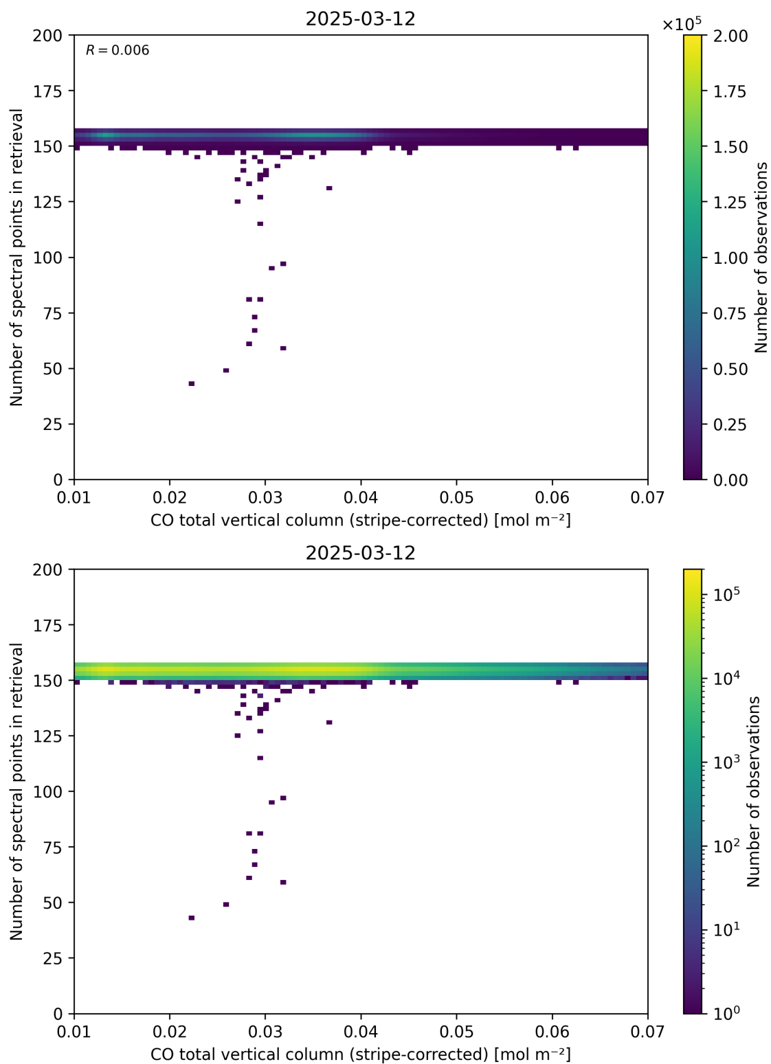
Figure 40: Scatter density plot of “CO total vertical column (stripe-corrected)” against “Number of spectral points in retrieval” for 2025-03-12 to 2025-03-13.
