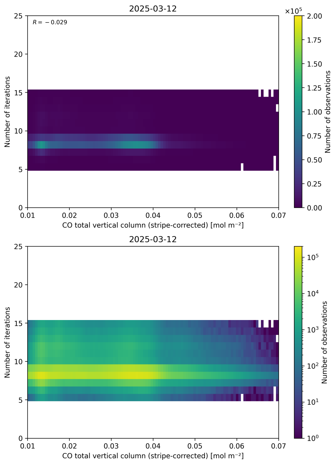
Figure 39: Scatter density plot of “CO total vertical column (stripe-corrected)” against “Number of iterations” for 2025-03-12 to 2025-03-13.
