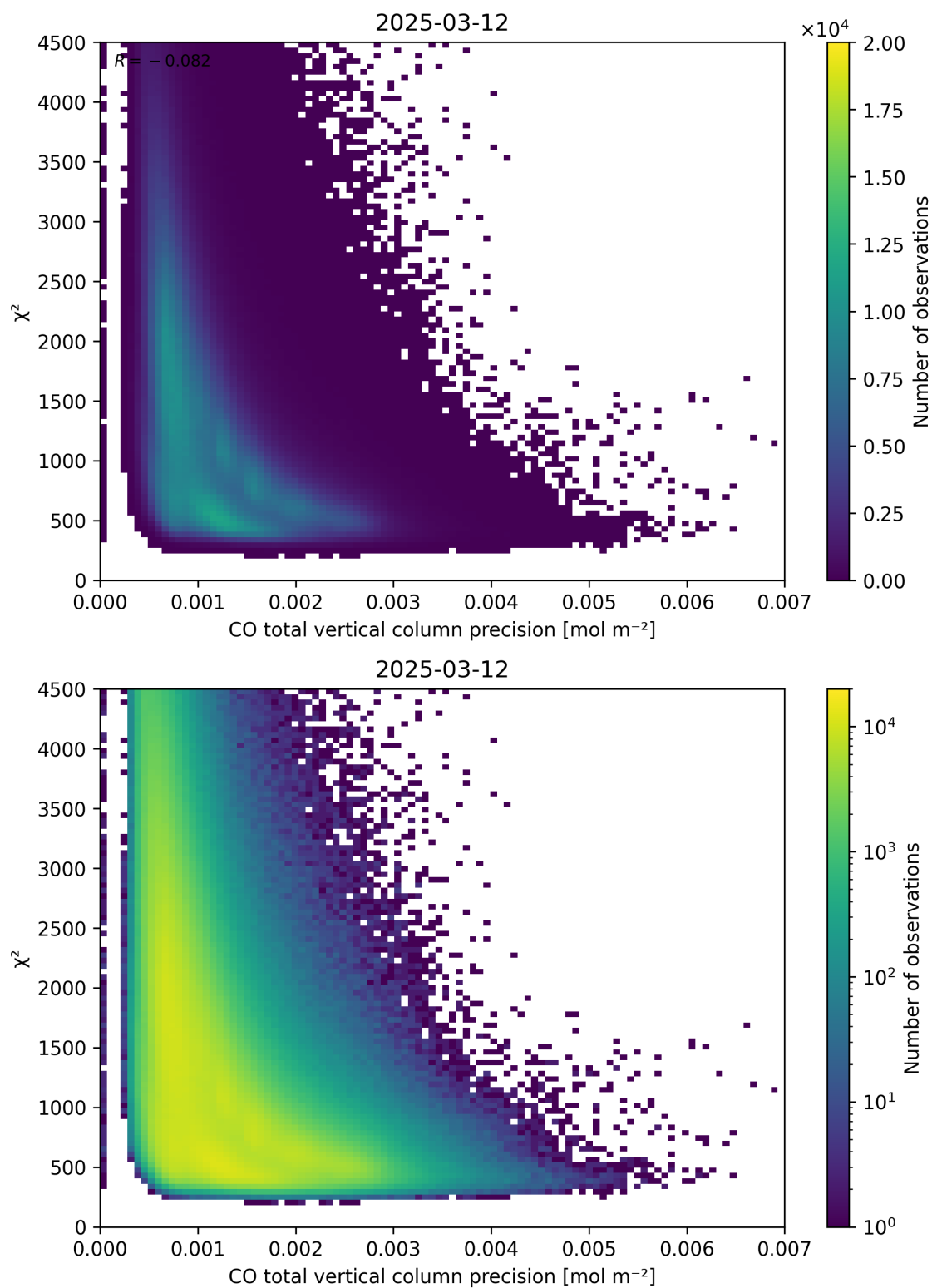
Figure 44: Scatter density plot of “CO total vertical column precision” against “ \chi^2 ” for 2025-03-12 to 2025-03-13.
