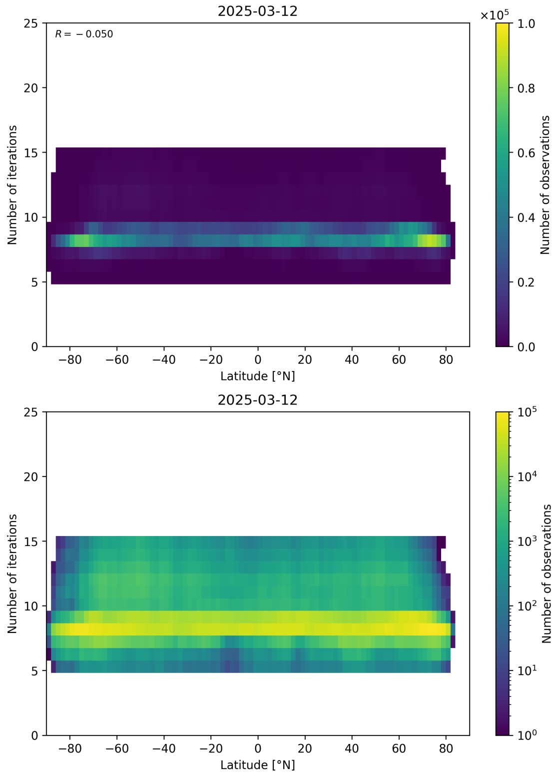
Figure 56: Scatter density plot of “Latitude” against “Number of iterations” for 2025-03-12 to 2025-03-13.
