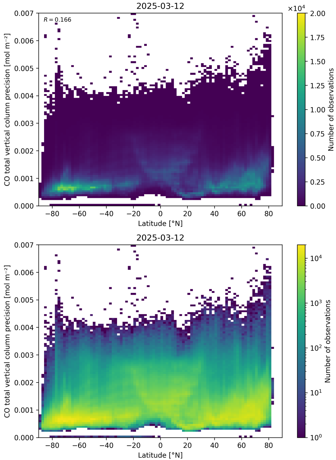
Figure 53: Scatter density plot of “Latitude” against “CO total vertical column precision” for 2025-03-12 to 2025-03-13.
