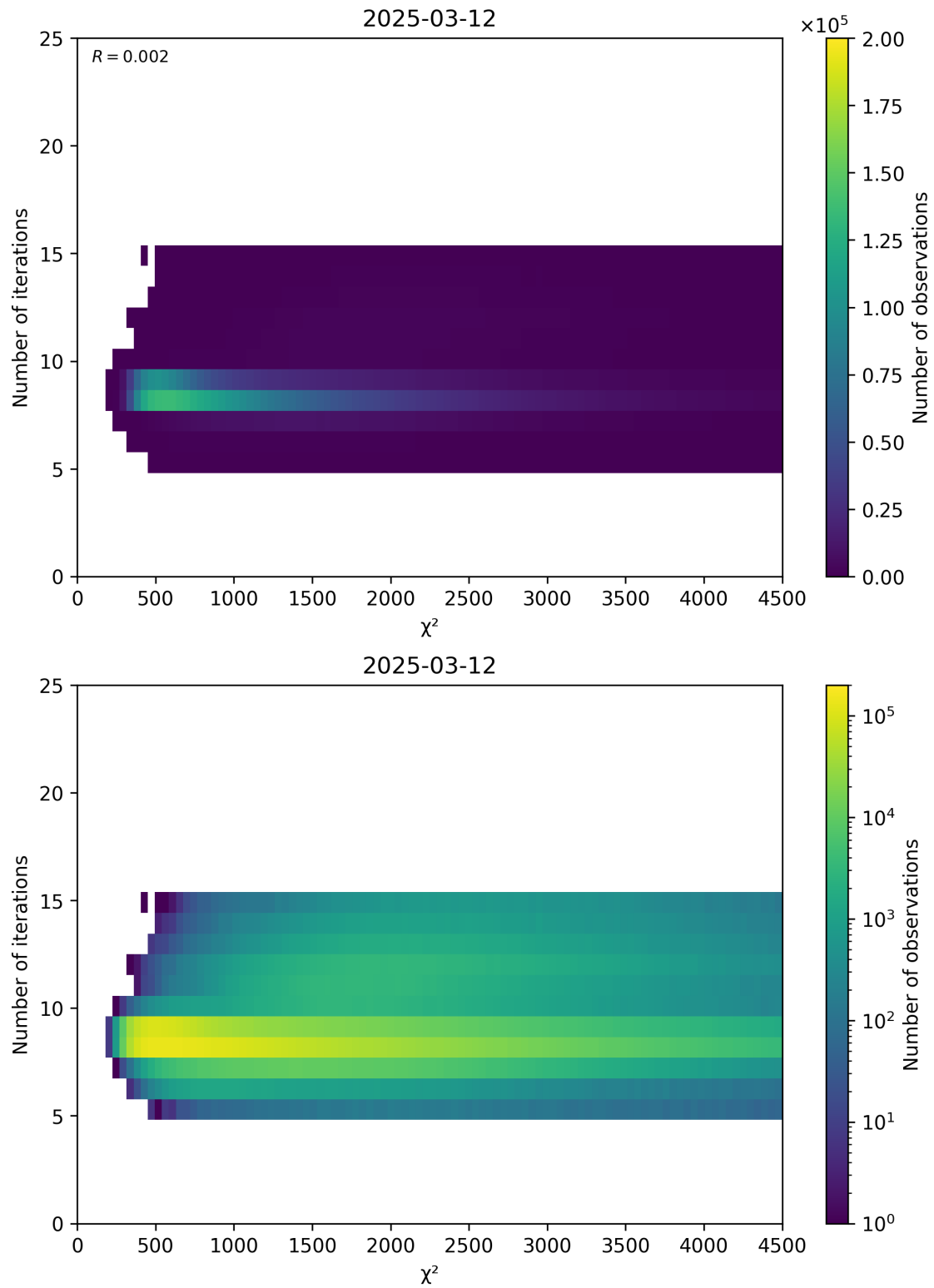
Figure 49: Scatter density plot of “ \chi^2 ” against “Number of iterations” for 2025-03-12 to 2025-03-13.
