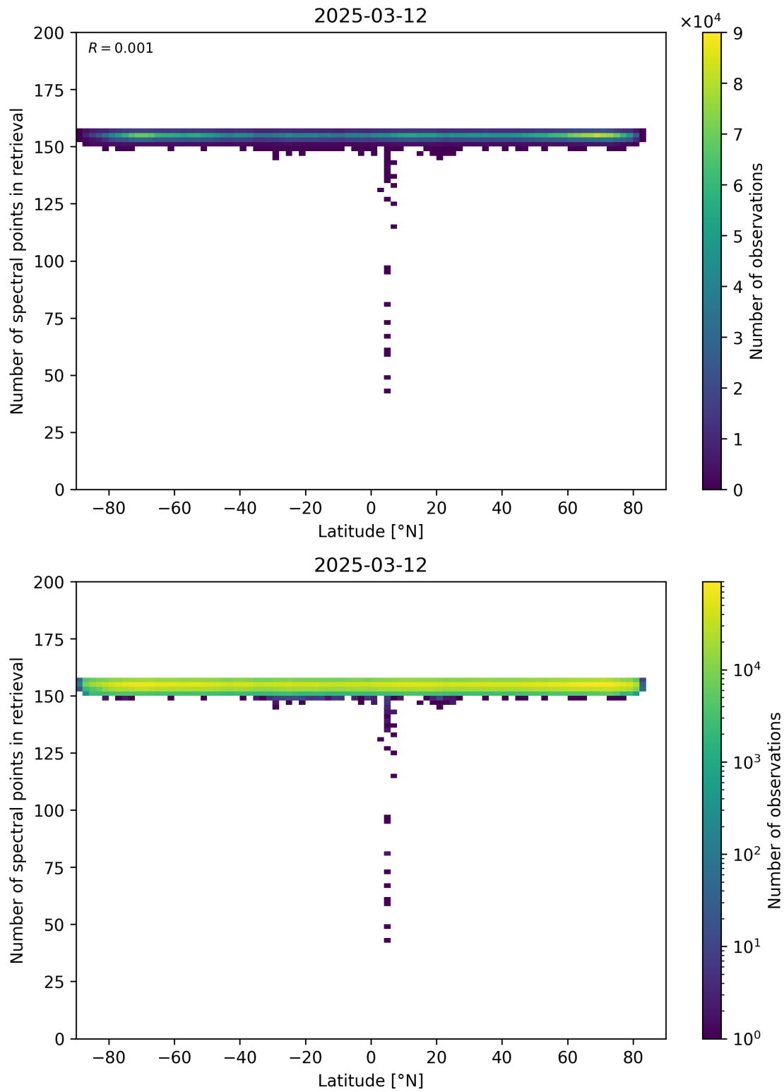
Figure 57: Scatter density plot of “Latitude” against “Number of spectral points in retrieval” for 2025-03-12 to 2025-03-13.
