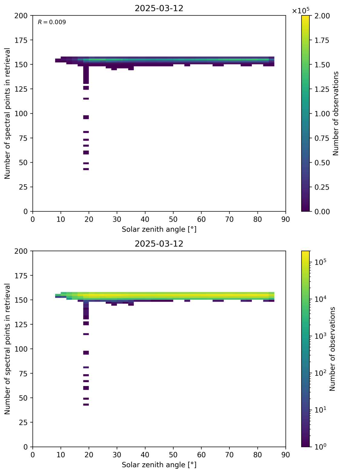
Figure 68: Scatter density plot of “Solar zenith angle” against “Number of spectral points in retrieval” for 2025-03-12 to 2025-03-13.
