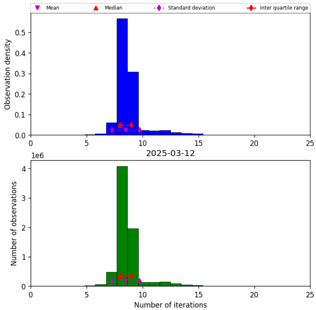
Figure 24: Histogram of “Number of iterations” for 2025-03-12 to 2025-03-13
