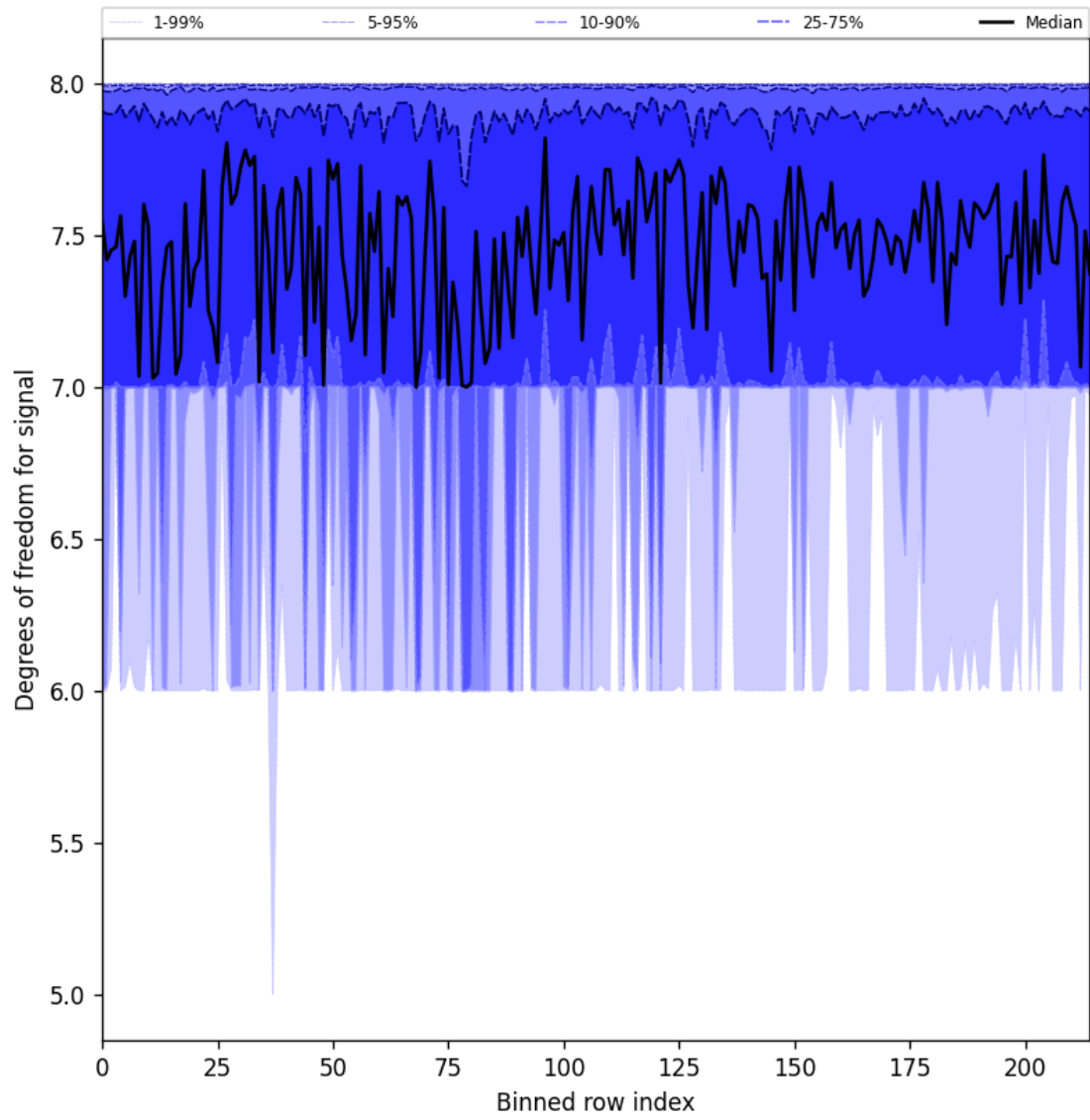
Figure 31: Along track statistics of “Degrees of freedom for signal” for 2025-03-12 to 2025-03-13
