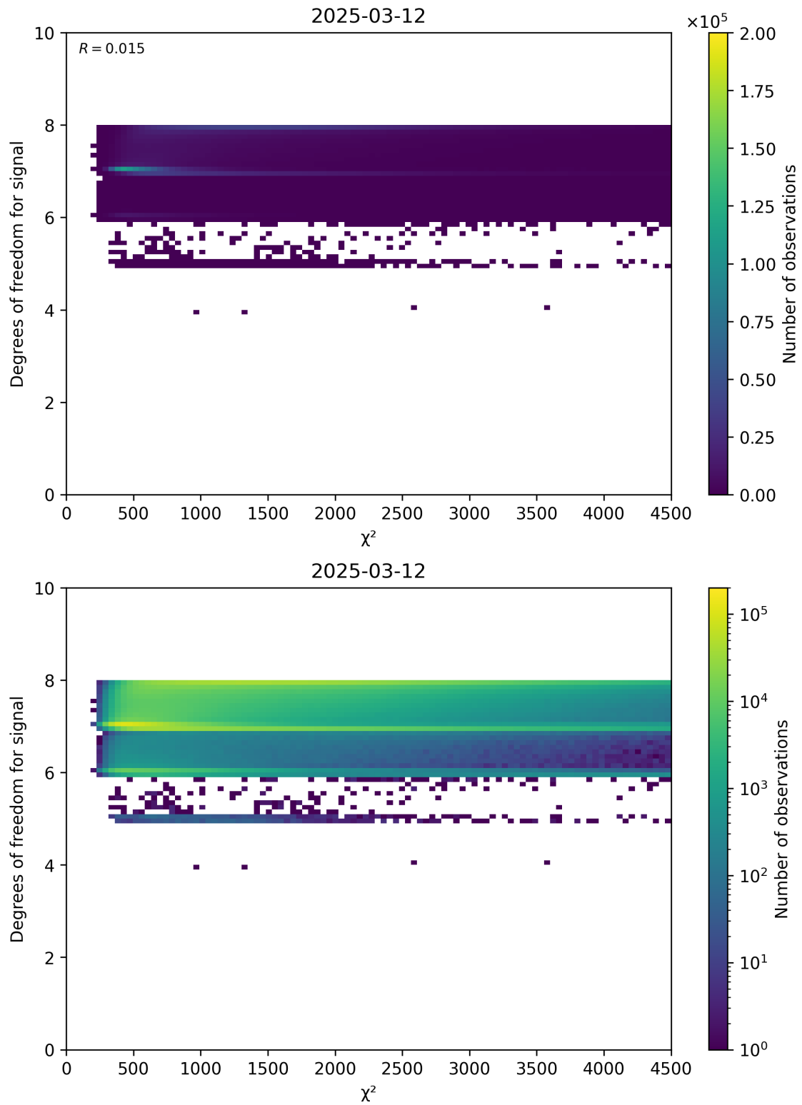
Figure 48: Scatter density plot of “ \chi^2 ” against “Degrees of freedom for signal” for 2025-03-12 to 2025-03-13.
