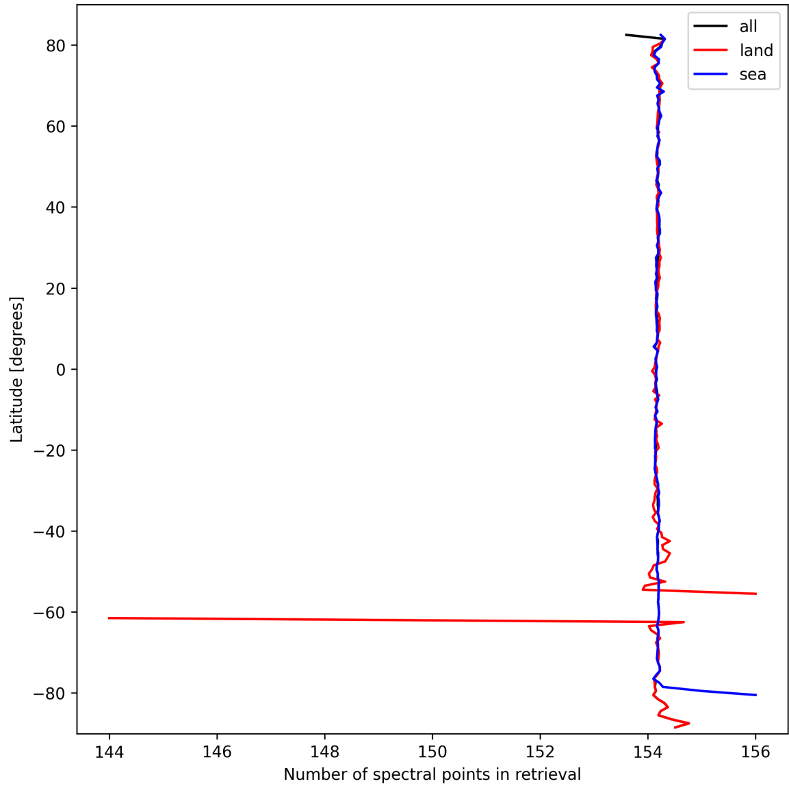
Figure 13: Zonal average of “Number of spectral points in retrieval” for 2025-03-12 to 2025-03-13.
