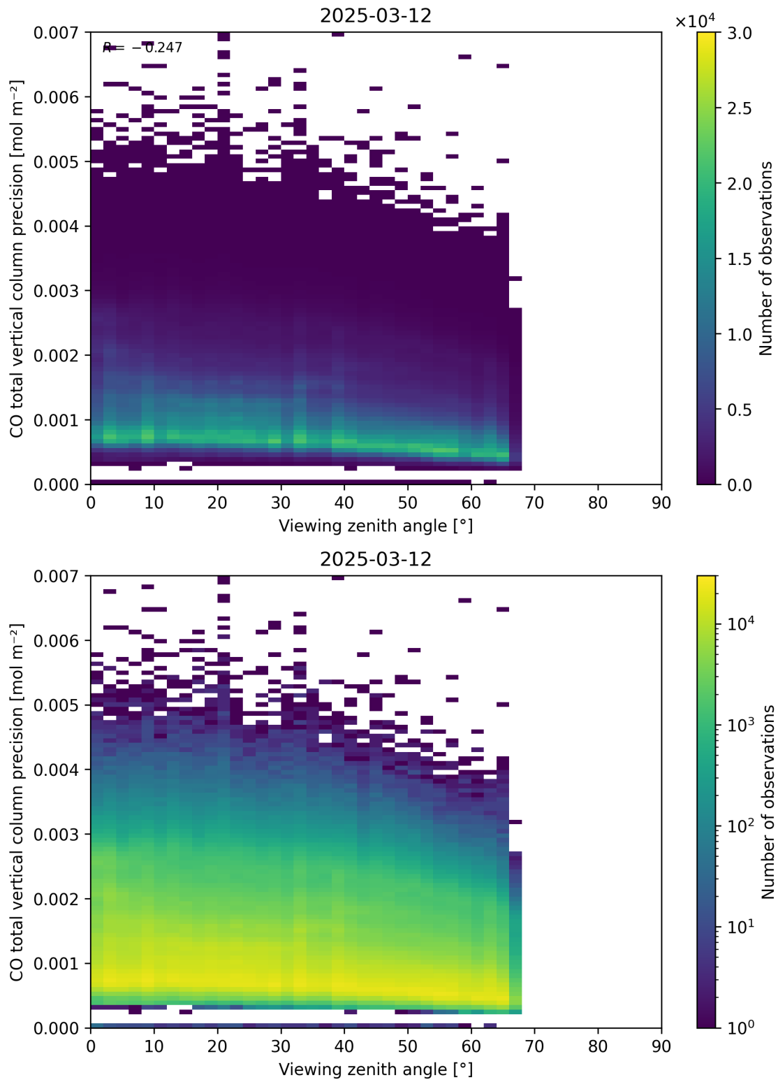
Figure 71: Scatter density plot of “Viewing zenith angle” against “CO total vertical column precision” for 2025-03-12 to 2025-03-13.
