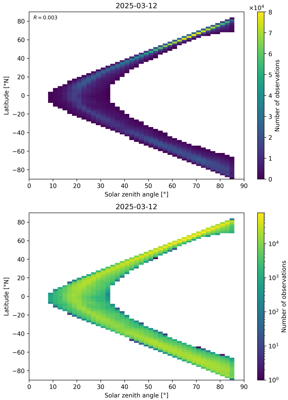
Figure 66: Scatter density plot of “Solar zenith angle” against “Latitude” for 2025-03-12 to 2025-03-13.
