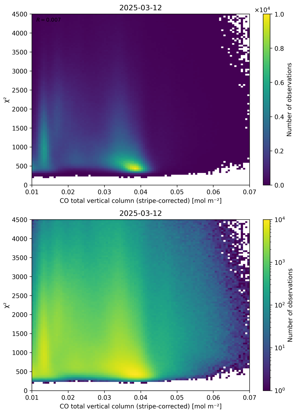
Figure 37: Scatter density plot of “CO total vertical column (stripe-corrected)” against “ \chi^2 ” for 2025-03-12 to 2025-03-13.
