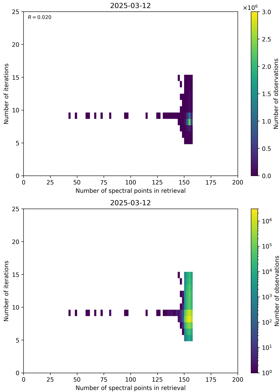
Figure 60: Scatter density plot of “Number of spectral points in retrieval” against “Number of iterations” for 2025-03-12 to 2025-03-13.
