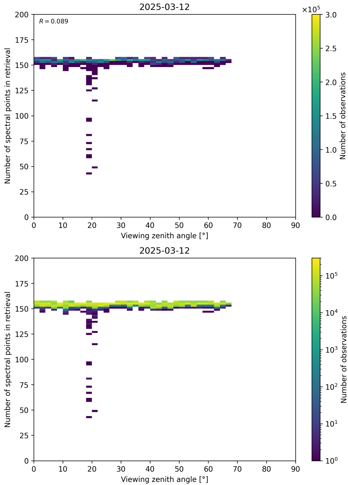
Figure 76: Scatter density plot of “Viewing zenith angle” against “Number of spectral points in retrieval” for 2025-03-12 to 2025-03-13.
