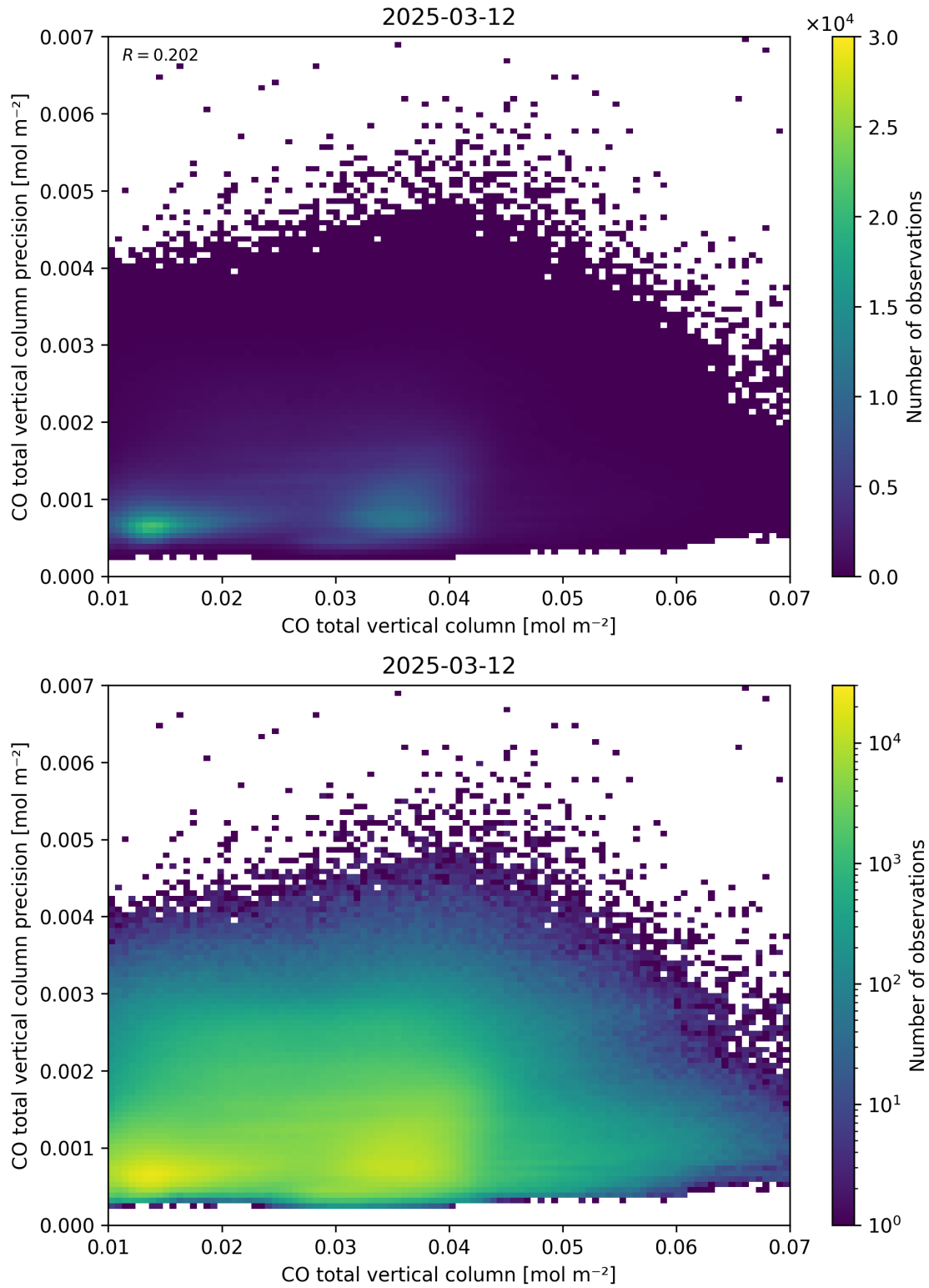
Figure 34: Scatter density plot of “CO total vertical column” against “CO total vertical column precision” for 2025-03-12 to 2025-03-13.
