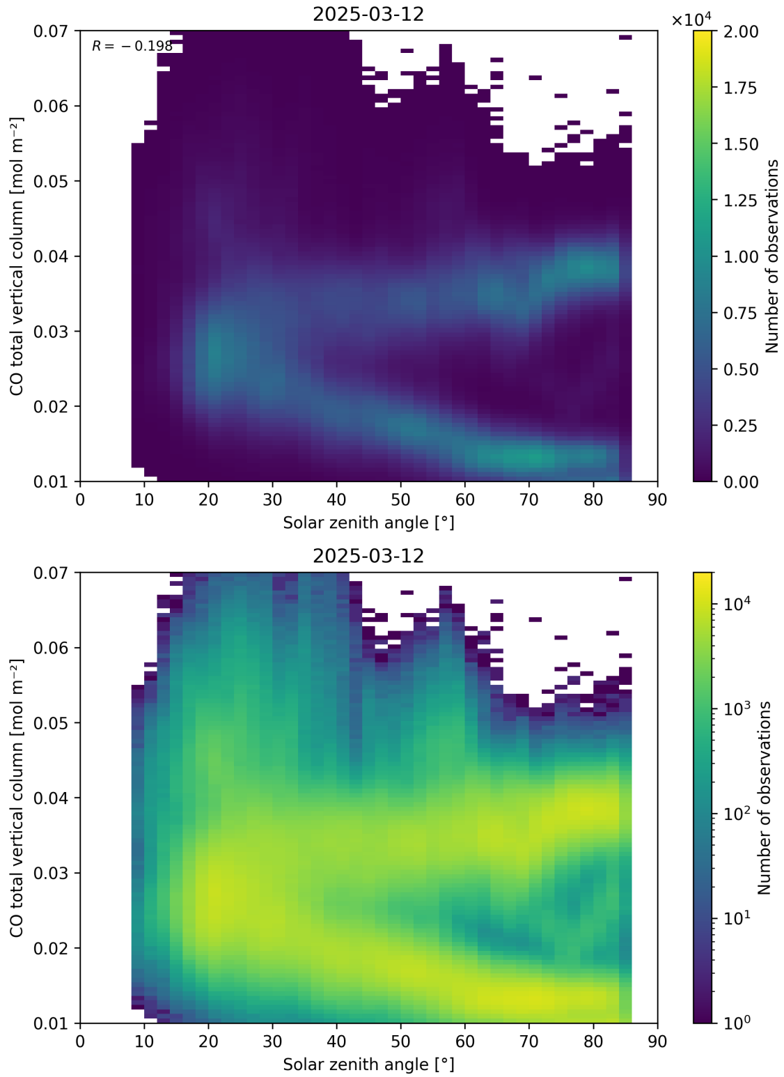
Figure 61: Scatter density plot of “Solar zenith angle” against “CO total vertical column” for 2025-03-12 to 2025-03-13.
