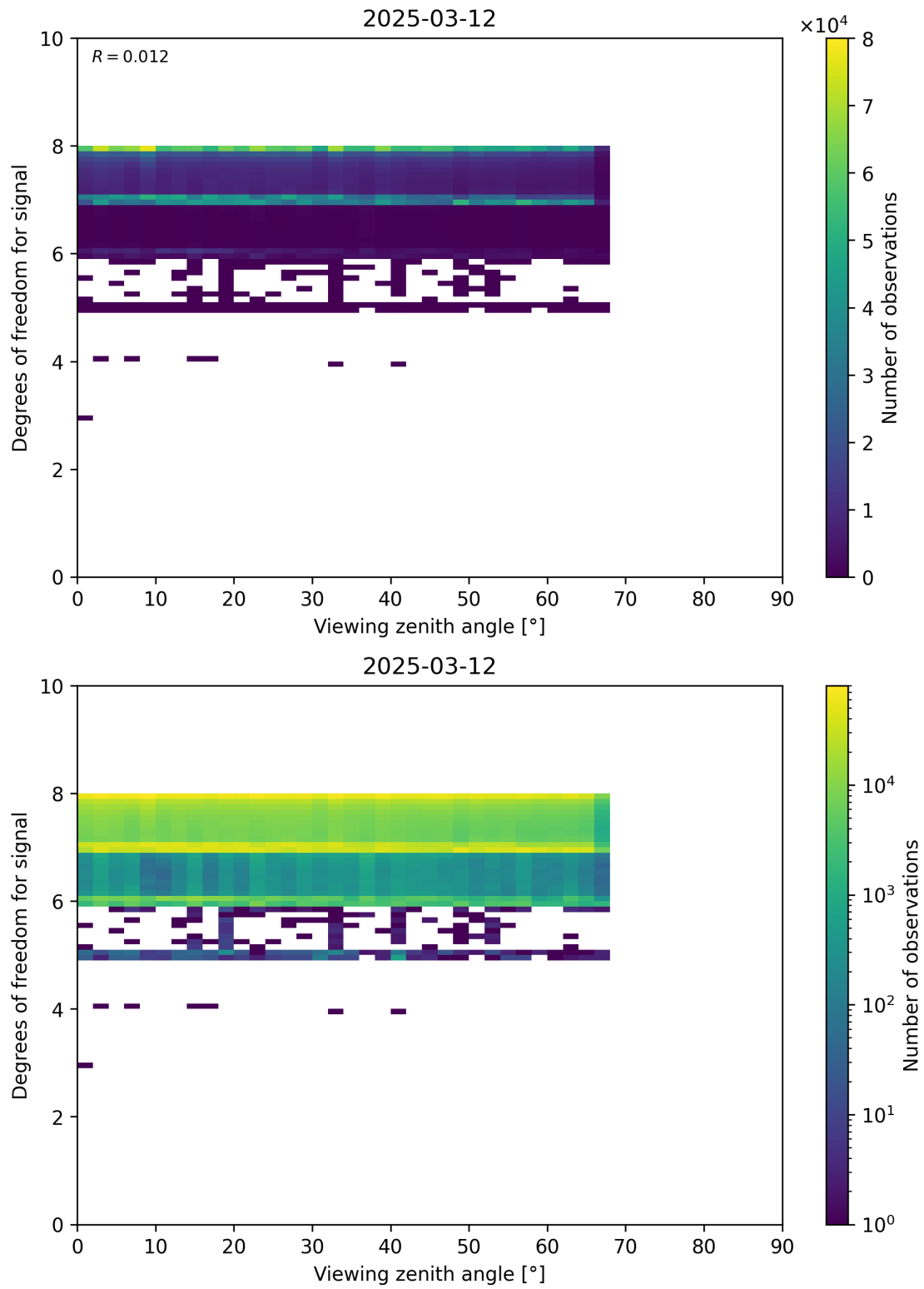
Figure 73: Scatter density plot of “Viewing zenith angle” against “Degrees of freedom for signal” for 2025-03-12 to 2025-03-13.
