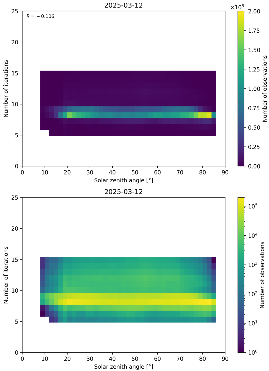
Figure 67: Scatter density plot of “Solar zenith angle” against “Number of iterations” for 2025-03-12 to 2025-03-13.
