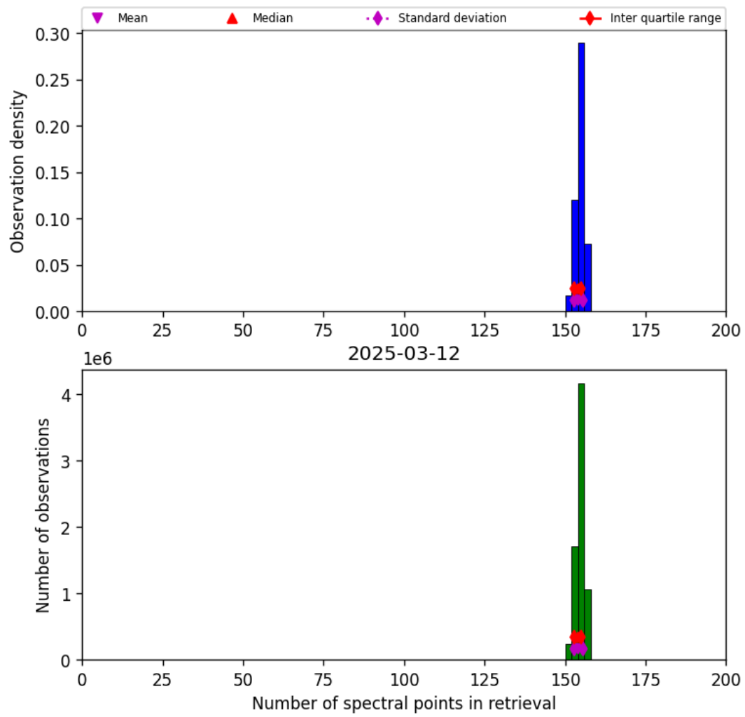
Figure 21: Histogram of “Number of spectral points in retrieval” for 2025-03-12 to 2025-03-13
