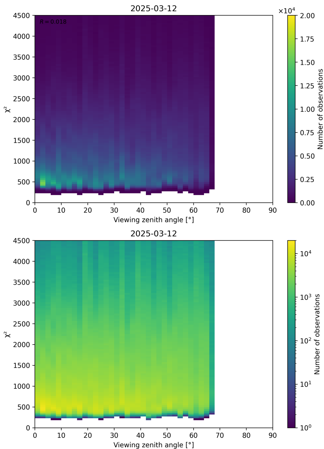
Figure 72: Scatter density plot of “Viewing zenith angle” against “ \chi^2 ” for 2025-03-12 to 2025-03-13.
