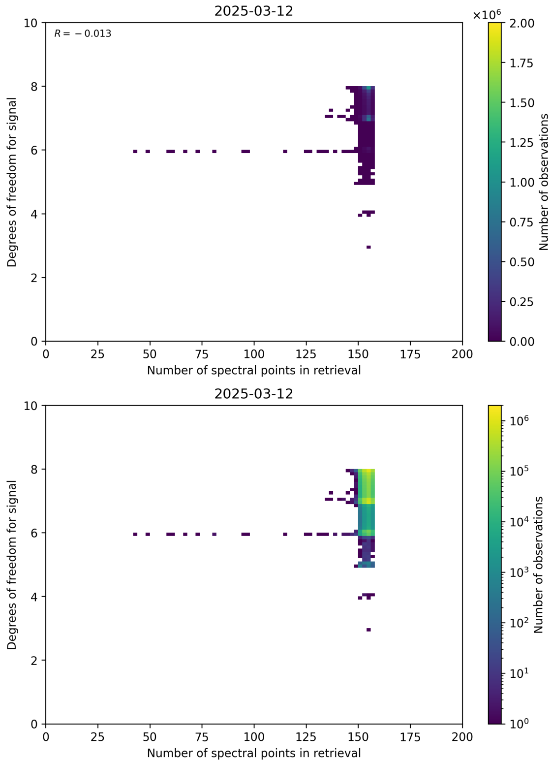
Figure 59: Scatter density plot of “Number of spectral points in retrieval” against “Degrees of freedom for signal” for 2025-03-12 to 2025-03-13.
