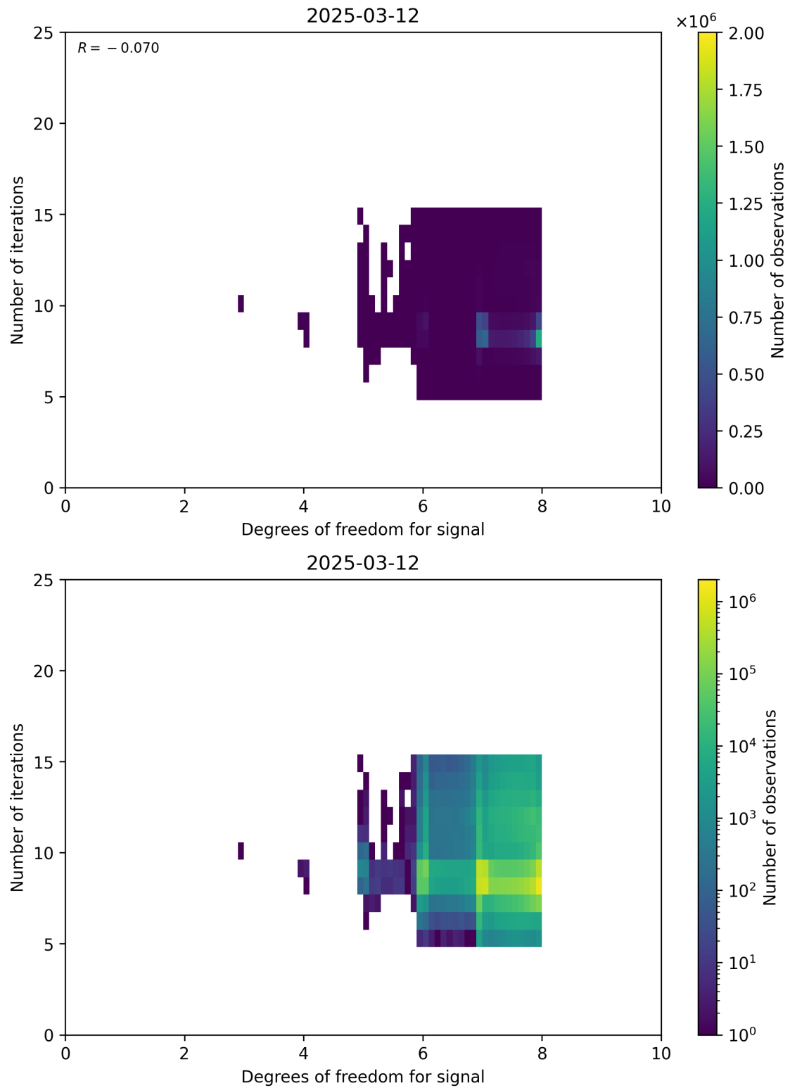
Figure 50: Scatter density plot of “Degrees of freedom for signal” against “Number of iterations” for 2025-03-12 to 2025-03-13.
