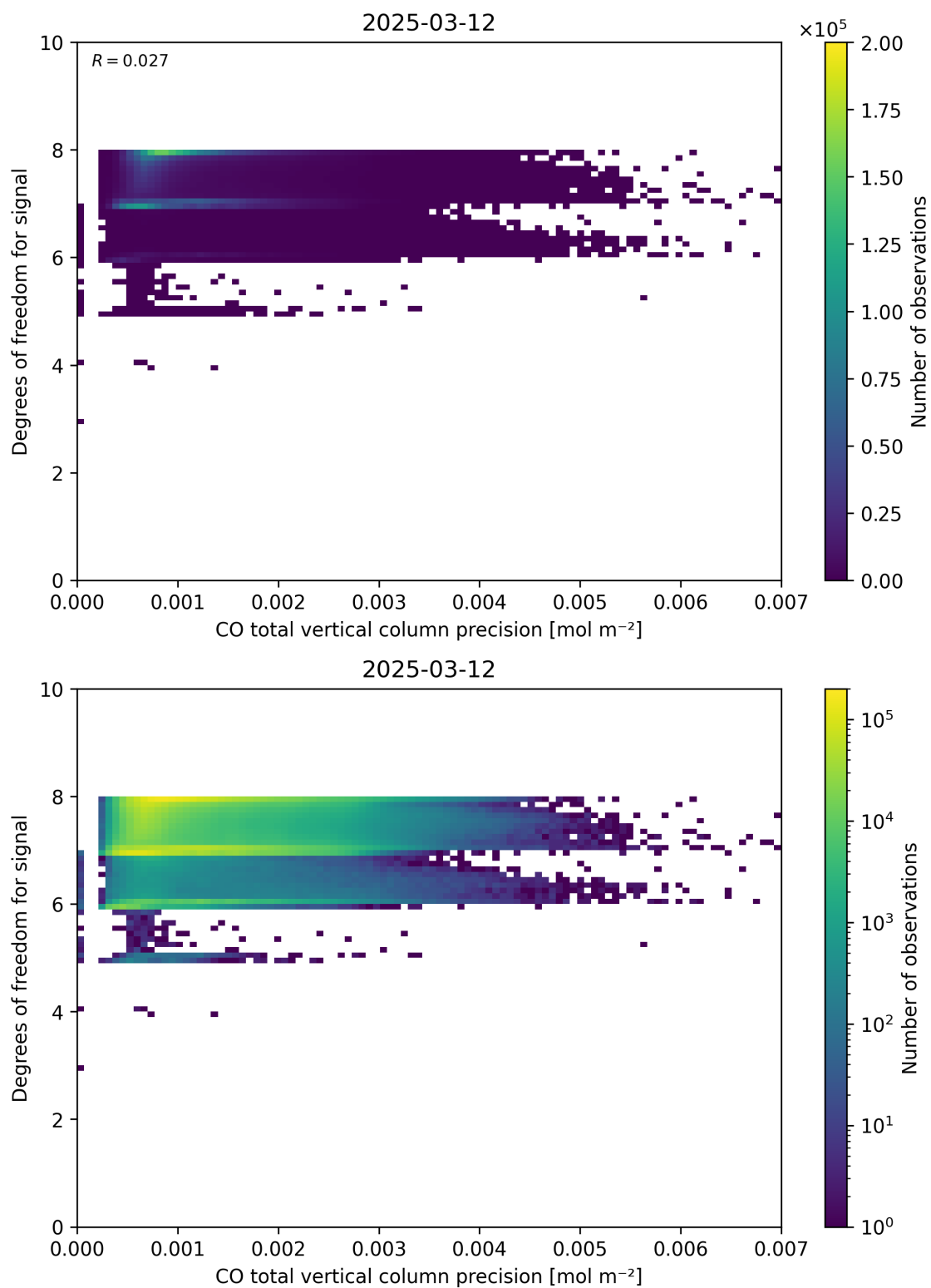
Figure 45: Scatter density plot of “CO total vertical column precision” against “Degrees of freedom for signal” for 2025-03-12 to 2025-03-13.
