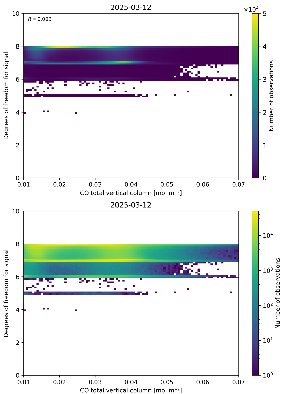
Figure 41: Scatter density plot of “CO total vertical column” against “Degrees of freedom for signal” for 2025-03-12 to 2025-03-13.
