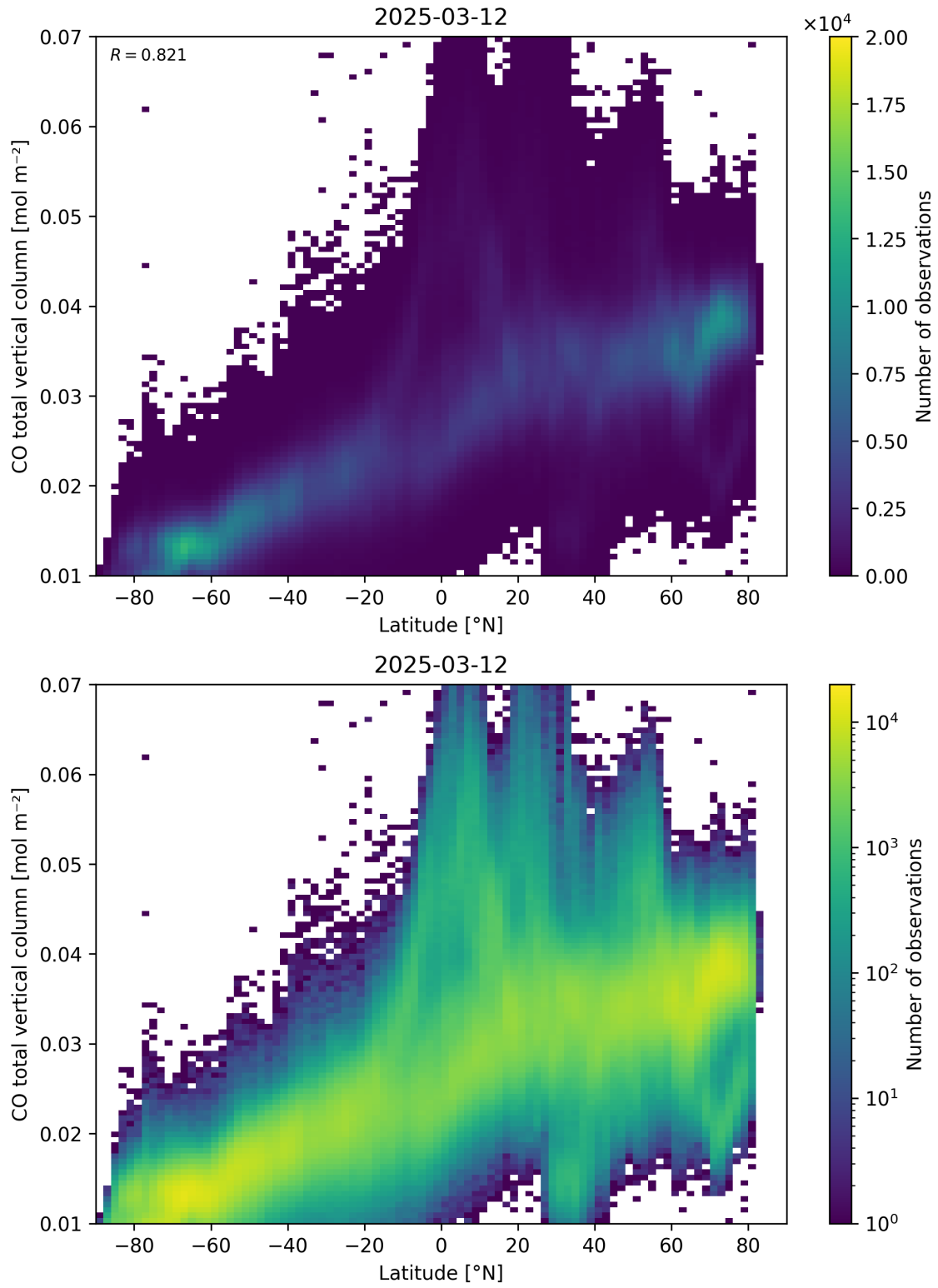
Figure 51: Scatter density plot of “Latitude” against “CO total vertical column” for 2025-03-12 to 2025-03-13.
