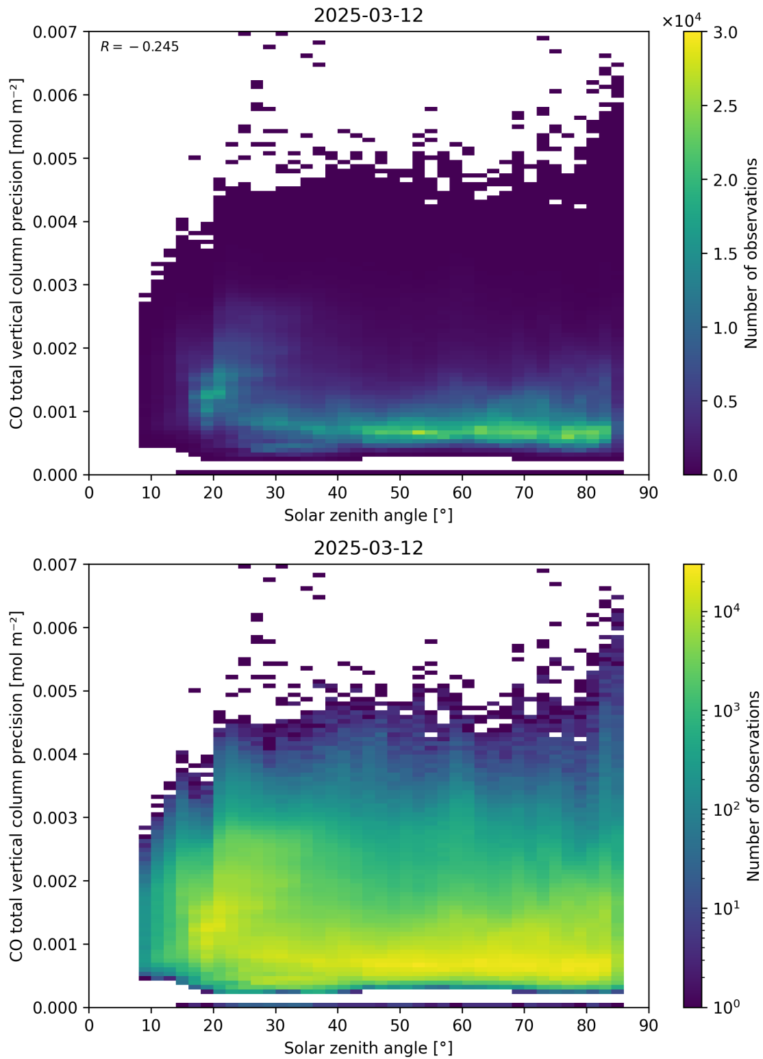
Figure 63: Scatter density plot of “Solar zenith angle” against “CO total vertical column precision” for 2025-03-12 to 2025-03-13.
