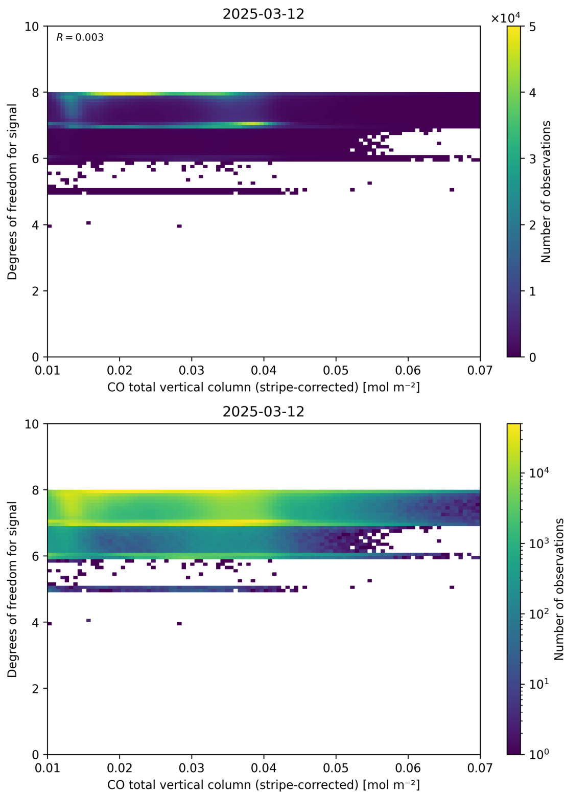
Figure 38: Scatter density plot of “CO total vertical column (stripe-corrected)” against “Degrees of freedom for signal” for 2025-03-12 to 2025-03-13.
