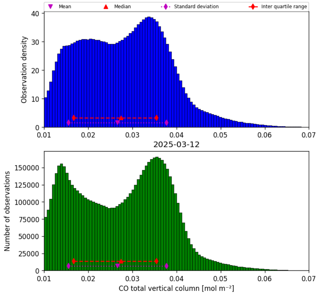
Figure 18: Histogram of “CO total vertical column” for 2025-03-12 to 2025-03-13
