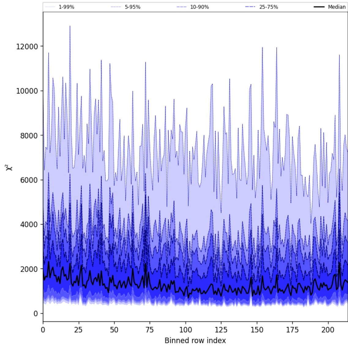
Figure 30: Along track statistics of “ \chi^2 ” for 2025-03-12 to 2025-03-13
