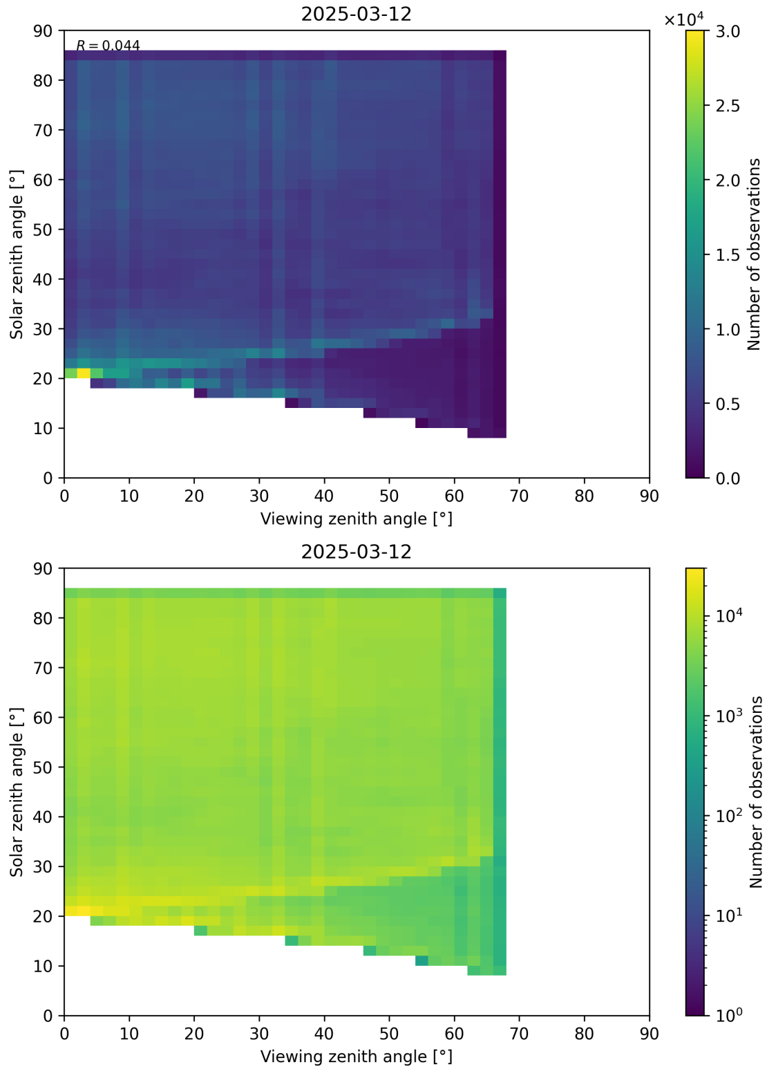
Figure 77: Scatter density plot of “Viewing zenith angle” against “Solar zenith angle” for 2025-03-12 to 2025-03-13.
