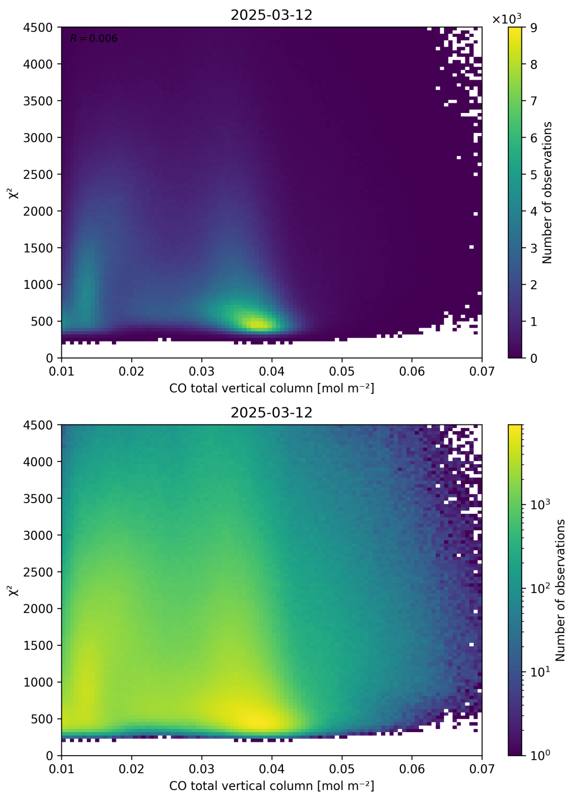
Figure 35: Scatter density plot of “CO total vertical column” against “ \chi^2 ” for 2025-03-12 to 2025-03-13.
