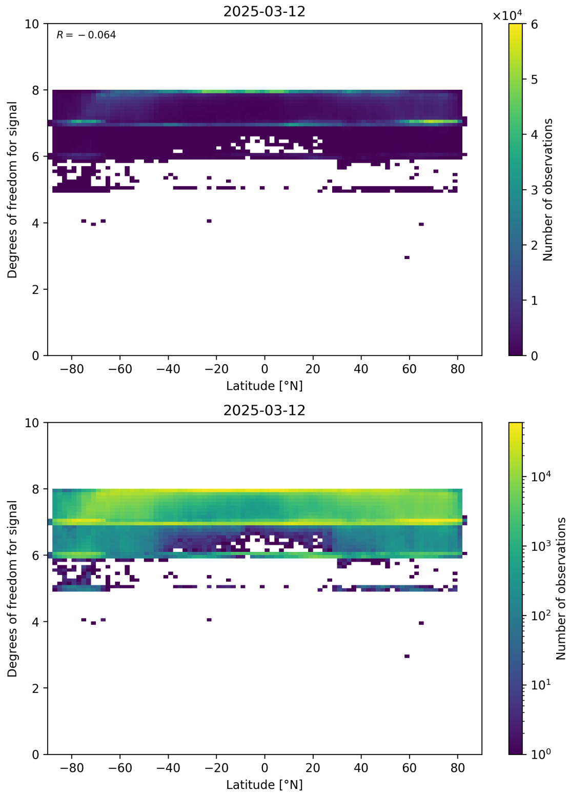
Figure 55: Scatter density plot of “Latitude” against “Degrees of freedom for signal” for 2025-03-12 to 2025-03-13.
