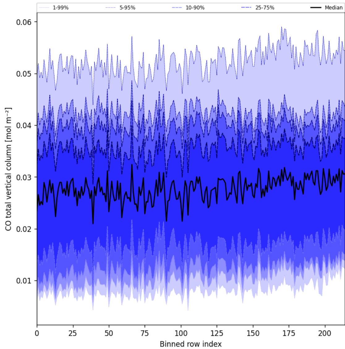
Figure 26: Along track statistics of “CO total vertical column” for 2025-03-12 to 2025-03-13
