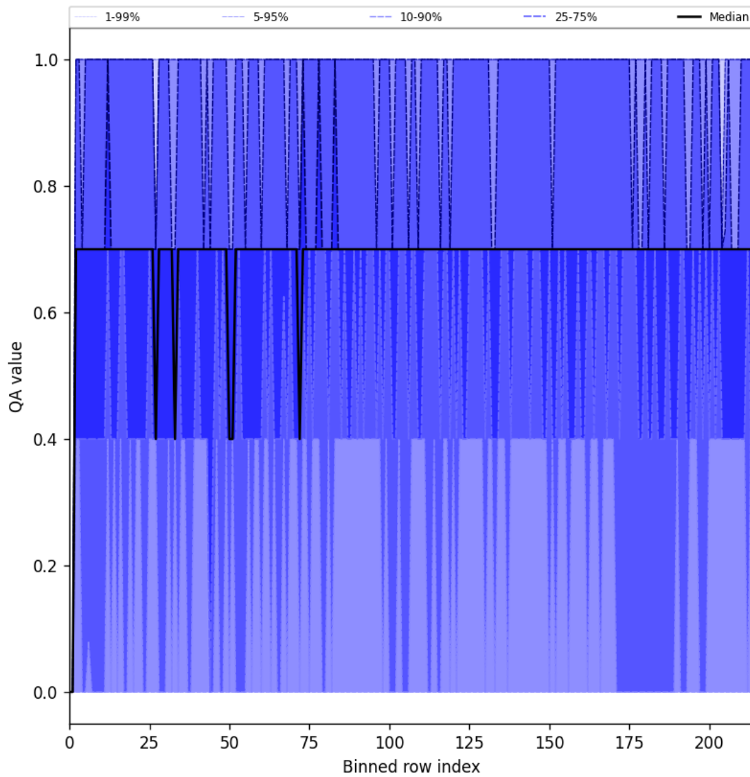
Figure 25: Along track statistics of “QA value” for 2025-03-12 to 2025-03-13
