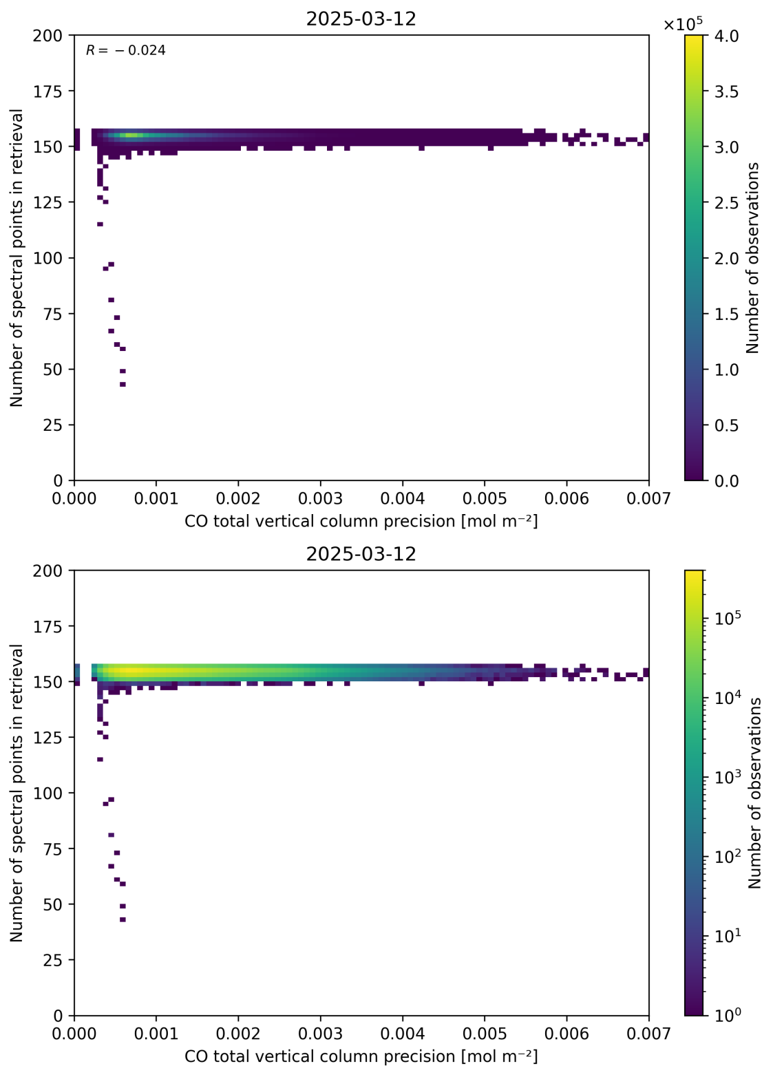
Figure 47: Scatter density plot of “CO total vertical column precision” against “Number of spectral points in retrieval” for 2025-03-12 to 2025-03-13.
