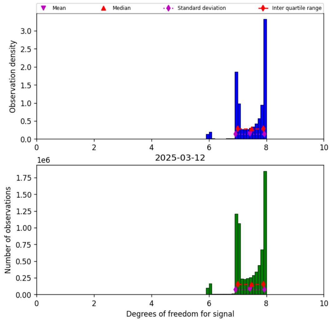
Figure 23: Histogram of “Degrees of freedom for signal” for 2025-03-12 to 2025-03-13
