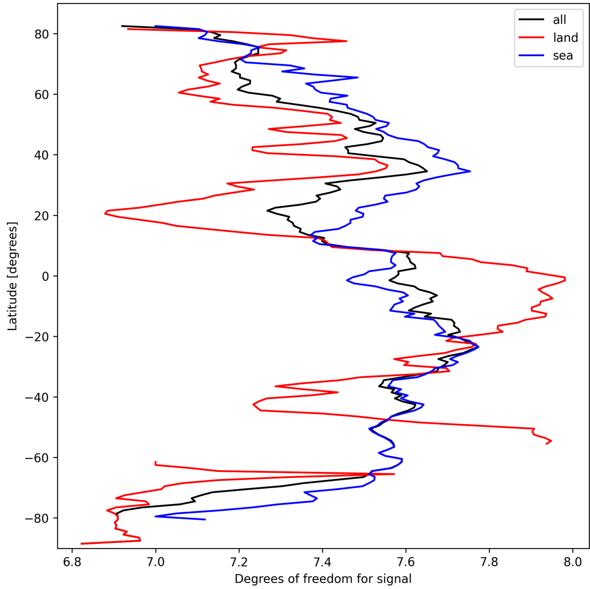
Figure 15: Zonal average of “Degrees of freedom for signal” for 2025-03-12 to 2025-03-13.
