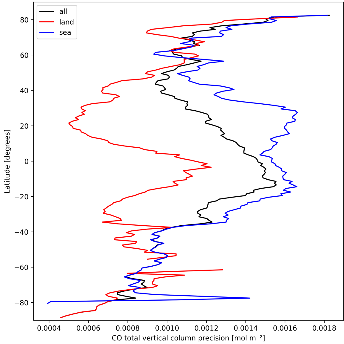
Figure 12: Zonal average of “CO total vertical column precision” for 2025-03-12 to 2025-03-13.
