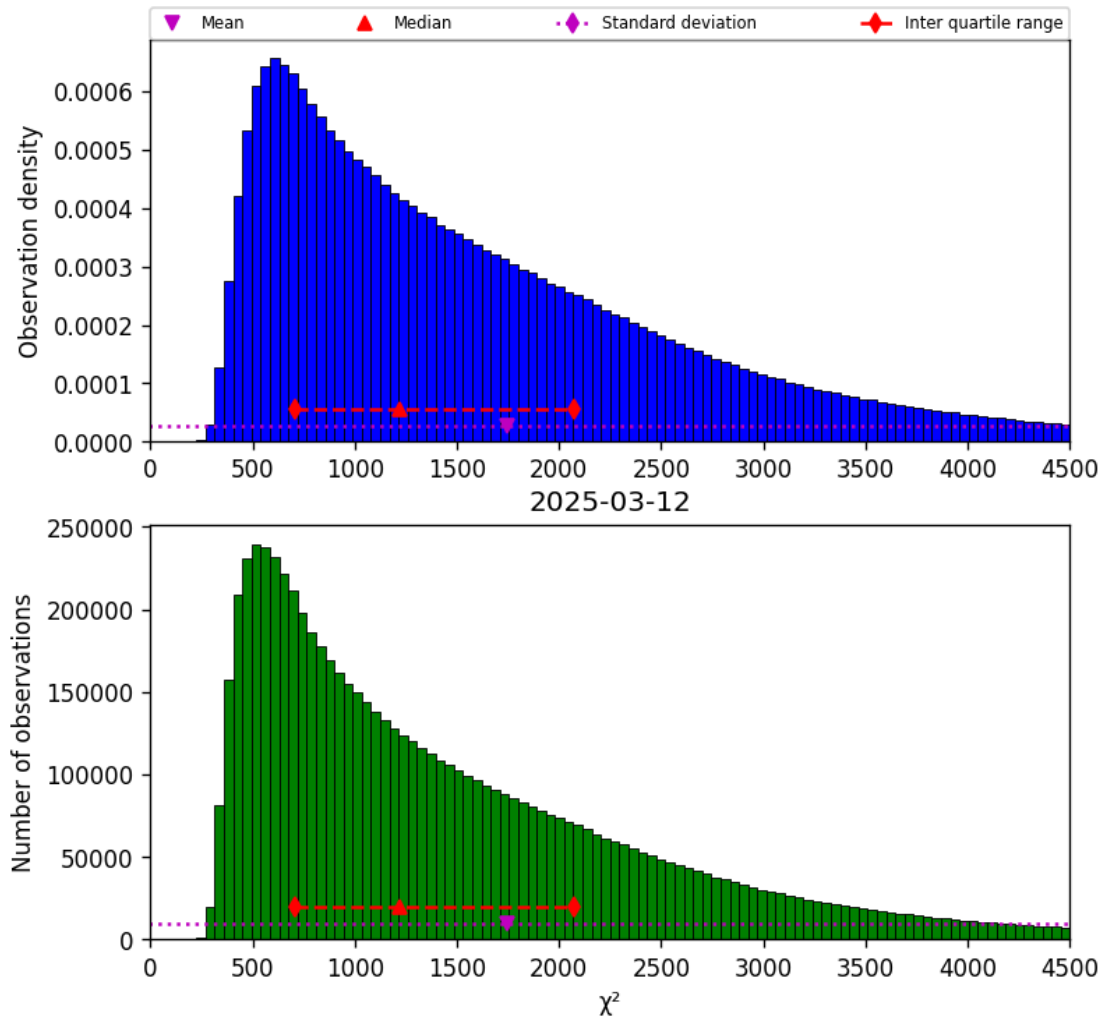
Figure 22: Histogram of “ \chi^2 ” for 2025-03-12 to 2025-03-13
