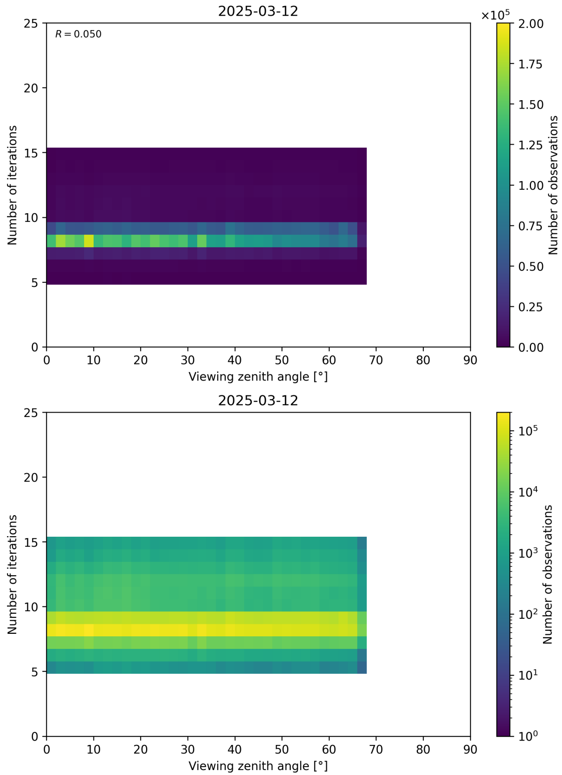
Figure 75: Scatter density plot of “Viewing zenith angle” against “Number of iterations” for 2025-03-12 to 2025-03-13.
