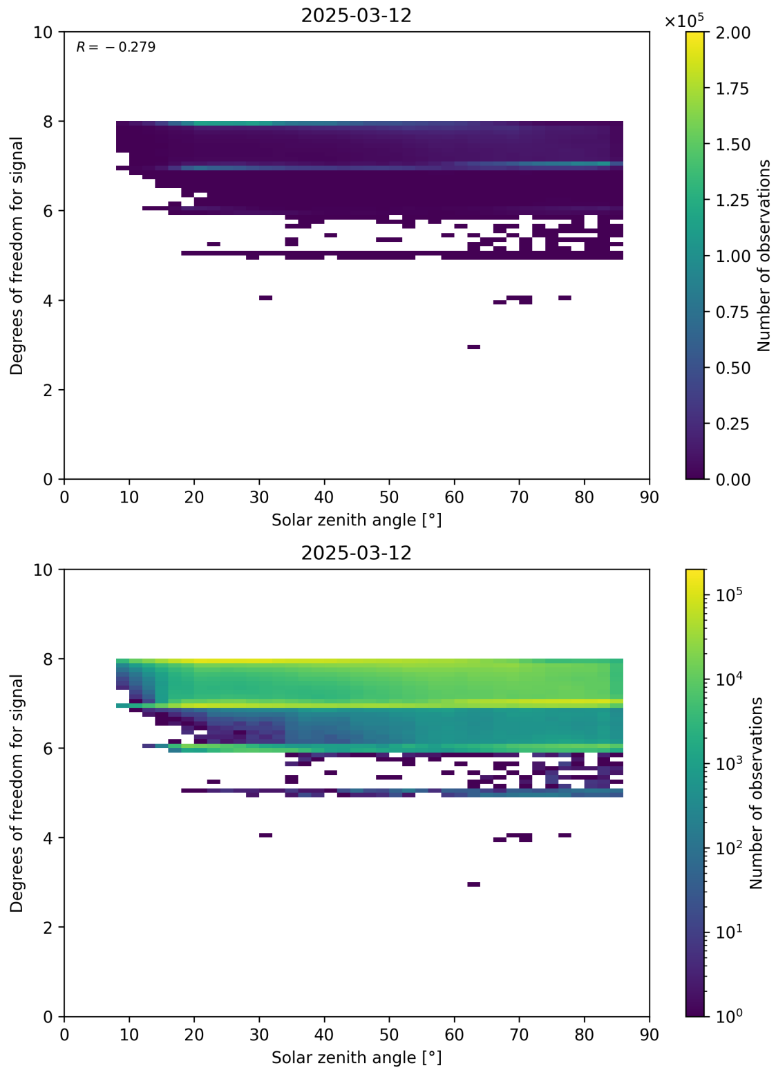
Figure 65: Scatter density plot of “Solar zenith angle” against “Degrees of freedom for signal” for 2025-03-12 to 2025-03-13.
