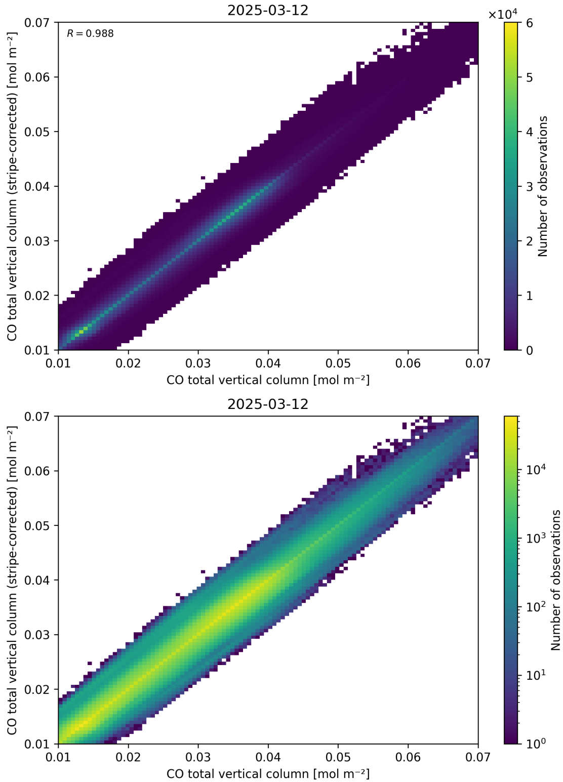
Figure 33: Scatter density plot of “CO total vertical column” against “CO total vertical column (stripe-corrected)” for 2025-03-12 to 2025-03-13.
