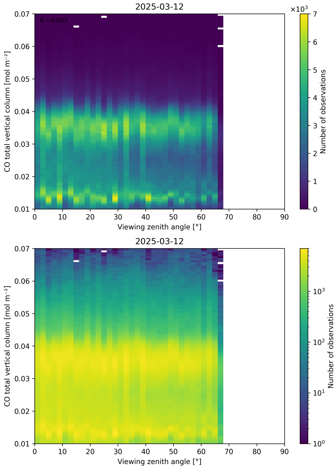
Figure 69: Scatter density plot of “Viewing zenith angle” against “CO total vertical column” for 2025-03-12 to 2025-03-13.
