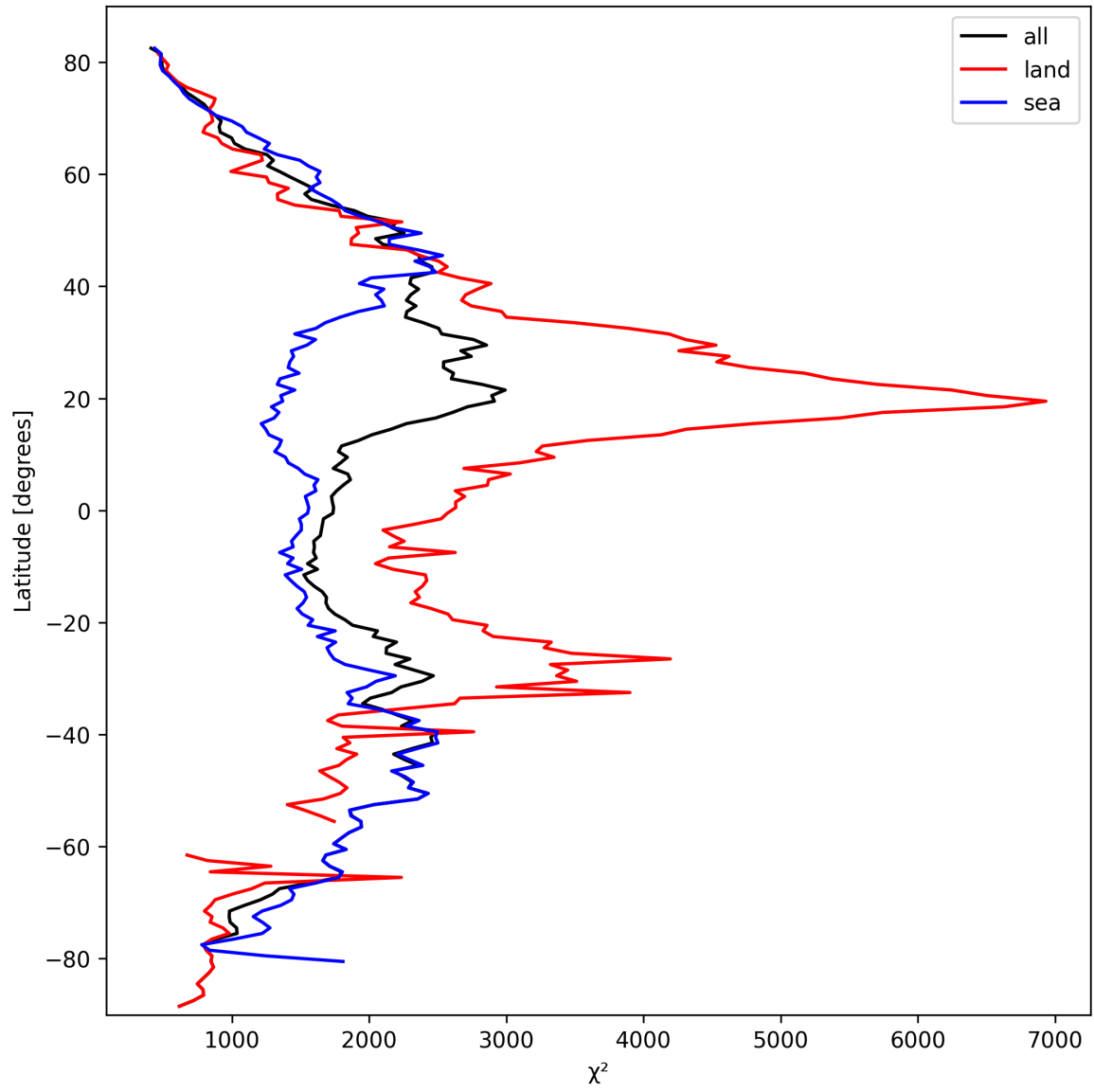
Figure 14: Zonal average of “ \chi^2 ” for 2025-03-12 to 2025-03-13.
