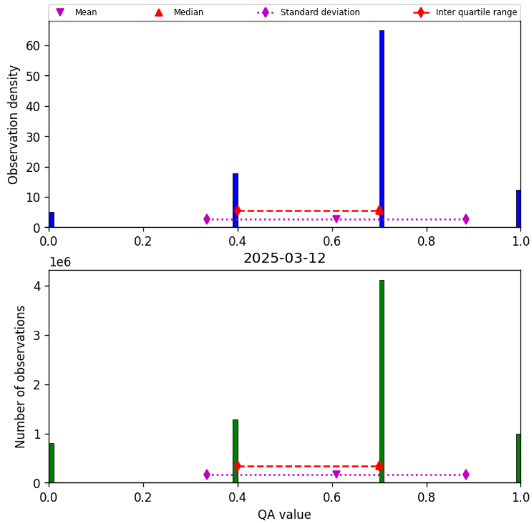
Figure 17: Histogram of “QA value” for 2025-03-12 to 2025-03-13
