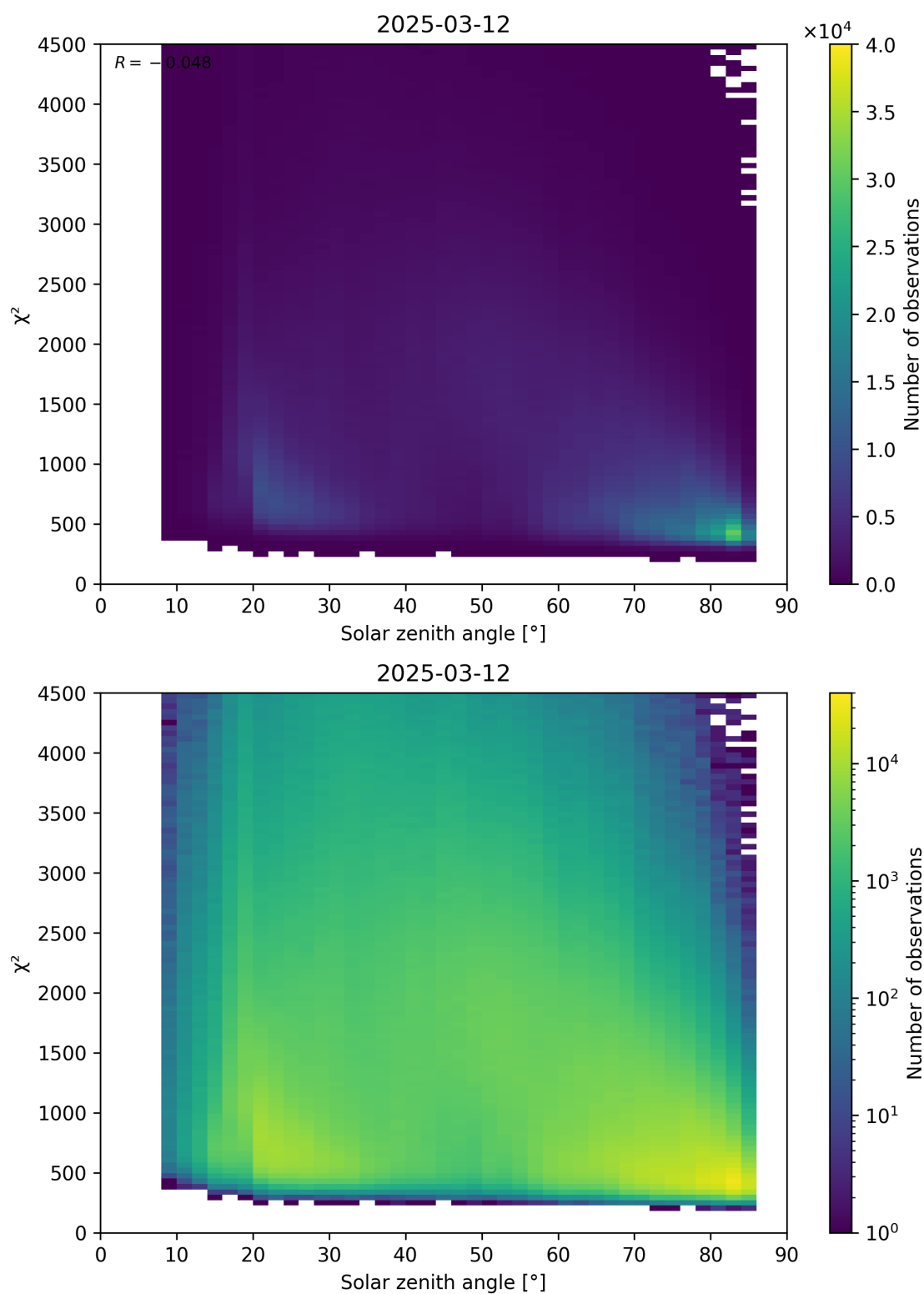
Figure 64: Scatter density plot of “Solar zenith angle” against “ \chi^2 ” for 2025-03-12 to 2025-03-13.
