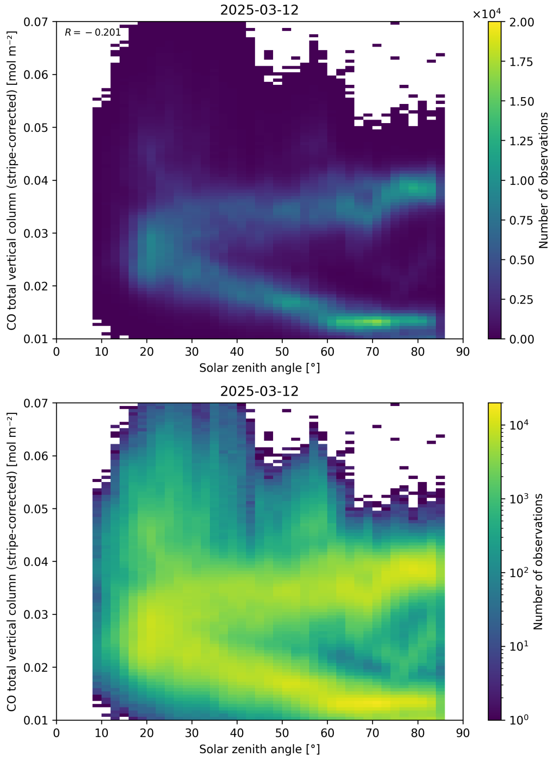
Figure 62: Scatter density plot of “Solar zenith angle” against “CO total vertical column (stripe-corrected)” for 2025-03-12 to 2025-03-13.
