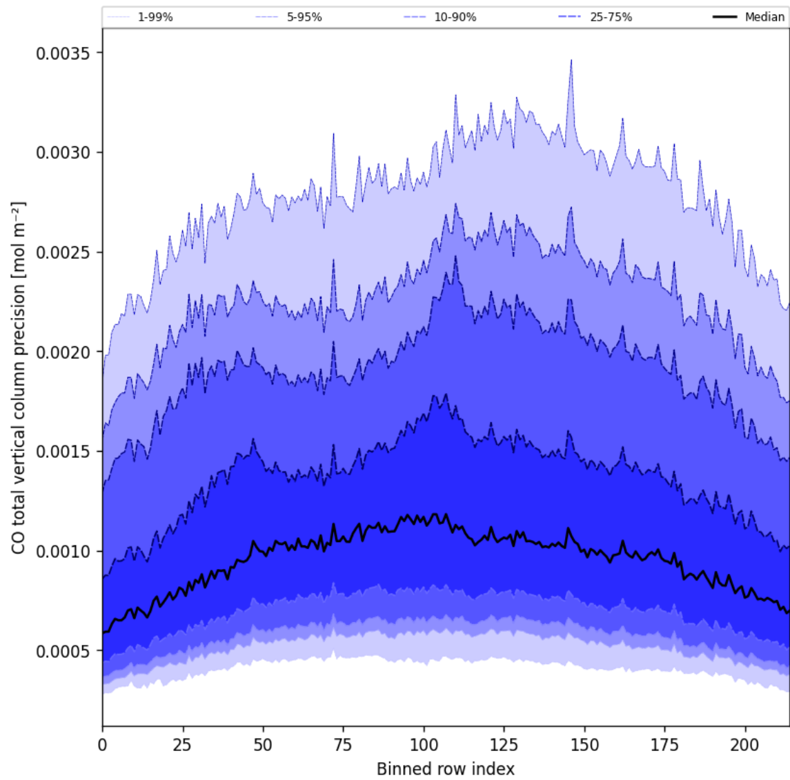
Figure 28: Along track statistics of “CO total vertical column precision” for 2025-03-12 to 2025-03-13
