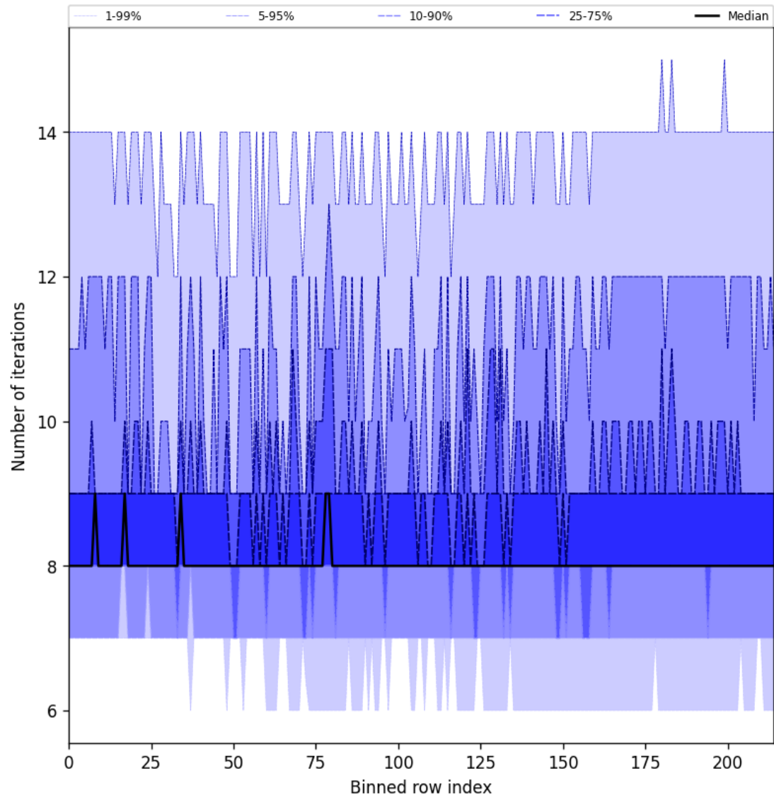
Figure 32: Along track statistics of “Number of iterations” for 2025-03-12 to 2025-03-13
