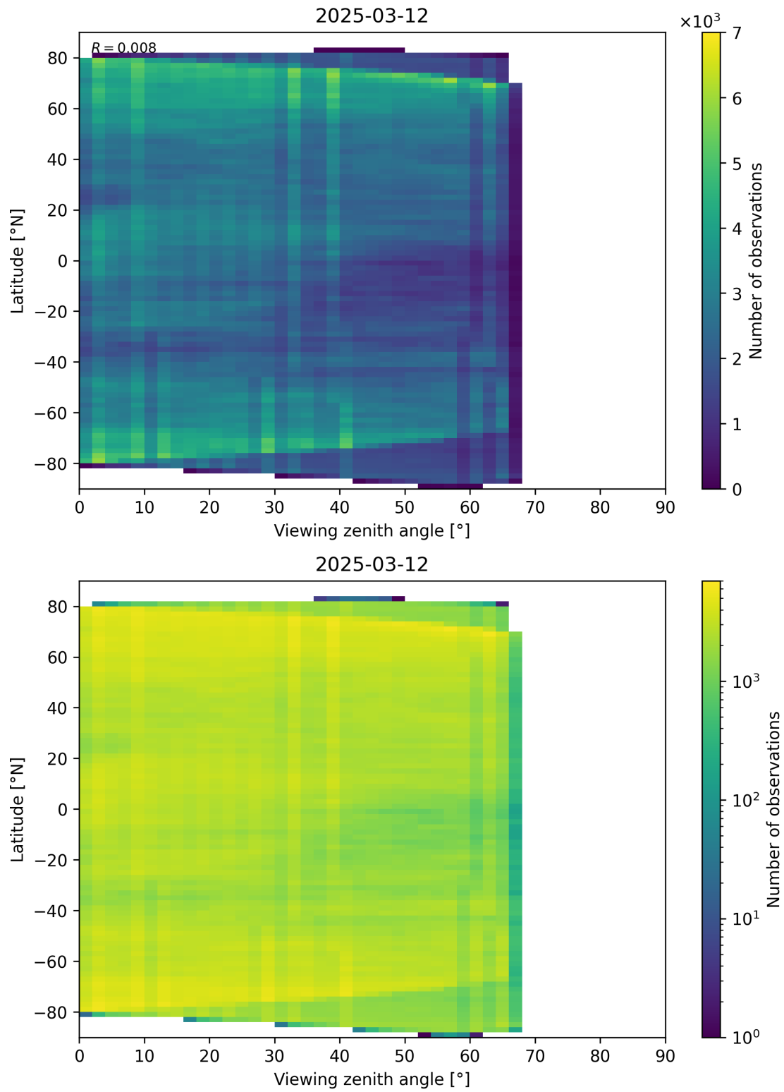
Figure 74: Scatter density plot of “Viewing zenith angle” against “Latitude” for 2025-03-12 to 2025-03-13.
