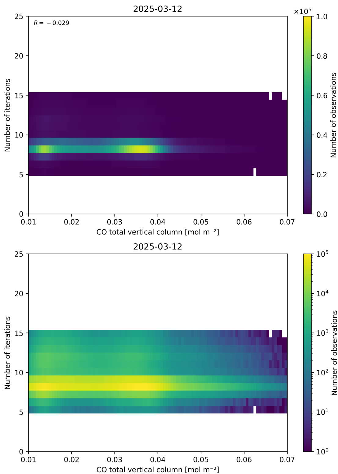
Figure 42: Scatter density plot of “CO total vertical column” against “Number of iterations” for 2025-03-12 to 2025-03-13.
