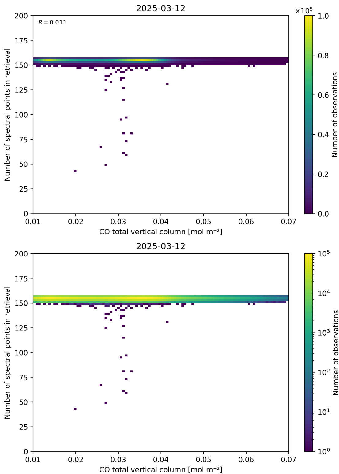
Figure 43: Scatter density plot of “CO total vertical column” against “Number of spectral points in retrieval” for 2025-03-12 to 2025-03-13.
