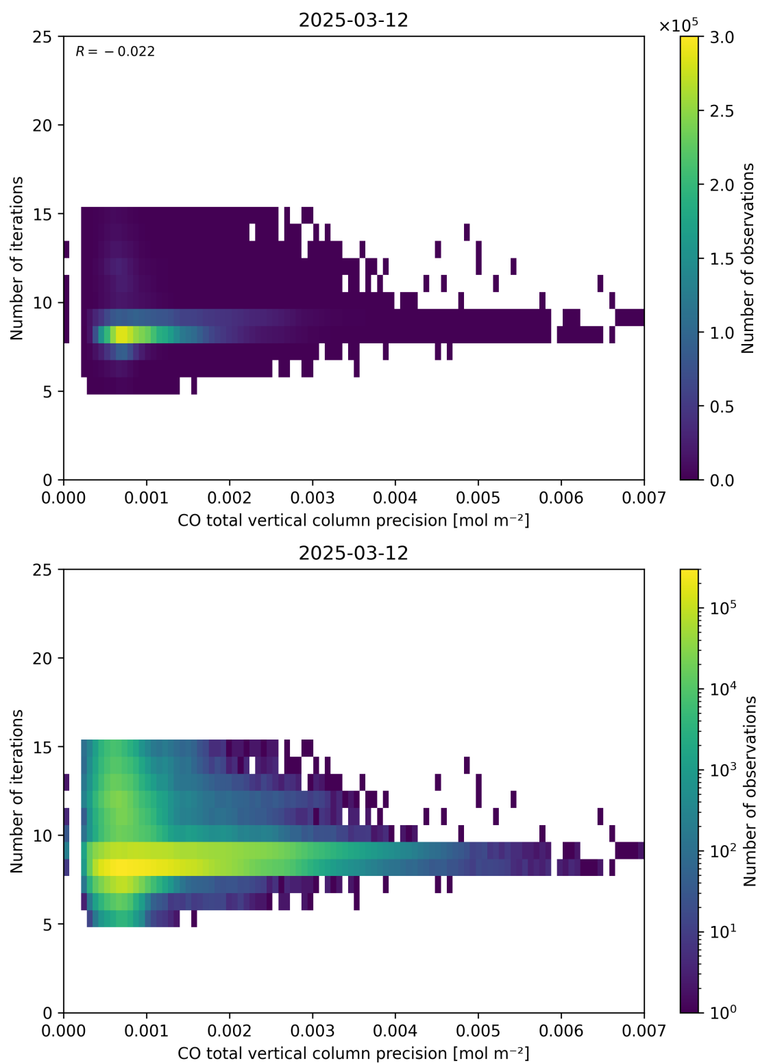
Figure 46: Scatter density plot of “CO total vertical column precision” against “Number of iterations” for 2025-03-12 to 2025-03-13.
