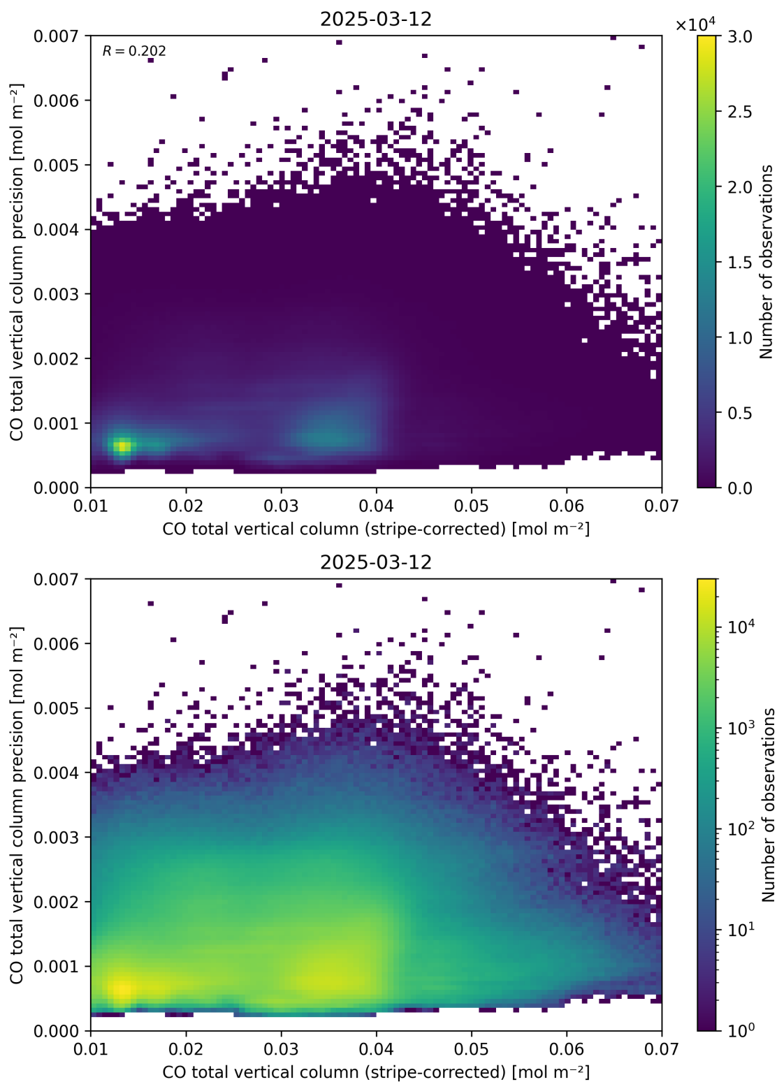
Figure 36: Scatter density plot of “CO total vertical column (stripe-corrected)” against “CO total vertical column precision” for 2025-03-12 to 2025-03-13.
