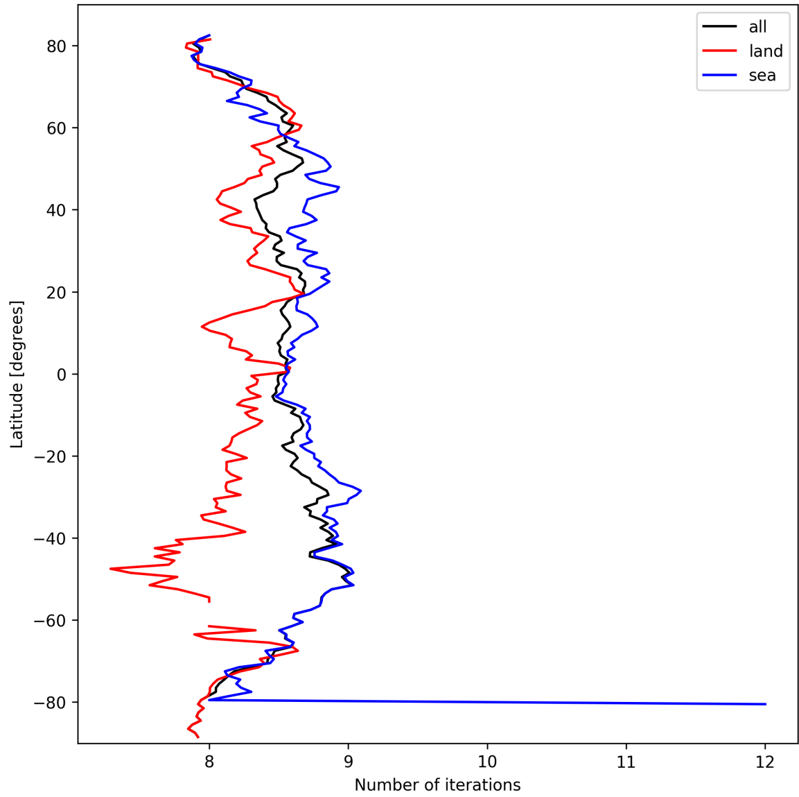
Figure 16: Zonal average of “Number of iterations” for 2025-03-12 to 2025-03-13.
