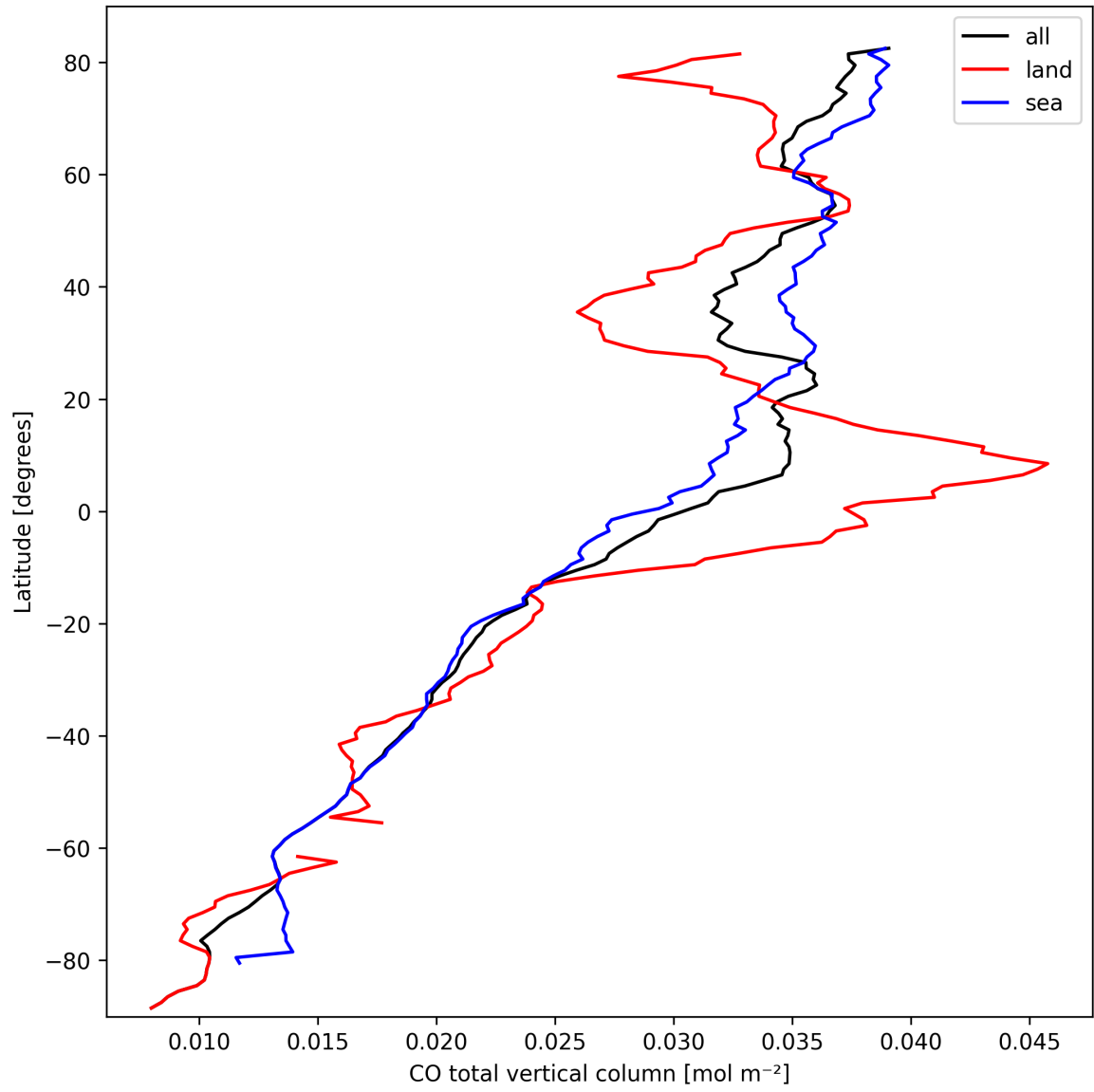
Figure 10: Zonal average of “CO total vertical column” for 2025-03-12 to 2025-03-13.
