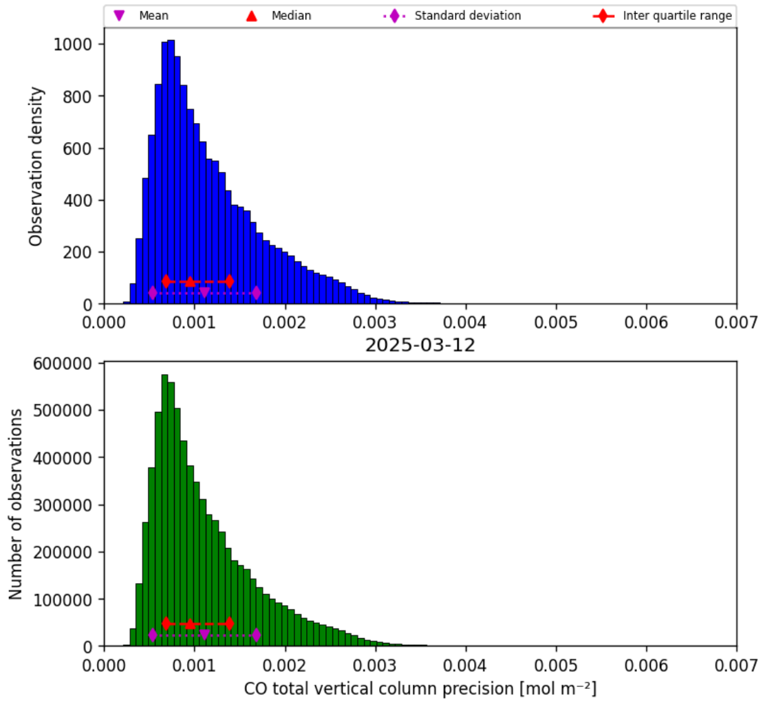
Figure 20: Histogram of “CO total vertical column precision” for 2025-03-12 to 2025-03-13
