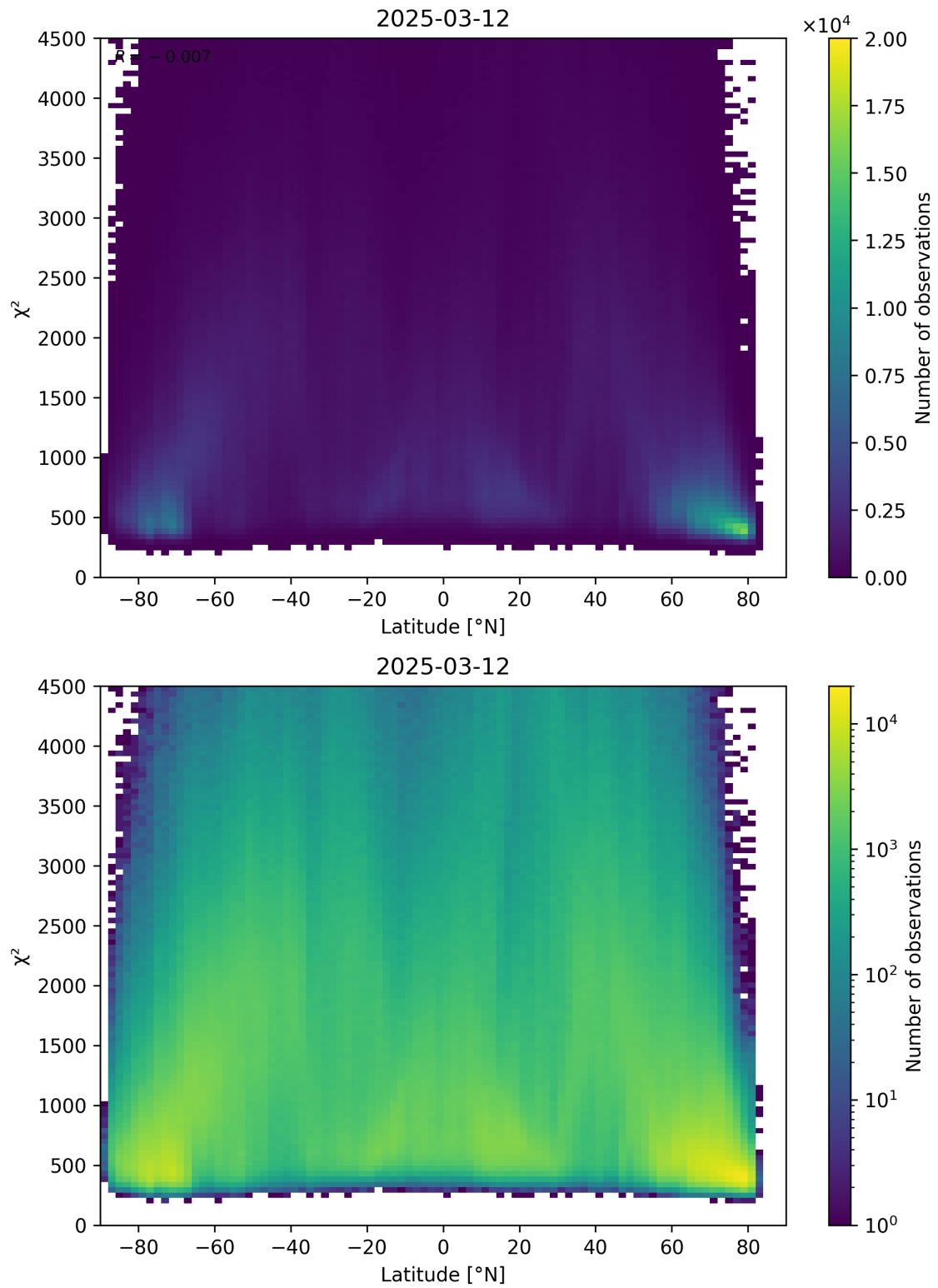
Figure 54: Scatter density plot of “Latitude” against “ \chi^2 ” for 2025-03-12 to 2025-03-13.
