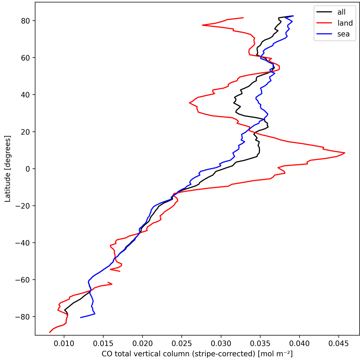
Figure 11: Zonal average of “CO total vertical column (stripe-corrected)” for 2025-03-12 to 2025-03-13.
