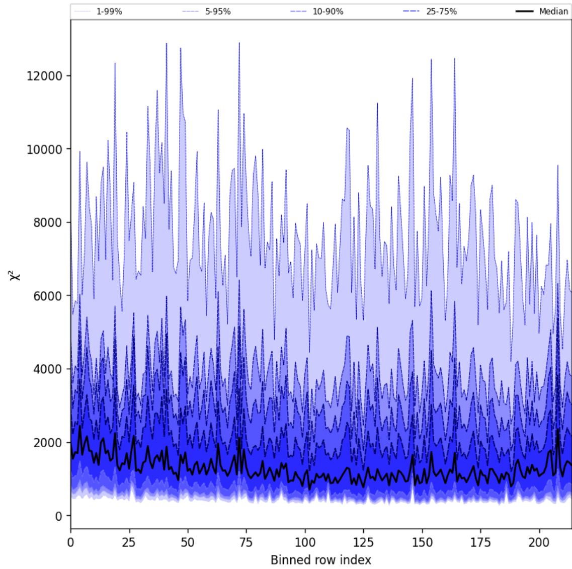
Figure 30: Along track statistics of “ \chi^2 ” for 2025-03-13 to 2025-03-15
