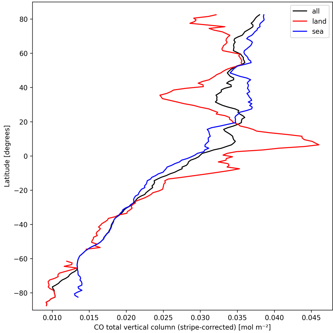
Figure 11: Zonal average of “CO total vertical column (stripe-corrected)” for 2025-03-13 to 2025-03-15.
