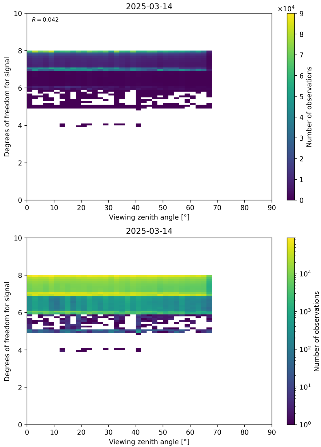
Figure 73: Scatter density plot of “Viewing zenith angle” against “Degrees of freedom for signal” for 2025-03-13 to 2025-03-15.
