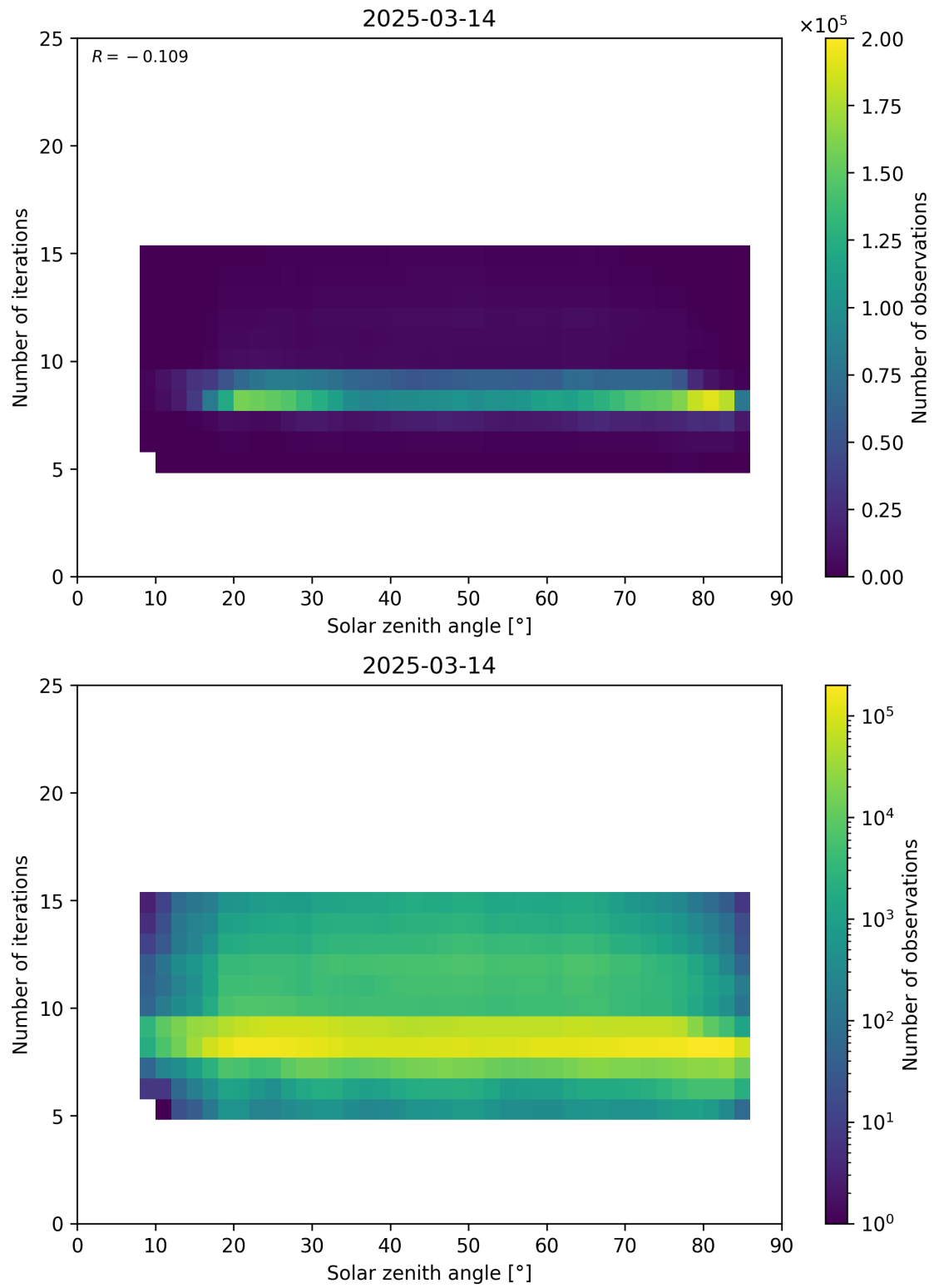
Figure 67: Scatter density plot of “Solar zenith angle” against “Number of iterations” for 2025-03-13 to 2025-03-15.
