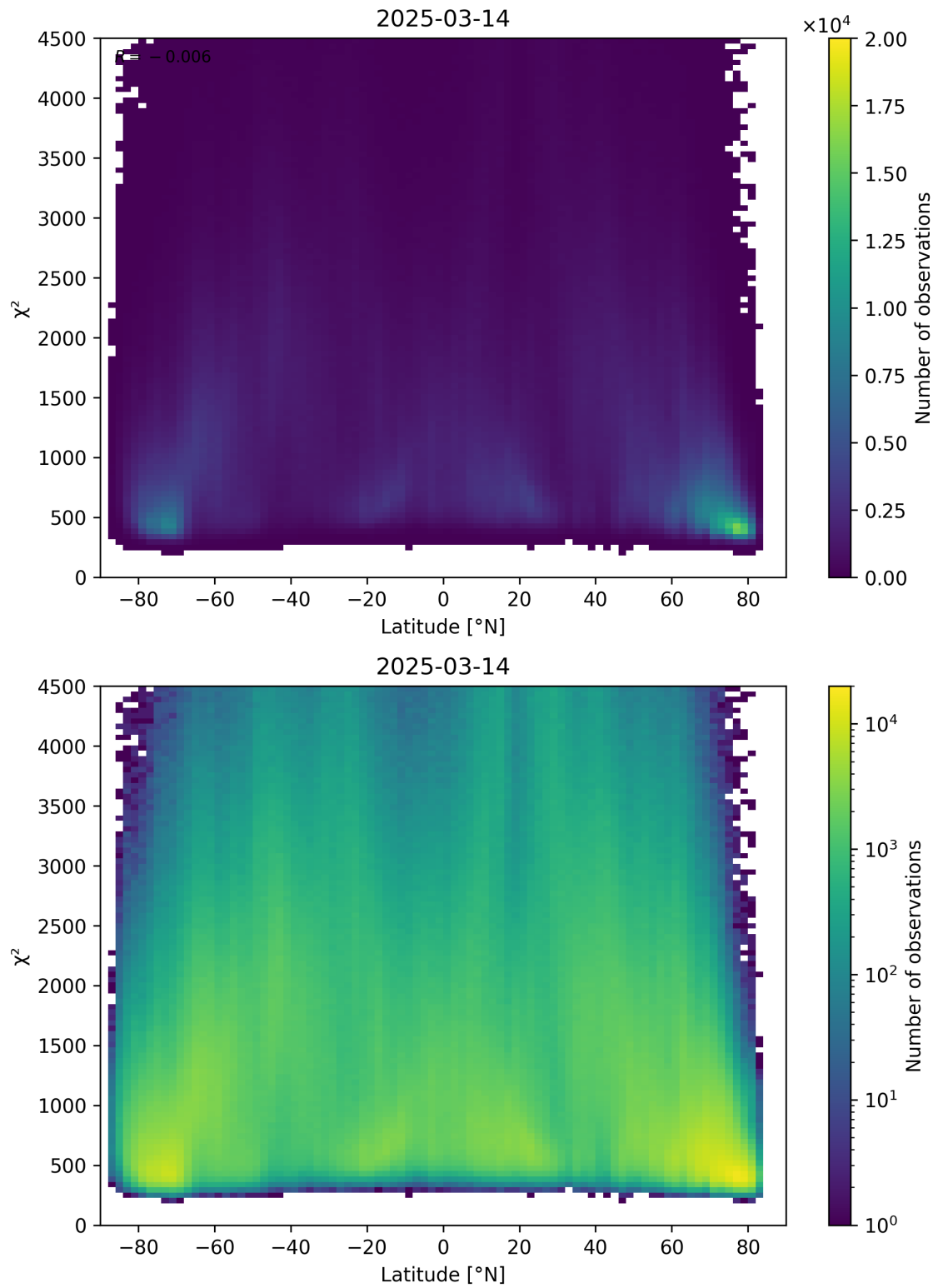
Figure 54: Scatter density plot of “Latitude” against “ \chi^2 ” for 2025-03-13 to 2025-03-15.
