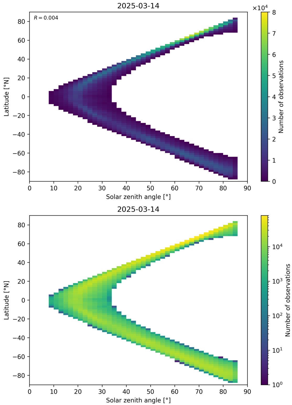
Figure 66: Scatter density plot of “Solar zenith angle” against “Latitude” for 2025-03-13 to 2025-03-15.
