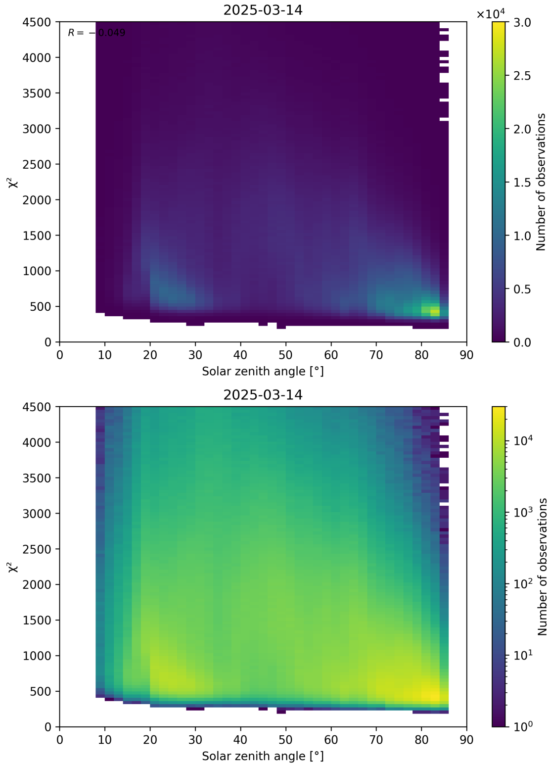
Figure 64: Scatter density plot of “Solar zenith angle” against “ \chi^2 ” for 2025-03-13 to 2025-03-15.
