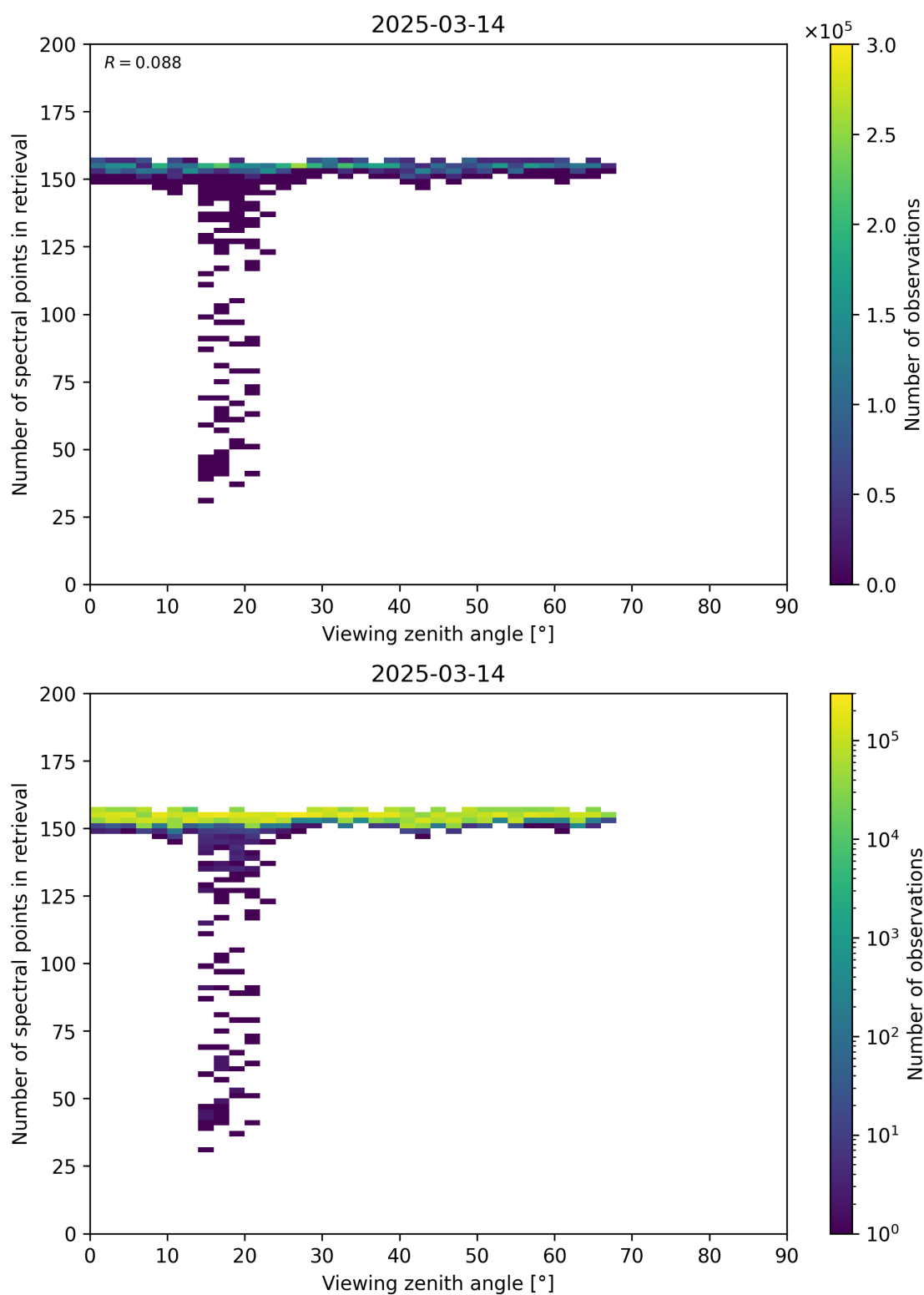
Figure 76: Scatter density plot of “Viewing zenith angle” against “Number of spectral points in retrieval” for 2025-03-13 to 2025-03-15.
