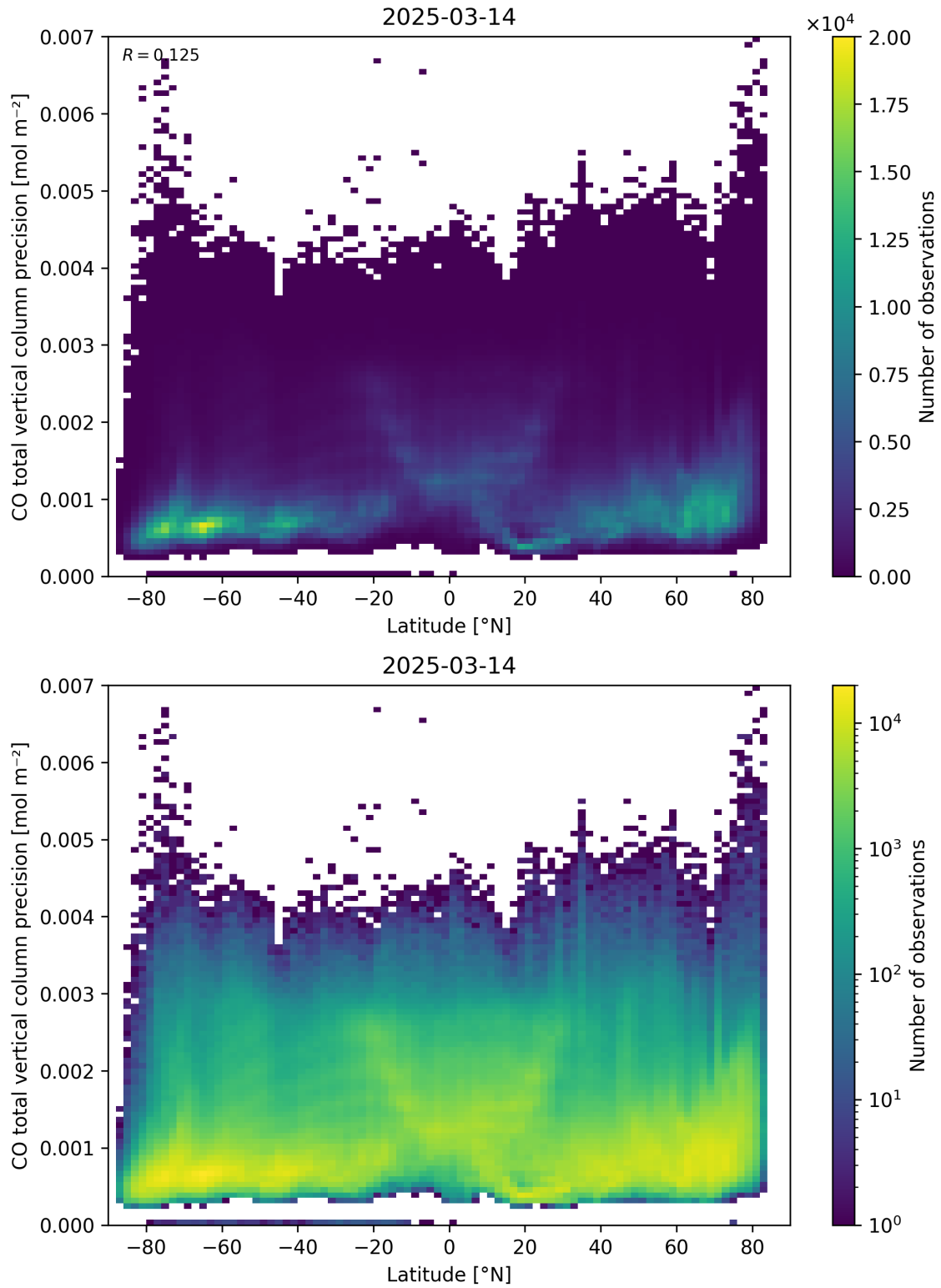
Figure 53: Scatter density plot of “Latitude” against “CO total vertical column precision” for 2025-03-13 to 2025-03-15.
