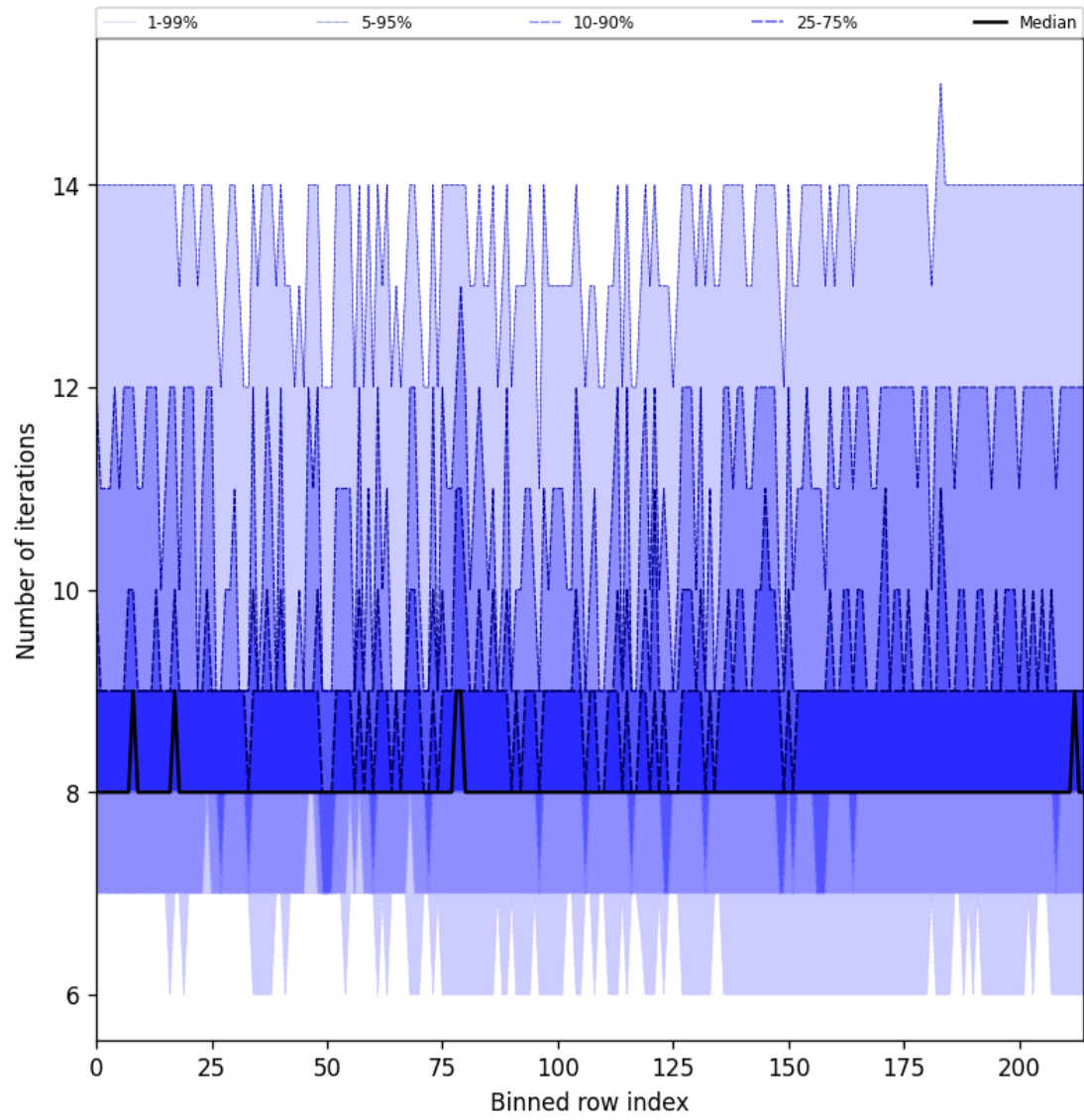
Figure 32: Along track statistics of “Number of iterations” for 2025-03-13 to 2025-03-15
