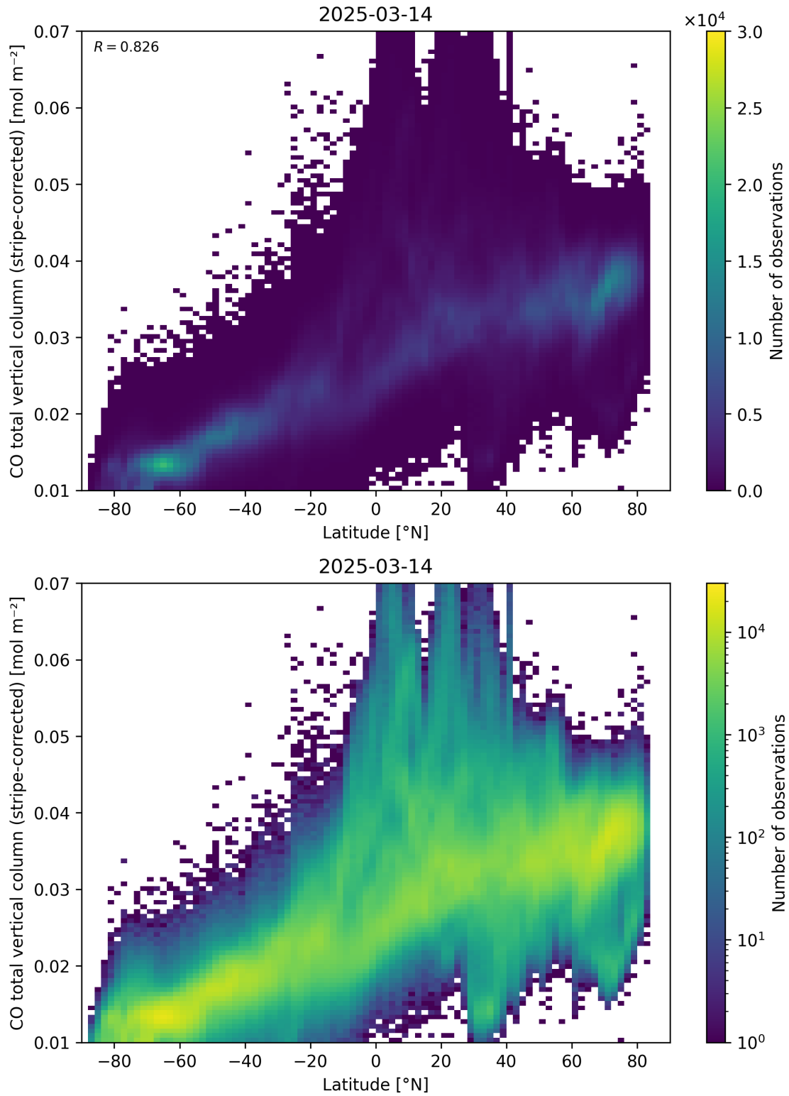
Figure 52: Scatter density plot of “Latitude” against “CO total vertical column (stripe-corrected)” for 2025-03-13 to 2025-03-15.
