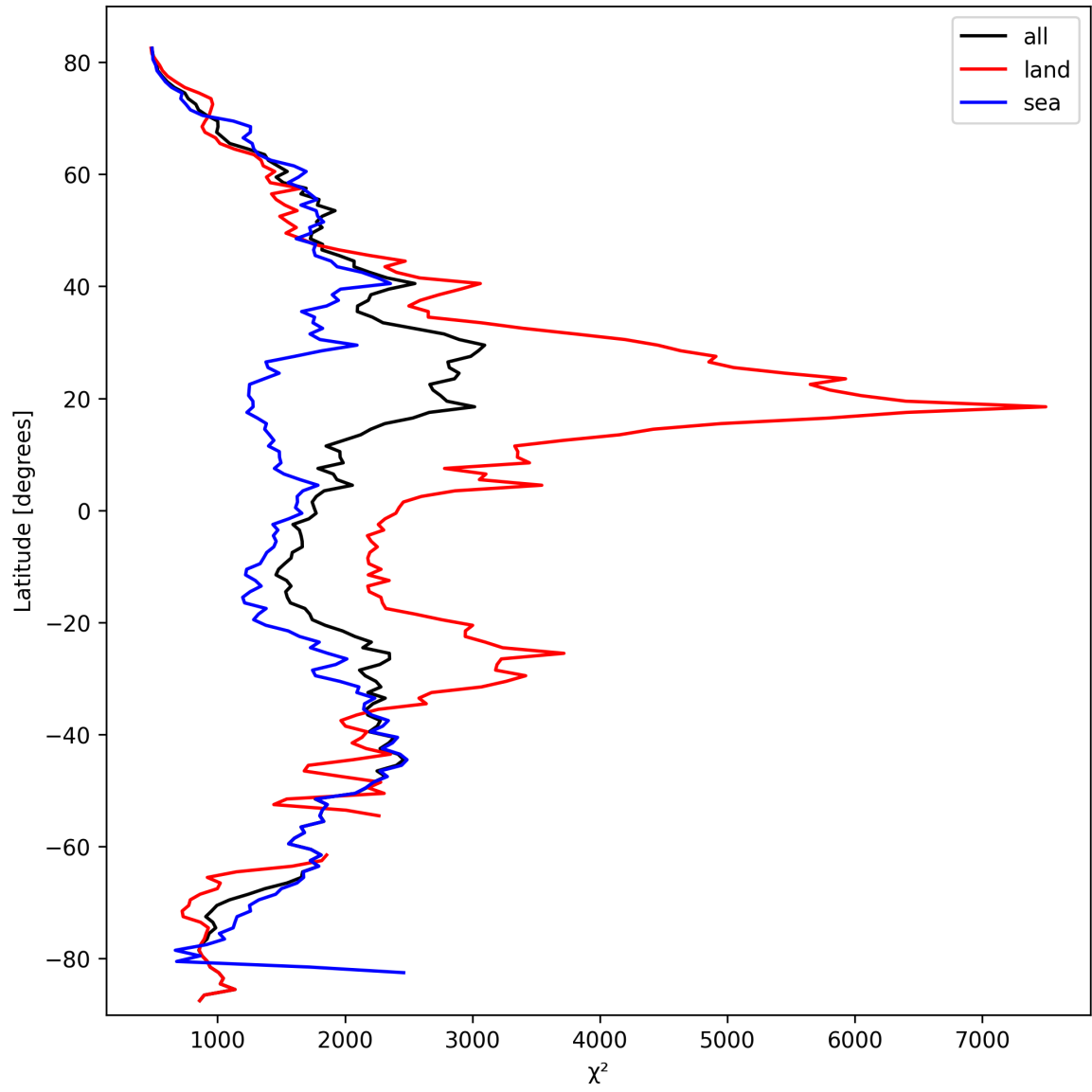
Figure 14: Zonal average of “ \chi^2 ” for 2025-03-13 to 2025-03-15.
