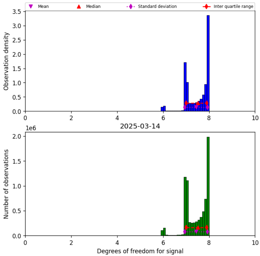
Figure 23: Histogram of “Degrees of freedom for signal” for 2025-03-13 to 2025-03-15
