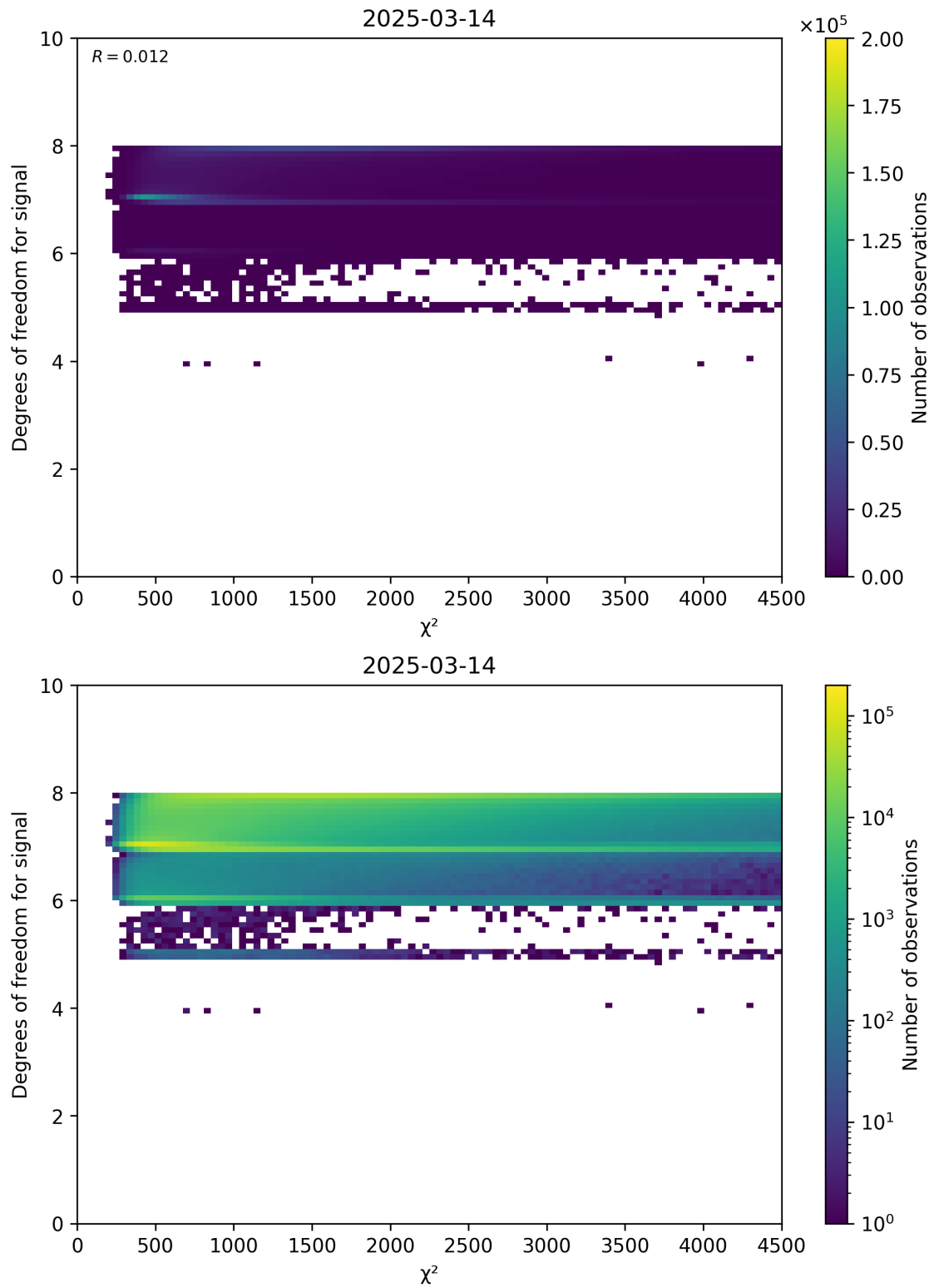
Figure 48: Scatter density plot of “ \chi^2 ” against “Degrees of freedom for signal” for 2025-03-13 to 2025-03-15.
