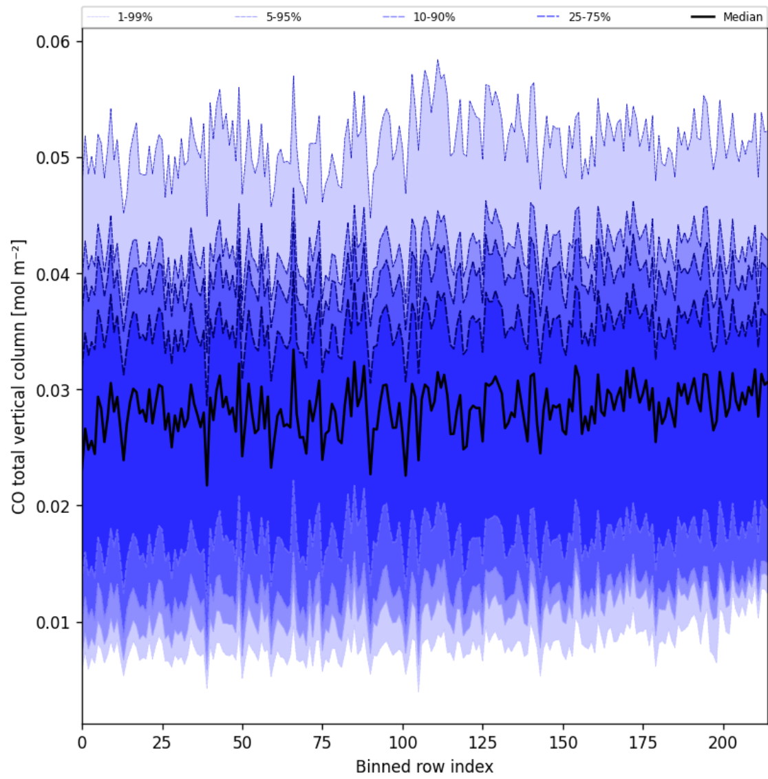
Figure 26: Along track statistics of “CO total vertical column” for 2025-03-13 to 2025-03-15
