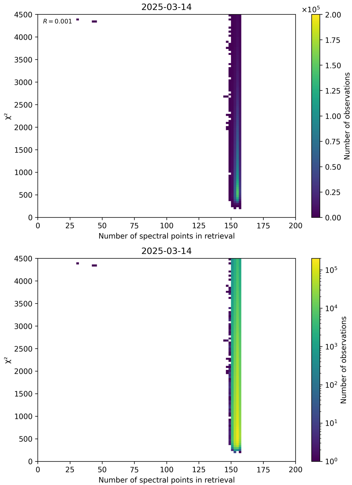
Figure 58: Scatter density plot of “Number of spectral points in retrieval” against “ \chi^2 ” for 2025-03-13 to 2025-03-15.
