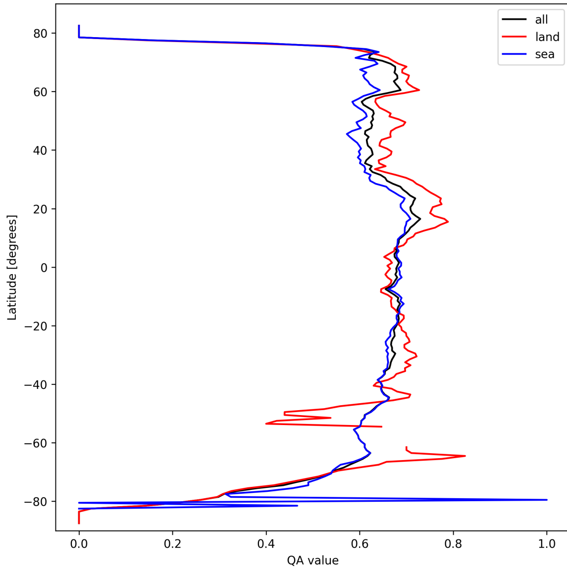
Figure 9: Zonal average of “QA value” for 2025-03-13 to 2025-03-15.
