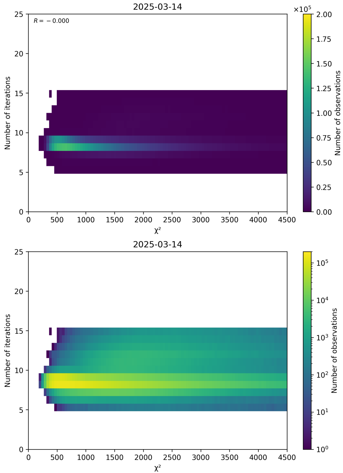
Figure 49: Scatter density plot of “ \chi^2 ” against “Number of iterations” for 2025-03-13 to 2025-03-15.
