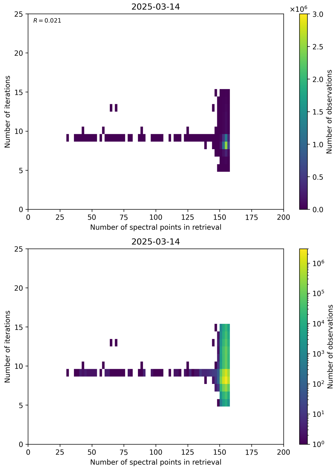
Figure 60: Scatter density plot of “Number of spectral points in retrieval” against “Number of iterations” for 2025-03-13 to 2025-03-15.
