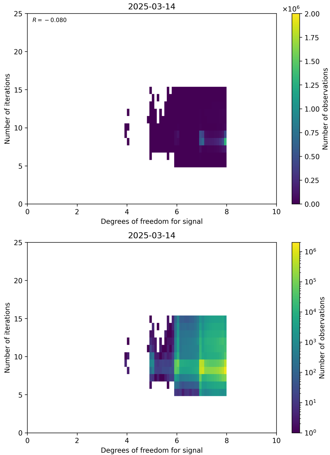
Figure 50: Scatter density plot of “Degrees of freedom for signal” against “Number of iterations” for 2025-03-13 to 2025-03-15.
