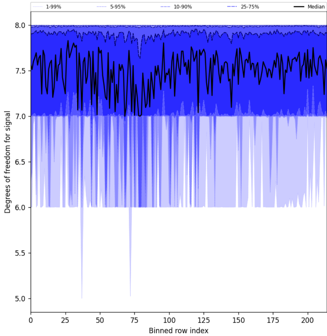
Figure 31: Along track statistics of “Degrees of freedom for signal” for 2025-03-13 to 2025-03-15
