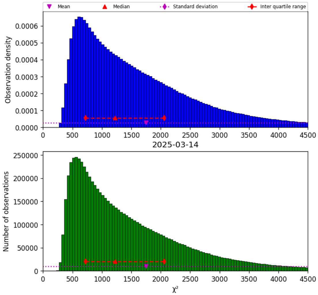
Figure 22: Histogram of “ \chi^2 ” for 2025-03-13 to 2025-03-15
