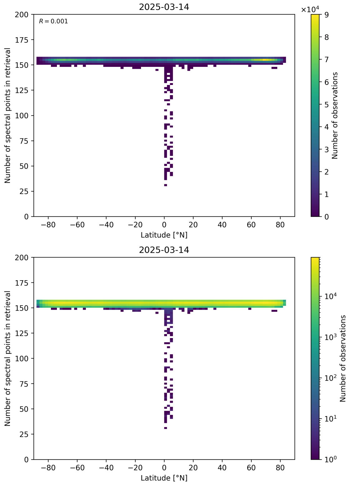
Figure 57: Scatter density plot of “Latitude” against “Number of spectral points in retrieval” for 2025-03-13 to 2025-03-15.
