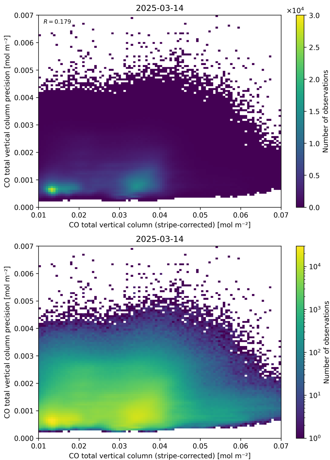
Figure 36: Scatter density plot of “CO total vertical column (stripe-corrected)” against “CO total vertical column precision” for 2025-03-13 to 2025-03-15.
