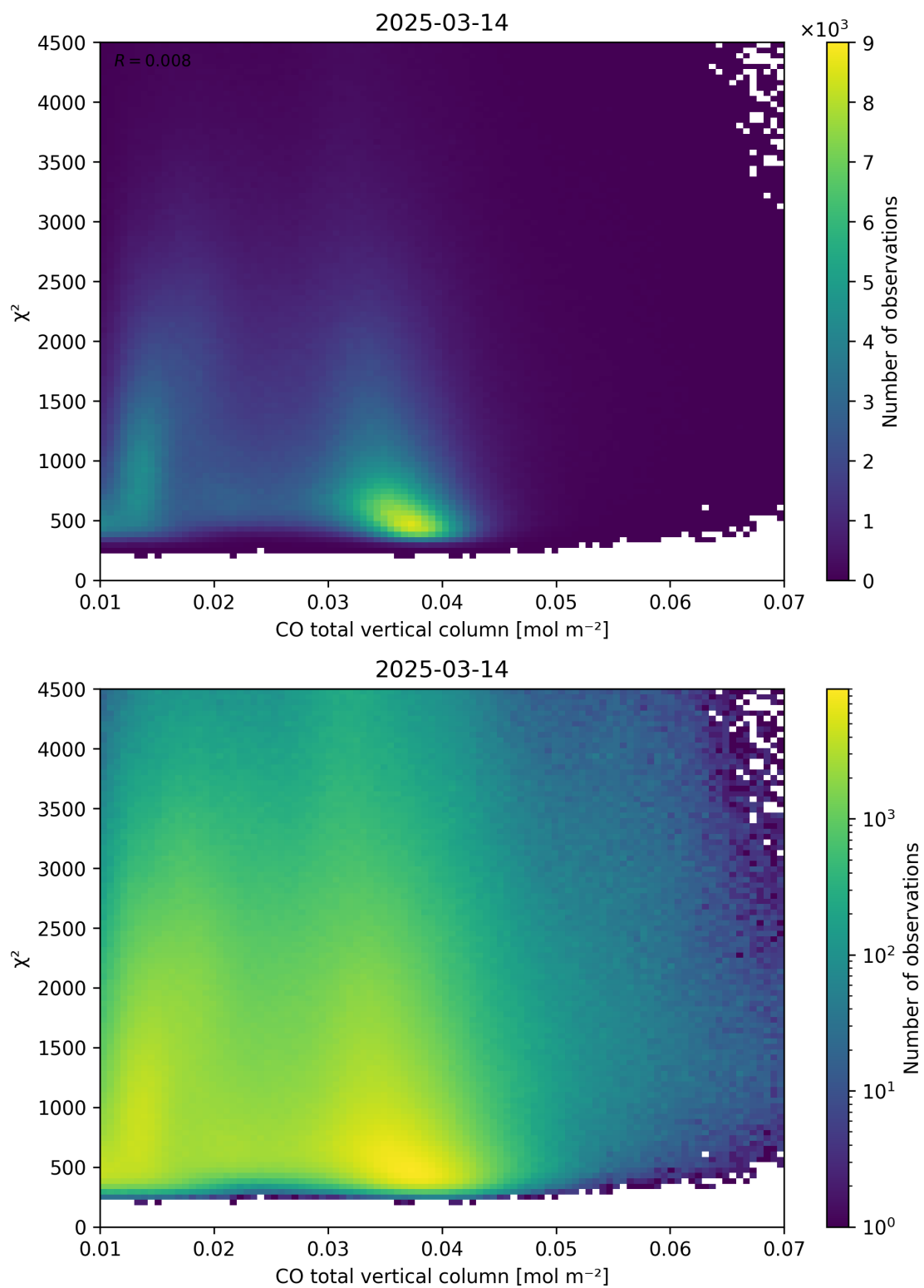
Figure 35: Scatter density plot of “CO total vertical column” against “ \chi^2 ” for 2025-03-13 to 2025-03-15.
