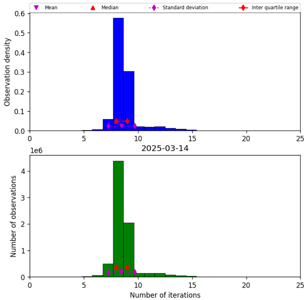
Figure 24: Histogram of “Number of iterations” for 2025-03-13 to 2025-03-15
