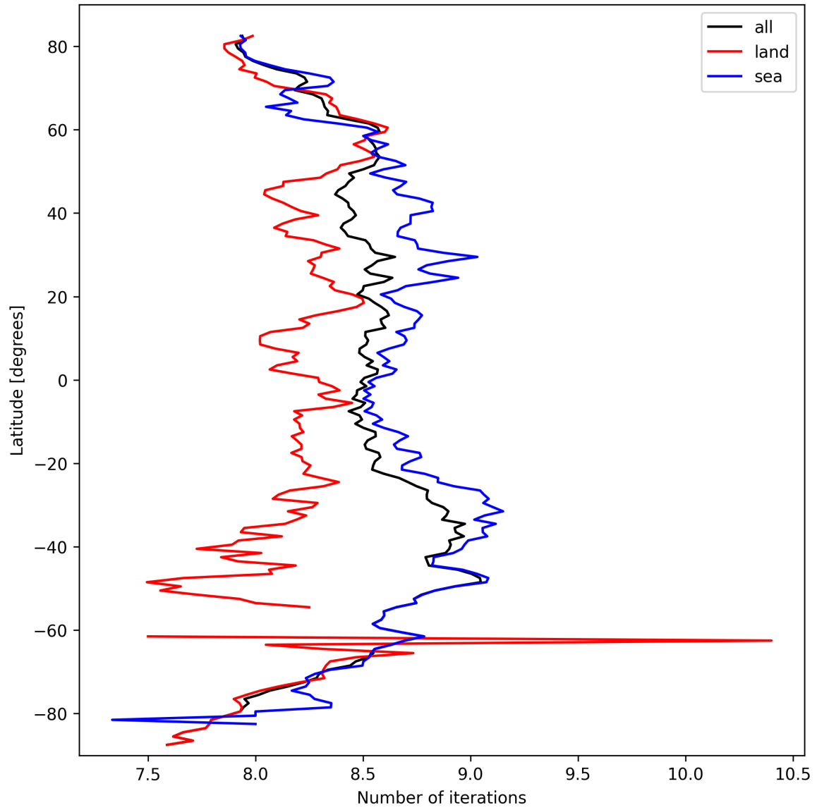
Figure 16: Zonal average of “Number of iterations” for 2025-03-13 to 2025-03-15.
