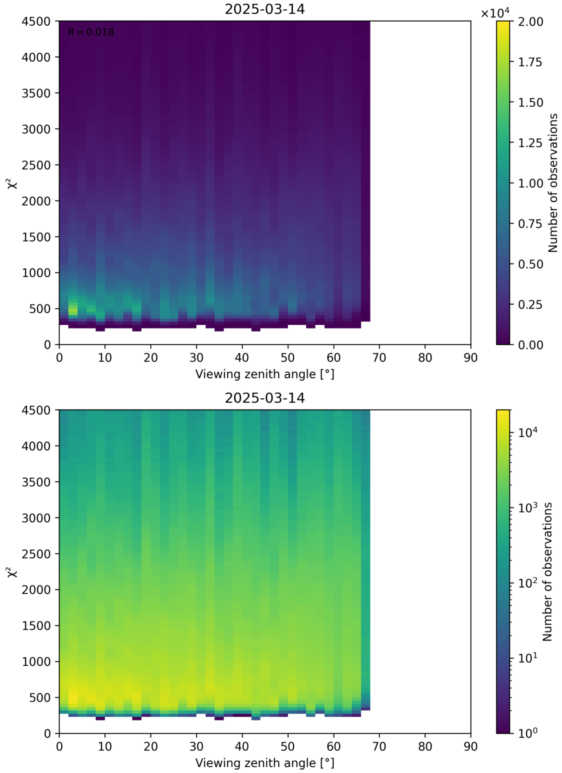
Figure 72: Scatter density plot of “Viewing zenith angle” against “ \chi^2 ” for 2025-03-13 to 2025-03-15.
