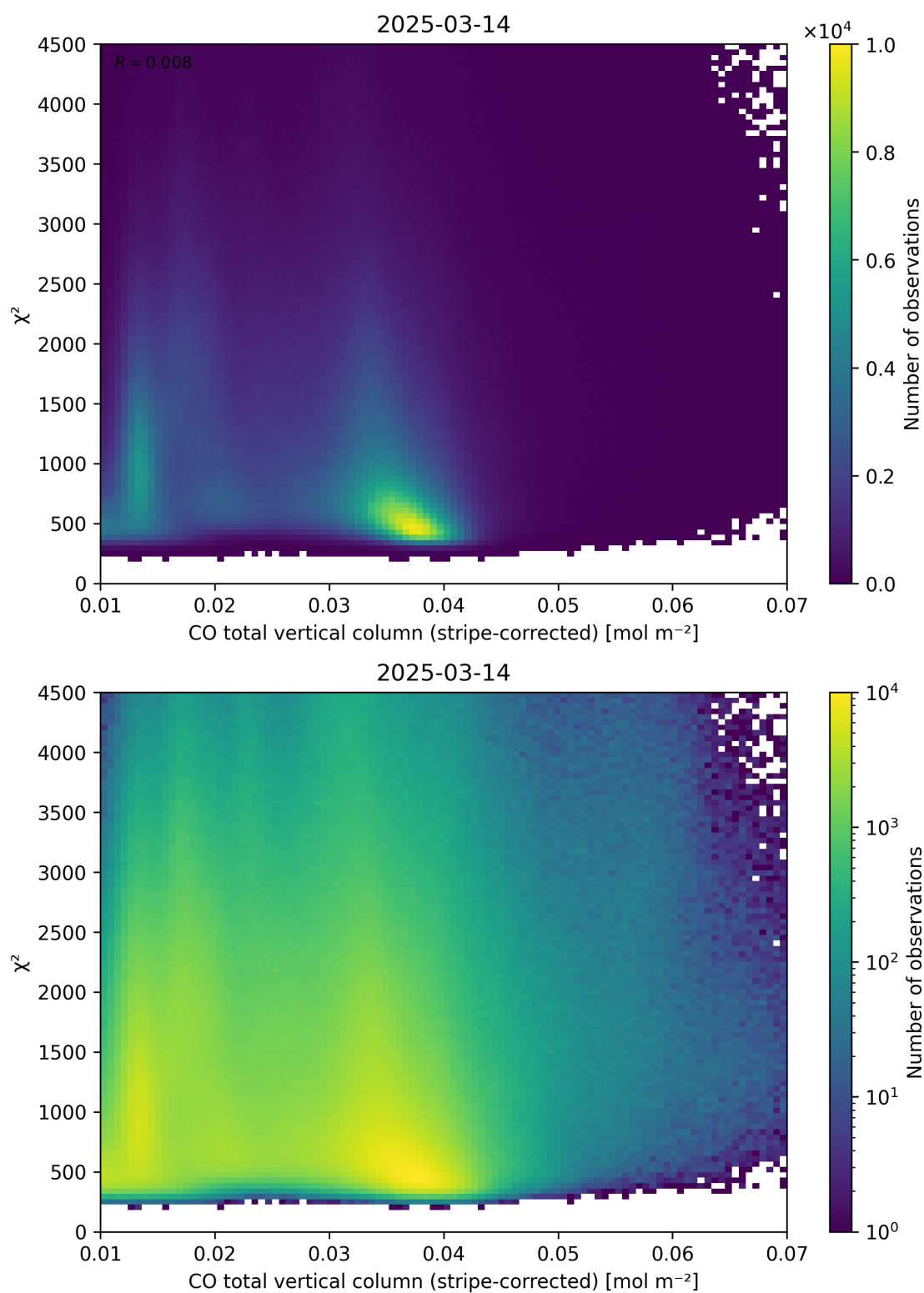
Figure 37: Scatter density plot of “CO total vertical column (stripe-corrected)” against “ \chi^2 ” for 2025-03-13 to 2025-03-15.
