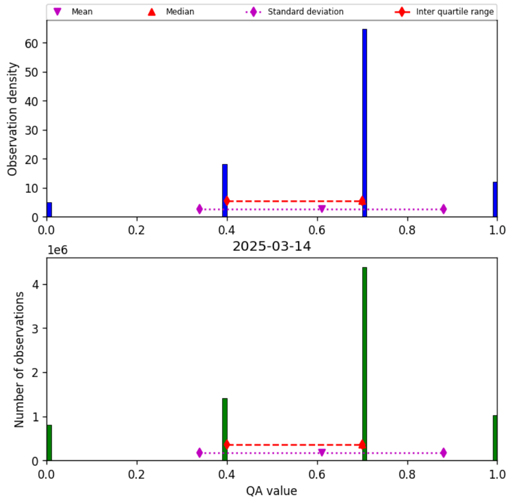
Figure 17: Histogram of “QA value” for 2025-03-13 to 2025-03-15
