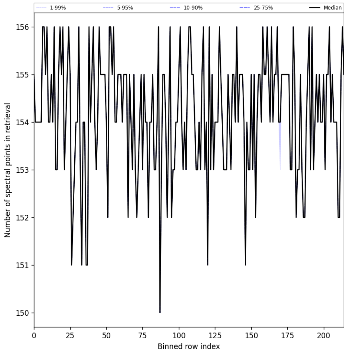
Figure 29: Along track statistics of “Number of spectral points in retrieval” for 2025-03-13 to 2025-03-15
