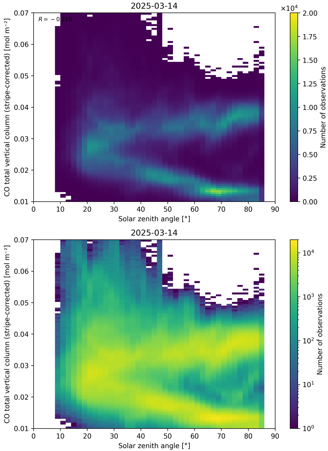
Figure 62: Scatter density plot of “Solar zenith angle” against “CO total vertical column (stripe-corrected)” for 2025-03-13 to 2025-03-15.
