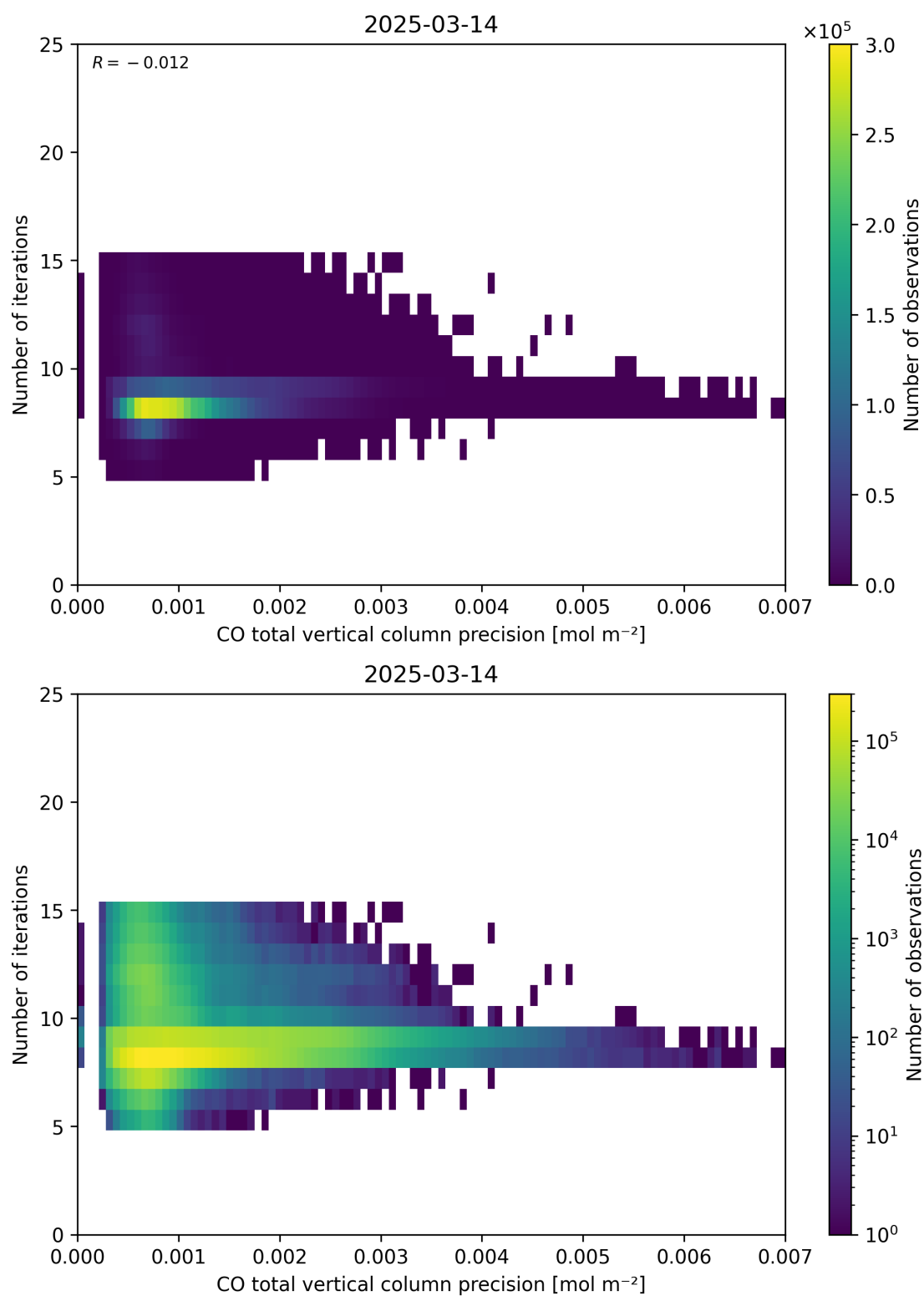
Figure 46: Scatter density plot of “CO total vertical column precision” against “Number of iterations” for 2025-03-13 to 2025-03-15.
