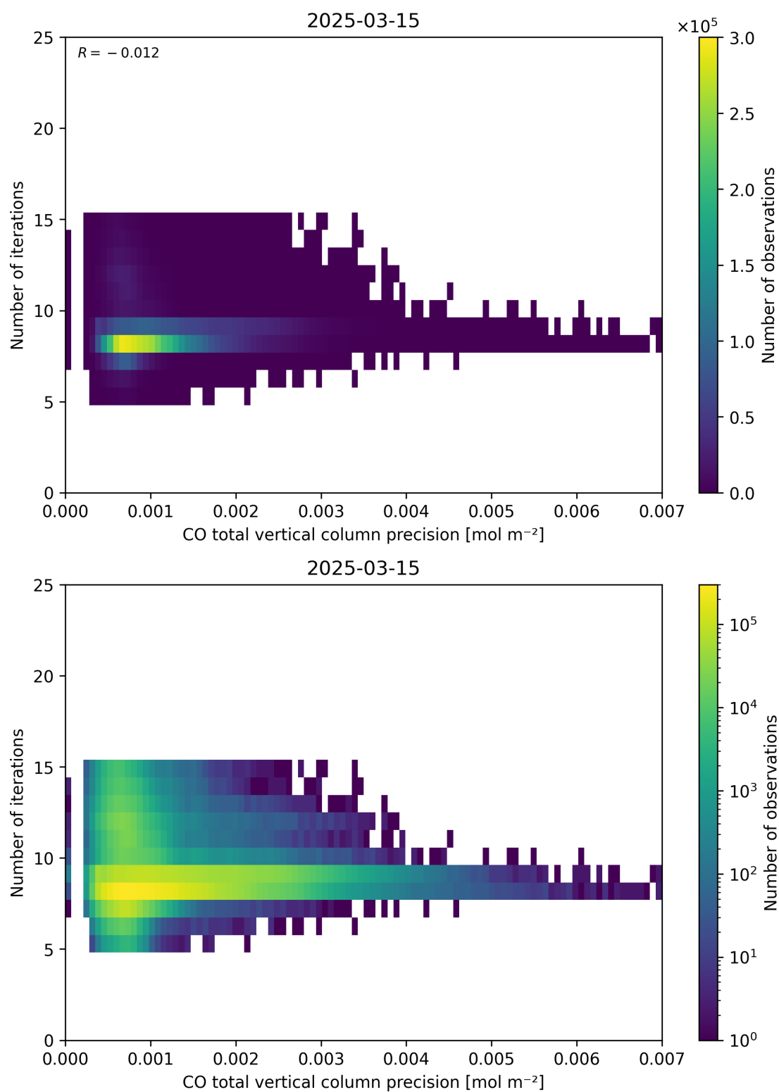
Figure 46: Scatter density plot of “CO total vertical column precision” against “Number of iterations” for 2025-03-14 to 2025-03-16.
