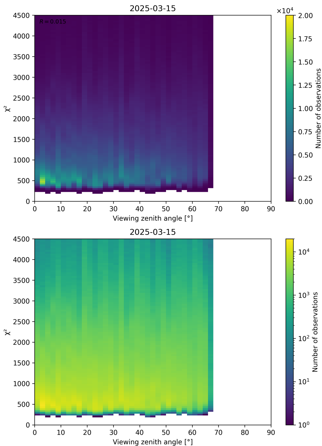
Figure 72: Scatter density plot of “Viewing zenith angle” against “ \chi^2 ” for 2025-03-14 to 2025-03-16.
