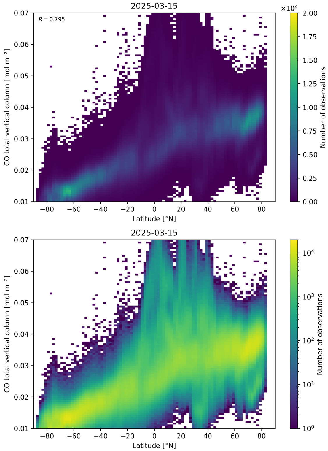
Figure 51: Scatter density plot of “Latitude” against “CO total vertical column” for 2025-03-14 to 2025-03-16.
