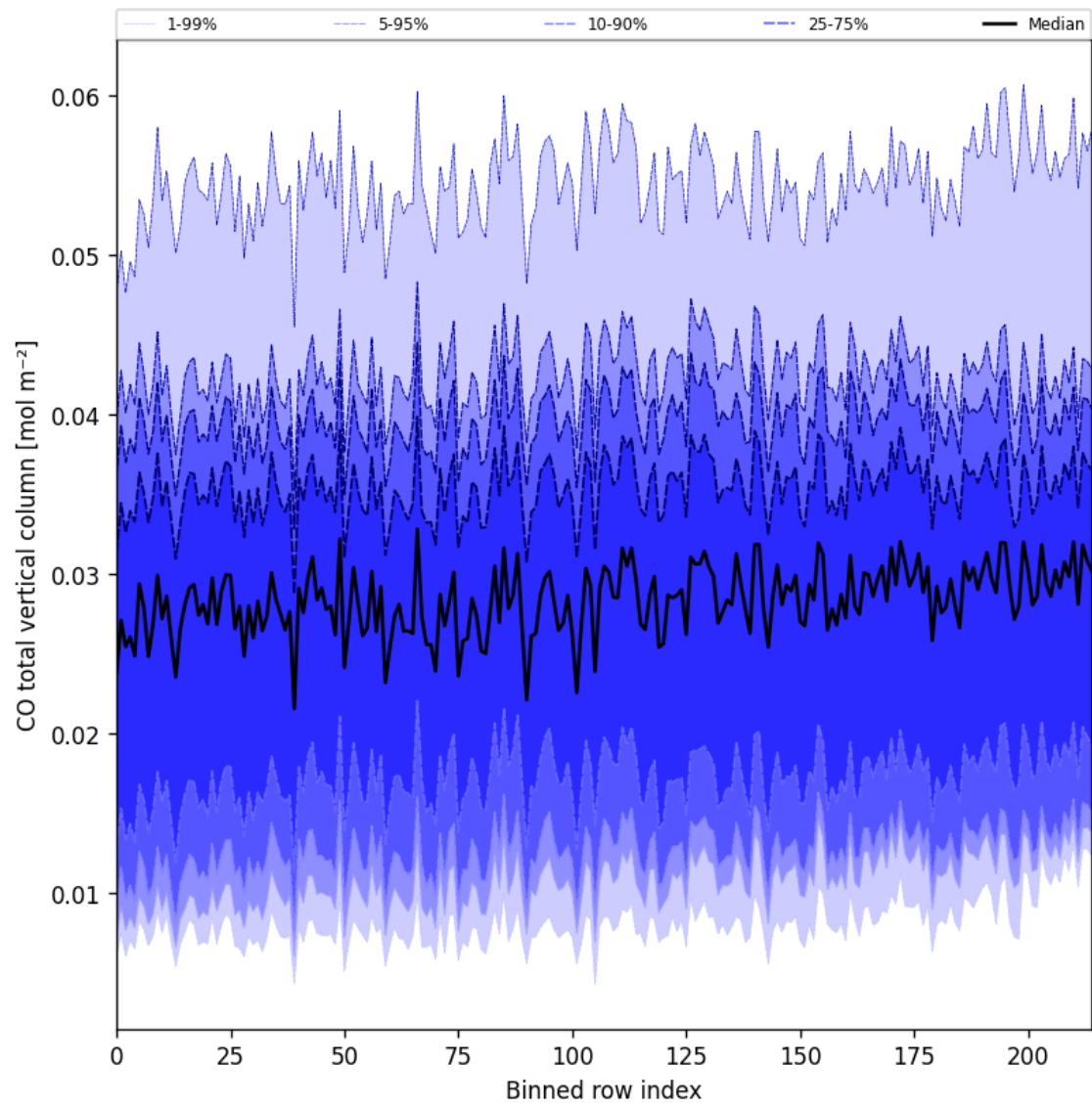
Figure 26: Along track statistics of “CO total vertical column” for 2025-03-14 to 2025-03-16
