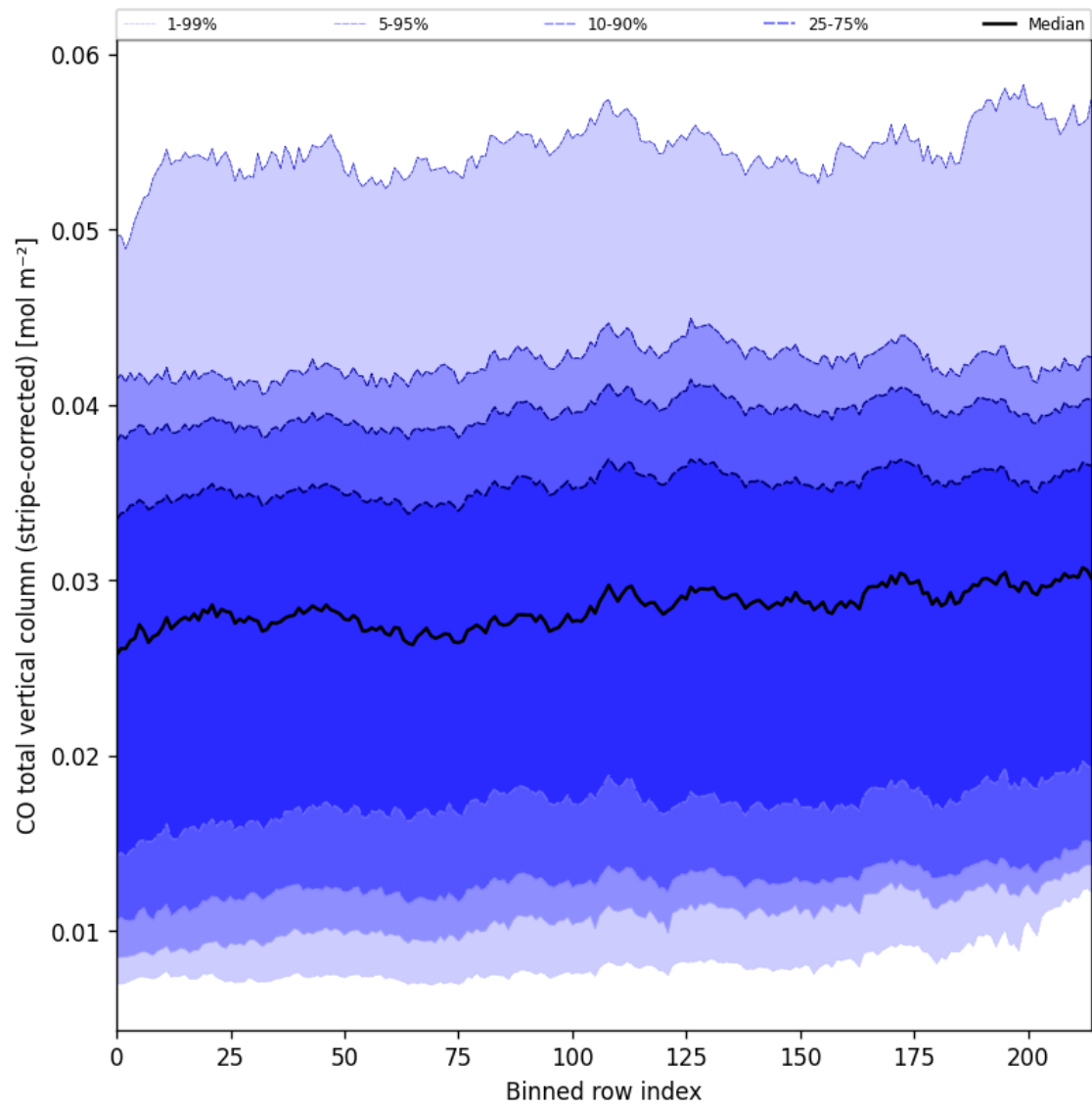
Figure 27: Along track statistics of “CO total vertical column (stripe-corrected)” for 2025-03-14 to 2025-03-16
