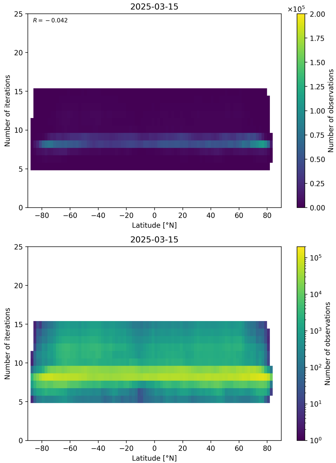
Figure 56: Scatter density plot of “Latitude” against “Number of iterations” for 2025-03-14 to 2025-03-16.
