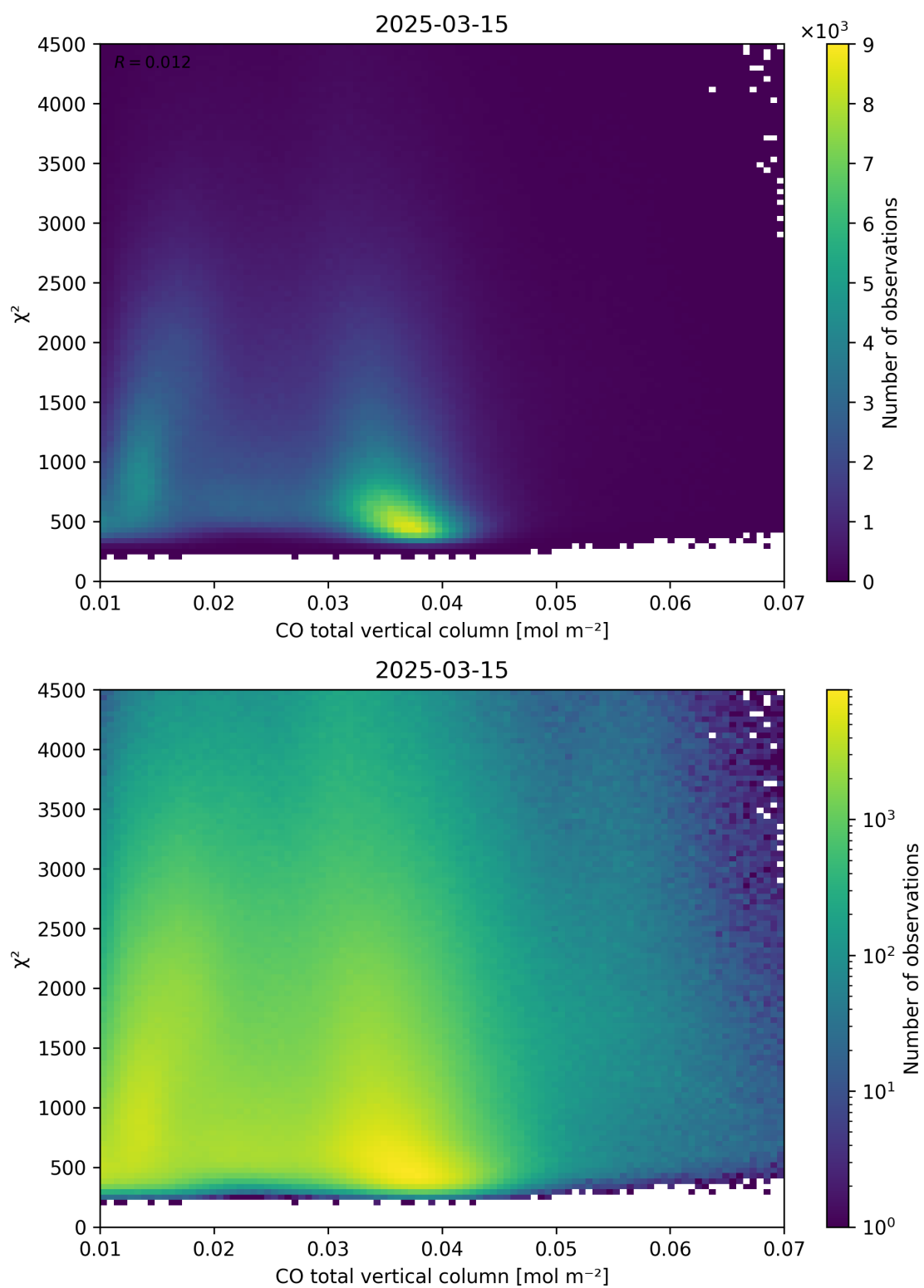
Figure 35: Scatter density plot of “CO total vertical column” against “ \chi^2 ” for 2025-03-14 to 2025-03-16.
