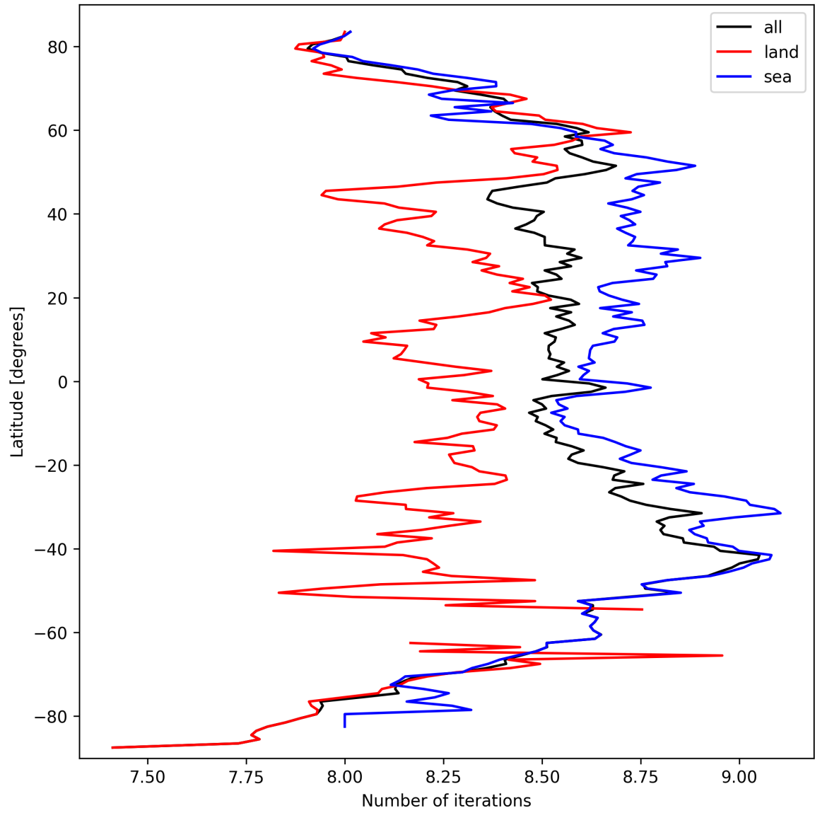
Figure 16: Zonal average of “Number of iterations” for 2025-03-14 to 2025-03-16.
