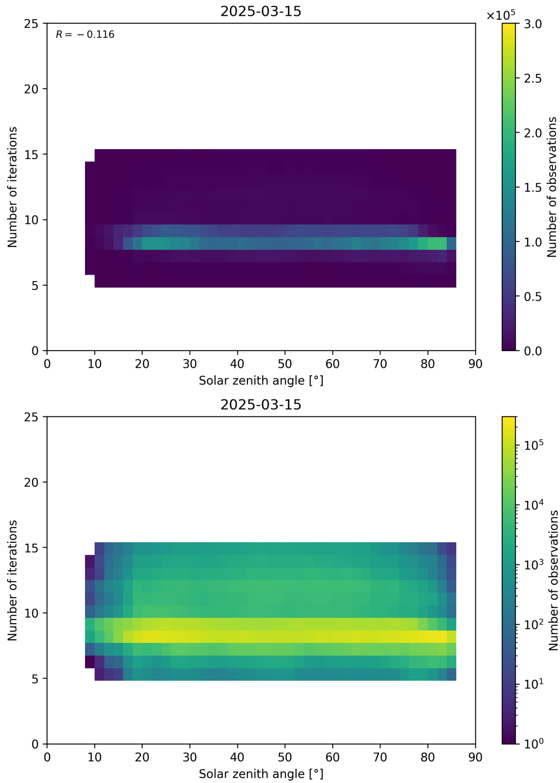
Figure 67: Scatter density plot of “Solar zenith angle” against “Number of iterations” for 2025-03-14 to 2025-03-16.
