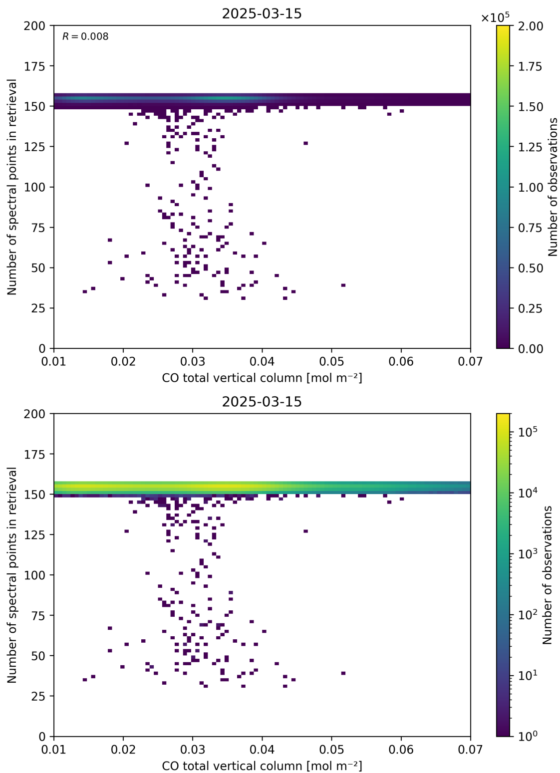
Figure 43: Scatter density plot of “CO total vertical column” against “Number of spectral points in retrieval” for 2025-03-14 to 2025-03-16.
