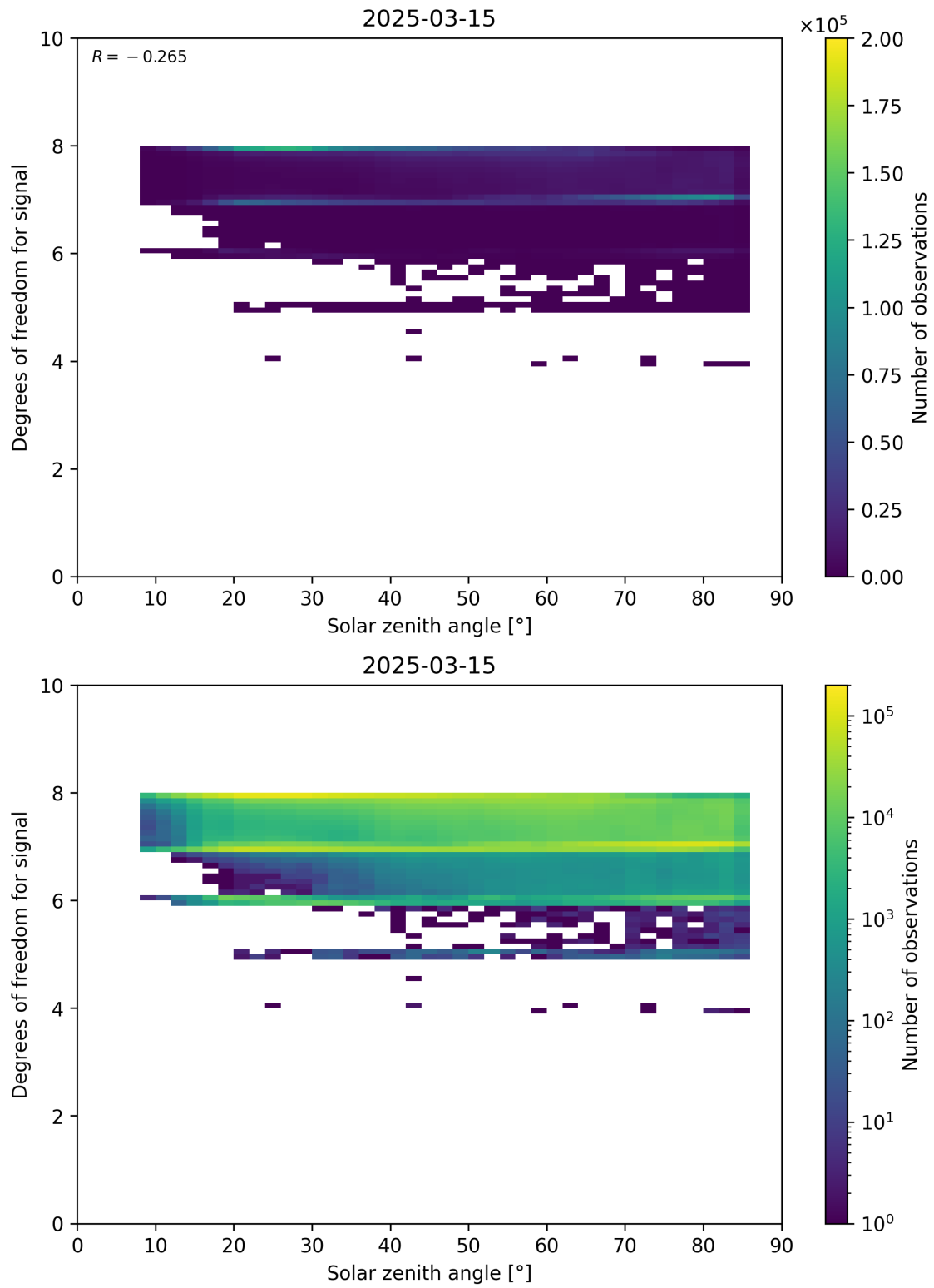
Figure 65: Scatter density plot of “Solar zenith angle” against “Degrees of freedom for signal” for 2025-03-14 to 2025-03-16.
