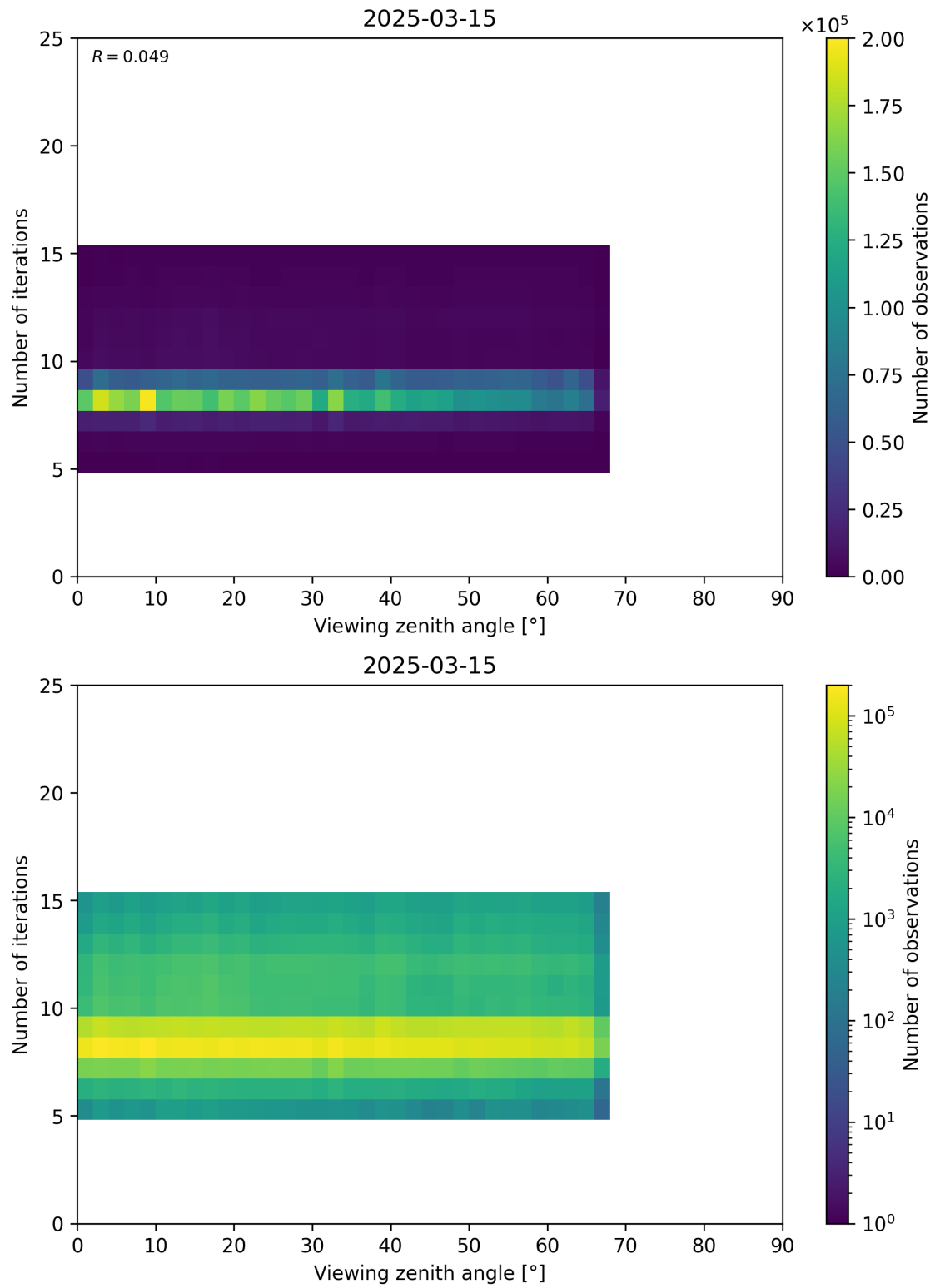
Figure 75: Scatter density plot of “Viewing zenith angle” against “Number of iterations” for 2025-03-14 to 2025-03-16.
