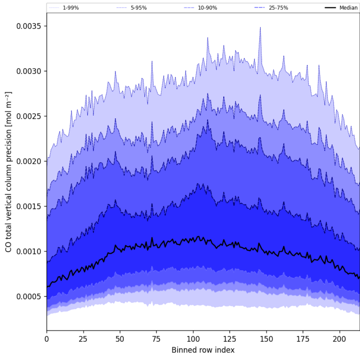
Figure 28: Along track statistics of “CO total vertical column precision” for 2025-03-14 to 2025-03-16
