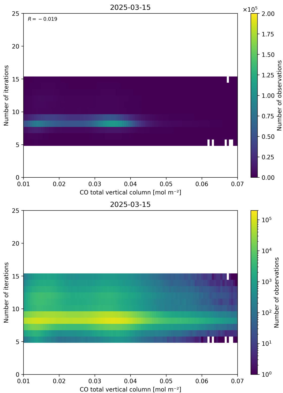
Figure 42: Scatter density plot of “CO total vertical column” against “Number of iterations” for 2025-03-14 to 2025-03-16.
