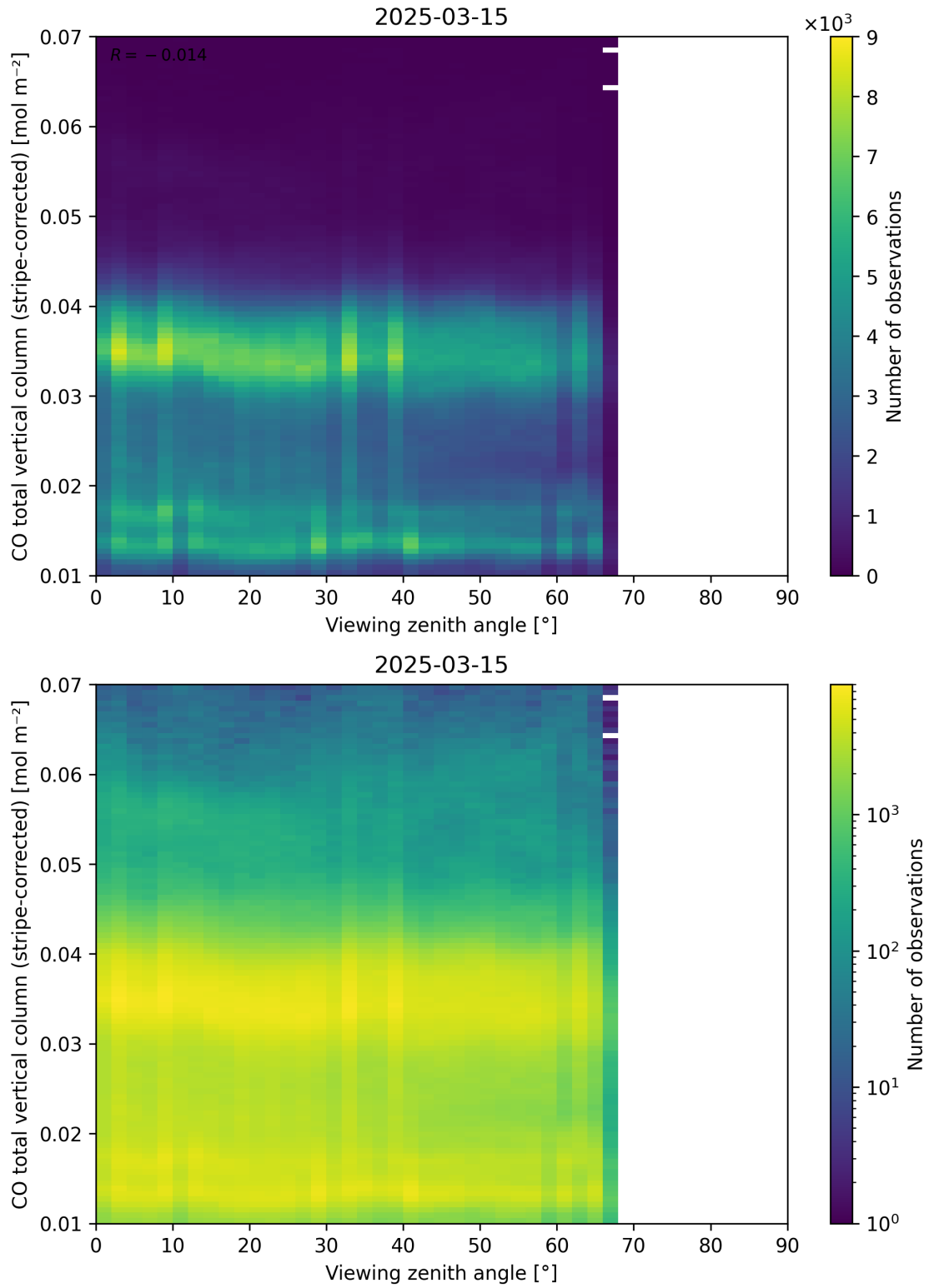
Figure 70: Scatter density plot of “Viewing zenith angle” against “CO total vertical column (stripe-corrected)” for 2025-03-14 to 2025-03-16.
