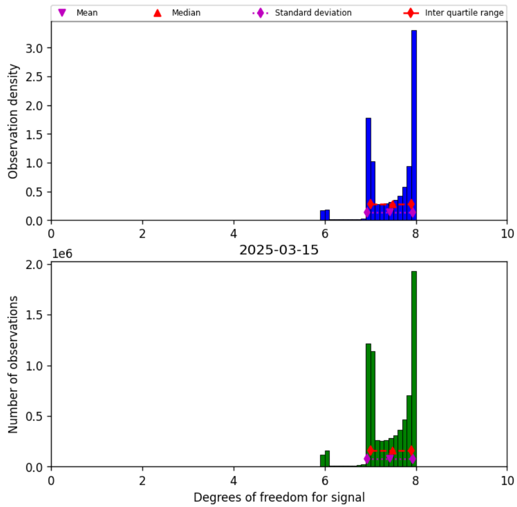
Figure 23: Histogram of “Degrees of freedom for signal” for 2025-03-14 to 2025-03-16
