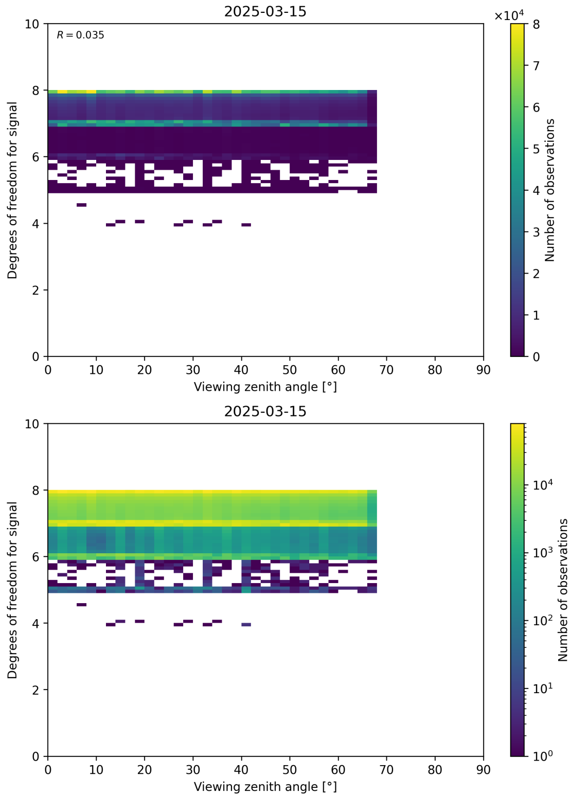
Figure 73: Scatter density plot of “Viewing zenith angle” against “Degrees of freedom for signal” for 2025-03-14 to 2025-03-16.
