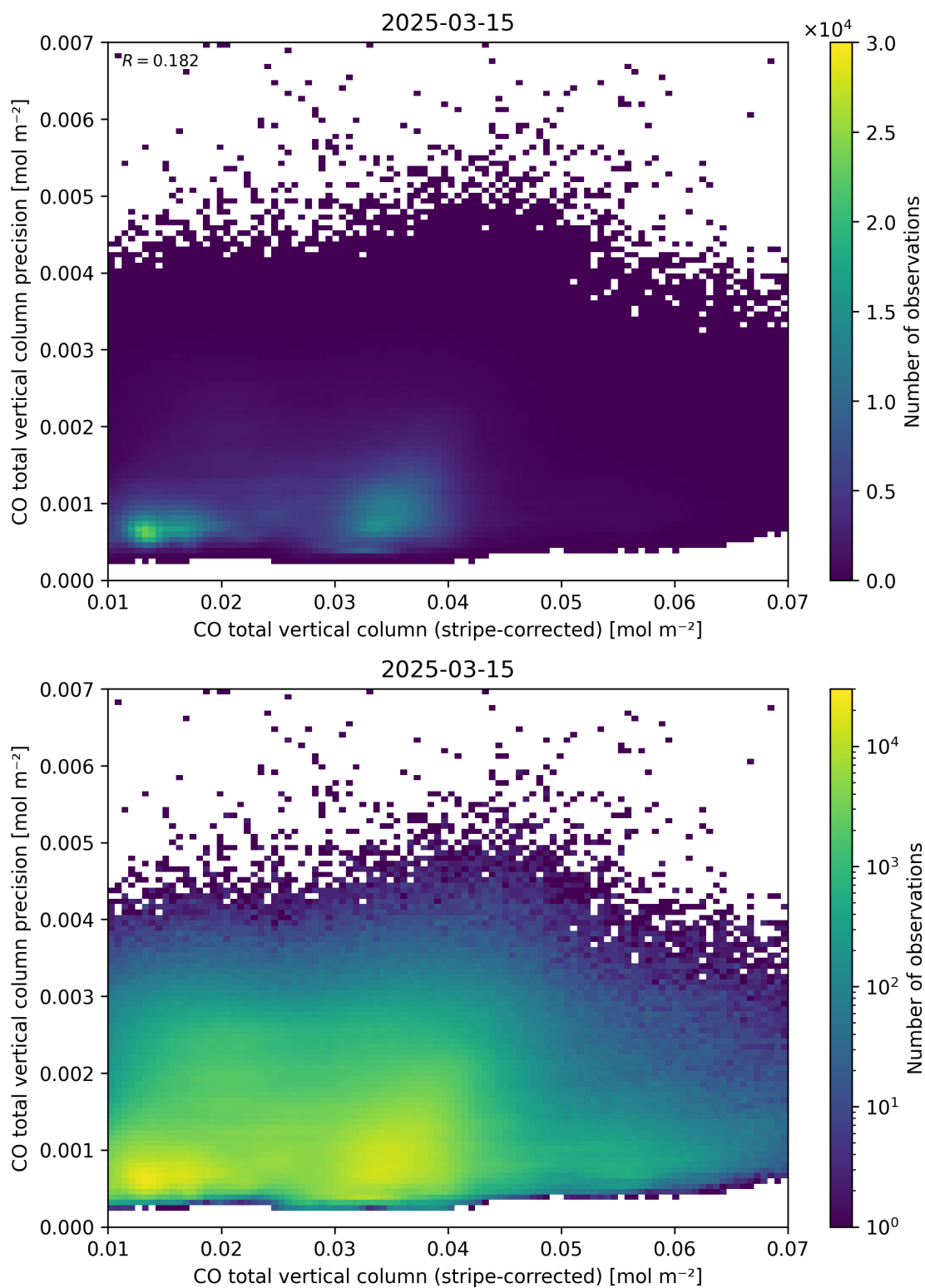
Figure 36: Scatter density plot of “CO total vertical column (stripe-corrected)” against “CO total vertical column precision” for 2025-03-14 to 2025-03-16.
