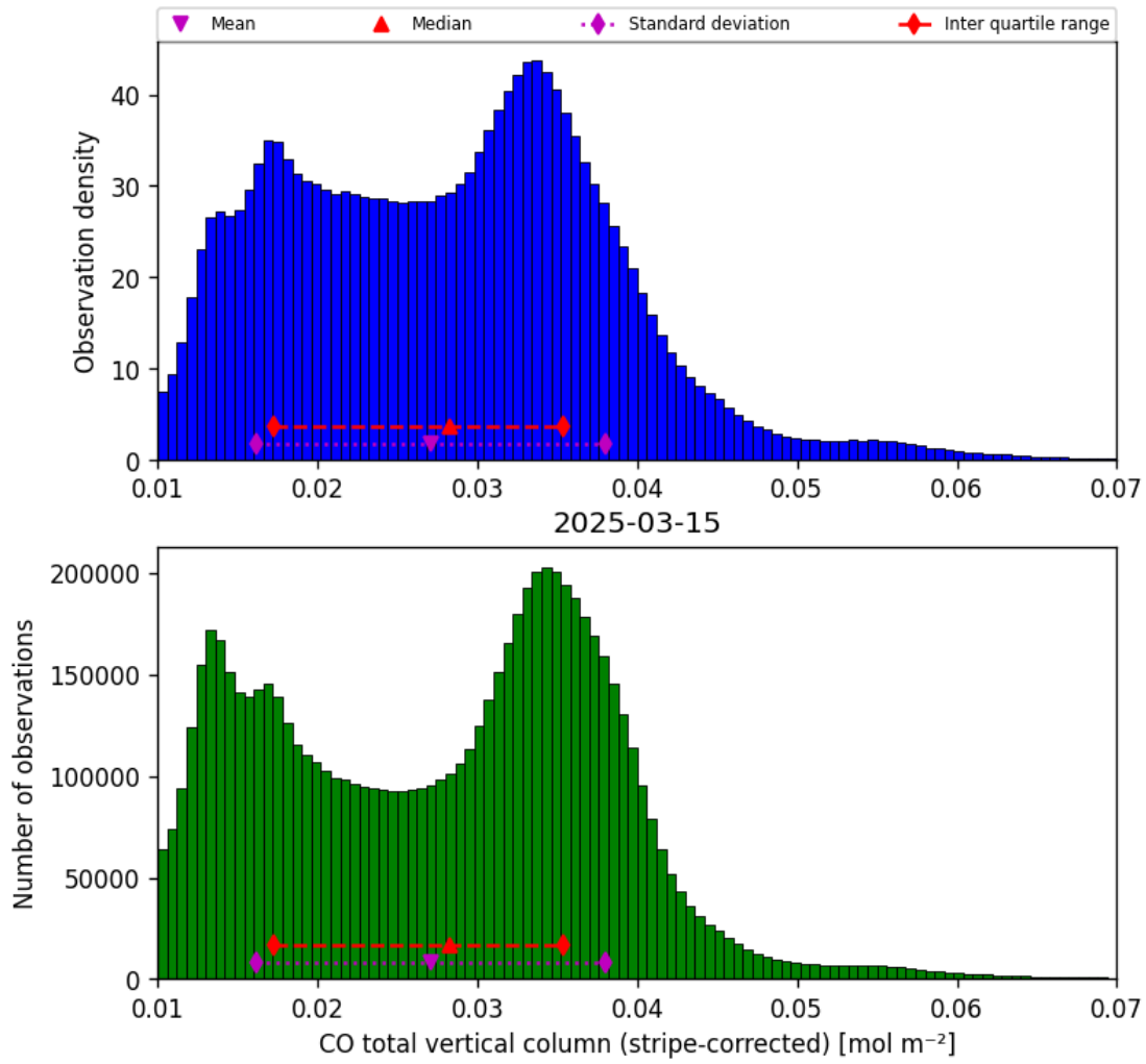
Figure 19: Histogram of “CO total vertical column (stripe-corrected)” for 2025-03-14 to 2025-03-16
