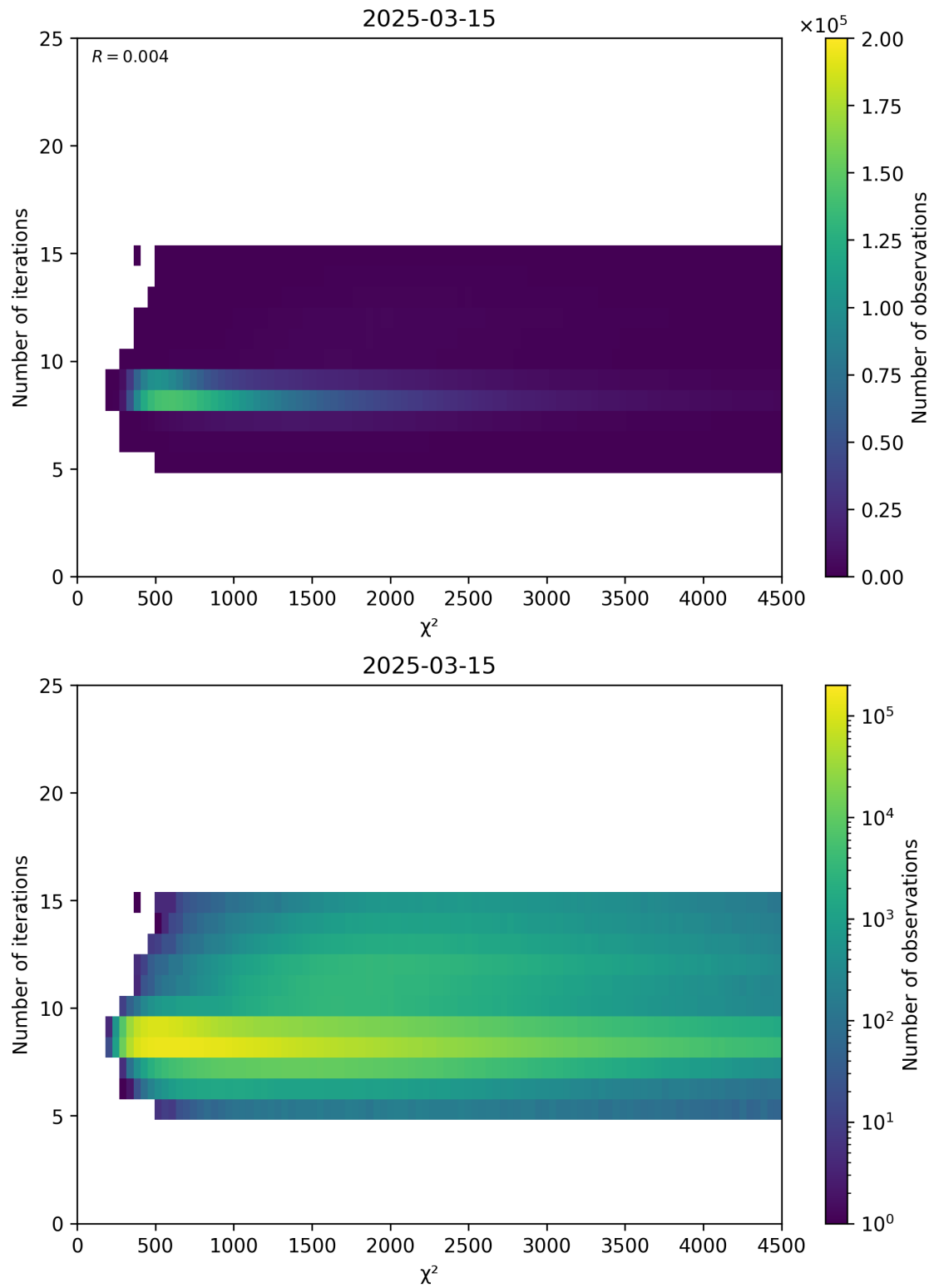
Figure 49: Scatter density plot of “ \chi^2 ” against “Number of iterations” for 2025-03-14 to 2025-03-16.
