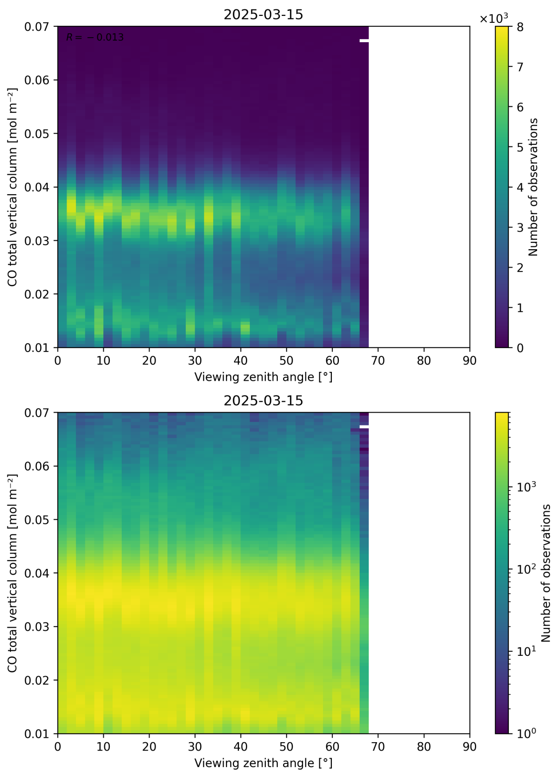
Figure 69: Scatter density plot of “Viewing zenith angle” against “CO total vertical column” for 2025-03-14 to 2025-03-16.
