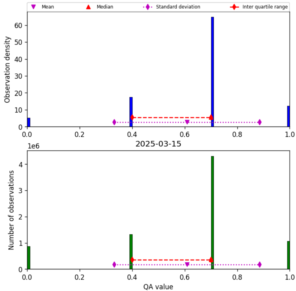
Figure 17: Histogram of “QA value” for 2025-03-14 to 2025-03-16
