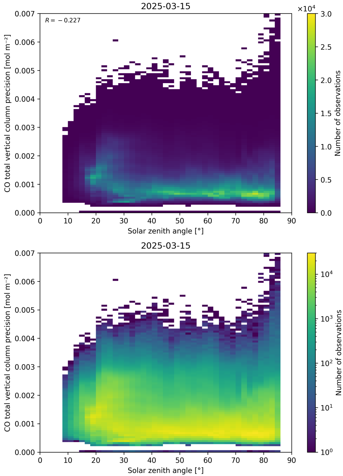
Figure 63: Scatter density plot of “Solar zenith angle” against “CO total vertical column precision” for 2025-03-14 to 2025-03-16.
