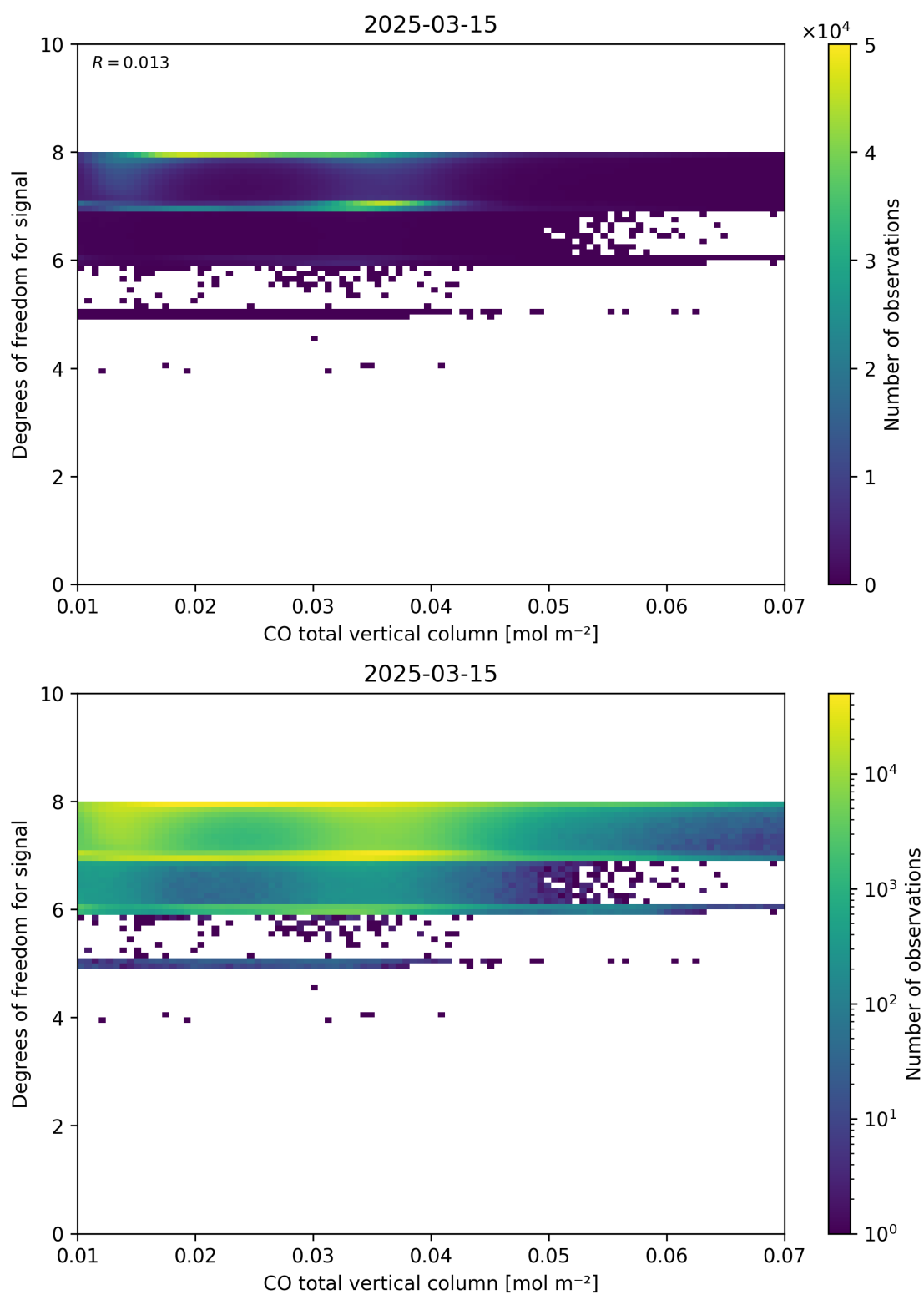
Figure 41: Scatter density plot of “CO total vertical column” against “Degrees of freedom for signal” for 2025-03-14 to 2025-03-16.
