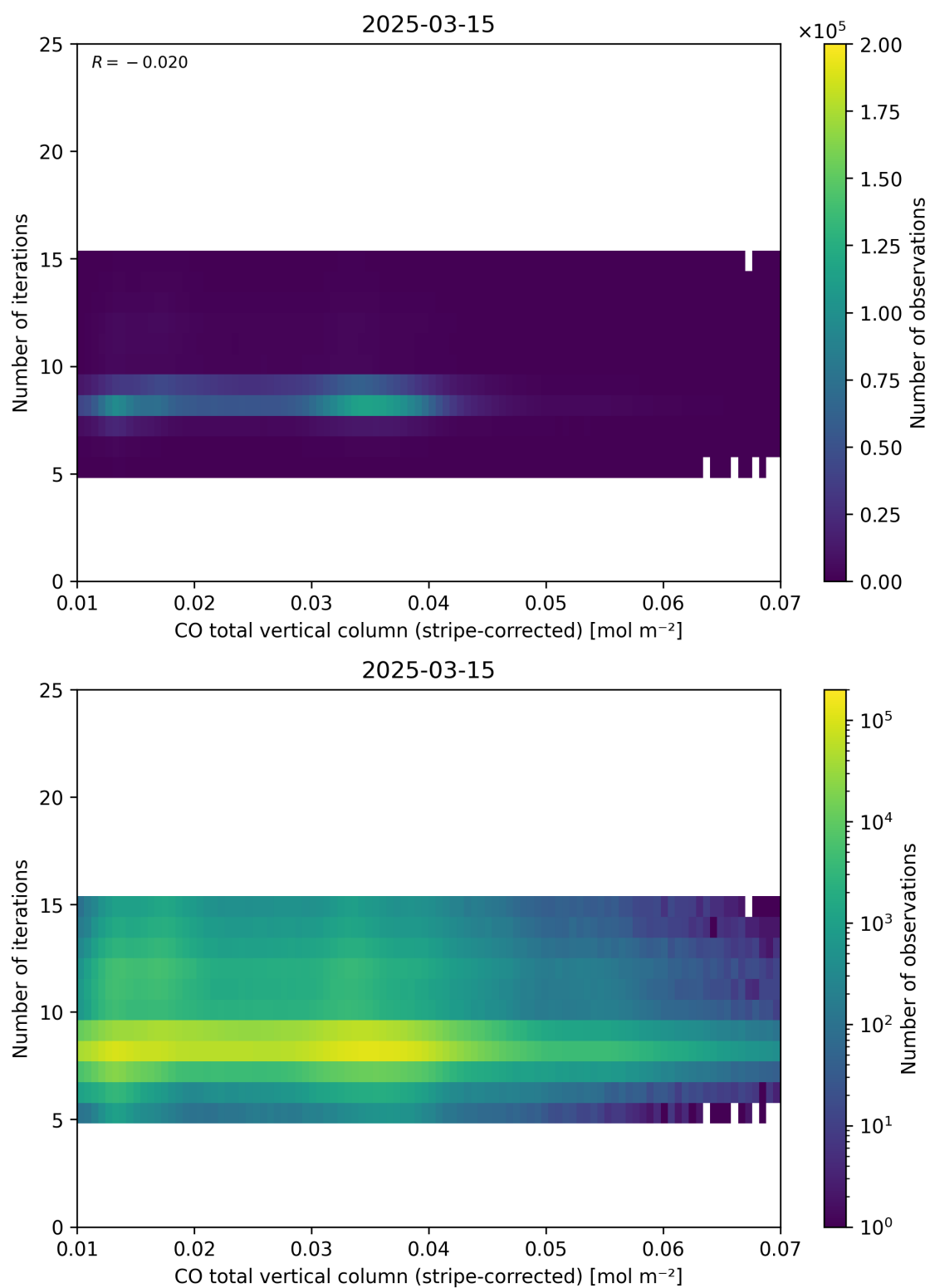
Figure 39: Scatter density plot of “CO total vertical column (stripe-corrected)” against “Number of iterations” for 2025-03-14 to 2025-03-16.
