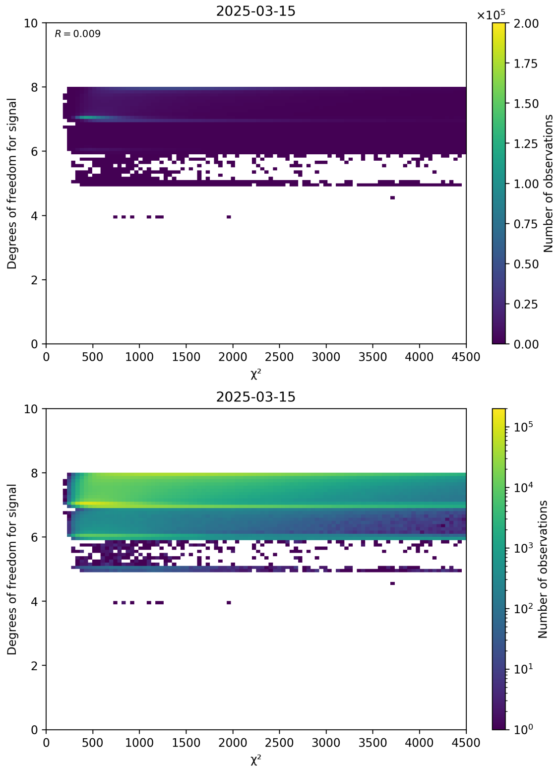
Figure 48: Scatter density plot of “ \chi^2 ” against “Degrees of freedom for signal” for 2025-03-14 to 2025-03-16.
