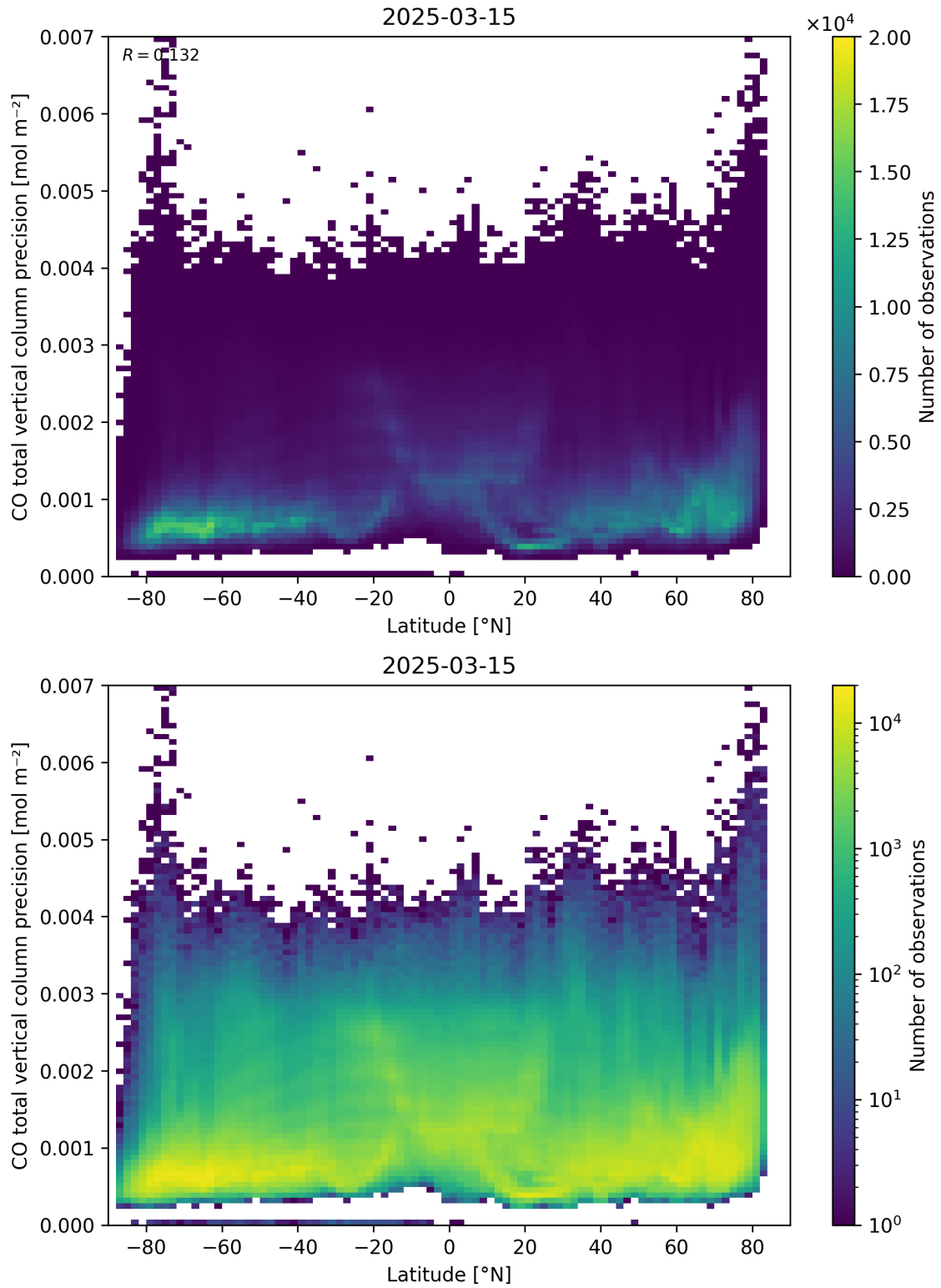
Figure 53: Scatter density plot of “Latitude” against “CO total vertical column precision” for 2025-03-14 to 2025-03-16.
