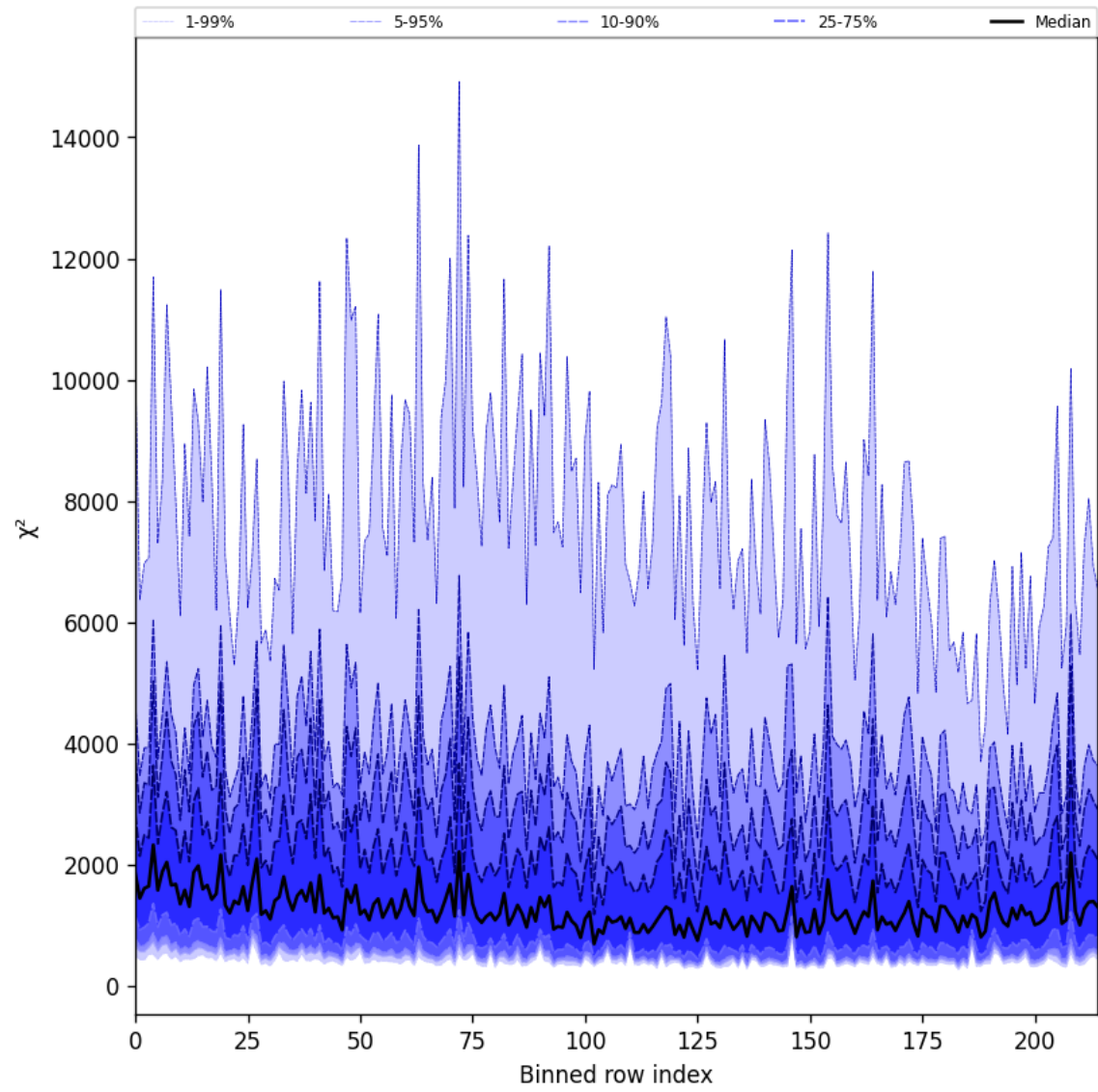
Figure 30: Along track statistics of “ \chi^2 ” for 2025-03-14 to 2025-03-16
