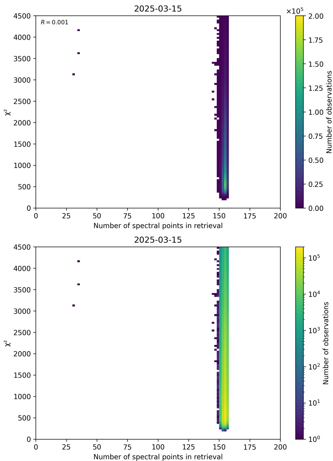
Figure 58: Scatter density plot of “Number of spectral points in retrieval” against “ \chi^2 ” for 2025-03-14 to 2025-03-16.
