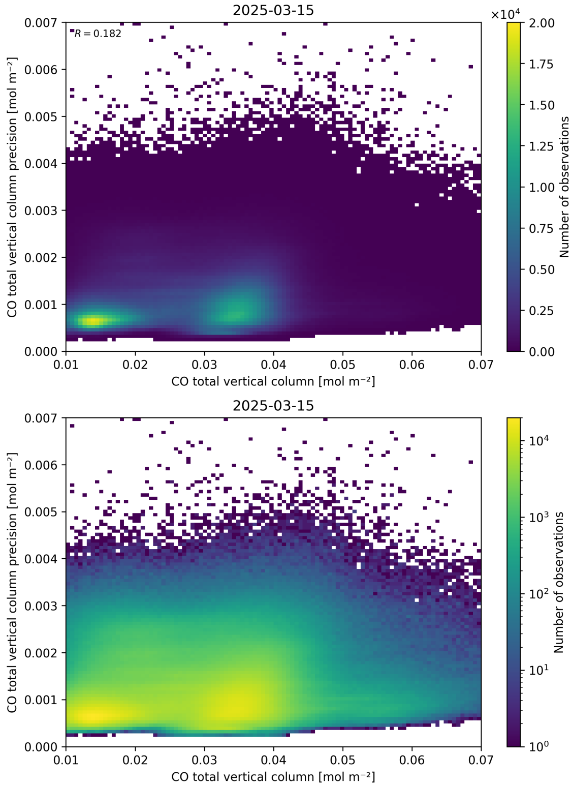
Figure 34: Scatter density plot of “CO total vertical column” against “CO total vertical column precision” for 2025-03-14 to 2025-03-16.
