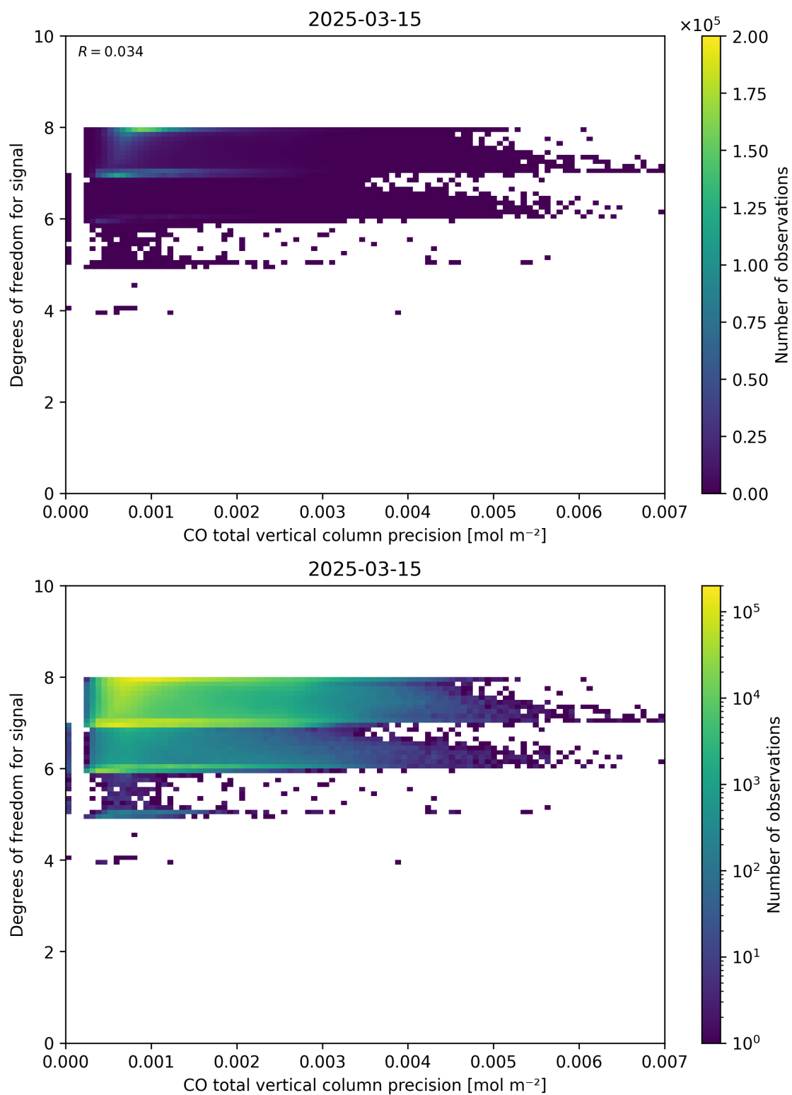
Figure 45: Scatter density plot of “CO total vertical column precision” against “Degrees of freedom for signal” for 2025-03-14 to 2025-03-16.
