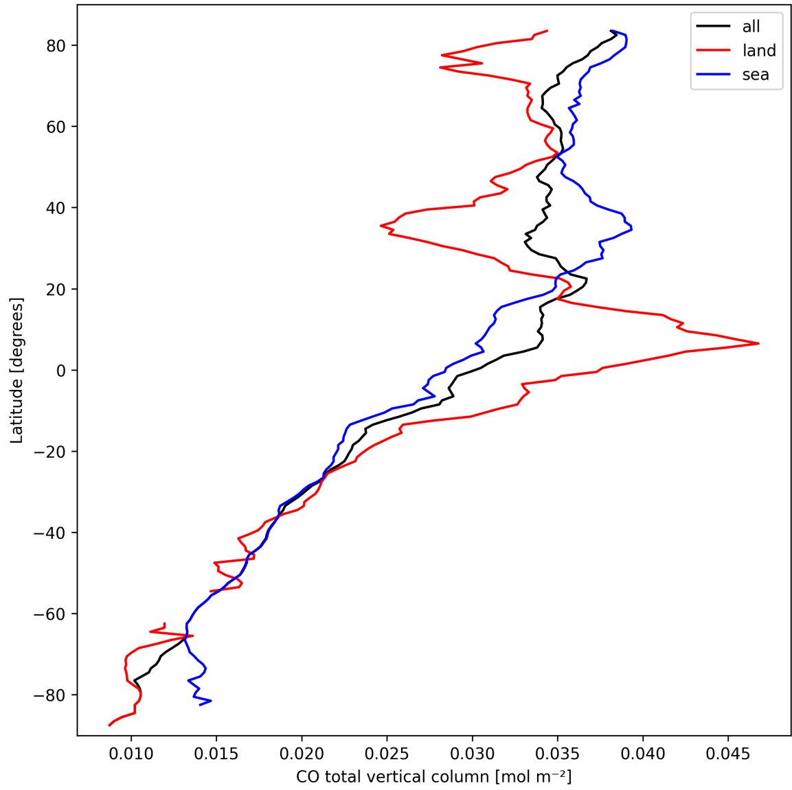
Figure 10: Zonal average of “CO total vertical column” for 2025-03-14 to 2025-03-16.
