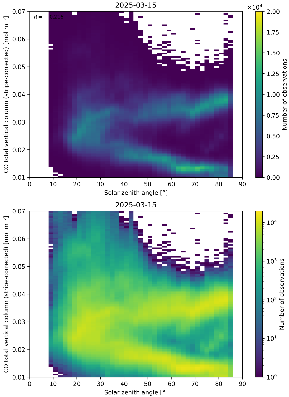
Figure 62: Scatter density plot of “Solar zenith angle” against “CO total vertical column (stripe-corrected)” for 2025-03-14 to 2025-03-16.
