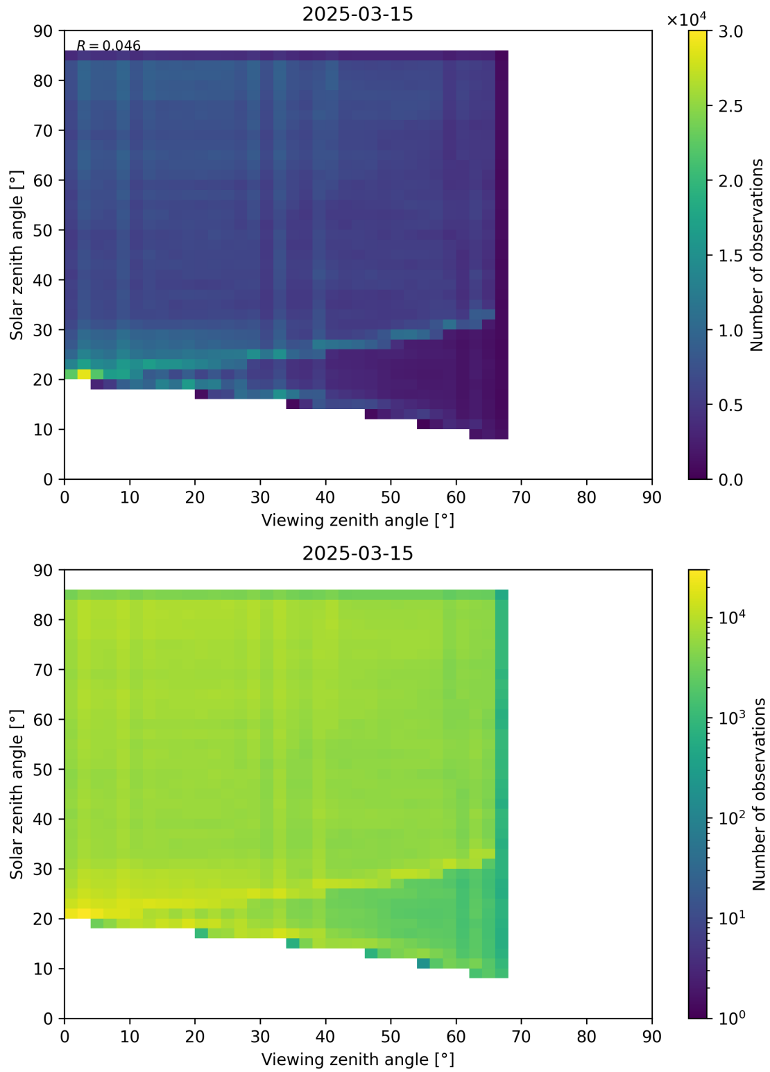
Figure 77: Scatter density plot of “Viewing zenith angle” against “Solar zenith angle” for 2025-03-14 to 2025-03-16.
