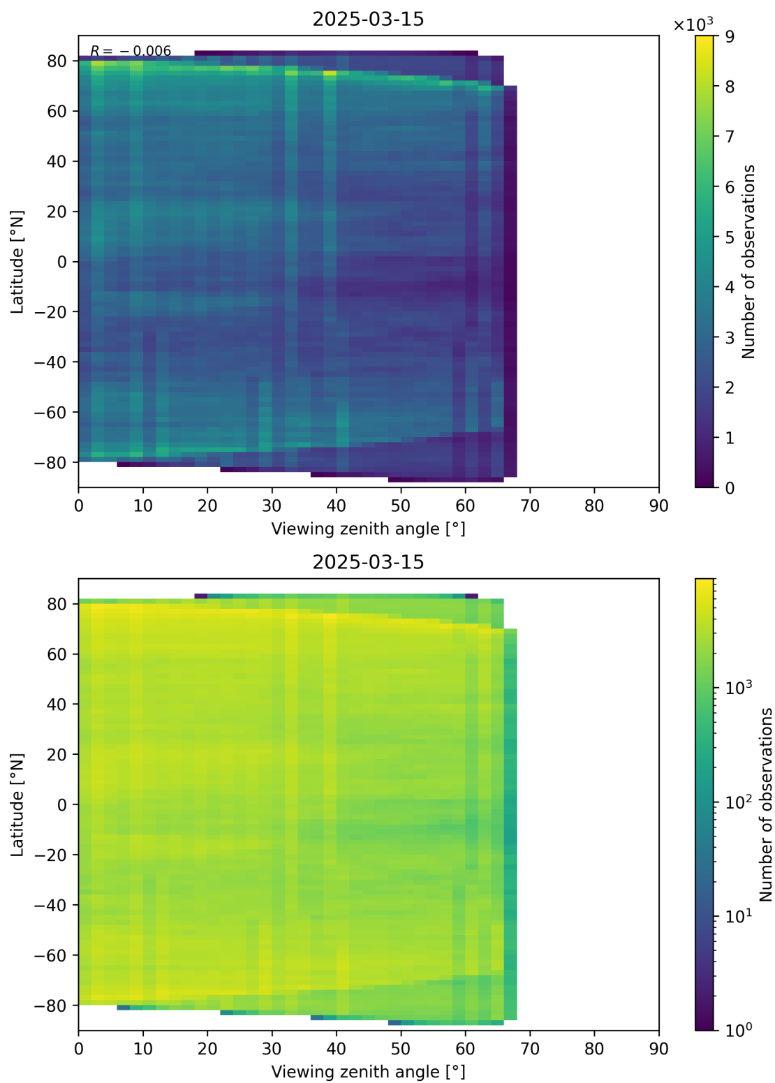
Figure 74: Scatter density plot of “Viewing zenith angle” against “Latitude” for 2025-03-14 to 2025-03-16.
