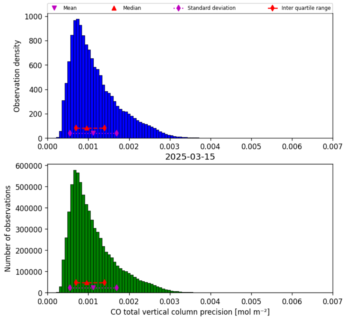
Figure 20: Histogram of “CO total vertical column precision” for 2025-03-14 to 2025-03-16
