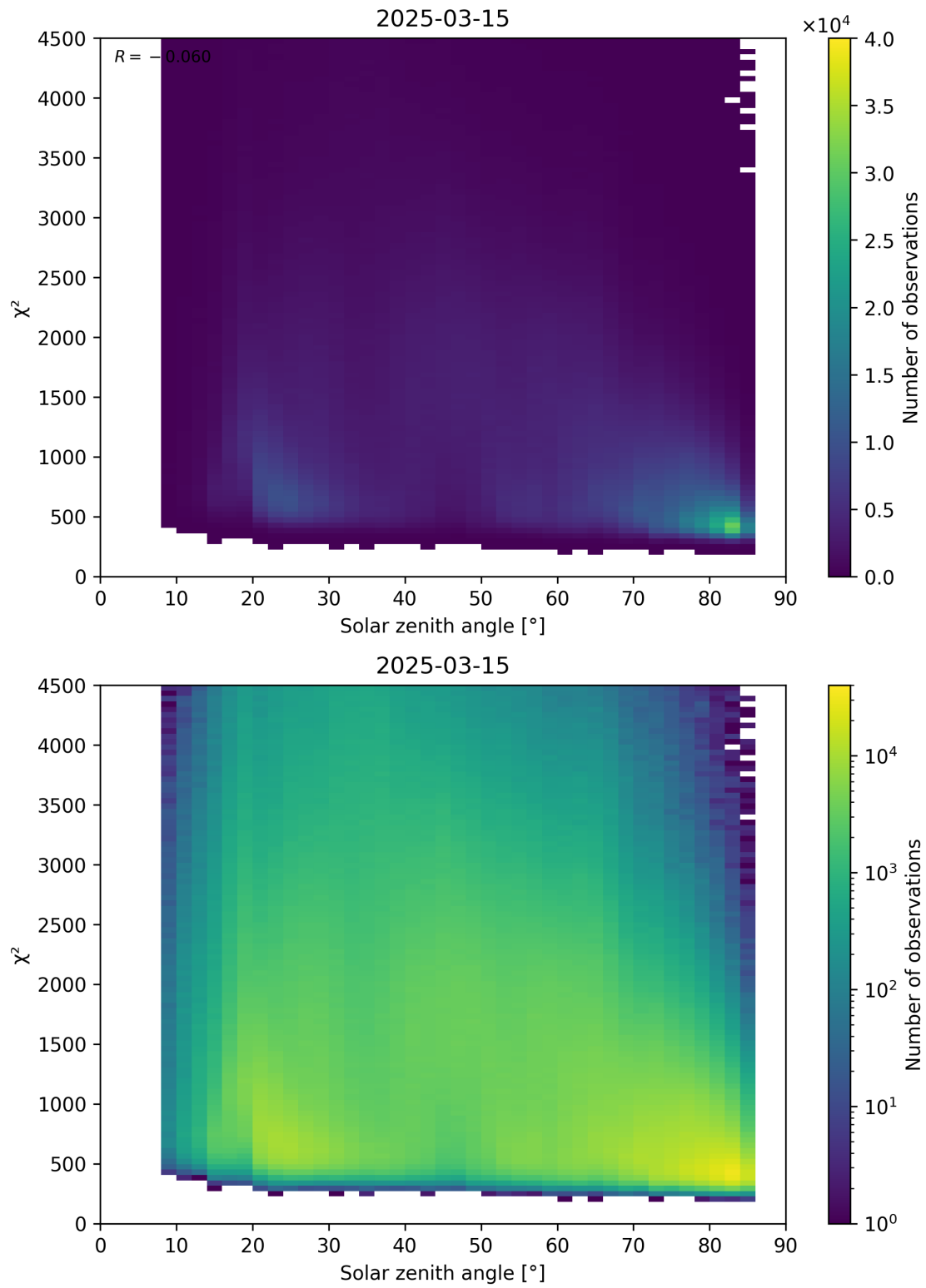
Figure 64: Scatter density plot of “Solar zenith angle” against “ \chi^2 ” for 2025-03-14 to 2025-03-16.
