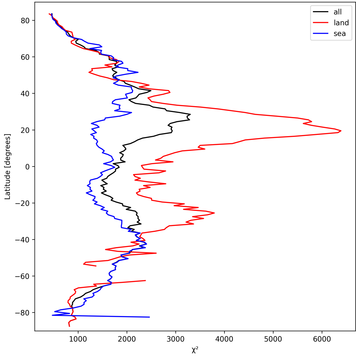
Figure 14: Zonal average of “ \chi^2 ” for 2025-03-14 to 2025-03-16.
