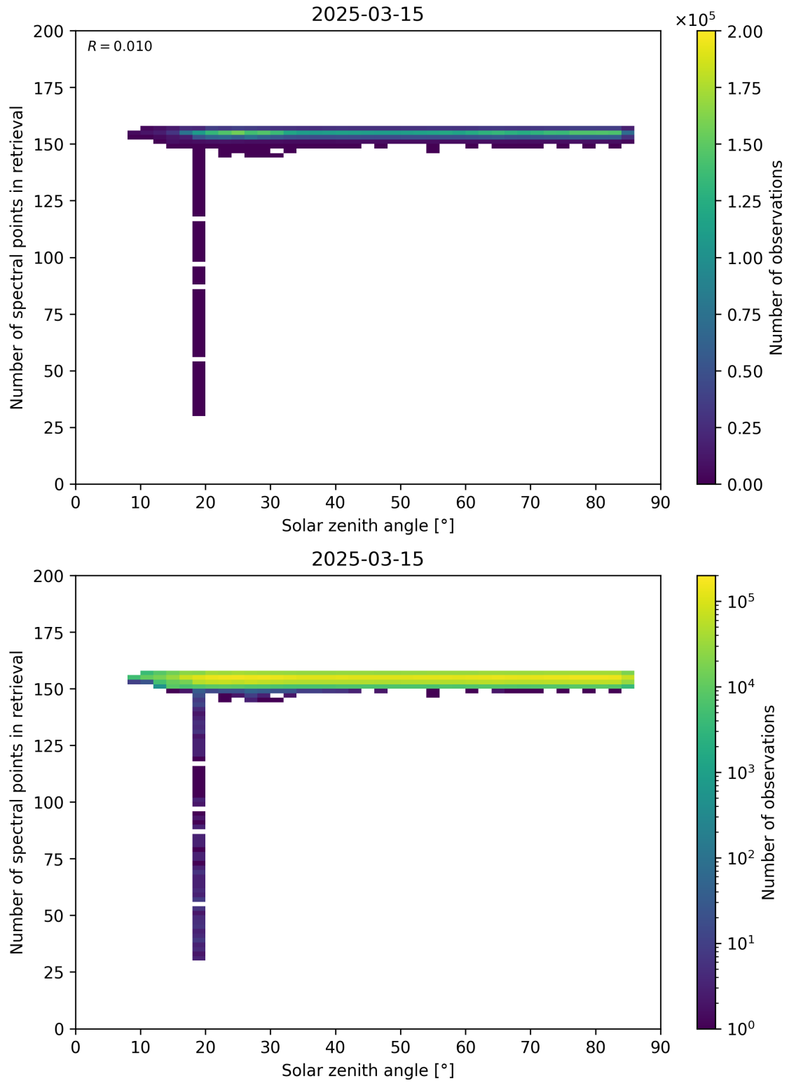
Figure 68: Scatter density plot of “Solar zenith angle” against “Number of spectral points in retrieval” for 2025-03-14 to 2025-03-16.
