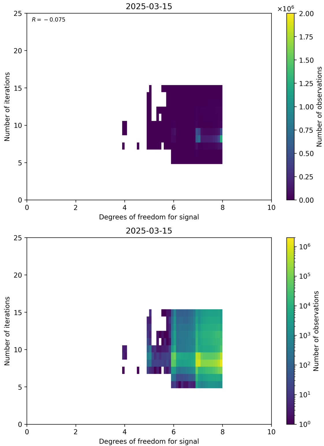
Figure 50: Scatter density plot of “Degrees of freedom for signal” against “Number of iterations” for 2025-03-14 to 2025-03-16.
