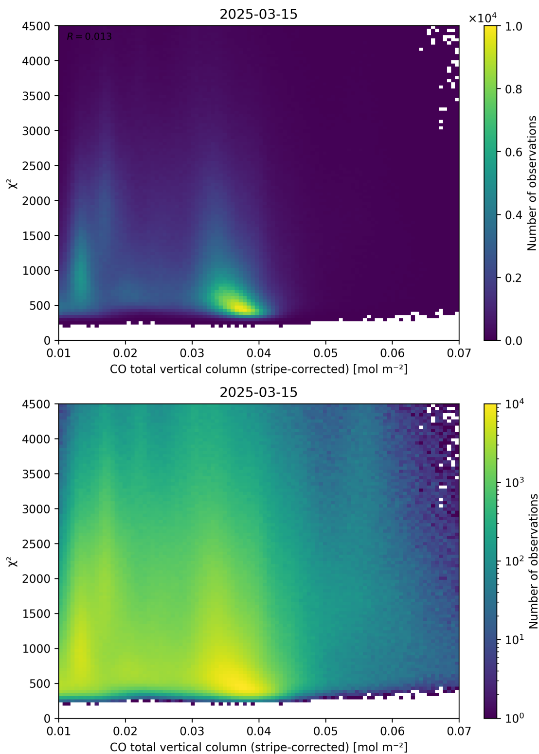
Figure 37: Scatter density plot of “CO total vertical column (stripe-corrected)” against “ \chi^2 ” for 2025-03-14 to 2025-03-16.
