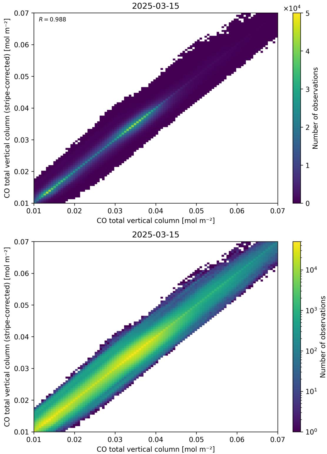
Figure 33: Scatter density plot of “CO total vertical column” against “CO total vertical column (stripe-corrected)” for 2025-03-14 to 2025-03-16.
