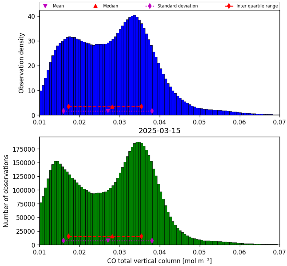
Figure 18: Histogram of “CO total vertical column” for 2025-03-14 to 2025-03-16
