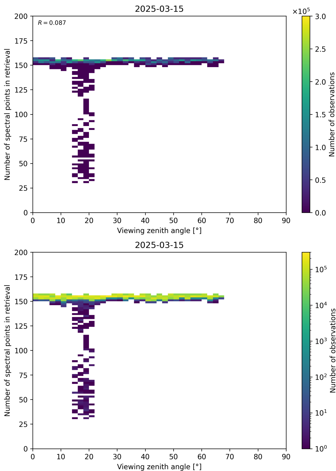
Figure 76: Scatter density plot of “Viewing zenith angle” against “Number of spectral points in retrieval” for 2025-03-14 to 2025-03-16.
