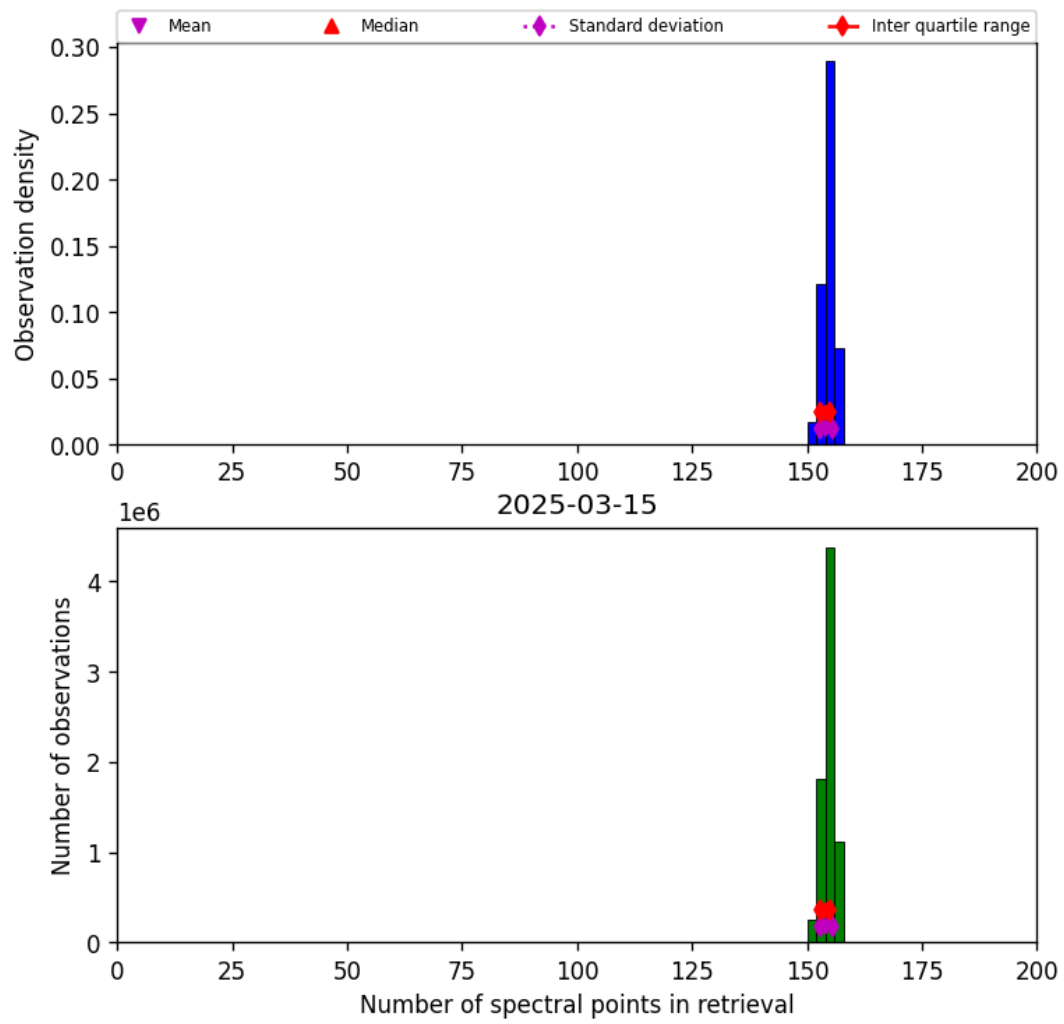
Figure 21: Histogram of “Number of spectral points in retrieval” for 2025-03-14 to 2025-03-16
