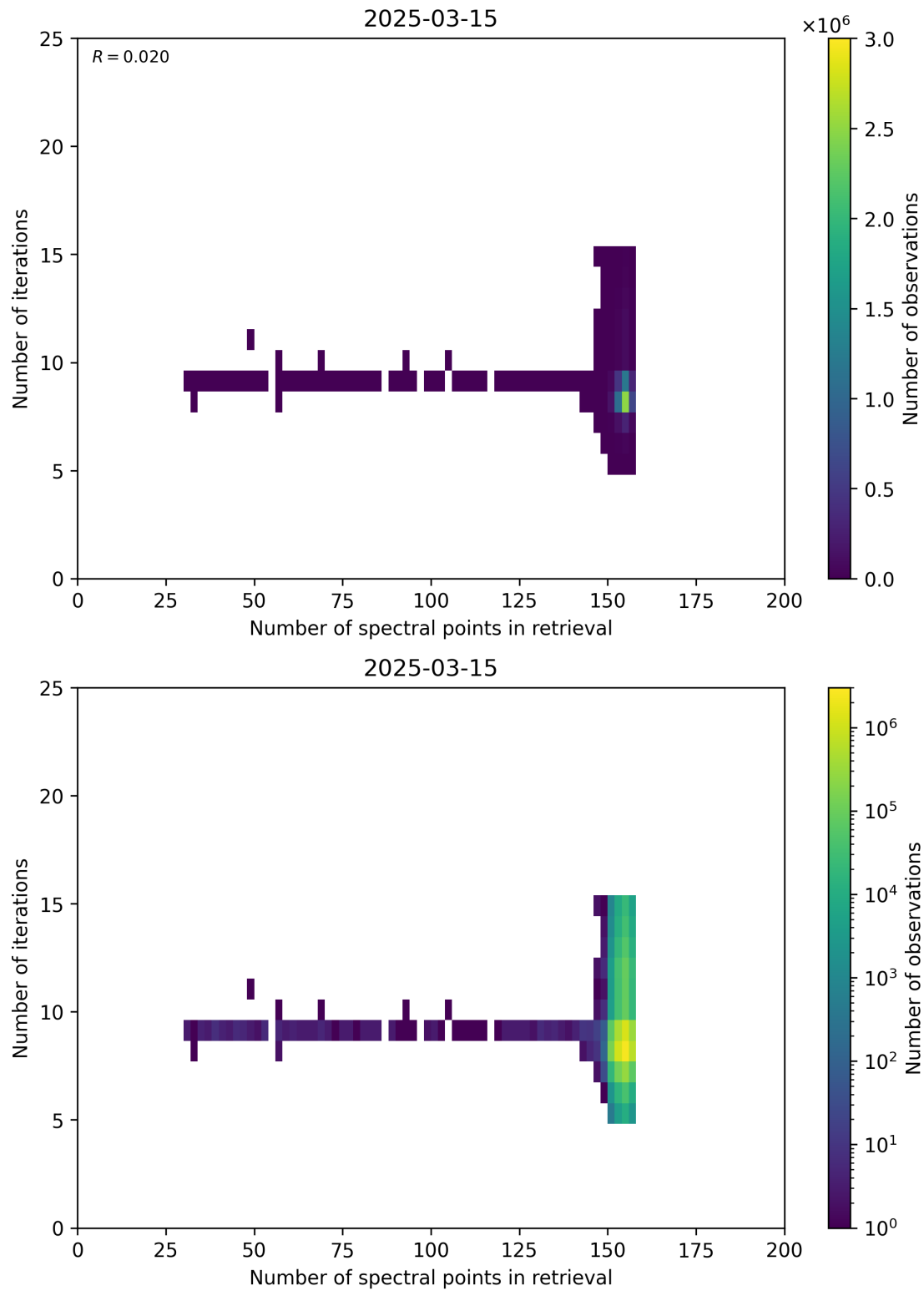
Figure 60: Scatter density plot of “Number of spectral points in retrieval” against “Number of iterations” for 2025-03-14 to 2025-03-16.
