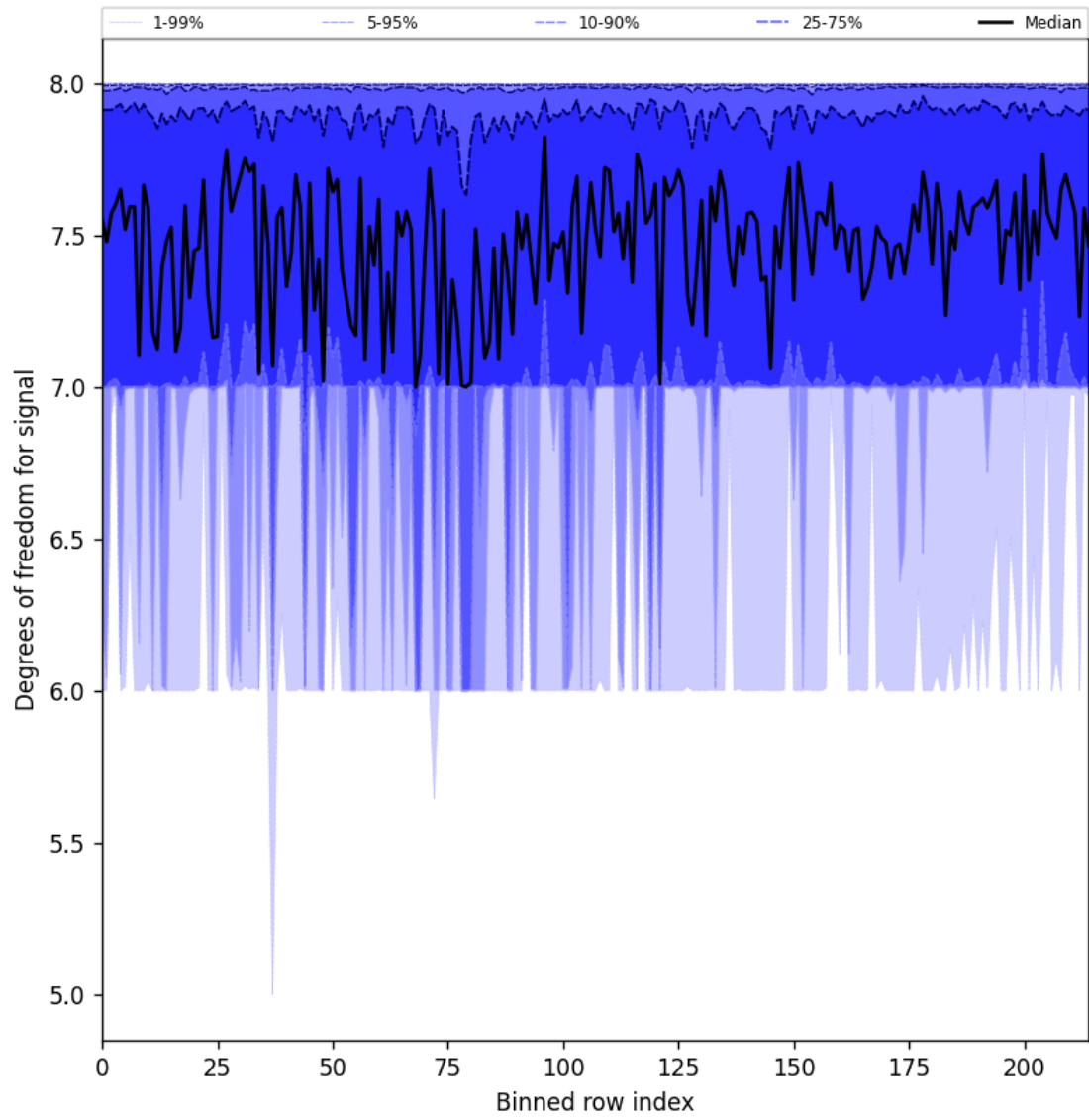
Figure 31: Along track statistics of “Degrees of freedom for signal” for 2025-03-14 to 2025-03-16
