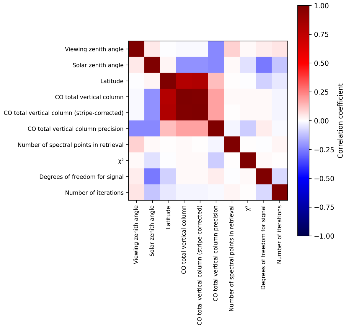
Figure 2: Map of correlation matrix for 2025-03-14 to 2025-03-16.
