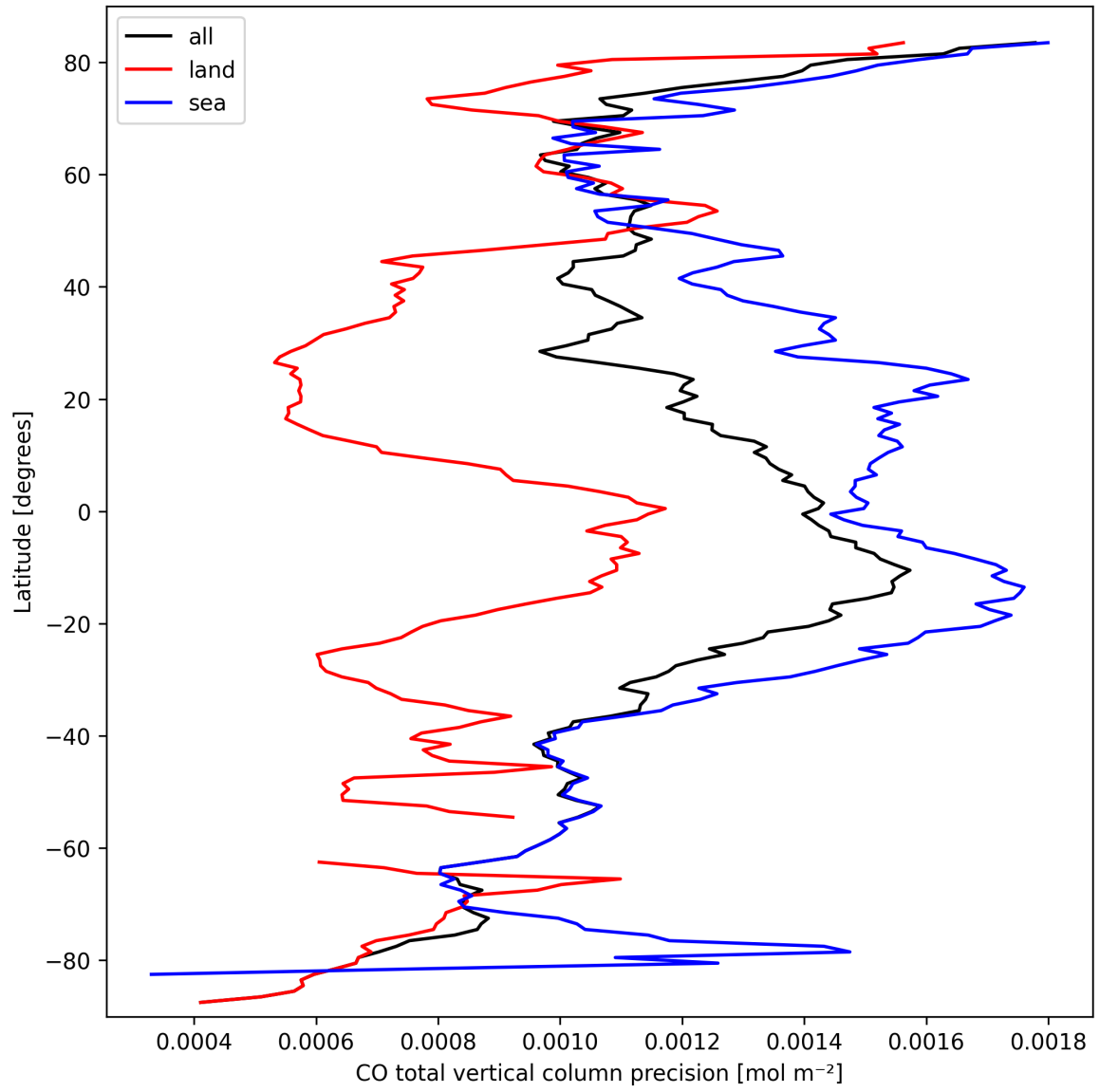
Figure 12: Zonal average of “CO total vertical column precision” for 2025-03-14 to 2025-03-16.
