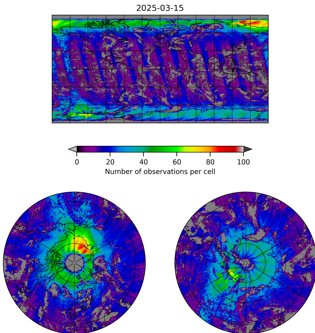
Figure 8: Map of the number of observations for 2025-03-14 to 2025-03-16
