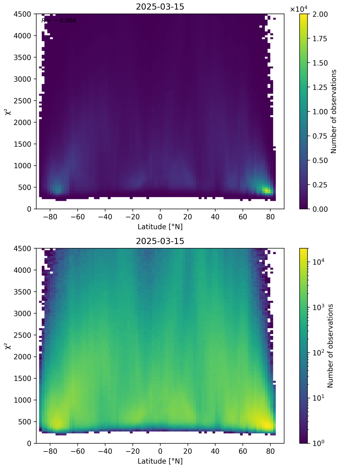
Figure 54: Scatter density plot of “Latitude” against “ \chi^2 ” for 2025-03-14 to 2025-03-16.
