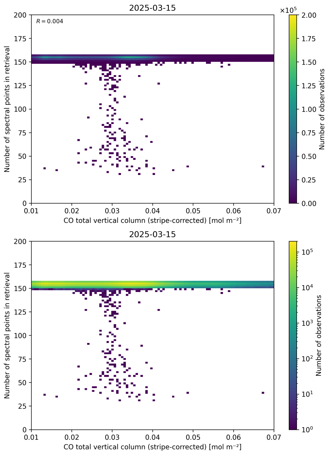
Figure 40: Scatter density plot of “CO total vertical column (stripe-corrected)” against “Number of spectral points in retrieval” for 2025-03-14 to 2025-03-16.
