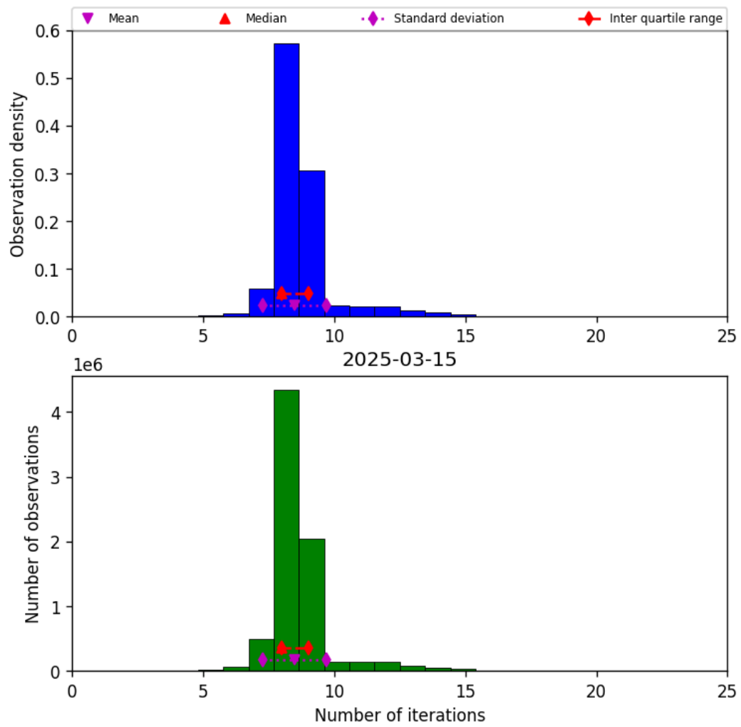
Figure 24: Histogram of “Number of iterations” for 2025-03-14 to 2025-03-16
