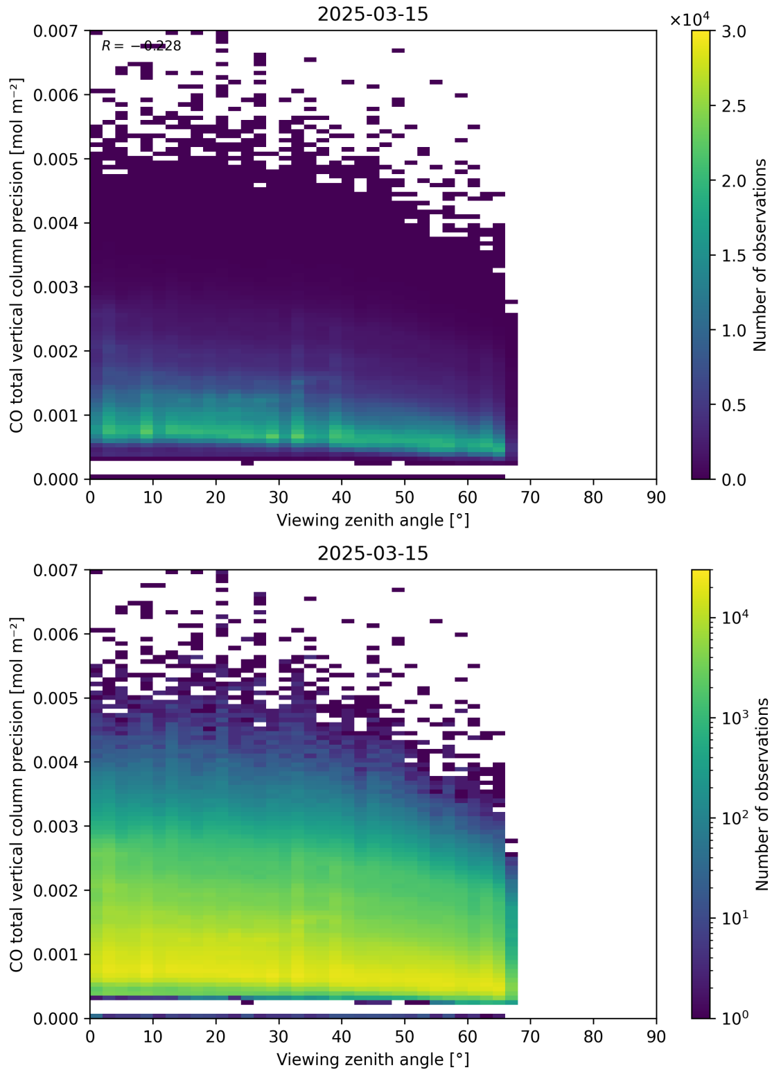
Figure 71: Scatter density plot of “Viewing zenith angle” against “CO total vertical column precision” for 2025-03-14 to 2025-03-16.
