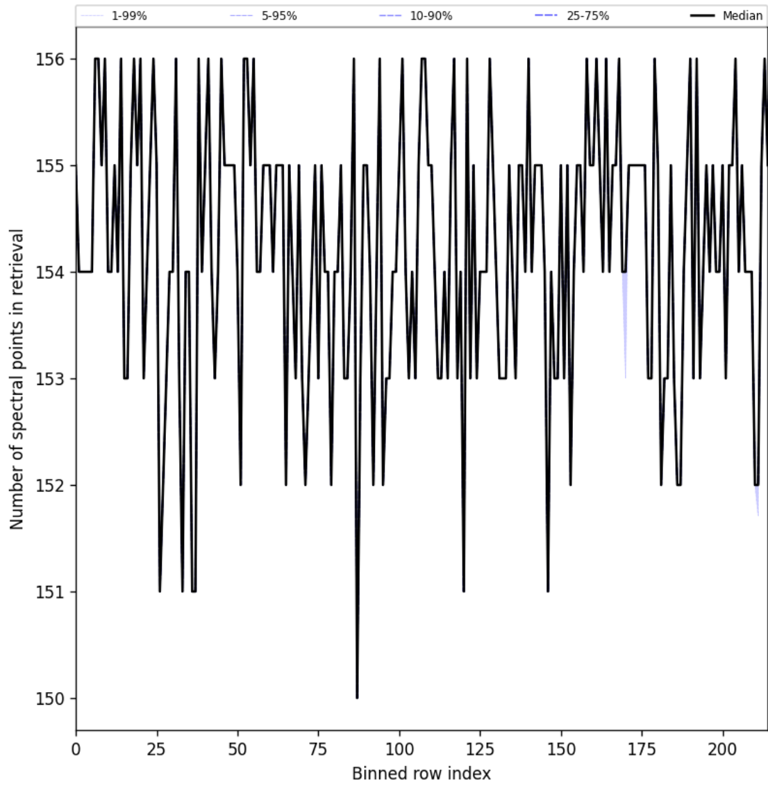
Figure 29: Along track statistics of “Number of spectral points in retrieval” for 2025-03-14 to 2025-03-16
