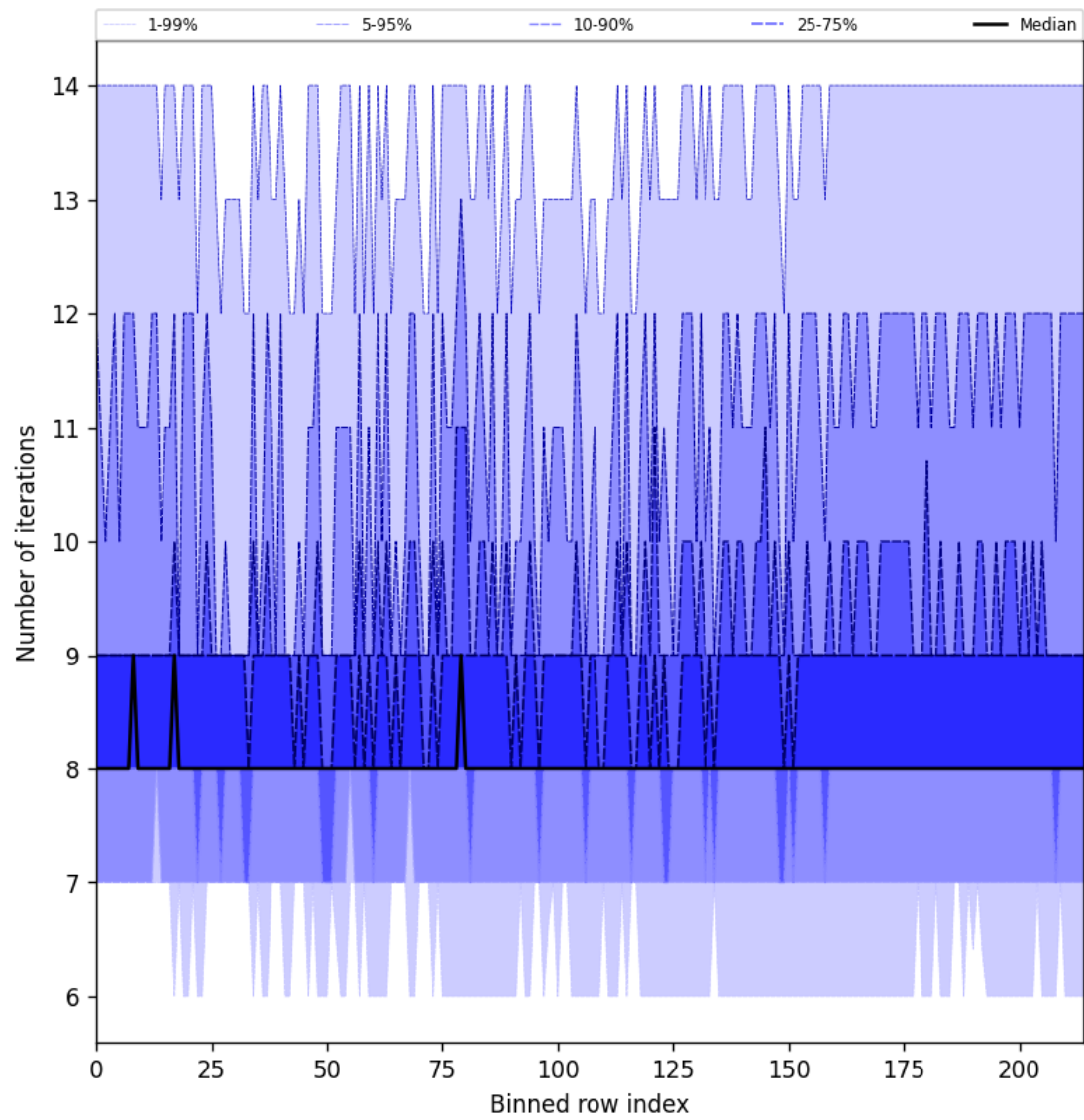
Figure 32: Along track statistics of “Number of iterations” for 2025-03-14 to 2025-03-16
