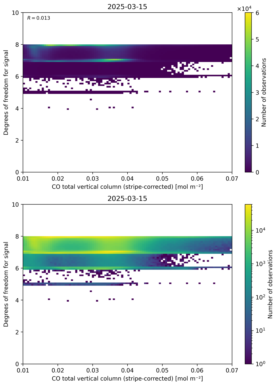
Figure 38: Scatter density plot of “CO total vertical column (stripe-corrected)” against “Degrees of freedom for signal” for 2025-03-14 to 2025-03-16.
