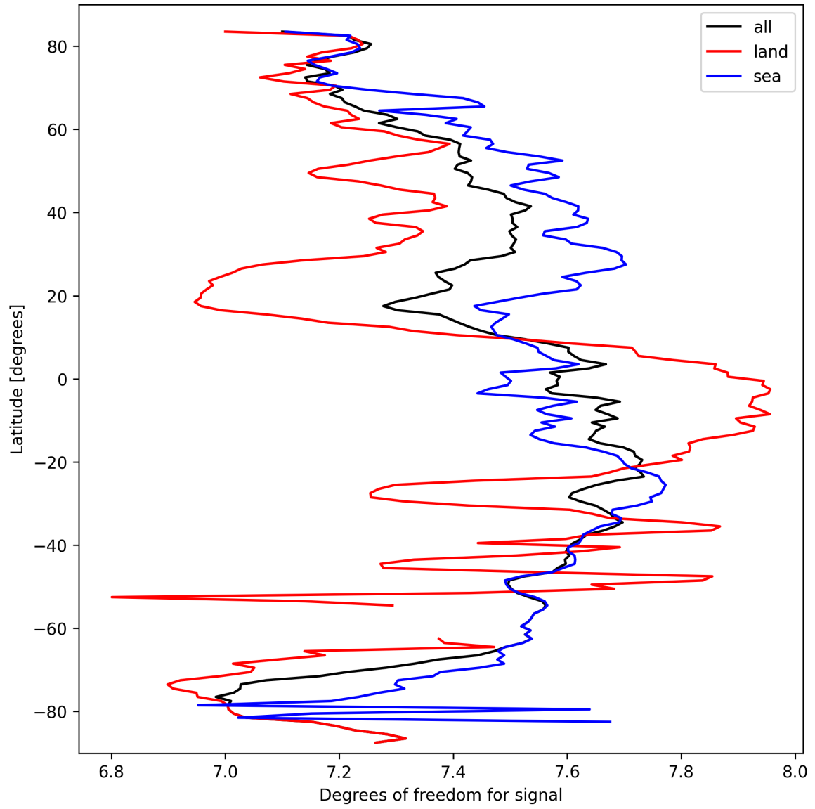
Figure 15: Zonal average of “Degrees of freedom for signal” for 2025-03-14 to 2025-03-16.
