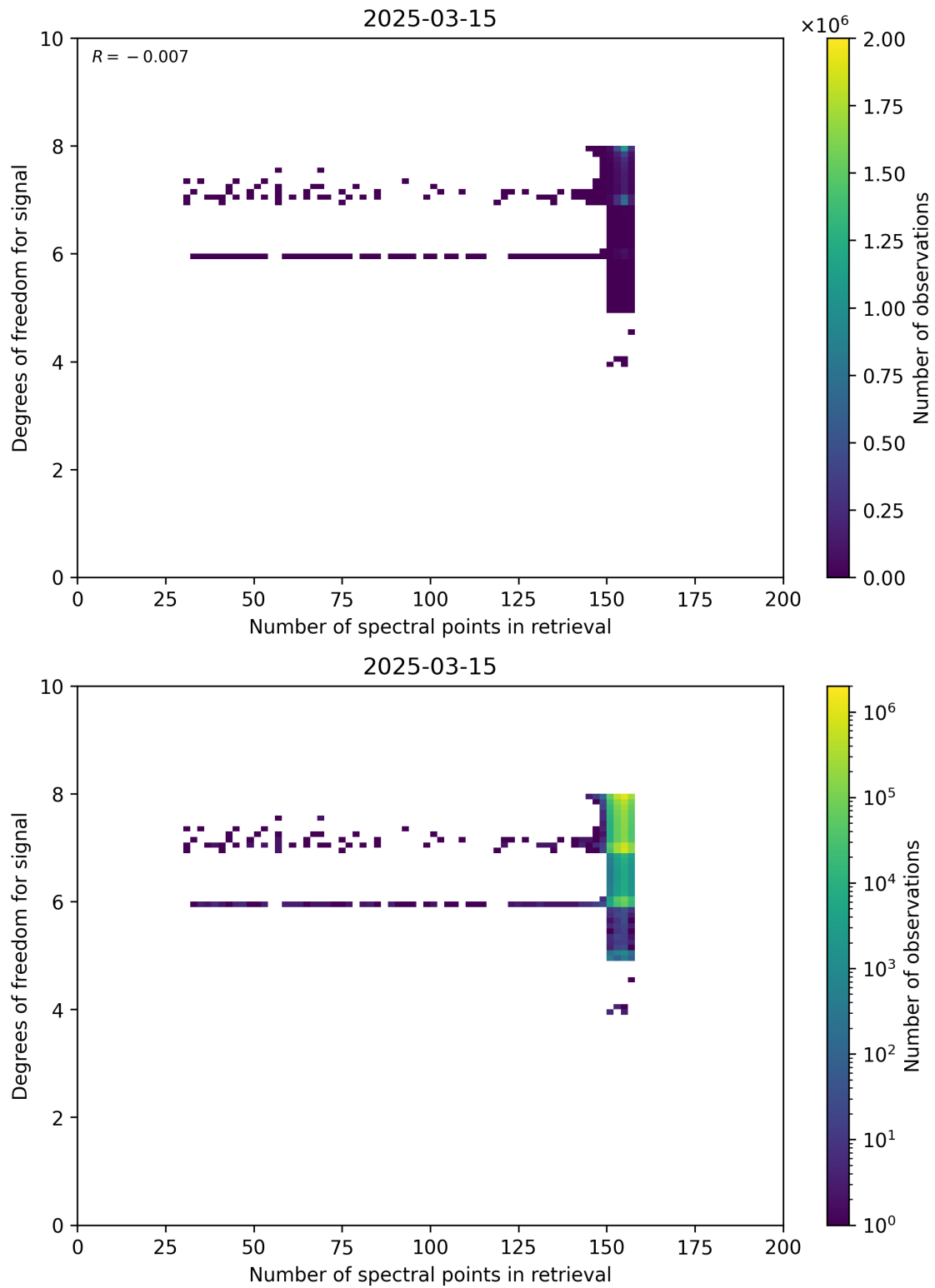
Figure 59: Scatter density plot of “Number of spectral points in retrieval” against “Degrees of freedom for signal” for 2025-03-14 to 2025-03-16.
