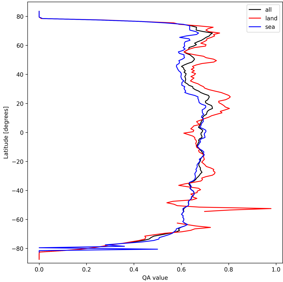
Figure 9: Zonal average of “QA value” for 2025-03-14 to 2025-03-16.
