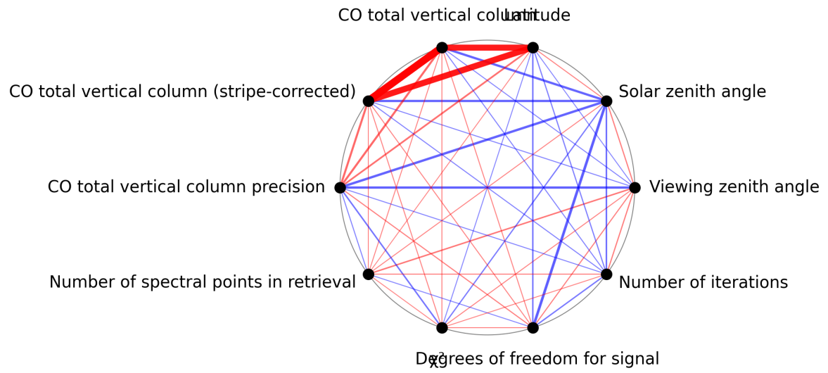
Figure 1: Map of correlation graph for 2025-03-14 to 2025-03-16.
