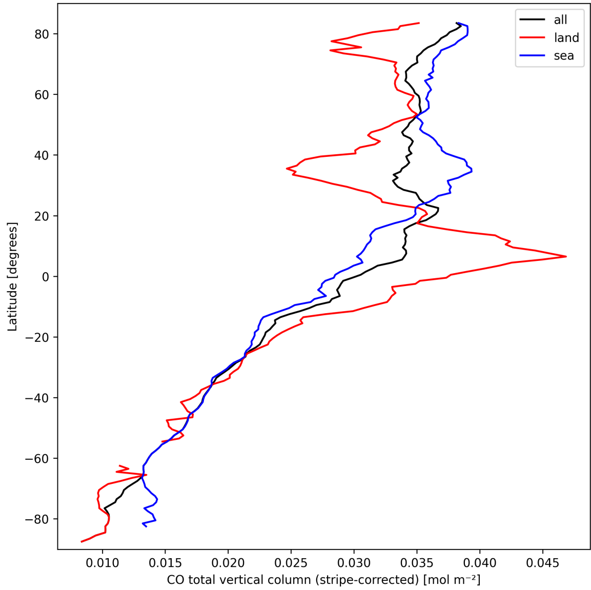
Figure 11: Zonal average of “CO total vertical column (stripe-corrected)” for 2025-03-14 to 2025-03-16.
