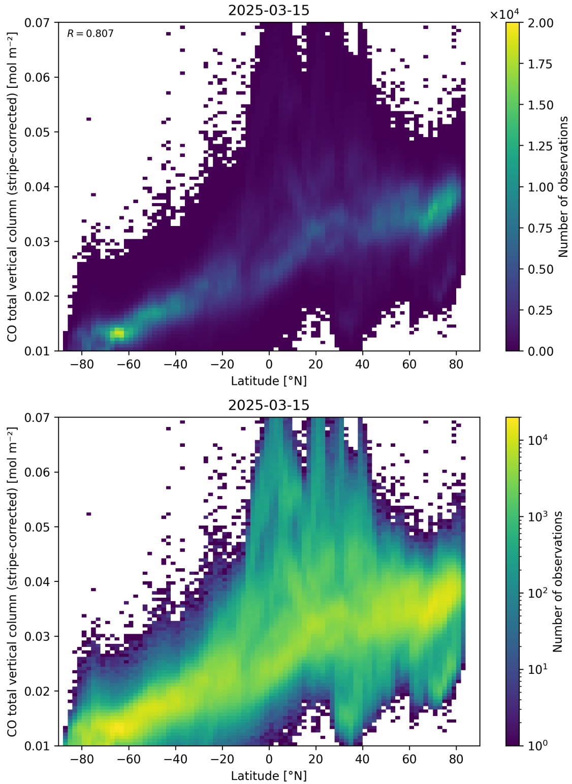
Figure 52: Scatter density plot of “Latitude” against “CO total vertical column (stripe-corrected)” for 2025-03-14 to 2025-03-16.
