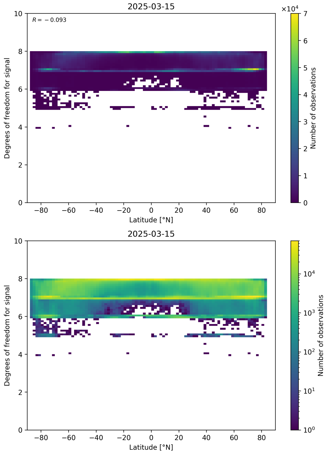
Figure 55: Scatter density plot of “Latitude” against “Degrees of freedom for signal” for 2025-03-14 to 2025-03-16.
