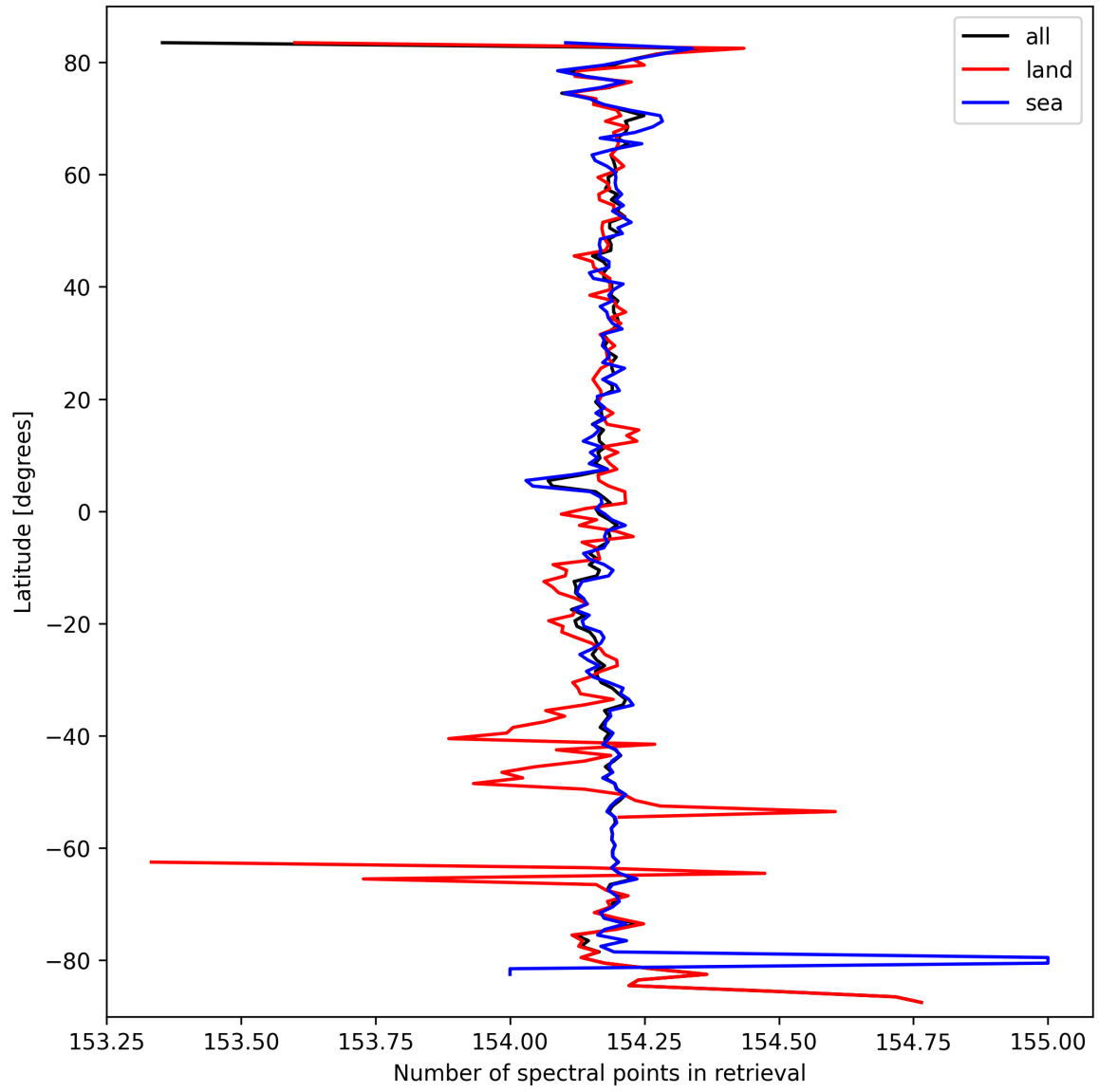
Figure 13: Zonal average of “Number of spectral points in retrieval” for 2025-03-14 to 2025-03-16.
