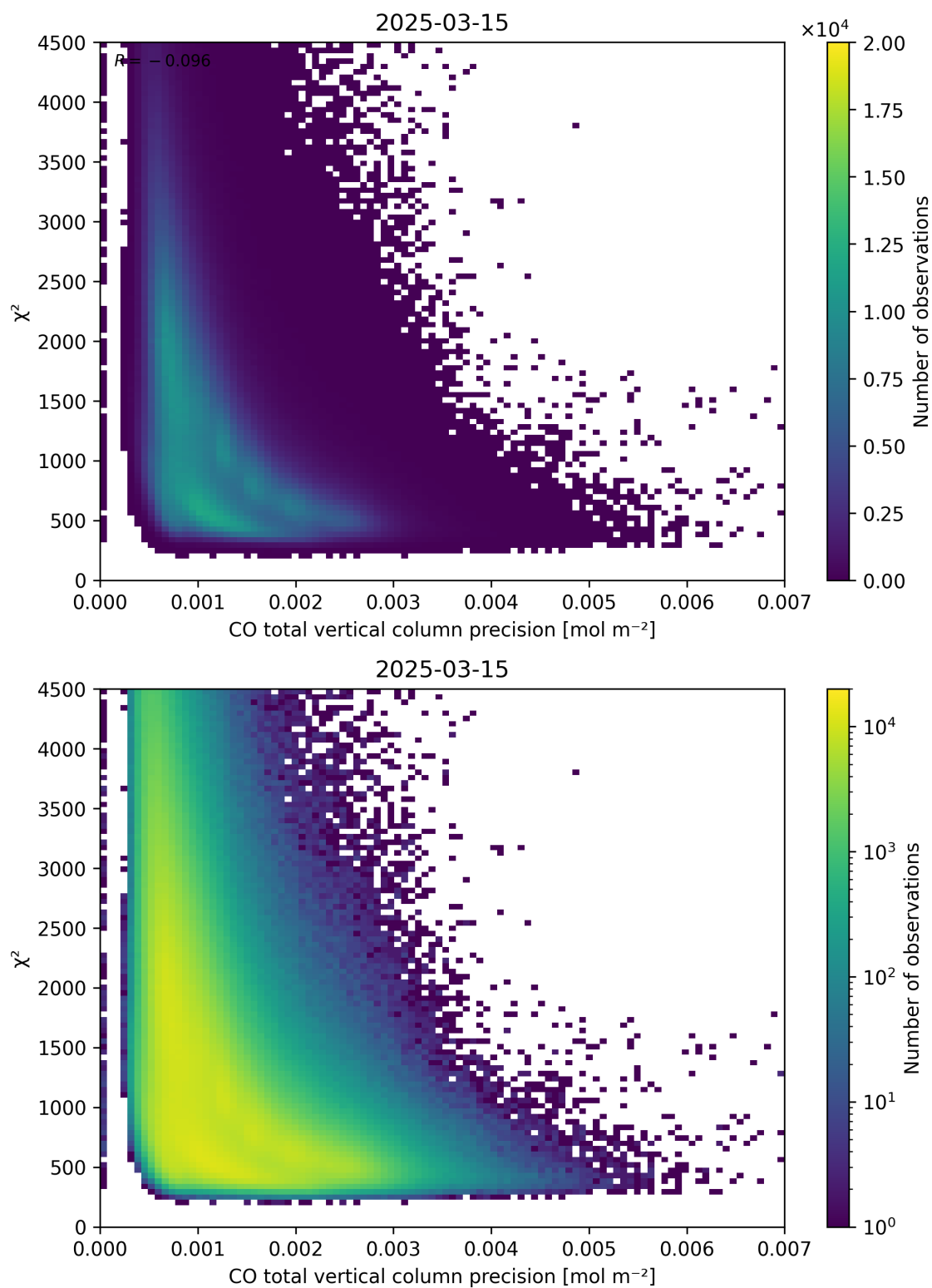
Figure 44: Scatter density plot of “CO total vertical column precision” against “ \chi^2 ” for 2025-03-14 to 2025-03-16.
