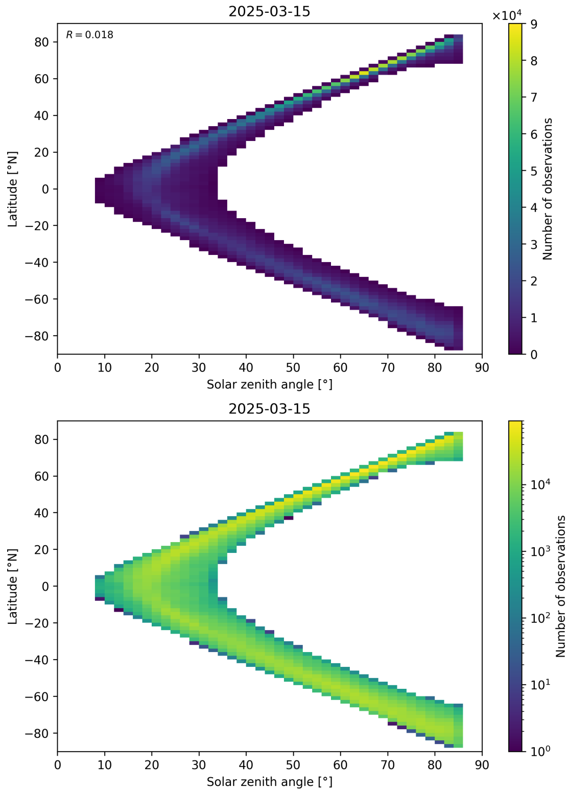
Figure 66: Scatter density plot of “Solar zenith angle” against “Latitude” for 2025-03-14 to 2025-03-16.
