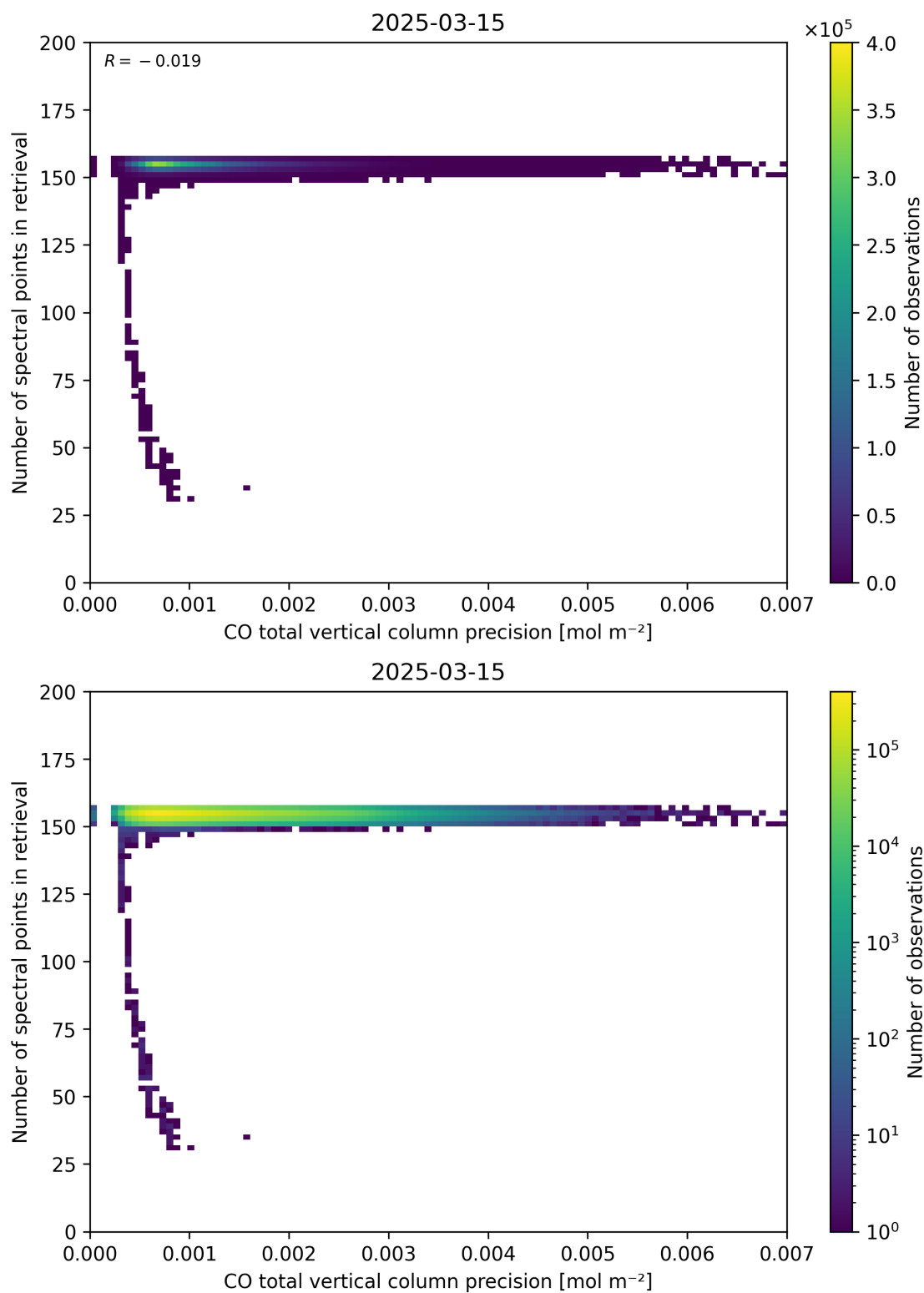
Figure 47: Scatter density plot of “CO total vertical column precision” against “Number of spectral points in retrieval” for 2025-03-14 to 2025-03-16.
