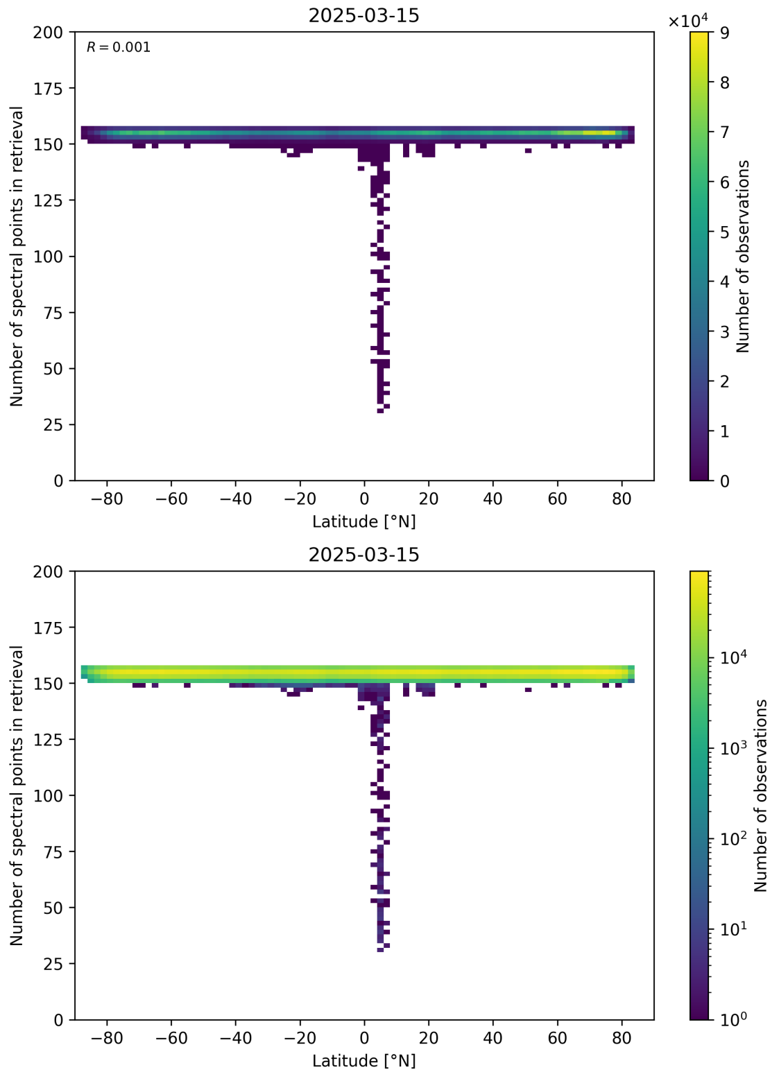
Figure 57: Scatter density plot of “Latitude” against “Number of spectral points in retrieval” for 2025-03-14 to 2025-03-16.
