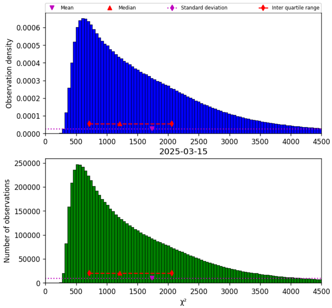
Figure 22: Histogram of “ \chi^2 ” for 2025-03-14 to 2025-03-16
