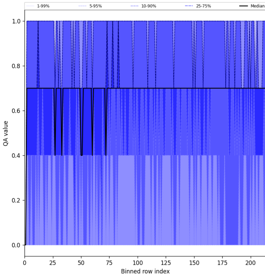
Figure 25: Along track statistics of “QA value” for 2025-03-14 to 2025-03-16
