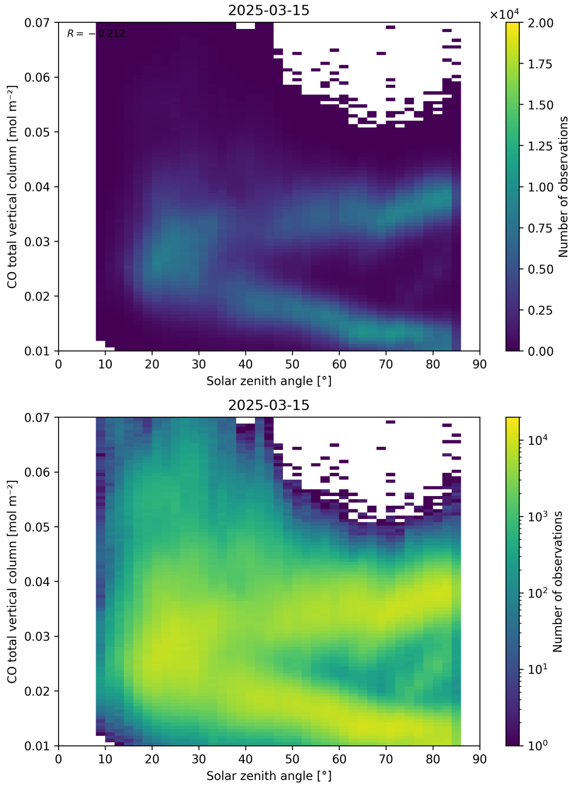
Figure 61: Scatter density plot of “Solar zenith angle” against “CO total vertical column” for 2025-03-14 to 2025-03-16.
