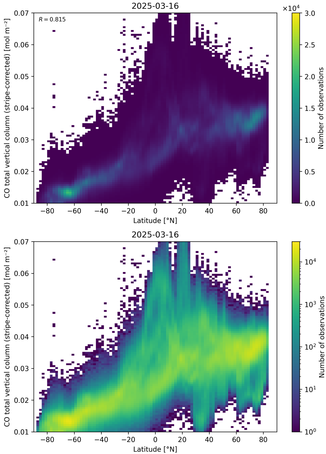
Figure 52: Scatter density plot of “Latitude” against “CO total vertical column (stripe-corrected)” for 2025-03-15 to 2025-03-17.
