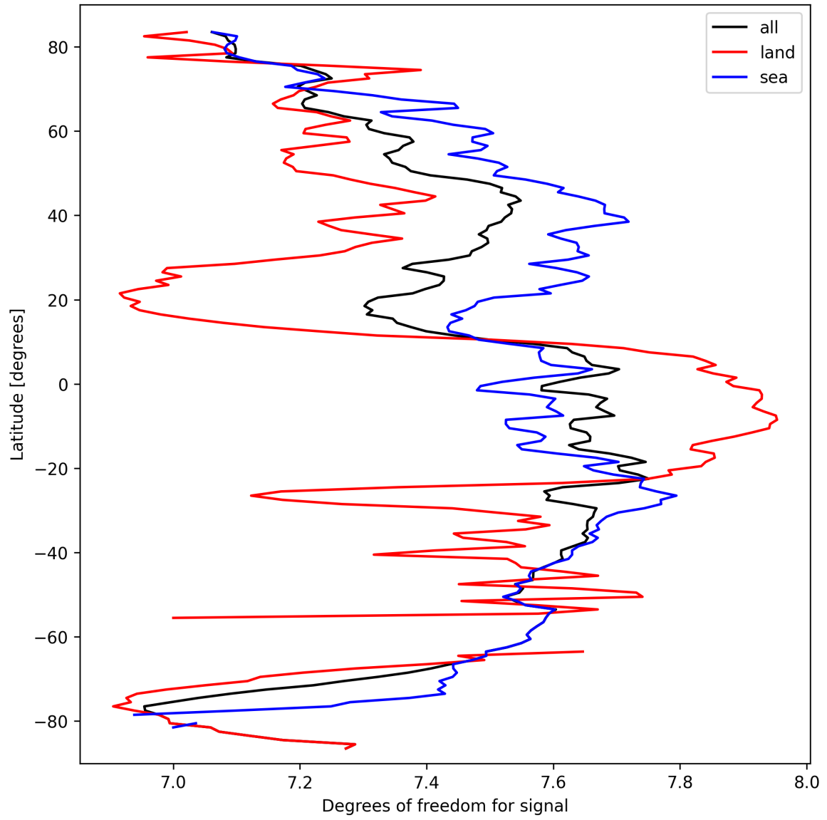
Figure 15: Zonal average of “Degrees of freedom for signal” for 2025-03-15 to 2025-03-17.
