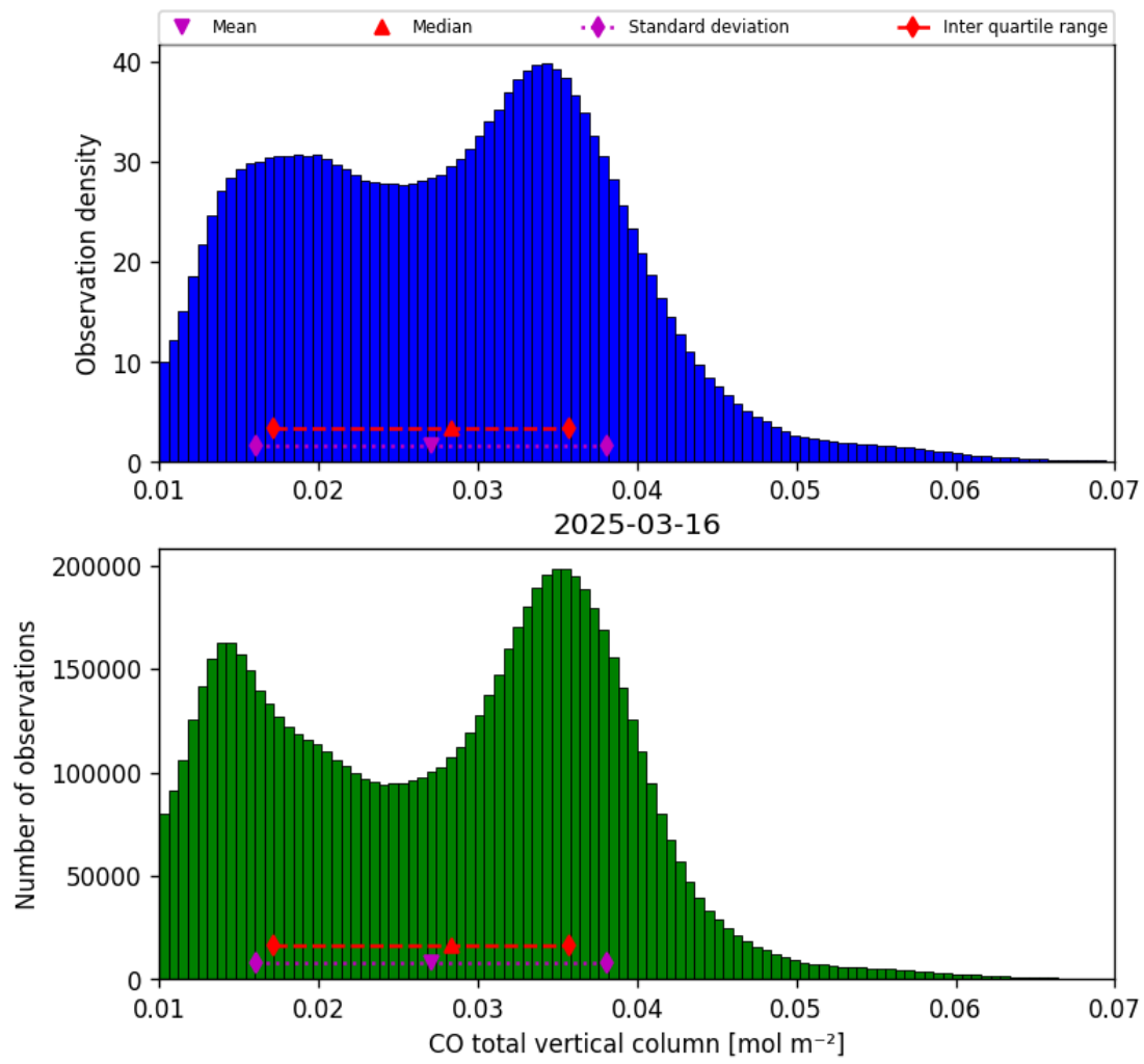
Figure 18: Histogram of “CO total vertical column” for 2025-03-15 to 2025-03-17
