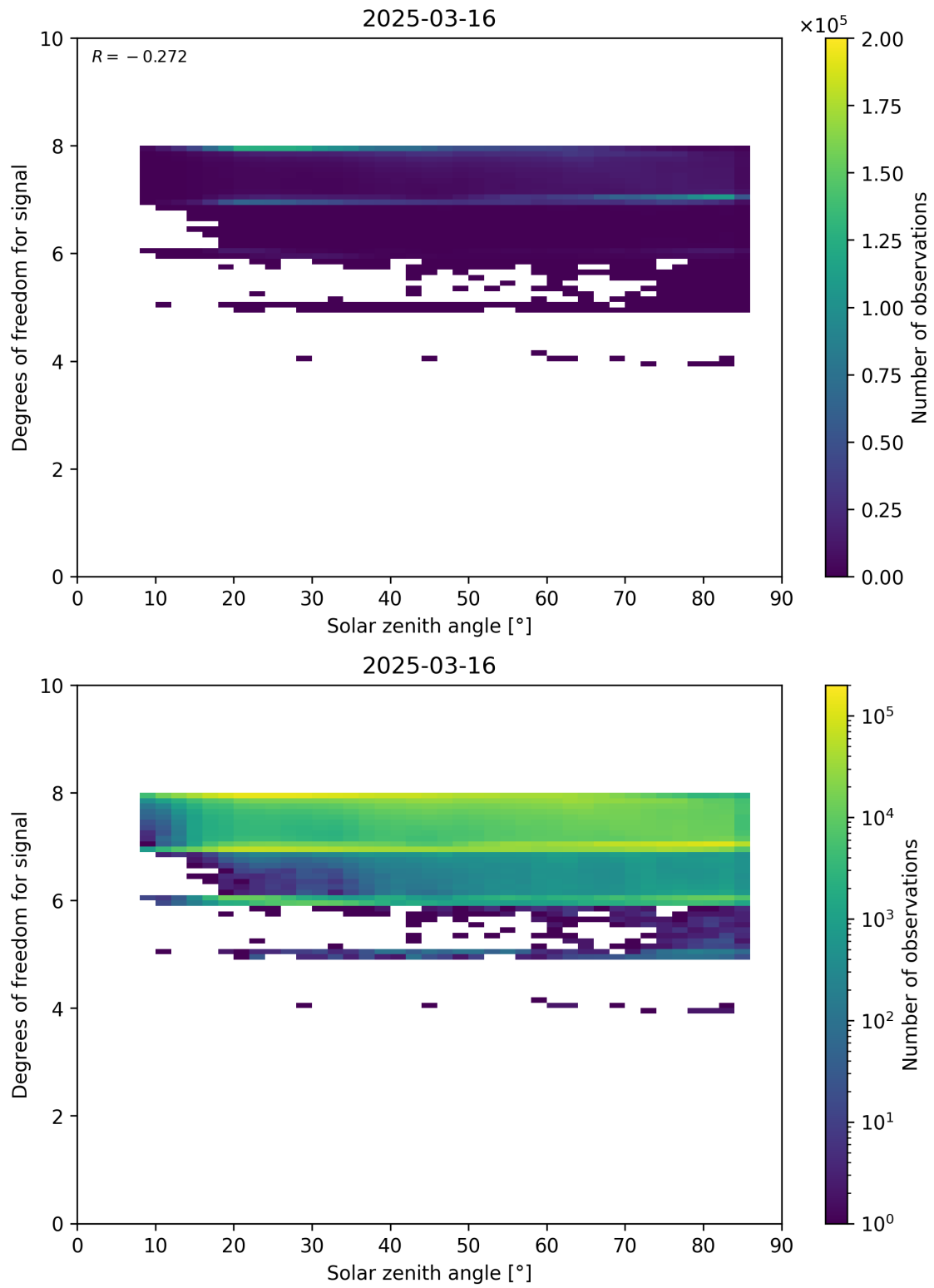
Figure 65: Scatter density plot of “Solar zenith angle” against “Degrees of freedom for signal” for 2025-03-15 to 2025-03-17.
