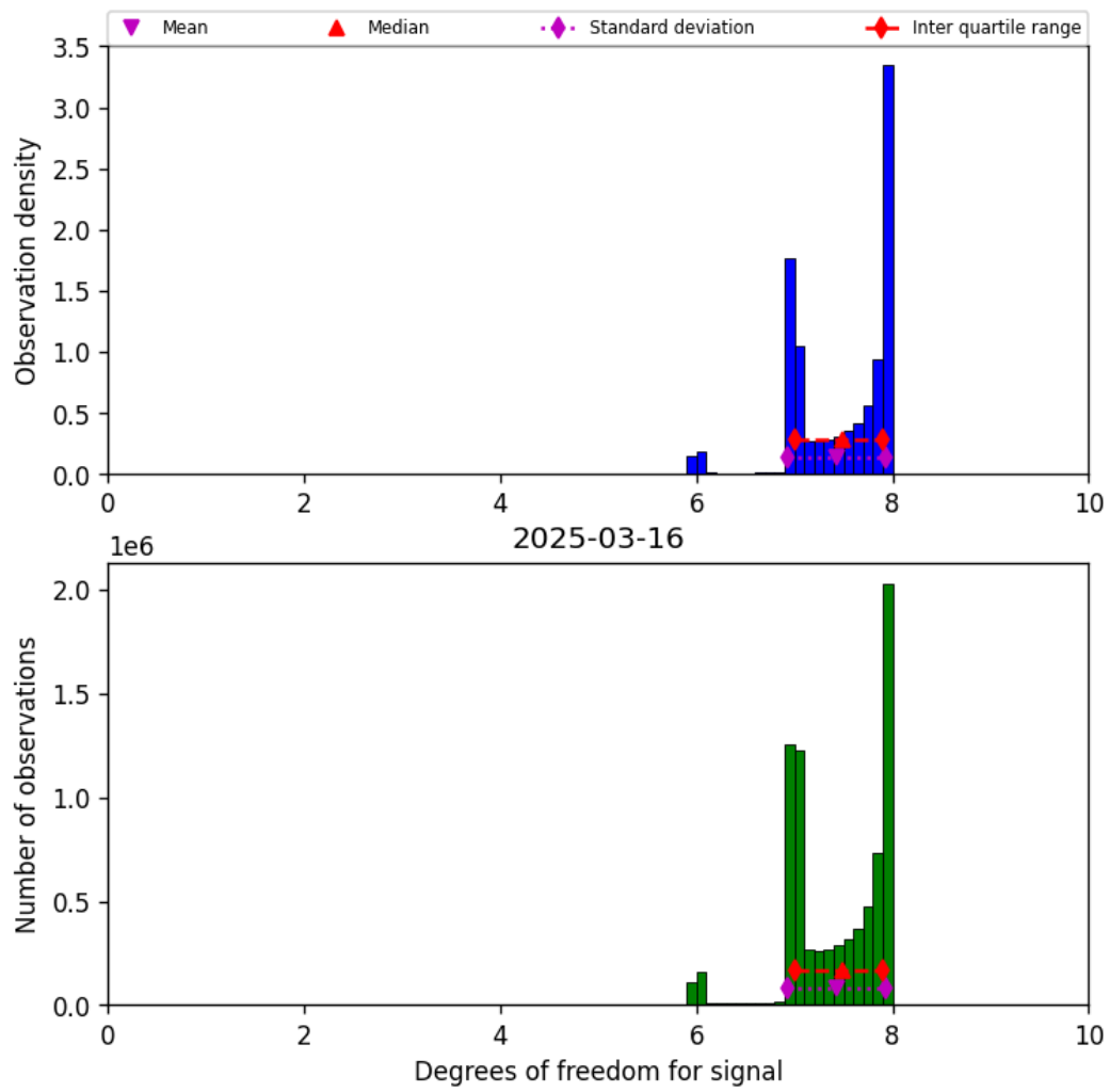
Figure 23: Histogram of “Degrees of freedom for signal” for 2025-03-15 to 2025-03-17
