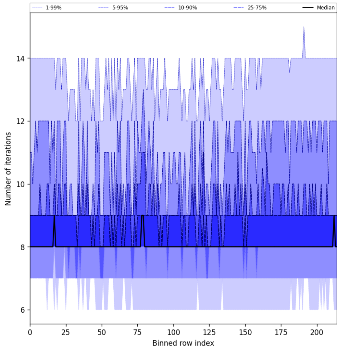
Figure 32: Along track statistics of “Number of iterations” for 2025-03-15 to 2025-03-17
