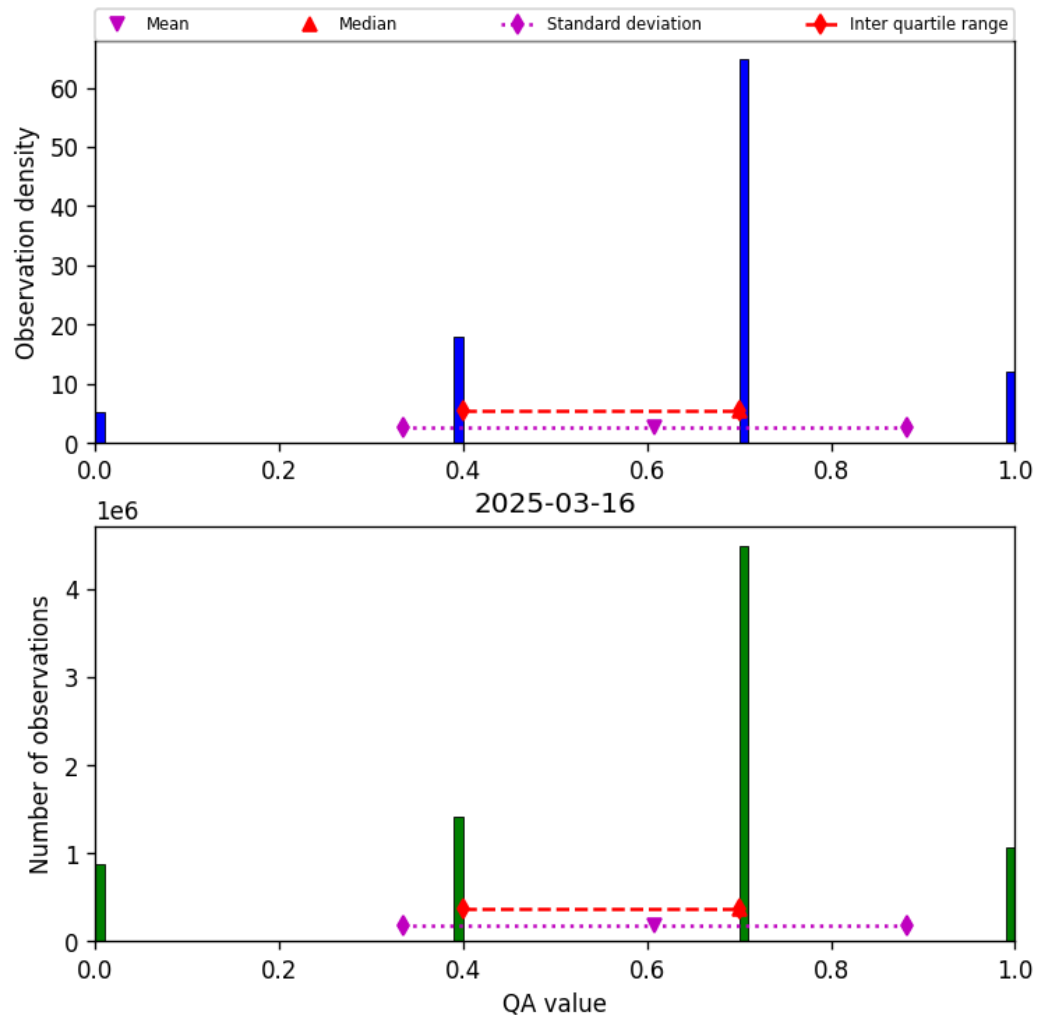
Figure 17: Histogram of “QA value” for 2025-03-15 to 2025-03-17
