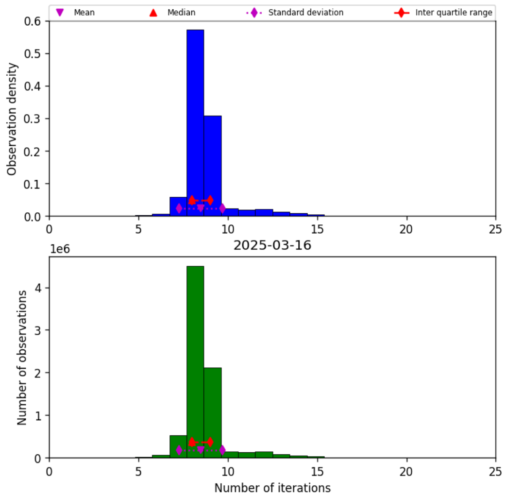
Figure 24: Histogram of “Number of iterations” for 2025-03-15 to 2025-03-17
