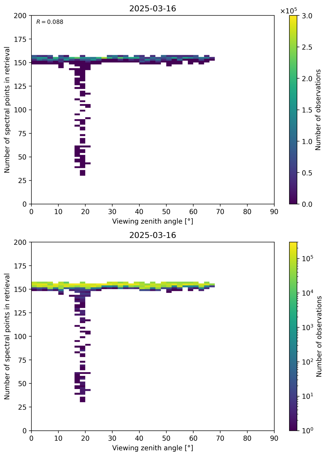
Figure 76: Scatter density plot of “Viewing zenith angle” against “Number of spectral points in retrieval” for 2025-03-15 to 2025-03-17.
