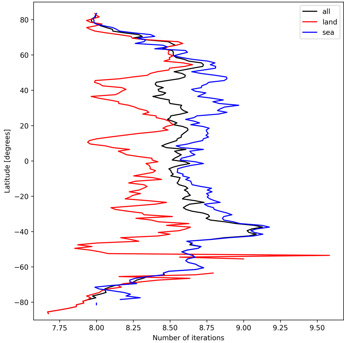
Figure 16: Zonal average of “Number of iterations” for 2025-03-15 to 2025-03-17.
