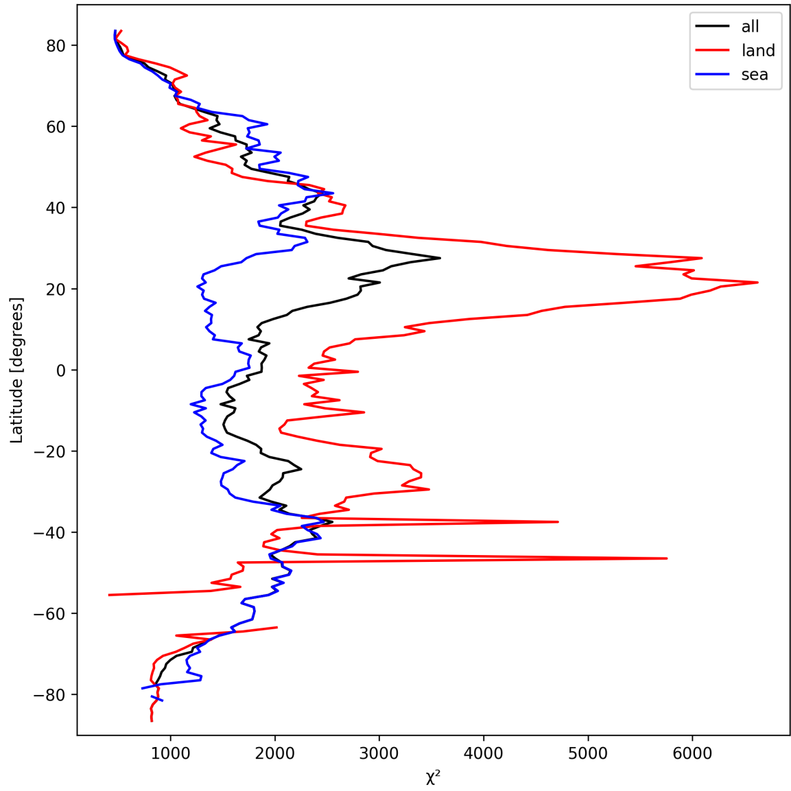
Figure 14: Zonal average of “ \chi^2 ” for 2025-03-15 to 2025-03-17.
