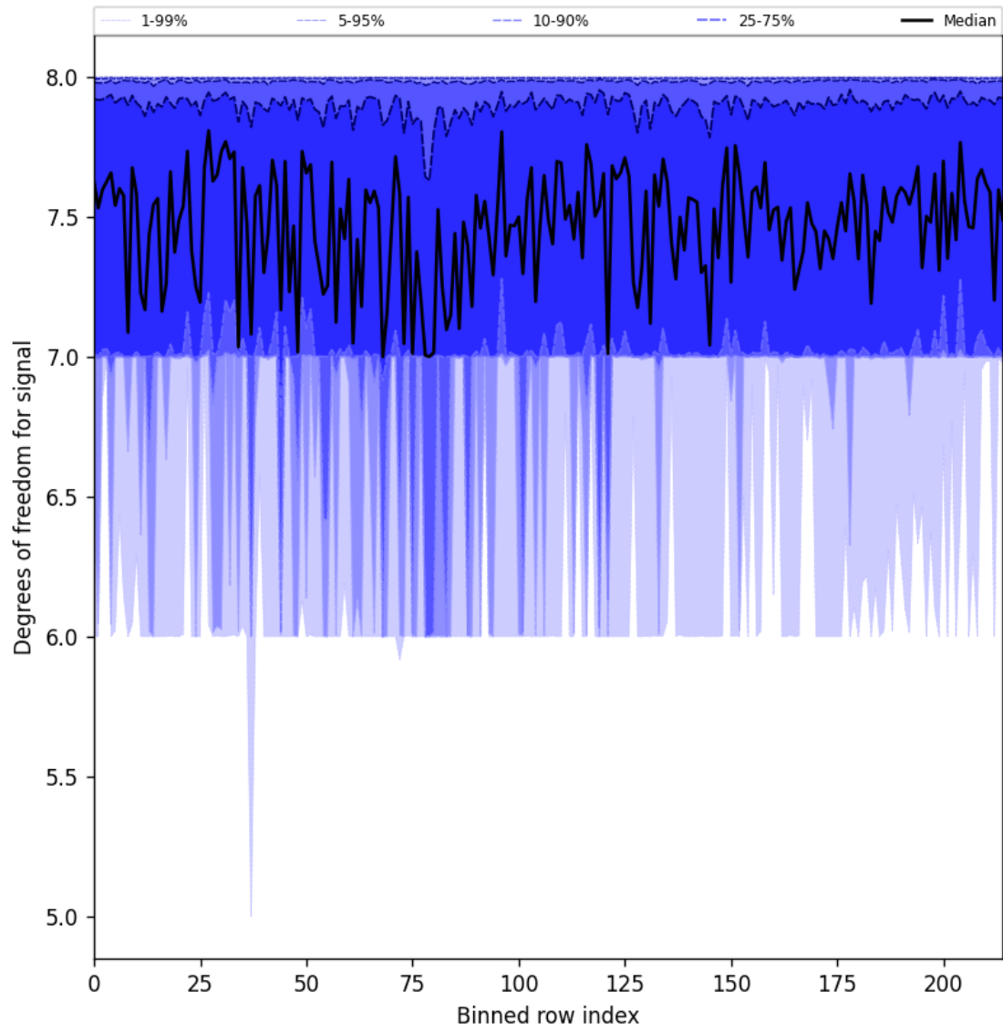
Figure 31: Along track statistics of “Degrees of freedom for signal” for 2025-03-15 to 2025-03-17
