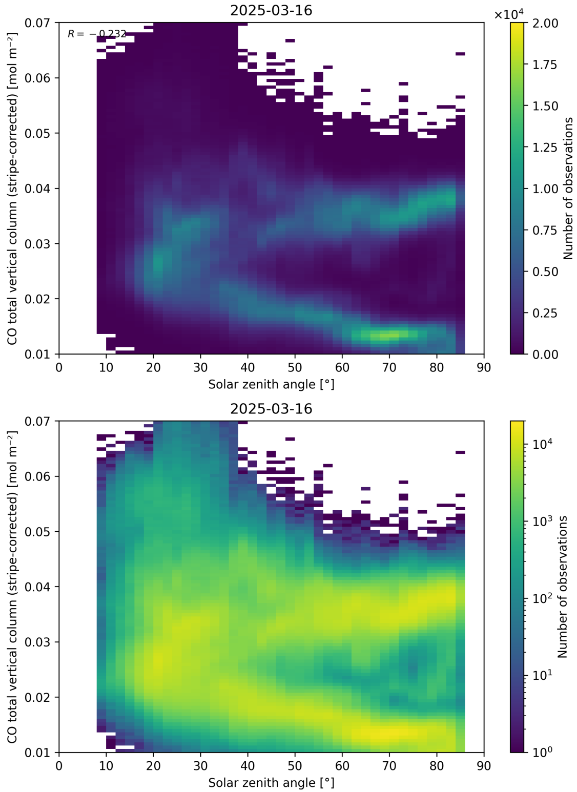
Figure 62: Scatter density plot of “Solar zenith angle” against “CO total vertical column (stripe-corrected)” for 2025-03-15 to 2025-03-17.
