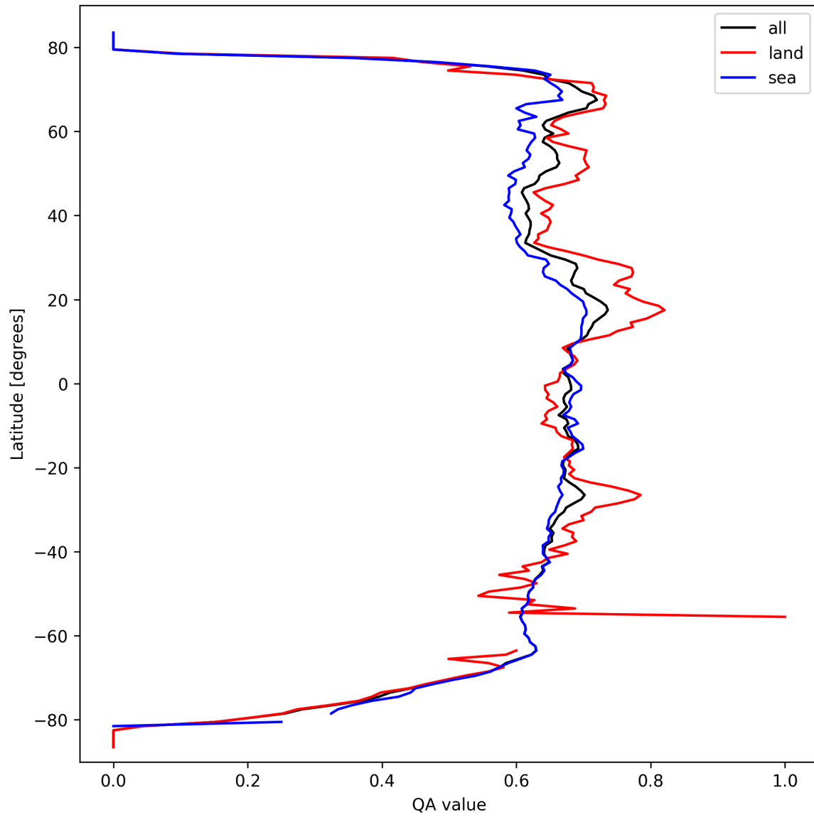
Figure 9: Zonal average of “QA value” for 2025-03-15 to 2025-03-17.
