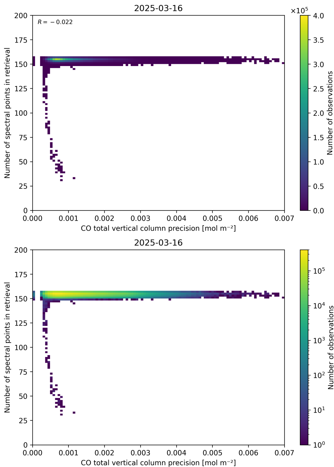
Figure 47: Scatter density plot of “CO total vertical column precision” against “Number of spectral points in retrieval” for 2025-03-15 to 2025-03-17.
