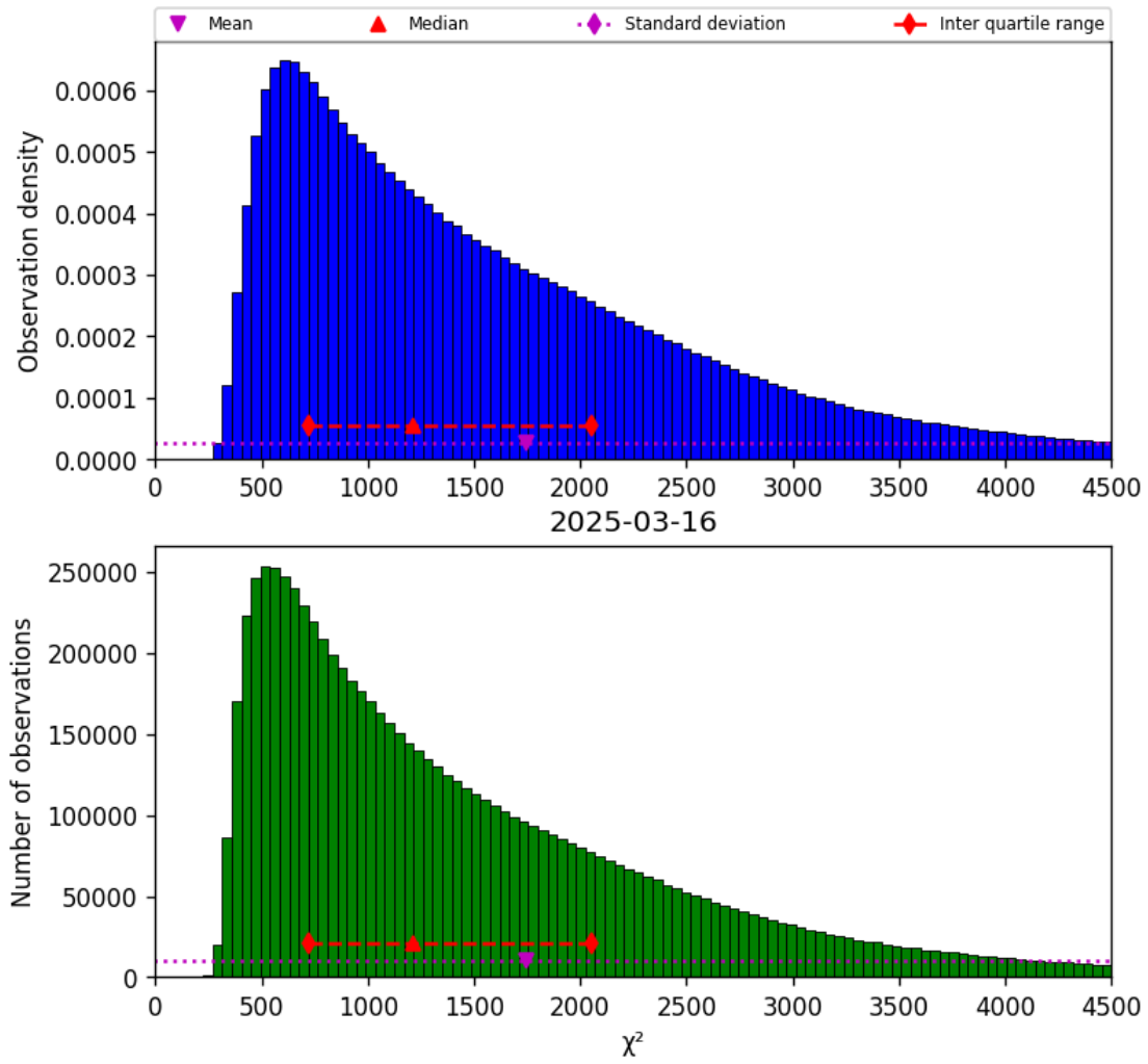
Figure 22: Histogram of “ \chi^2 ” for 2025-03-15 to 2025-03-17
