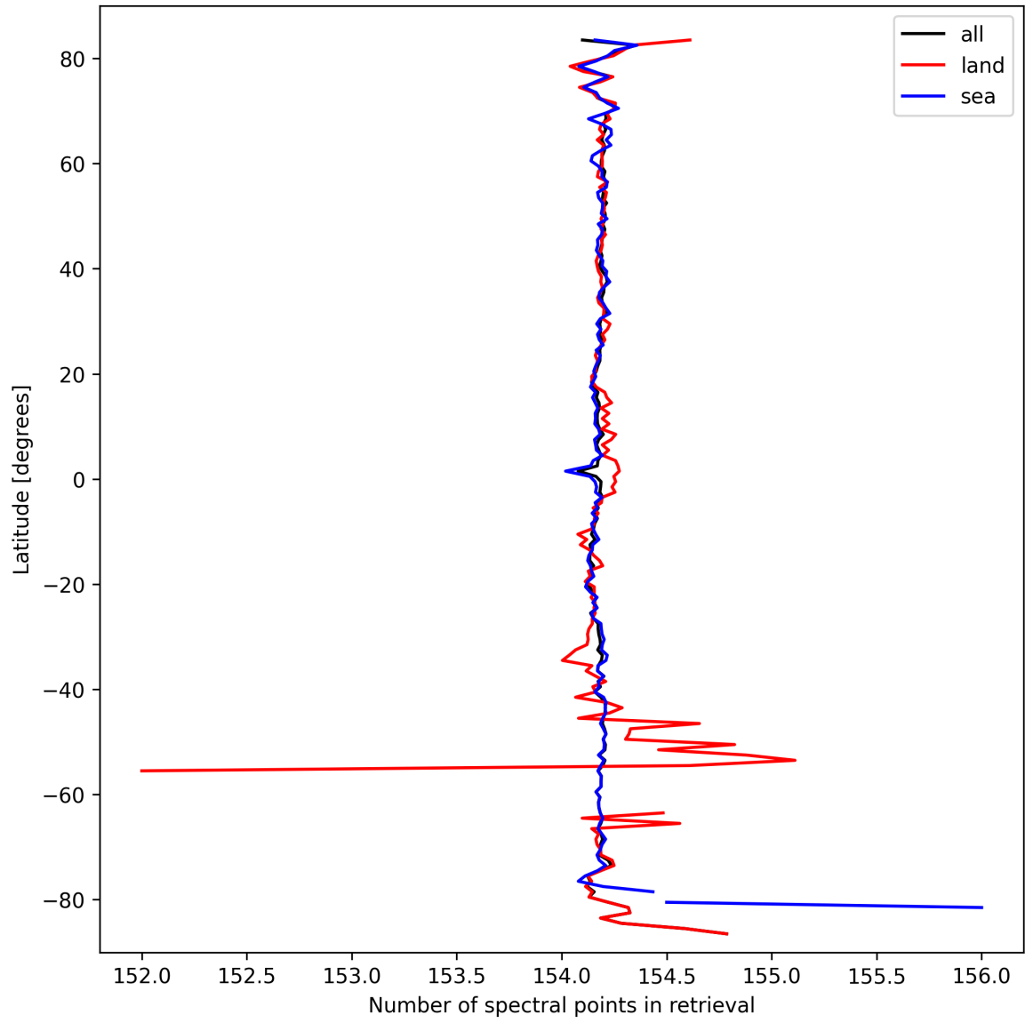
Figure 13: Zonal average of “Number of spectral points in retrieval” for 2025-03-15 to 2025-03-17.
