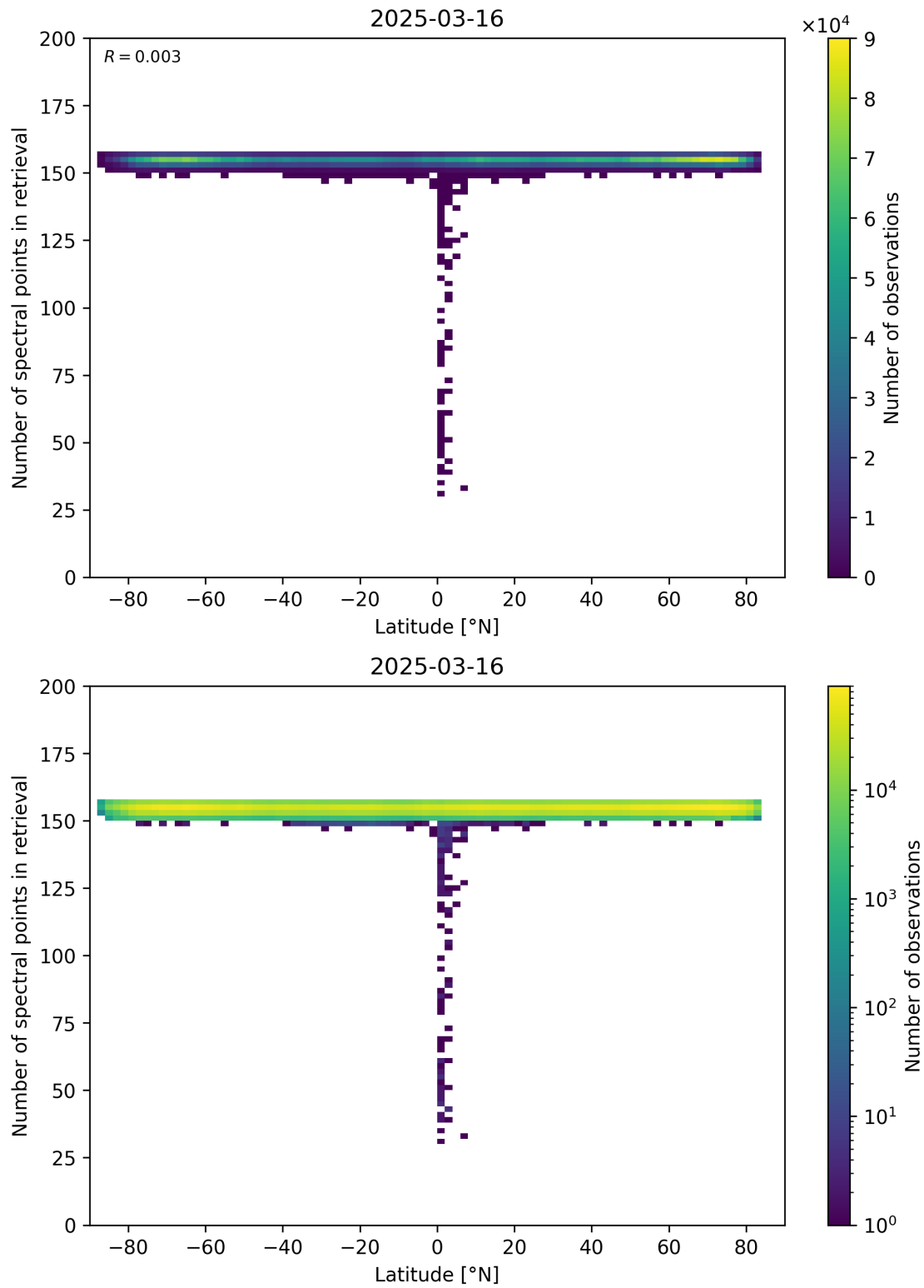
Figure 57: Scatter density plot of “Latitude” against “Number of spectral points in retrieval” for 2025-03-15 to 2025-03-17.
