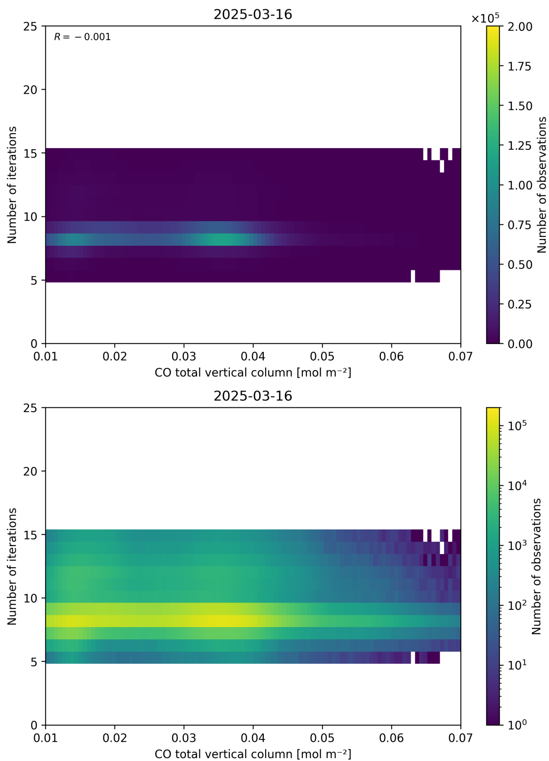
Figure 42: Scatter density plot of “CO total vertical column” against “Number of iterations” for 2025-03-15 to 2025-03-17.
