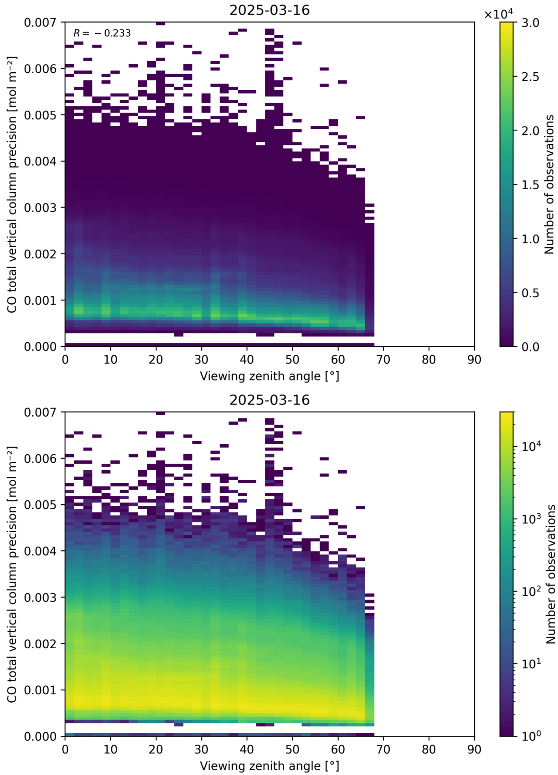
Figure 71: Scatter density plot of “Viewing zenith angle” against “CO total vertical column precision” for 2025-03-15 to 2025-03-17.
