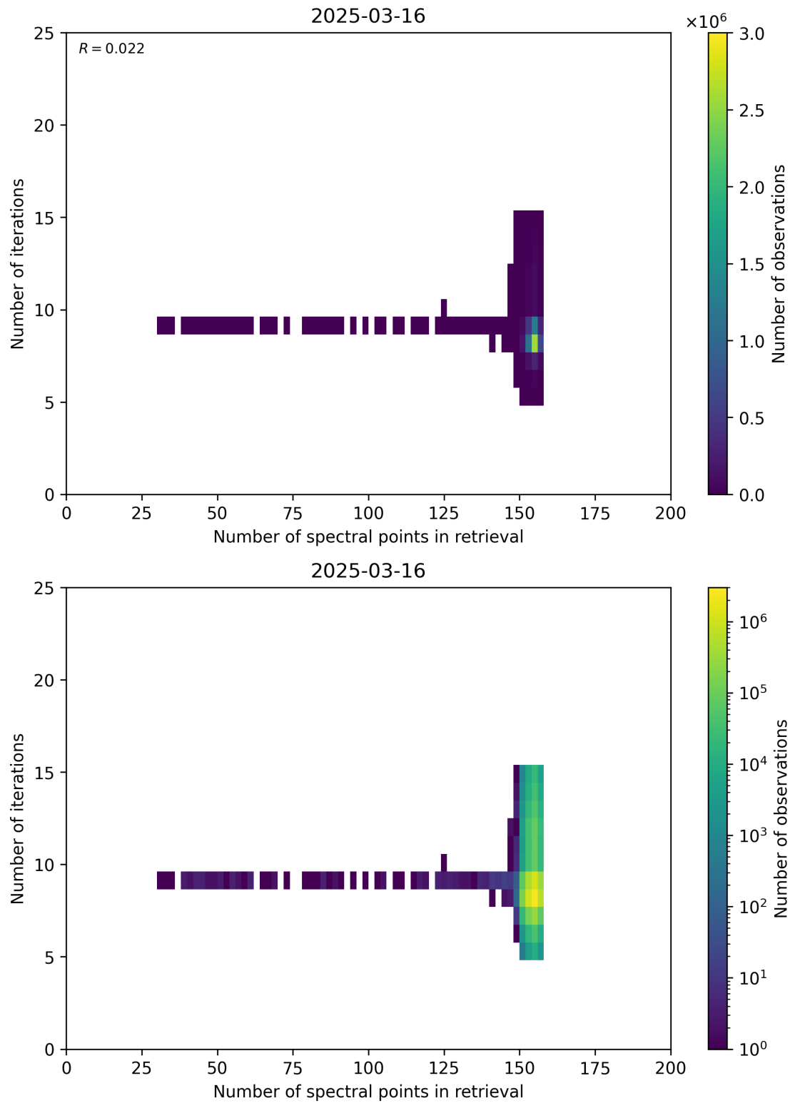
Figure 60: Scatter density plot of “Number of spectral points in retrieval” against “Number of iterations” for 2025-03-15 to 2025-03-17.
