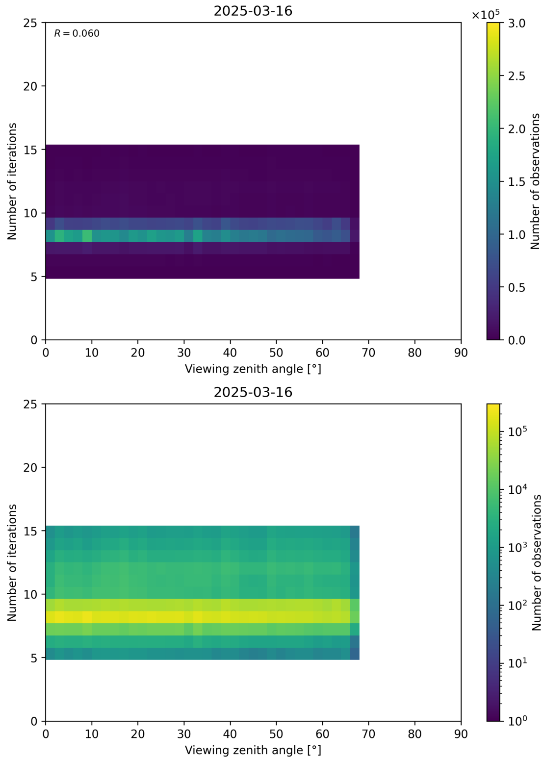
Figure 75: Scatter density plot of “Viewing zenith angle” against “Number of iterations” for 2025-03-15 to 2025-03-17.
