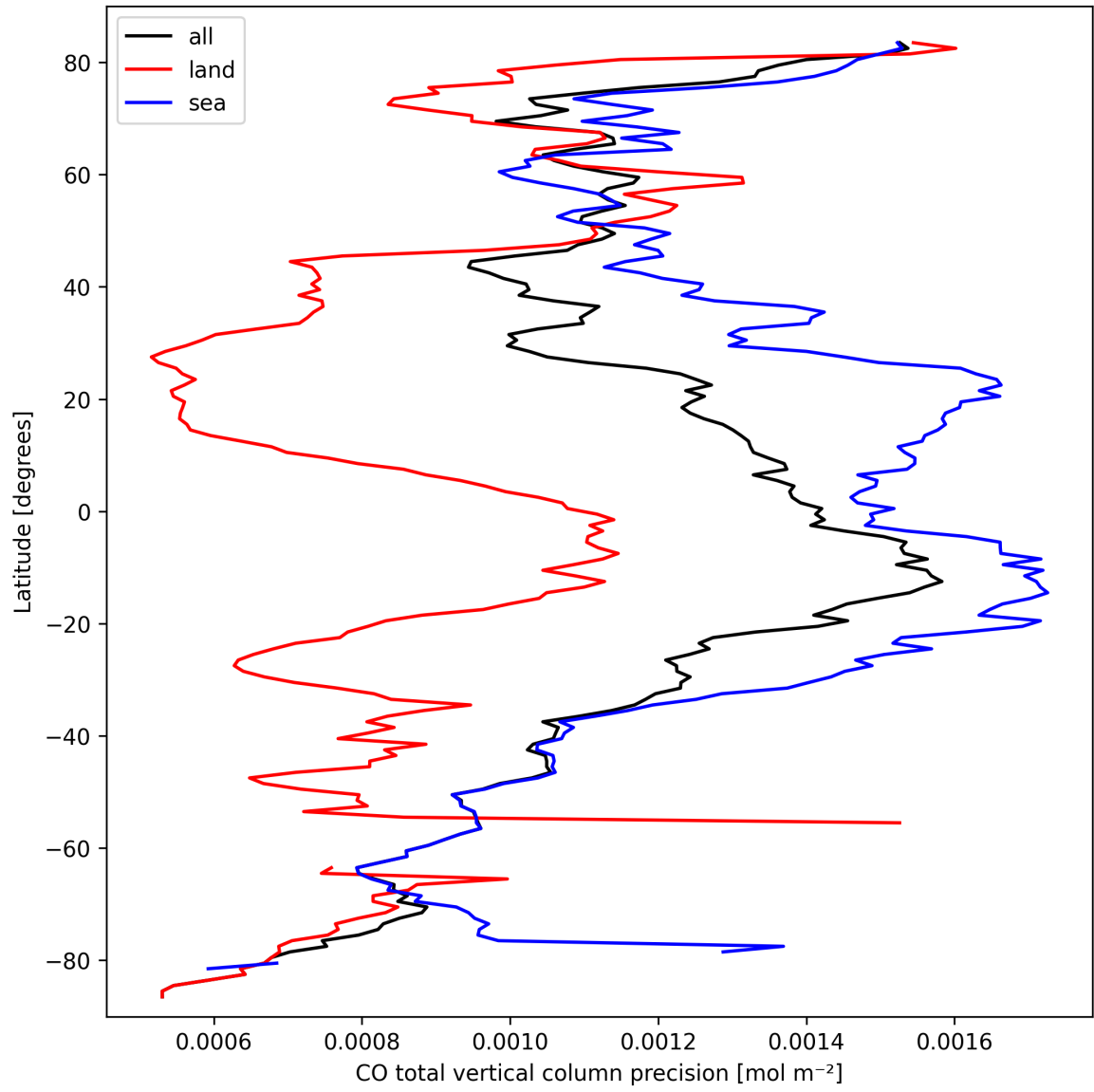
Figure 12: Zonal average of “CO total vertical column precision” for 2025-03-15 to 2025-03-17.
