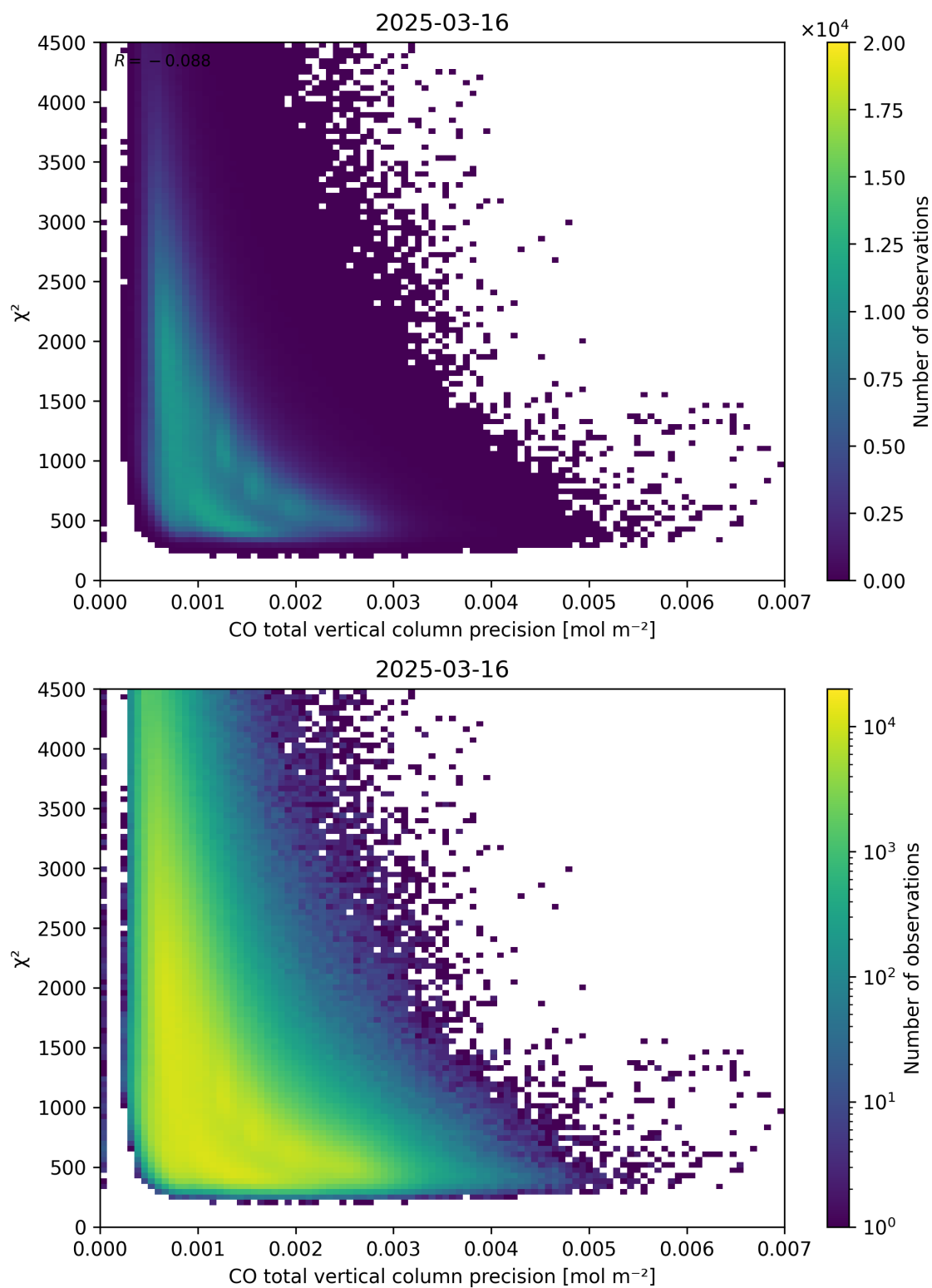
Figure 44: Scatter density plot of “CO total vertical column precision” against “ \chi^2 ” for 2025-03-15 to 2025-03-17.
