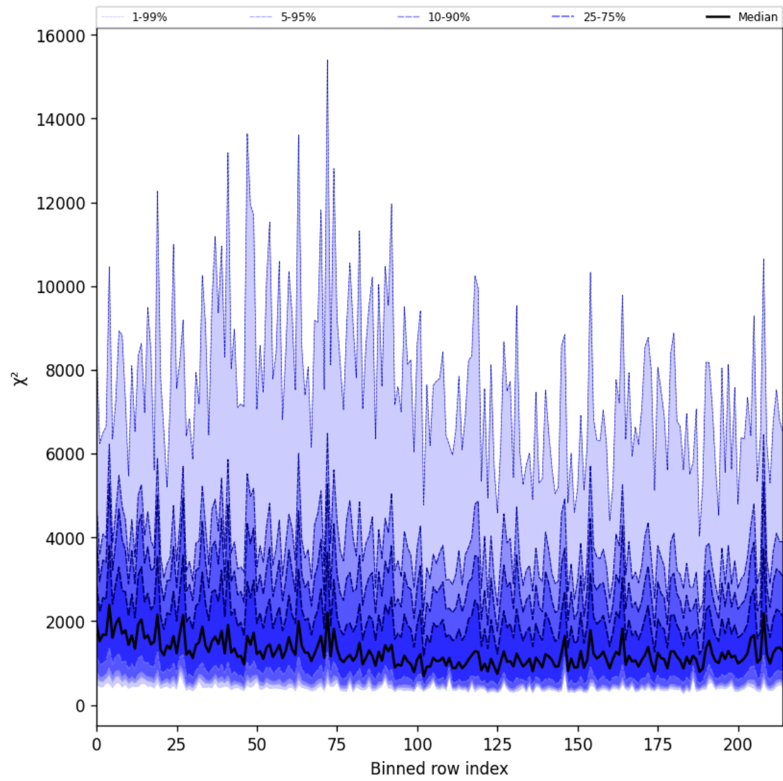
Figure 30: Along track statistics of “ \chi^2 ” for 2025-03-15 to 2025-03-17
