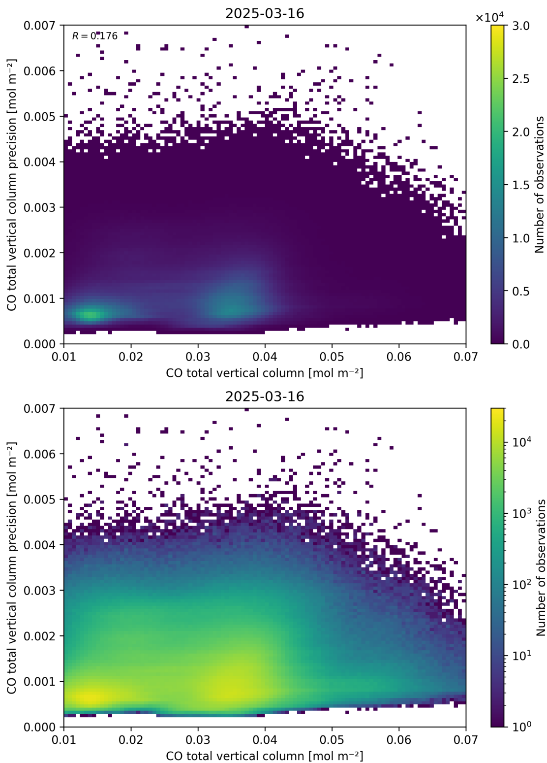
Figure 34: Scatter density plot of “CO total vertical column” against “CO total vertical column precision” for 2025-03-15 to 2025-03-17.
