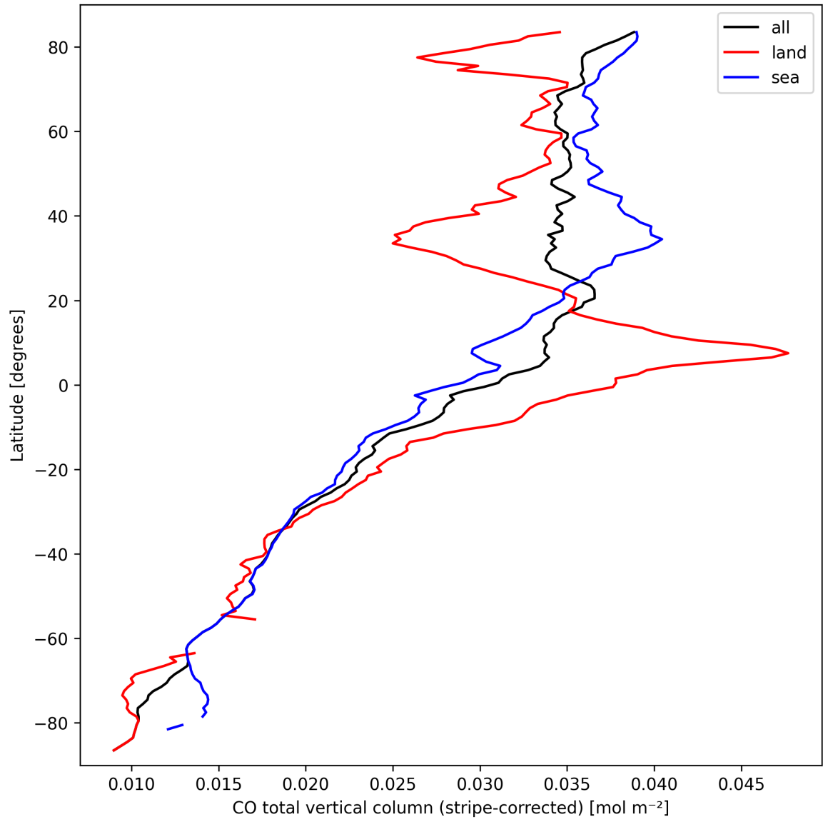
Figure 11: Zonal average of “CO total vertical column (stripe-corrected)” for 2025-03-15 to 2025-03-17.
