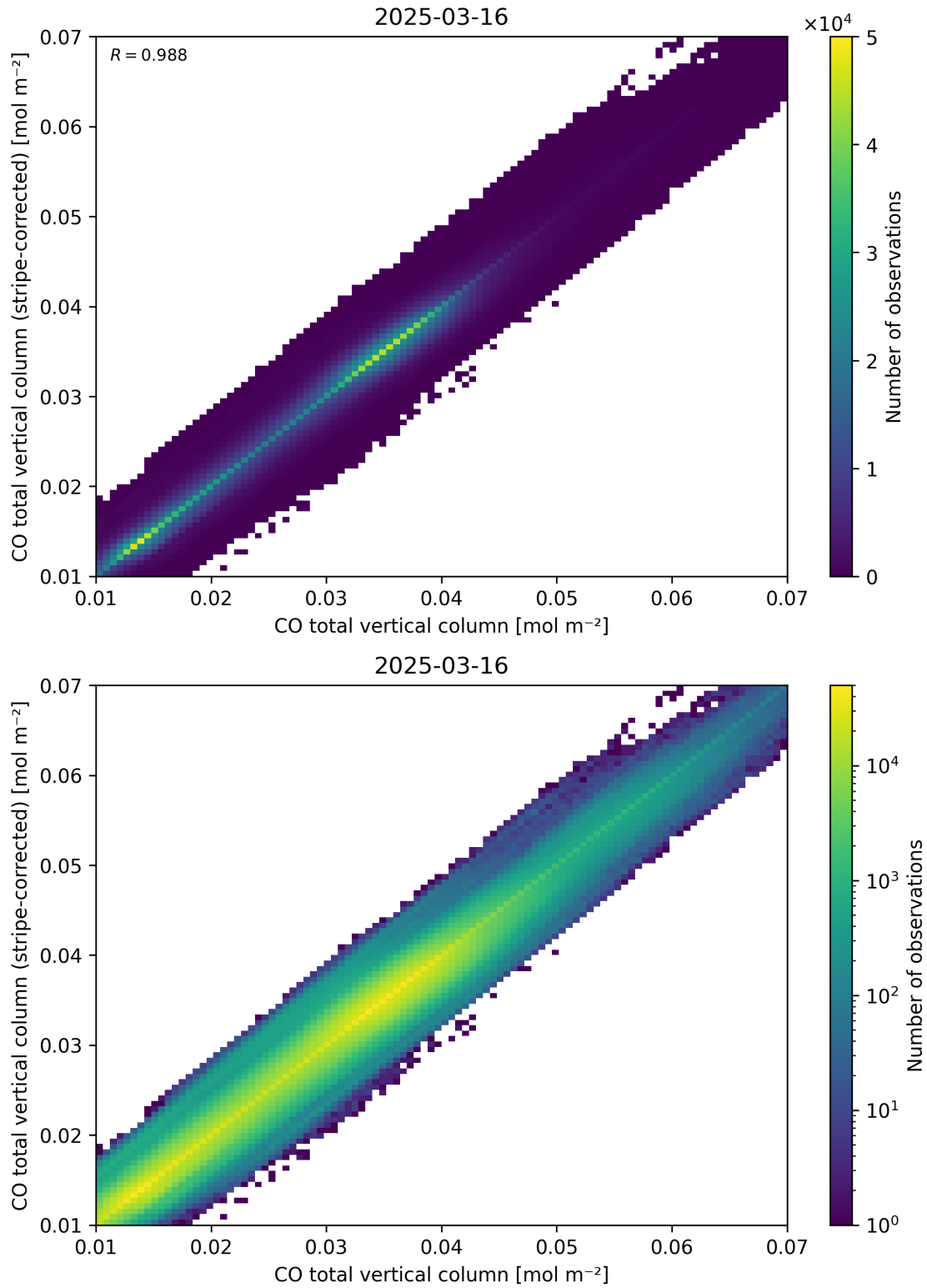
Figure 33: Scatter density plot of “CO total vertical column” against “CO total vertical column (stripe-corrected)” for 2025-03-15 to 2025-03-17.
