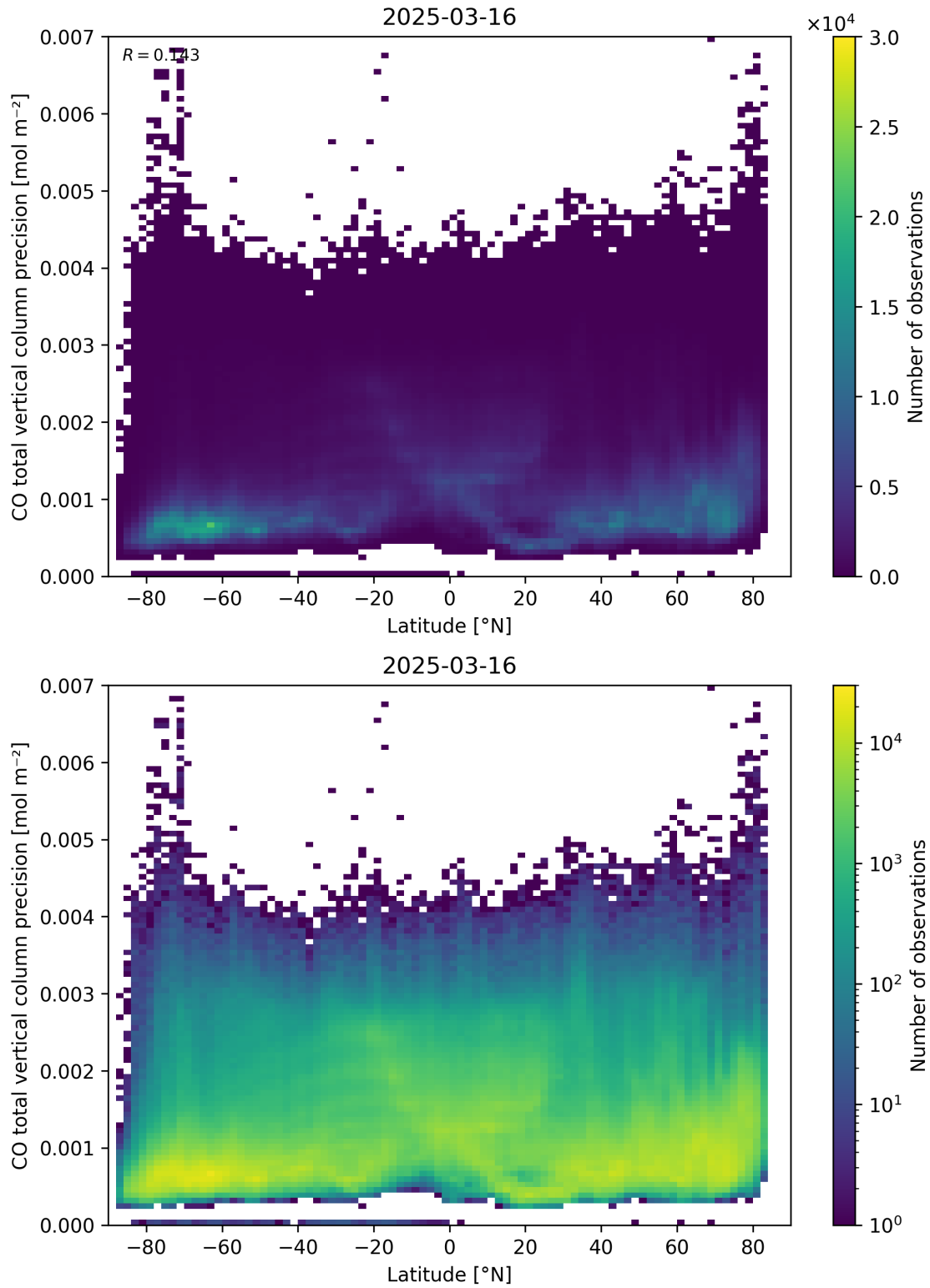
Figure 53: Scatter density plot of “Latitude” against “CO total vertical column precision” for 2025-03-15 to 2025-03-17.
