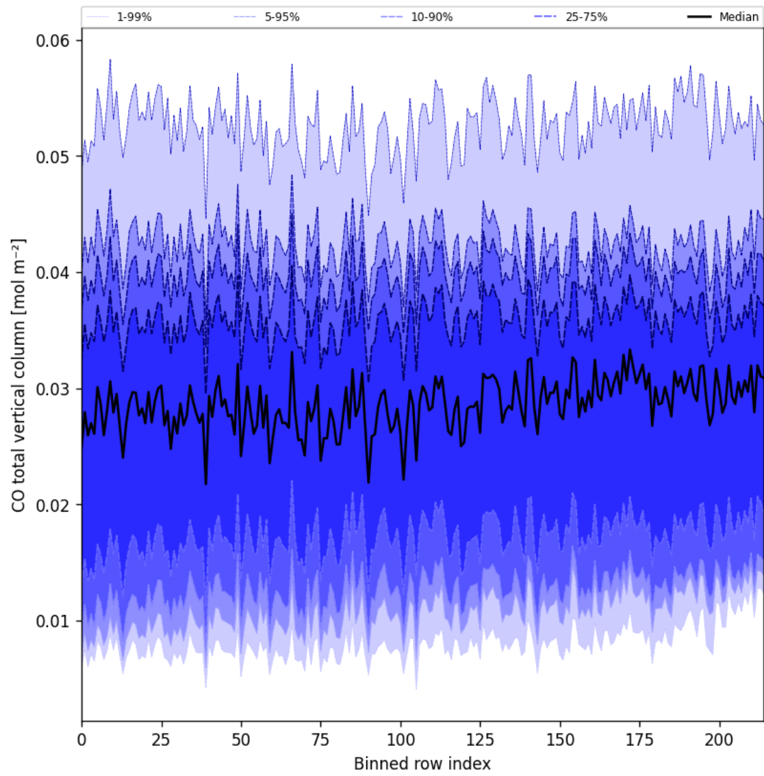
Figure 26: Along track statistics of “CO total vertical column” for 2025-03-15 to 2025-03-17
