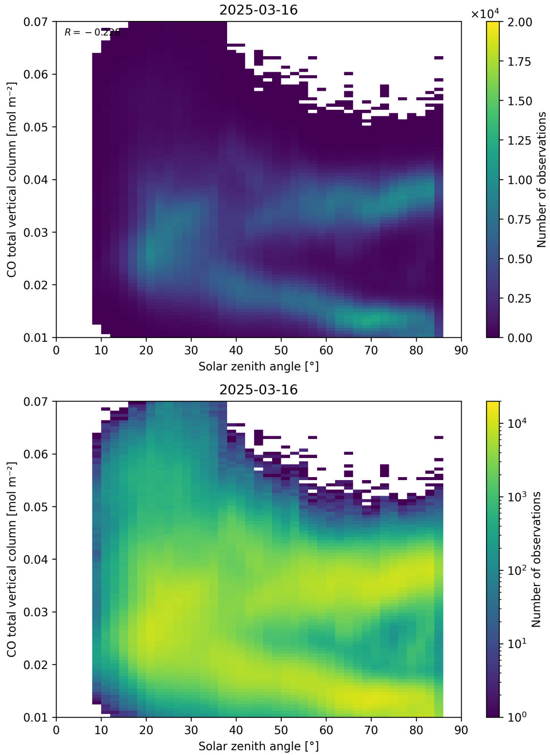
Figure 61: Scatter density plot of “Solar zenith angle” against “CO total vertical column” for 2025-03-15 to 2025-03-17.
