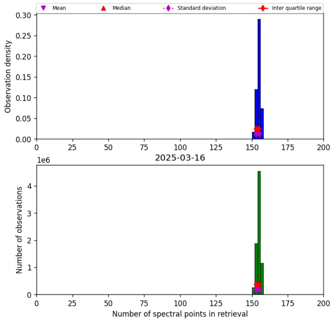
Figure 21: Histogram of “Number of spectral points in retrieval” for 2025-03-15 to 2025-03-17
