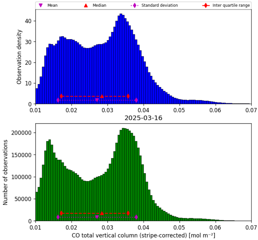
Figure 19: Histogram of “CO total vertical column (stripe-corrected)” for 2025-03-15 to 2025-03-17
