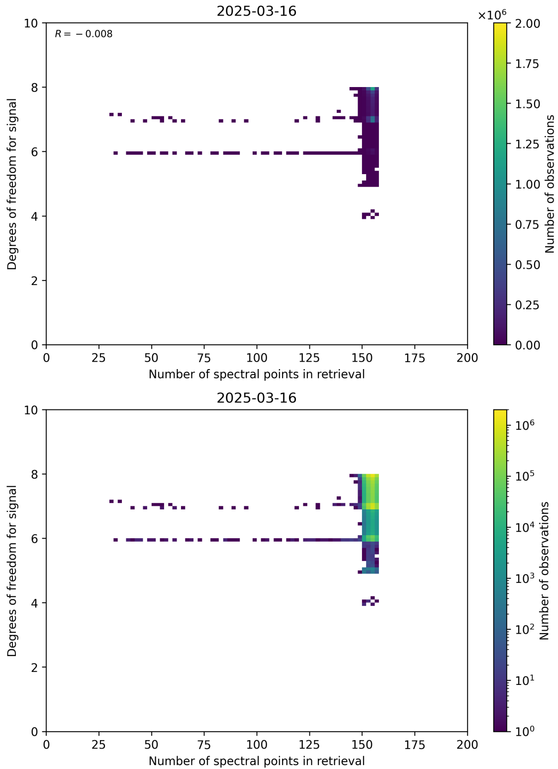
Figure 59: Scatter density plot of “Number of spectral points in retrieval” against “Degrees of freedom for signal” for 2025-03-15 to 2025-03-17.
