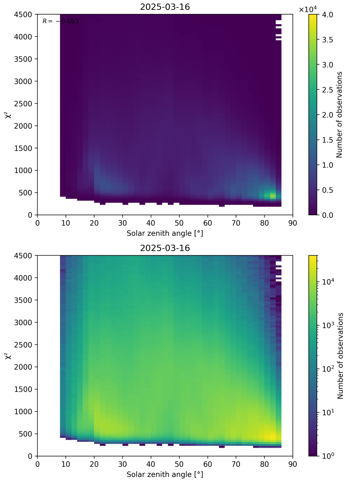
Figure 64: Scatter density plot of “Solar zenith angle” against “ \chi^2 ” for 2025-03-15 to 2025-03-17.
