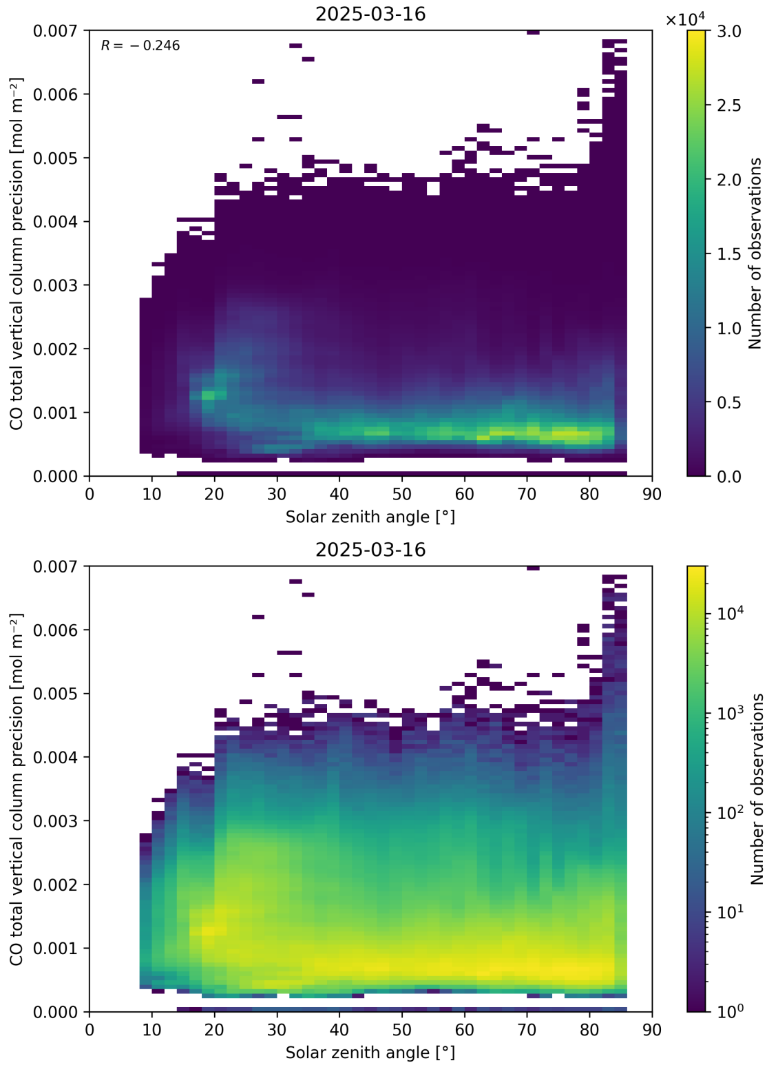
Figure 63: Scatter density plot of “Solar zenith angle” against “CO total vertical column precision” for 2025-03-15 to 2025-03-17.
