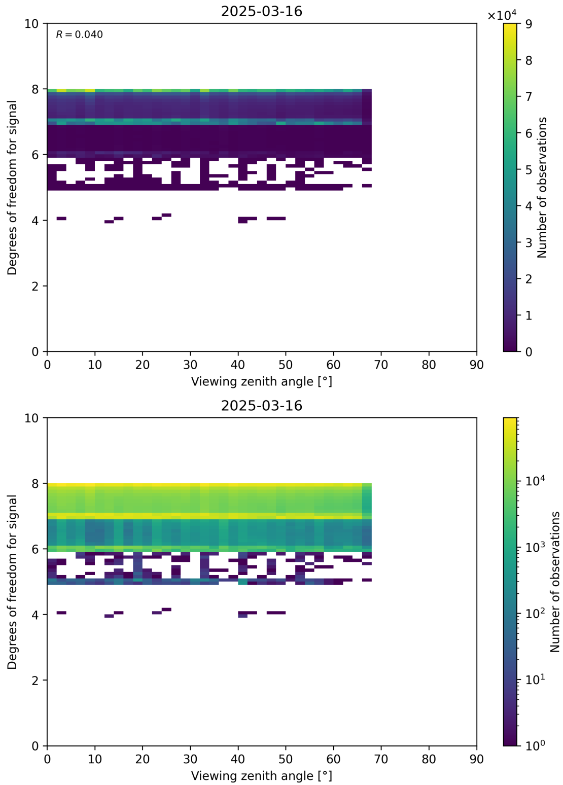
Figure 73: Scatter density plot of “Viewing zenith angle” against “Degrees of freedom for signal” for 2025-03-15 to 2025-03-17.
