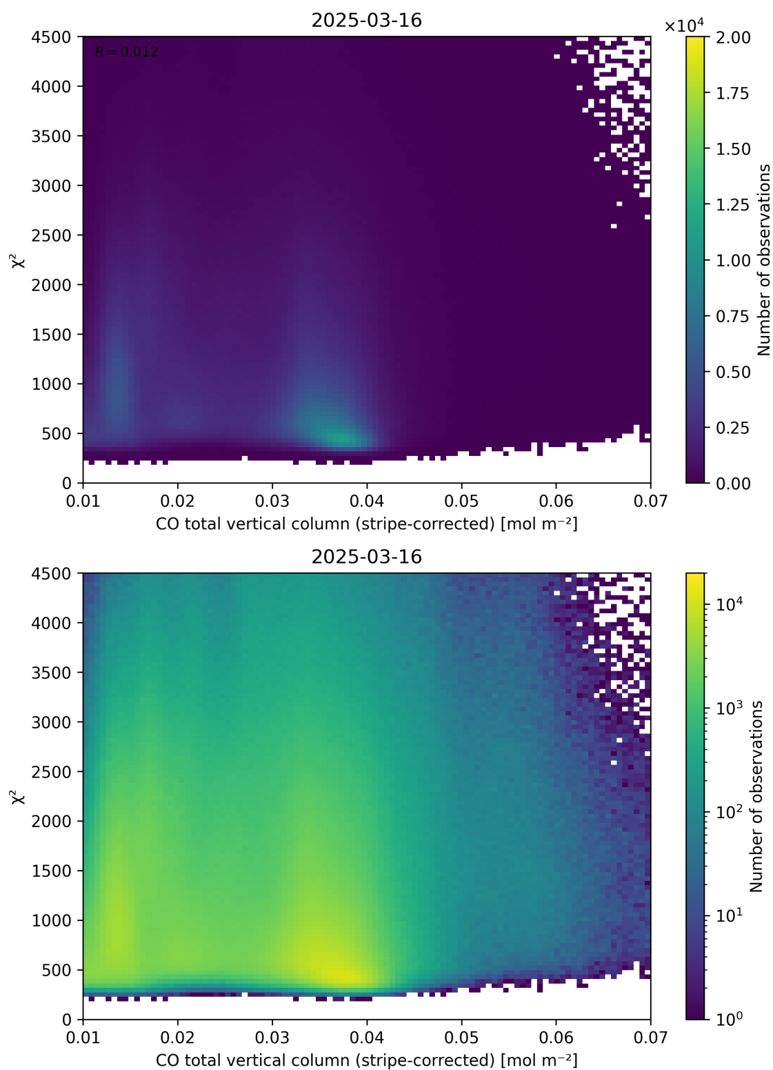
Figure 37: Scatter density plot of “CO total vertical column (stripe-corrected)” against “ \chi^2 ” for 2025-03-15 to 2025-03-17.
