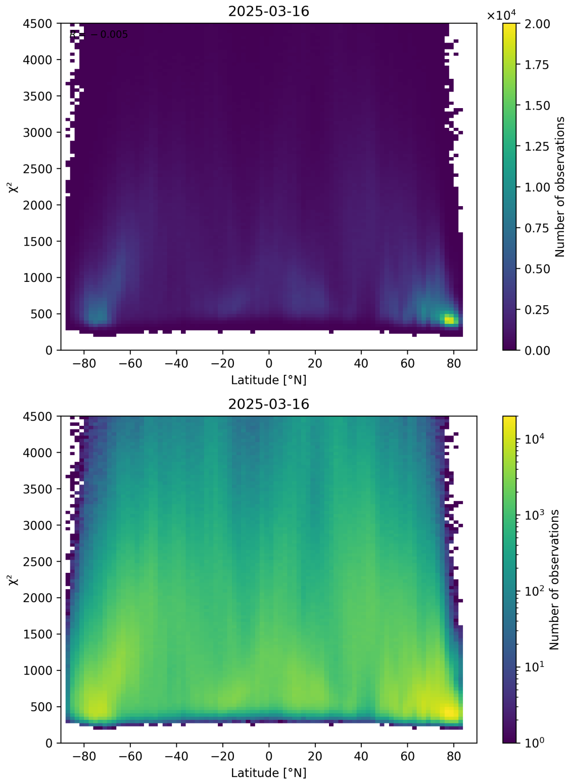
Figure 54: Scatter density plot of “Latitude” against “ \chi^2 ” for 2025-03-15 to 2025-03-17.
