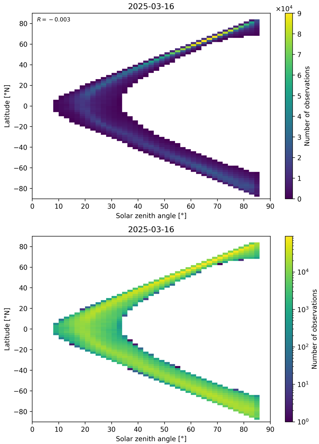
Figure 66: Scatter density plot of “Solar zenith angle” against “Latitude” for 2025-03-15 to 2025-03-17.
