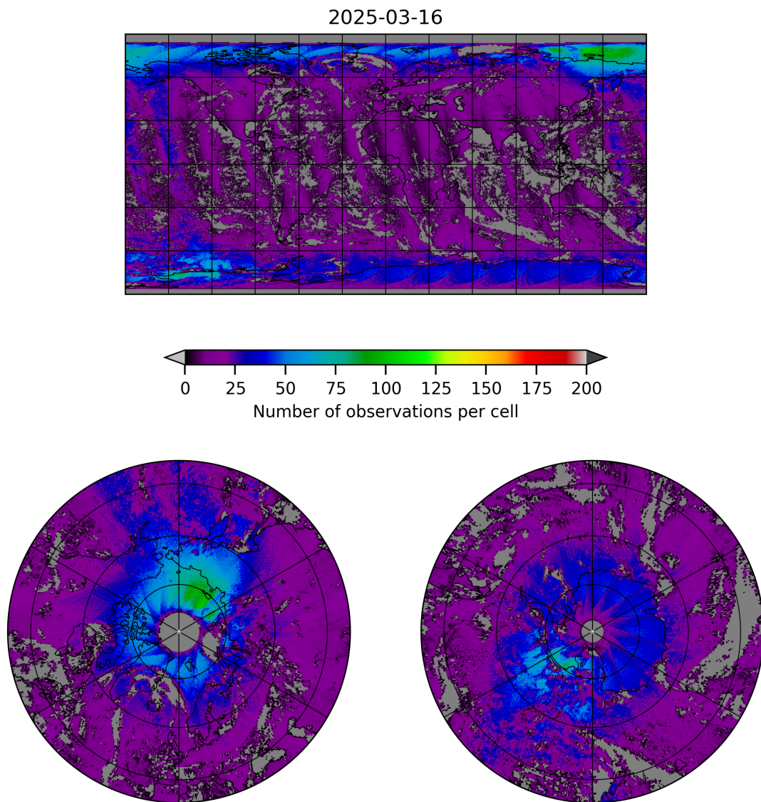
Figure 8: Map of the number of observations for 2025-03-15 to 2025-03-17
