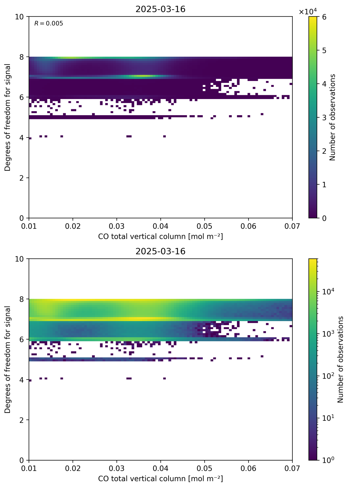
Figure 41: Scatter density plot of “CO total vertical column” against “Degrees of freedom for signal” for 2025-03-15 to 2025-03-17.
