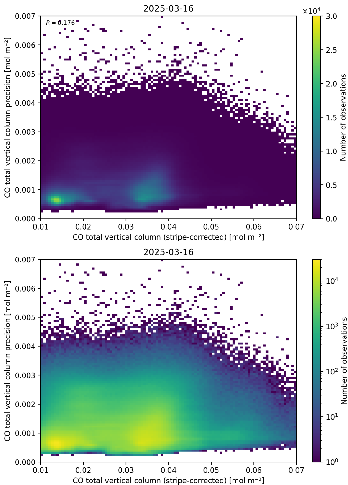
Figure 36: Scatter density plot of “CO total vertical column (stripe-corrected)” against “CO total vertical column precision” for 2025-03-15 to 2025-03-17.
