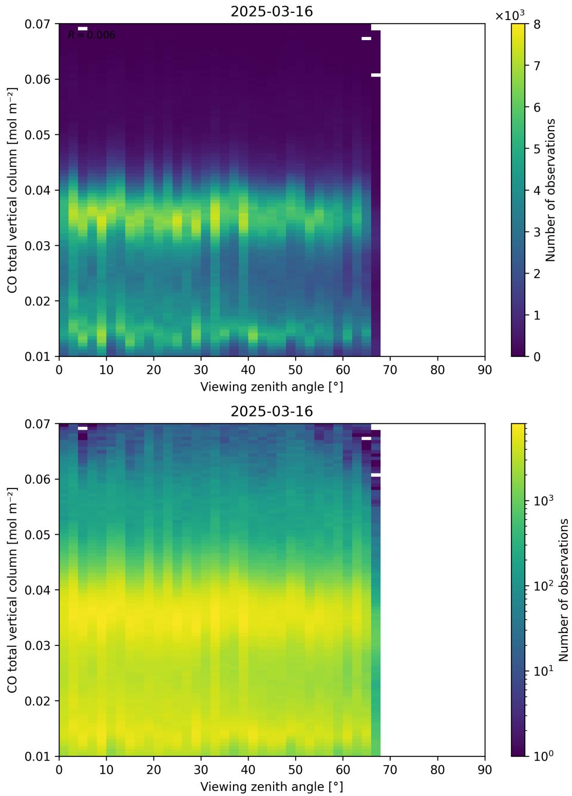
Figure 69: Scatter density plot of “Viewing zenith angle” against “CO total vertical column” for 2025-03-15 to 2025-03-17.
