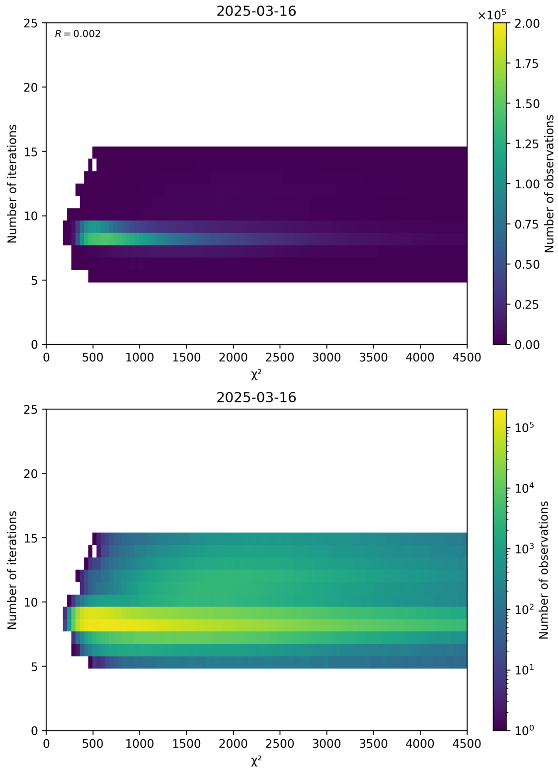
Figure 49: Scatter density plot of “ \chi^2 ” against “Number of iterations” for 2025-03-15 to 2025-03-17.
