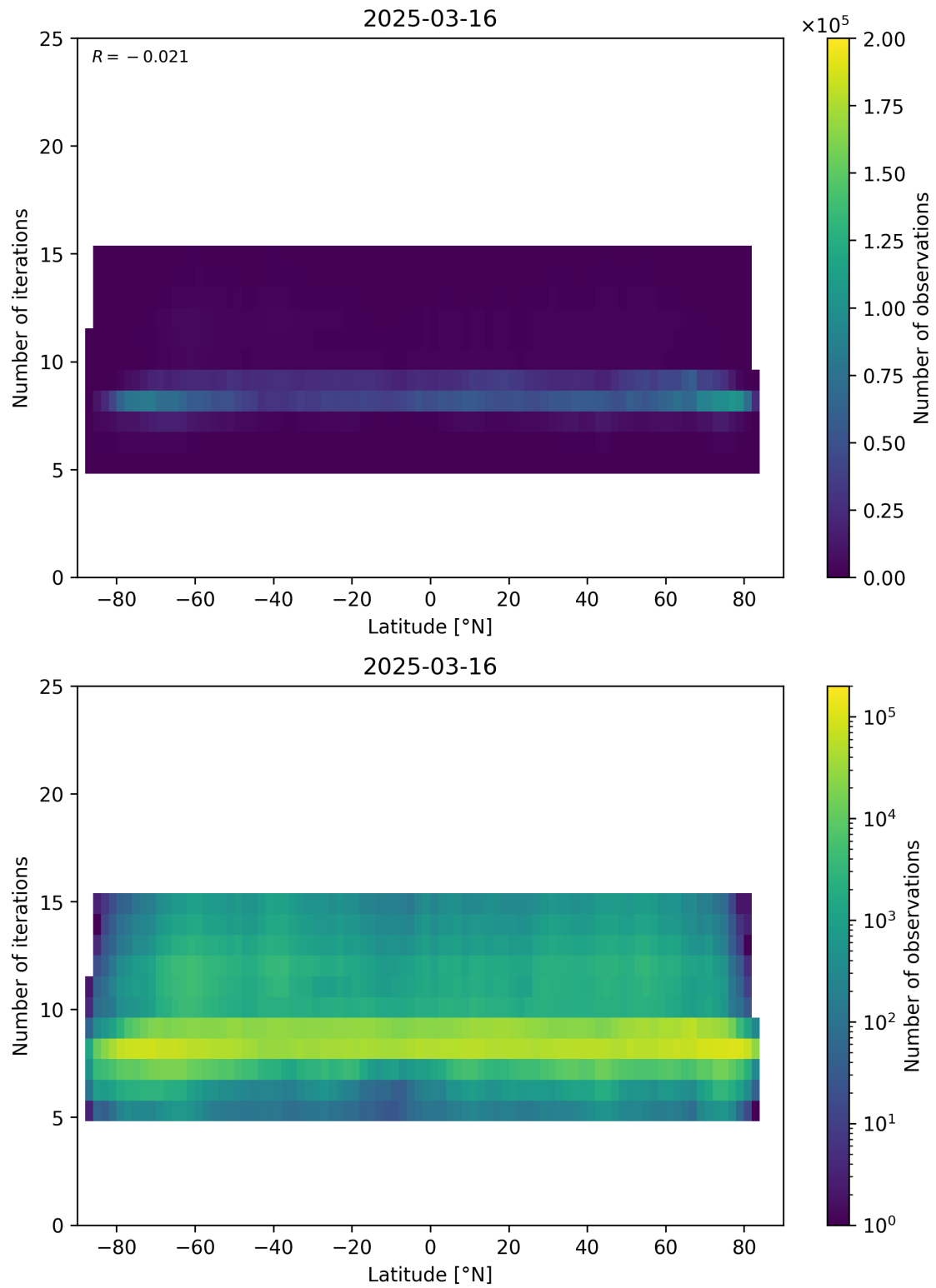
Figure 56: Scatter density plot of “Latitude” against “Number of iterations” for 2025-03-15 to 2025-03-17.
