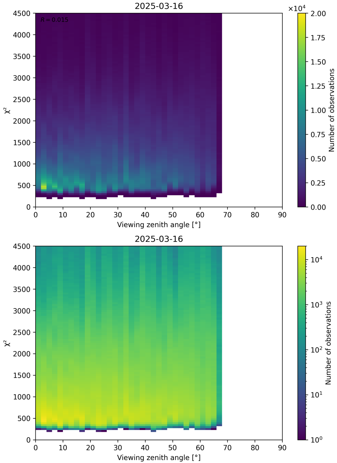
Figure 72: Scatter density plot of “Viewing zenith angle” against “ \chi^2 ” for 2025-03-15 to 2025-03-17.
