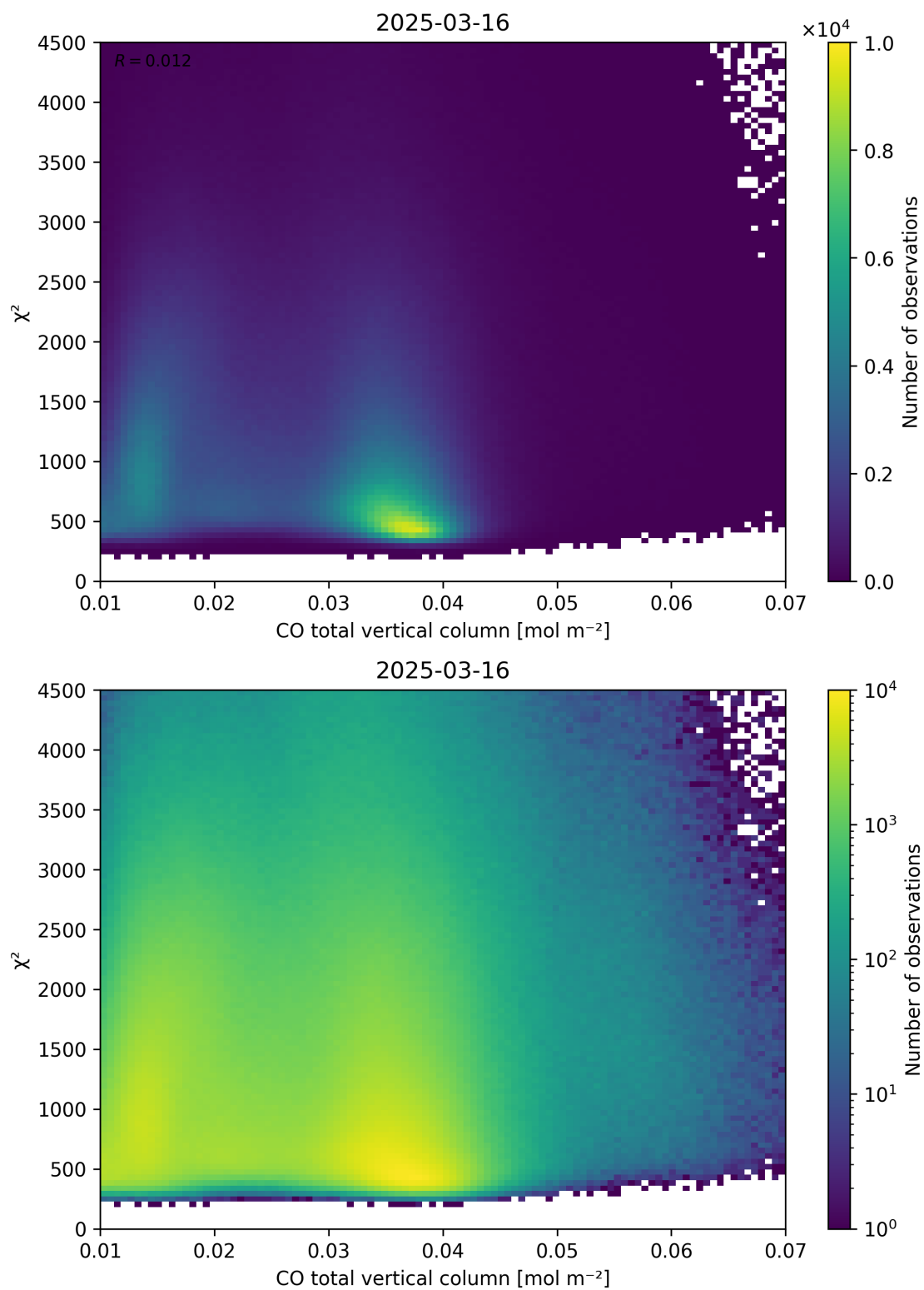
Figure 35: Scatter density plot of “CO total vertical column” against “ \chi^2 ” for 2025-03-15 to 2025-03-17.
