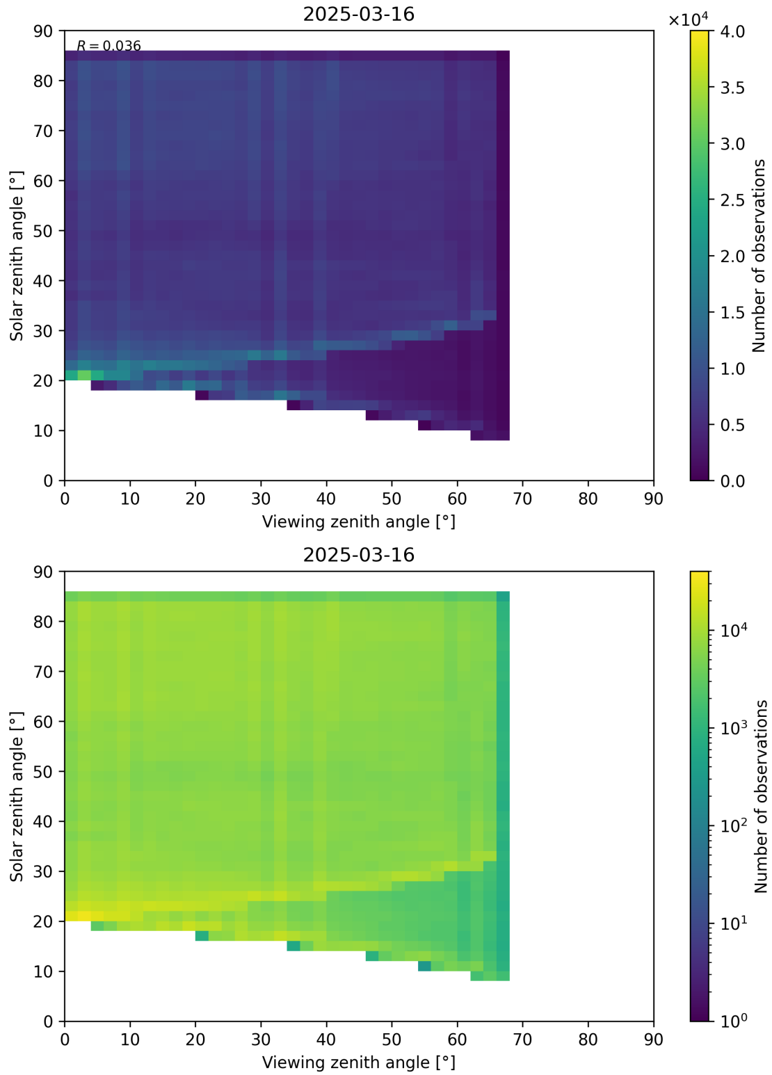
Figure 77: Scatter density plot of “Viewing zenith angle” against “Solar zenith angle” for 2025-03-15 to 2025-03-17.
