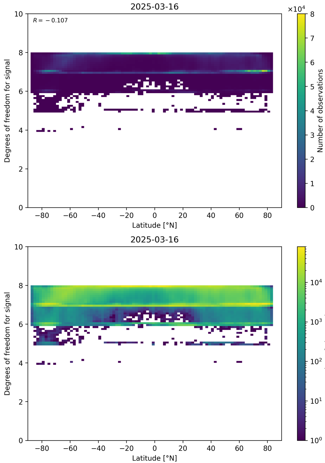
Figure 55: Scatter density plot of “Latitude” against “Degrees of freedom for signal” for 2025-03-15 to 2025-03-17.
