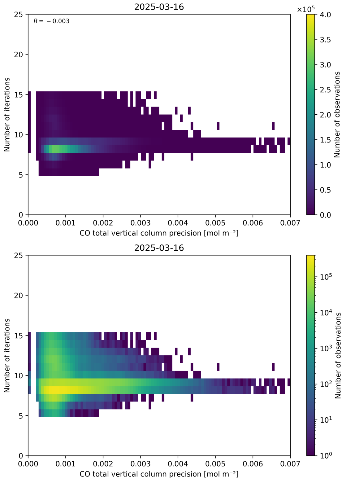
Figure 46: Scatter density plot of “CO total vertical column precision” against “Number of iterations” for 2025-03-15 to 2025-03-17.
