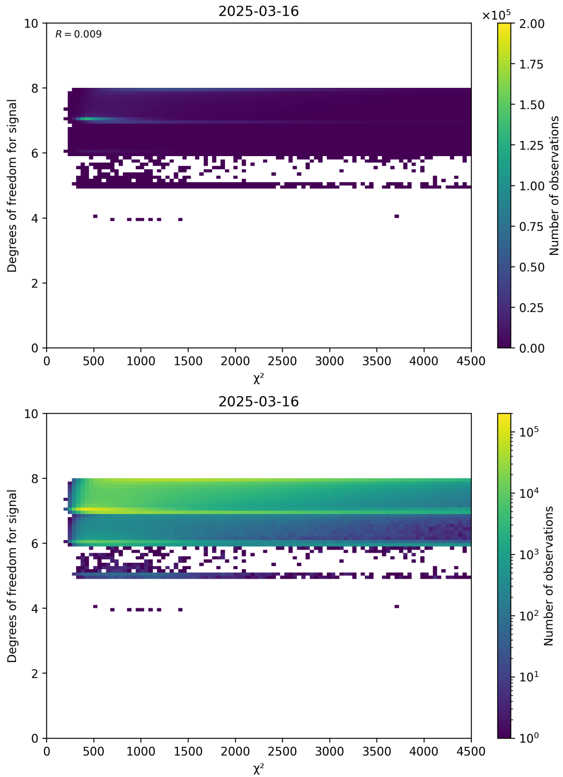
Figure 48: Scatter density plot of “ \chi^2 ” against “Degrees of freedom for signal” for 2025-03-15 to 2025-03-17.
