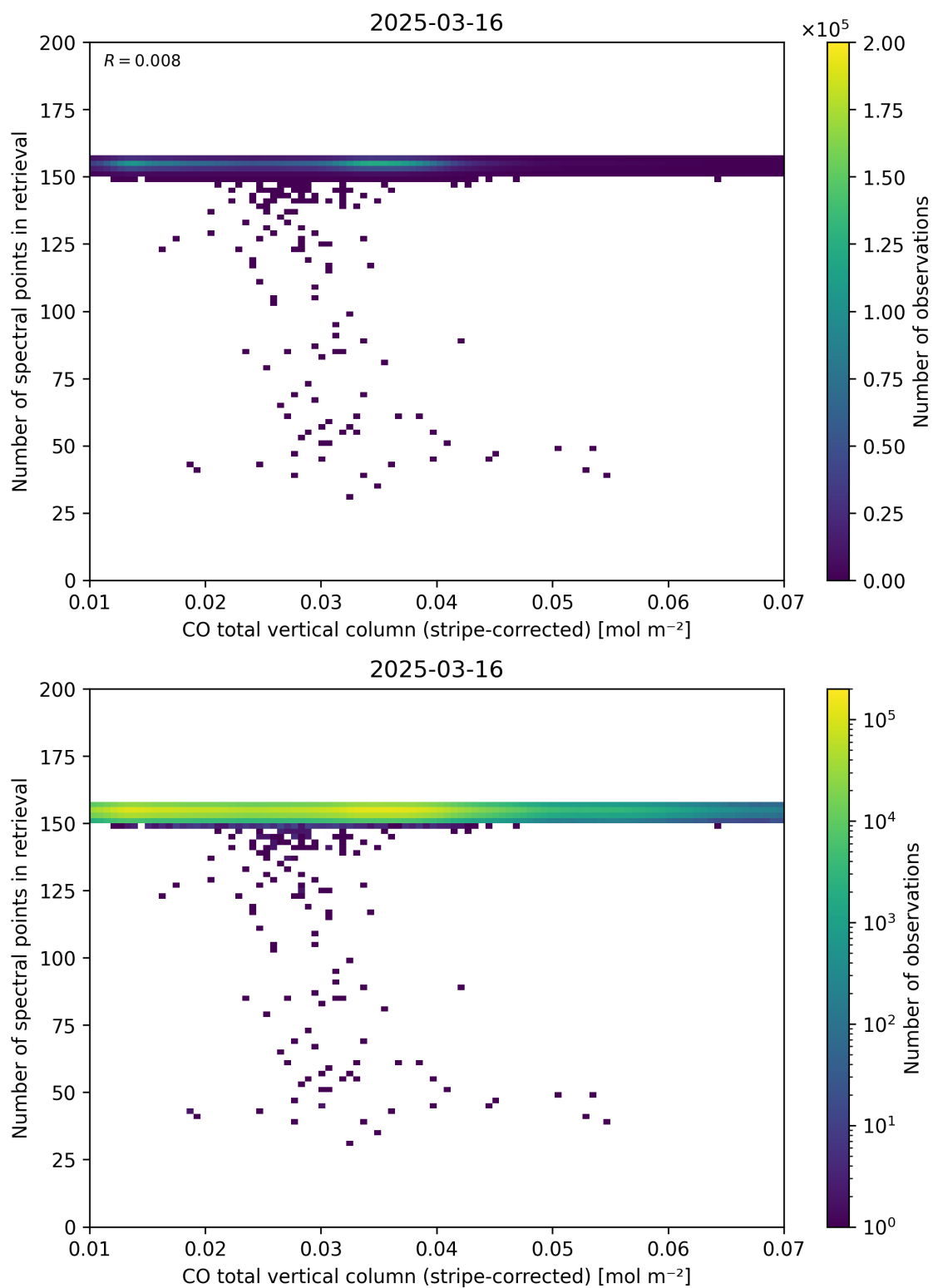
Figure 40: Scatter density plot of “CO total vertical column (stripe-corrected)” against “Number of spectral points in retrieval” for 2025-03-15 to 2025-03-17.
