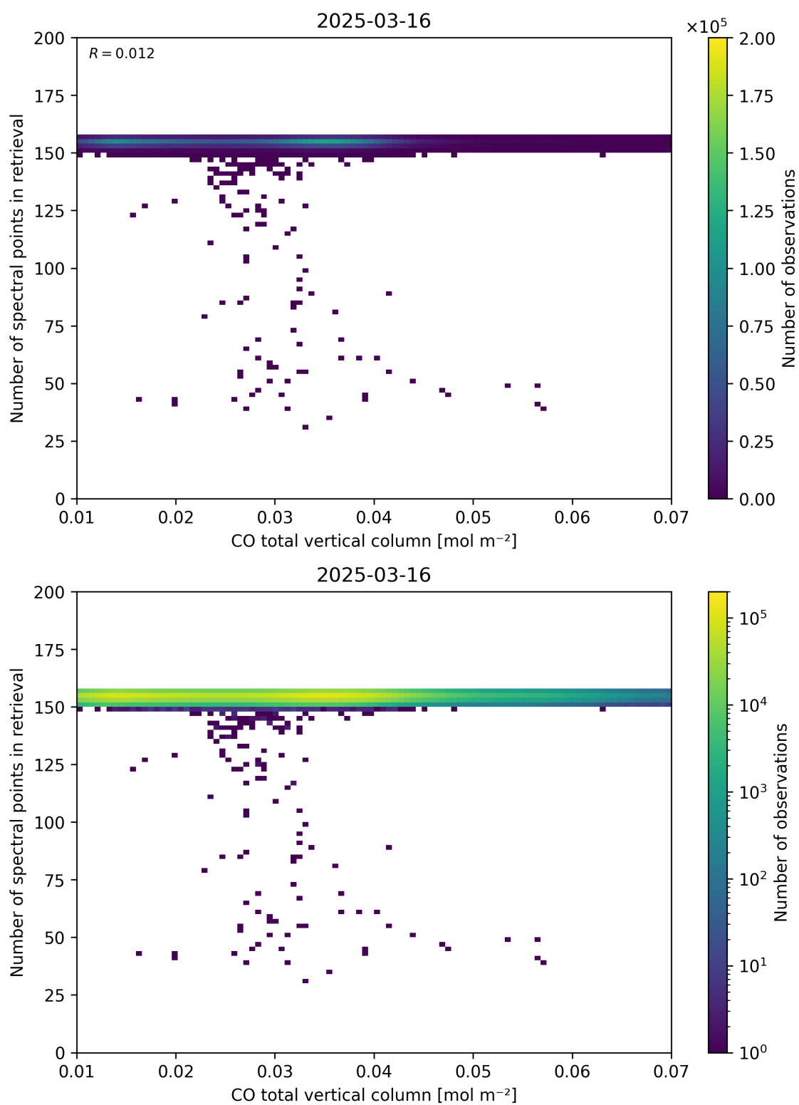
Figure 43: Scatter density plot of “CO total vertical column” against “Number of spectral points in retrieval” for 2025-03-15 to 2025-03-17.
