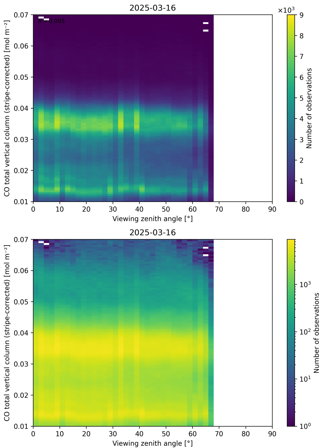
Figure 70: Scatter density plot of “Viewing zenith angle” against “CO total vertical column (stripe-corrected)” for 2025-03-15 to 2025-03-17.
