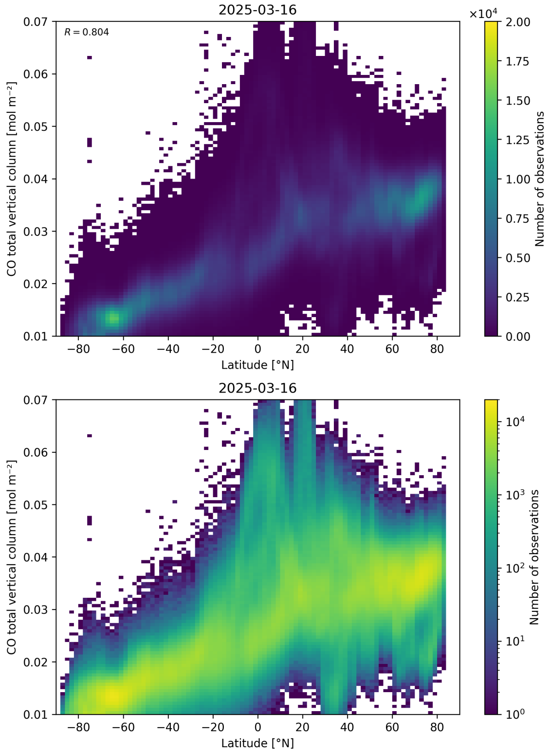
Figure 51: Scatter density plot of “Latitude” against “CO total vertical column” for 2025-03-15 to 2025-03-17.
