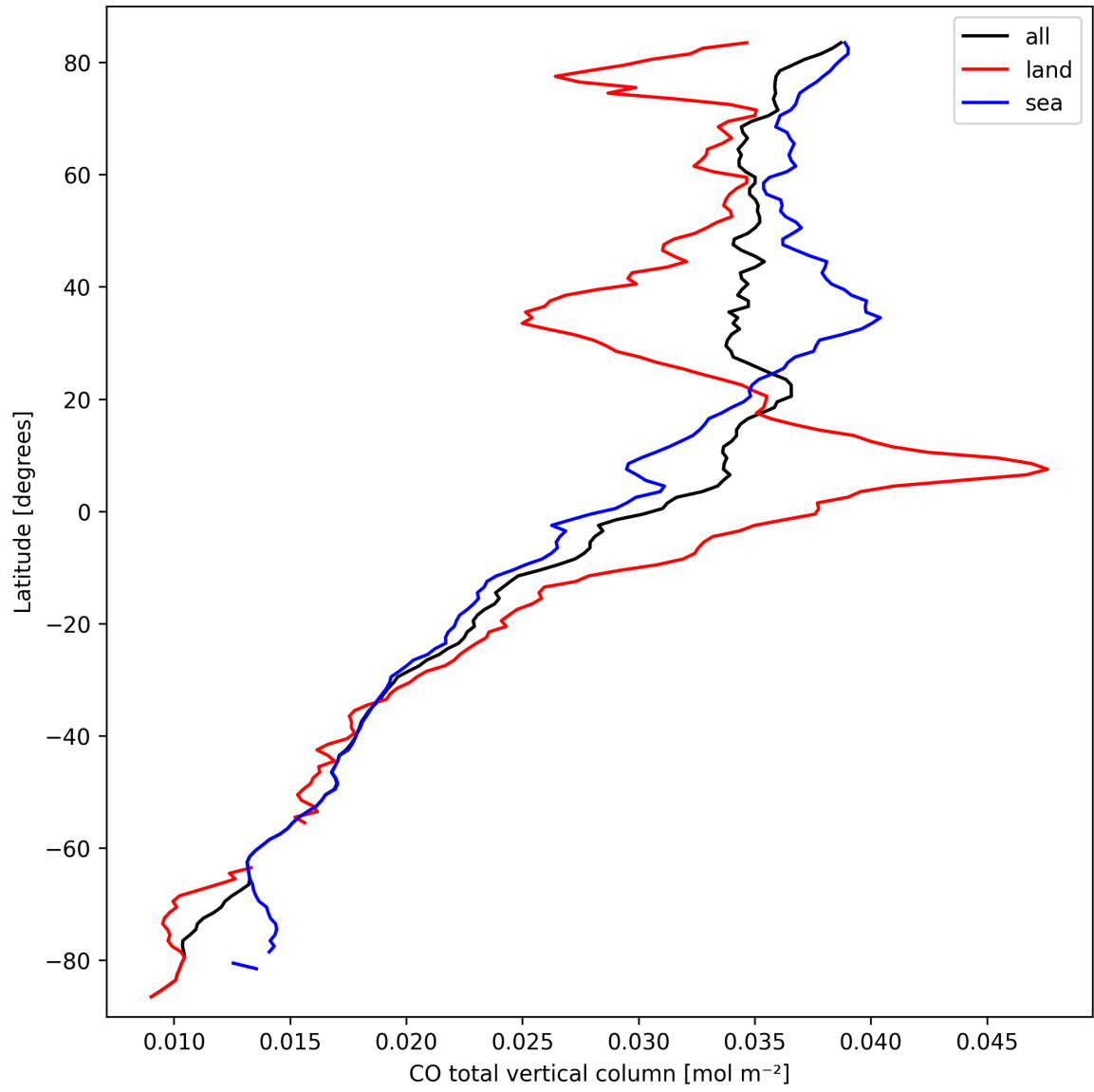
Figure 10: Zonal average of “CO total vertical column” for 2025-03-15 to 2025-03-17.
