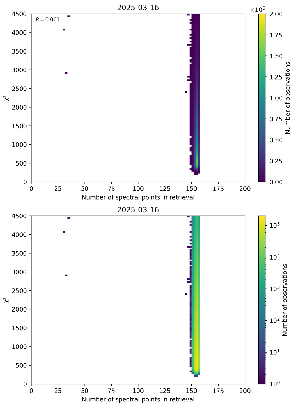
Figure 58: Scatter density plot of “Number of spectral points in retrieval” against “ \chi^2 ” for 2025-03-15 to 2025-03-17.
