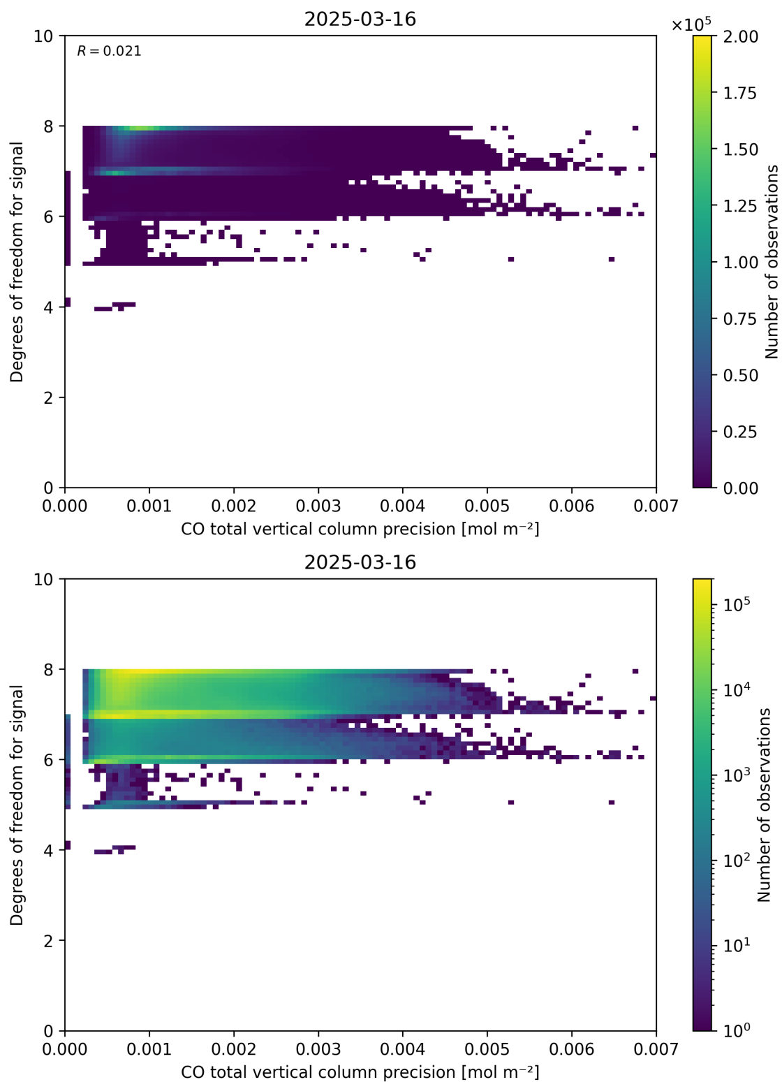
Figure 45: Scatter density plot of “CO total vertical column precision” against “Degrees of freedom for signal” for 2025-03-15 to 2025-03-17.
