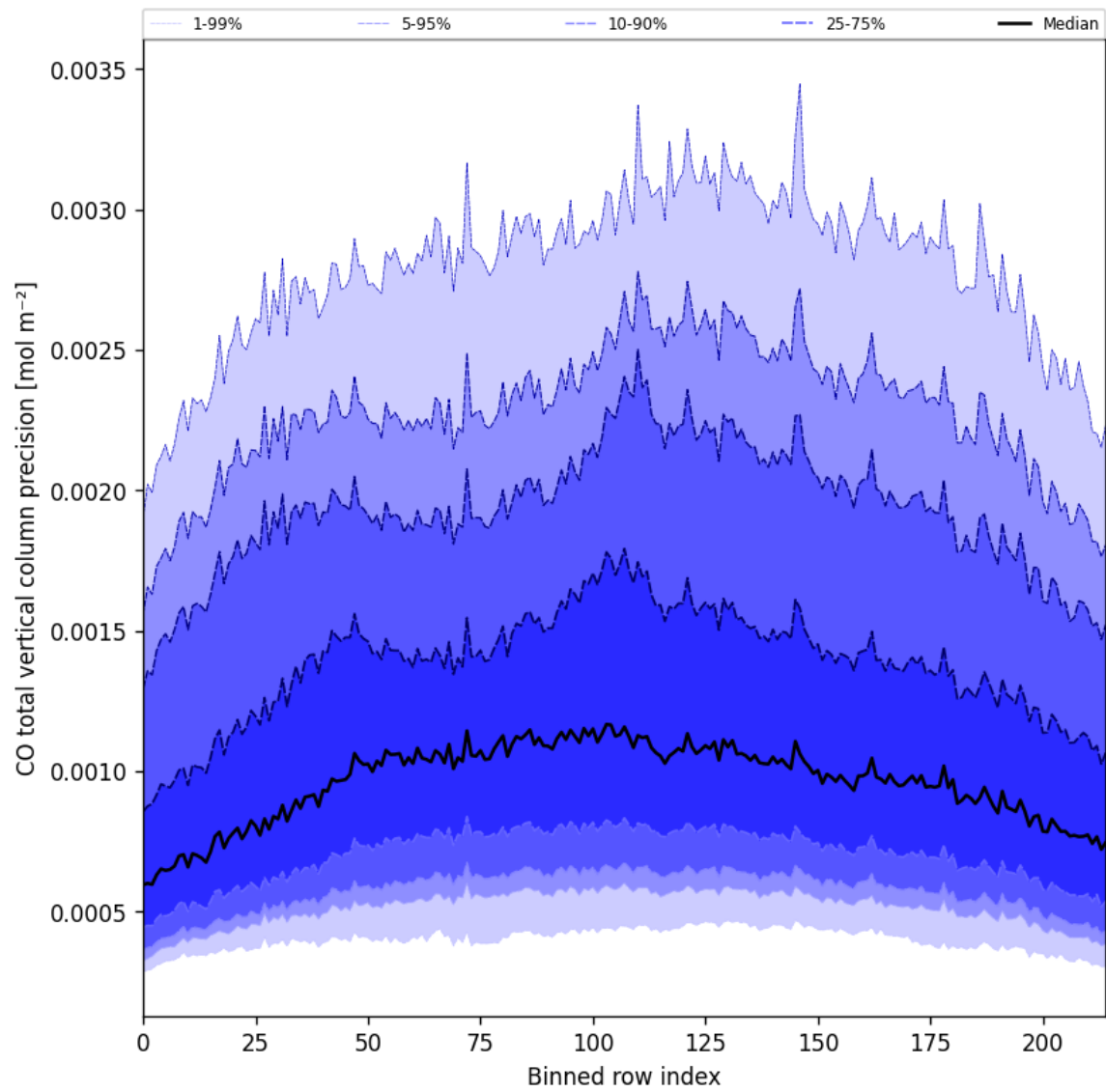
Figure 28: Along track statistics of “CO total vertical column precision” for 2025-03-15 to 2025-03-17
