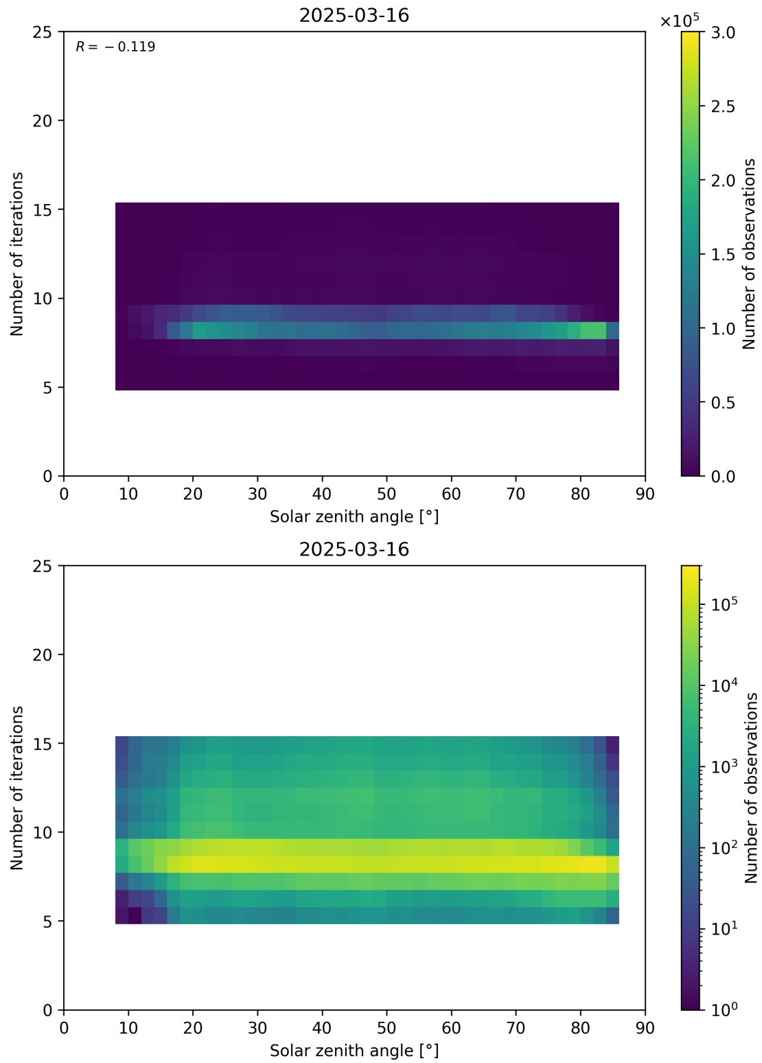
Figure 67: Scatter density plot of “Solar zenith angle” against “Number of iterations” for 2025-03-15 to 2025-03-17.
