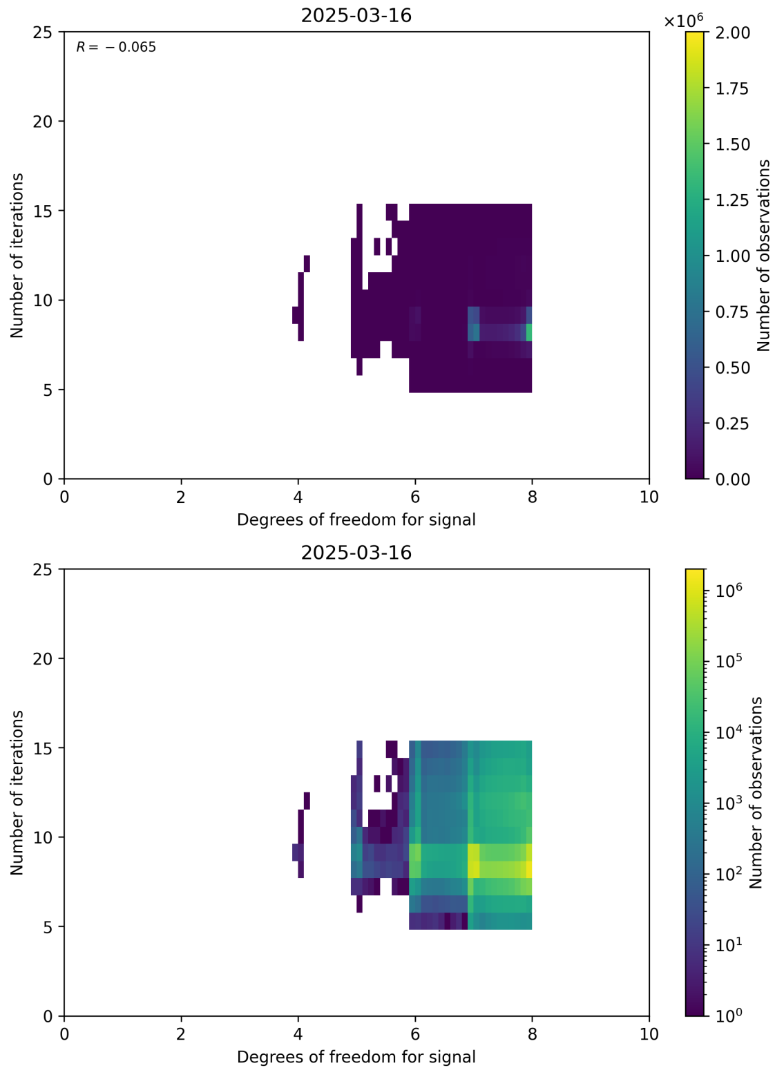
Figure 50: Scatter density plot of “Degrees of freedom for signal” against “Number of iterations” for 2025-03-15 to 2025-03-17.
