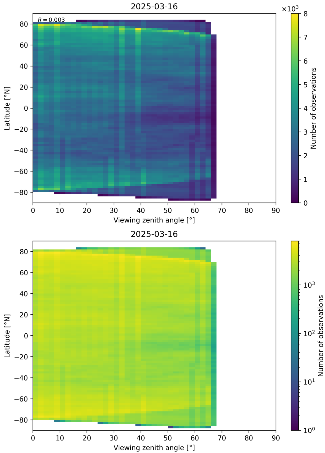
Figure 74: Scatter density plot of “Viewing zenith angle” against “Latitude” for 2025-03-15 to 2025-03-17.
