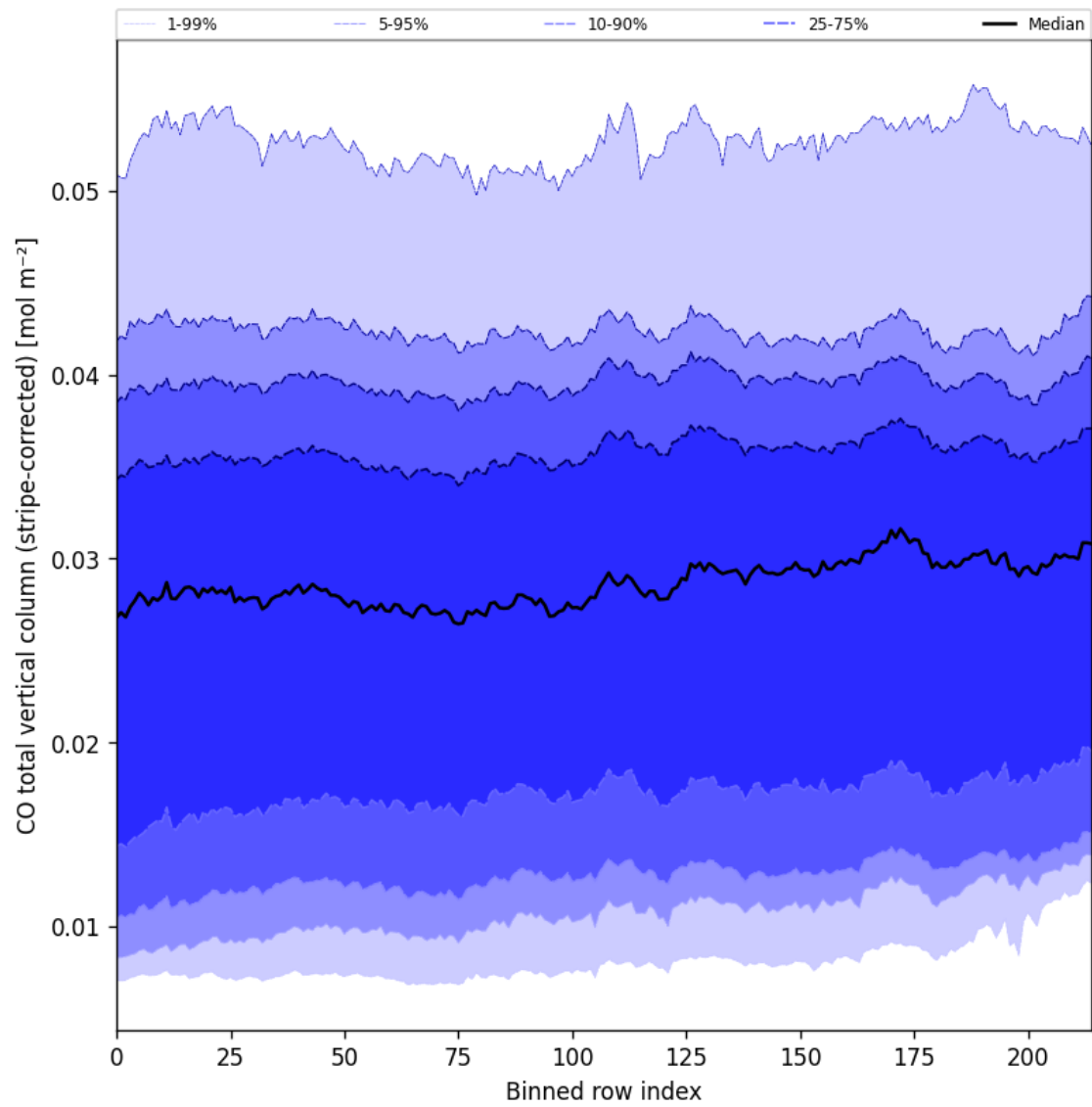
Figure 27: Along track statistics of “CO total vertical column (stripe-corrected)” for 2025-03-15 to 2025-03-17
