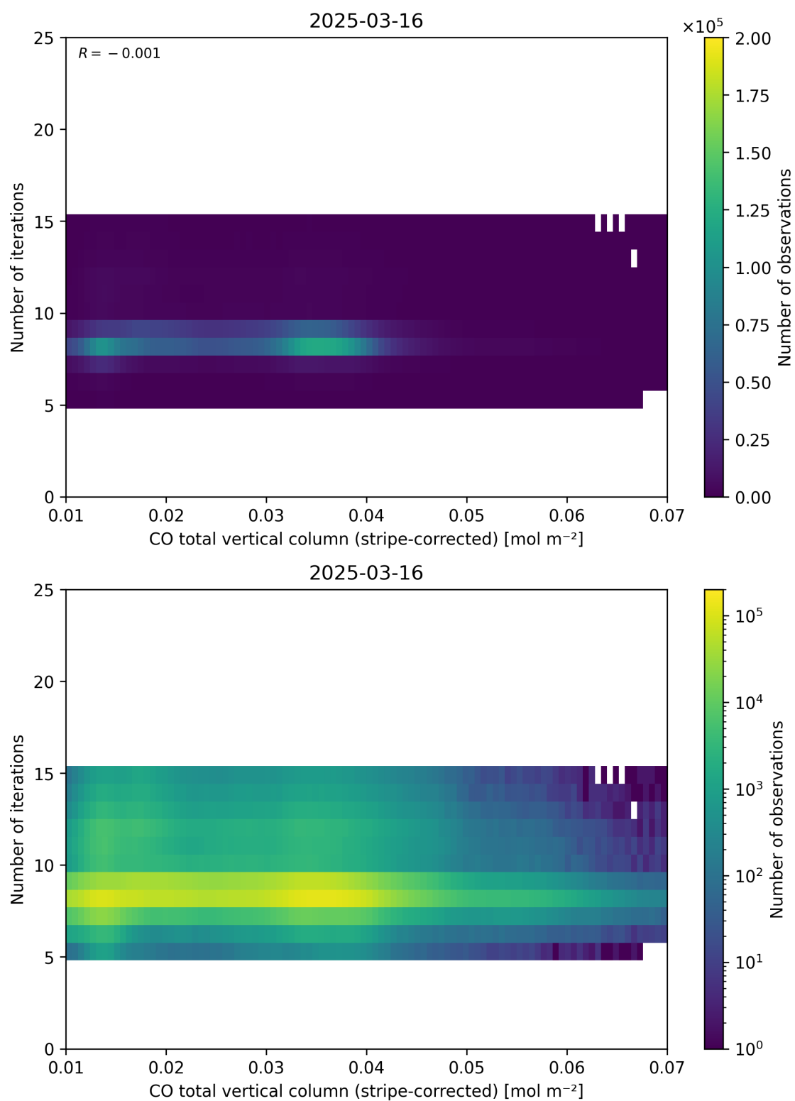
Figure 39: Scatter density plot of “CO total vertical column (stripe-corrected)” against “Number of iterations” for 2025-03-15 to 2025-03-17.
