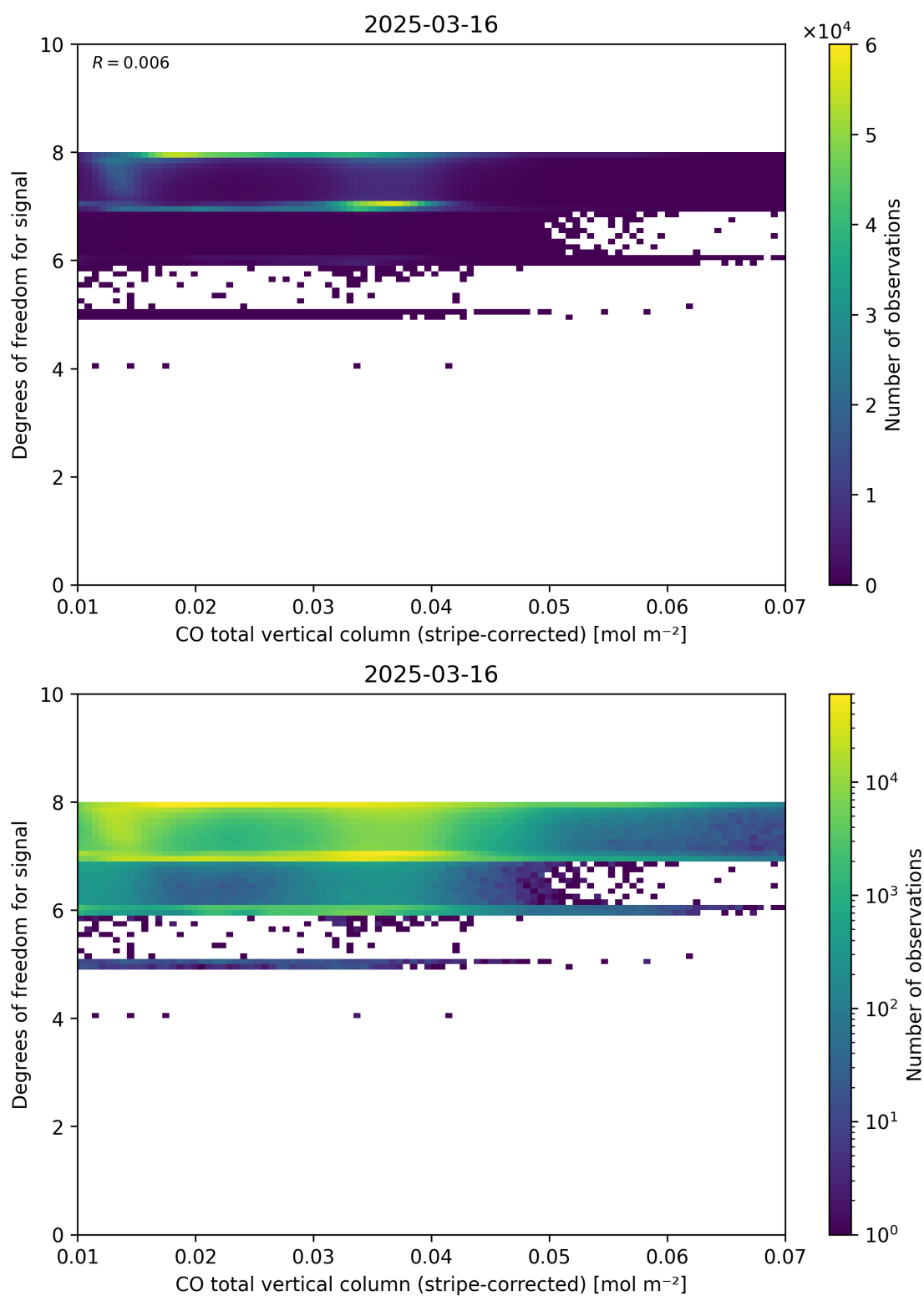
Figure 38: Scatter density plot of “CO total vertical column (stripe-corrected)” against “Degrees of freedom for signal” for 2025-03-15 to 2025-03-17.
