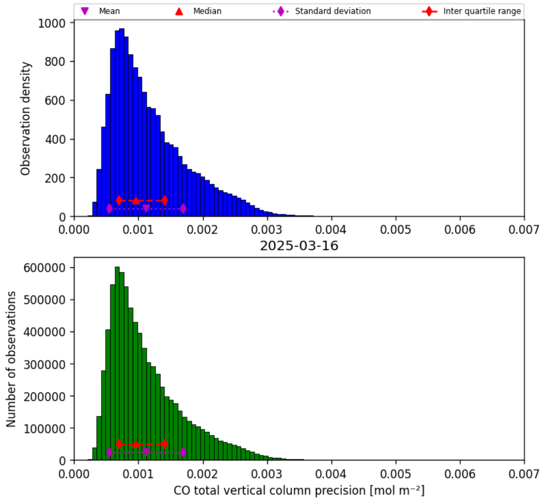
Figure 20: Histogram of “CO total vertical column precision” for 2025-03-15 to 2025-03-17
