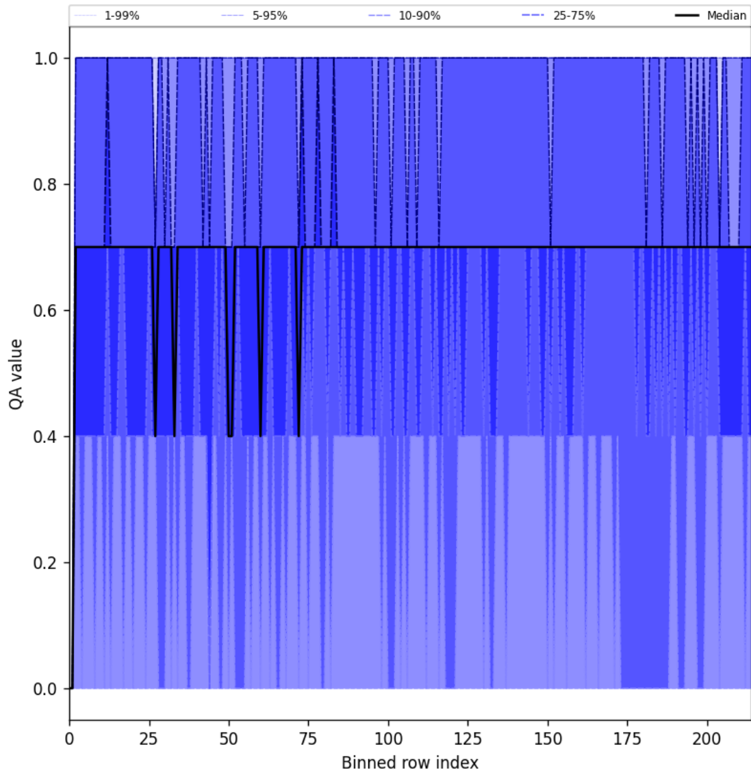
Figure 25: Along track statistics of “QA value” for 2025-03-15 to 2025-03-17
