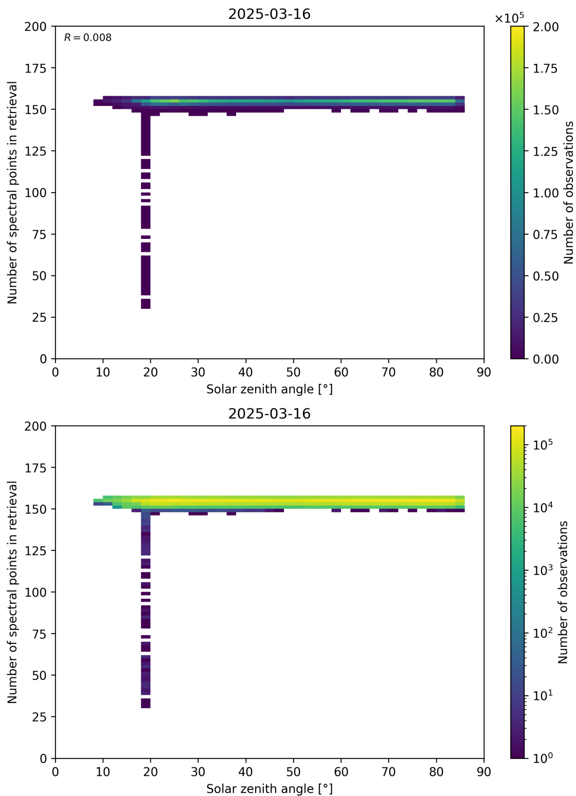
Figure 68: Scatter density plot of “Solar zenith angle” against “Number of spectral points in retrieval” for 2025-03-15 to 2025-03-17.
