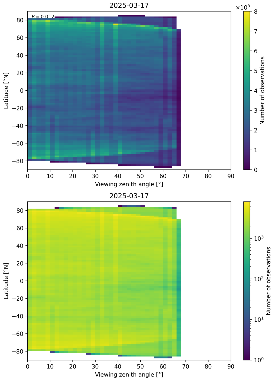
Figure 74: Scatter density plot of “Viewing zenith angle” against “Latitude” for 2025-03-17 to 2025-03-18.
