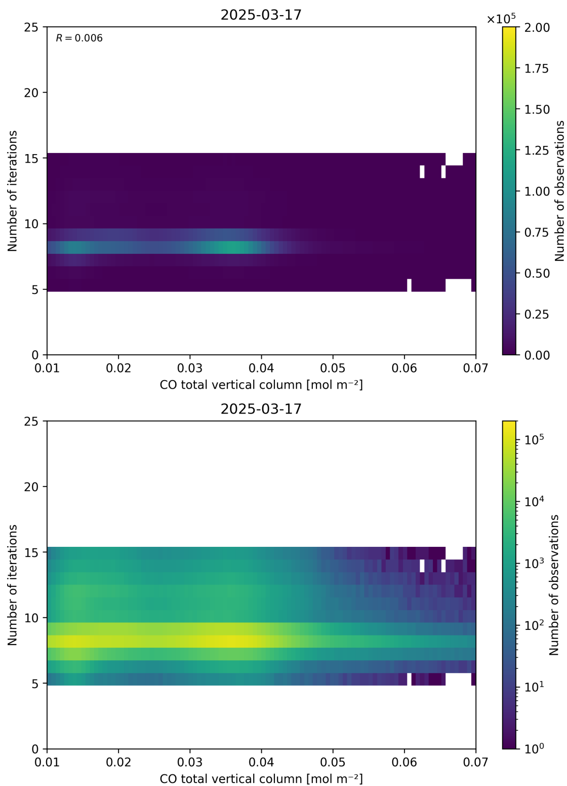
Figure 42: Scatter density plot of “CO total vertical column” against “Number of iterations” for 2025-03-17 to 2025-03-18.
