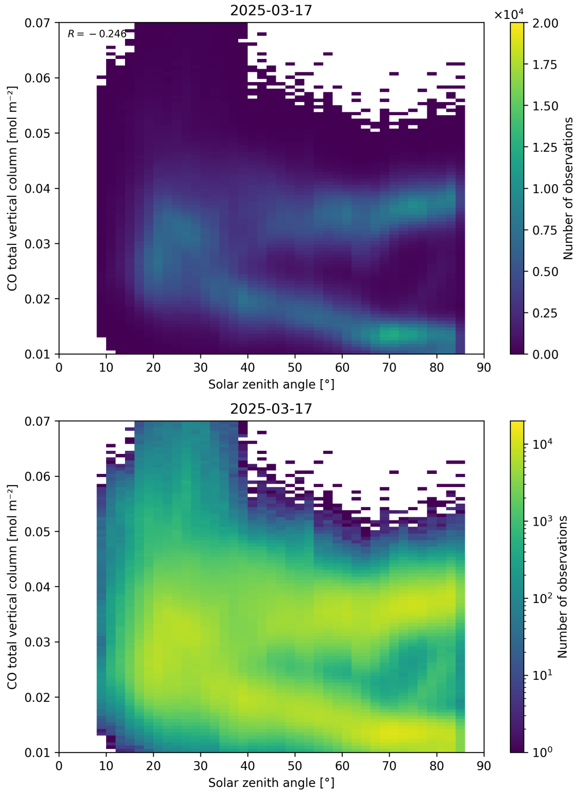
Figure 61: Scatter density plot of “Solar zenith angle” against “CO total vertical column” for 2025-03-17 to 2025-03-18.
