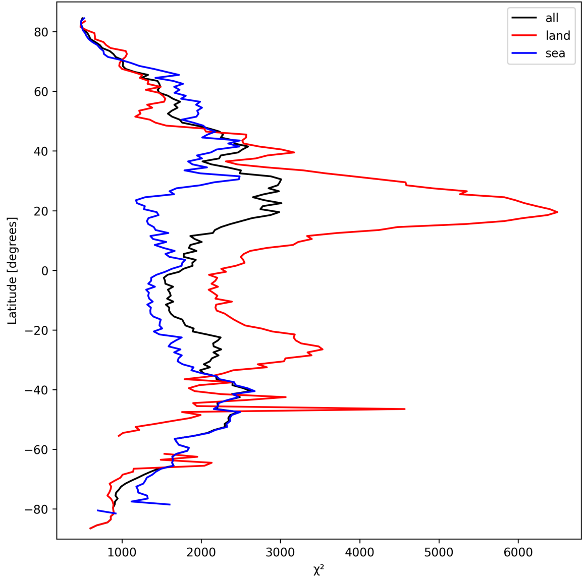
Figure 14: Zonal average of “ \chi^2 ” for 2025-03-17 to 2025-03-18.
