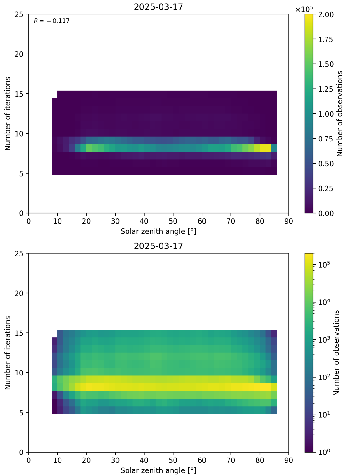
Figure 67: Scatter density plot of “Solar zenith angle” against “Number of iterations” for 2025-03-17 to 2025-03-18.
