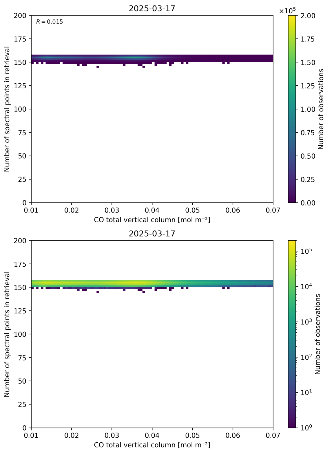
Figure 43: Scatter density plot of “CO total vertical column” against “Number of spectral points in retrieval” for 2025-03-17 to 2025-03-18.
