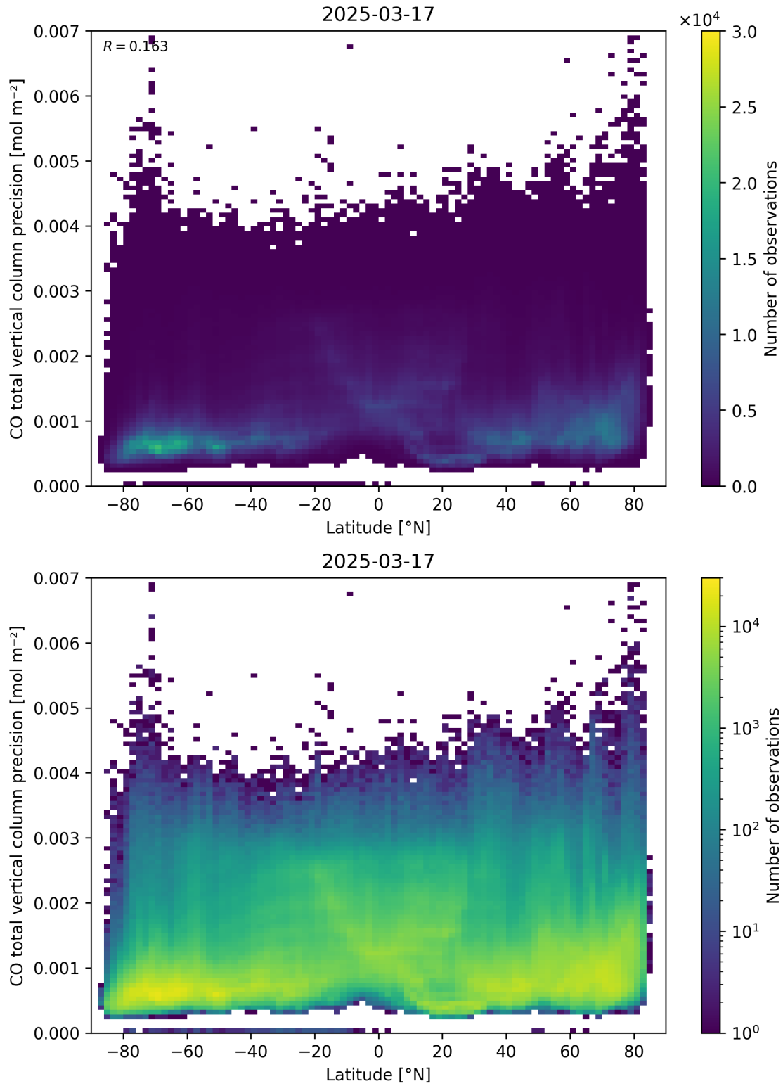
Figure 53: Scatter density plot of “Latitude” against “CO total vertical column precision” for 2025-03-17 to 2025-03-18.
