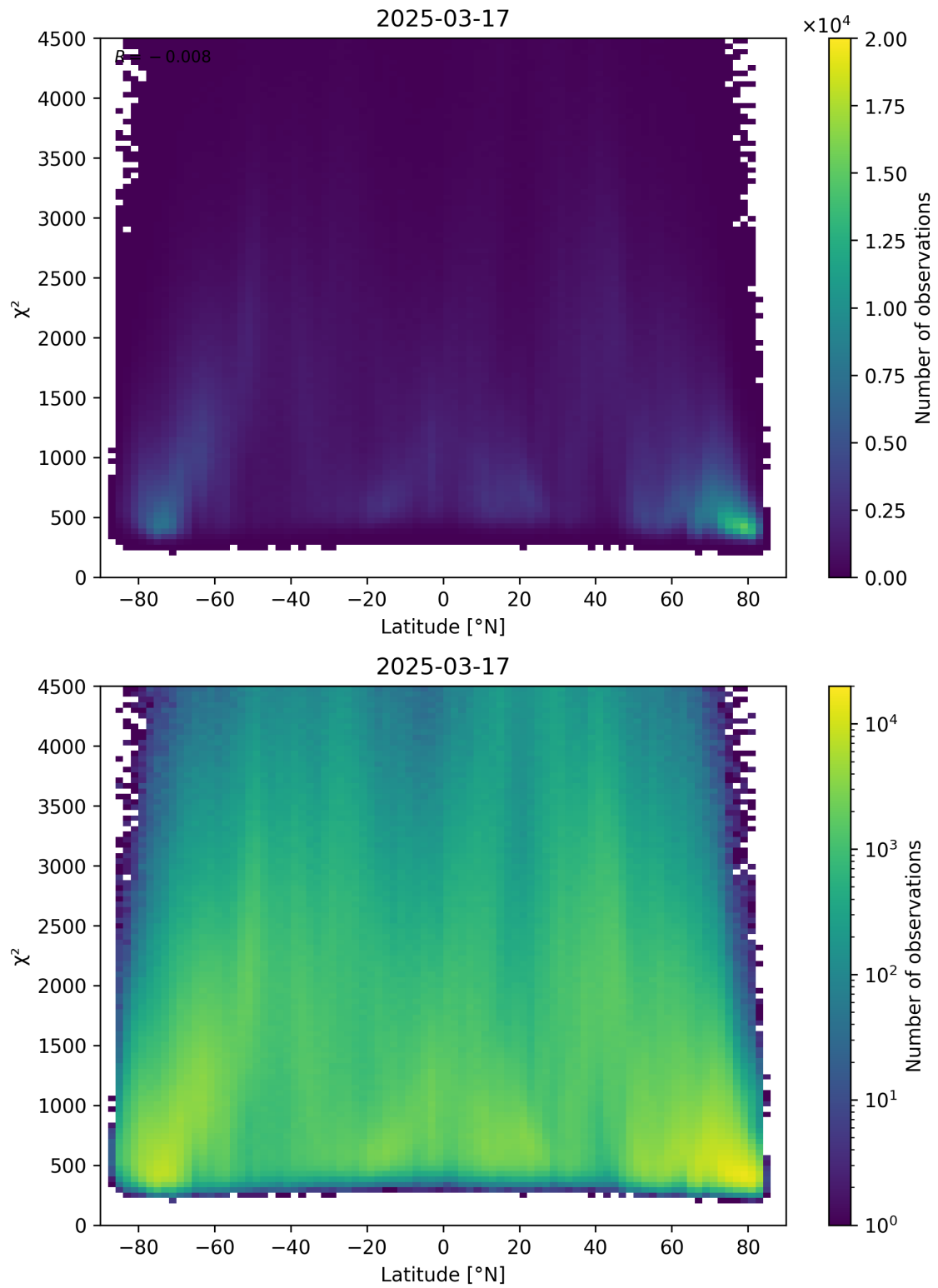
Figure 54: Scatter density plot of “Latitude” against “ \chi^2 ” for 2025-03-17 to 2025-03-18.
