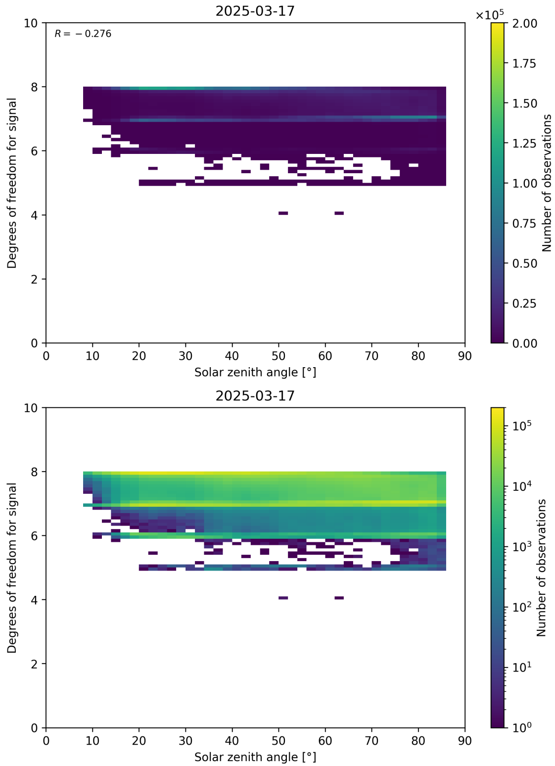
Figure 65: Scatter density plot of “Solar zenith angle” against “Degrees of freedom for signal” for 2025-03-17 to 2025-03-18.
