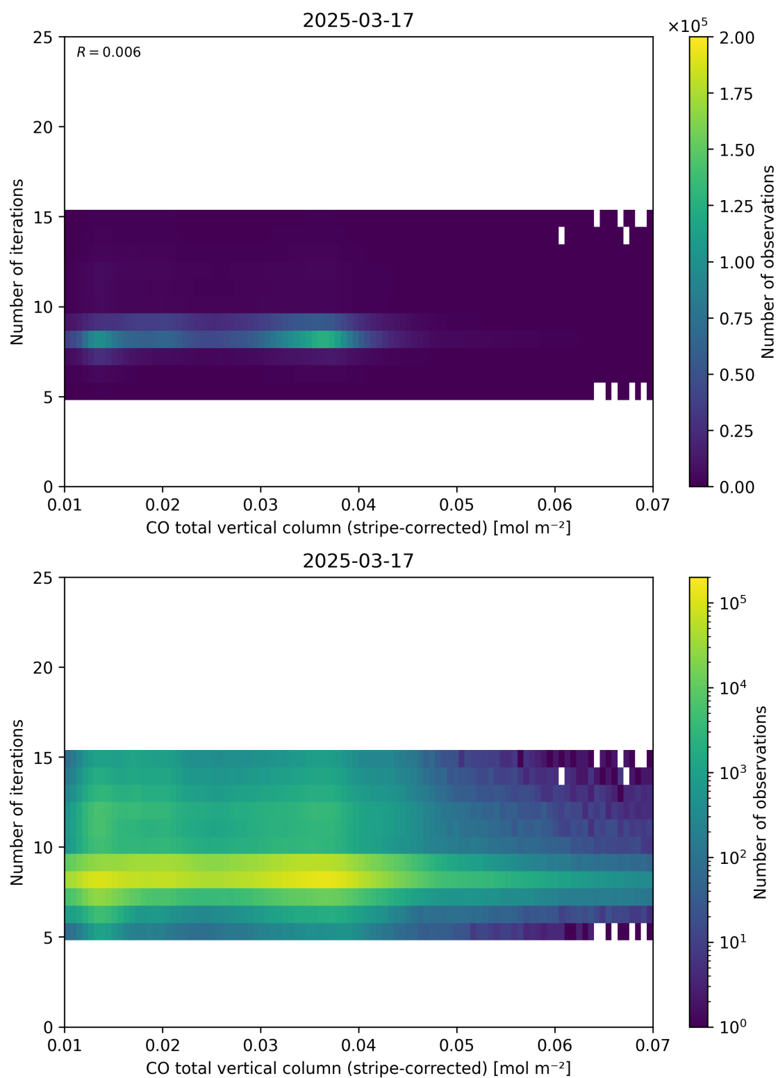
Figure 39: Scatter density plot of “CO total vertical column (stripe-corrected)” against “Number of iterations” for 2025-03-17 to 2025-03-18.
