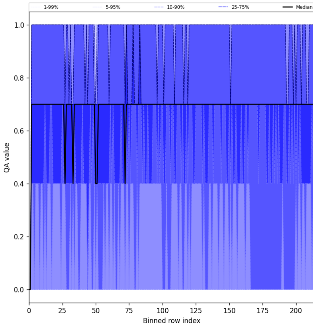
Figure 25: Along track statistics of “QA value” for 2025-03-17 to 2025-03-18
