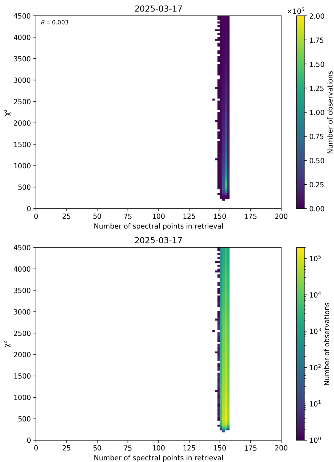
Figure 58: Scatter density plot of “Number of spectral points in retrieval” against “ \chi^2 ” for 2025-03-17 to 2025-03-18.
