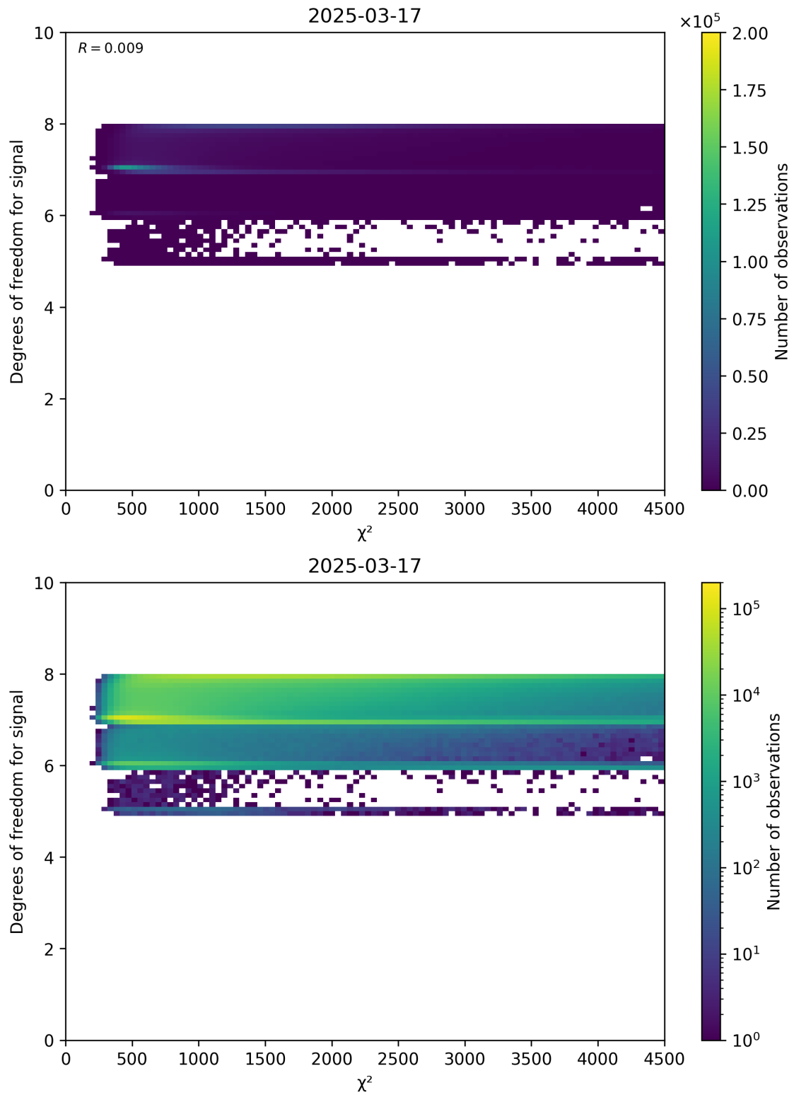
Figure 48: Scatter density plot of “ \chi^2 ” against “Degrees of freedom for signal” for 2025-03-17 to 2025-03-18.
