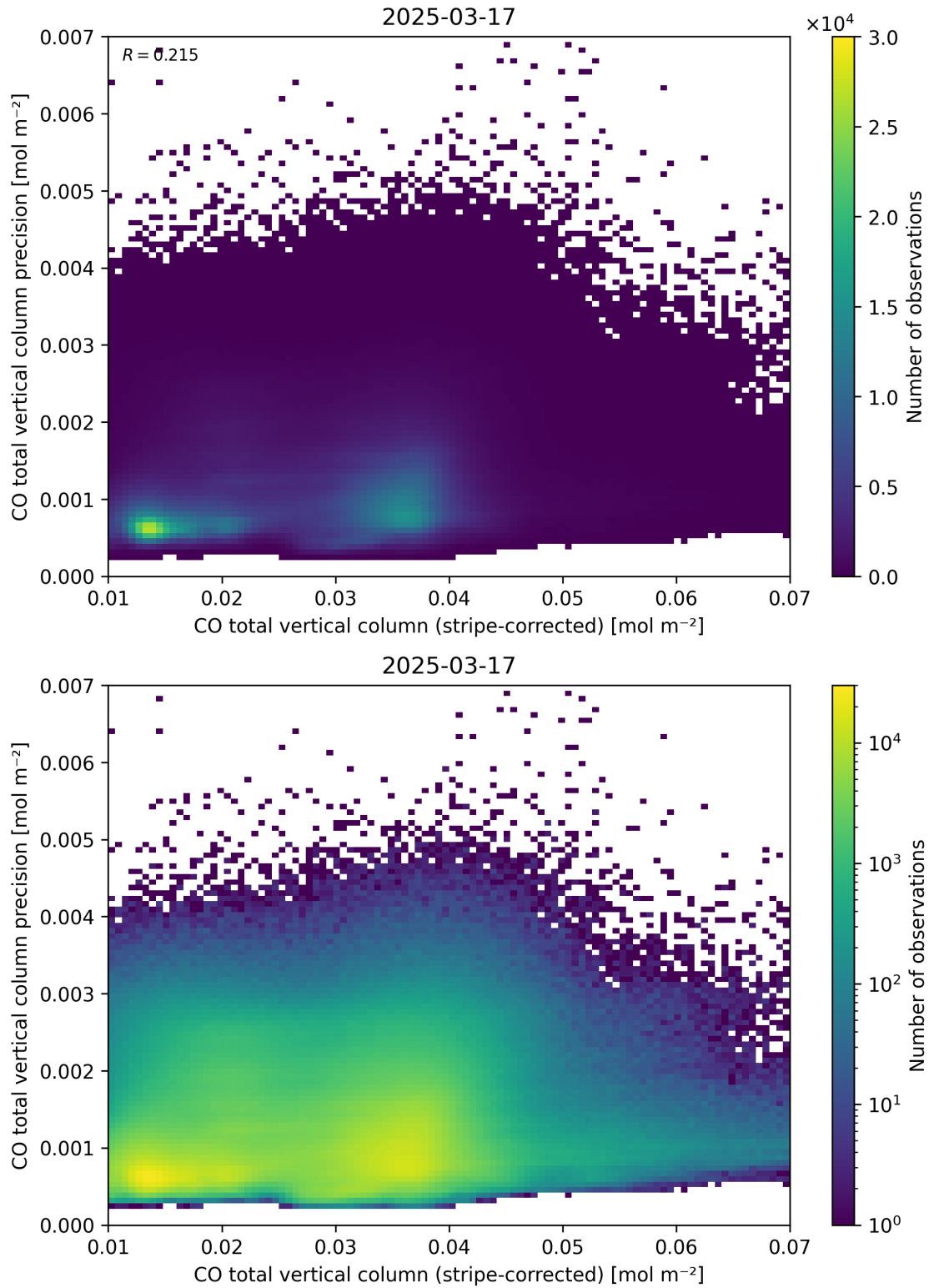
Figure 36: Scatter density plot of “CO total vertical column (stripe-corrected)” against “CO total vertical column precision” for 2025-03-17 to 2025-03-18.
