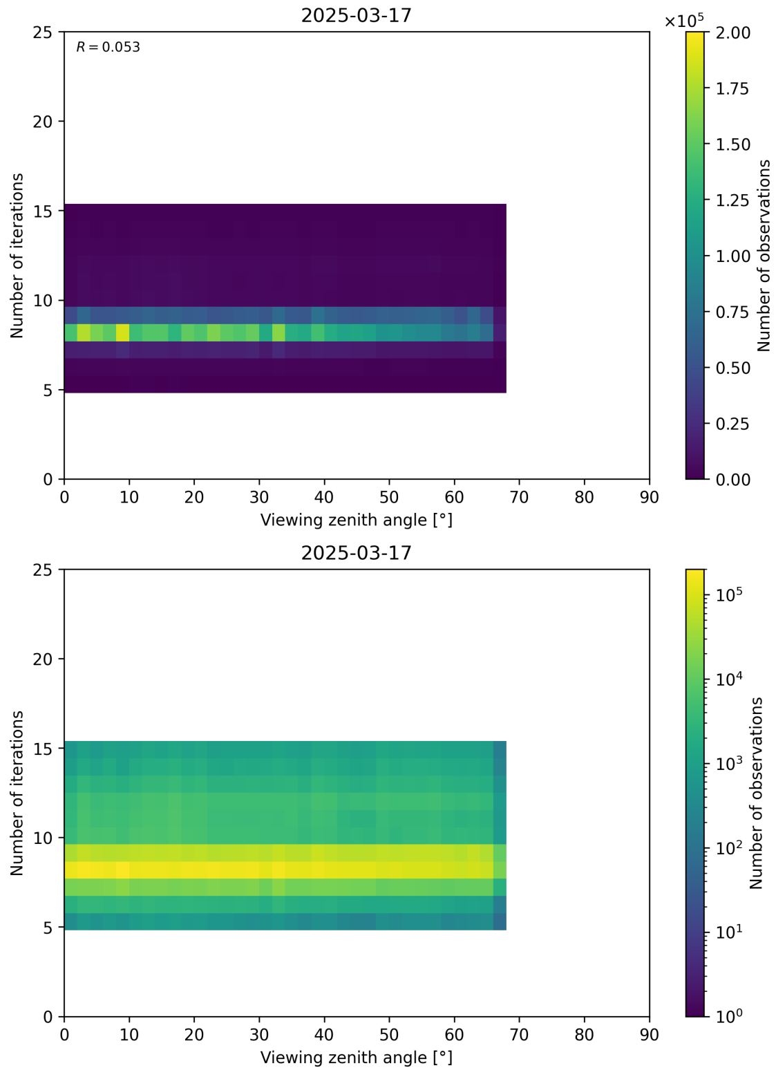
Figure 75: Scatter density plot of “Viewing zenith angle” against “Number of iterations” for 2025-03-17 to 2025-03-18.
