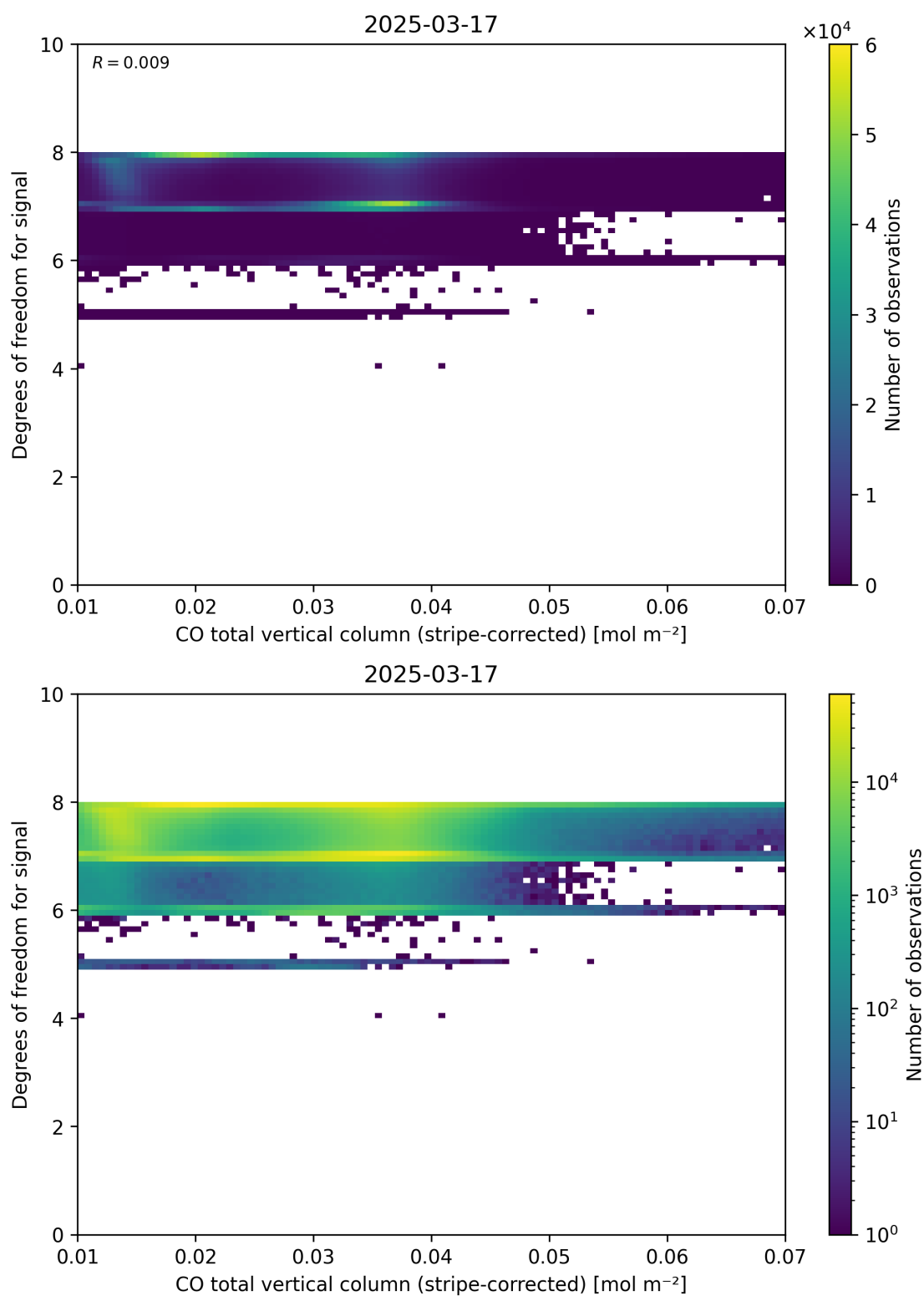
Figure 38: Scatter density plot of “CO total vertical column (stripe-corrected)” against “Degrees of freedom for signal” for 2025-03-17 to 2025-03-18.
