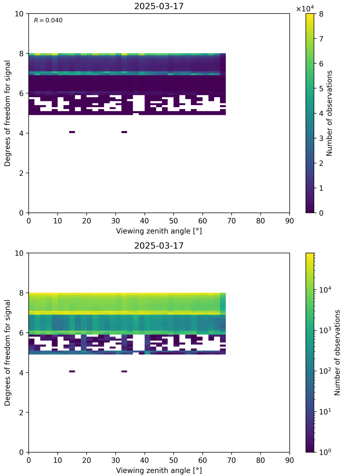
Figure 73: Scatter density plot of “Viewing zenith angle” against “Degrees of freedom for signal” for 2025-03-17 to 2025-03-18.
