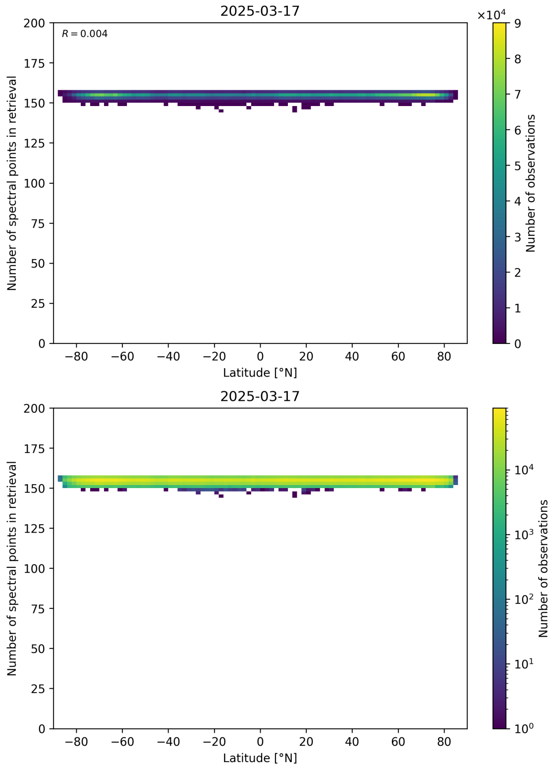
Figure 57: Scatter density plot of “Latitude” against “Number of spectral points in retrieval” for 2025-03-17 to 2025-03-18.
