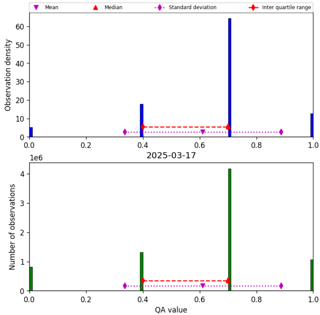
Figure 17: Histogram of “QA value” for 2025-03-17 to 2025-03-18
