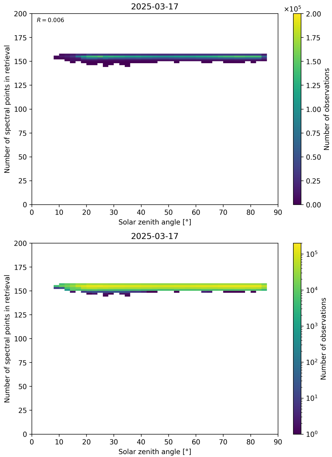
Figure 68: Scatter density plot of “Solar zenith angle” against “Number of spectral points in retrieval” for 2025-03-17 to 2025-03-18.
