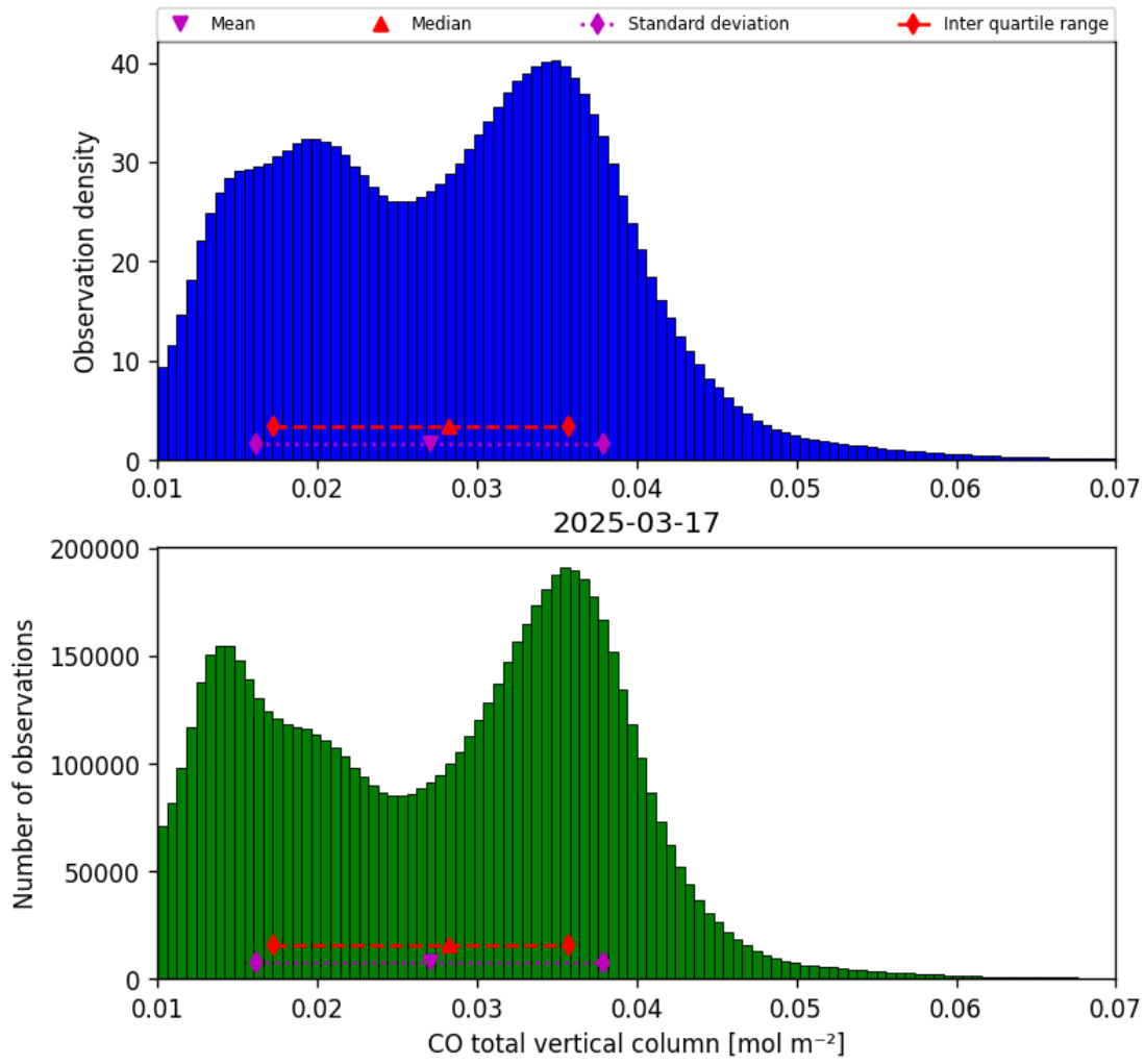
Figure 18: Histogram of “CO total vertical column” for 2025-03-17 to 2025-03-18
