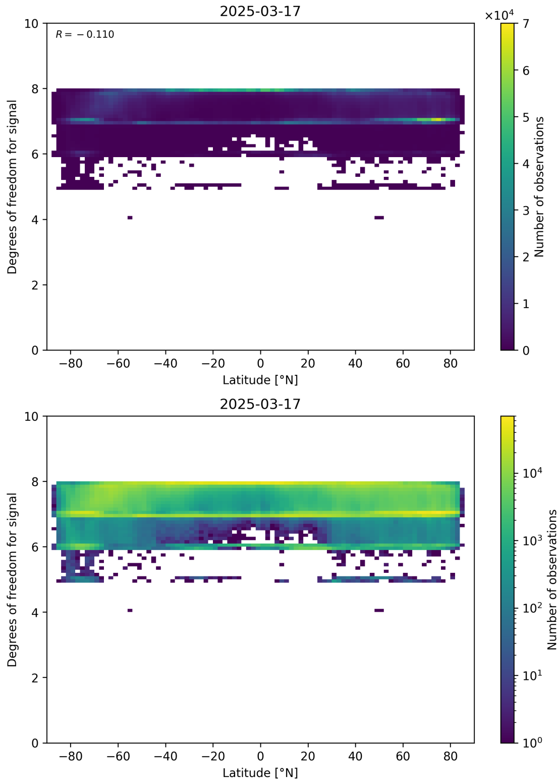
Figure 55: Scatter density plot of “Latitude” against “Degrees of freedom for signal” for 2025-03-17 to 2025-03-18.
