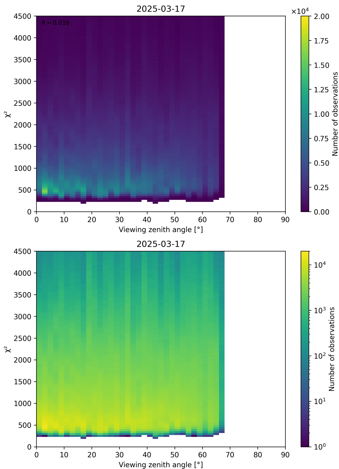
Figure 72: Scatter density plot of “Viewing zenith angle” against “ \chi^2 ” for 2025-03-17 to 2025-03-18.
