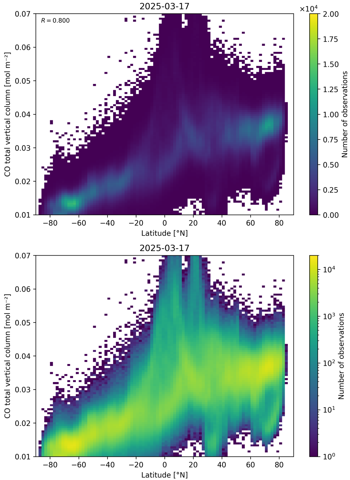
Figure 51: Scatter density plot of “Latitude” against “CO total vertical column” for 2025-03-17 to 2025-03-18.
