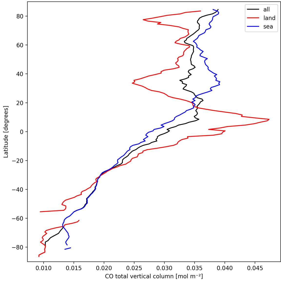
Figure 10: Zonal average of “CO total vertical column” for 2025-03-17 to 2025-03-18.
