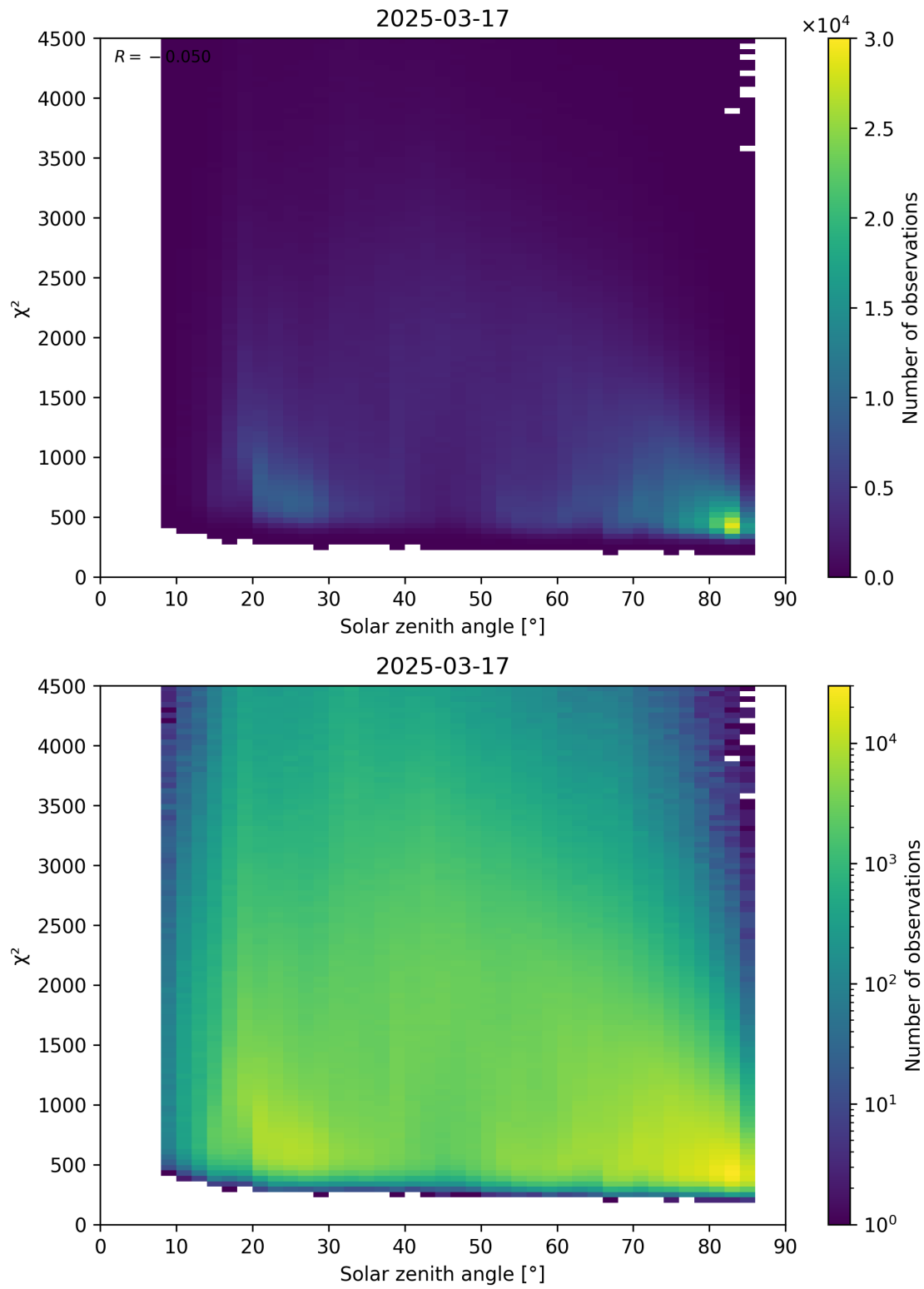
Figure 64: Scatter density plot of “Solar zenith angle” against “ \chi^2 ” for 2025-03-17 to 2025-03-18.
