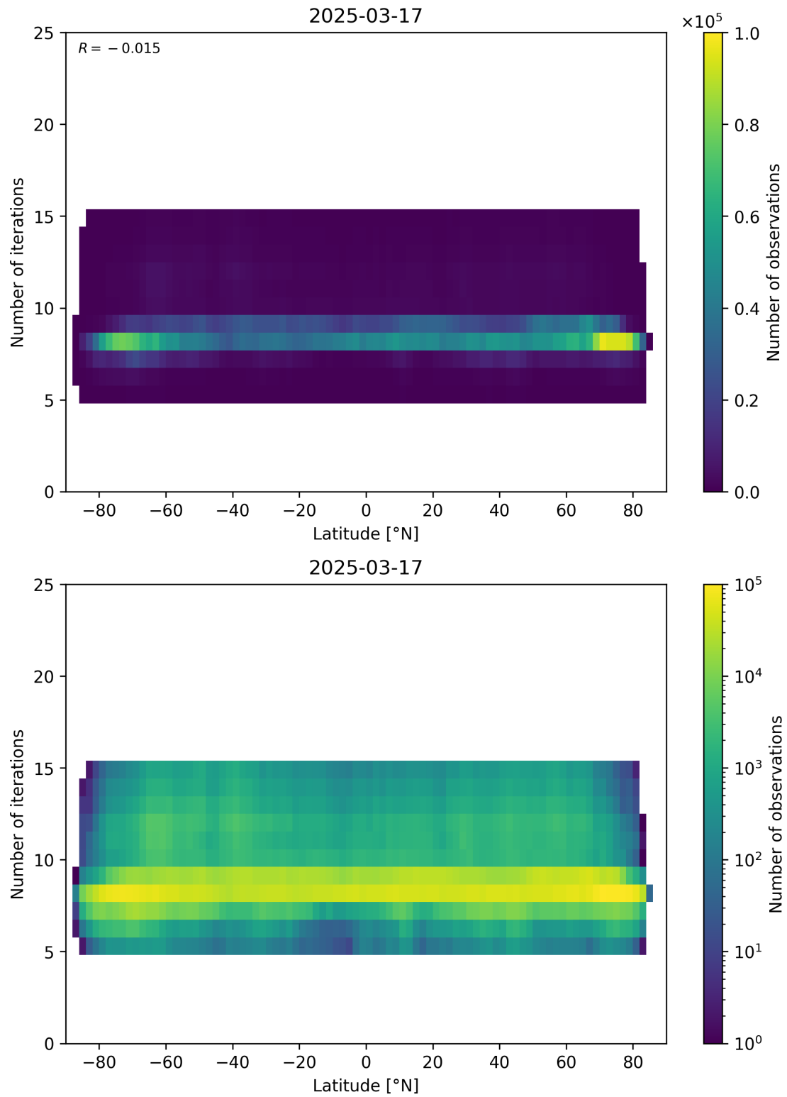
Figure 56: Scatter density plot of “Latitude” against “Number of iterations” for 2025-03-17 to 2025-03-18.
