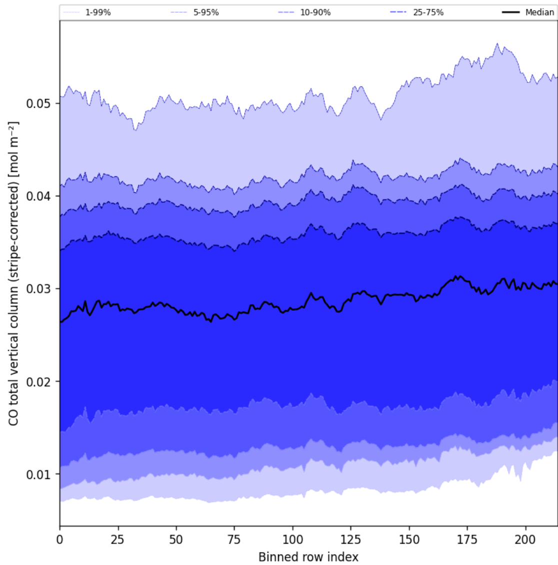
Figure 27: Along track statistics of “CO total vertical column (stripe-corrected)” for 2025-03-17 to 2025-03-18
