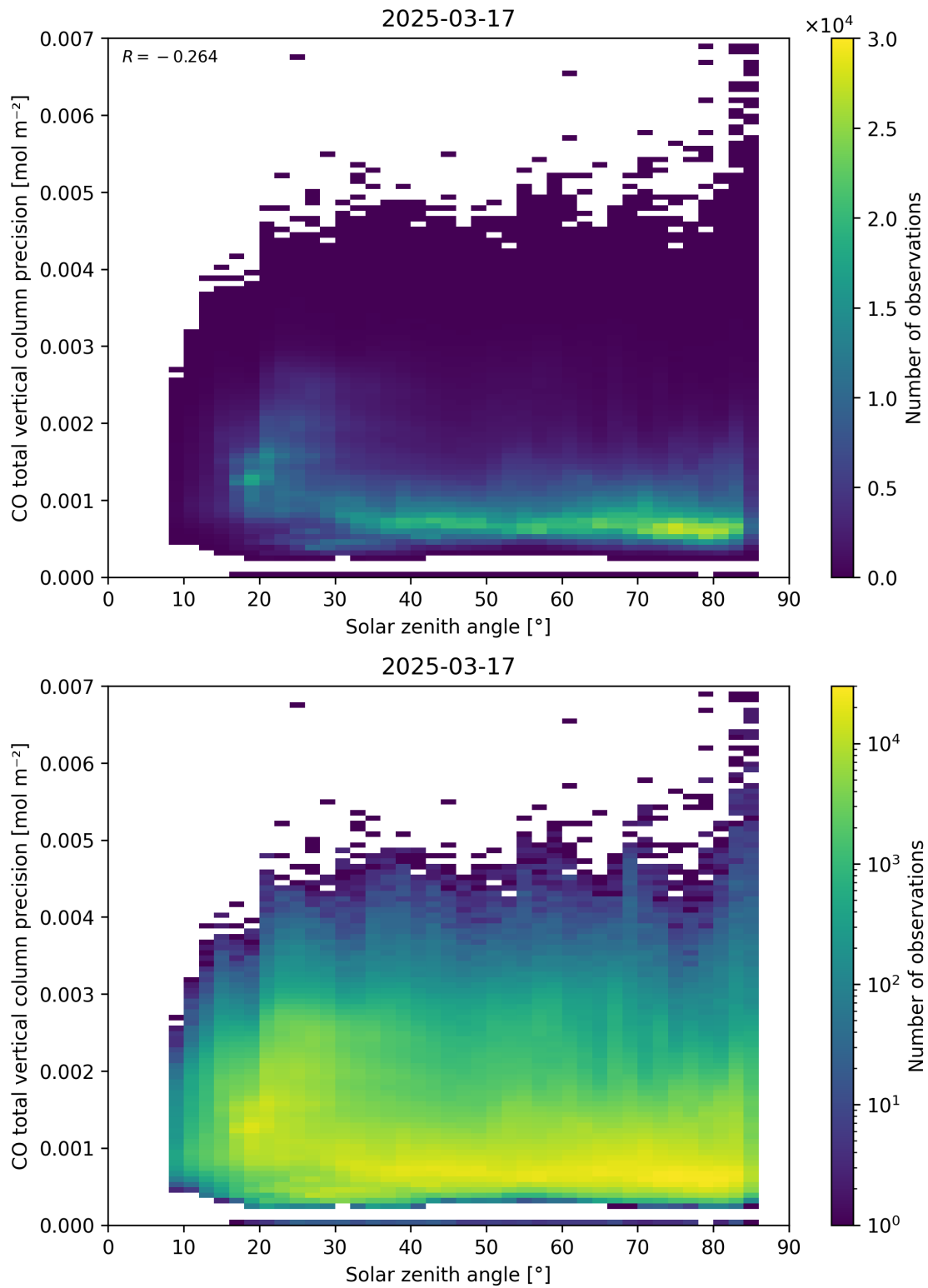
Figure 63: Scatter density plot of “Solar zenith angle” against “CO total vertical column precision” for 2025-03-17 to 2025-03-18.
