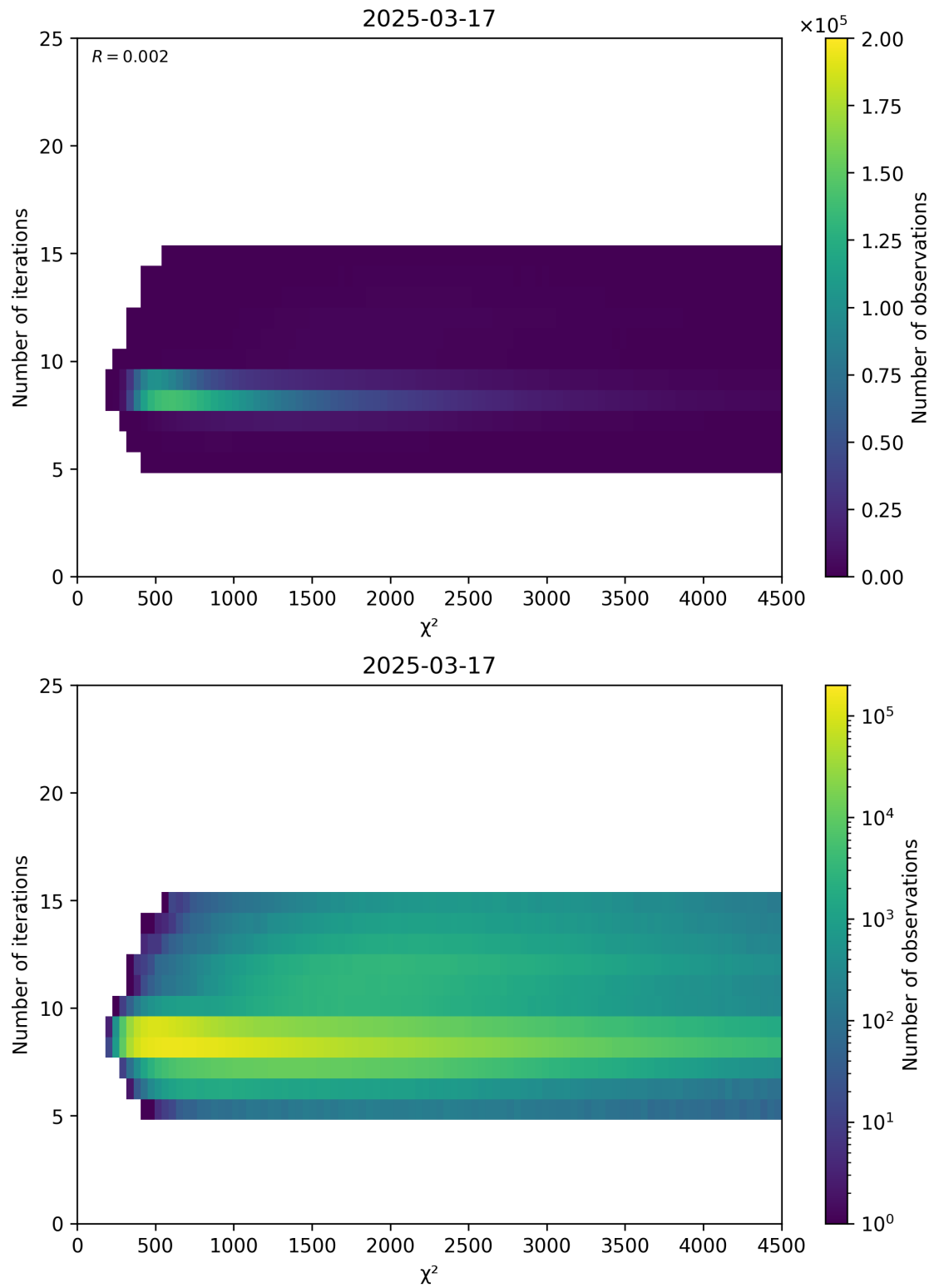
Figure 49: Scatter density plot of “ \chi^2 ” against “Number of iterations” for 2025-03-17 to 2025-03-18.
