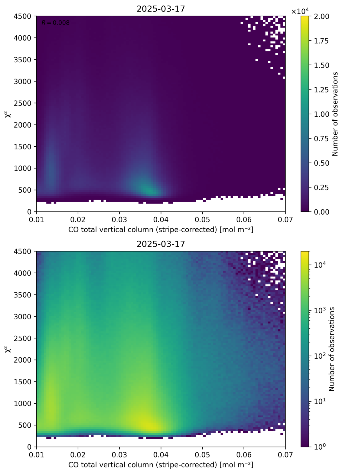
Figure 37: Scatter density plot of “CO total vertical column (stripe-corrected)” against “ \chi^2 ” for 2025-03-17 to 2025-03-18.
