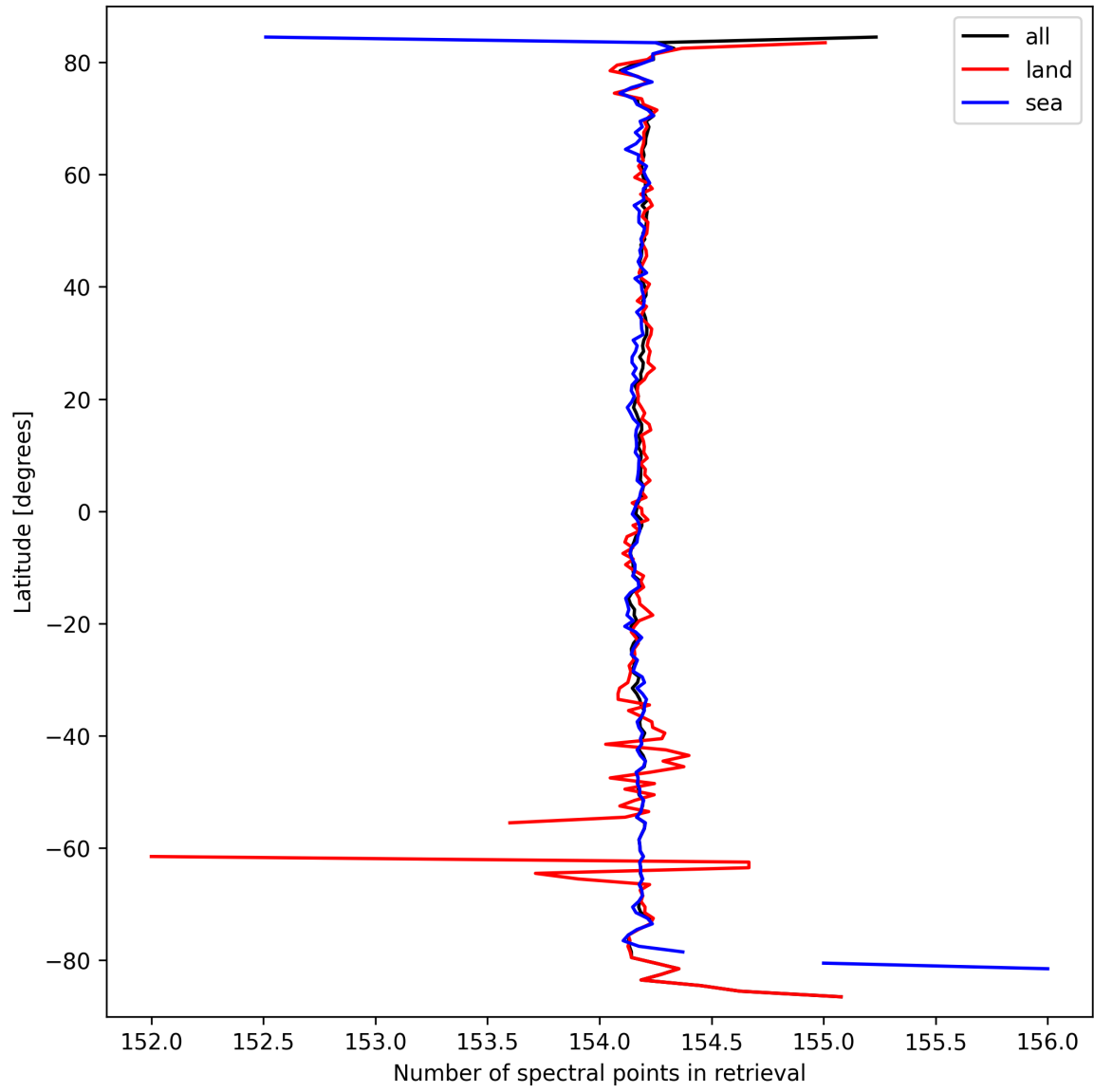
Figure 13: Zonal average of “Number of spectral points in retrieval” for 2025-03-17 to 2025-03-18.
