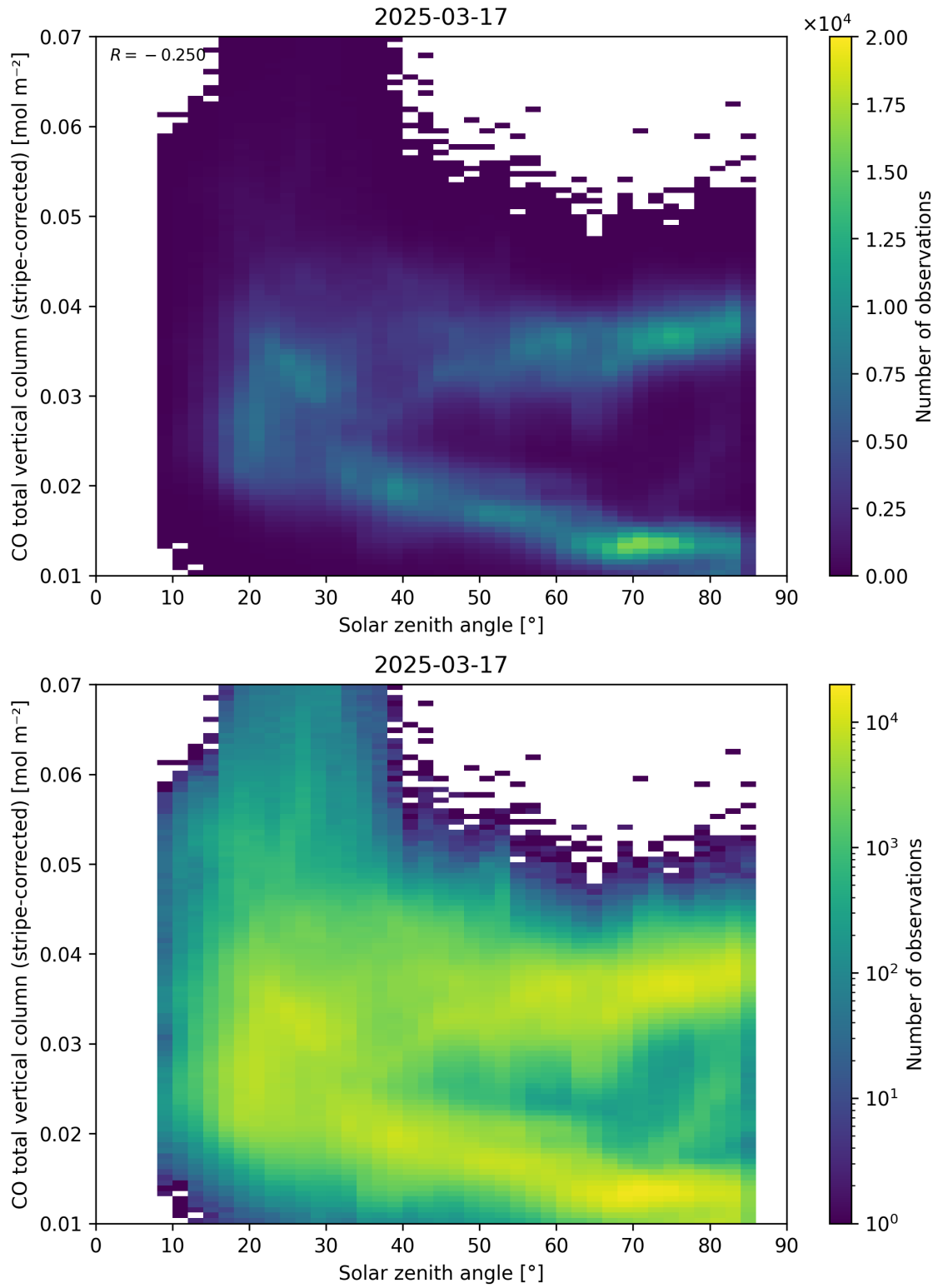
Figure 62: Scatter density plot of “Solar zenith angle” against “CO total vertical column (stripe-corrected)” for 2025-03-17 to 2025-03-18.
