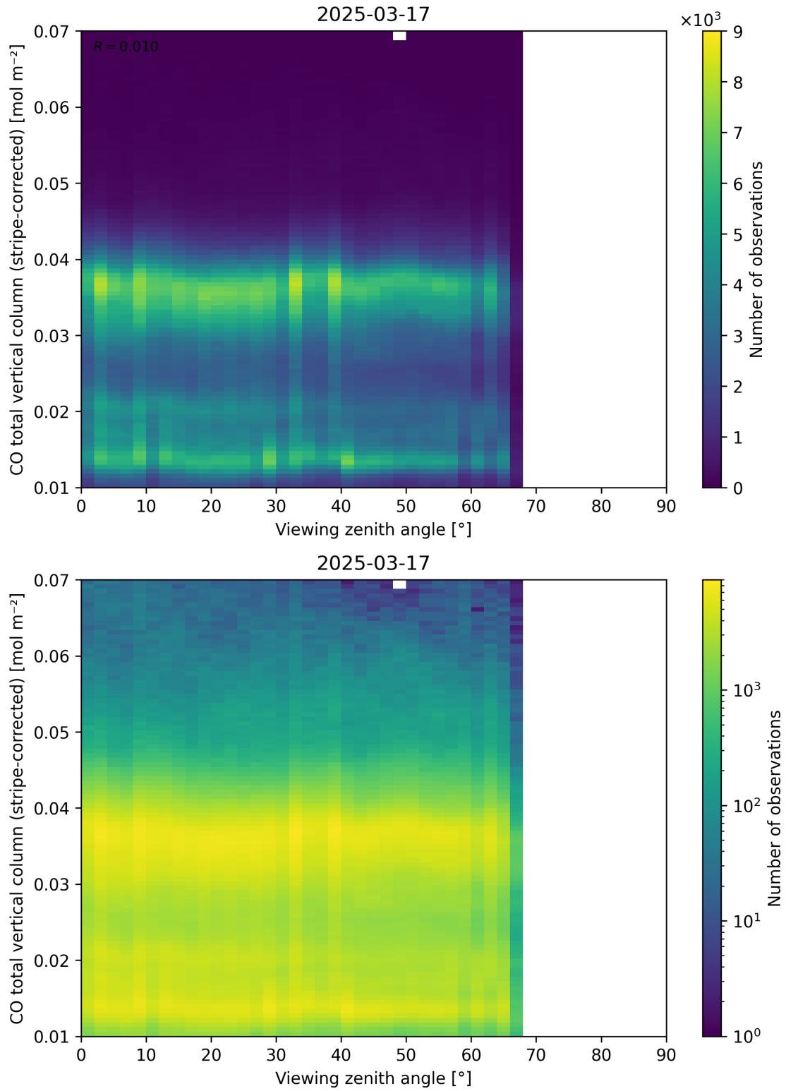
Figure 70: Scatter density plot of “Viewing zenith angle” against “CO total vertical column (stripe-corrected)” for 2025-03-17 to 2025-03-18.
