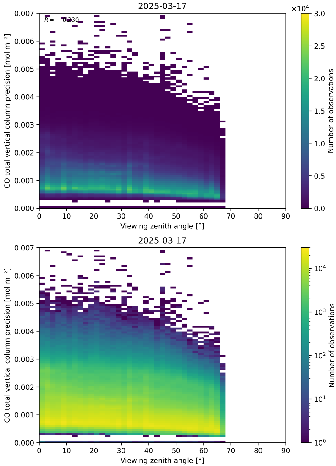
Figure 71: Scatter density plot of “Viewing zenith angle” against “CO total vertical column precision” for 2025-03-17 to 2025-03-18.
