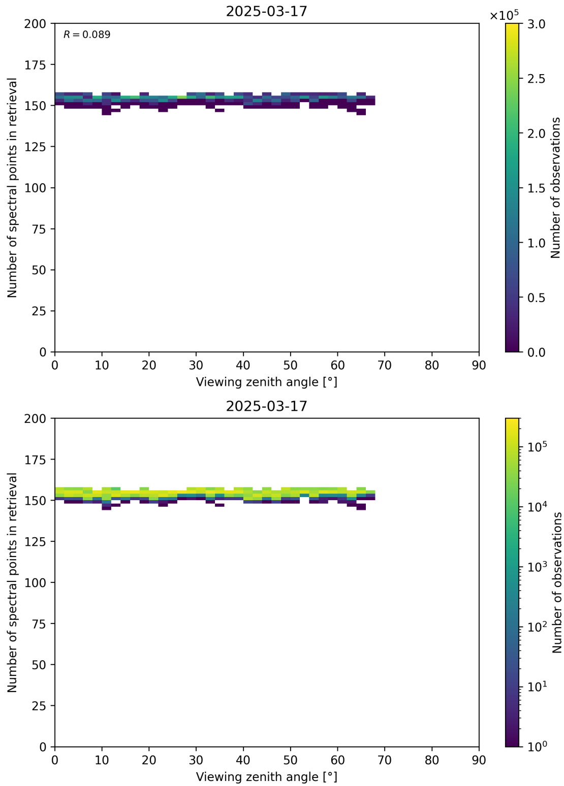
Figure 76: Scatter density plot of “Viewing zenith angle” against “Number of spectral points in retrieval” for 2025-03-17 to 2025-03-18.
