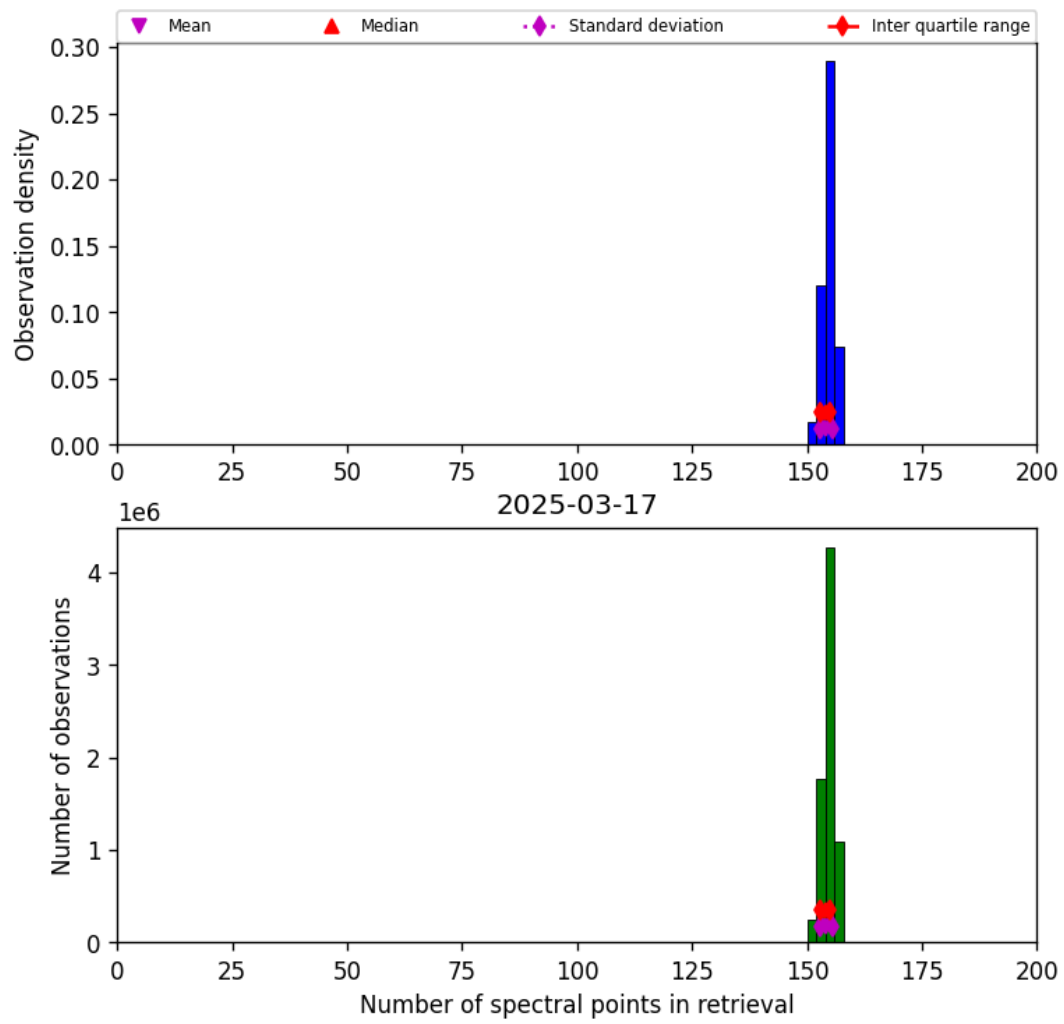
Figure 21: Histogram of “Number of spectral points in retrieval” for 2025-03-17 to 2025-03-18
