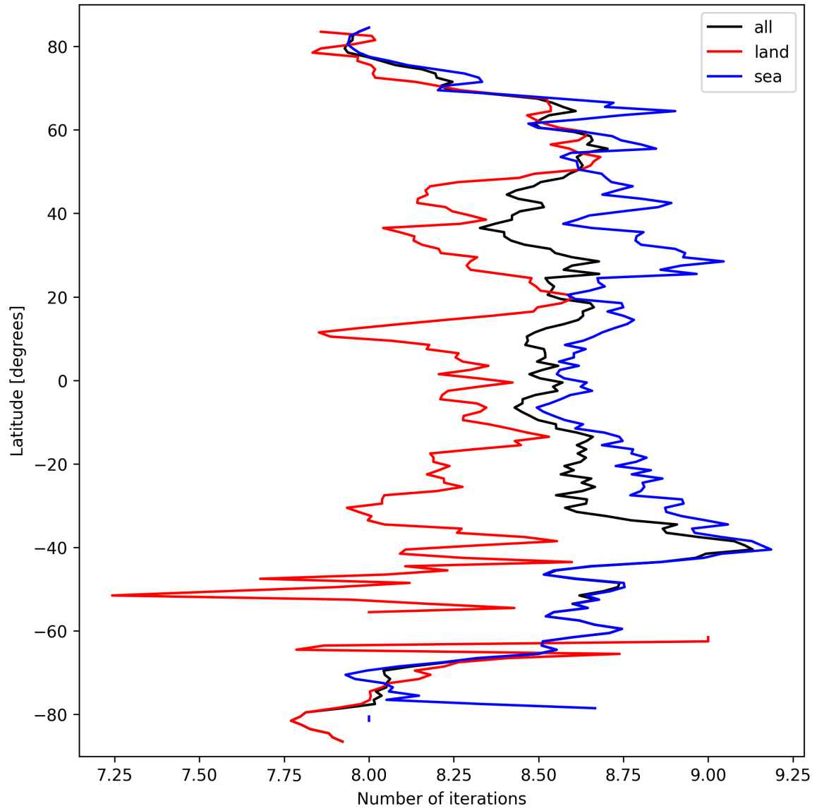
Figure 16: Zonal average of “Number of iterations” for 2025-03-17 to 2025-03-18.
