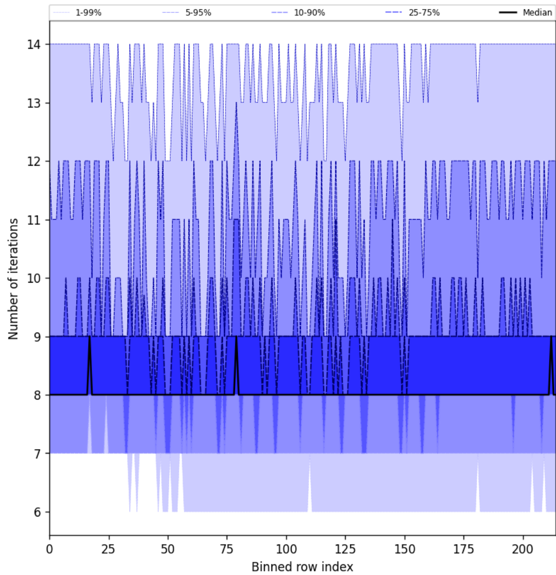
Figure 32: Along track statistics of “Number of iterations” for 2025-03-17 to 2025-03-18
