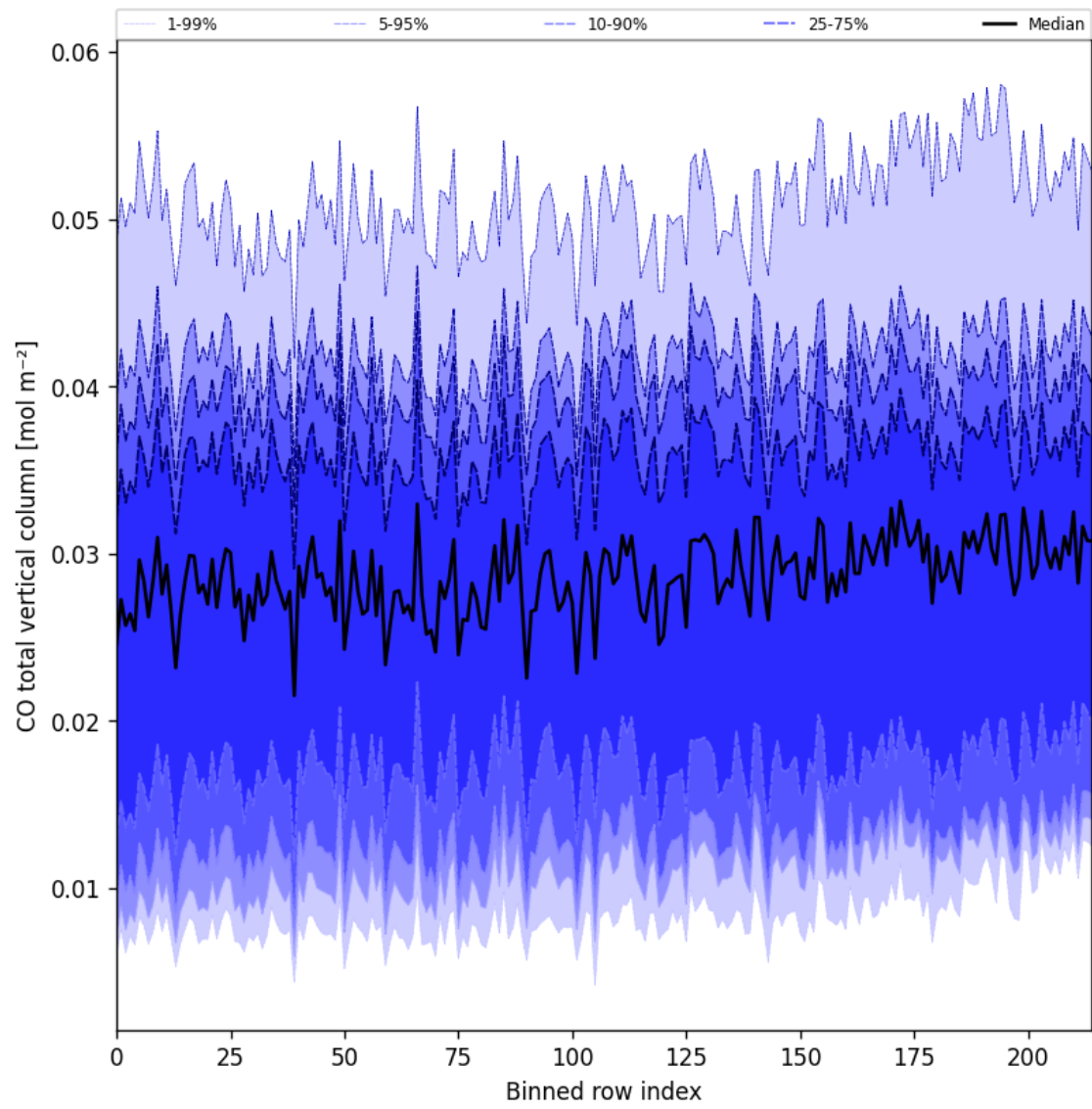
Figure 26: Along track statistics of “CO total vertical column” for 2025-03-17 to 2025-03-18
