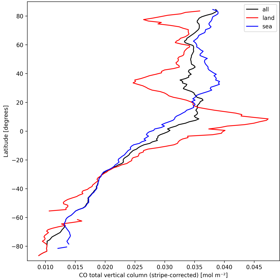
Figure 11: Zonal average of “CO total vertical column (stripe-corrected)” for 2025-03-17 to 2025-03-18.
