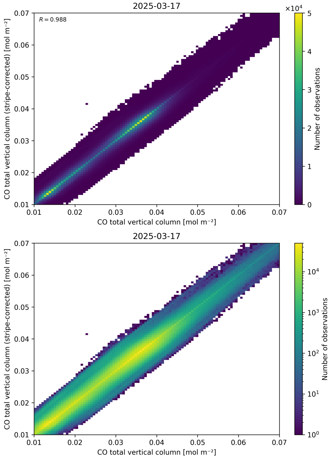
Figure 33: Scatter density plot of “CO total vertical column” against “CO total vertical column (stripe-corrected)” for 2025-03-17 to 2025-03-18.
