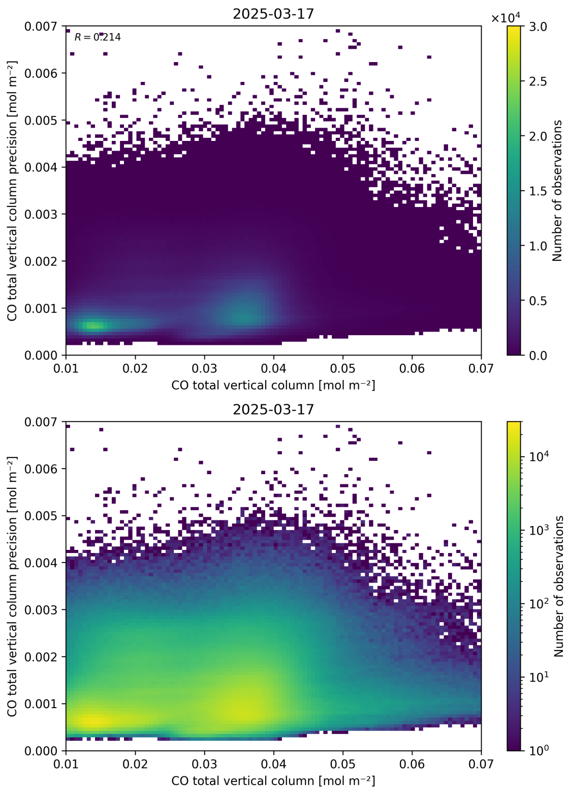
Figure 34: Scatter density plot of “CO total vertical column” against “CO total vertical column precision” for 2025-03-17 to 2025-03-18.
