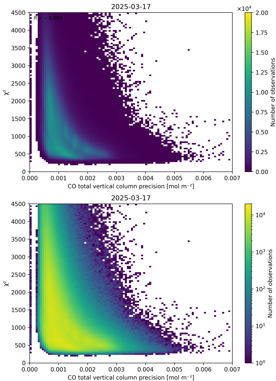
Figure 44: Scatter density plot of “CO total vertical column precision” against “ \chi^2 ” for 2025-03-17 to 2025-03-18.
