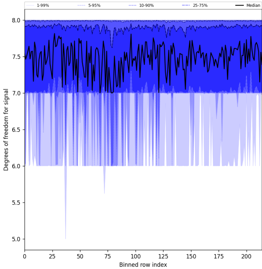
Figure 31: Along track statistics of “Degrees of freedom for signal” for 2025-03-17 to 2025-03-18
