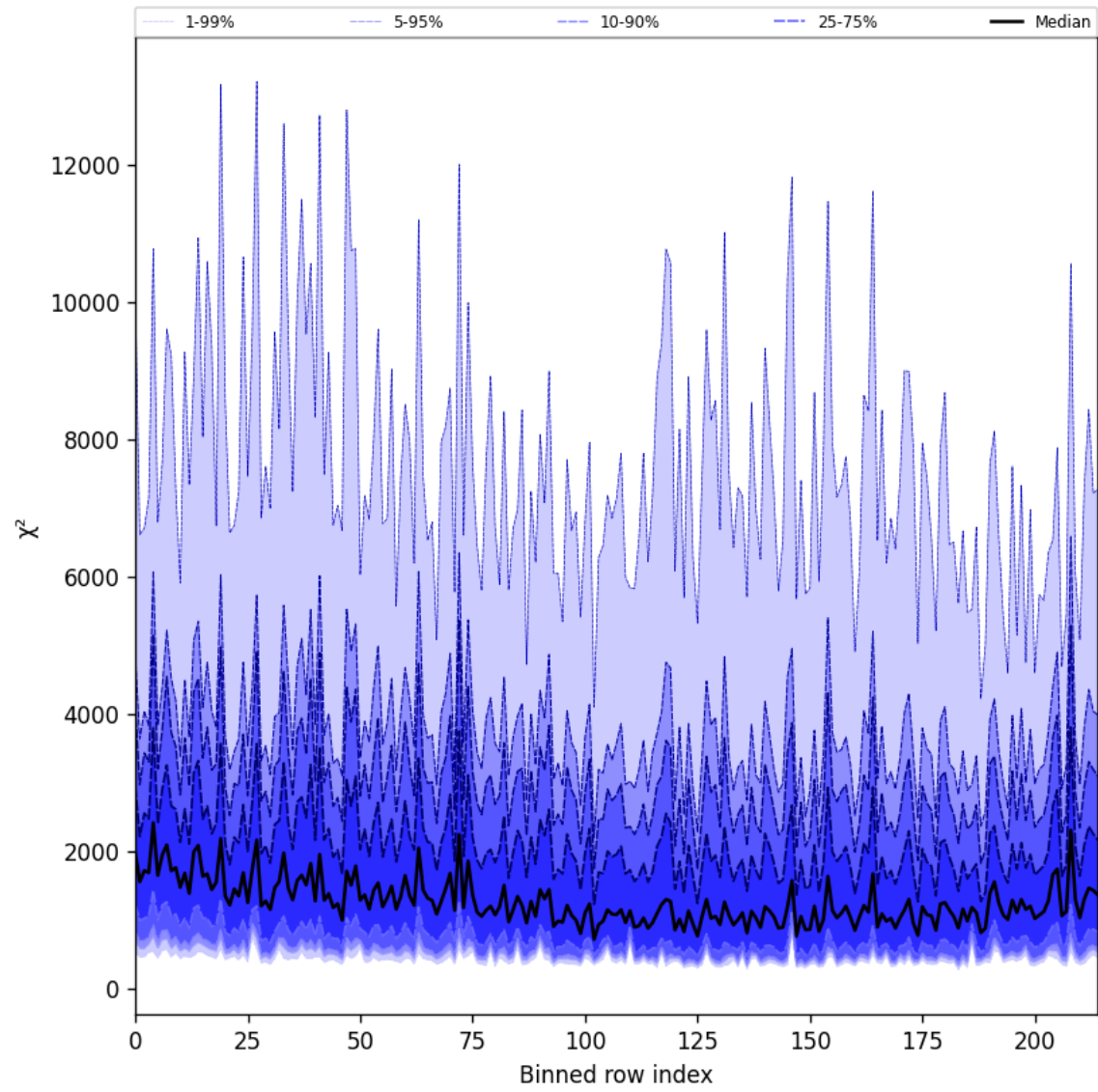
Figure 30: Along track statistics of “ \chi^2 ” for 2025-03-17 to 2025-03-18
