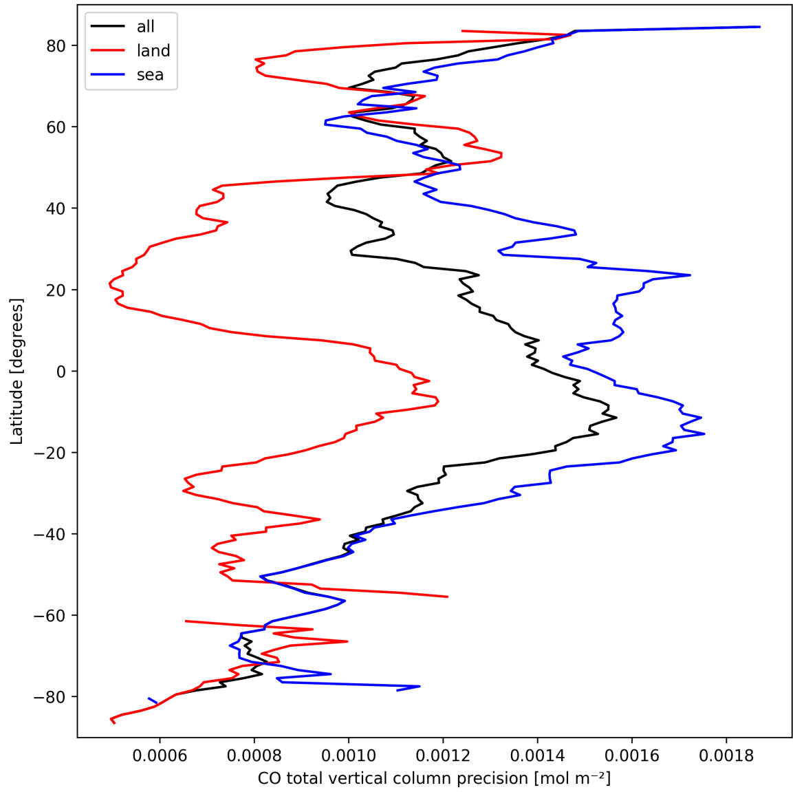
Figure 12: Zonal average of “CO total vertical column precision” for 2025-03-17 to 2025-03-18.
