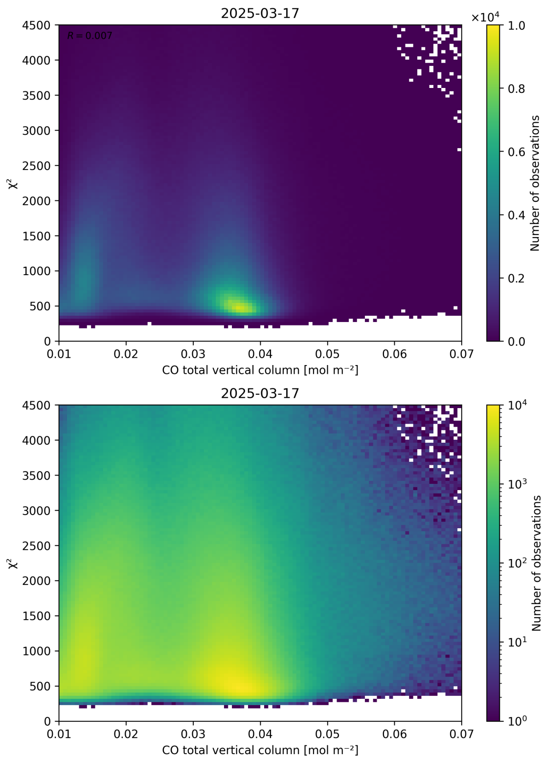
Figure 35: Scatter density plot of “CO total vertical column” against “ \chi^2 ” for 2025-03-17 to 2025-03-18.
