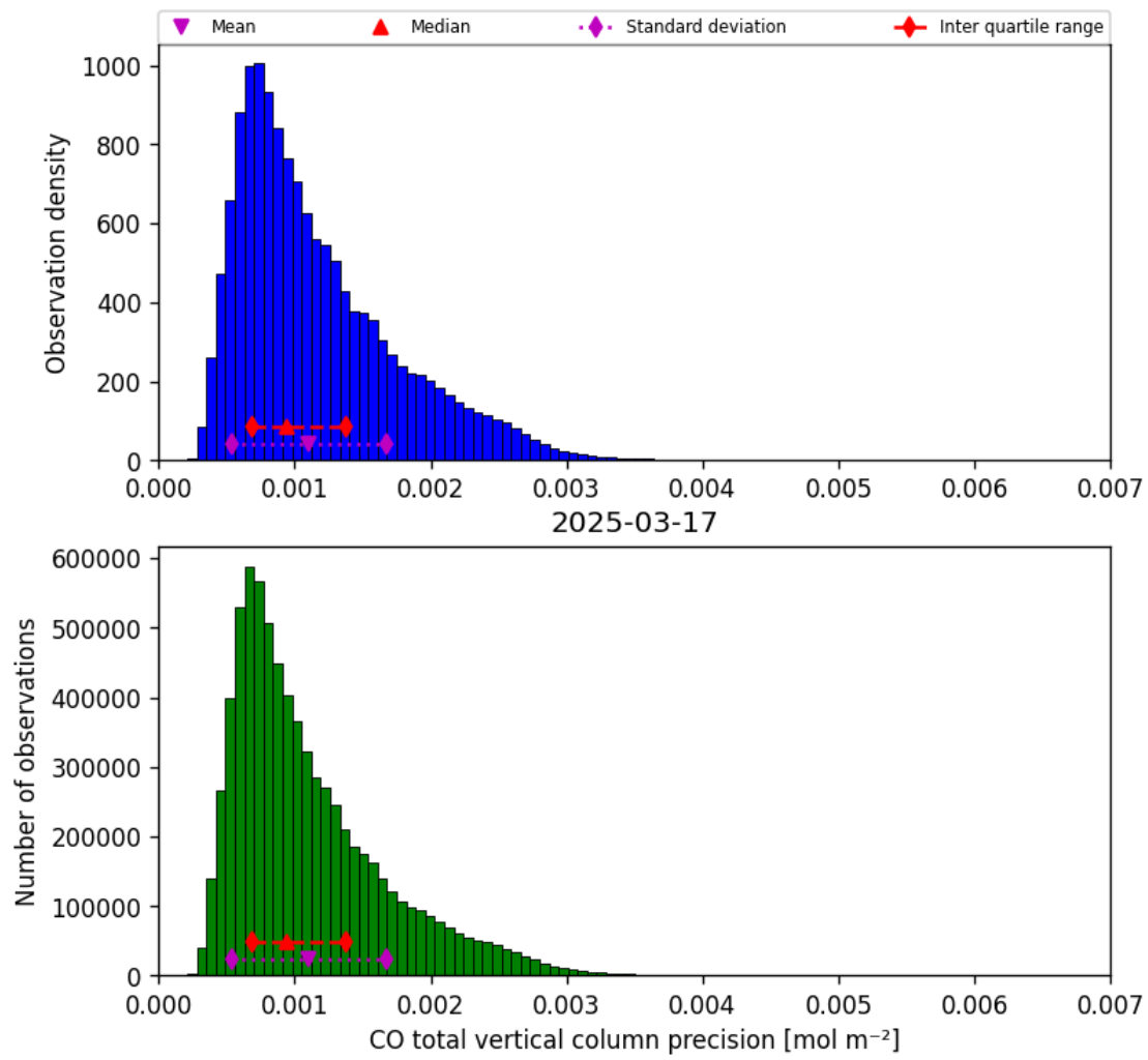
Figure 20: Histogram of “CO total vertical column precision” for 2025-03-17 to 2025-03-18
