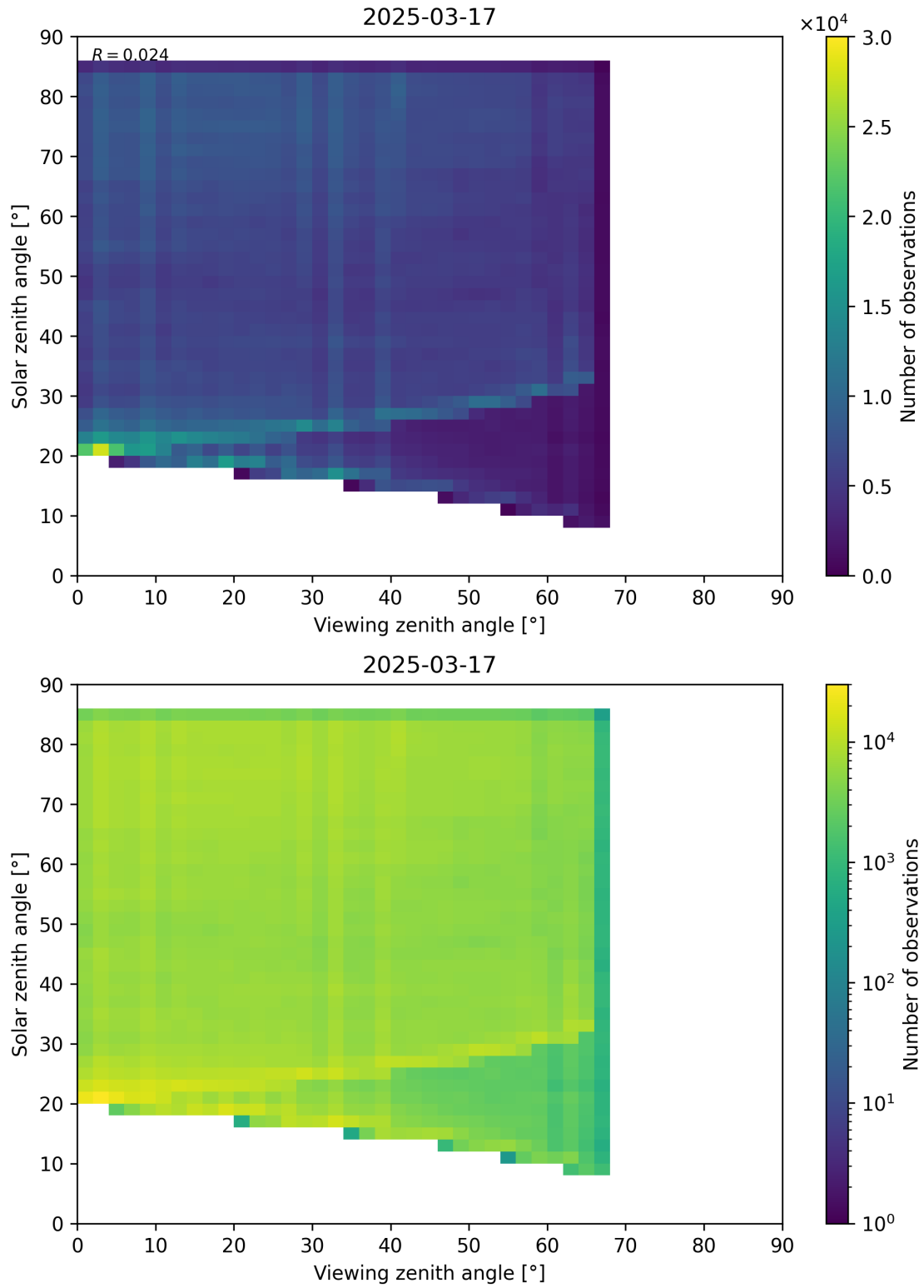
Figure 77: Scatter density plot of “Viewing zenith angle” against “Solar zenith angle” for 2025-03-17 to 2025-03-18.
