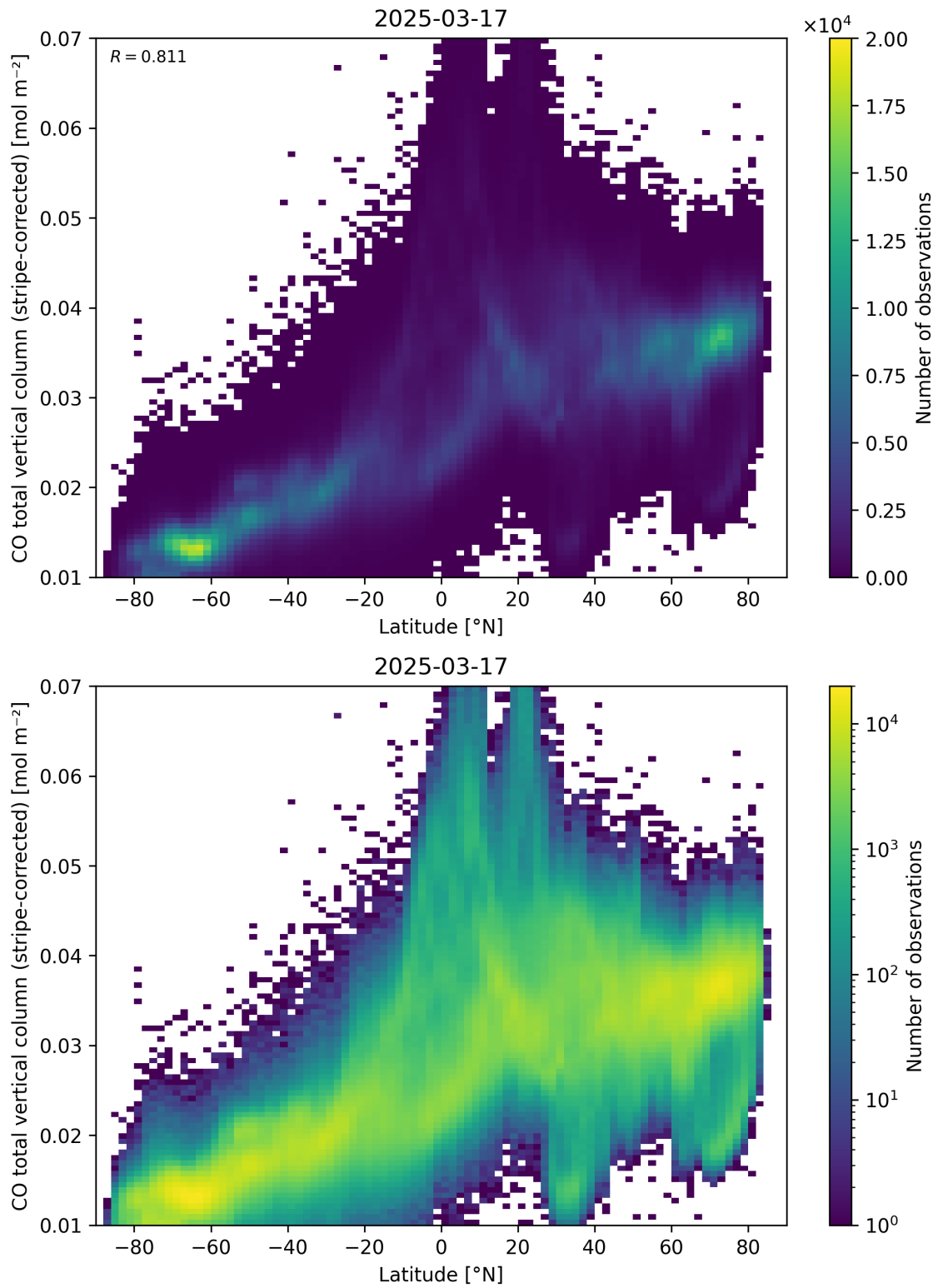
Figure 52: Scatter density plot of “Latitude” against “CO total vertical column (stripe-corrected)” for 2025-03-17 to 2025-03-18.
