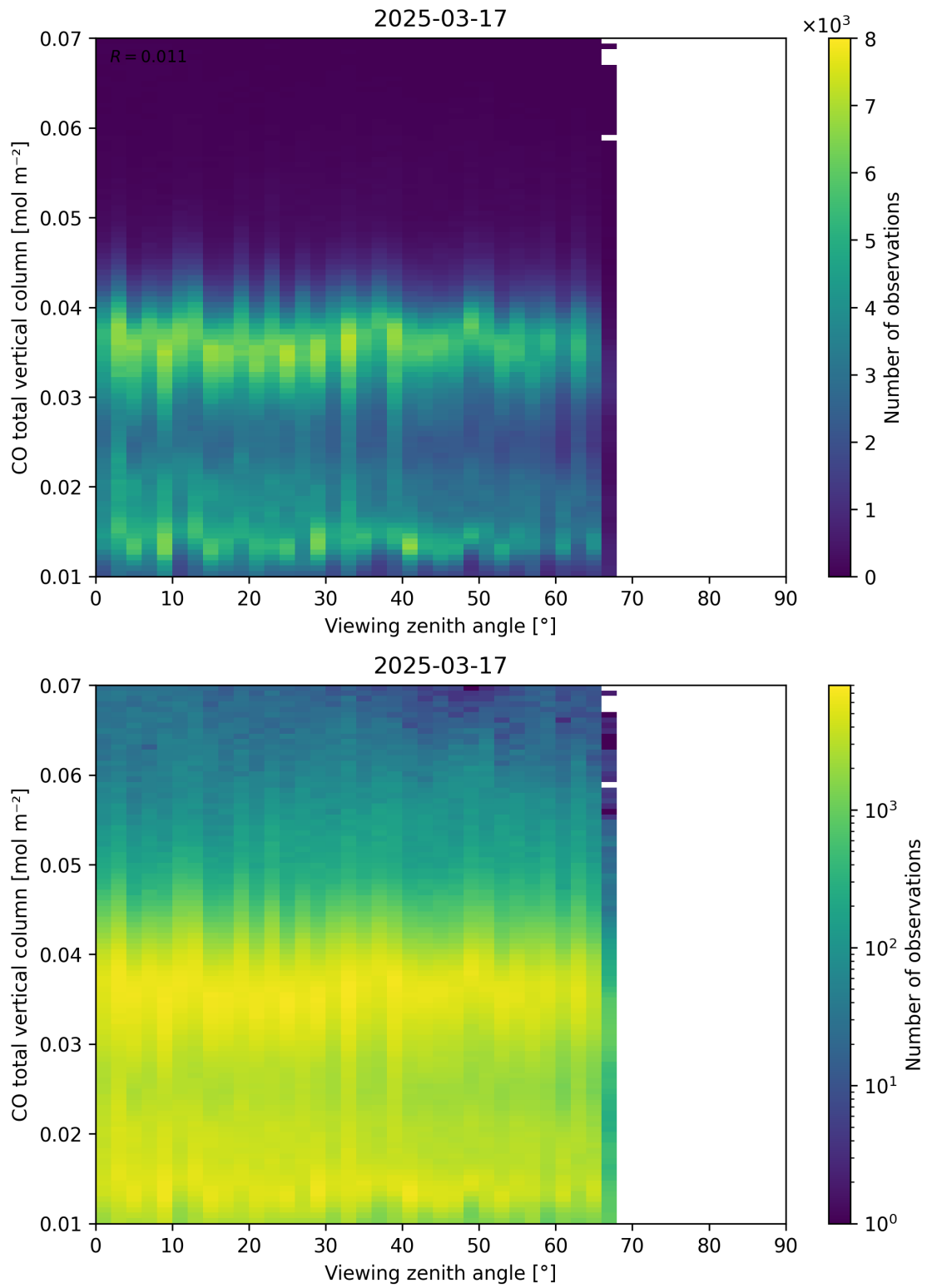
Figure 69: Scatter density plot of “Viewing zenith angle” against “CO total vertical column” for 2025-03-17 to 2025-03-18.
