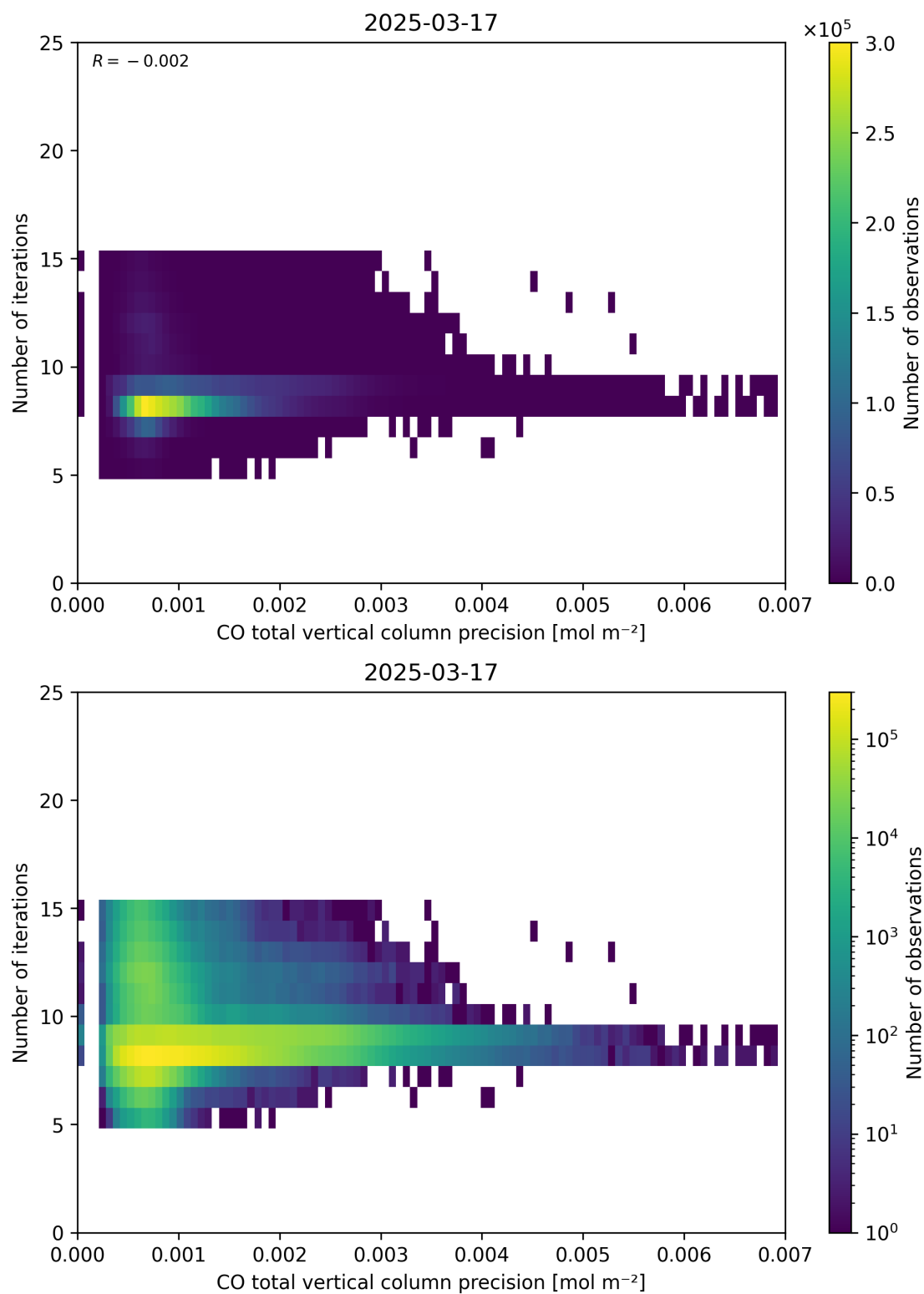
Figure 46: Scatter density plot of “CO total vertical column precision” against “Number of iterations” for 2025-03-17 to 2025-03-18.
