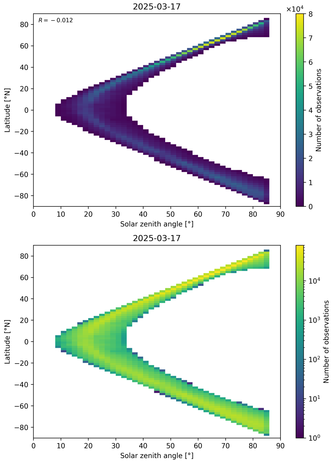
Figure 66: Scatter density plot of “Solar zenith angle” against “Latitude” for 2025-03-17 to 2025-03-18.
