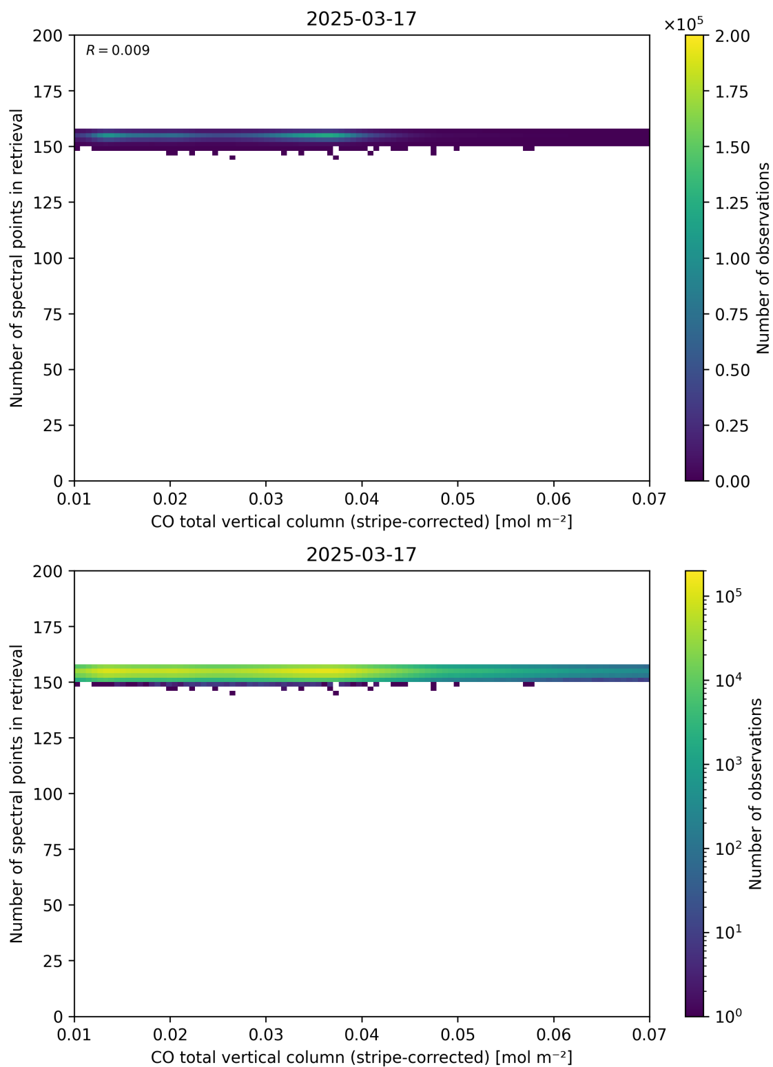
Figure 40: Scatter density plot of “CO total vertical column (stripe-corrected)” against “Number of spectral points in retrieval” for 2025-03-17 to 2025-03-18.
