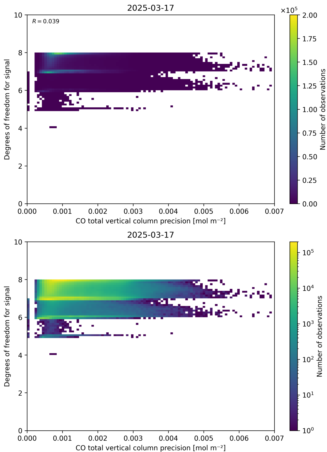
Figure 45: Scatter density plot of “CO total vertical column precision” against “Degrees of freedom for signal” for 2025-03-17 to 2025-03-18.
