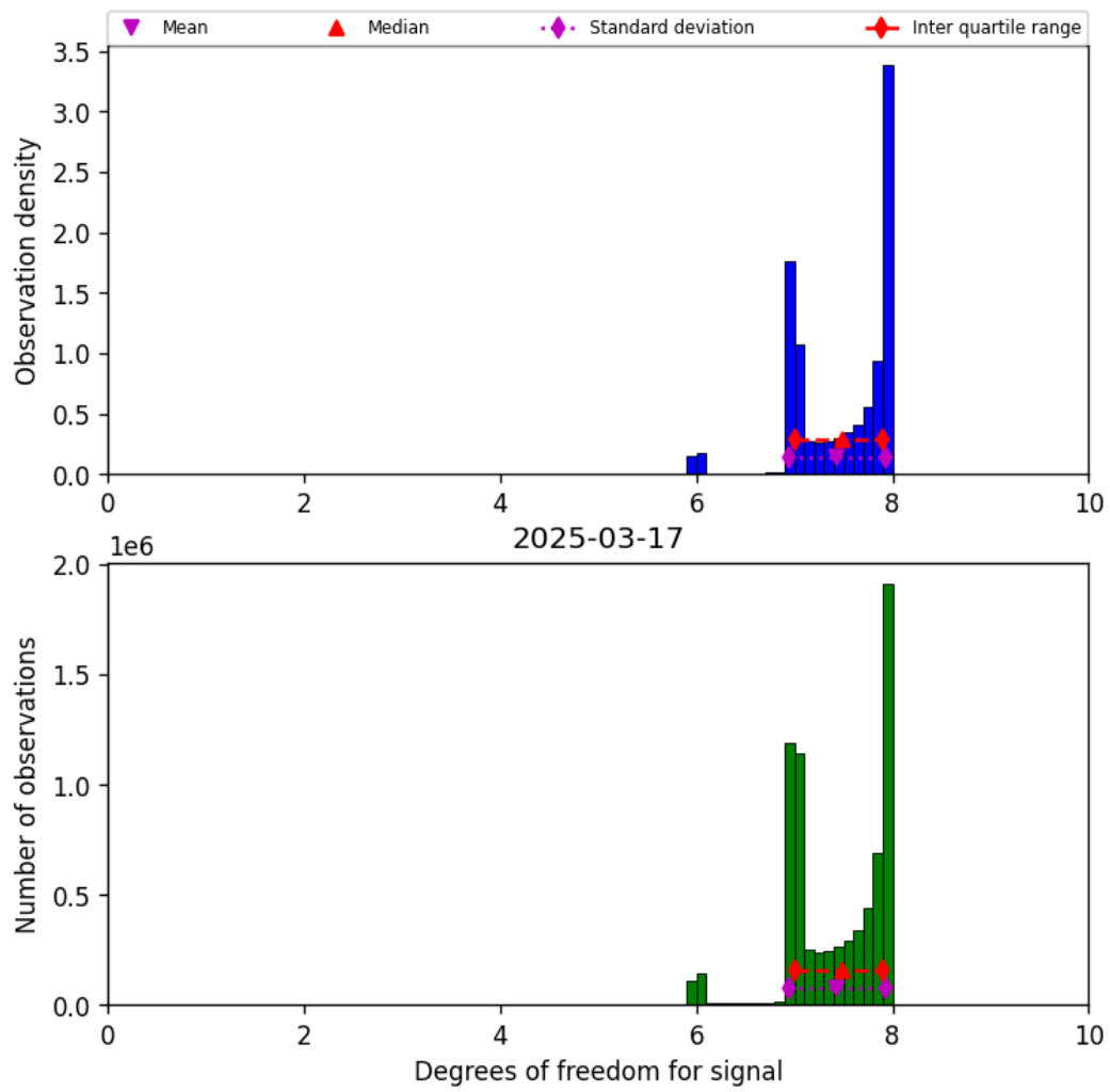
Figure 23: Histogram of “Degrees of freedom for signal” for 2025-03-17 to 2025-03-18
