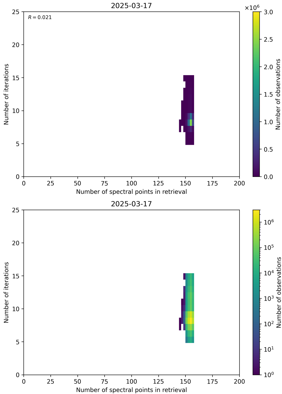
Figure 60: Scatter density plot of “Number of spectral points in retrieval” against “Number of iterations” for 2025-03-17 to 2025-03-18.
