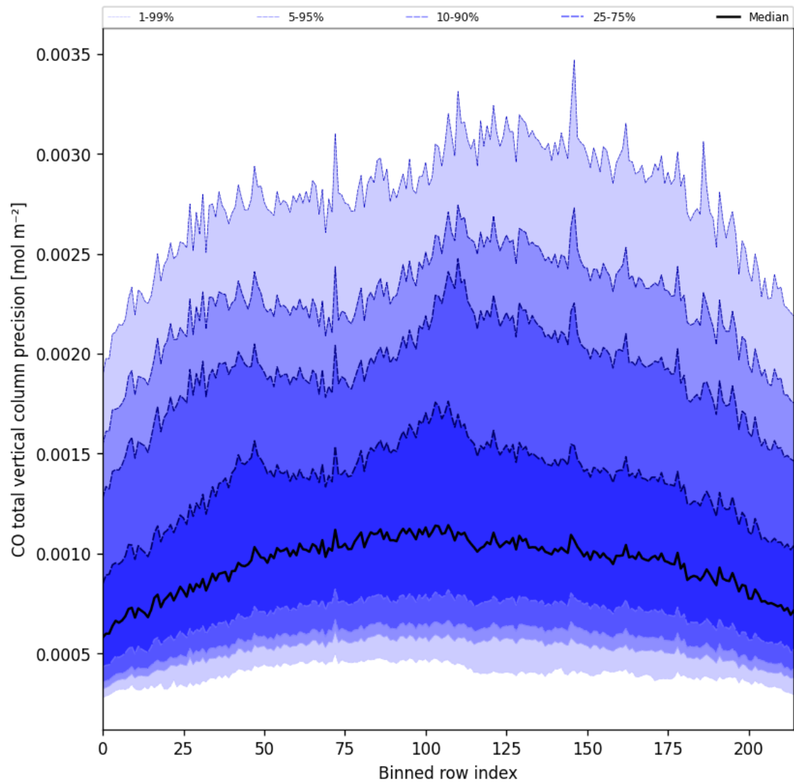
Figure 28: Along track statistics of “CO total vertical column precision” for 2025-03-17 to 2025-03-18
