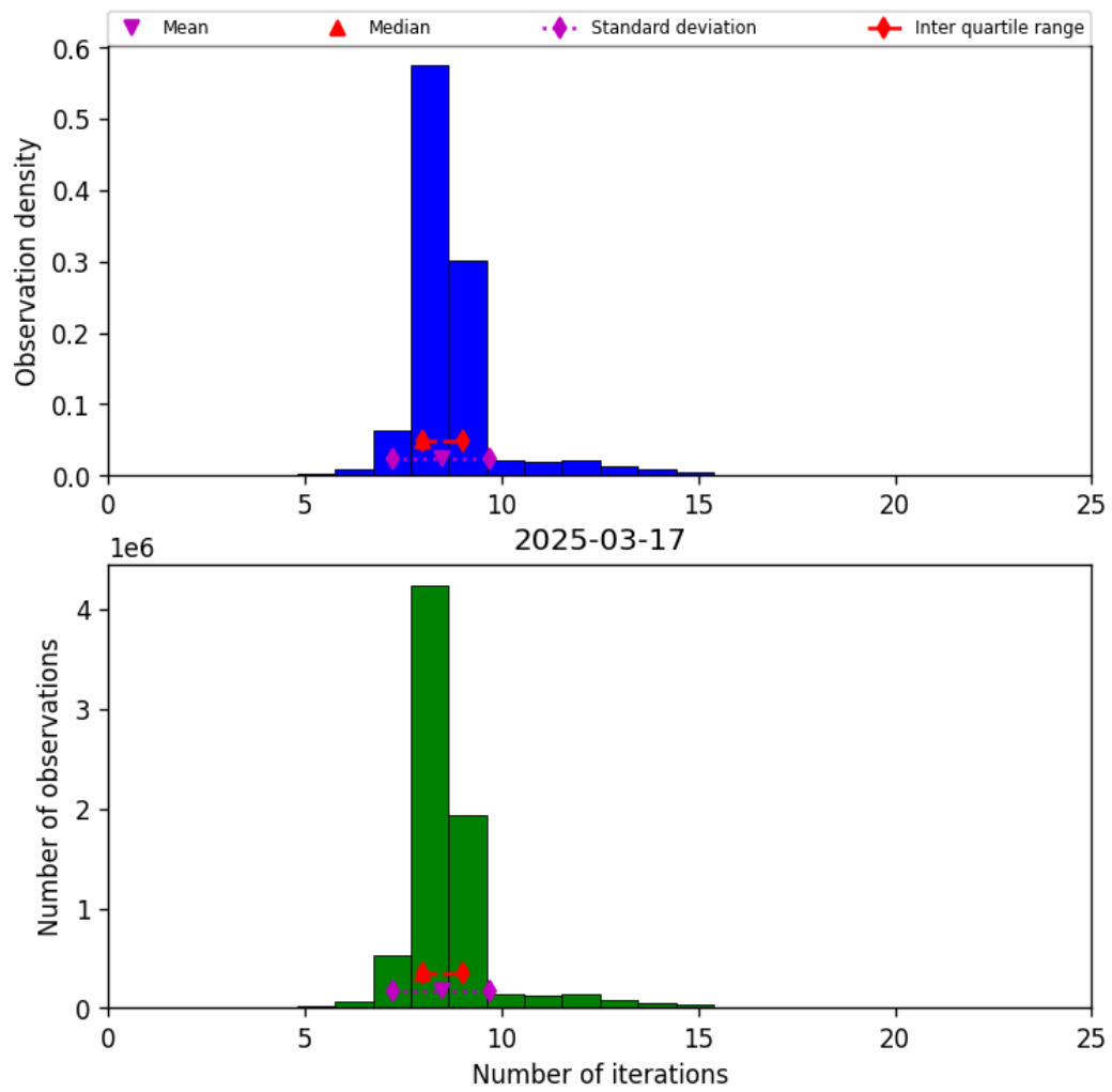
Figure 24: Histogram of “Number of iterations” for 2025-03-17 to 2025-03-18
