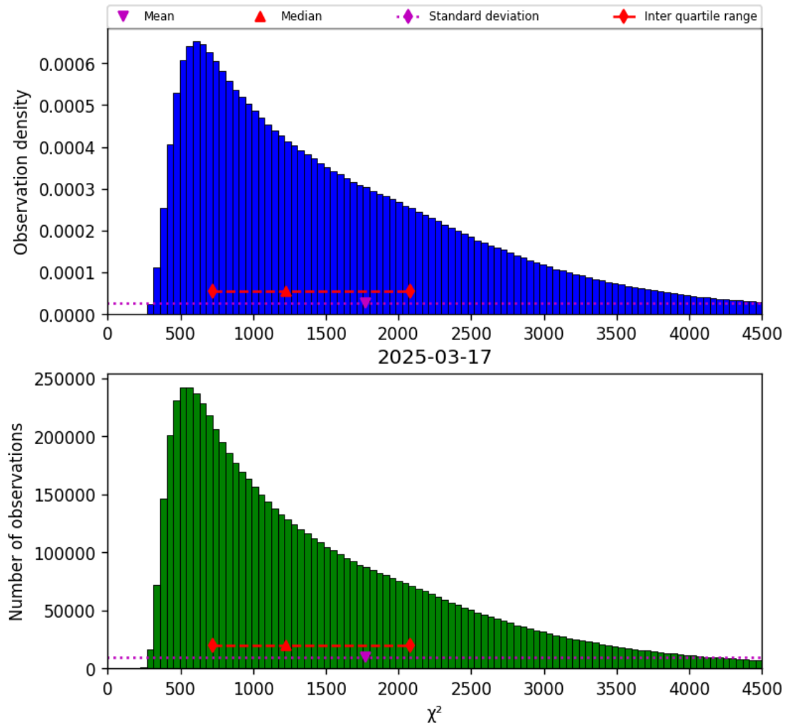
Figure 22: Histogram of “ \chi^2 ” for 2025-03-17 to 2025-03-18
