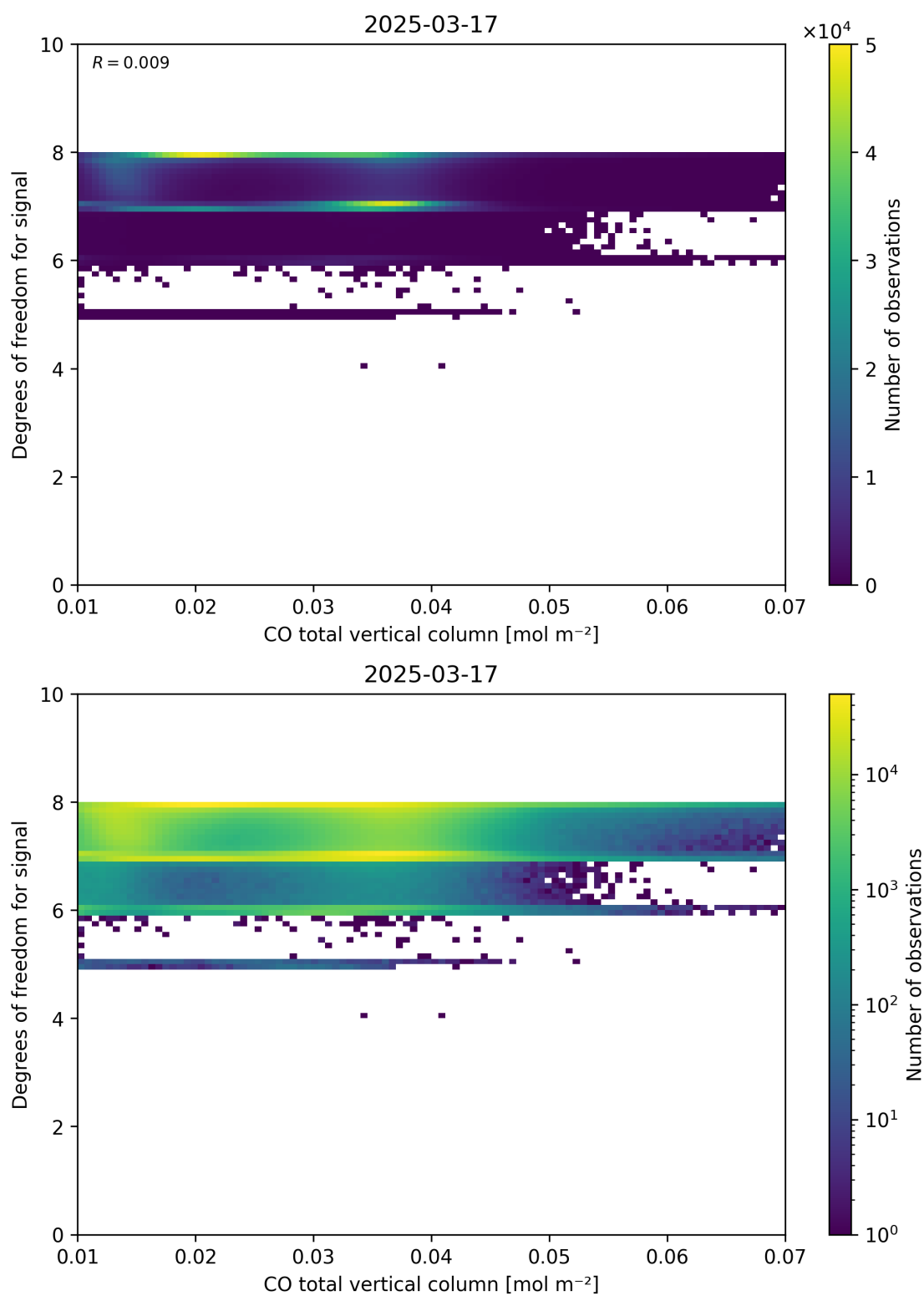
Figure 41: Scatter density plot of “CO total vertical column” against “Degrees of freedom for signal” for 2025-03-17 to 2025-03-18.
