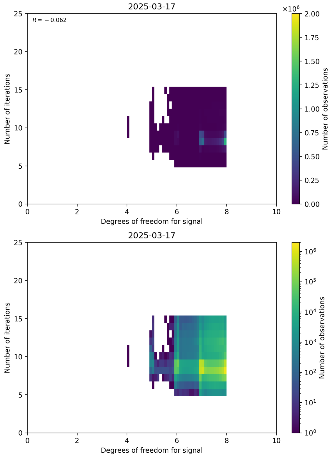
Figure 50: Scatter density plot of “Degrees of freedom for signal” against “Number of iterations” for 2025-03-17 to 2025-03-18.
