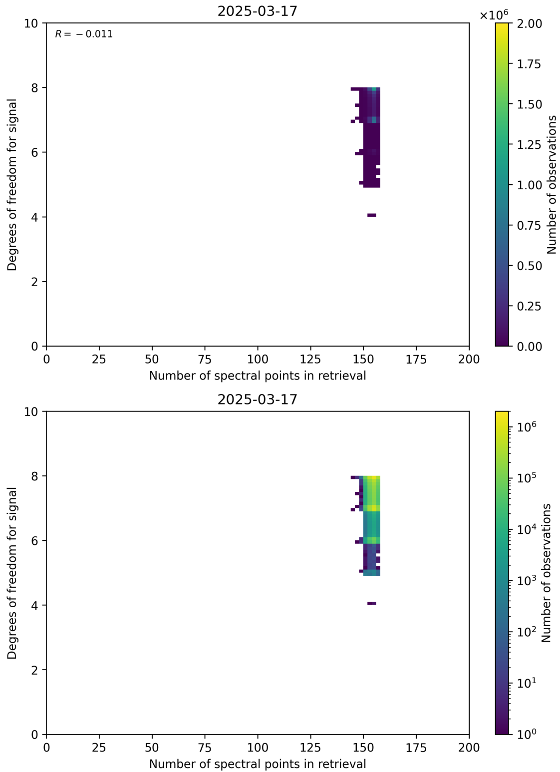
Figure 59: Scatter density plot of “Number of spectral points in retrieval” against “Degrees of freedom for signal” for 2025-03-17 to 2025-03-18.
