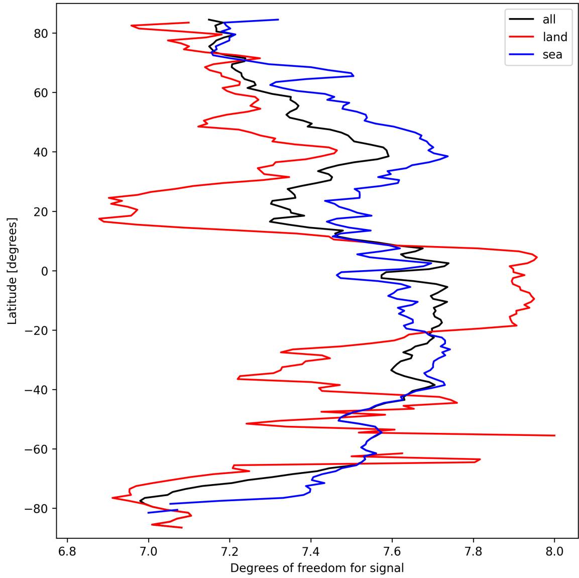
Figure 15: Zonal average of “Degrees of freedom for signal” for 2025-03-17 to 2025-03-18.
