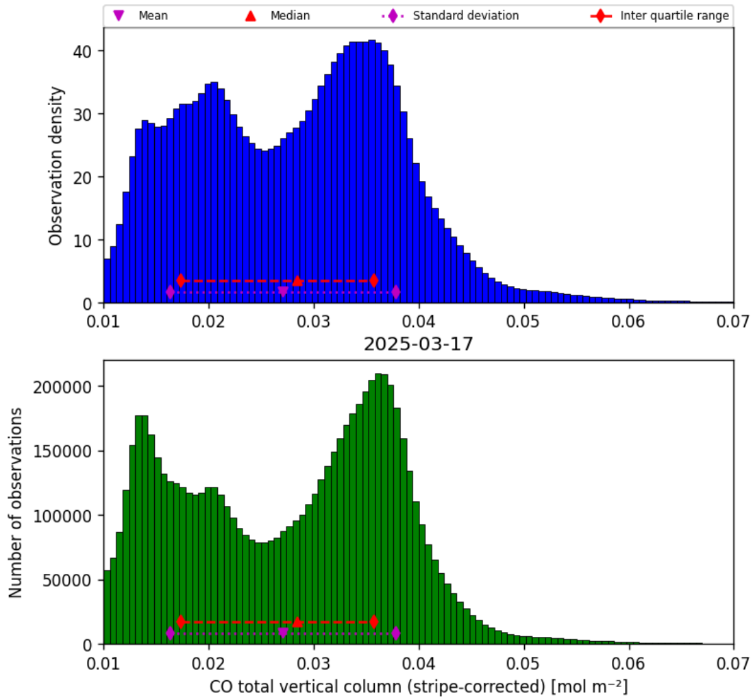
Figure 19: Histogram of “CO total vertical column (stripe-corrected)” for 2025-03-17 to 2025-03-18
