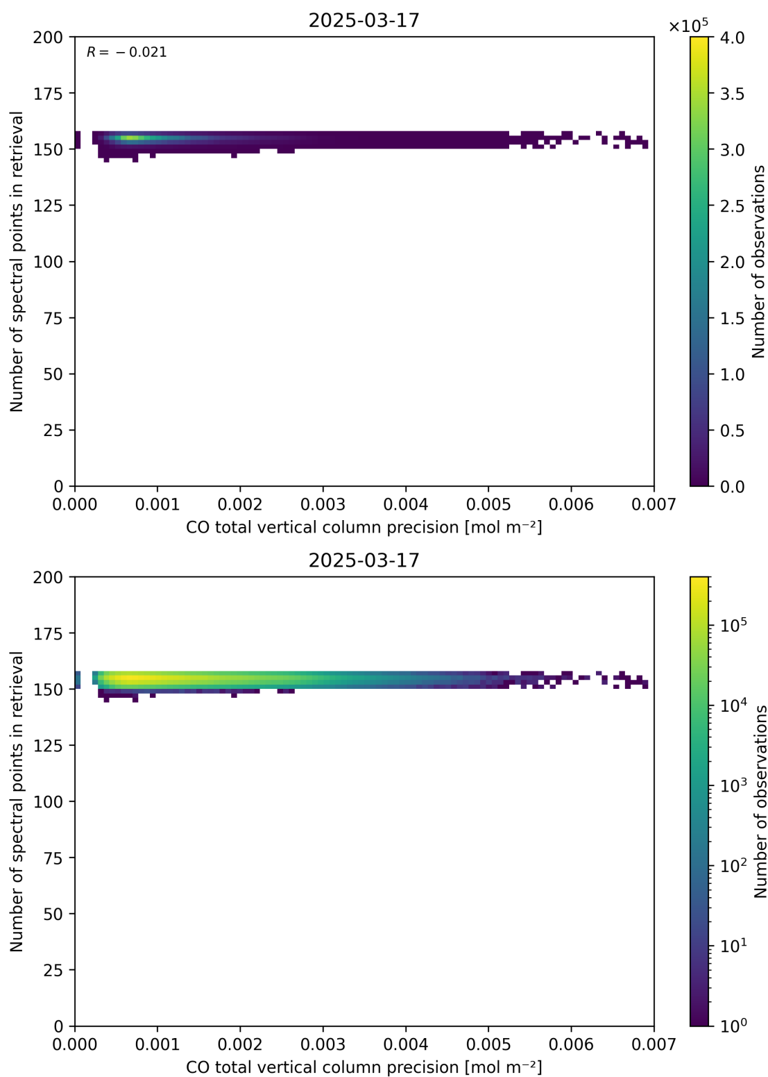
Figure 47: Scatter density plot of “CO total vertical column precision” against “Number of spectral points in retrieval” for 2025-03-17 to 2025-03-18.
