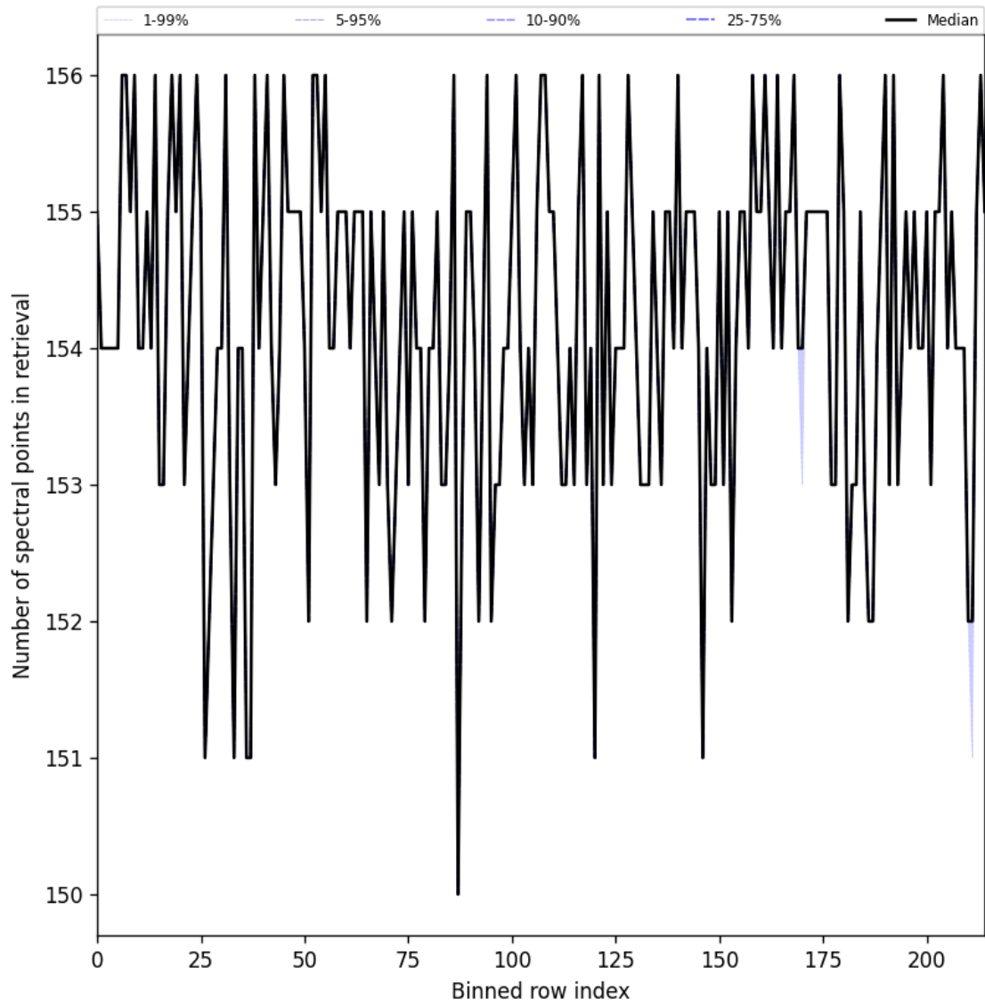
Figure 29: Along track statistics of “Number of spectral points in retrieval” for 2025-03-17 to 2025-03-18
